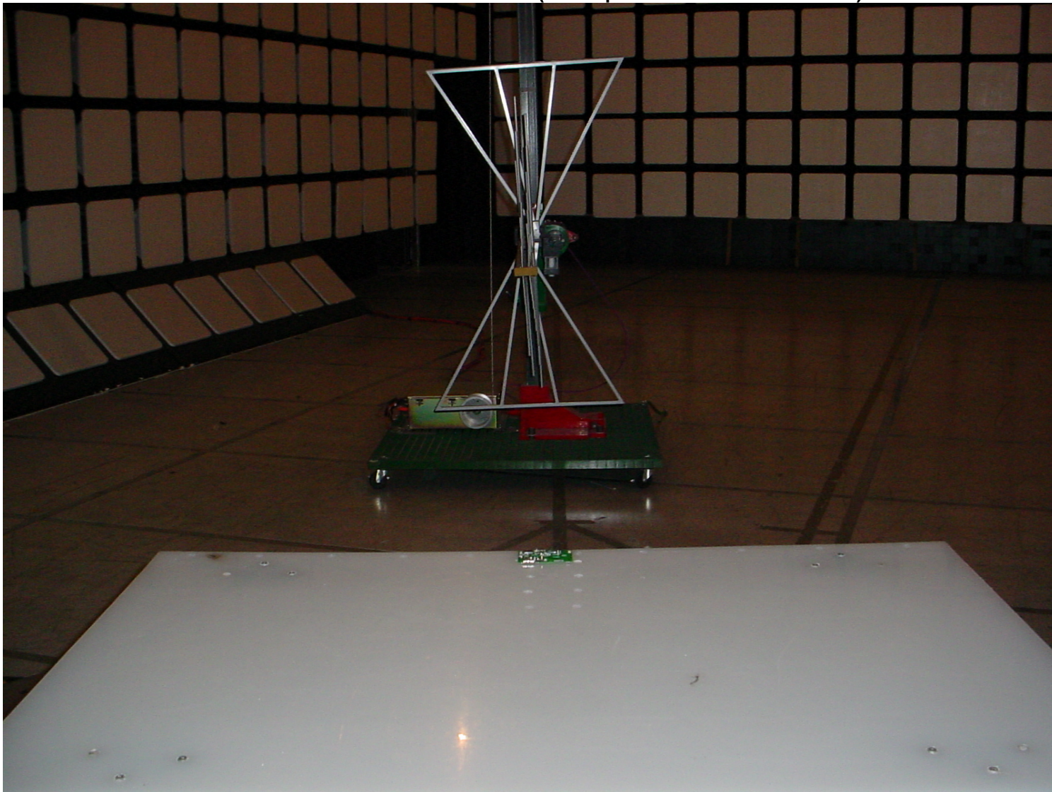
Radiated Emissions at 10 m Distance (for frequencies at or above 30 MHz)
