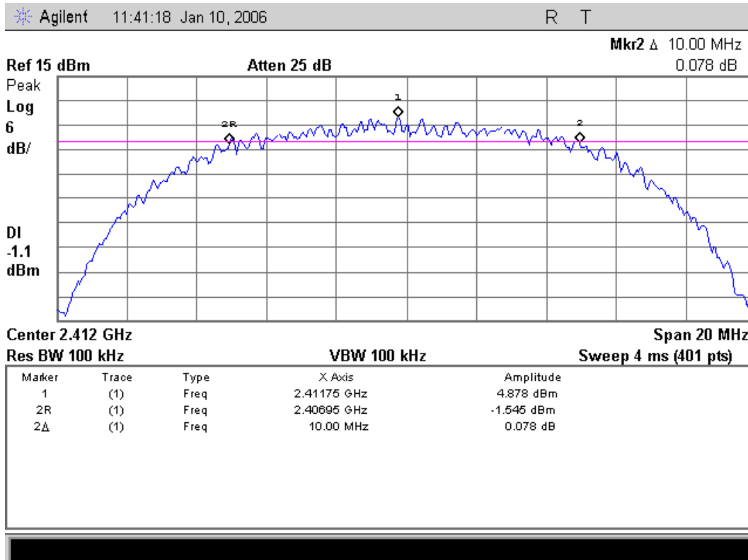
Figure 1. Plot of the 6dB Bandwidth (Conducted)
