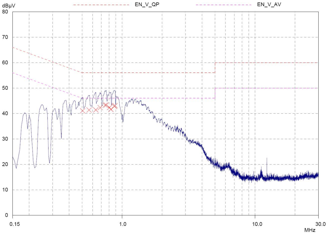
Figure 6. Plot of the Conducted Emissions Transmitting at 2437 MHz: LINE - PE
