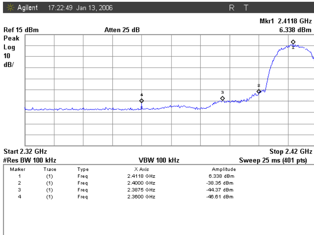
Figure 4. Plot of the Band Edge (Conducted) Lowest Channel (operating at 2412 MHz)
