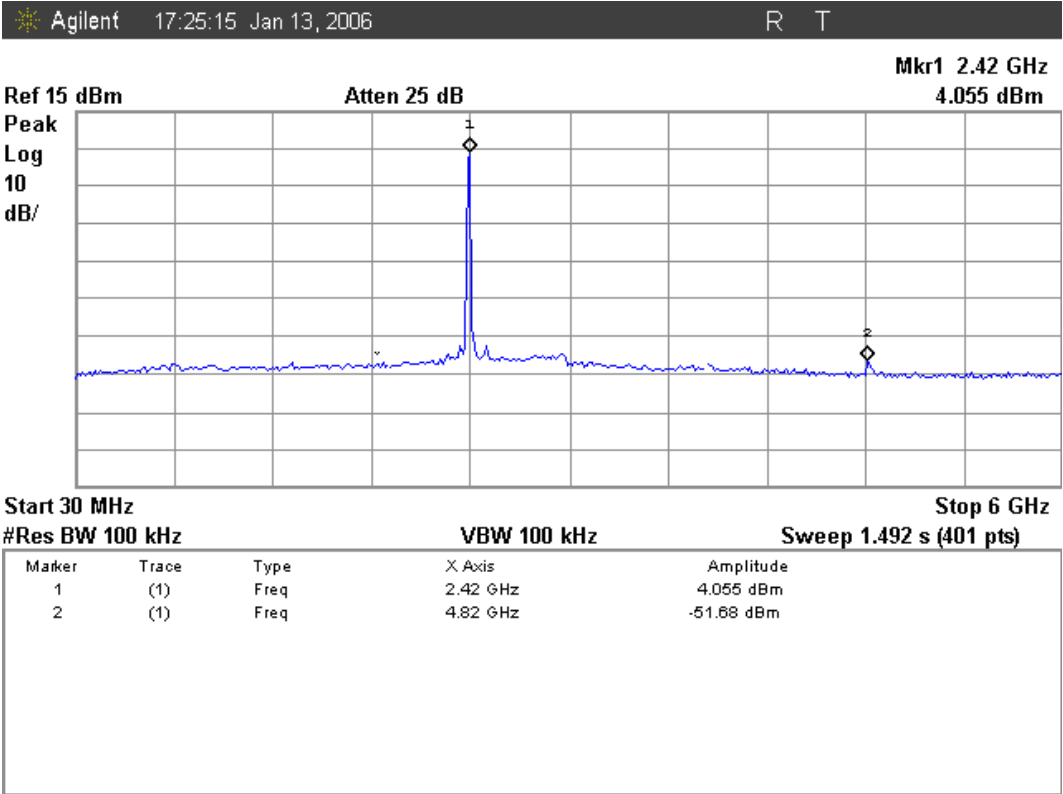
Figure 2. Plot of the RF antenna port emissions (Conducted) Lowest Channel (operating at 2412 MHz): 30 MHz ~ 6 GHz
