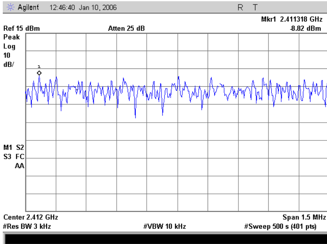
Figure 5. Plot of the Peak Power Spectral Density (Conducted) Lowest Channel (operating at 2412 MHz)
