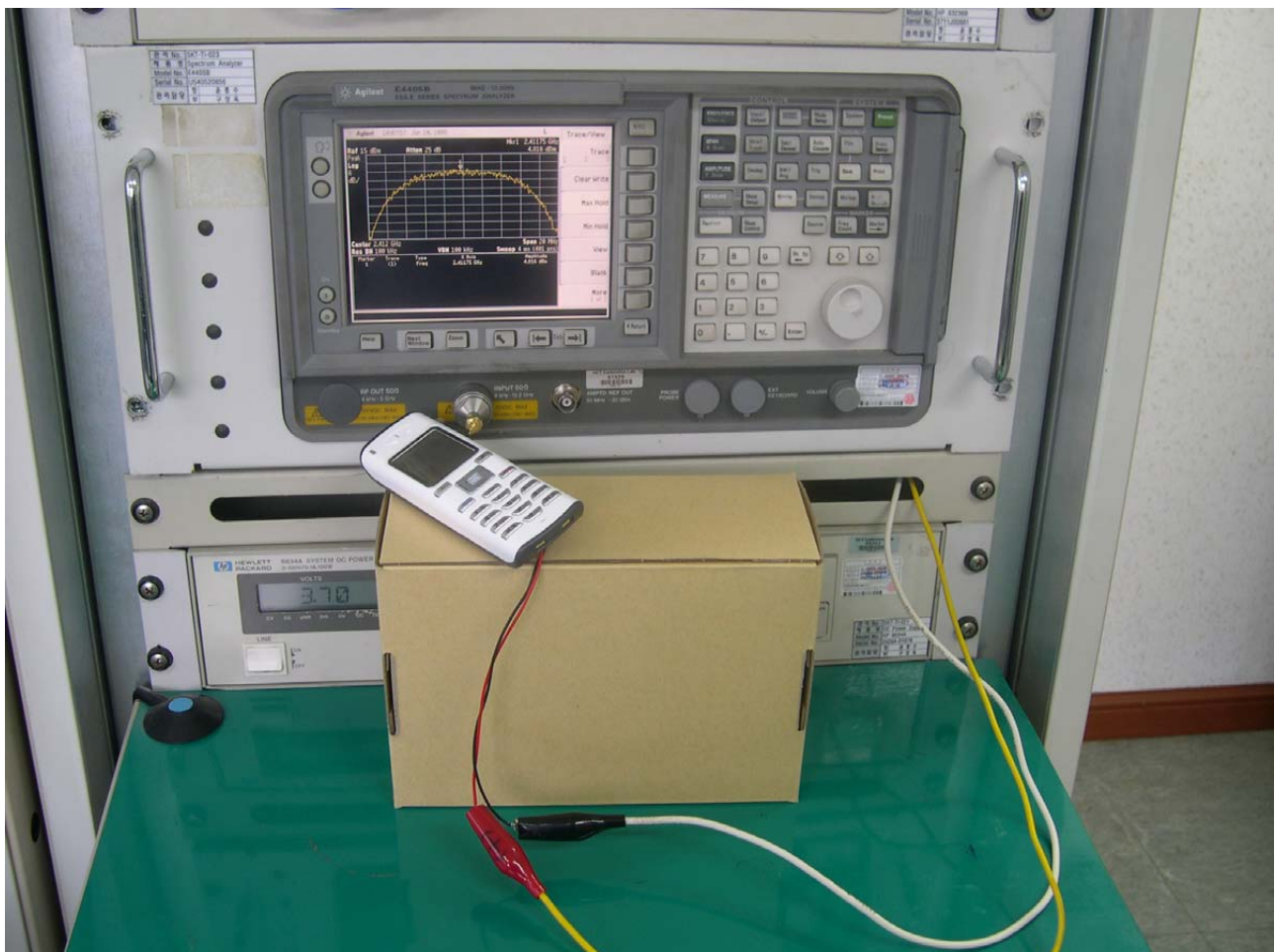
The antenna port of the EUT was directly connected to the spectrum analyzer using SMA gender
