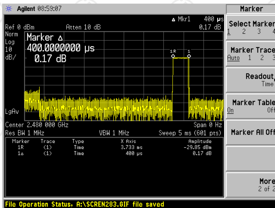
Channel 79_ 2480 MHz_DH1
