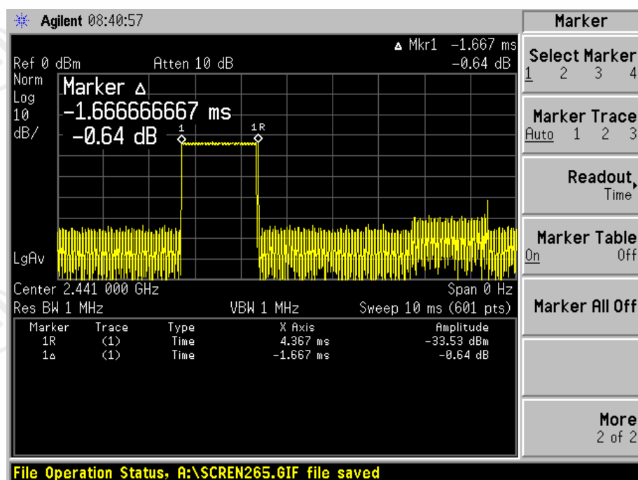
Channel 40_ 2441 MHz_DH3
