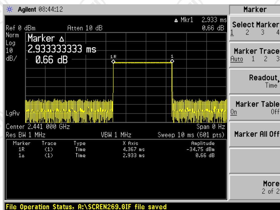
Channel 40_ 2441 MHz_DH5
