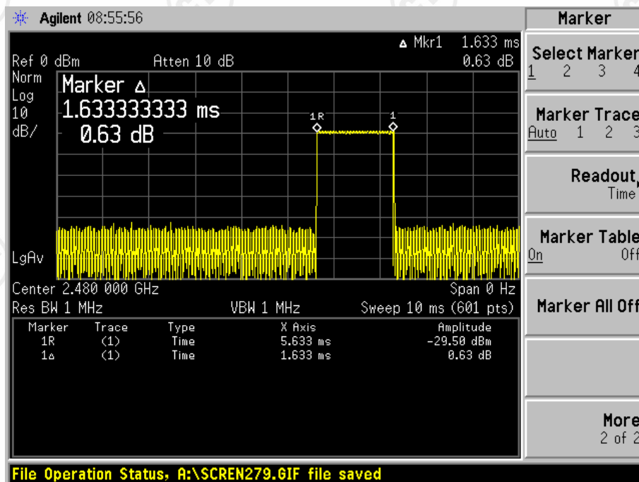
Channel 79_ 2480 MHz_DH3
