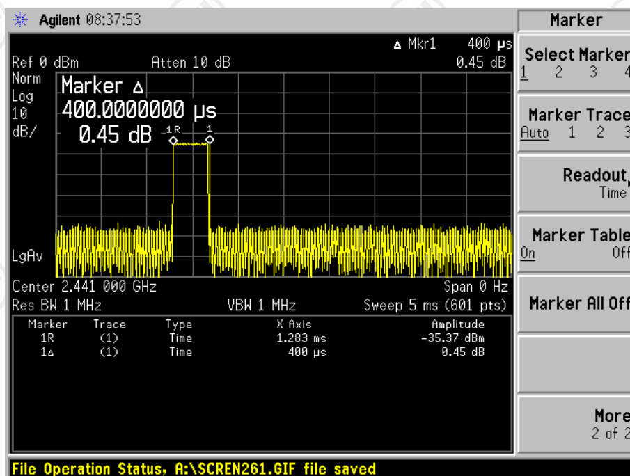
Channel 40_ 2441 MHz_DH1
