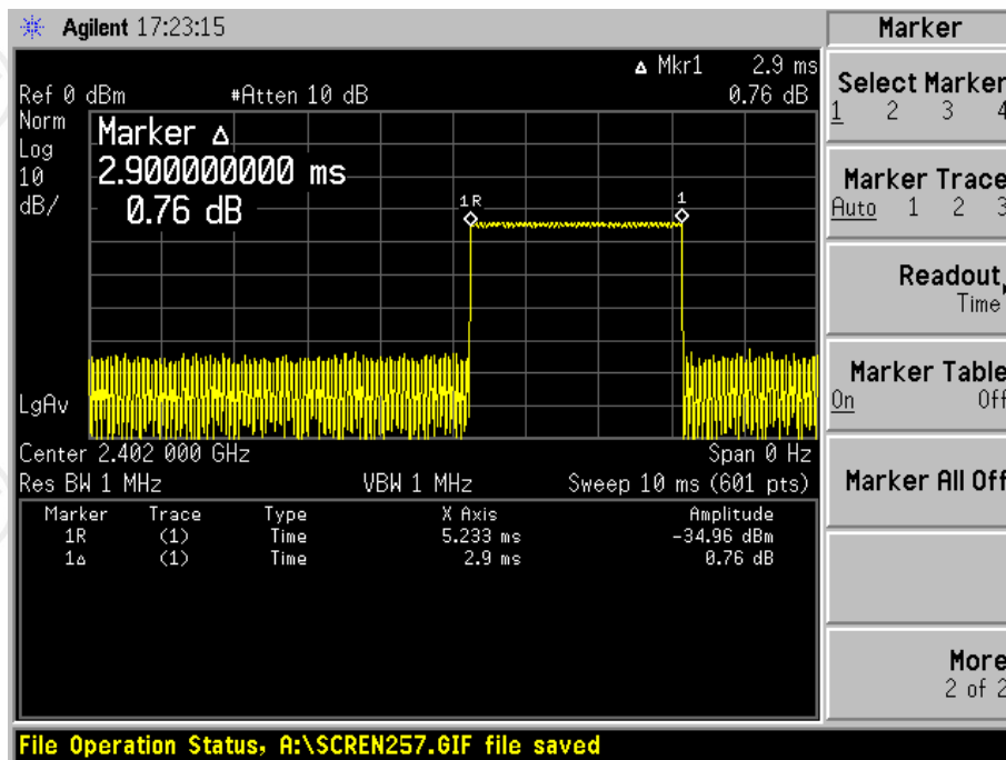
Channel 1_ 2402 MHz_DH5
