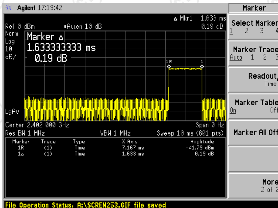
Channel 1_ 2402 MHz_DH3
