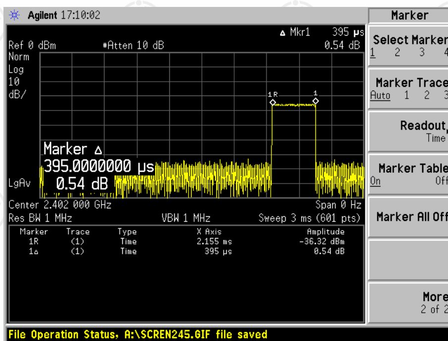
Channel 1_ 2402 MHz_DH1
