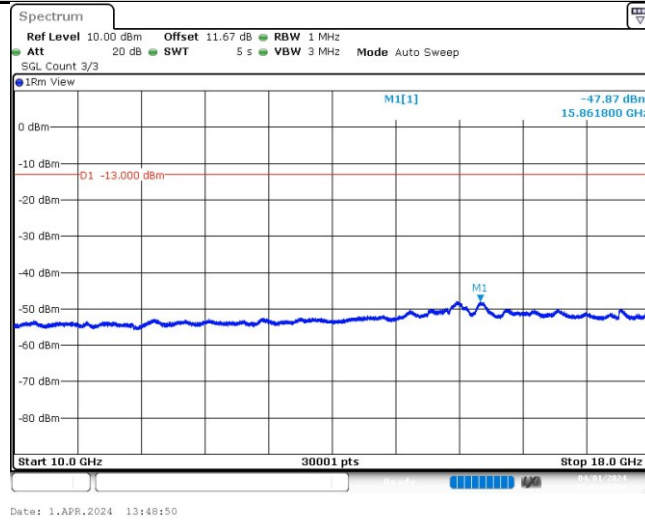
Band5-4233-1-10000~18000MHz
