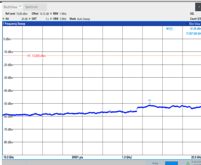
Band4-1312-3-10000~20000MHz
