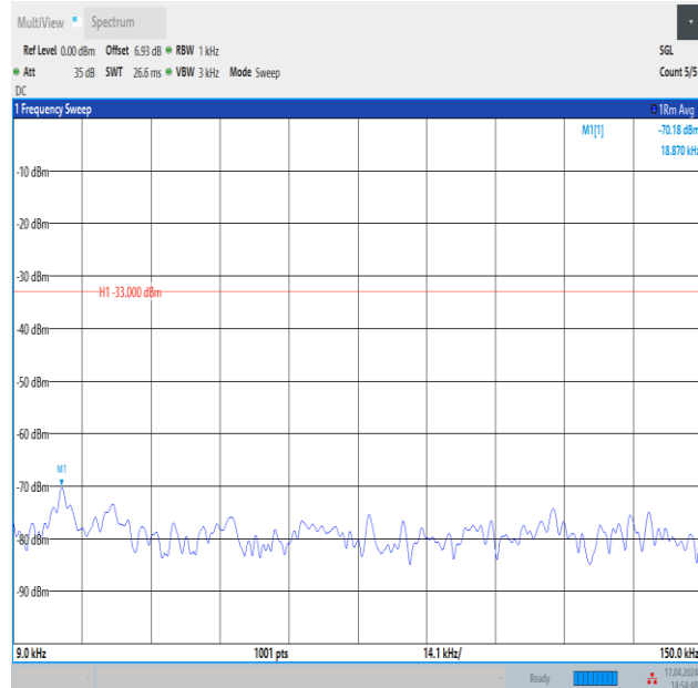
Band12_3MHz_QPSK_23025_1RB#0_0.009~0.15_0.009~0.15
