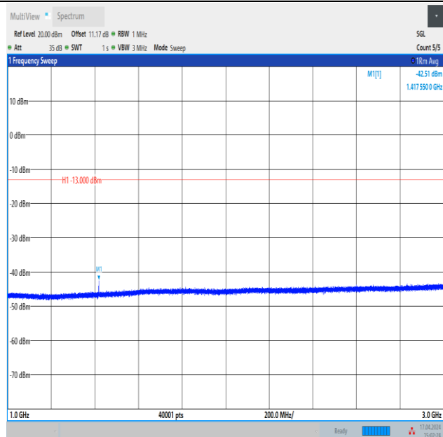
Band12_3MHz_QPSK_23095_1RB#14_1000~3000_1000~3000
