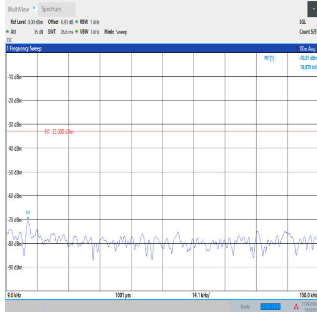
Band12_5MHz_16QAM_23155_1RB#24_0.009~0.15_0.009~0.15
