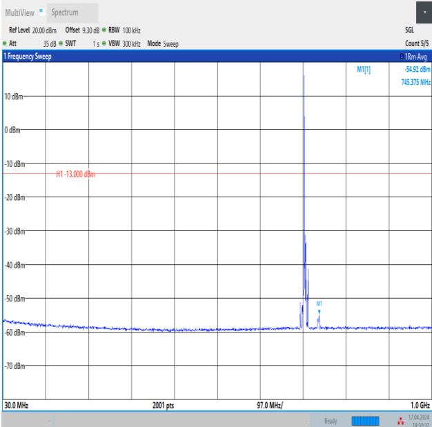
Band12_5MHz_16QAM_23155_1RB#0_30~1000_30~1000
