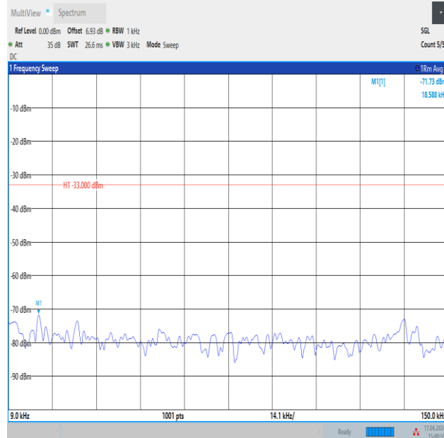
Band12_3MHz_16QAM_23095_1RB#0_0.009~0.15_0.009~0.15
