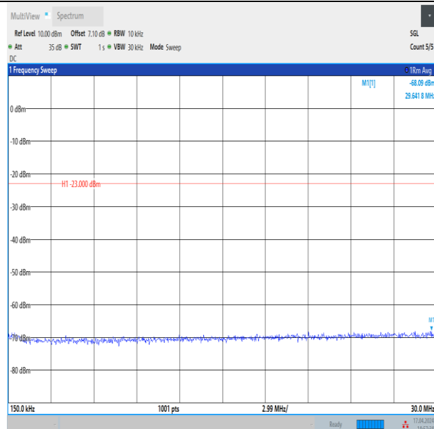
Band12_3MHz_16QAM_23025_1RB#14_0.15~30_0.15~30
