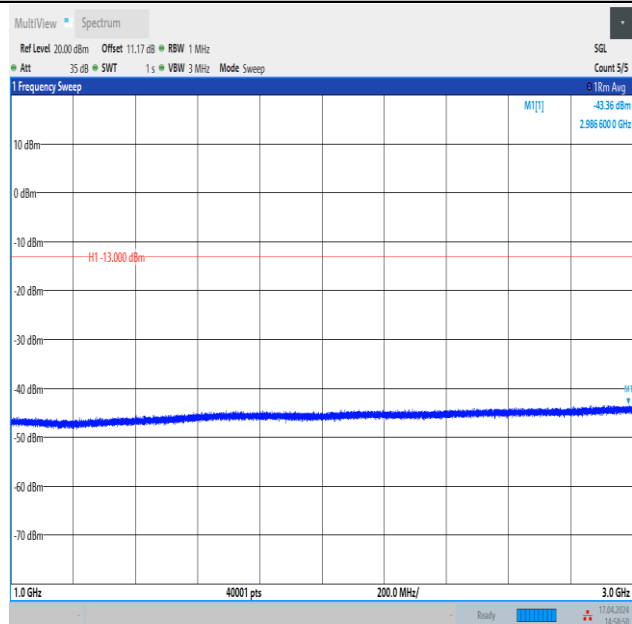
Band12_3MHz_QPSK_23025_15RB#0_1000~3000_1000~3000
