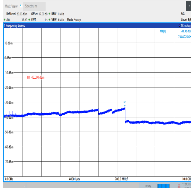
Band12_5MHz_QPSK_23095_1RB#24_3000~10000_3000~10000
