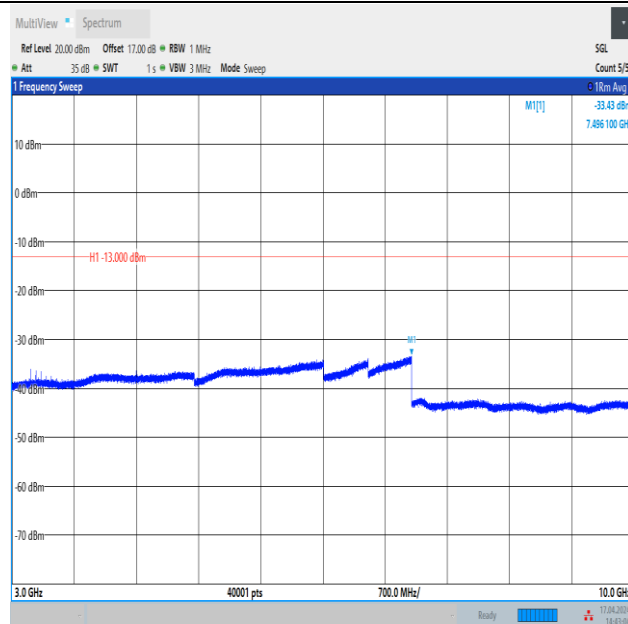
Band12_5MHz_QPSK_23035_25RB#0_3000~10000_3000~10000
