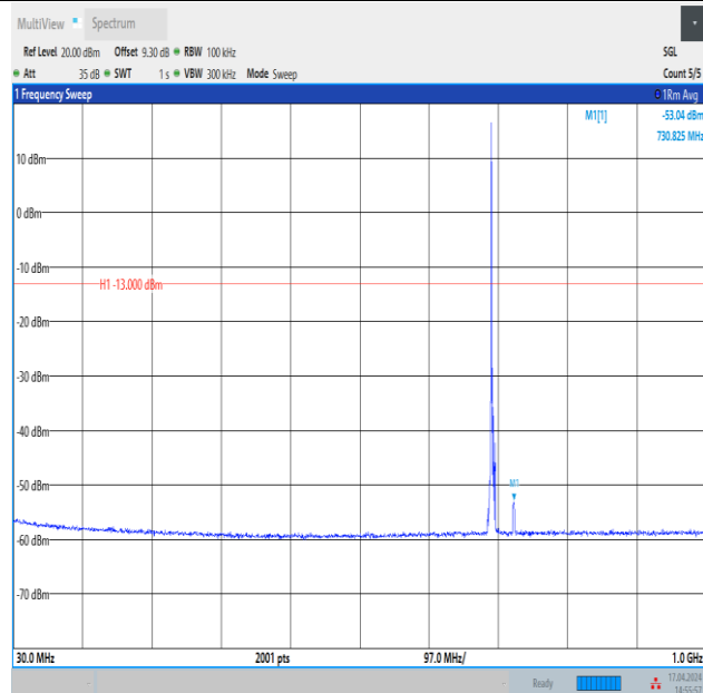
Band12_3MHz_16QAM_23025_1RB#0_30~1000_30~1000
