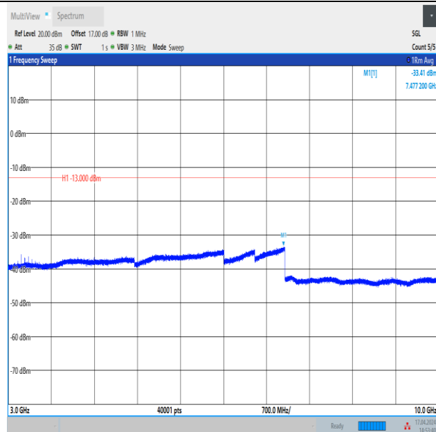
Band12_5MHz_QPSK_23155_25RB#0_3000~10000_3000~10000
