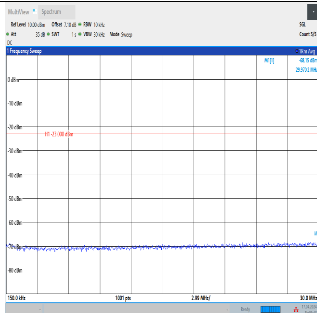
Band12_3MHz_16QAM_23095_15RB#0_0.15~30_0.15~30
