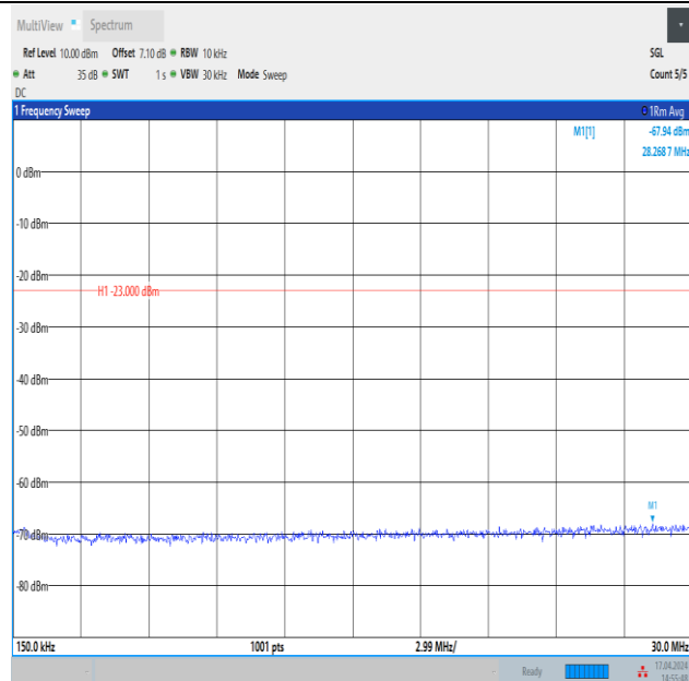
Band12_3MHz_16QAM_23025_1RB#0_0.15~30_0.15~30
