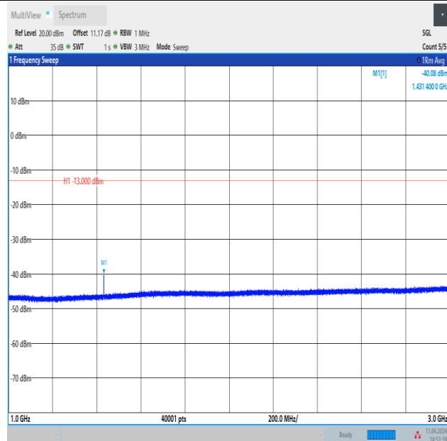
Band12_5MHz_QPSK_23155_1RB#24_1000~3000_1000~3000
