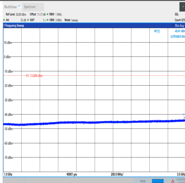
Band12_3MHz_16QAM_23025_15RB#0_1000~3000_1000~3000
