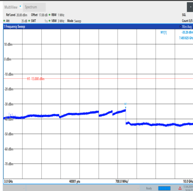
Band12_3MHz_16QAM_23025_1RB#0_3000~10000_3000~10000
