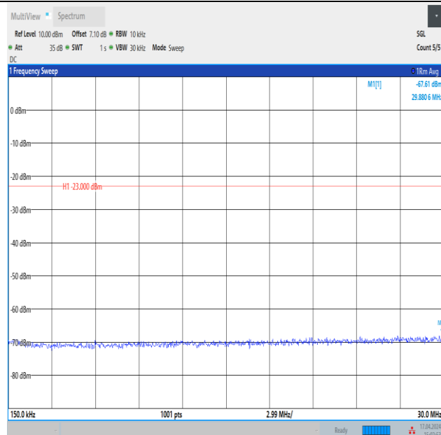
Band12_3MHz_16QAM_23095_1RB#14_0.15~30_0.15~30
