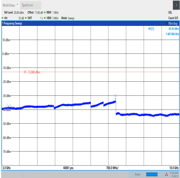
Band12_3MHz_16QAM_23025_1RB#14_3000~10000_3000~10000
