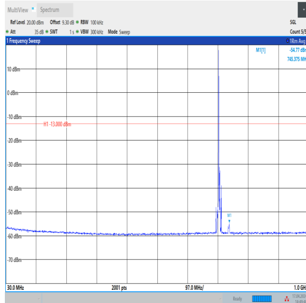
Band12_5MHz_QPSK_23155_1RB#0_30~1000_30~1000
