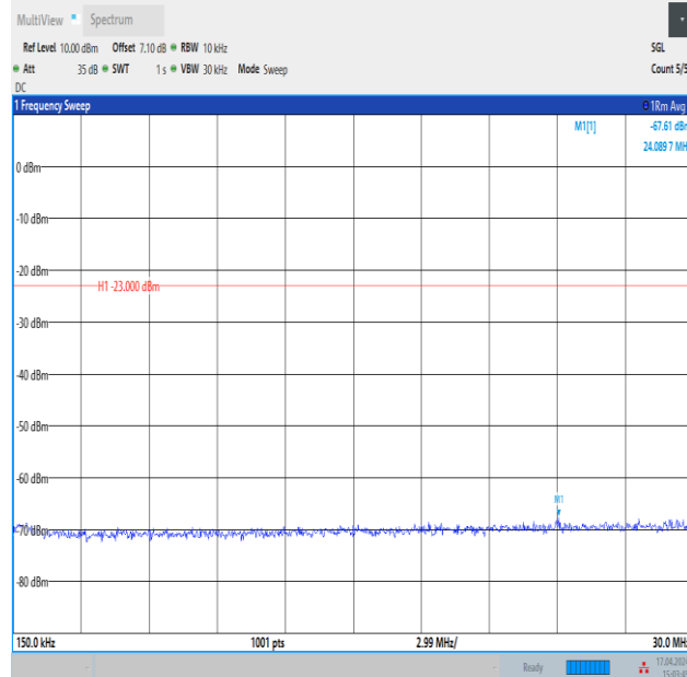
Band12_3MHz_QPSK_23095_15RB#0_0.15~30_0.15~30
