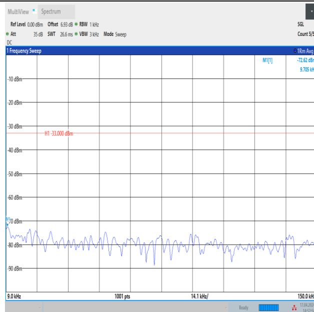
Band12_5MHz_QPSK_23155_25RB#0_0.009~0.15_0.009~0.15
