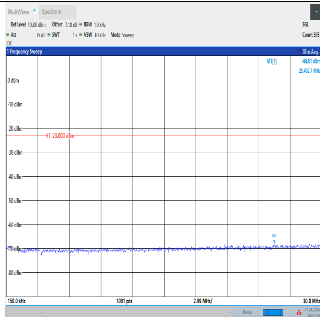
Band12_5MHz_16QAM_23155_1RB#24_0.15~30_0.15~30
