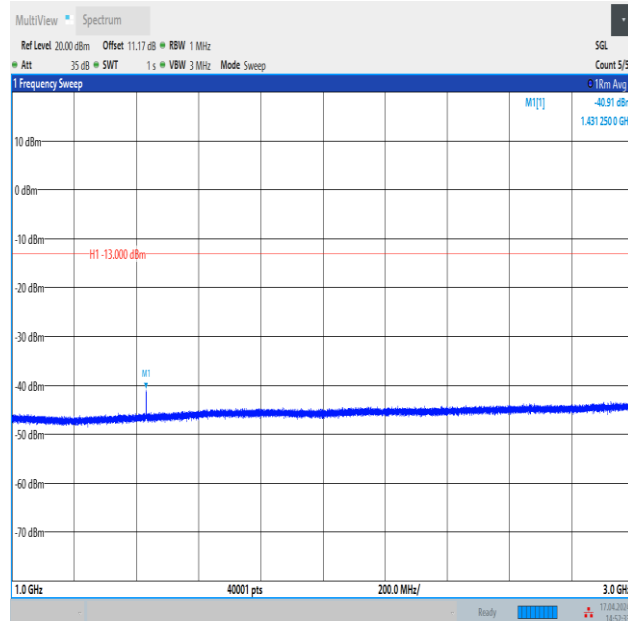
Band12_5MHz_16QAM_23155_1RB#24_1000~3000_1000~3000
