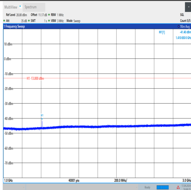
Band12_5MHz_QPSK_23095_1RB#0_1000~3000_1000~3000
