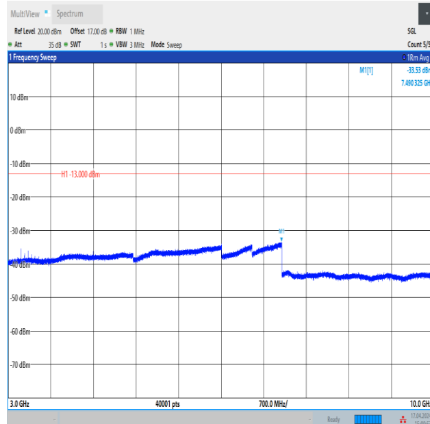
Band12_3MHz_QPSK_23095_1RB#0_3000~10000_3000~10000
