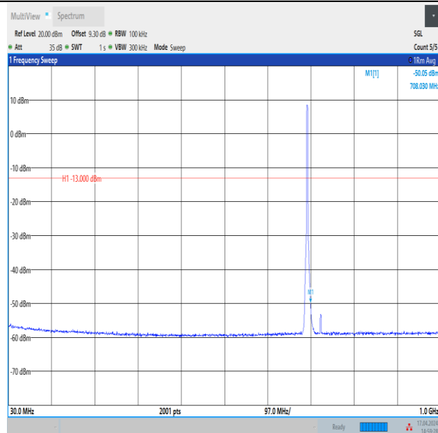
Band12_3MHz_16QAM_23025_15RB#0_30~1000_30~1000
