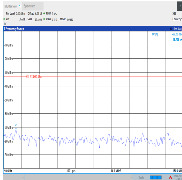
Band12_5MHz_16QAM_23095_1RB#24_0.009~0.15_0.009~0.15
