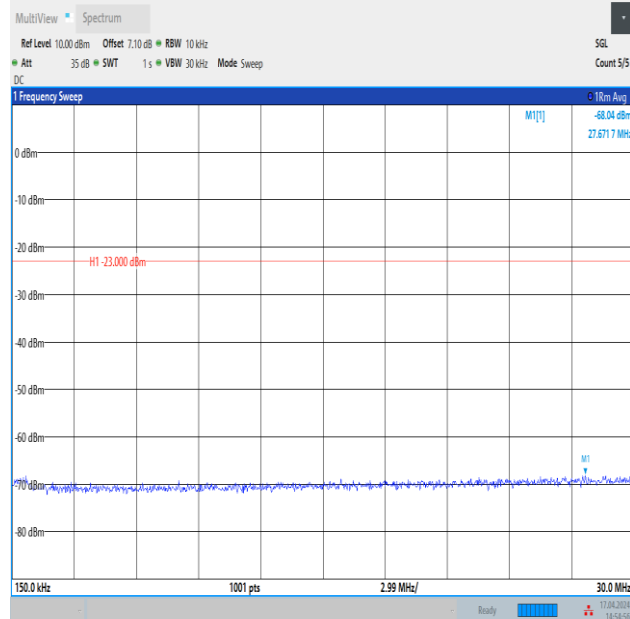
Band12_3MHz_QPSK_23025_1RB#0_0.15~30_0.15~30
