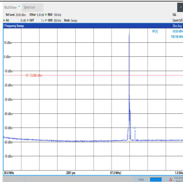
Band12_5MHz_QPSK_23095_1RB#0_30~1000_30~1000
