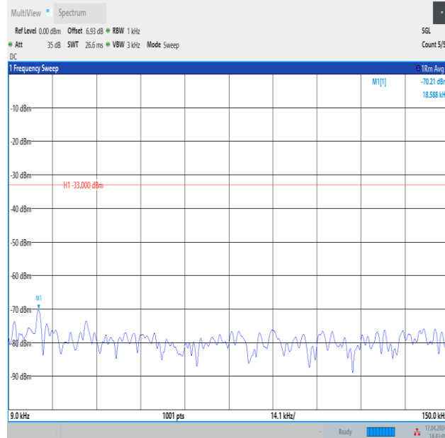
Band12_5MHz_16QAM_23035_25RB#0_0.009~0.15_0.009~0.15
