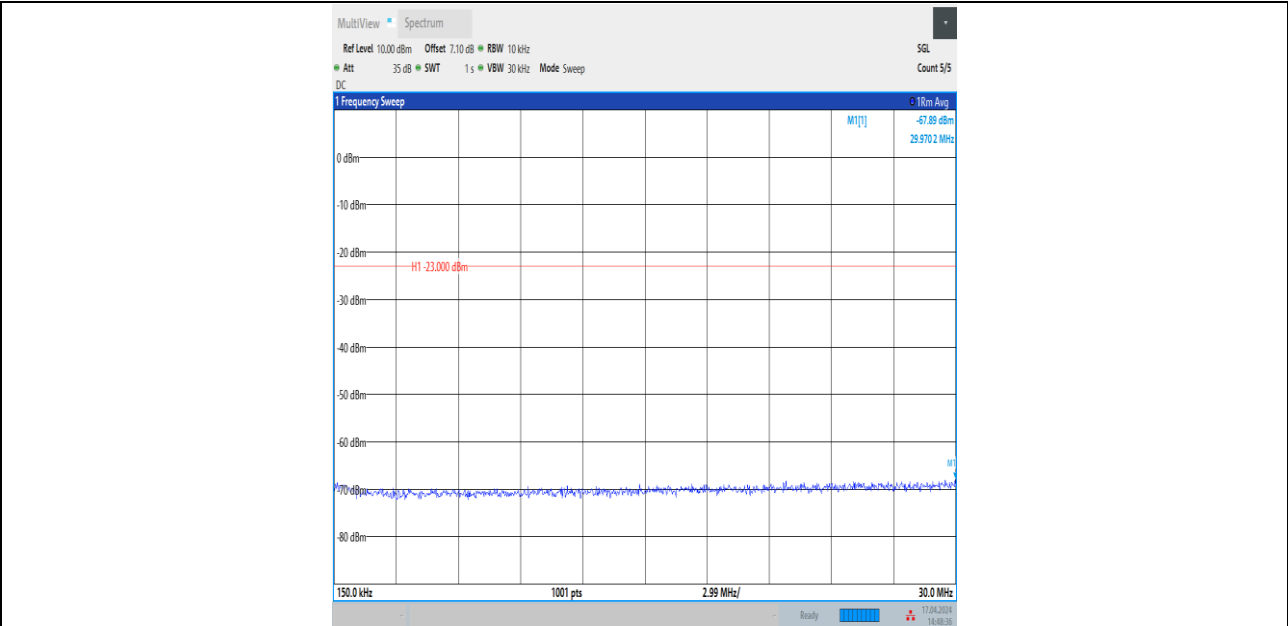
Band12_5MHz_16QAM_23095_25RB#0_0.15~30_0.15~30
