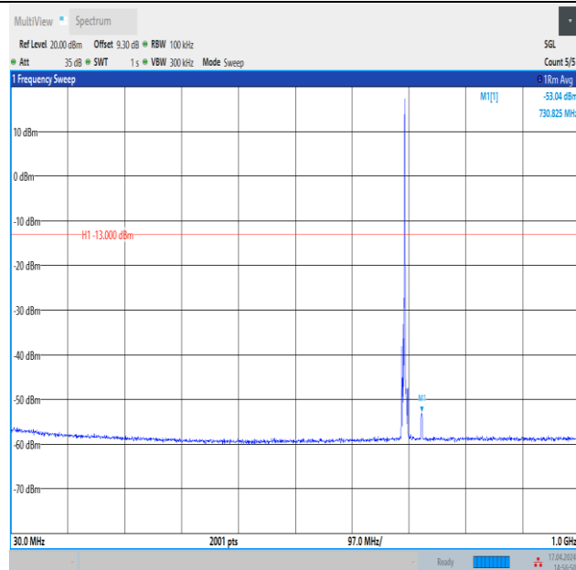
Band12_3MHz_QPSK_23025_1RB#14_30~1000_30~1000
