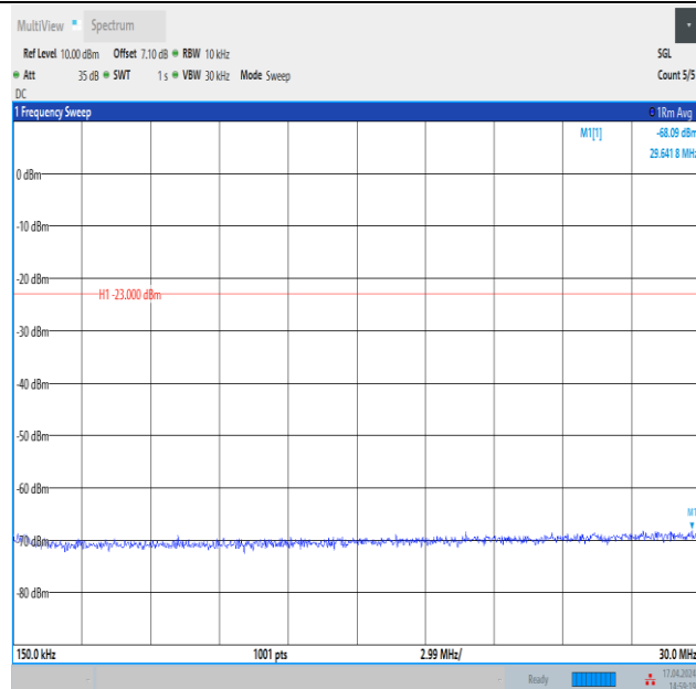
Band12_3MHz_16QAM_23025_15RB#0_0.15~30_0.15~30
