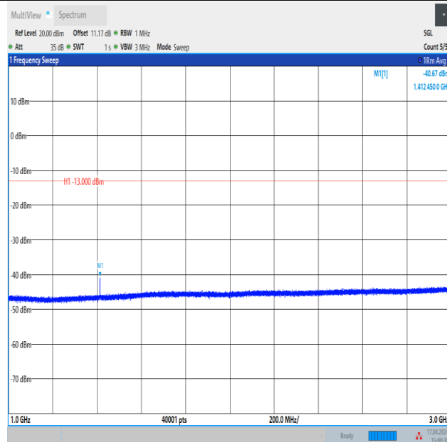
Band12_3MHz_QPSK_23095_1RB#0_1000~3000_1000~3000
