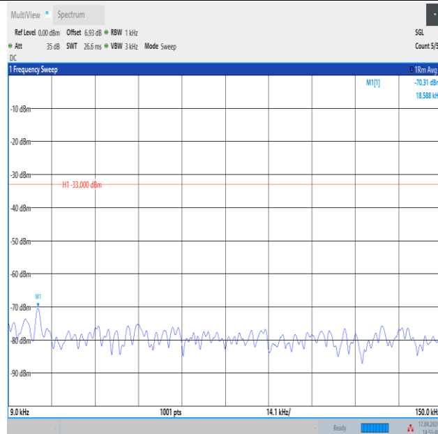
Band12_3MHz_16QAM_23025_1RB#0_0.009~0.15_0.009~0.15
