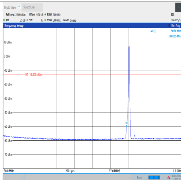
Band12_5MHz_QPSK_23155_25RB#0_30~1000_30~1000
