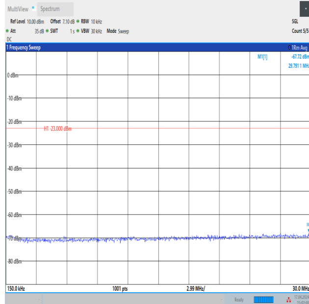
Band12_3MHz_QPSK_23095_1RB#14_0.15~30_0.15~30
