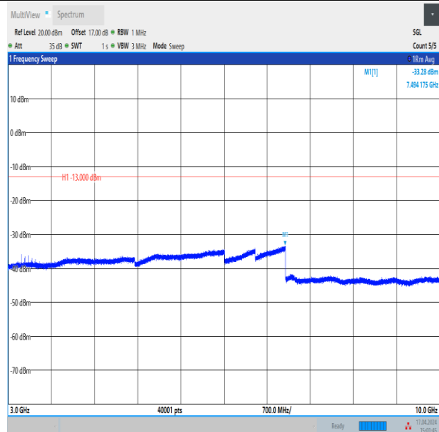
Band12_3MHz_16QAM_23095_1RB#0_3000~10000_3000~10000
