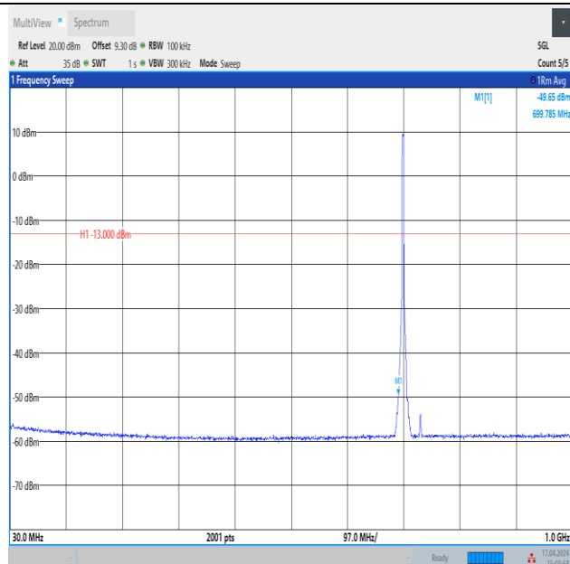
Band12_3MHz_QPSK_23095_15RB#0_30~1000_30~1000
