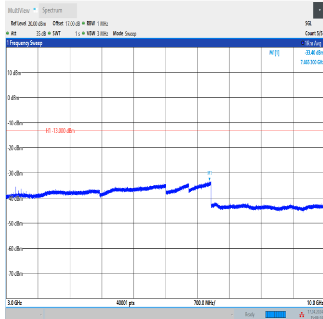
Band12_3MHz_QPSK_23095_15RB#0_3000~10000_3000~10000
