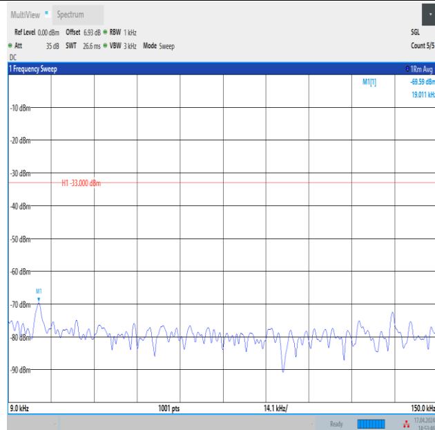
Band12_5MHz_16QAM_23155_25RB#0_0.009~0.15_0.009~0.15
