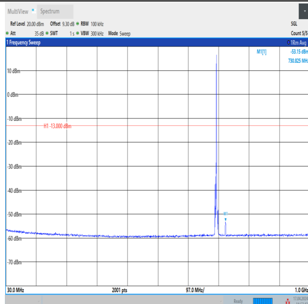
Band12_3MHz_16QAM_23025_1RB#14_30~1000_30~1000
