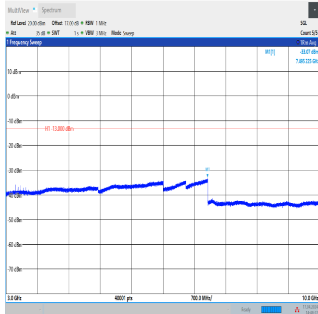
Band12_5MHz_QPSK_23095_25RB#0_3000~10000_3000~10000
