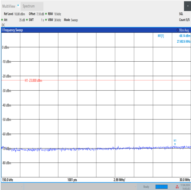
Band12_5MHz_16QAM_23095_1RB#0_0.15~30_0.15~30
