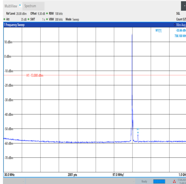
Band12_3MHz_QPSK_23095_1RB#0_30~1000_30~1000
