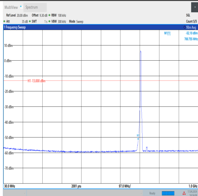
Band12_5MHz_16QAM_23155_25RB#0_30~1000_30~1000
