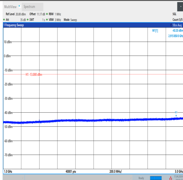
Band12_3MHz_16QAM_23025_1RB#0_1000~3000_1000~3000
