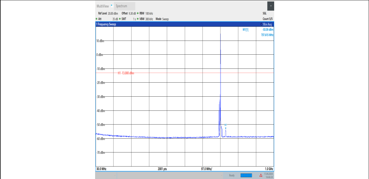
Band12_5MHz_16QAM_23095_1RB#24_30~1000_30~1000
