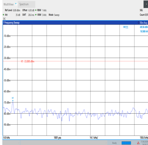
Band12_3MHz_16QAM_23025_15RB#0_0.009~0.15_0.009~0.15
