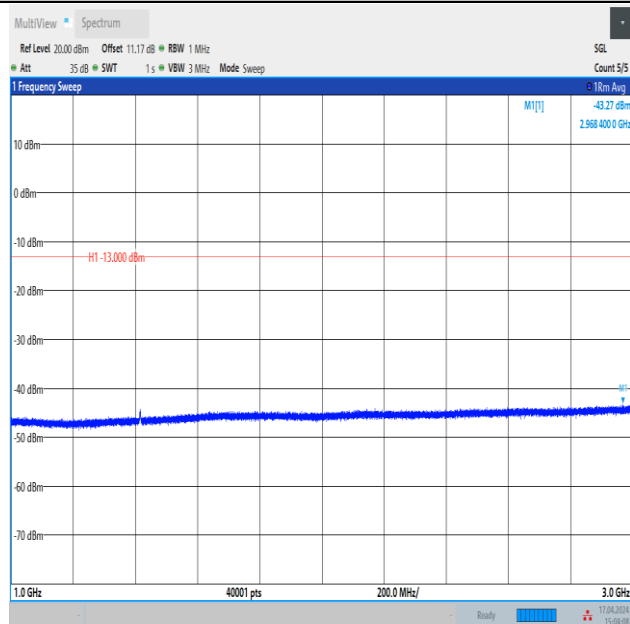
Band12_3MHz_QPSK_23095_15RB#0_1000~3000_1000~3000
