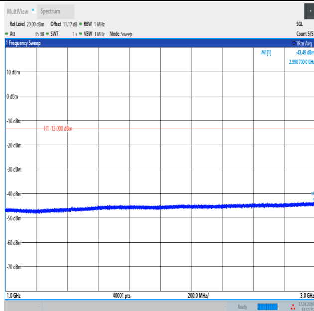
Band12_5MHz_QPSK_23155_25RB#0_1000~3000_1000~3000
