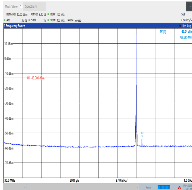
Band12_3MHz_16QAM_23095_1RB#14_30~1000_30~1000
