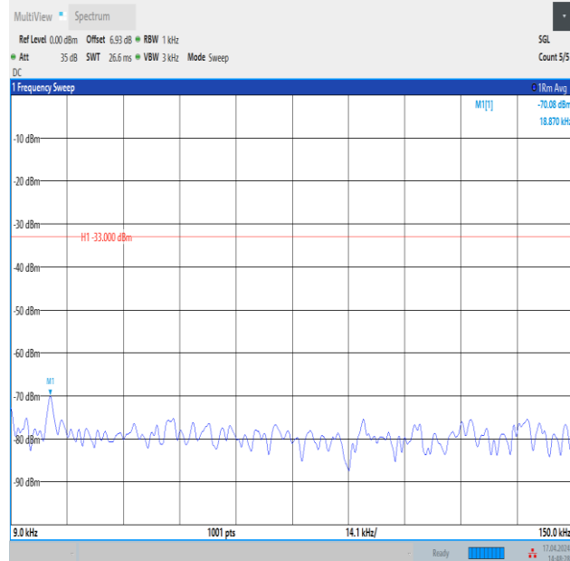
Band12_5MHz_16QAM_23095_25RB#0_0.009~0.15_0.009~0.15
