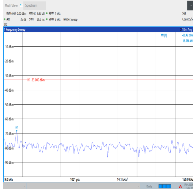
Band12_3MHz_16QAM_23095_15RB#0_0.009~0.15_0.009~0.15
