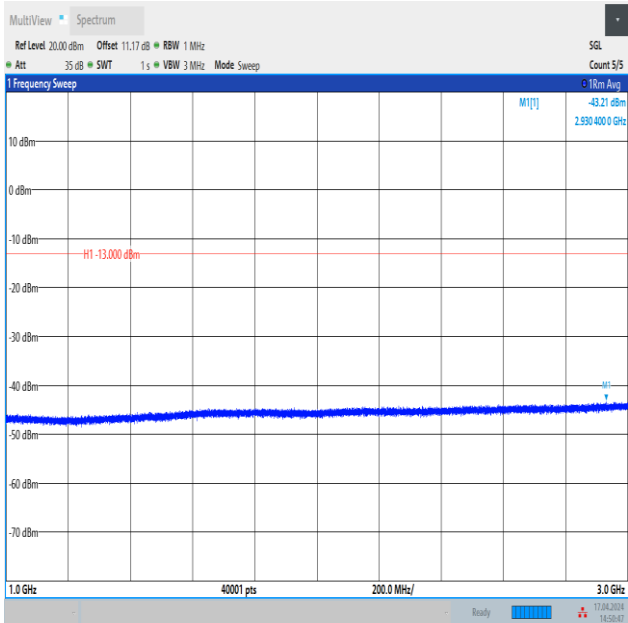
Band12_5MHz_16QAM_23155_1RB#0_1000~3000_1000~3000
