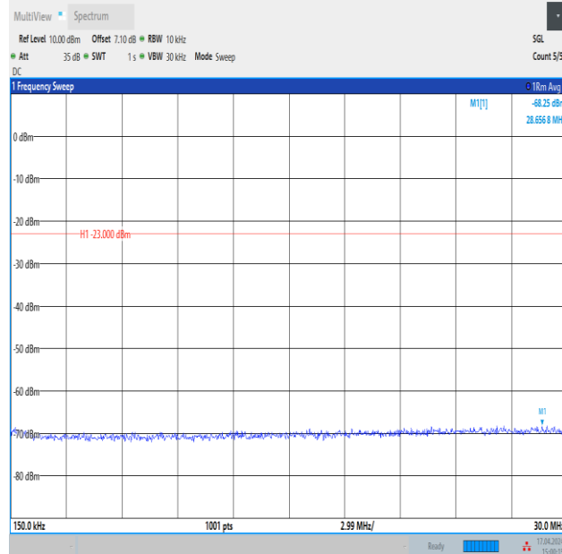
Band12_3MHz_QPSK_23095_1RB#0_0.15~30_0.15~30
