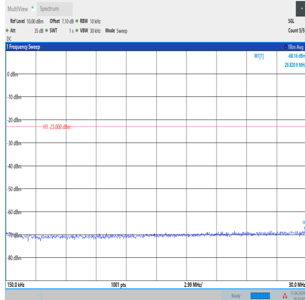
Band12_3MHz_QPSK_23025_1RB#14_0.15~30_0.15~30
