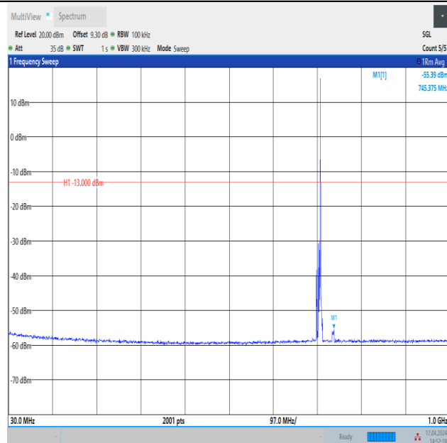
Band12_5MHz_16QAM_23155_1RB#24_30~1000_30~1000
