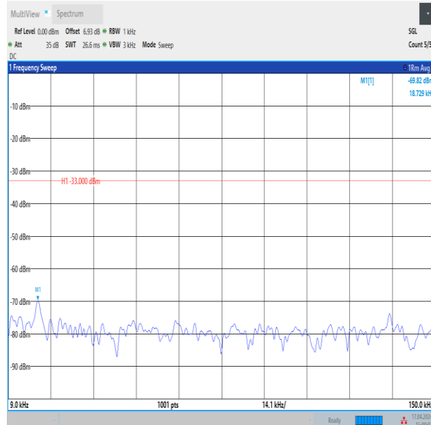
Band12_3MHz_QPSK_23095_1RB#0_0.009~0.15_0.009~0.15
