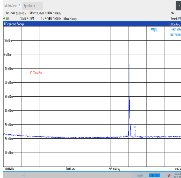
Band12_5MHz_QPSK_23155_1RB#24_30~1000_30~1000
