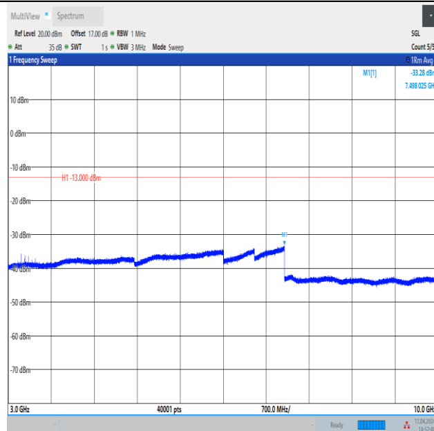
Band12_5MHz_16QAM_23155_1RB#24_3000~10000_3000~10000
