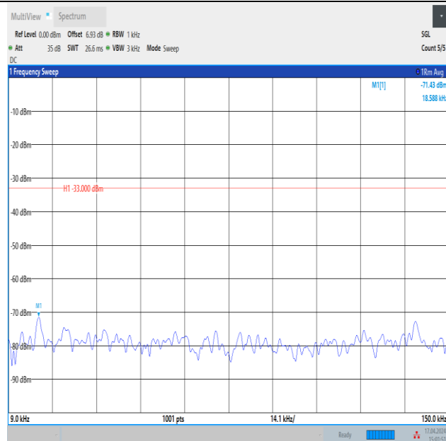
Band12_3MHz_QPSK_23095_1RB#14_0.009~0.15_0.009~0.15
