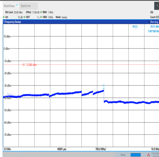
Band12_3MHz_QPSK_23025_1RB#14_3000~10000_3000~10000
