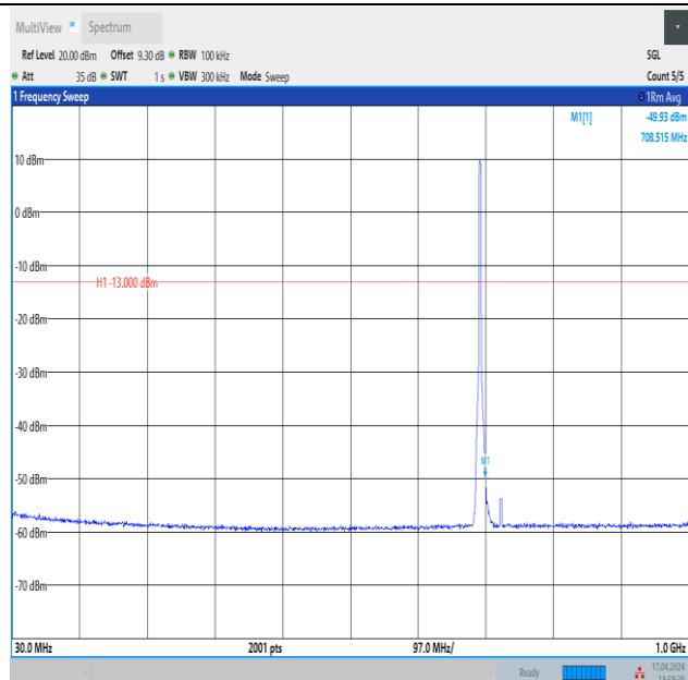
Band12_3MHz_QPSK_23025_15RB#0_30~1000_30~1000
