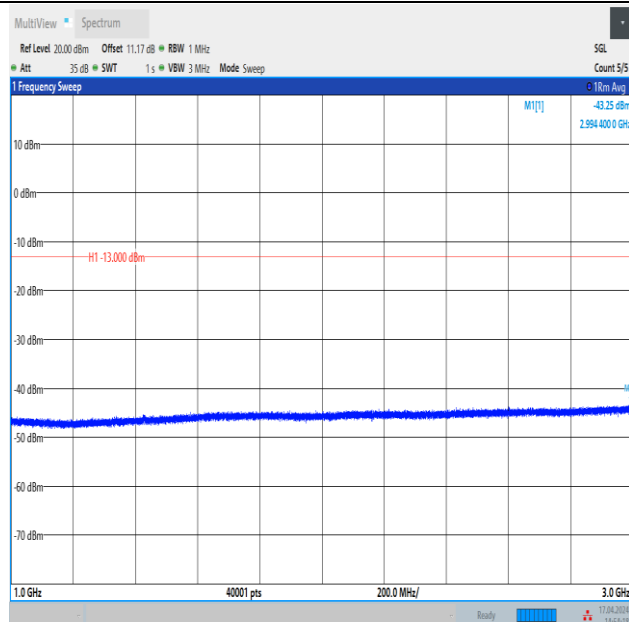
Band12_5MHz_16QAM_23155_25RB#0_1000~3000_1000~3000
