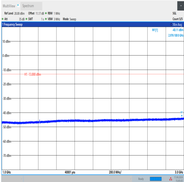
Band12_3MHz_16QAM_23095_15RB#0_1000~3000_1000~3000
