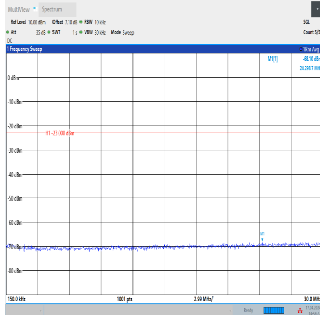
Band12_3MHz_QPSK_23025_15RB#0_0.15~30_0.15~30
