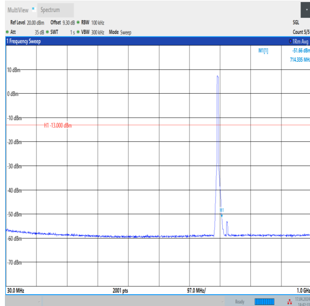
Band12_5MHz_QPSK_23035_25RB#0_30~1000_30~1000
