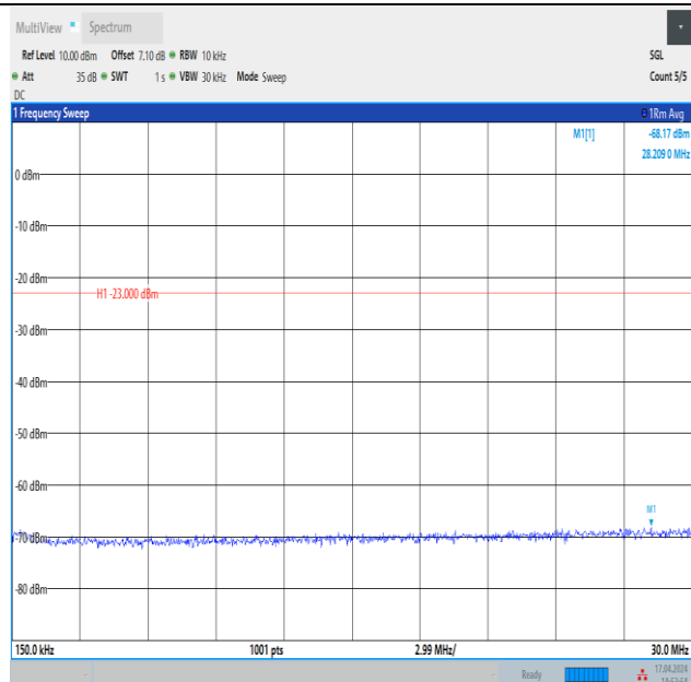
Band12_5MHz_16QAM_23155_25RB#0_0.15~30_0.15~30
