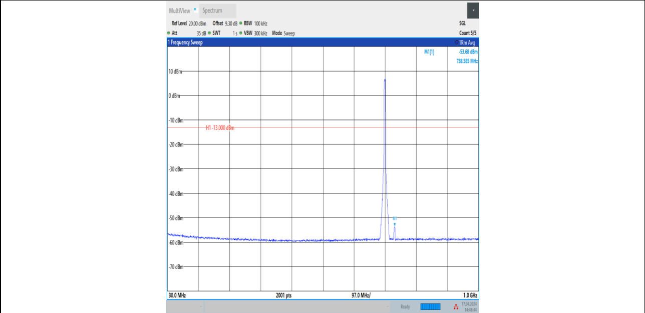
Band12_5MHz_16QAM_23095_25RB#0_30~1000_30~1000
