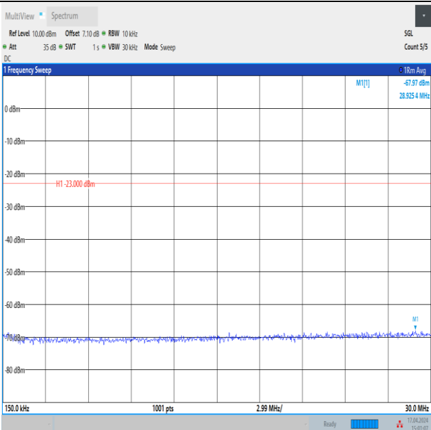
Band12_3MHz_16QAM_23095_1RB#0_0.15~30_0.15~30
