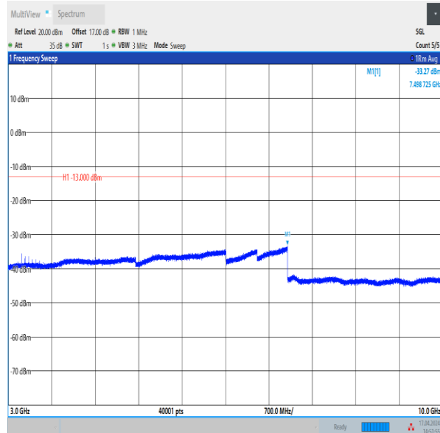
Band12_5MHz_QPSK_23155_1RB#24_3000~10000_3000~10000
