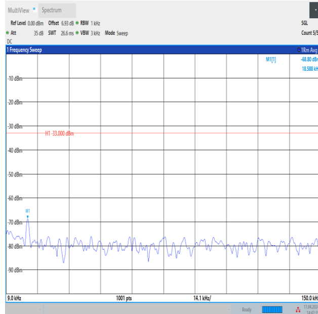
Band12_5MHz_QPSK_23095_25RB#0_0.009~0.15_0.009~0.15
