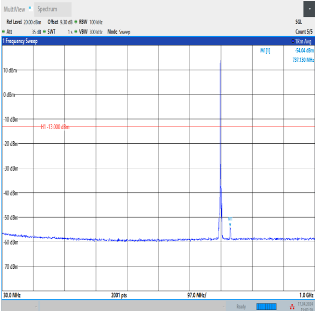
Band12_3MHz_16QAM_23095_1RB#0_30~1000_30~1000
