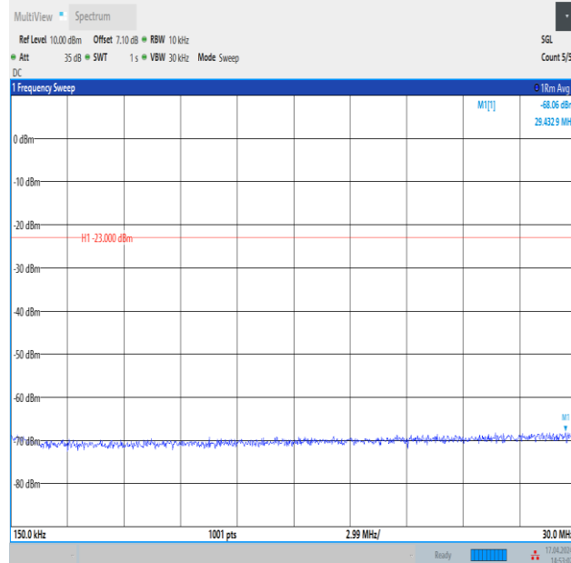
Band12_5MHz_QPSK_23155_25RB#0_0.15~30_0.15~30
