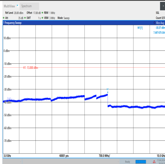
Band12_5MHz_16QAM_23155_25RB#0_3000~10000_3000~10000
