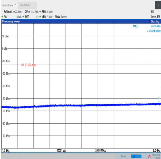
Band12_5MHz_16QAM_23095_25RB#0_1000~3000_1000~3000
