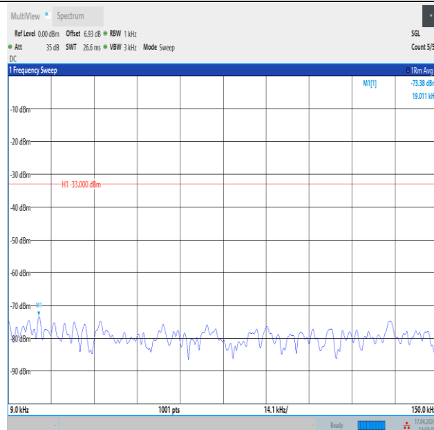
Band12_3MHz_QPSK_23025_15RB#0_0.009~0.15_0.009~0.15
