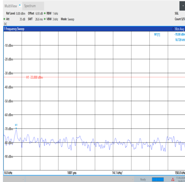
Band12_5MHz_QPSK_23155_1RB#0_0.009~0.15_0.009~0.15
