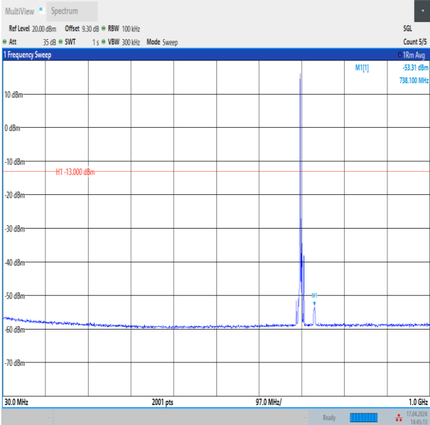
Band12_5MHz_16QAM_23095_1RB#0_30~1000_30~1000
