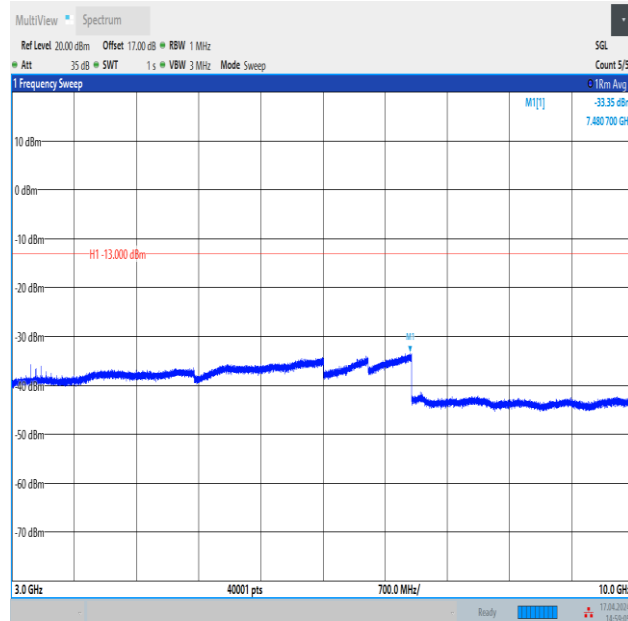
Band12_3MHz_QPSK_23025_15RB#0_3000~10000_3000~10000
