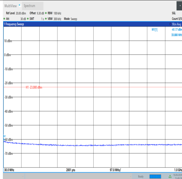
Band4_20MHz_16QAM_20300_1RB#0_30~1000_30~1000
