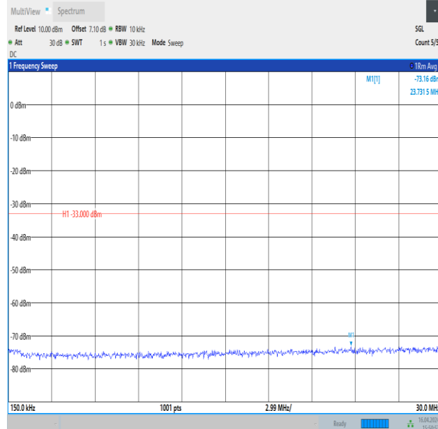
Band4_20MHz_16QAM_20300_1RB#99_0.15~30_0.15~30
