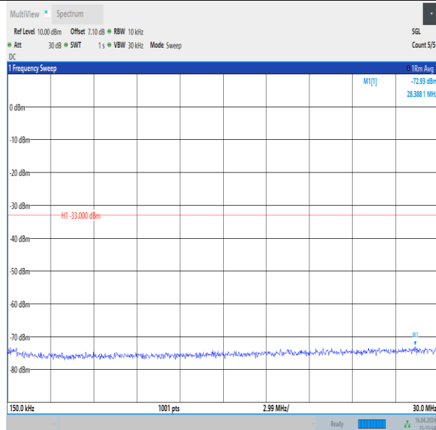
Band4_1.4MHz_QPSK_20393_1RB#5_0.15~30_0.15~30
