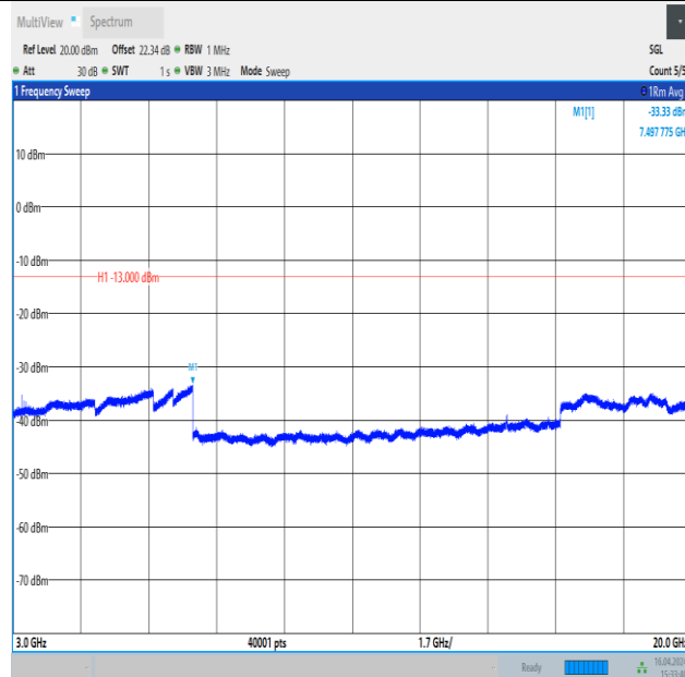
Band4_1.4MHz_16QAM_20393_1RB#0_3000~20000_3000~20000
