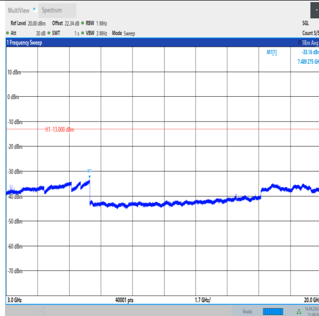
Band4_20MHz_16QAM_20175_1RB#99_3000~20000_3000~20000
