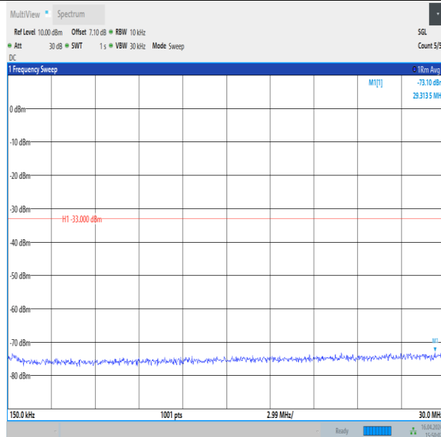
Band4_20MHz_QPSK_20300_1RB#99_0.15~30_0.15~30
