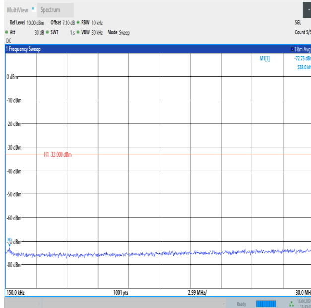
Band4_20MHz_QPSK_20050_1RB#99_0.15~30_0.15~30
