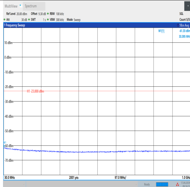
Band4_3MHz_16QAM_19965_1RB#0_30~1000_30~1000
