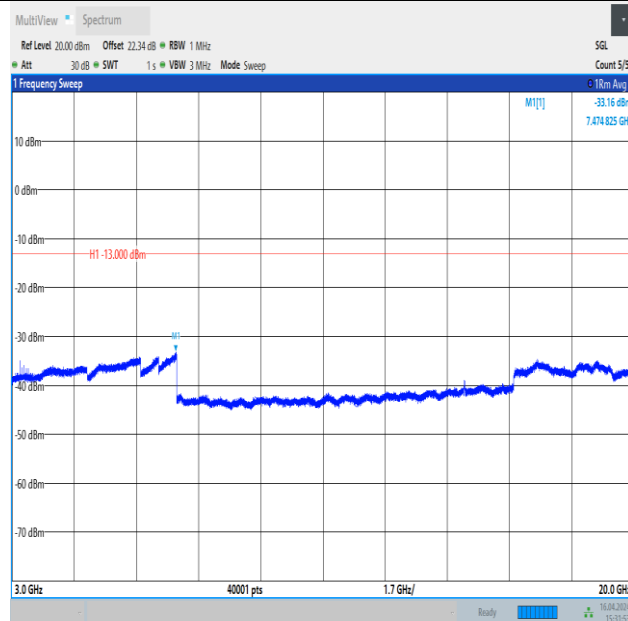
Band4_1.4MHz_16QAM_20175_6RB#0_3000~20000_3000~20000
