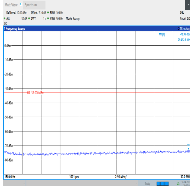
Band4_20MHz_16QAM_20175_1RB#99_0.15~30_0.15~30
