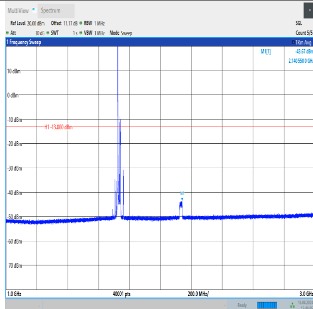
Band4_20MHz_16QAM_20175_1RB#0_1000~3000_1000~3000
