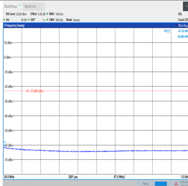
Band4_3MHz_QPSK_19965_1RB#0_30~1000_30~1000
