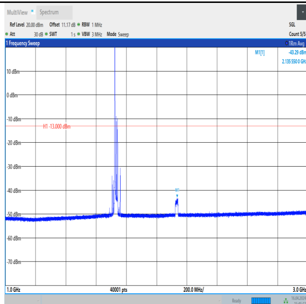
Band4_20MHz_QPSK_20175_1RB#0_1000~3000_1000~3000
