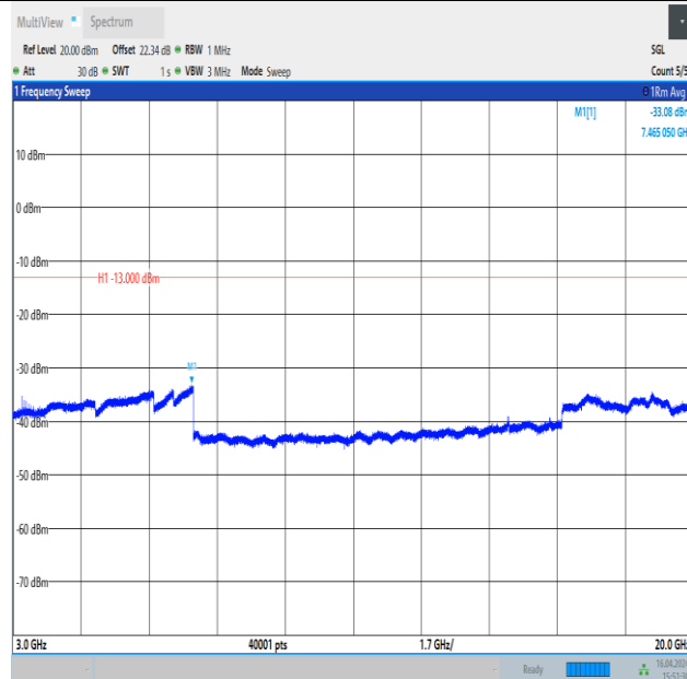
Band4_20MHz_16QAM_20300_1RB#99_3000~20000_3000~20000
