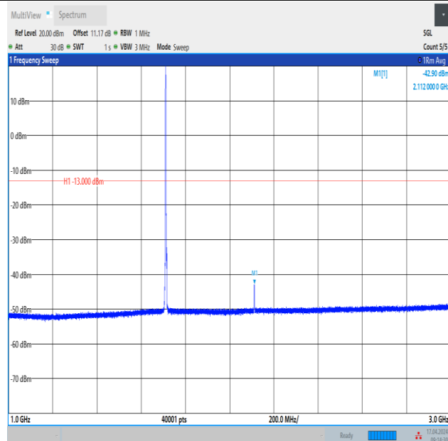
Band4_3MHz_16QAM_19965_1RB#0_1000~3000_1000~3000
