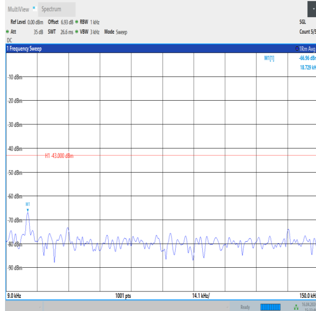
Band4_1.4MHz_QPSK_20393_1RB#5_0.009~0.15_0.009~0.15
