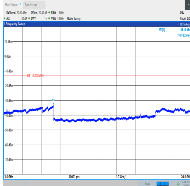
Band4_1.4MHz_QPSK_20393_1RB#5_3000~20000_3000~20000
