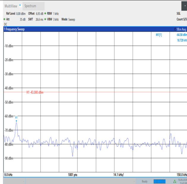
Band4_20MHz_16QAM_20050_1RB#0_0.009~0.15_0.009~0.15
