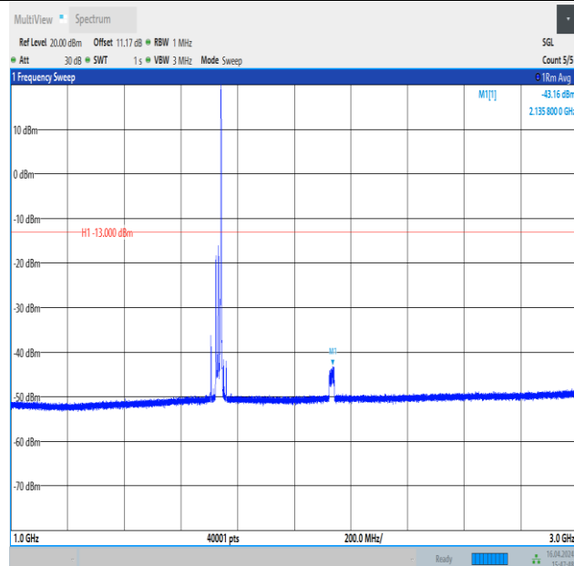
Band4_20MHz_16QAM_20175_1RB#99_1000~3000_1000~3000
