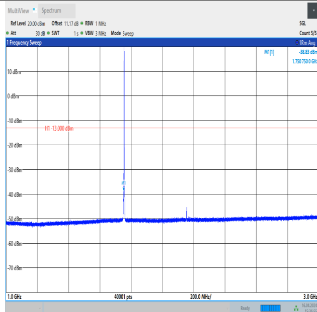
Band4_1.4MHz_16QAM_20393_6RB#0_1000~3000_1000~3000
