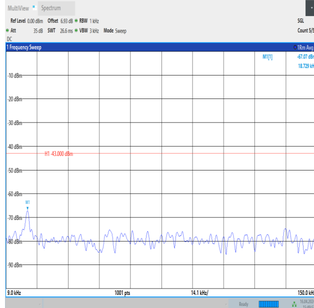
Band4_20MHz_QPSK_20300_1RB#99_0.009~0.15_0.009~0.15
