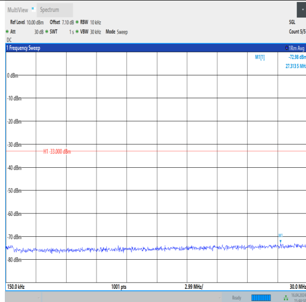
Band4_20MHz_QPSK_20175_1RB#0_0.15~30_0.15~30
