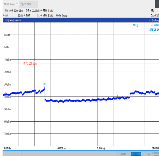
Band4_20MHz_QPSK_20300_1RB#99_3000~20000_3000~20000
