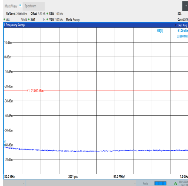
Band4_20MHz_16QAM_20175_1RB#99_30~1000_30~1000
