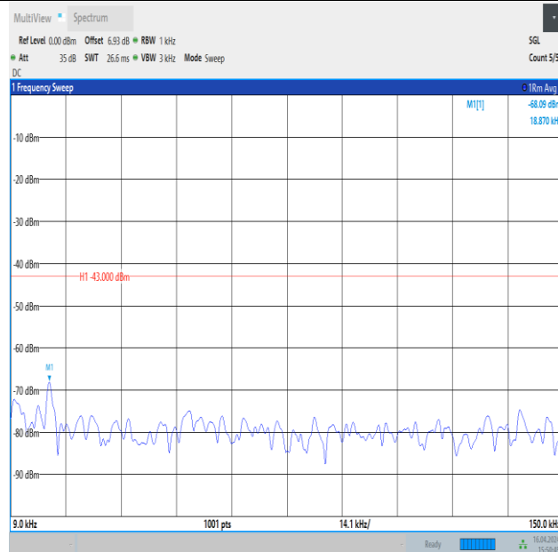
Band4_20MHz_16QAM_20300_1RB#99_0.009~0.15_0.009~0.15
