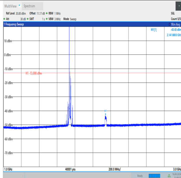
Band4_20MHz_16QAM_20300_1RB#0_1000~3000_1000~3000
