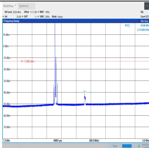
Band4_20MHz_QPSK_20050_1RB#0_1000~3000_1000~3000
