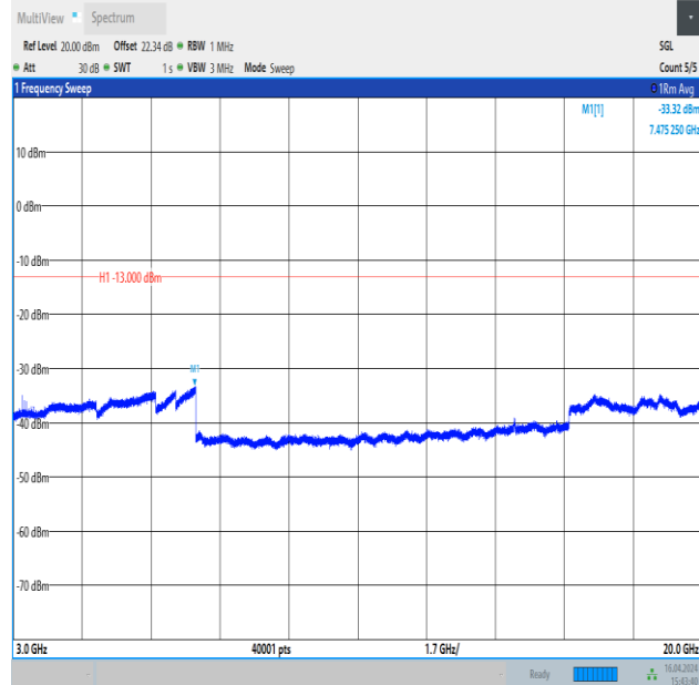
Band4_20MHz_QPSK_20050_1RB#99_3000~20000_3000~20000
