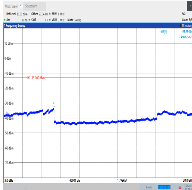
Band4_3MHz_16QAM_19965_1RB#0_3000~20000_3000~20000
