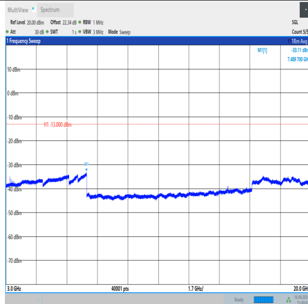
Band4_20MHz_16QAM_20300_1RB#0_3000~20000_3000~20000
