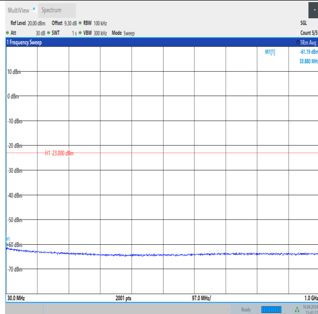
Band4_20MHz_16QAM_20050_1RB#0_30~1000_30~1000
