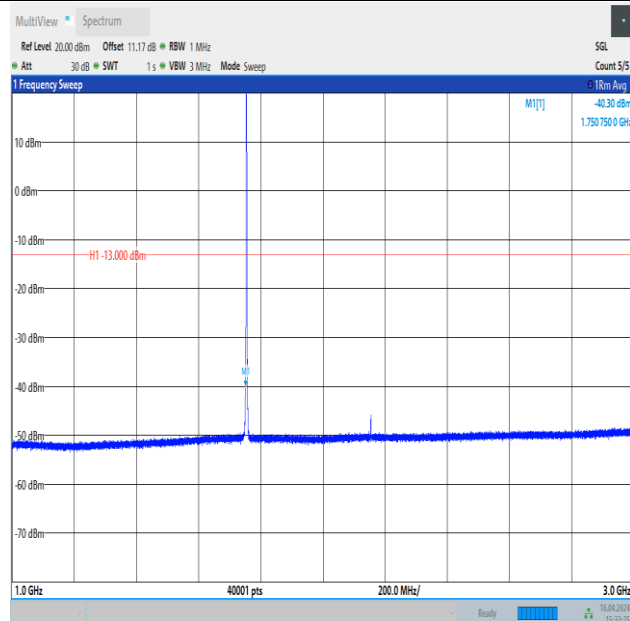
Band4_1.4MHz_16QAM_20393_1RB#0_1000~3000_1000~3000
