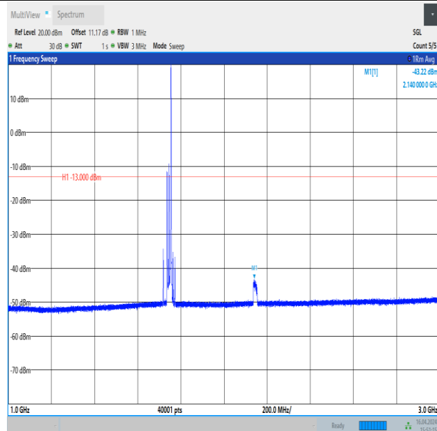
Band4_20MHz_16QAM_20300_1RB#99_1000~3000_1000~3000
