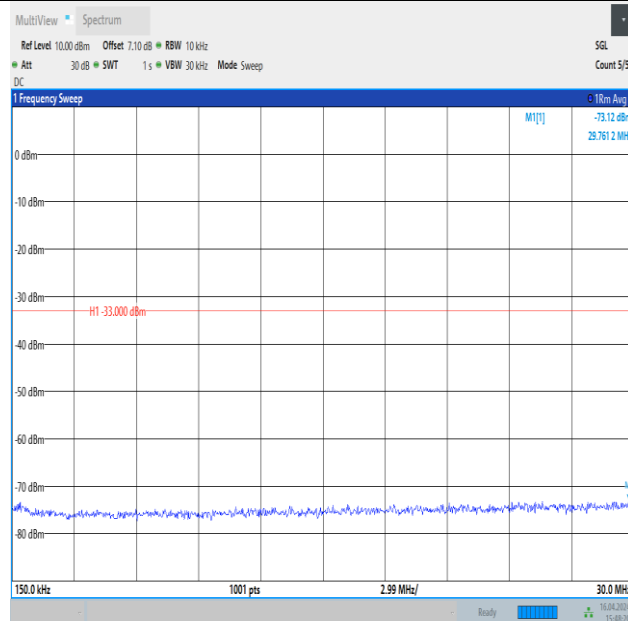
Band4_20MHz_QPSK_20300_1RB#0_0.15~30_0.15~30
