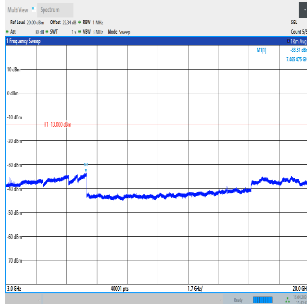
Band4_20MHz_16QAM_20050_1RB#0_3000~20000_3000~20000
