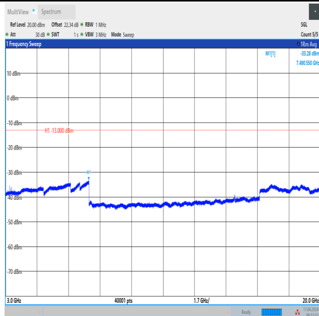
Band4_3MHz_QPSK_19965_1RB#0_3000~20000_3000~20000
