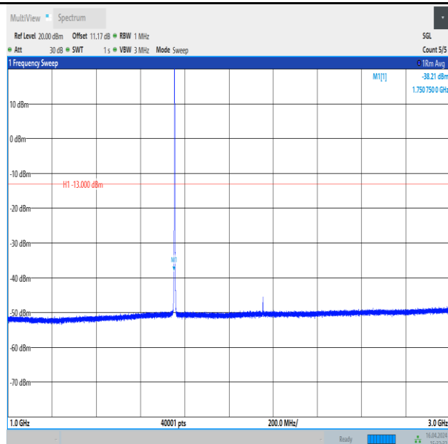
Band4_1.4MHz_QPSK_20393_1RB#0_1000~3000_1000~3000
