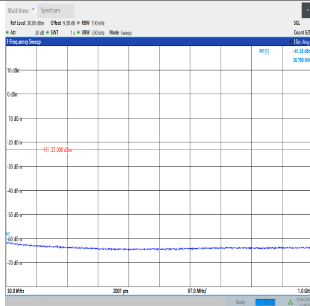
Band4_20MHz_QPSK_20300_1RB#0_30~1000_30~1000
