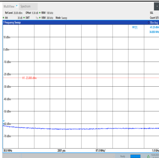
Band4_1.4MHz_16QAM_20393_1RB#5_30~1000_30~1000
