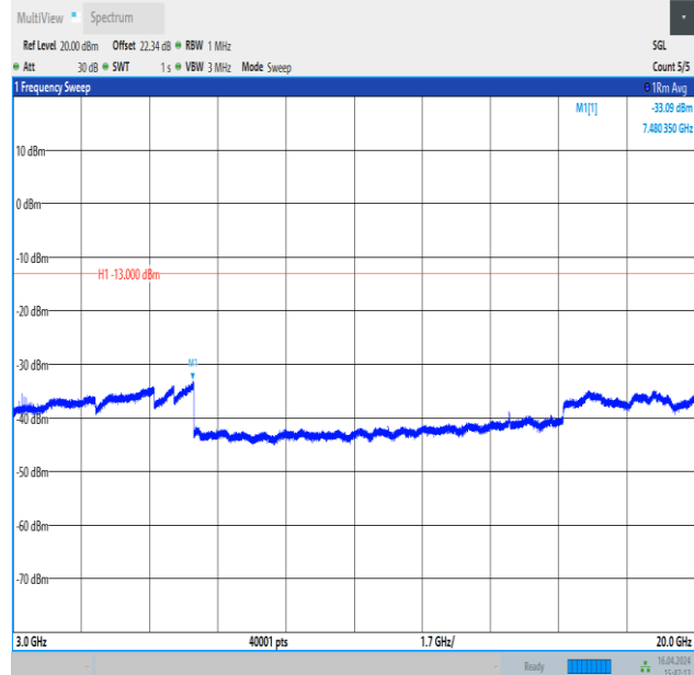
Band4_20MHz_QPSK_20175_1RB#99_3000~20000_3000~20000
