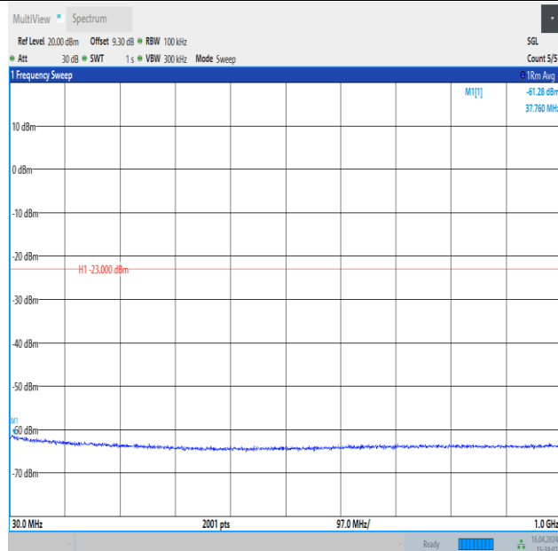
Band4_1.4MHz_QPSK_20393_1RB#5_30~1000_30~1000
