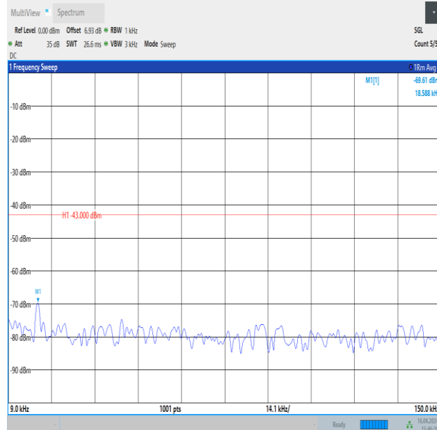
Band4_20MHz_QPSK_20175_1RB#99_0.009~0.15_0.009~0.15
