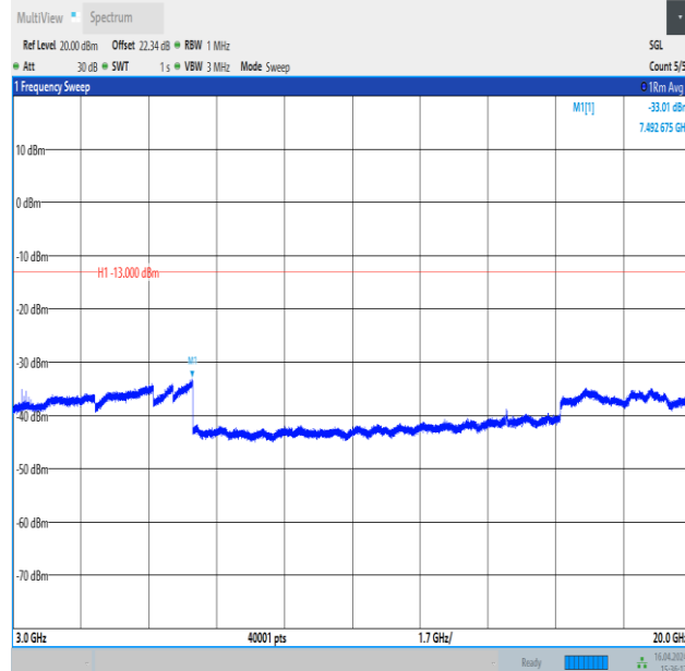
Band4_1.4MHz_QPSK_20393_6RB#0_3000~20000_3000~20000
