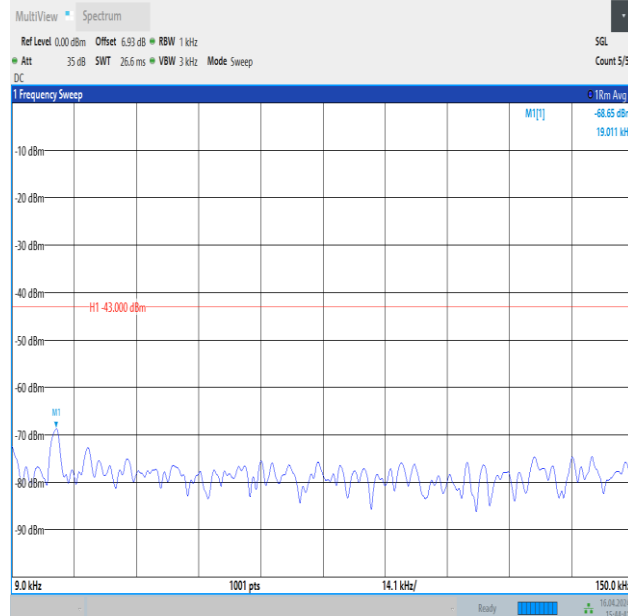
Band4_20MHz_QPSK_20175_1RB#0_0.009~0.15_0.009~0.15
