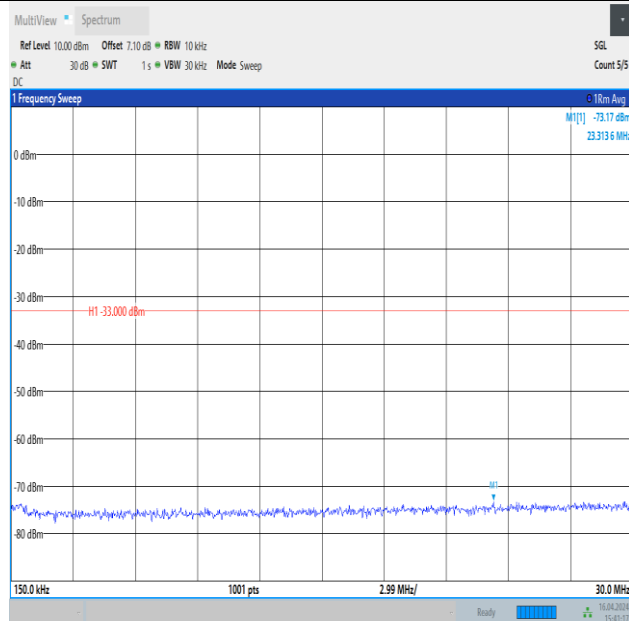
Band4_20MHz_QPSK_20050_1RB#0_0.15~30_0.15~30
