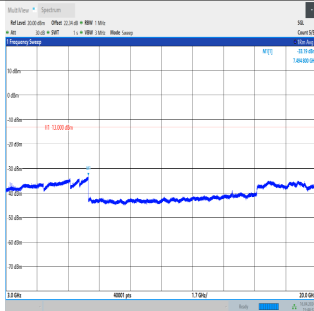
Band4_20MHz_16QAM_20050_1RB#99_3000~20000_3000~20000
