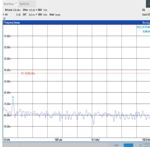
Band4_20MHz_QPSK_20050_1RB#0_0.009~0.15_0.009~0.15
