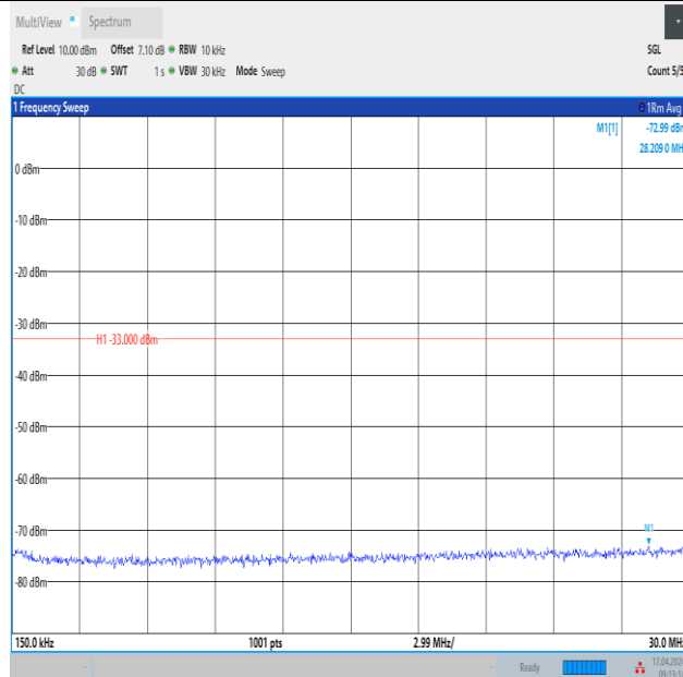
Band4_3MHz_QPSK_19965_1RB#0_0.15~30_0.15~30
