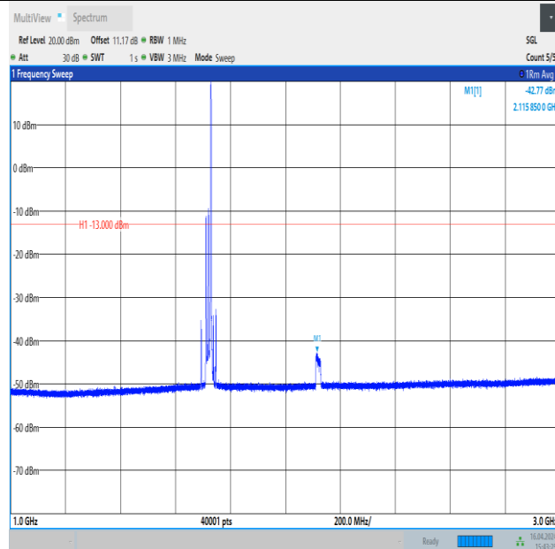
Band4_20MHz_QPSK_20050_1RB#99_1000~3000_1000~3000
