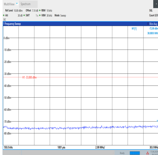
Band4_3MHz_16QAM_19965_1RB#0_0.15~30_0.15~30
