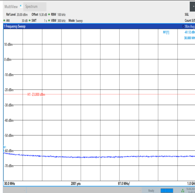
Band4_20MHz_QPSK_20050_1RB#99_30~1000_30~1000
