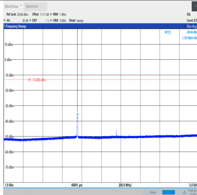
Band4_1.4MHz_QPSK_20393_1RB#5_1000~3000_1000~3000
