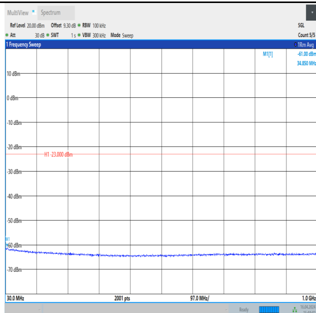
Band4_20MHz_16QAM_20050_1RB#99_30~1000_30~1000
