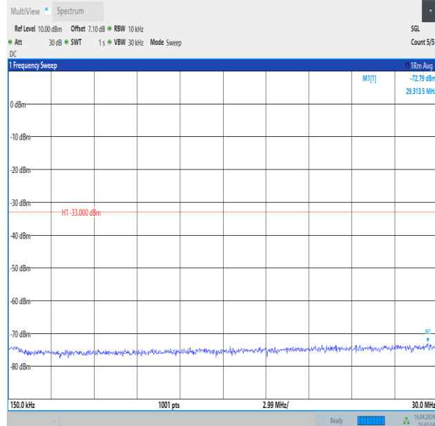
Band4_20MHz_16QAM_20050_1RB#99_0.15~30_0.15~30
