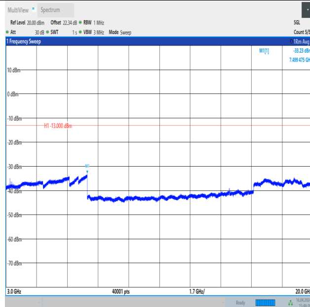
Band4_20MHz_16QAM_20175_1RB#0_3000~20000_3000~20000
