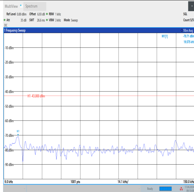
Band4_3MHz_16QAM_19965_1RB#0_0.009~0.15_0.009~0.15
