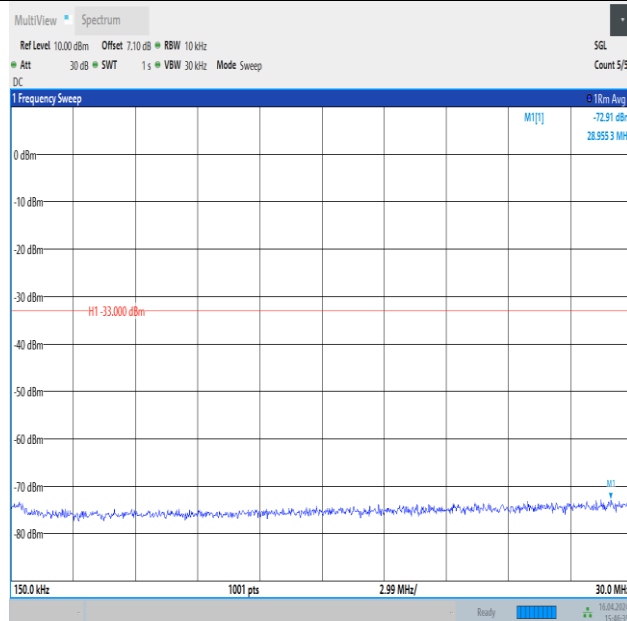
Band4_20MHz_QPSK_20175_1RB#99_0.15~30_0.15~30
