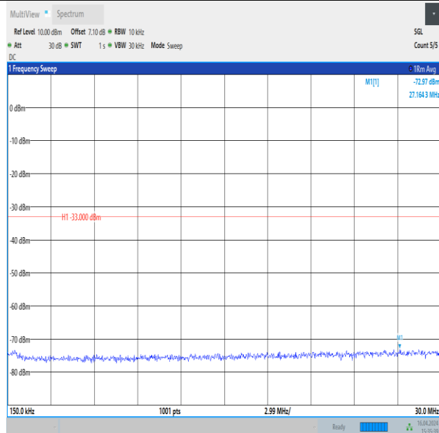
Band4_1.4MHz_QPSK_20393_6RB#0_0.15~30_0.15~30
