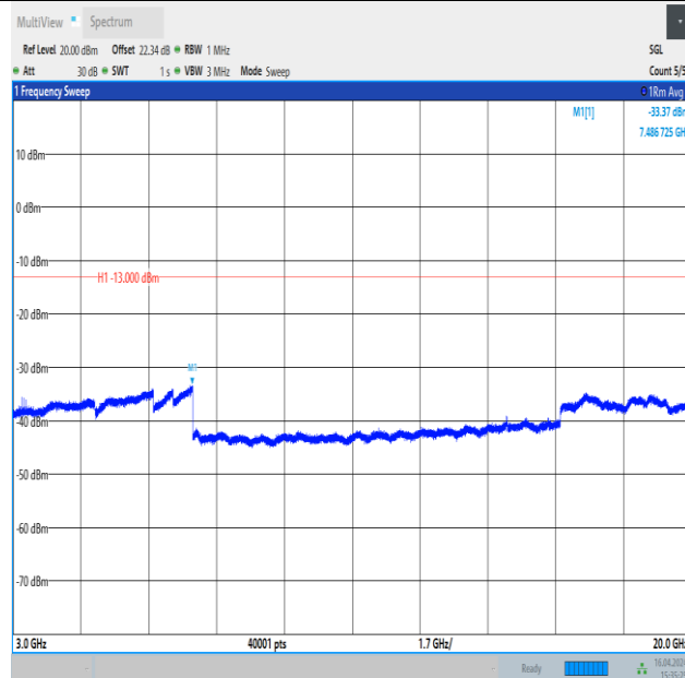
Band4_1.4MHz_16QAM_20393_1RB#5_3000~20000_3000~20000
