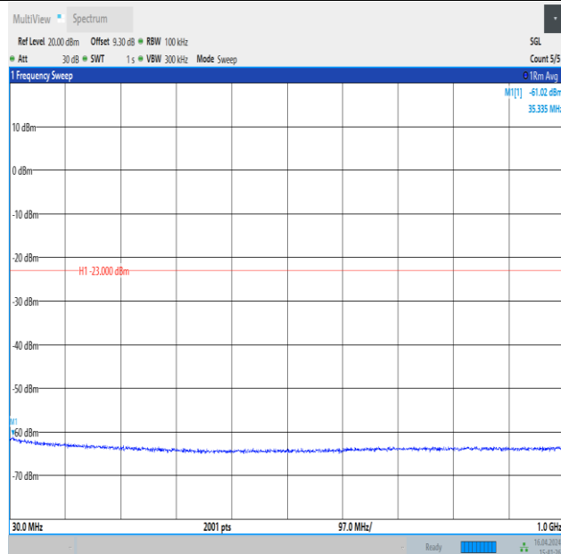
Band4_20MHz_QPSK_20050_1RB#0_30~1000_30~1000
