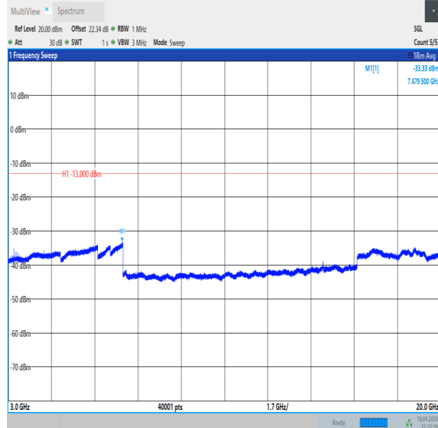
Band4_1.4MHz_QPSK_19957_1RB#0_3000~20000_3000~20000
