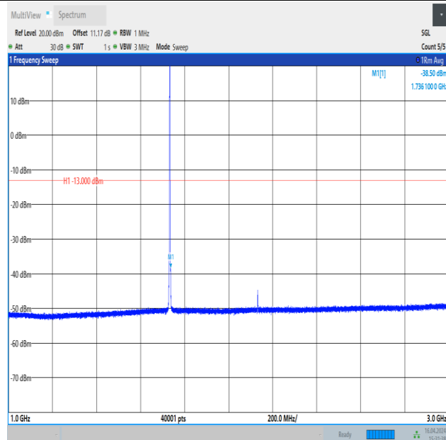
Band4_1.4MHz_16QAM_20175_6RB#0_1000~3000_1000~3000
