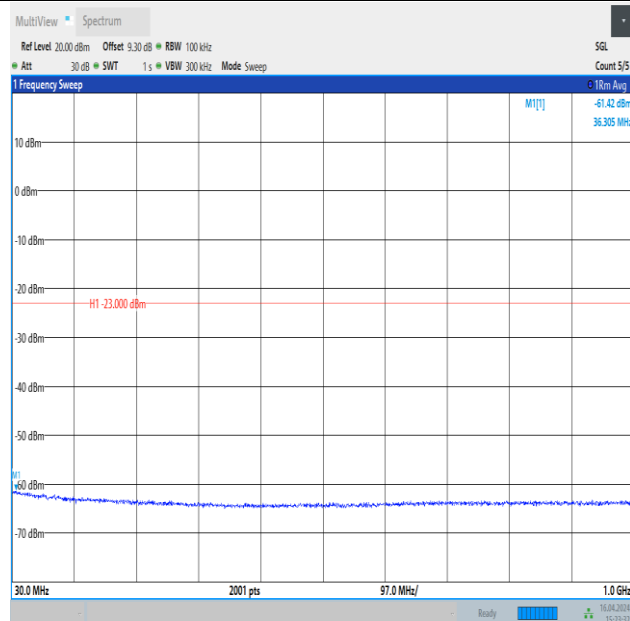
Band4_1.4MHz_QPSK_19957_1RB#5_30~1000_30~1000
