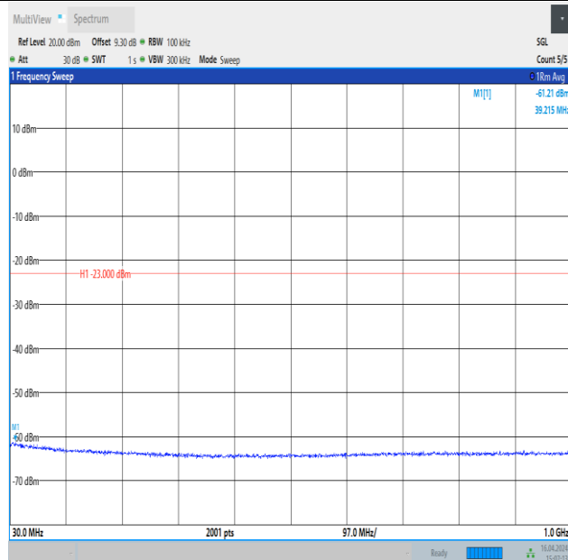
Band4_15MHz_QPSK_20025_75RB#0_30~1000_30~1000
