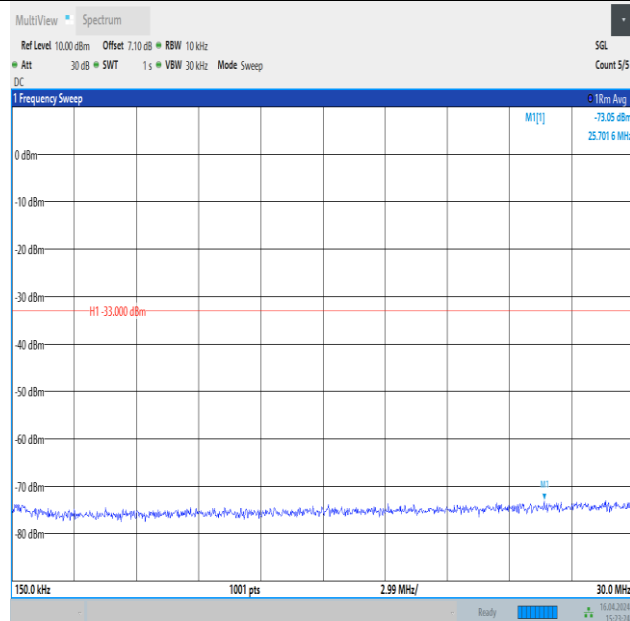
Band4_1.4MHz_QPSK_19957_1RB#5_0.15~30_0.15~30
