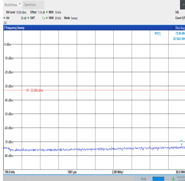
Band4_20MHz_QPSK_20300_100RB#0_0.15~30_0.15~30
