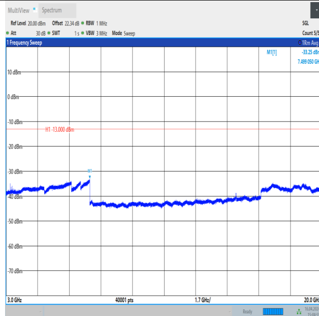
Band4_10MHz_16QAM_20350_1RB#0_3000~20000_3000~20000
