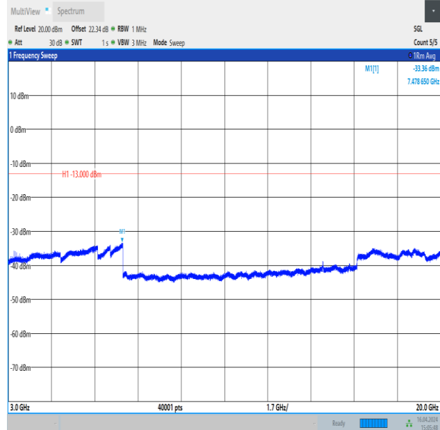
Band4_10MHz_QPSK_20350_1RB#49_3000~20000_3000~20000
