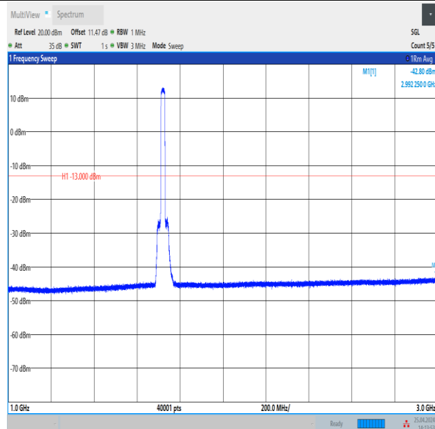
Band4_20MHz_QPSK_20050_100RB#0_1000~3000_1000~3000
