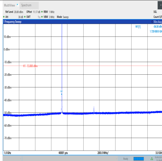
Band4_1.4MHz_QPSK_20175_6RB#0_1000~3000_1000~3000
