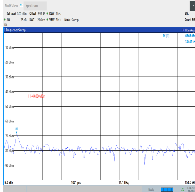
Band4_20MHz_QPSK_20175_100RB#0_0.009~0.15_0.009~0.15
