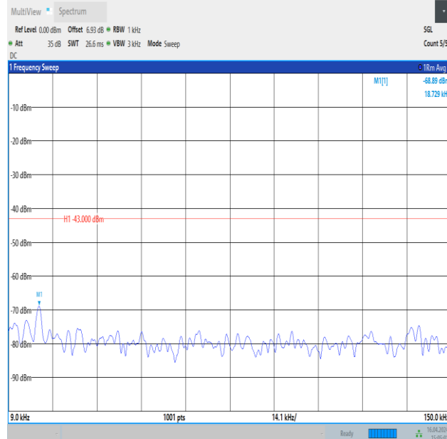
Band4_10MHz_QPSK_20350_1RB#49_0.009~0.15_0.009~0.15
