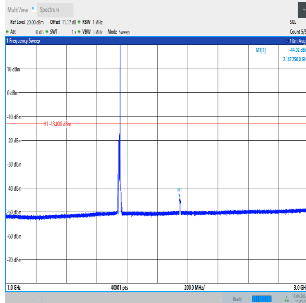
Band4_10MHz_QPSK_20350_1RB#49_1000~3000_1000~3000
