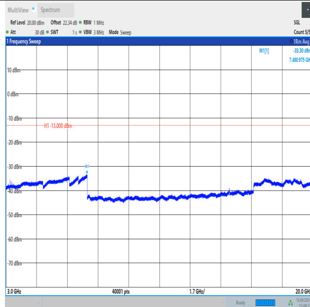
Band4_15MHz_QPSK_20175_75RB#0_3000~20000_3000~20000
