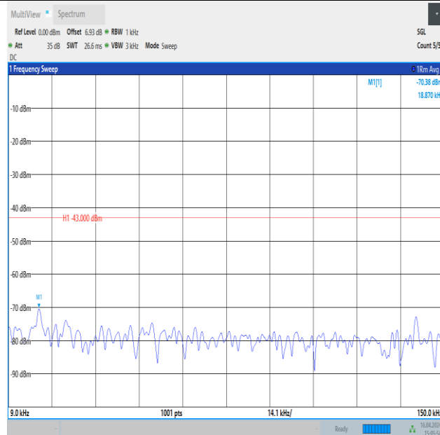
Band4_10MHz_16QAM_20350_1RB#49_0.009~0.15_0.009~0.15
