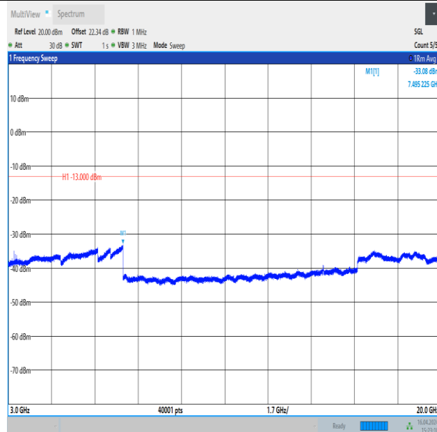
Band4_1.4MHz_16QAM_19957_1RB#0_3000~20000_3000~20000
