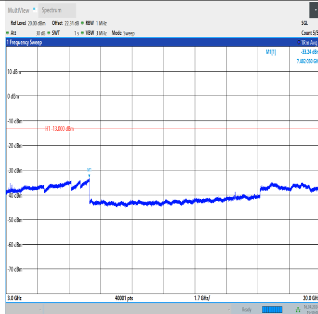
Band4_1.4MHz_16QAM_20175_1RB#5_3000~20000_3000~20000
