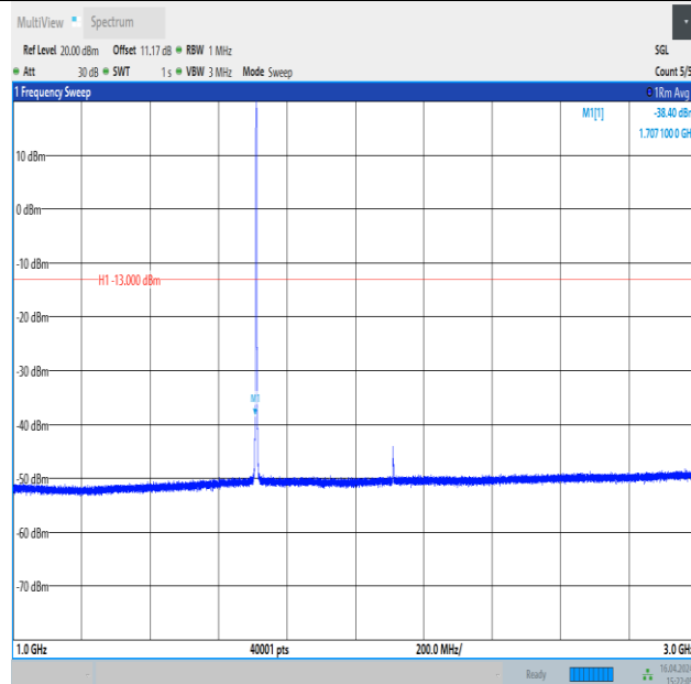
Band4_1.4MHz_QPSK_19957_1RB#0_1000~3000_1000~3000
