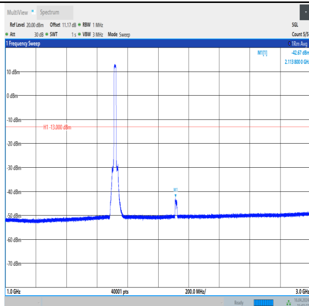
Band4_15MHz_QPSK_20025_75RB#0_1000~3000_1000~3000
