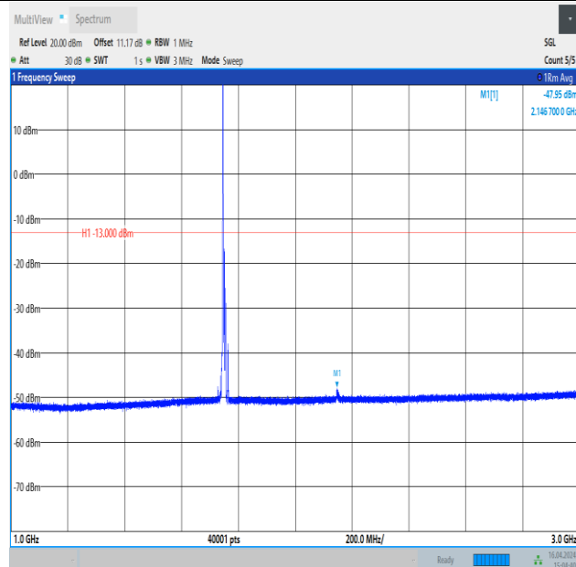
Band4_10MHz_16QAM_20350_1RB#0_1000~3000_1000~3000
