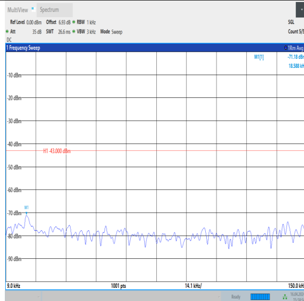
Band4_20MHz_QPSK_20300_100RB#0_0.009~0.15_0.009~0.15
