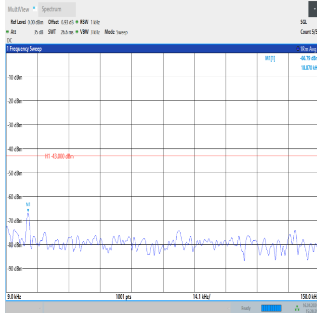
Band4_1.4MHz_QPSK_20175_1RB#5_0.009~0.15_0.009~0.15
