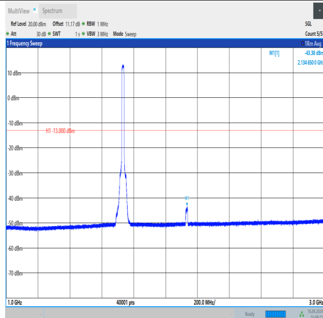
Band4_15MHz_QPSK_20175_75RB#0_1000~3000_1000~3000
