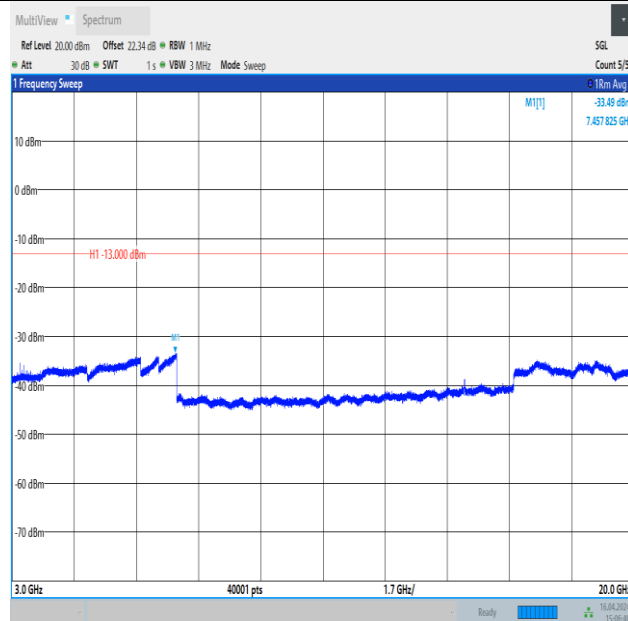
Band4_10MHz_16QAM_20350_1RB#49_3000~20000_3000~20000
