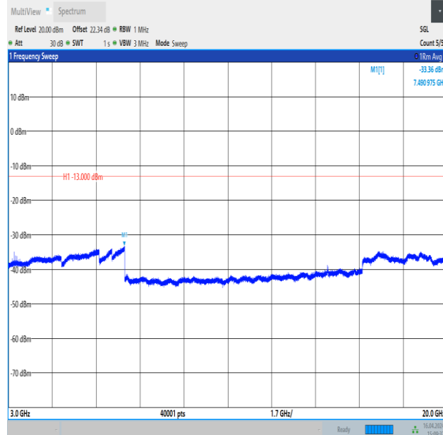
Band4_15MHz_QPSK_20325_75RB#0_3000~20000_3000~20000
