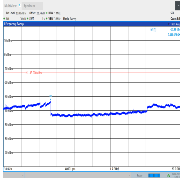
Band4_1.4MHz_16QAM_19957_6RB#0_3000~20000_3000~20000
