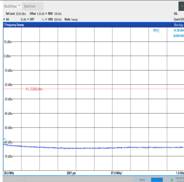
Band4_1.4MHz_QPSK_19957_6RB#0_30~1000_30~1000
