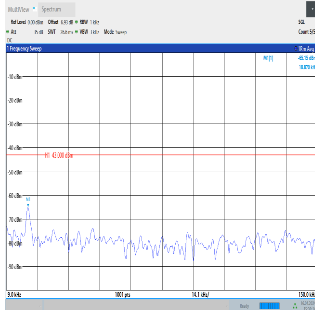
Band4_1.4MHz_QPSK_20175_6RB#0_0.009~0.15_0.009~0.15
