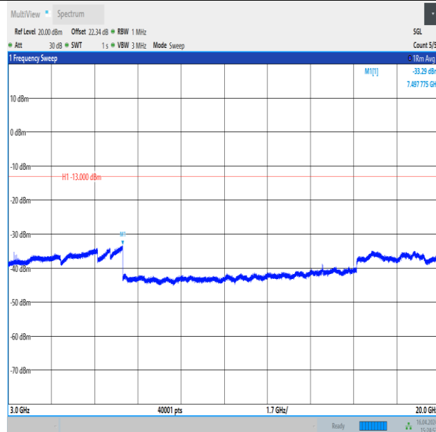
Band4_1.4MHz_16QAM_19957_1RB#5_3000~20000_3000~20000
