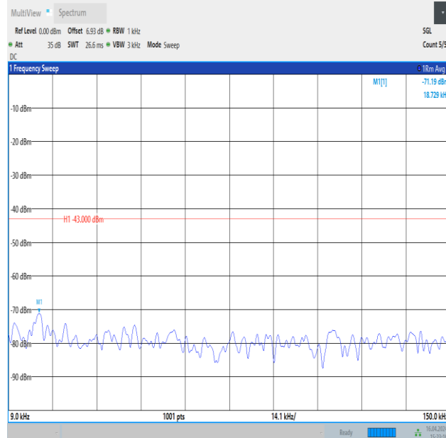
Band4_1.4MHz_QPSK_19957_1RB#5_0.009~0.15_0.009~0.15
