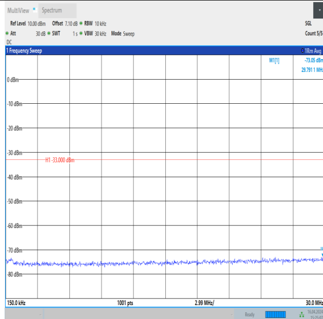
Band4_1.4MHz_QPSK_19957_6RB#0_0.15~30_0.15~30
