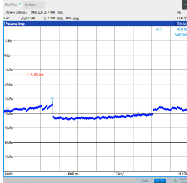
Band4_1.4MHz_QPSK_20175_6RB#0_3000~20000_3000~20000
