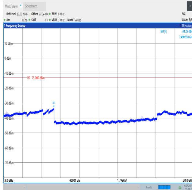
Band4_1.4MHz_16QAM_20175_1RB#0_3000~20000_3000~20000
