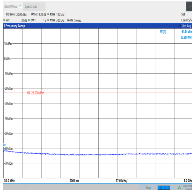
Band4_15MHz_QPSK_20325_75RB#0_30~1000_30~1000
