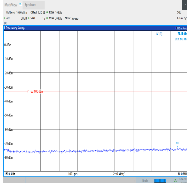
Band4_15MHz_QPSK_20175_75RB#0_0.15~30_0.15~30
