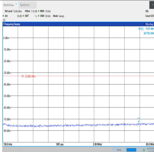
Band4_1.4MHz_QPSK_19957_1RB#0_0.15~30_0.15~30
