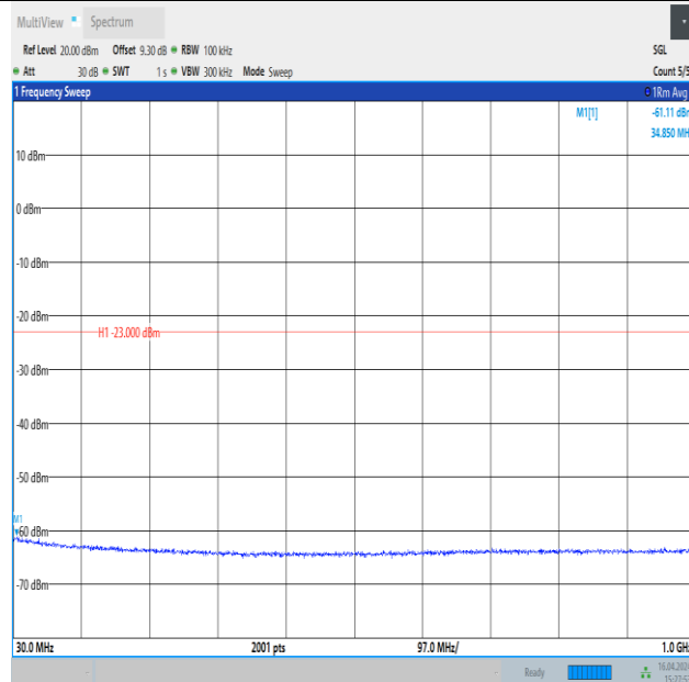
Band4_1.4MHz_16QAM_20175_1RB#0_30~1000_30~1000
