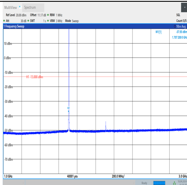
Band4_1.4MHz_QPSK_19957_6RB#0_1000~3000_1000~3000
