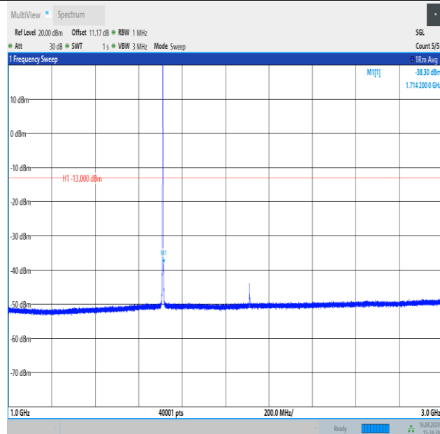
Band4_1.4MHz_16QAM_19957_1RB#5_1000~3000_1000~3000
