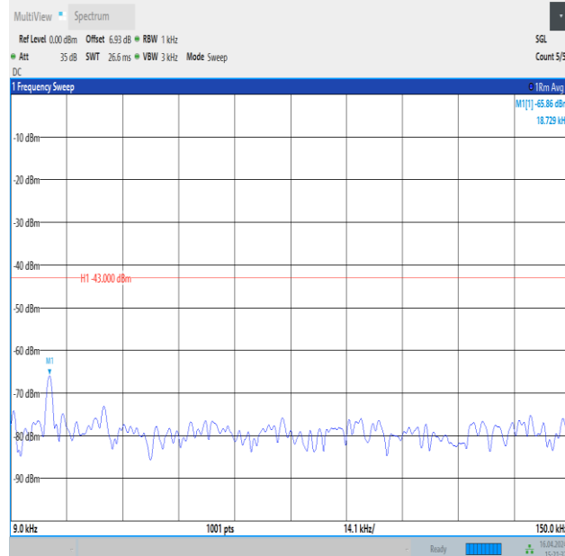
Band4_1.4MHz_QPSK_19957_1RB#0_0.009~0.15_0.009~0.15
