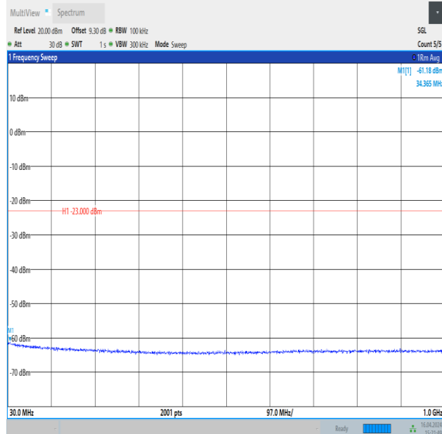
Band4_1.4MHz_QPSK_19957_1RB#0_30~1000_30~1000
