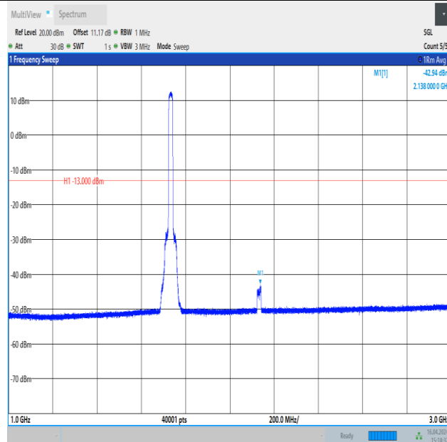
Band4_20MHz_QPSK_20175_100RB#0_1000~3000_1000~3000
