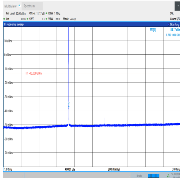
Band4_1.4MHz_16QAM_20175_1RB#5_1000~3000_1000~3000
