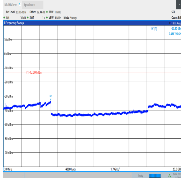
Band4_1.4MHz_QPSK_19957_1RB#5_3000~20000_3000~20000
