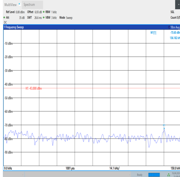
Band4_15MHz_QPSK_20325_75RB#0_0.009~0.15_0.009~0.15
