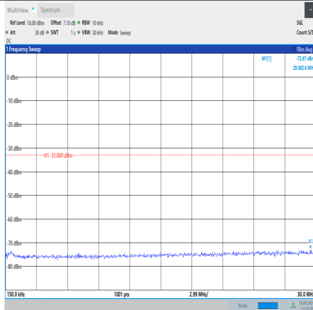
Band4_10MHz_QPSK_20350_1RB#49_0.15~30_0.15~30
