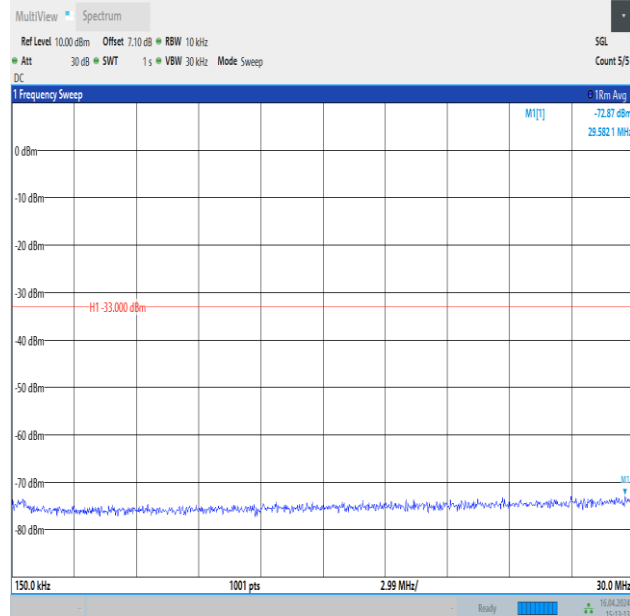
Band4_20MHz_QPSK_20050_100RB#0_0.15~30_0.15~30
