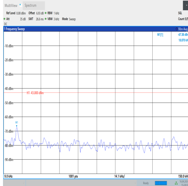
Band4_1.4MHz_QPSK_19957_6RB#0_0.009~0.15_0.009~0.15
