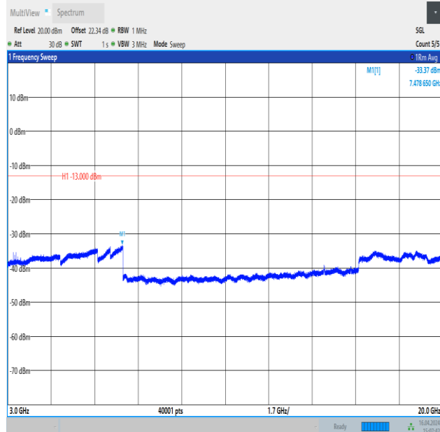
Band4_15MHz_QPSK_20025_75RB#0_3000~20000_3000~20000
