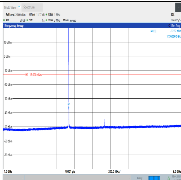
Band4_1.4MHz_QPSK_20175_1RB#5_1000~3000_1000~3000
