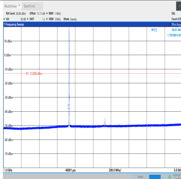
Band4_1.4MHz_16QAM_20175_1RB#0_1000~3000_1000~3000
