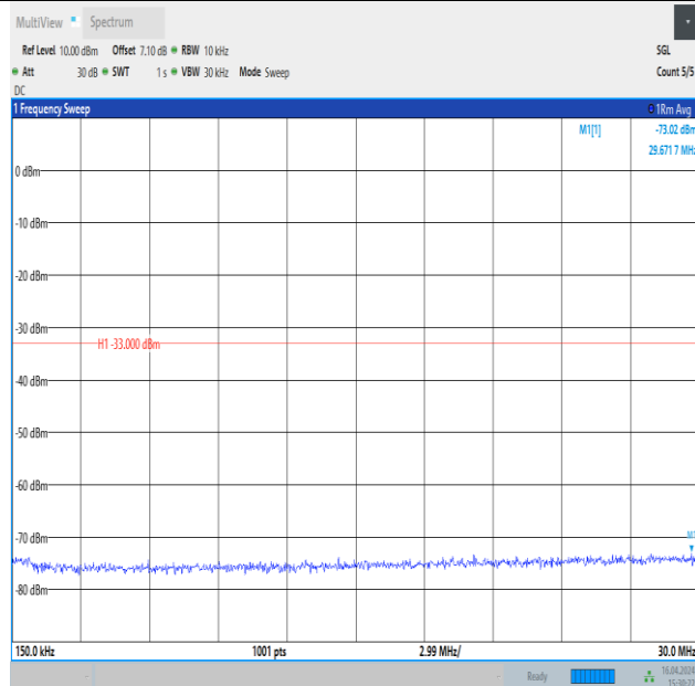
Band4_1.4MHz_QPSK_20175_6RB#0_0.15~30_0.15~30
