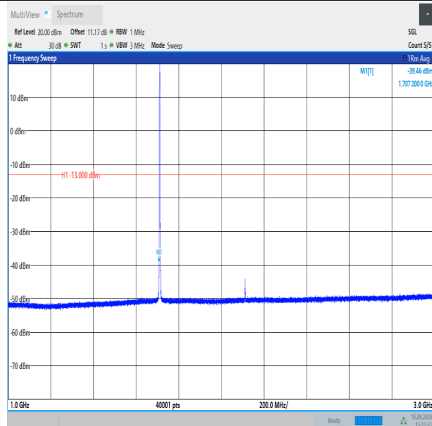
Band4_1.4MHz_16QAM_19957_1RB#0_1000~3000_1000~3000
