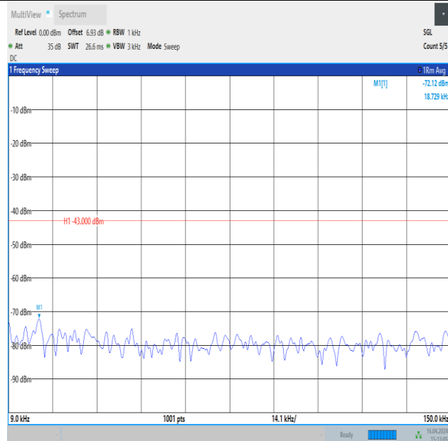
Band4_20MHz_QPSK_20050_100RB#0_0.009~0.15_0.009~0.15
