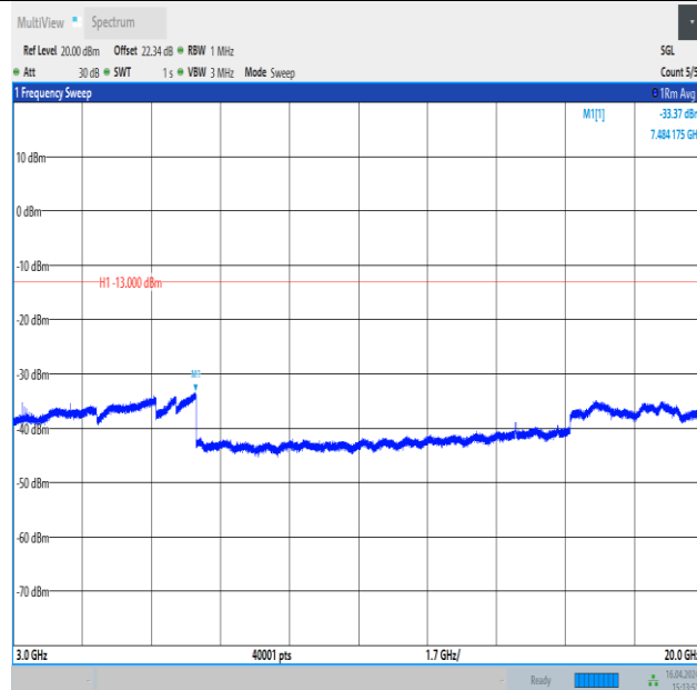
Band4_20MHz_QPSK_20050_100RB#0_3000~20000_3000~20000
