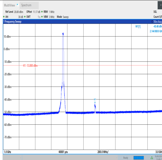
Band4_15MHz_QPSK_20325_75RB#0_1000~3000_1000~3000
