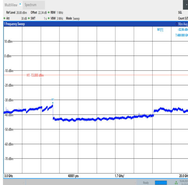
Band4_1.4MHz_QPSK_20175_1RB#0_3000~20000_3000~20000
