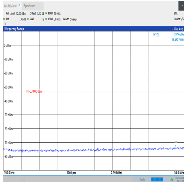
Band4_1.4MHz_QPSK_20175_1RB#0_0.15~30_0.15~30
