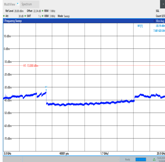
Band4_10MHz_QPSK_20000_1RB#49_3000~20000_3000~20000
