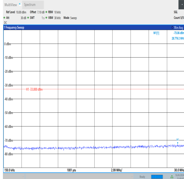
Band4_10MHz_16QAM_20175_1RB#0_0.15~30_0.15~30
