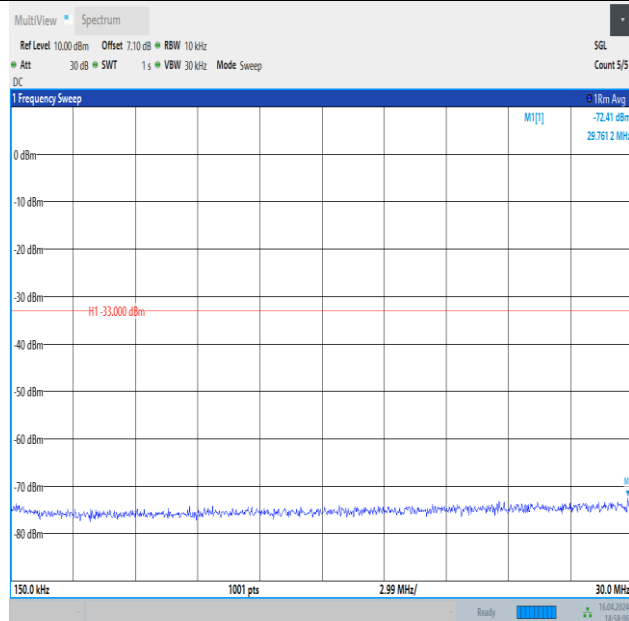
Band4_10MHz_QPSK_20000_1RB#49_0.15~30_0.15~30
