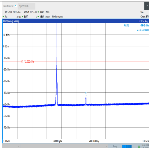
Band4_10MHz_QPSK_20175_1RB#0_1000~3000_1000~3000
