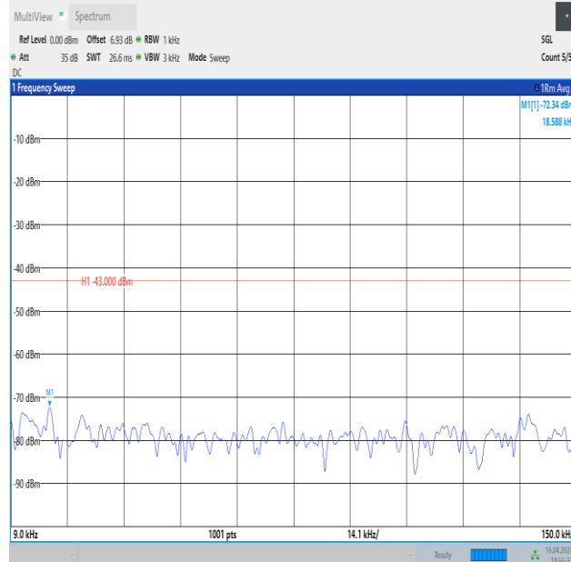
Band4_10MHz_QPSK_20000_1RB#0_0.009~0.15_0.009~0.15
