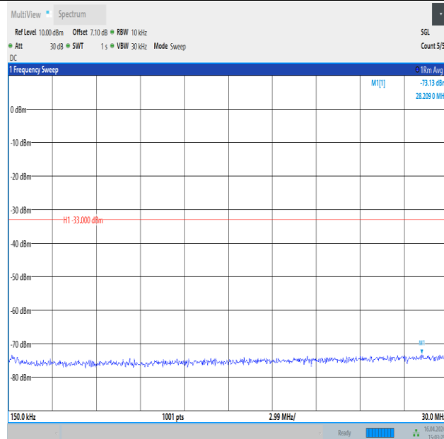
Band4_10MHz_QPSK_20350_1RB#0_0.15~30_0.15~30
