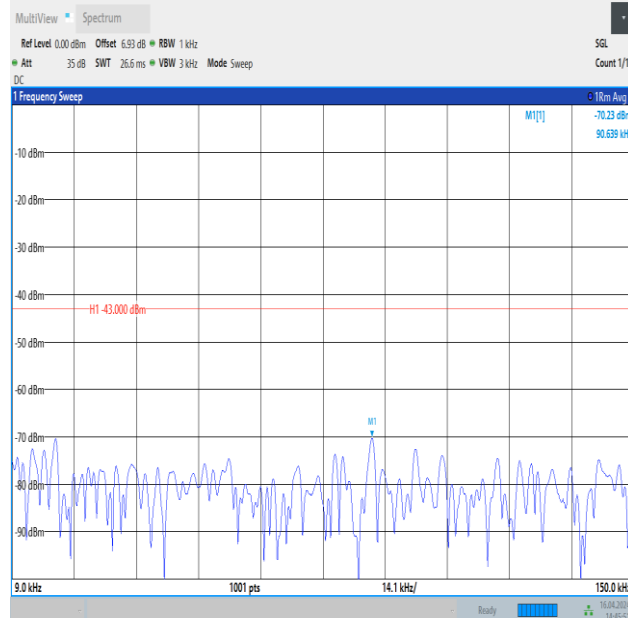
Band4_15MHz_16QAM_20175_1RB#74_0.009~0.15_0.009~0.15
