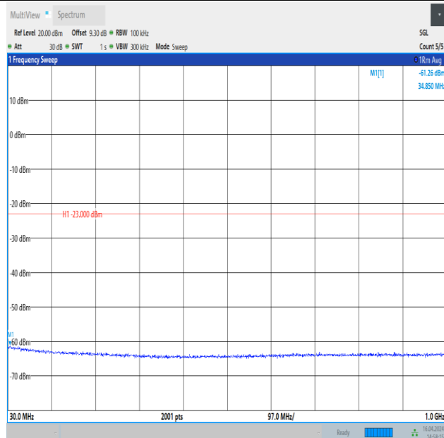
Band4_10MHz_QPSK_20000_1RB#49_30~1000_30~1000
