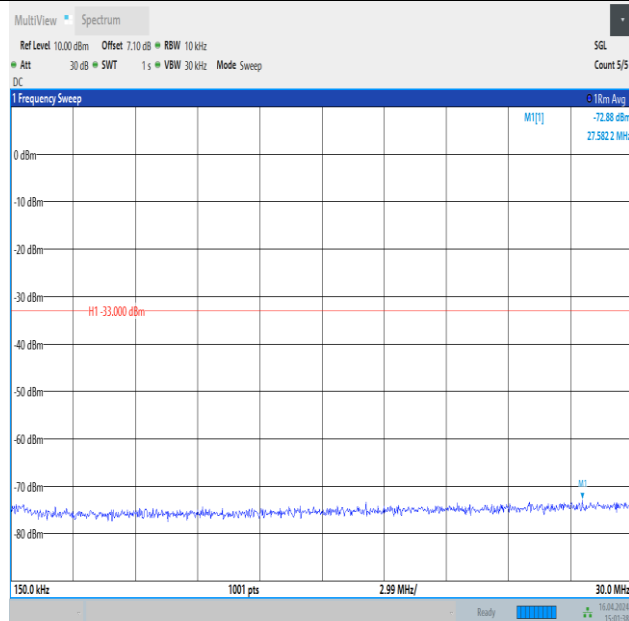
Band4_10MHz_QPSK_20175_1RB#49_0.15~30_0.15~30
