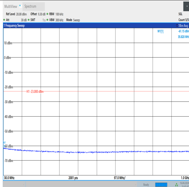
Band4_10MHz_QPSK_20175_1RB#49_30~1000_30~1000
