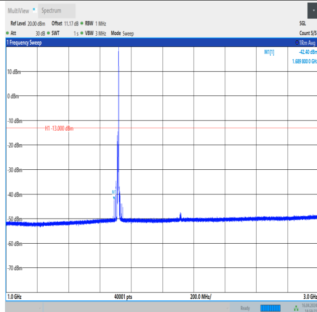
Band4_10MHz_16QAM_20000_1RB#49_1000~3000_1000~3000
