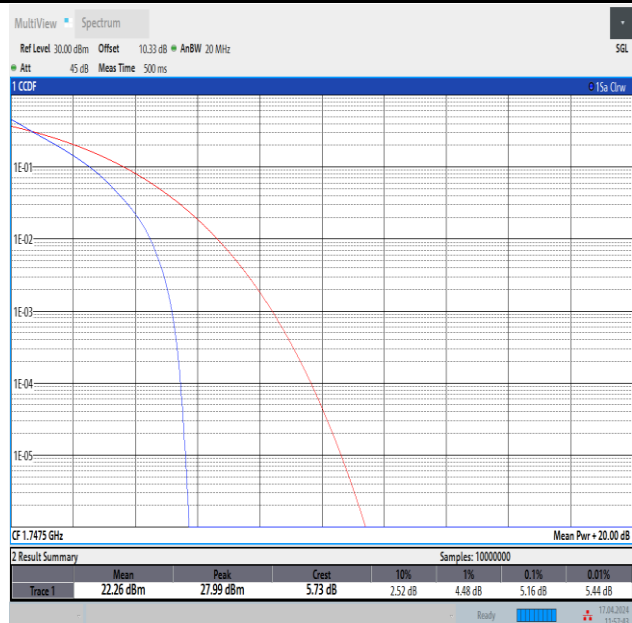
Band4-15MHz-QPSK-20325-75RB#0-PASS
