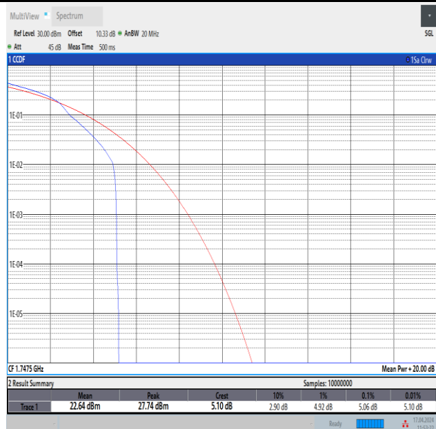
Band4-15MHz-16QAM-20325-1RB#0-PASS
