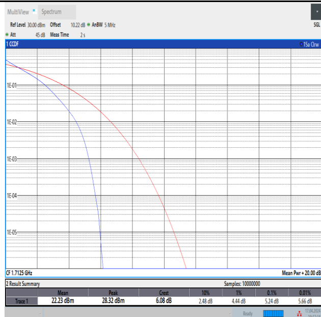
Band4-5MHz-QPSK-19975-25RB#0-PASS
