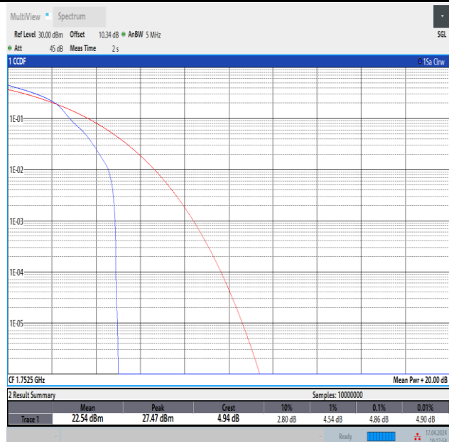
Band4-5MHz-16QAM-20375-1RB#0-PASS
