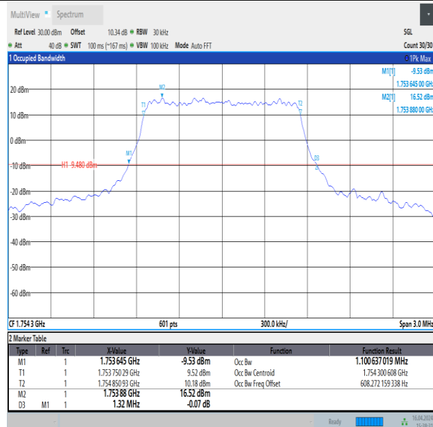
Band4-1.4MHz-16QAM-20393-6RB#0-PASS
