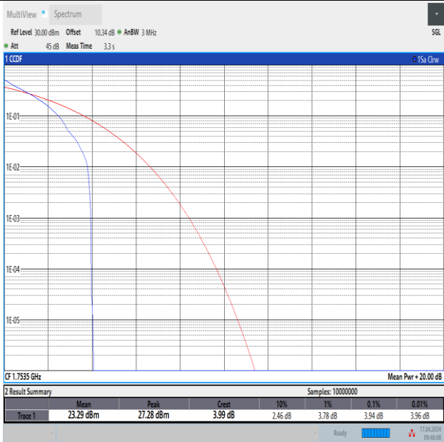
Band4-3MHz-QPSK-20385-1RB#0-PASS
