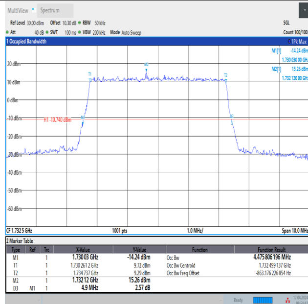
Band4-5MHz-16QAM-20175-25RB#0-PASS
