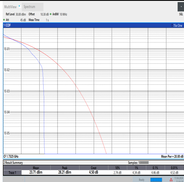
Band4-10MHz-QPSK-20175-1RB#0-PASS
