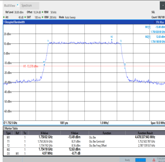
Band4-5MHz-16QAM-20375-25RB#0-PASS
