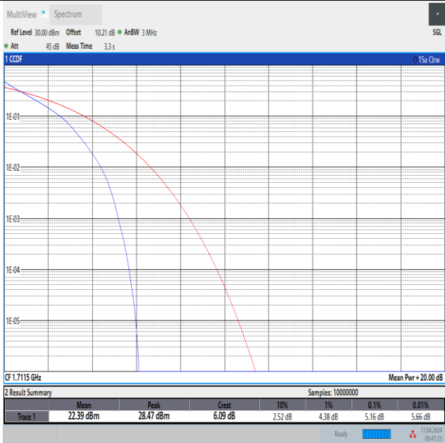
Band4-3MHz-QPSK-19965-15RB#0-PASS
