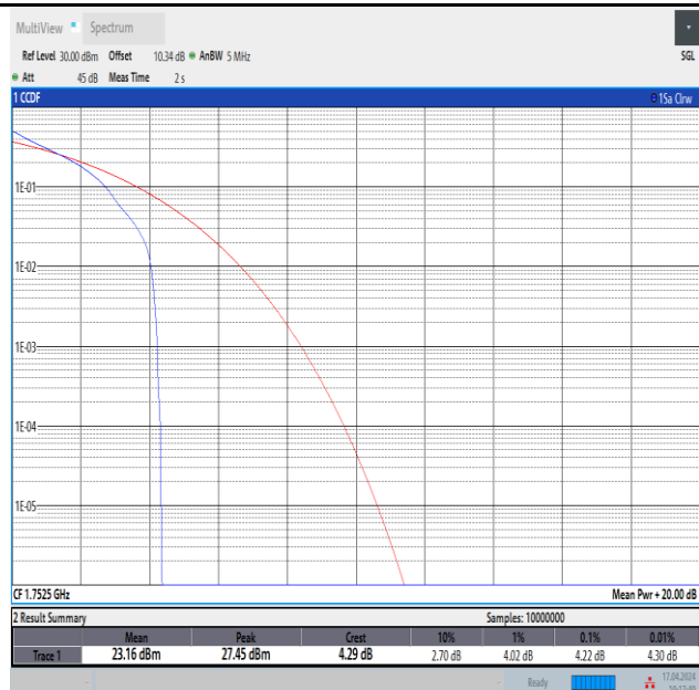
Band4-5MHz-QPSK-20375-1RB#0-PASS
