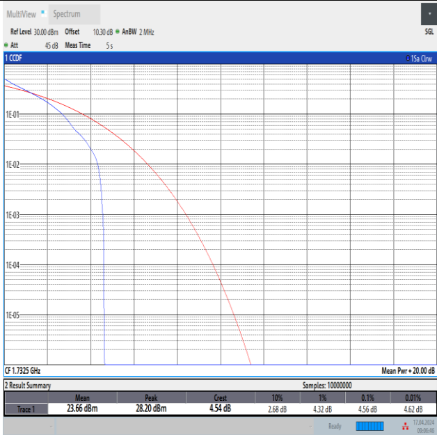
Band4-1.4MHz-QPSK-20175-1RB#0-PASS
