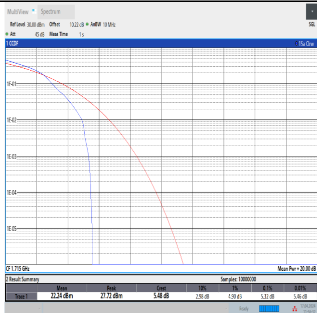
Band4-10MHz-16QAM-20000-1RB#0-PASS
