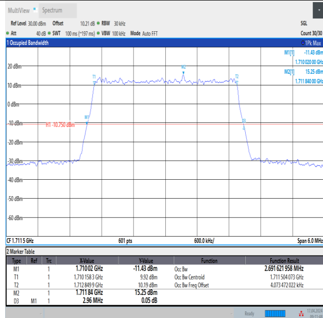
Band4-3MHz-QPSK-19965-15RB#0-PASS
