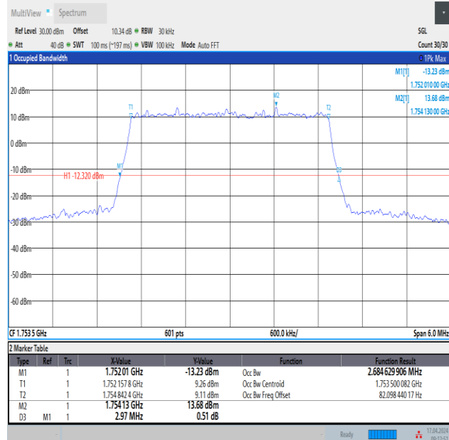
Band4-3MHz-16QAM-20385-15RB#0-PASS
