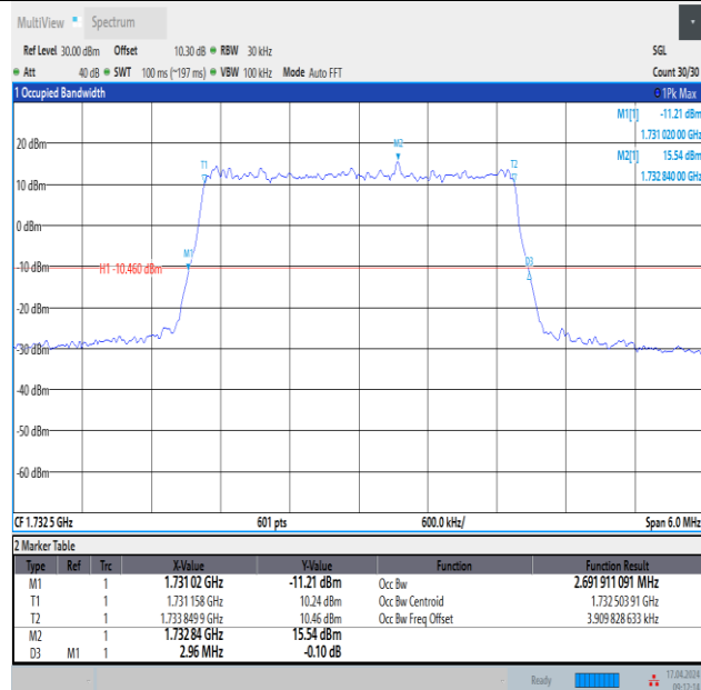
Band4-3MHz-QPSK-20175-15RB#0-PASS
