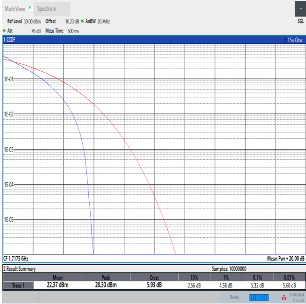
Band4-15MHz-QPSK-20025-75RB#0-PASS
