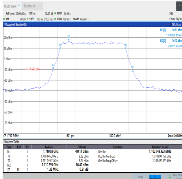
Band4-1.4MHz-16QAM-19957-6RB#0-PASS
