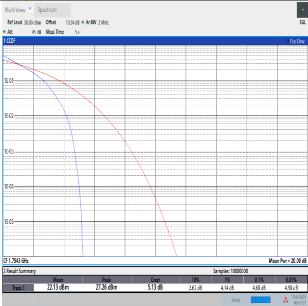
Band4-1.4MHz-QPSK-20393-6RB#0-PASS
