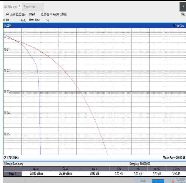
Band4-1.4MHz-QPSK-20393-1RB#0-PASS
