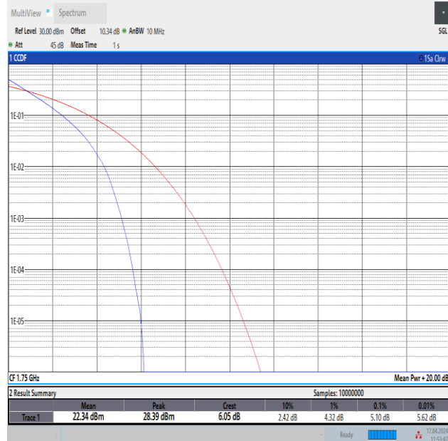
Band4-10MHz-QPSK-20350-50RB#0-PASS
