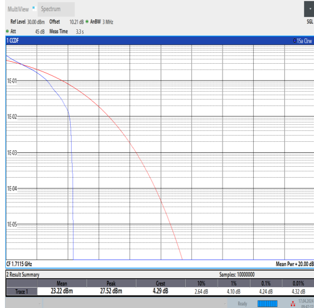
Band4-3MHz-QPSK-19965-1RB#0-PASS
