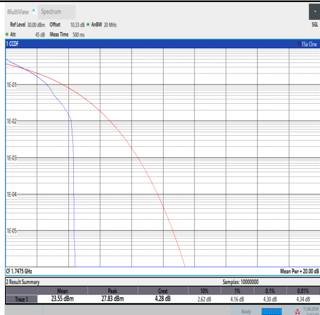
Band4-15MHz-QPSK-20325-1RB#0-PASS
