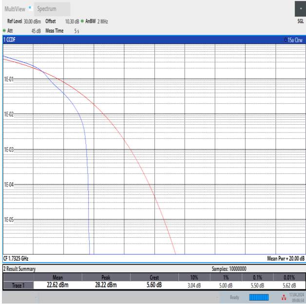
Band4-1.4MHz-16QAM-20175-1RB#0-PASS
