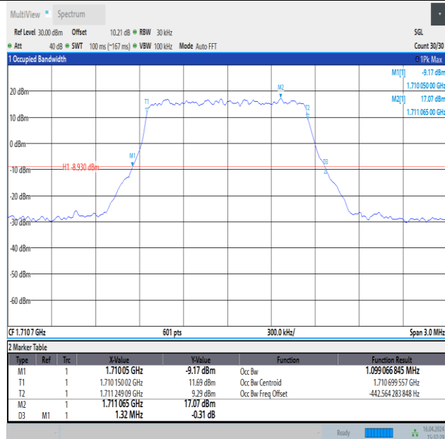
Band4-1.4MHz-QPSK-19957-6RB#0-PASS
