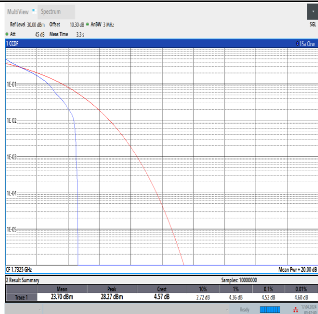
Band4-3MHz-QPSK-20175-1RB#0-PASS
