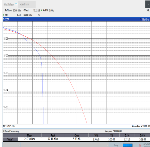
Band4-5MHz-16QAM-19975-1RB#0-PASS
