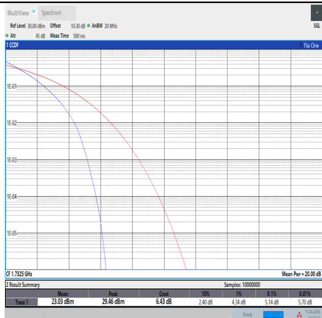
Band4-20MHz-QPSK-20175-100RB#0-PASS
