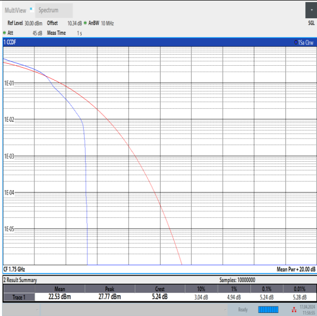
Band4-10MHz-16QAM-20350-1RB#0-PASS
