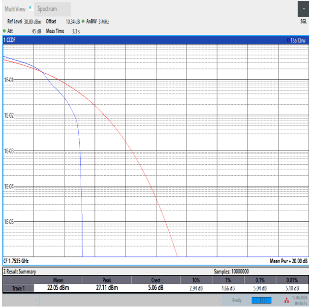
Band4-3MHz-16QAM-20385-1RB#0-PASS
