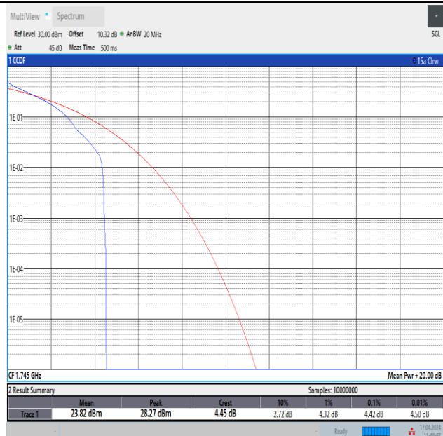
Band4-20MHz-QPSK-20300-1RB#0-PASS
