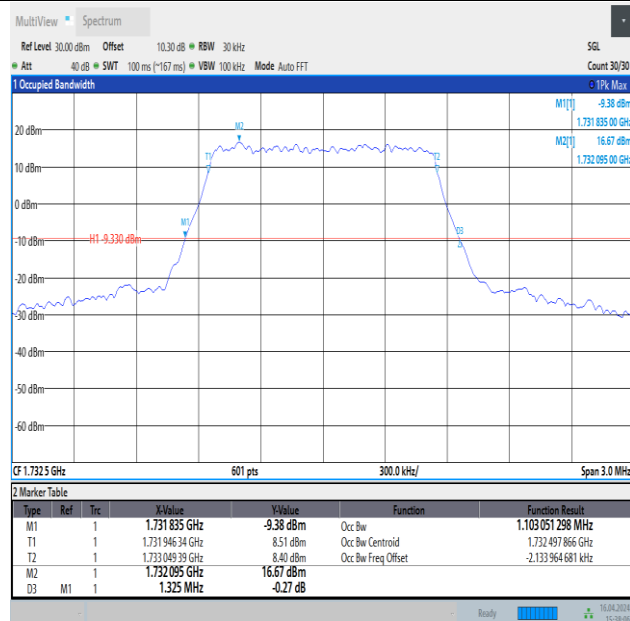
Band4-1.4MHz-16QAM-20175-6RB#0-PASS
