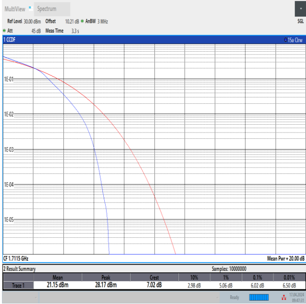
Band4-3MHz-16QAM-19965-15RB#0-PASS
