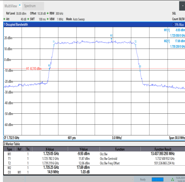
Band4-15MHz-QPSK-20175-75RB#0-PASS
