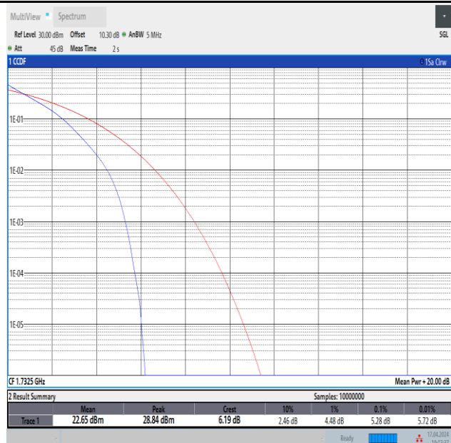
Band4-5MHz-QPSK-20175-25RB#0-PASS
