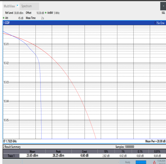
Band4-5MHz-QPSK-20175-1RB#0-PASS
