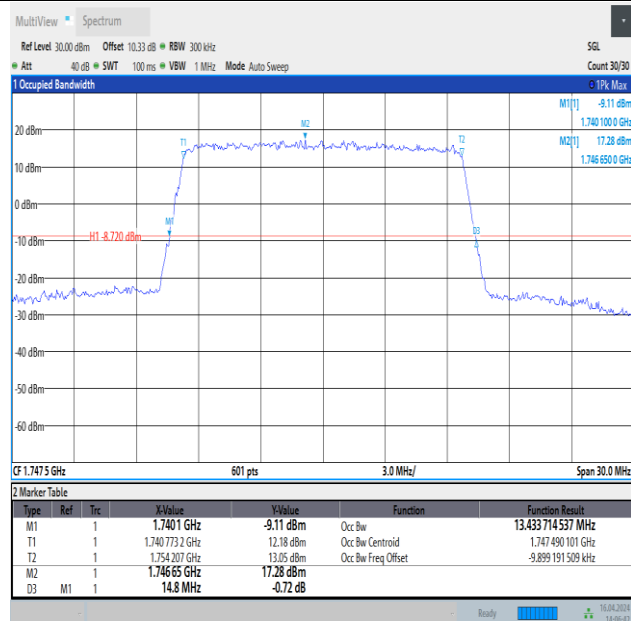
Band4-15MHz-QPSK-20325-75RB#0-PASS
