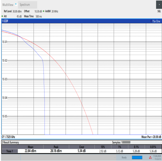
Band4-15MHz-16QAM-20175-1RB#0-PASS
