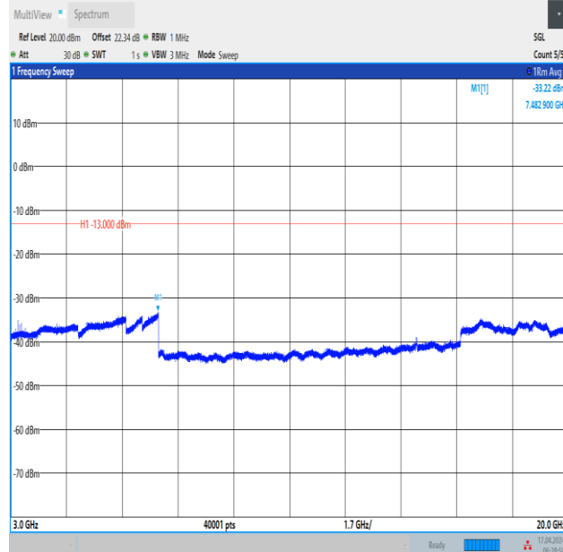
Band2_5MHz_16QAM_18625_25RB#0_3000~20000_3000~20000
