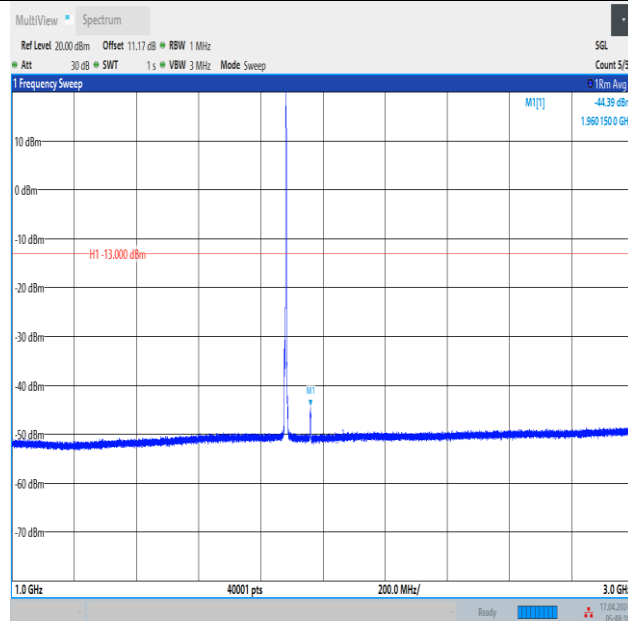
Band2_3MHz_16QAM_18900_1RB#14_1000~3000_1000~3000
