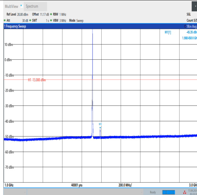
Band2_3MHz_16QAM_19185_1RB#14_1000~3000_1000~3000
