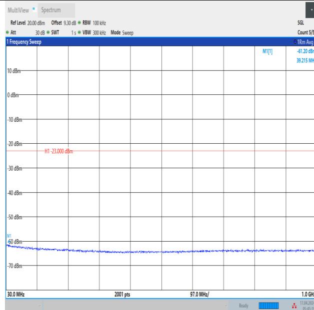
Band2_3MHz_QPSK_18900_1RB#0_30~1000_30~1000
