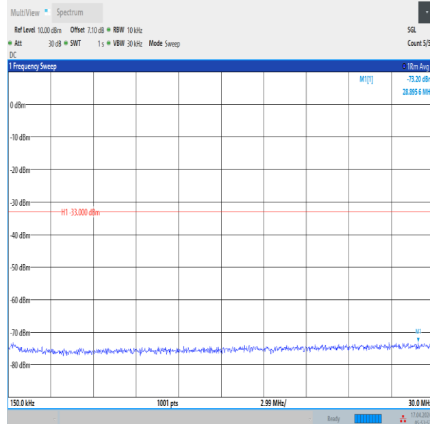
Band2_3MHz_QPSK_19185_15RB#0_0.15~30_0.15~30
