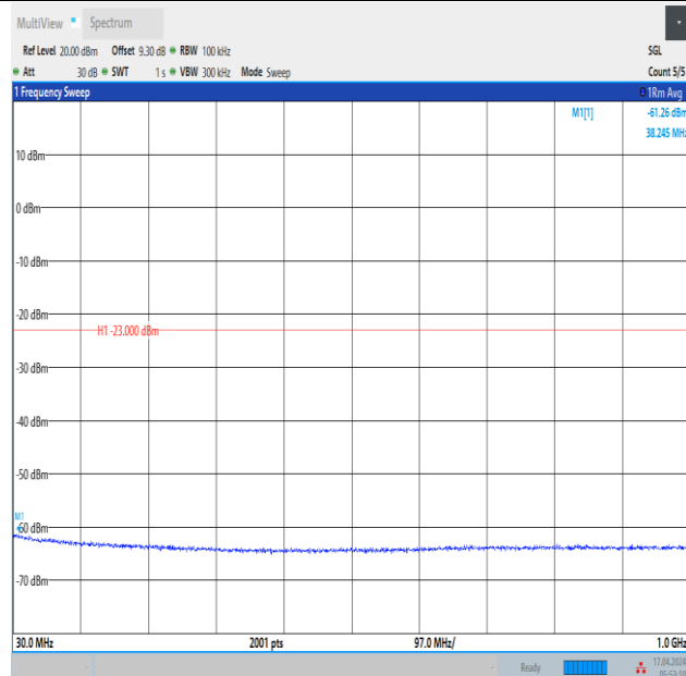
Band2_3MHz_16QAM_19185_1RB#14_30~1000_30~1000
