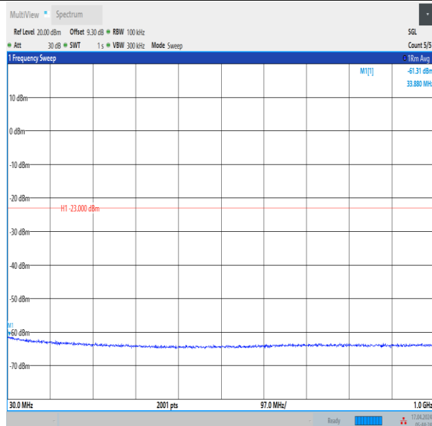
Band2_3MHz_16QAM_18615_15RB#0_30~1000_30~1000
