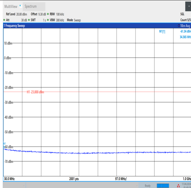
Band2_3MHz_16QAM_18900_15RB#0_30~1000_30~1000
