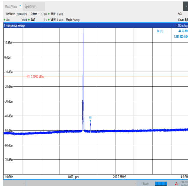
Band2_5MHz_QPSK_18625_1RB#24_1000~3000_1000~3000
