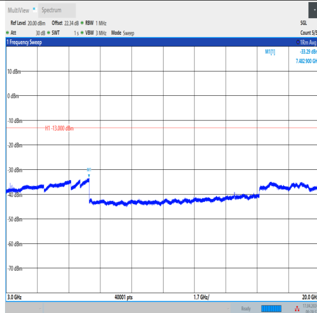
Band2_5MHz_QPSK_18625_1RB#0_3000~20000_3000~20000
