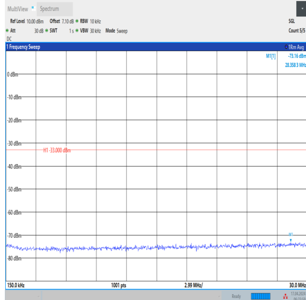
Band2_5MHz_QPSK_18625_1RB#0_0.15~30_0.15~30
