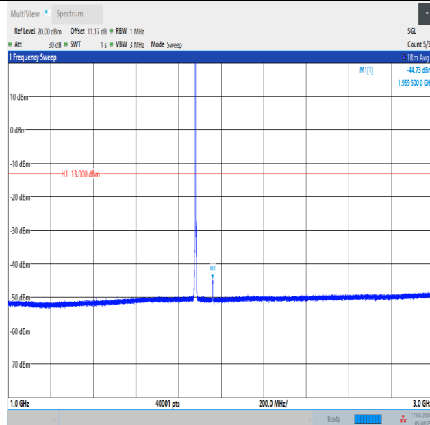
Band2_3MHz_16QAM_18900_1RB#0_1000~3000_1000~3000
