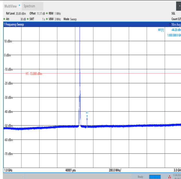
Band2_5MHz_QPSK_18625_1RB#0_1000~3000_1000~3000
