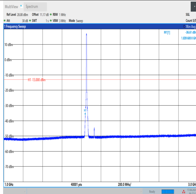
Band2_5MHz_QPSK_18625_25RB#0_1000~3000_1000~3000
