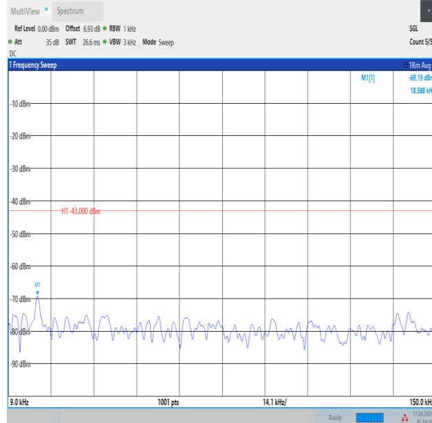
Band2_3MHz_16QAM_19185_15RB#0_0.009~0.15_0.009~0.15
