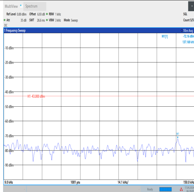
Band2_5MHz_QPSK_18900_1RB#0_0.009~0.15_0.009~0.15
