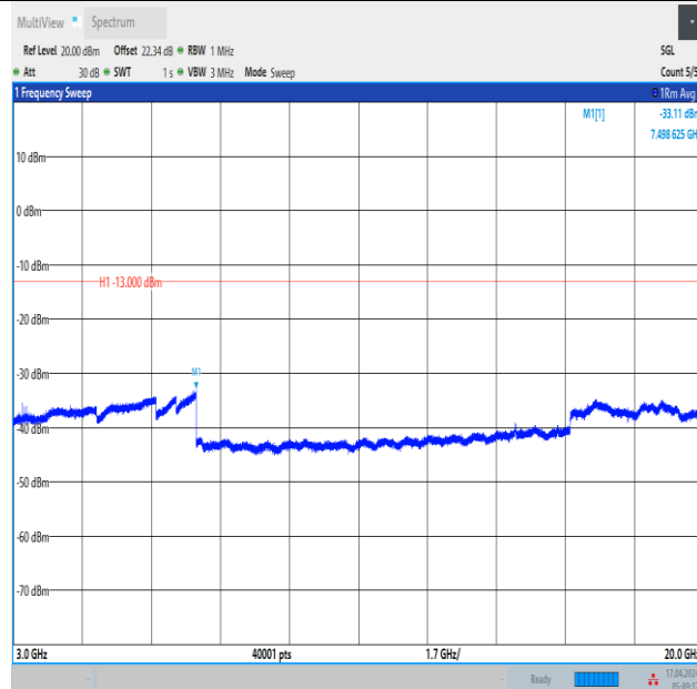
Band2_3MHz_QPSK_18900_15RB#0_3000~20000_3000~20000
