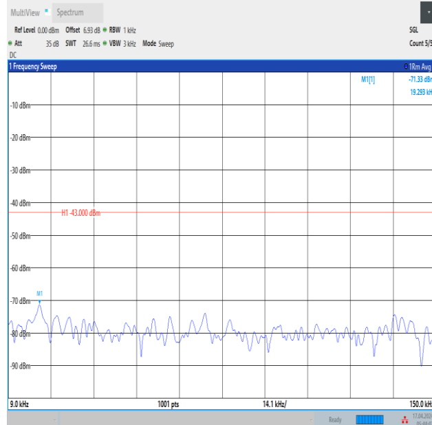
Band2_3MHz_16QAM_18615_15RB#0_0.009~0.15_0.009~0.15
