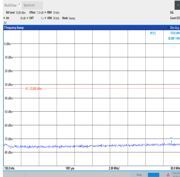
Band2_5MHz_QPSK_18900_1RB#0_0.15~30_0.15~30
