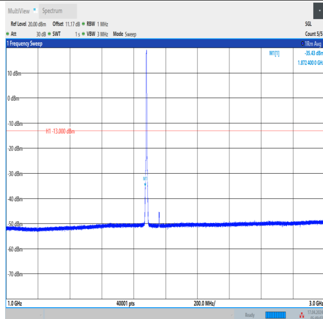
Band2_3MHz_QPSK_18900_15RB#0_1000~3000_1000~3000
