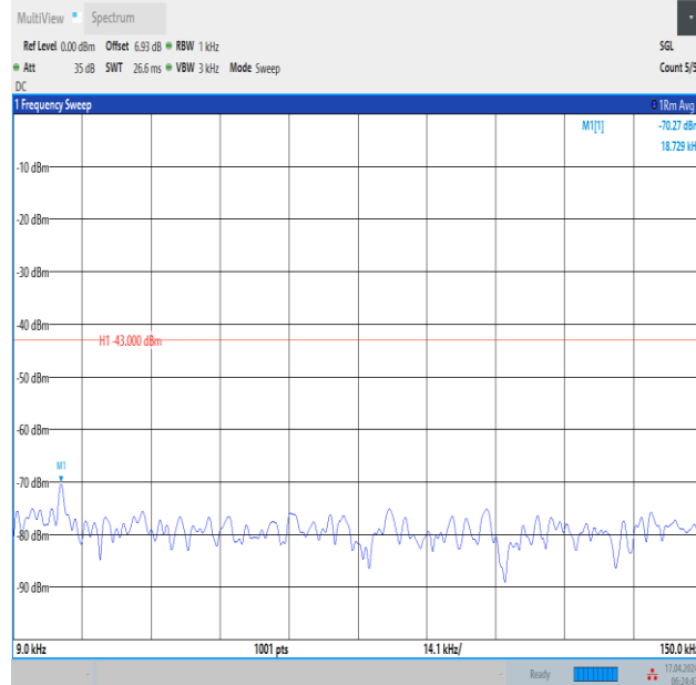
Band2_5MHz_16QAM_18625_1RB#0_0.009~0.15_0.009~0.15
