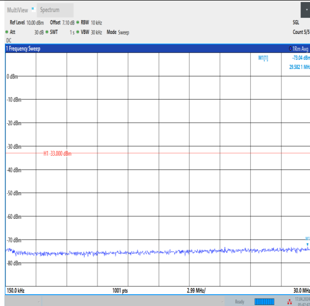
Band2_3MHz_16QAM_18900_1RB#14_0.15~30_0.15~30
