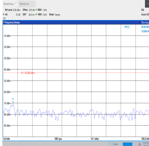
Band2_3MHz_16QAM_19185_1RB#0_0.009~0.15_0.009~0.15
