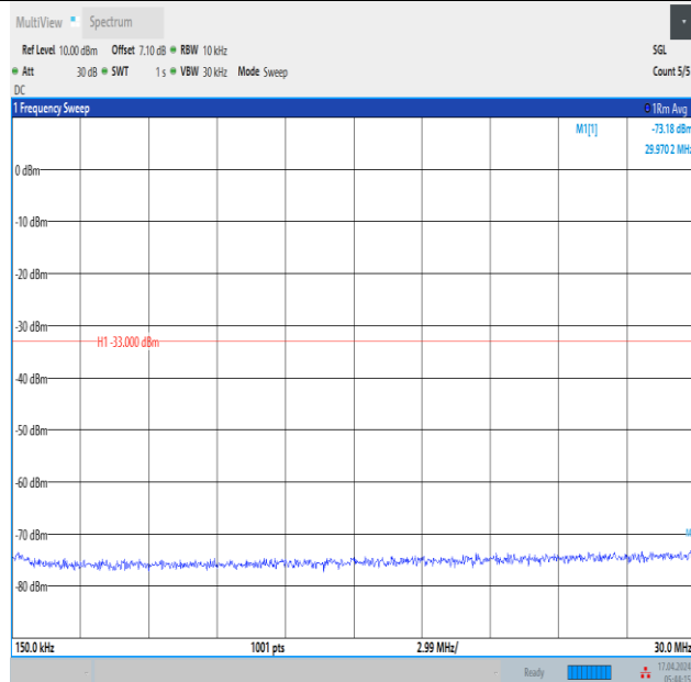
Band2_3MHz_16QAM_18615_15RB#0_0.15~30_0.15~30
