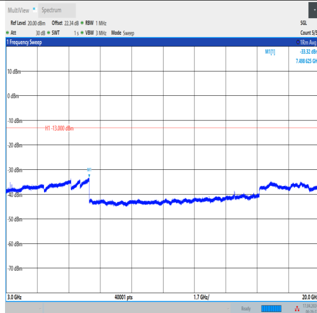
Band2_5MHz_QPSK_18625_1RB#24_3000~20000_3000~20000
