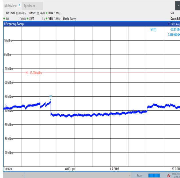
Band2_5MHz_QPSK_18625_25RB#0_3000~20000_3000~20000
