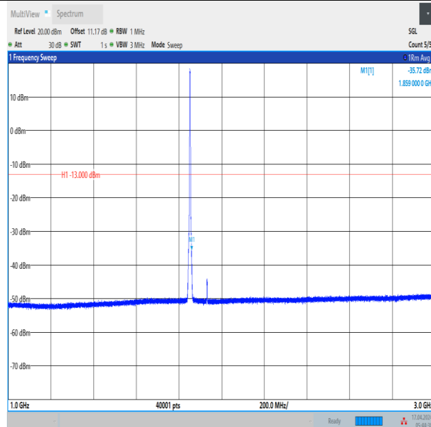
Band2_3MHz_16QAM_18615_15RB#0_1000~3000_1000~3000
