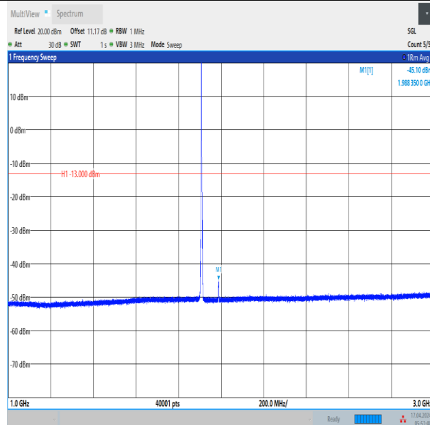
Band2_3MHz_16QAM_19185_1RB#0_1000~3000_1000~3000
