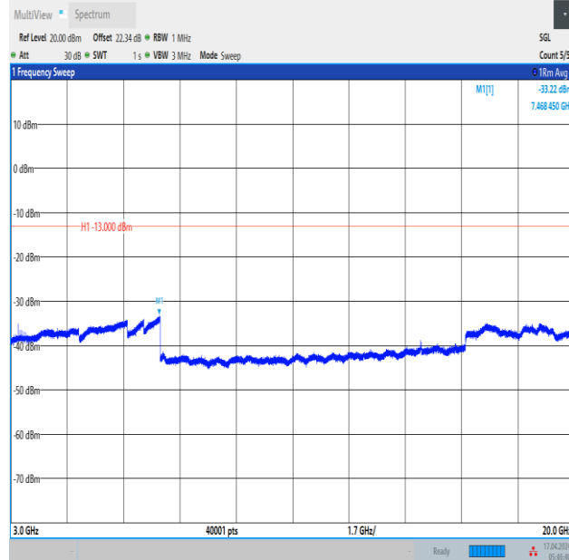
Band2_3MHz_16QAM_18900_1RB#0_3000~20000_3000~20000
