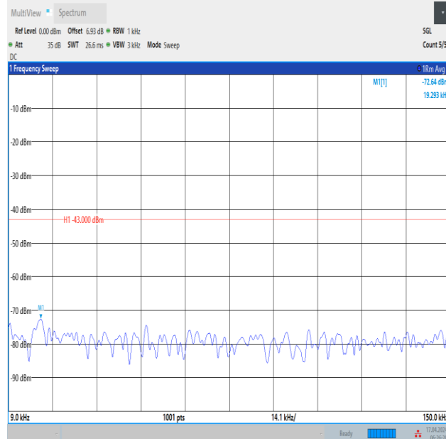
Band2_5MHz_16QAM_18625_1RB#24_0.009~0.15_0.009~0.15
