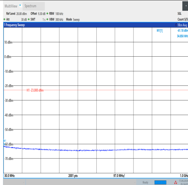
Band2_3MHz_QPSK_19185_15RB#0_30~1000_30~1000
