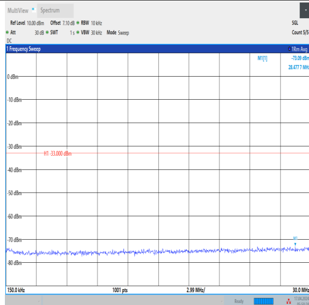
Band2_3MHz_QPSK_19185_1RB#0_0.15~30_0.15~30
