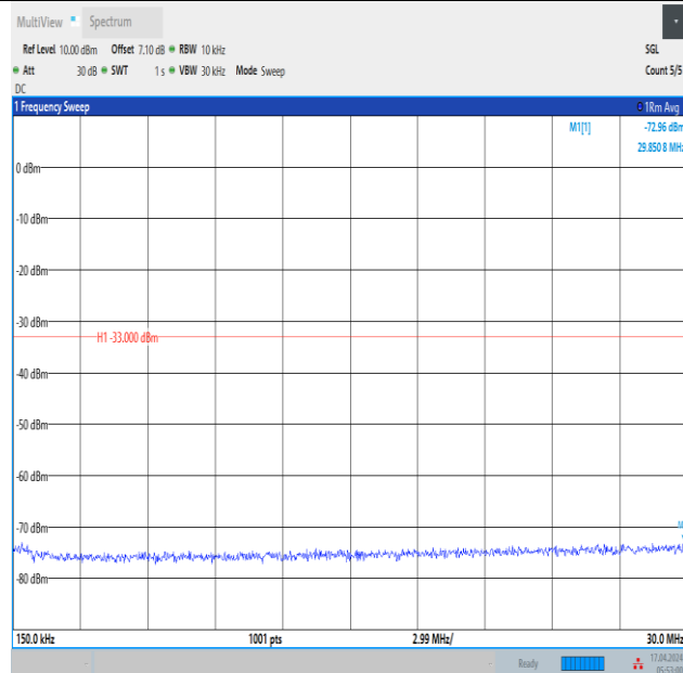
Band2_3MHz_16QAM_19185_1RB#14_0.15~30_0.15~30
