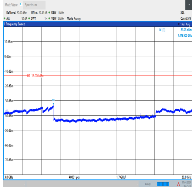
Band2_5MHz_16QAM_18625_1RB#0_3000~20000_3000~20000
