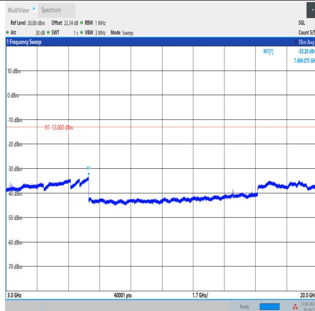
Band2_3MHz_QPSK_19185_15RB#0_3000~20000_3000~20000
