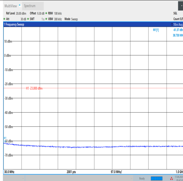
Band2_3MHz_QPSK_18900_1RB#14_30~1000_30~1000
