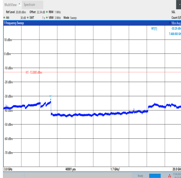
Band2_3MHz_16QAM_19185_1RB#14_3000~20000_3000~20000
