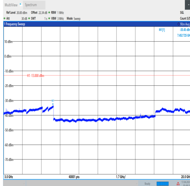
Band2_3MHz_16QAM_18900_1RB#14_3000~20000_3000~20000
