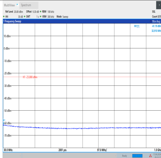
Band2_3MHz_QPSK_19185_1RB#14_30~1000_30~1000
