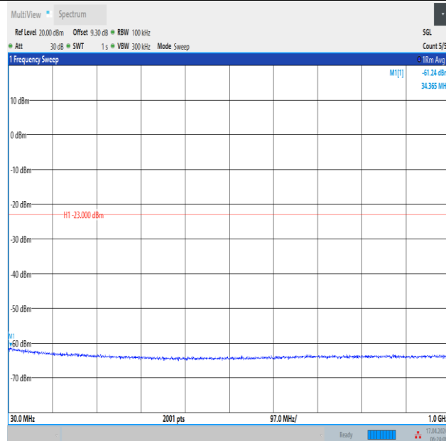
Band2_5MHz_QPSK_18625_1RB#0_30~1000_30~1000
