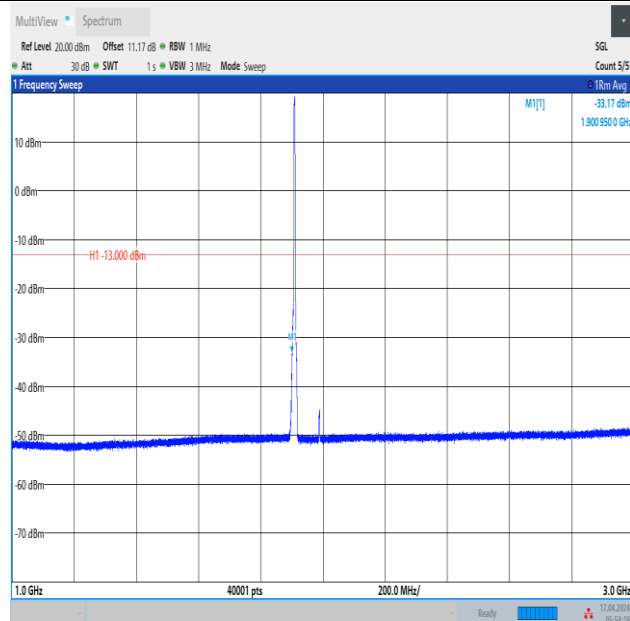
Band2_3MHz_QPSK_19185_15RB#0_1000~3000_1000~3000
