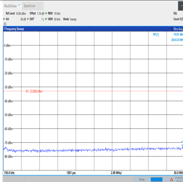
Band2_3MHz_16QAM_19185_1RB#0_0.15~30_0.15~30
