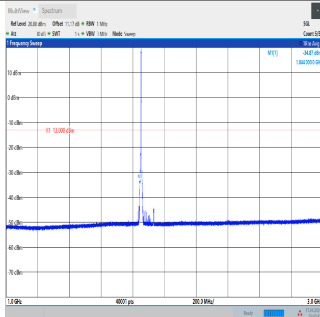
Band2_3MHz_QPSK_18615_15RB#0_1000~3000_1000~3000
