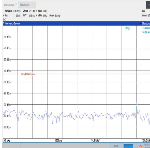
Band2_3MHz_QPSK_19185_15RB#0_0.009~0.15_0.009~0.15
