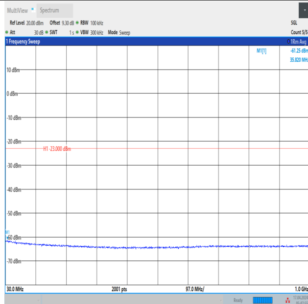
Band2_3MHz_16QAM_18900_1RB#14_30~1000_30~1000
