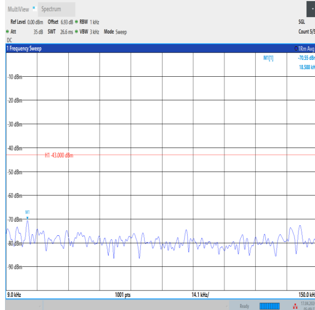
Band2_3MHz_16QAM_18900_15RB#0_0.009~0.15_0.009~0.15
