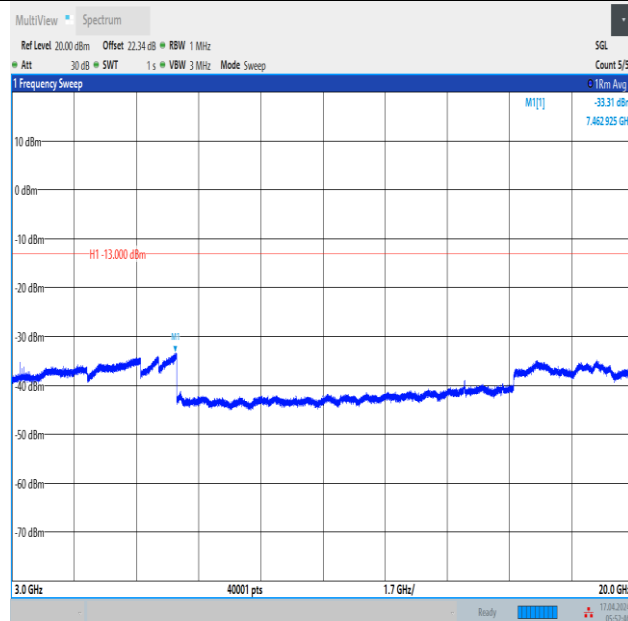
Band2_3MHz_QPSK_19185_1RB#14_3000~20000_3000~20000
