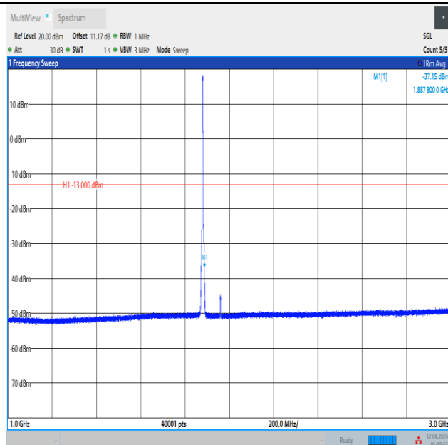
Band2_3MHz_16QAM_18900_15RB#0_1000~3000_1000~3000
