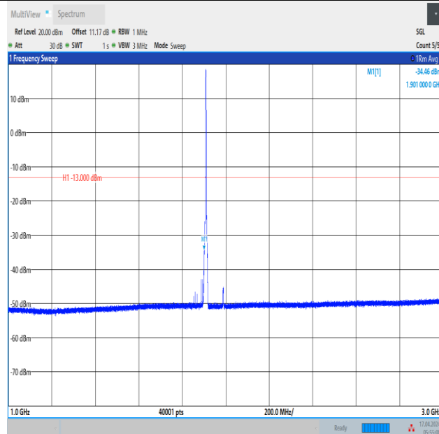
Band2_3MHz_16QAM_19185_15RB#0_1000~3000_1000~3000
