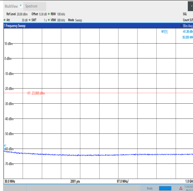
Band2_5MHz_QPSK_18625_1RB#24_30~1000_30~1000
