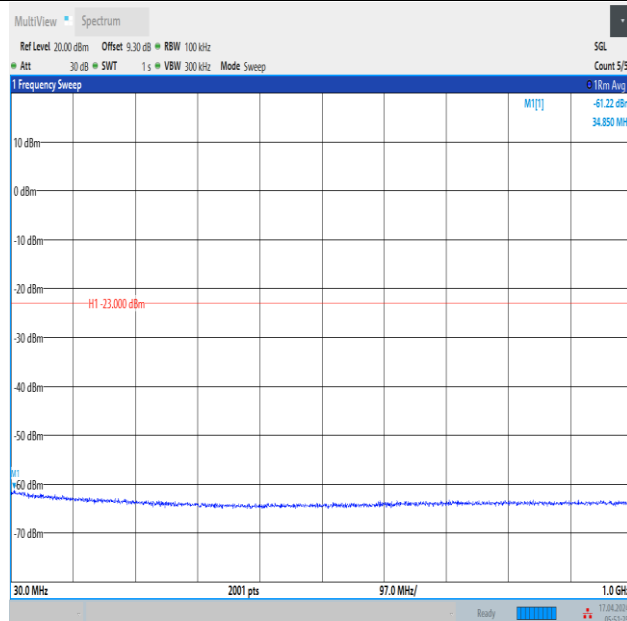
Band2_3MHz_16QAM_19185_1RB#0_30~1000_30~1000
