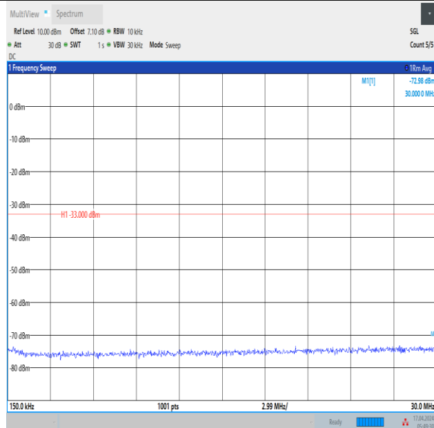
Band2_3MHz_16QAM_18900_15RB#0_0.15~30_0.15~30
