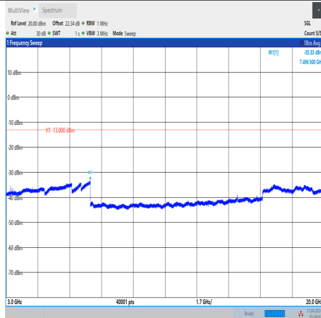
Band2_3MHz_QPSK_18615_15RB#0_3000~20000_3000~20000
