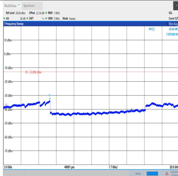
Band2_3MHz_QPSK_18900_1RB#0_3000~20000_3000~20000
