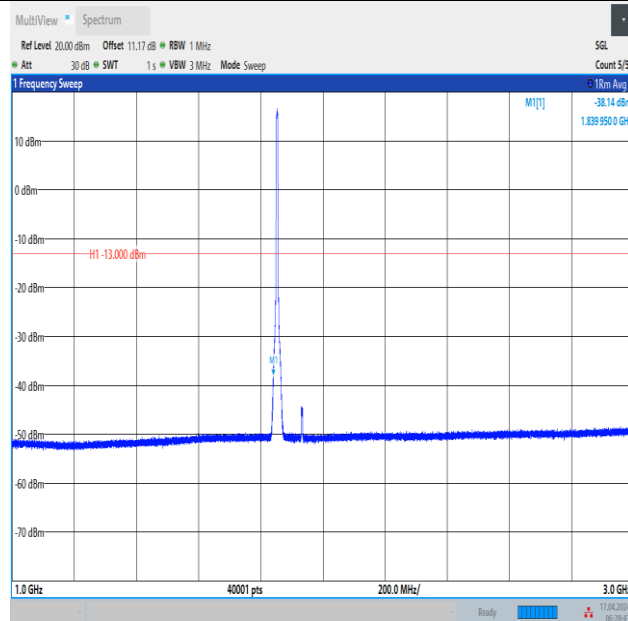
Band2_5MHz_16QAM_18625_25RB#0_1000~3000_1000~3000
