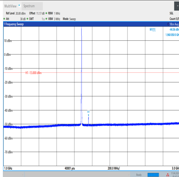
Band2_3MHz_QPSK_18900_1RB#14_1000~3000_1000~3000
