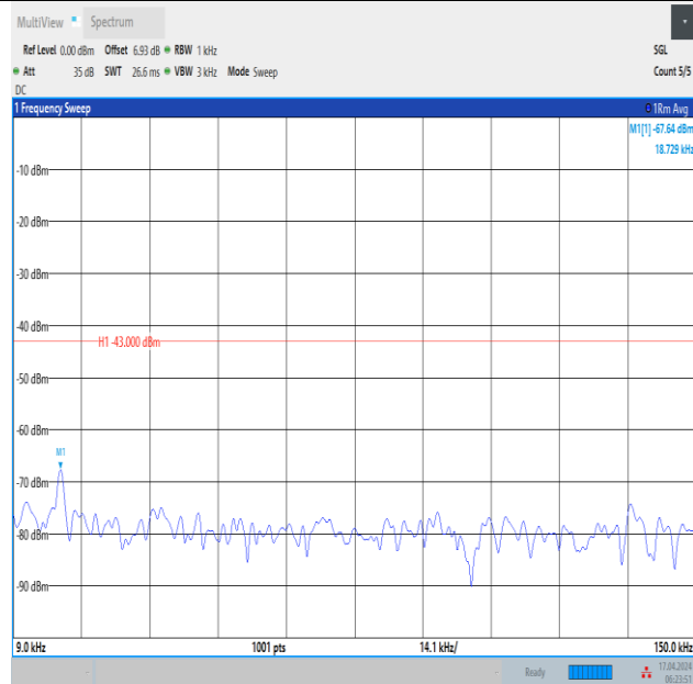
Band2_5MHz_QPSK_18625_1RB#0_0.009~0.15_0.009~0.15
