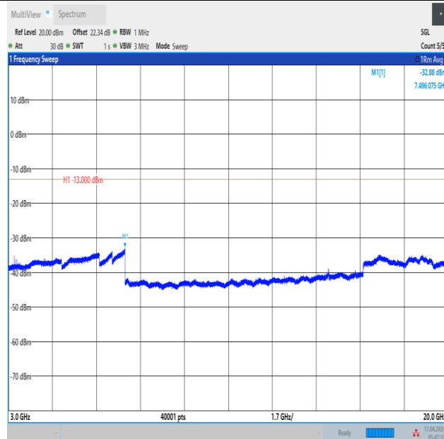
Band2_3MHz_QPSK_18900_1RB#14_3000~20000_3000~20000
