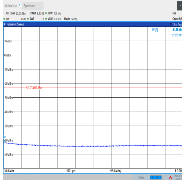
Band2_5MHz_QPSK_18625_25RB#0_30~1000_30~1000
