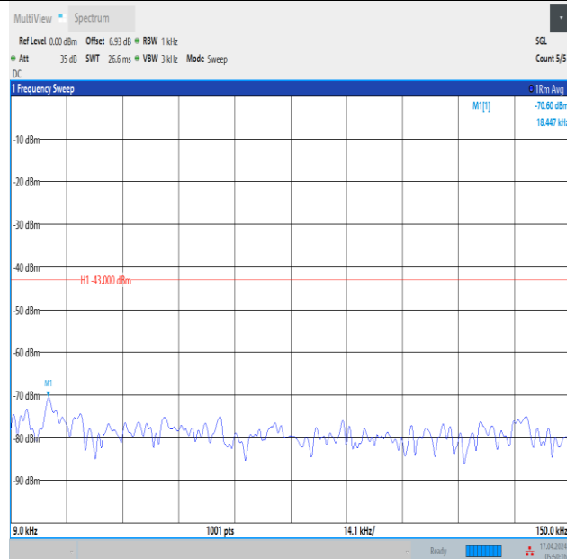
Band2_3MHz_QPSK_19185_1RB#0_0.009~0.15_0.009~0.15
