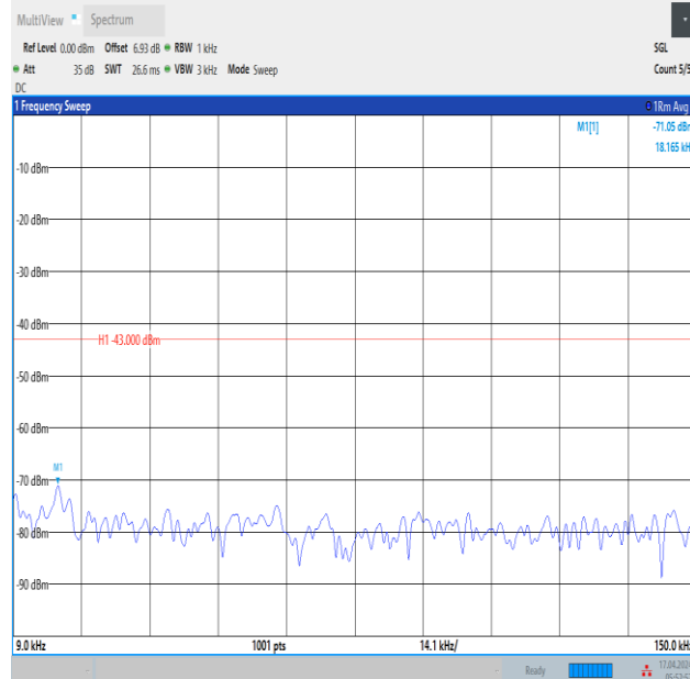
Band2_3MHz_16QAM_19185_1RB#14_0.009~0.15_0.009~0.15
