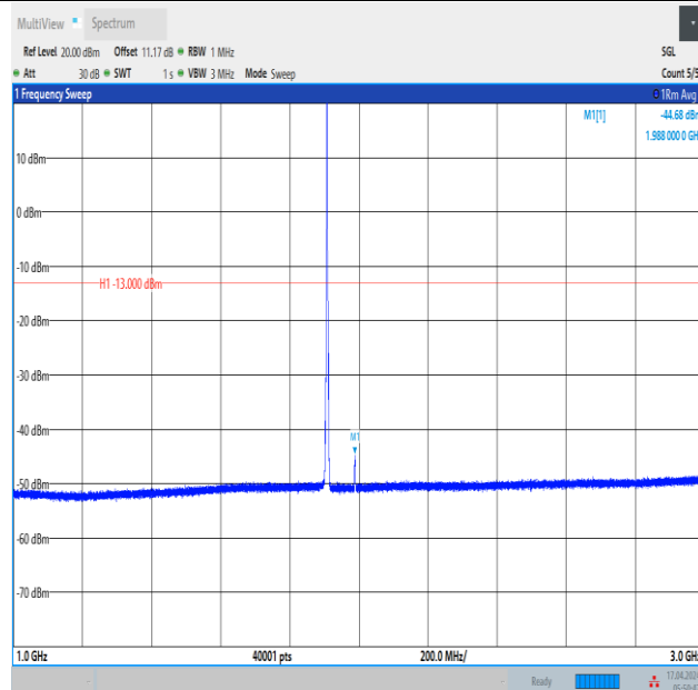
Band2_3MHz_QPSK_19185_1RB#0_1000~3000_1000~3000
