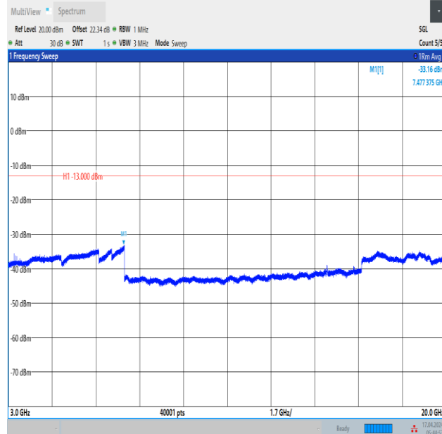
Band2_3MHz_16QAM_18615_15RB#0_3000~20000_3000~20000
