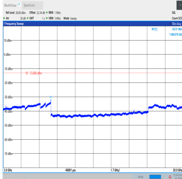
Band2_3MHz_16QAM_18900_15RB#0_3000~20000_3000~20000
