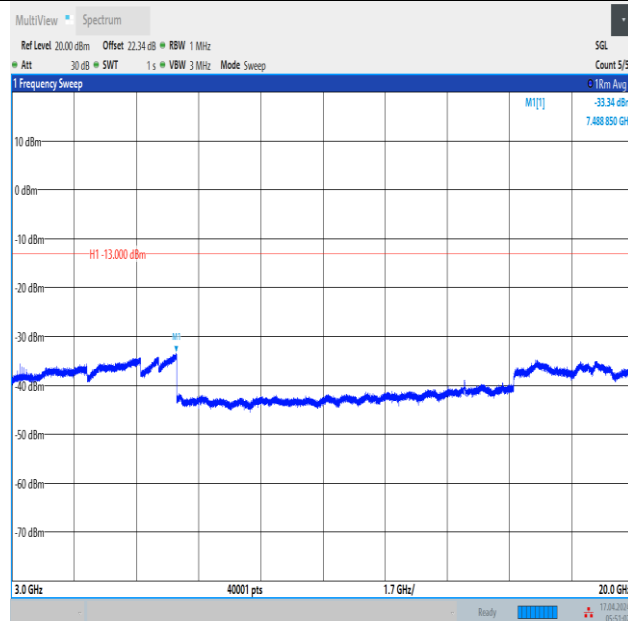
Band2_3MHz_QPSK_19185_1RB#0_3000~20000_3000~20000
