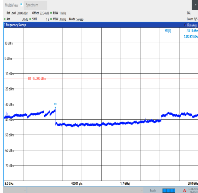
Band2_3MHz_16QAM_19185_1RB#0_3000~20000_3000~20000
