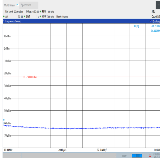
Band2_3MHz_QPSK_18615_15RB#0_30~1000_30~1000
