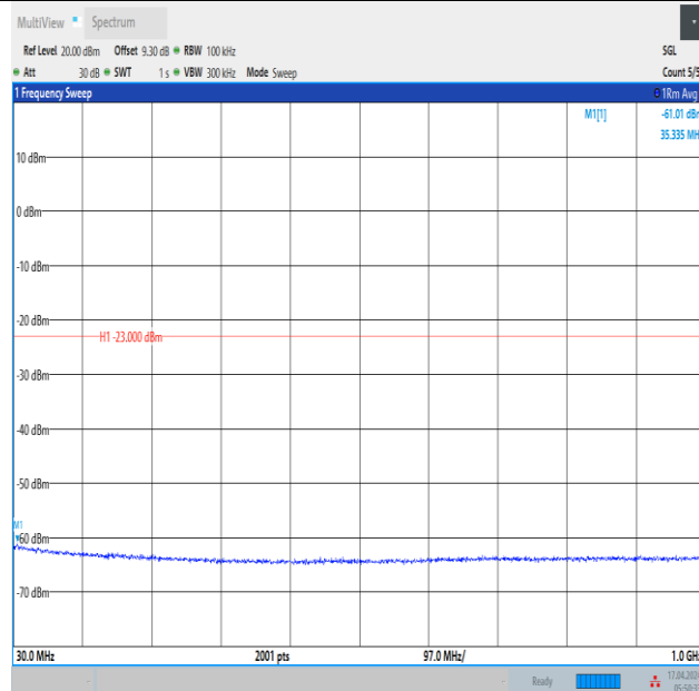
Band2_3MHz_QPSK_19185_1RB#0_30~1000_30~1000
