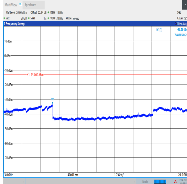
Band2_3MHz_16QAM_19185_15RB#0_3000~20000_3000~20000
