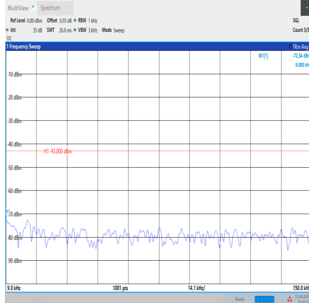
Band2_3MHz_16QAM_18900_1RB#0_0.009~0.15_0.009~0.15
