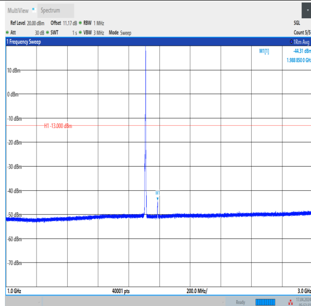
Band2_3MHz_QPSK_19185_1RB#14_1000~3000_1000~3000
