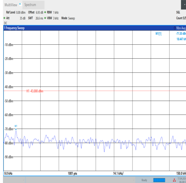
Band2_5MHz_16QAM_18625_25RB#0_0.009~0.15_0.009~0.15
