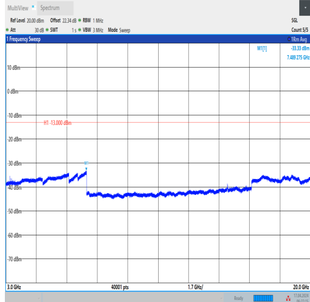
Band2_5MHz_16QAM_18625_1RB#24_3000~20000_3000~20000
