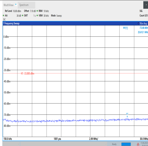
Band2_3MHz_QPSK_18900_1RB#0_0.15~30_0.15~30
