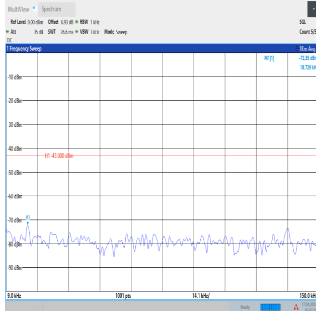
Band2_3MHz_16QAM_18900_1RB#14_0.009~0.15_0.009~0.15
