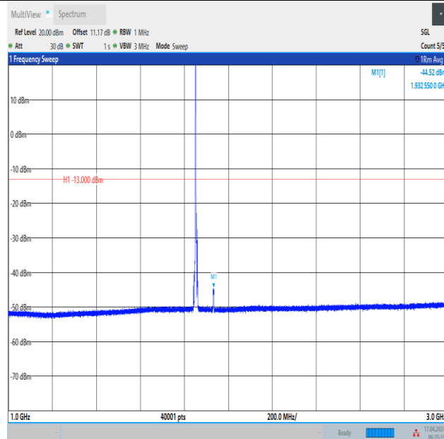
Band2_5MHz_16QAM_18625_1RB#0_1000~3000_1000~3000
