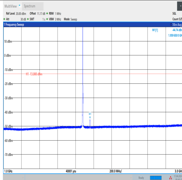
Band2_3MHz_QPSK_18900_1RB#0_1000~3000_1000~3000
