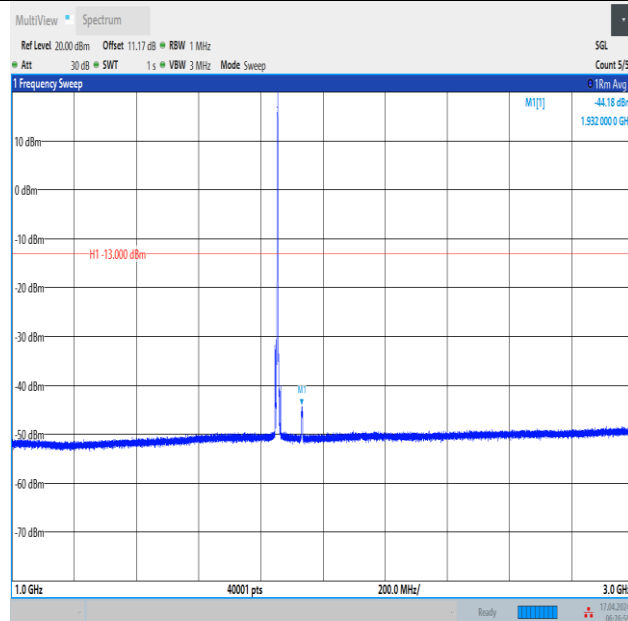
Band2_5MHz_16QAM_18625_1RB#24_1000~3000_1000~3000
