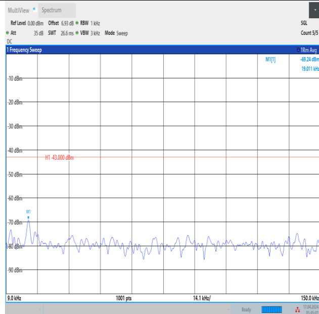
Band2_3MHz_QPSK_18900_1RB#0_0.009~0.15_0.009~0.15
