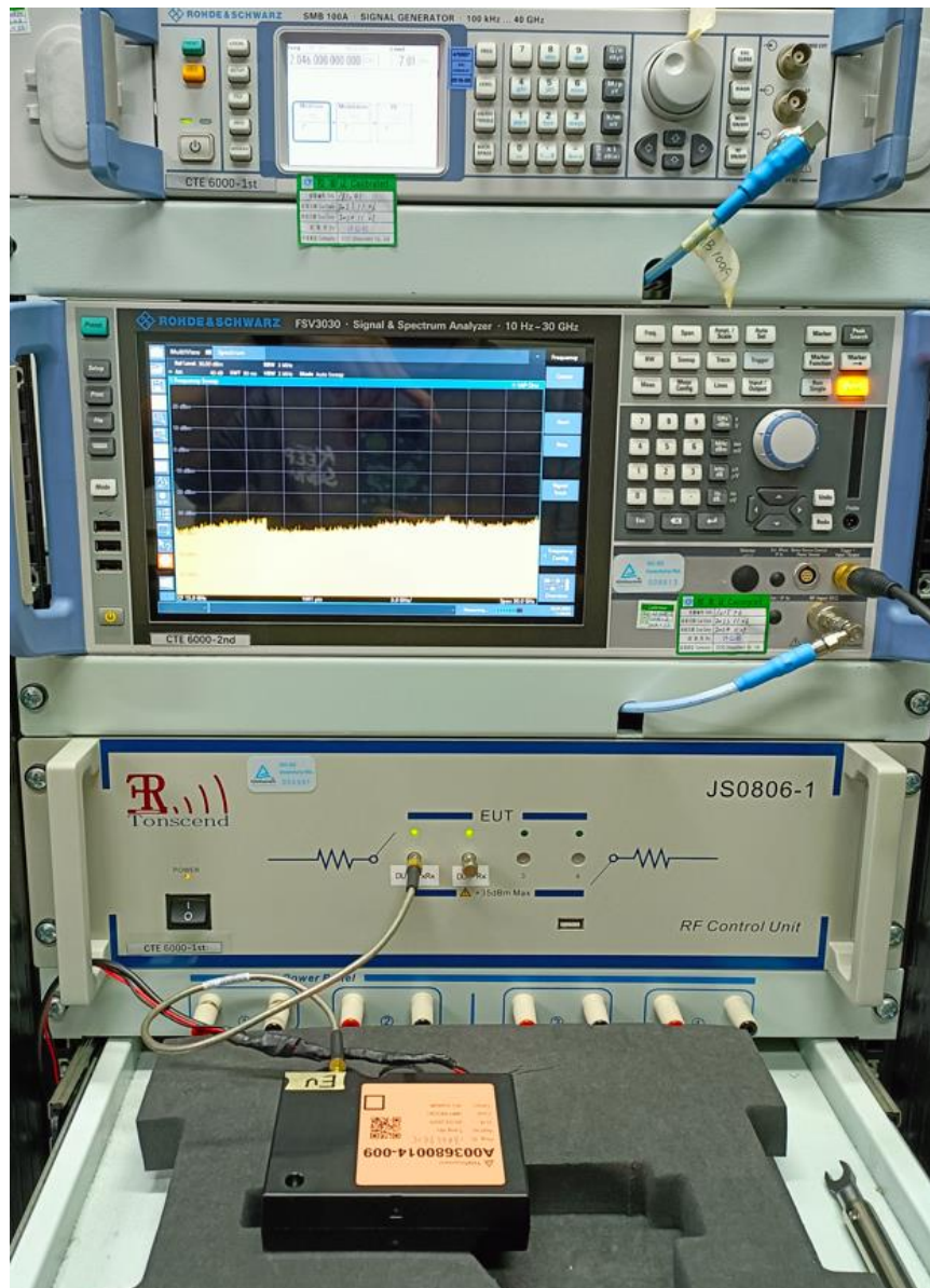
Photograph 3: Set-up photo for Conducted Measurement
