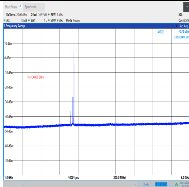
Band66_20MHz_16QAM_132322_1RB#99_1000~3000_1000~3000
