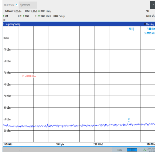
Band66_15MHz_QPSK_132047_75RB#0_0.15~30_0.15~30
