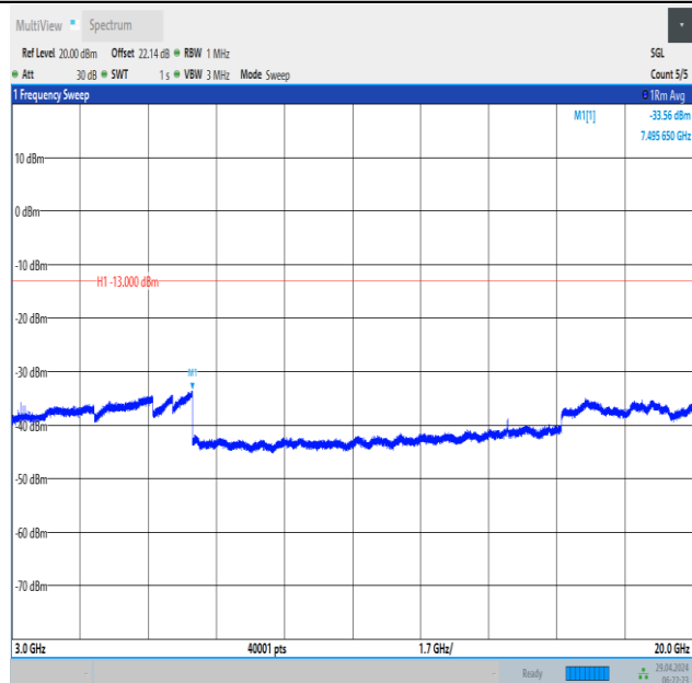
Band66_15MHz_QPSK_132047_75RB#0_3000~20000_3000~20000
