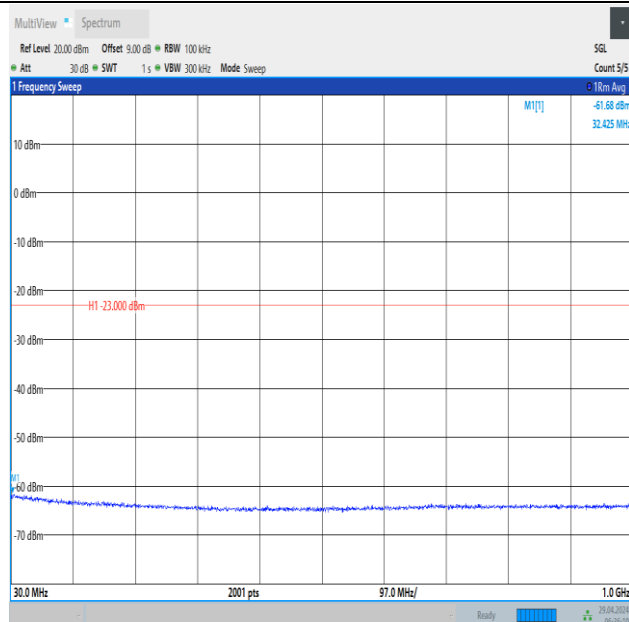
Band66_20MHz_QPSK_132572_100RB#0_30~1000_30~1000
