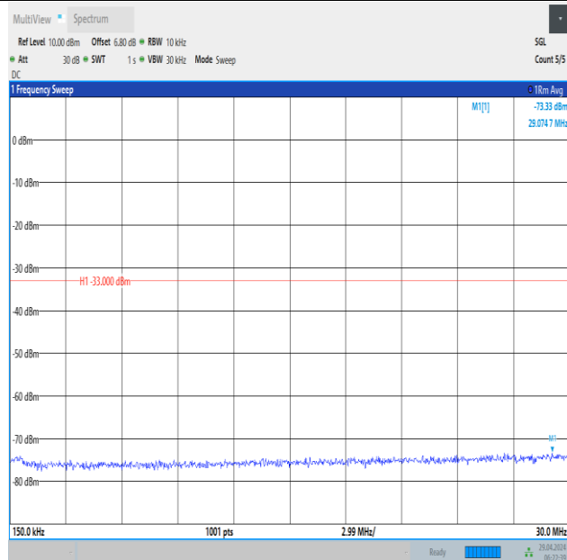
Band66_15MHz_QPSK_132322_75RB#0_0.15~30_0.15~30
