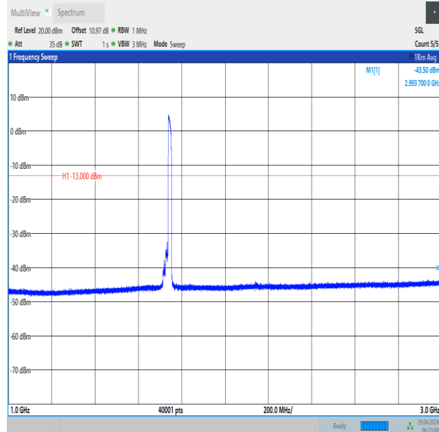
Band66_15MHz_QPSK_132322_75RB#0_1000~3000_1000~3000
