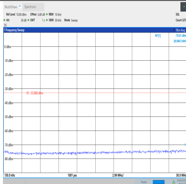
Band66_20MHz_16QAM_132572_1RB#99_0.15~30_0.15~30
