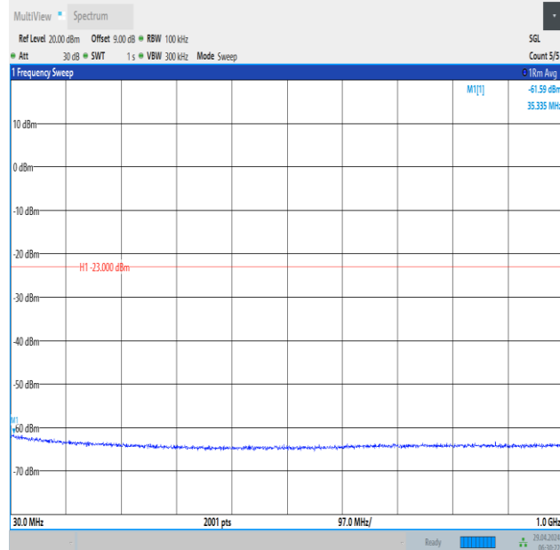
Band66_20MHz_16QAM_132322_1RB#99_30~1000_30~1000
