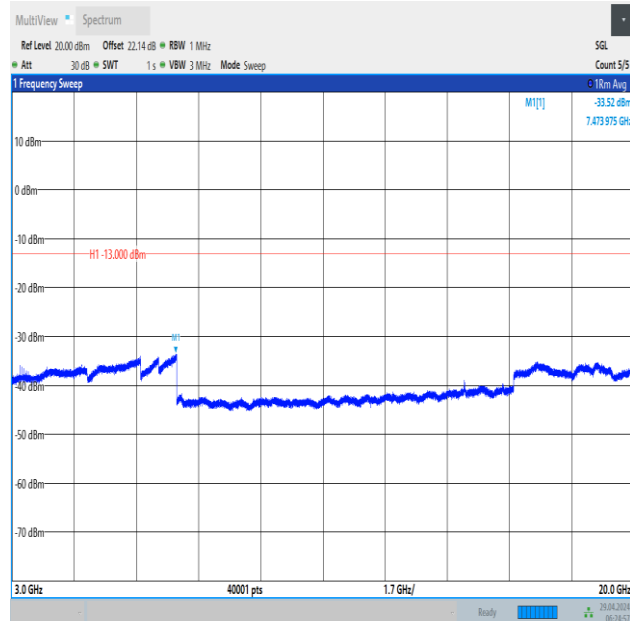
Band66_20MHz_QPSK_132072_1RB#0_3000~20000_3000~20000
