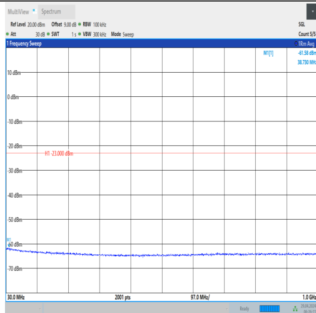
Band66_20MHz_QPSK_132072_1RB#99_30~1000_30~1000
