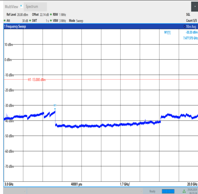
Band66_20MHz_QPSK_132322_100RB#0_3000~20000_3000~20000
