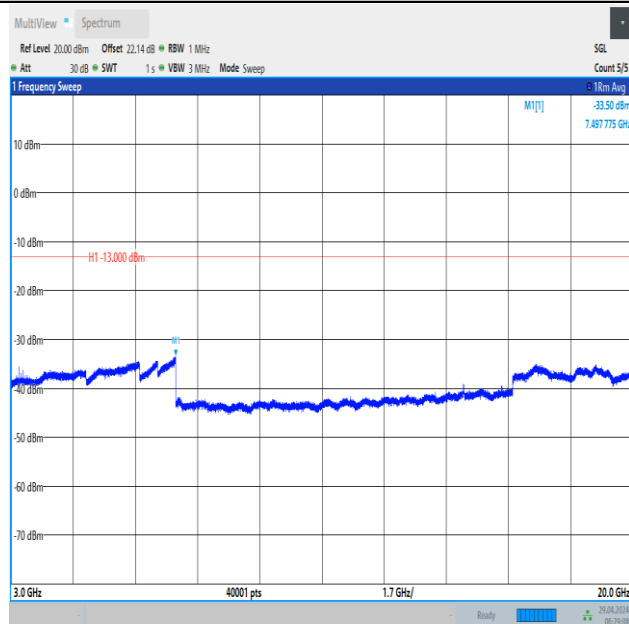
Band66_20MHz_16QAM_132322_1RB#0_3000~20000_3000~20000
