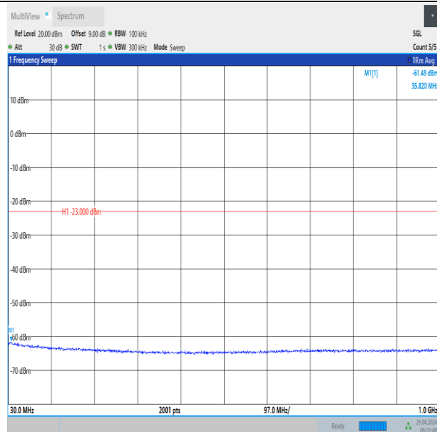
Band66_15MHz_QPSK_132322_75RB#0_30~1000_30~1000
