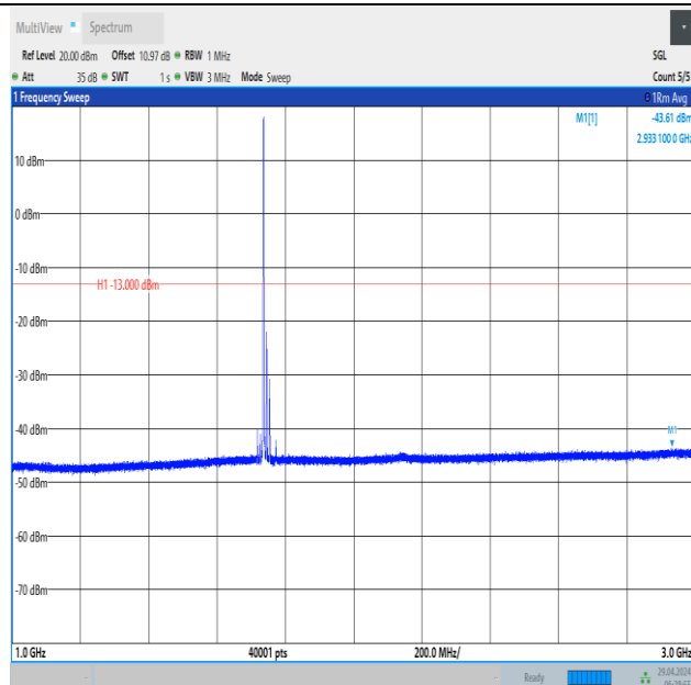
Band66_20MHz_16QAM_132322_1RB#0_1000~3000_1000~3000
