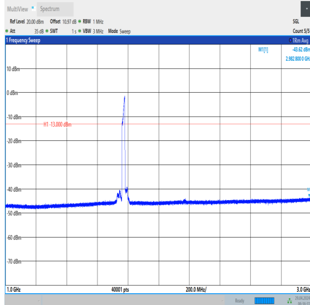
Band66_20MHz_QPSK_132572_100RB#0_1000~3000_1000~3000
