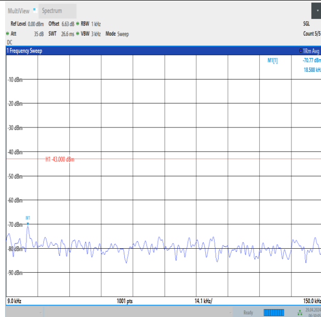
Band66_20MHz_16QAM_132322_1RB#99_0.009~0.15_0.009~0.15
