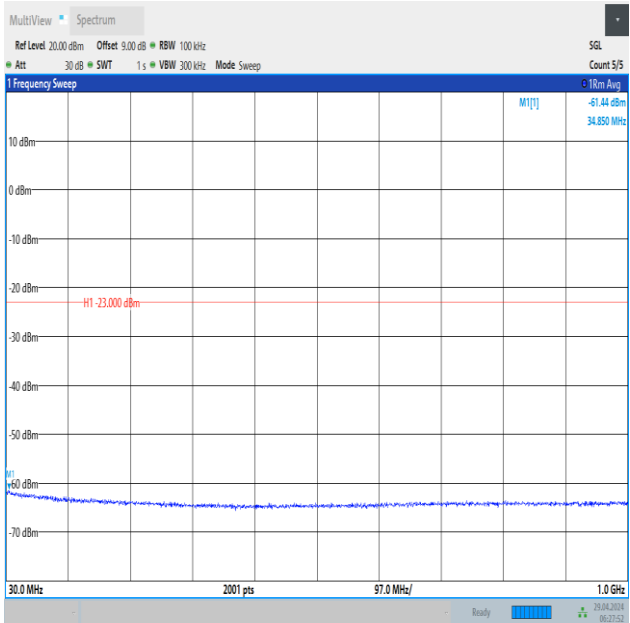
Band66_20MHz_QPSK_132322_1RB#0_30~1000_30~1000
