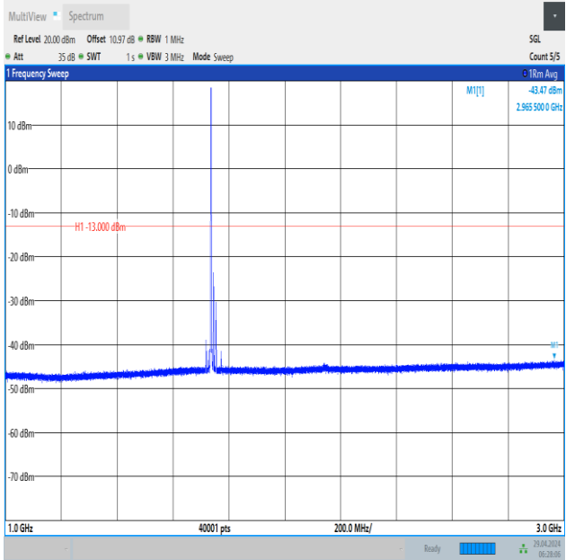
Band66_20MHz_QPSK_132322_1RB#0_1000~3000_1000~3000
