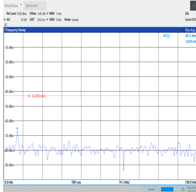
Band66_20MHz_16QAM_132572_1RB#99_0.009~0.15_0.009~0.15
