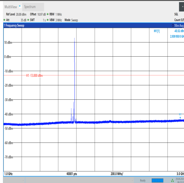
Band66_20MHz_16QAM_132572_1RB#99_1000~3000_1000~3000
