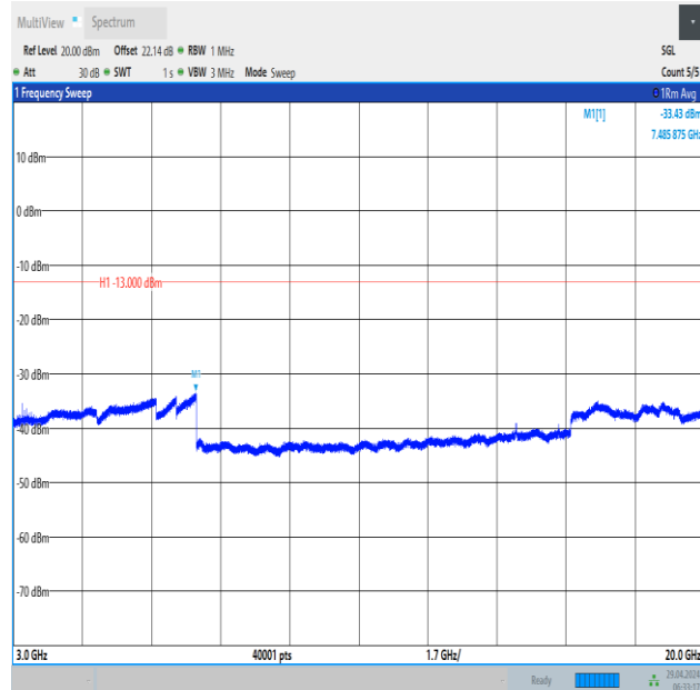
Band66_20MHz_QPSK_132572_1RB#99_3000~20000_3000~20000
