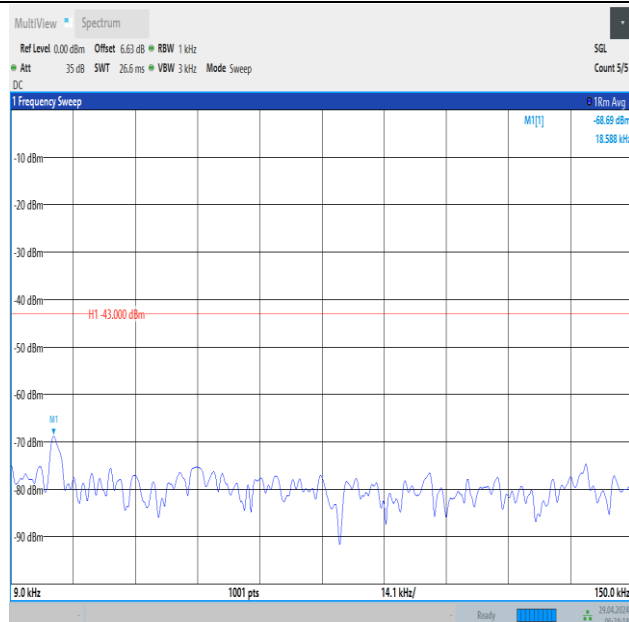
Band66_20MHz_QPSK_132072_1RB#0_0.009~0.15_0.009~0.15
