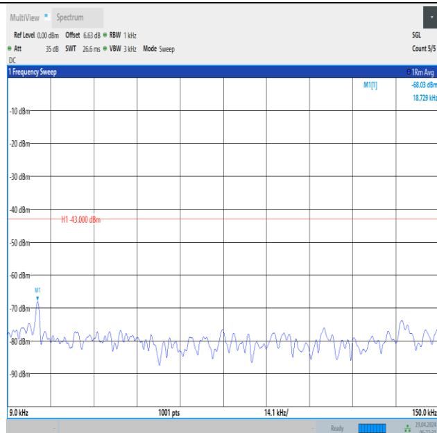
Band66_15MHz_QPSK_132322_75RB#0_0.009~0.15_0.009~0.15
