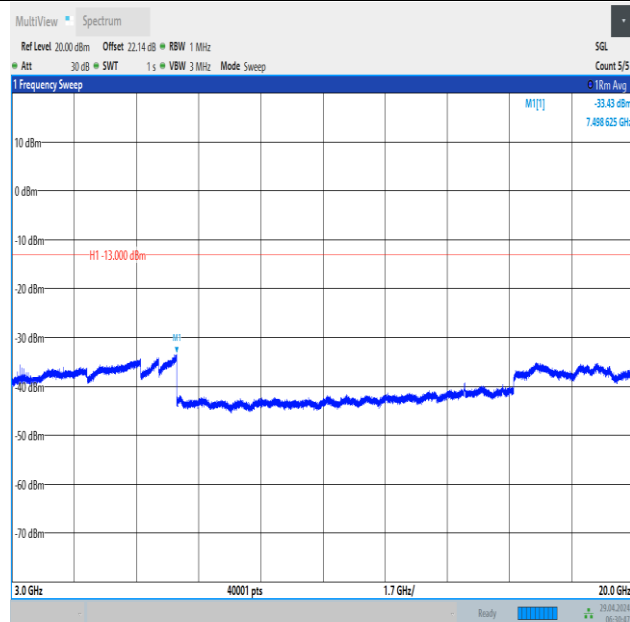
Band66_20MHz_16QAM_132322_1RB#99_3000~20000_3000~20000
