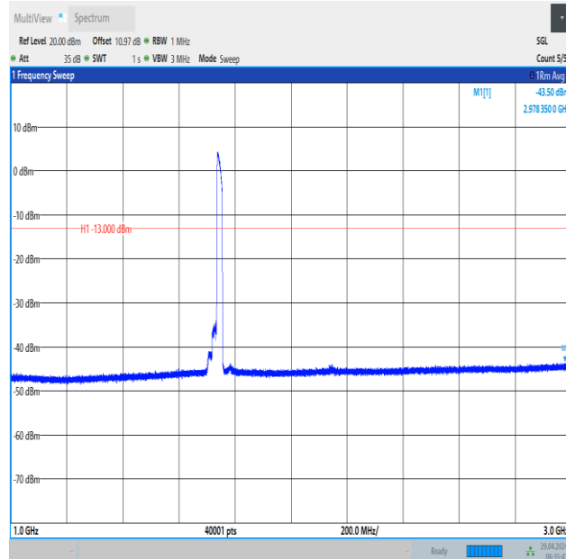
Band66_20MHz_QPSK_132322_100RB#0_1000~3000_1000~3000
