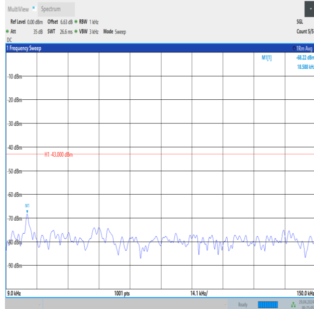
Band66_20MHz_16QAM_132072_1RB#0_0.009~0.15_0.009~0.15
