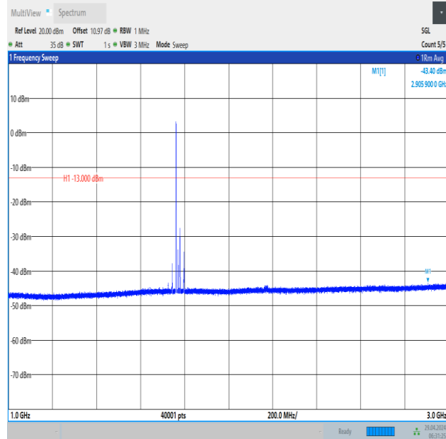
Band66_20MHz_QPSK_132572_1RB#0_1000~3000_1000~3000
