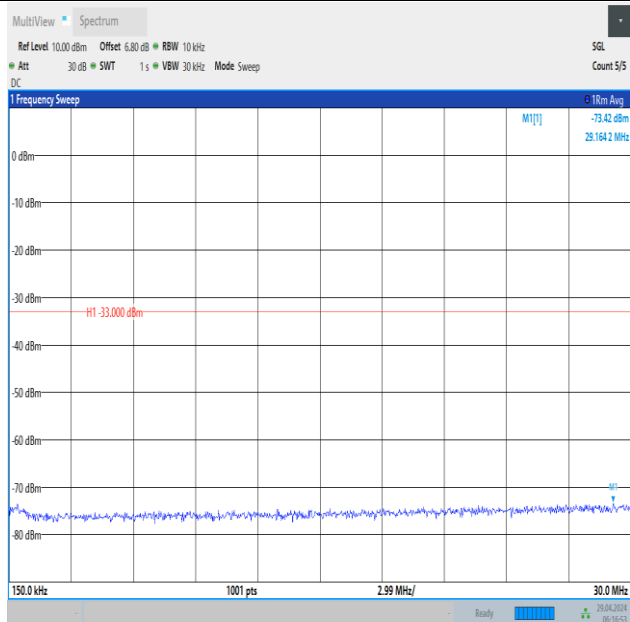
Band66_15MHz_16QAM_132597_1RB#74_0.15~30_0.15~30
