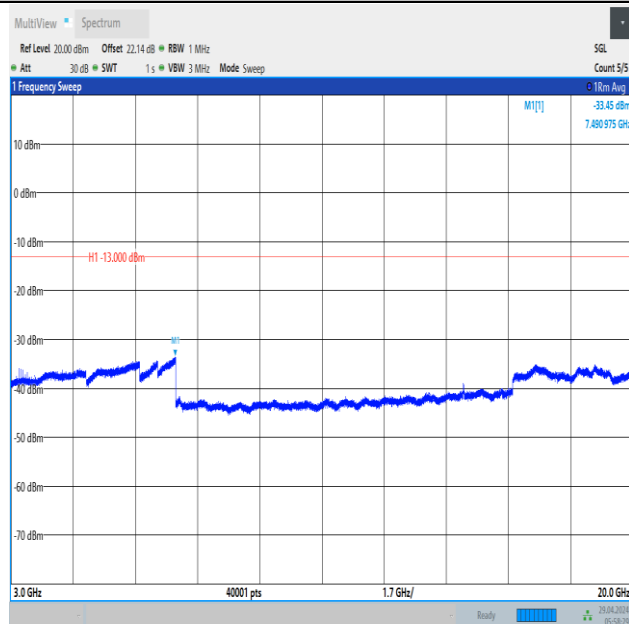
Band66_10MHz_16QAM_132322_1RB#0_3000~20000_3000~20000
