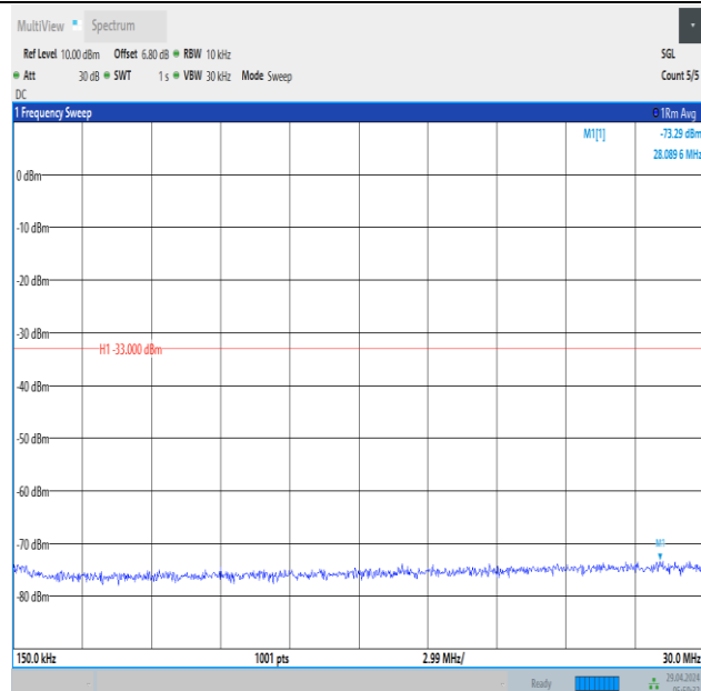
Band66_10MHz_16QAM_132322_1RB#49_0.15~30_0.15~30
