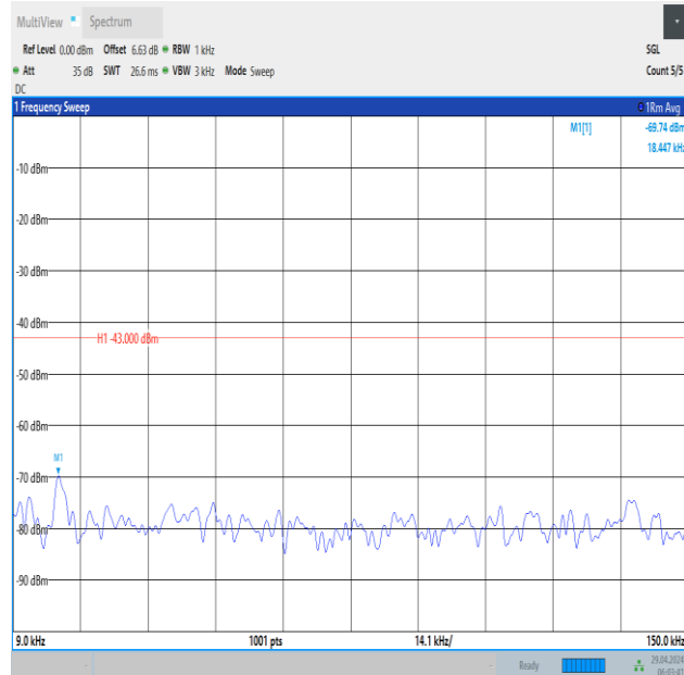
Band66_10MHz_QPSK_132022_50RB#0_0.009~0.15_0.009~0.15
