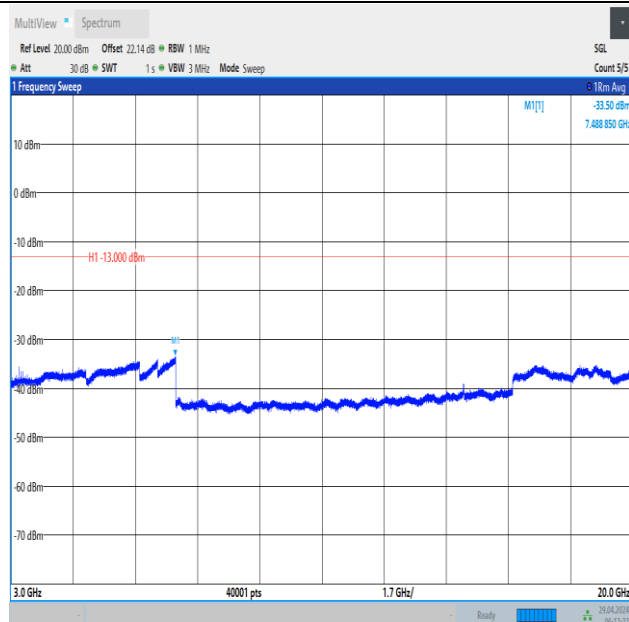
Band66_15MHz_16QAM_132322_1RB#0_3000~20000_3000~20000
