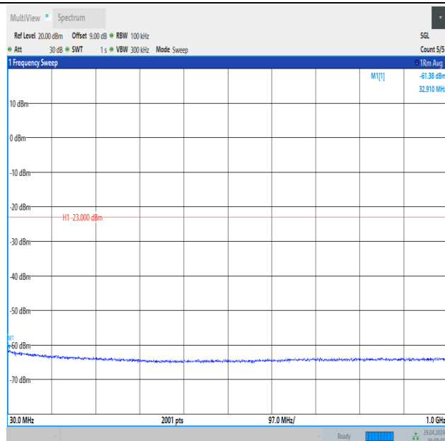
Band66_15MHz_16QAM_132047_1RB#0_30~1000_30~1000
