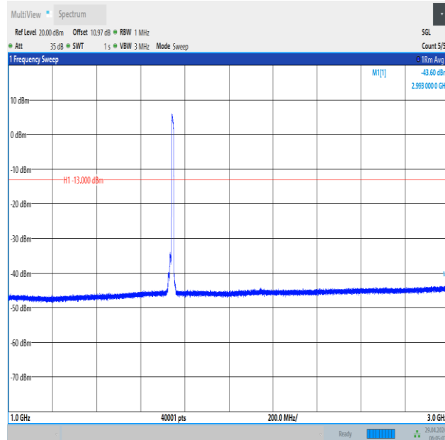
Band66_10MHz_QPSK_132322_50RB#0_1000~3000_1000~3000
