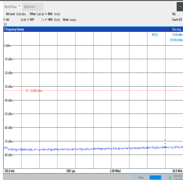
Band66_15MHz_QPSK_132322_1RB#74_0.15~30_0.15~30
