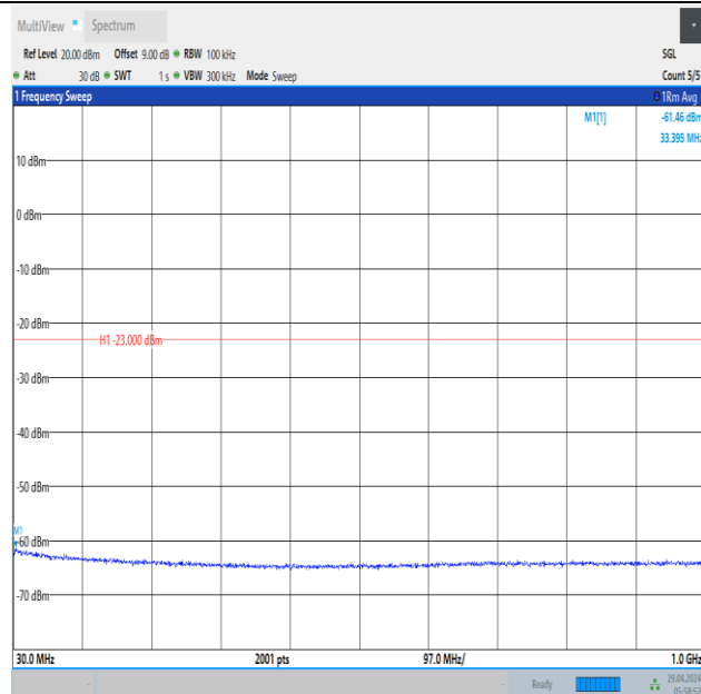
Band66_10MHz_QPSK_132322_1RB#49_30~1000_30~1000
