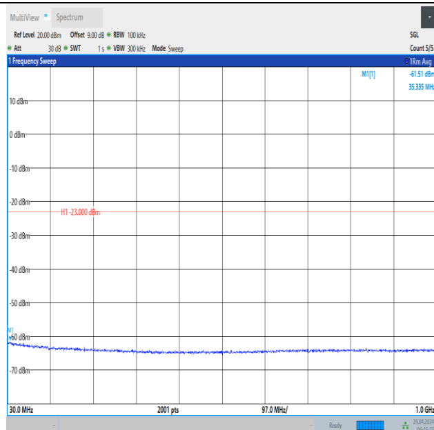
Band66_15MHz_16QAM_132597_1RB#0_30~1000_30~1000
