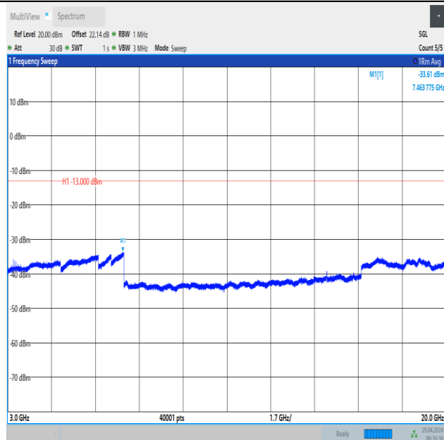
Band66_15MHz_QPSK_132597_1RB#74_3000~20000_3000~20000
