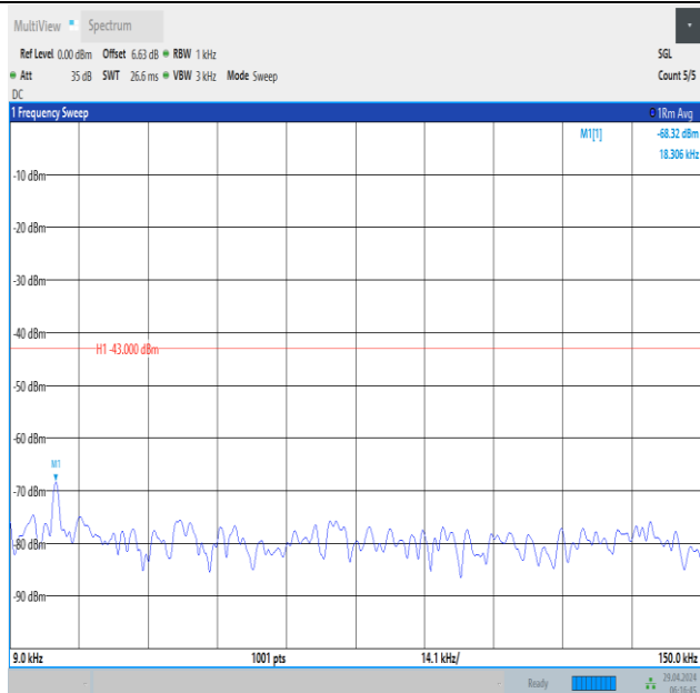
Band66_15MHz_16QAM_132597_1RB#74_0.009~0.15_0.009~0.15
