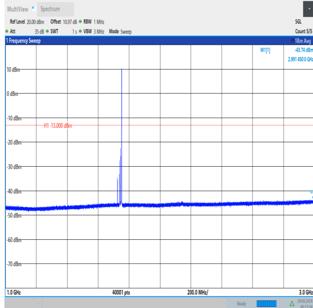
Band66_15MHz_16QAM_132322_1RB#74_1000~3000_1000~3000
