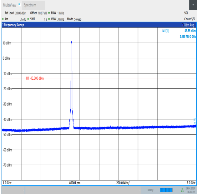
Band66_10MHz_QPSK_132022_50RB#0_1000~3000_1000~3000
