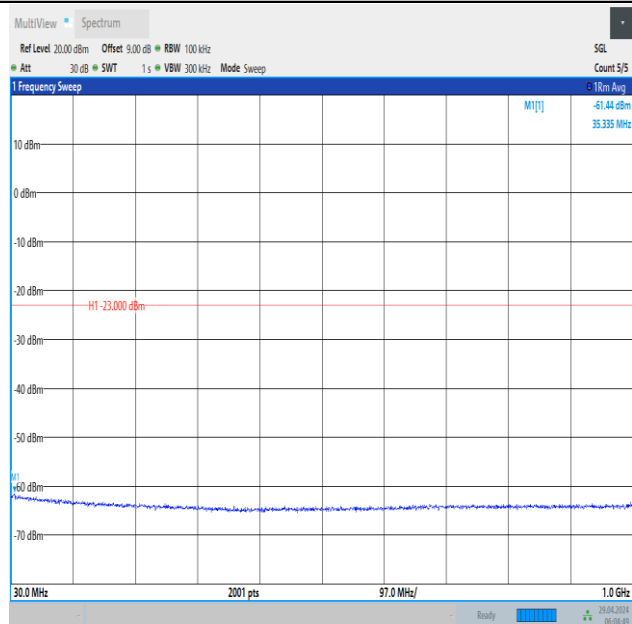
Band66_10MHz_QPSK_132322_50RB#0_30~1000_30~1000
