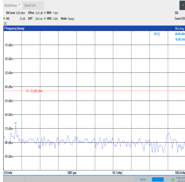
Band66_15MHz_QPSK_132597_1RB#0_0.009~0.15_0.009~0.15
