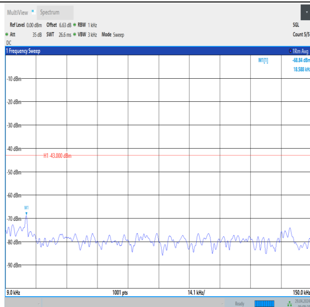
Band66_15MHz_16QAM_132047_1RB#0_0.009~0.15_0.009~0.15
