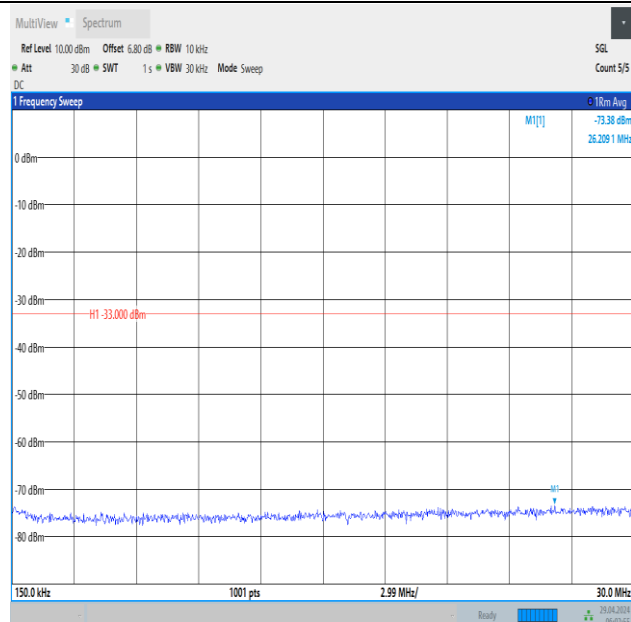
Band66_10MHz_16QAM_132622_1RB#49_0.15~30_0.15~30
