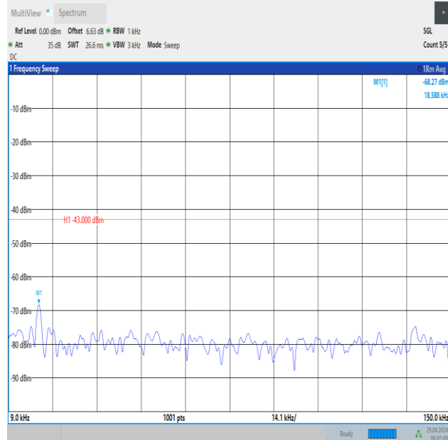
Band66_10MHz_16QAM_132622_1RB#0_0.009~0.15_0.009~0.15
