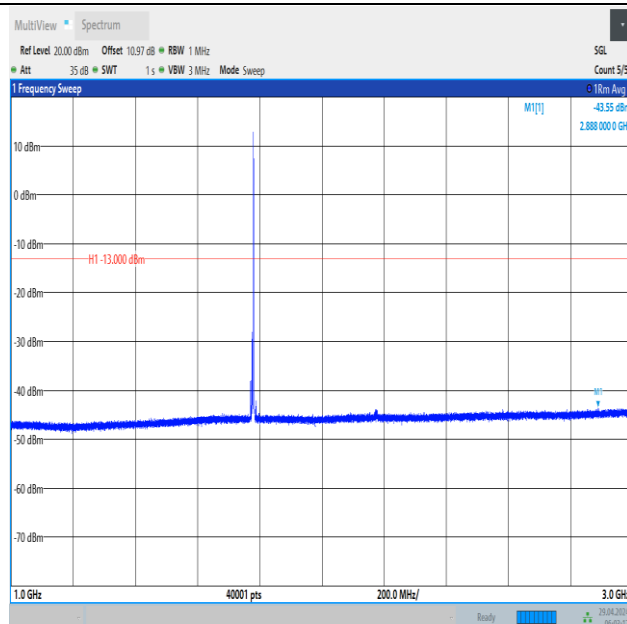
Band66_10MHz_16QAM_132622_1RB#49_1000~3000_1000~3000
