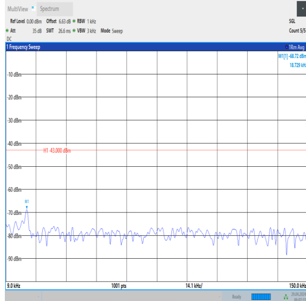
Band66_15MHz_QPSK_132047_1RB#0_0.009~0.15_0.009~0.15
