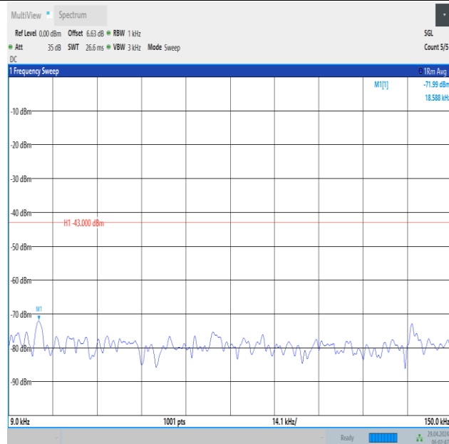
Band66_10MHz_16QAM_132622_1RB#49_0.009~0.15_0.009~0.15
