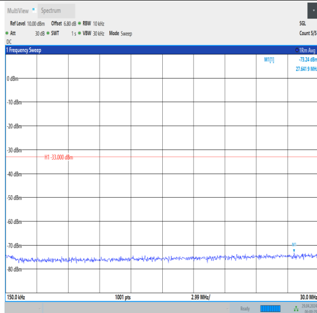
Band66_10MHz_QPSK_132622_1RB#0_0.15~30_0.15~30
