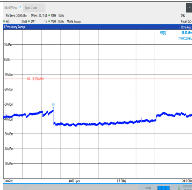
Band66_15MHz_16QAM_132047_1RB#74_3000~20000_3000~20000
