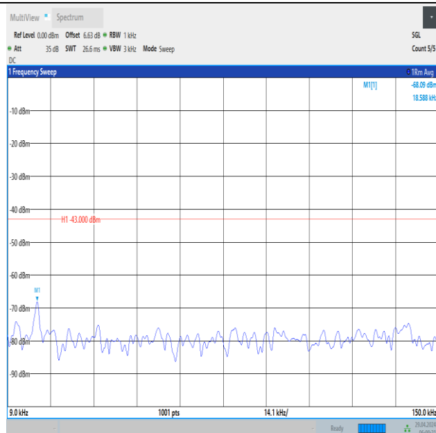
Band66_10MHz_QPSK_132622_1RB#0_0.009~0.15_0.009~0.15
