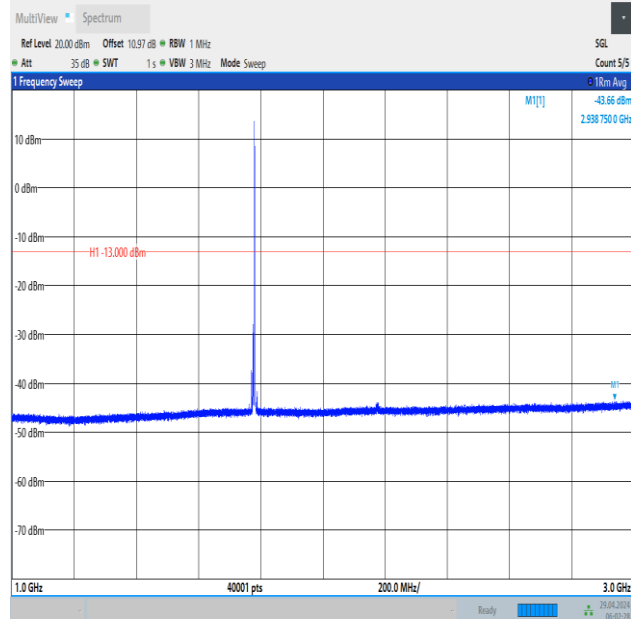
Band66_10MHz_QPSK_132622_1RB#49_1000~3000_1000~3000
