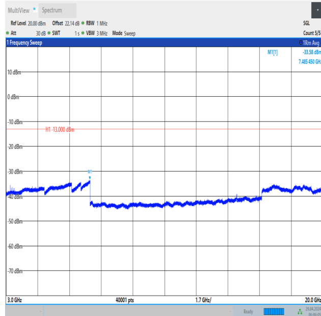
Band66_10MHz_QPSK_132622_50RB#0_3000~20000_3000~20000
