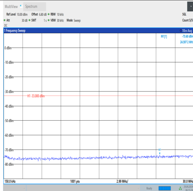
Band66_15MHz_16QAM_132597_1RB#0_0.15~30_0.15~30
