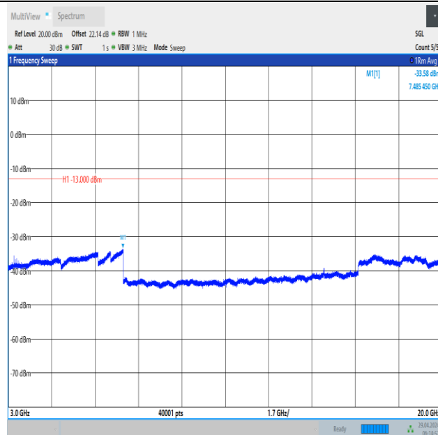
Band66_15MHz_QPSK_132597_1RB#0_3000~20000_3000~20000
