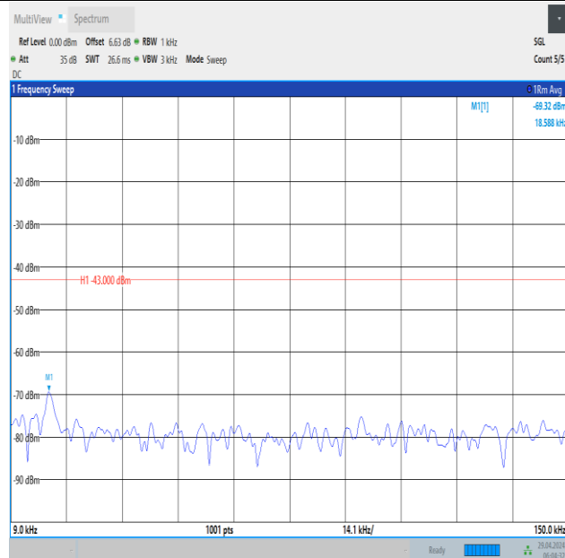
Band66_10MHz_QPSK_132322_50RB#0_0.009~0.15_0.009~0.15
