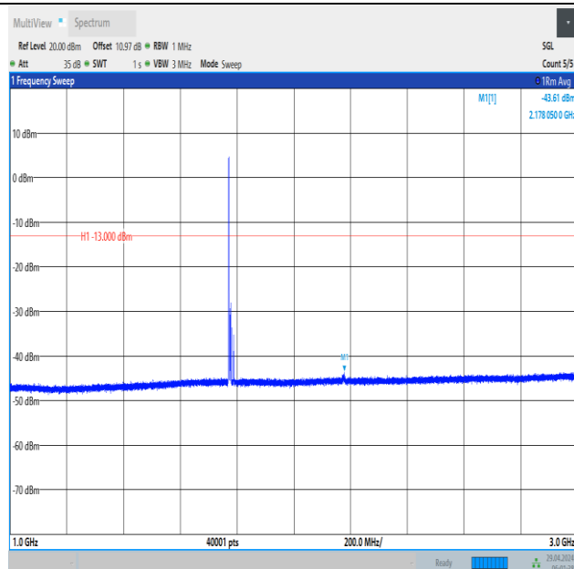
Band66_10MHz_16QAM_132622_1RB#0_1000~3000_1000~3000
