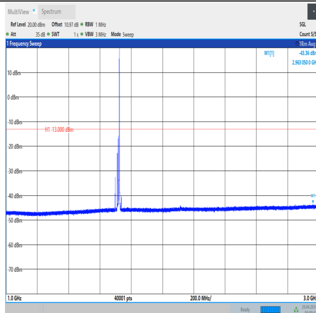
Band66_15MHz_QPSK_132047_1RB#74_1000~3000_1000~3000
