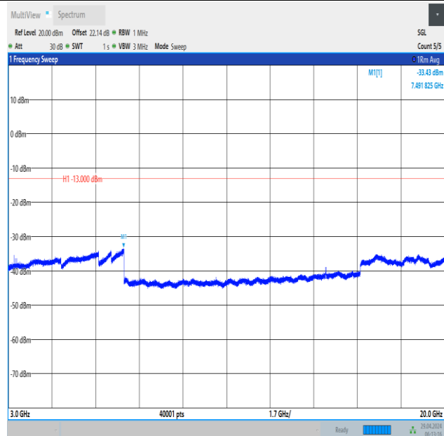
Band66_15MHz_QPSK_132322_1RB#74_3000~20000_3000~20000
