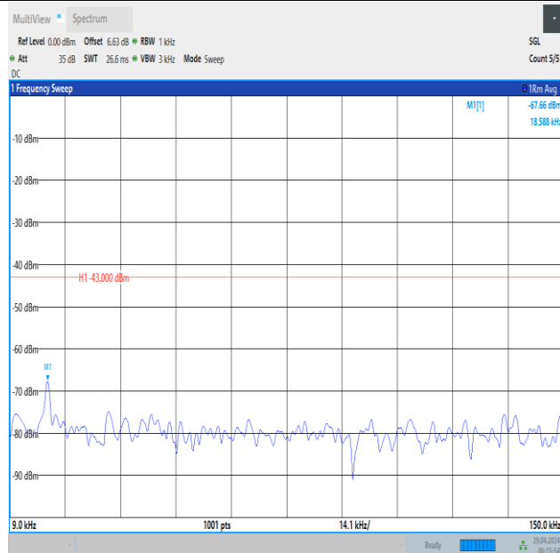
Band66_15MHz_QPSK_132597_1RB#74_0.009~0.15_0.009~0.15
