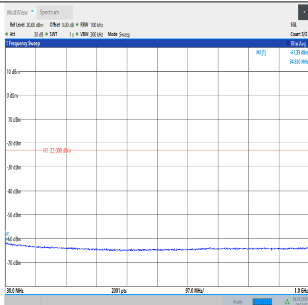
Band66_15MHz_16QAM_132322_1RB#74_30~1000_30~1000
