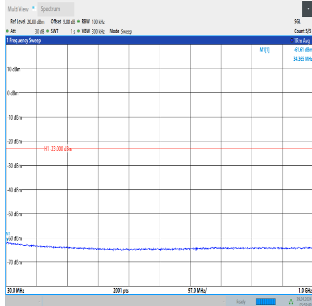
Band66_10MHz_16QAM_132322_1RB#49_30~1000_30~1000
