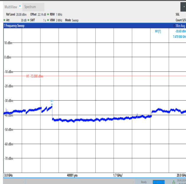
Band66_10MHz_QPSK_132022_1RB#49_3000~20000_3000~20000
