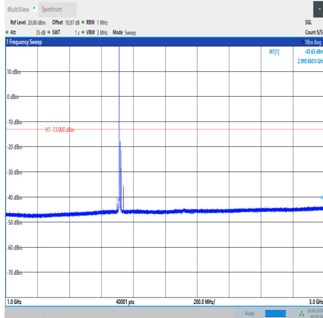
Band66_15MHz_16QAM_132047_1RB#0_1000~3000_1000~3000
