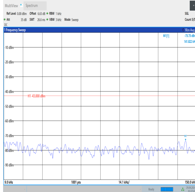
Band66_10MHz_16QAM_132322_1RB#0_0.009~0.15_0.009~0.15
