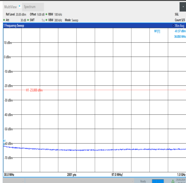
Band66_15MHz_QPSK_132047_1RB#74_30~1000_30~1000
