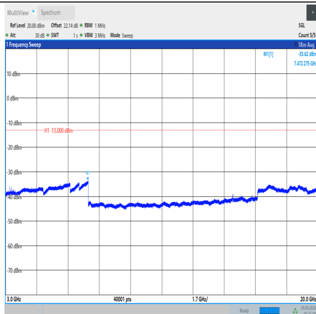
Band66_15MHz_16QAM_132597_1RB#0_3000~20000_3000~20000
