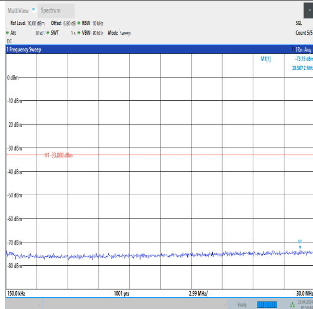
Band66_10MHz_QPSK_132322_1RB#49_0.15~30_0.15~30
