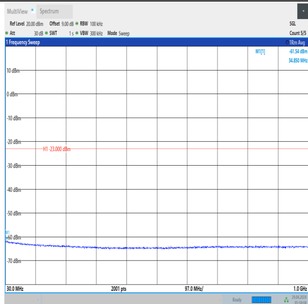
Band66_10MHz_16QAM_132322_1RB#0_30~1000_30~1000
