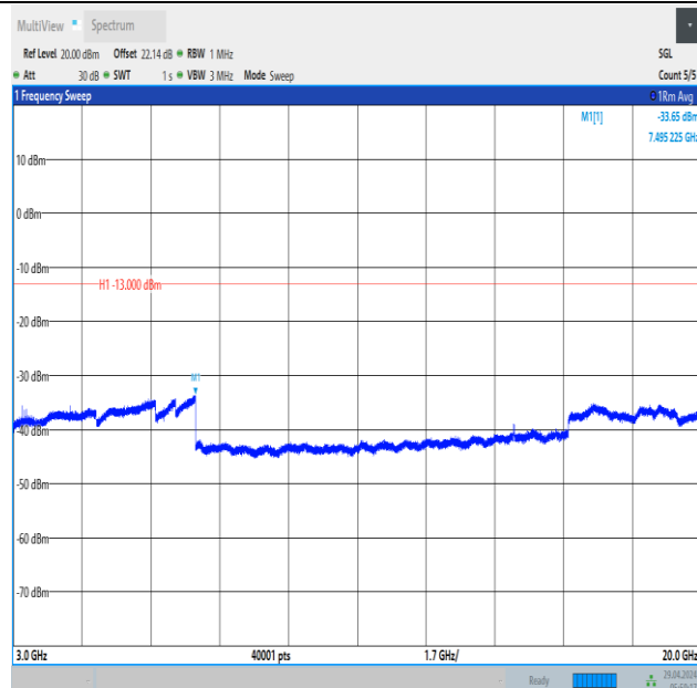
Band66_10MHz_QPSK_132322_1RB#49_3000~20000_3000~20000
