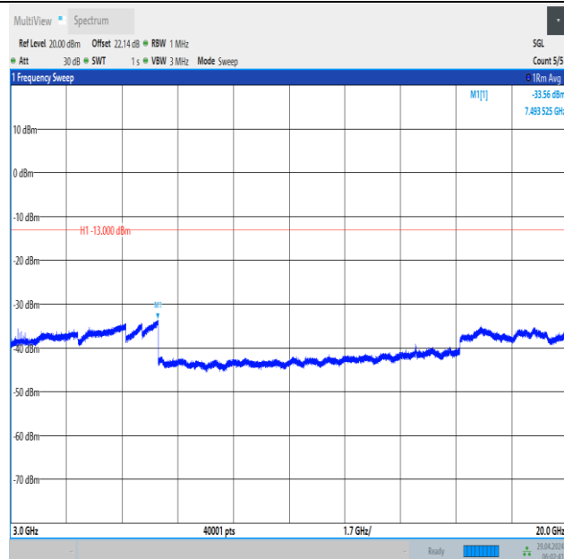
Band66_10MHz_QPSK_132622_1RB#49_3000~20000_3000~20000
