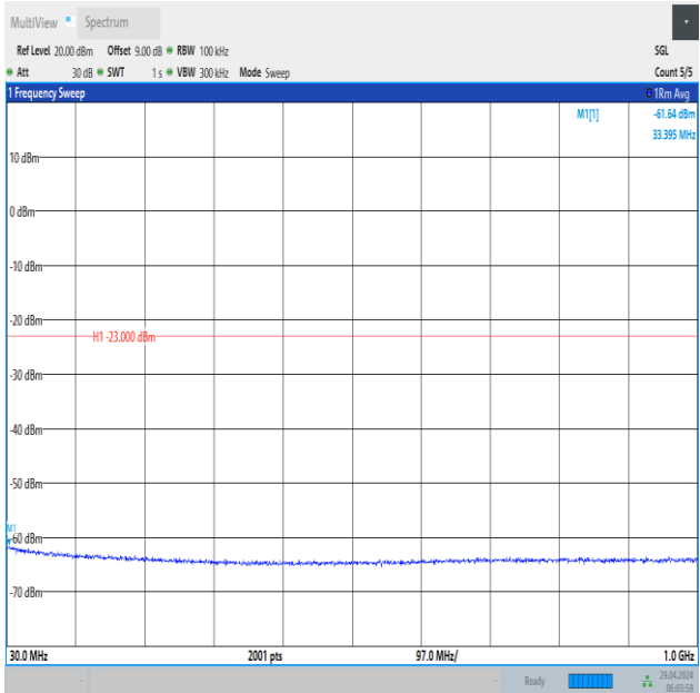
Band66_10MHz_QPSK_132022_50RB#0_30~1000_30~1000
