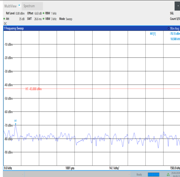
Band66_15MHz_QPSK_132047_1RB#74_0.009~0.15_0.009~0.15
