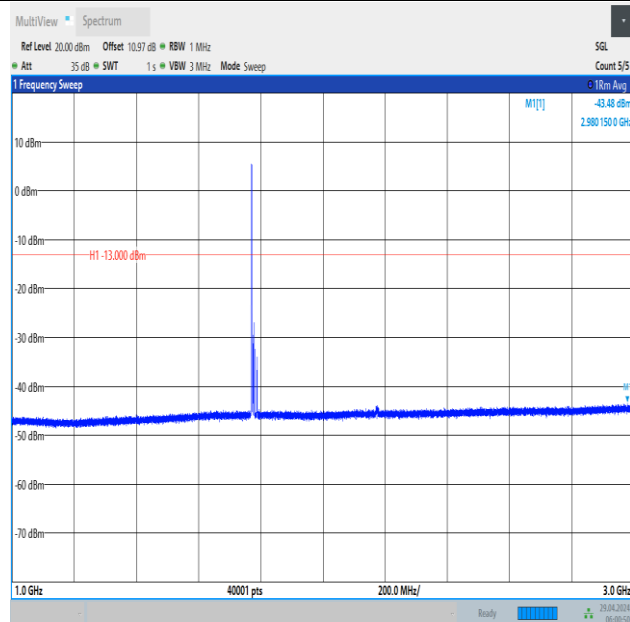
Band66_10MHz_QPSK_132622_1RB#0_1000~3000_1000~3000
