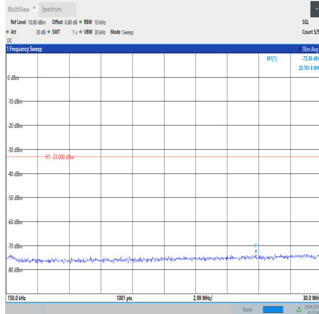
Band66_10MHz_QPSK_132322_1RB#0_0.15~30_0.15~30
