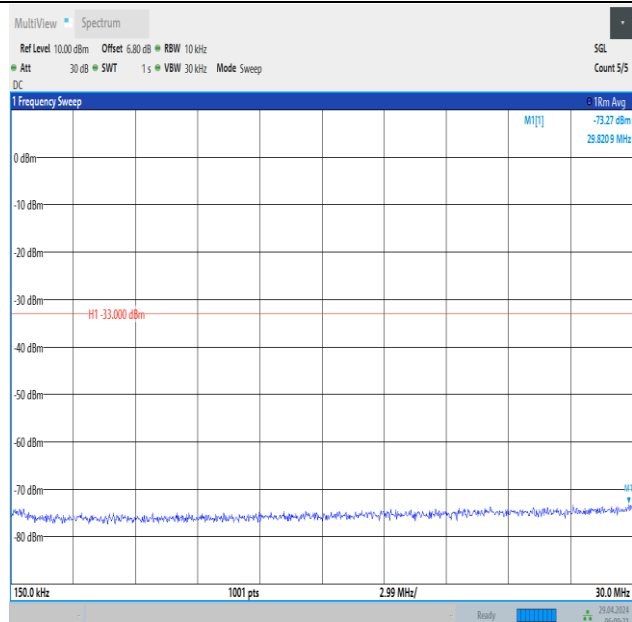
Band66_15MHz_QPSK_132047_1RB#74_0.15~30_0.15~30
