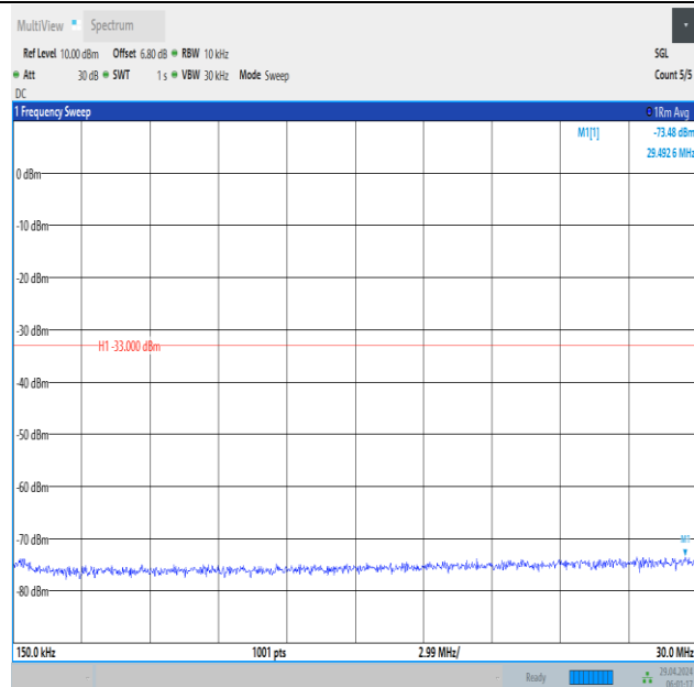
Band66_10MHz_16QAM_132622_1RB#0_0.15~30_0.15~30
