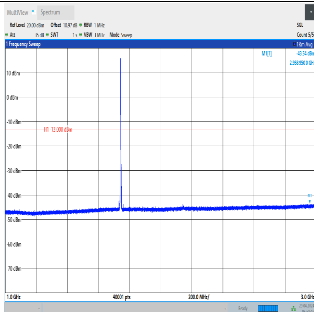
Band66_10MHz_16QAM_132322_1RB#0_1000~3000_1000~3000
