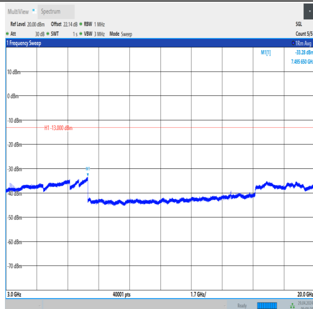
Band66_10MHz_QPSK_132022_50RB#0_3000~20000_3000~20000
