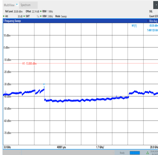
Band66_15MHz_16QAM_132322_1RB#74_3000~20000_3000~20000
