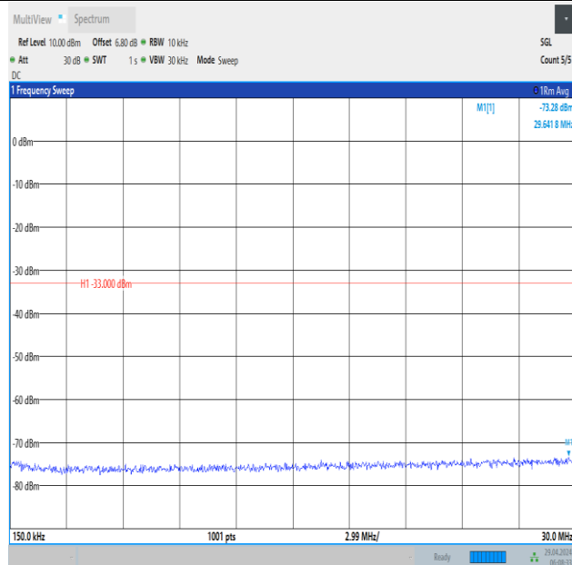
Band66_15MHz_16QAM_132047_1RB#0_0.15~30_0.15~30
