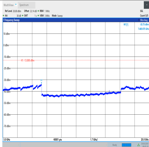
Band66_10MHz_QPSK_132322_50RB#0_3000~20000_3000~20000
