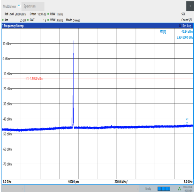
Band66_10MHz_16QAM_132322_1RB#49_1000~3000_1000~3000
