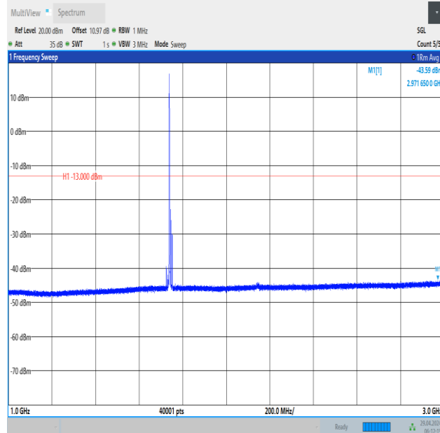
Band66_15MHz_16QAM_132322_1RB#0_1000~3000_1000~3000
