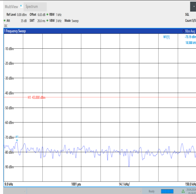
Band66_10MHz_16QAM_132022_1RB#49_0.009~0.15_0.009~0.15
