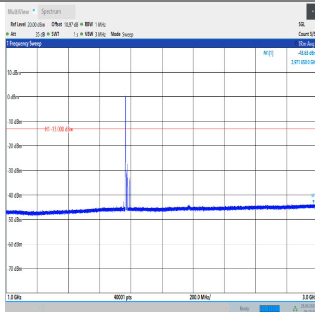
Band66_15MHz_QPSK_132597_1RB#0_1000~3000_1000~3000
