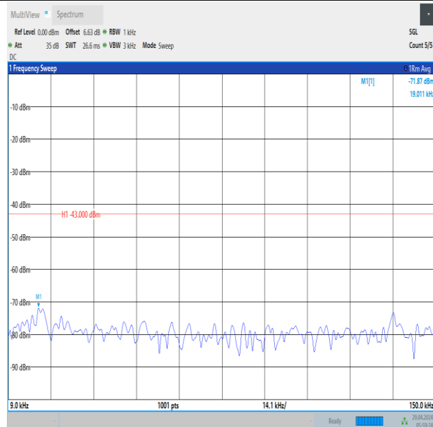
Band66_10MHz_16QAM_132322_1RB#49_0.009~0.15_0.009~0.15
