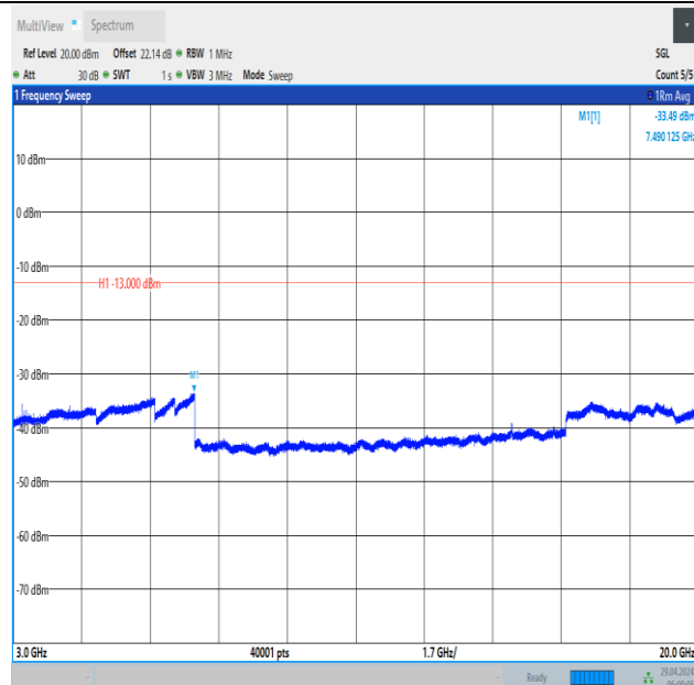
Band66_15MHz_16QAM_132047_1RB#0_3000~20000_3000~20000
