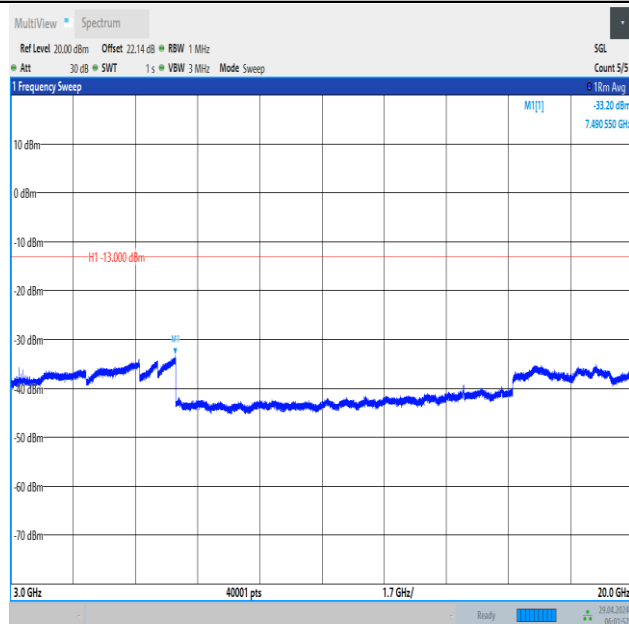
Band66_10MHz_16QAM_132622_1RB#0_3000~20000_3000~20000
