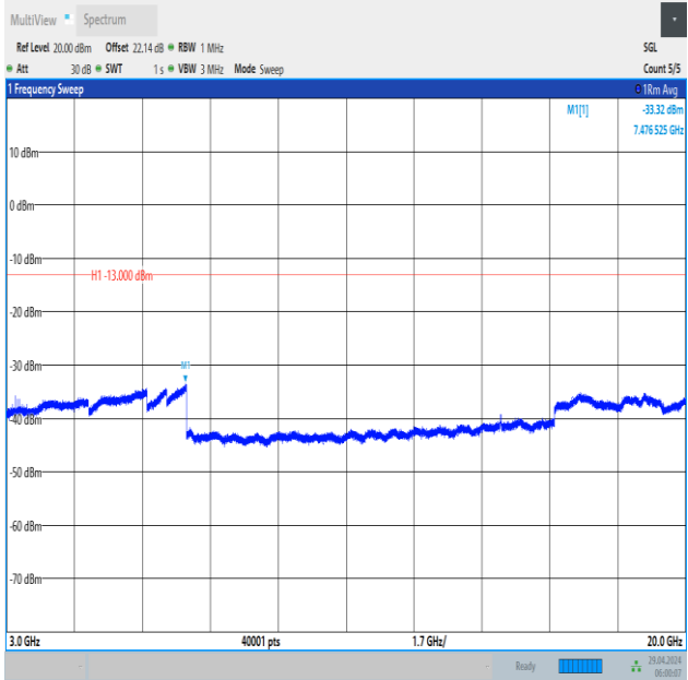
Band66_10MHz_16QAM_132322_1RB#49_3000~20000_3000~20000
