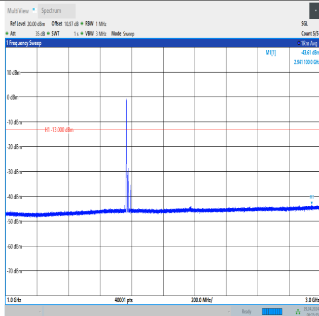
Band66_15MHz_16QAM_132597_1RB#0_1000~3000_1000~3000
