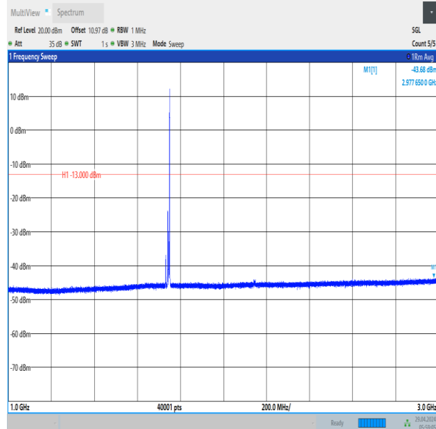
Band66_10MHz_QPSK_132322_1RB#49_1000~3000_1000~3000
