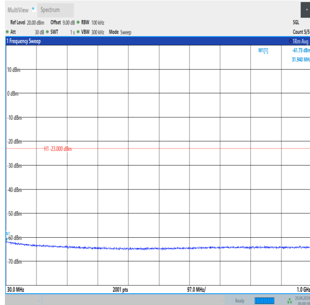
Band66_10MHz_QPSK_132622_1RB#0_30~1000_30~1000
