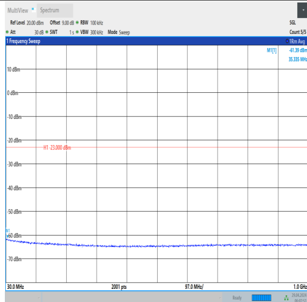
Band66_15MHz_QPSK_132047_1RB#0_30~1000_30~1000
