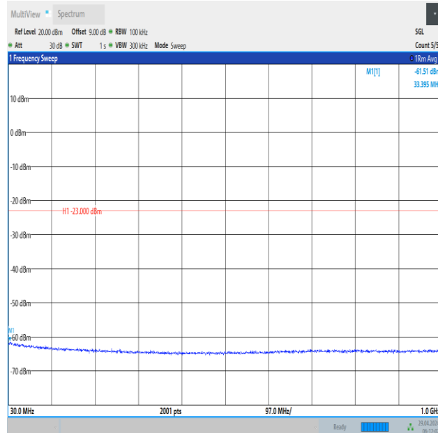
Band66_15MHz_16QAM_132322_1RB#0_30~1000_30~1000
