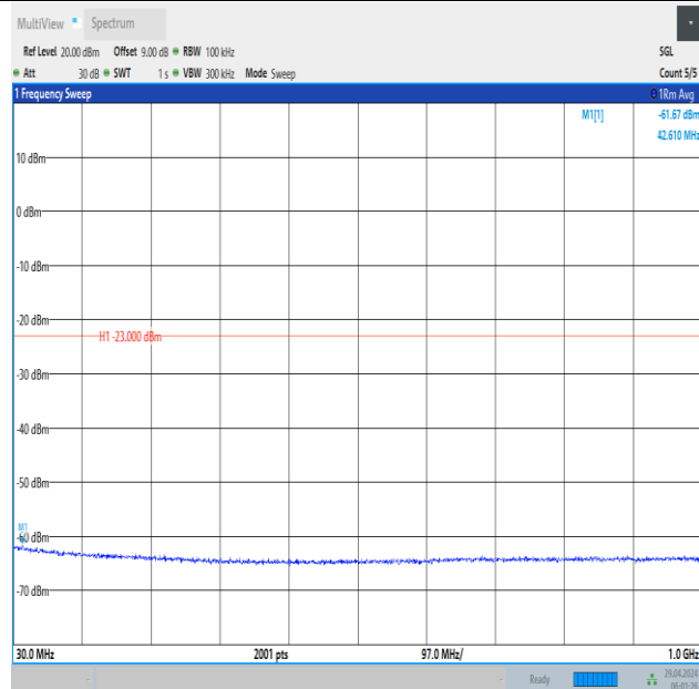
Band66_10MHz_16QAM_132622_1RB#0_30~1000_30~1000
