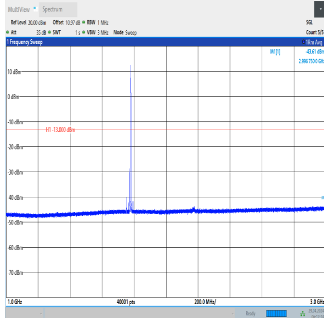
Band66_15MHz_16QAM_132597_1RB#74_1000~3000_1000~3000
