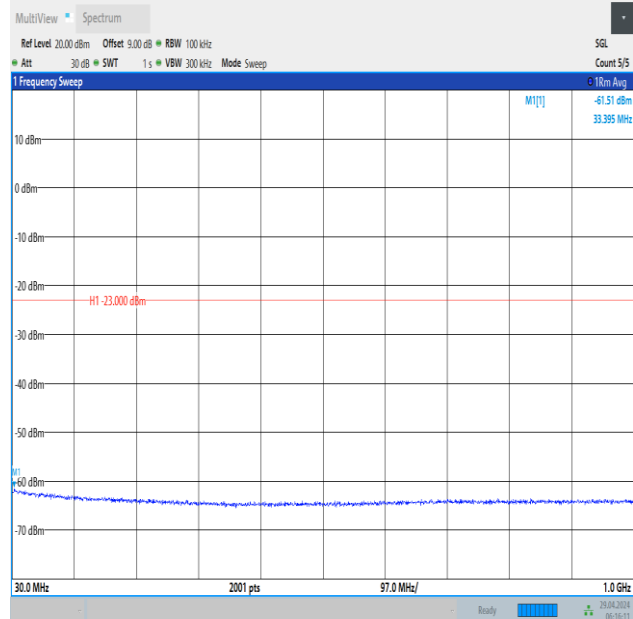
Band66_15MHz_QPSK_132597_1RB#74_30~1000_30~1000
