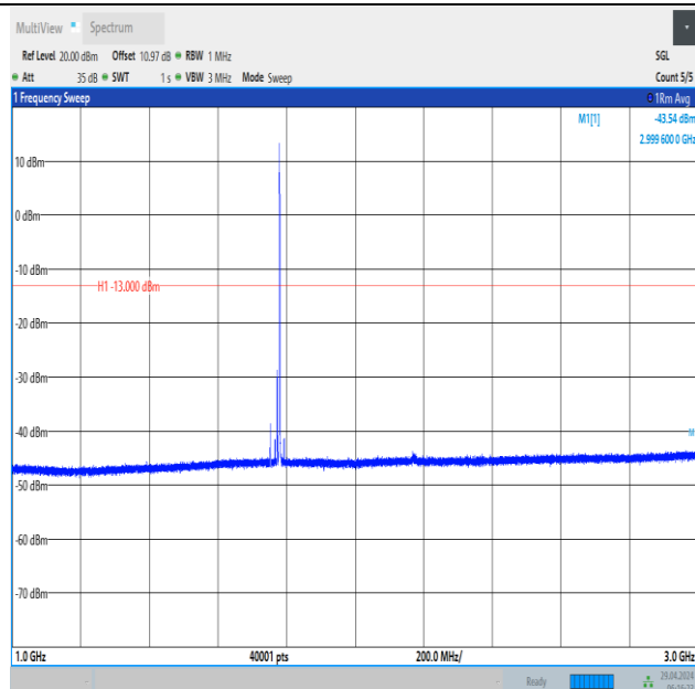
Band66_15MHz_QPSK_132597_1RB#74_1000~3000_1000~3000
