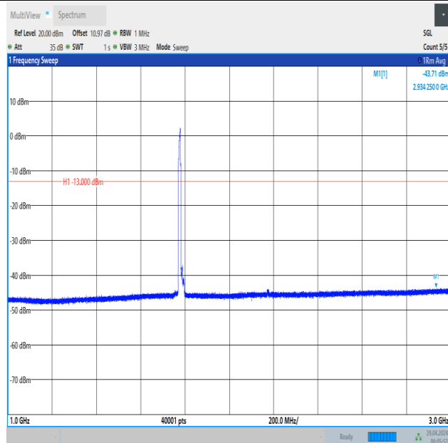
Band66_10MHz_QPSK_132622_50RB#0_1000~3000_1000~3000
