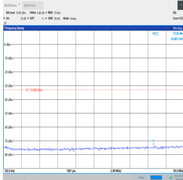
Band66_10MHz_QPSK_132022_50RB#0_0.15~30_0.15~30
