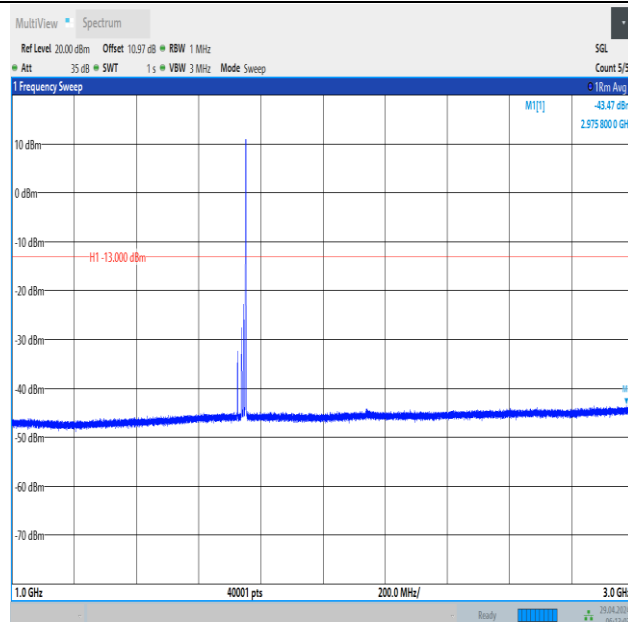
Band66_15MHz_QPSK_132322_1RB#74_1000~3000_1000~3000
