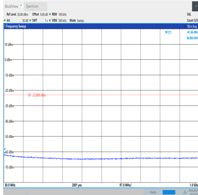
Band66_10MHz_QPSK_132322_1RB#0_30~1000_30~1000
