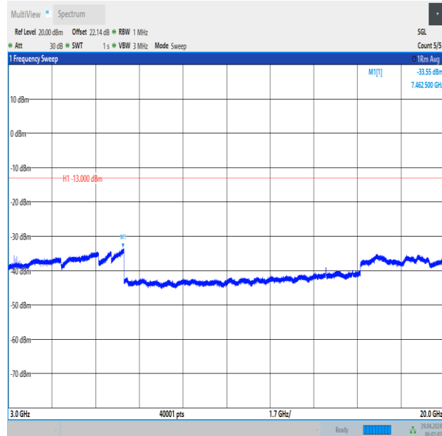
Band66_10MHz_QPSK_132622_1RB#0_3000~20000_3000~20000
