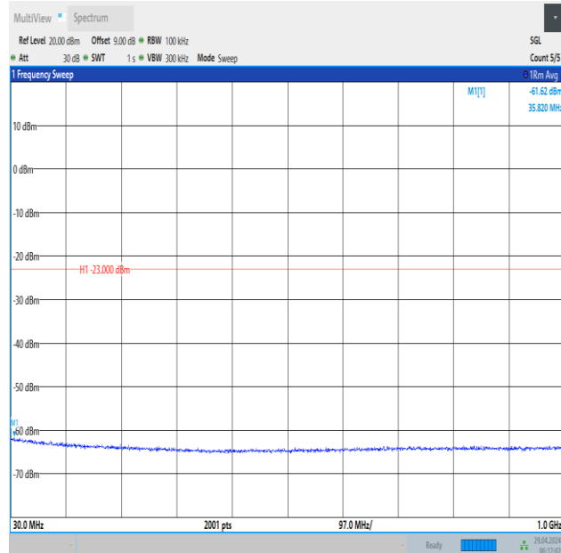
Band66_15MHz_16QAM_132597_1RB#74_30~1000_30~1000
