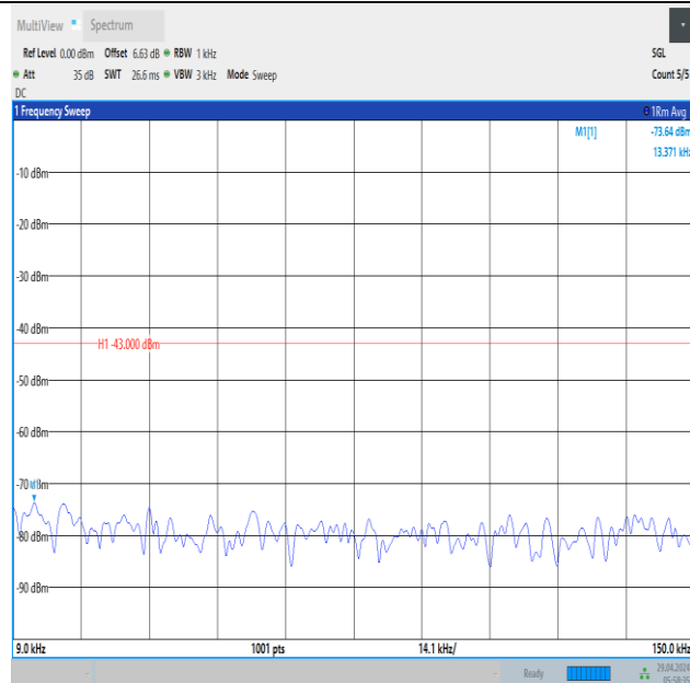
Band66_10MHz_QPSK_132322_1RB#49_0.009~0.15_0.009~0.15
