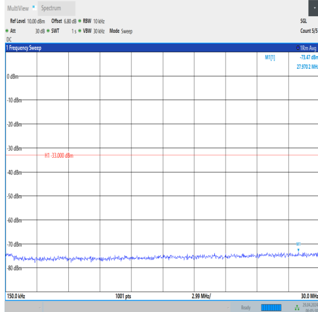
Band66_10MHz_QPSK_132622_50RB#0_0.15~30_0.15~30
