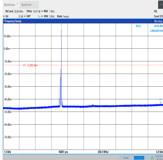
Band66_15MHz_16QAM_132047_1RB#74_1000~3000_1000~3000
