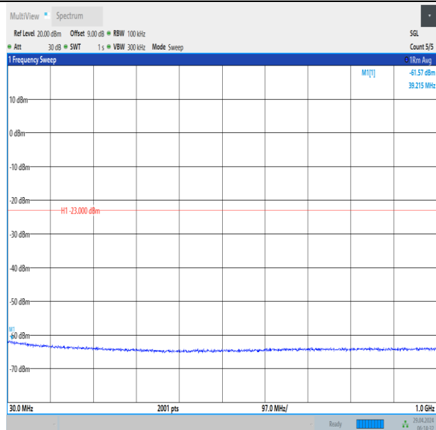
Band66_15MHz_QPSK_132597_1RB#0_30~1000_30~1000
