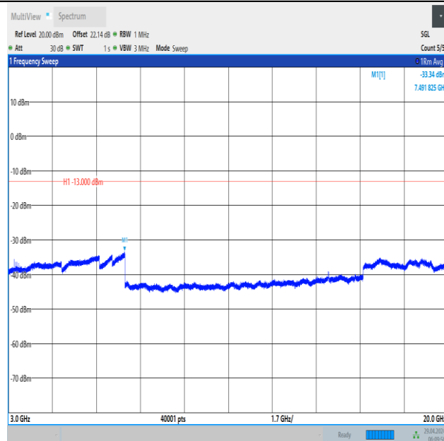
Band66_15MHz_QPSK_132047_1RB#74_3000~20000_3000~20000
