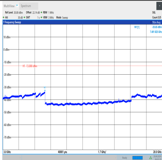
Band66_10MHz_16QAM_132622_1RB#49_3000~20000_3000~20000
