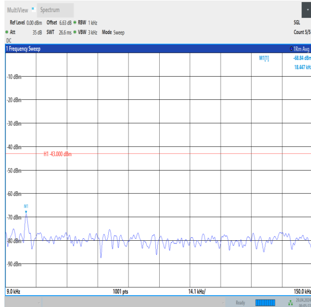
Band66_10MHz_QPSK_132622_50RB#0_0.009~0.15_0.009~0.15
