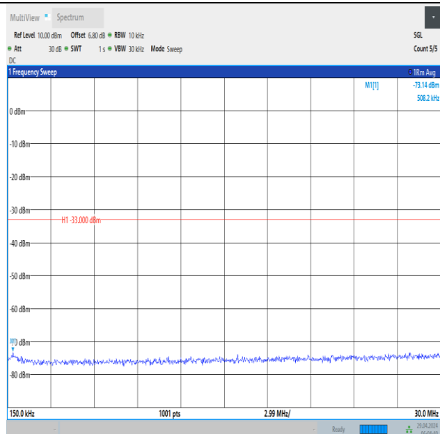
Band66_10MHz_QPSK_132322_50RB#0_0.15~30_0.15~30
