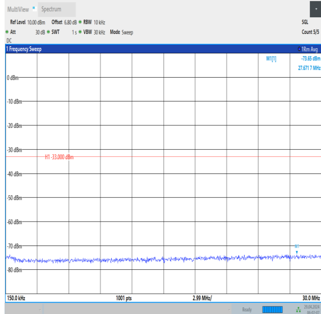
Band66_10MHz_QPSK_132622_1RB#49_0.15~30_0.15~30
