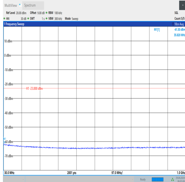
Band66_10MHz_16QAM_132622_1RB#49_30~1000_30~1000
