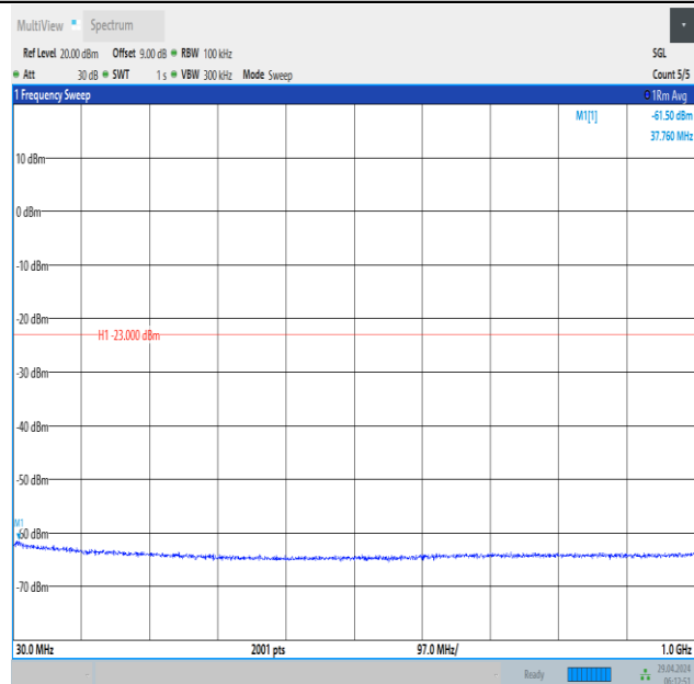
Band66_15MHz_QPSK_132322_1RB#74_30~1000_30~1000
