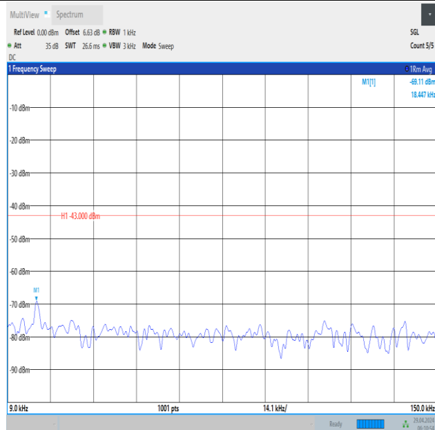
Band66_15MHz_QPSK_132322_1RB#0_0.009~0.15_0.009~0.15
