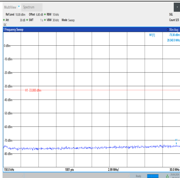
Band66_15MHz_QPSK_132597_1RB#0_0.15~30_0.15~30
