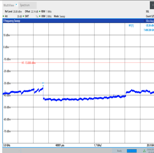
Band66_10MHz_16QAM_132022_1RB#49_3000~20000_3000~20000
