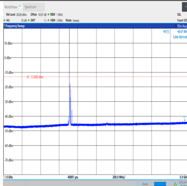
Band66_15MHz_QPSK_132047_1RB#0_1000~3000_1000~3000
