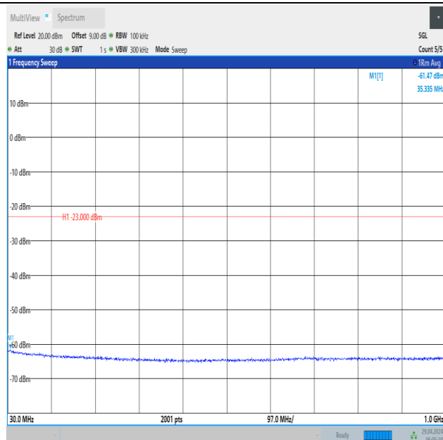
Band66_10MHz_QPSK_132622_50RB#0_30~1000_30~1000
