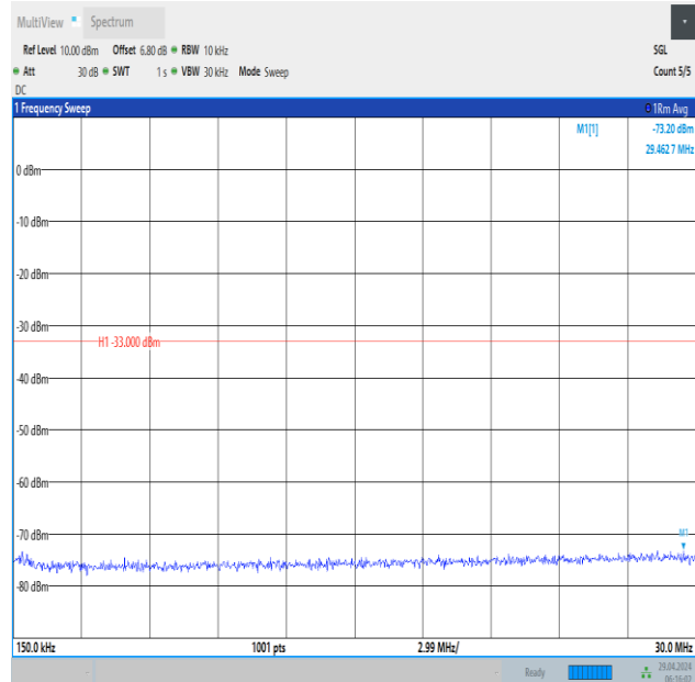
Band66_15MHz_QPSK_132597_1RB#74_0.15~30_0.15~30
