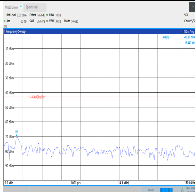
Band66_15MHz_16QAM_132597_1RB#0_0.009~0.15_0.009~0.15
