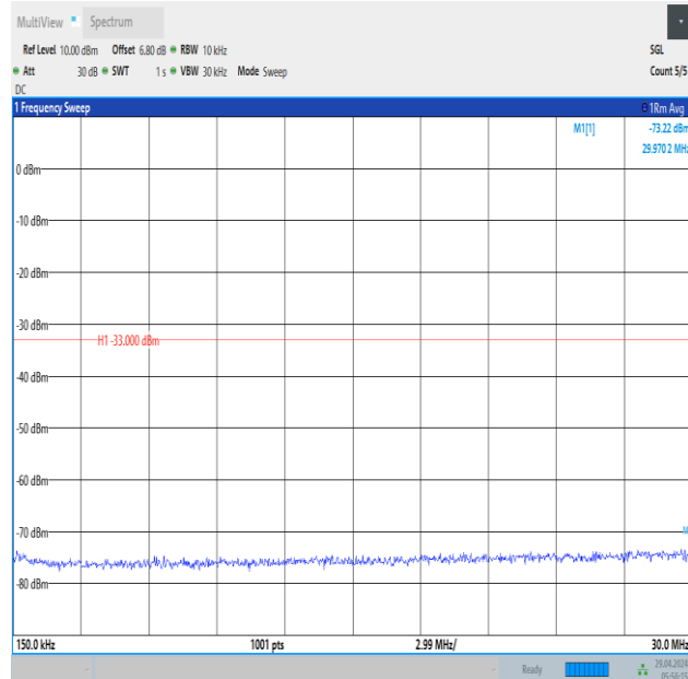
Band66_10MHz_16QAM_132022_1RB#49_0.15~30_0.15~30
