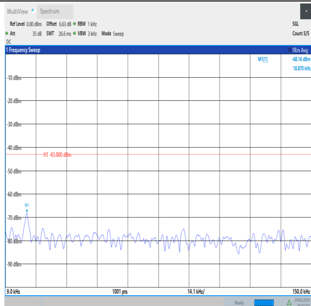
Band66_10MHz_QPSK_132622_1RB#49_0.009~0.15_0.009~0.15
