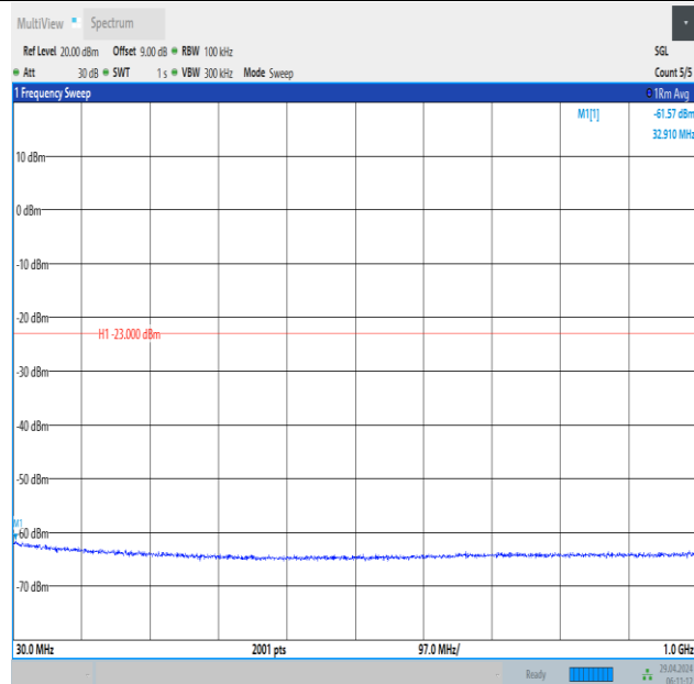
Band66_15MHz_QPSK_132322_1RB#0_30~1000_30~1000
