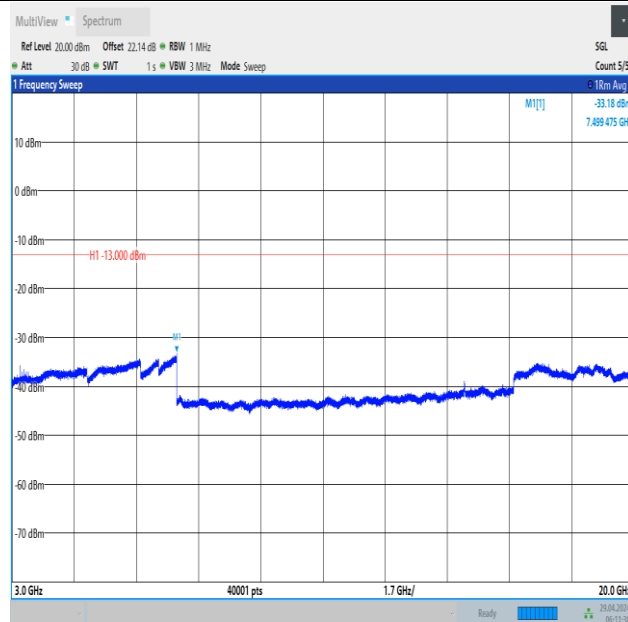
Band66_15MHz_QPSK_132322_1RB#0_3000~20000_3000~20000
