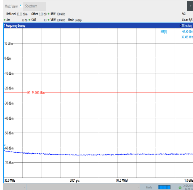
Band66_10MHz_QPSK_132622_1RB#49_30~1000_30~1000
