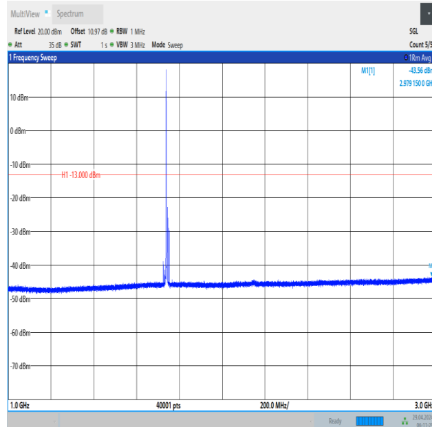
Band66_15MHz_QPSK_132322_1RB#0_1000~3000_1000~3000
