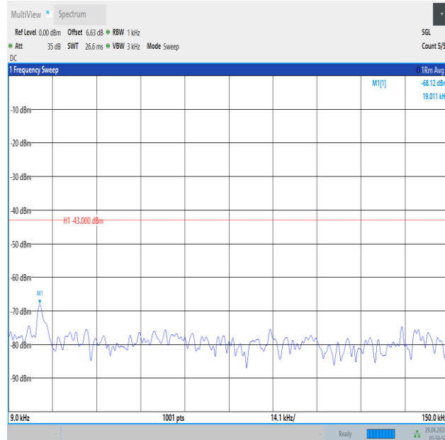
Band66_10MHz_QPSK_132322_1RB#0_0.009~0.15_0.009~0.15
