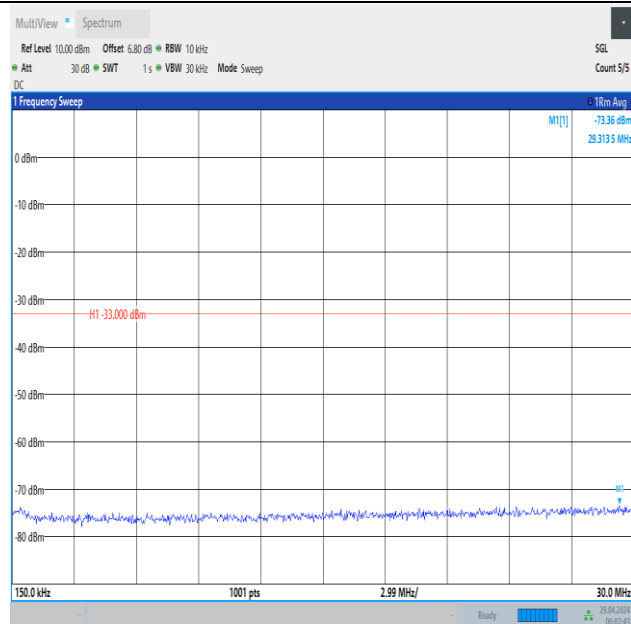
Band66_15MHz_QPSK_132047_1RB#0_0.15~30_0.15~30
