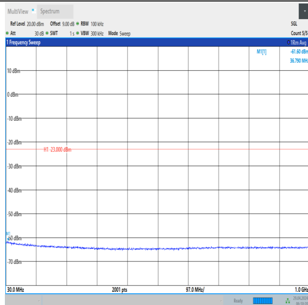
Band66_15MHz_16QAM_132047_1RB#74_30~1000_30~1000
