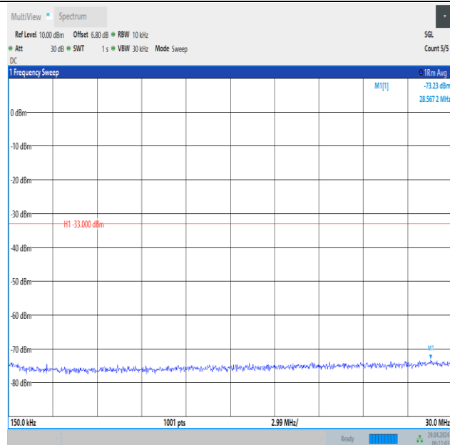
Band66_15MHz_QPSK_132322_1RB#0_0.15~30_0.15~30
