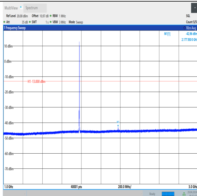
Band66_5MHz_16QAM_132647_1RB#24_1000~3000_1000~3000
