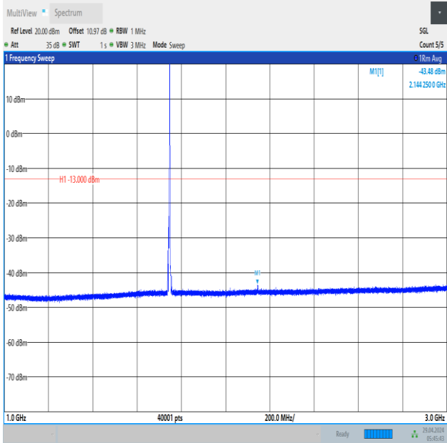
Band66_5MHz_QPSK_132322_1RB#24_1000~3000_1000~3000
