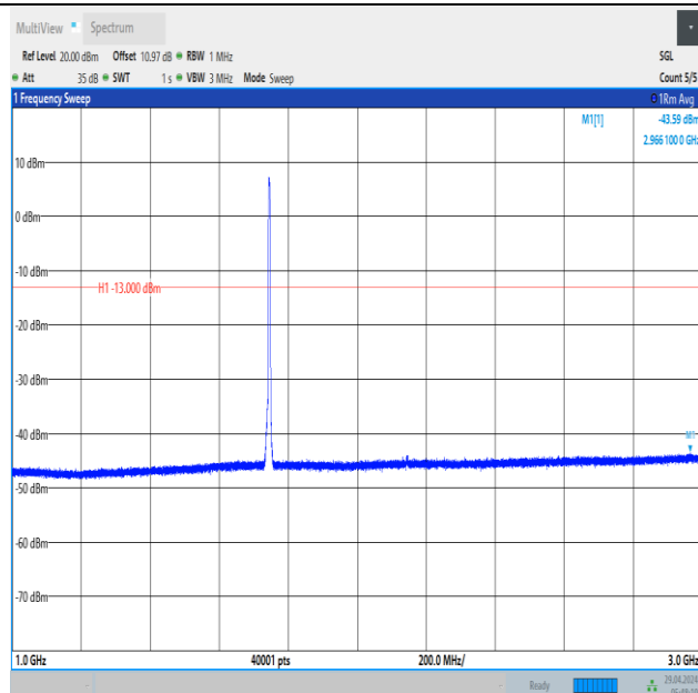
Band66_5MHz_16QAM_132322_25RB#0_1000~3000_1000~3000
