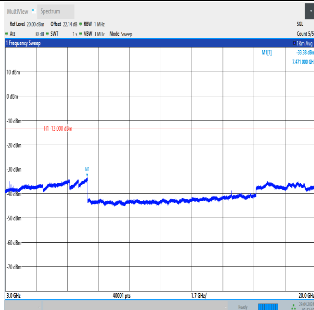
Band66_5MHz_QPSK_131997_25RB#0_3000~20000_3000~20000
