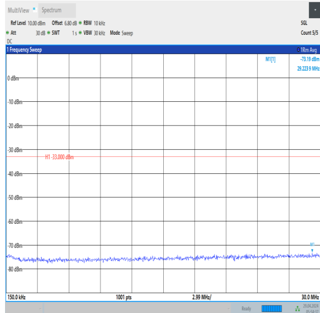
Band66_10MHz_16QAM_132022_1RB#0_0.15~30_0.15~30
