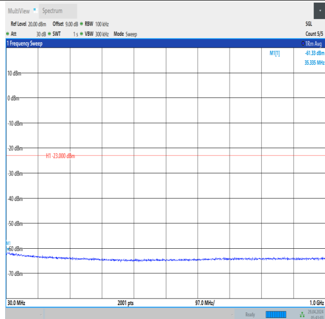
Band66_5MHz_16QAM_131997_25RB#0_30~1000_30~1000
