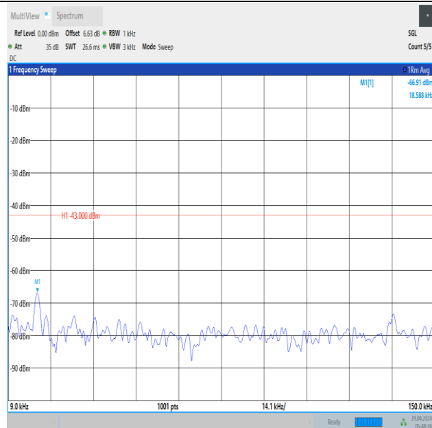
Band66_5MHz_QPSK_132647_1RB#0_0.009~0.15_0.009~0.15
