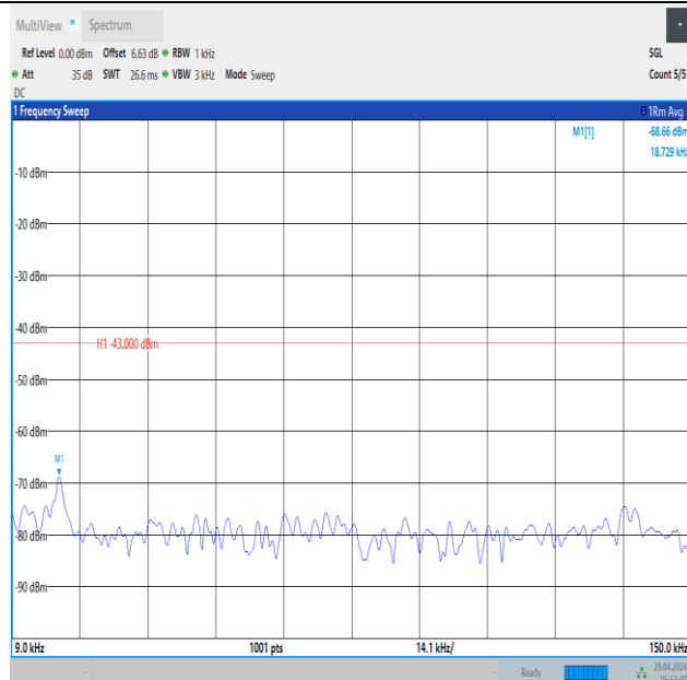
Band66_10MHz_QPSK_132022_1RB#0_0.009~0.15_0.009~0.15
