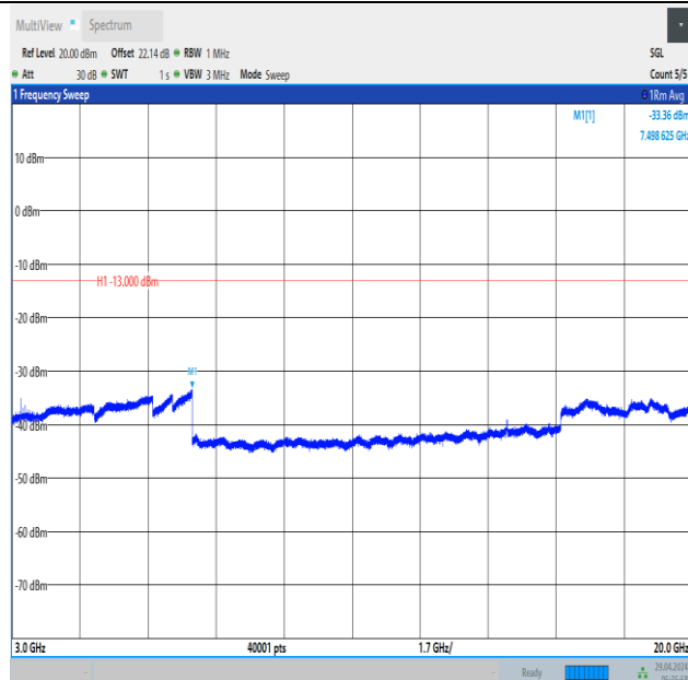
Band66_3MHz_QPSK_132657_1RB#14_3000~20000_3000~20000
