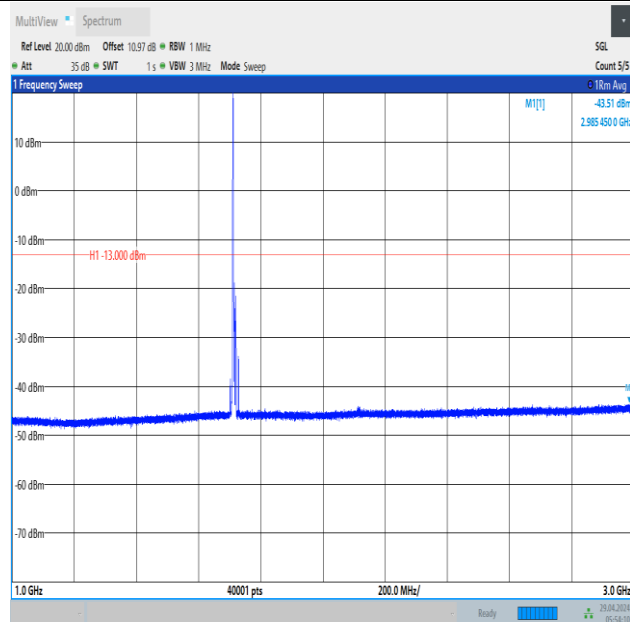
Band66_10MHz_QPSK_132022_1RB#0_1000~3000_1000~3000
