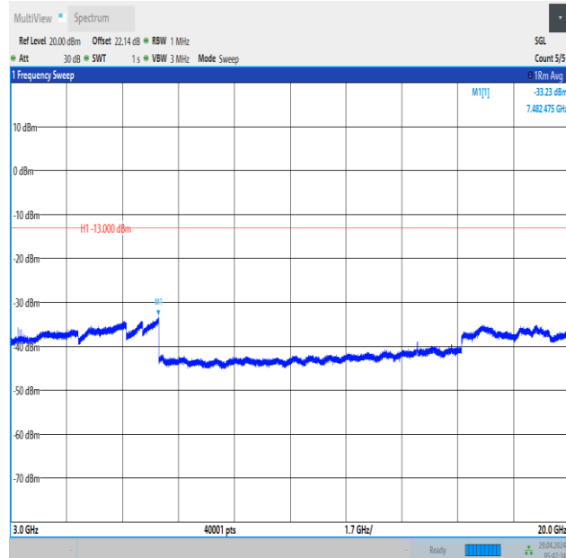
Band66_5MHz_QPSK_132322_25RB#0_3000~20000_3000~20000
