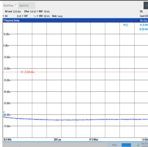
Band66_5MHz_QPSK_132322_1RB#0_30~1000_30~1000
