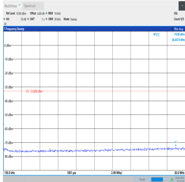
Band66_5MHz_16QAM_132322_25RB#0_0.15~30_0.15~30
