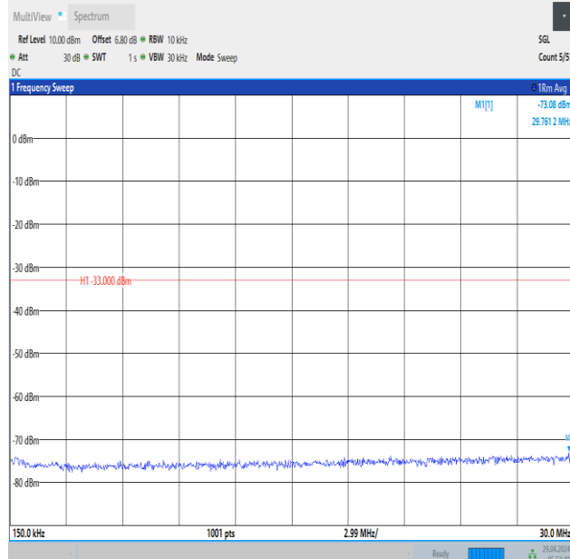
Band66_10MHz_QPSK_132022_1RB#0_0.15~30_0.15~30
