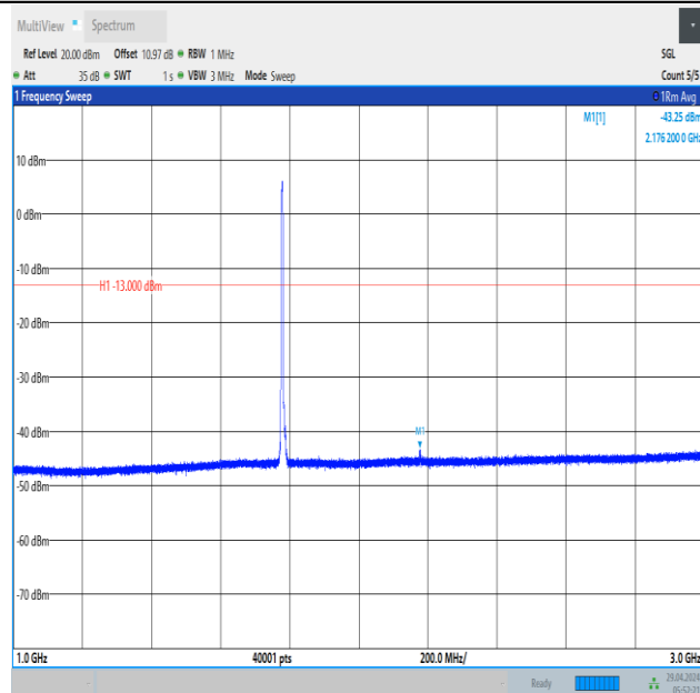
Band66_5MHz_QPSK_132647_25RB#0_1000~3000_1000~3000
