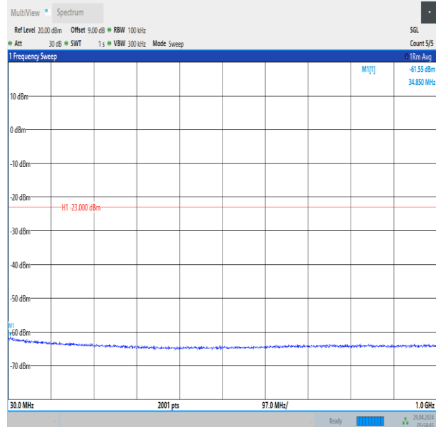
Band66_10MHz_16QAM_132022_1RB#0_30~1000_30~1000
