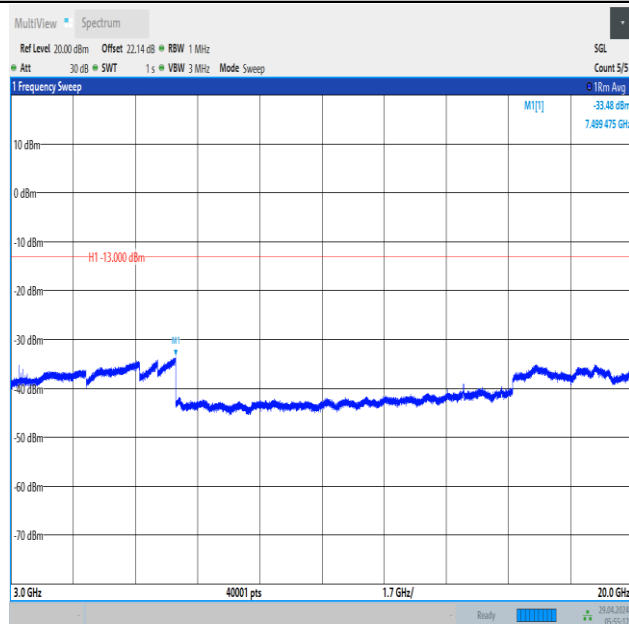
Band66_10MHz_16QAM_132022_1RB#0_3000~20000_3000~20000
