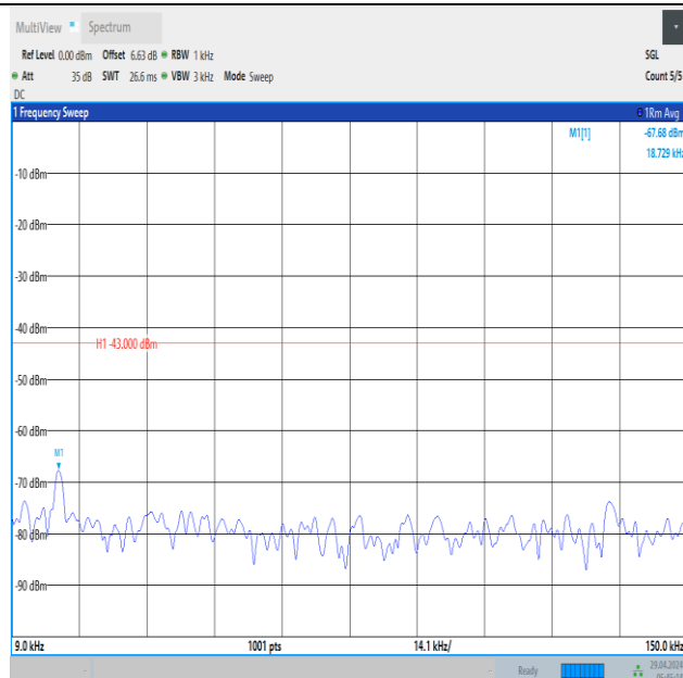
Band66_5MHz_QPSK_132322_1RB#24_0.009~0.15_0.009~0.15
