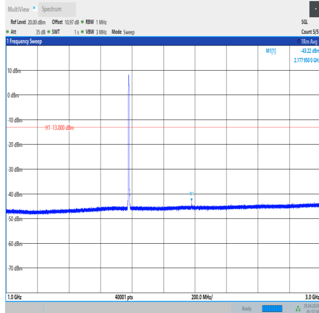
Band66_3MHz_QPSK_132657_15RB#0_1000~3000_1000~3000
