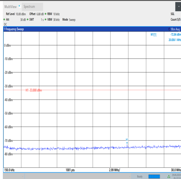
Band66_3MHz_16QAM_132657_15RB#0_0.15~30_0.15~30
