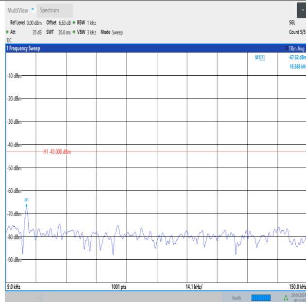
Band66_5MHz_16QAM_132647_1RB#24_0.009~0.15_0.009~0.15
