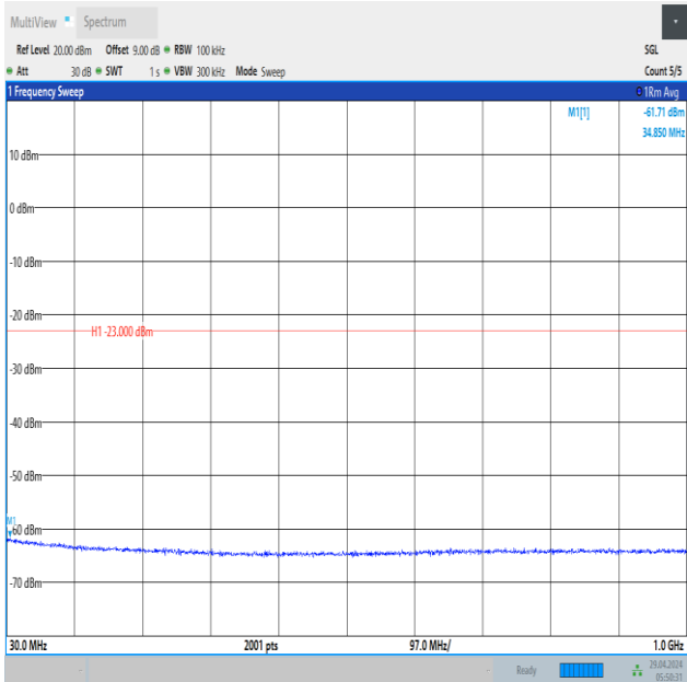
Band66_5MHz_QPSK_132647_1RB#24_30~1000_30~1000
