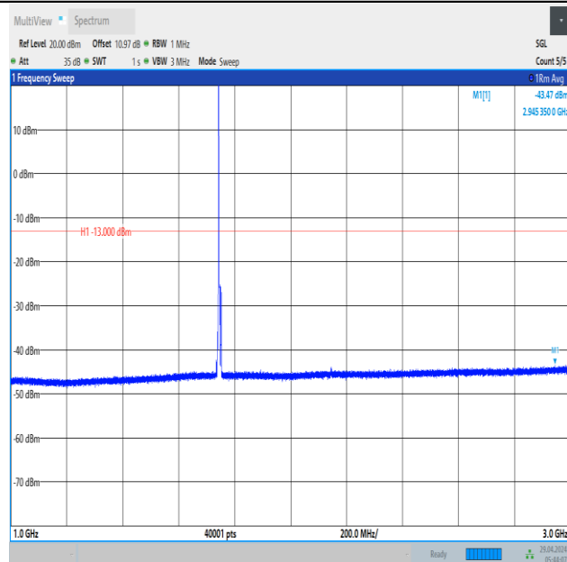
Band66_5MHz_QPSK_132322_1RB#0_1000~3000_1000~3000
