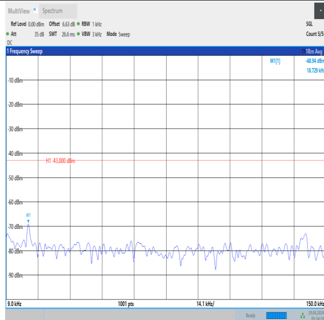
Band66_10MHz_16QAM_132022_1RB#0_0.009~0.15_0.009~0.15
