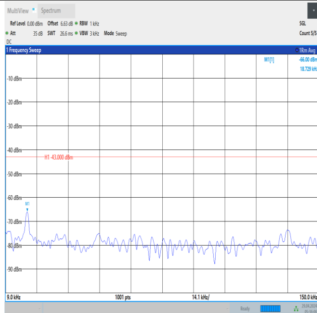
Band66_3MHz_16QAM_132657_1RB#14_0.009~0.15_0.009~0.15
