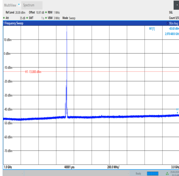
Band66_10MHz_QPSK_132022_1RB#49_1000~3000_1000~3000
