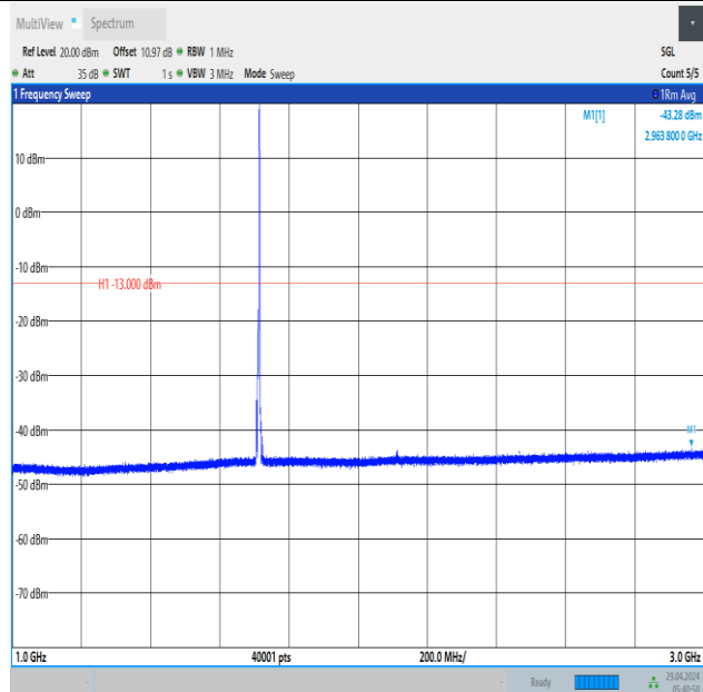
Band66_5MHz_QPSK_131997_1RB#24_1000~3000_1000~3000
