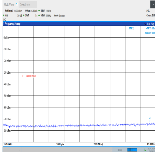
Band66_5MHz_QPSK_131997_1RB#0_0.15~30_0.15~30
