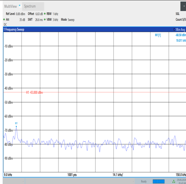
Band66_5MHz_16QAM_131997_25RB#0_0.009~0.15_0.009~0.15
