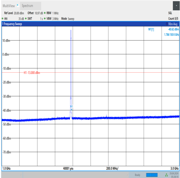
Band66_3MHz_16QAM_132657_15RB#0_1000~3000_1000~3000
