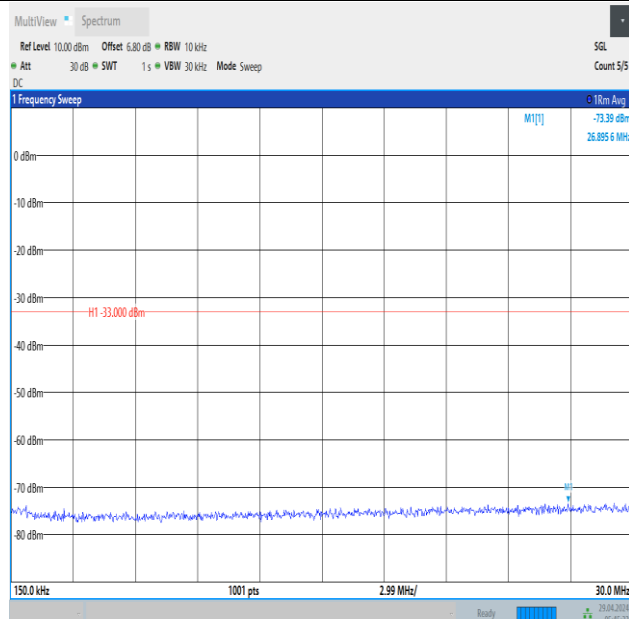
Band66_5MHz_QPSK_132322_1RB#24_0.15~30_0.15~30
