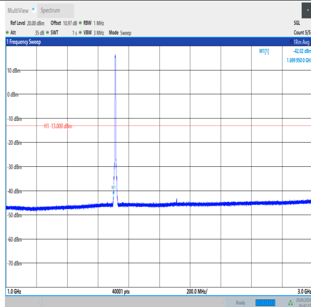
Band66_5MHz_QPSK_131997_25RB#0_1000~3000_1000~3000
