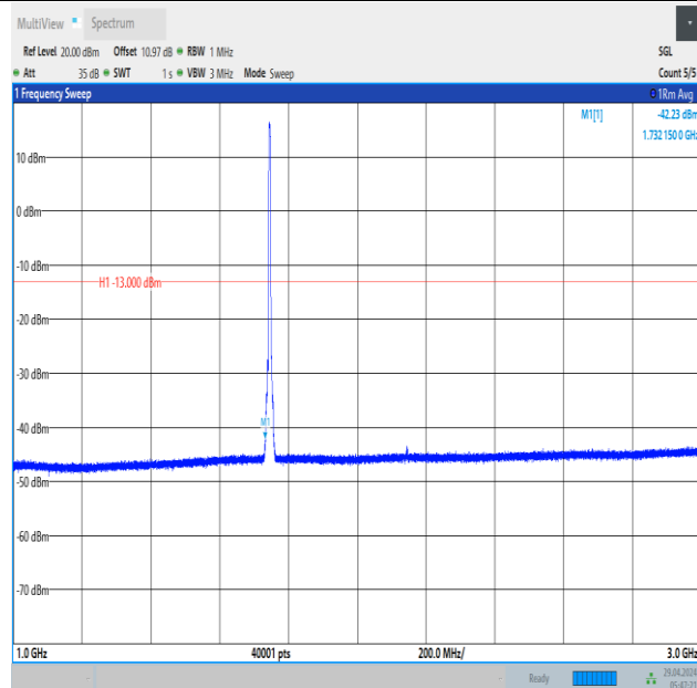
Band66_5MHz_QPSK_132322_25RB#0_1000~3000_1000~3000
