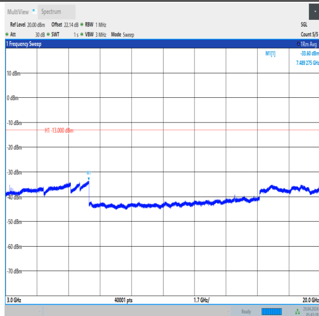
Band66_5MHz_16QAM_131997_25RB#0_3000~20000_3000~20000
