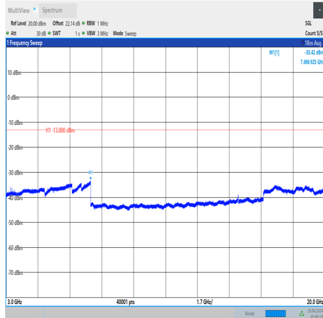
Band66_5MHz_QPSK_132647_1RB#0_3000~20000_3000~20000
