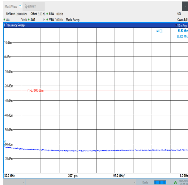
Band66_5MHz_16QAM_132647_1RB#24_30~1000_30~1000
