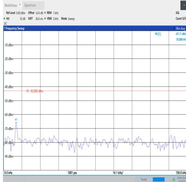
Band66_5MHz_16QAM_132647_1RB#0_0.009~0.15_0.009~0.15
