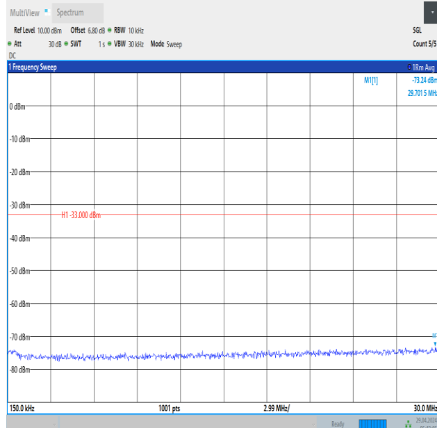
Band66_5MHz_QPSK_131997_25RB#0_0.15~30_0.15~30
