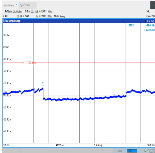
Band66_5MHz_16QAM_131997_1RB#0_3000~20000_3000~20000
