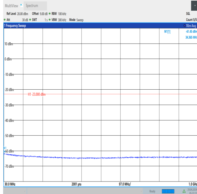
Band66_3MHz_QPSK_132657_15RB#0_30~1000_30~1000
