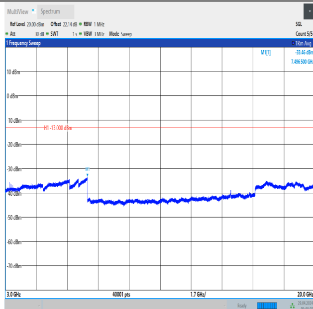
Band66_5MHz_QPSK_132322_1RB#0_3000~20000_3000~20000
