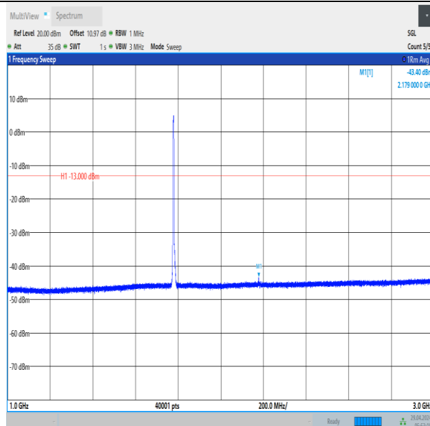
Band66_5MHz_16QAM_132647_25RB#0_1000~3000_1000~3000
