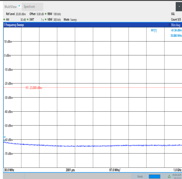
Band66_5MHz_16QAM_132647_25RB#0_30~1000_30~1000
