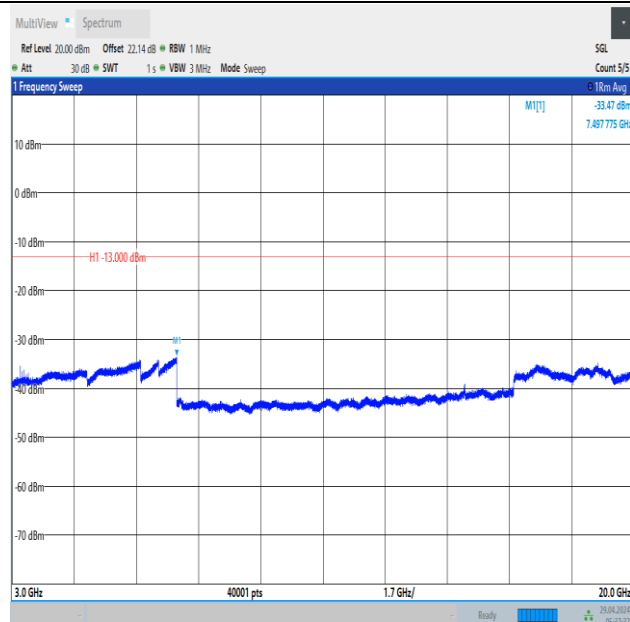
Band66_3MHz_QPSK_132657_15RB#0_3000~20000_3000~20000
