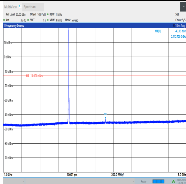
Band66_5MHz_QPSK_131997_1RB#0_1000~3000_1000~3000
