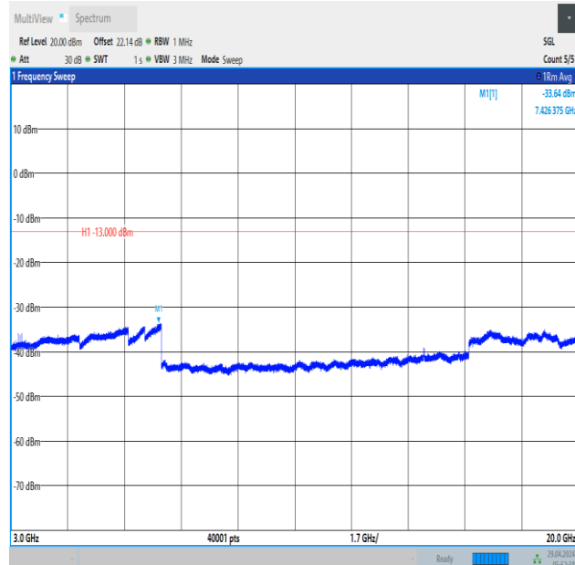
Band66_5MHz_QPSK_132647_25RB#0_3000~20000_3000~20000
