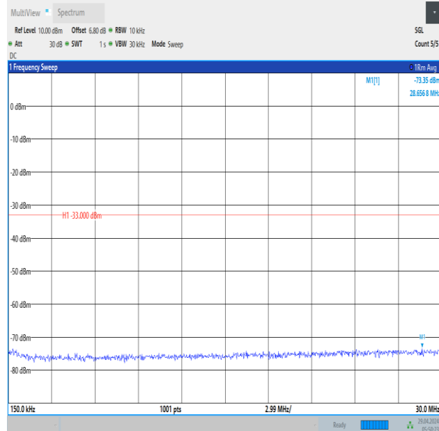
Band66_5MHz_QPSK_132647_1RB#24_0.15~30_0.15~30
