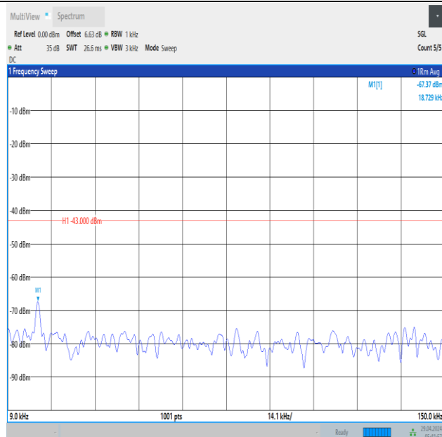
Band66_5MHz_QPSK_131997_25RB#0_0.009~0.15_0.009~0.15
