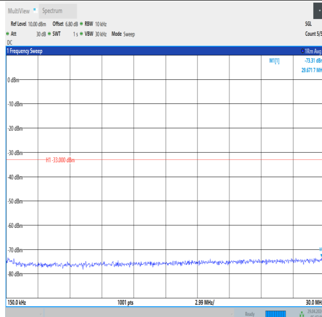
Band66_5MHz_QPSK_132322_25RB#0_0.15~30_0.15~30
