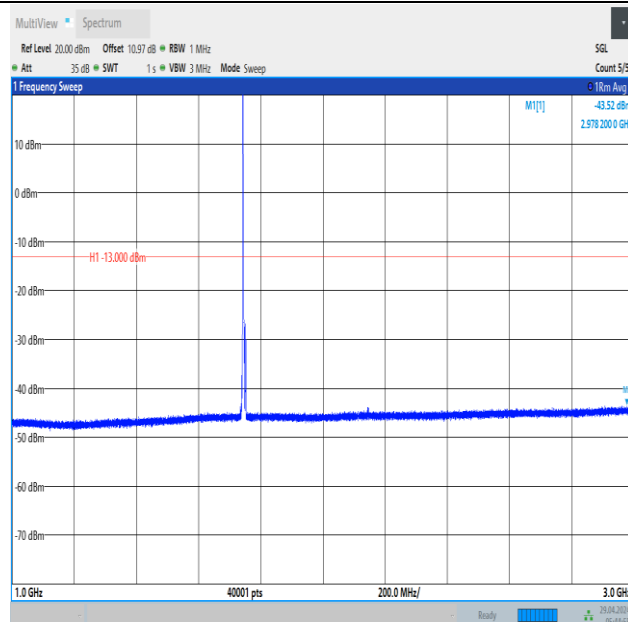
Band66_5MHz_16QAM_132322_1RB#0_1000~3000_1000~3000
