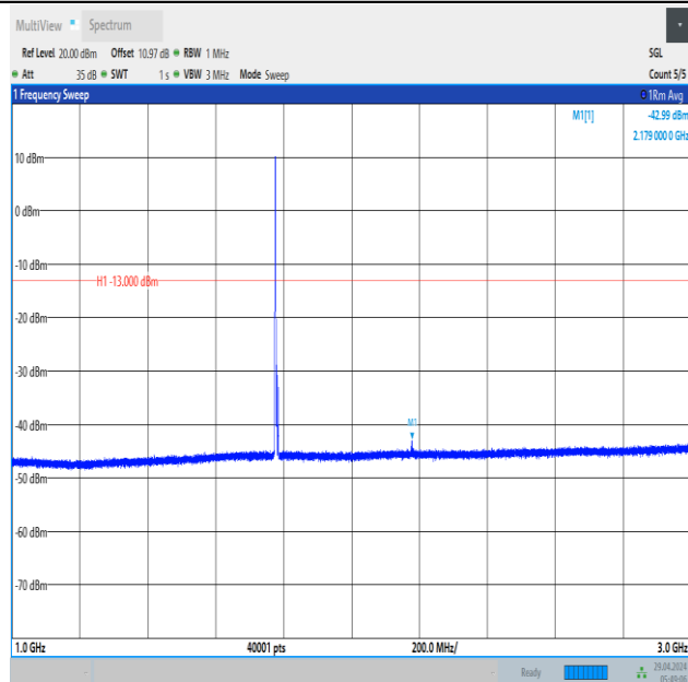
Band66_5MHz_QPSK_132647_1RB#0_1000~3000_1000~3000
