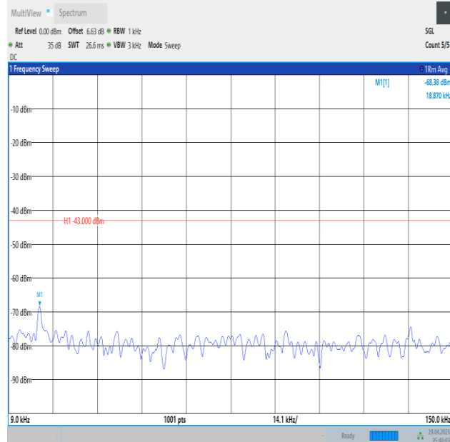
Band66_5MHz_16QAM_132322_1RB#24_0.009~0.15_0.009~0.15
