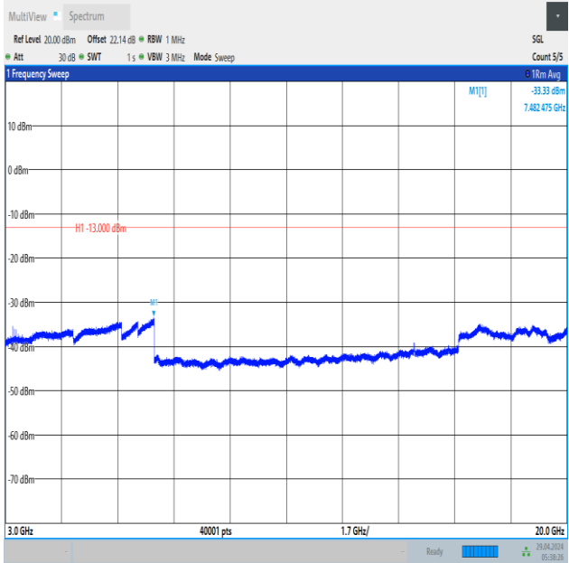
Band66_3MHz_16QAM_132657_15RB#0_3000~20000_3000~20000
