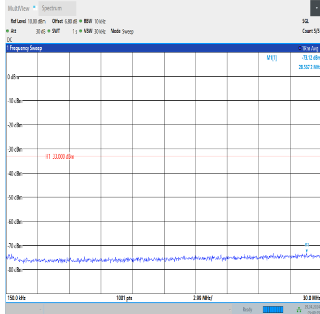
Band66_5MHz_QPSK_131997_1RB#24_0.15~30_0.15~30
