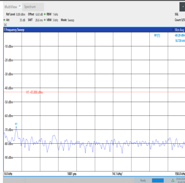
Band66_5MHz_QPSK_132322_1RB#0_0.009~0.15_0.009~0.15
