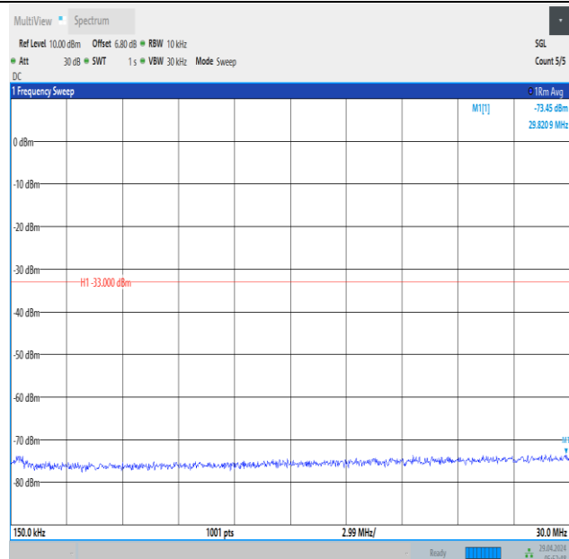
Band66_5MHz_16QAM_132647_25RB#0_0.15~30_0.15~30
