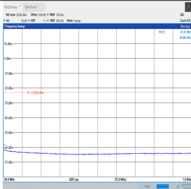
Band66_5MHz_QPSK_131997_1RB#0_30~1000_30~1000
