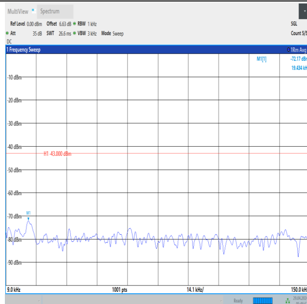
Band66_5MHz_QPSK_132322_25RB#0_0.009~0.15_0.009~0.15
