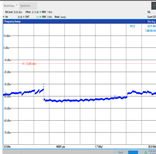
Band66_5MHz_QPSK_132647_1RB#24_3000~20000_3000~20000
