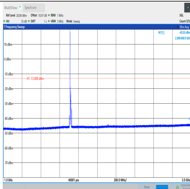
Band66_10MHz_16QAM_132022_1RB#0_1000~3000_1000~3000
