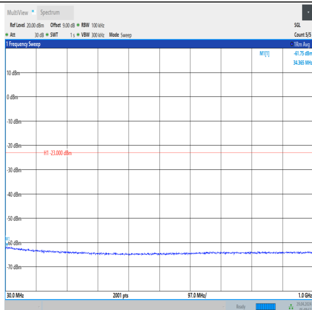
Band66_5MHz_QPSK_132647_1RB#0_30~1000_30~1000
