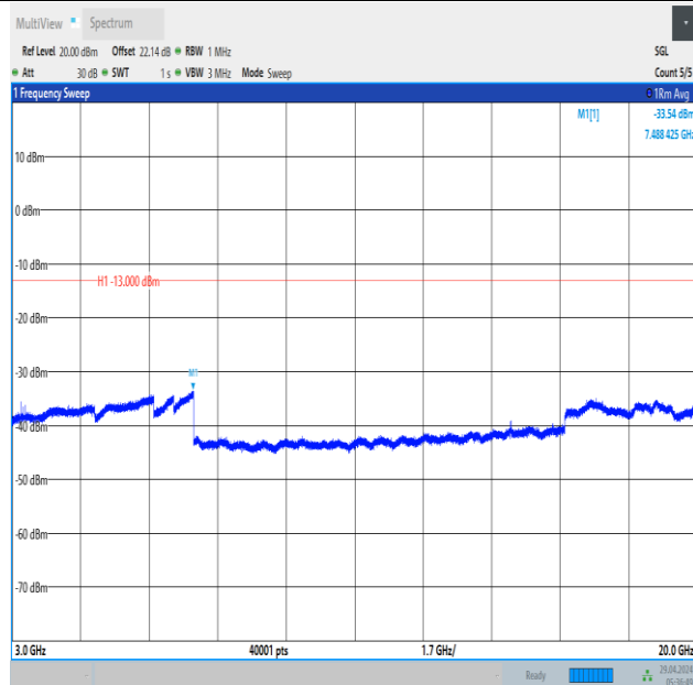
Band66_3MHz_16QAM_132657_1RB#14_3000~20000_3000~20000
