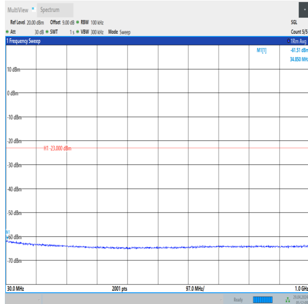
Band66_5MHz_QPSK_132647_25RB#0_30~1000_30~1000
