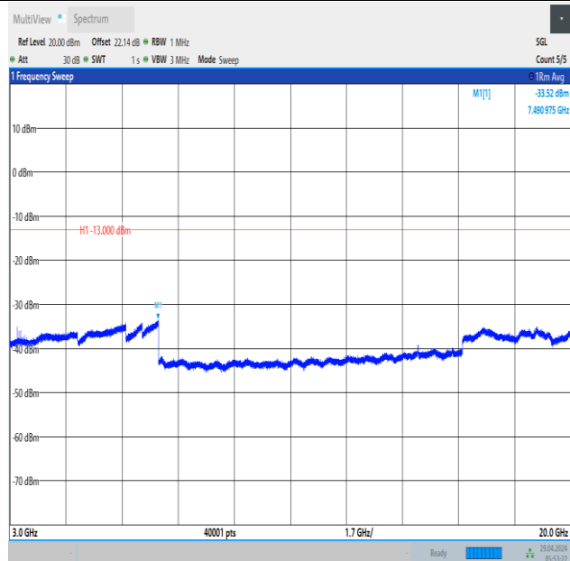
Band66_5MHz_16QAM_132647_25RB#0_3000~20000_3000~20000
