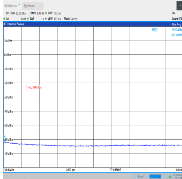
Band66_5MHz_QPSK_132322_25RB#0_30~1000_30~1000
