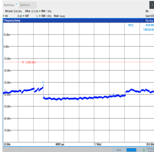
Band66_5MHz_QPSK_131997_1RB#0_3000~20000_3000~20000
