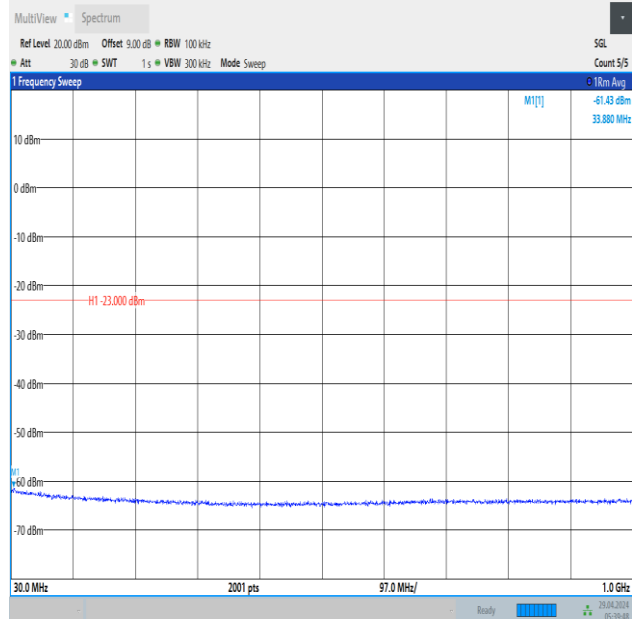
Band66_5MHz_16QAM_131997_1RB#0_30~1000_30~1000
