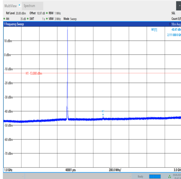
Band66_5MHz_16QAM_131997_1RB#24_1000~3000_1000~3000
