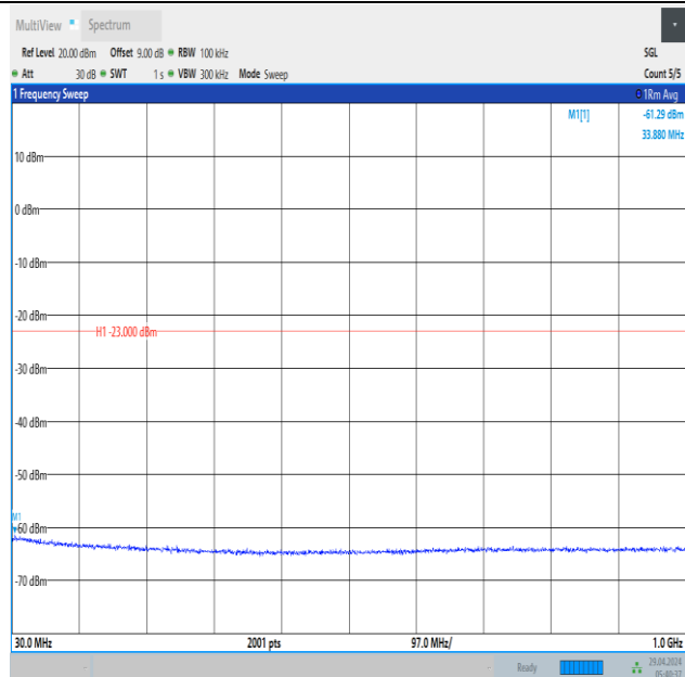
Band66_5MHz_QPSK_131997_1RB#24_30~1000_30~1000
