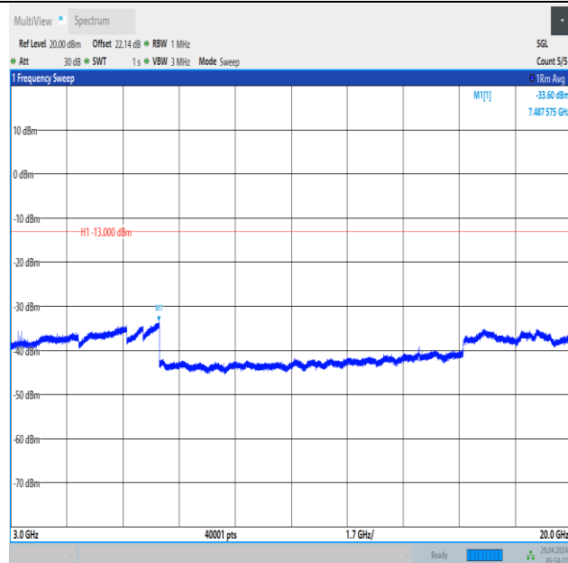
Band66_10MHz_QPSK_132022_1RB#0_3000~20000_3000~20000
