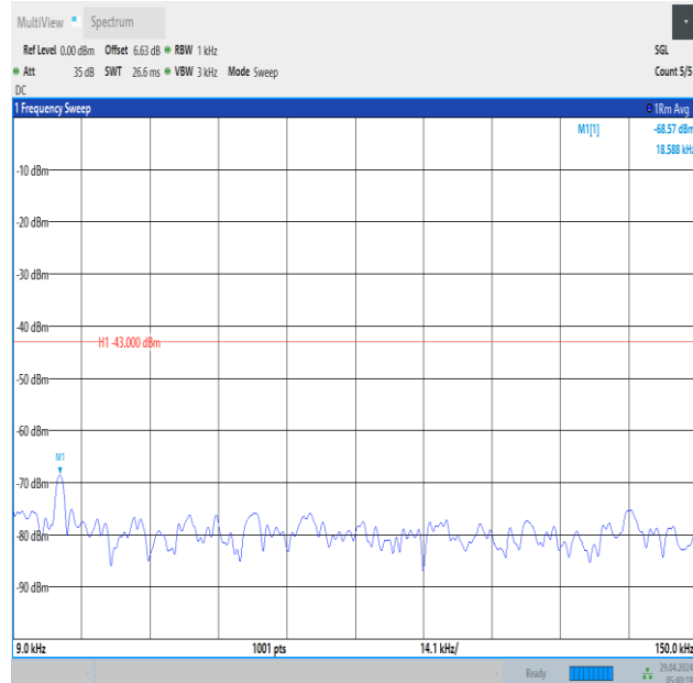
Band66_5MHz_QPSK_131997_1RB#24_0.009~0.15_0.009~0.15
