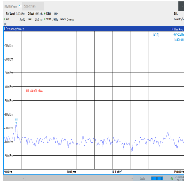
Band66_5MHz_16QAM_131997_1RB#24_0.009~0.15_0.009~0.15
