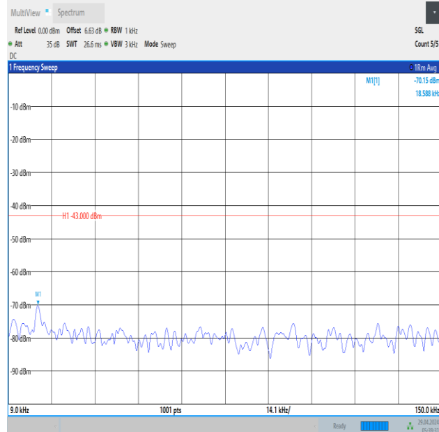
Band66_5MHz_16QAM_131997_1RB#0_0.009~0.15_0.009~0.15
