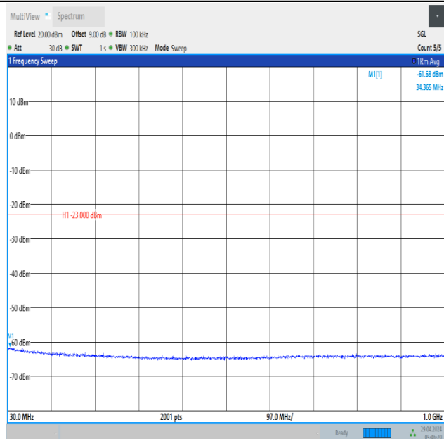
Band66_5MHz_16QAM_132322_1RB#24_30~1000_30~1000
