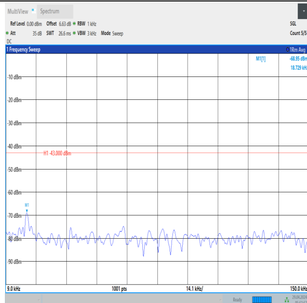
Band66_5MHz_QPSK_132647_25RB#0_0.009~0.15_0.009~0.15
