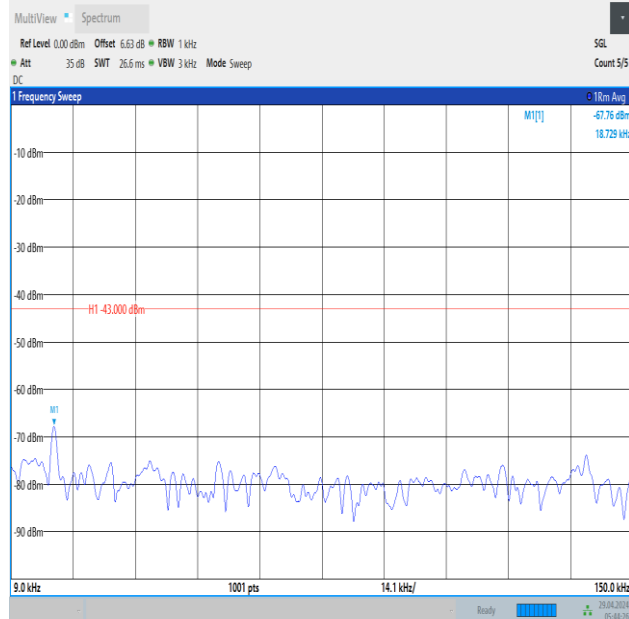
Band66_5MHz_16QAM_132322_1RB#0_0.009~0.15_0.009~0.15
