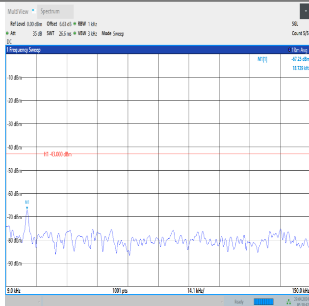
Band66_5MHz_QPSK_131997_1RB#0_0.009~0.15_0.009~0.15
