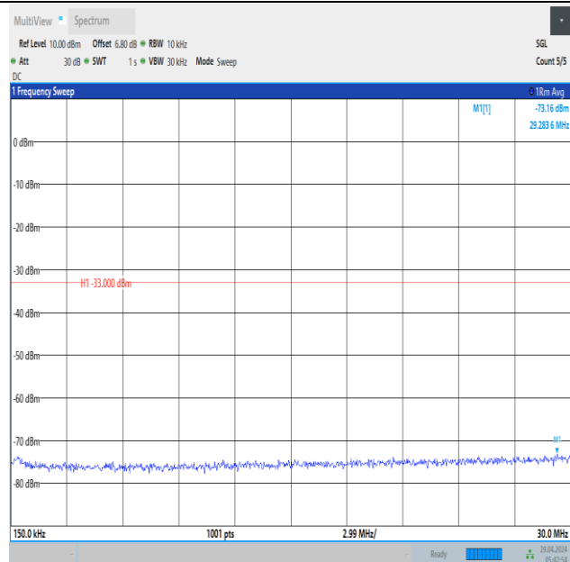
Band66_5MHz_16QAM_131997_25RB#0_0.15~30_0.15~30
