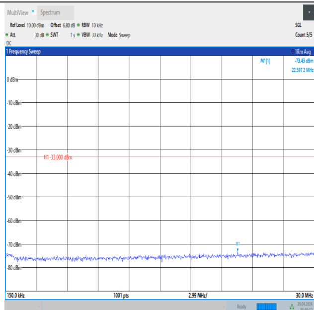
Band66_5MHz_16QAM_132322_1RB#24_0.15~30_0.15~30
