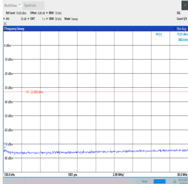
Band66_5MHz_16QAM_131997_1RB#0_0.15~30_0.15~30
