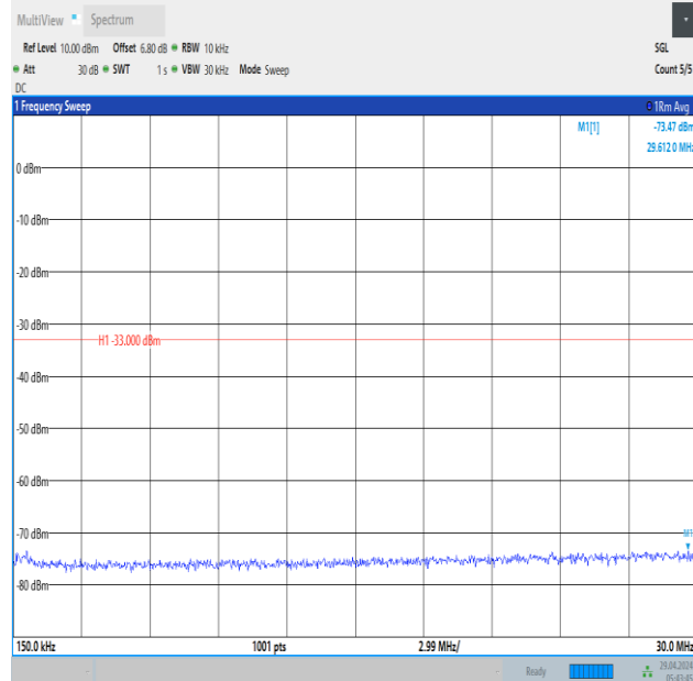
Band66_5MHz_QPSK_132322_1RB#0_0.15~30_0.15~30
