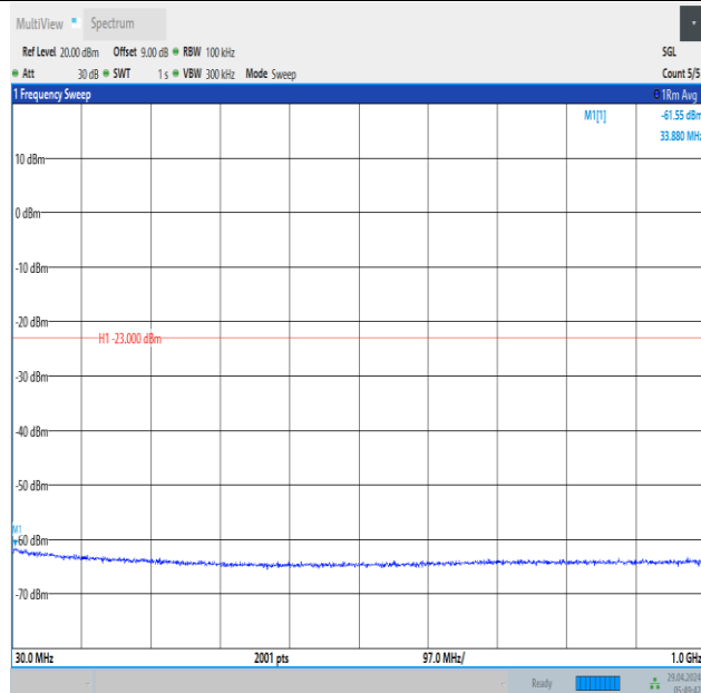
Band66_5MHz_16QAM_132647_1RB#0_30~1000_30~1000
