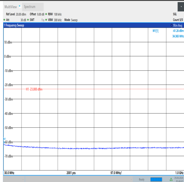
Band66_5MHz_16QAM_132322_1RB#0_30~1000_30~1000
