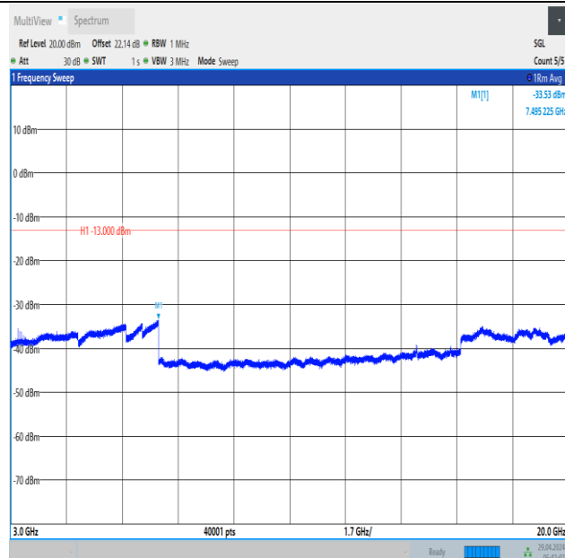
Band66_5MHz_QPSK_131997_1RB#24_3000~20000_3000~20000
