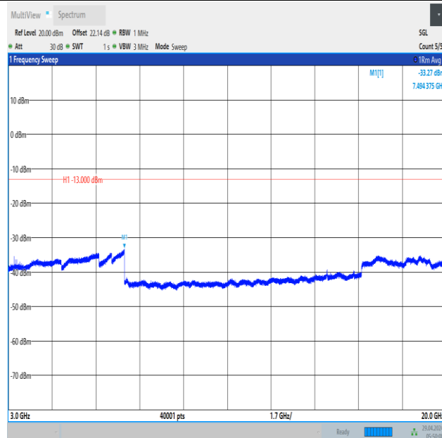
Band66_5MHz_16QAM_132647_1RB#0_3000~20000_3000~20000
