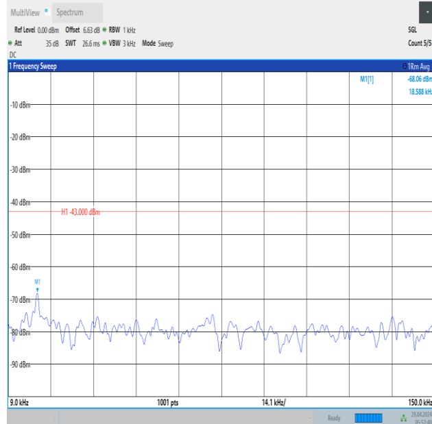
Band66_5MHz_16QAM_132647_25RB#0_0.009~0.15_0.009~0.15
