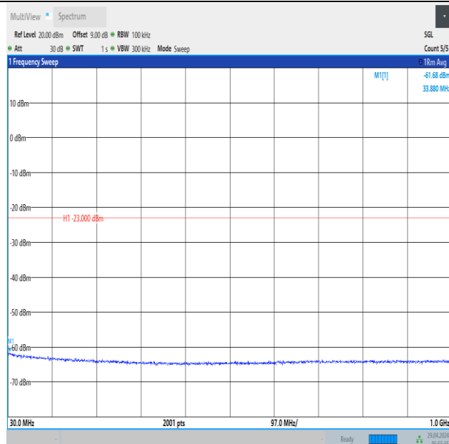
Band66_10MHz_QPSK_132022_1RB#49_30~1000_30~1000
