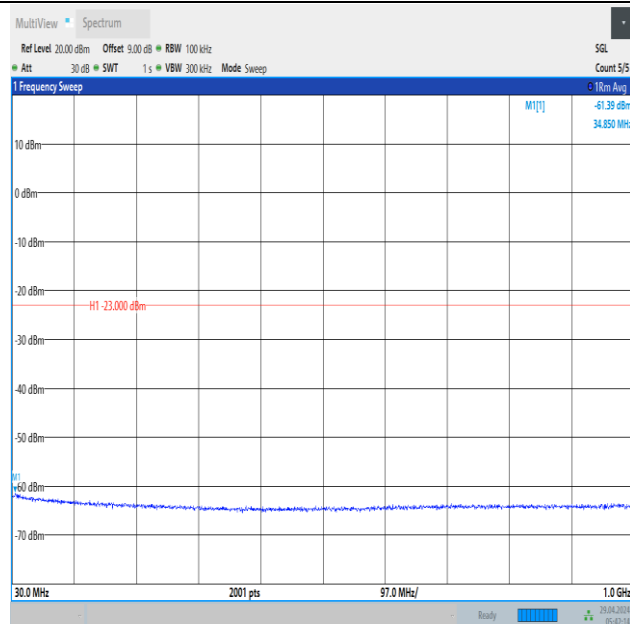
Band66_5MHz_QPSK_131997_25RB#0_30~1000_30~1000
