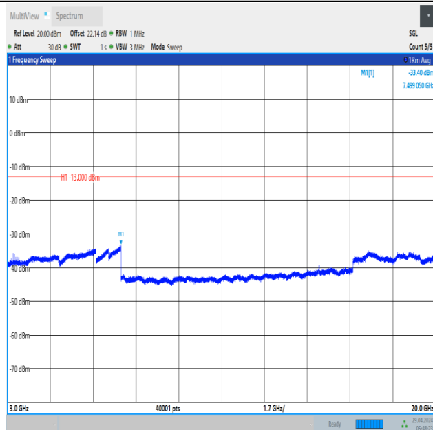
Band66_5MHz_16QAM_132322_25RB#0_3000~20000_3000~20000
