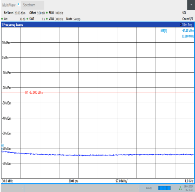
Band66_3MHz_16QAM_132657_1RB#14_30~1000_30~1000
