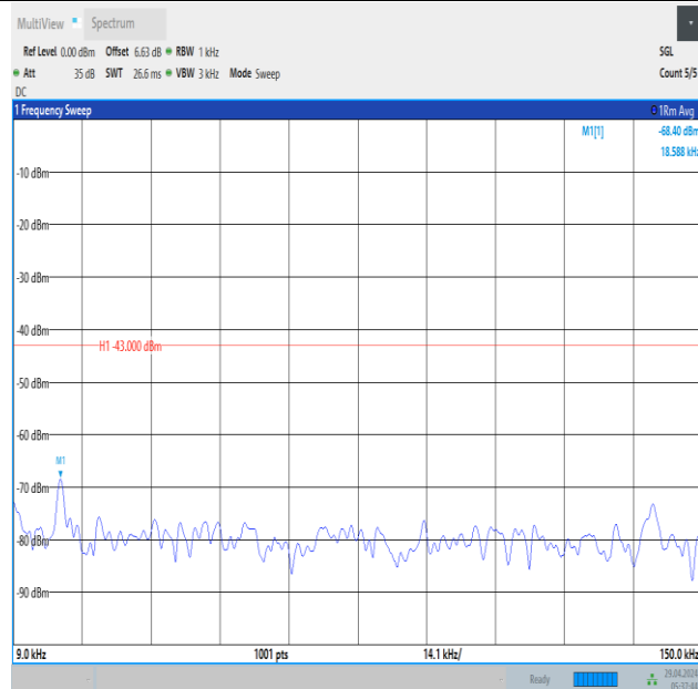
Band66_3MHz_16QAM_132657_15RB#0_0.009~0.15_0.009~0.15
