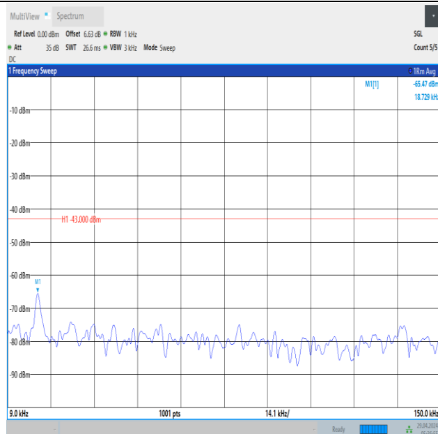
Band66_3MHz_QPSK_132657_15RB#0_0.009~0.15_0.009~0.15
