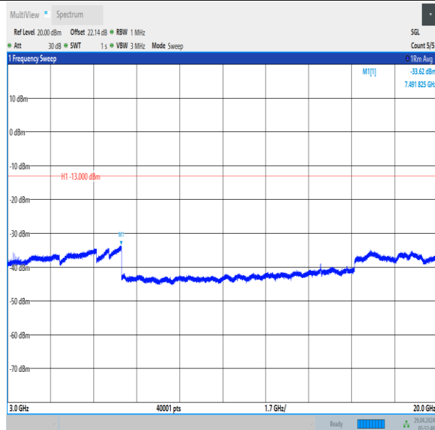
Band66_5MHz_16QAM_132647_1RB#24_3000~20000_3000~20000
