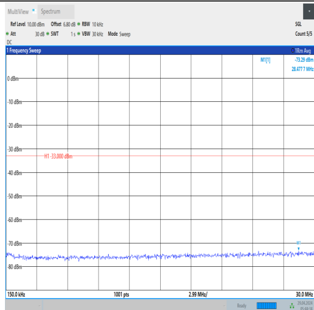
Band66_5MHz_16QAM_132322_1RB#0_0.15~30_0.15~30
