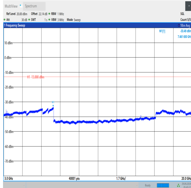
Band66_5MHz_QPSK_132322_1RB#24_3000~20000_3000~20000
