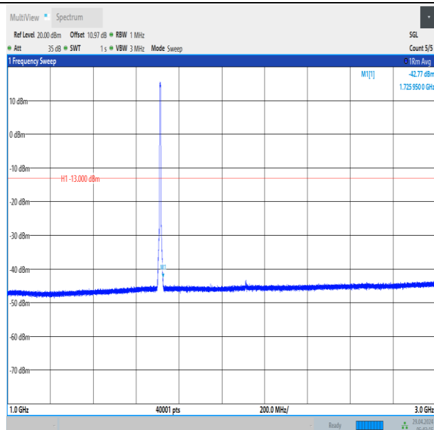
Band66_5MHz_16QAM_131997_25RB#0_1000~3000_1000~3000
