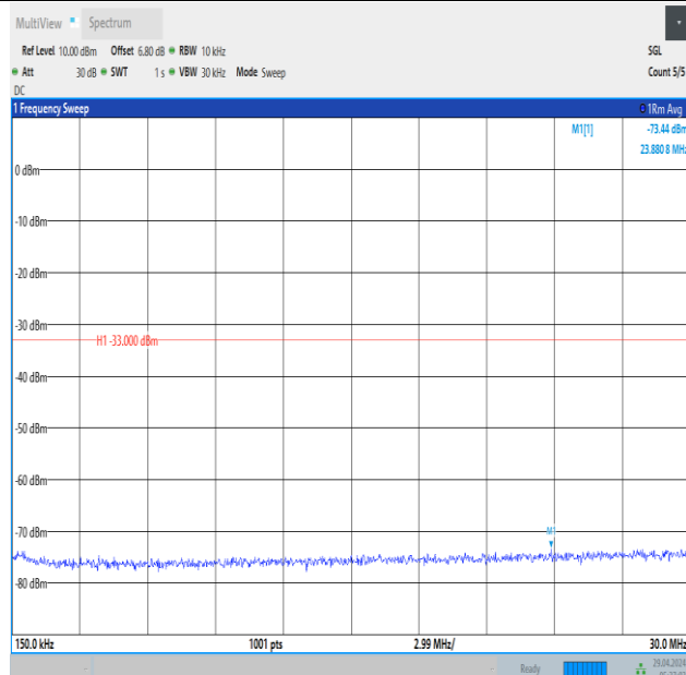
Band66_3MHz_QPSK_132657_15RB#0_0.15~30_0.15~30
