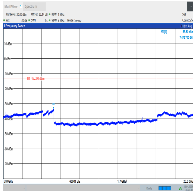
Band66_5MHz_16QAM_132322_1RB#24_3000~20000_3000~20000
