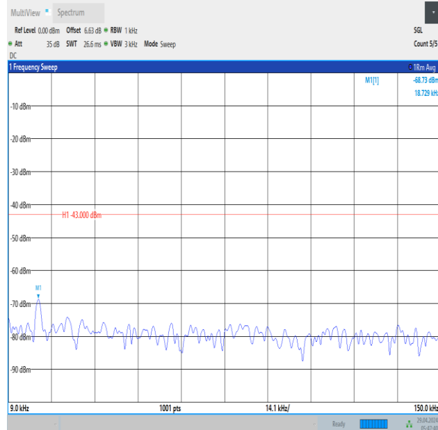
Band66_5MHz_16QAM_132322_25RB#0_0.009~0.15_0.009~0.15
