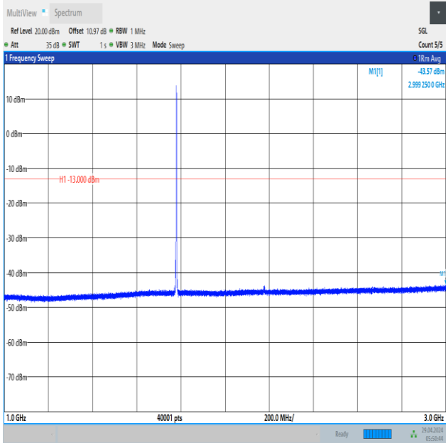
Band66_5MHz_QPSK_132647_1RB#24_1000~3000_1000~3000
