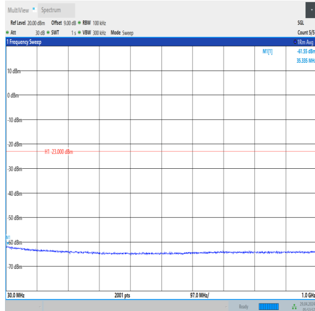
Band66_10MHz_QPSK_132022_1RB#0_30~1000_30~1000
