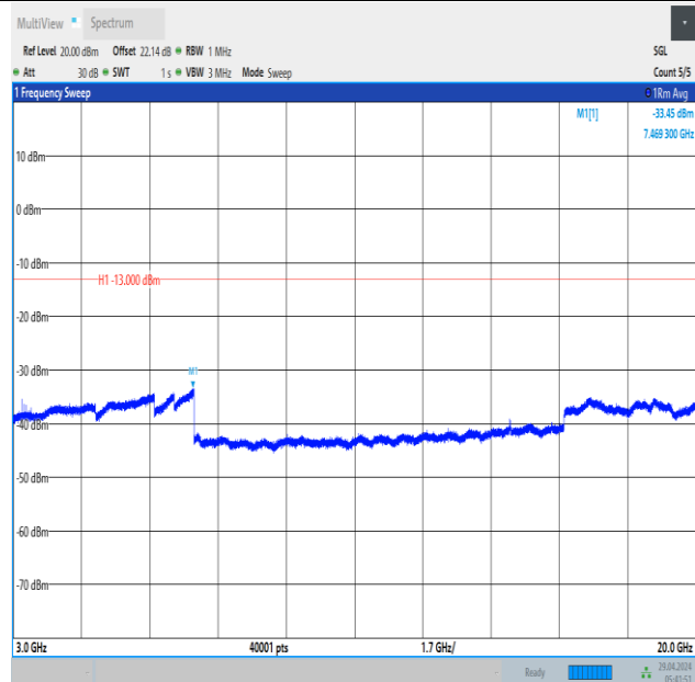
Band66_5MHz_16QAM_131997_1RB#24_3000~20000_3000~20000
