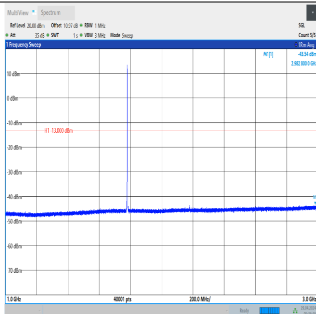
Band66_3MHz_16QAM_132657_1RB#14_1000~3000_1000~3000
