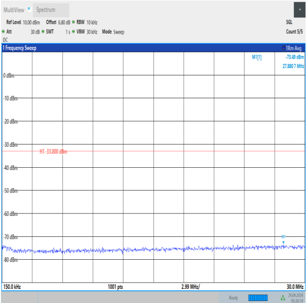
Band66_3MHz_16QAM_132657_1RB#14_0.15~30_0.15~30
