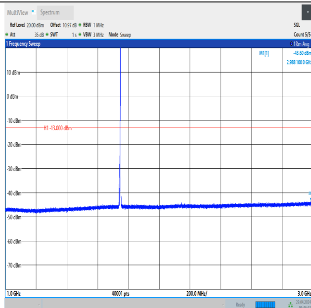
Band66_5MHz_16QAM_132322_1RB#24_1000~3000_1000~3000
