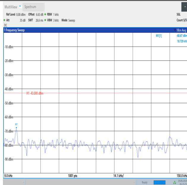
Band66_3MHz_QPSK_131987_1RB#14_0.009~0.15_0.009~0.15
