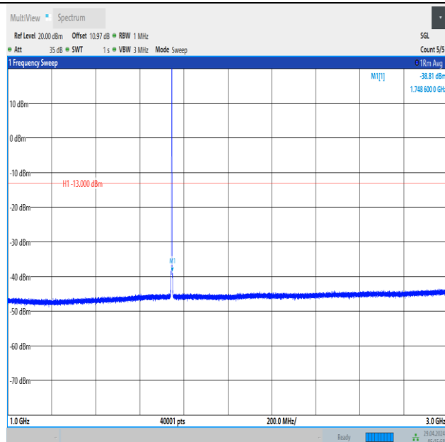
Band66_1.4MHz_16QAM_132322_1RB#5_1000~3000_1000~3000
