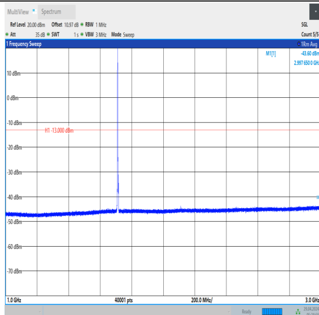
Band66_3MHz_16QAM_131987_1RB#0_1000~3000_1000~3000
