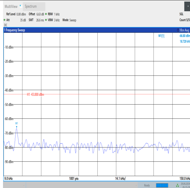
Band66_1.4MHz_16QAM_132322_1RB#5_0.009~0.15_0.009~0.15
