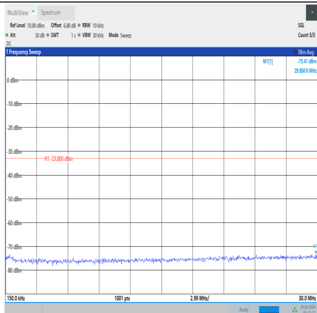
Band66_3MHz_16QAM_132322_1RB#14_0.15~30_0.15~30
