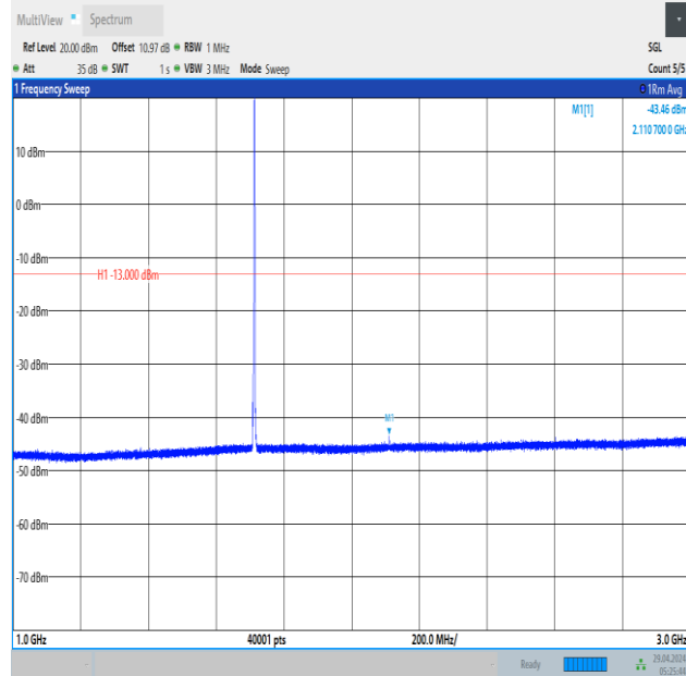
Band66_3MHz_QPSK_131987_1RB#14_1000~3000_1000~3000
