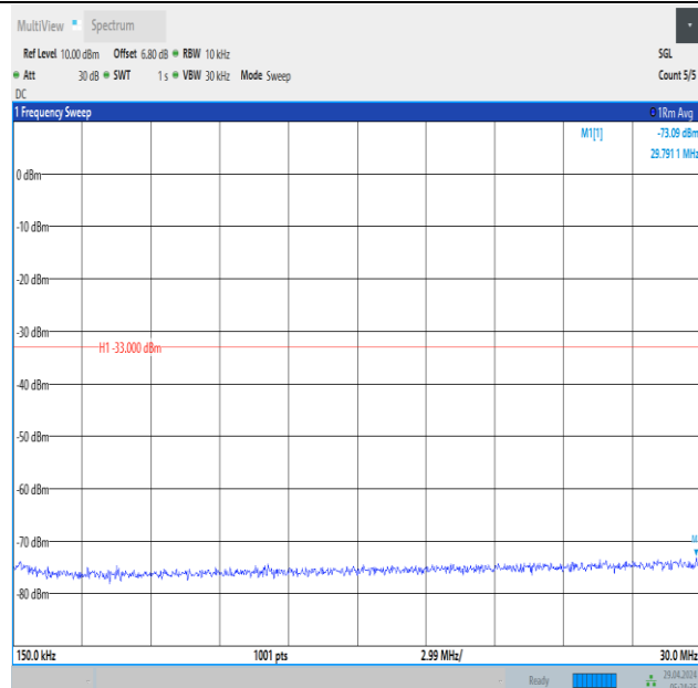
Band66_3MHz_16QAM_131987_1RB#0_0.15~30_0.15~30
