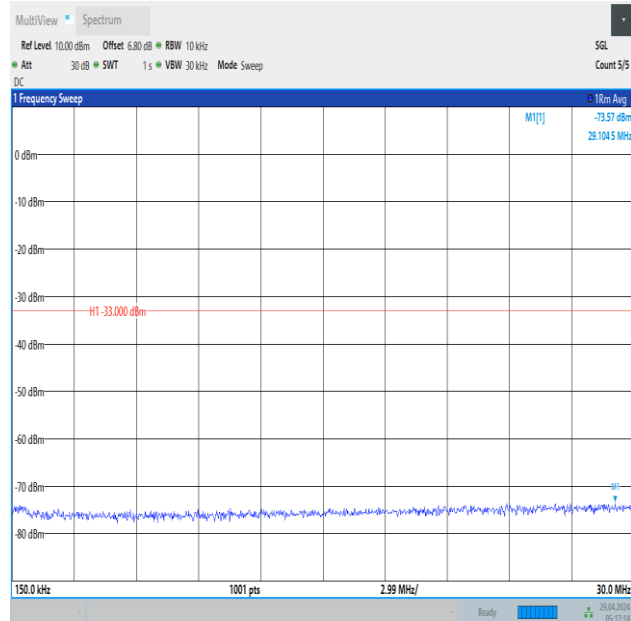
Band66_1.4MHz_16QAM_132322_6RB#0_0.15~30_0.15~30
