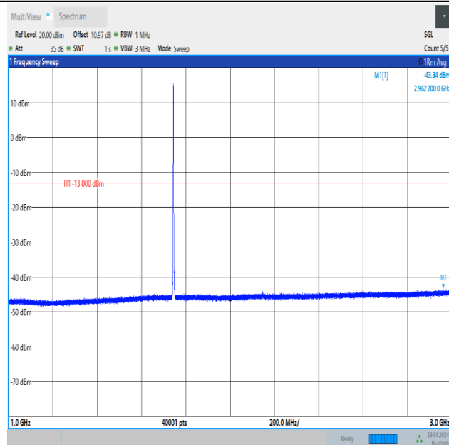
Band66_3MHz_QPSK_132322_1RB#0_1000~3000_1000~3000
