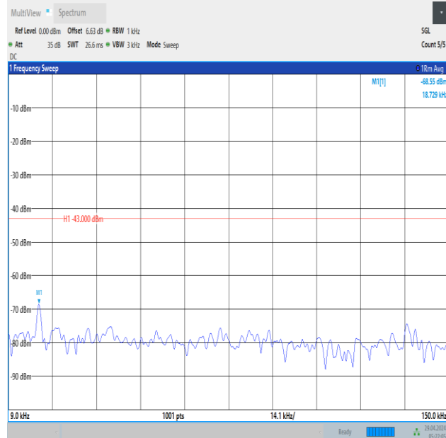
Band66_1.4MHz_16QAM_132665_6RB#0_0.009~0.15_0.009~0.15
