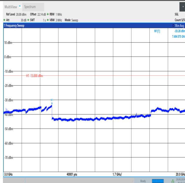
Band66_1.4MHz_QPSK_132322_1RB#5_3000~20000_3000~20000
