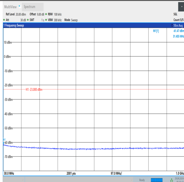
Band66_3MHz_QPSK_132657_1RB#14_30~1000_30~1000
