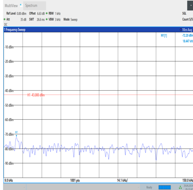
Band66_3MHz_16QAM_132322_15RB#0_0.009~0.15_0.009~0.15
