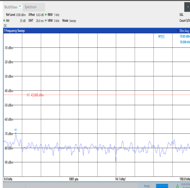
Band66_1.4MHz_QPSK_132665_1RB#0_0.009~0.15_0.009~0.15
