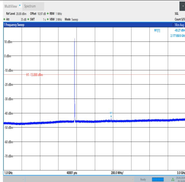
Band66_3MHz_QPSK_132657_1RB#0_1000~3000_1000~3000
