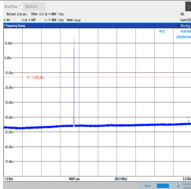
Band66_3MHz_QPSK_132322_1RB#14_1000~3000_1000~3000
