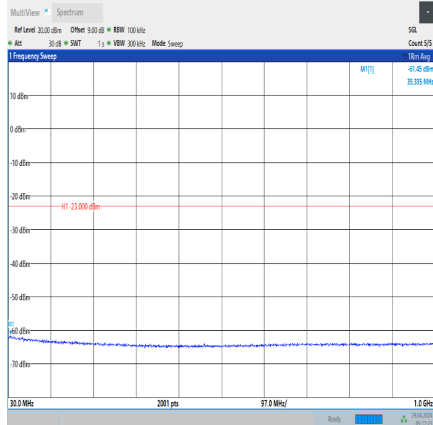
Band66_1.4MHz_16QAM_132322_6RB#0_30~1000_30~1000
