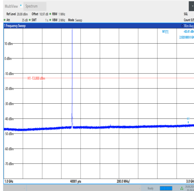
Band66_3MHz_16QAM_131987_1RB#14_1000~3000_1000~3000
