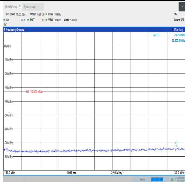
Band66_3MHz_16QAM_132657_1RB#0_0.15~30_0.15~30
