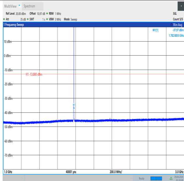
Band66_1.4MHz_QPSK_132665_1RB#5_1000~3000_1000~3000
