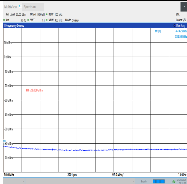
Band66_3MHz_16QAM_132322_1RB#14_30~1000_30~1000
