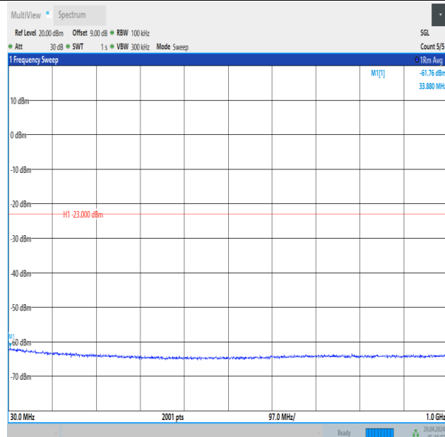
Band66_1.4MHz_16QAM_132665_1RB#0_30~1000_30~1000
