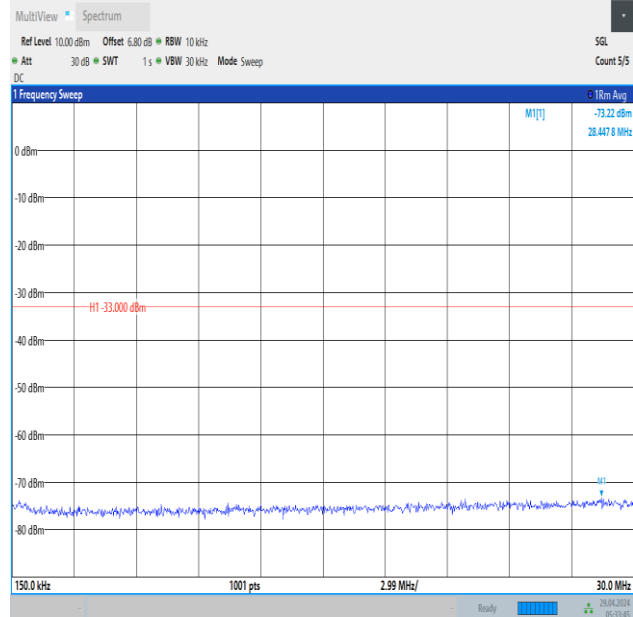
Band66_3MHz_QPSK_132657_1RB#0_0.15~30_0.15~30
