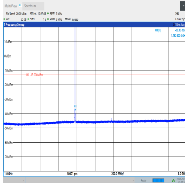
Band66_1.4MHz_16QAM_132665_1RB#5_1000~3000_1000~3000
