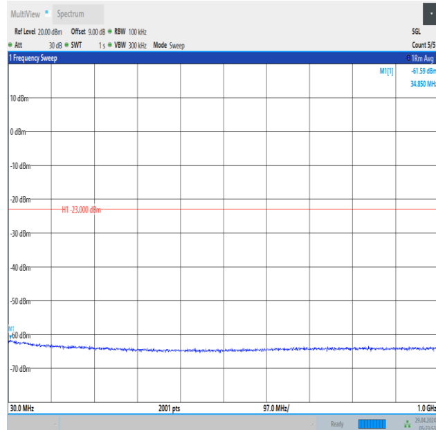
Band66_3MHz_QPSK_131987_1RB#0_30~1000_30~1000
