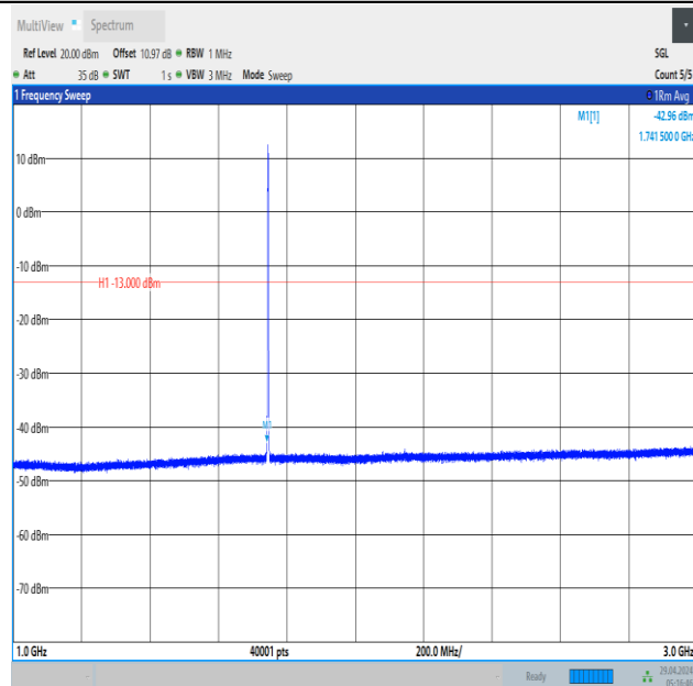
Band66_1.4MHz_QPSK_132322_6RB#0_1000~3000_1000~3000
