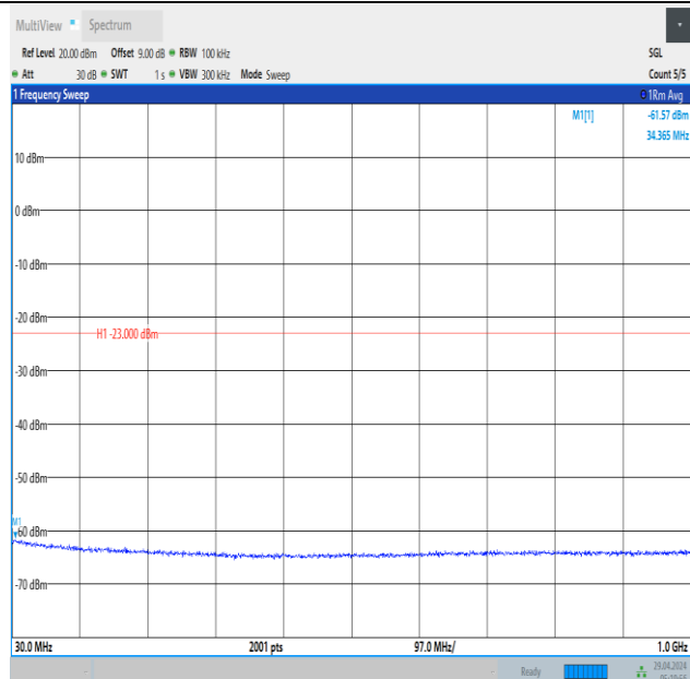
Band66_1.4MHz_QPSK_132665_1RB#5_30~1000_30~1000
