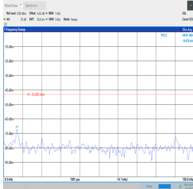
Band66_3MHz_16QAM_132657_1RB#0_0.009~0.15_0.009~0.15
