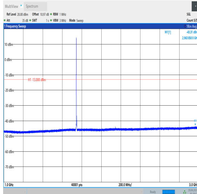
Band66_3MHz_16QAM_132322_1RB#0_1000~3000_1000~3000
