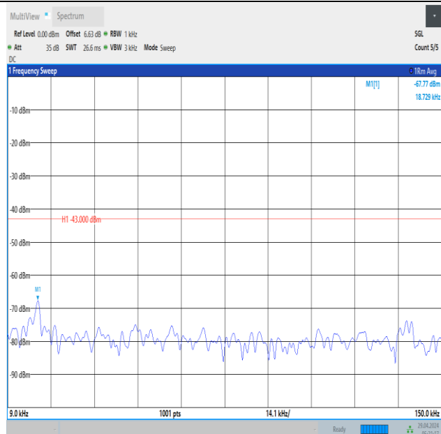
Band66_1.4MHz_QPSK_132665_6RB#0_0.009~0.15_0.009~0.15
