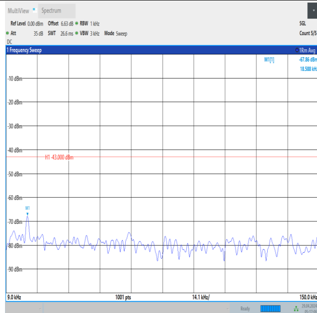
Band66_1.4MHz_16QAM_132322_6RB#0_0.009~0.15_0.009~0.15
