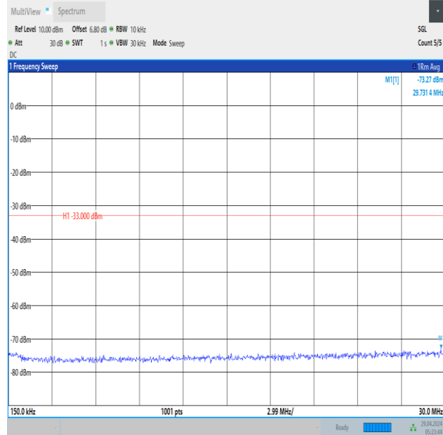
Band66_3MHz_QPSK_131987_1RB#0_0.15~30_0.15~30
