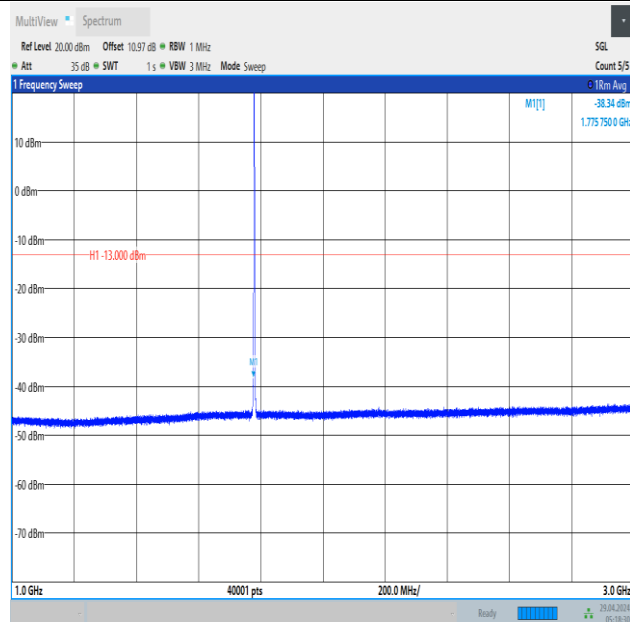
Band66_1.4MHz_QPSK_132665_1RB#0_1000~3000_1000~3000
