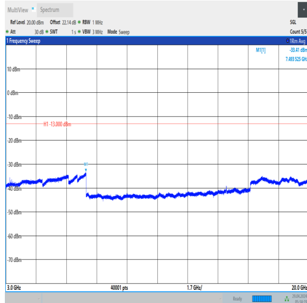
Band66_3MHz_QPSK_132657_1RB#0_3000~20000_3000~20000
