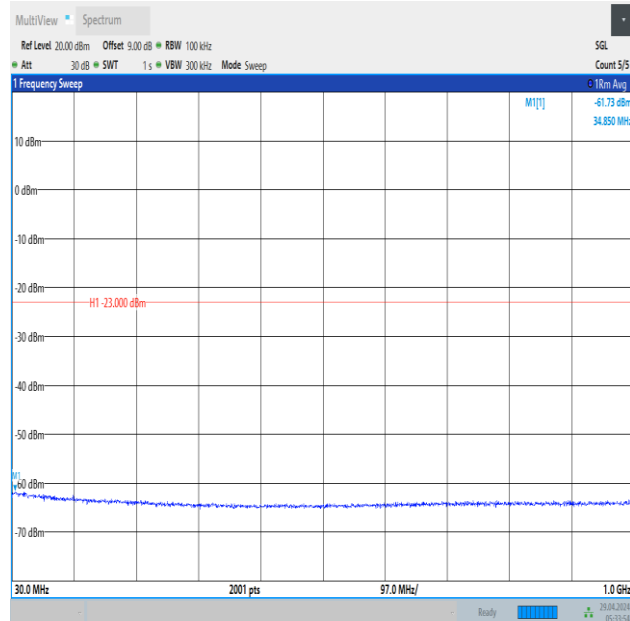
Band66_3MHz_QPSK_132657_1RB#0_30~1000_30~1000
