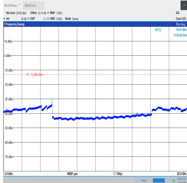
Band66_3MHz_16QAM_131987_1RB#14_3000~20000_3000~20000
