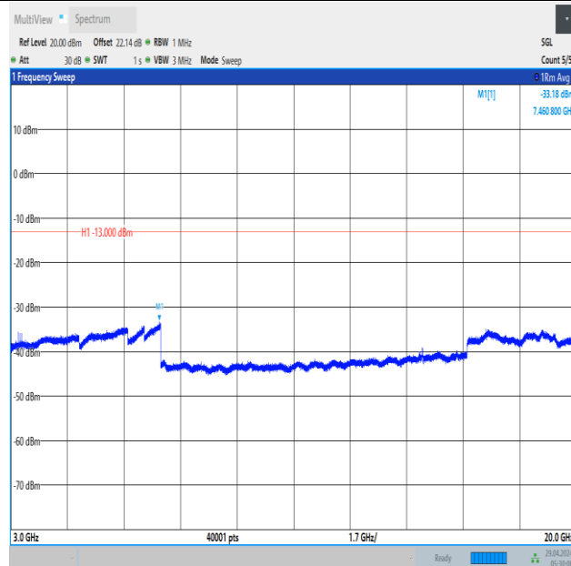
Band66_3MHz_16QAM_132322_1RB#0_3000~20000_3000~20000
