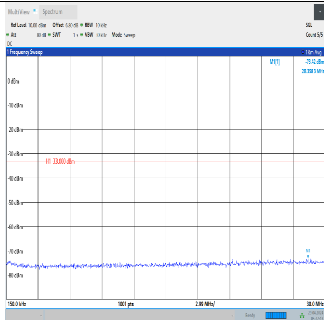
Band66_1.4MHz_16QAM_132665_6RB#0_0.15~30_0.15~30
