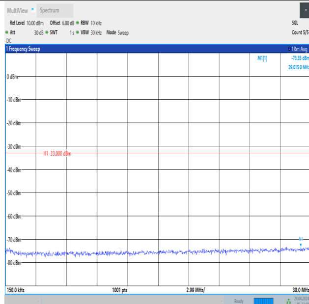
Band66_3MHz_QPSK_132322_15RB#0_0.15~30_0.15~30
