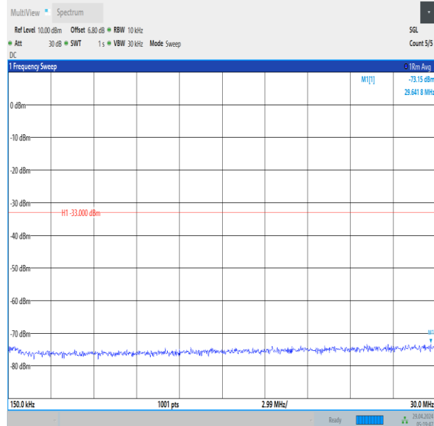
Band66_1.4MHz_QPSK_132665_1RB#5_0.15~30_0.15~30
