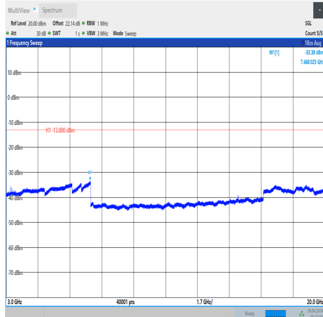
Band66_3MHz_QPSK_131987_15RB#0_3000~20000_3000~20000
