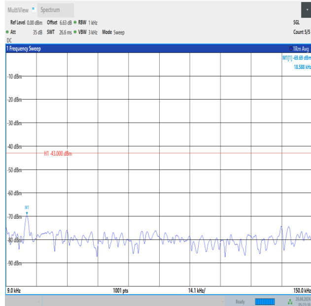
Band66_3MHz_QPSK_131987_1RB#0_0.009~0.15_0.009~0.15
