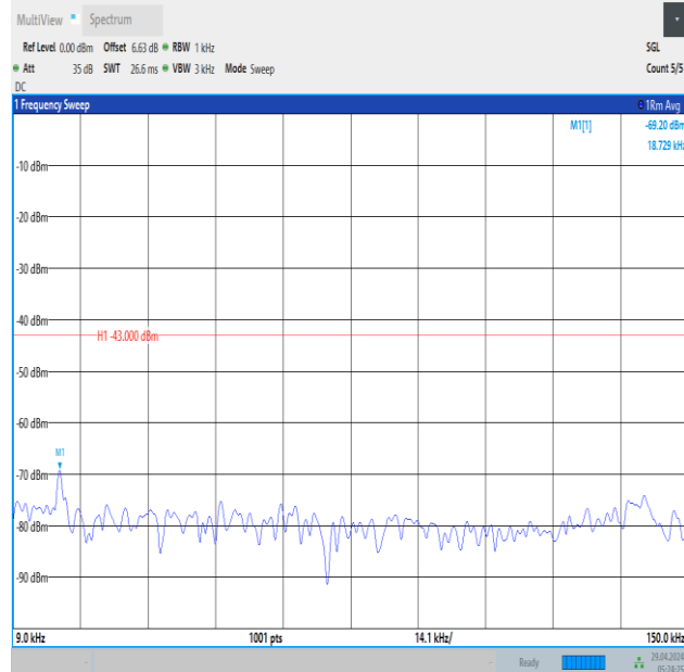
Band66_3MHz_16QAM_131987_1RB#0_0.009~0.15_0.009~0.15
