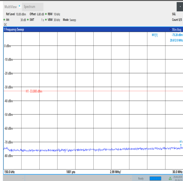
Band66_3MHz_16QAM_131987_1RB#14_0.15~30_0.15~30
