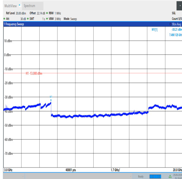
Band66_1.4MHz_QPSK_132665_1RB#0_3000~20000_3000~20000
