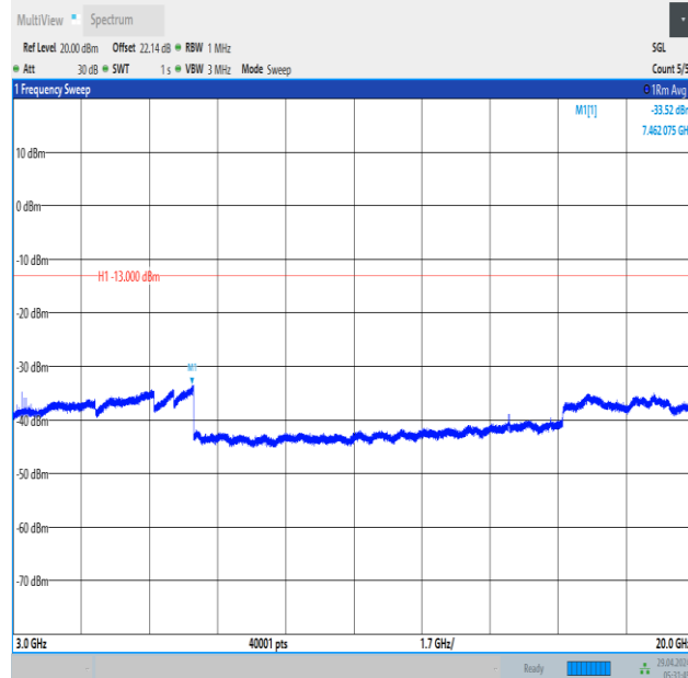
Band66_3MHz_16QAM_132322_1RB#14_3000~20000_3000~20000
