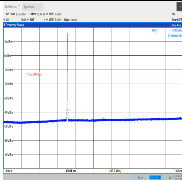
Band66_3MHz_QPSK_131987_15RB#0_1000~3000_1000~3000
