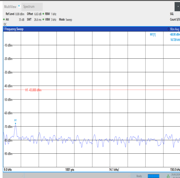
Band66_3MHz_QPSK_132322_1RB#0_0.009~0.15_0.009~0.15
