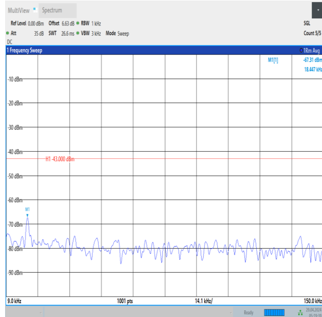
Band66_1.4MHz_QPSK_132665_1RB#5_0.009~0.15_0.009~0.15
