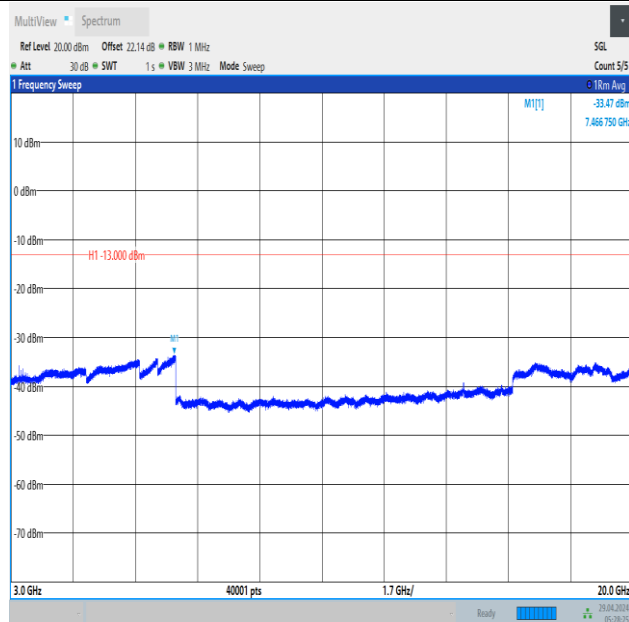
Band66_3MHz_16QAM_131987_15RB#0_3000~20000_3000~20000
