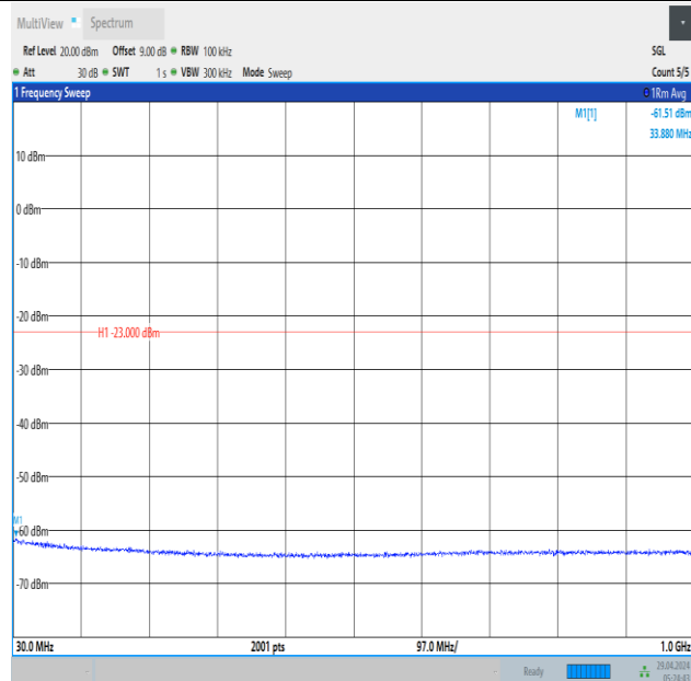
Band66_3MHz_16QAM_131987_1RB#0_30~1000_30~1000
