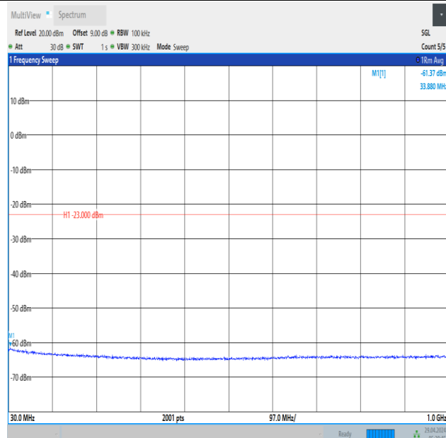
Band66_1.4MHz_16QAM_132665_1RB#5_30~1000_30~1000
