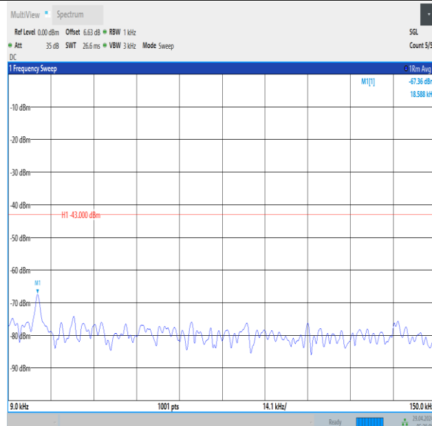
Band66_3MHz_16QAM_131987_1RB#14_0.009~0.15_0.009~0.15
