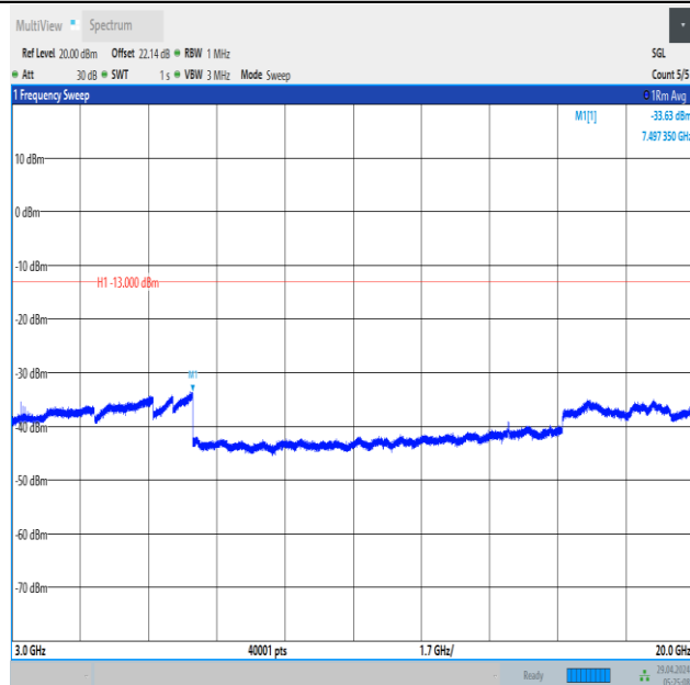
Band66_3MHz_16QAM_131987_1RB#0_3000~20000_3000~20000
