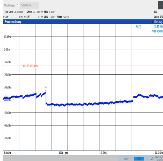
Band66_3MHz_QPSK_132322_1RB#14_3000~20000_3000~20000
