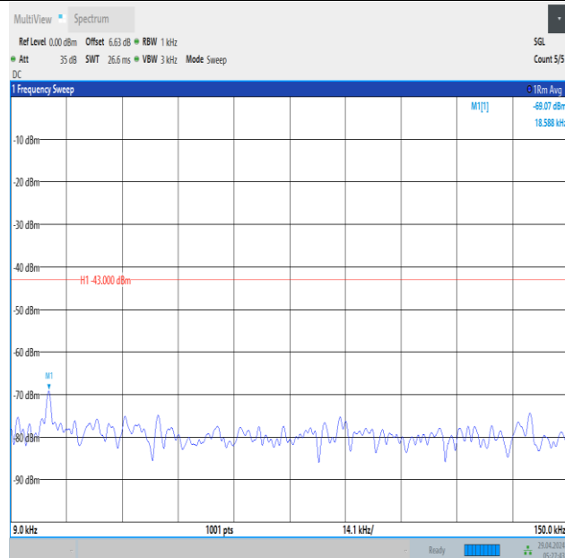
Band66_3MHz_16QAM_131987_15RB#0_0.009~0.15_0.009~0.15
