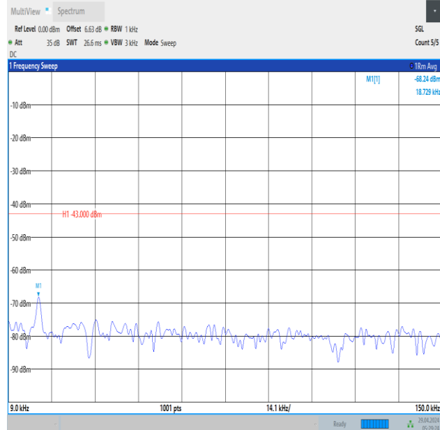
Band66_3MHz_16QAM_132322_1RB#0_0.009~0.15_0.009~0.15
