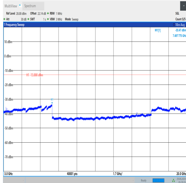
Band66_3MHz_QPSK_132322_1RB#0_3000~20000_3000~20000
