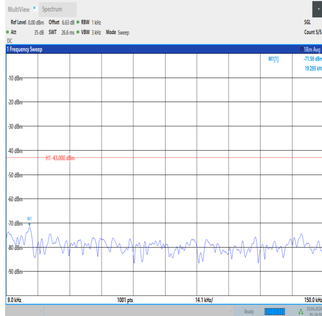
Band66_1.4MHz_16QAM_132665_1RB#0_0.009~0.15_0.009~0.15
