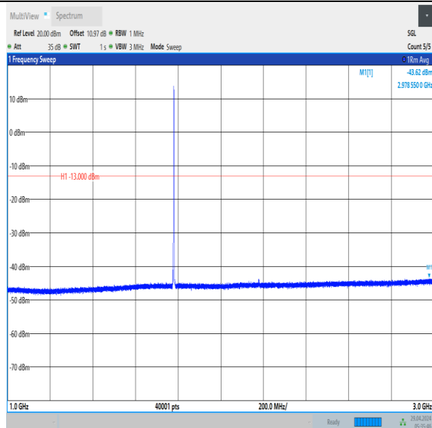
Band66_3MHz_QPSK_132657_1RB#14_1000~3000_1000~3000
