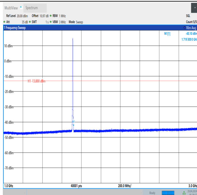
Band66_3MHz_16QAM_131987_15RB#0_1000~3000_1000~3000
