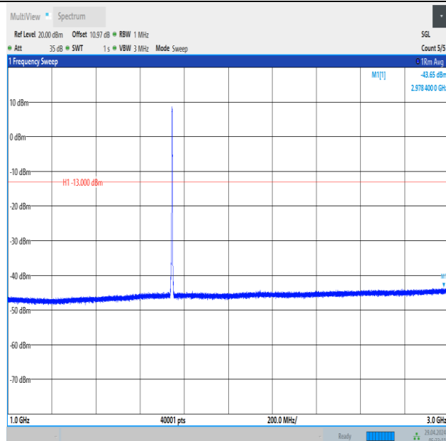
Band66_3MHz_16QAM_132322_15RB#0_1000~3000_1000~3000
