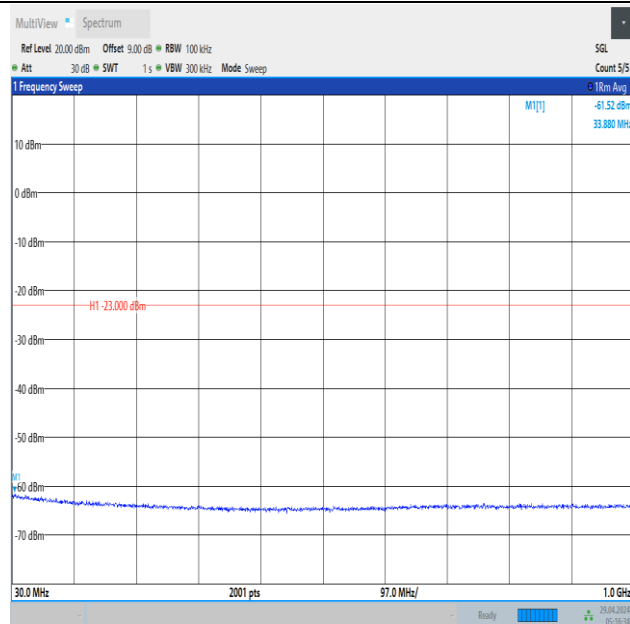
Band66_1.4MHz_QPSK_132322_6RB#0_30~1000_30~1000
