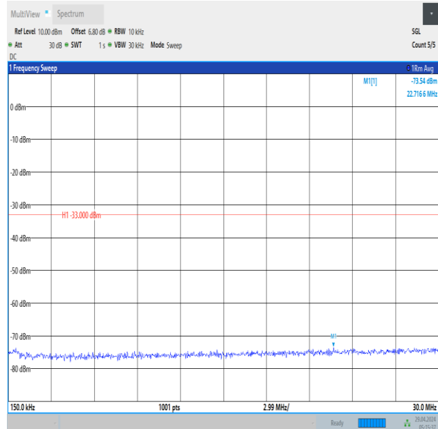
Band66_1.4MHz_16QAM_132322_1RB#5_0.15~30_0.15~30
