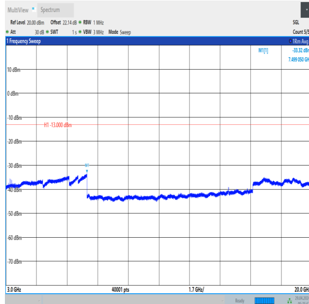
Band66_3MHz_QPSK_131987_1RB#14_3000~20000_3000~20000
