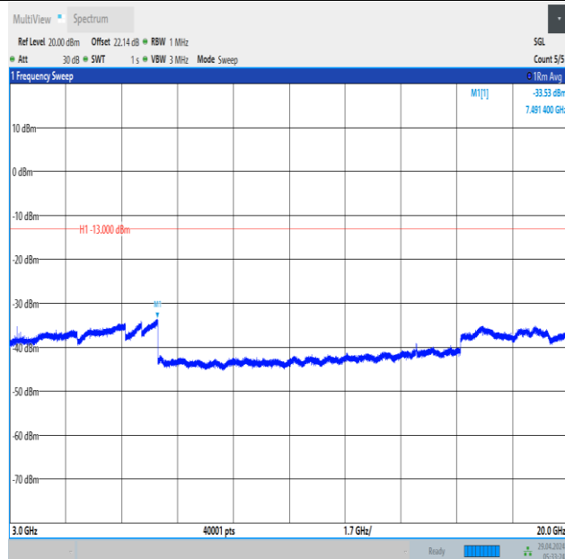
Band66_3MHz_16QAM_132322_15RB#0_3000~20000_3000~20000
