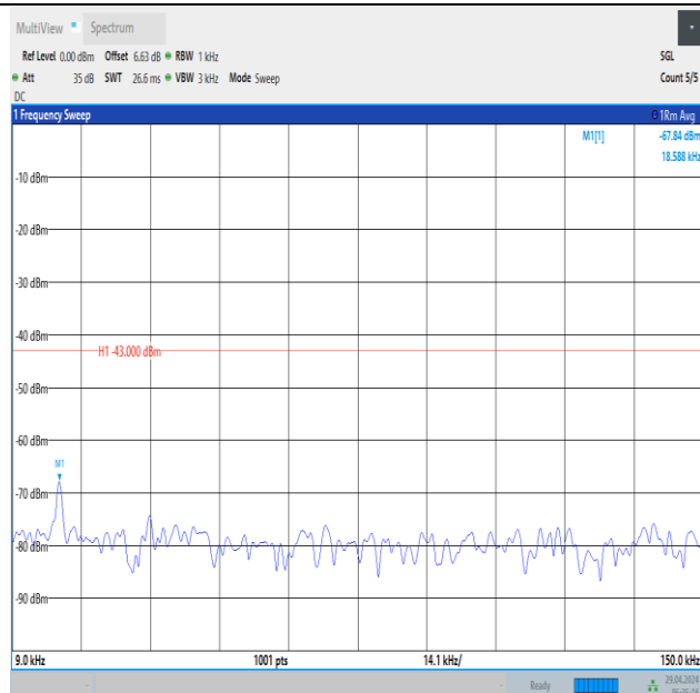
Band66_3MHz_QPSK_132657_1RB#14_0.009~0.15_0.009~0.15
