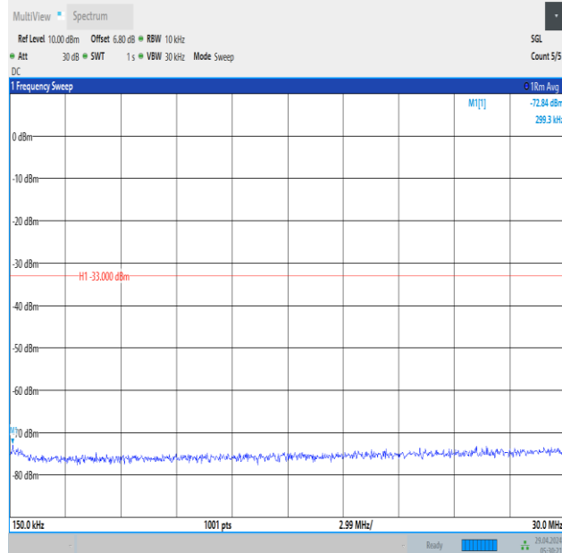
Band66_3MHz_QPSK_132322_1RB#14_0.15~30_0.15~30
