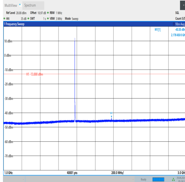
Band66_3MHz_16QAM_132657_1RB#0_1000~3000_1000~3000
