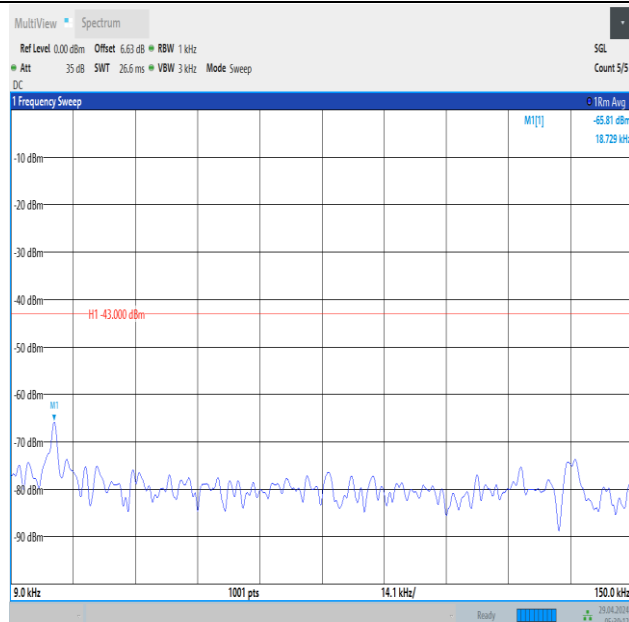
Band66_3MHz_QPSK_132322_1RB#14_0.009~0.15_0.009~0.15
