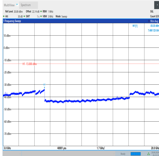
Band66_3MHz_QPSK_132322_15RB#0_3000~20000_3000~20000
