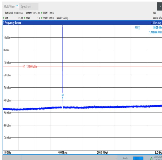
Band66_1.4MHz_16QAM_132322_6RB#0_1000~3000_1000~3000
