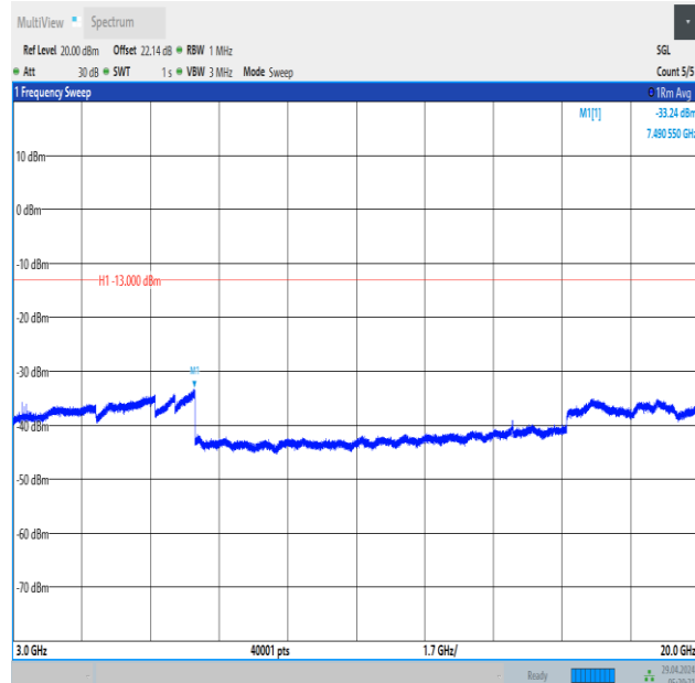
Band66_1.4MHz_QPSK_132665_1RB#5_3000~20000_3000~20000
