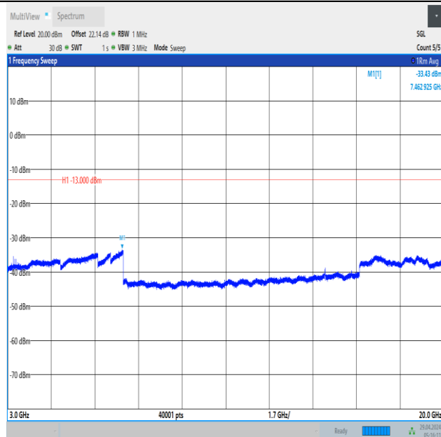
Band66_1.4MHz_16QAM_132322_1RB#5_3000~20000_3000~20000
