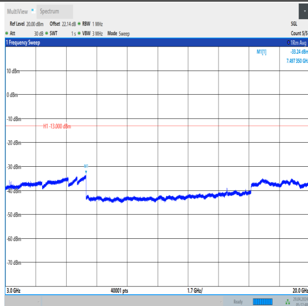
Band66_1.4MHz_16QAM_132322_6RB#0_3000~20000_3000~20000
