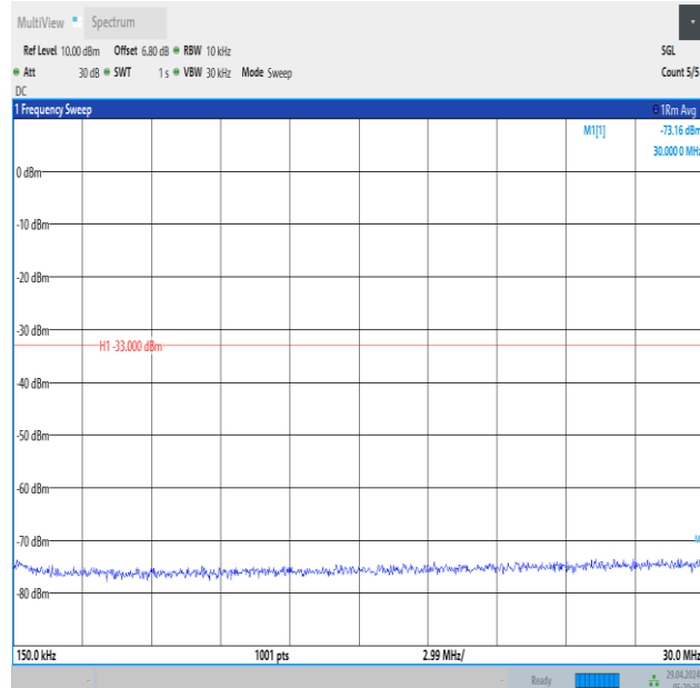
Band66_1.4MHz_16QAM_132665_1RB#5_0.15~30_0.15~30
