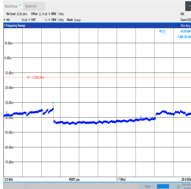
Band66_3MHz_QPSK_131987_1RB#0_3000~20000_3000~20000
