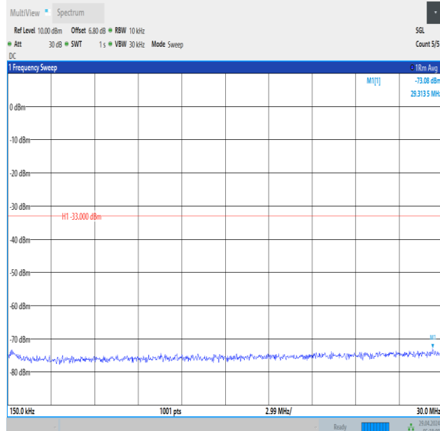
Band66_1.4MHz_QPSK_132665_1RB#0_0.15~30_0.15~30
