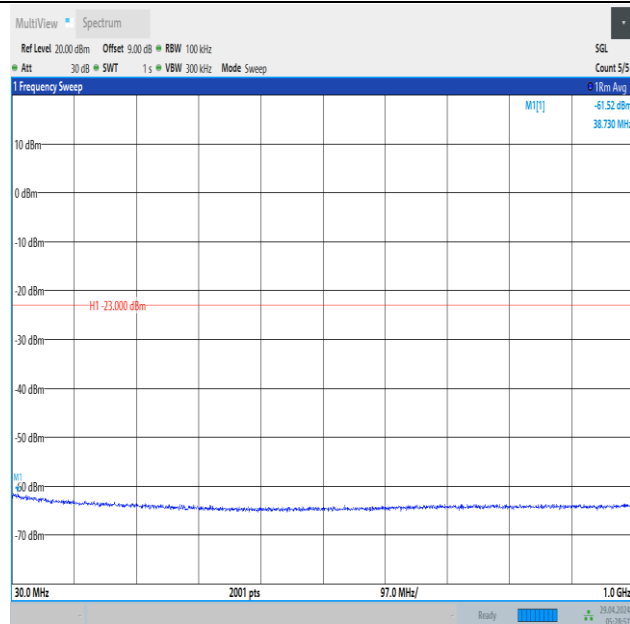
Band66_3MHz_QPSK_132322_1RB#0_30~1000_30~1000
