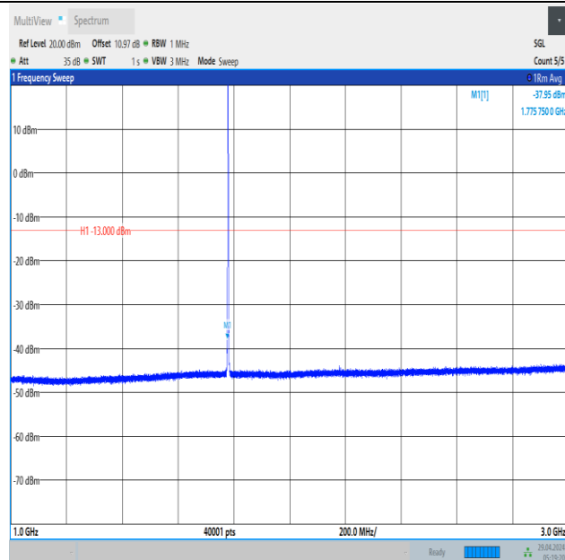
Band66_1.4MHz_16QAM_132665_1RB#0_1000~3000_1000~3000
