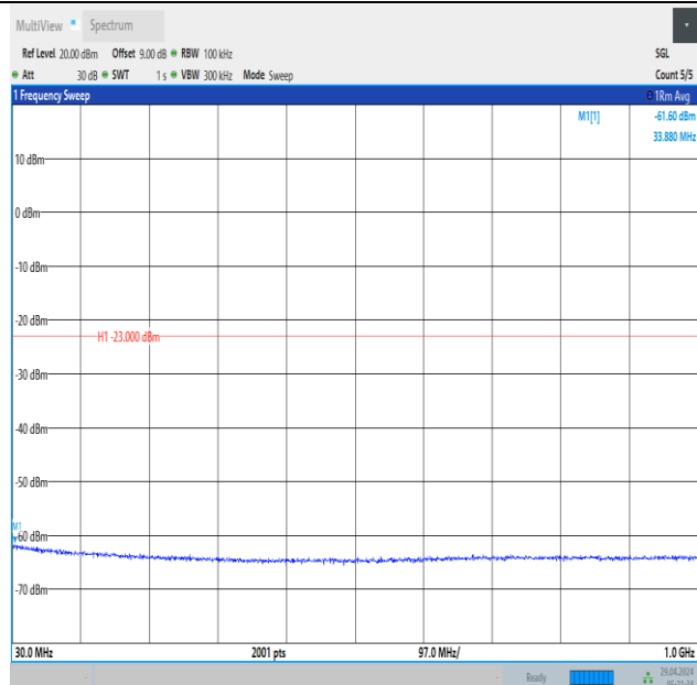
Band66_1.4MHz_QPSK_132665_6RB#0_30~1000_30~1000
