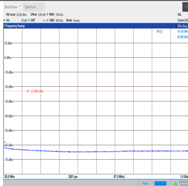
Band66_1.4MHz_QPSK_132665_1RB#0_30~1000_30~1000
