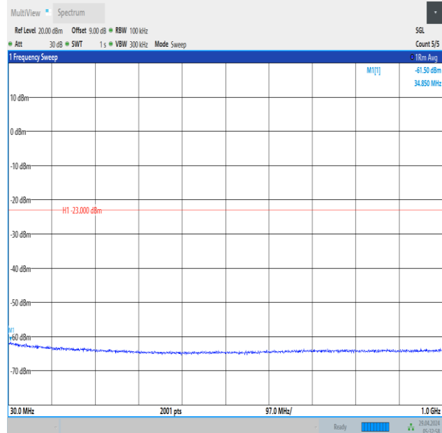
Band66_3MHz_16QAM_132322_15RB#0_30~1000_30~1000
