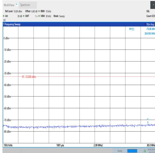
Band66_3MHz_16QAM_131987_15RB#0_0.15~30_0.15~30
