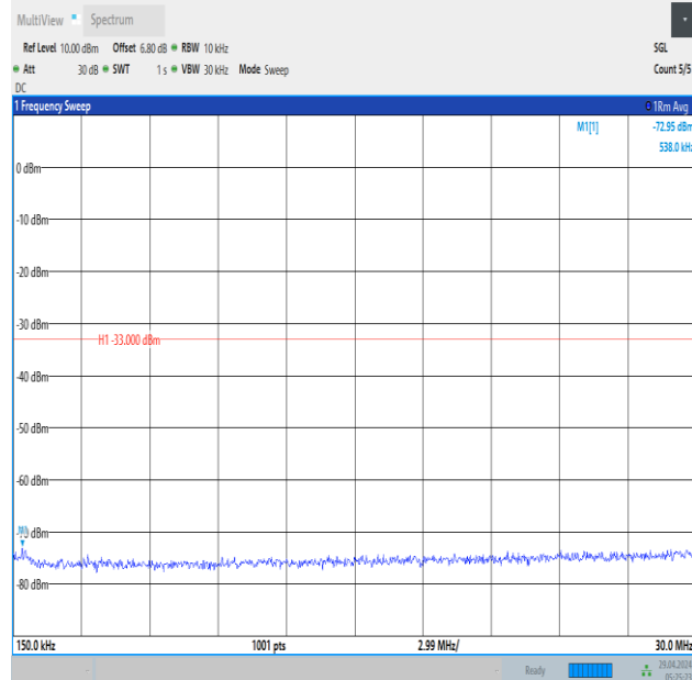
Band66_3MHz_QPSK_131987_1RB#14_0.15~30_0.15~30
