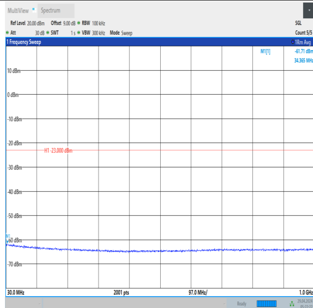
Band66_1.4MHz_16QAM_132665_6RB#0_30~1000_30~1000
