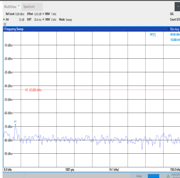
Band66_3MHz_QPSK_132322_15RB#0_0.009~0.15_0.009~0.15
