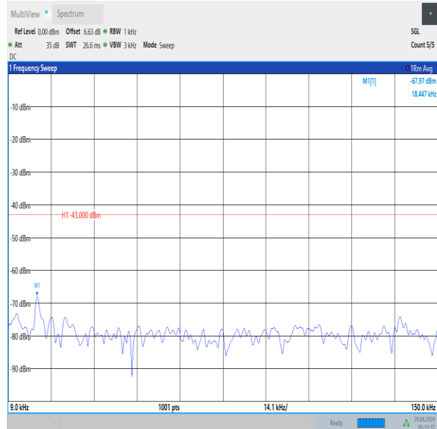
Band66_3MHz_QPSK_132657_1RB#0_0.009~0.15_0.009~0.15
