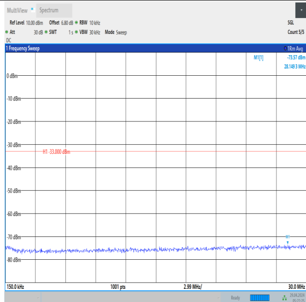
Band66_1.4MHz_QPSK_132665_6RB#0_0.15~30_0.15~30
