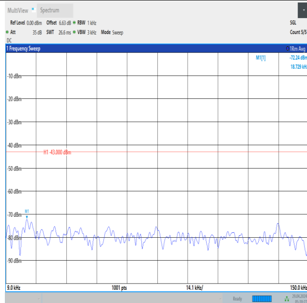
Band66_1.4MHz_16QAM_132665_1RB#5_0.009~0.15_0.009~0.15
