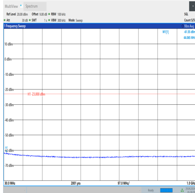
Band66_3MHz_QPSK_132322_1RB#14_30~1000_30~1000
