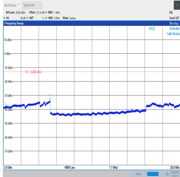
Band66_1.4MHz_16QAM_132665_1RB#5_3000~20000_3000~20000
