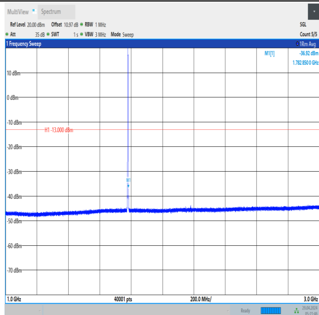
Band66_1.4MHz_QPSK_132665_6RB#0_1000~3000_1000~3000
