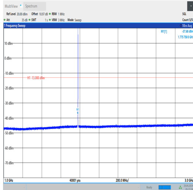
Band66_1.4MHz_16QAM_132665_6RB#0_1000~3000_1000~3000
