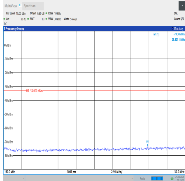
Band66_3MHz_16QAM_132322_1RB#0_0.15~30_0.15~30
