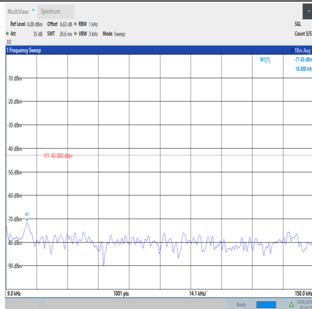
Band66_1.4MHz_QPSK_132322_6RB#0_0.009~0.15_0.009~0.15
