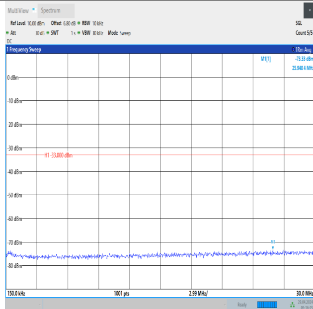
Band66_1.4MHz_QPSK_132322_6RB#0_0.15~30_0.15~30
