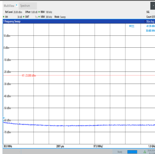
Band66_3MHz_QPSK_132322_15RB#0_30~1000_30~1000
