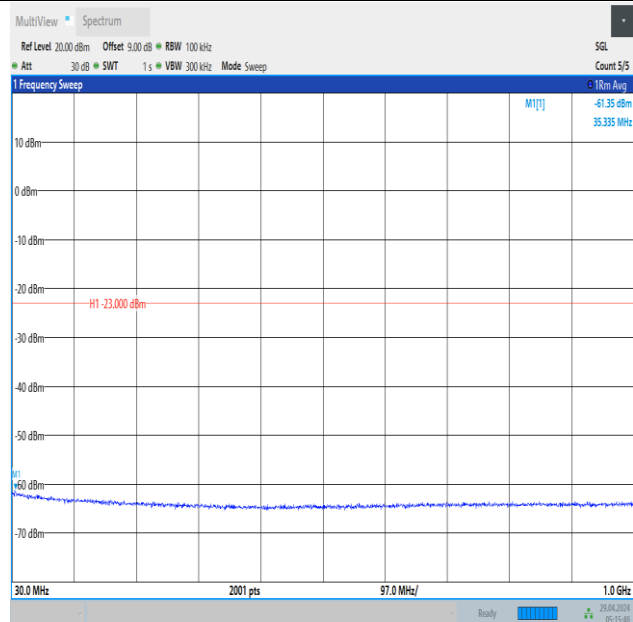
Band66_1.4MHz_16QAM_132322_1RB#5_30~1000_30~1000
