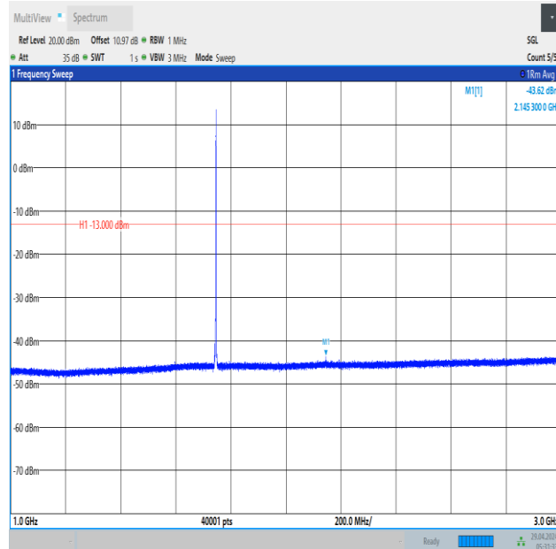
Band66_3MHz_16QAM_132322_1RB#14_1000~3000_1000~3000
