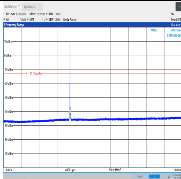
Band66_3MHz_QPSK_132322_15RB#0_1000~3000_1000~3000
