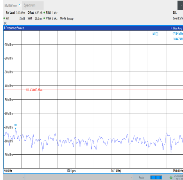
Band66_3MHz_16QAM_132322_1RB#14_0.009~0.15_0.009~0.15
