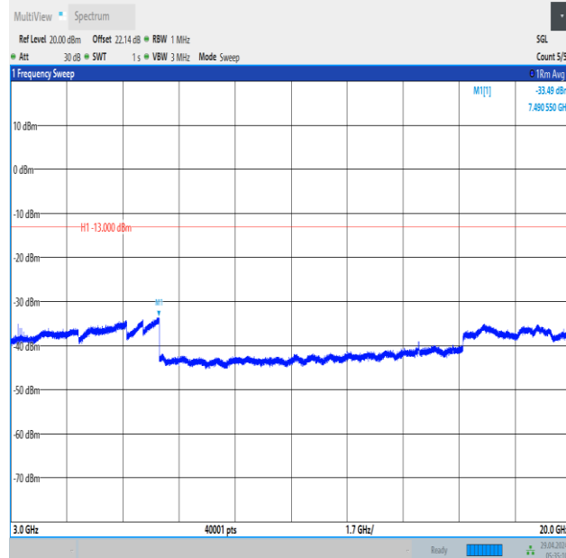
Band66_3MHz_16QAM_132657_1RB#0_3000~20000_3000~20000
