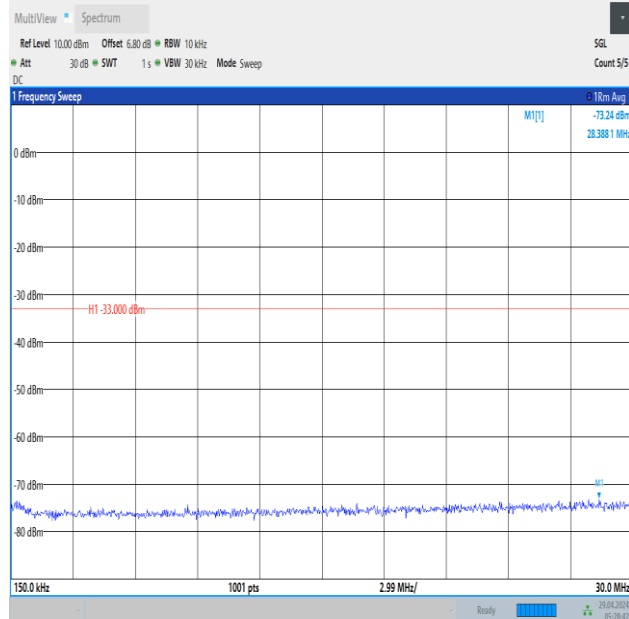
Band66_3MHz_QPSK_132322_1RB#0_0.15~30_0.15~30
