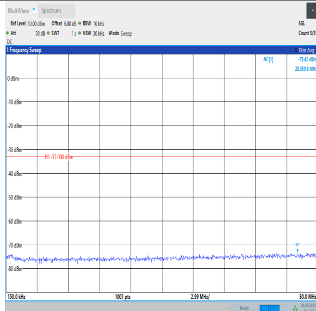
Band66_3MHz_QPSK_131987_15RB#0_0.15~30_0.15~30
