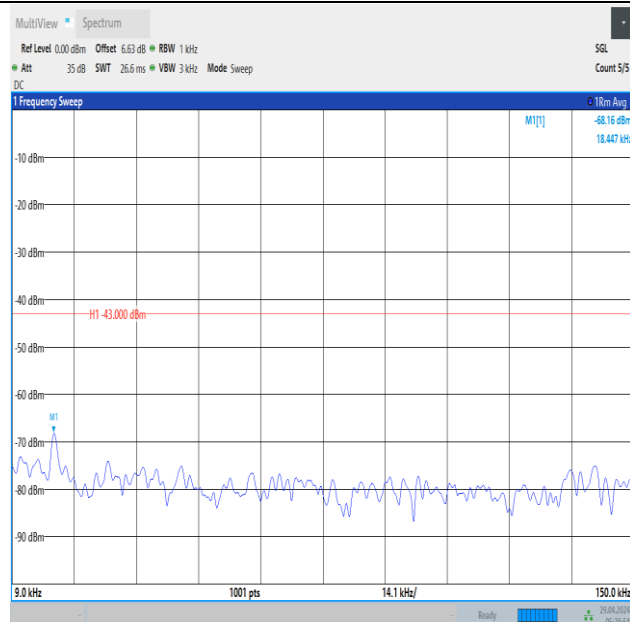
Band66_3MHz_QPSK_131987_15RB#0_0.009~0.15_0.009~0.15
