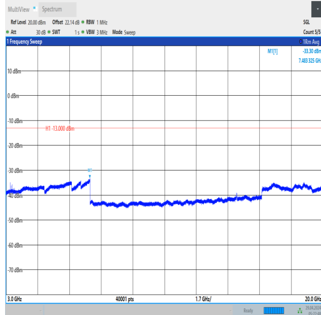
Band66_1.4MHz_16QAM_132665_6RB#0_3000~20000_3000~20000
