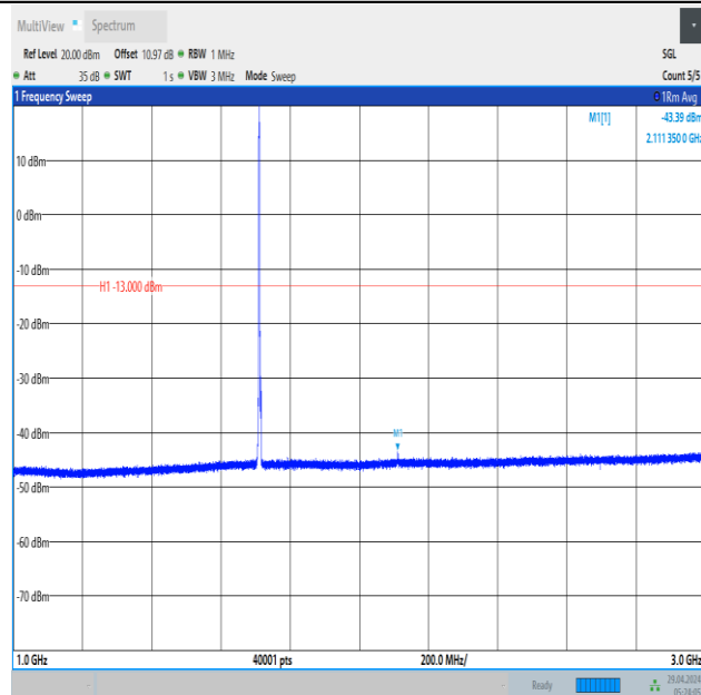
Band66_3MHz_QPSK_131987_1RB#0_1000~3000_1000~3000
