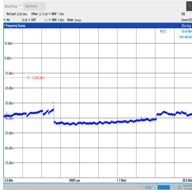
Band66_1.4MHz_QPSK_132665_6RB#0_3000~20000_3000~20000
