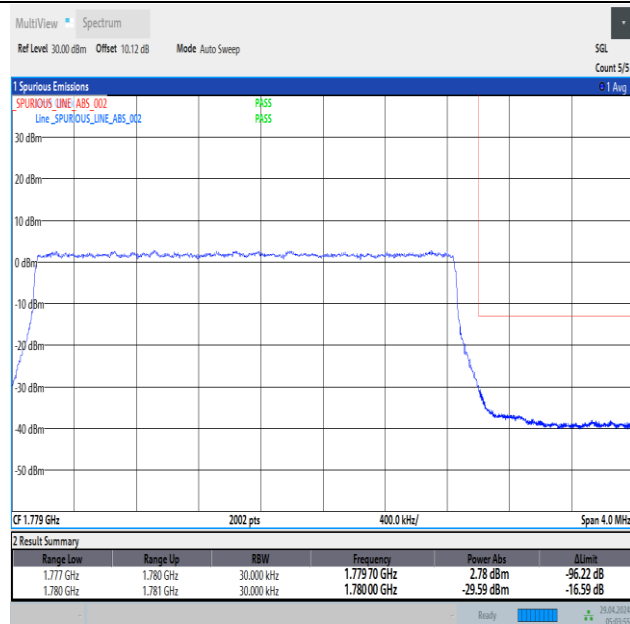
Band66_3MHz_QPSK_132657_15RB#0
