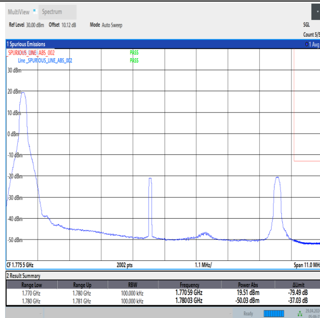
Band66_10MHz_QPSK_132622_1RB#0
