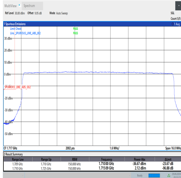
Band66_15MHz_QPSK_132047_75RB#0
