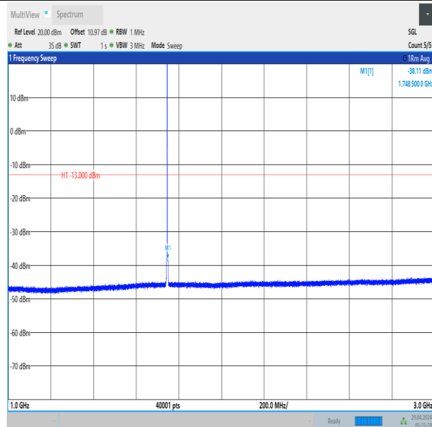
Band66_1.4MHz_QPSK_132322_1RB#5_1000~3000_1000~3000
