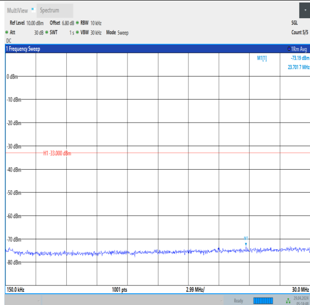
Band66_1.4MHz_QPSK_132322_1RB#5_0.15~30_0.15~30
