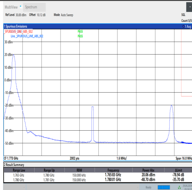
Band66_15MHz_16QAM_132597_1RB#0
