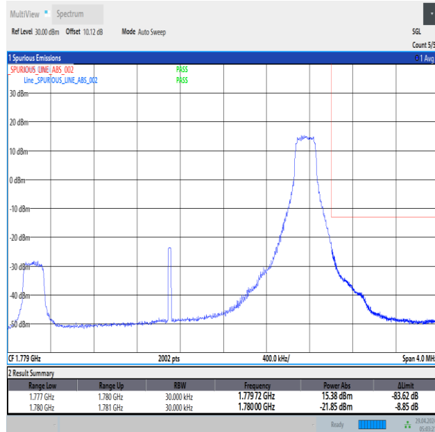
Band66_3MHz_QPSK_132657_1RB#14
