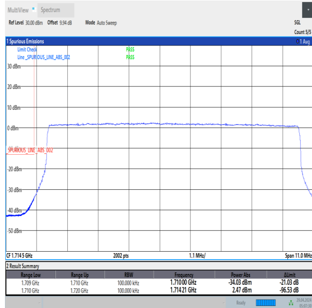
Band66_10MHz_QPSK_132022_50RB#0
