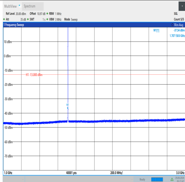
Band66_1.4MHz_QPSK_131979_6RB#0_1000~3000_1000~3000
