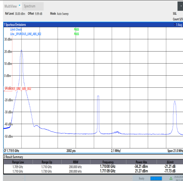
Band66_20MHz_16QAM_132072_1RB#0
