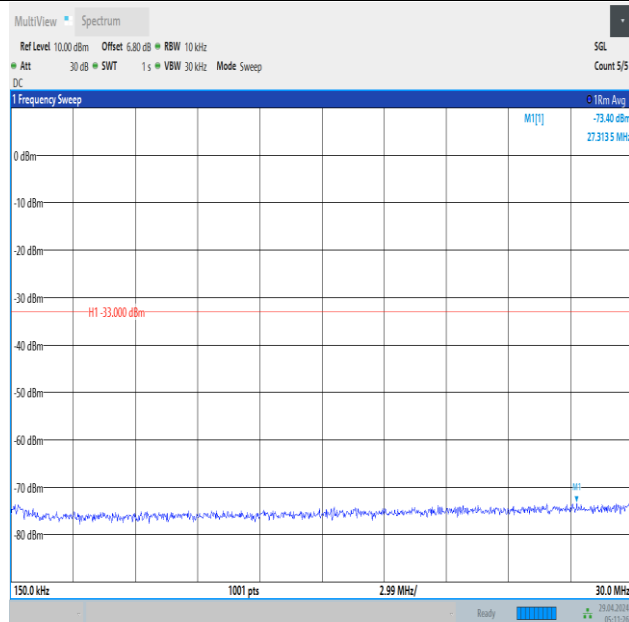
Band66_1.4MHz_QPSK_131979_6RB#0_0.15~30_0.15~30
