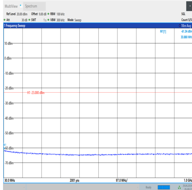
Band66_1.4MHz_QPSK_131979_1RB#5_30~1000_30~1000
