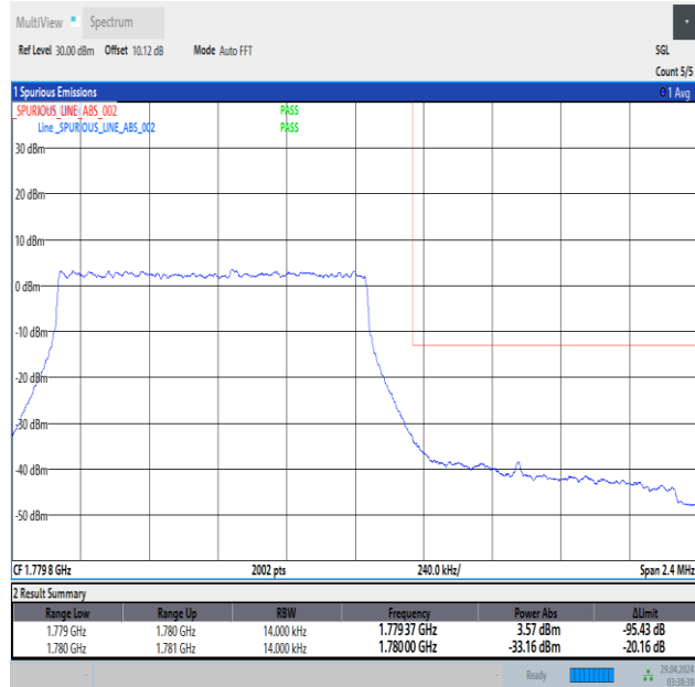
Band66_1.4MHz_QPSK_132665_6RB#0
