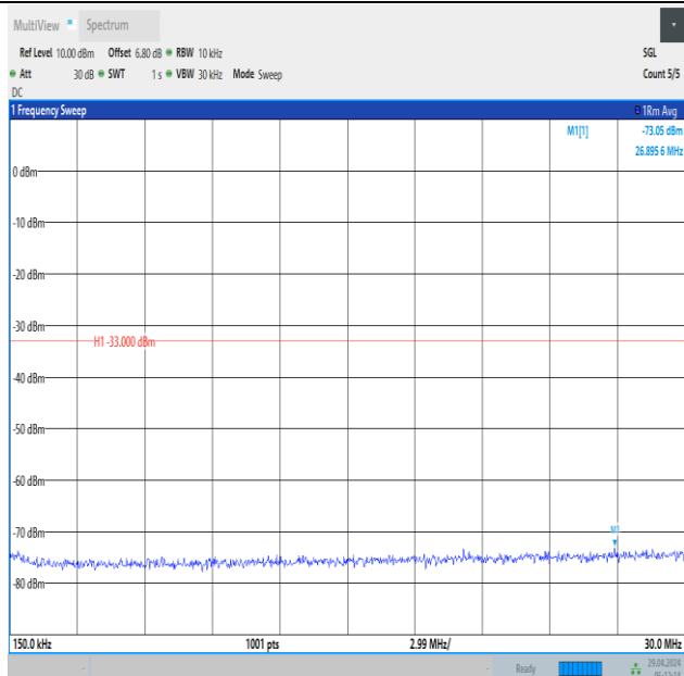
Band66_1.4MHz_16QAM_131979_6RB#0_0.15~30_0.15~30
