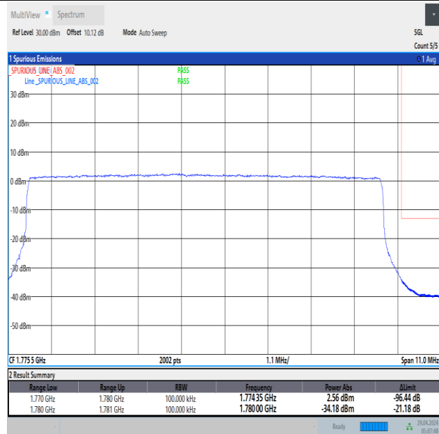
Band66_10MHz_QPSK_132622_50RB#0
