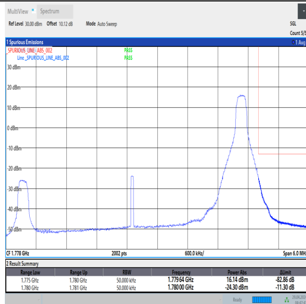
Band66_5MHz_16QAM_132647_1RB#24
