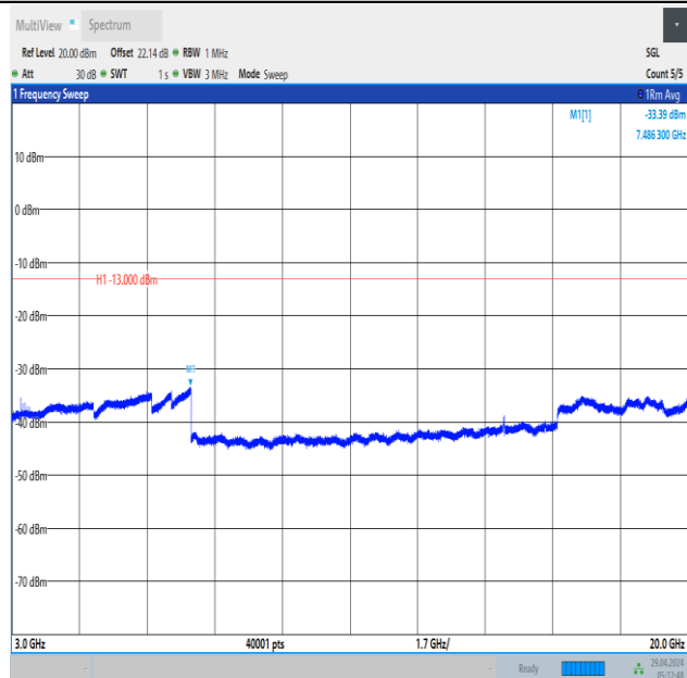
Band66_1.4MHz_16QAM_131979_6RB#0_3000~20000_3000~20000
