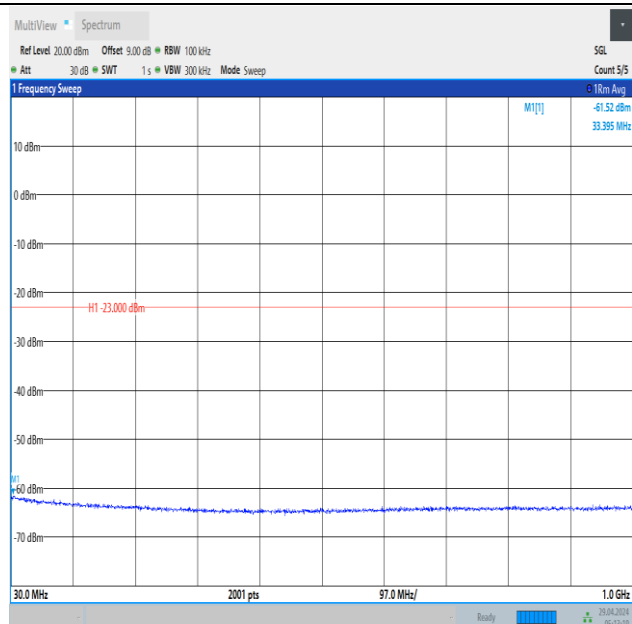
Band66_1.4MHz_QPSK_132322_1RB#0_30~1000_30~1000
