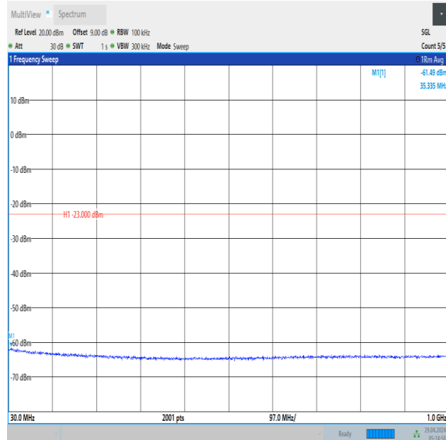
Band66_1.4MHz_QPSK_132322_1RB#5_30~1000_30~1000
