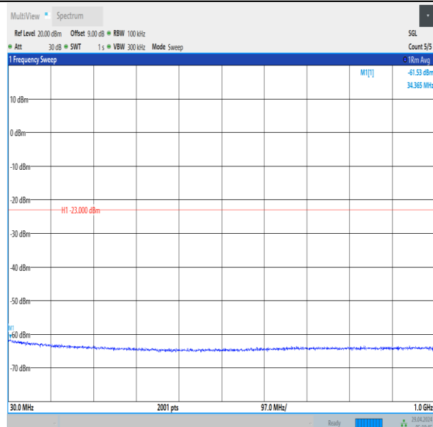
Band66_1.4MHz_16QAM_131979_1RB#5_30~1000_30~1000
