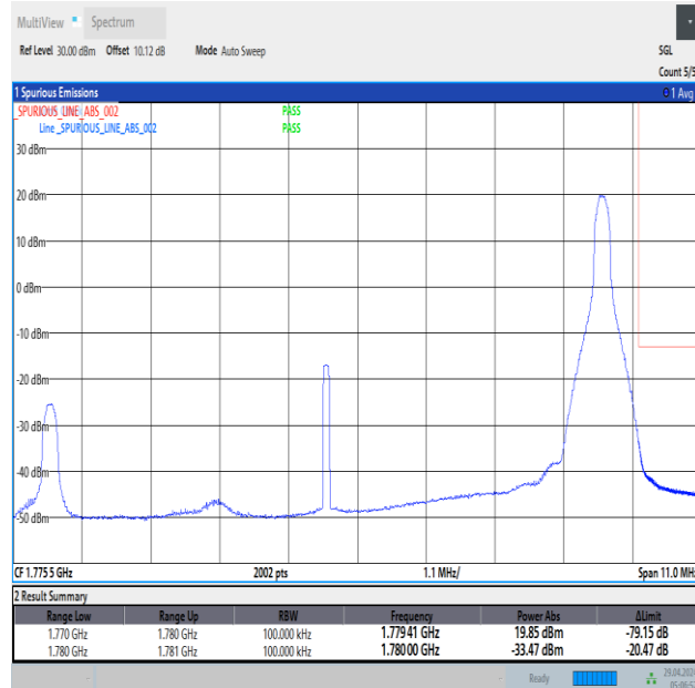
Band66_10MHz_QPSK_132622_1RB#49
