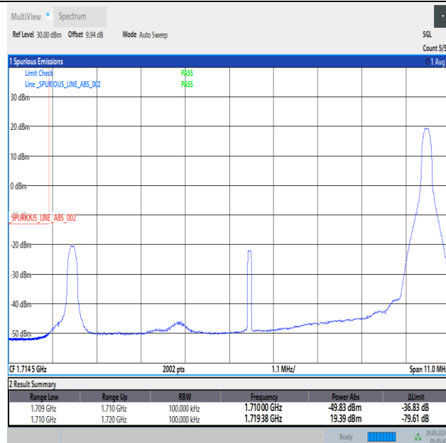
Band66_10MHz_QPSK_132022_1RB#49
