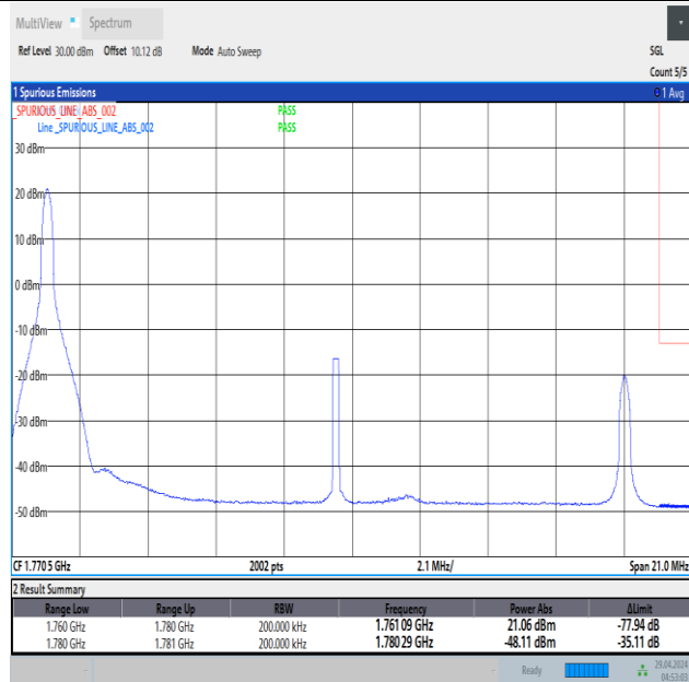
Band66_20MHz_16QAM_132572_1RB#0
