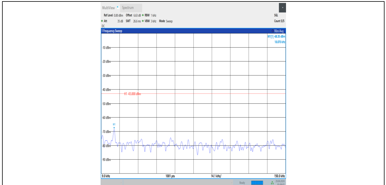
Band66_1.4MHz_QPSK_131979_1RB#0_0.009~0.15_0.009~0.15
