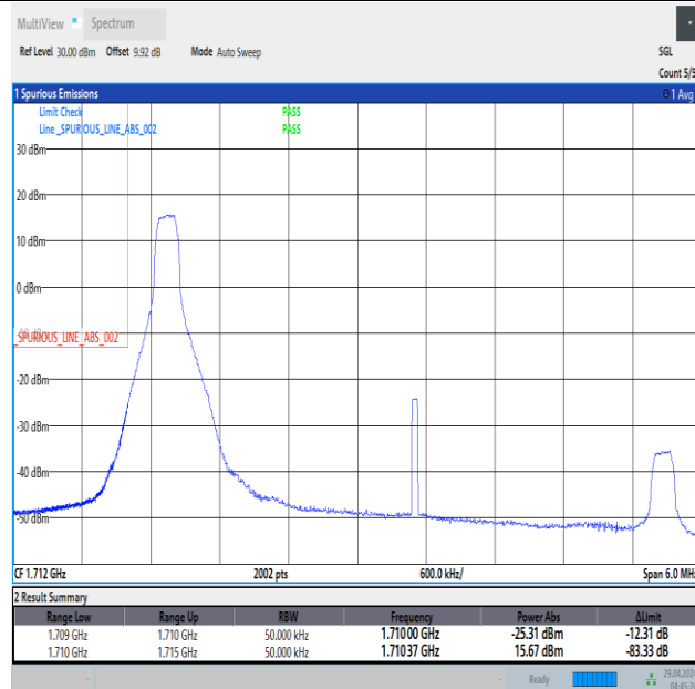
Band66_5MHz_16QAM_131997_1RB#0
