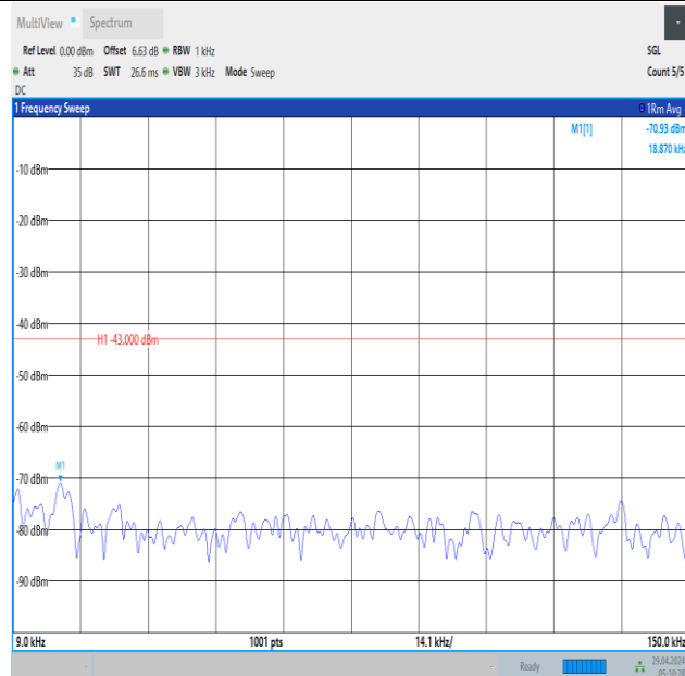
Band66_1.4MHz_16QAM_131979_1RB#5_0.009~0.15_0.009~0.15
