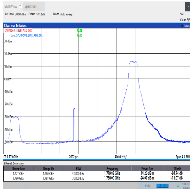
Band66_3MHz_16QAM_132657_1RB#14
