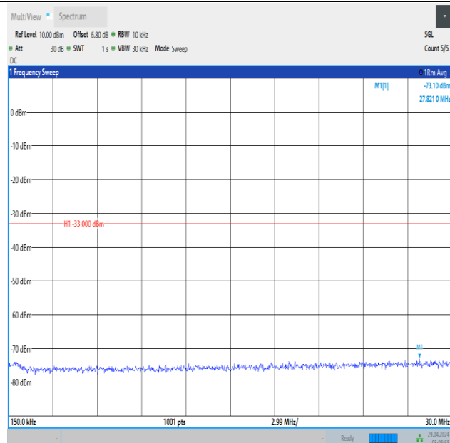
Band66_1.4MHz_16QAM_131979_1RB#0_0.15~30_0.15~30
