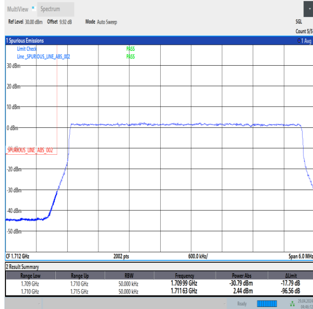
Band66_5MHz_QPSK_131997_25RB#0
