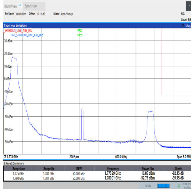
Band66_5MHz_QPSK_132647_1RB#0
