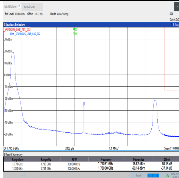
Band66_10MHz_16QAM_132622_1RB#0
