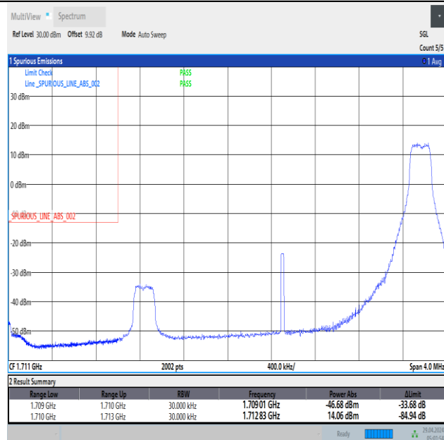
Band66_3MHz_16QAM_131987_1RB#14
