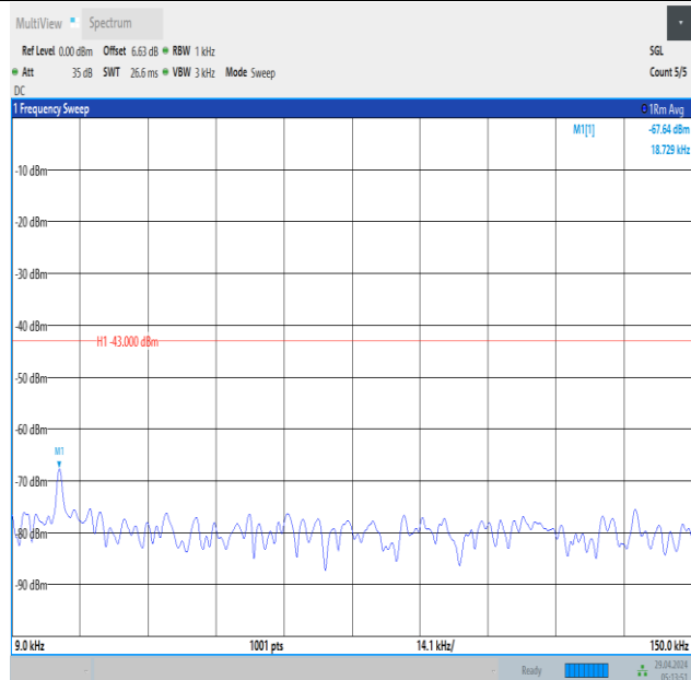
Band66_1.4MHz_16QAM_132322_1RB#0_0.009~0.15_0.009~0.15
