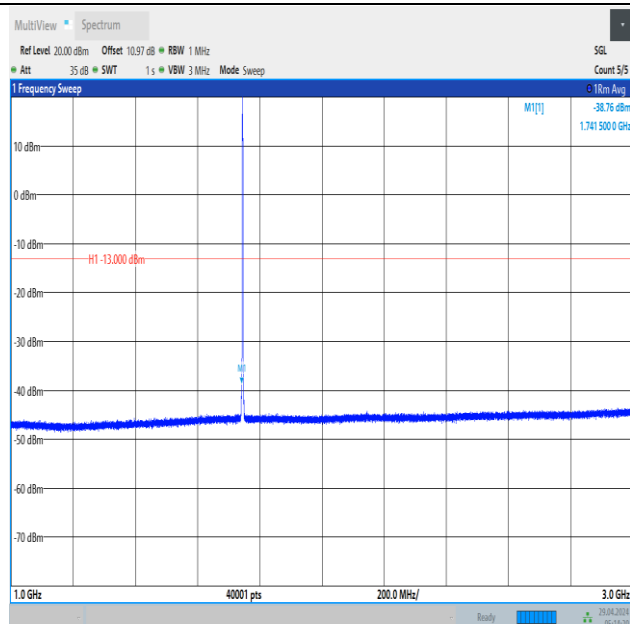
Band66_1.4MHz_16QAM_132322_1RB#0_1000~3000_1000~3000
