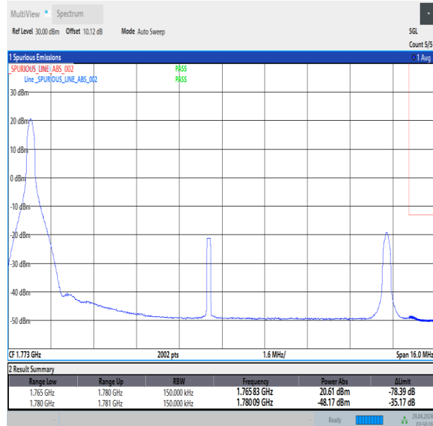
Band66_15MHz_QPSK_132597_1RB#0
