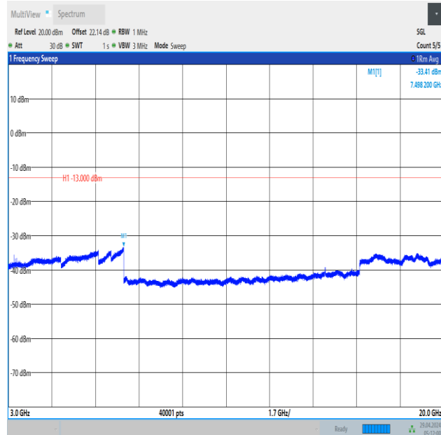
Band66_1.4MHz_QPSK_131979_6RB#0_3000~20000_3000~20000
