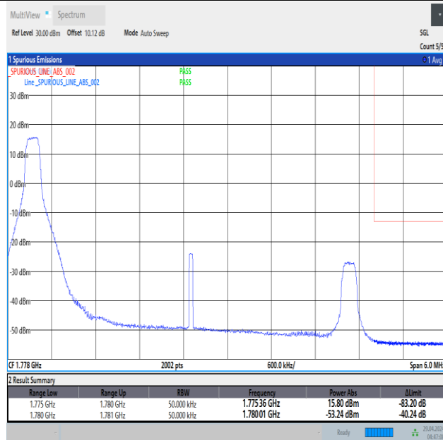
Band66_5MHz_16QAM_132647_1RB#0
