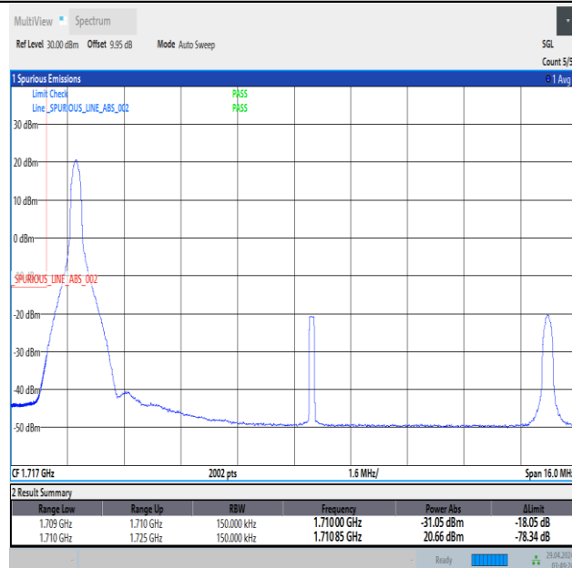
Band66_15MHz_16QAM_132047_1RB#0
