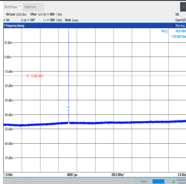
Band66_1.4MHz_QPSK_131979_1RB#0_1000~3000_1000~3000
