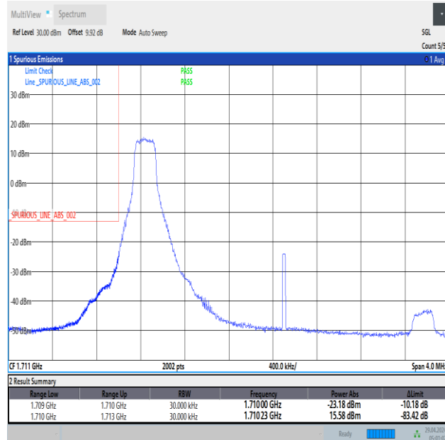
Band66_3MHz_QPSK_131987_1RB#0
