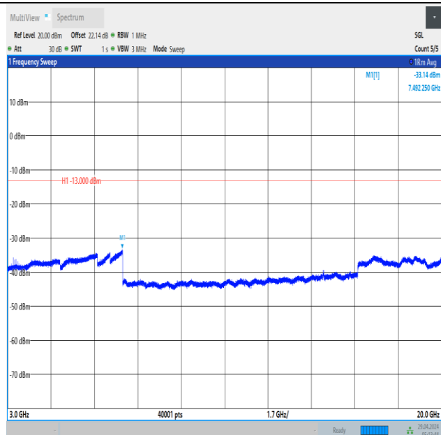
Band66_1.4MHz_QPSK_132322_1RB#0_3000~20000_3000~20000
