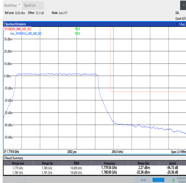
Band66_1.4MHz_16QAM_132665_6RB#0
