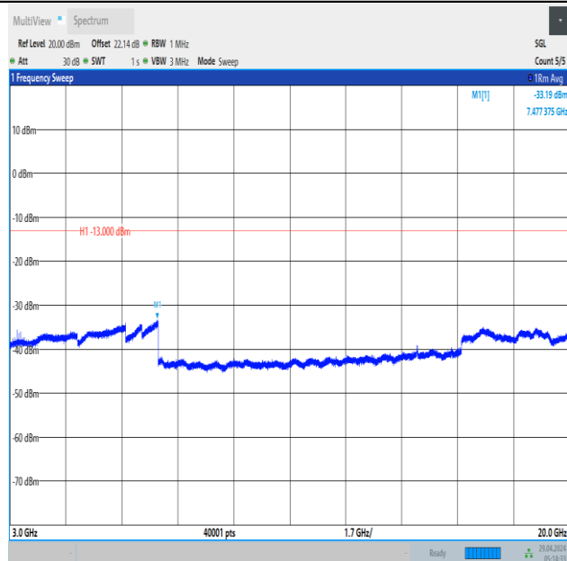
Band66_1.4MHz_16QAM_132322_1RB#0_3000~20000_3000~20000
