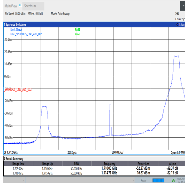
Band66_5MHz_QPSK_131997_1RB#24
