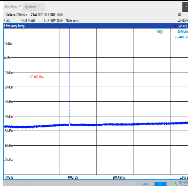
Band66_1.4MHz_16QAM_131979_1RB#5_1000~3000_1000~3000
