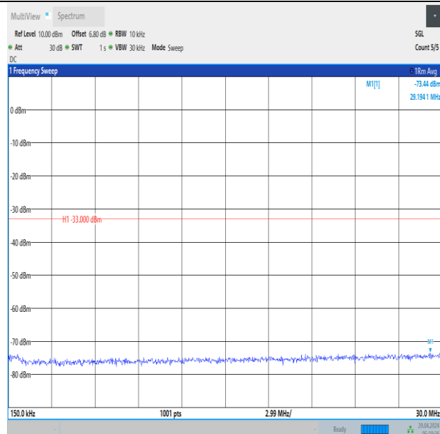
Band66_1.4MHz_16QAM_131979_1RB#5_0.15~30_0.15~30
