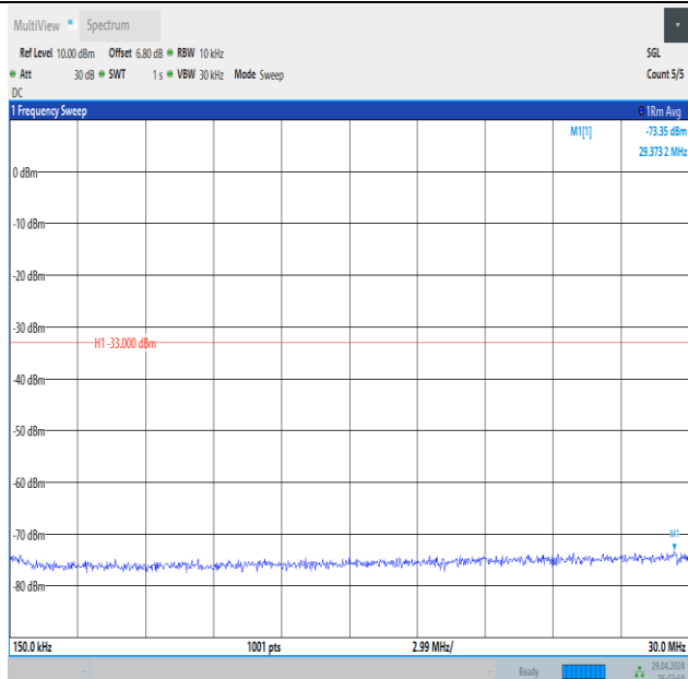
Band66_1.4MHz_16QAM_132322_1RB#0_0.15~30_0.15~30
