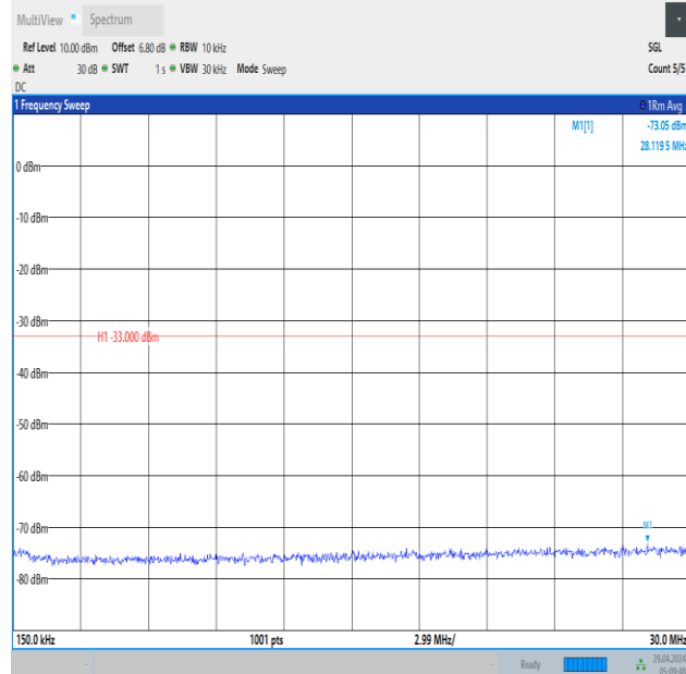
Band66_1.4MHz_QPSK_131979_1RB#5_0.15~30_0.15~30
