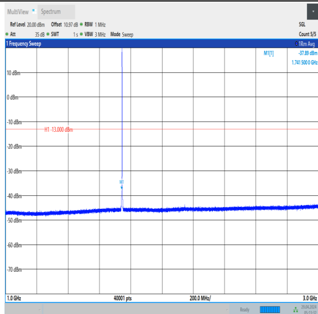
Band66_1.4MHz_QPSK_132322_1RB#0_1000~3000_1000~3000
