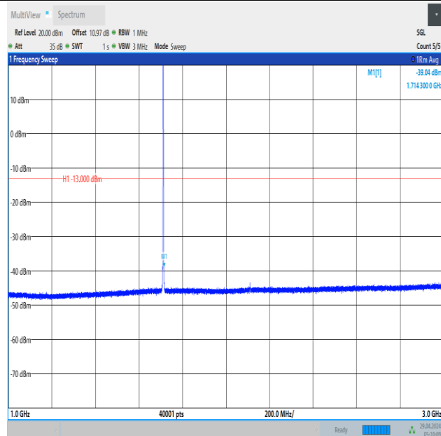
Band66_1.4MHz_QPSK_131979_1RB#5_1000~3000_1000~3000
