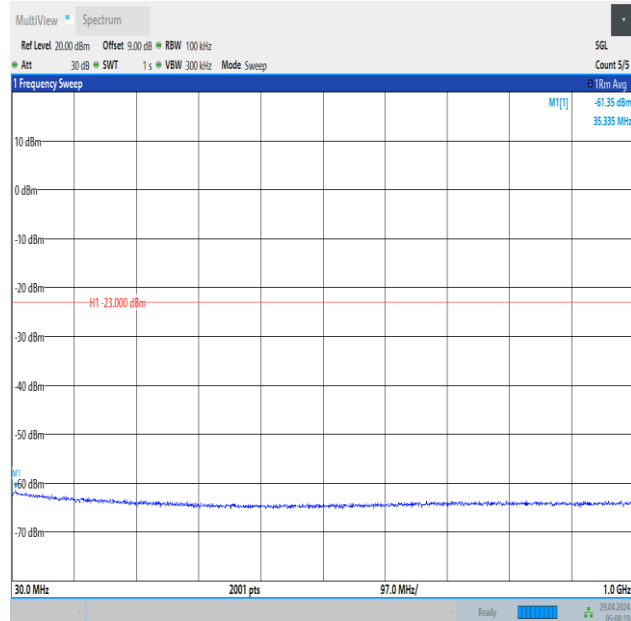
Band66_1.4MHz_QPSK_131979_1RB#0_30~1000_30~1000
