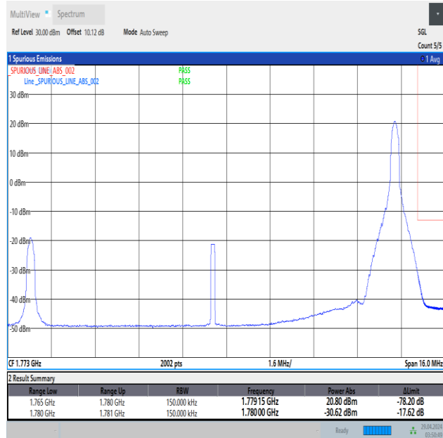
Band66_15MHz_QPSK_132597_1RB#74
