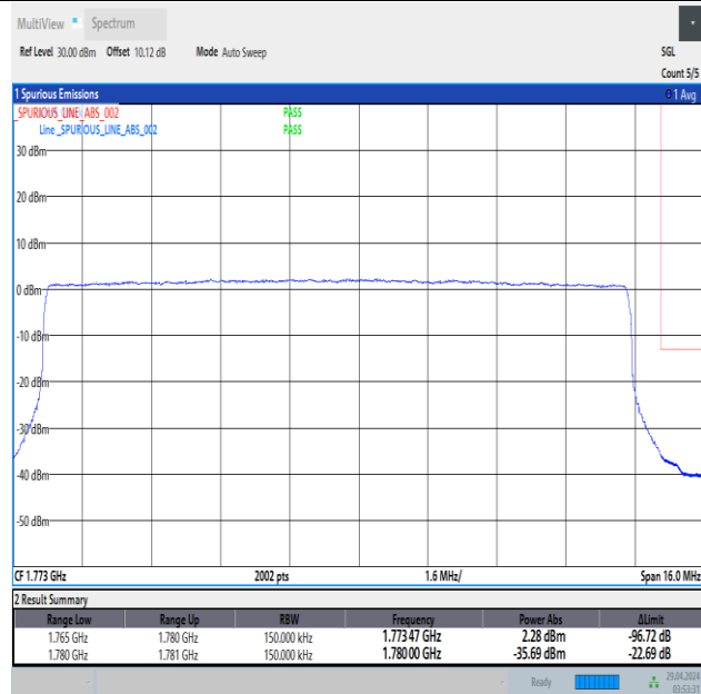
Band66_15MHz_QPSK_132597_75RB#0
