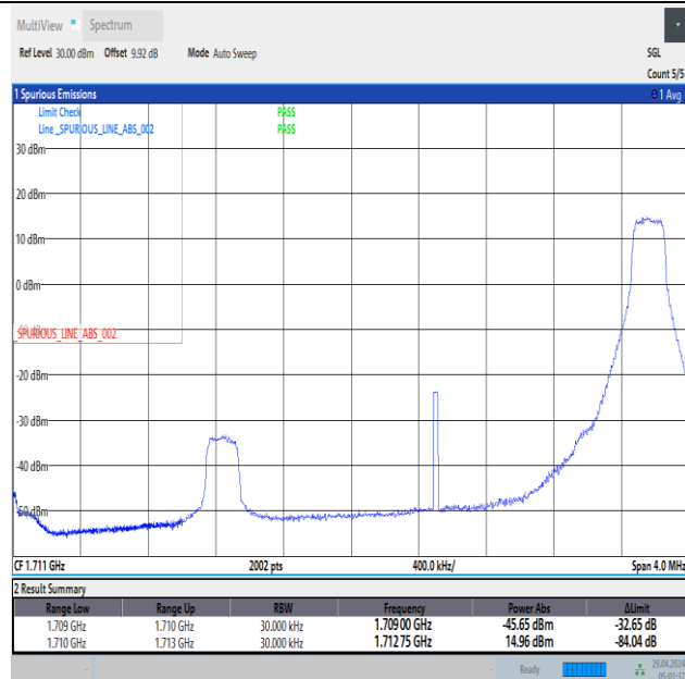
Band66_3MHz_QPSK_131987_1RB#14
