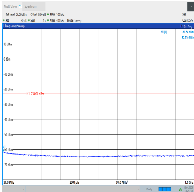
Band66_1.4MHz_16QAM_131979_6RB#0_30~1000_30~1000
