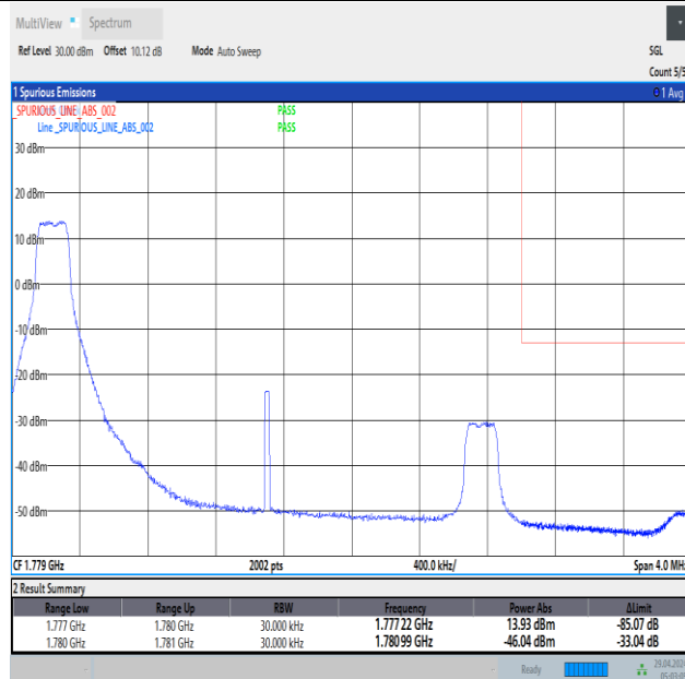
Band66_3MHz_16QAM_132657_1RB#0
