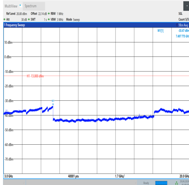
Band66_1.4MHz_QPSK_131979_1RB#0_3000~20000_3000~20000
