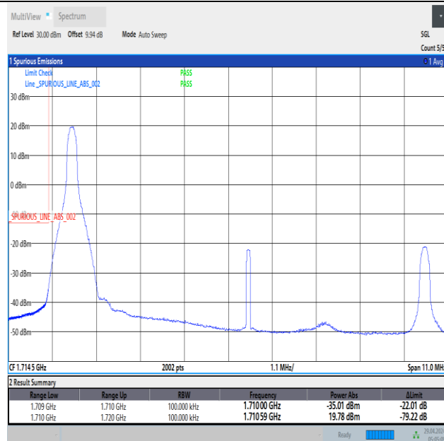
Band66_10MHz_QPSK_132022_1RB#0
