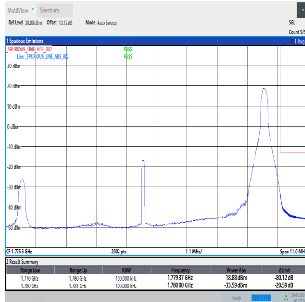
Band66_10MHz_16QAM_132622_1RB#49
