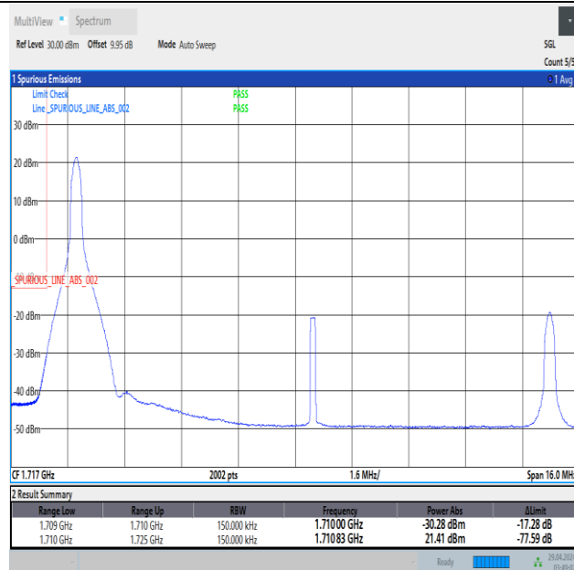
Band66_15MHz_QPSK_132047_1RB#0
