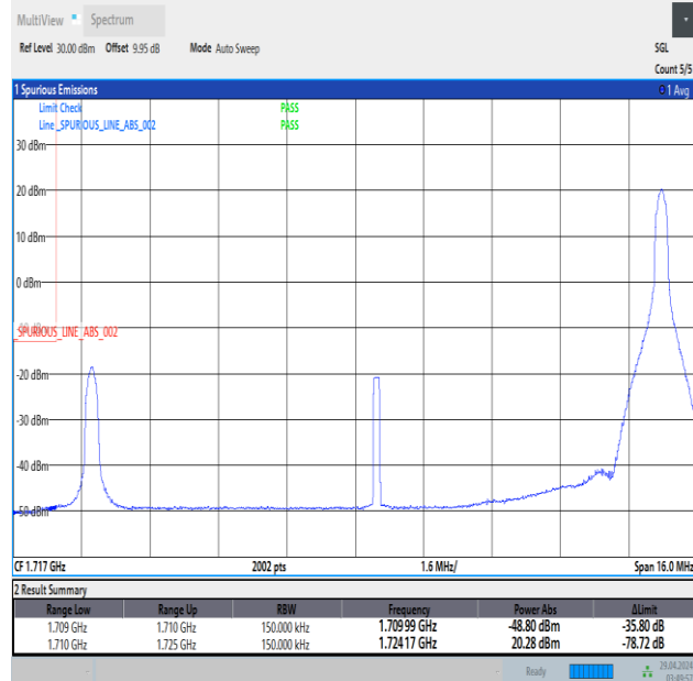
Band66_15MHz_16QAM_132047_1RB#74
