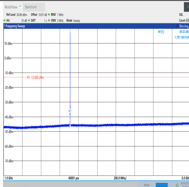
Band66_1.4MHz_16QAM_131979_1RB#0_1000~3000_1000~3000
