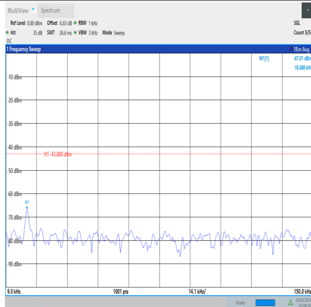
Band66_1.4MHz_16QAM_131979_1RB#0_0.009~0.15_0.009~0.15
