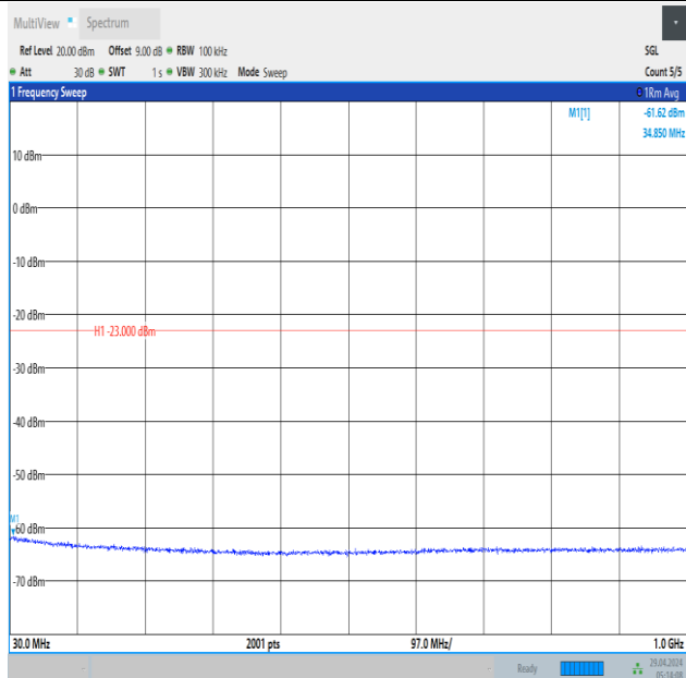
Band66_1.4MHz_16QAM_132322_1RB#0_30~1000_30~1000
