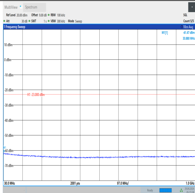
Band66_1.4MHz_QPSK_131979_6RB#0_30~1000_30~1000
