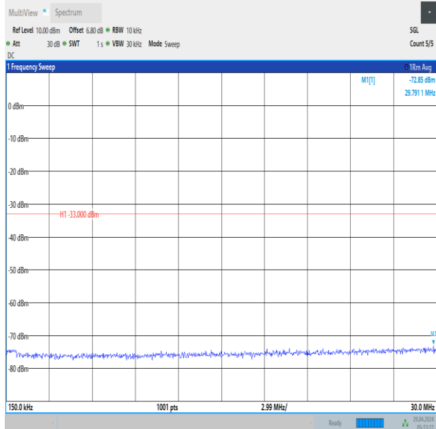
Band66_1.4MHz_QPSK_132322_1RB#0_0.15~30_0.15~30
