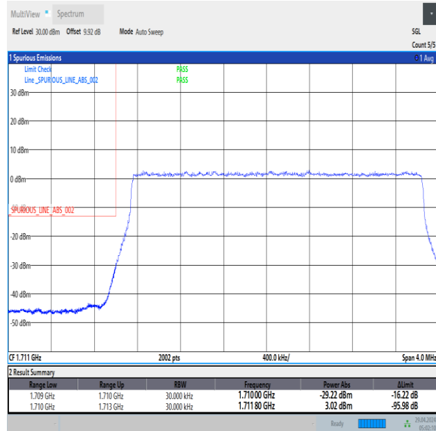
Band66_3MHz_QPSK_131987_15RB#0
