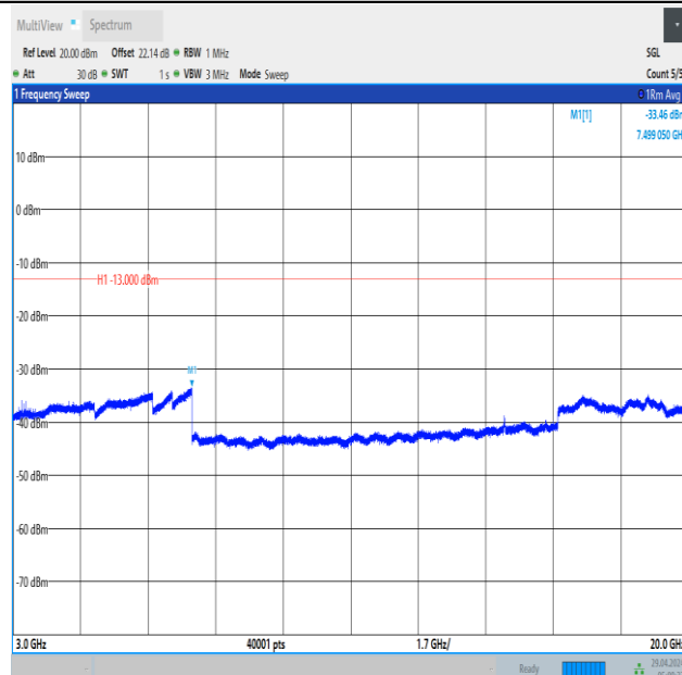
Band66_1.4MHz_16QAM_131979_1RB#0_3000~20000_3000~20000
