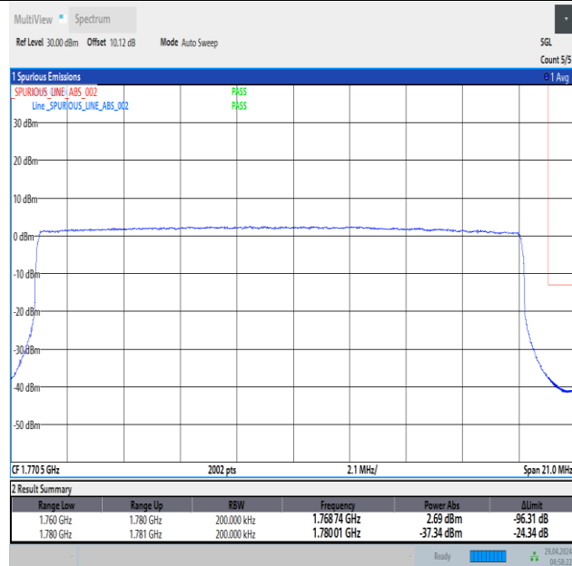
Band66_20MHz_QPSK_132572_100RB#0
