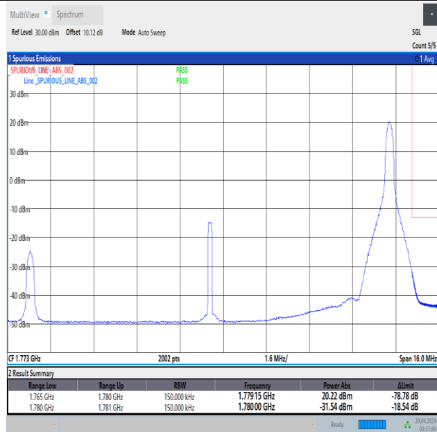
Band66_15MHz_16QAM_132597_1RB#74
