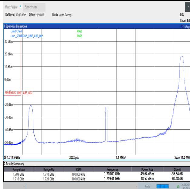
Band66_10MHz_16QAM_132022_1RB#49
