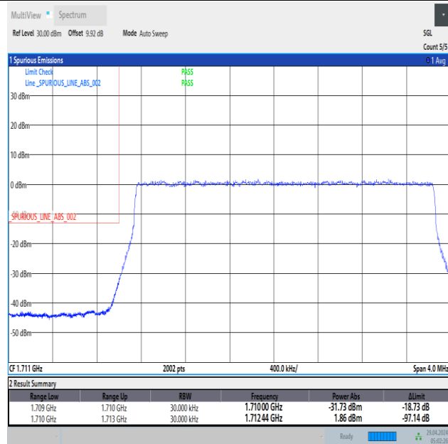
Band66_3MHz_16QAM_131987_15RB#0
