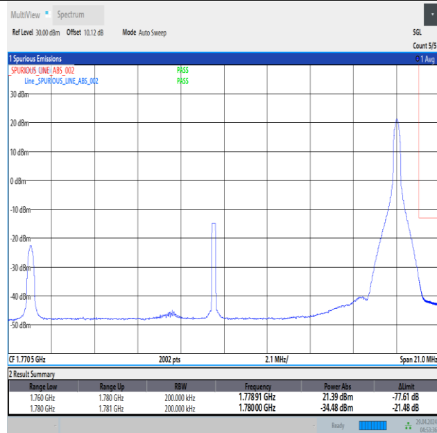
Band66_20MHz_16QAM_132572_1RB#99
