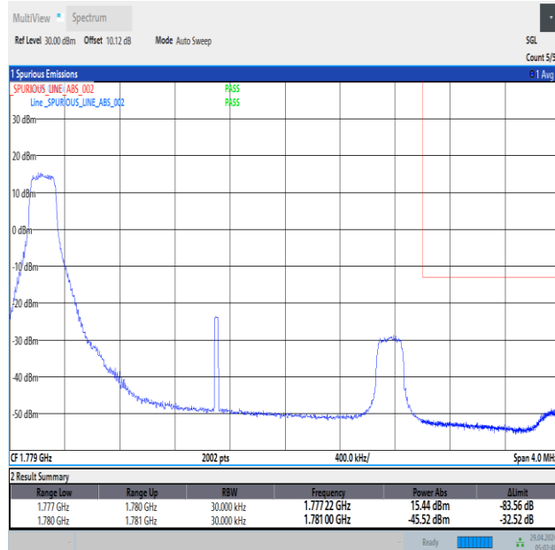
Band66_3MHz_QPSK_132657_1RB#0
