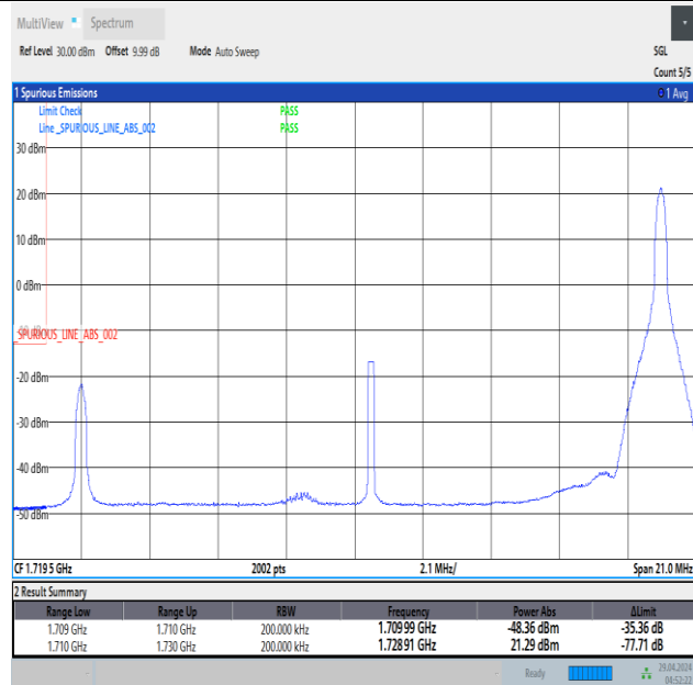
Band66_20MHz_16QAM_132072_1RB#99
