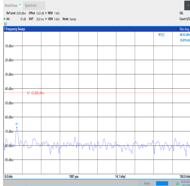
Band66_1.4MHz_16QAM_131979_6RB#0_0.009~0.15_0.009~0.15
