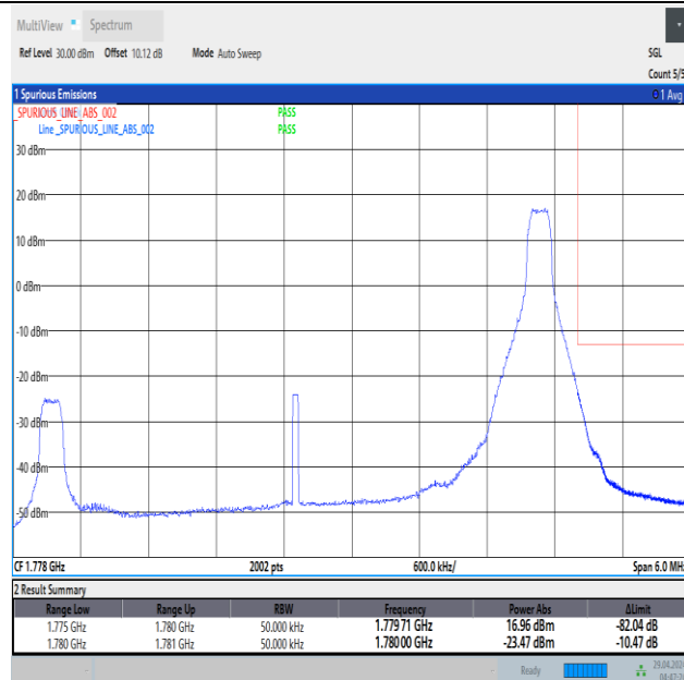
Band66_5MHz_QPSK_132647_1RB#24
