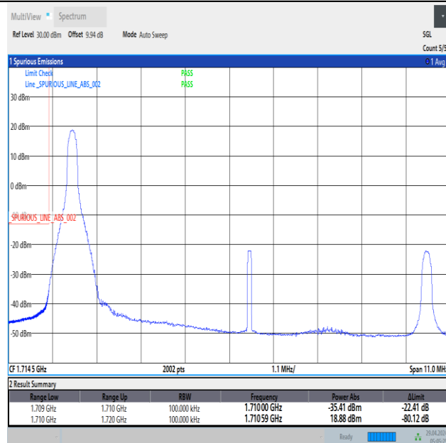
Band66_10MHz_16QAM_132022_1RB#0
