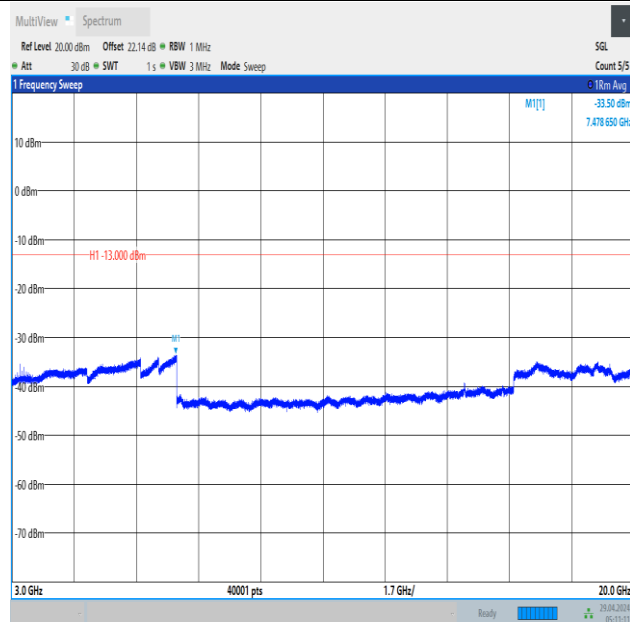
Band66_1.4MHz_16QAM_131979_1RB#5_3000~20000_3000~20000
