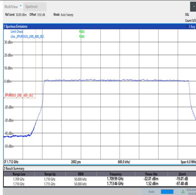
Band66_5MHz_16QAM_131997_25RB#0
