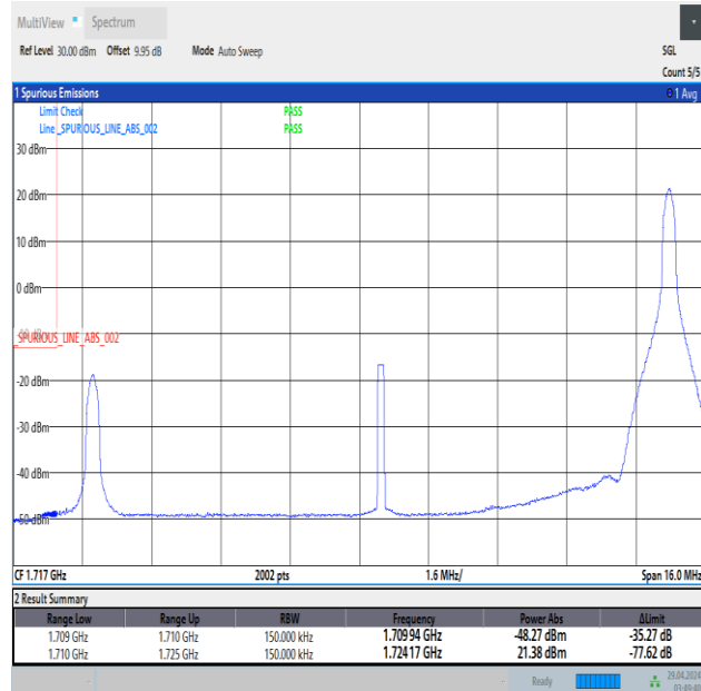
Band66_15MHz_QPSK_132047_1RB#74
