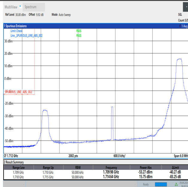
Band66_5MHz_16QAM_131997_1RB#24
