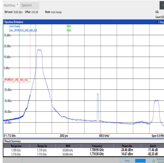
Band66_5MHz_QPSK_131997_1RB#0
