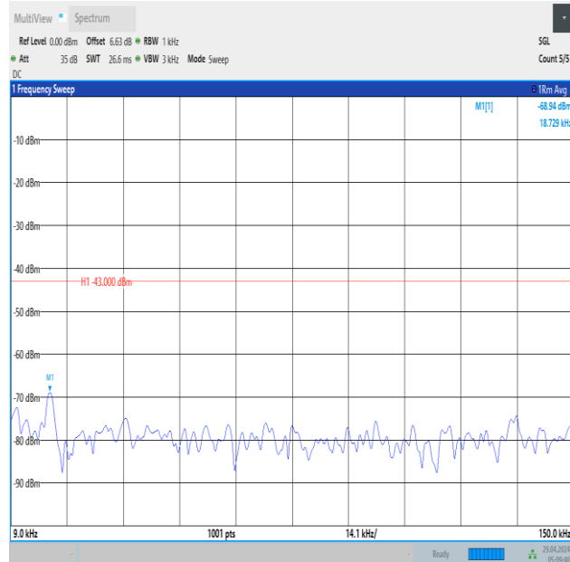
Band66_1.4MHz_QPSK_131979_1RB#5_0.009~0.15_0.009~0.15
