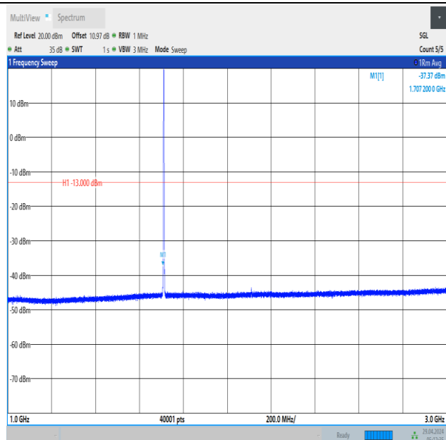
Band66_1.4MHz_16QAM_131979_6RB#0_1000~3000_1000~3000
