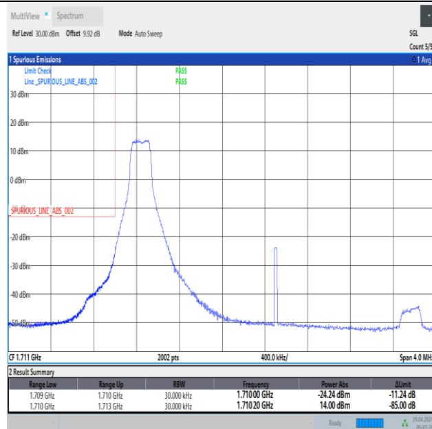
Band66_3MHz_16QAM_131987_1RB#0
