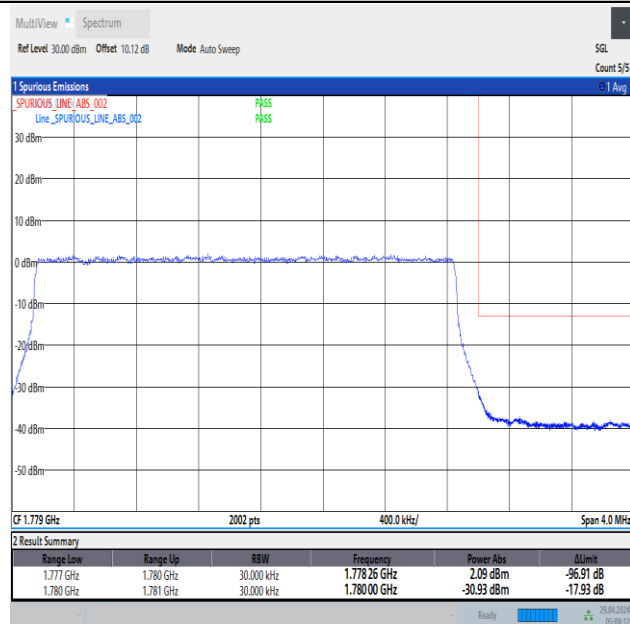
Band66_3MHz_16QAM_132657_15RB#0
