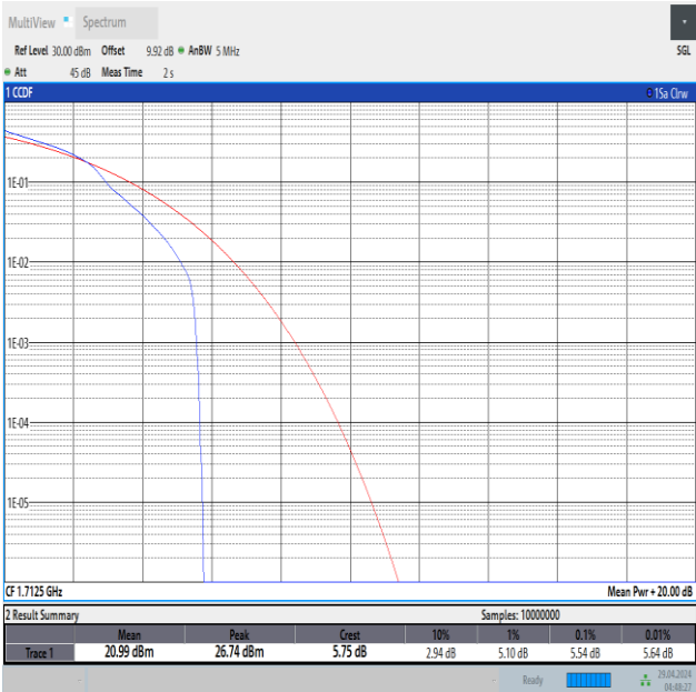
Band66-5MHz-16QAM-131997-1RB#0-PASS
