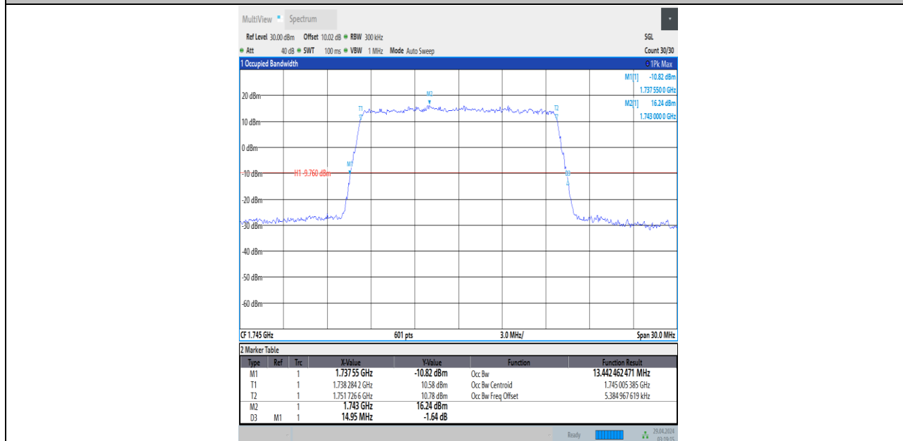
Band66-15MHz-QPSK-132322-75RB#0-PASS
