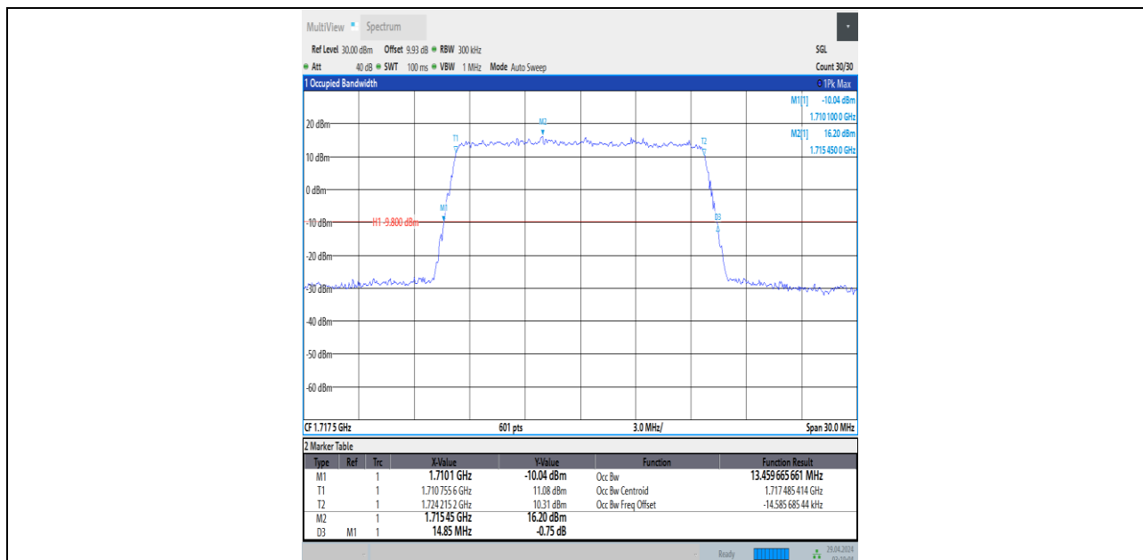
Band66-15MHz-QPSK-132047-75RB#0-PASS
