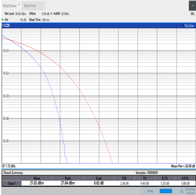
Band66-20MHz-QPSK-132072-100RB#0-PASS
