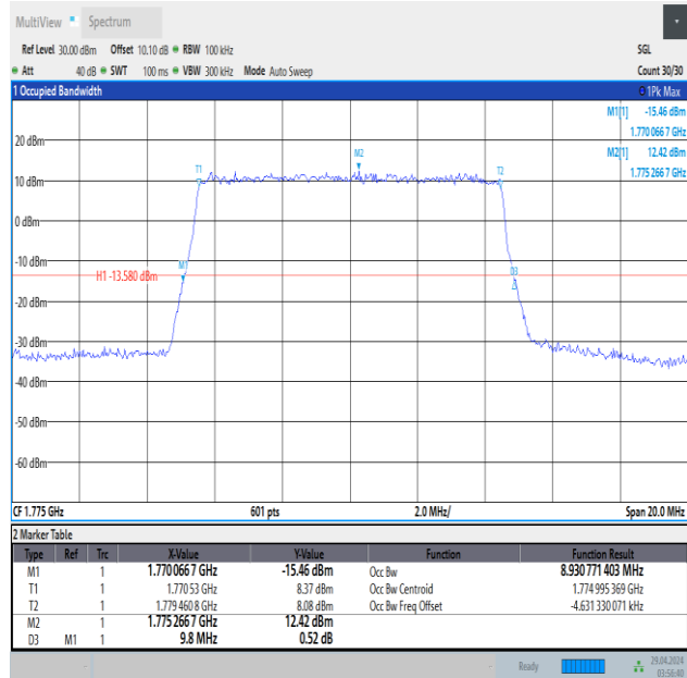
Band66-10MHz-QPSK-132622-50RB#0-PASS
