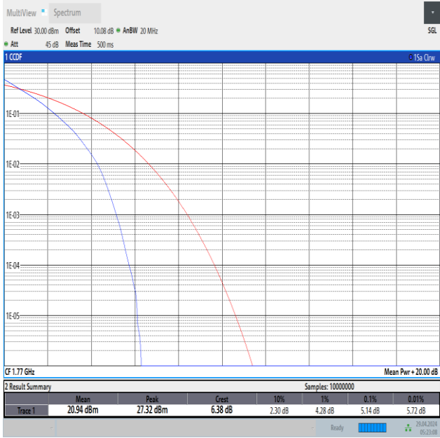
Band66-20MHz-QPSK-132572-100RB#0-PASS
