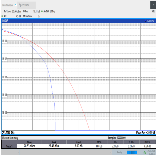
Band66-1.4MHz-16QAM-132665-6RB#0-PASS
