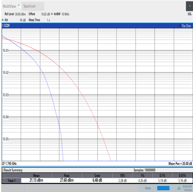
Band66-10MHz-QPSK-132322-50RB#0-PASS
