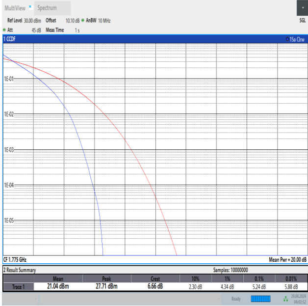
Band66-10MHz-QPSK-132622-50RB#0-PASS
