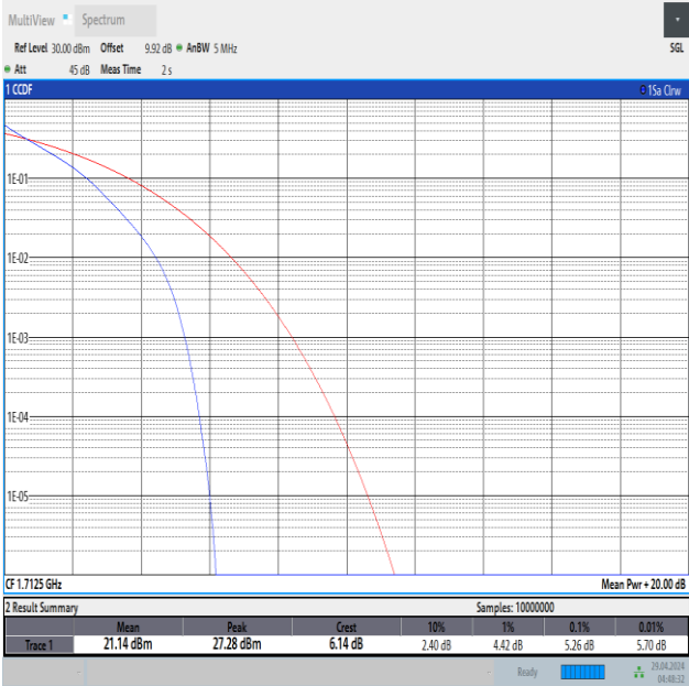
Band66-5MHz-QPSK-131997-25RB#0-PASS
