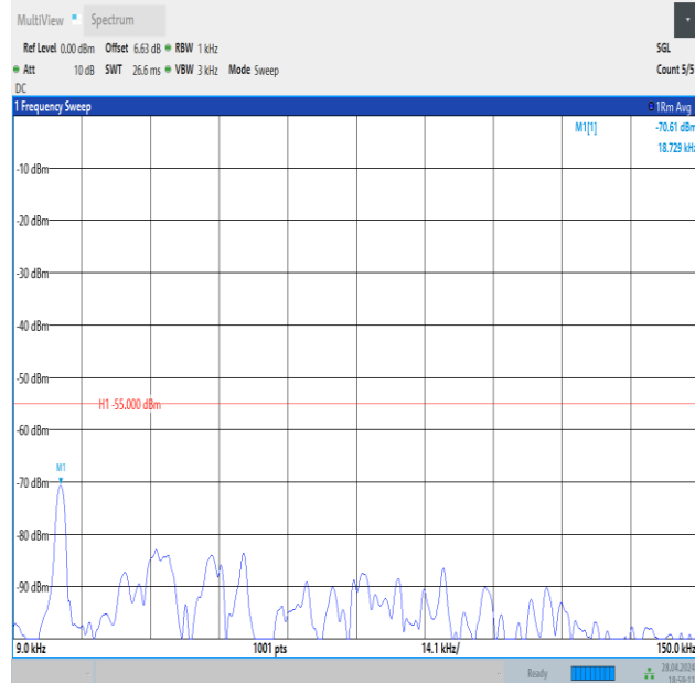
Band41_20MHz_QPSK_40620_1RB#99_0.009~0.15_0.009~0.15
