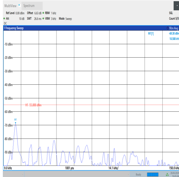
Band41_15MHz_QPSK_40620_75RB#0_0.009~0.15_0.009~0.15
