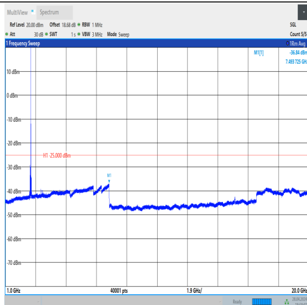
Band41_20MHz_QPSK_40620_1RB#0_1000~20000_1000~20000
