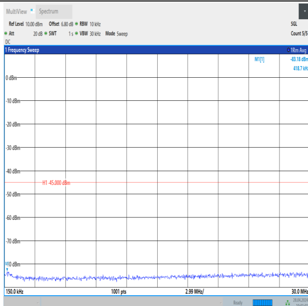
Band41_20MHz_QPSK_41490_1RB#0_0.15~30_0.15~30
