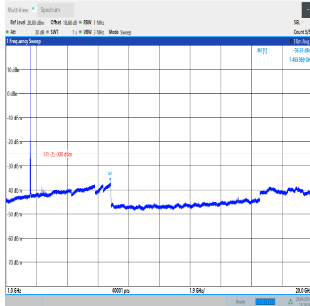
Band41_15MHz_16QAM_39725_1RB#74_1000~20000_1000~20000
