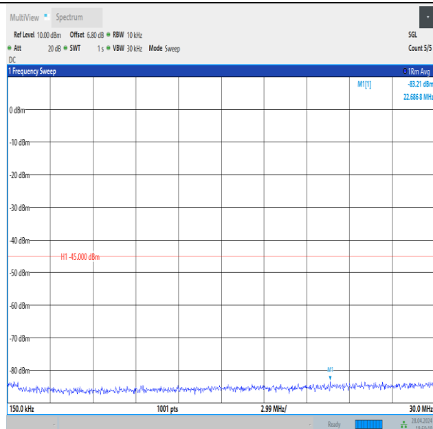
Band41_20MHz_QPSK_40620_1RB#99_0.15~30_0.15~30
