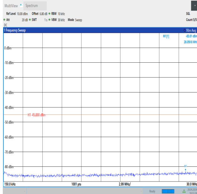
Band41_20MHz_QPSK_41490_100RB#0_0.15~30_0.15~30
