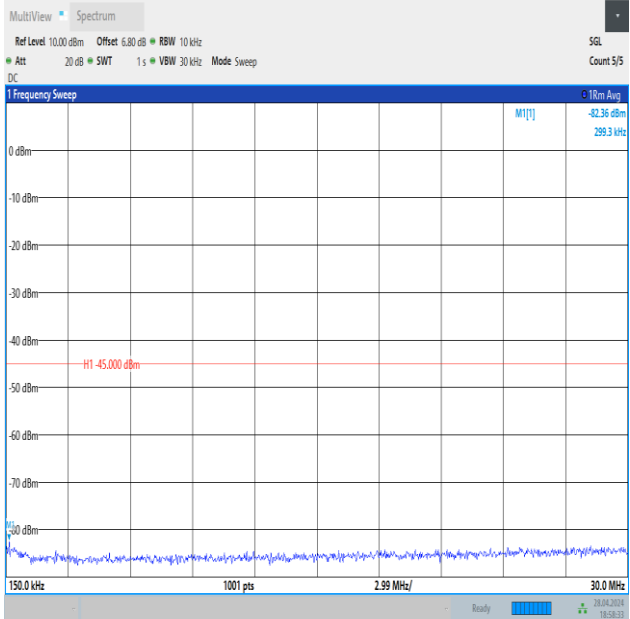
Band41_20MHz_16QAM_40620_1RB#0_0.15~30_0.15~30
