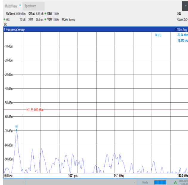
Band41_20MHz_16QAM_39750_1RB#99_0.009~0.15_0.009~0.15
