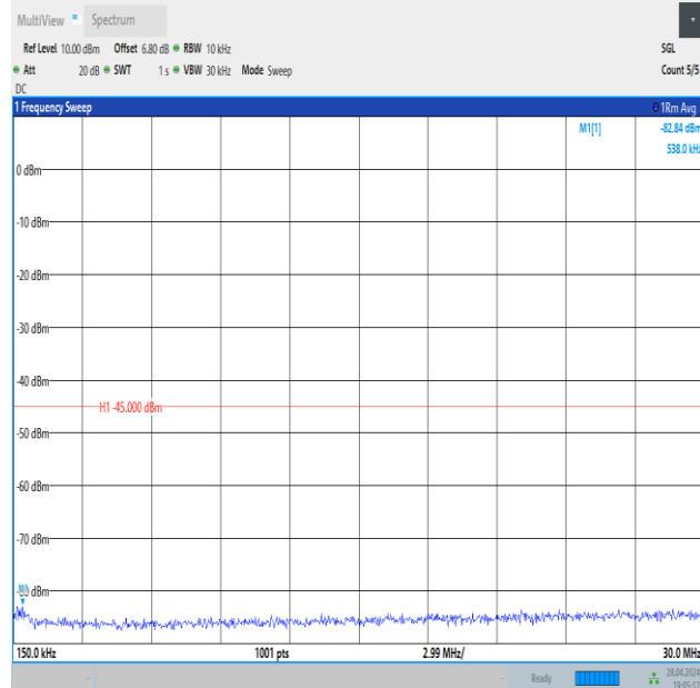
Band41_15MHz_QPSK_40620_75RB#0_0.15~30_0.15~30
