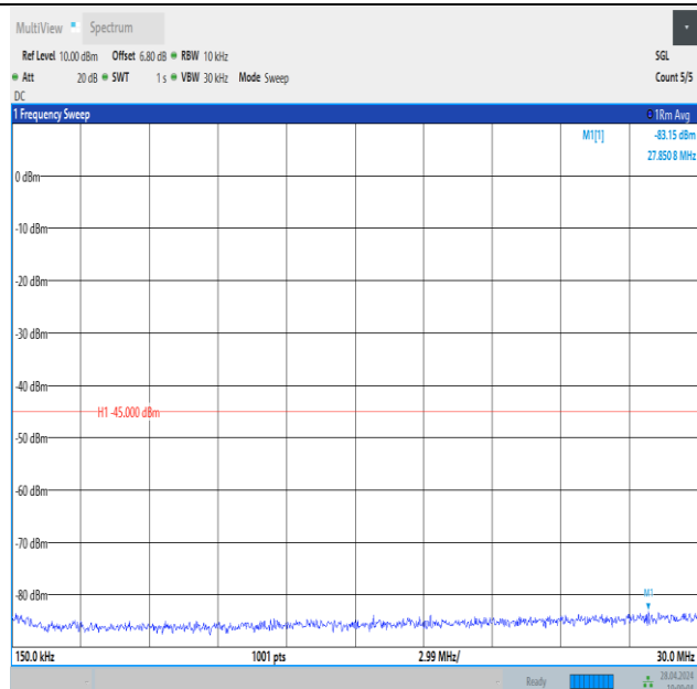
Band41_15MHz_16QAM_39725_1RB#0_0.15~30_0.15~30
