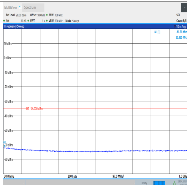
Band41_20MHz_16QAM_41490_1RB#99_30~1000_30~1000
