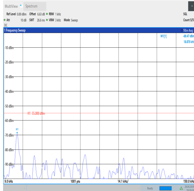
Band41_20MHz_16QAM_40620_1RB#99_0.009~0.15_0.009~0.15
