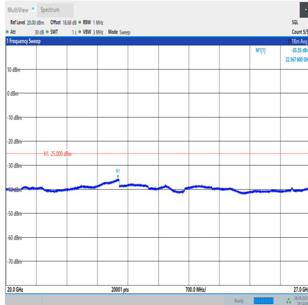
Band41_20MHz_QPSK_41490_100RB#0_20000~27000_20000~27000
