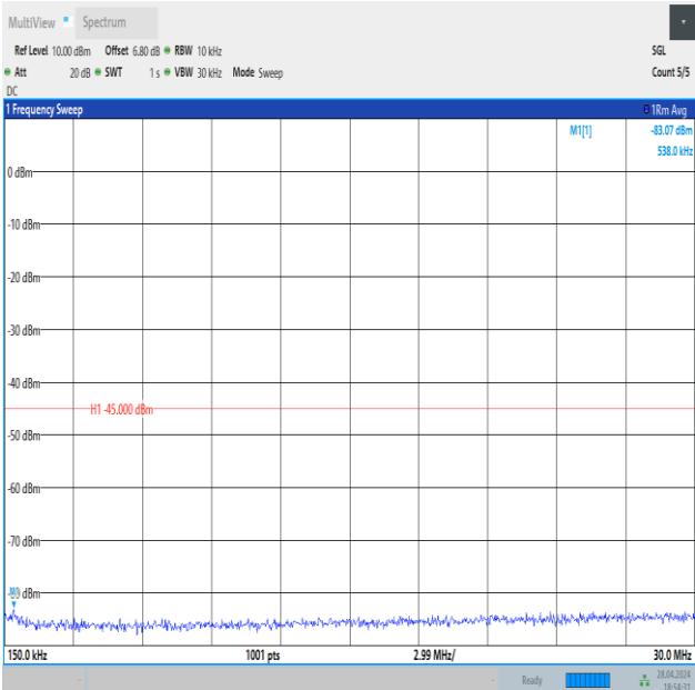
Band41_20MHz_QPSK_39750_1RB#0_0.15~30_0.15~30
