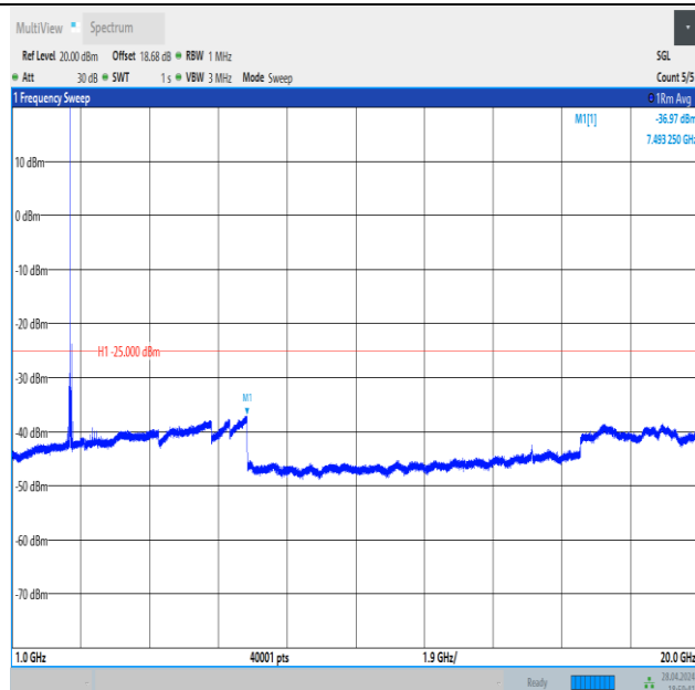
Band41_20MHz_QPSK_40620_1RB#99_1000~20000_1000~20000
