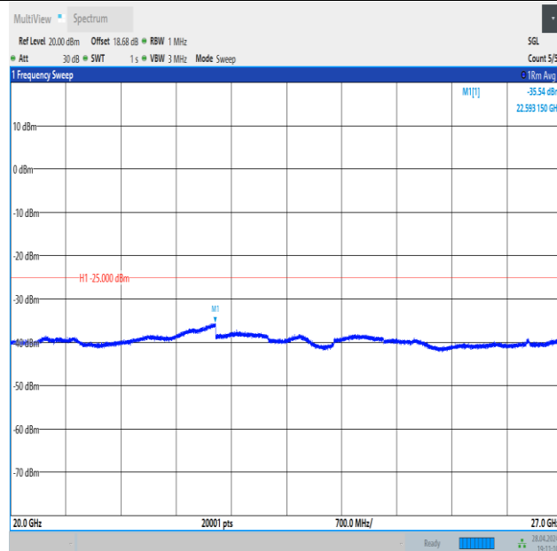
Band41_15MHz_16QAM_39725_1RB#74_20000~27000_20000~27000
