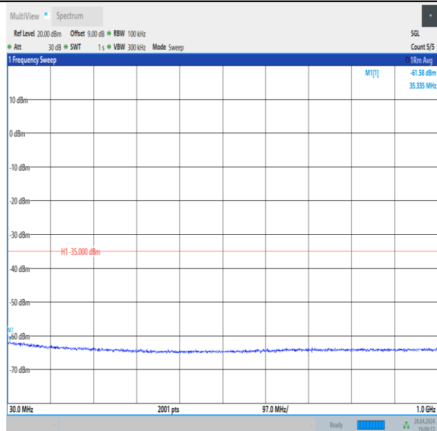
Band41_15MHz_16QAM_39725_1RB#0_30~1000_30~1000
