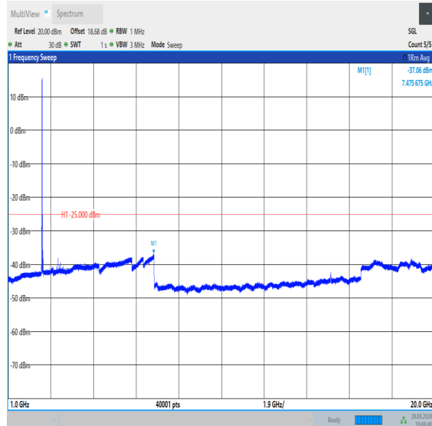
Band41_15MHz_QPSK_39725_75RB#0_1000~20000_1000~20000
