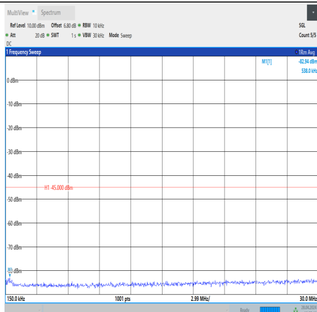
Band41_20MHz_QPSK_40620_1RB#0_0.15~30_0.15~30
