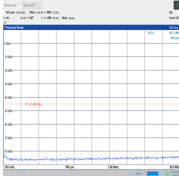
Band41_20MHz_16QAM_41490_1RB#99_0.15~30_0.15~30
