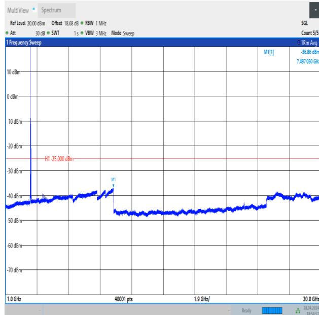
Band41_20MHz_QPSK_39750_1RB#0_1000~20000_1000~20000
