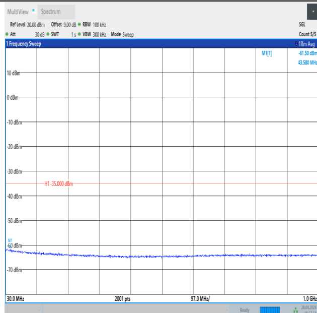
Band41_20MHz_QPSK_40620_1RB#0_30~1000_30~1000
