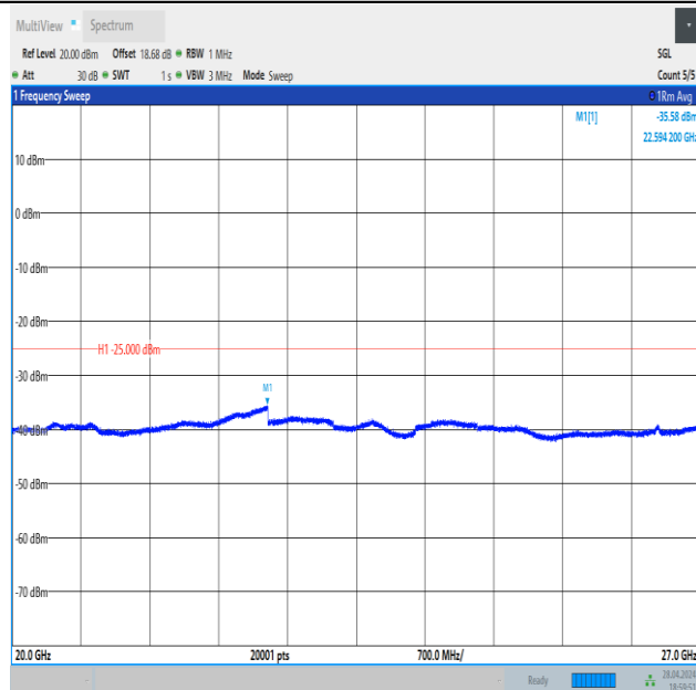
Band41_20MHz_QPSK_40620_1RB#99_20000~27000_20000~27000
