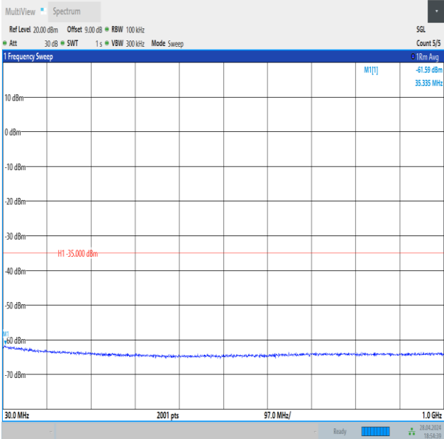
Band41_20MHz_QPSK_39750_1RB#0_30~1000_30~1000
