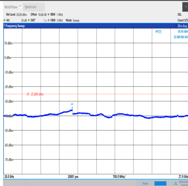
Band41_15MHz_QPSK_40620_75RB#0_20000~27000_20000~27000
