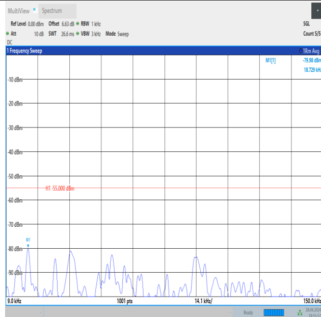
Band41_20MHz_QPSK_39750_1RB#99_0.009~0.15_0.009~0.15
