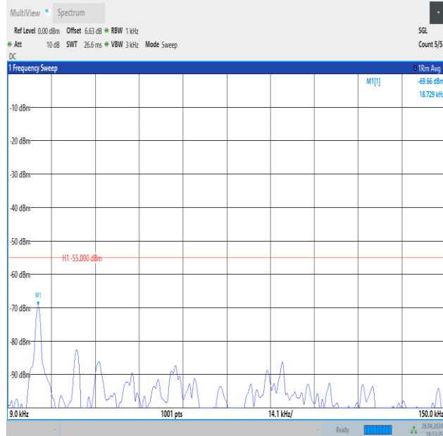
Band41_20MHz_QPSK_41490_100RB#0_0.009~0.15_0.009~0.15
