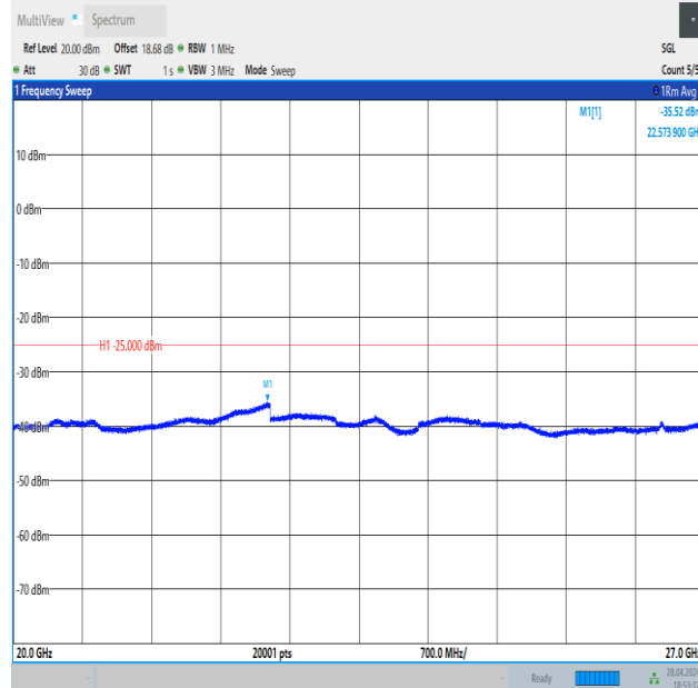
Band41_20MHz_QPSK_40620_100RB#0_20000~27000_20000~27000
