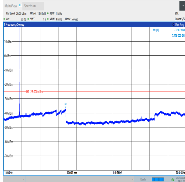
Band41_20MHz_QPSK_41490_1RB#99_1000~20000_1000~20000
