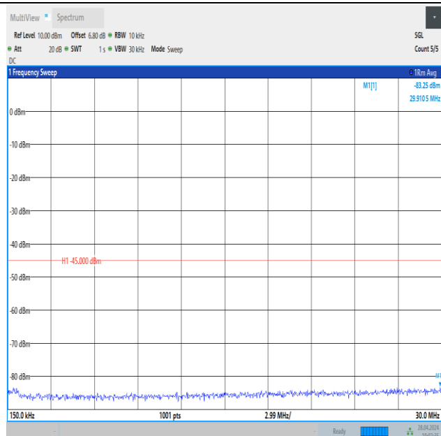
Band41_20MHz_QPSK_41490_1RB#99_0.15~30_0.15~30
