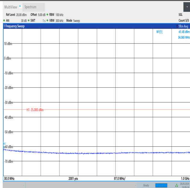
Band41_15MHz_QPSK_39725_1RB#74_30~1000_30~1000
