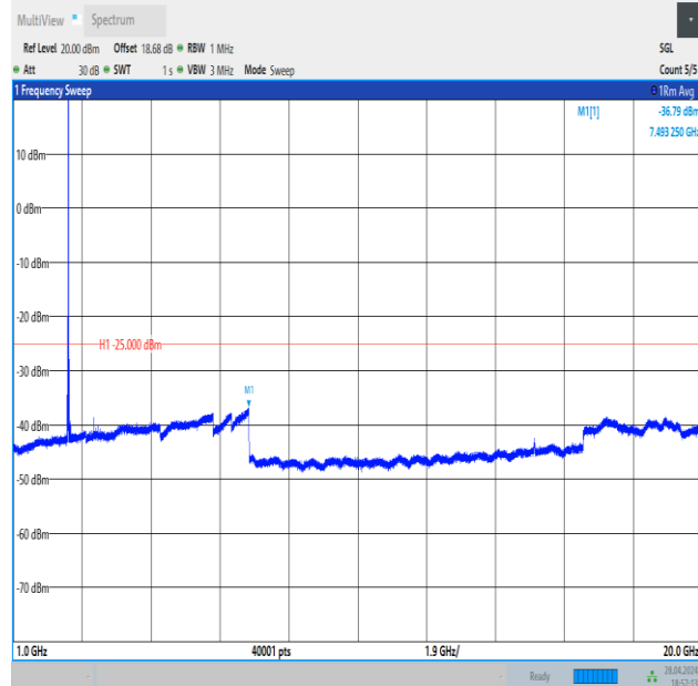
Band41_20MHz_16QAM_39750_1RB#99_1000~20000_1000~20000
