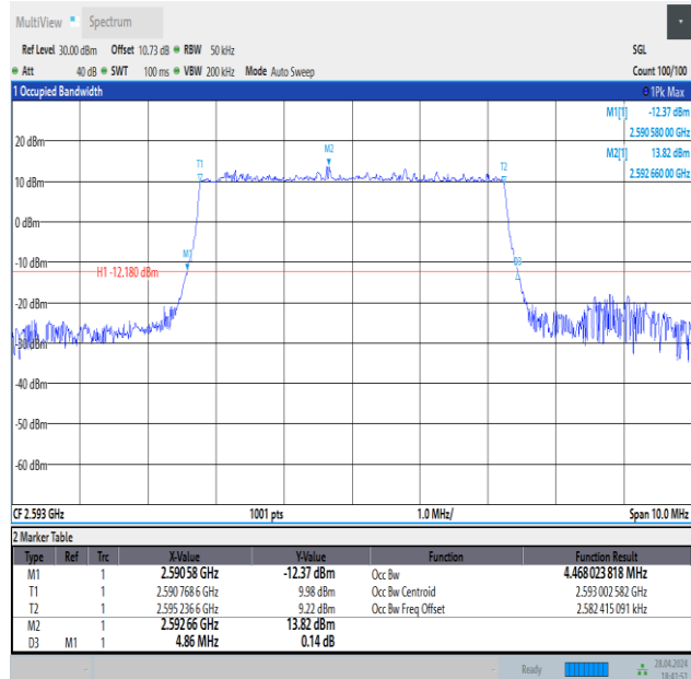
Band41-5MHz-QPSK-40620-25RB#0-PASS
