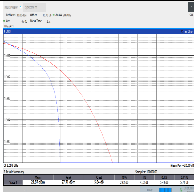
Band41-15MHz-QPSK-40620-75RB#0-PASS
