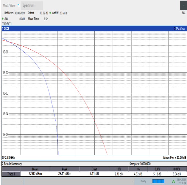
Band41-20MHz-QPSK-41490-100RB#0-PASS
