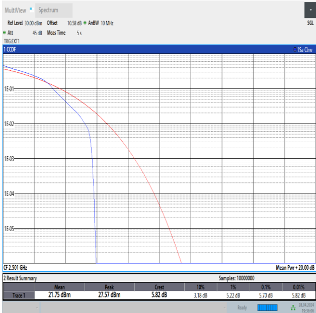
Band41-10MHz-16QAM-39700-1RB#0-PASS
