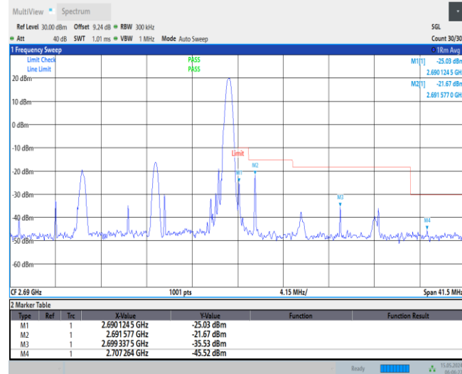
Band41-15MHz-QPSK-41515-75RB#0
