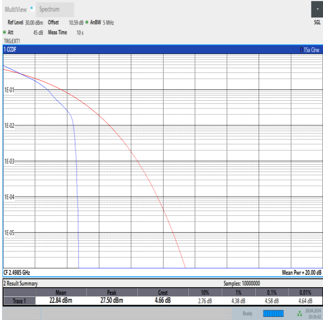
Band41-5MHz-QPSK-39675-1RB#0-PASS
