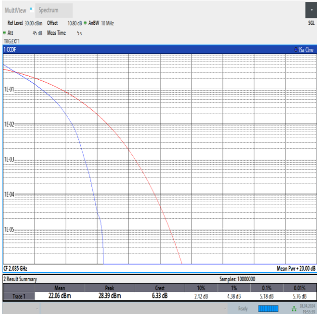
Band41-10MHz-QPSK-41540-50RB#0-PASS
