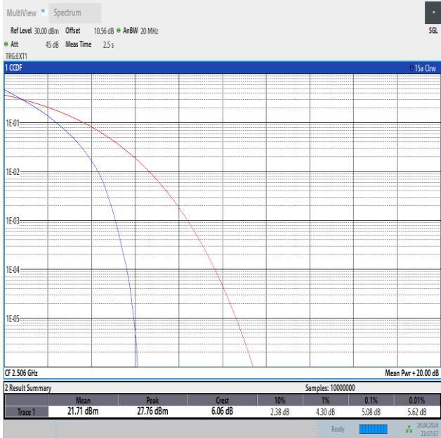
Band41-20MHz-QPSK-39750-100RB#0-PASS
