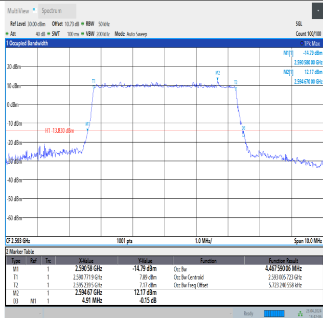
Band41-5MHz-16QAM-40620-25RB#0-PASS
