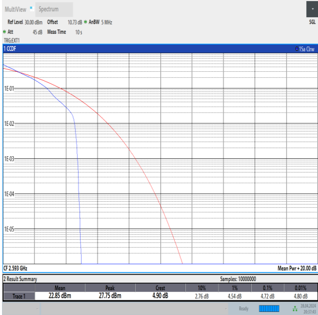
Band41-5MHz-QPSK-40620-1RB#0-PASS
