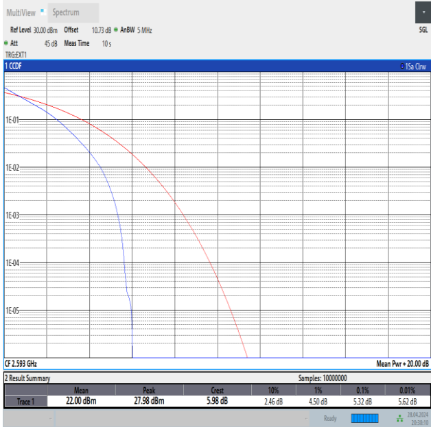
Band41-5MHz-QPSK-40620-25RB#0-PASS
