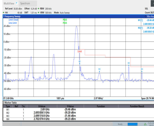
Band41-10MHz-QPSK-41540-50RB#0
