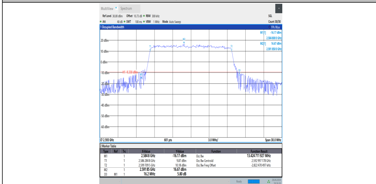
Band41-15MHz-QPSK-40620-75RB#0-PASS
