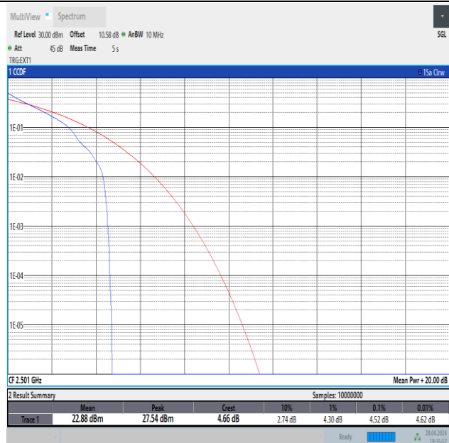
Band41-10MHz-QPSK-39700-1RB#0-PASS
