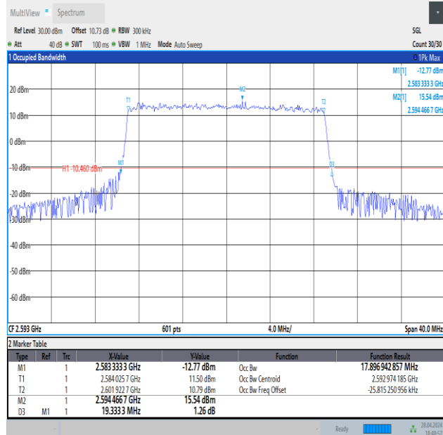
Band41-20MHz-QPSK-40620-100RB#0-PASS
