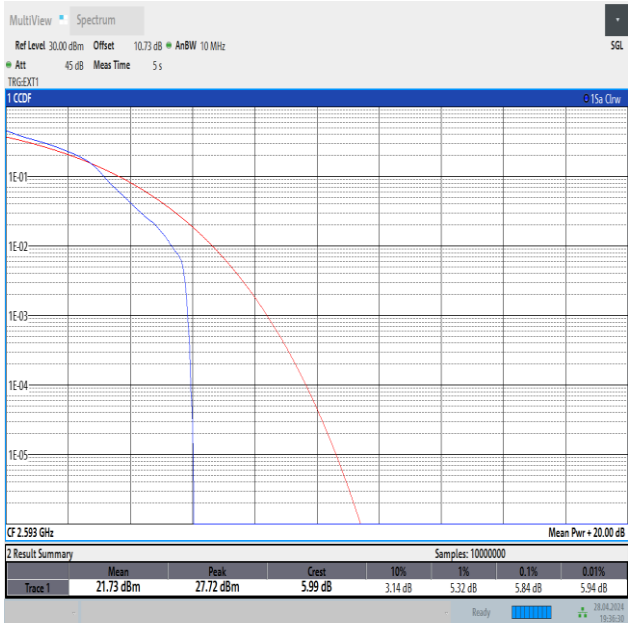
Band41-10MHz-16QAM-40620-1RB#0-PASS
