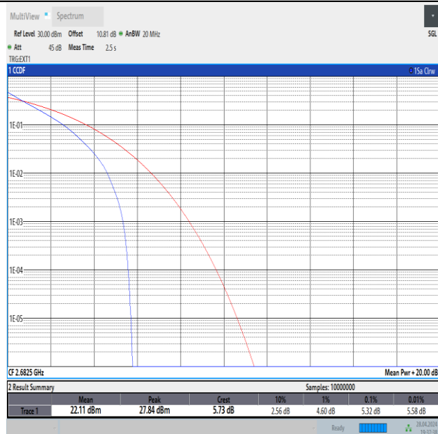
Band41-15MHz-QPSK-41515-75RB#0-PASS
