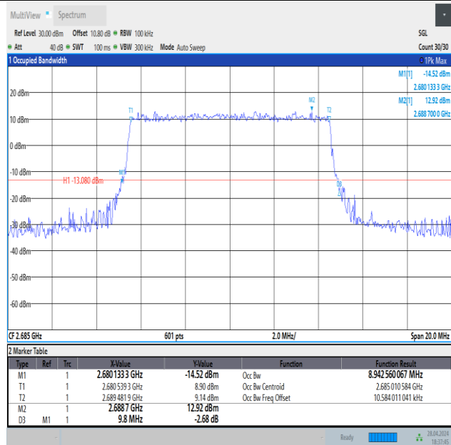
Band41-10MHz-QPSK-41540-50RB#0-PASS
