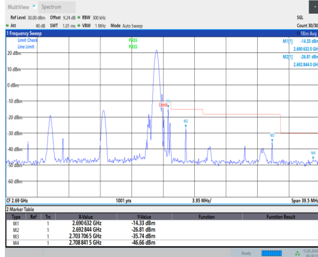
Band41-20MHz-QPSK-39750-1RB#0
