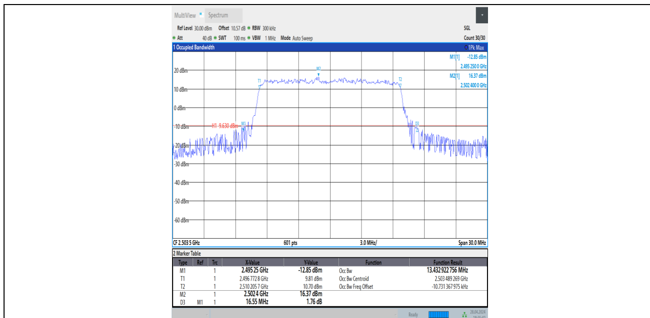
Band41-15MHz-QPSK-39725-75RB#0-PASS
