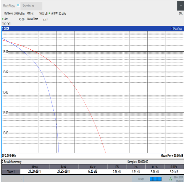
Band41-20MHz-QPSK-40620-100RB#0-PASS
