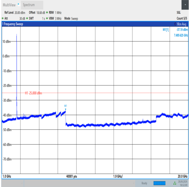
Band41_20MHz_QPSK_39750_100RB#0_1000~20000_1000~20000
