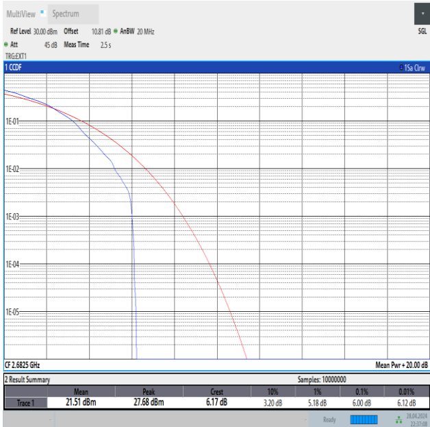
Band41-15MHz-16QAM-41515-1RB#0-PASS
