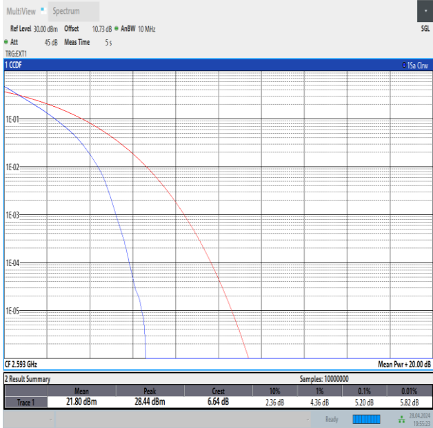
Band41-10MHz-QPSK-40620-50RB#0-PASS
