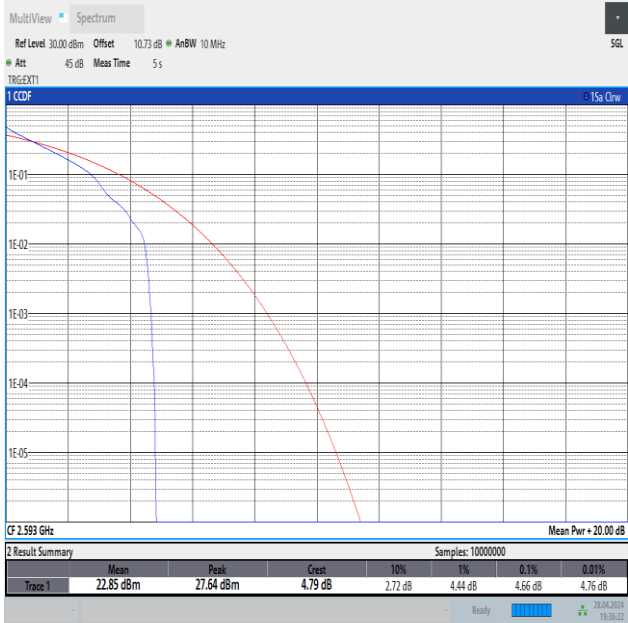
Band41-10MHz-QPSK-40620-1RB#0-PASS
