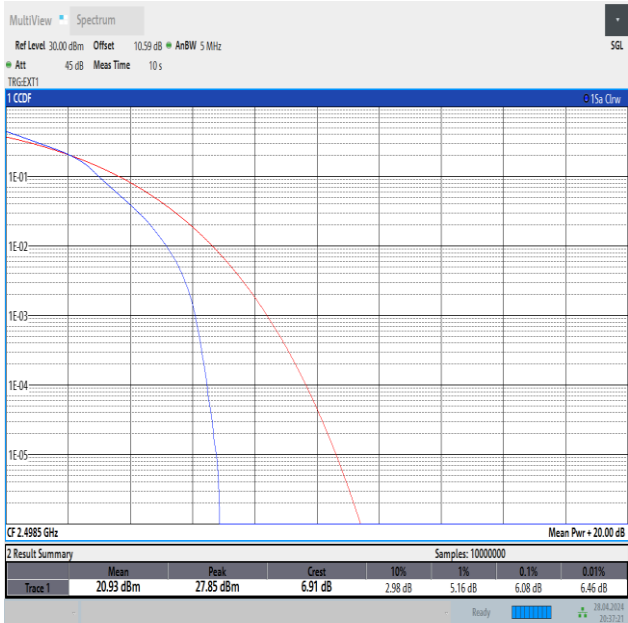
Band41-5MHz-16QAM-39675-25RB#0-PASS
