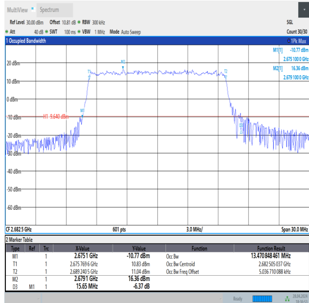
Band41-15MHz-QPSK-41515-75RB#0-PASS
