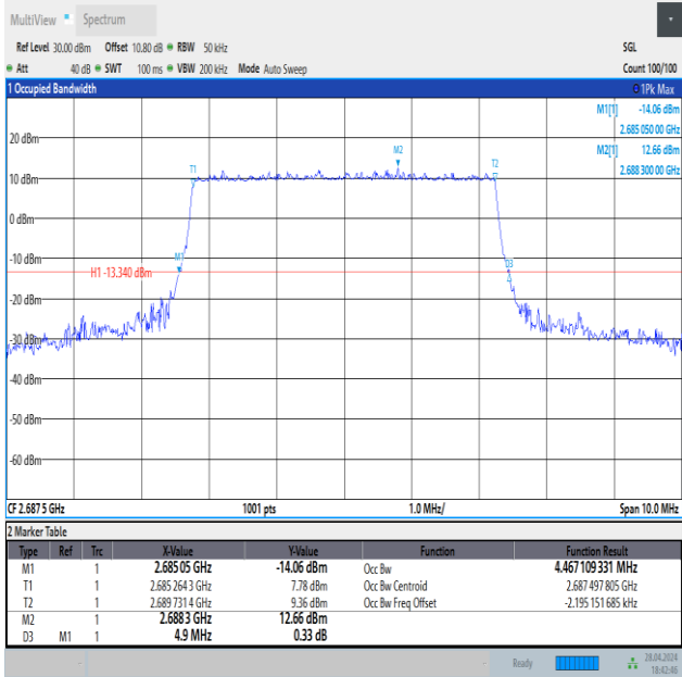
Band41-5MHz-16QAM-41565-25RB#0-PASS
