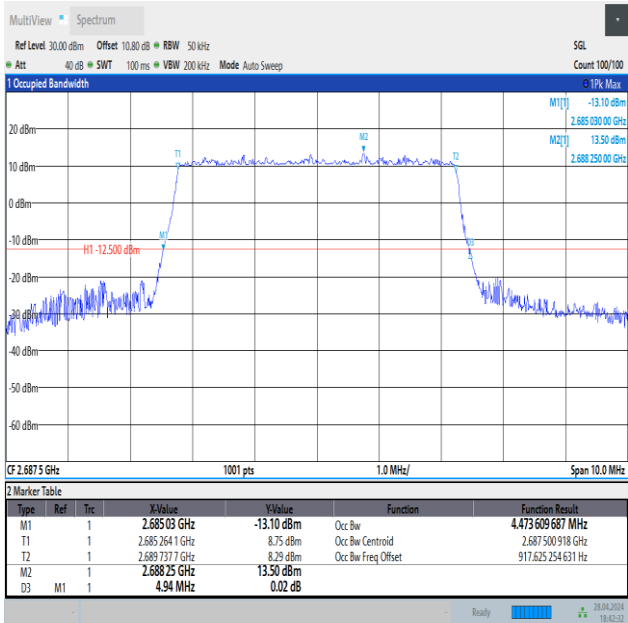
Band41-5MHz-QPSK-41565-25RB#0-PASS
