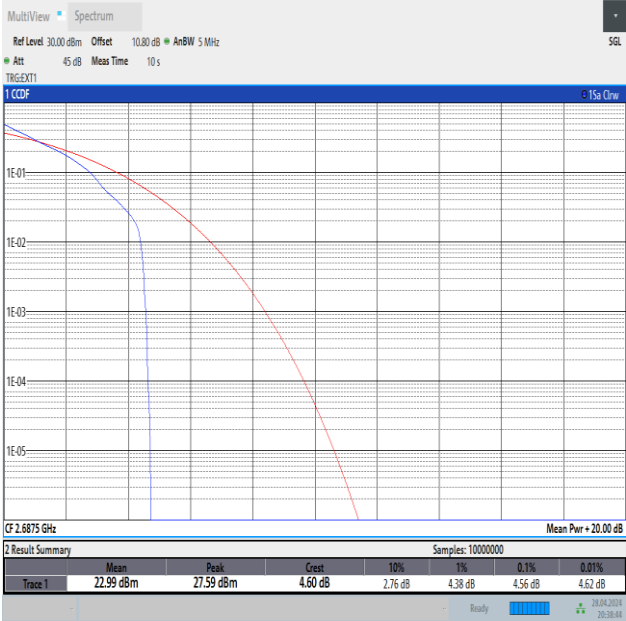
Band41-5MHz-QPSK-41565-1RB#0-PASS
