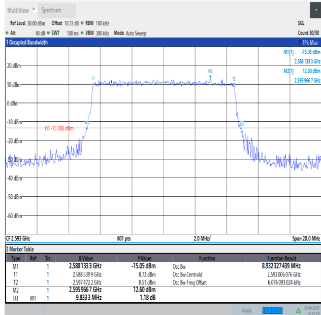
Band41-10MHz-QPSK-40620-50RB#0-PASS
