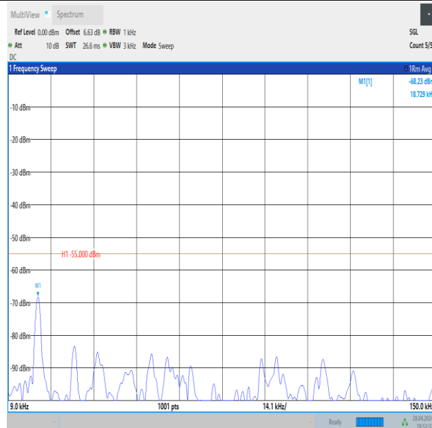
Band41_20MHz_QPSK_40620_100RB#0_0.009~0.15_0.009~0.15
