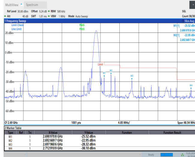
Band41-20MHz-QPSK-41490-100RB#0
