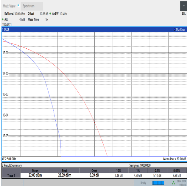
Band41-10MHz-QPSK-39700-50RB#0-PASS
