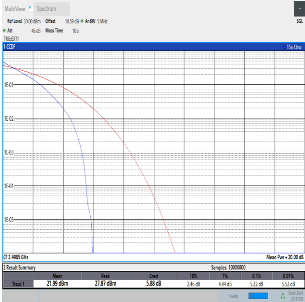
Band41-5MHz-QPSK-39675-25RB#0-PASS
