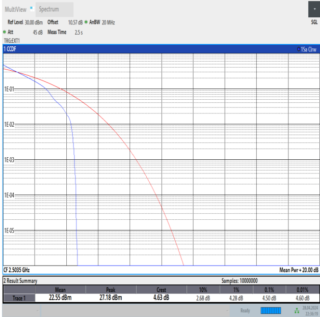
Band41-15MHz-QPSK-39725-1RB#0-PASS
