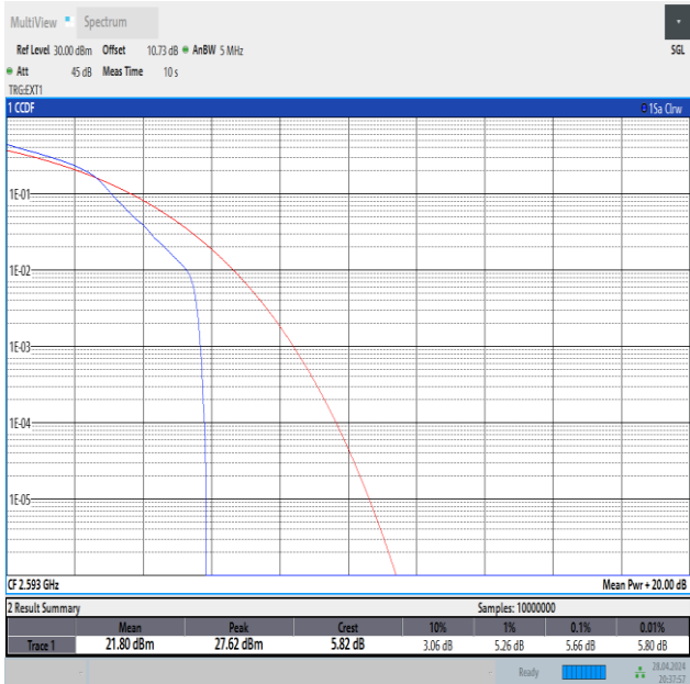
Band41-5MHz-16QAM-40620-1RB#0-PASS
