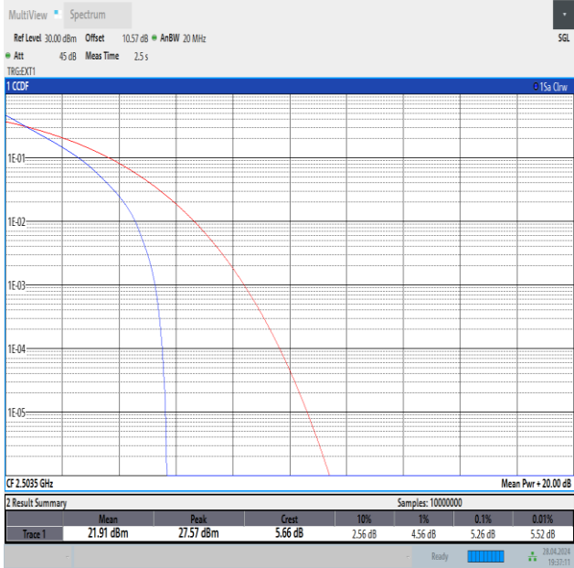
Band41-15MHz-QPSK-39725-75RB#0-PASS
