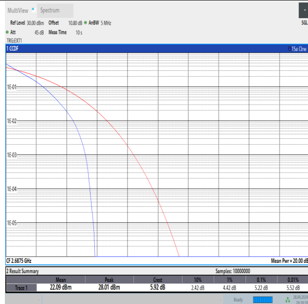
Band41-5MHz-QPSK-41565-25RB#0-PASS
