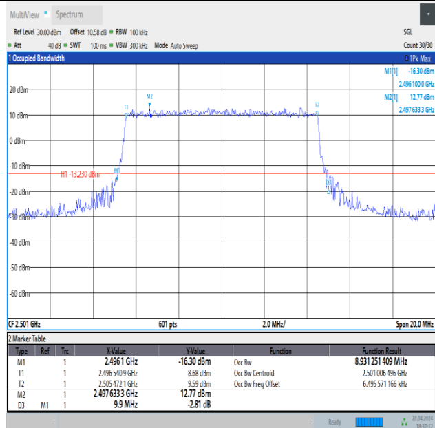
Band41-10MHz-QPSK-39700-50RB#0-PASS
