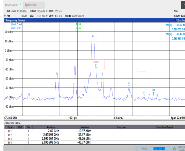
Band41-5MHz-16QAM-41565-25RB#0
