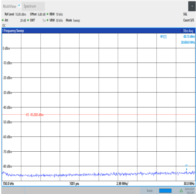
Band41_20MHz_QPSK_40620_100RB#0_0.15~30_0.15~30
