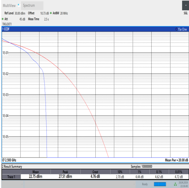
Band41-15MHz-QPSK-40620-1RB#0-PASS
