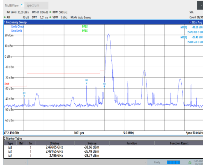
Band41-20MHz-QPSK-39750-100RB#0
