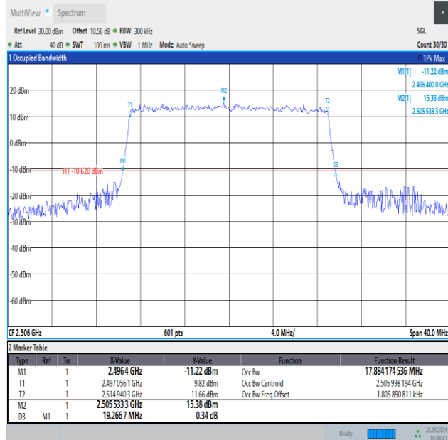
Band41-20MHz-QPSK-39750-100RB#0-PASS
