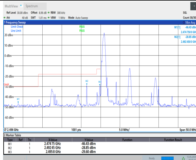
Band41-15MHz-QPSK-39725-75RB#0
