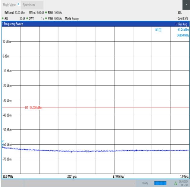
Band41_20MHz_QPSK_40620_100RB#0_30~1000_30~1000
