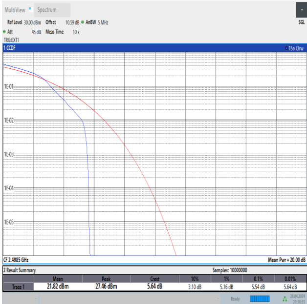
Band41-5MHz-16QAM-39675-1RB#0-PASS
