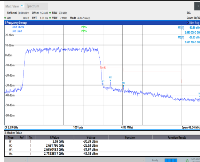
Band41-20MHz-16QAM-39750-1RB#0
