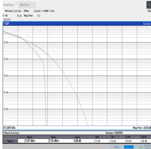
Band41-5MHz-16QAM-41565-1RB#0-PASS
