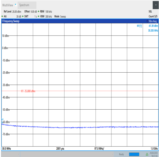
Band41_20MHz_QPSK_39750_100RB#0_30~1000_30~1000
