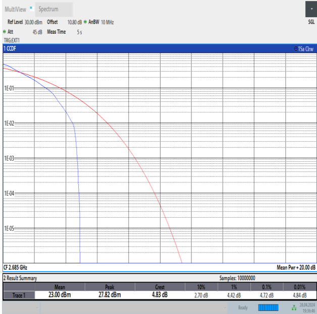
Band41-10MHz-QPSK-41540-1RB#0-PASS
