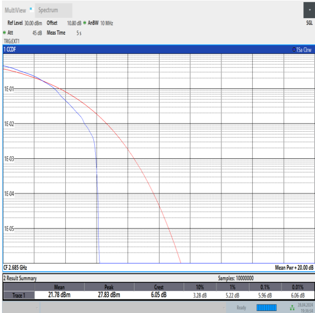
Band41-10MHz-16QAM-41540-1RB#0-PASS
