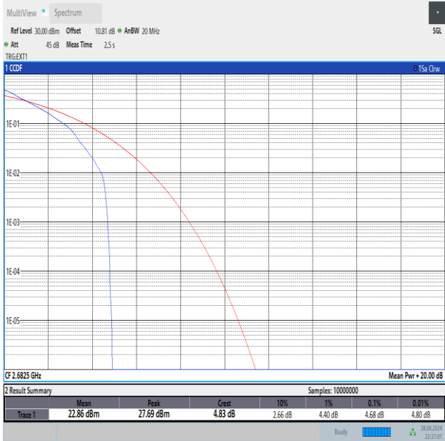
Band41-15MHz-QPSK-41515-1RB#0-PASS
