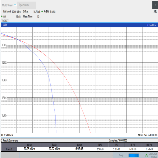
Band41-5MHz-16QAM-40620-25RB#0-PASS
