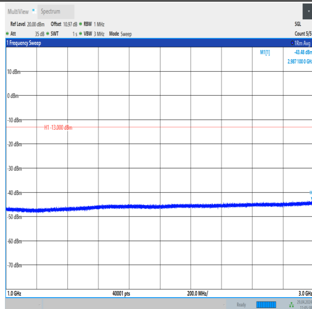
Band26_5MHz_QPSK_27015_1RB#24_1000~3000_1000~3000
