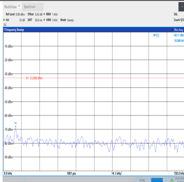
Band26_10MHz_QPSK_26915_1RB#0_0.009~0.15_0.009~0.15
