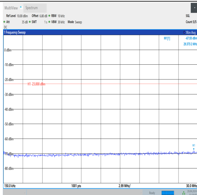
Band26_10MHz_16QAM_26840_1RB#49_0.15~30_0.15~30
