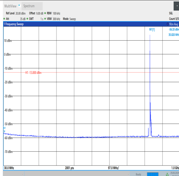
Band26_5MHz_16QAM_26915_1RB#0_30~1000_30~1000
