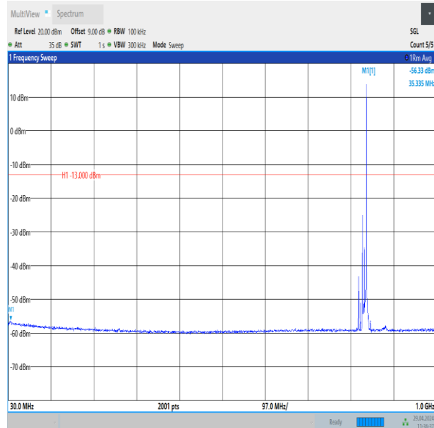
Band26_10MHz_QPSK_26915_1RB#49_30~1000_30~1000
