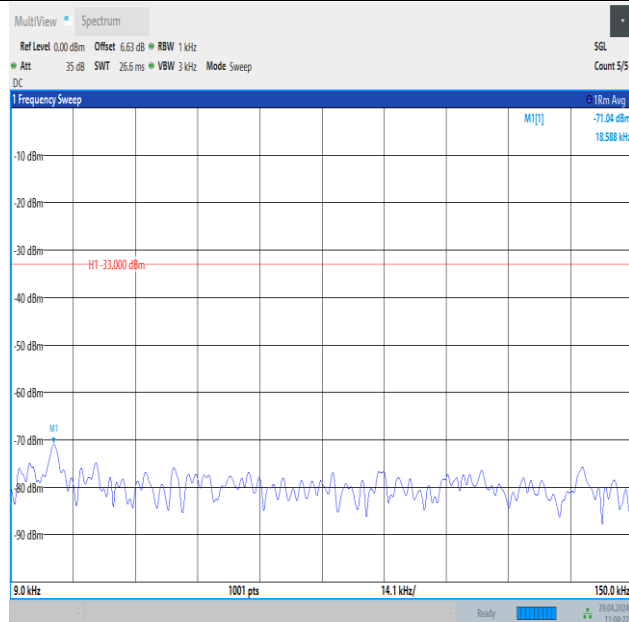
Band26_5MHz_16QAM_27015_1RB#0_0.009~0.15_0.009~0.15
