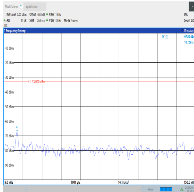
Band26_5MHz_16QAM_26815_25RB#0_0.009~0.15_0.009~0.15
