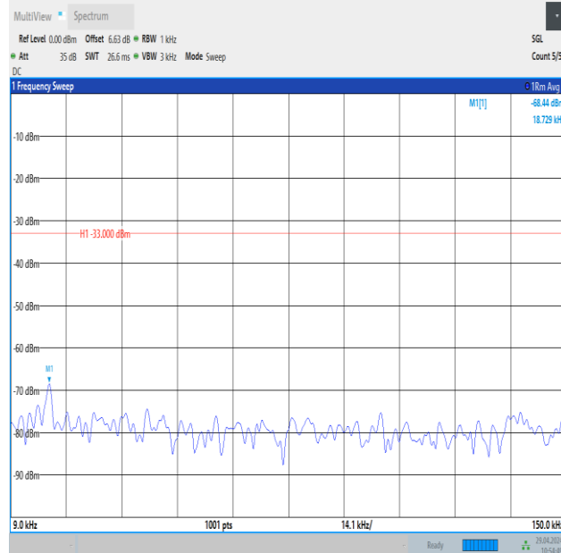
Band26_5MHz_16QAM_26815_1RB#0_0.009~0.15_0.009~0.15
