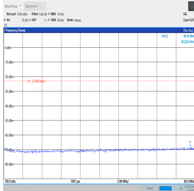
Band26_5MHz_16QAM_27015_1RB#24_0.15~30_0.15~30
