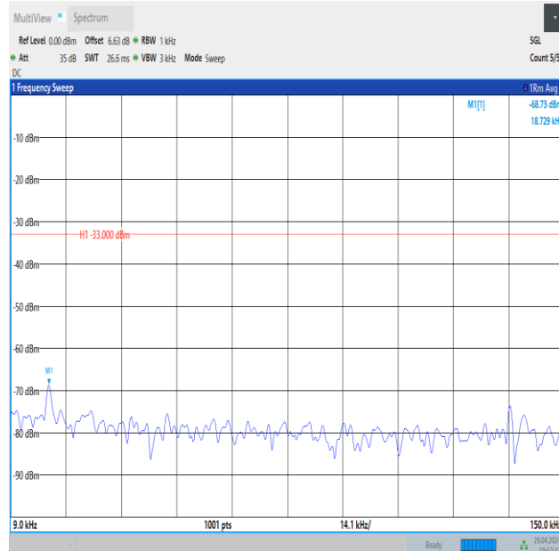
Band26_5MHz_QPSK_26815_25RB#0_0.009~0.15_0.009~0.15
