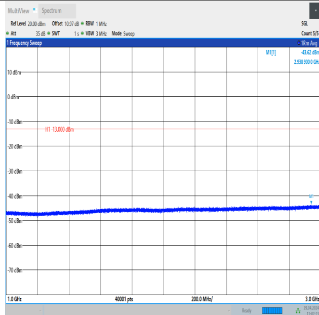
Band26_5MHz_QPSK_27015_25RB#0_1000~3000_1000~3000
