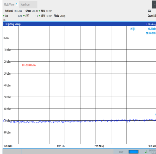
Band26_5MHz_QPSK_26915_25RB#0_0.15~30_0.15~30
