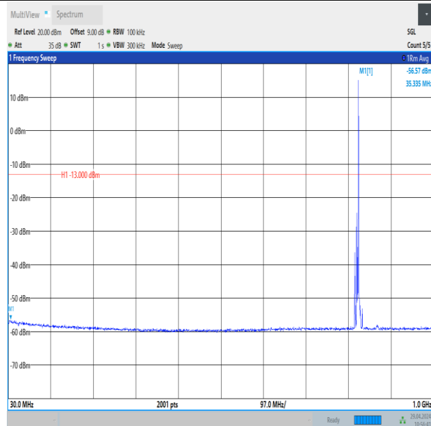
Band26_5MHz_16QAM_26815_1RB#24_30~1000_30~1000
