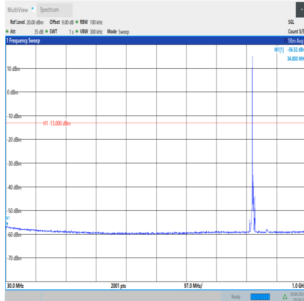
Band26_5MHz_QPSK_26815_1RB#0_30~1000_30~1000
