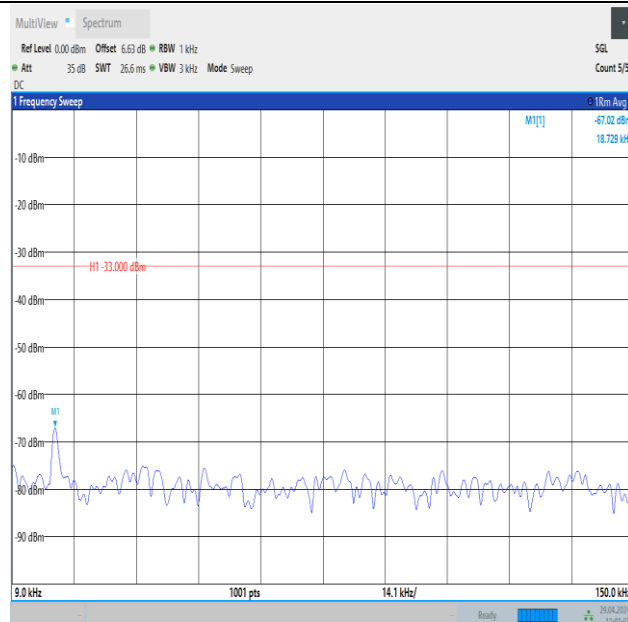
Band26_5MHz_QPSK_26915_25RB#0_0.009~0.15_0.009~0.15
