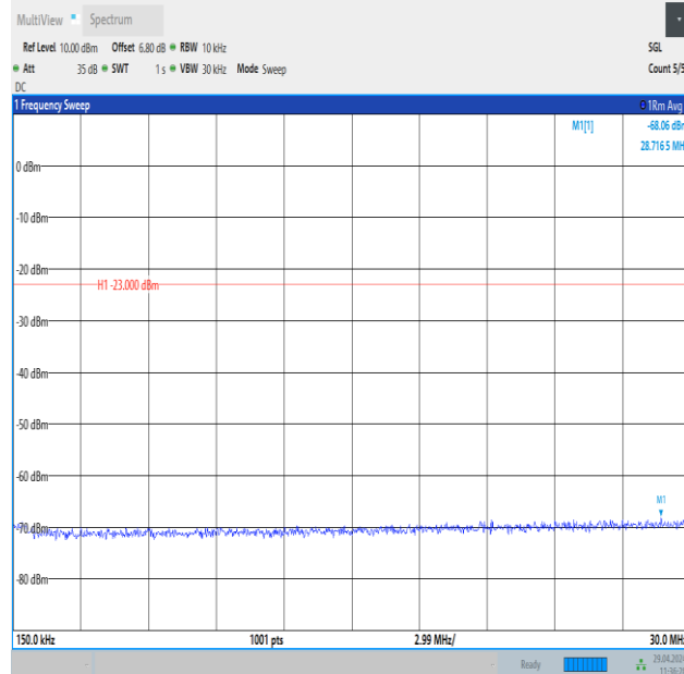
Band26_10MHz_QPSK_26915_1RB#49_0.15~30_0.15~30
