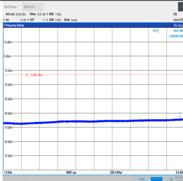
Band26_5MHz_16QAM_26815_25RB#0_1000~3000_1000~3000
