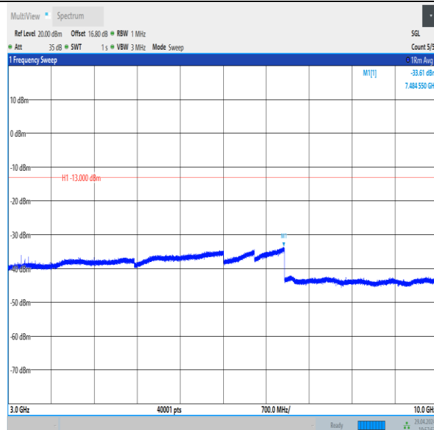
Band26_5MHz_QPSK_26815_25RB#0_3000~10000_3000~10000
