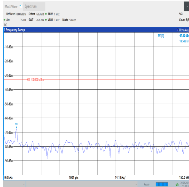
Band26_10MHz_16QAM_26840_1RB#0_0.009~0.15_0.009~0.15
