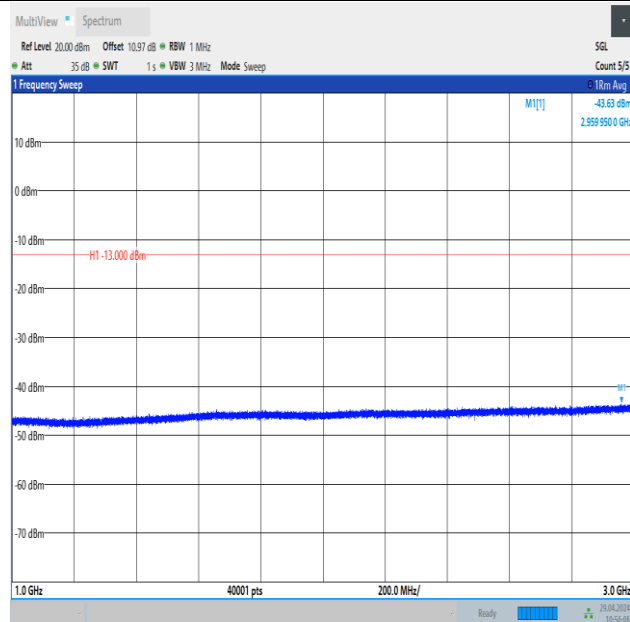
Band26_5MHz_QPSK_26815_1RB#24_1000~3000_1000~3000
