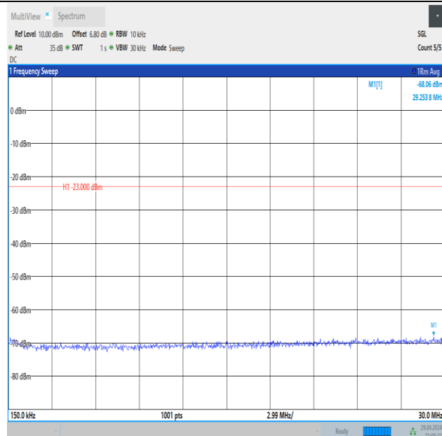
Band26_5MHz_16QAM_27015_1RB#0_0.15~30_0.15~30
