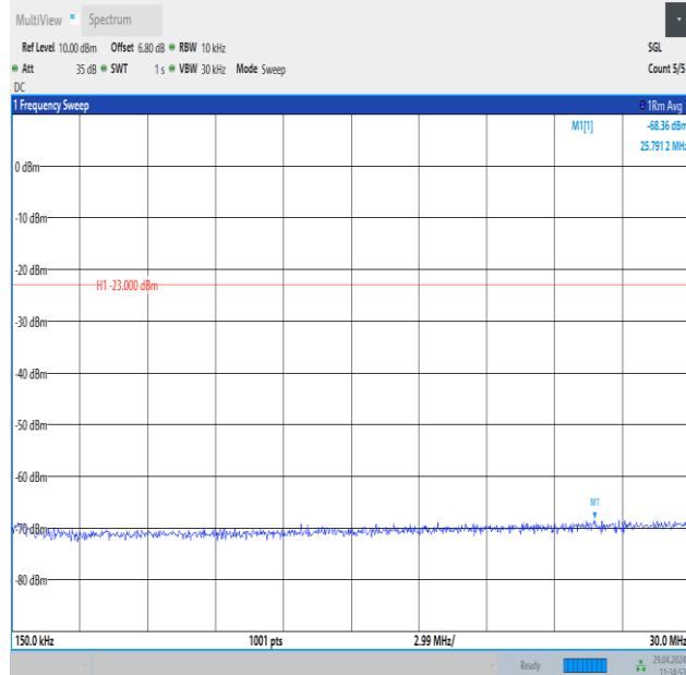
Band26_10MHz_QPSK_26915_1RB#0_0.15~30_0.15~30
