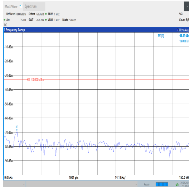
Band26_10MHz_16QAM_26915_1RB#49_0.009~0.15_0.009~0.15
