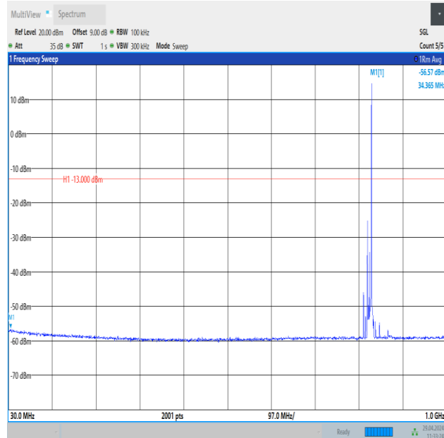
Band26_10MHz_QPSK_26840_1RB#49_30~1000_30~1000
