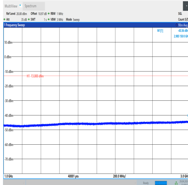
Band26_5MHz_16QAM_27015_1RB#0_1000~3000_1000~3000
