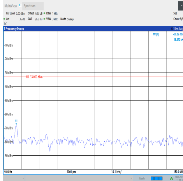
Band26_10MHz_QPSK_26915_1RB#49_0.009~0.15_0.009~0.15
