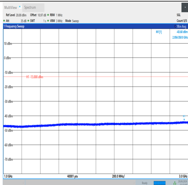
Band26_10MHz_16QAM_26840_1RB#0_1000~3000_1000~3000
