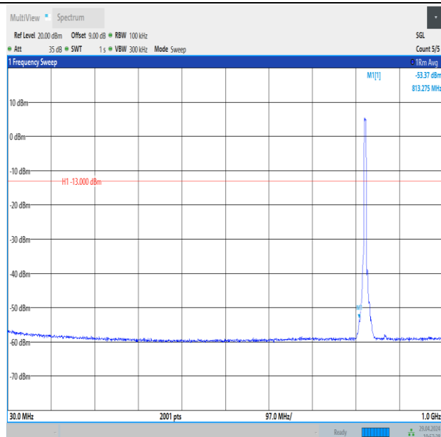
Band26_5MHz_QPSK_26815_25RB#0_30~1000_30~1000
