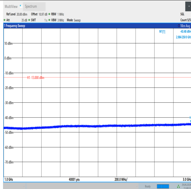
Band26_5MHz_QPSK_26915_1RB#24_1000~3000_1000~3000
