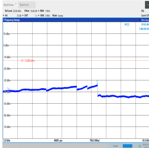
Band26_5MHz_QPSK_27015_1RB#24_3000~10000_3000~10000
