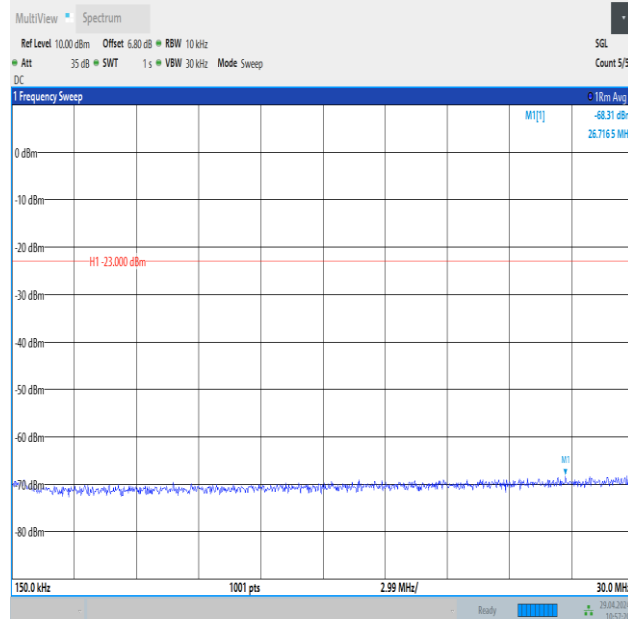
Band26_5MHz_QPSK_26815_25RB#0_0.15~30_0.15~30
