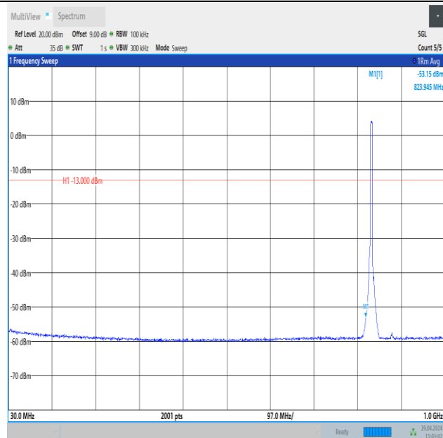
Band26_5MHz_16QAM_26915_25RB#0_30~1000_30~1000
