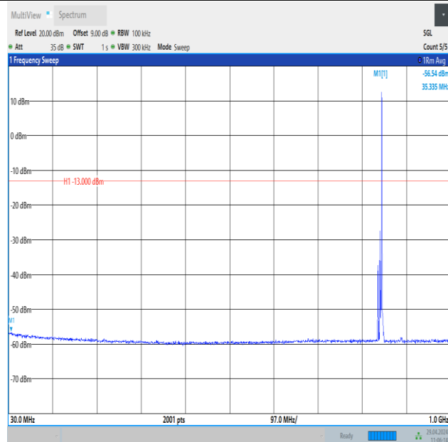
Band26_5MHz_16QAM_27015_1RB#24_30~1000_30~1000
