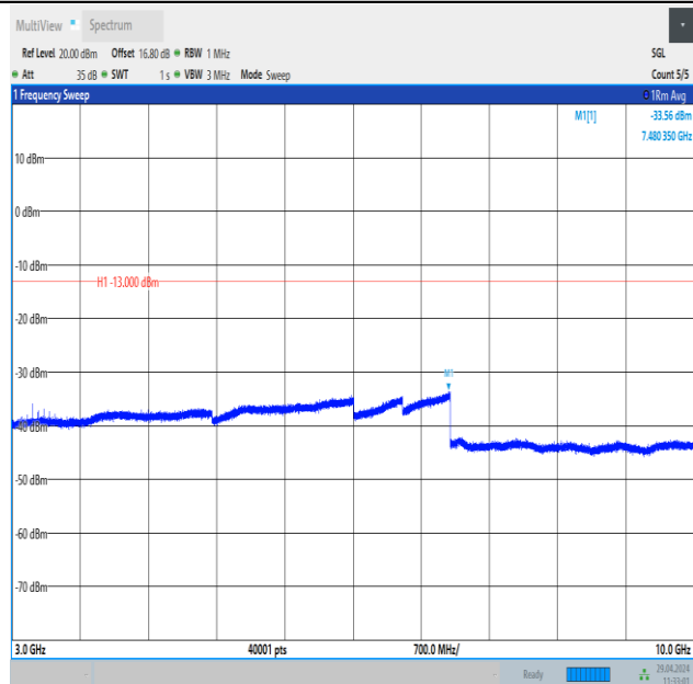
Band26_10MHz_16QAM_26840_1RB#0_3000~10000_3000~10000
