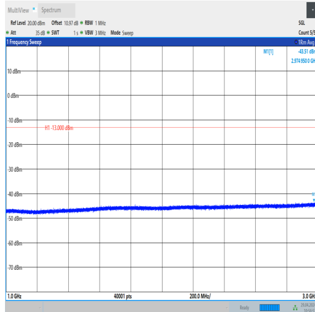
Band26_5MHz_16QAM_26815_1RB#24_1000~3000_1000~3000
