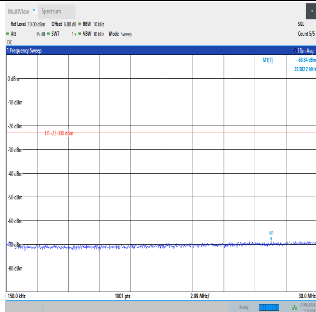
Band26_5MHz_16QAM_26915_25RB#0_0.15~30_0.15~30
