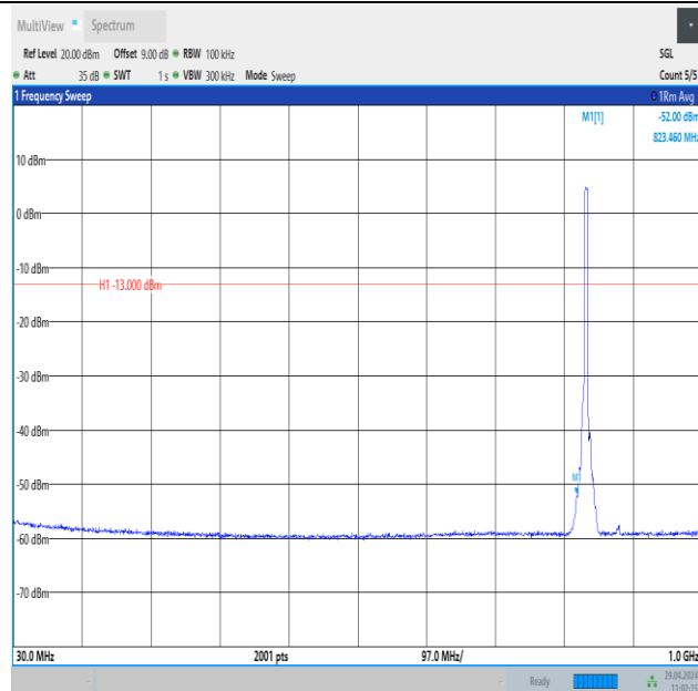
Band26_5MHz_QPSK_26915_25RB#0_30~1000_30~1000
