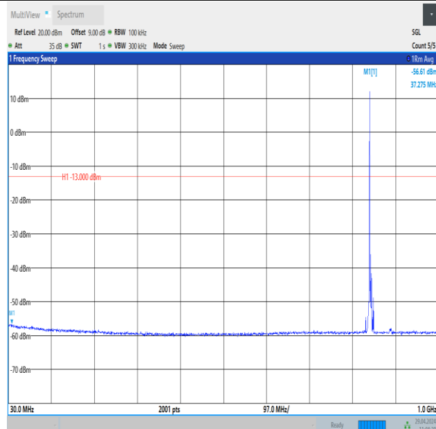
Band26_5MHz_16QAM_27015_1RB#0_30~1000_30~1000
