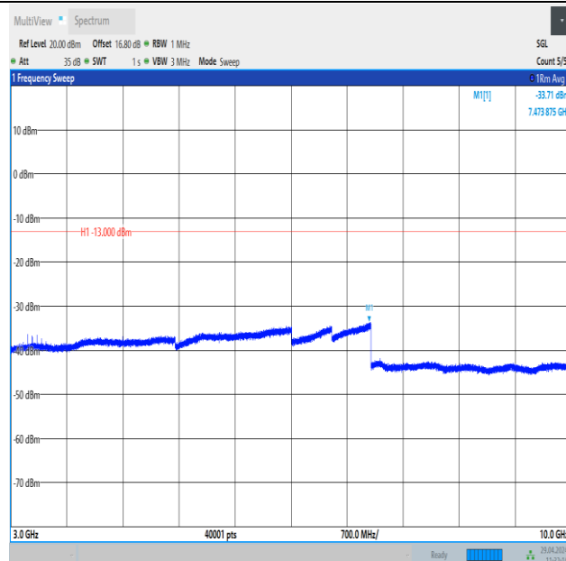
Band26_10MHz_QPSK_26840_1RB#0_3000~10000_3000~10000
