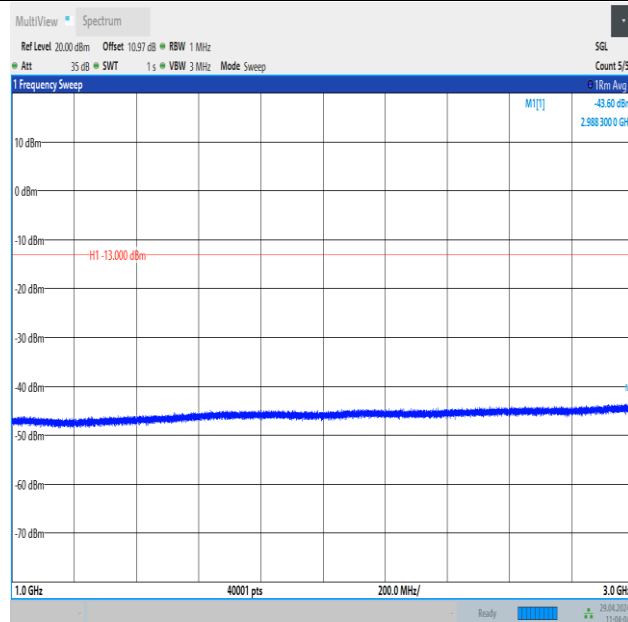
Band26_5MHz_QPSK_27015_1RB#0_1000~3000_1000~3000
