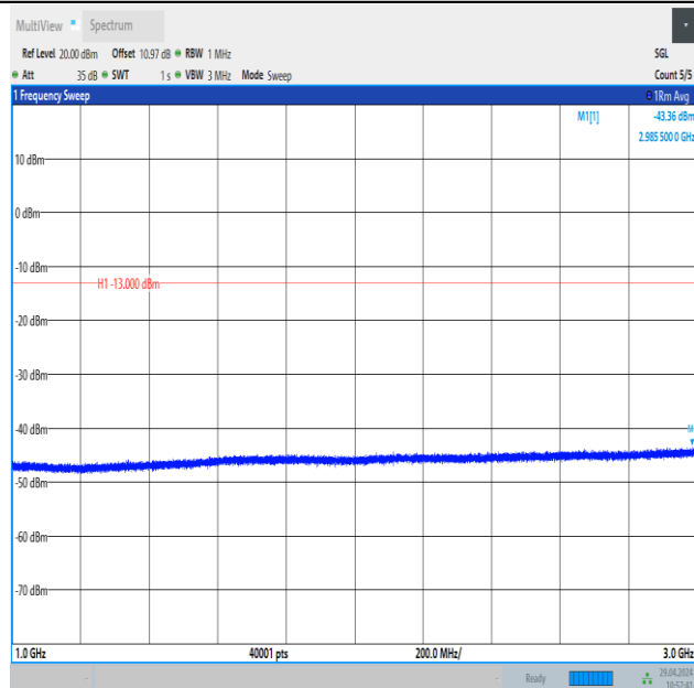
Band26_5MHz_QPSK_26815_25RB#0_1000~3000_1000~3000
