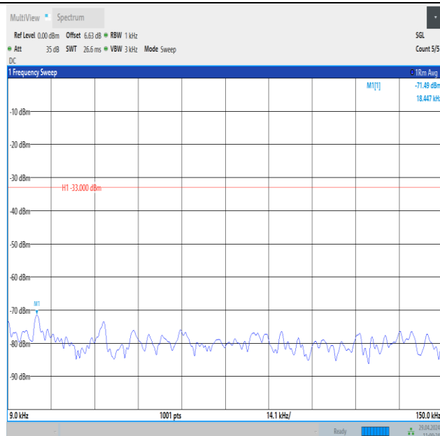
Band26_5MHz_QPSK_26915_1RB#24_0.009~0.15_0.009~0.15
