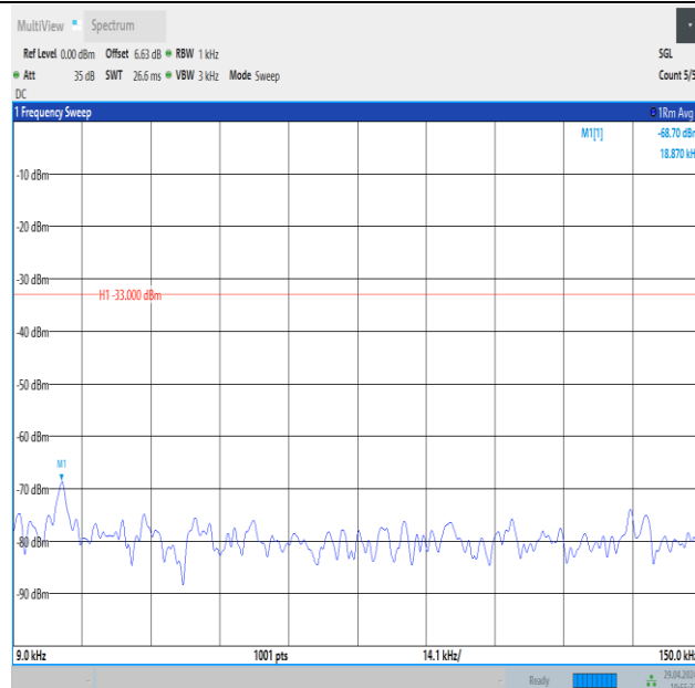
Band26_5MHz_QPSK_26815_1RB#24_0.009~0.15_0.009~0.15
