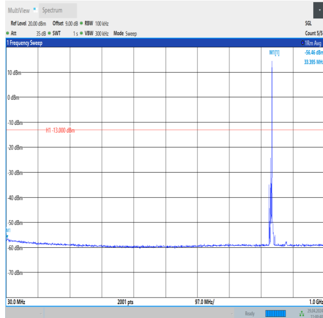
Band26_5MHz_QPSK_26915_1RB#24_30~1000_30~1000
