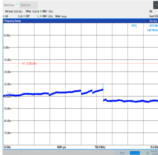
Band26_5MHz_QPSK_26915_1RB#24_3000~10000_3000~10000
