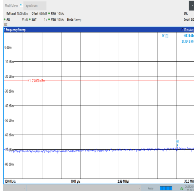
Band26_5MHz_QPSK_27015_1RB#24_0.15~30_0.15~30
