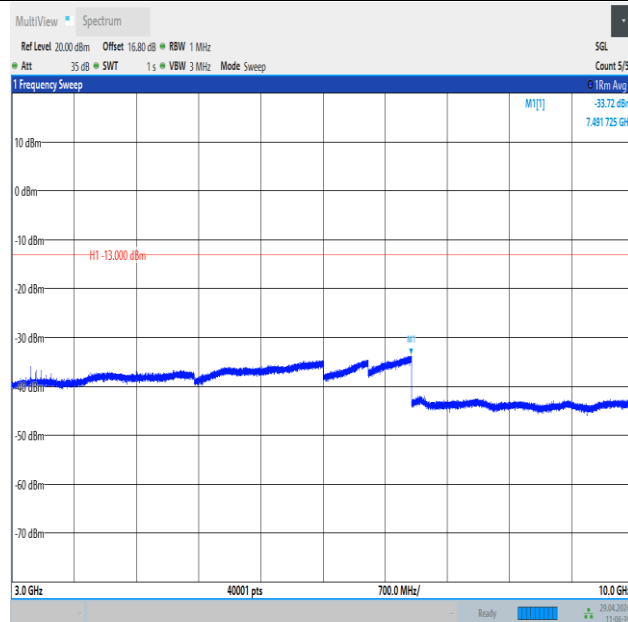
Band26_5MHz_16QAM_27015_1RB#24_3000~10000_3000~10000
