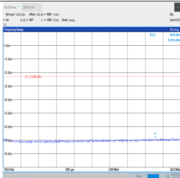
Band26_5MHz_16QAM_26815_1RB#0_0.15~30_0.15~30
