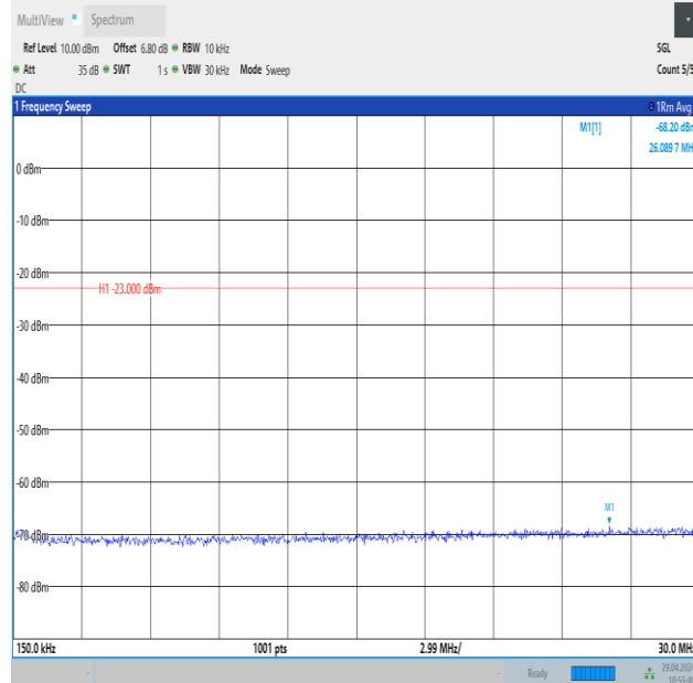
Band26_5MHz_QPSK_26815_1RB#24_0.15~30_0.15~30
