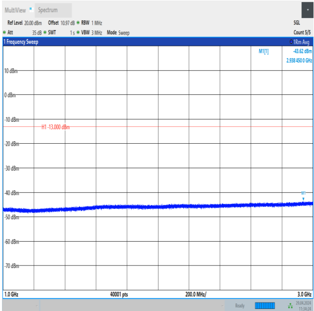
Band26_10MHz_16QAM_26840_1RB#49_1000~3000_1000~3000
