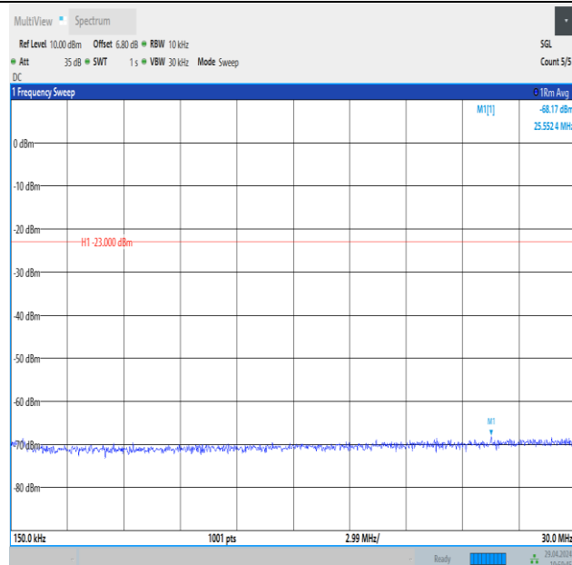
Band26_5MHz_16QAM_26915_1RB#0_0.15~30_0.15~30
