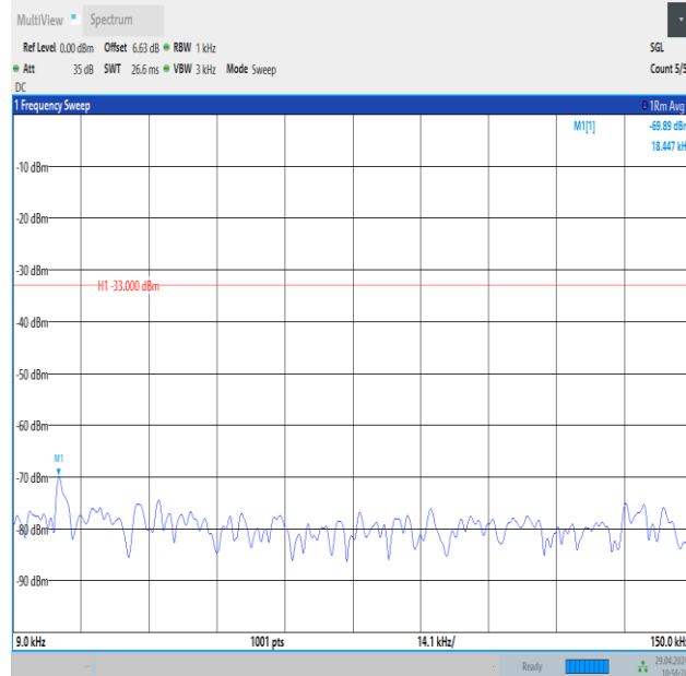
Band26_5MHz_16QAM_26815_1RB#24_0.009~0.15_0.009~0.15
