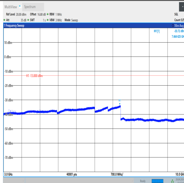
Band26_10MHz_QPSK_26915_1RB#49_3000~10000_3000~10000
