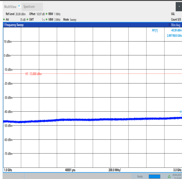
Band26_10MHz_QPSK_26840_1RB#0_1000~3000_1000~3000
