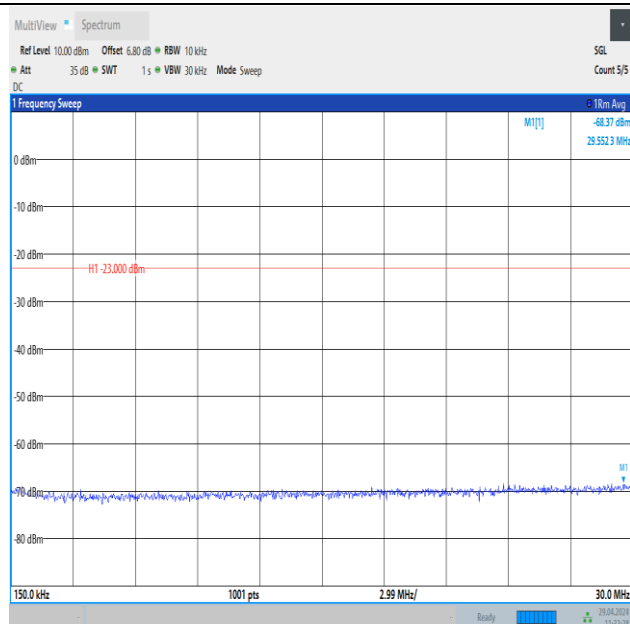
Band26_10MHz_16QAM_26840_1RB#0_0.15~30_0.15~30
