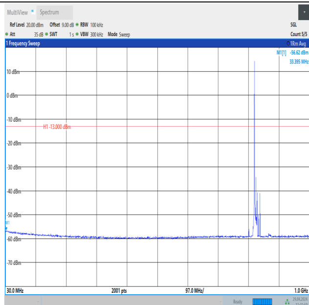
Band26_10MHz_QPSK_26840_1RB#0_30~1000_30~1000
