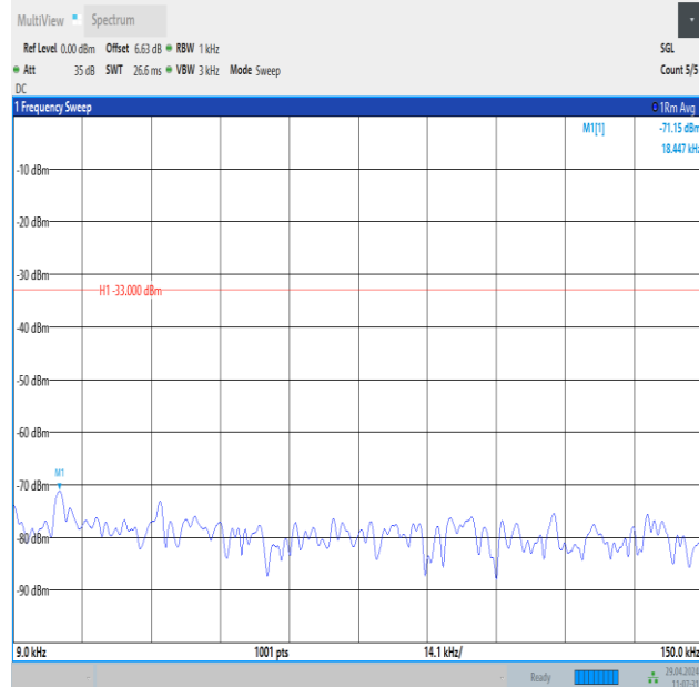
Band26_5MHz_16QAM_27015_25RB#0_0.009~0.15_0.009~0.15
