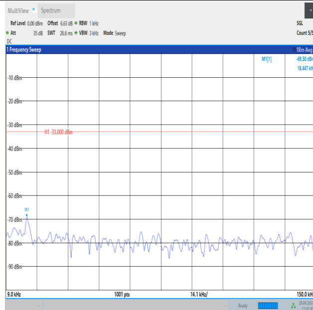
Band26_5MHz_16QAM_26915_25RB#0_0.009~0.15_0.009~0.15
