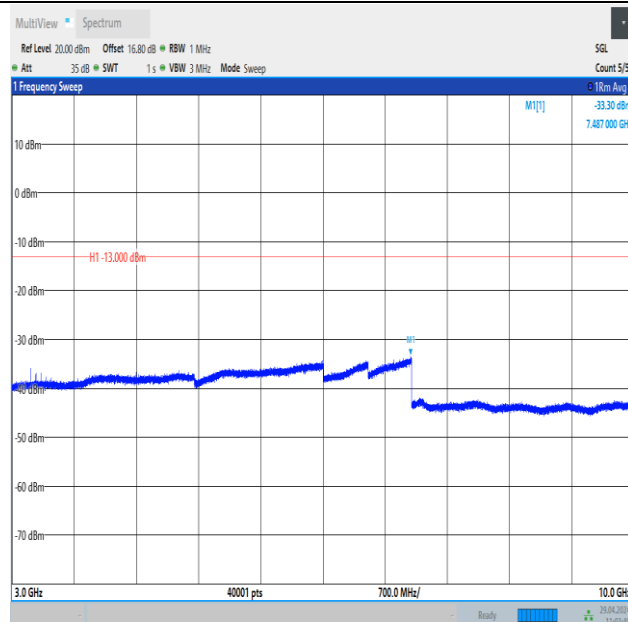
Band26_5MHz_QPSK_26915_25RB#0_3000~10000_3000~10000
