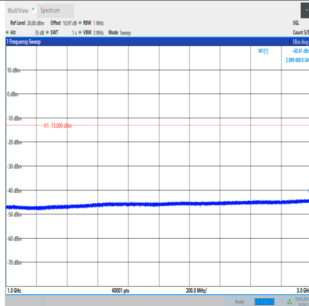
Band26_5MHz_QPSK_26915_1RB#0_1000~3000_1000~3000
