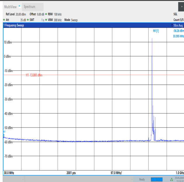
Band26_10MHz_16QAM_26840_1RB#0_30~1000_30~1000
