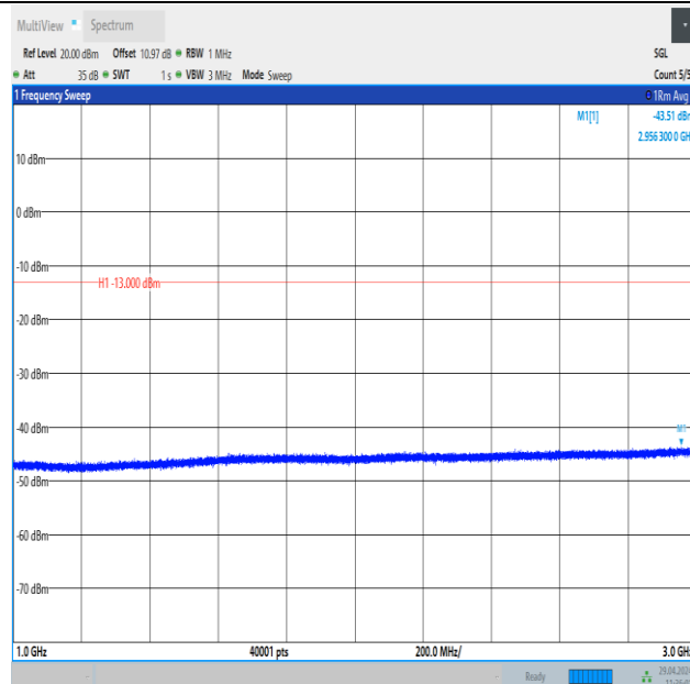
Band26_10MHz_16QAM_26915_1RB#0_1000~3000_1000~3000
