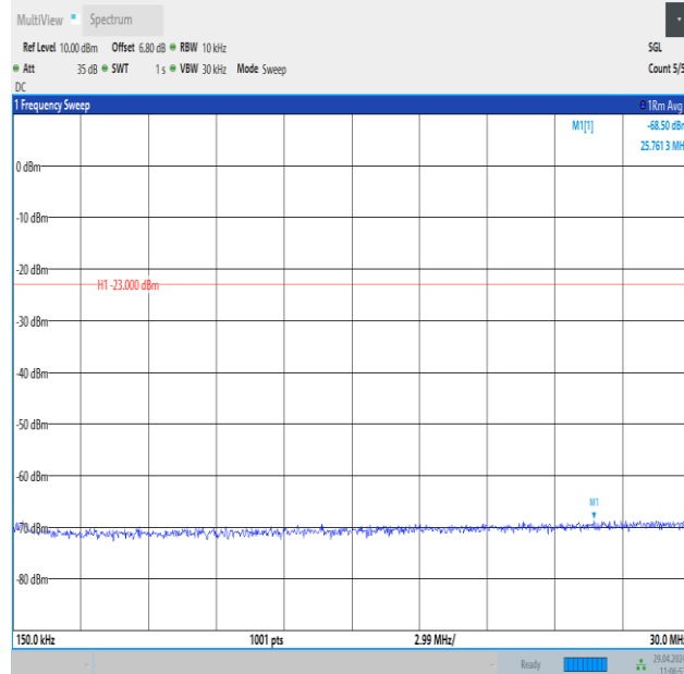
Band26_5MHz_QPSK_27015_25RB#0_0.15~30_0.15~30
