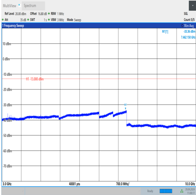
Band26_5MHz_16QAM_26915_1RB#0_3000~10000_3000~10000
