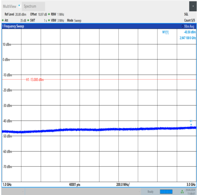
Band26_5MHz_16QAM_27015_25RB#0_1000~3000_1000~3000
