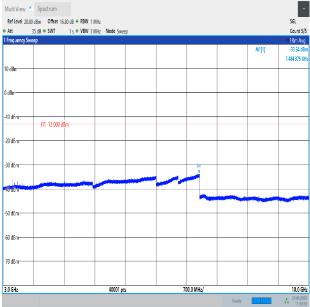
Band26_10MHz_16QAM_26840_1RB#49_3000~10000_3000~10000
