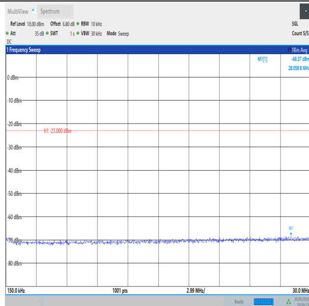
Band26_5MHz_16QAM_26815_1RB#24_0.15~30_0.15~30
