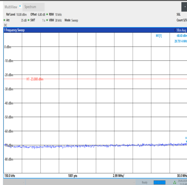
Band26_10MHz_16QAM_26915_1RB#0_0.15~30_0.15~30
