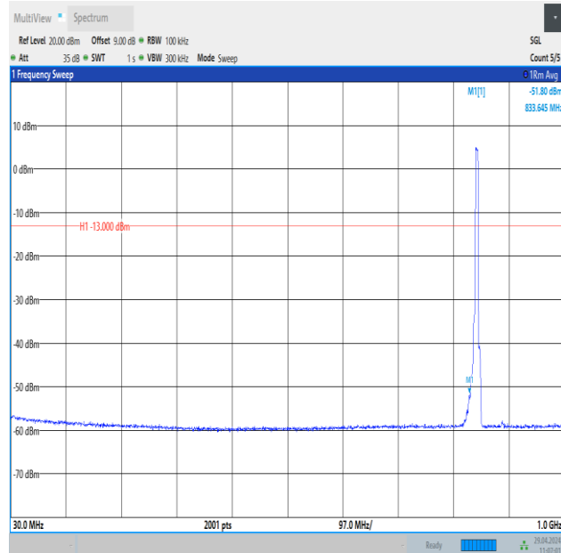
Band26_5MHz_QPSK_27015_25RB#0_30~1000_30~1000
