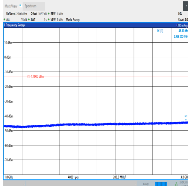
Band26_5MHz_16QAM_27015_1RB#24_1000~3000_1000~3000
