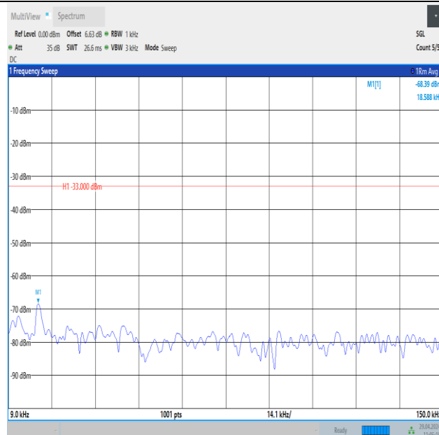
Band26_5MHz_QPSK_27015_1RB#24_0.009~0.15_0.009~0.15
