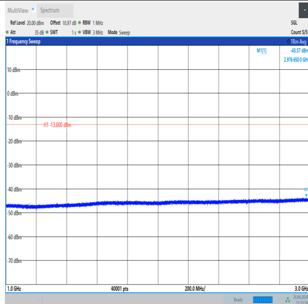
Band26_10MHz_QPSK_26840_1RB#49_1000~3000_1000~3000
