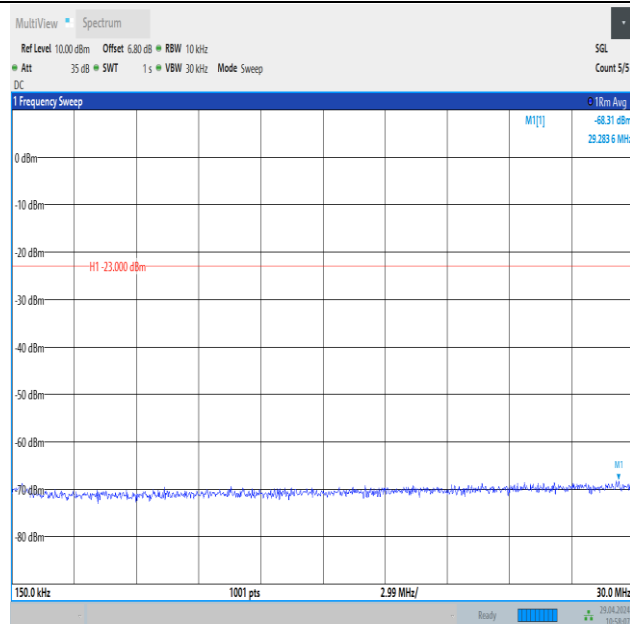
Band26_5MHz_16QAM_26815_25RB#0_0.15~30_0.15~30
