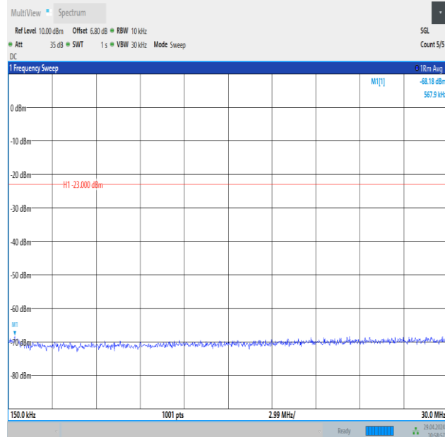
Band26_5MHz_QPSK_26915_1RB#0_0.15~30_0.15~30
