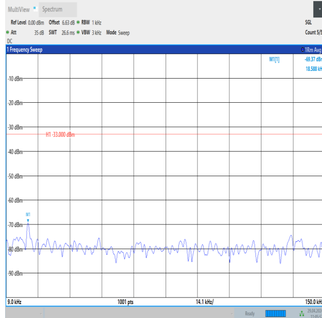
Band26_5MHz_16QAM_27015_1RB#24_0.009~0.15_0.009~0.15
