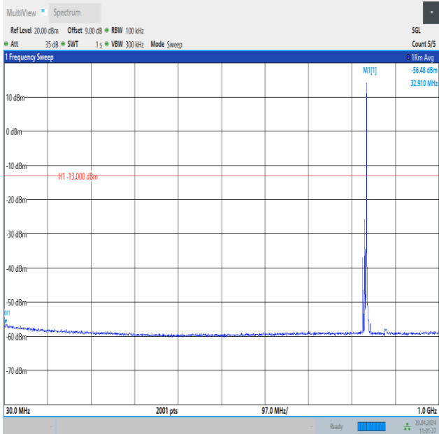
Band26_5MHz_16QAM_26915_1RB#24_30~1000_30~1000
