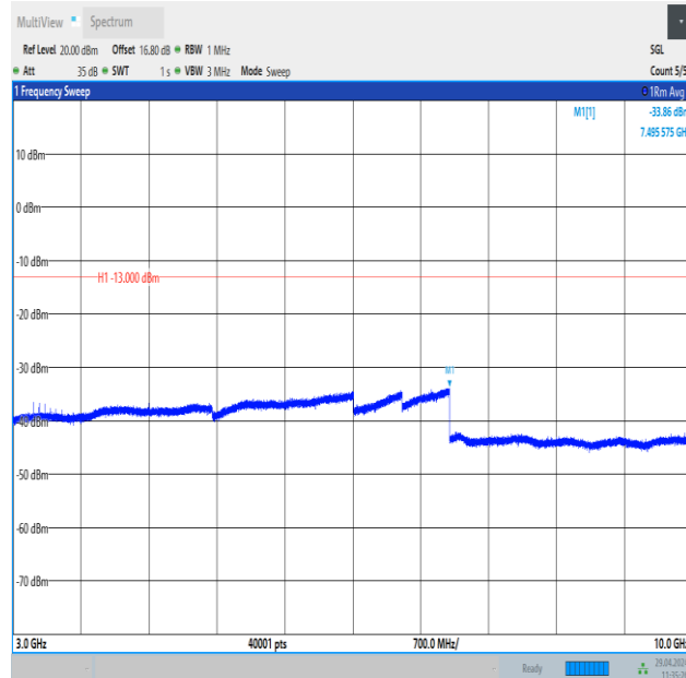
Band26_10MHz_QPSK_26915_1RB#0_3000~10000_3000~10000
