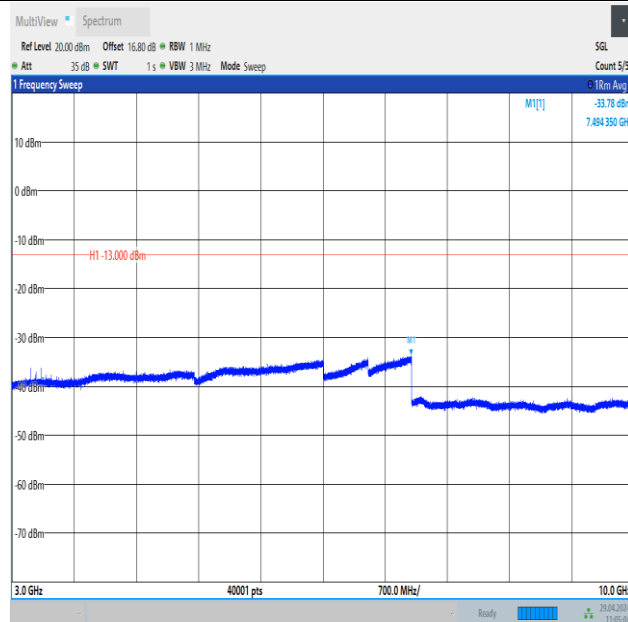
Band26_5MHz_16QAM_27015_1RB#0_3000~10000_3000~10000
