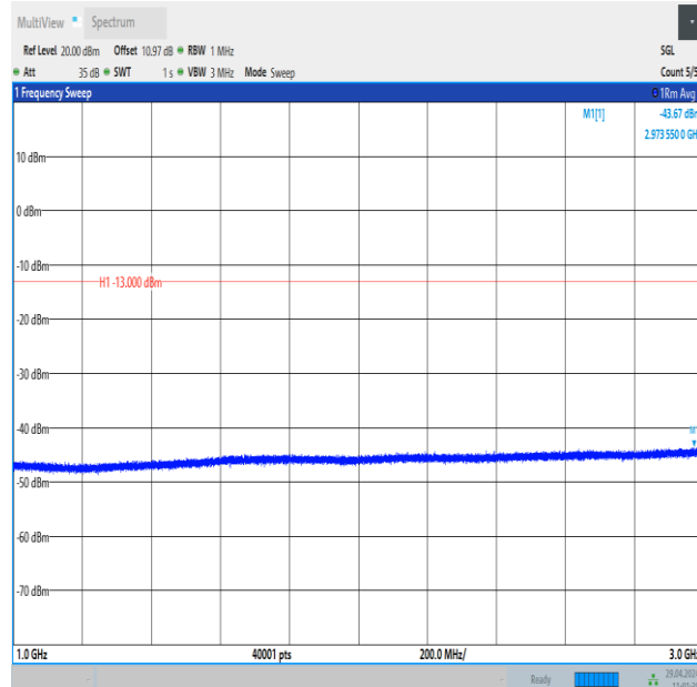
Band26_5MHz_16QAM_26915_1RB#24_1000~3000_1000~3000
