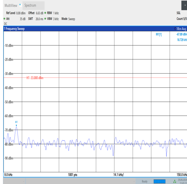
Band26_5MHz_16QAM_26915_1RB#24_0.009~0.15_0.009~0.15
