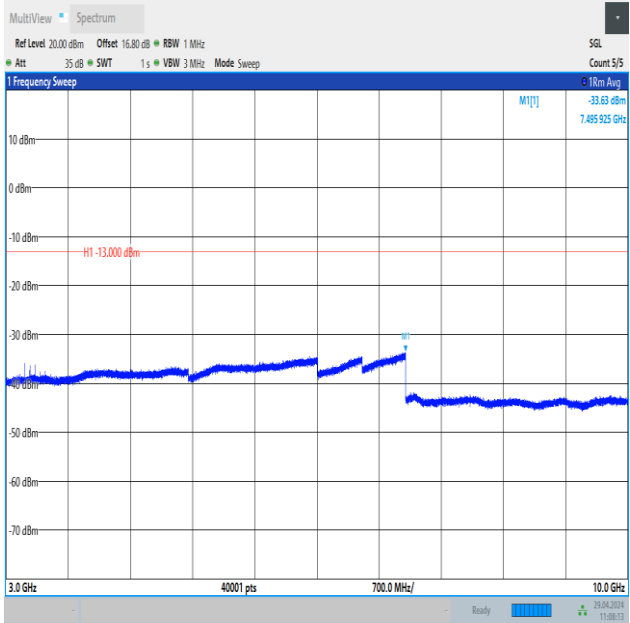
Band26_5MHz_16QAM_27015_25RB#0_3000~10000_3000~10000
