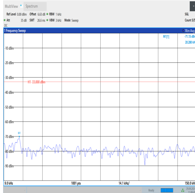
Band26_5MHz_QPSK_27015_25RB#0_0.009~0.15_0.009~0.15
