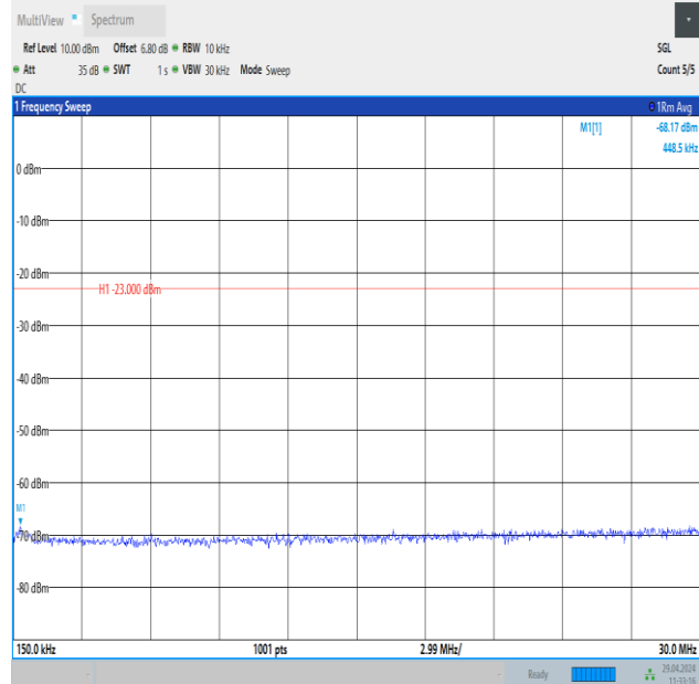
Band26_10MHz_QPSK_26840_1RB#49_0.15~30_0.15~30
