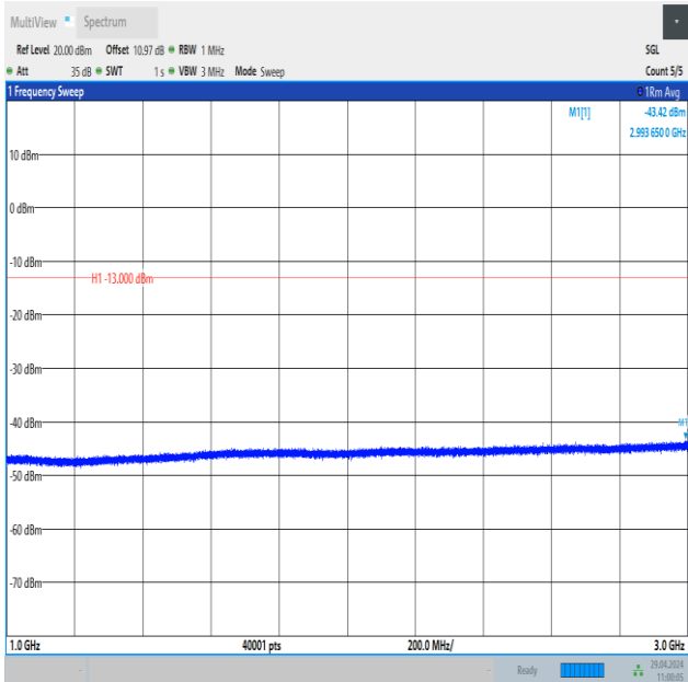
Band26_5MHz_16QAM_26915_1RB#0_1000~3000_1000~3000
