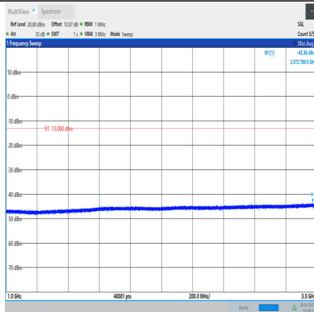
Band26_5MHz_QPSK_26815_1RB#0_1000~3000_1000~3000
