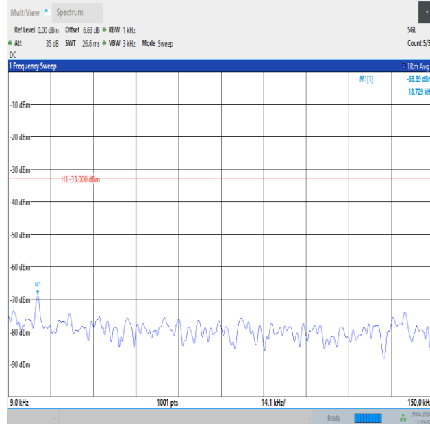
Band26_10MHz_16QAM_26915_1RB#0_0.009~0.15_0.009~0.15
