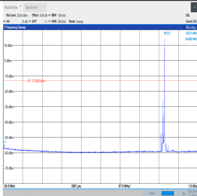
Band26_10MHz_16QAM_26840_1RB#49_30~1000_30~1000
