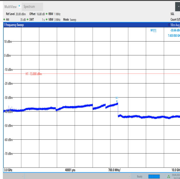
Band26_5MHz_16QAM_26815_1RB#24_3000~10000_3000~10000
