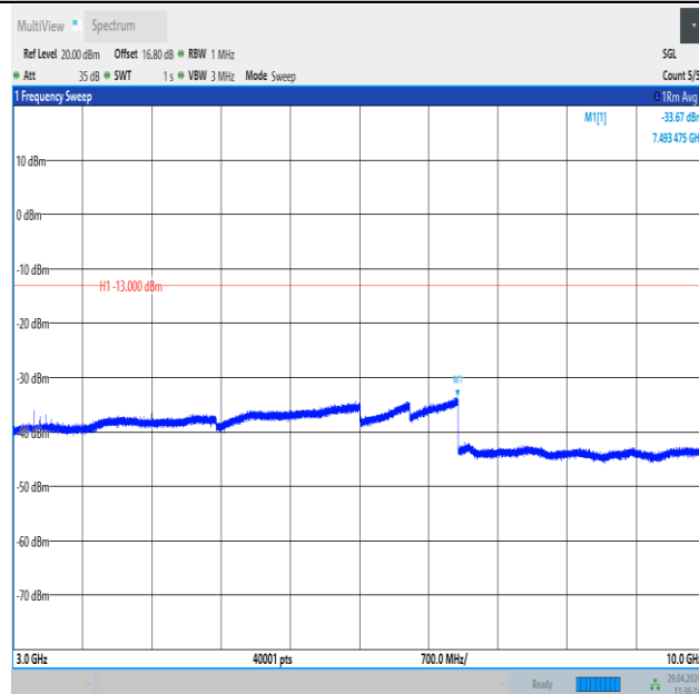
Band26_10MHz_16QAM_26915_1RB#0_3000~10000_3000~10000
