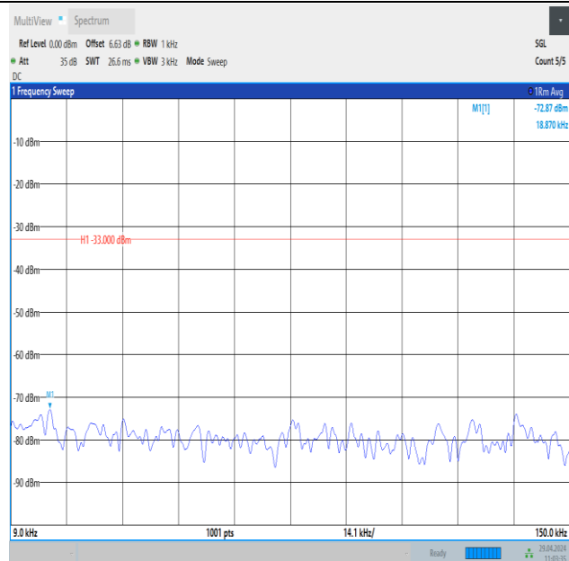
Band26_5MHz_QPSK_27015_1RB#0_0.009~0.15_0.009~0.15
