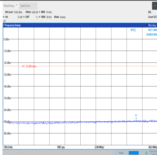
Band26_5MHz_16QAM_27015_25RB#0_0.15~30_0.15~30
