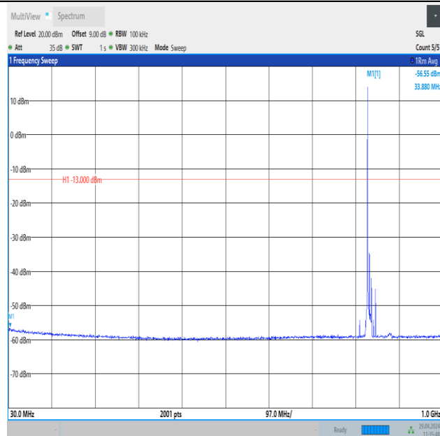
Band26_10MHz_16QAM_26915_1RB#0_30~1000_30~1000
