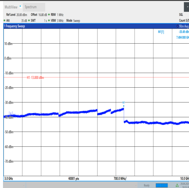
Band26_5MHz_16QAM_26815_1RB#0_3000~10000_3000~10000
