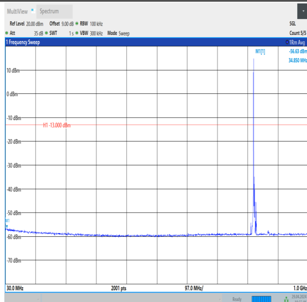
Band26_5MHz_16QAM_26815_1RB#0_30~1000_30~1000
