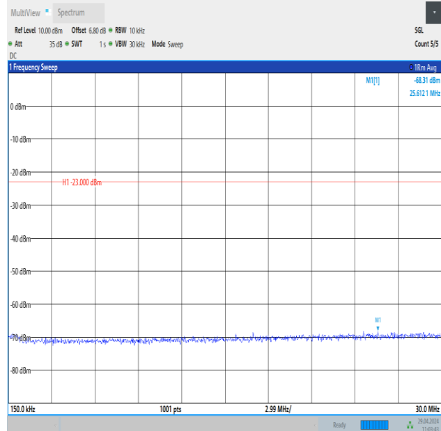
Band26_5MHz_QPSK_27015_1RB#0_0.15~30_0.15~30
