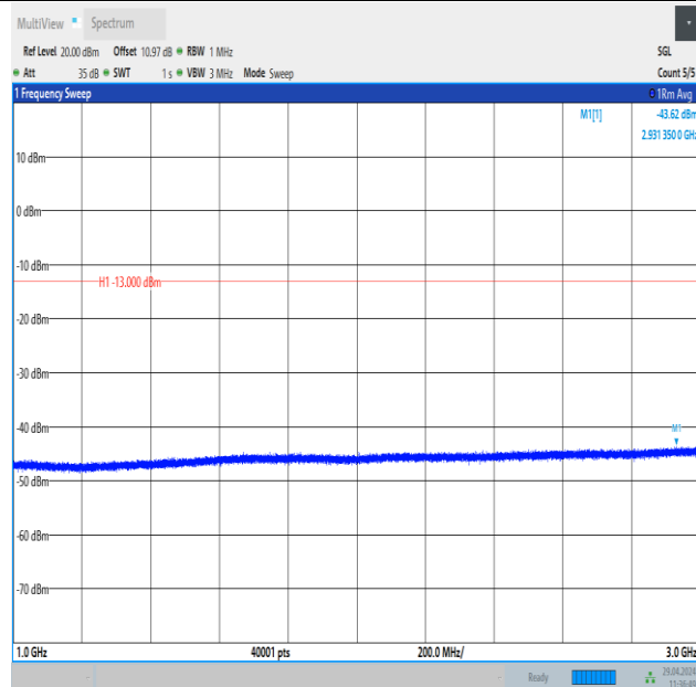
Band26_10MHz_QPSK_26915_1RB#49_1000~3000_1000~3000
