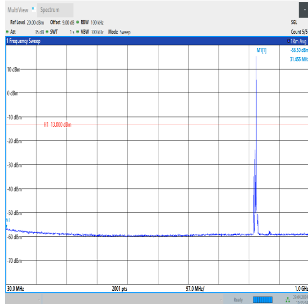
Band26_5MHz_QPSK_26815_1RB#24_30~1000_30~1000
