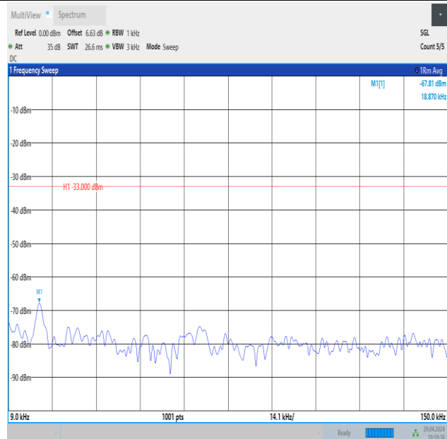
Band26_5MHz_16QAM_26915_1RB#0_0.009~0.15_0.009~0.15
