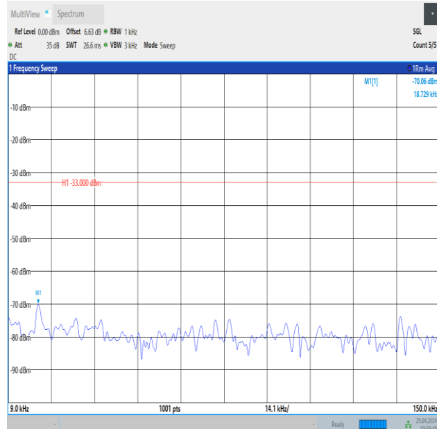
Band26_5MHz_QPSK_26915_1RB#0_0.009~0.15_0.009~0.15
