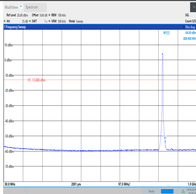
Band26_5MHz_16QAM_26815_25RB#0_30~1000_30~1000
