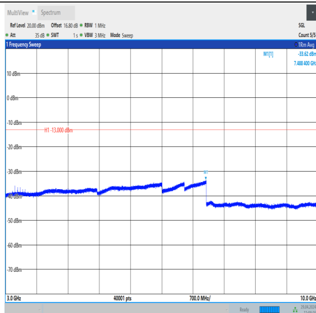
Band26_5MHz_QPSK_27015_1RB#0_3000~10000_3000~10000
