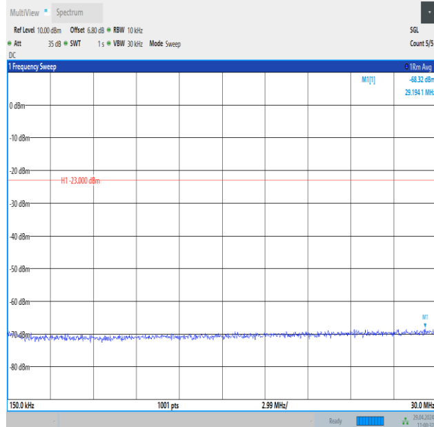
Band26_5MHz_QPSK_26915_1RB#24_0.15~30_0.15~30
