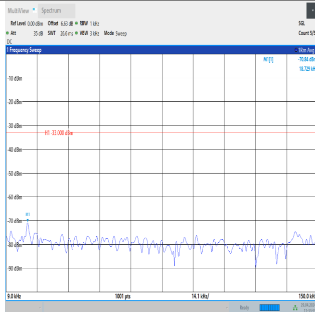
Band26_10MHz_16QAM_26840_1RB#49_0.009~0.15_0.009~0.15
