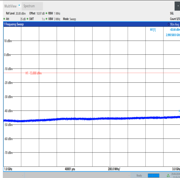
Band26_10MHz_QPSK_26915_1RB#0_1000~3000_1000~3000
