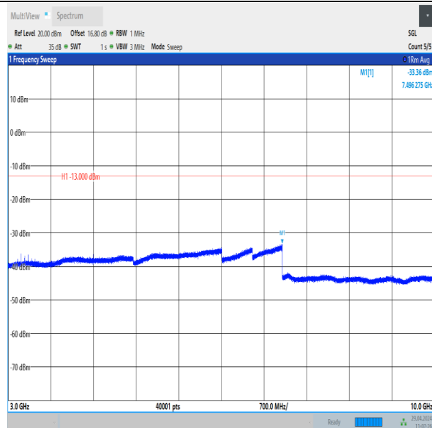
Band26_5MHz_QPSK_27015_25RB#0_3000~10000_3000~10000
