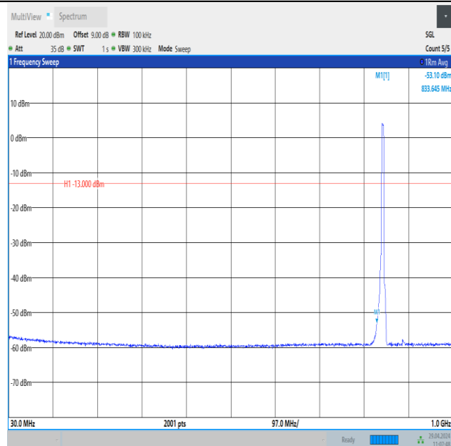
Band26_5MHz_16QAM_27015_25RB#0_30~1000_30~1000
