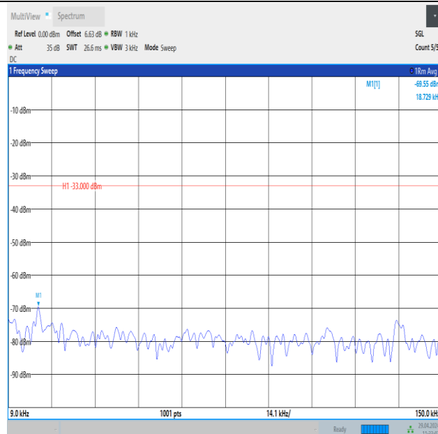
Band26_10MHz_QPSK_26840_1RB#49_0.009~0.15_0.009~0.15
