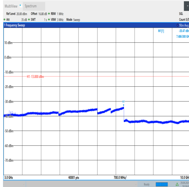
Band26_5MHz_QPSK_26815_1RB#0_3000~10000_3000~10000
