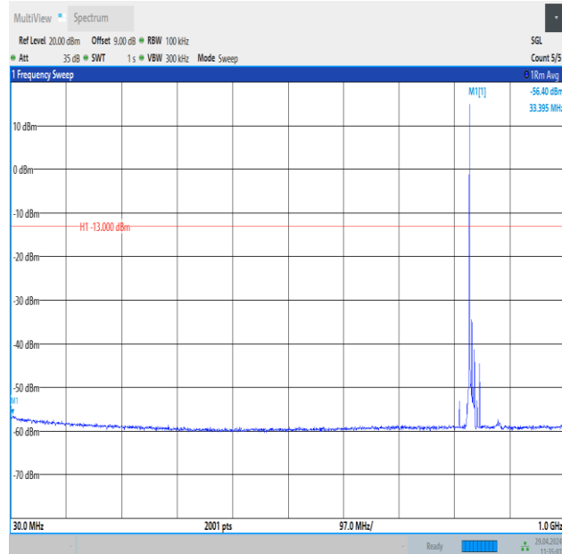
Band26_10MHz_QPSK_26915_1RB#0_30~1000_30~1000
