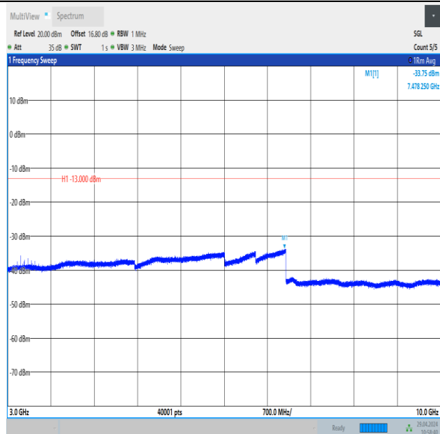
Band26_5MHz_16QAM_26815_25RB#0_3000~10000_3000~10000
