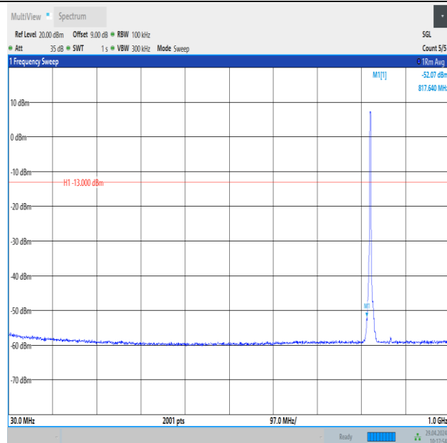
Band26_3MHz_QPSK_26805_15RB#0_30~1000_30~1000
