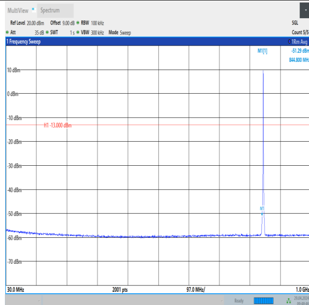
Band26_1.4MHz_16QAM_27033_6RB#0_30~1000_30~1000
