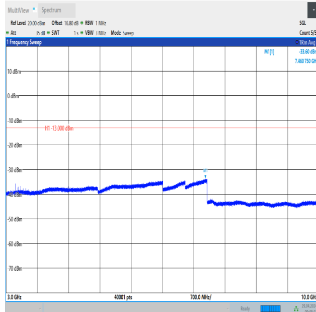
Band26_1.4MHz_QPSK_27033_6RB#0_3000~10000_3000~10000
