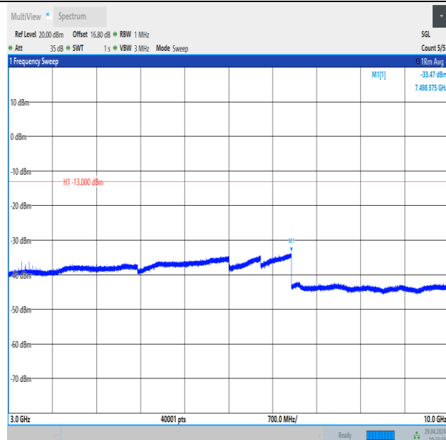
Band26_3MHz_QPSK_26915_15RB#0_3000~10000_3000~10000
