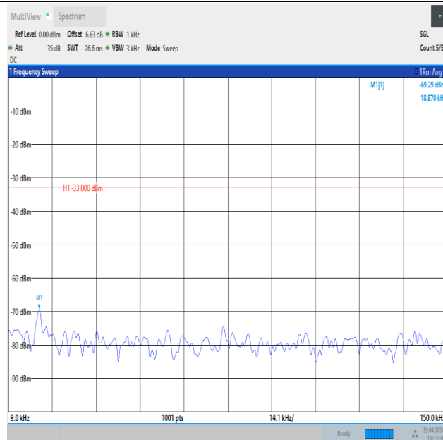
Band26_3MHz_QPSK_26805_15RB#0_0.009~0.15_0.009~0.15
