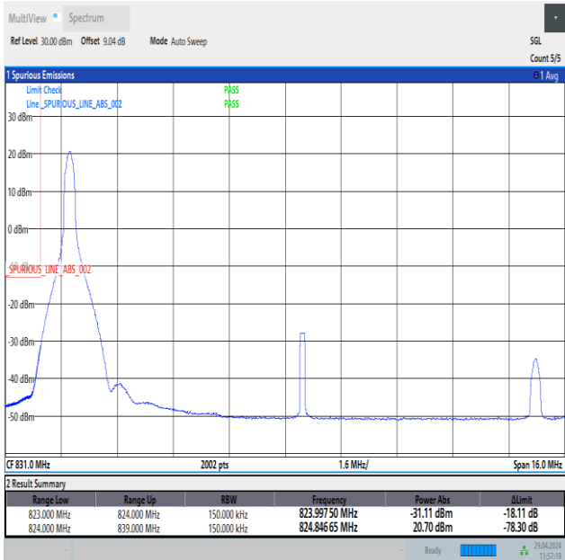
Band26_15MHz_QPSK_26865_1RB#0
