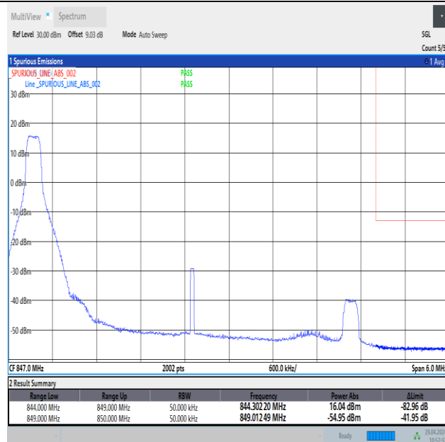
Band26_5MHz_QPSK_27015_1RB#0
