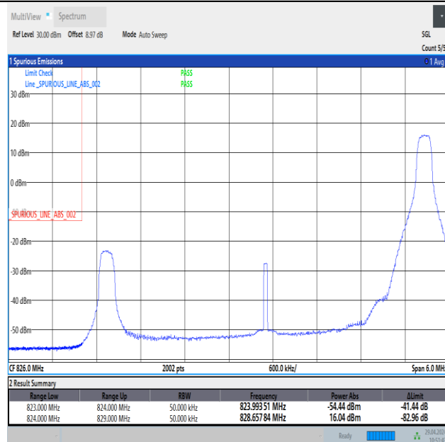
Band26_5MHz_16QAM_26815_1RB#24
