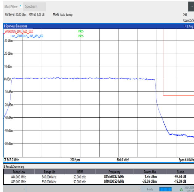
Band26_5MHz_16QAM_27015_25RB#0
