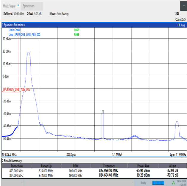
Band26_10MHz_QPSK_26840_1RB#0
