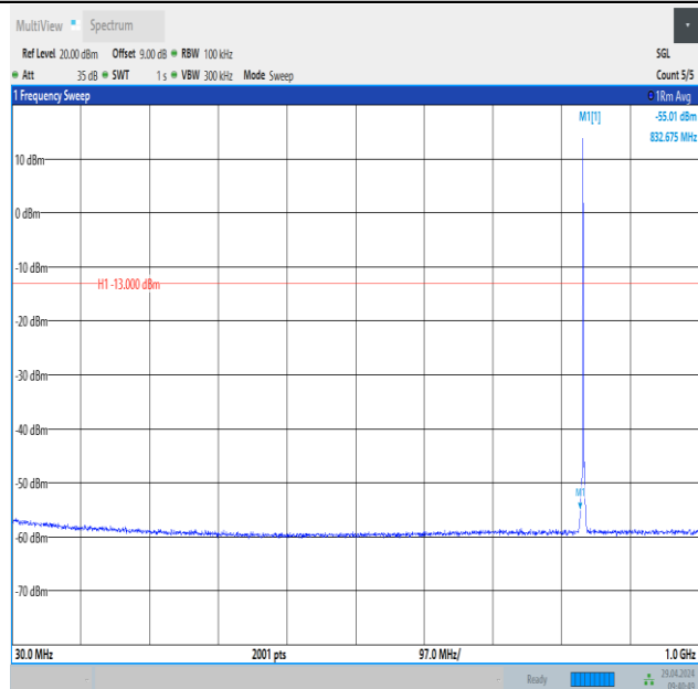
Band26_1.4MHz_16QAM_26915_1RB#0_30~1000_30~1000
