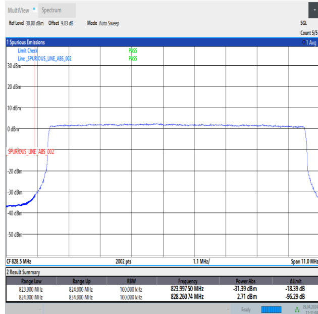
Band26_10MHz_QPSK_26840_50RB#0
