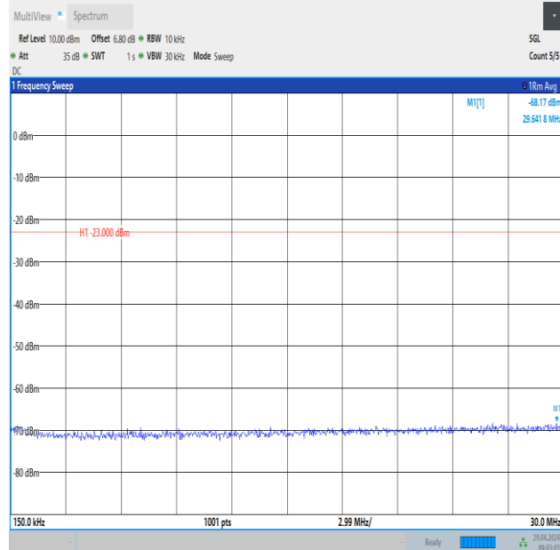
Band26_1.4MHz_QPSK_26915_6RB#0_0.15~30_0.15~30
