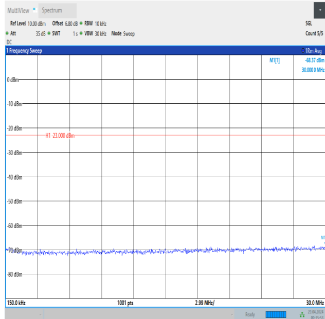
Band26_1.4MHz_16QAM_26797_1RB#0_0.15~30_0.15~30
