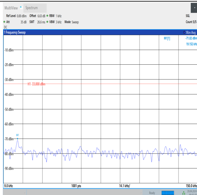
Band26_1.4MHz_QPSK_26915_1RB#5_0.009~0.15_0.009~0.15
