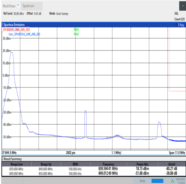
Band26_10MHz_QPSK_26990_1RB#0
