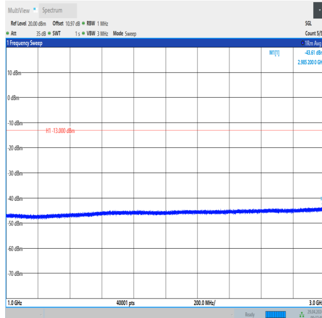
Band26_1.4MHz_16QAM_26797_1RB#5_1000~3000_1000~3000
