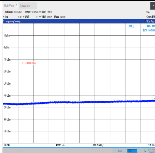
Band26_1.4MHz_QPSK_26915_6RB#0_1000~3000_1000~3000
