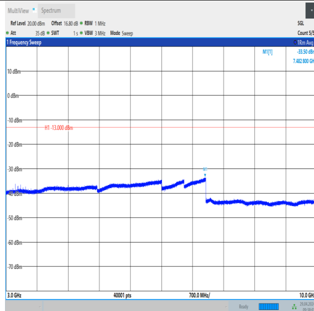
Band26_1.4MHz_16QAM_26797_1RB#5_3000~10000_3000~10000
