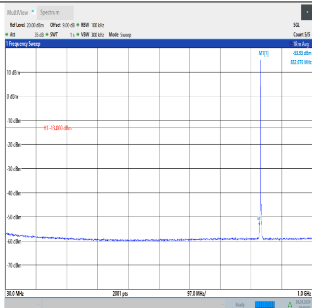
Band26_1.4MHz_QPSK_26915_1RB#0_30~1000_30~1000
