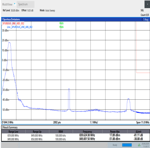
Band26_10MHz_16QAM_26990_1RB#0
