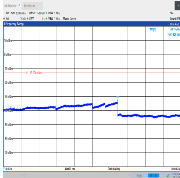
Band26_1.4MHz_QPSK_26797_1RB#0_3000~10000_3000~10000
