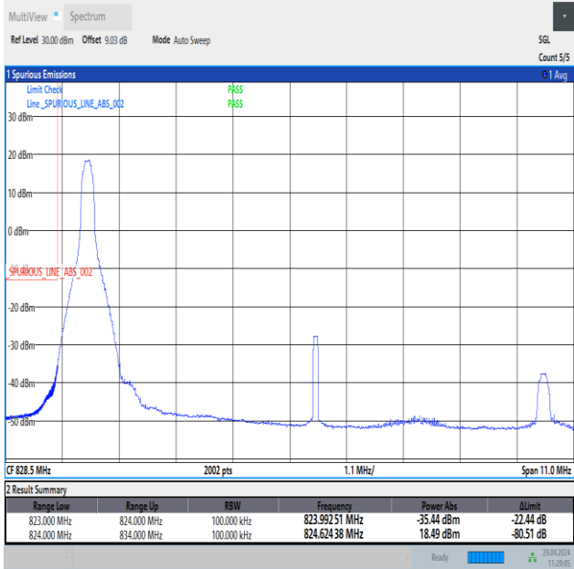
Band26_10MHz_16QAM_26840_1RB#0
