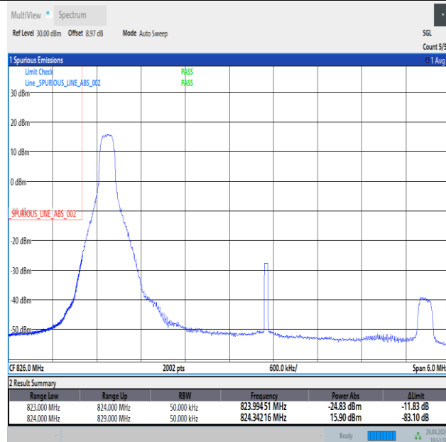
Band26_5MHz_16QAM_26815_1RB#0
