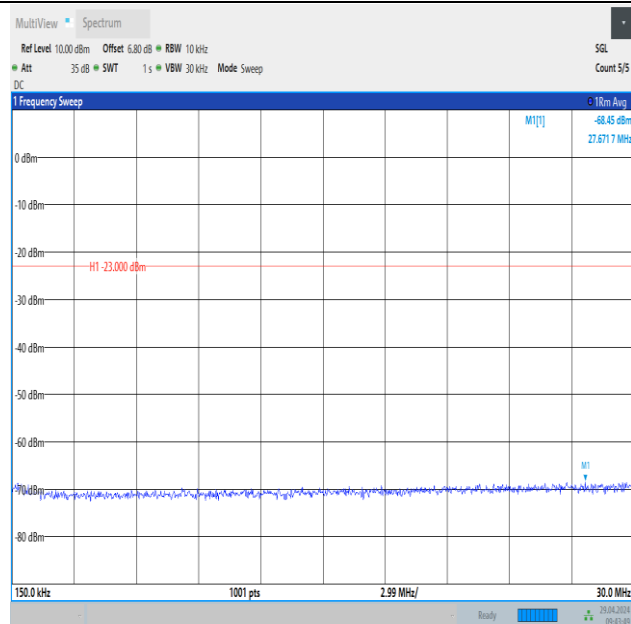
Band26_1.4MHz_16QAM_26915_6RB#0_0.15~30_0.15~30
