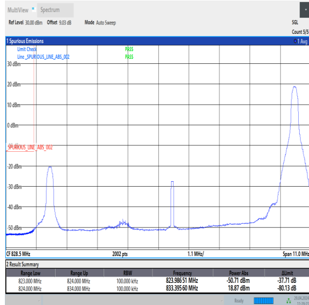
Band26_10MHz_QPSK_26840_1RB#49
