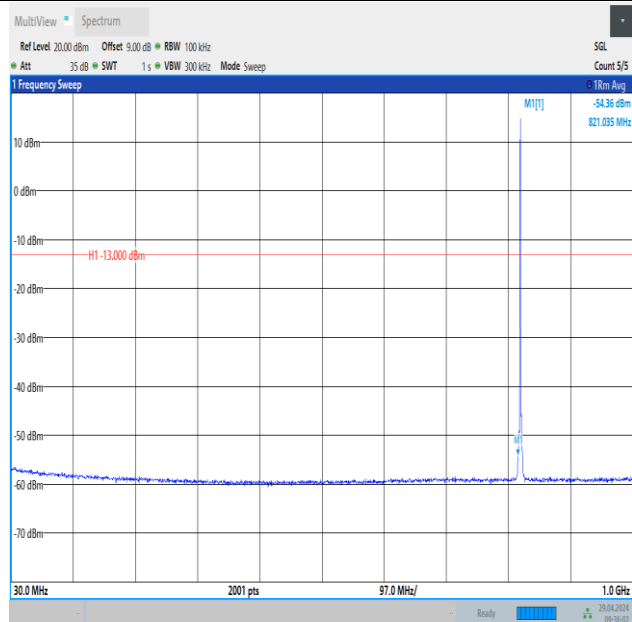
Band26_1.4MHz_16QAM_26797_1RB#0_30~1000_30~1000
