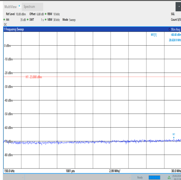
Band26_1.4MHz_16QAM_26797_1RB#5_0.15~30_0.15~30
