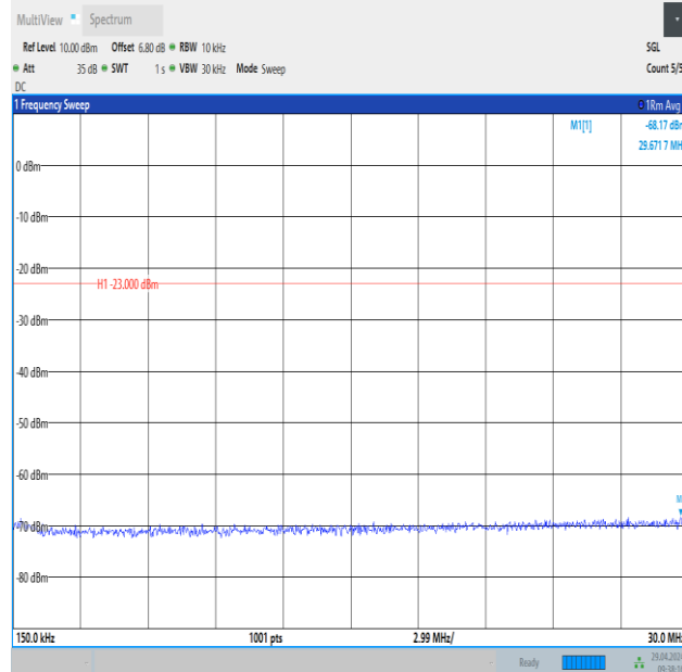
Band26_1.4MHz_QPSK_26797_6RB#0_0.15~30_0.15~30
