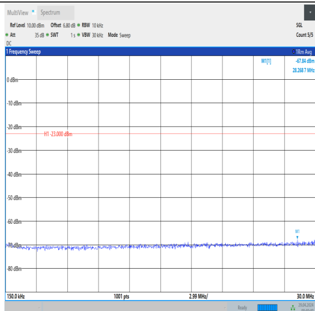
Band26_1.4MHz_16QAM_26915_1RB#0_0.15~30_0.15~30
