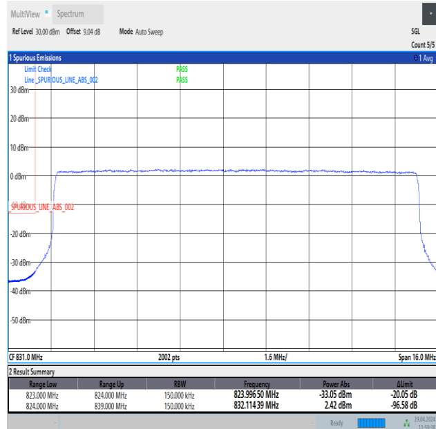
Band26_15MHz_QPSK_26865_75RB#0
