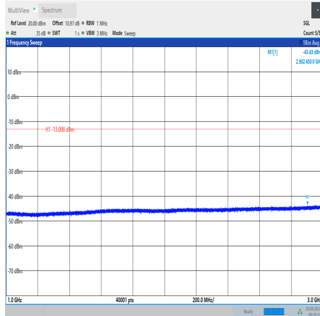
Band26_1.4MHz_16QAM_26797_1RB#0_1000~3000_1000~3000
