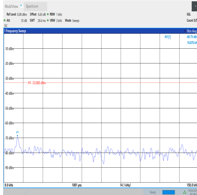
Band26_1.4MHz_QPSK_26797_6RB#0_0.009~0.15_0.009~0.15
