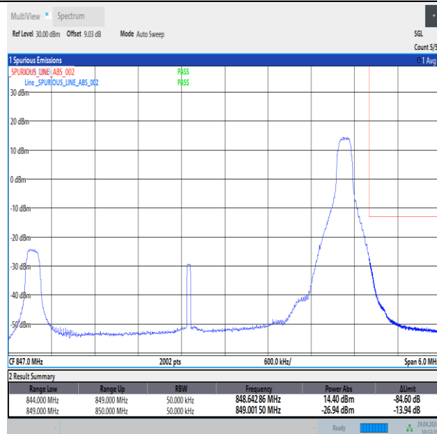
Band26_5MHz_16QAM_27015_1RB#24
