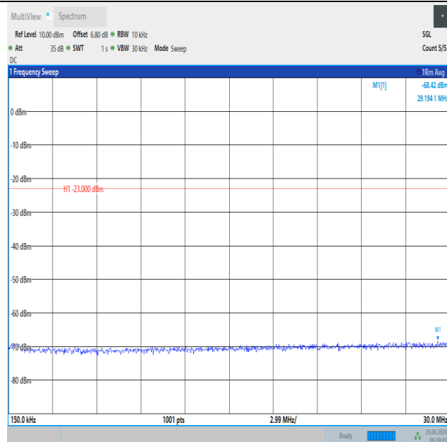
Band26_1.4MHz_16QAM_26797_6RB#0_0.15~30_0.15~30
