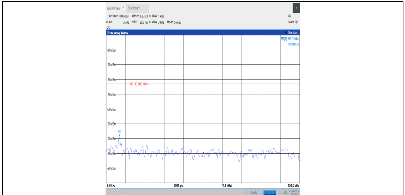
Band26_1.4MHz_QPSK_26797_1RB#0_0.009~0.15_0.009~0.15
