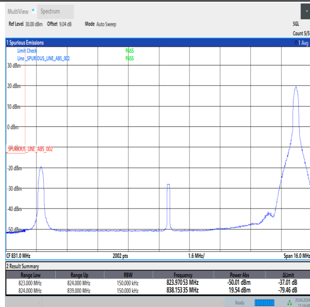
Band26_15MHz_16QAM_26865_1RB#74
