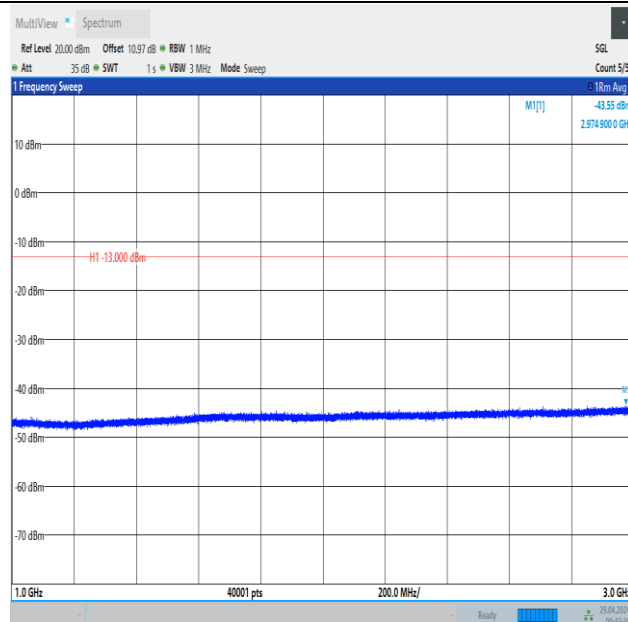
Band26_1.4MHz_16QAM_26915_1RB#5_1000~3000_1000~3000
