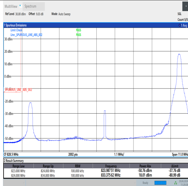
Band26_10MHz_16QAM_26840_1RB#49
