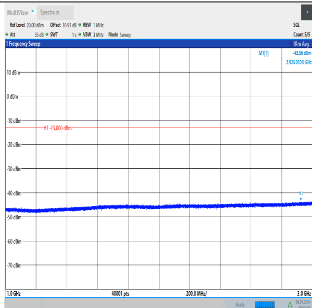
Band26_1.4MHz_16QAM_26915_1RB#0_1000~3000_1000~3000
