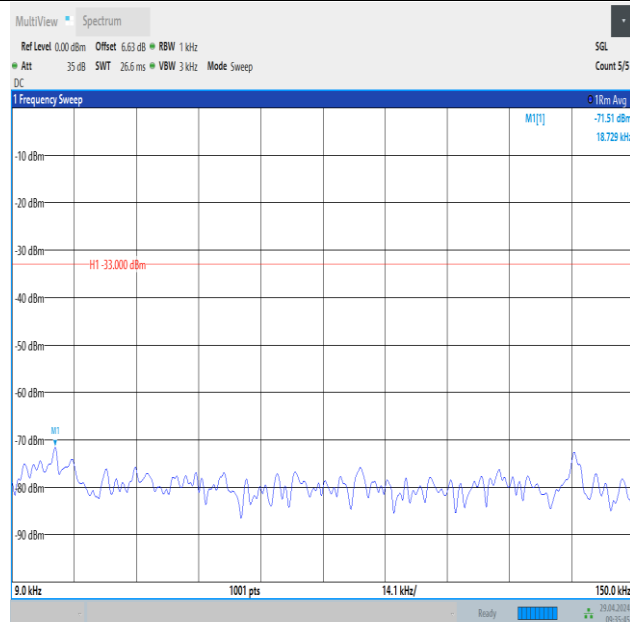
Band26_1.4MHz_16QAM_26797_1RB#0_0.009~0.15_0.009~0.15
