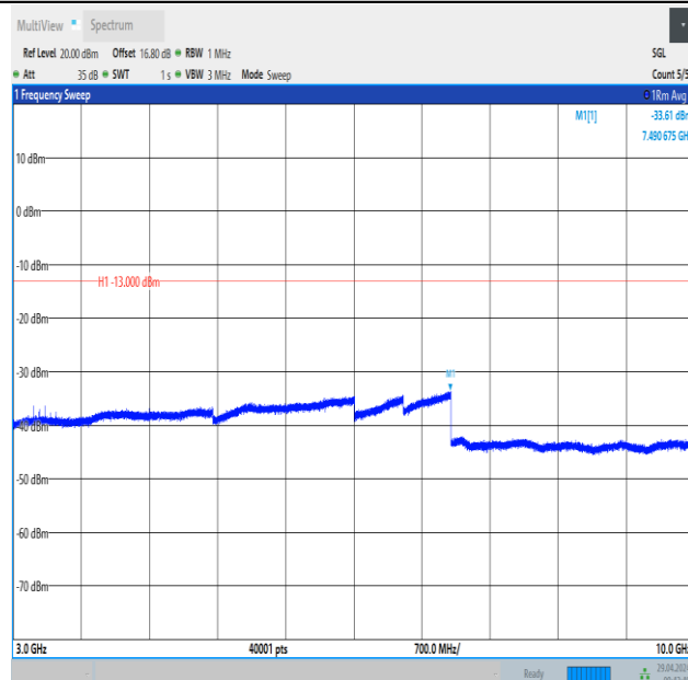
Band26_1.4MHz_16QAM_26915_1RB#5_3000~10000_3000~10000
