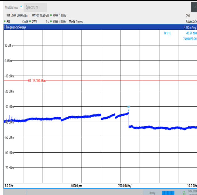
Band26_1.4MHz_QPSK_26915_1RB#0_3000~10000_3000~10000
