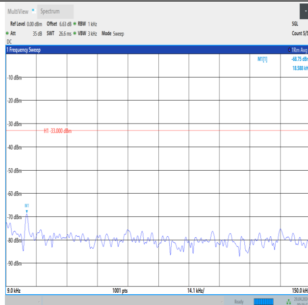
Band26_1.4MHz_QPSK_26797_1RB#5_0.009~0.15_0.009~0.15
