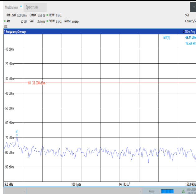
Band26_1.4MHz_16QAM_26797_6RB#0_0.009~0.15_0.009~0.15
