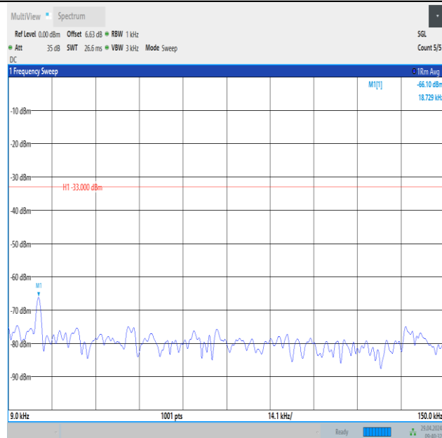
Band26_1.4MHz_16QAM_26915_1RB#0_0.009~0.15_0.009~0.15
