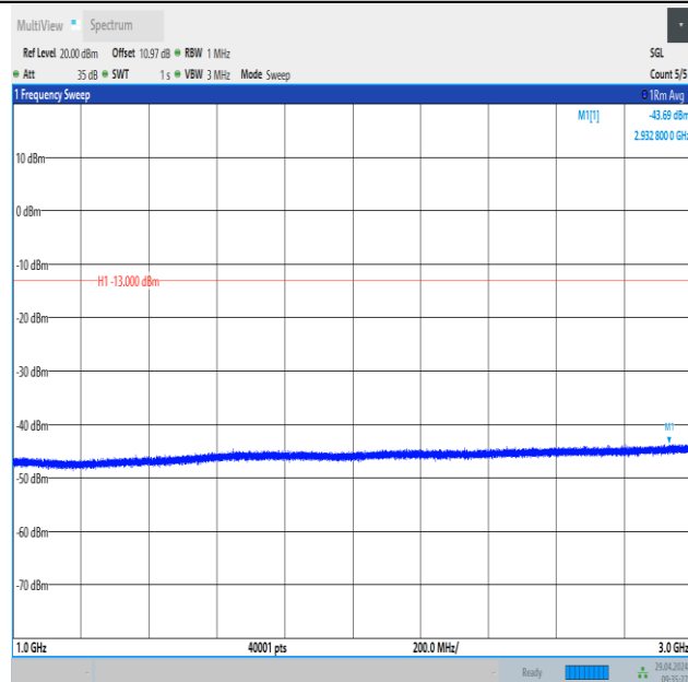
Band26_1.4MHz_QPSK_26797_1RB#0_1000~3000_1000~3000
