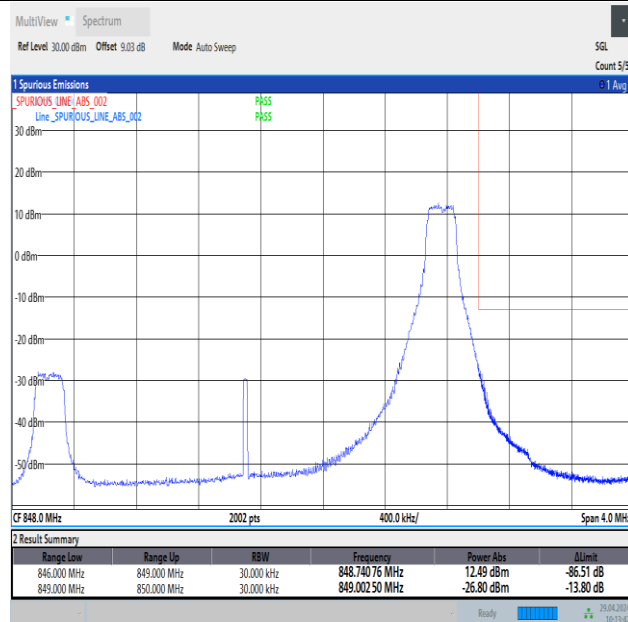
Band26_3MHz_16QAM_27025_1RB#14
