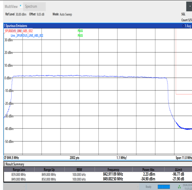
Band26_10MHz_QPSK_26990_50RB#0
