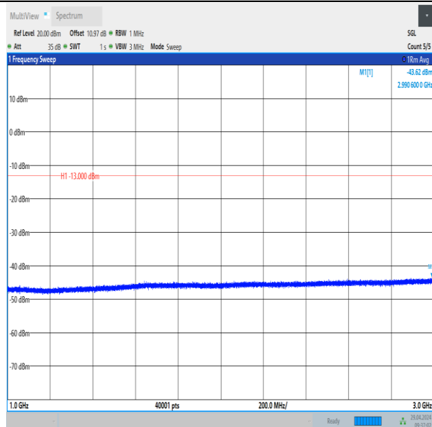
Band26_1.4MHz_QPSK_26797_1RB#5_1000~3000_1000~3000
