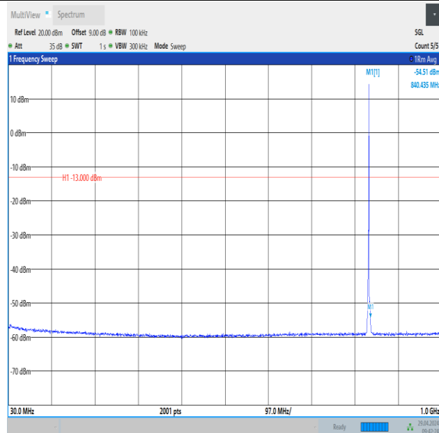
Band26_1.4MHz_16QAM_26915_1RB#5_30~1000_30~1000
