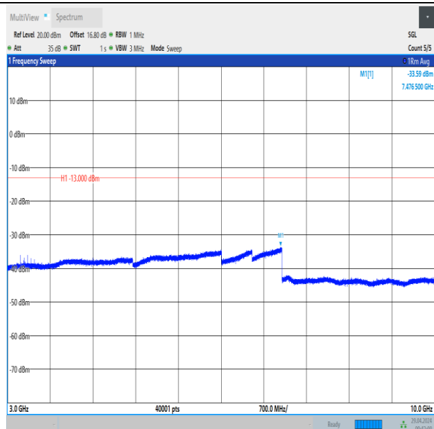
Band26_1.4MHz_QPSK_26915_1RB#5_3000~10000_3000~10000
