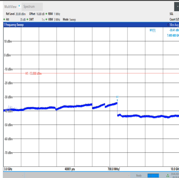
Band26_1.4MHz_16QAM_26797_6RB#0_3000~10000_3000~10000
