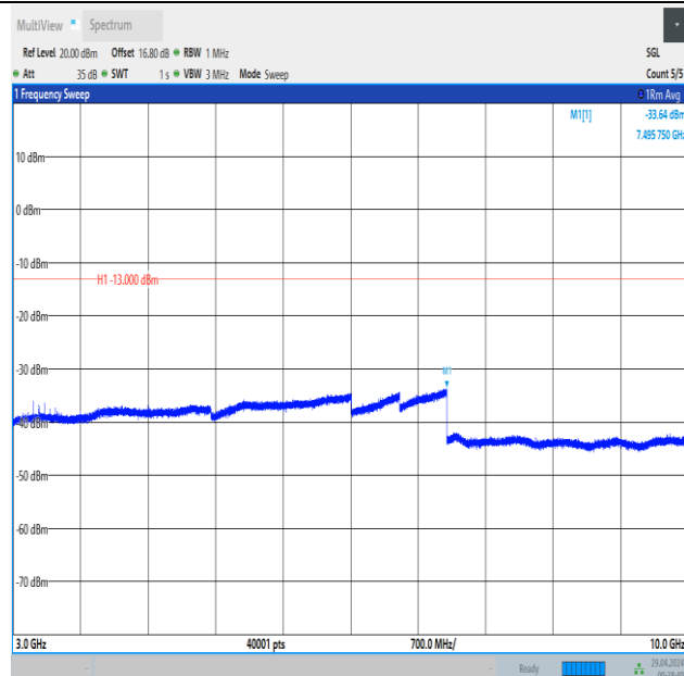
Band26_1.4MHz_QPSK_26797_6RB#0_3000~10000_3000~10000
