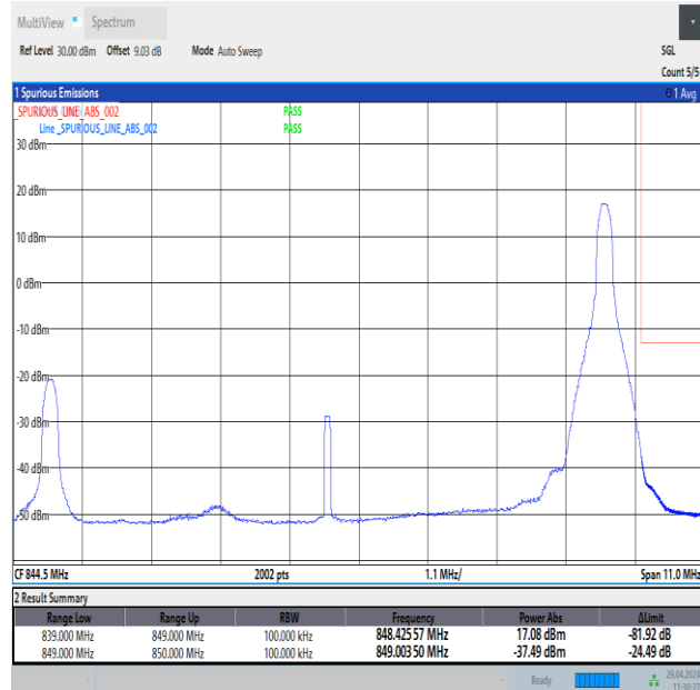
Band26_10MHz_QPSK_26990_1RB#49
