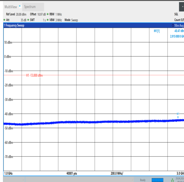
Band26_1.4MHz_16QAM_26797_6RB#0_1000~3000_1000~3000
