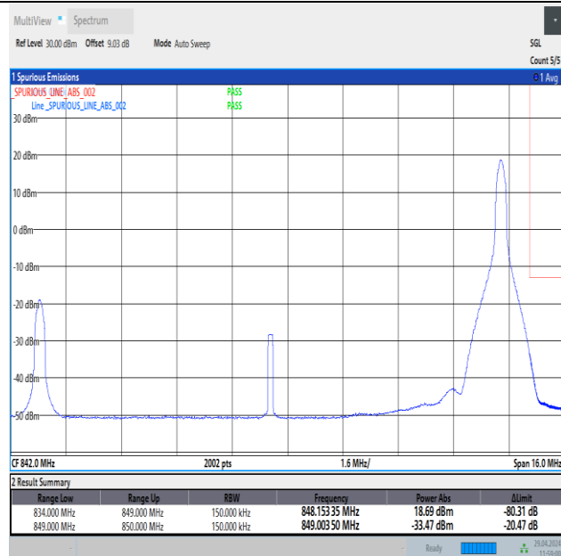
Band26_15MHz_QPSK_26965_1RB#74
