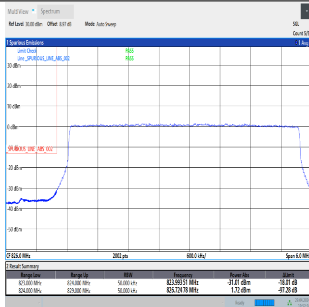
Band26_5MHz_16QAM_26815_25RB#0
