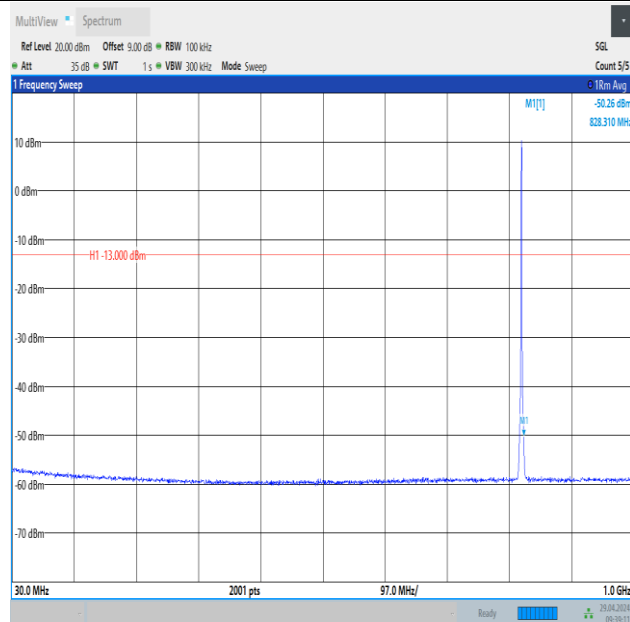
Band26_1.4MHz_16QAM_26797_6RB#0_30~1000_30~1000
