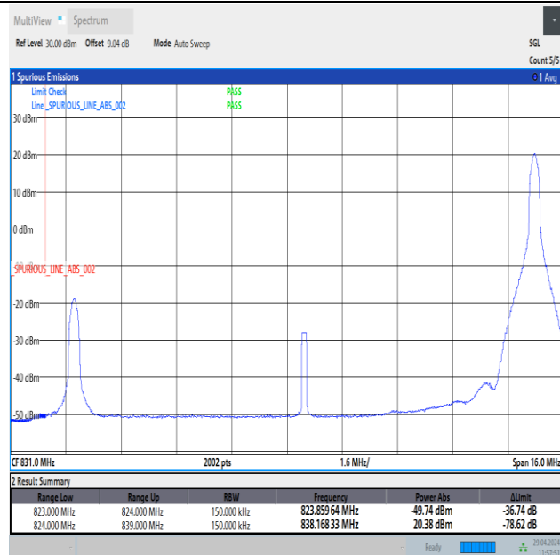
Band26_15MHz_QPSK_26865_1RB#74
