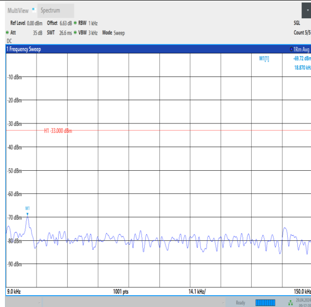
Band26_1.4MHz_16QAM_26797_1RB#5_0.009~0.15_0.009~0.15
