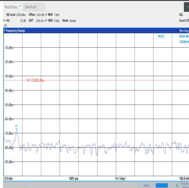
Band26_1.4MHz_16QAM_26915_6RB#0_0.009~0.15_0.009~0.15
