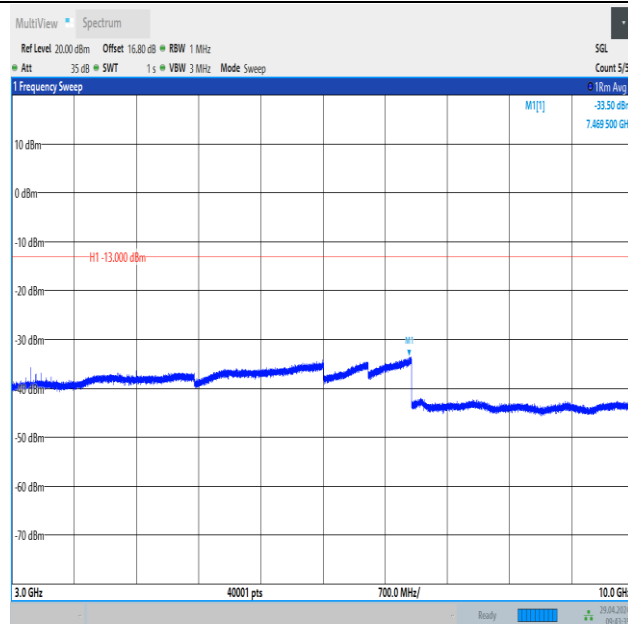
Band26_1.4MHz_QPSK_26915_6RB#0_3000~10000_3000~10000
