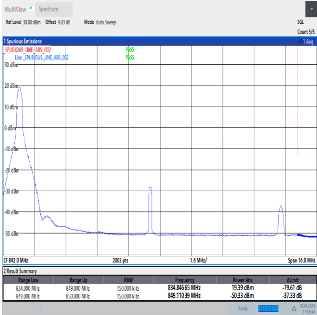
Band26_15MHz_16QAM_26965_1RB#0
