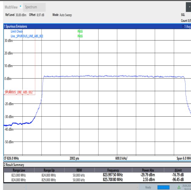
Band26_5MHz_QPSK_26815_25RB#0
