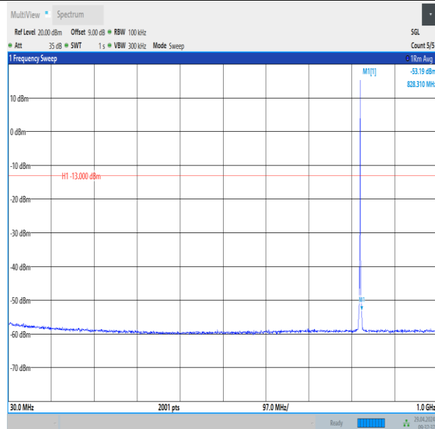
Band26_1.4MHz_16QAM_26797_1RB#5_30~1000_30~1000
