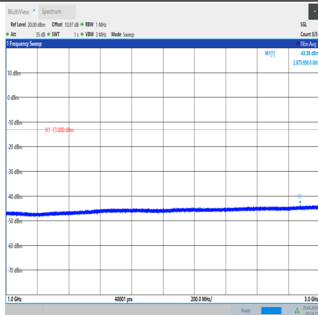
Band26_1.4MHz_QPSK_26797_6RB#0_1000~3000_1000~3000
