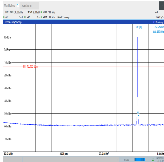
Band26_1.4MHz_16QAM_26915_6RB#0_30~1000_30~1000
