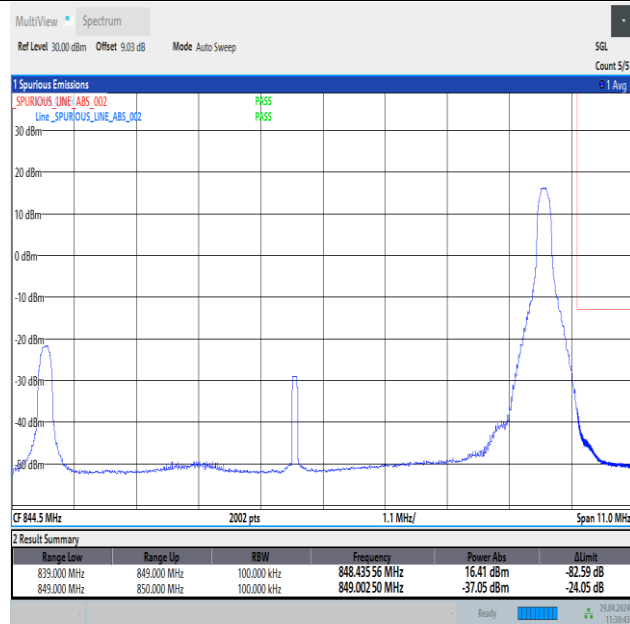
Band26_10MHz_16QAM_26990_1RB#49
