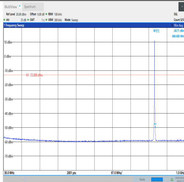
Band26_1.4MHz_QPSK_26915_6RB#0_30~1000_30~1000
