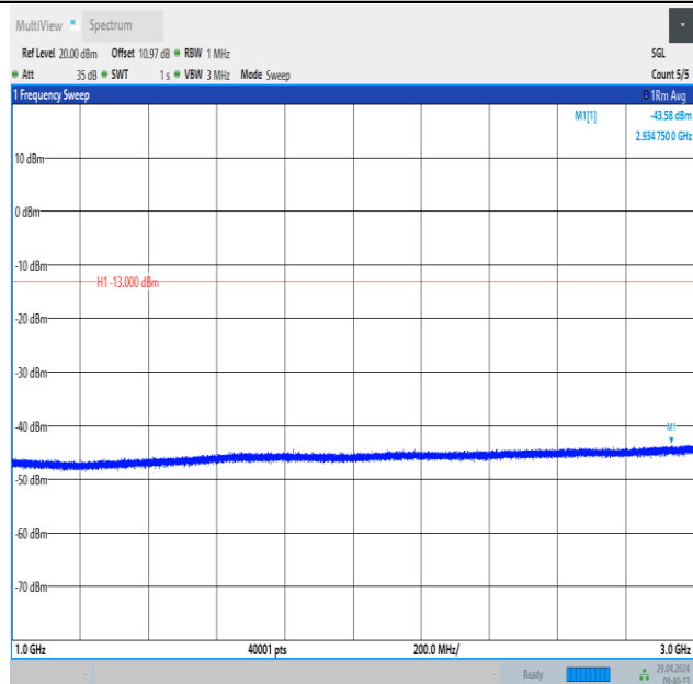
Band26_1.4MHz_QPSK_26915_1RB#0_1000~3000_1000~3000
