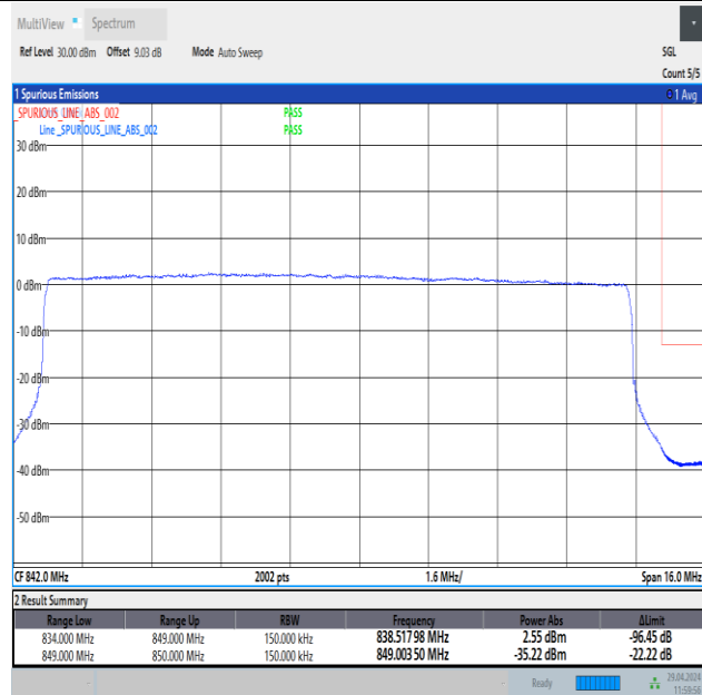
Band26_15MHz_QPSK_26965_75RB#0
