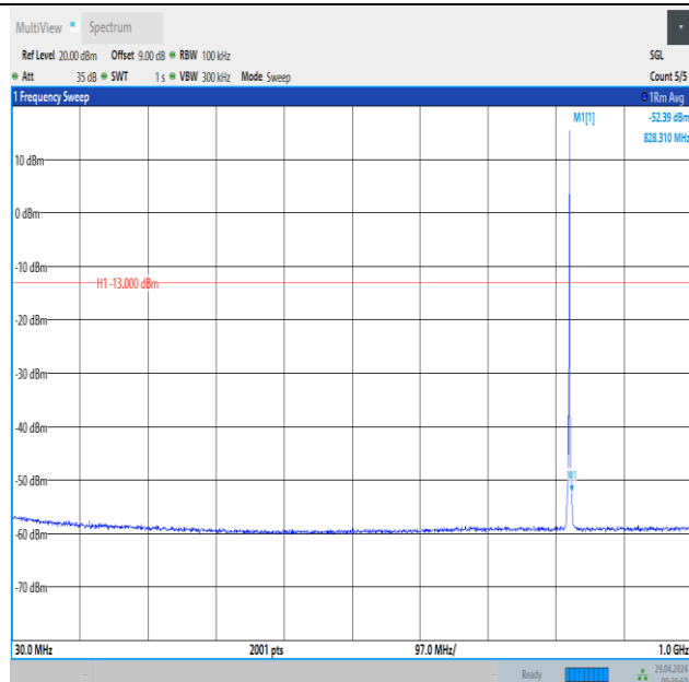
Band26_1.4MHz_QPSK_26797_1RB#5_30~1000_30~1000
