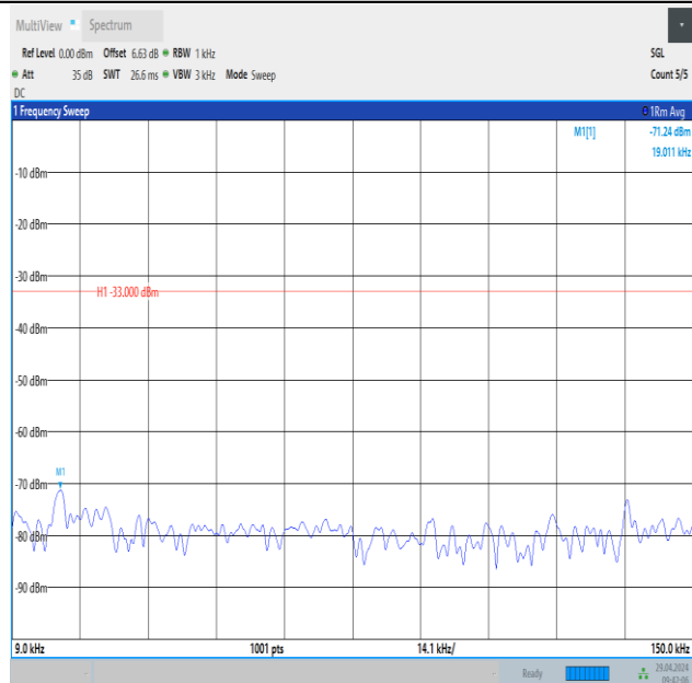
Band26_1.4MHz_16QAM_26915_1RB#5_0.009~0.15_0.009~0.15
