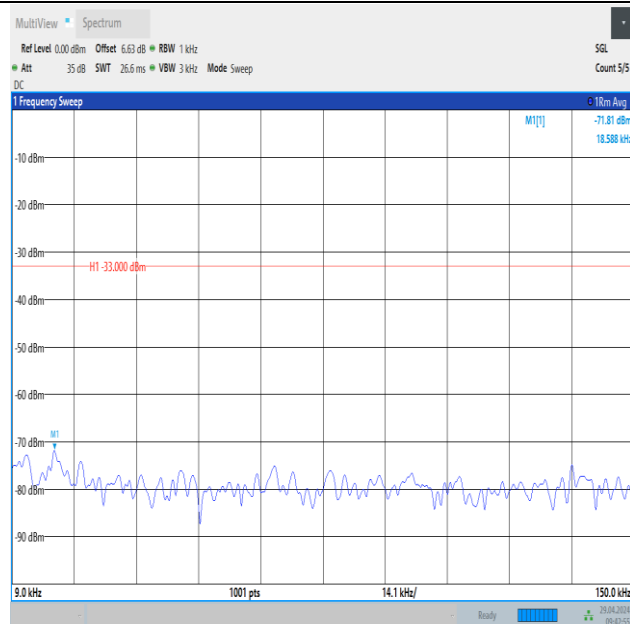
Band26_1.4MHz_QPSK_26915_6RB#0_0.009~0.15_0.009~0.15
