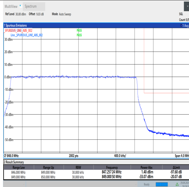
Band26_3MHz_16QAM_27025_15RB#0
