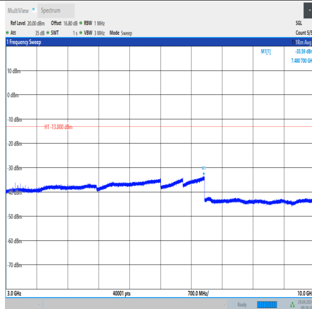
Band26_1.4MHz_16QAM_26797_1RB#0_3000~10000_3000~10000
