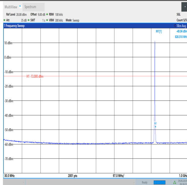
Band26_1.4MHz_QPSK_26797_6RB#0_30~1000_30~1000
