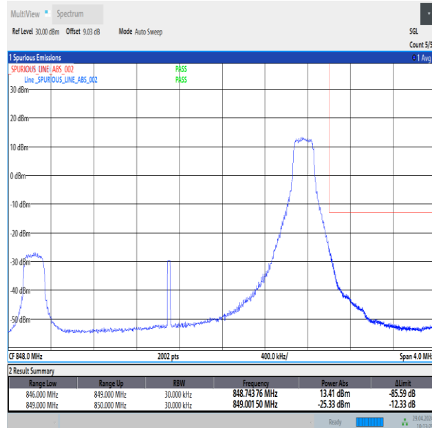
Band26_3MHz_QPSK_27025_1RB#14
