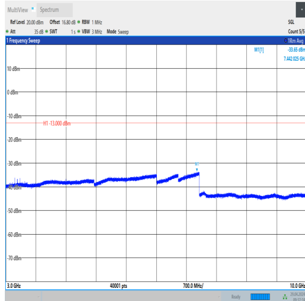
Band26_1.4MHz_QPSK_26797_1RB#5_3000~10000_3000~10000
