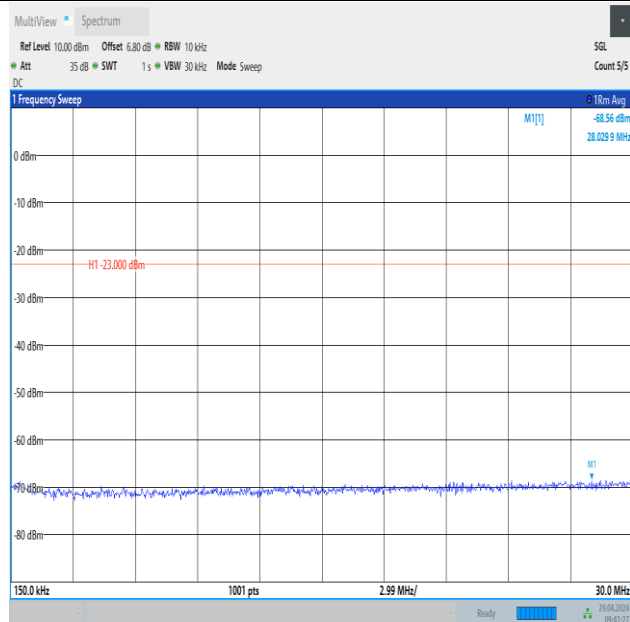
Band26_1.4MHz_QPSK_26915_1RB#5_0.15~30_0.15~30
