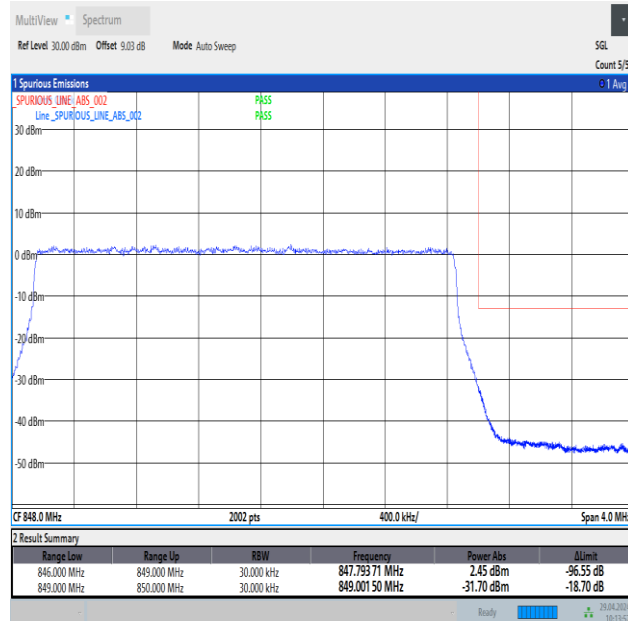
Band26_3MHz_QPSK_27025_15RB#0
