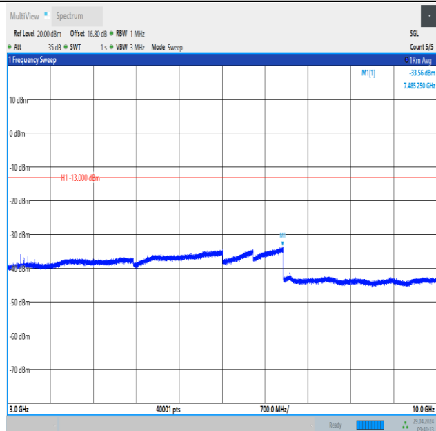
Band26_1.4MHz_16QAM_26915_1RB#0_3000~10000_3000~10000
