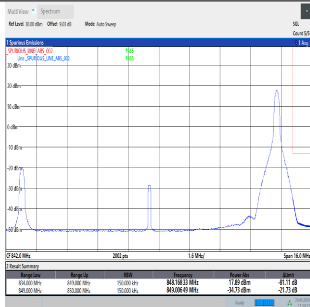
Band26_15MHz_16QAM_26965_1RB#74
