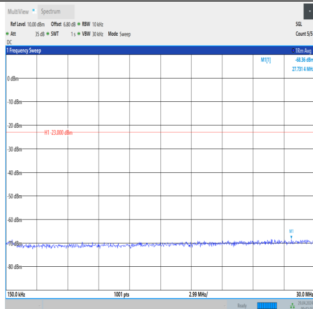
Band26_1.4MHz_16QAM_26915_1RB#5_0.15~30_0.15~30
