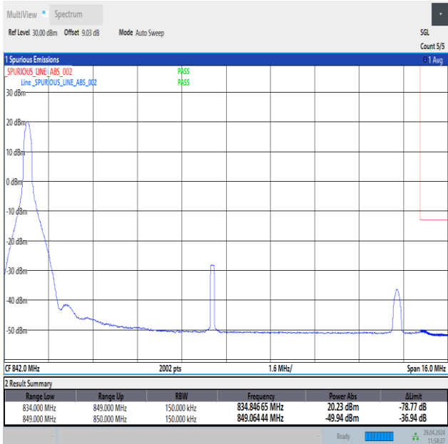
Band26_15MHz_QPSK_26965_1RB#0
