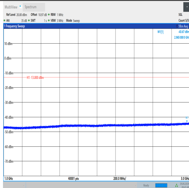
Band26_1.4MHz_QPSK_26915_1RB#5_1000~3000_1000~3000
