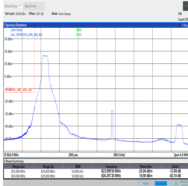
Band26_5MHz_QPSK_26815_1RB#0
