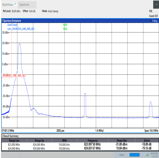
Band26_15MHz_16QAM_26865_1RB#0
