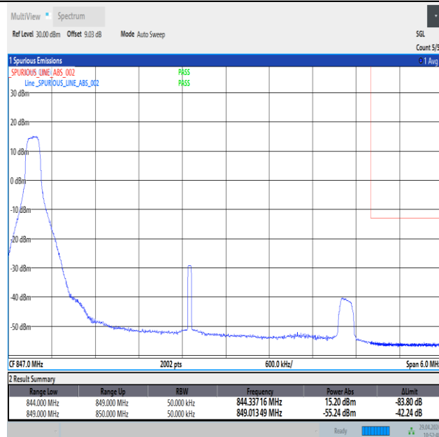
Band26_5MHz_16QAM_27015_1RB#0
