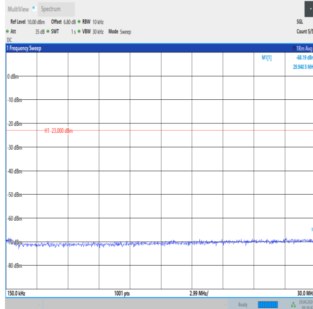
Band26_1.4MHz_QPSK_26797_1RB#5_0.15~30_0.15~30
