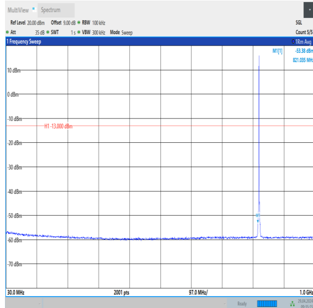
Band26_1.4MHz_QPSK_26797_1RB#0_30~1000_30~1000
