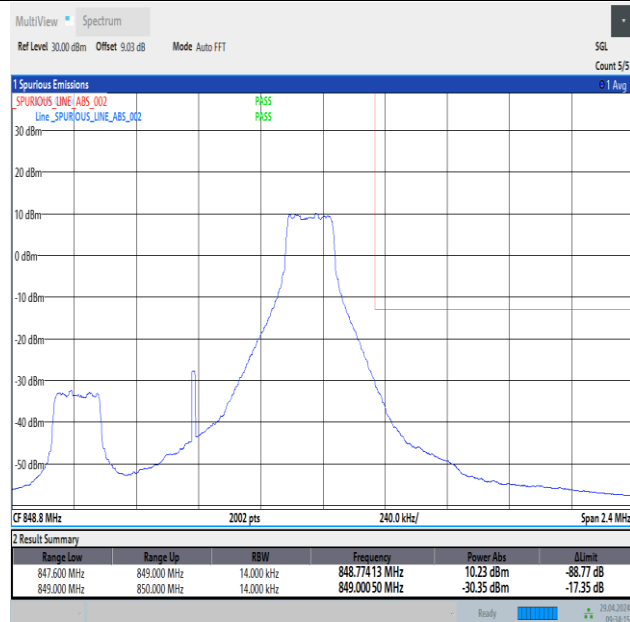
Band26_1.4MHz_16QAM_27033_1RB#5
