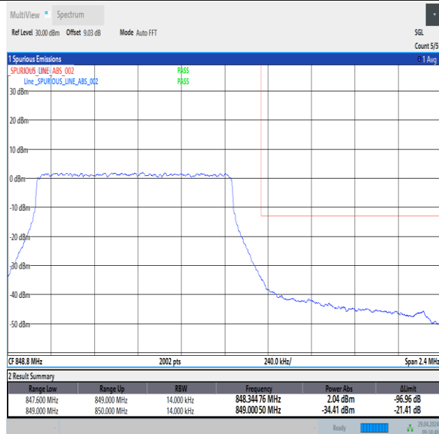
Band26_1.4MHz_16QAM_27033_6RB#0
