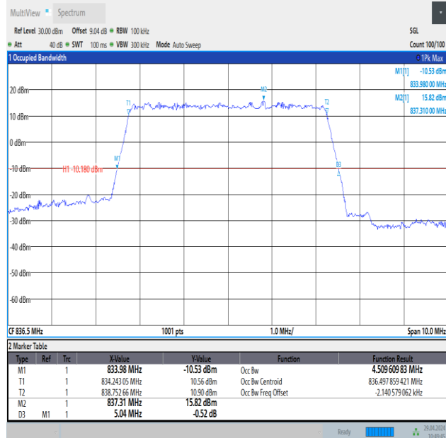
Band26(824-849)-5MHz-QPSK-26915-25RB#0-PASS
