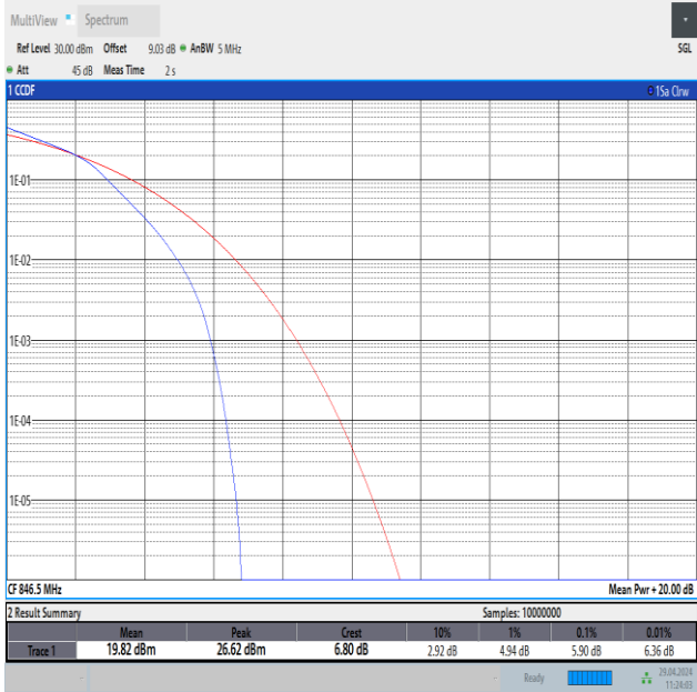
Band26(824-849)-5MHz-16QAM-27015-25RB#0-PASS
