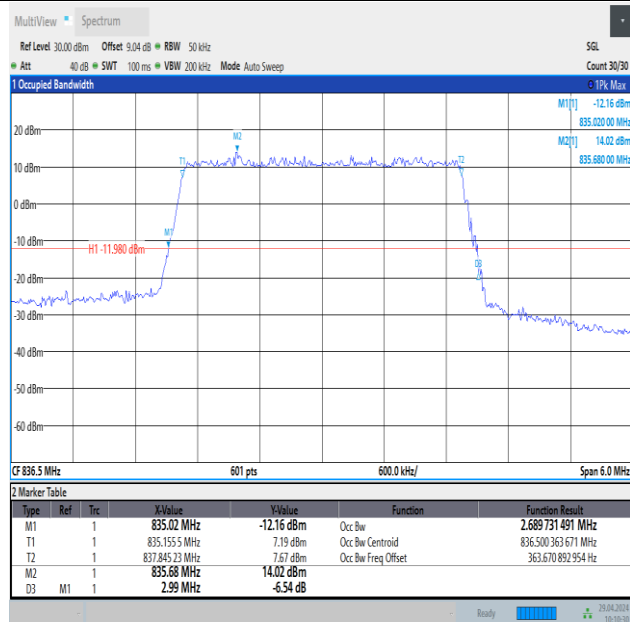
Band26(824-849)-3MHz-16QAM-26915-15RB#0-PASS
