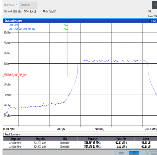
Band26_1.4MHz_QPSK_26797_6RB#0
