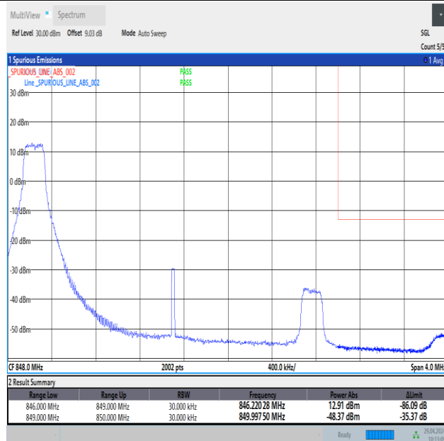
Band26_3MHz_16QAM_27025_1RB#0
