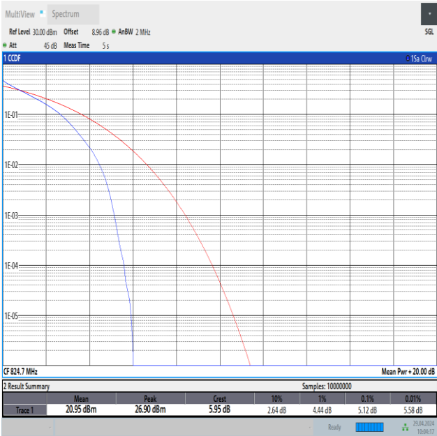
Band26(824-849)-1.4MHz-QPSK-26797-6RB#0-PASS
