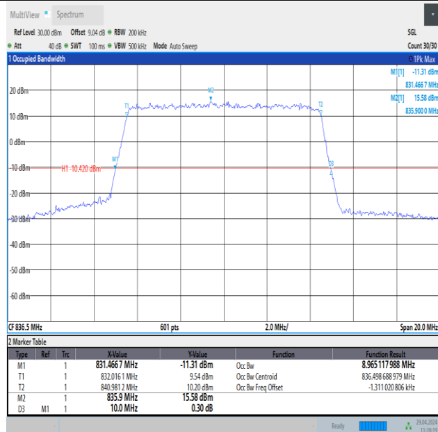
Band26(824-849)-10MHz-QPSK-26915-50RB#0-PASS
