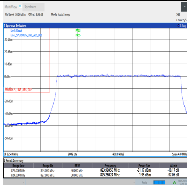
Band26_3MHz_16QAM_26805_15RB#0
