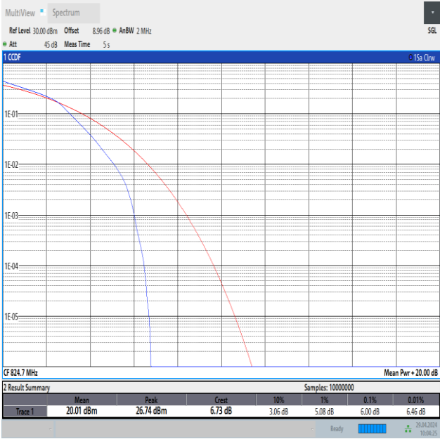
Band26(824-849)-1.4MHz-16QAM-26797-6RB#0-PASS
