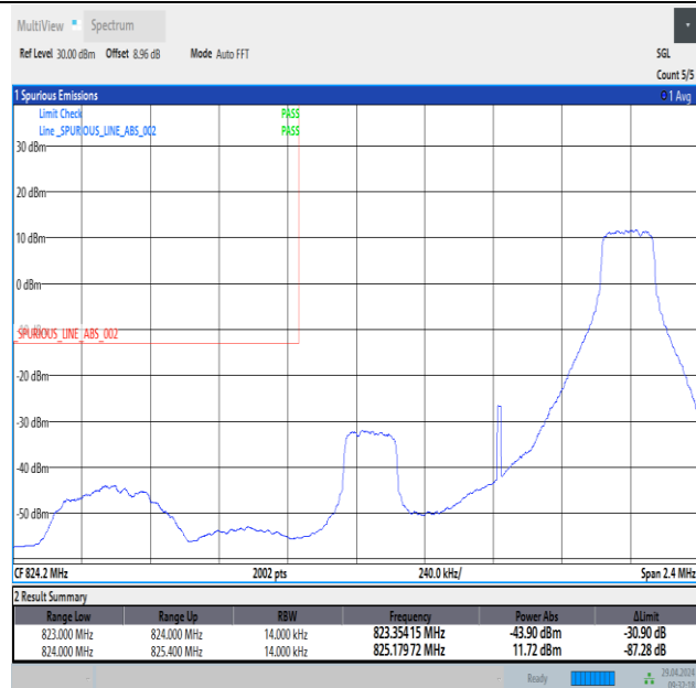
Band26_1.4MHz_QPSK_26797_1RB#5
