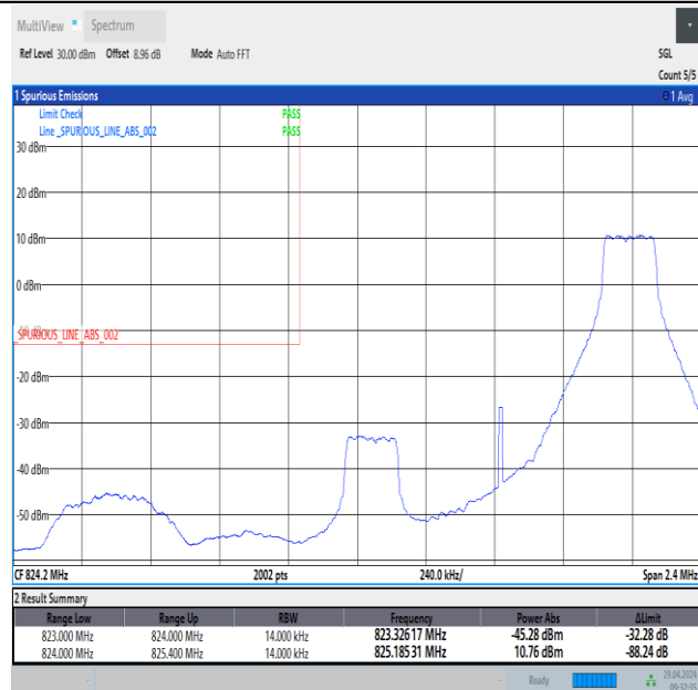
Band26_1.4MHz_16QAM_26797_1RB#5
