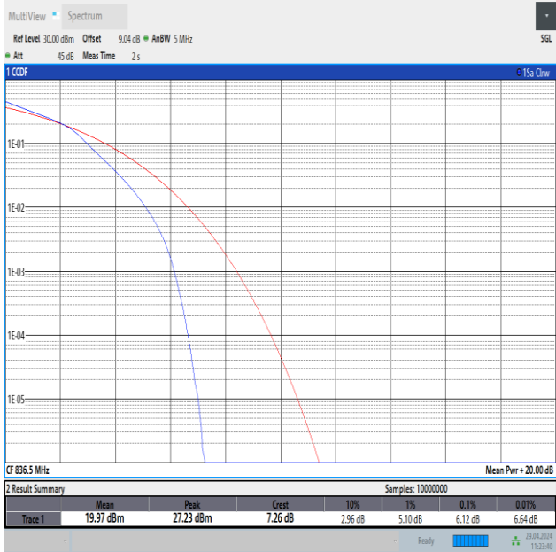
Band26(824-849)-5MHz-16QAM-26915-25RB#0-PASS
