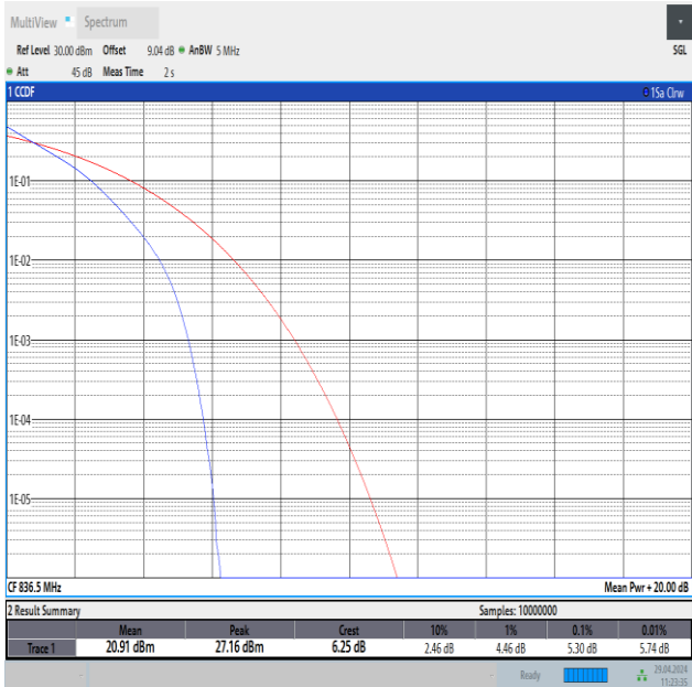
Band26(824-849)-5MHz-QPSK-26915-25RB#0-PASS
