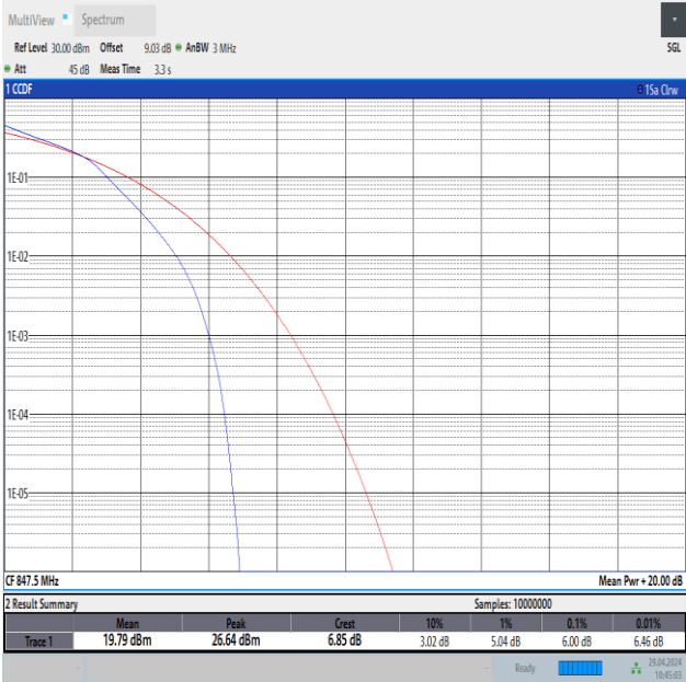
Band26(824-849)-3MHz-16QAM-27025-15RB#0-PASS
