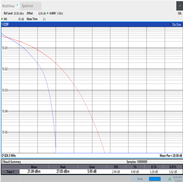
Band26(824-849)-5MHz-QPSK-26815-25RB#0-PASS
