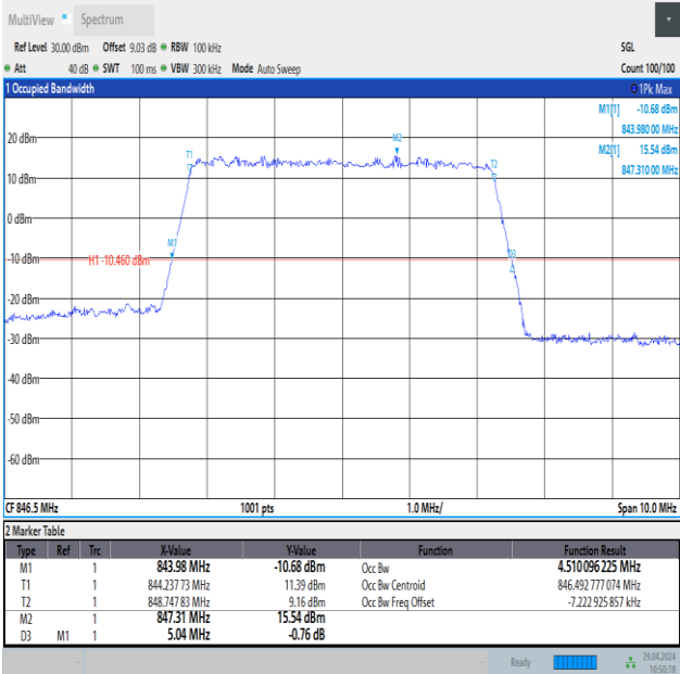
Band26(824-849)-5MHz-QPSK-27015-25RB#0-PASS
