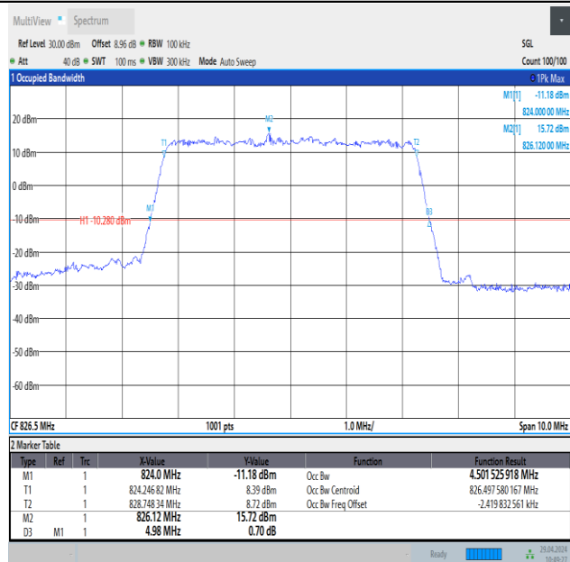
Band26(824-849)-5MHz-16QAM-26815-25RB#0-PASS
