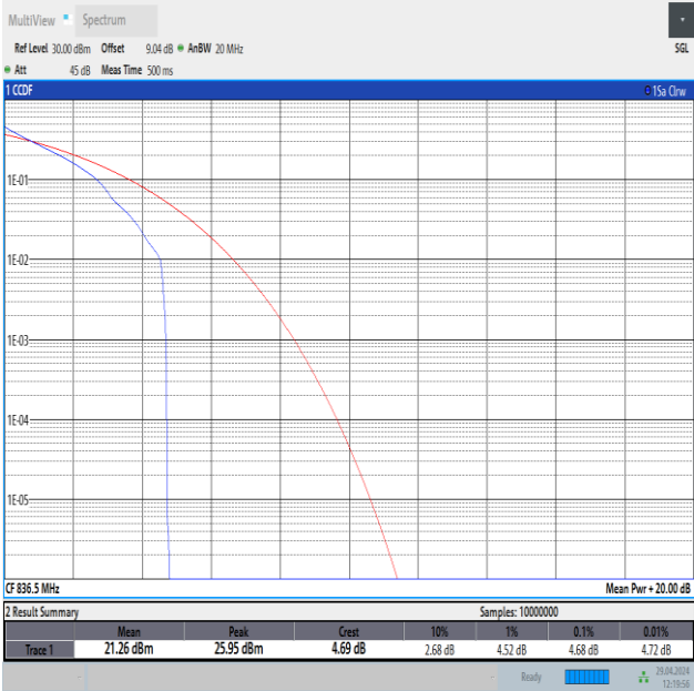
Band26(824-849)-15MHz-QPSK-26915-1RB#0-PASS
