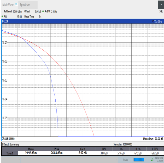
Band26(824-849)-1.4MHz-16QAM-26915-6RB#0-PASS
