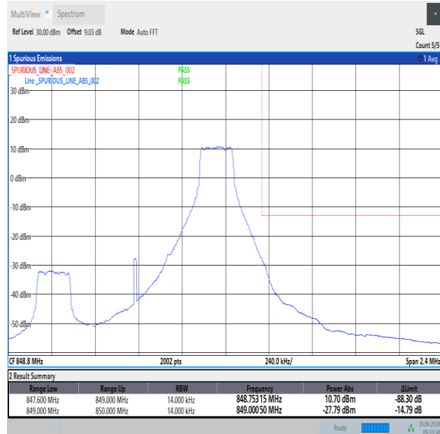
Band26_1.4MHz_QPSK_27033_1RB#5
