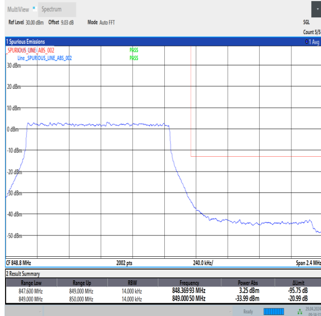
Band26_1.4MHz_QPSK_27033_6RB#0
