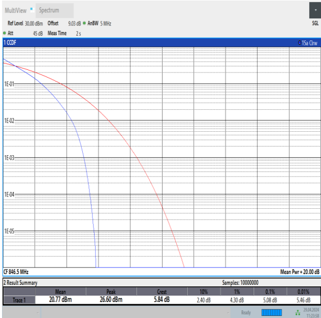
Band26(824-849)-5MHz-QPSK-27015-25RB#0-PASS
