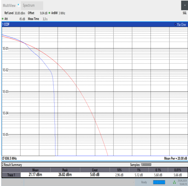
Band26(824-849)-3MHz-16QAM-26915-1RB#0-PASS
