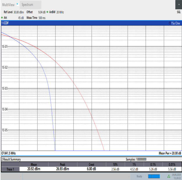
Band26(824-849)-15MHz-QPSK-26965-75RB#0-PASS
