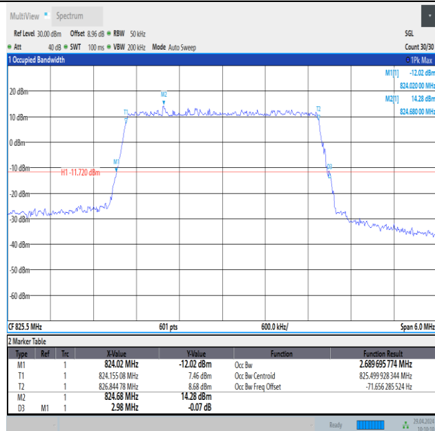
Band26(824-849)-3MHz-16QAM-26805-15RB#0-PASS
