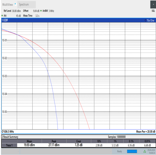
Band26(824-849)-3MHz-16QAM-26915-15RB#0-PASS
