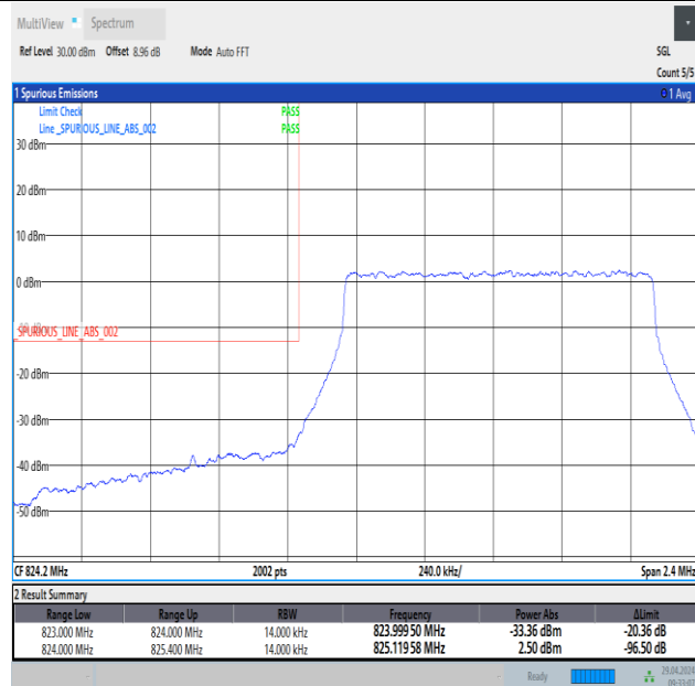
Band26_1.4MHz_16QAM_26797_6RB#0
