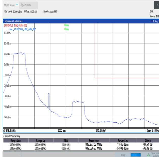
Band26_1.4MHz_QPSK_27033_1RB#0
