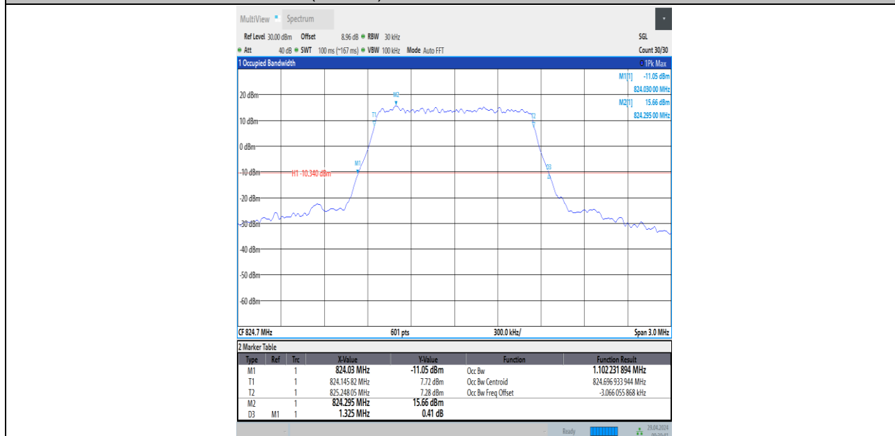
Band26(824-849)-1.4MHz-16QAM-26797-6RB#0-PASS
