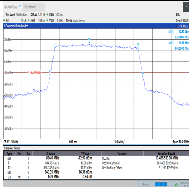
Band26(824-849)-15MHz-QPSK-26965-75RB#0-PASS
