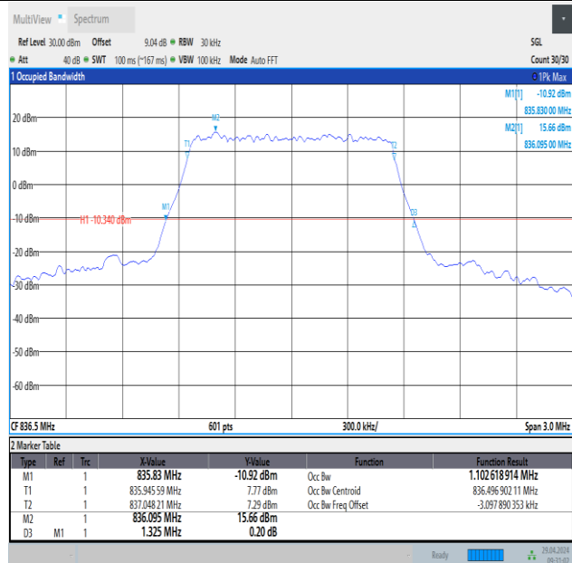
Band26(824-849)-1.4MHz-16QAM-26915-6RB#0-PASS
