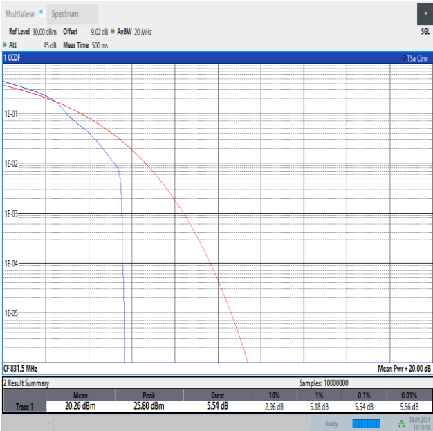
Band26(824-849)-15MHz-16QAM-26865-1RB#0-PASS
