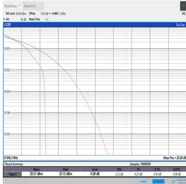
Band26(824-849)-1.4MHz-QPSK-27033-1RB#0-PASS
