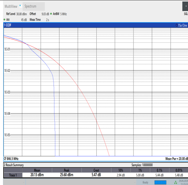
Band26(824-849)-5MHz-16QAM-27015-1RB#0-PASS
