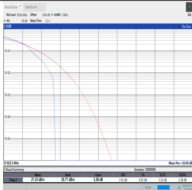
Band26(824-849)-3MHz-16QAM-26805-1RB#0-PASS
