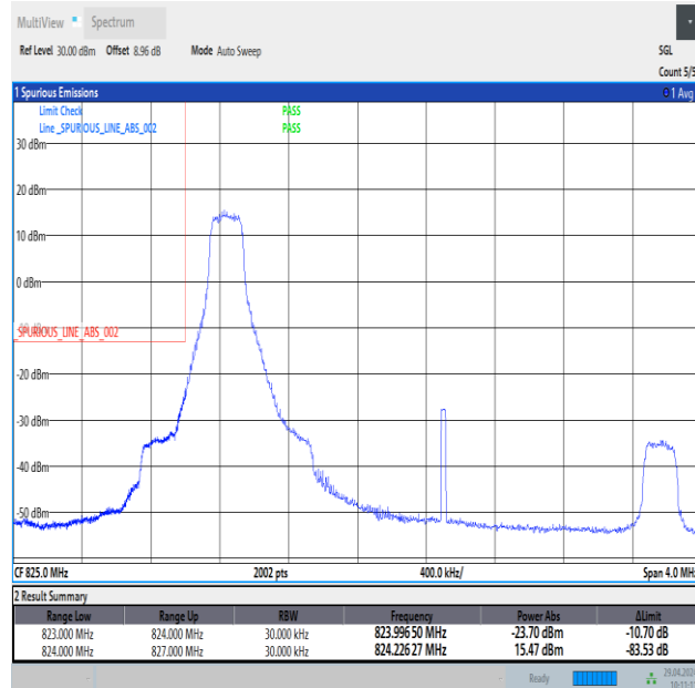
Band26_3MHz_QPSK_26805_1RB#0
