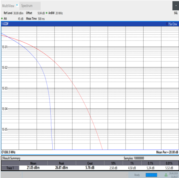
Band26(824-849)-15MHz-QPSK-26915-75RB#0-PASS
