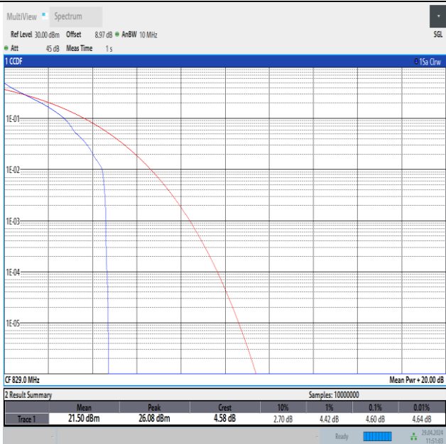
Band26(824-849)-10MHz-QPSK-26840-1RB#0-PASS
