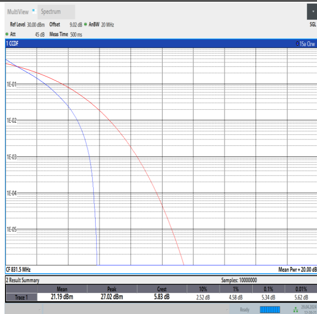
Band26(824-849)-15MHz-QPSK-26865-75RB#0-PASS
