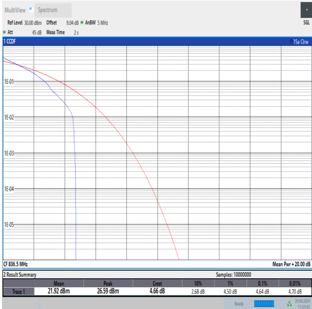
Band26(824-849)-5MHz-QPSK-26915-1RB#0-PASS
