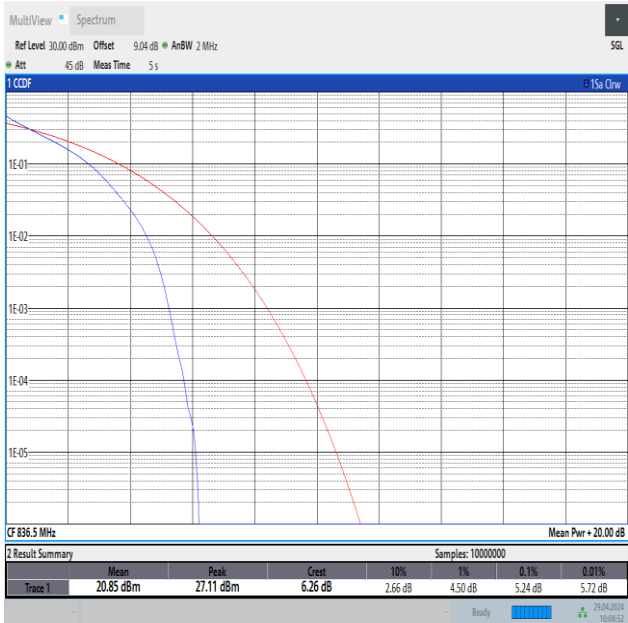
Band26(824-849)-1.4MHz-QPSK-26915-6RB#0-PASS
