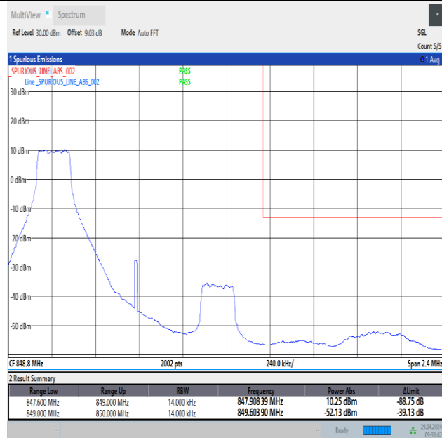
Band26_1.4MHz_16QAM_27033_1RB#0
