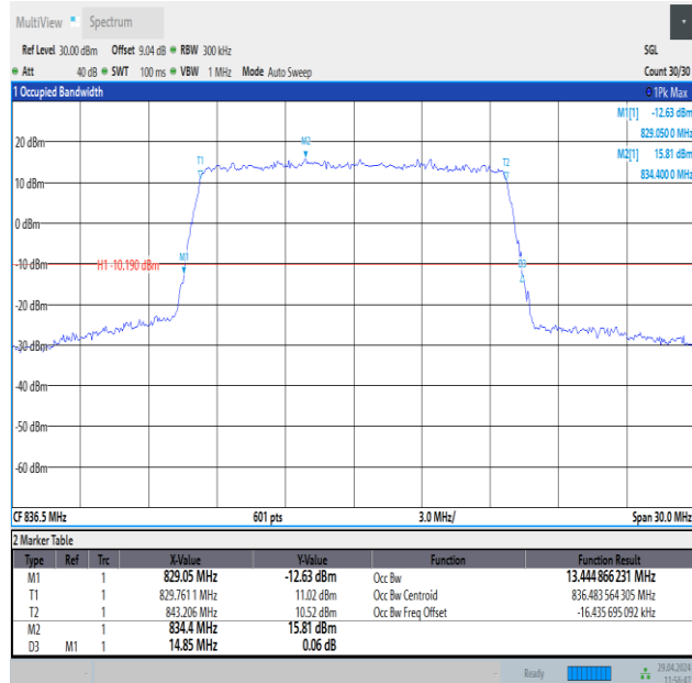
Band26(824-849)-15MHz-QPSK-26915-75RB#0-PASS
