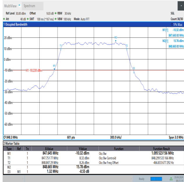
Band26(824-849)-1.4MHz-QPSK-27033-6RB#0-PASS
