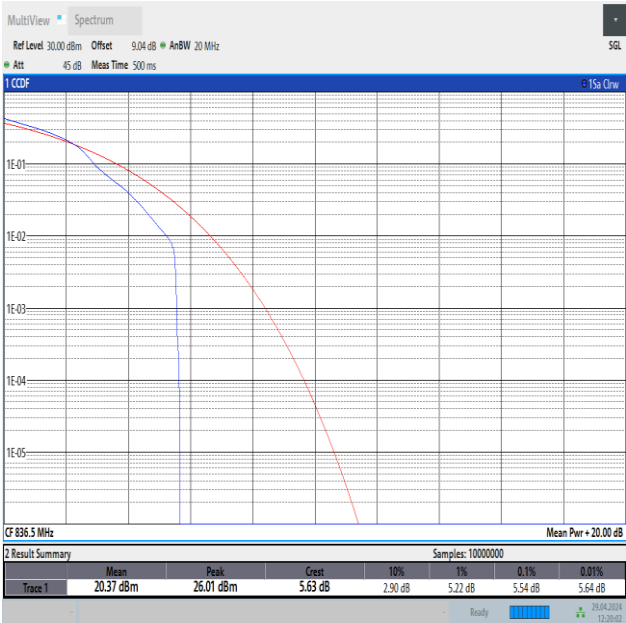
Band26(824-849)-15MHz-16QAM-26915-1RB#0-PASS
