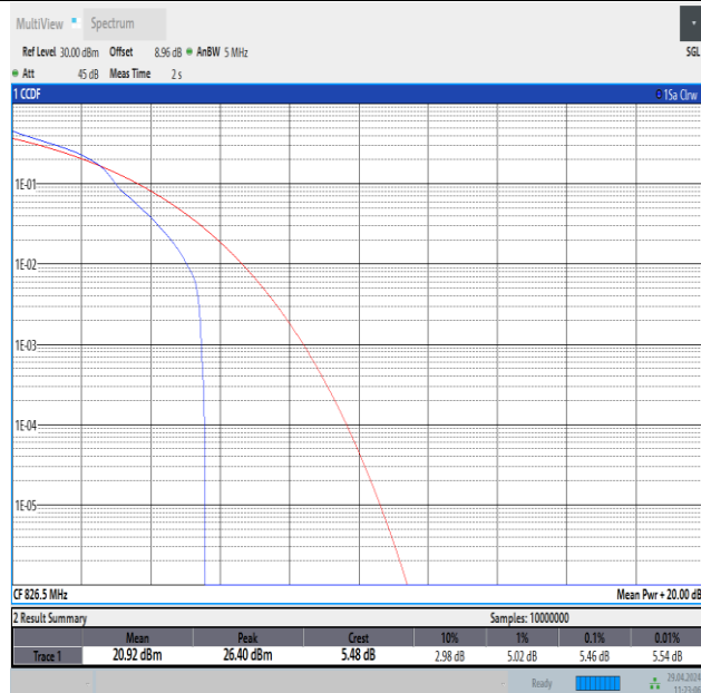
Band26(824-849)-5MHz-16QAM-26815-1RB#0-PASS
