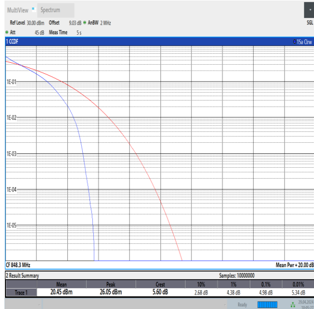
Band26(824-849)-1.4MHz-QPSK-27033-6RB#0-PASS
