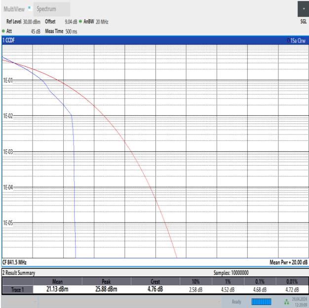
Band26(824-849)-15MHz-QPSK-26965-1RB#0-PASS
