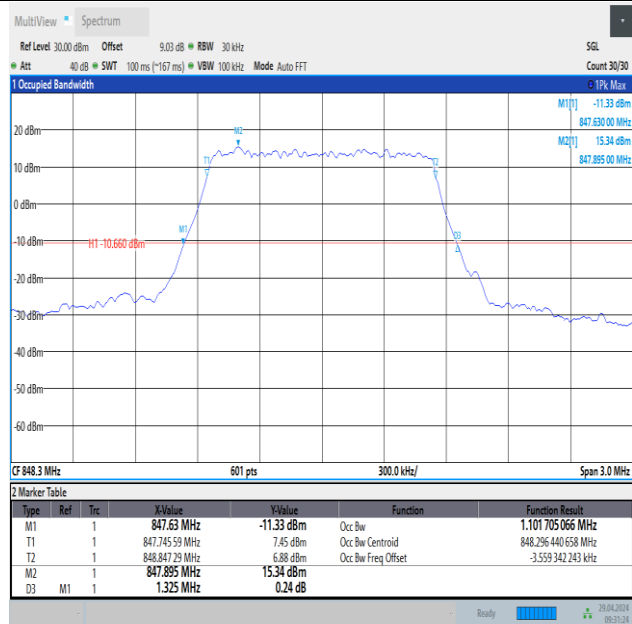
Band26(824-849)-1.4MHz-16QAM-27033-6RB#0-PASS
