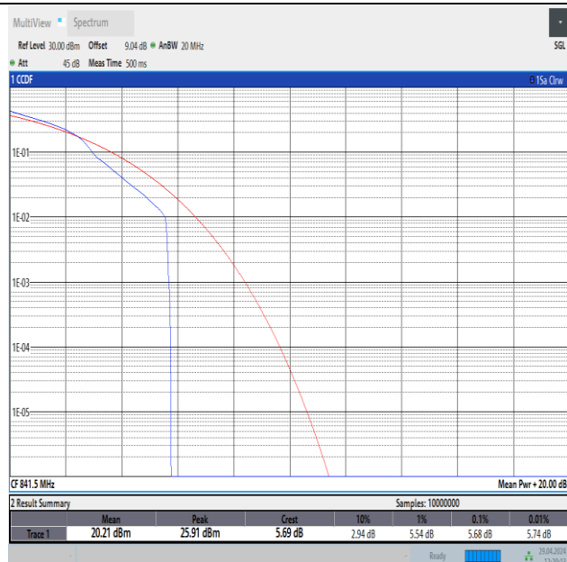
Band26(824-849)-15MHz-16QAM-26965-1RB#0-PASS
