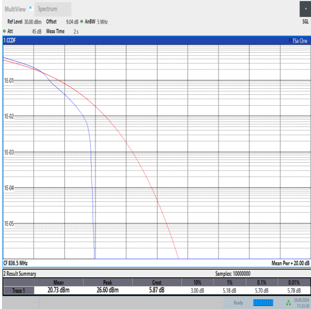
Band26(824-849)-5MHz-16QAM-26915-1RB#0-PASS
