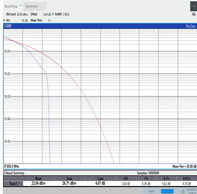
Band26(824-849)-1.4MHz-QPSK-26915-1RB#0-PASS
