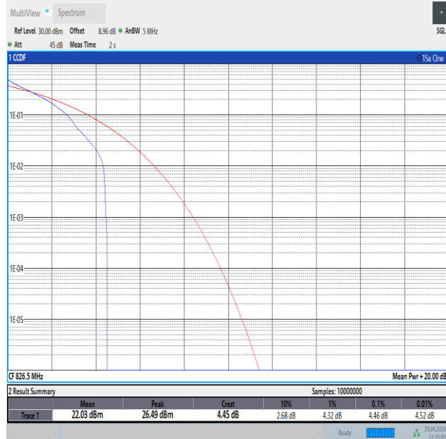
Band26(824-849)-5MHz-QPSK-26815-1RB#0-PASS
