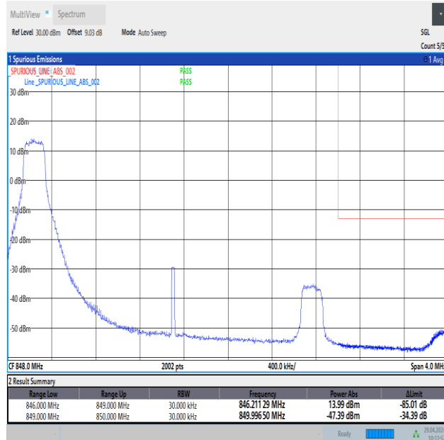
Band26_3MHz_QPSK_27025_1RB#0
