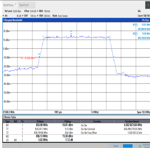
Band26(824-849)-5MHz-16QAM-26915-25RB#0-PASS
