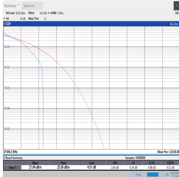
Band26(824-849)-5MHz-QPSK-27015-1RB#0-PASS
