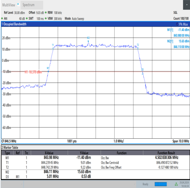
Band26(824-849)-5MHz-16QAM-27015-25RB#0-PASS
