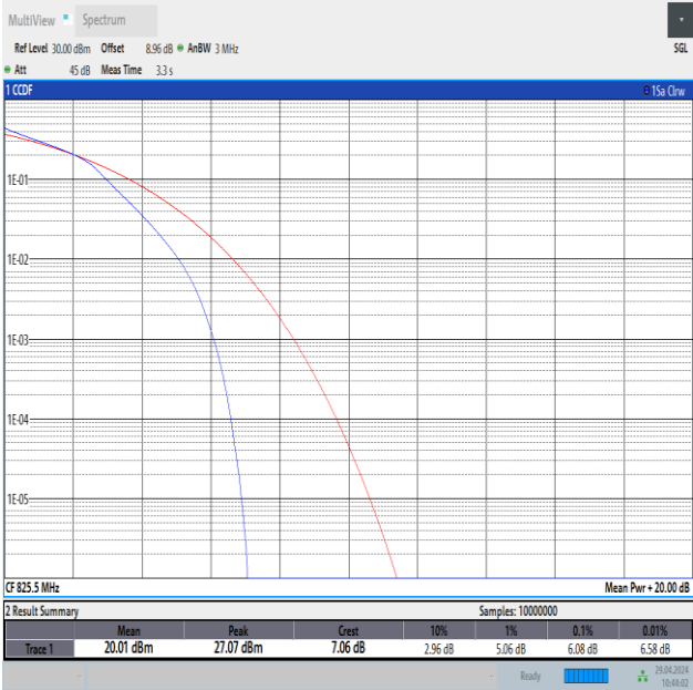
Band26(824-849)-3MHz-16QAM-26805-15RB#0-PASS
