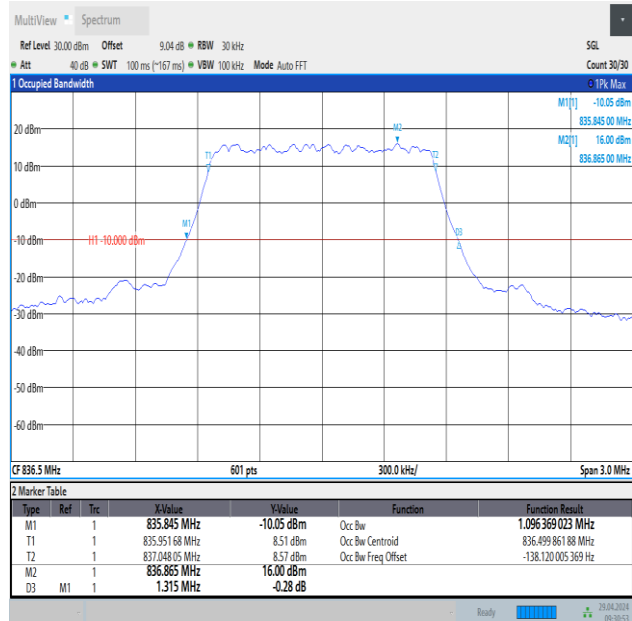
Band26(824-849)-1.4MHz-QPSK-26915-6RB#0-PASS
