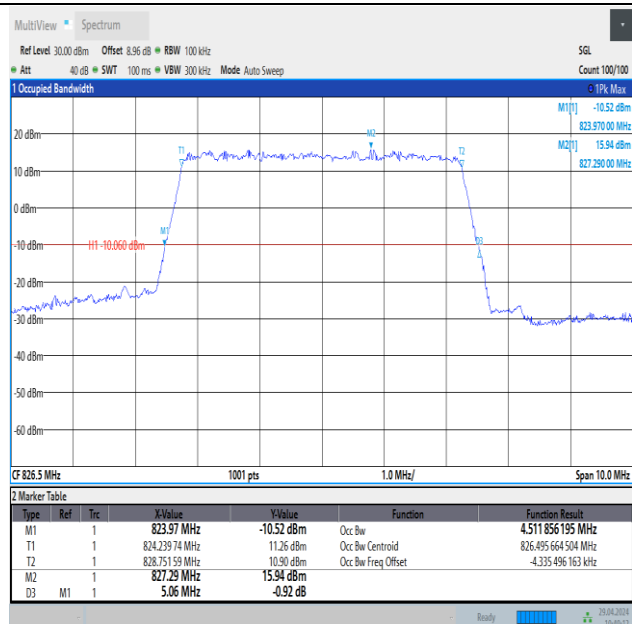
Band26(824-849)-5MHz-QPSK-26815-25RB#0-PASS
