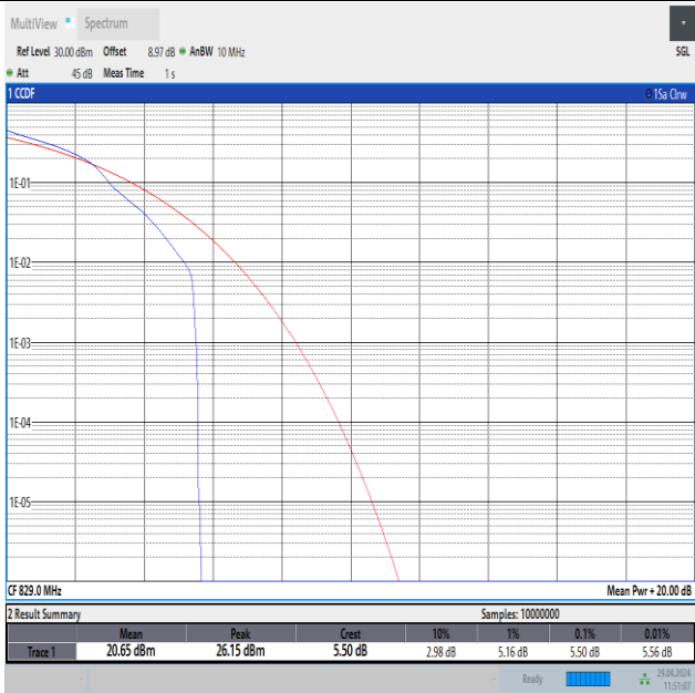
Band26(824-849)-10MHz-16QAM-26840-1RB#0-PASS
