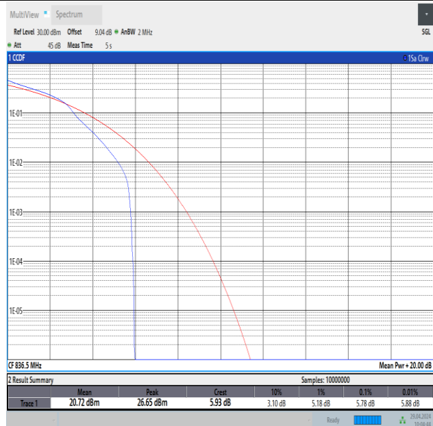
Band26(824-849)-1.4MHz-16QAM-26915-1RB#0-PASS
