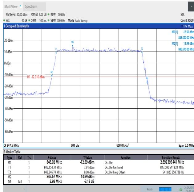
Band26(824-849)-3MHz-16QAM-27025-15RB#0-PASS
