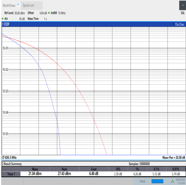
Band26(824-849)-10MHz-QPSK-26915-50RB#0-PASS
