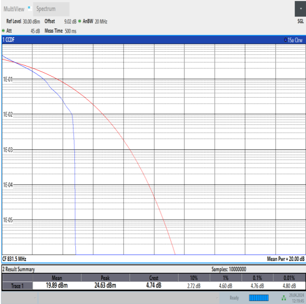
Band26(824-849)-15MHz-QPSK-26865-1RB#0-PASS
