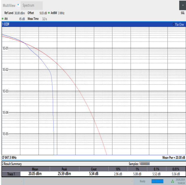
Band26(824-849)-3MHz-16QAM-27025-1RB#0-PASS
