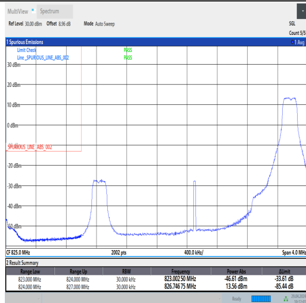
Band26_3MHz_16QAM_26805_1RB#14
