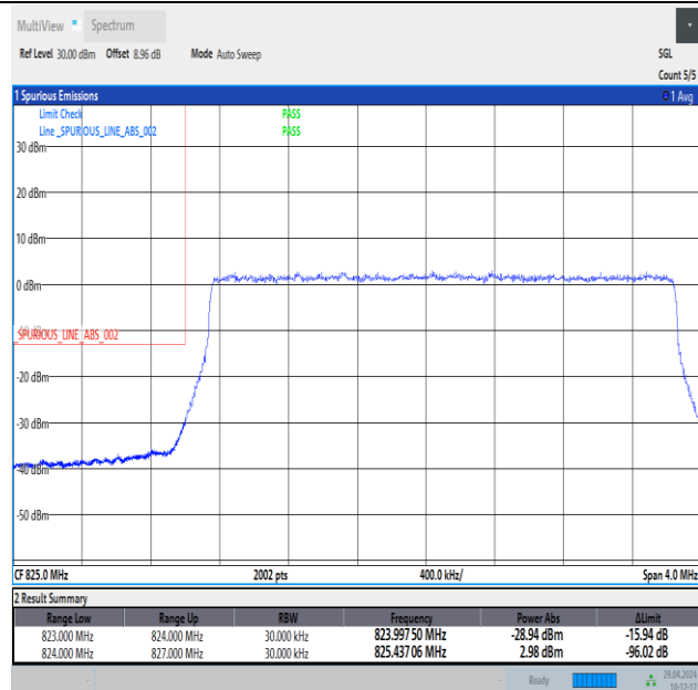
Band26_3MHz_QPSK_26805_15RB#0
