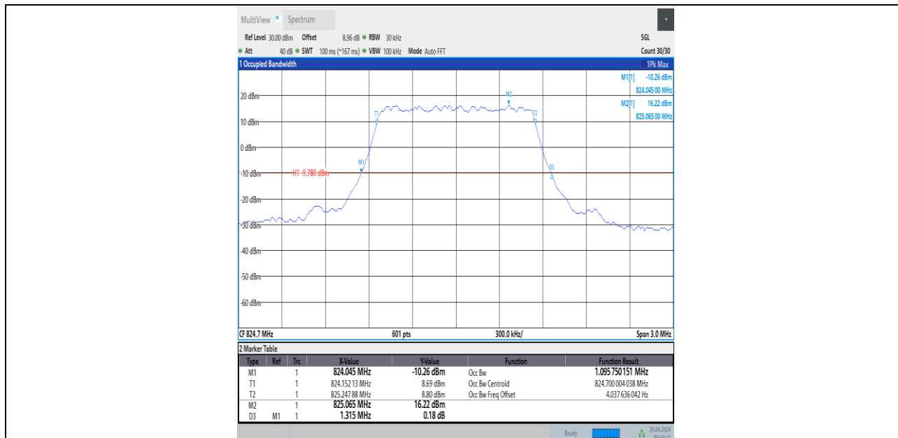
Band26(824-849)-1.4MHz-QPSK-26797-6RB#0-PASS
