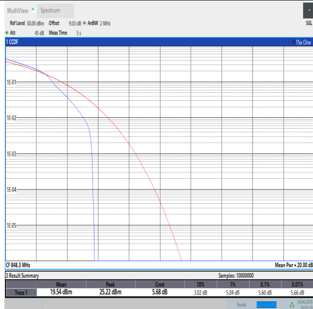
Band26(824-849)-1.4MHz-16QAM-27033-1RB#0-PASS
