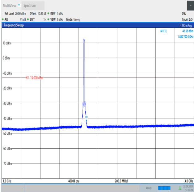
Band25_10MHz_QPSK_26090_50RB#0_1000~3000_1000~3000
