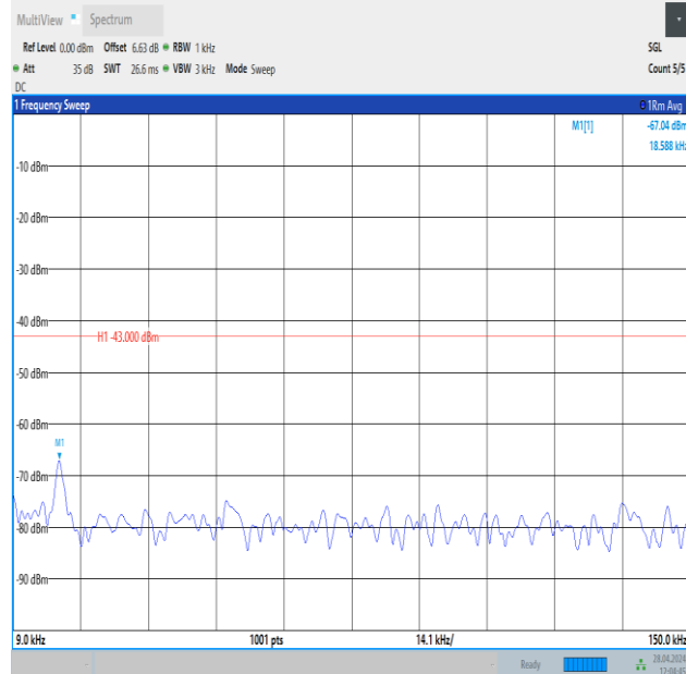
Band25_3MHz_16QAM_26675_1RB#14_0.009~0.15_0.009~0.15
