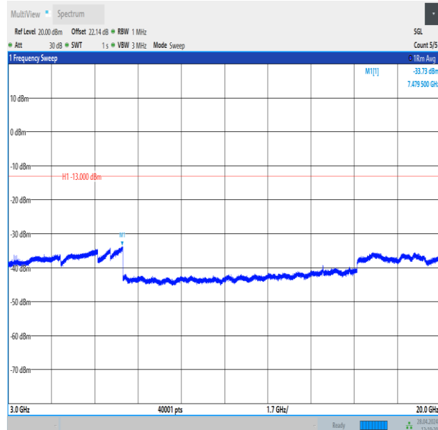
Band25_15MHz_QPSK_26615_1RB#74_3000~20000_3000~20000
