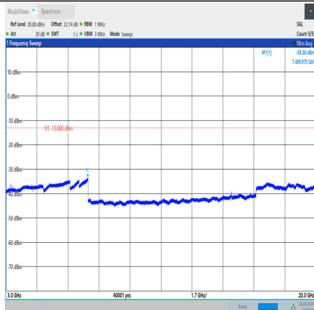
Band25_3MHz_QPSK_26675_1RB#14_3000~20000_3000~20000
