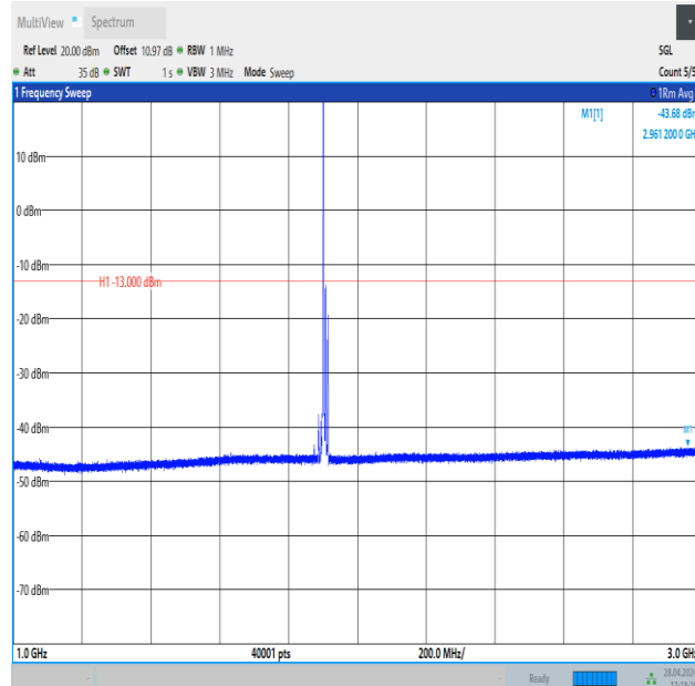
Band25_15MHz_16QAM_26615_1RB#0_1000~3000_1000~3000
