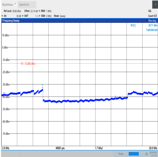
Band25_15MHz_16QAM_26115_1RB#0_3000~20000_3000~20000
