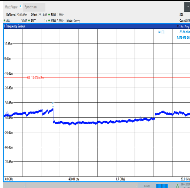
Band25_15MHz_QPSK_26615_1RB#0_3000~20000_3000~20000
