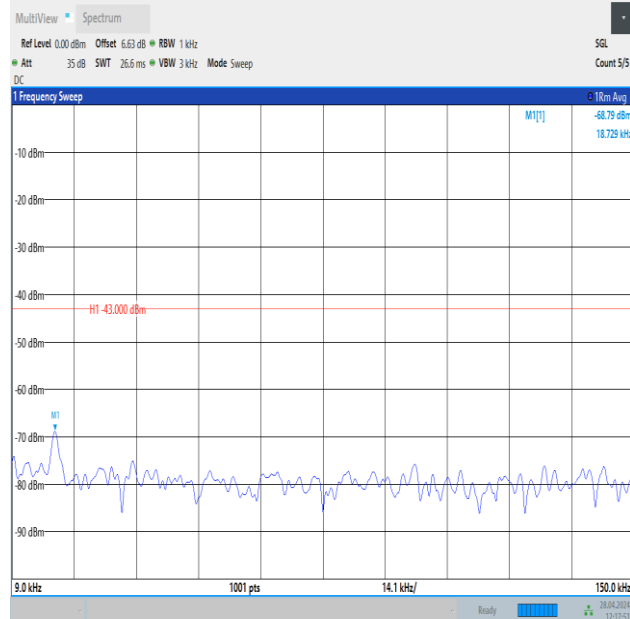
Band25_15MHz_16QAM_26615_1RB#0_0.009~0.15_0.009~0.15
