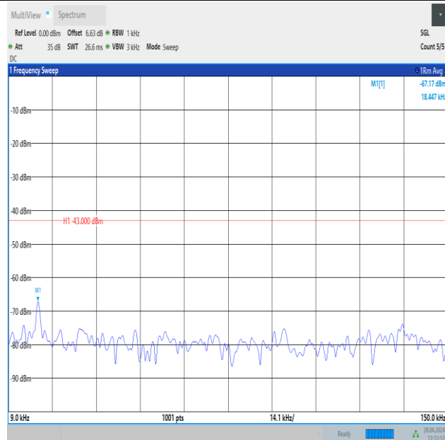
Band25_15MHz_16QAM_26115_1RB#74_0.009~0.15_0.009~0.15
