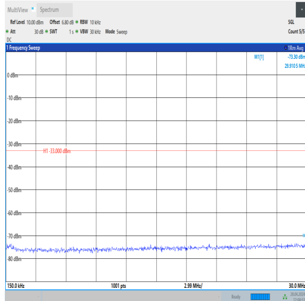
Band25_3MHz_16QAM_26675_1RB#14_0.15~30_0.15~30
