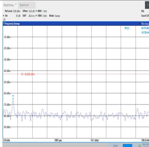
Band25_3MHz_16QAM_26675_1RB#0_0.009~0.15_0.009~0.15
