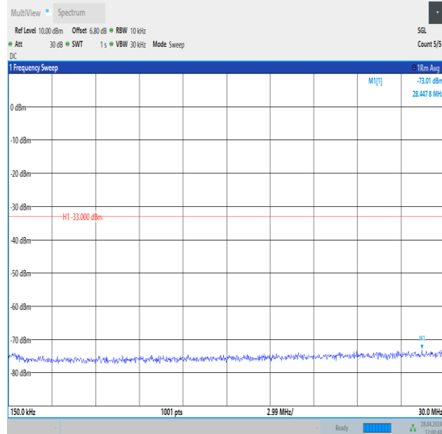
Band25_3MHz_QPSK_26365_15RB#0_0.15~30_0.15~30
