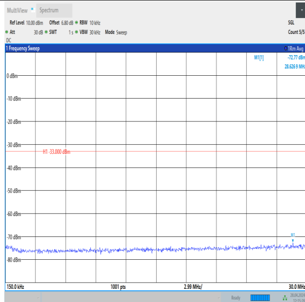
Band25_15MHz_QPSK_26365_1RB#74_0.15~30_0.15~30
