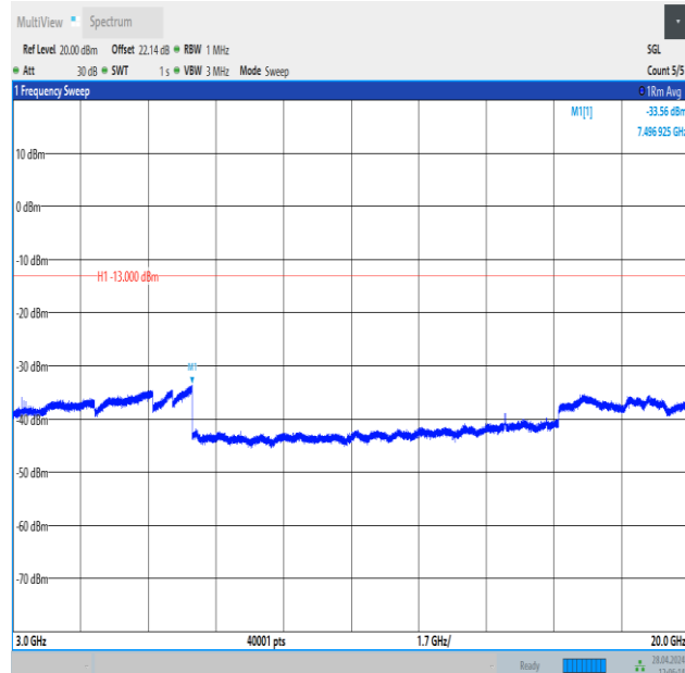
Band25_3MHz_QPSK_26675_15RB#0_3000~20000_3000~20000
