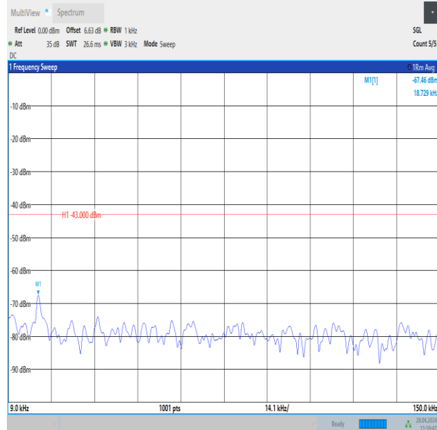
Band25_3MHz_16QAM_26365_1RB#14_0.009~0.15_0.009~0.15
