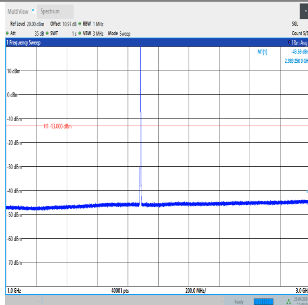
Band25_3MHz_16QAM_26365_1RB#14_1000~3000_1000~3000
