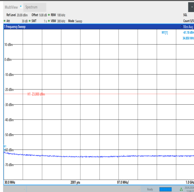
Band25_3MHz_QPSK_26675_1RB#14_30~1000_30~1000
