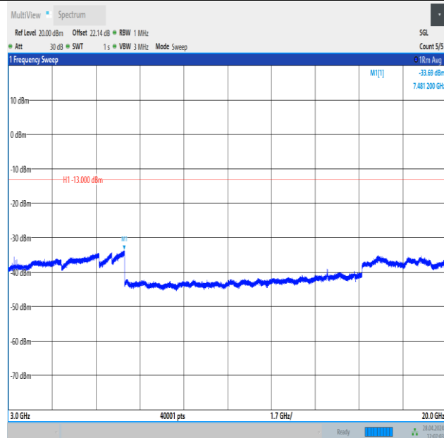
Band25_3MHz_16QAM_26675_15RB#0_3000~20000_3000~20000
