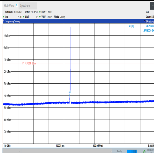
Band25_3MHz_16QAM_26365_15RB#0_1000~3000_1000~3000
