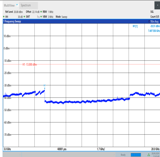
Band25_3MHz_16QAM_26675_1RB#0_3000~20000_3000~20000
