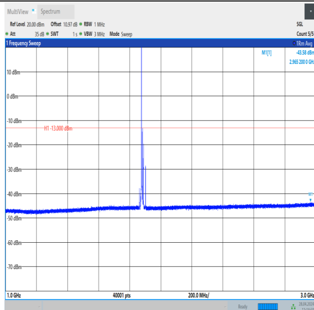
Band25_15MHz_16QAM_26365_1RB#0_1000~3000_1000~3000
