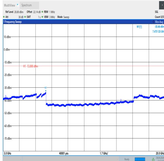
Band25_15MHz_QPSK_26115_1RB#74_3000~20000_3000~20000
