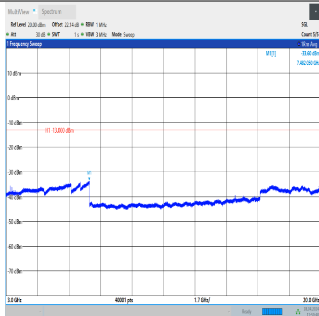
Band25_3MHz_QPSK_26365_1RB#14_3000~20000_3000~20000
