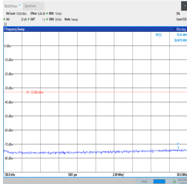
Band25_15MHz_16QAM_26365_1RB#74_0.15~30_0.15~30
