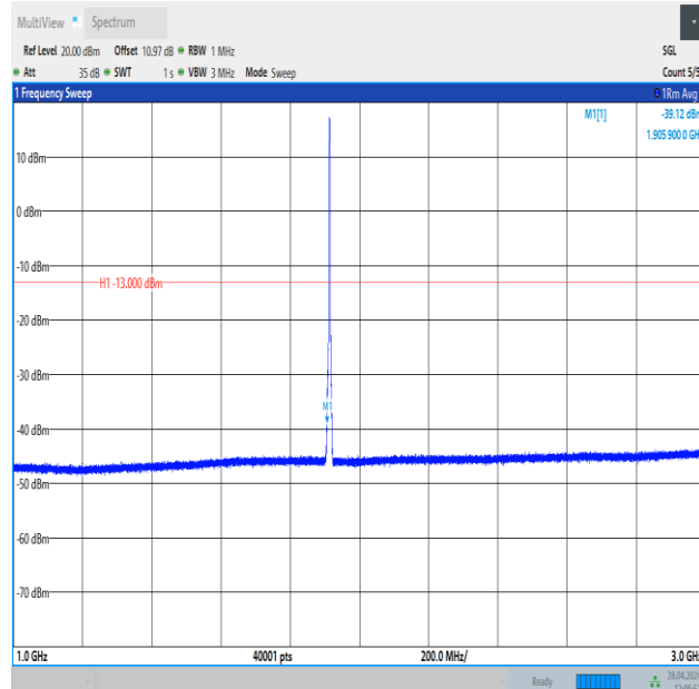
Band25_3MHz_16QAM_26675_15RB#0_1000~3000_1000~3000
