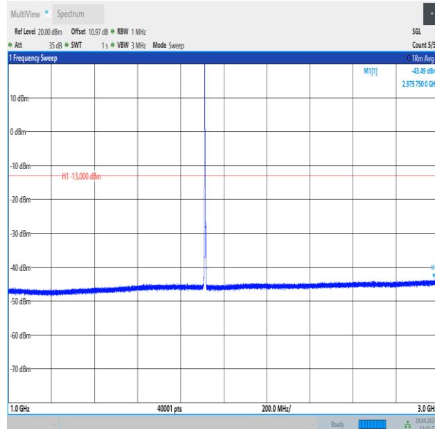
Band25_3MHz_16QAM_26675_1RB#0_1000~3000_1000~3000
