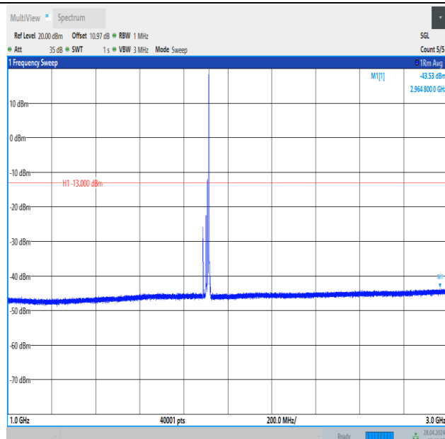
Band25_15MHz_16QAM_26615_1RB#74_1000~3000_1000~3000
