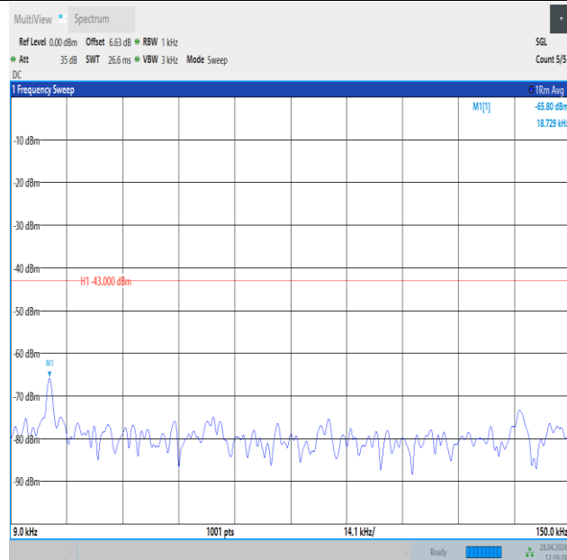
Band25_15MHz_16QAM_26615_1RB#74_0.009~0.15_0.009~0.15
