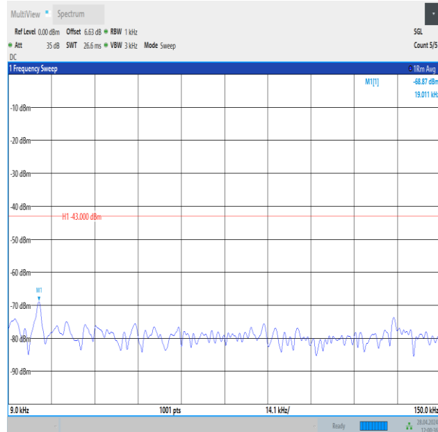
Band25_3MHz_QPSK_26365_15RB#0_0.009~0.15_0.009~0.15
