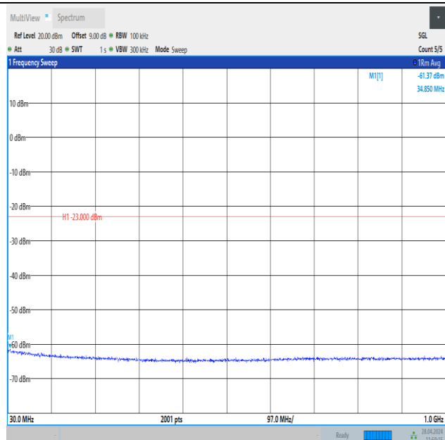
Band25_3MHz_QPSK_26365_1RB#14_30~1000_30~1000
