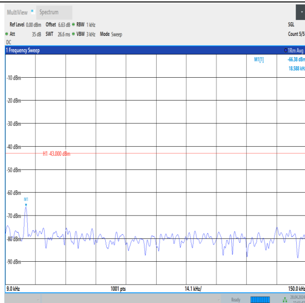
Band25_3MHz_QPSK_26055_15RB#0_0.009~0.15_0.009~0.15
