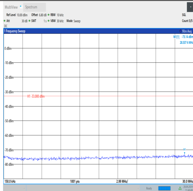
Band25_20MHz_QPSK_26140_100RB#0_0.15~30_0.15~30
