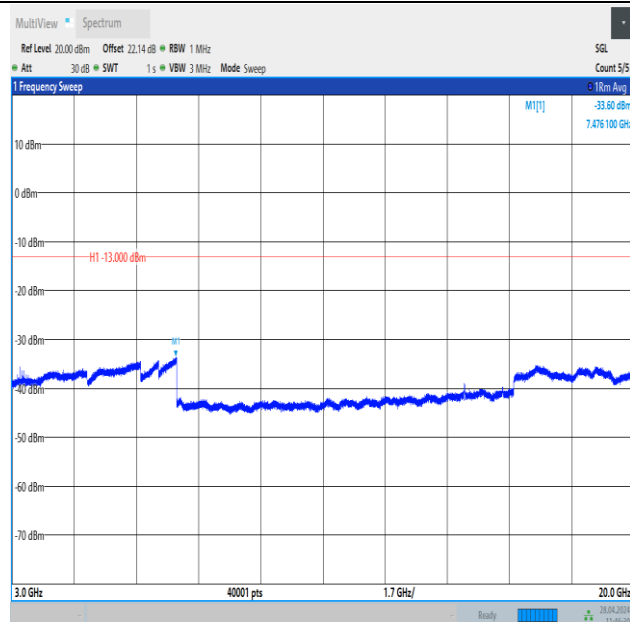
Band25_20MHz_QPSK_26365_1RB#0_3000~20000_3000~20000
