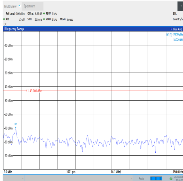
Band25_20MHz_QPSK_26140_100RB#0_0.009~0.15_0.009~0.15
