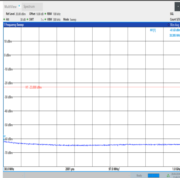
Band25_20MHz_QPSK_26590_1RB#0_30~1000_30~1000
