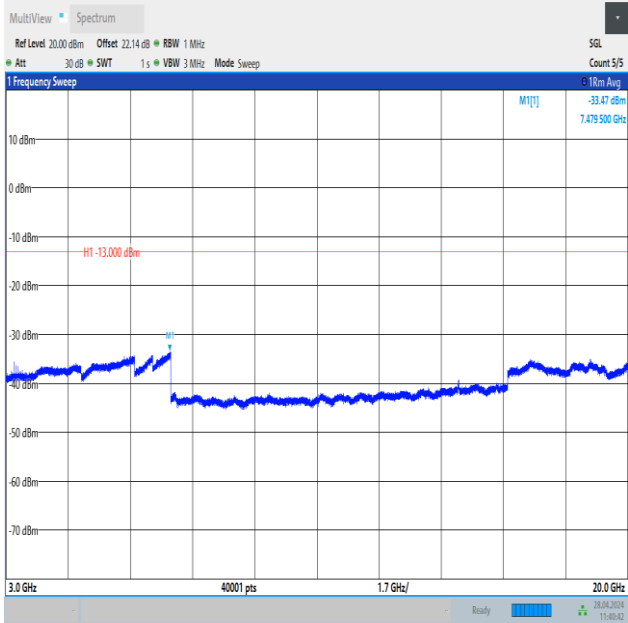
Band25_20MHz_QPSK_26140_100RB#0_3000~20000_3000~20000
