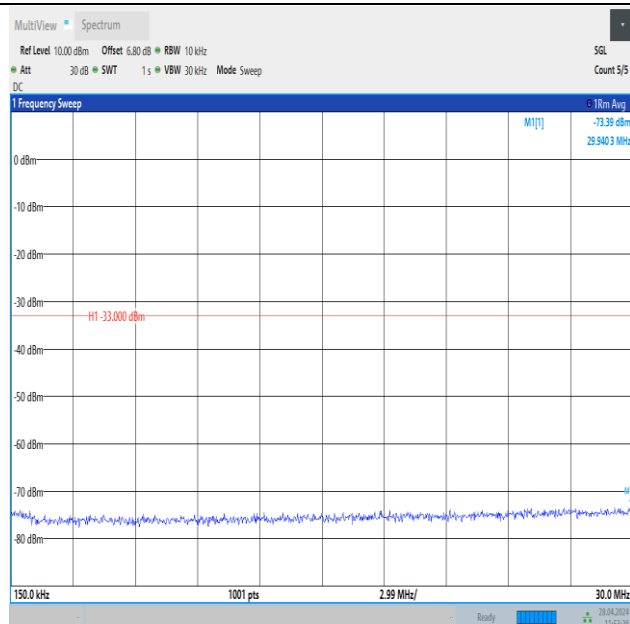
Band25_3MHz_16QAM_26055_1RB#0_0.15~30_0.15~30
