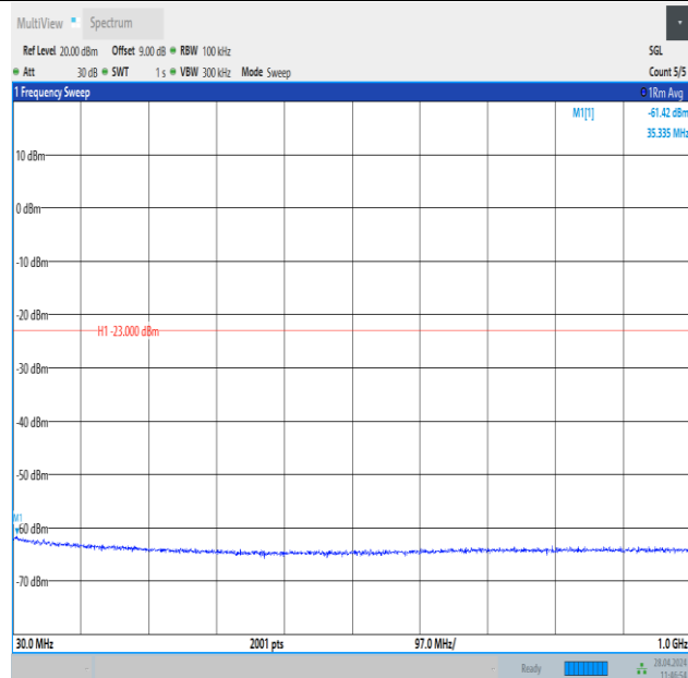
Band25_20MHz_16QAM_26365_1RB#0_30~1000_30~1000
