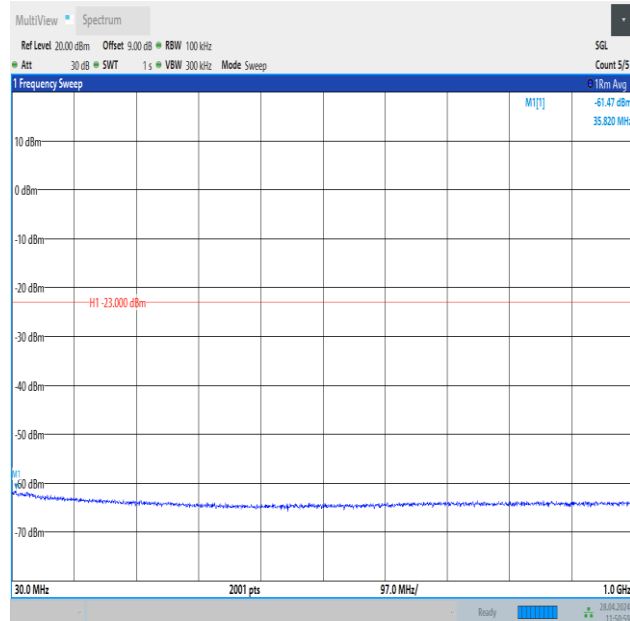
Band25_20MHz_QPSK_26590_1RB#99_30~1000_30~1000
