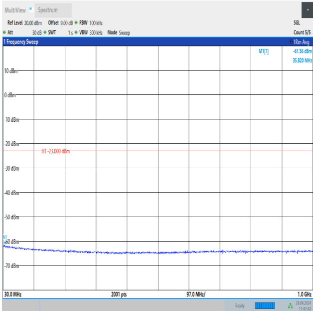
Band25_20MHz_QPSK_26365_1RB#99_30~1000_30~1000
