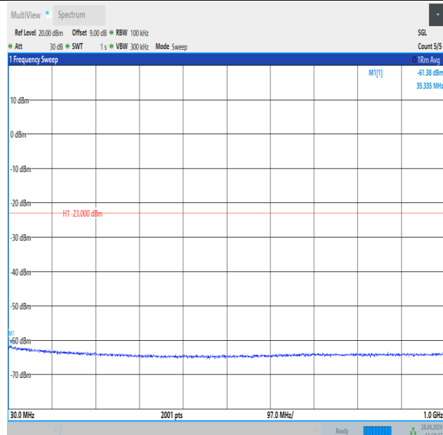
Band25_3MHz_16QAM_26365_1RB#0_30~1000_30~1000
