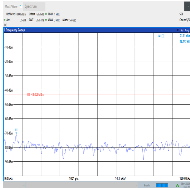
Band25_20MHz_16QAM_26365_1RB#99_0.009~0.15_0.009~0.15
