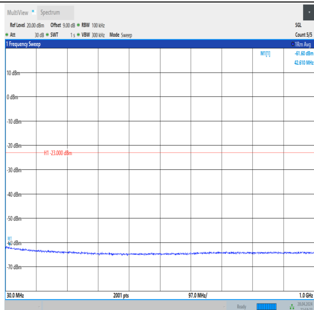
Band25_3MHz_QPSK_26055_1RB#14_30~1000_30~1000
