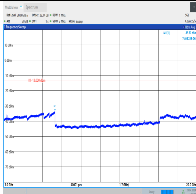
Band25_20MHz_QPSK_26590_1RB#0_3000~20000_3000~20000
