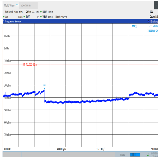
Band25_20MHz_16QAM_26590_1RB#0_3000~20000_3000~20000
