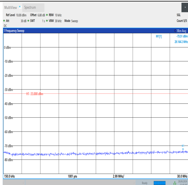
Band25_20MHz_16QAM_26140_1RB#99_0.15~30_0.15~30
