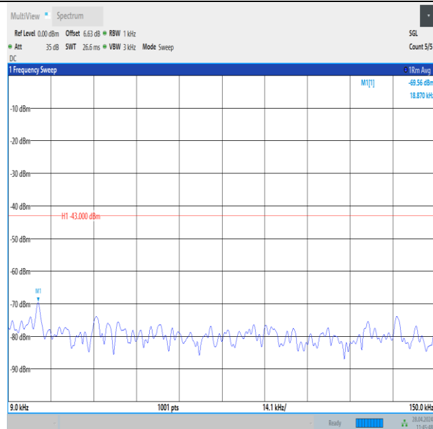
Band25_20MHz_QPSK_26365_1RB#0_0.009~0.15_0.009~0.15
