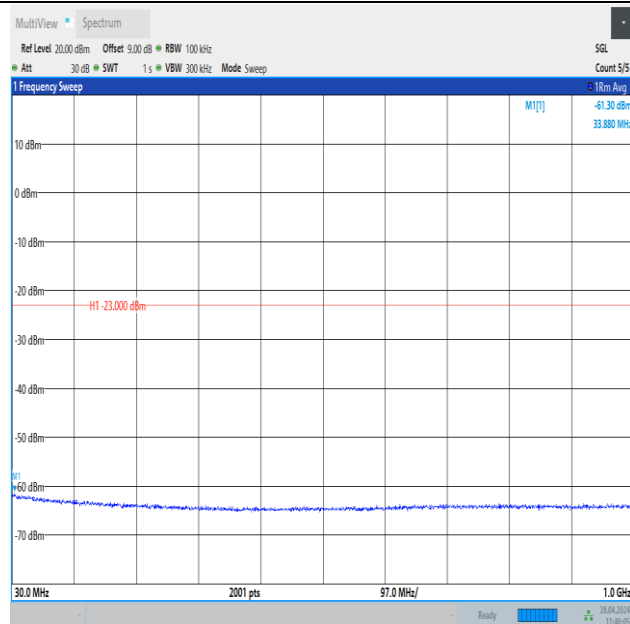
Band25_20MHz_QPSK_26365_1RB#0_30~1000_30~1000
