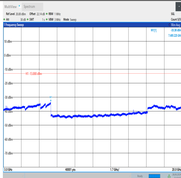
Band25_3MHz_QPSK_26055_1RB#14_3000~20000_3000~20000
