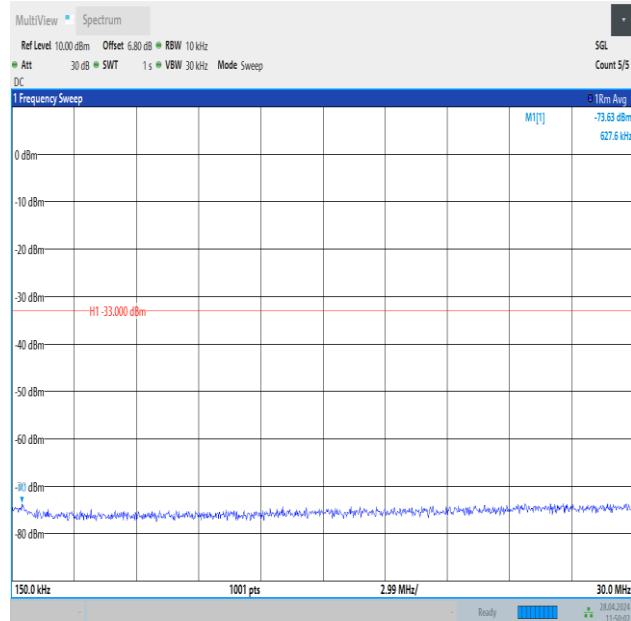
Band25_20MHz_16QAM_26590_1RB#0_0.15~30_0.15~30
