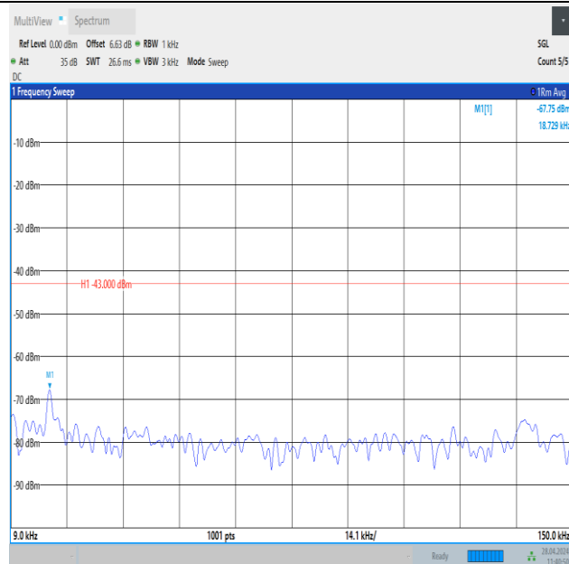
Band25_20MHz_QPSK_26365_100RB#0_0.009~0.15_0.009~0.15
