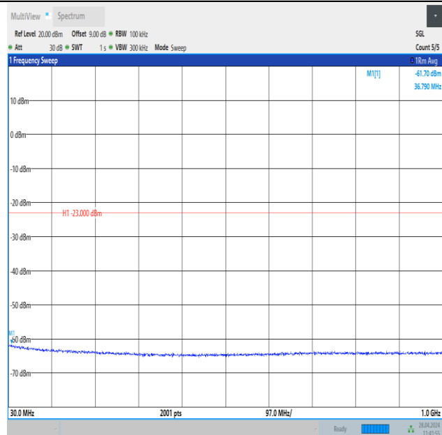
Band25_20MHz_QPSK_26590_100RB#0_30~1000_30~1000
