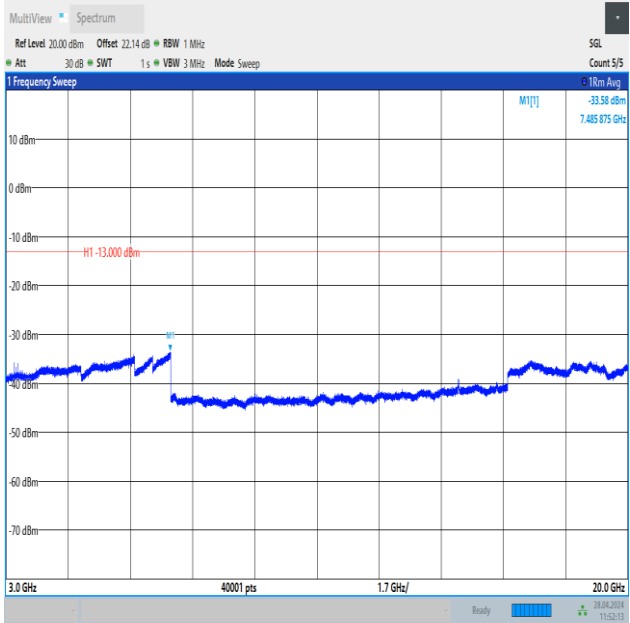
Band25_20MHz_16QAM_26590_1RB#99_3000~20000_3000~20000
