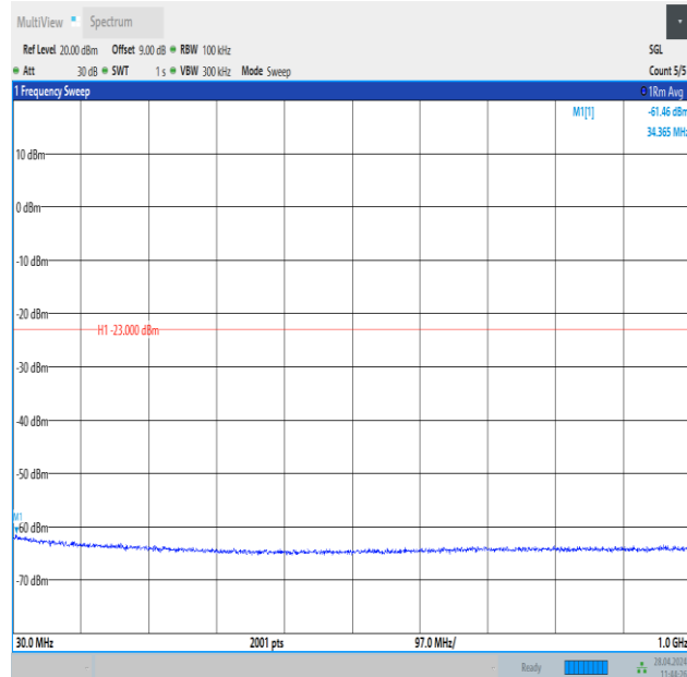
Band25_20MHz_QPSK_26140_1RB#99_30~1000_30~1000
