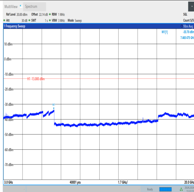
Band25_3MHz_16QAM_26055_15RB#0_3000~20000_3000~20000
