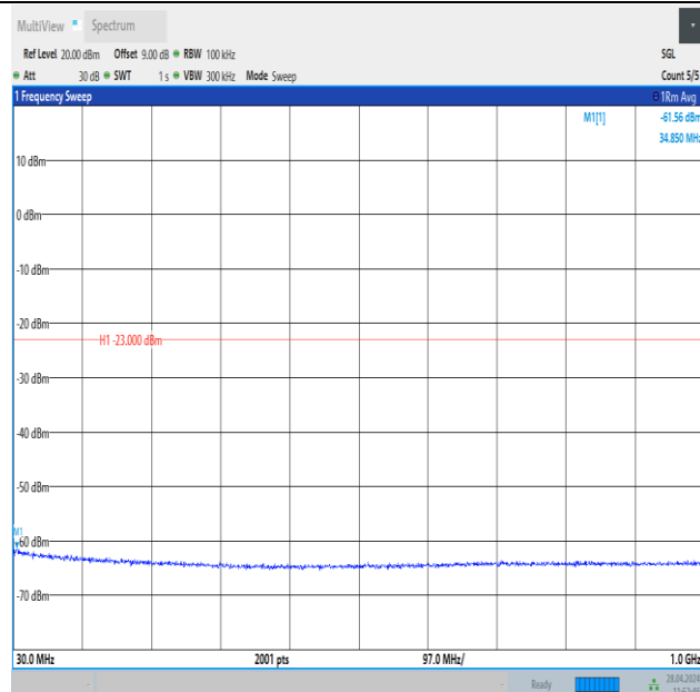
Band25_3MHz_QPSK_26055_1RB#0_30~1000_30~1000
