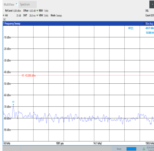
Band25_20MHz_16QAM_26140_1RB#0_0.009~0.15_0.009~0.15
