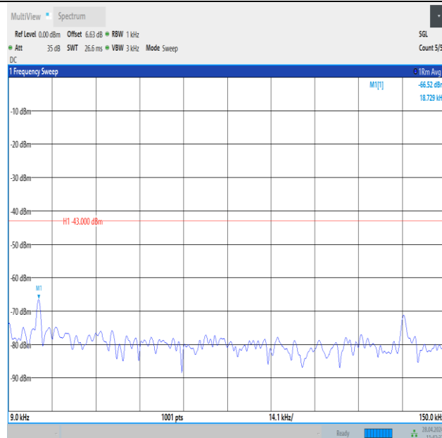
Band25_20MHz_QPSK_26140_1RB#0_0.009~0.15_0.009~0.15
