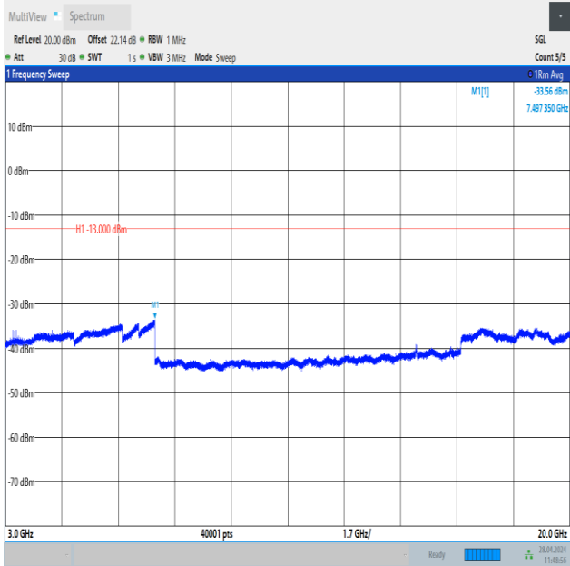
Band25_20MHz_16QAM_26365_1RB#99_3000~20000_3000~20000
