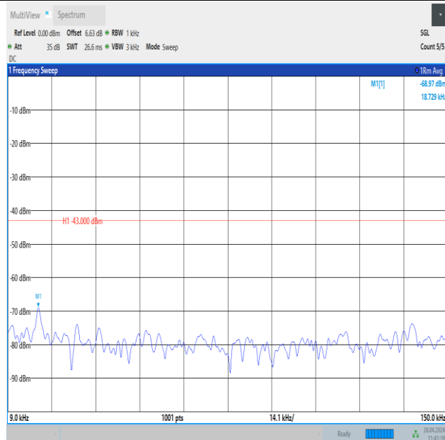
Band25_20MHz_QPSK_26590_100RB#0_0.009~0.15_0.009~0.15
