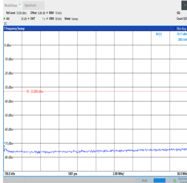
Band25_3MHz_QPSK_26055_1RB#14_0.15~30_0.15~30
