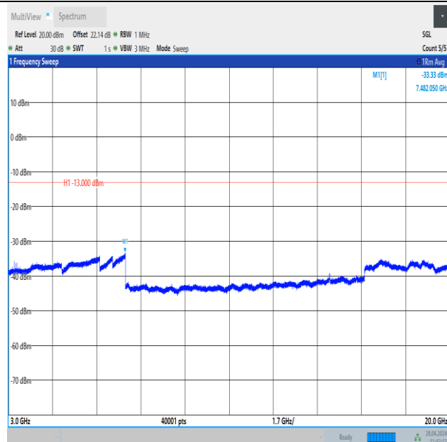
Band25_20MHz_QPSK_26140_1RB#0_3000~20000_3000~20000
