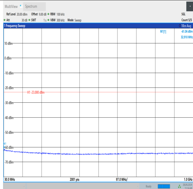
Band25_3MHz_16QAM_26055_15RB#0_30~1000_30~1000
