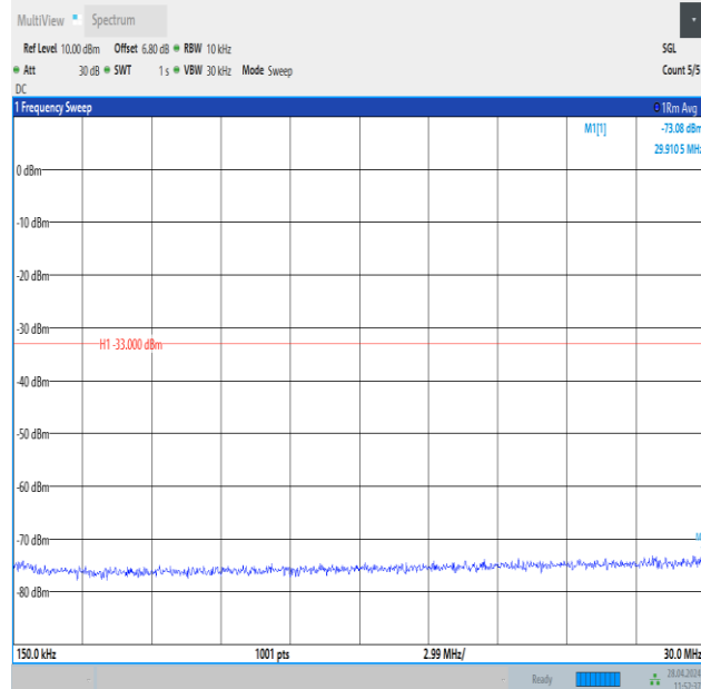
Band25_3MHz_QPSK_26055_1RB#0_0.15~30_0.15~30
