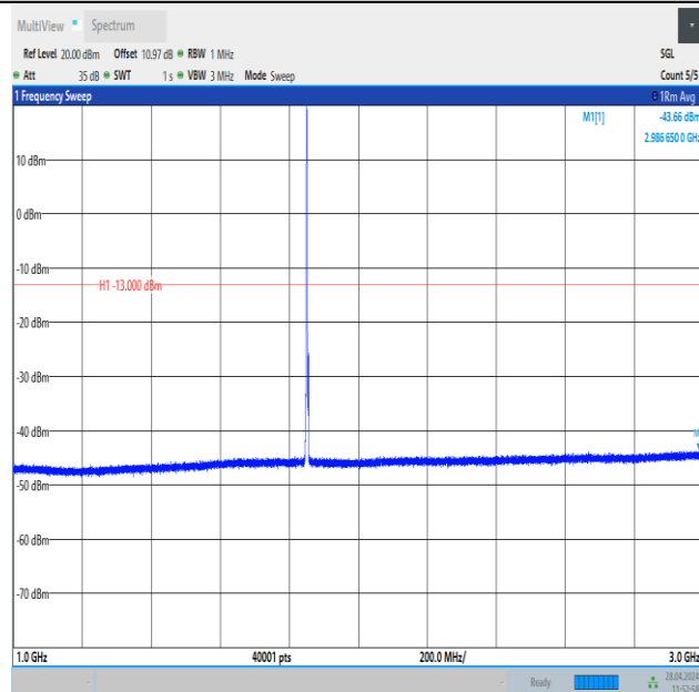
Band25_3MHz_QPSK_26055_1RB#0_1000~3000_1000~3000
