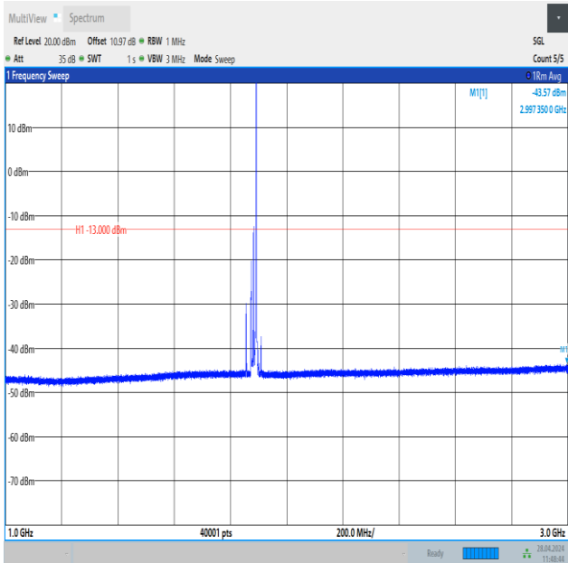
Band25_20MHz_16QAM_26365_1RB#99_1000~3000_1000~3000
