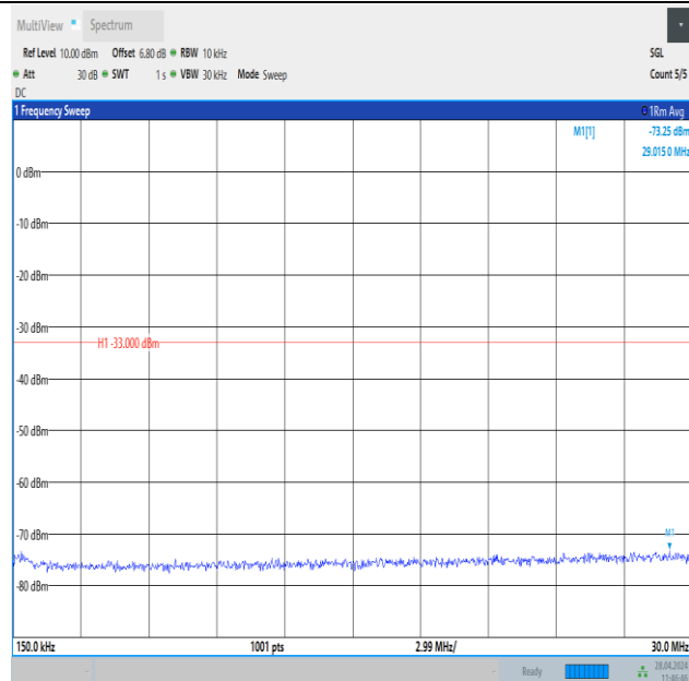
Band25_20MHz_16QAM_26365_1RB#0_0.15~30_0.15~30
