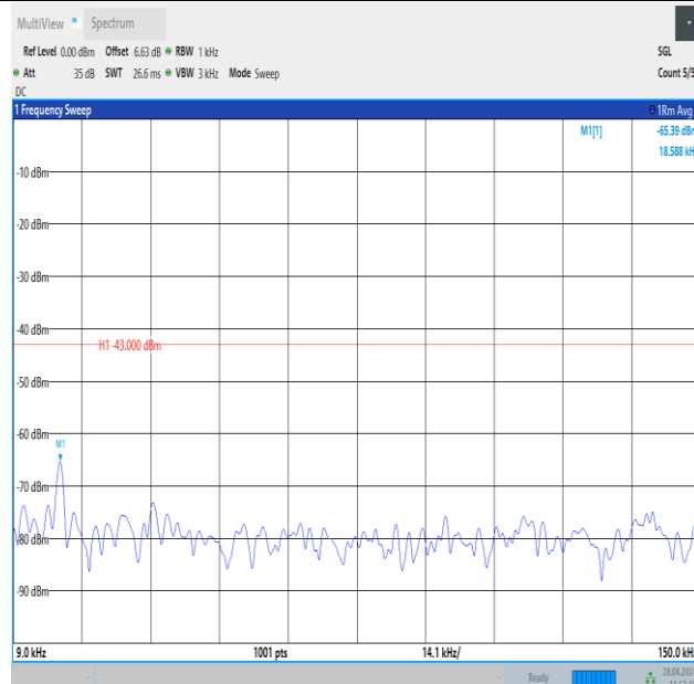
Band25_3MHz_16QAM_26055_1RB#0_0.009~0.15_0.009~0.15
