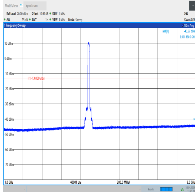
Band25_20MHz_QPSK_26365_100RB#0_1000~3000_1000~3000
