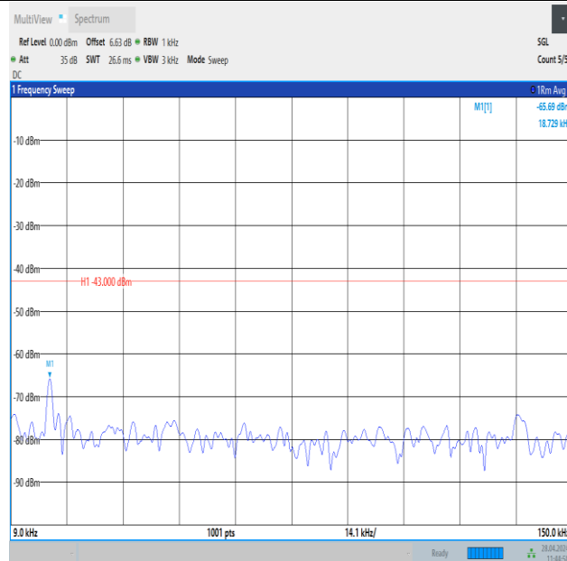
Band25_20MHz_16QAM_26140_1RB#99_0.009~0.15_0.009~0.15
