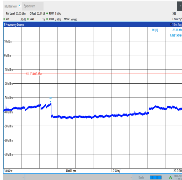
Band25_3MHz_16QAM_26055_1RB#0_3000~20000_3000~20000
