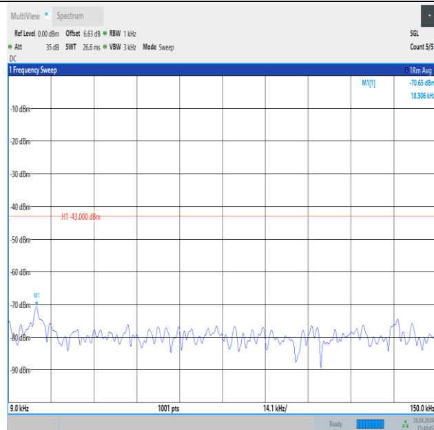
Band25_20MHz_QPSK_26590_1RB#0_0.009~0.15_0.009~0.15
