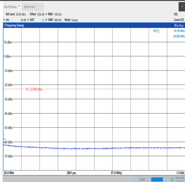
Band25_3MHz_16QAM_26055_1RB#14_30~1000_30~1000
