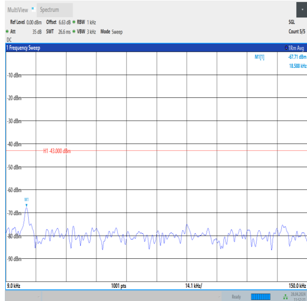
Band25_3MHz_QPSK_26365_1RB#0_0.009~0.15_0.009~0.15
