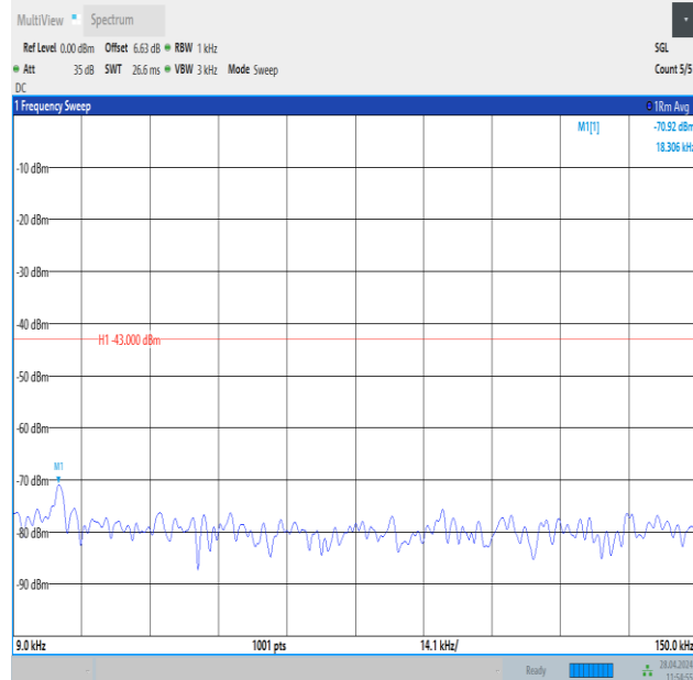
Band25_3MHz_16QAM_26055_1RB#14_0.009~0.15_0.009~0.15
