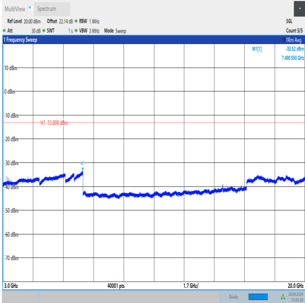
Band25_20MHz_QPSK_26590_100RB#0_3000~20000_3000~20000
