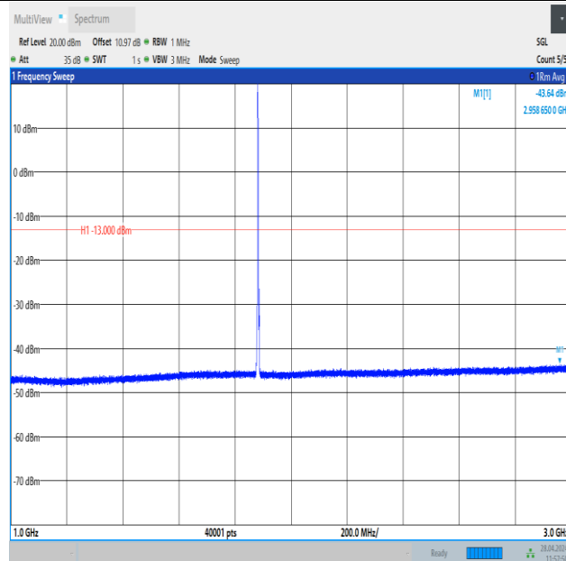
Band25_3MHz_QPSK_26365_1RB#0_1000~3000_1000~3000
