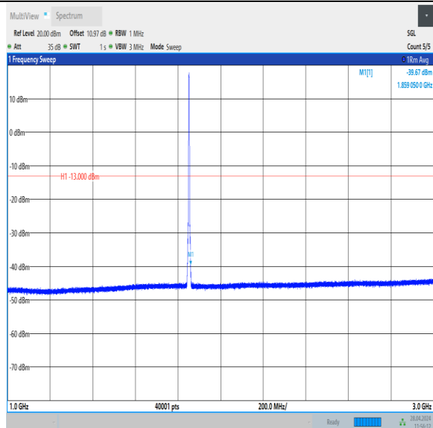
Band25_3MHz_QPSK_26055_15RB#0_1000~3000_1000~3000
