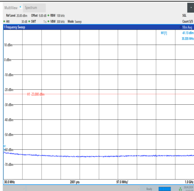
Band25_3MHz_QPSK_26055_15RB#0_30~1000_30~1000
