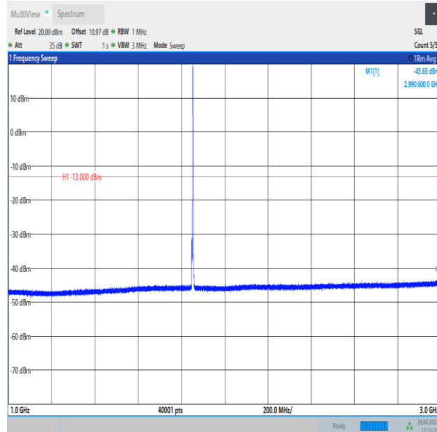
Band25_3MHz_16QAM_26055_1RB#14_1000~3000_1000~3000
