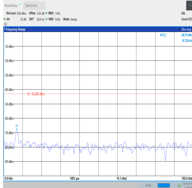
Band25_20MHz_16QAM_26590_1RB#0_0.009~0.15_0.009~0.15
