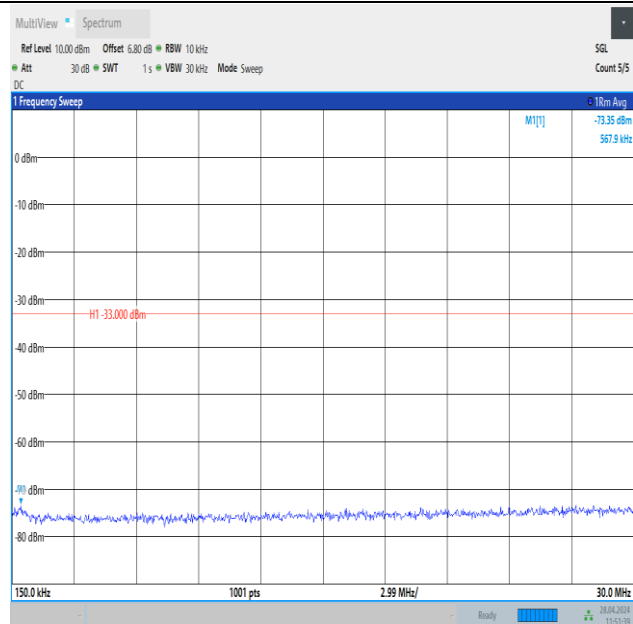
Band25_20MHz_16QAM_26590_1RB#99_0.15~30_0.15~30
