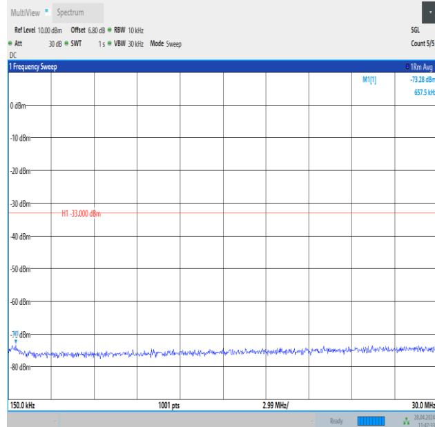
Band25_20MHz_QPSK_26365_1RB#99_0.15~30_0.15~30
