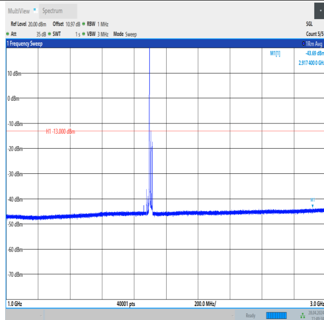
Band25_20MHz_QPSK_26590_1RB#0_1000~3000_1000~3000
