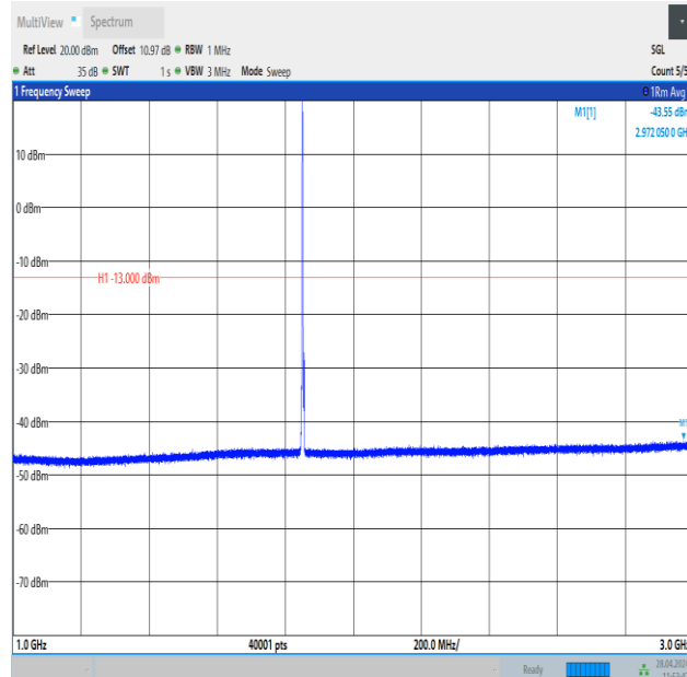
Band25_3MHz_16QAM_26055_1RB#0_1000~3000_1000~3000
