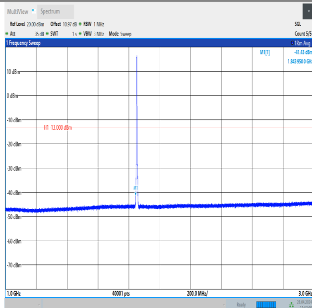
Band25_3MHz_16QAM_26055_15RB#0_1000~3000_1000~3000
