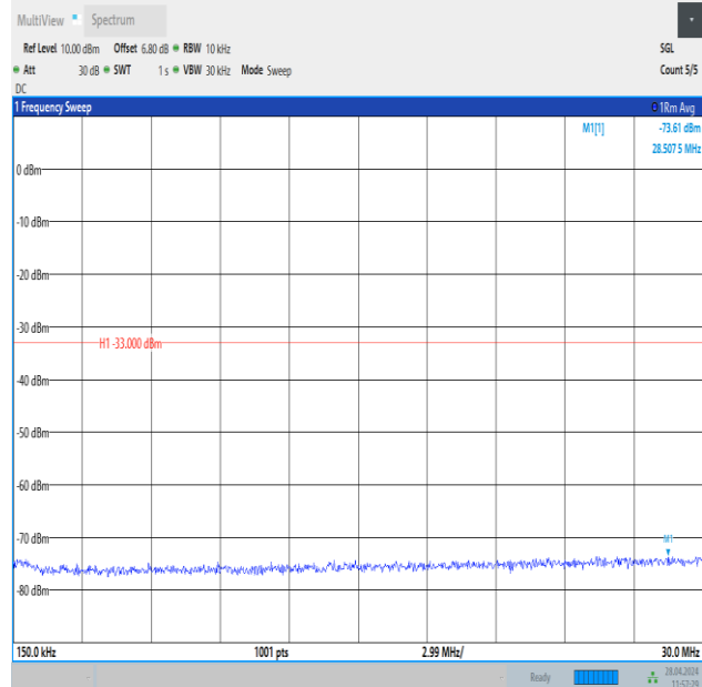
Band25_3MHz_QPSK_26365_1RB#0_0.15~30_0.15~30
