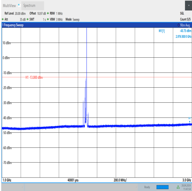
Band25_20MHz_QPSK_26365_1RB#99_1000~3000_1000~3000
