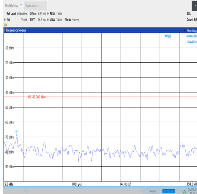
Band25_3MHz_16QAM_26055_15RB#0_0.009~0.15_0.009~0.15
