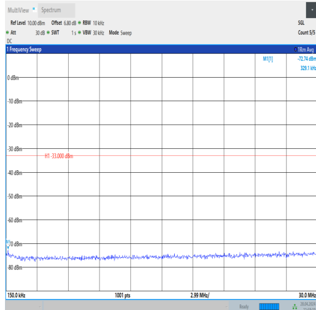
Band25_3MHz_16QAM_26365_1RB#0_0.15~30_0.15~30
