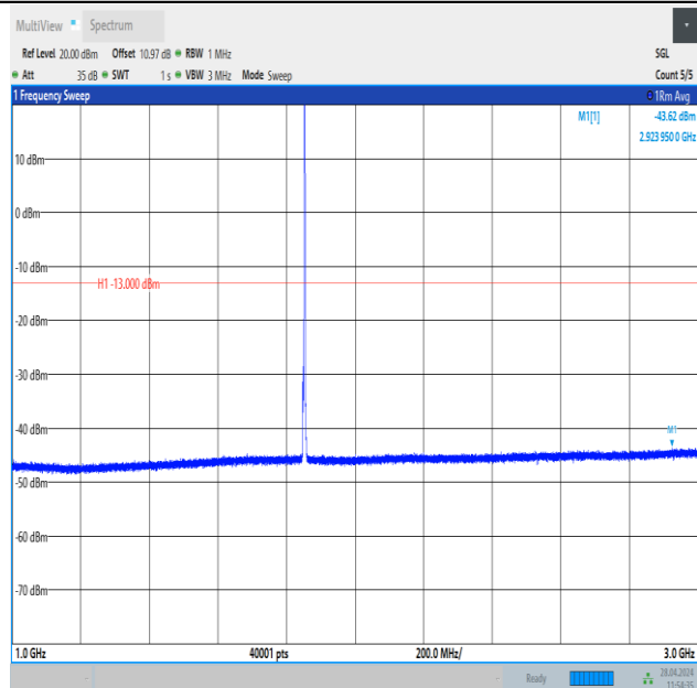
Band25_3MHz_QPSK_26055_1RB#14_1000~3000_1000~3000
