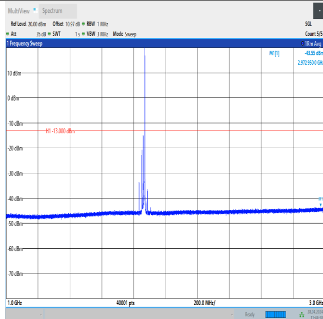
Band25_20MHz_QPSK_26140_1RB#99_1000~3000_1000~3000
