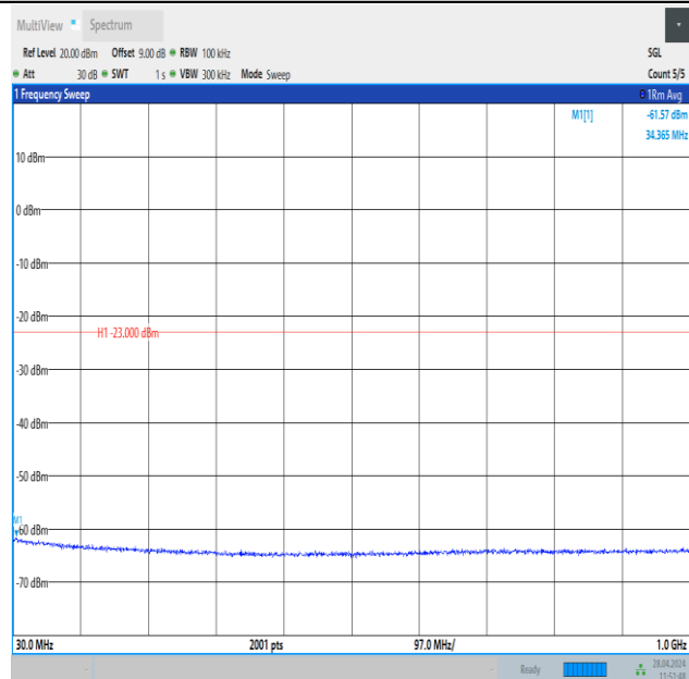
Band25_20MHz_16QAM_26590_1RB#99_30~1000_30~1000
