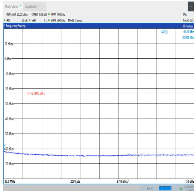
Band25_20MHz_16QAM_26590_1RB#0_30~1000_30~1000
