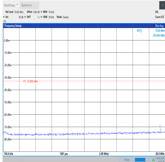
Band25_3MHz_16QAM_26055_15RB#0_0.15~30_0.15~30
