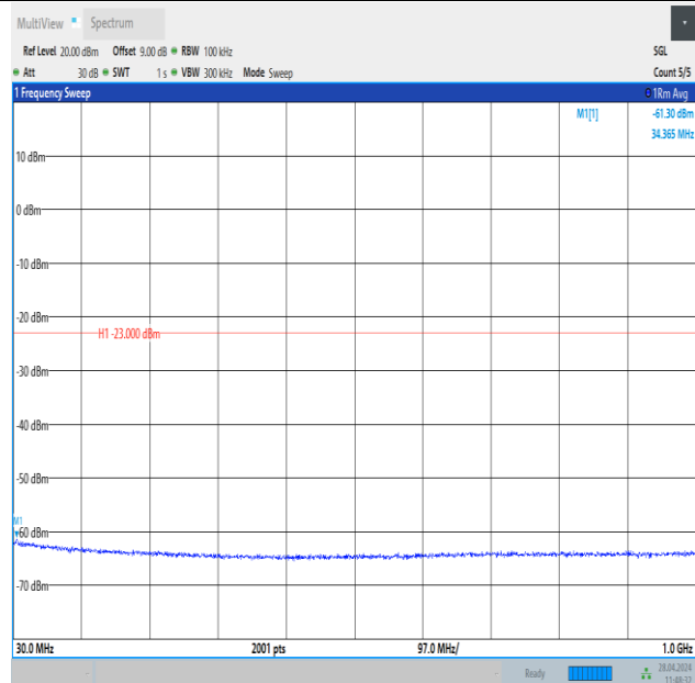
Band25_20MHz_16QAM_26365_1RB#99_30~1000_30~1000
