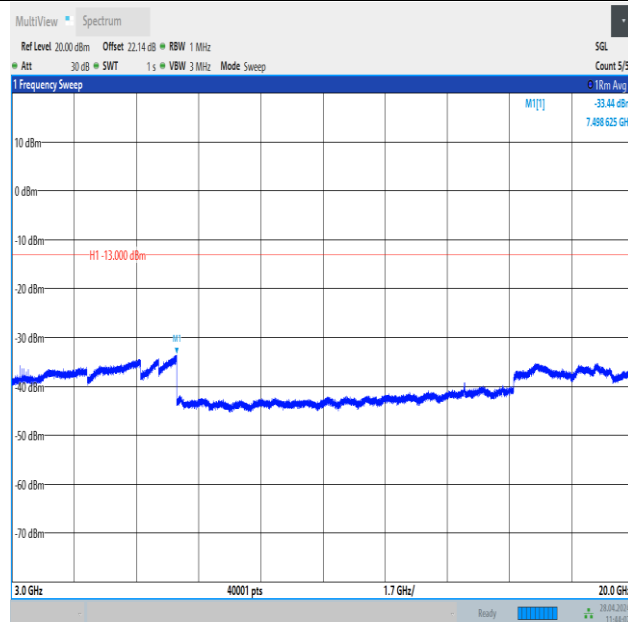
Band25_20MHz_16QAM_26140_1RB#0_3000~20000_3000~20000
