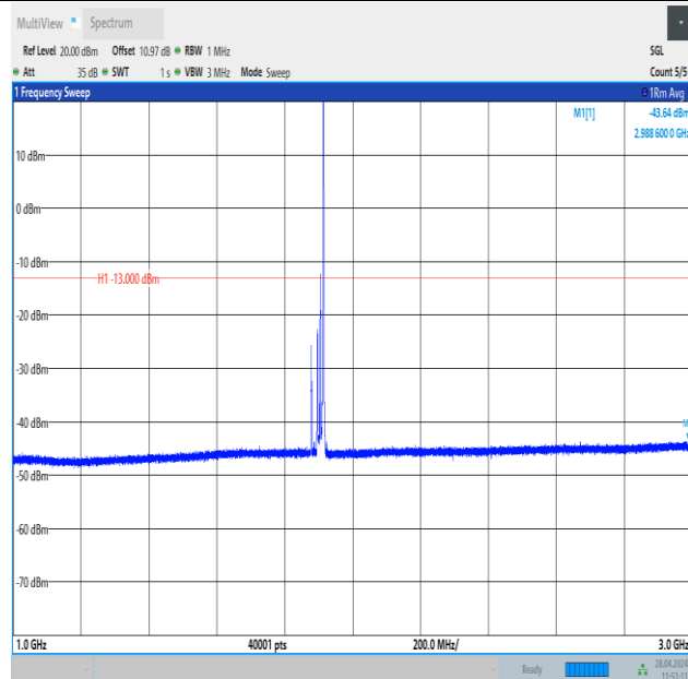
Band25_20MHz_QPSK_26590_1RB#99_1000~3000_1000~3000
