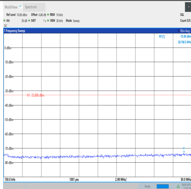
Band25_20MHz_16QAM_26140_1RB#0_0.15~30_0.15~30
