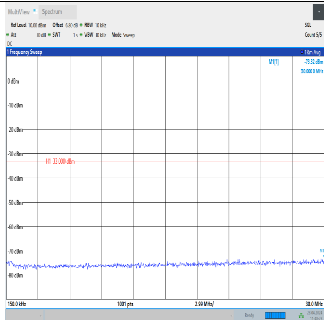
Band25_20MHz_16QAM_26365_1RB#99_0.15~30_0.15~30
