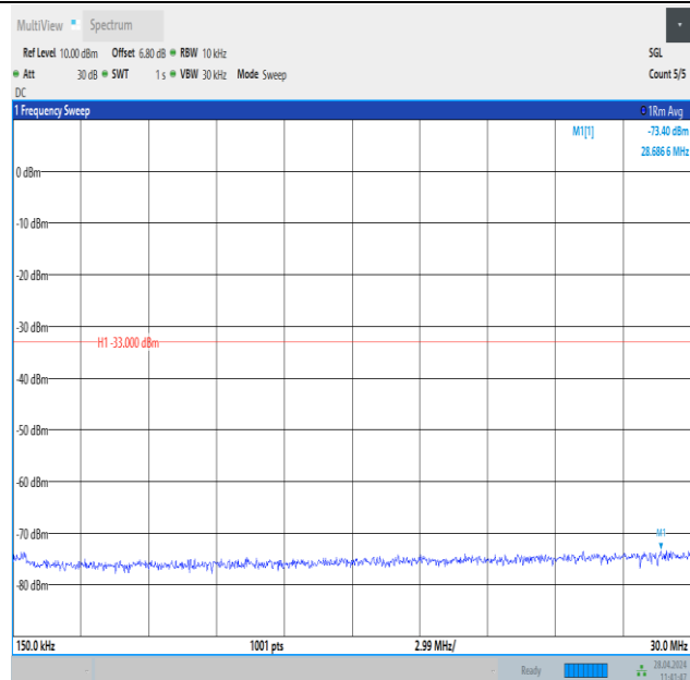
Band25_20MHz_QPSK_26590_100RB#0_0.15~30_0.15~30
