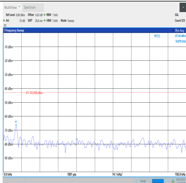
Band25_3MHz_QPSK_26365_1RB#14_0.009~0.15_0.009~0.15
