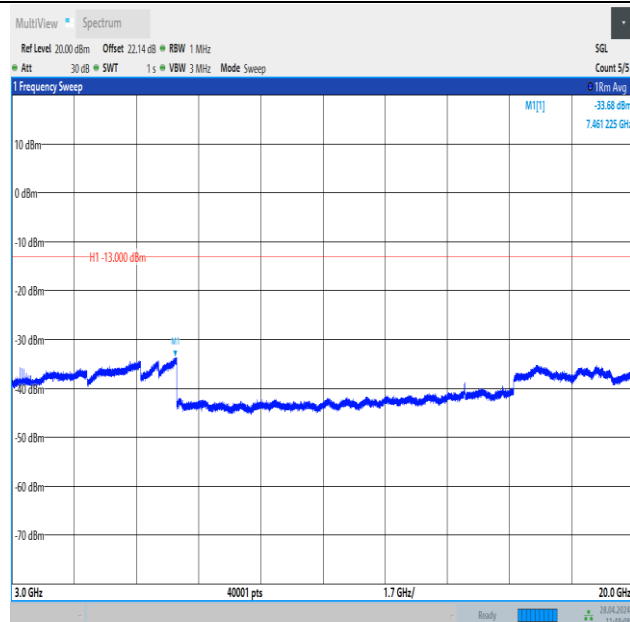
Band25_20MHz_QPSK_26365_1RB#99_3000~20000_3000~20000
