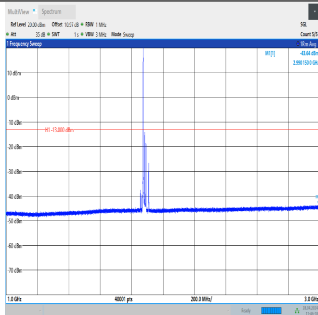
Band25_20MHz_QPSK_26365_1RB#0_1000~3000_1000~3000
