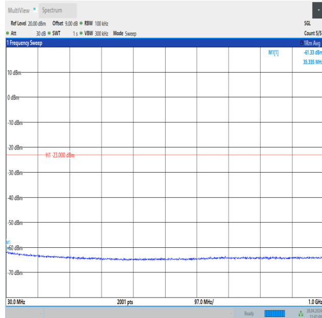
Band25_20MHz_QPSK_26365_100RB#0_30~1000_30~1000
