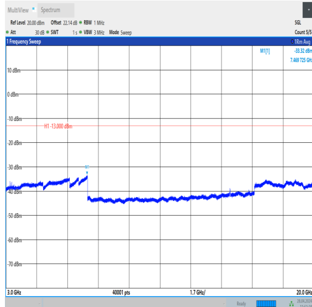
Band25_20MHz_QPSK_26590_1RB#99_3000~20000_3000~20000
