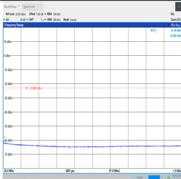
Band25_3MHz_16QAM_26055_1RB#0_30~1000_30~1000
