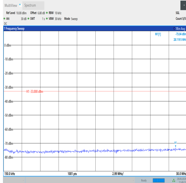
Band25_20MHz_QPSK_26590_1RB#0_0.15~30_0.15~30
