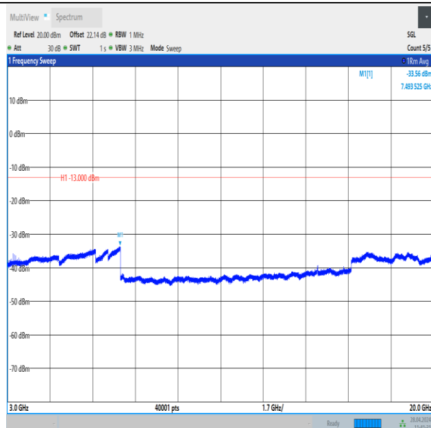
Band25_20MHz_QPSK_26365_100RB#0_3000~20000_3000~20000
