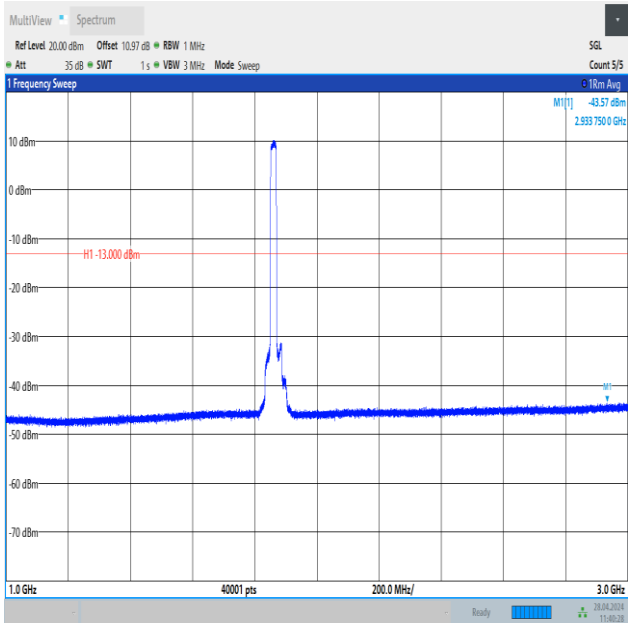
Band25_20MHz_QPSK_26140_100RB#0_1000~3000_1000~3000
