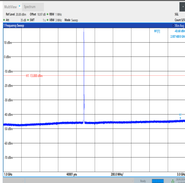
Band25_3MHz_16QAM_26365_1RB#0_1000~3000_1000~3000
