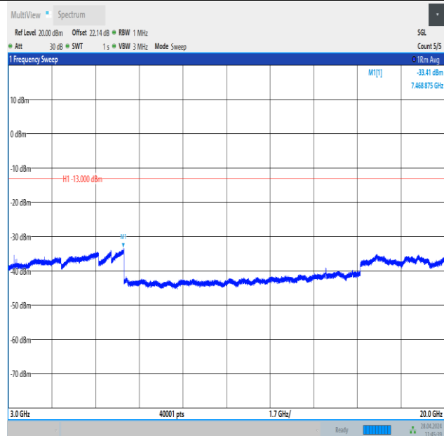
Band25_20MHz_16QAM_26140_1RB#99_3000~20000_3000~20000
