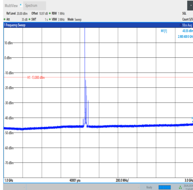
Band25_20MHz_QPSK_26140_1RB#0_1000~3000_1000~3000
