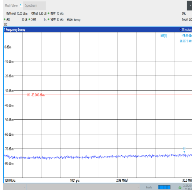
Band25_20MHz_QPSK_26140_1RB#0_0.15~30_0.15~30
