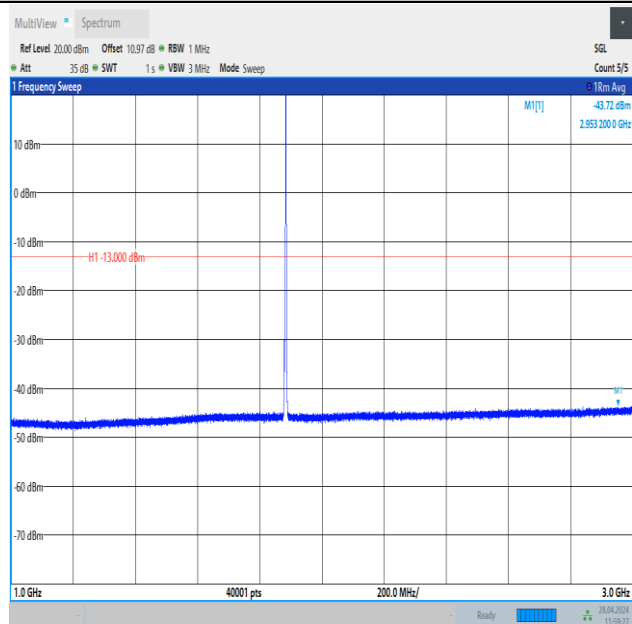
Band25_3MHz_QPSK_26365_1RB#14_1000~3000_1000~3000
