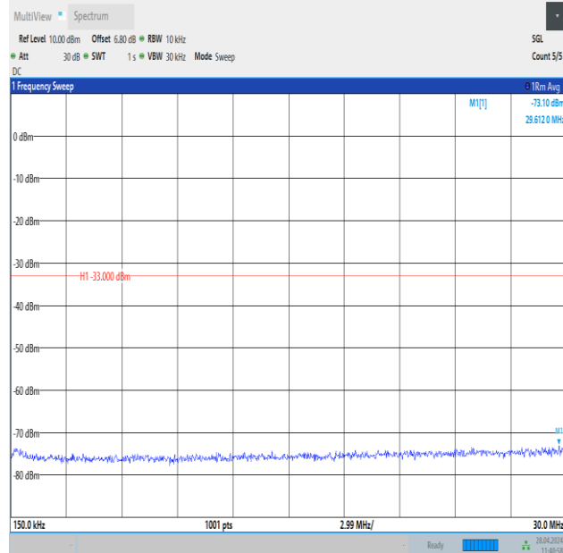
Band25_20MHz_QPSK_26365_100RB#0_0.15~30_0.15~30
