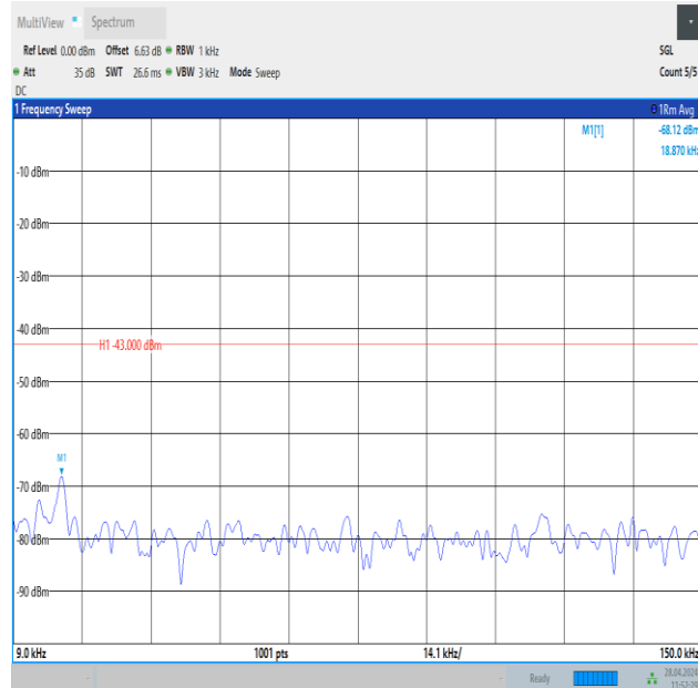
Band25_3MHz_QPSK_26055_1RB#0_0.009~0.15_0.009~0.15
