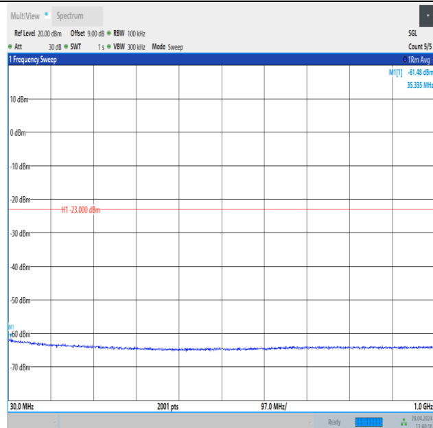
Band25_20MHz_QPSK_26140_100RB#0_30~1000_30~1000
