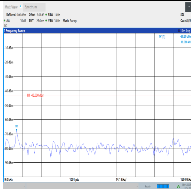
Band25_3MHz_QPSK_26055_1RB#14_0.009~0.15_0.009~0.15
