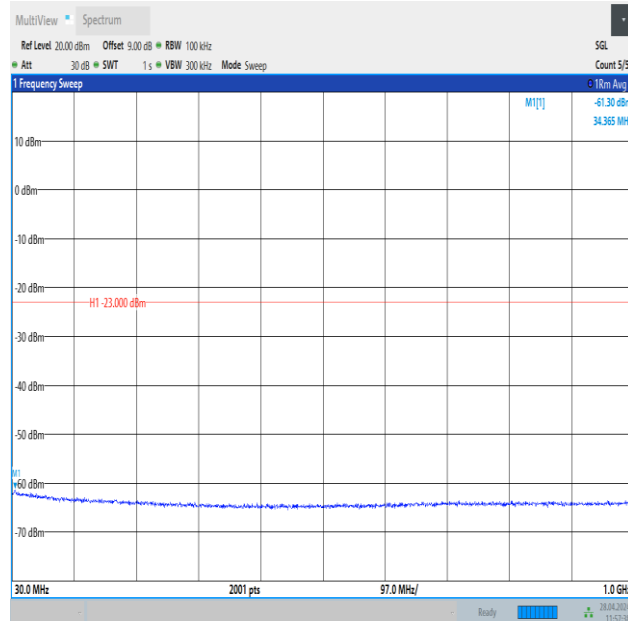
Band25_3MHz_QPSK_26365_1RB#0_30~1000_30~1000
