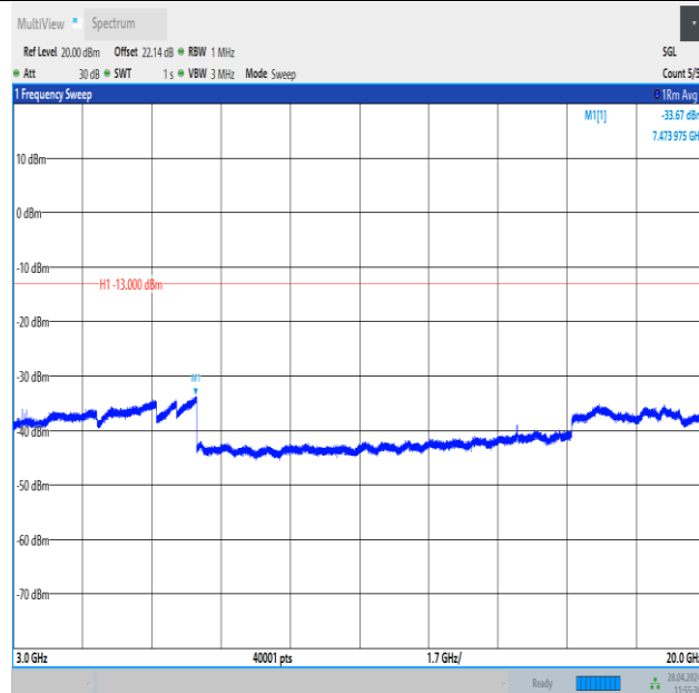
Band25_3MHz_16QAM_26055_1RB#14_3000~20000_3000~20000
