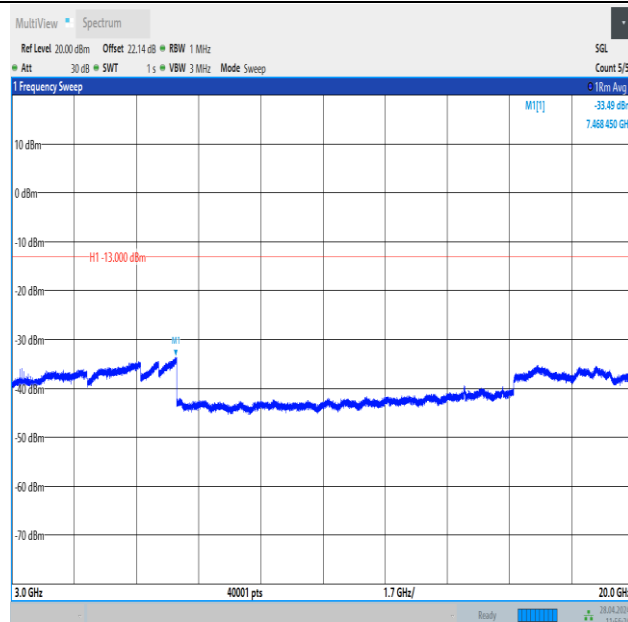
Band25_3MHz_QPSK_26055_15RB#0_3000~20000_3000~20000
