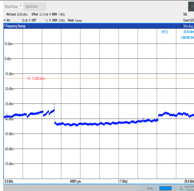
Band25_20MHz_16QAM_26365_1RB#0_3000~20000_3000~20000
