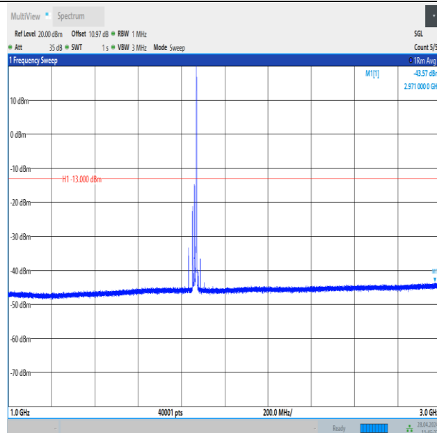
Band25_20MHz_16QAM_26140_1RB#99_1000~3000_1000~3000
