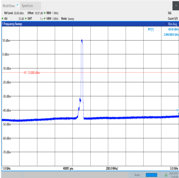
Band25_20MHz_QPSK_26590_100RB#0_1000~3000_1000~3000
