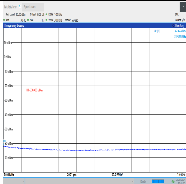
Band25_20MHz_16QAM_26140_1RB#99_30~1000_30~1000
