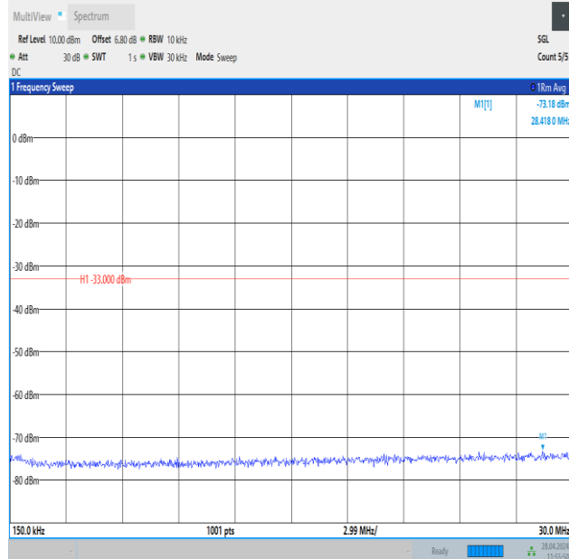
Band25_3MHz_QPSK_26055_15RB#0_0.15~30_0.15~30
