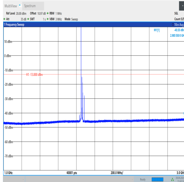
Band25_20MHz_16QAM_26140_1RB#0_1000~3000_1000~3000
