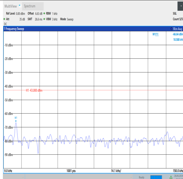
Band25_20MHz_16QAM_26590_1RB#99_0.009~0.15_0.009~0.15
