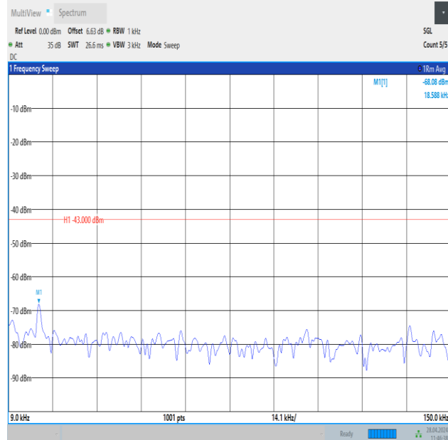
Band25_20MHz_16QAM_26365_1RB#0_0.009~0.15_0.009~0.15
