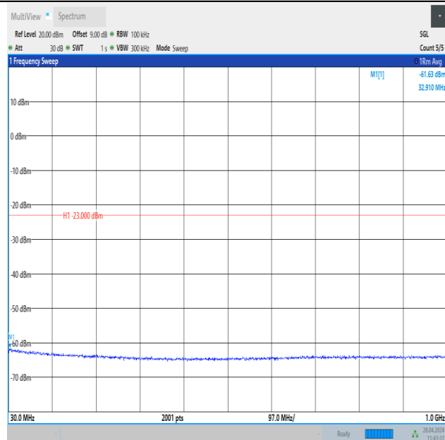
Band25_20MHz_16QAM_26140_1RB#0_30~1000_30~1000
