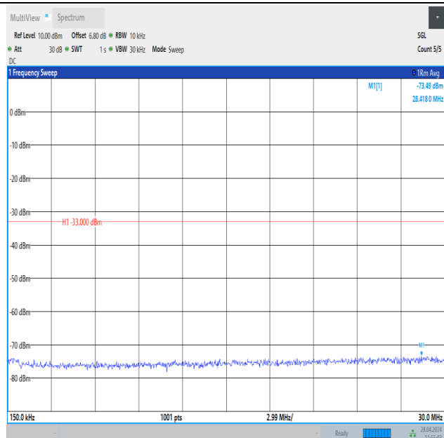
Band25_3MHz_16QAM_26055_1RB#14_0.15~30_0.15~30
