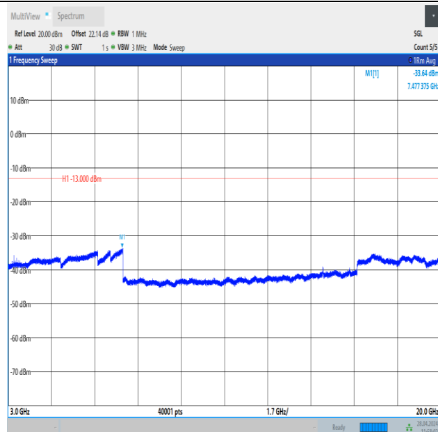
Band25_3MHz_QPSK_26365_1RB#0_3000~20000_3000~20000
