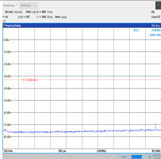
Band25_3MHz_QPSK_26365_1RB#14_0.15~30_0.15~30
