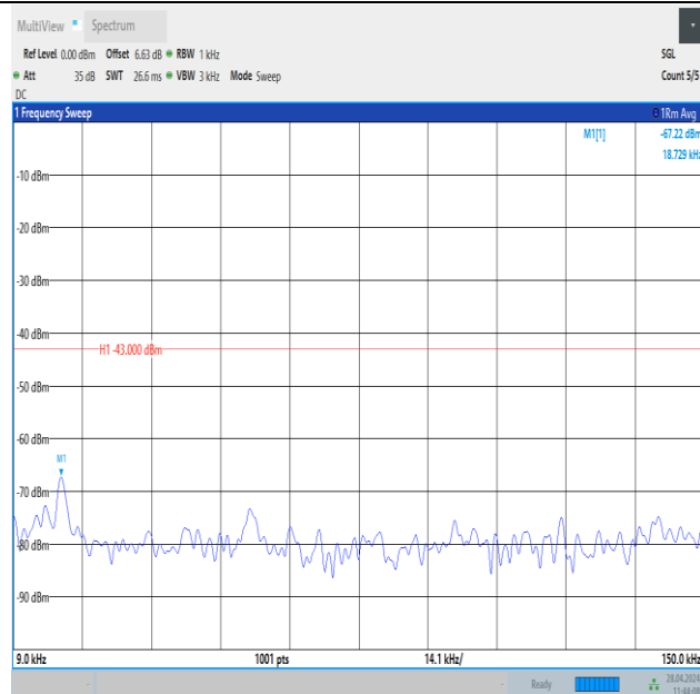
Band25_20MHz_QPSK_26140_1RB#99_0.009~0.15_0.009~0.15
