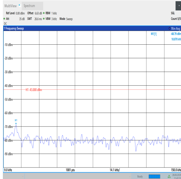
Band25_20MHz_QPSK_26365_1RB#99_0.009~0.15_0.009~0.15
