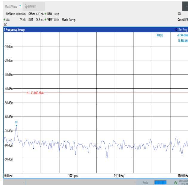
Band25_3MHz_16QAM_26365_1RB#0_0.009~0.15_0.009~0.15
