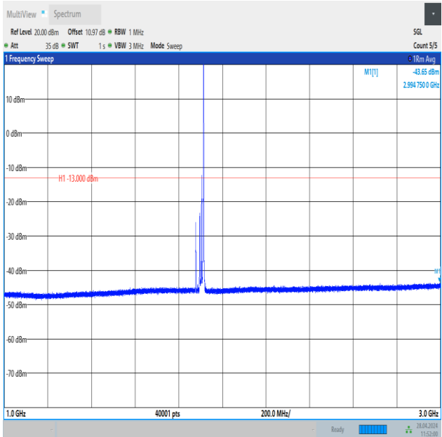
Band25_20MHz_16QAM_26590_1RB#99_1000~3000_1000~3000
