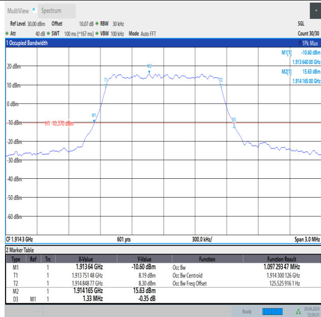
Band25-1.4MHz-QPSK-26683-6RB#0-PASS
