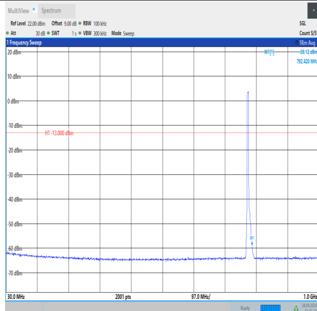
Band13_5MHz_16QAM_23205_25RB#0_30~1000_30~1000
