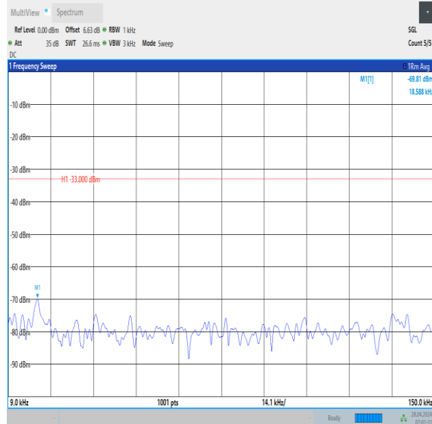
Band13_5MHz_16QAM_23205_1RB#0_0.009~0.15_0.009~0.15
