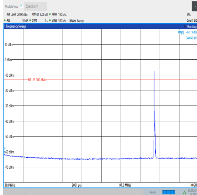
Band13_5MHz_QPSK_23205_1RB#0_30~1000_30~1000
