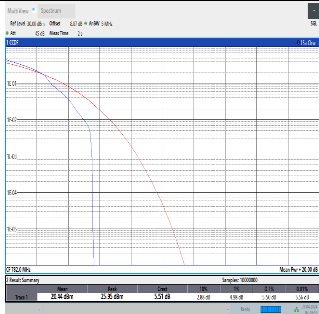
Band13-5MHz-16QAM-23230-1RB#0-PASS
