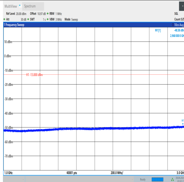
Band13_5MHz_QPSK_23205_1RB#0_1000~3000_1000~3000
