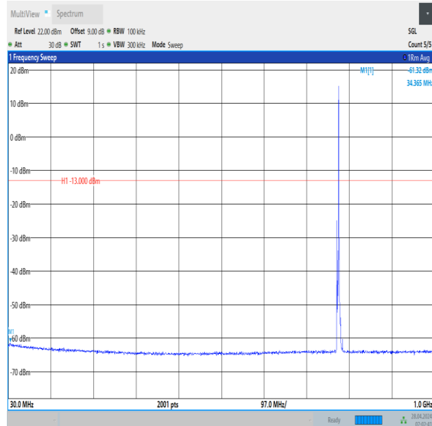
Band13_5MHz_QPSK_23205_1RB#24_30~1000_30~1000
