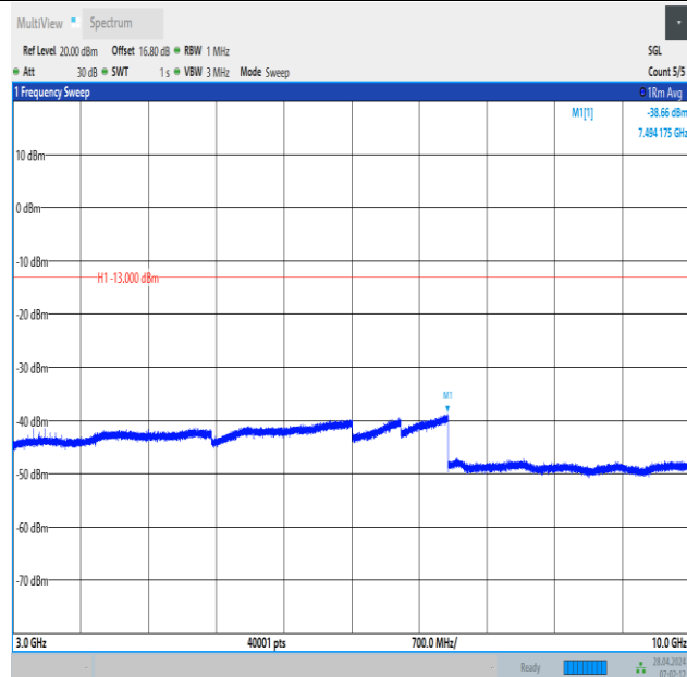
Band13_5MHz_16QAM_23205_1RB#0_3000~10000_3000~10000
