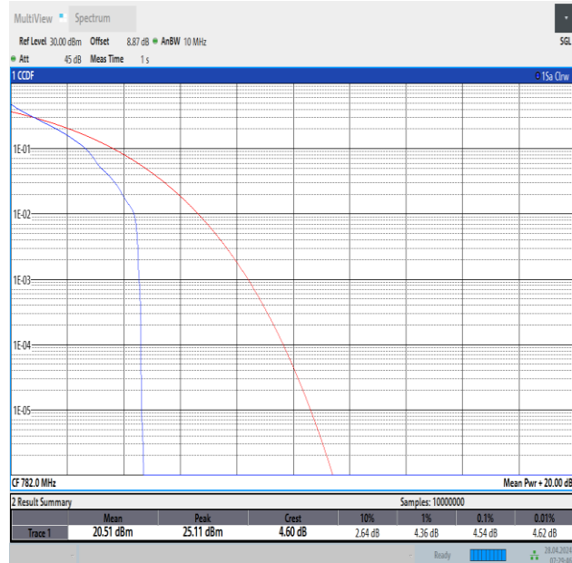
Band13-10MHz-QPSK-23230-1RB#0-PASS
