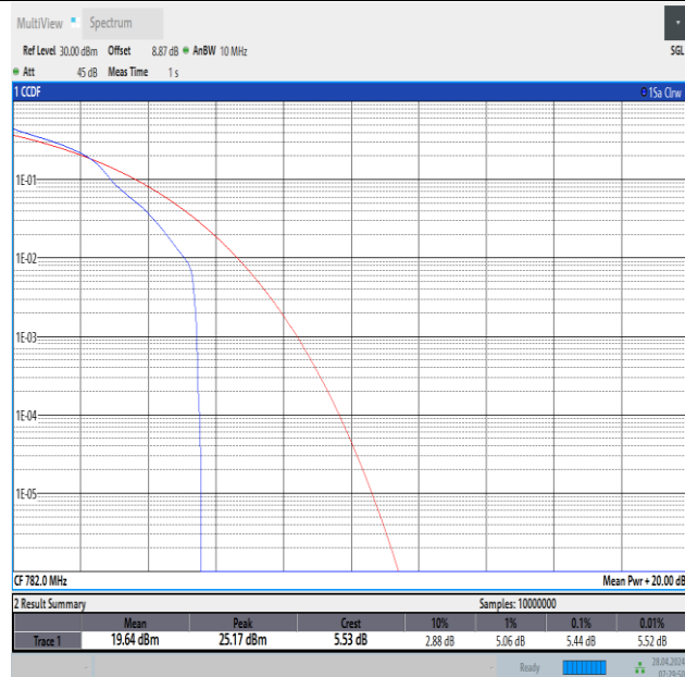
Band13-10MHz-16QAM-23230-1RB#0-PASS
