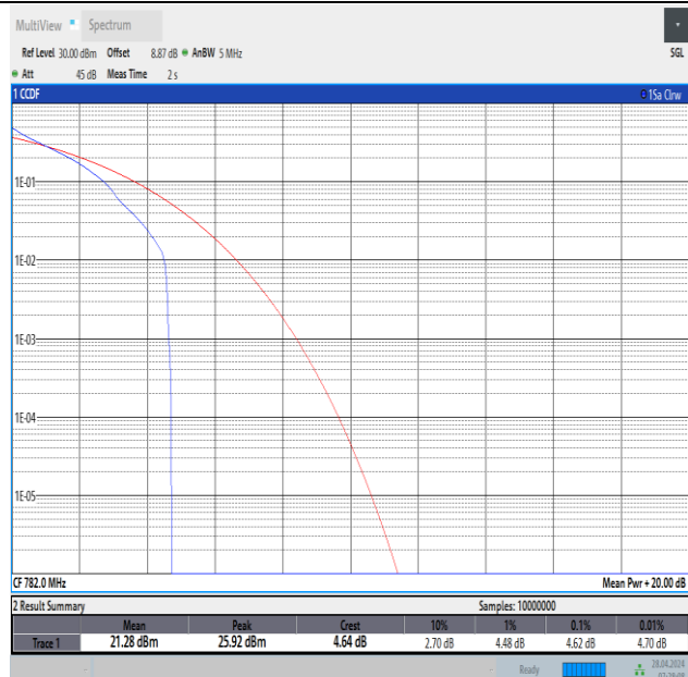
Band13-5MHz-QPSK-23230-1RB#0-PASS
