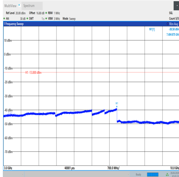
Band13_5MHz_QPSK_23205_1RB#0_3000~10000_3000~10000
