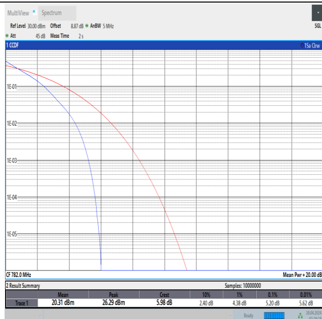
Band13-5MHz-QPSK-23230-25RB#0-PASS
