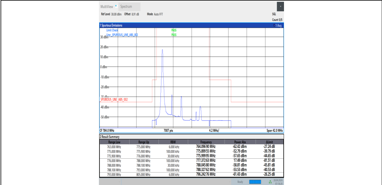
Band13_5MHz_16QAM_23205_1RB#0
