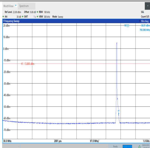
Band13_5MHz_QPSK_23205_25RB#0_30~1000_30~1000
