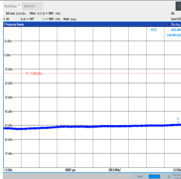
Band26_1.4MHz_QPSK_26740_6RB#0_1000~3000_1000~3000
