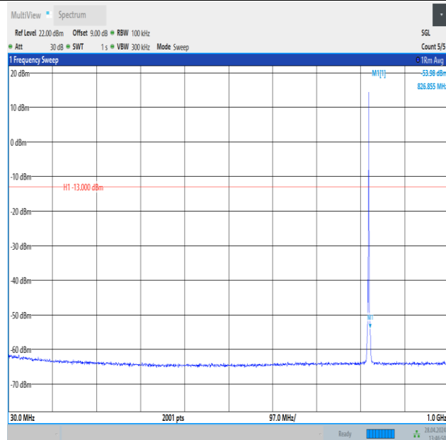
Band26_1.4MHz_16QAM_26783_1RB#5_30~1000_30~1000
