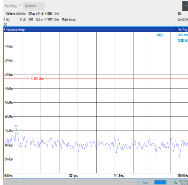
Band26_1.4MHz_QPSK_26697_1RB#5_0.009~0.15_0.009~0.15
