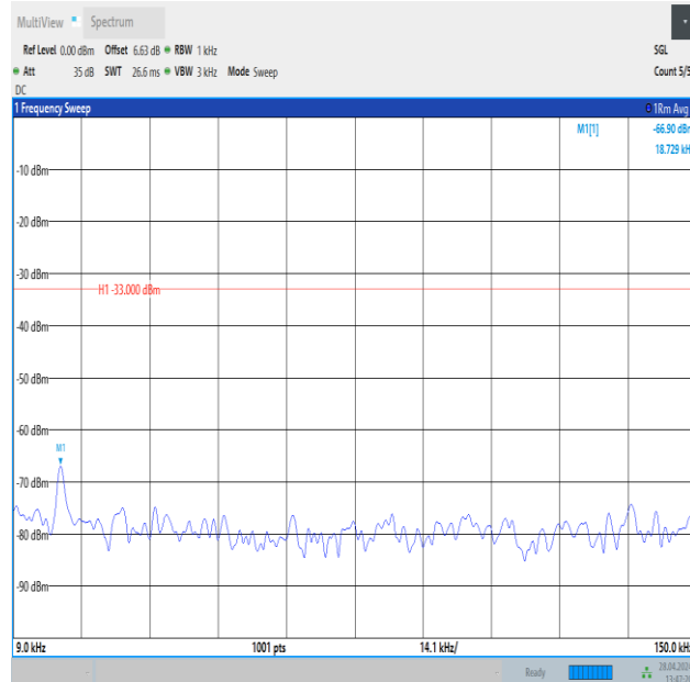
Band26_1.4MHz_QPSK_26783_6RB#0_0.009~0.15_0.009~0.15
