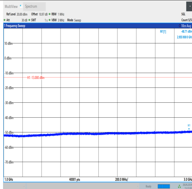
Band26_1.4MHz_QPSK_26697_6RB#0_1000~3000_1000~3000
