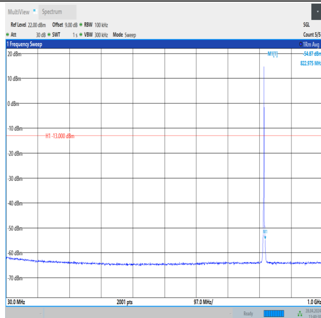
Band26_1.4MHz_QPSK_26740_1RB#5_30~1000_30~1000
