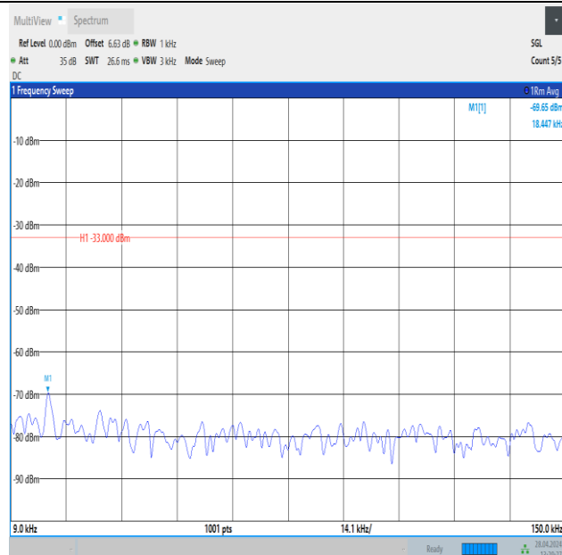
Band26_3MHz_QPSK_26775_1RB#14_0.009~0.15_0.009~0.15
