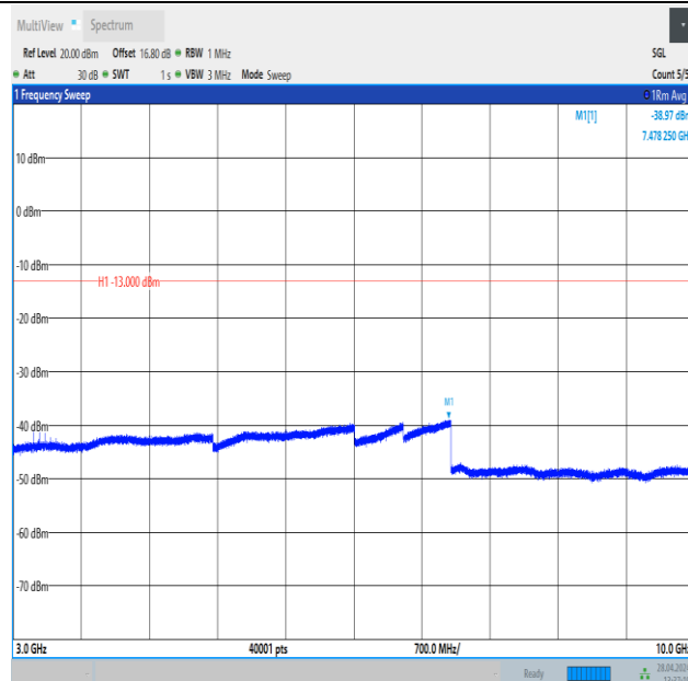
Band26_1.4MHz_QPSK_26697_6RB#0_3000~10000_3000~10000
