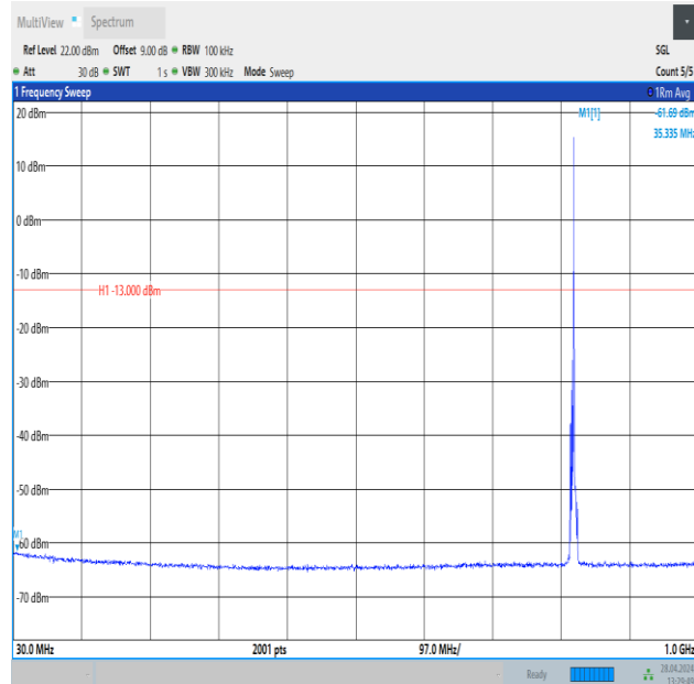
Band26_3MHz_QPSK_26775_1RB#14_30~1000_30~1000
