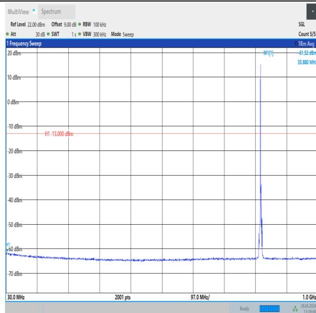
Band26_3MHz_QPSK_26775_1RB#0_30~1000_30~1000
