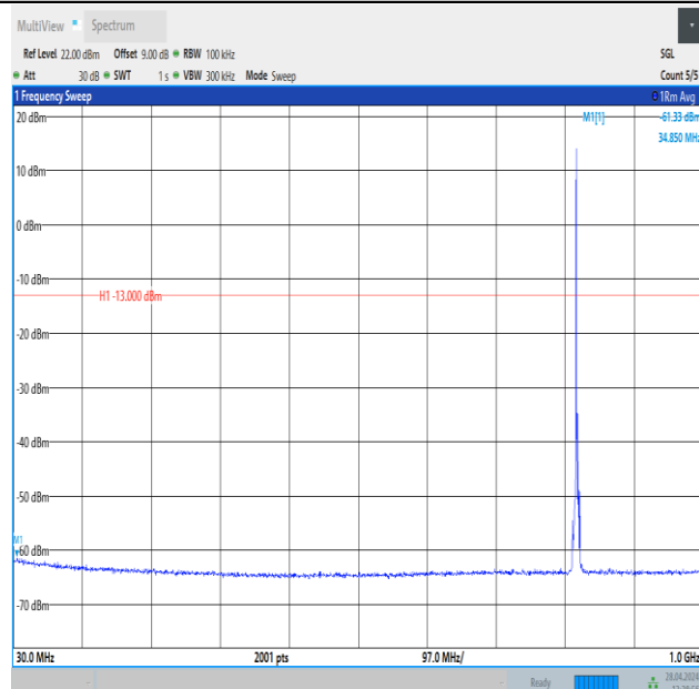
Band26_3MHz_16QAM_26775_1RB#0_30~1000_30~1000
