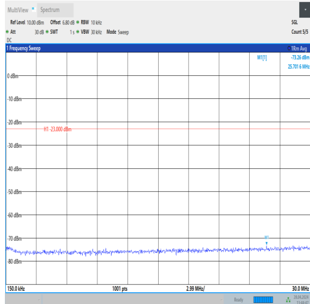
Band26_1.4MHz_16QAM_26783_1RB#0_0.15~30_0.15~30
