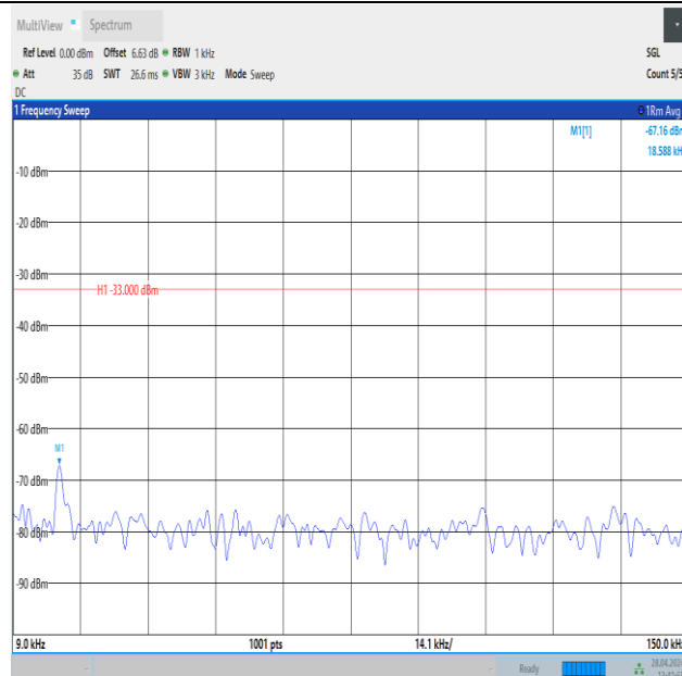
Band26_1.4MHz_QPSK_26740_6RB#0_0.009~0.15_0.009~0.15
