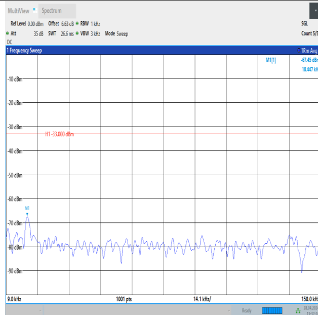
Band26_1.4MHz_16QAM_26697_6RB#0_0.009~0.15_0.009~0.15
