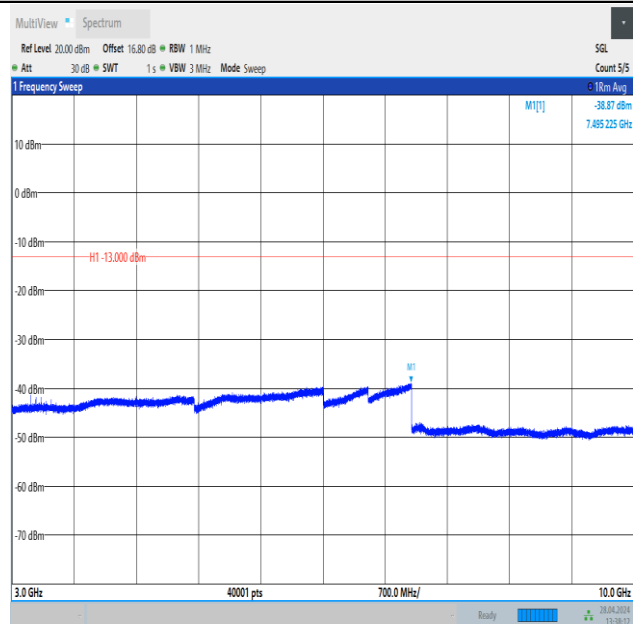
Band26_1.4MHz_16QAM_26697_6RB#0_3000~10000_3000~10000
