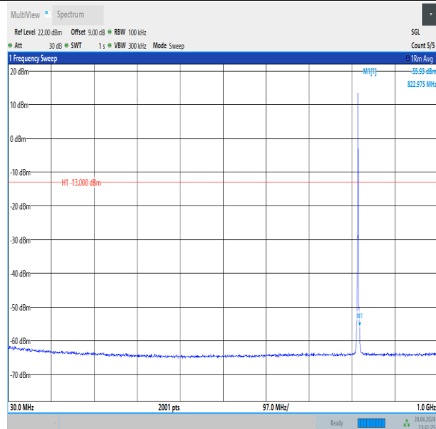
Band26_1.4MHz_16QAM_26740_1RB#5_30~1000_30~1000
