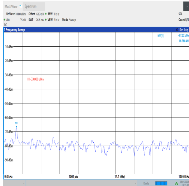
Band26_1.4MHz_16QAM_26697_1RB#5_0.009~0.15_0.009~0.15
