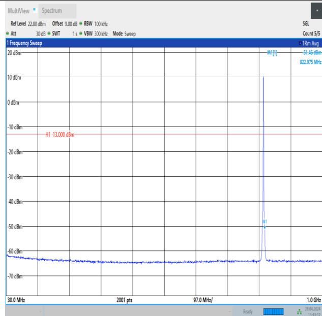
Band26_1.4MHz_16QAM_26740_6RB#0_30~1000_30~1000
