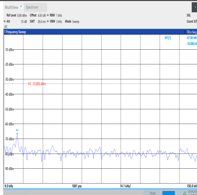
Band26_1.4MHz_16QAM_26740_1RB#5_0.009~0.15_0.009~0.15
