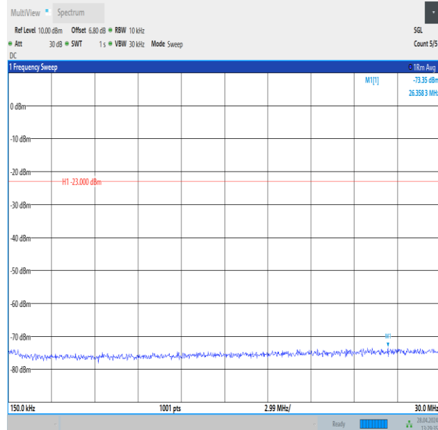
Band26_3MHz_QPSK_26775_1RB#14_0.15~30_0.15~30
