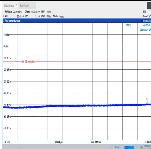
Band26_1.4MHz_16QAM_26740_1RB#0_1000~3000_1000~3000
