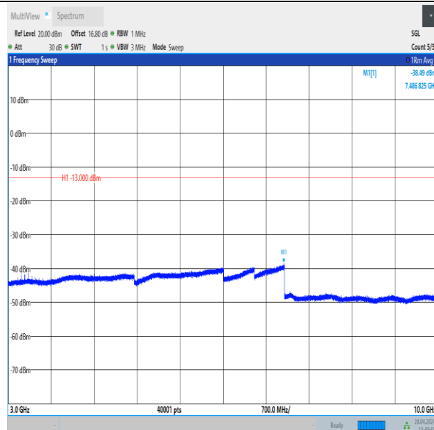
Band26_1.4MHz_QPSK_26740_1RB#5_3000~10000_3000~10000
