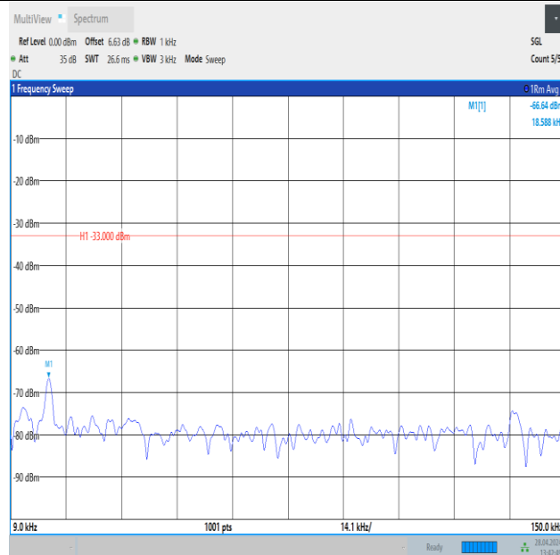
Band26_1.4MHz_16QAM_26740_6RB#0_0.009~0.15_0.009~0.15
