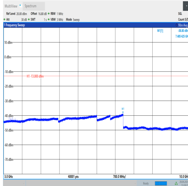
Band26_3MHz_QPSK_26775_1RB#14_3000~10000_3000~10000
