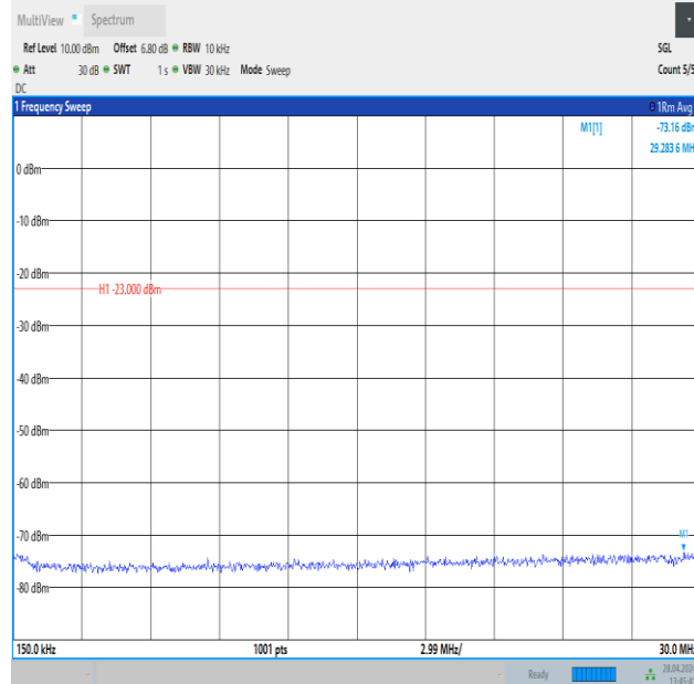
Band26_1.4MHz_QPSK_26783_1RB#5_0.15~30_0.15~30
