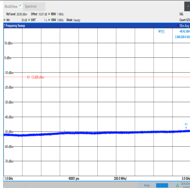
Band26_3MHz_QPSK_26775_1RB#14_1000~3000_1000~3000
