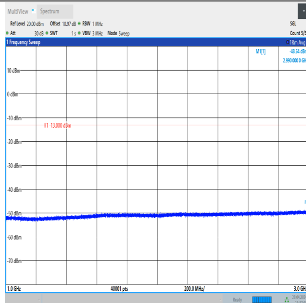
Band26_1.4MHz_16QAM_26697_6RB#0_1000~3000_1000~3000
