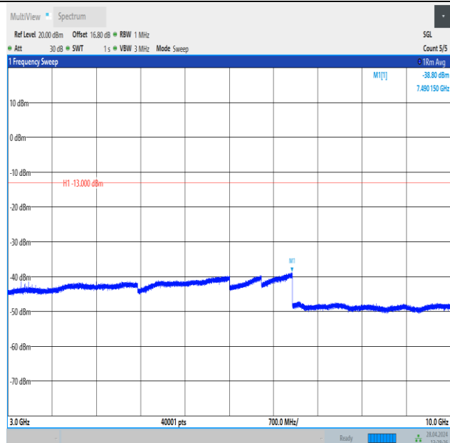
Band26_3MHz_QPSK_26775_1RB#0_3000~10000_3000~10000
