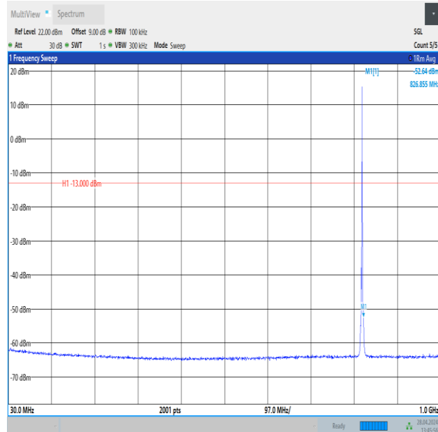
Band26_1.4MHz_QPSK_26783_1RB#5_30~1000_30~1000
