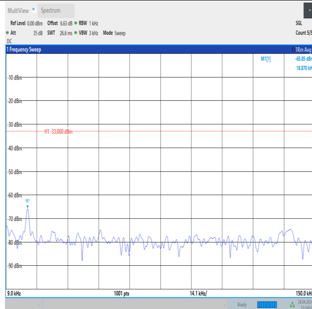
Band26_1.4MHz_16QAM_26697_1RB#0_0.009~0.15_0.009~0.15
