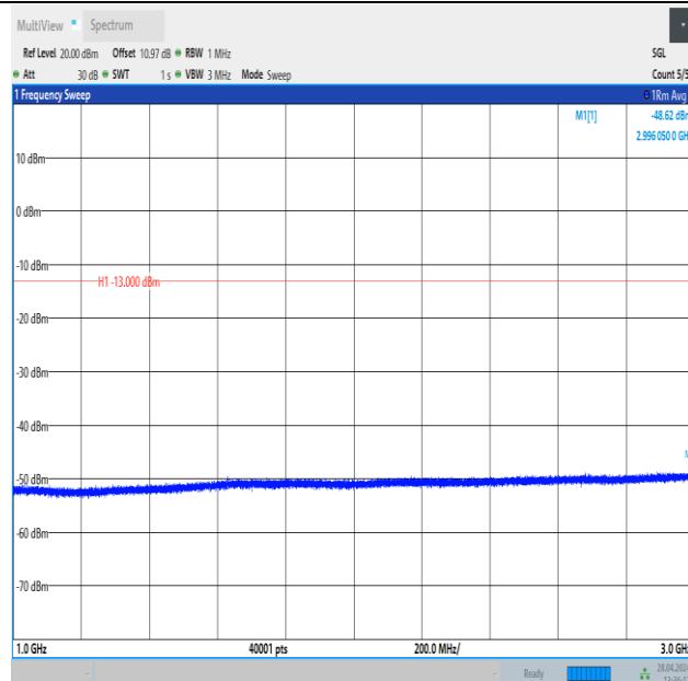
Band26_1.4MHz_16QAM_26697_1RB#5_1000~3000_1000~3000
