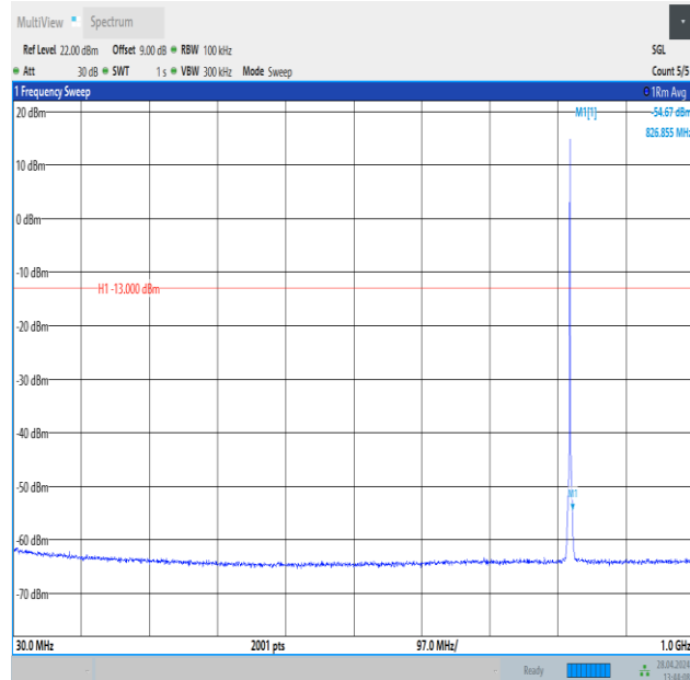
Band26_1.4MHz_QPSK_26783_1RB#0_30~1000_30~1000
