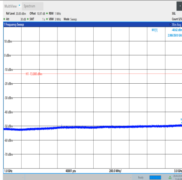
Band26_1.4MHz_QPSK_26783_1RB#5_1000~3000_1000~3000
