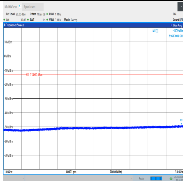
Band26_1.4MHz_QPSK_26740_1RB#5_1000~3000_1000~3000
