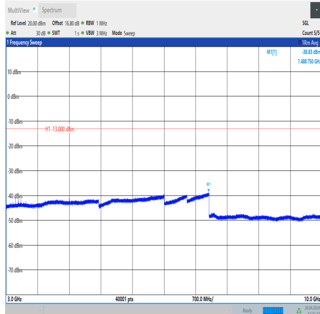
Band26_1.4MHz_QPSK_26697_1RB#5_3000~10000_3000~10000
