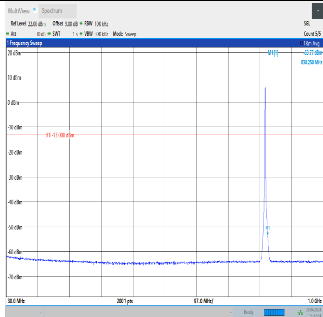
Band26_3MHz_16QAM_26775_15RB#0_30~1000_30~1000
