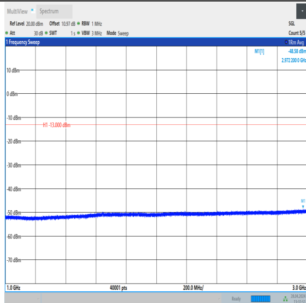
Band26_3MHz_QPSK_26775_15RB#0_1000~3000_1000~3000
