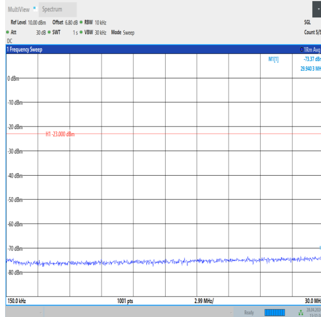
Band26_3MHz_QPSK_26775_15RB#0_0.15~30_0.15~30
