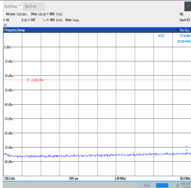
Band26_1.4MHz_QPSK_26740_1RB#0_0.15~30_0.15~30
