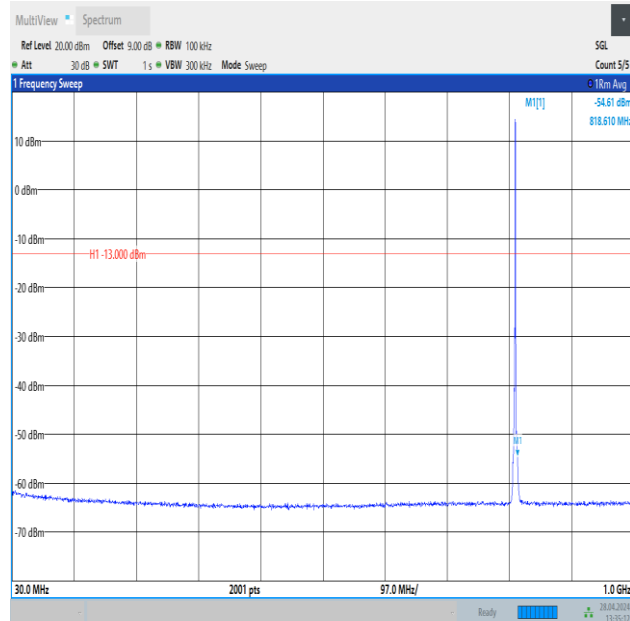
Band26_1.4MHz_QPSK_26697_1RB#5_30~1000_30~1000
