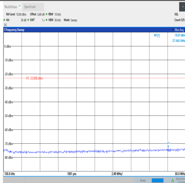
Band26_1.4MHz_16QAM_26740_1RB#5_0.15~30_0.15~30
