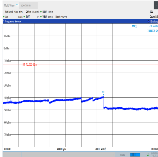
Band26_1.4MHz_16QAM_26783_1RB#5_3000~10000_3000~10000
