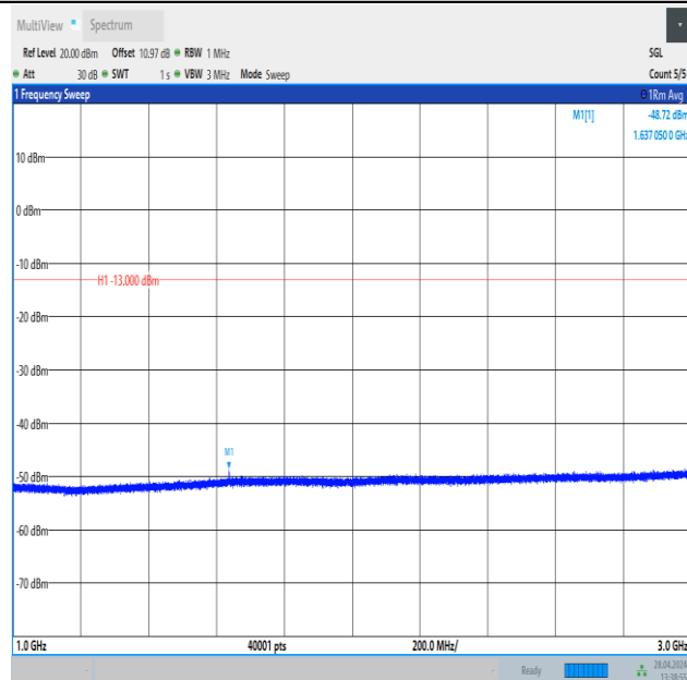
Band26_1.4MHz_QPSK_26740_1RB#0_1000~3000_1000~3000
