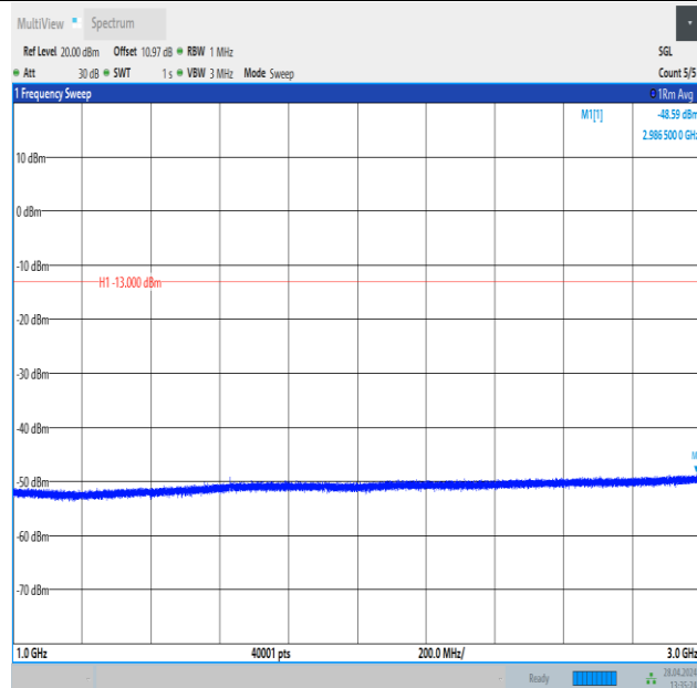
Band26_1.4MHz_QPSK_26697_1RB#5_1000~3000_1000~3000
