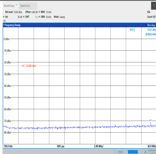
Band26_1.4MHz_16QAM_26697_6RB#0_0.15~30_0.15~30
