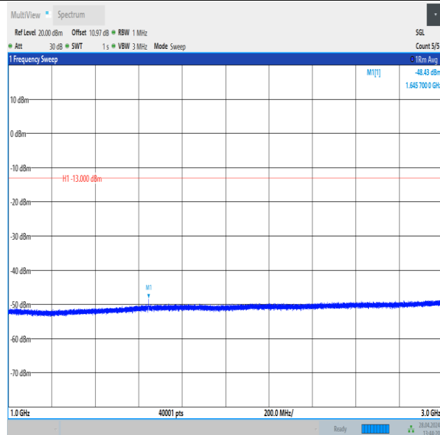
Band26_1.4MHz_QPSK_26783_1RB#0_1000~3000_1000~3000
