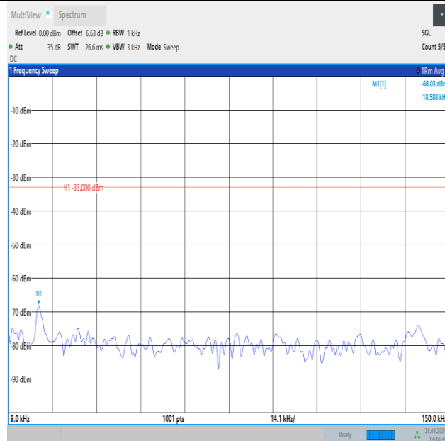
Band26_1.4MHz_16QAM_26783_1RB#0_0.009~0.15_0.009~0.15
