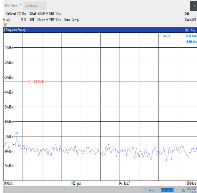
Band26_3MHz_16QAM_26775_1RB#0_0.009~0.15_0.009~0.15
