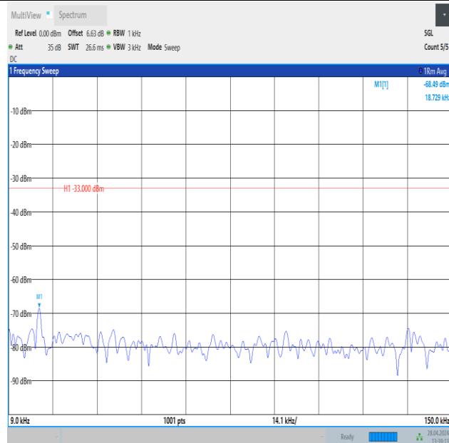
Band26_1.4MHz_16QAM_26740_1RB#0_0.009~0.15_0.009~0.15
