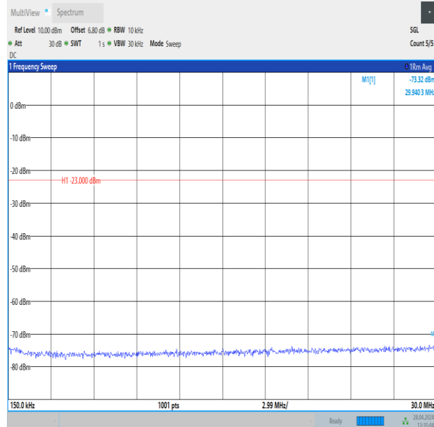
Band26_1.4MHz_QPSK_26697_1RB#5_0.15~30_0.15~30
