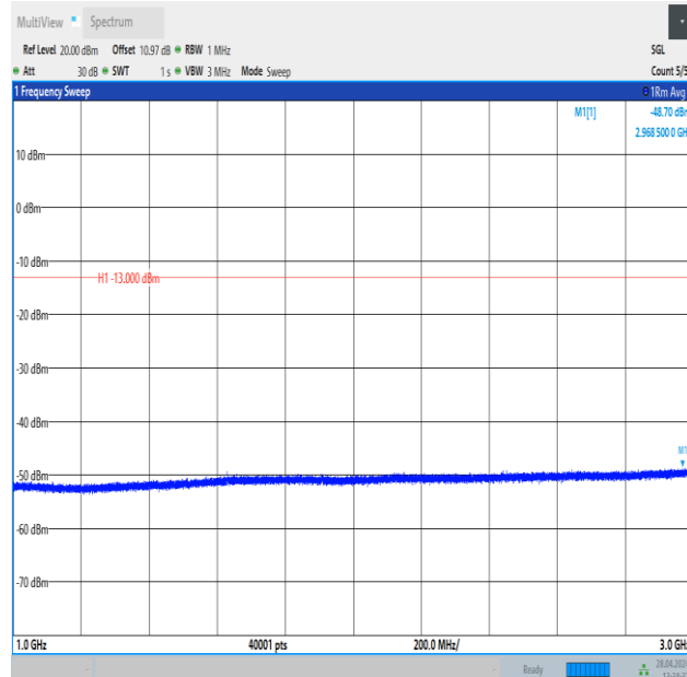
Band26_1.4MHz_16QAM_26697_1RB#0_1000~3000_1000~3000
