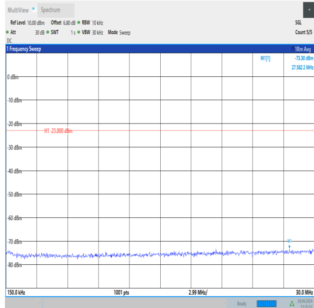
Band26_1.4MHz_16QAM_26697_1RB#5_0.15~30_0.15~30
