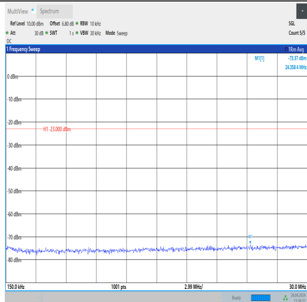
Band26_3MHz_16QAM_26775_1RB#14_0.15~30_0.15~30
