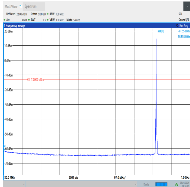
Band26_3MHz_16QAM_26775_1RB#14_30~1000_30~1000
