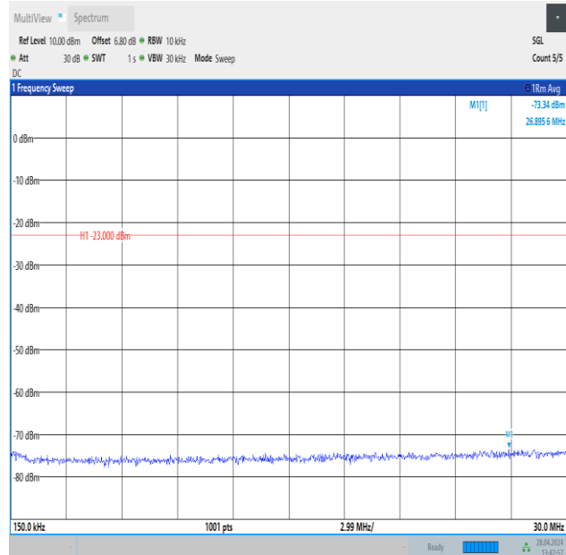
Band26_1.4MHz_16QAM_26740_6RB#0_0.15~30_0.15~30
