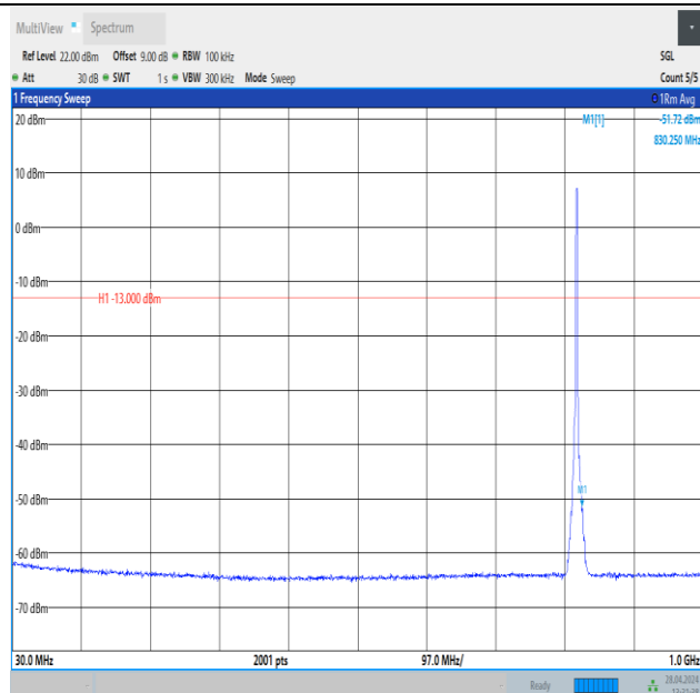
Band26_3MHz_QPSK_26775_15RB#0_30~1000_30~1000
