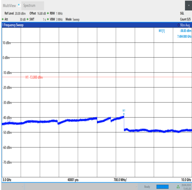
Band26_1.4MHz_16QAM_26783_1RB#0_3000~10000_3000~10000
