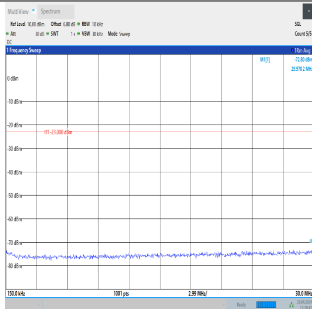
Band26_3MHz_16QAM_26775_1RB#0_0.15~30_0.15~30
