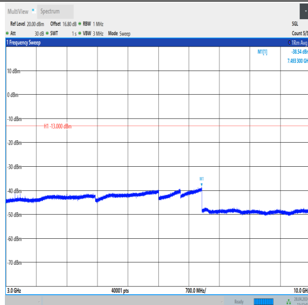
Band26_3MHz_QPSK_26775_15RB#0_3000~10000_3000~10000
