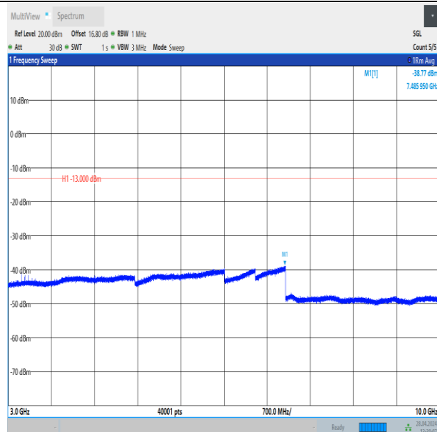
Band26_1.4MHz_QPSK_26740_1RB#0_3000~10000_3000~10000
