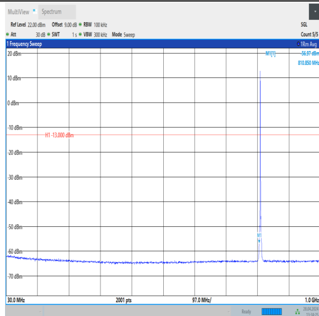
Band26_1.4MHz_16QAM_26697_1RB#0_30~1000_30~1000
