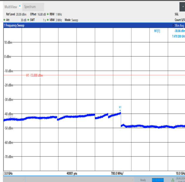
Band26_1.4MHz_QPSK_26783_1RB#5_3000~10000_3000~10000
