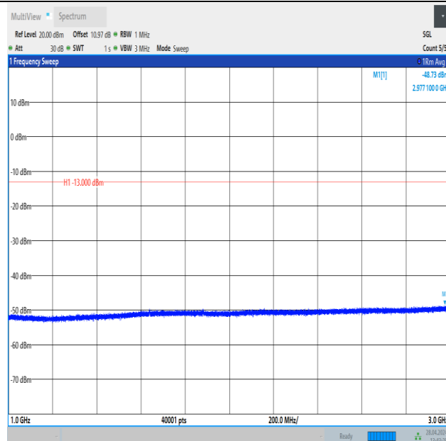
Band26_1.4MHz_16QAM_26740_6RB#0_1000~3000_1000~3000
