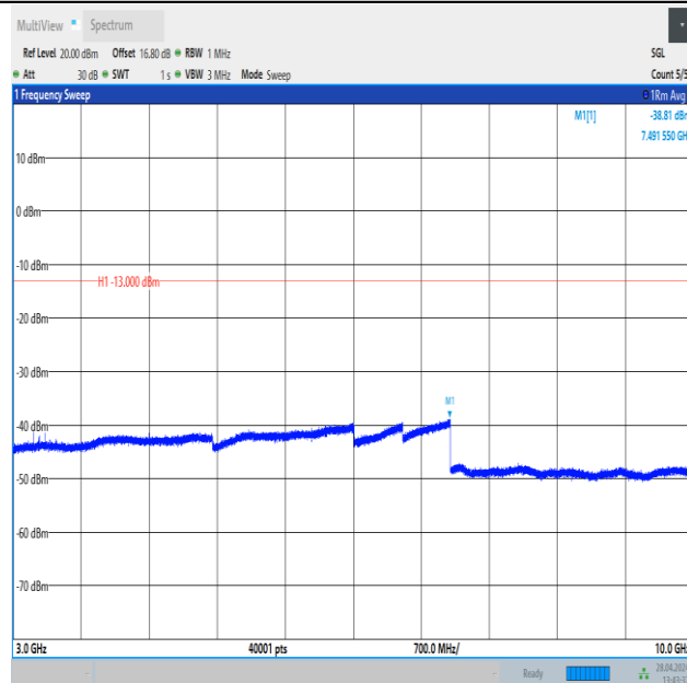
Band26_1.4MHz_16QAM_26740_6RB#0_3000~10000_3000~10000
