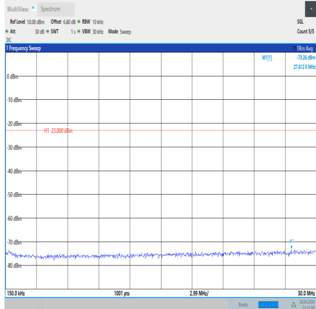
Band26_3MHz_QPSK_26775_1RB#0_0.15~30_0.15~30
