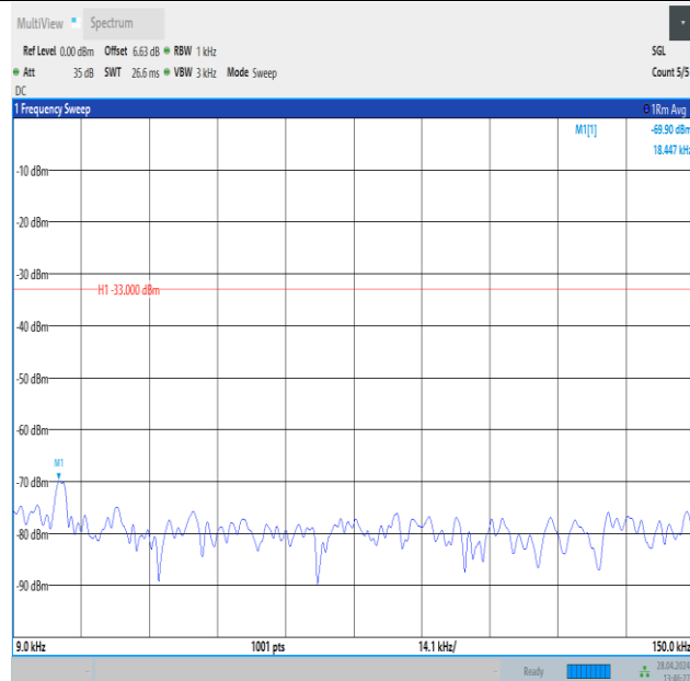
Band26_1.4MHz_16QAM_26783_1RB#5_0.009~0.15_0.009~0.15
