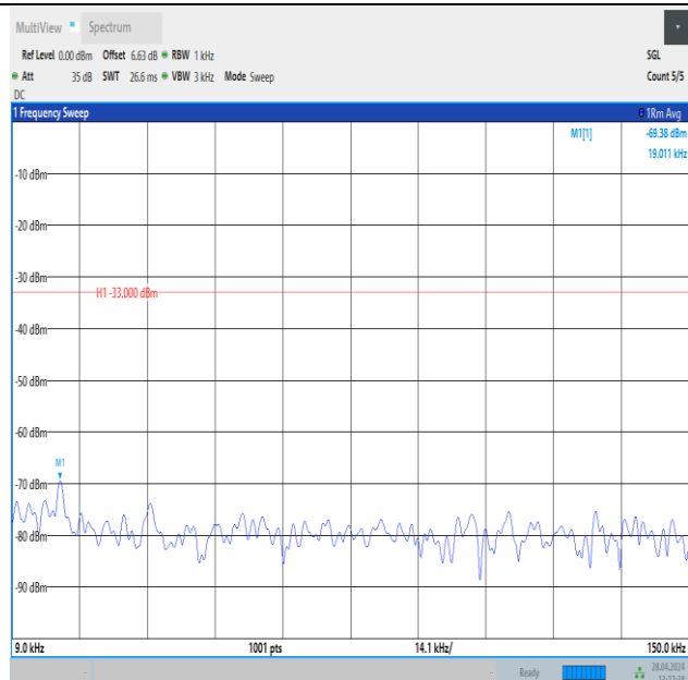
Band26_3MHz_QPSK_26775_1RB#0_0.009~0.15_0.009~0.15
