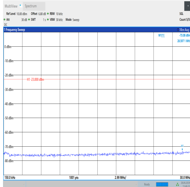
Band26_1.4MHz_16QAM_26783_1RB#5_0.15~30_0.15~30
