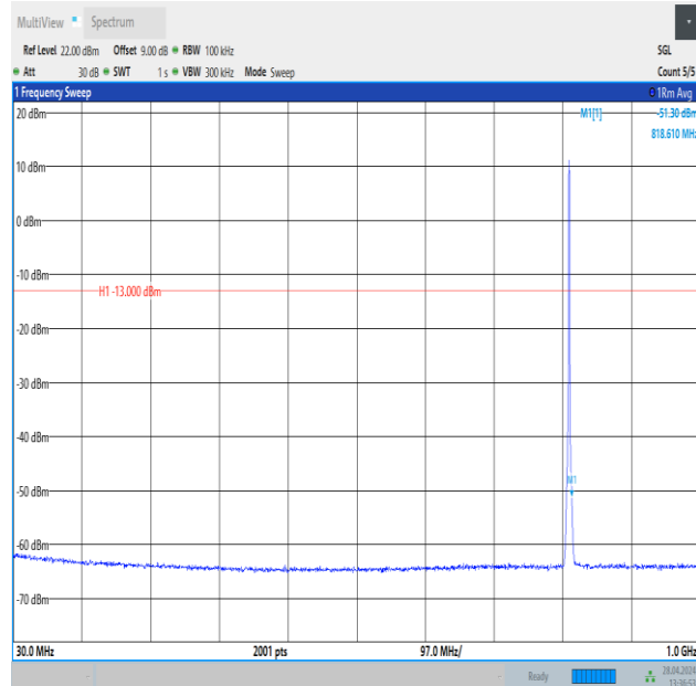
Band26_1.4MHz_QPSK_26697_6RB#0_30~1000_30~1000
