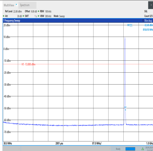
Band26_1.4MHz_16QAM_26697_6RB#0_30~1000_30~1000
