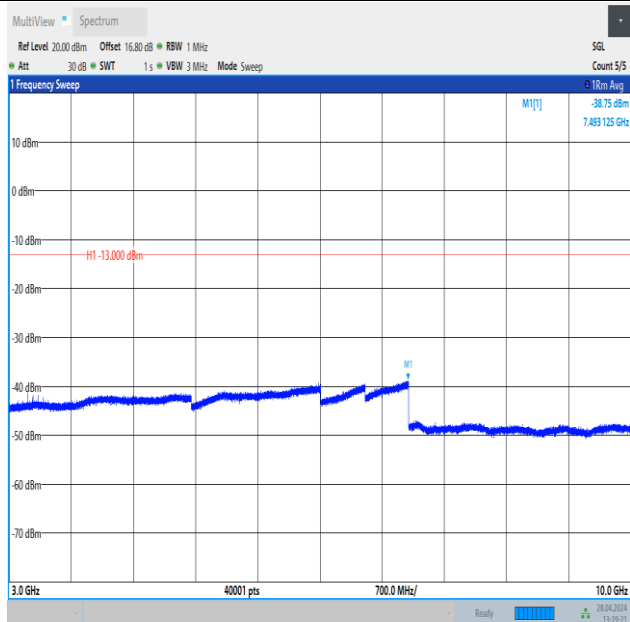
Band26_3MHz_16QAM_26775_1RB#0_3000~10000_3000~10000
