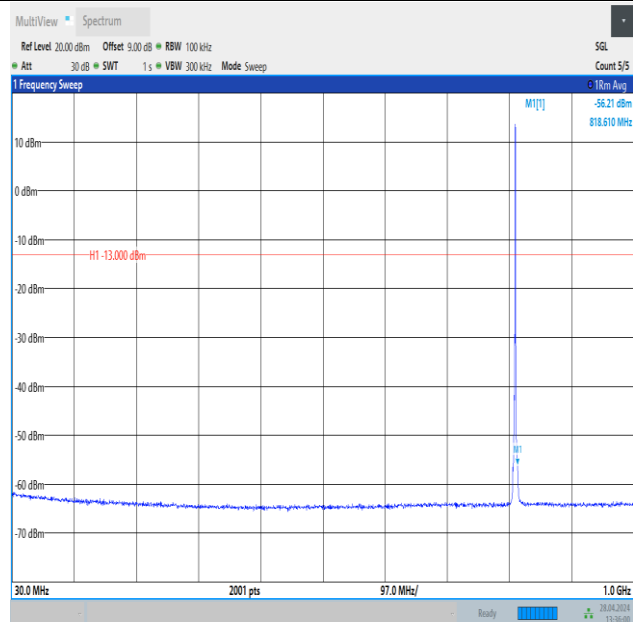
Band26_1.4MHz_16QAM_26697_1RB#5_30~1000_30~1000
