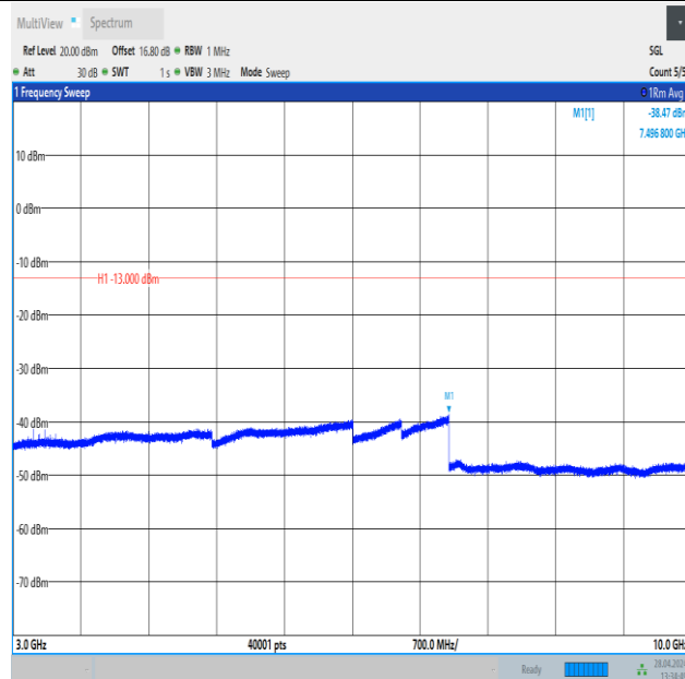
Band26_1.4MHz_16QAM_26697_1RB#0_3000~10000_3000~10000
