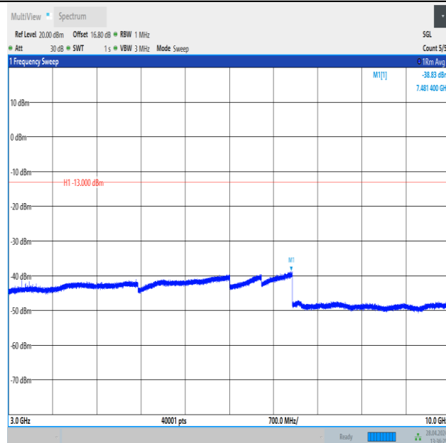
Band26_1.4MHz_16QAM_26697_1RB#5_3000~10000_3000~10000
