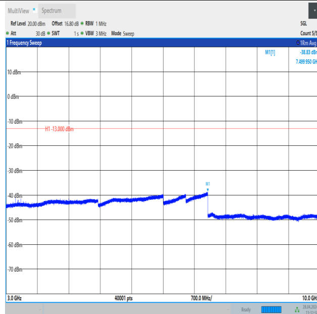
Band26_3MHz_16QAM_26775_15RB#0_3000~10000_3000~10000
