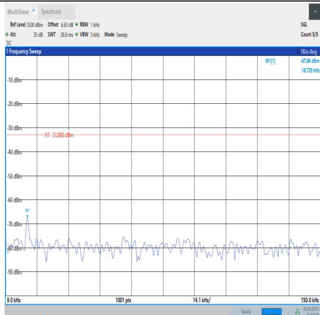
Band26_1.4MHz_QPSK_26740_1RB#5_0.009~0.15_0.009~0.15
