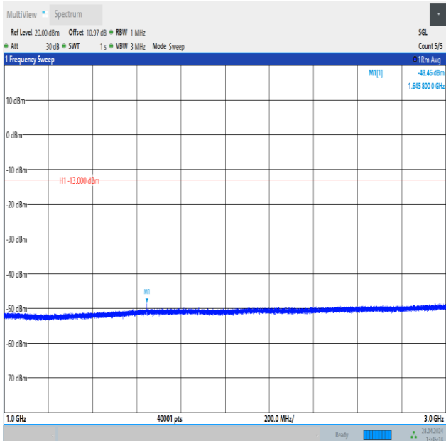
Band26_1.4MHz_16QAM_26783_1RB#0_1000~3000_1000~3000
