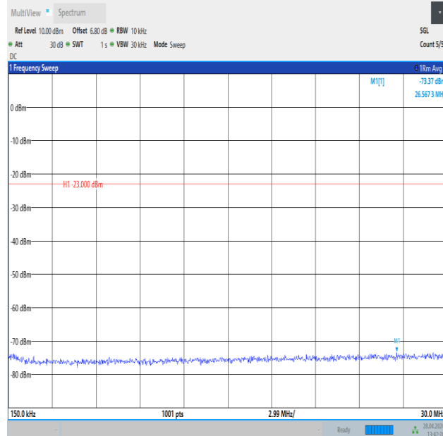
Band26_1.4MHz_QPSK_26783_6RB#0_0.15~30_0.15~30
