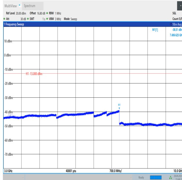
Band26_1.4MHz_QPSK_26783_1RB#0_3000~10000_3000~10000
