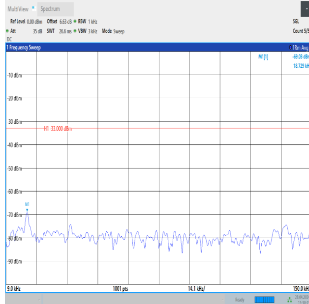
Band26_3MHz_16QAM_26775_1RB#14_0.009~0.15_0.009~0.15
