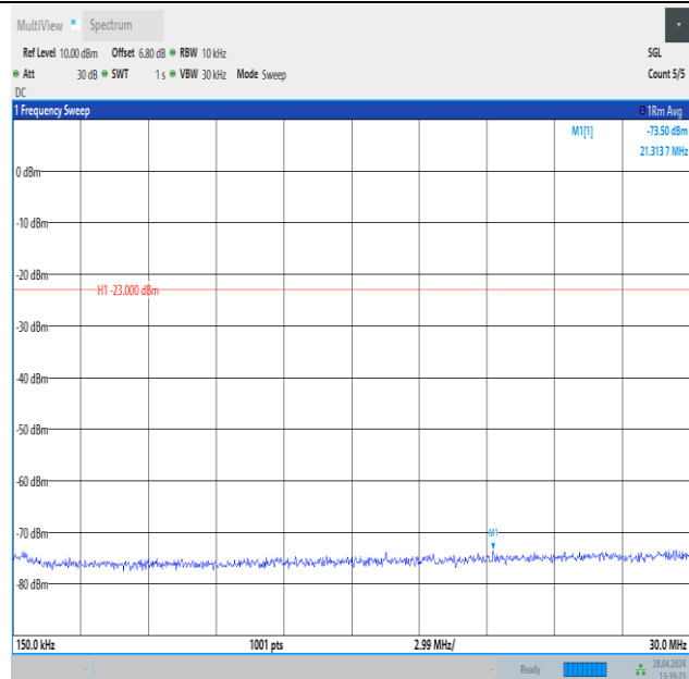
Band26_1.4MHz_16QAM_26740_1RB#0_0.15~30_0.15~30
