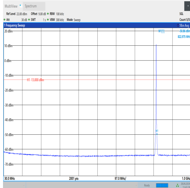
Band26_1.4MHz_QPSK_26740_6RB#0_30~1000_30~1000
