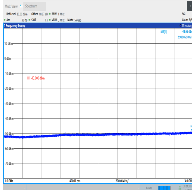
Band26_1.4MHz_16QAM_26783_1RB#5_1000~3000_1000~3000
