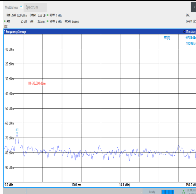
Band26_3MHz_QPSK_26775_15RB#0_0.009~0.15_0.009~0.15
