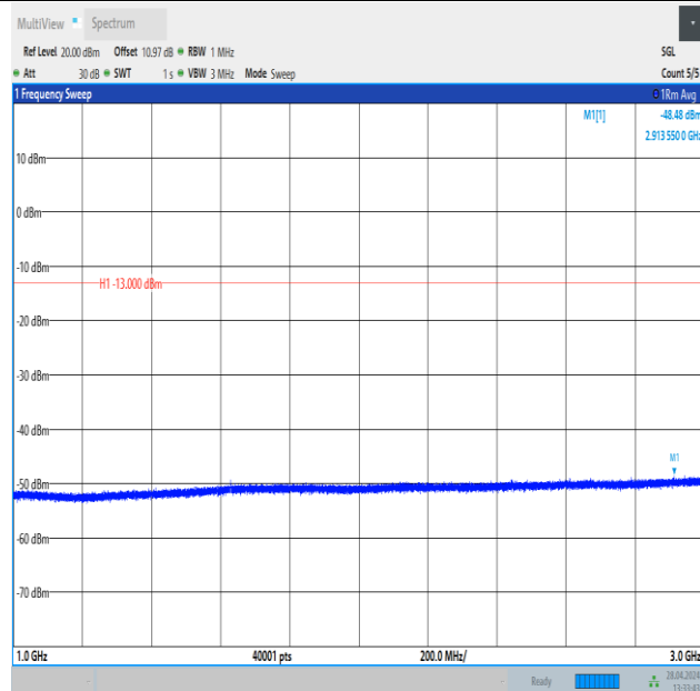
Band26_1.4MHz_QPSK_26697_1RB#0_1000~3000_1000~3000
