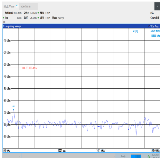
Band26_1.4MHz_QPSK_26740_1RB#0_0.009~0.15_0.009~0.15
