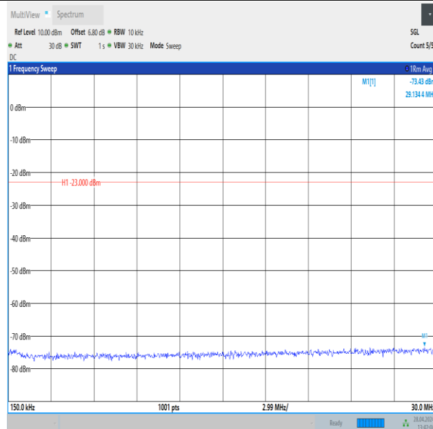
Band26_1.4MHz_QPSK_26740_6RB#0_0.15~30_0.15~30
