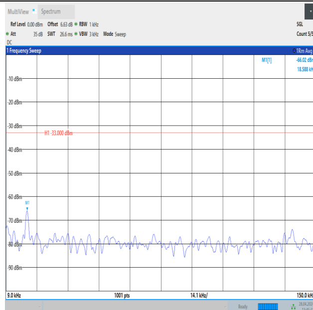
Band26_1.4MHz_QPSK_26783_1RB#5_0.009~0.15_0.009~0.15
