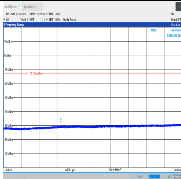
Band26_3MHz_QPSK_26775_1RB#0_1000~3000_1000~3000
