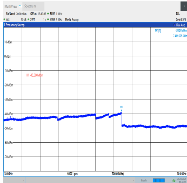
Band26_1.4MHz_16QAM_26740_1RB#0_3000~10000_3000~10000
