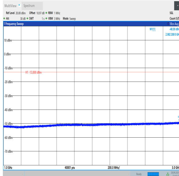
Band26_1.4MHz_16QAM_26740_1RB#5_1000~3000_1000~3000
