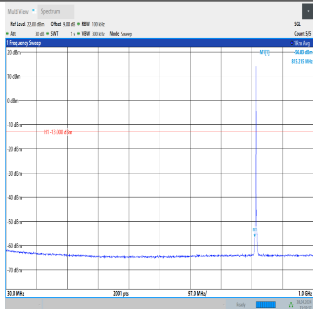
Band26_1.4MHz_16QAM_26740_1RB#0_30~1000_30~1000
