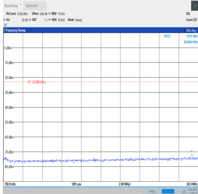
Band26_1.4MHz_QPSK_26740_1RB#5_0.15~30_0.15~30
