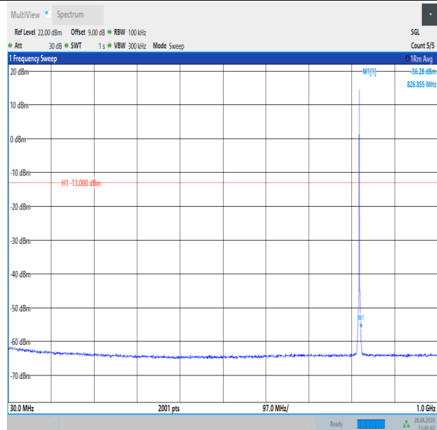
Band26_1.4MHz_16QAM_26783_1RB#0_30~1000_30~1000
