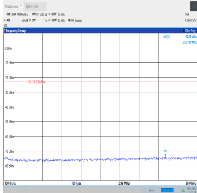
Band26_3MHz_16QAM_26775_15RB#0_0.15~30_0.15~30
