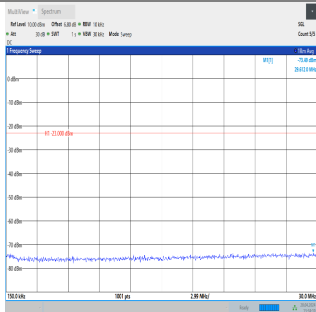
Band26_1.4MHz_16QAM_26697_1RB#0_0.15~30_0.15~30
