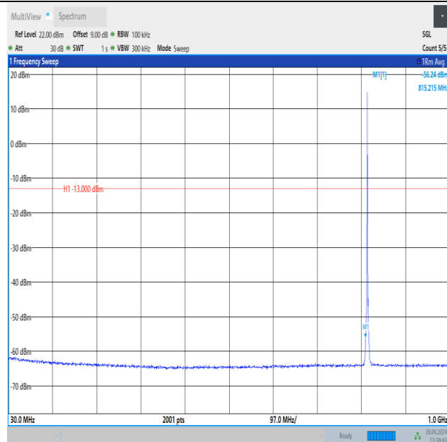
Band26_1.4MHz_QPSK_26740_1RB#0_30~1000_30~1000
