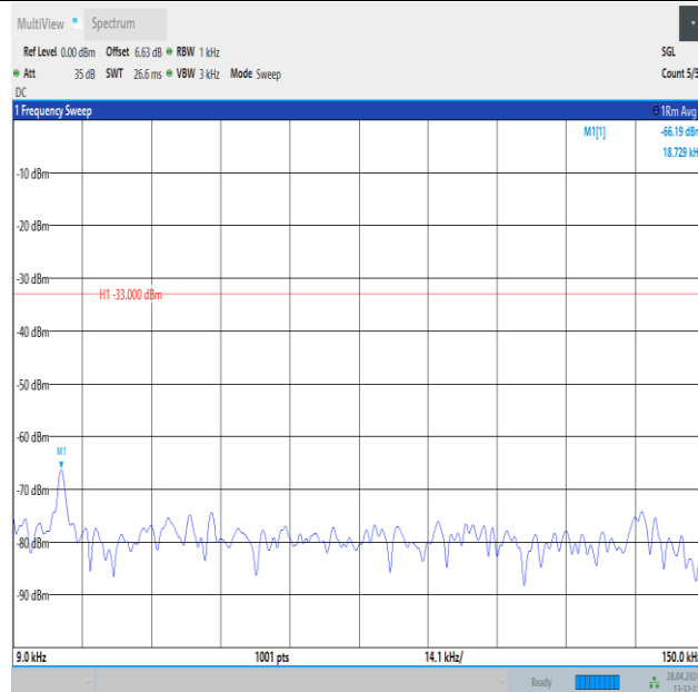
Band26_3MHz_16QAM_26775_15RB#0_0.009~0.15_0.009~0.15
