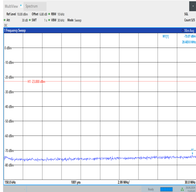
Band26_10MHz_16QAM_26740_1RB#49_0.15~30_0.15~30
