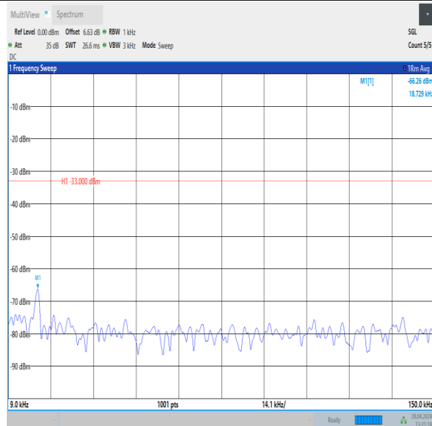
Band26_3MHz_16QAM_26705_15RB#0_0.009~0.15_0.009~0.15
