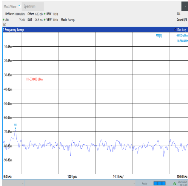
Band26_3MHz_16QAM_26740_15RB#0_0.009~0.15_0.009~0.15
