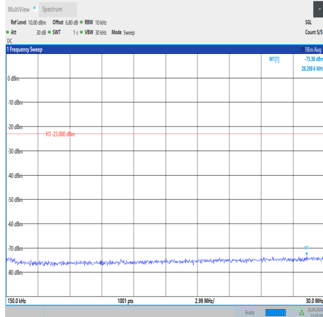
Band26_10MHz_QPSK_26740_1RB#49_0.15~30_0.15~30
