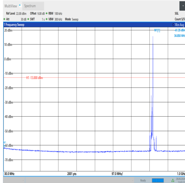
Band26_10MHz_QPSK_26740_1RB#49_30~1000_30~1000
