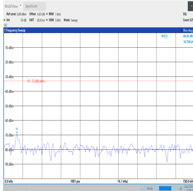
Band26_3MHz_QPSK_26705_15RB#0_0.009~0.15_0.009~0.15
