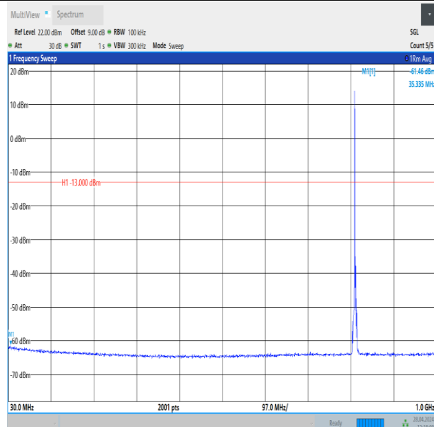
Band26_3MHz_16QAM_26705_1RB#0_30~1000_30~1000
