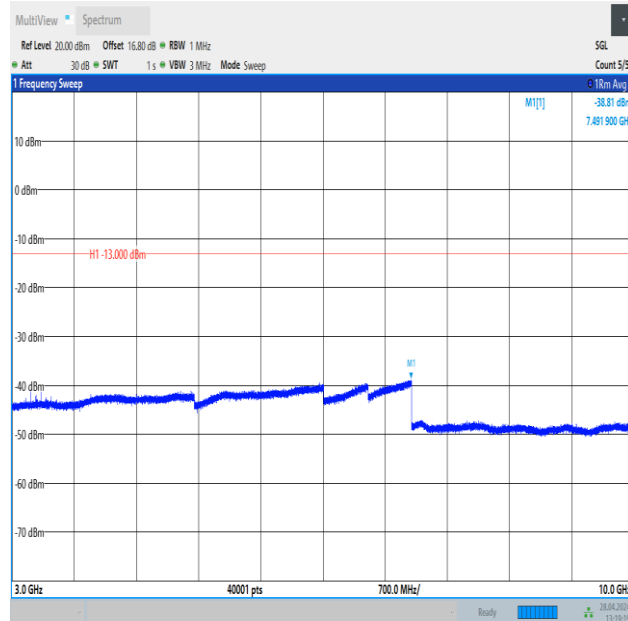
Band26_3MHz_QPSK_26705_1RB#14_3000~10000_3000~10000
