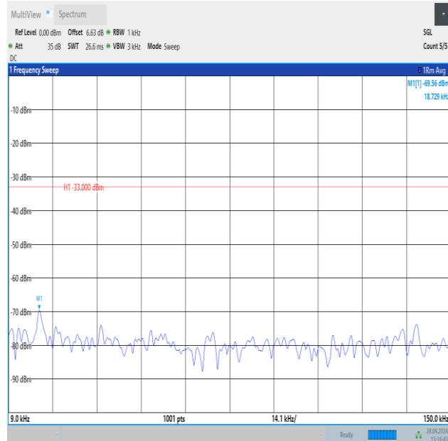
Band26_3MHz_QPSK_26705_1RB#0_0.009~0.15_0.009~0.15
