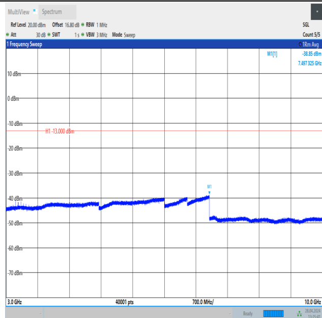
Band26_3MHz_16QAM_26740_1RB#14_3000~10000_3000~10000
