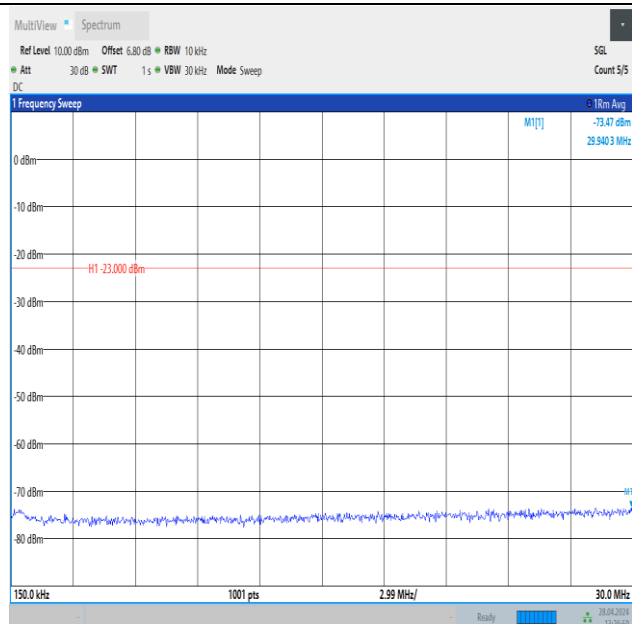
Band26_3MHz_16QAM_26740_15RB#0_0.15~30_0.15~30
