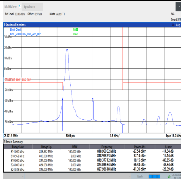
Band26_5MHz_16QAM_26765_1RB#0
