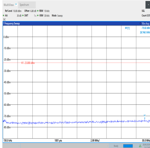
Band26_3MHz_16QAM_26705_1RB#0_0.15~30_0.15~30
