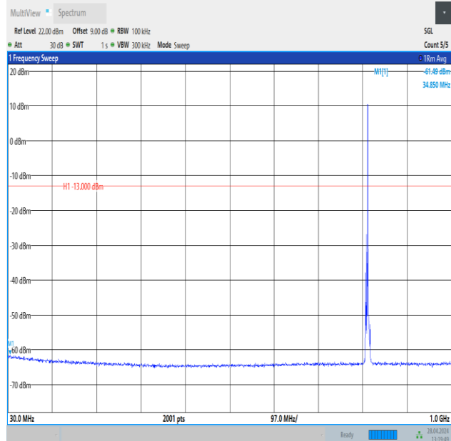
Band26_3MHz_16QAM_26705_1RB#14_30~1000_30~1000
