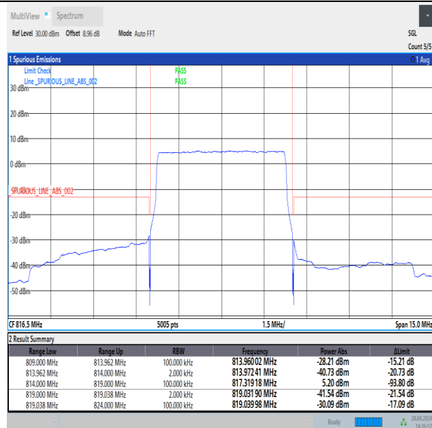
Band26_5MHz_QPSK_26715_25RB#0
