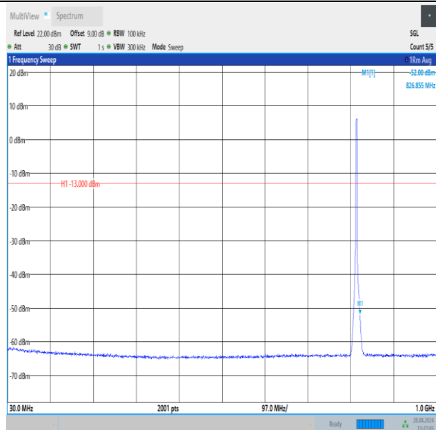
Band26_3MHz_16QAM_26740_15RB#0_30~1000_30~1000
