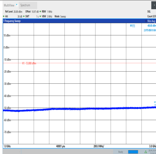
Band26_3MHz_QPSK_26740_15RB#0_1000~3000_1000~3000
