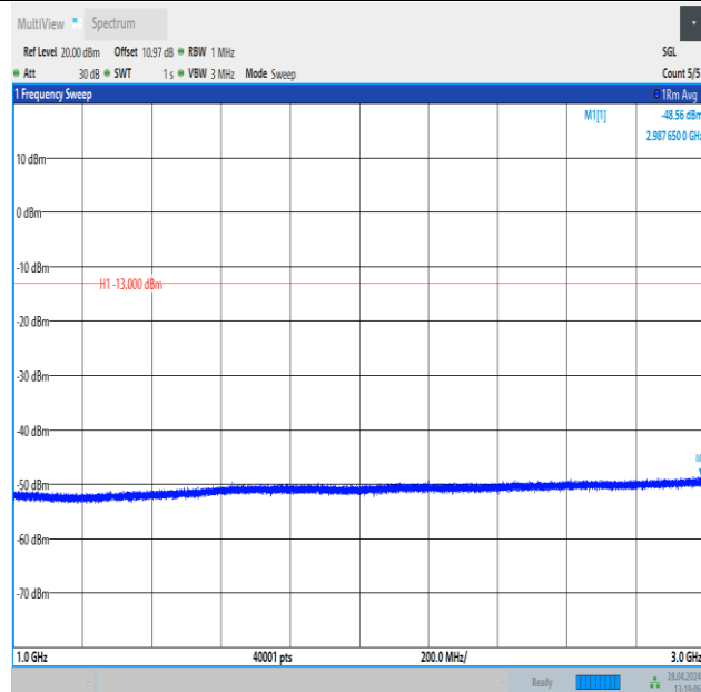
Band26_3MHz_QPSK_26705_1RB#14_1000~3000_1000~3000
