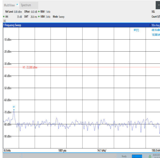
Band26_3MHz_QPSK_26740_15RB#0_0.009~0.15_0.009~0.15
