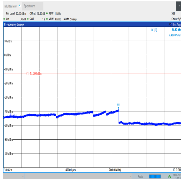
Band26_10MHz_16QAM_26740_1RB#0_3000~10000_3000~10000
