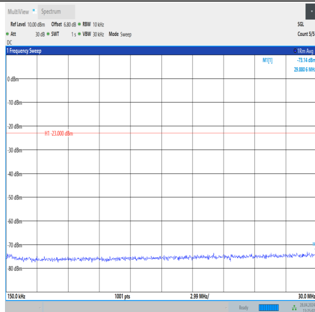
Band26_3MHz_16QAM_26740_1RB#14_0.15~30_0.15~30
