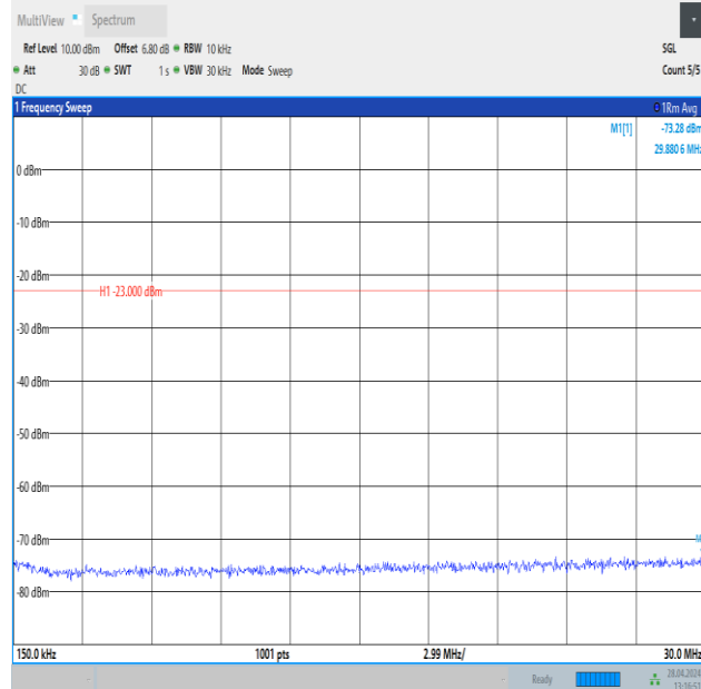
Band26_3MHz_QPSK_26705_1RB#0_0.15~30_0.15~30
