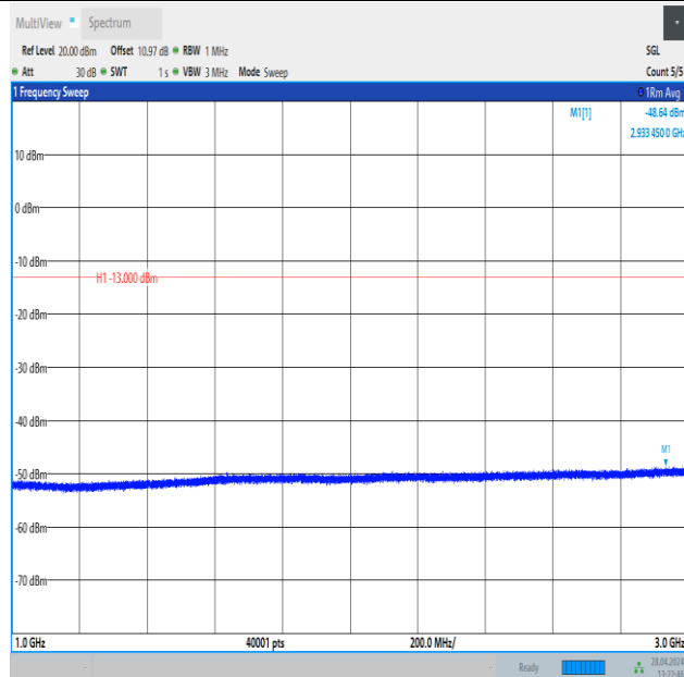
Band26_3MHz_QPSK_26740_1RB#0_1000~3000_1000~3000
