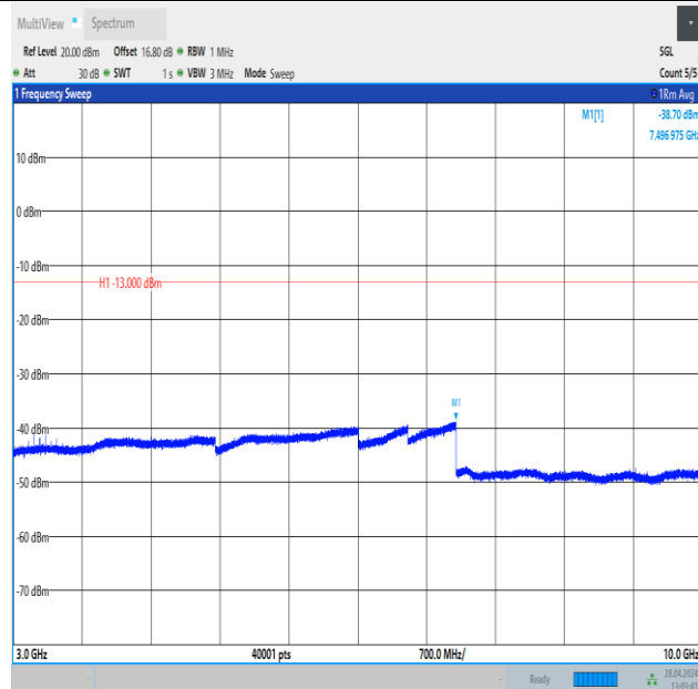
Band26_10MHz_16QAM_26740_1RB#49_3000~10000_3000~10000
