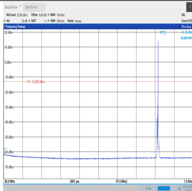
Band26_3MHz_QPSK_26740_1RB#14_30~1000_30~1000
