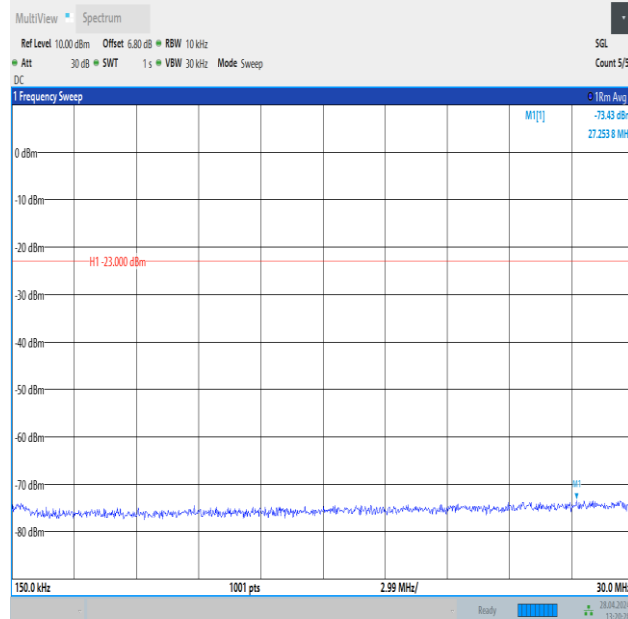
Band26_3MHz_QPSK_26705_15RB#0_0.15~30_0.15~30
