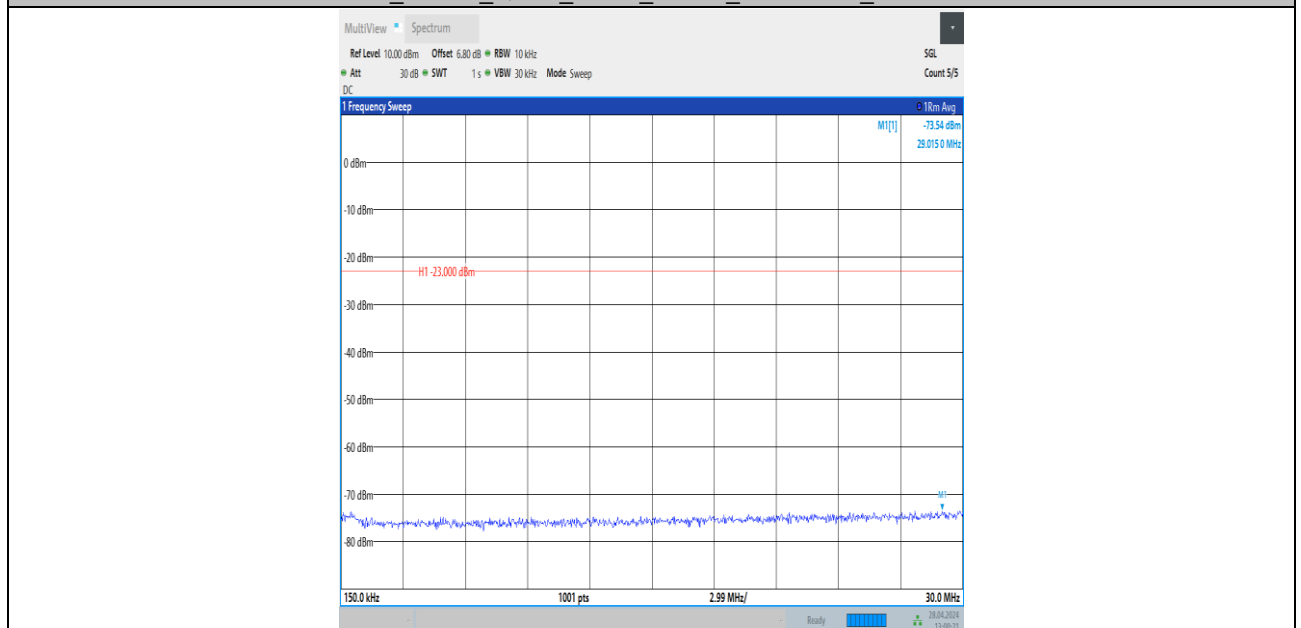
Band26_10MHz_QPSK_26740_1RB#0_0.15~30_0.15~30
