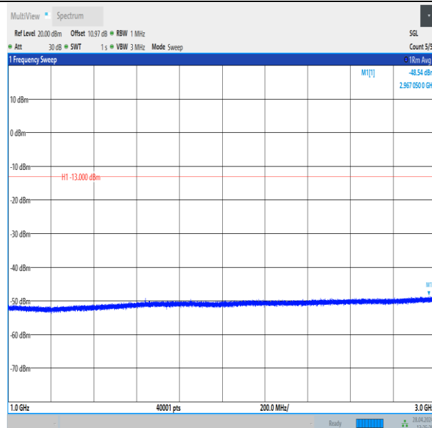
Band26_3MHz_16QAM_26740_1RB#14_1000~3000_1000~3000
