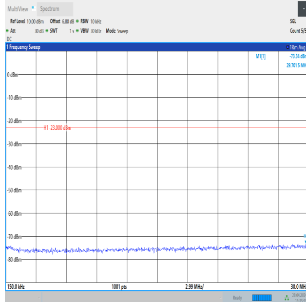
Band26_3MHz_QPSK_26740_15RB#0_0.15~30_0.15~30
