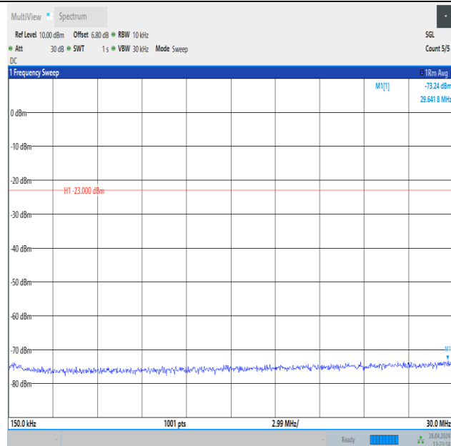
Band26_3MHz_16QAM_26740_1RB#0_0.15~30_0.15~30
