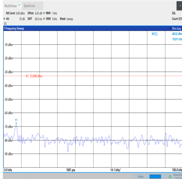
Band26_3MHz_QPSK_26740_1RB#0_0.009~0.15_0.009~0.15
