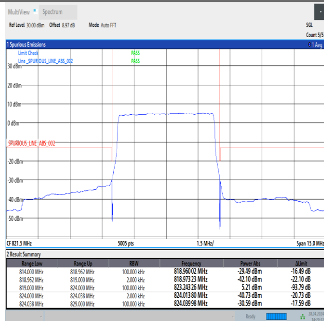
Band26_5MHz_QPSK_26765_25RB#0
