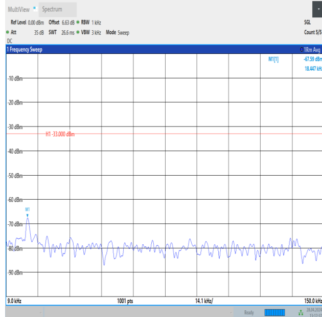
Band26_3MHz_16QAM_26705_1RB#0_0.009~0.15_0.009~0.15
