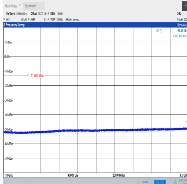
Band26_3MHz_16QAM_26705_1RB#14_1000~3000_1000~3000
