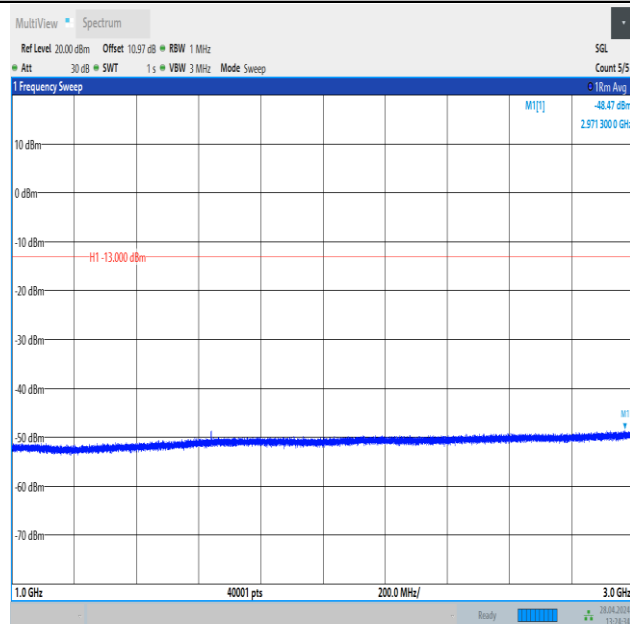
Band26_3MHz_QPSK_26740_1RB#14_1000~3000_1000~3000
