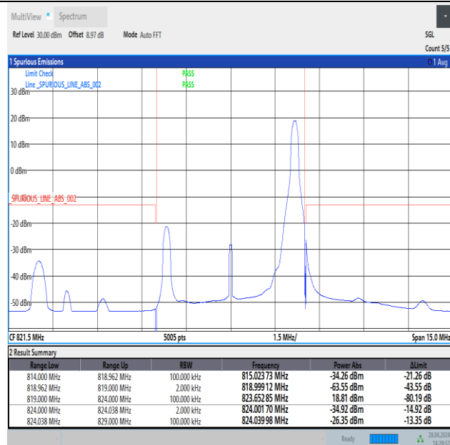
Band26_5MHz_16QAM_26765_1RB#24
