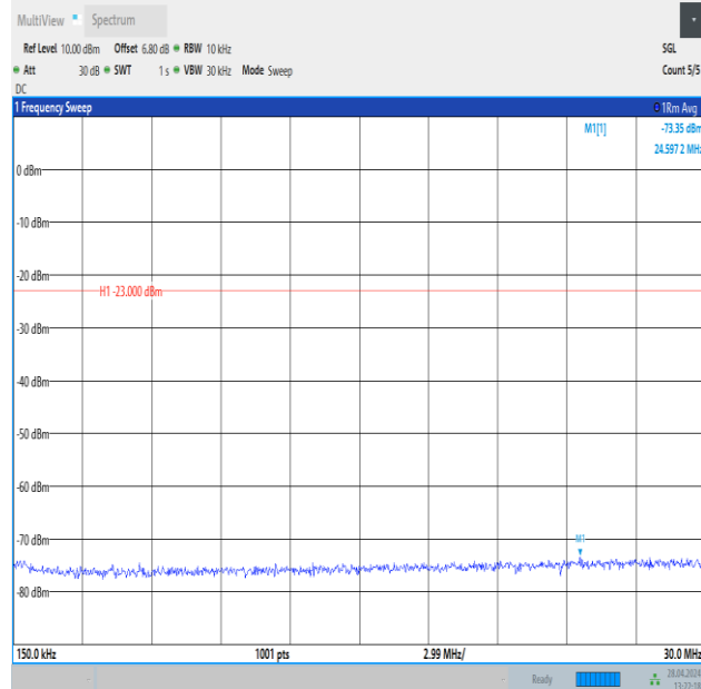
Band26_3MHz_QPSK_26740_1RB#0_0.15~30_0.15~30
