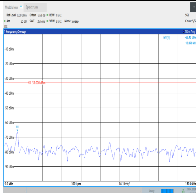
Band26_3MHz_QPSK_26740_1RB#14_0.009~0.15_0.009~0.15
