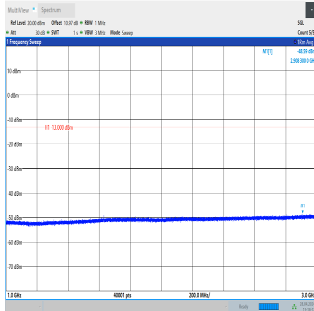
Band26_3MHz_16QAM_26705_1RB#0_1000~3000_1000~3000
