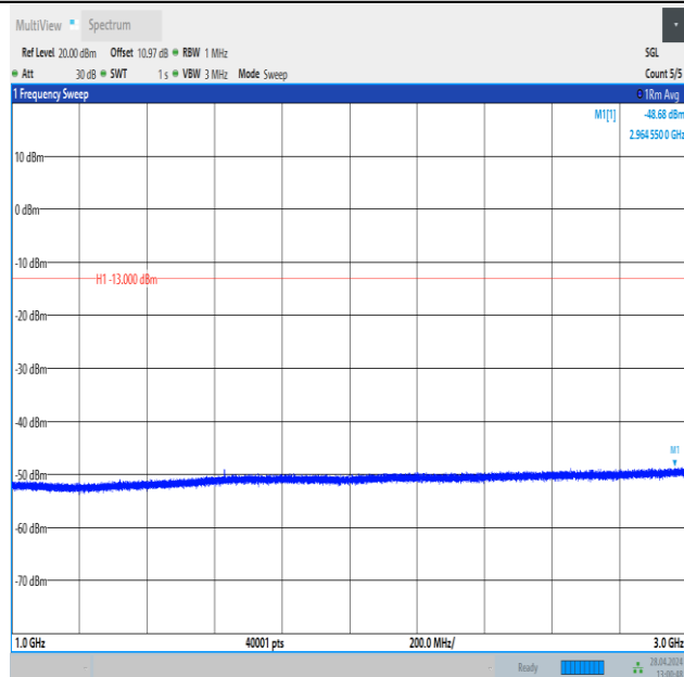
Band26_10MHz_QPSK_26740_1RB#0_1000~3000_1000~3000
