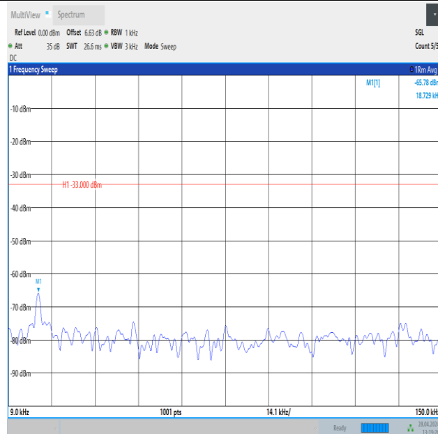
Band26_3MHz_16QAM_26705_1RB#14_0.009~0.15_0.009~0.15
