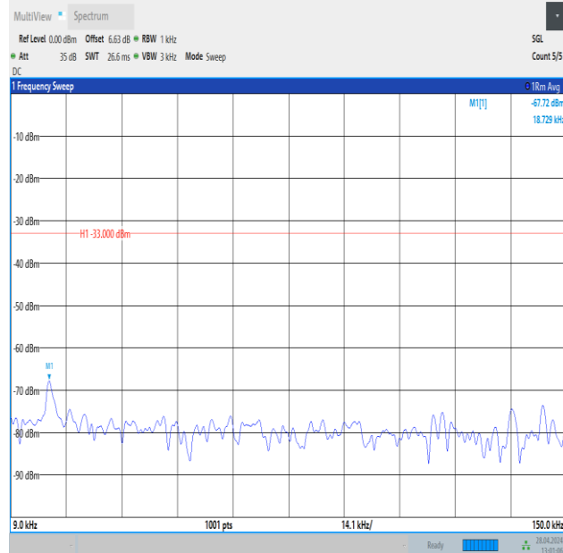
Band26_10MHz_16QAM_26740_1RB#0_0.009~0.15_0.009~0.15
