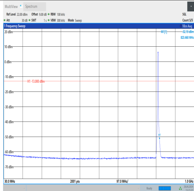
Band26_3MHz_16QAM_26705_15RB#0_30~1000_30~1000
