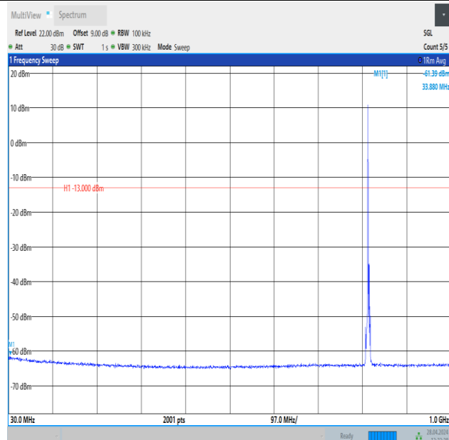
Band26_3MHz_16QAM_26740_1RB#0_30~1000_30~1000
