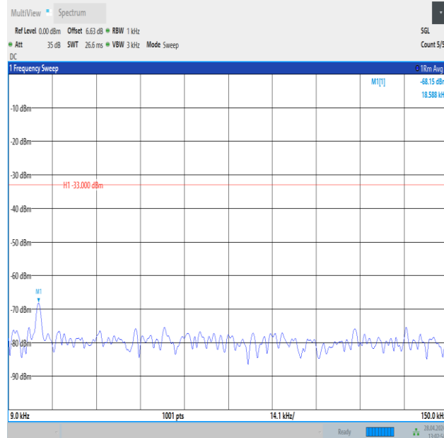
Band26_10MHz_16QAM_26740_1RB#49_0.009~0.15_0.009~0.15
