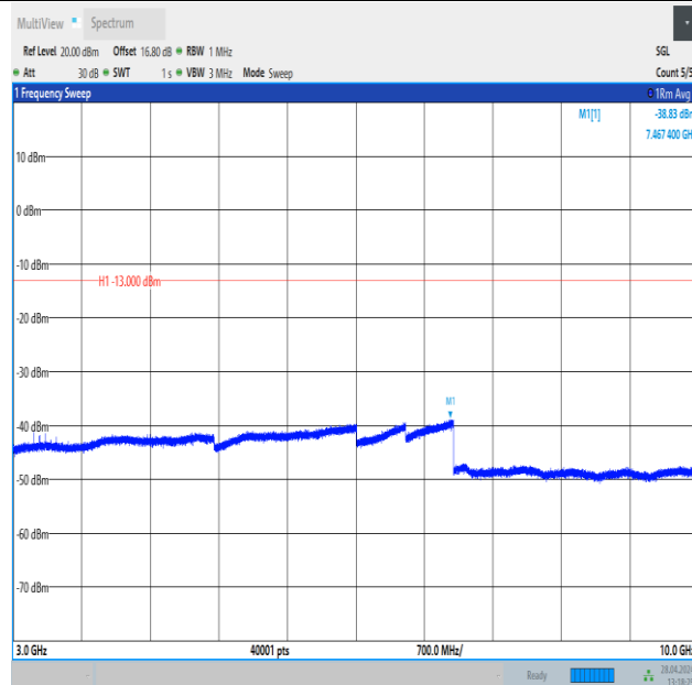
Band26_3MHz_16QAM_26705_1RB#0_3000~10000_3000~10000
