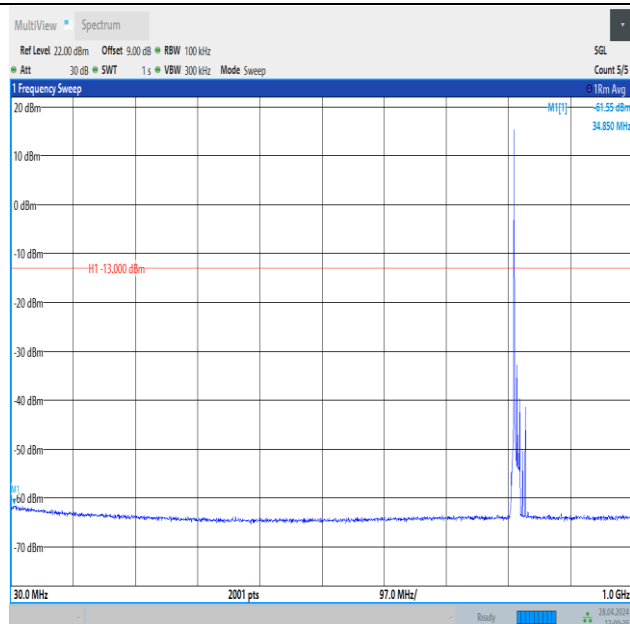
Band26_10MHz_QPSK_26740_1RB#0_30~1000_30~1000
