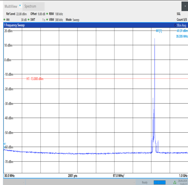
Band26_10MHz_16QAM_26740_1RB#49_30~1000_30~1000
