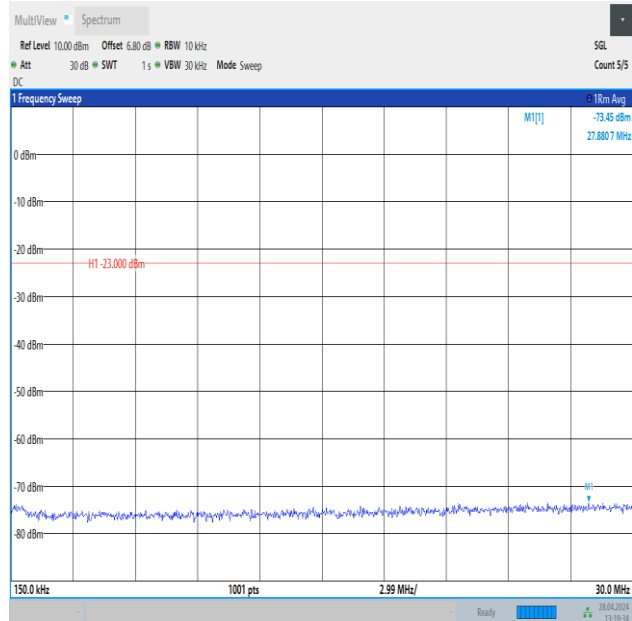
Band26_3MHz_16QAM_26705_1RB#14_0.15~30_0.15~30
