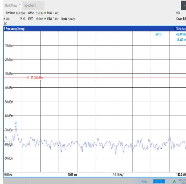
Band26_3MHz_16QAM_26740_1RB#0_0.009~0.15_0.009~0.15
