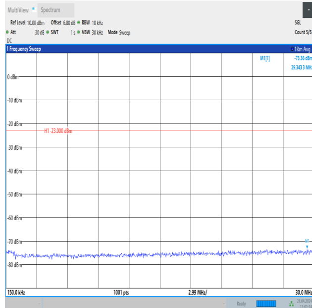
Band26_10MHz_16QAM_26740_1RB#0_0.15~30_0.15~30
