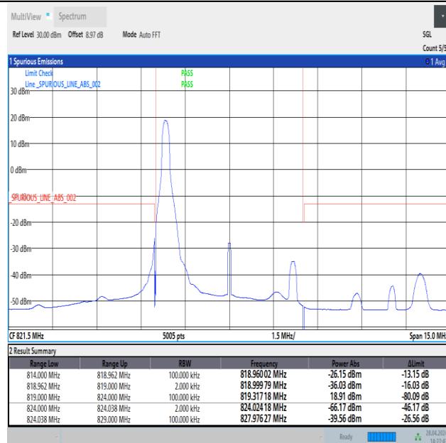
Band26_5MHz_QPSK_26765_1RB#0
