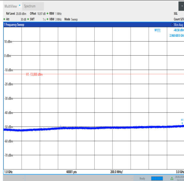
Band26_3MHz_QPSK_26705_1RB#0_1000~3000_1000~3000
