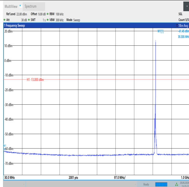
Band26_3MHz_16QAM_26740_1RB#14_30~1000_30~1000
