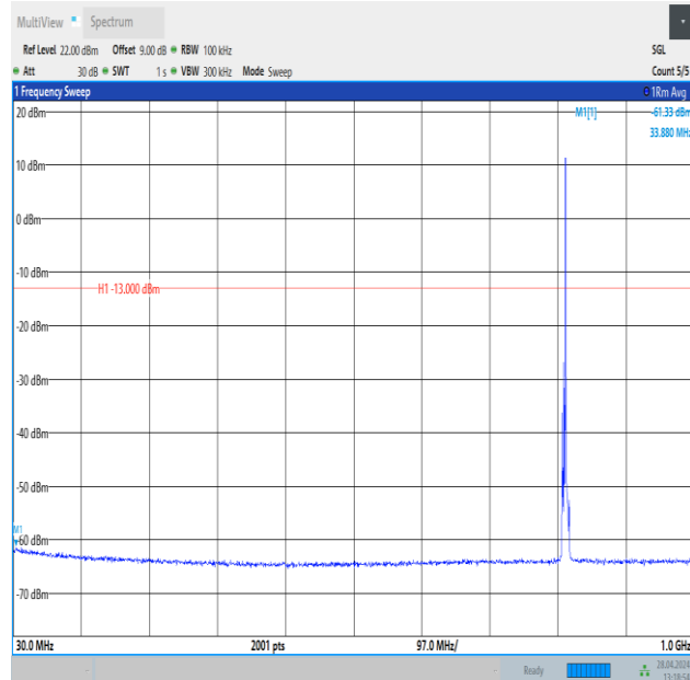
Band26_3MHz_QPSK_26705_1RB#14_30~1000_30~1000
