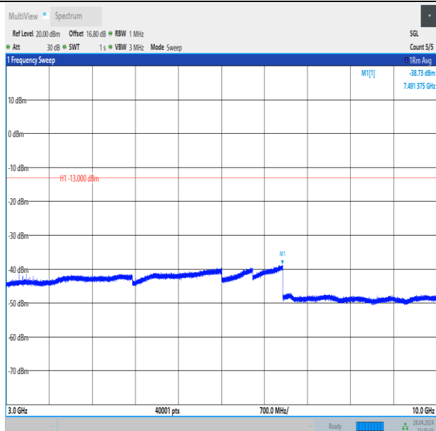
Band26_3MHz_QPSK_26740_15RB#0_3000~10000_3000~10000
