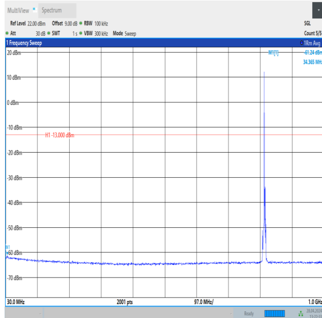
Band26_3MHz_QPSK_26740_1RB#0_30~1000_30~1000
