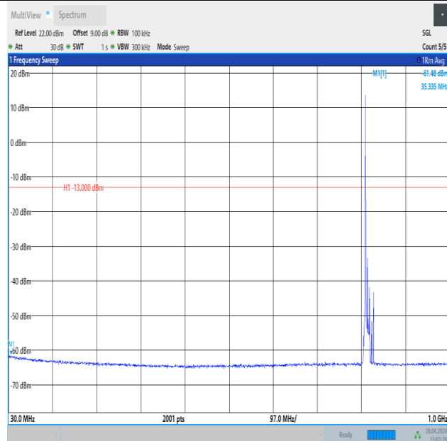
Band26_10MHz_16QAM_26740_1RB#0_30~1000_30~1000
