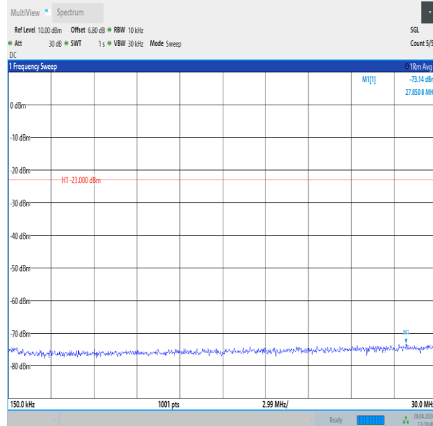
Band26_3MHz_QPSK_26705_1RB#14_0.15~30_0.15~30
