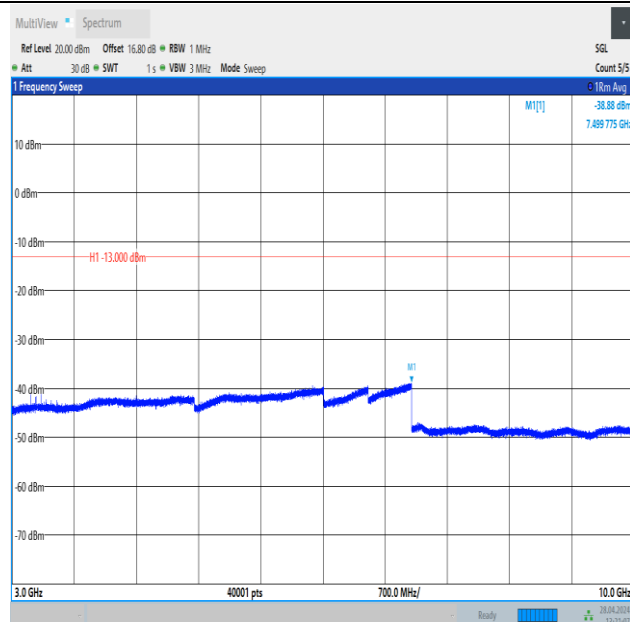
Band26_3MHz_QPSK_26705_15RB#0_3000~10000_3000~10000
