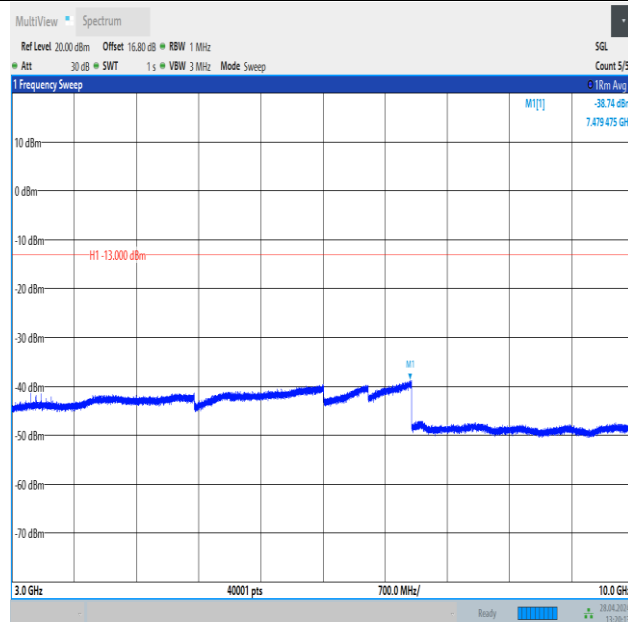
Band26_3MHz_16QAM_26705_1RB#14_3000~10000_3000~10000
