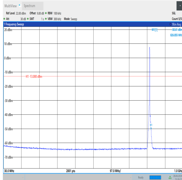
Band26_3MHz_QPSK_26740_15RB#0_30~1000_30~1000
