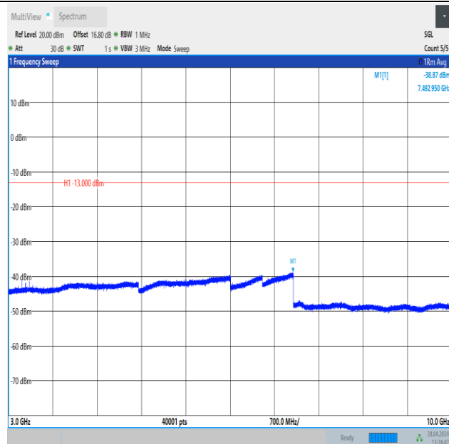
Band26_3MHz_QPSK_26740_1RB#14_3000~10000_3000~10000
