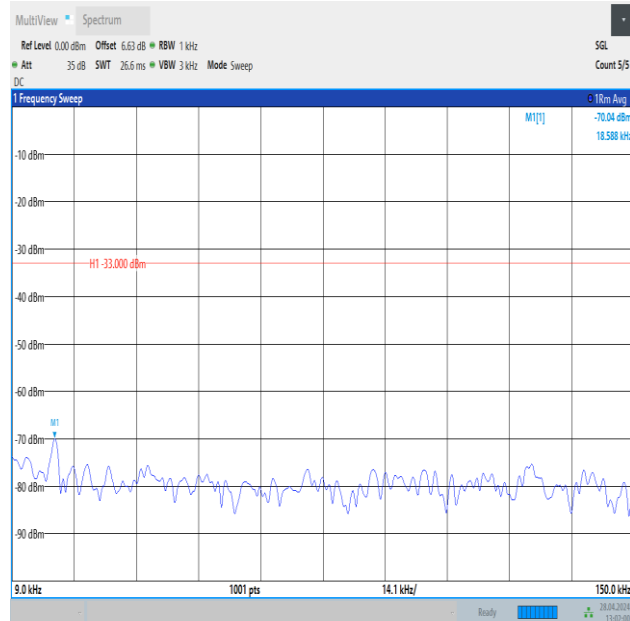
Band26_10MHz_QPSK_26740_1RB#49_0.009~0.15_0.009~0.15
