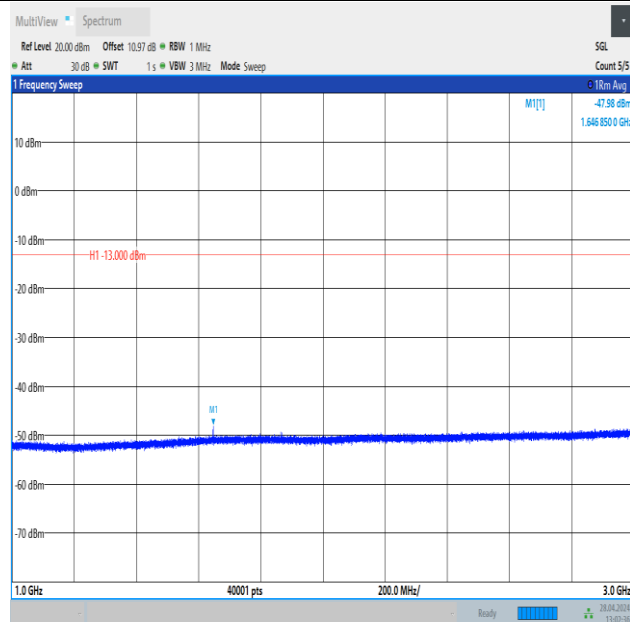
Band26_10MHz_QPSK_26740_1RB#49_1000~3000_1000~3000
