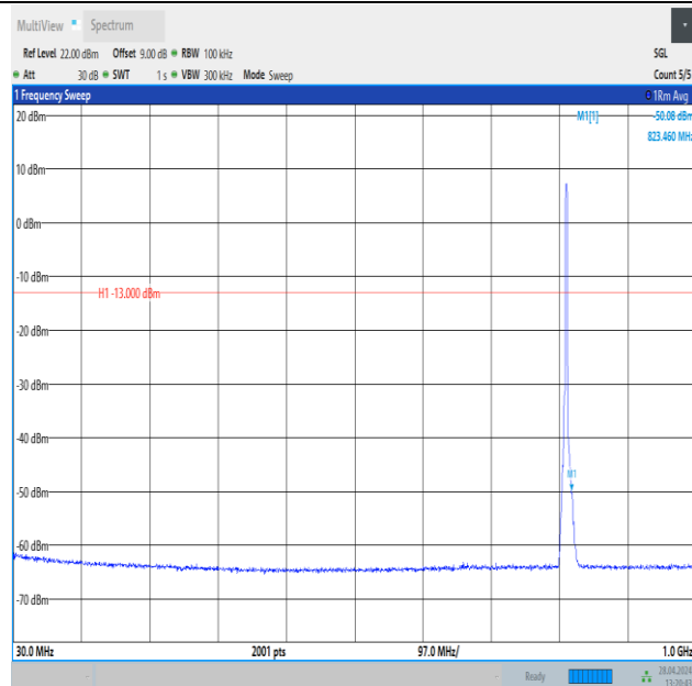
Band26_3MHz_QPSK_26705_15RB#0_30~1000_30~1000
