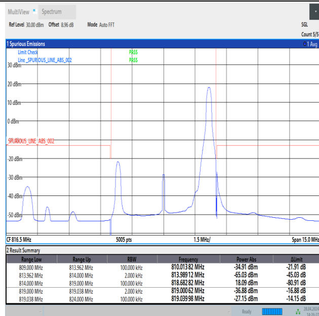
Band26_5MHz_16QAM_26715_1RB#24
