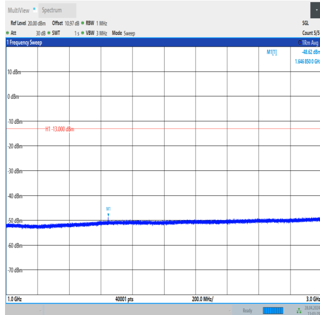
Band26_10MHz_16QAM_26740_1RB#49_1000~3000_1000~3000
