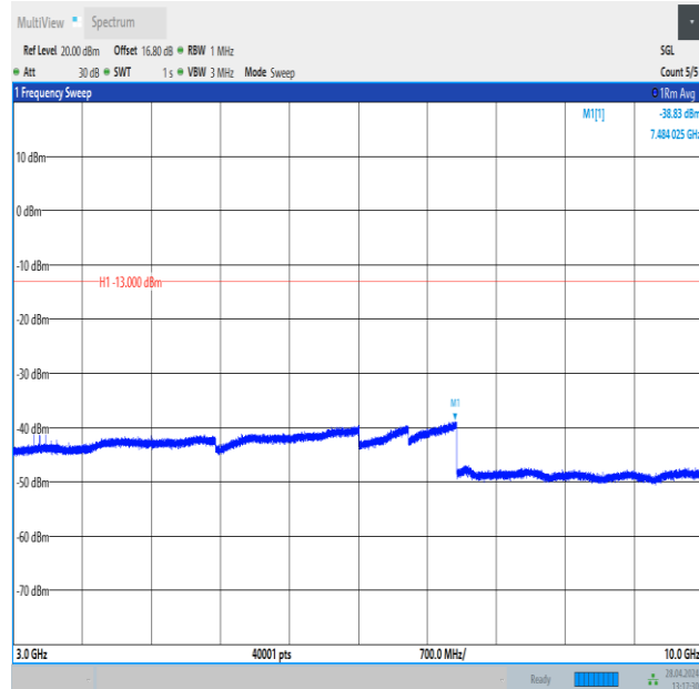
Band26_3MHz_QPSK_26705_1RB#0_3000~10000_3000~10000
