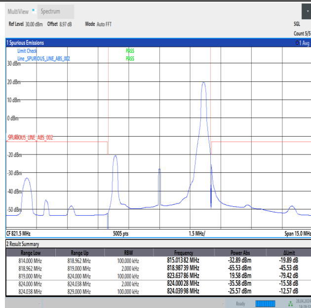
Band26_5MHz_QPSK_26765_1RB#24
