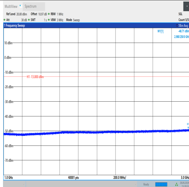
Band26_3MHz_QPSK_26705_15RB#0_1000~3000_1000~3000
