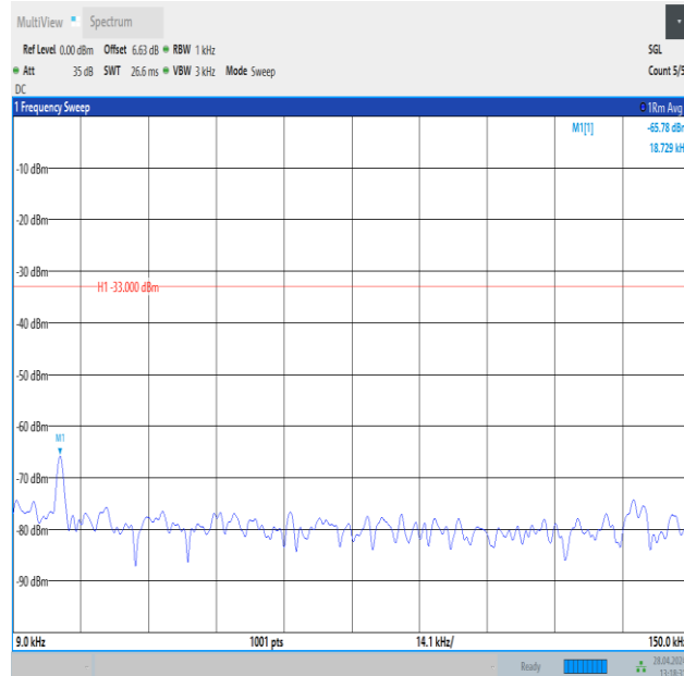
Band26_3MHz_QPSK_26705_1RB#14_0.009~0.15_0.009~0.15
