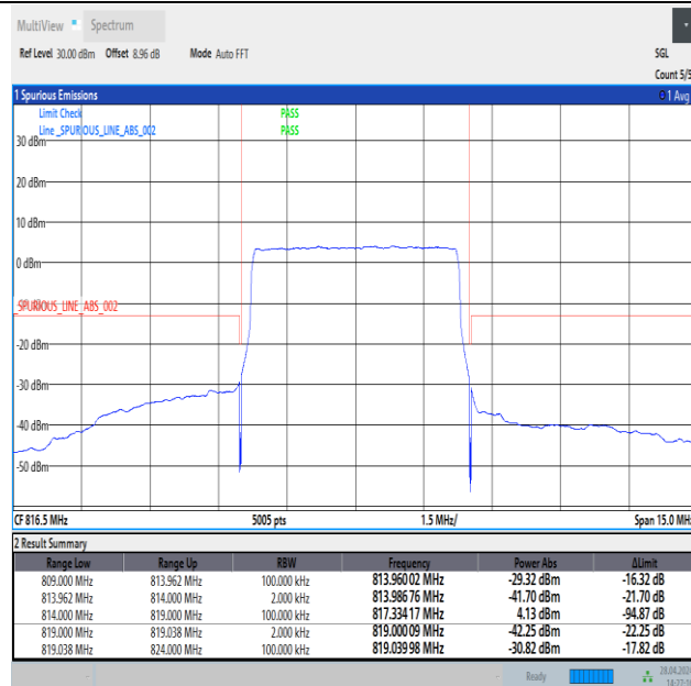
Band26_5MHz_16QAM_26715_25RB#0
