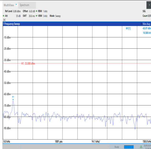
Band26_3MHz_16QAM_26740_1RB#14_0.009~0.15_0.009~0.15
