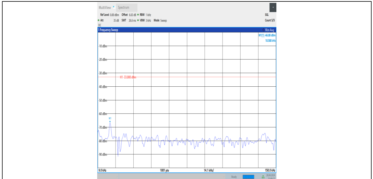
Band26_10MHz_QPSK_26740_1RB#0_0.009~0.15_0.009~0.15
