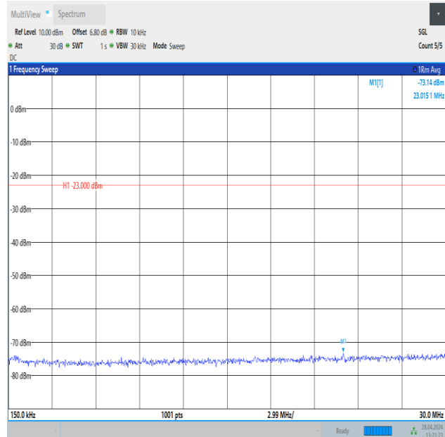
Band26_3MHz_16QAM_26705_15RB#0_0.15~30_0.15~30
