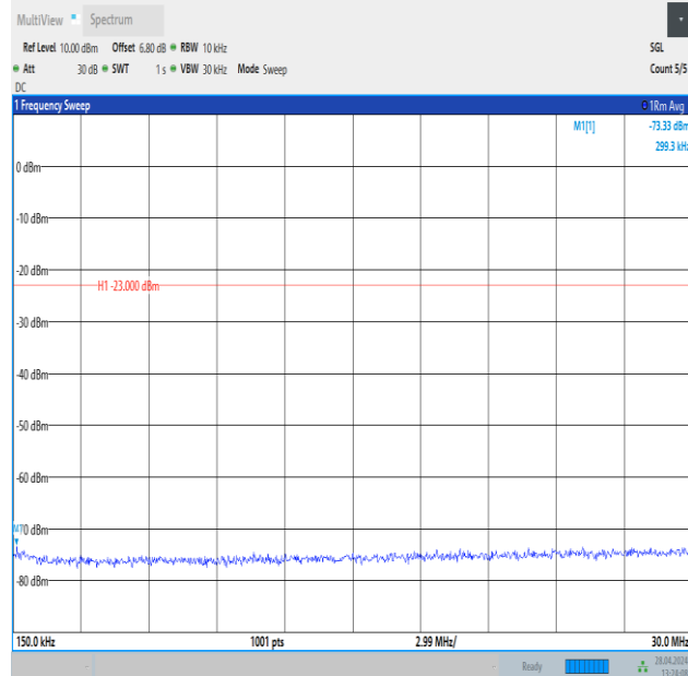
Band26_3MHz_QPSK_26740_1RB#14_0.15~30_0.15~30
