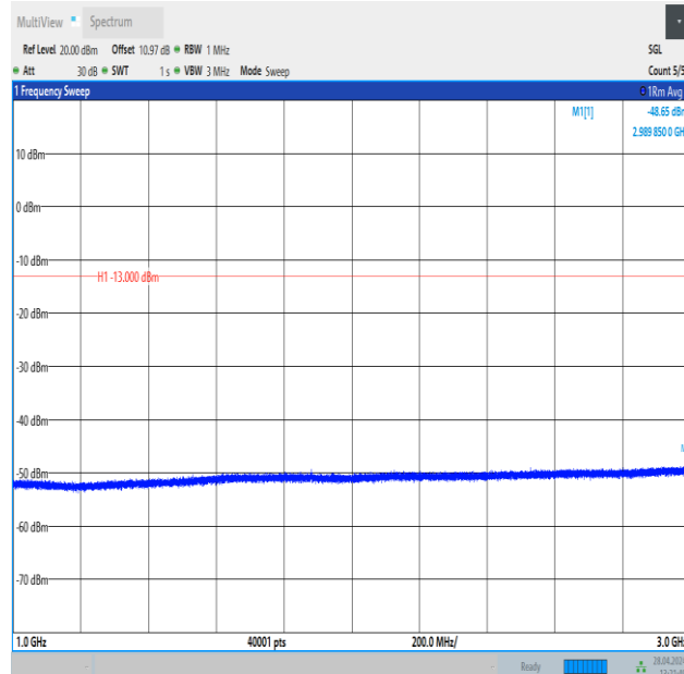
Band26_3MHz_16QAM_26705_15RB#0_1000~3000_1000~3000
