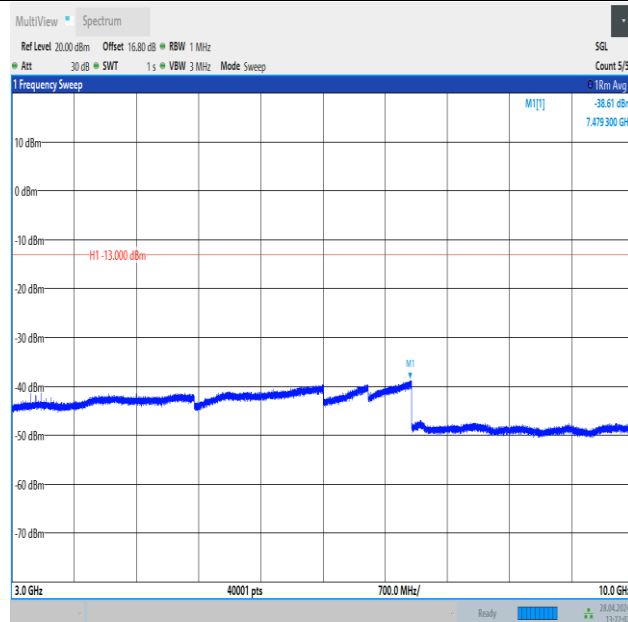
Band26_3MHz_16QAM_26705_15RB#0_3000~10000_3000~10000
