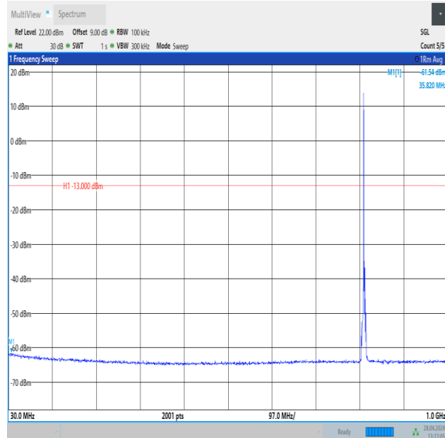
Band26_3MHz_QPSK_26705_1RB#0_30~1000_30~1000
