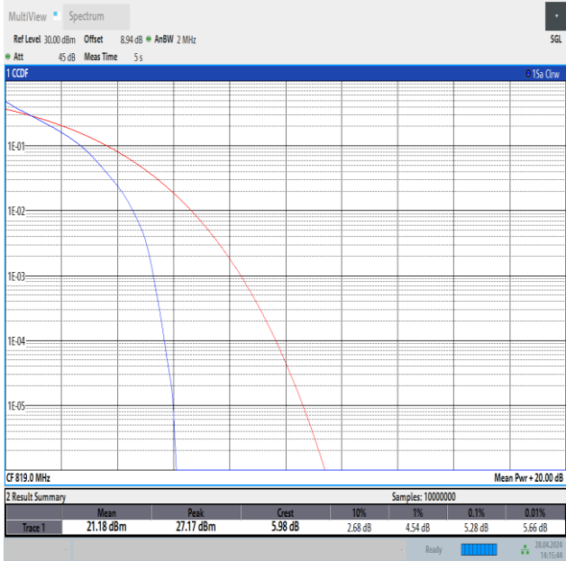
Band26(814-824)-1.4MHz-QPSK-26740-6RB#0-PASS
