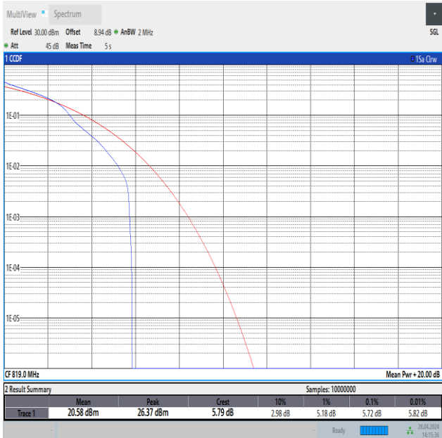
Band26(814-824)-1.4MHz-16QAM-26740-1RB#0-PASS
