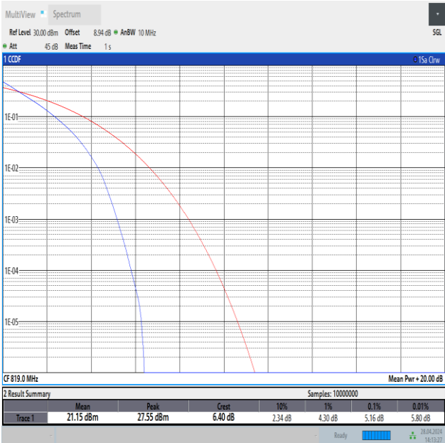
Band26(814-824)-10MHz-QPSK-26740-50RB#0-PASS
