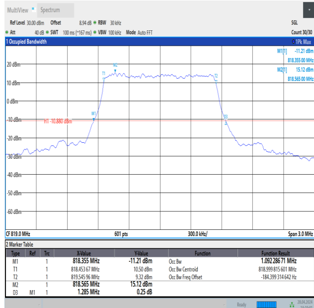
Band26(814-824)-1.4MHz-16QAM-26740-6RB#0-PASS
