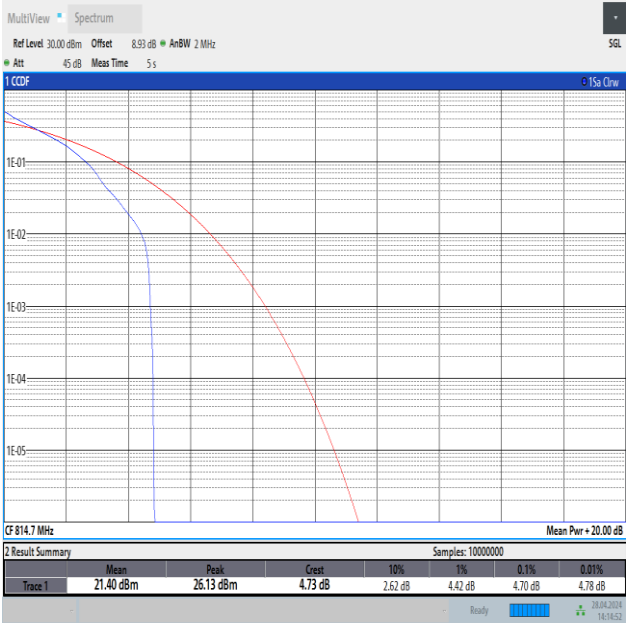
Band26(814-824)-1.4MHz-QPSK-26697-1RB#0-PASS
