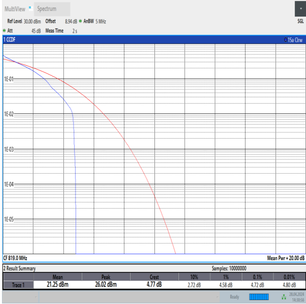
Band26(814-824)-5MHz-QPSK-26740-1RB#0-PASS
