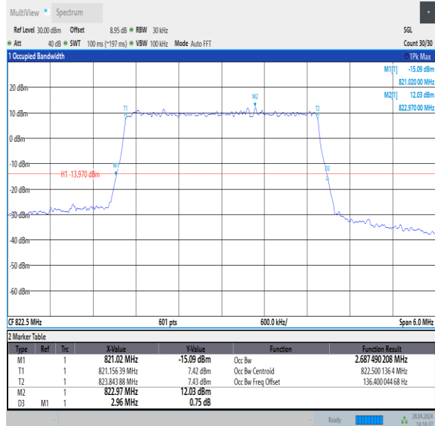
Band26(814-824)-3MHz-16QAM-26775-15RB#0-PASS
