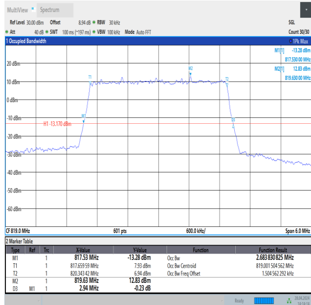
Band26(814-824)-3MHz-16QAM-26740-15RB#0-PASS
