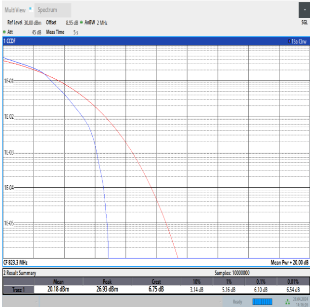
Band26(814-824)-1.4MHz-16QAM-26783-6RB#0-PASS
