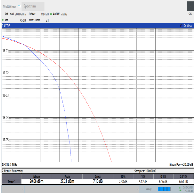
Band26(814-824)-5MHz-16QAM-26715-25RB#0-PASS
