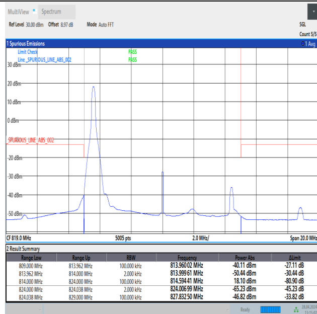
Band26_10MHz_QPSK_26740_1RB#0
