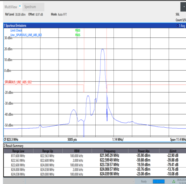
Band26_1.4MHz_QPSK_26783_1RB#5
