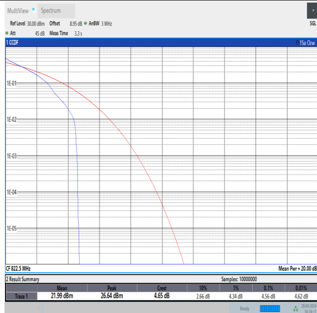
Band26(814-824)-3MHz-QPSK-26775-1RB#0-PASS
