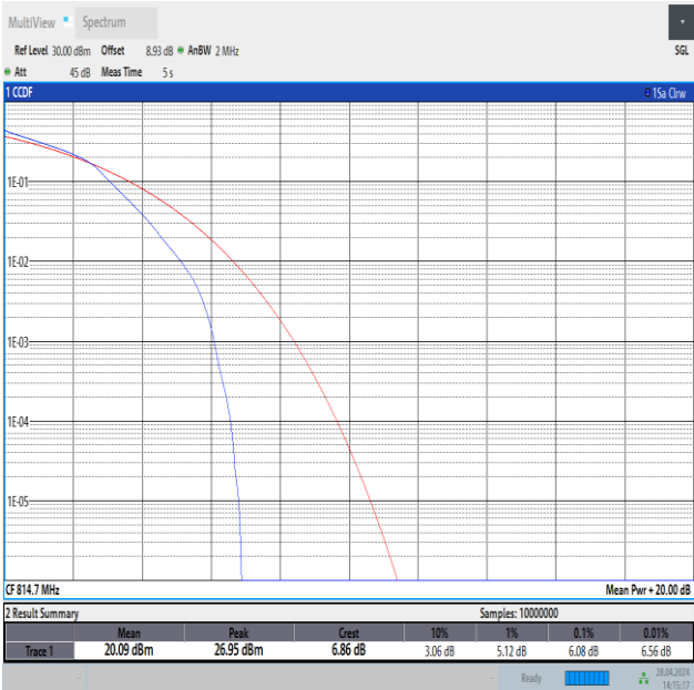
Band26(814-824)-1.4MHz-16QAM-26697-6RB#0-PASS
