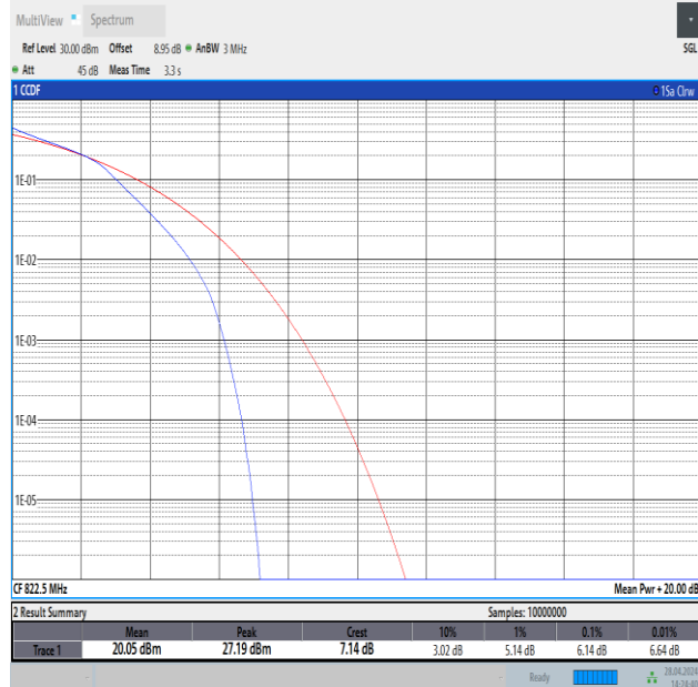
Band26(814-824)-3MHz-16QAM-26775-15RB#0-PASS
