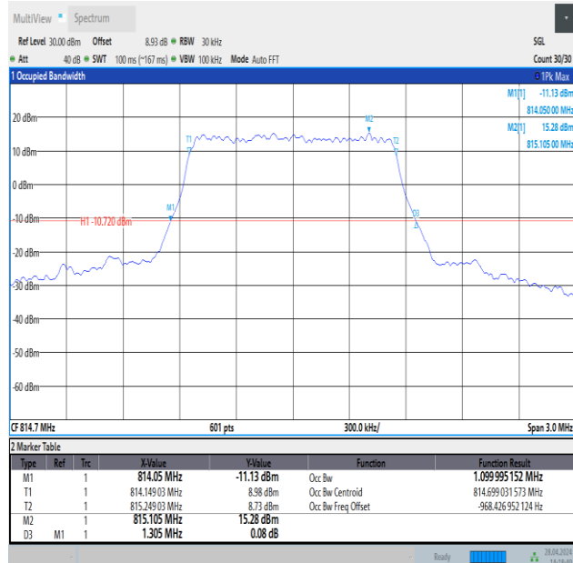
Band26(814-824)-1.4MHz-16QAM-26697-6RB#0-PASS
