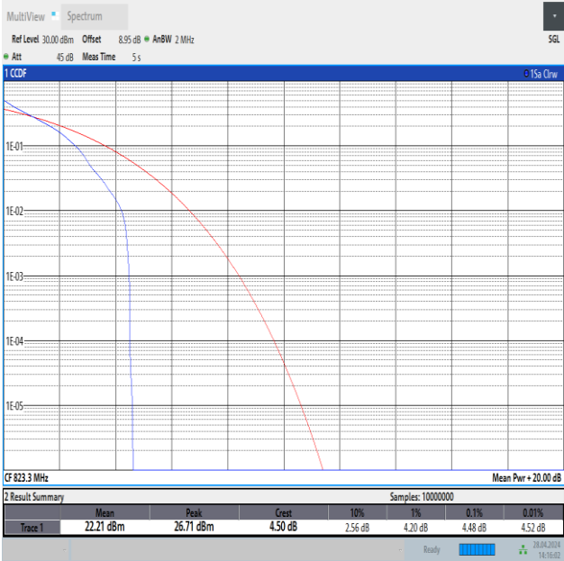
Band26(814-824)-1.4MHz-QPSK-26783-1RB#0-PASS
