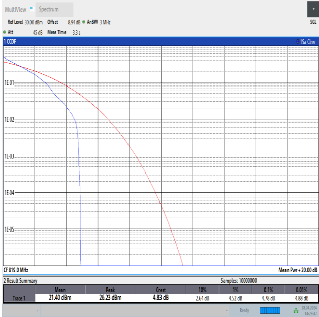
Band26(814-824)-3MHz-QPSK-26740-1RB#0-PASS
