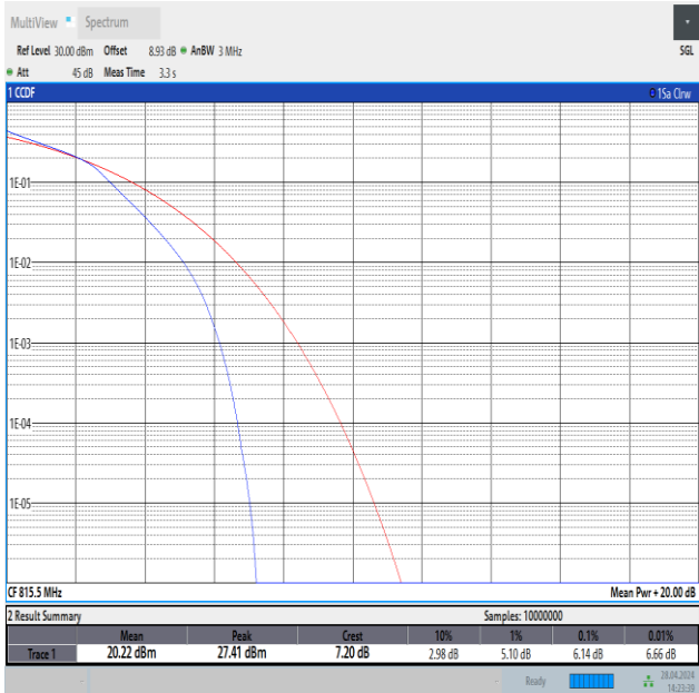
Band26(814-824)-3MHz-16QAM-26705-15RB#0-PASS
