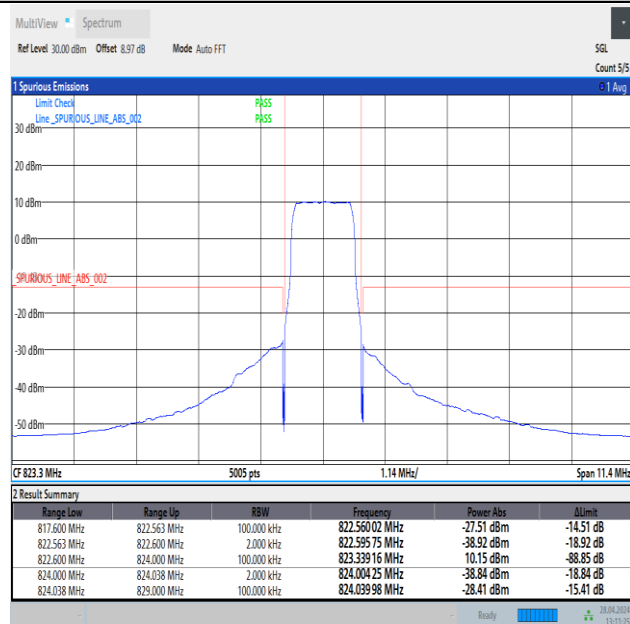
Band26_1.4MHz_16QAM_26783_6RB#0
