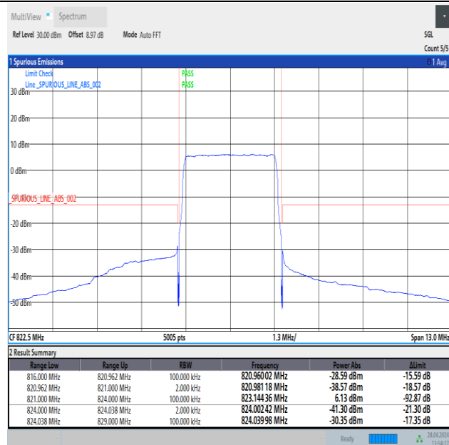
Band26_3MHz_16QAM_26775_15RB#0
