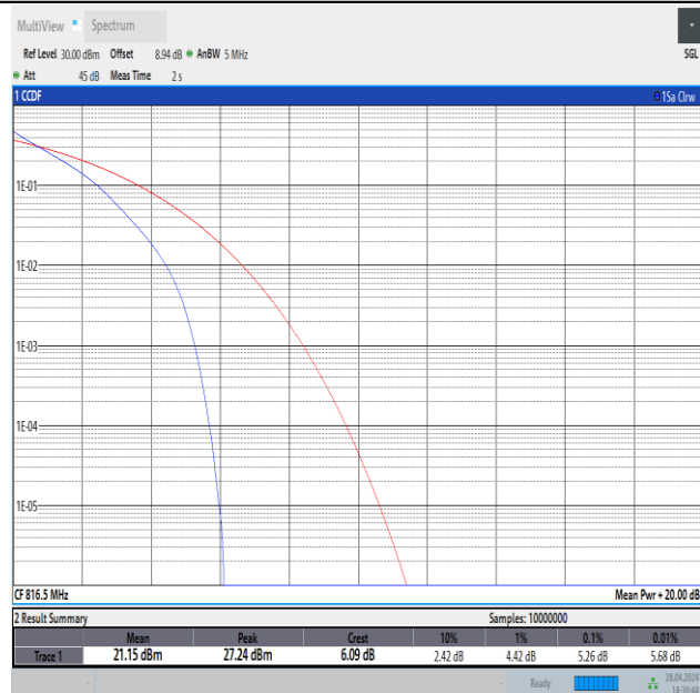
Band26(814-824)-5MHz-QPSK-26715-25RB#0-PASS
