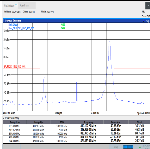
Band26_10MHz_16QAM_26740_1RB#49
