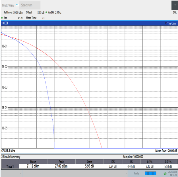
Band26(814-824)-1.4MHz-QPSK-26783-6RB#0-PASS
