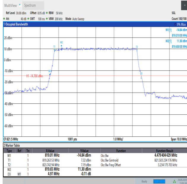
Band26(814-824)-5MHz-16QAM-26765-25RB#0-PASS
