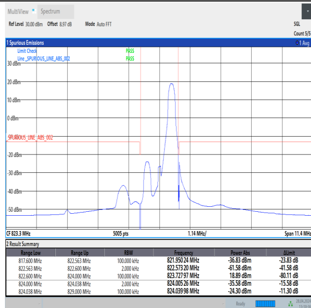
Band26_1.4MHz_16QAM_26783_1RB#5
