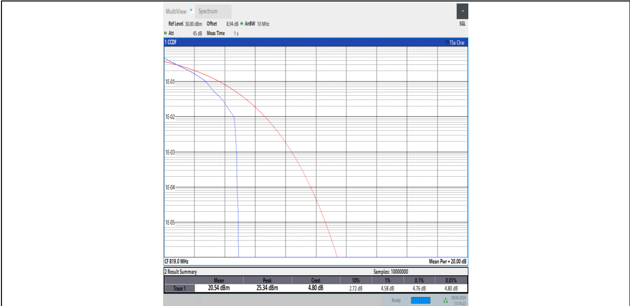
Band26(814-824)-10MHz-QPSK-26740-1RB#0-PASS
