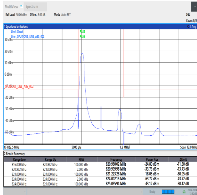
Band26_3MHz_16QAM_26775_1RB#0
