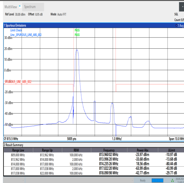
Band26_3MHz_QPSK_26705_1RB#0
