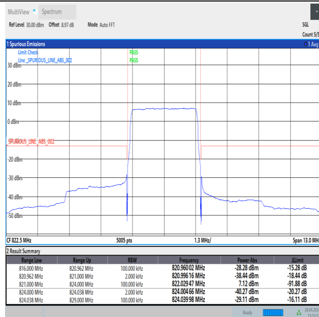
Band26_3MHz_QPSK_26775_15RB#0
