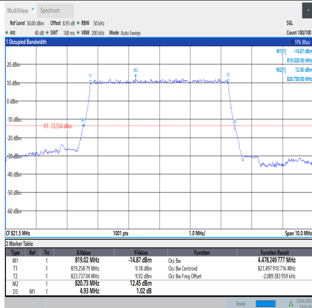
Band26(814-824)-5MHz-QPSK-26765-25RB#0-PASS
