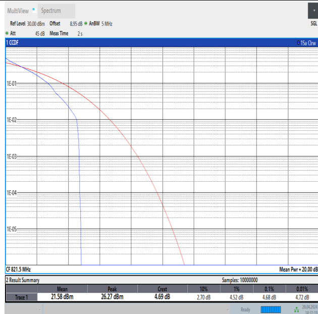
Band26(814-824)-5MHz-QPSK-26765-1RB#0-PASS
