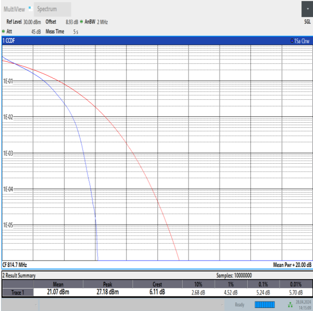
Band26(814-824)-1.4MHz-QPSK-26697-6RB#0-PASS
