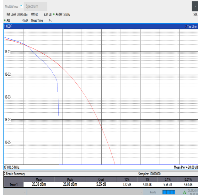
Band26(814-824)-5MHz-16QAM-26715-1RB#0-PASS
