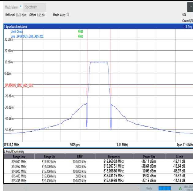
Band26_1.4MHz_16QAM_26697_6RB#0
