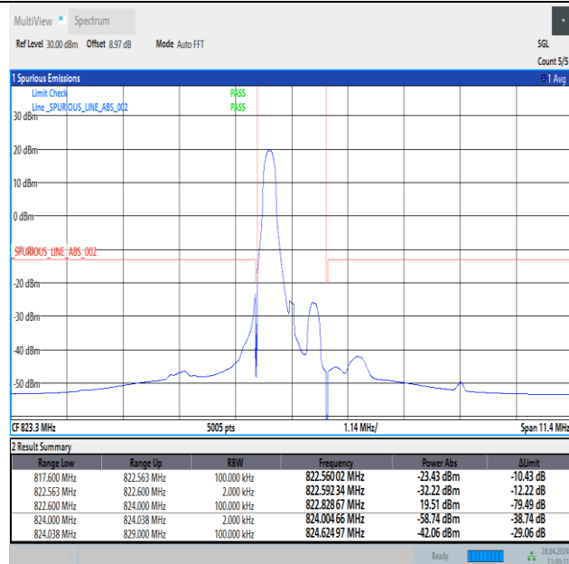
Band26_1.4MHz_QPSK_26783_1RB#0
