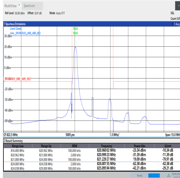
Band26_3MHz_QPSK_26775_1RB#0
