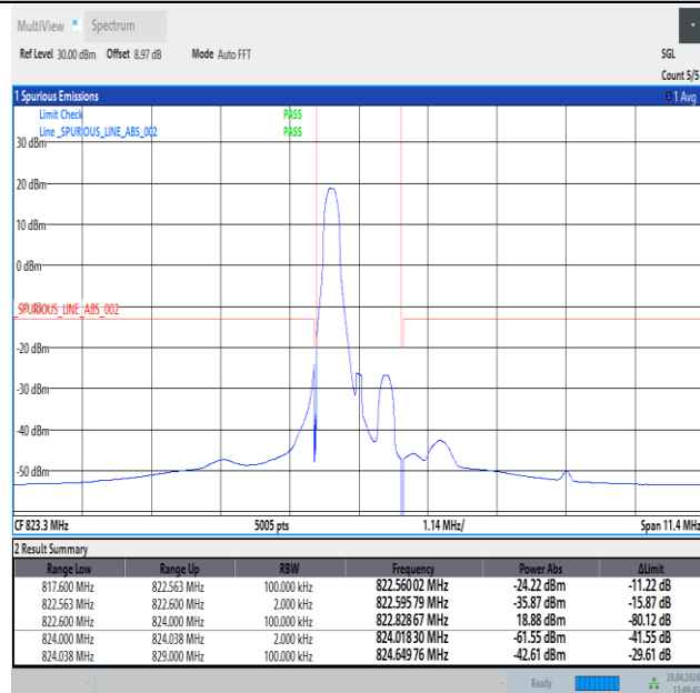
Band26_1.4MHz_16QAM_26783_1RB#0
