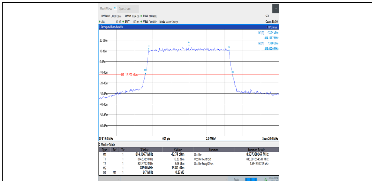
Band26(814-824)-10MHz-QPSK-26740-50RB#0-PASS
