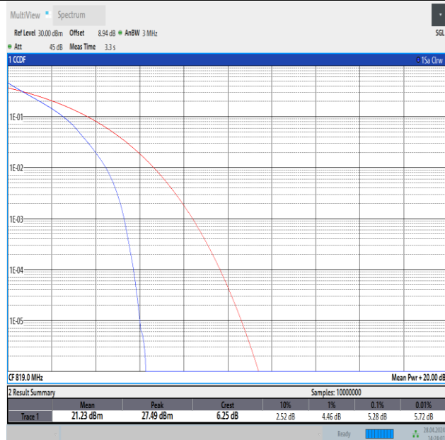
Band26(814-824)-3MHz-QPSK-26740-15RB#0-PASS
