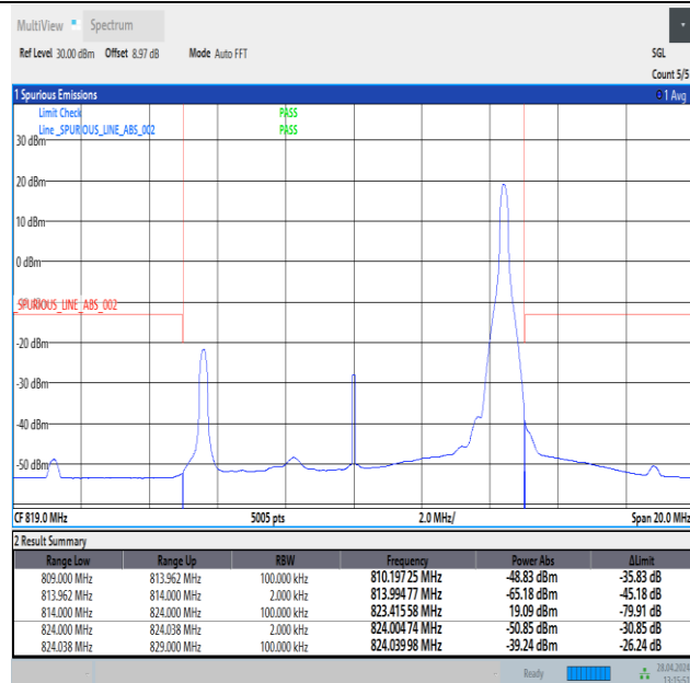
Band26_10MHz_QPSK_26740_1RB#49
