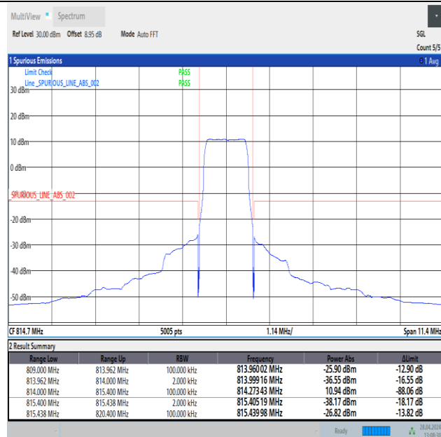
Band26_1.4MHz_QPSK_26697_6RB#0
