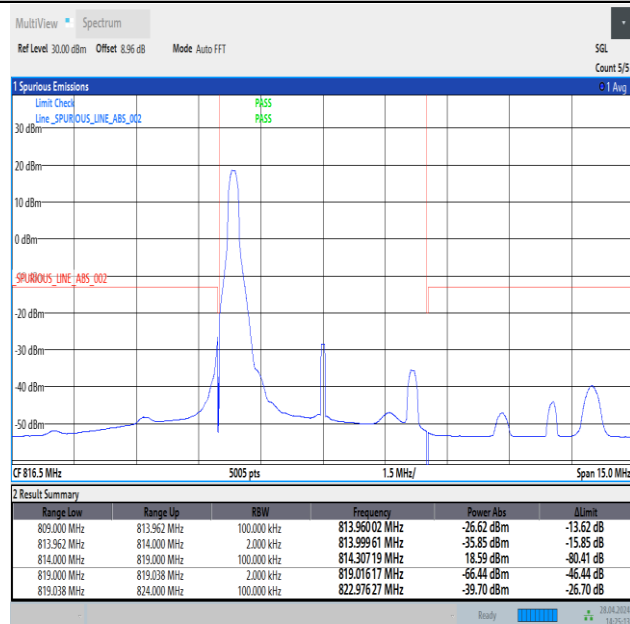
Band26_5MHz_QPSK_26715_1RB#0
