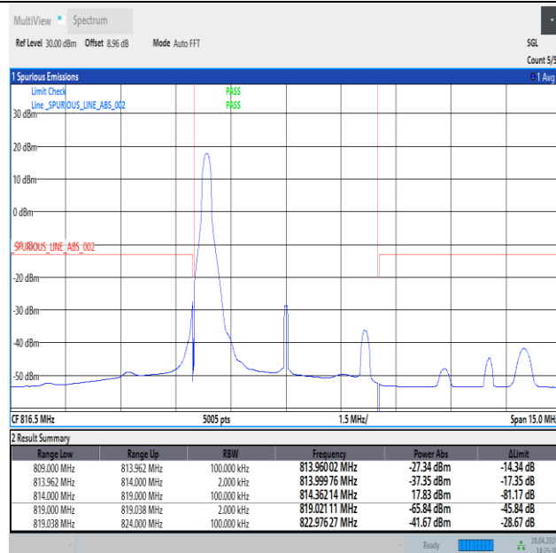
Band26_5MHz_16QAM_26715_1RB#0
