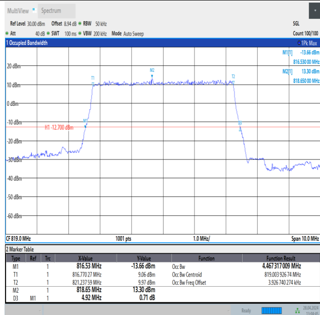
Band26(814-824)-5MHz-QPSK-26740-25RB#0-PASS
