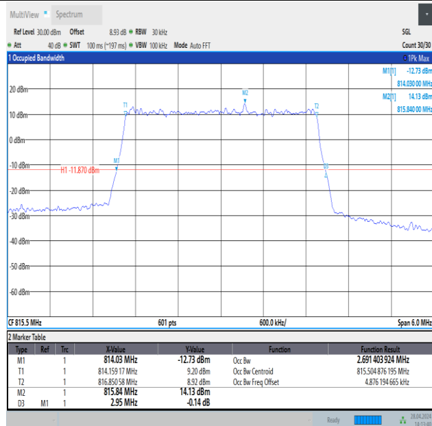
Band26(814-824)-3MHz-QPSK-26705-15RB#0-PASS
