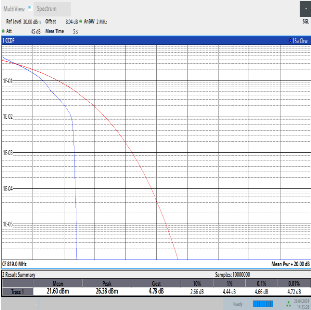
Band26(814-824)-1.4MHz-QPSK-26740-1RB#0-PASS
