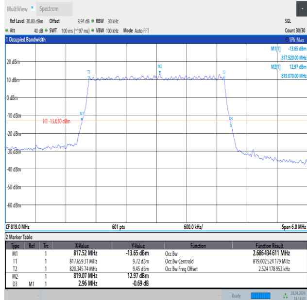
Band26(814-824)-3MHz-QPSK-26740-15RB#0-PASS
