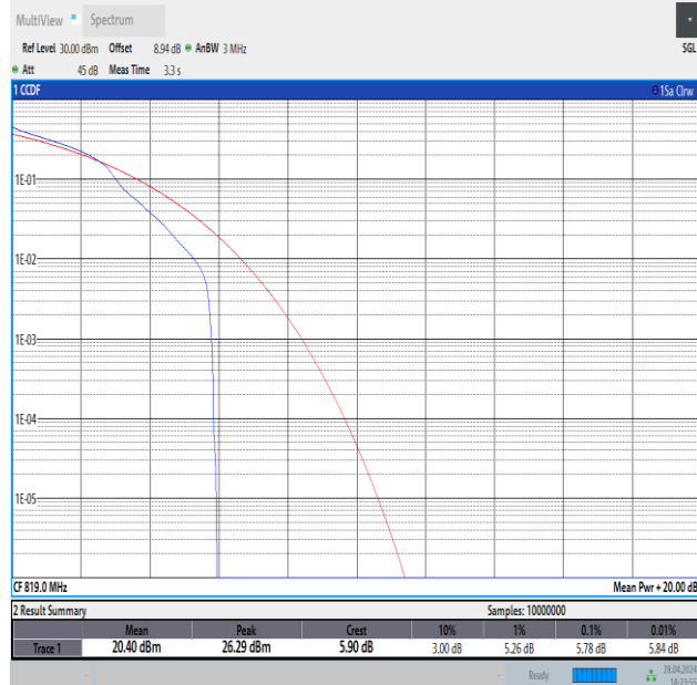
Band26(814-824)-3MHz-16QAM-26740-1RB#0-PASS
