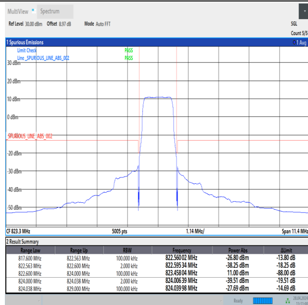
Band26_1.4MHz_QPSK_26783_6RB#0
