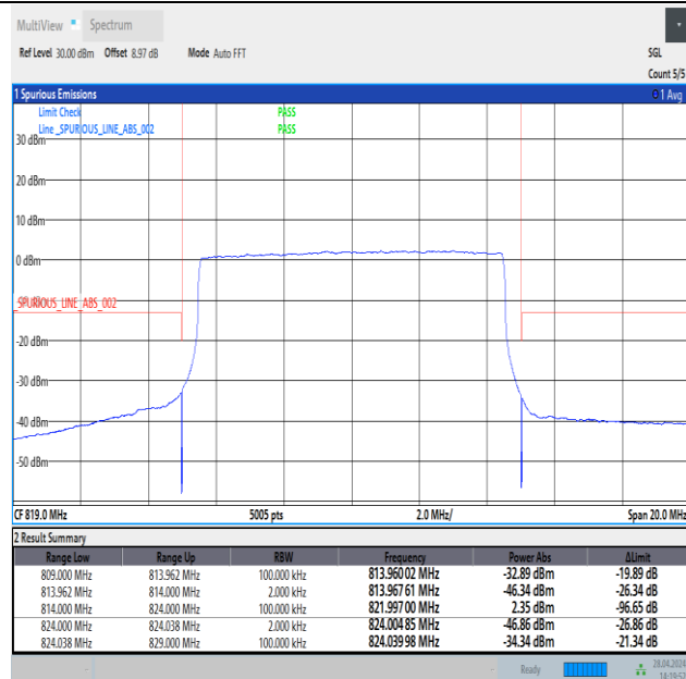
Band26_10MHz_QPSK_26740_50RB#0
