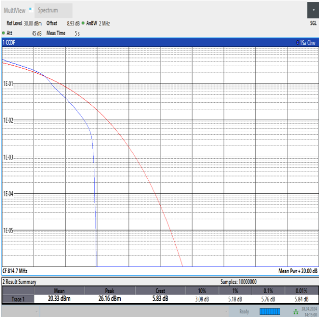
Band26(814-824)-1.4MHz-16QAM-26697-1RB#0-PASS
