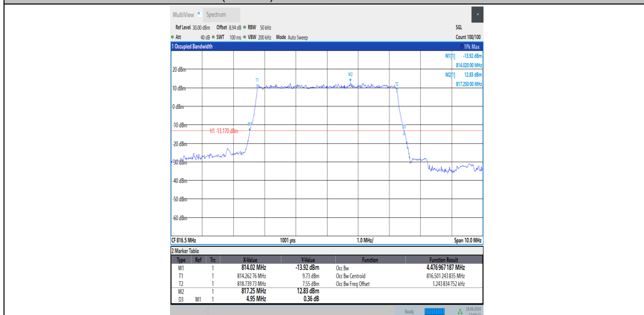
Band26(814-824)-5MHz-QPSK-26715-25RB#0-PASS
