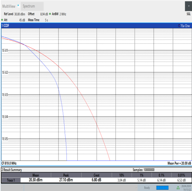
Band26(814-824)-1.4MHz-16QAM-26740-6RB#0-PASS
