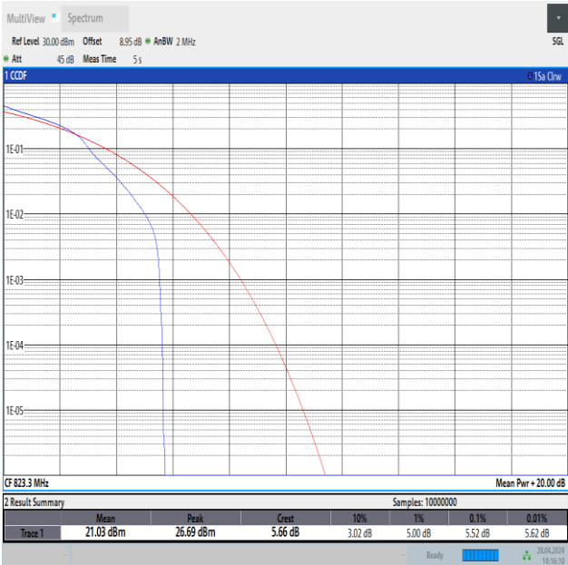
Band26(814-824)-1.4MHz-16QAM-26783-1RB#0-PASS
