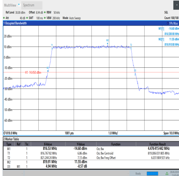
Band26(814-824)-5MHz-16QAM-26740-25RB#0-PASS
