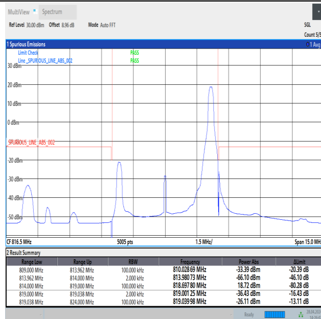
Band26_5MHz_QPSK_26715_1RB#24
