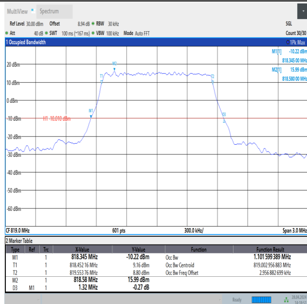
Band26(814-824)-1.4MHz-QPSK-26740-6RB#0-PASS
