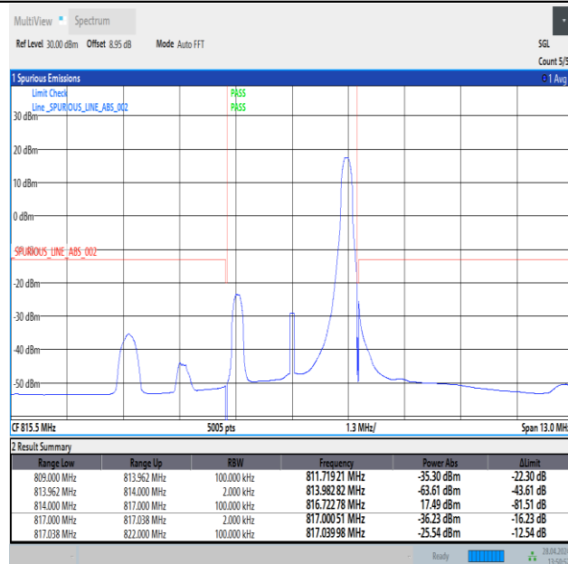
Band26_3MHz_16QAM_26705_1RB#14
