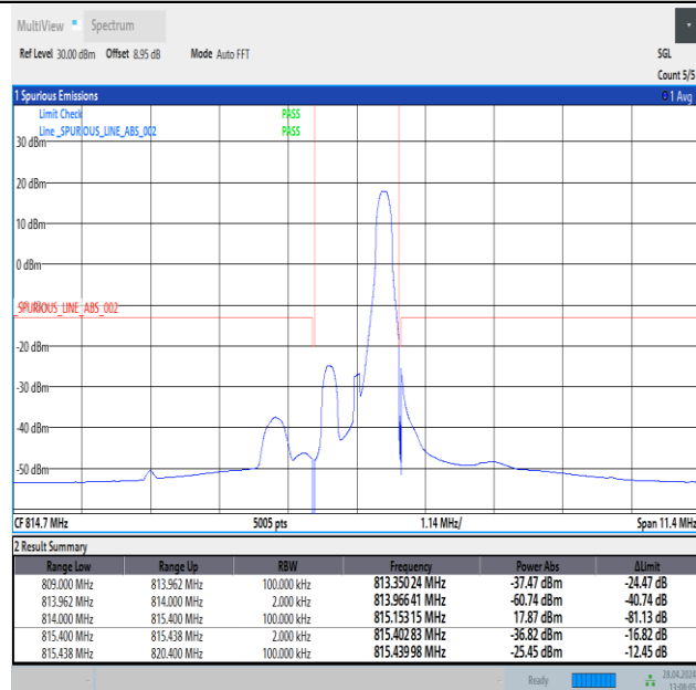
Band26_1.4MHz_16QAM_26697_1RB#5
