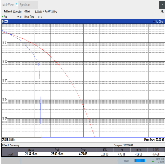
Band26(814-824)-3MHz-QPSK-26705-1RB#0-PASS
