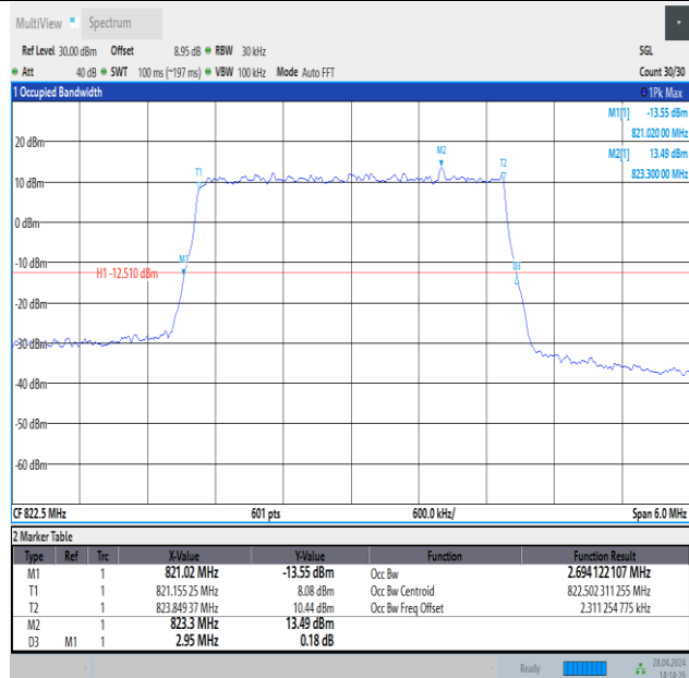
Band26(814-824)-3MHz-QPSK-26775-15RB#0-PASS
