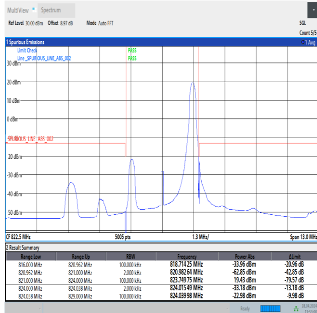
Band26_3MHz_QPSK_26775_1RB#14
