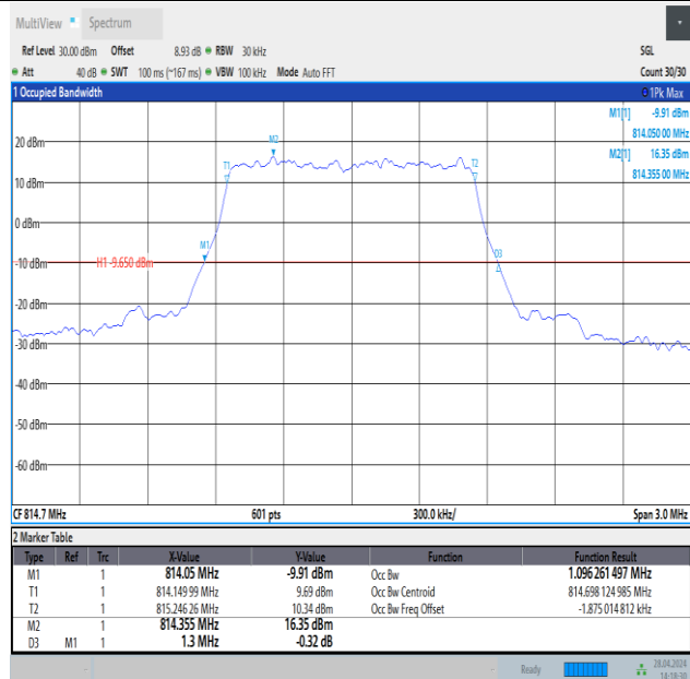
Band26(814-824)-1.4MHz-QPSK-26697-6RB#0-PASS
