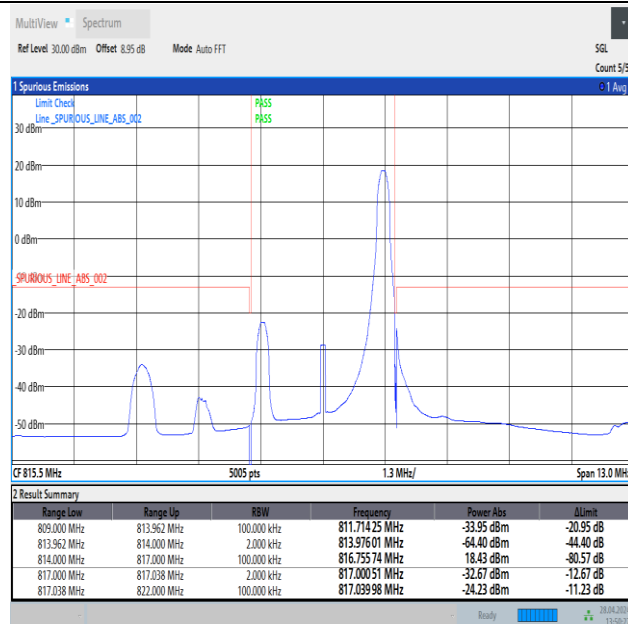
Band26_3MHz_QPSK_26705_1RB#14
