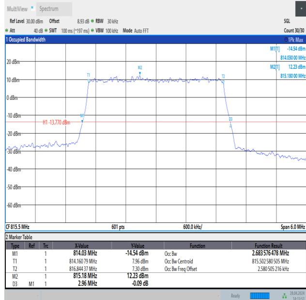
Band26(814-824)-3MHz-16QAM-26705-15RB#0-PASS
