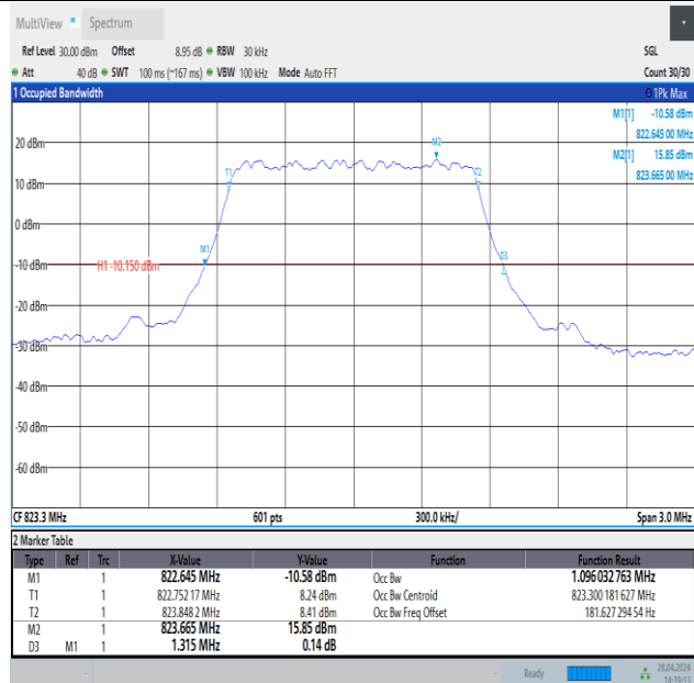
Band26(814-824)-1.4MHz-QPSK-26783-6RB#0-PASS
