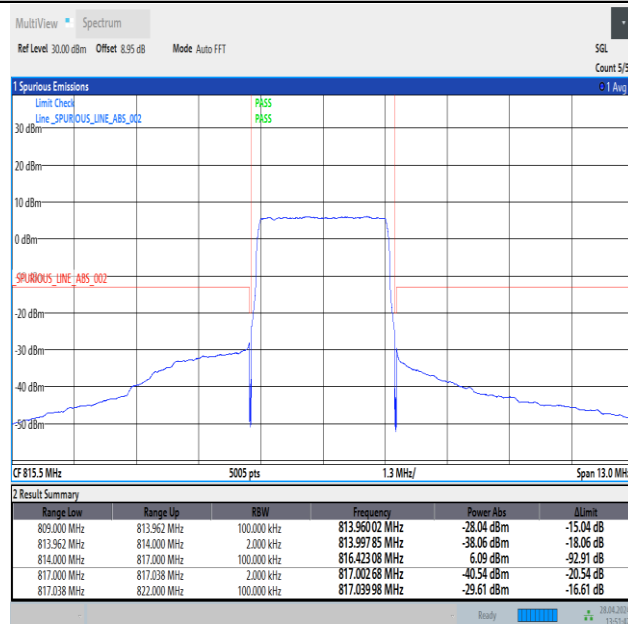
Band26_3MHz_16QAM_26705_15RB#0
