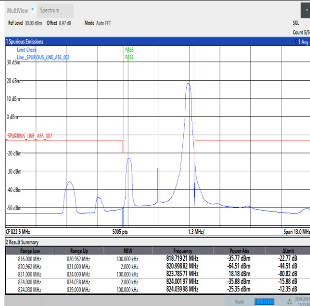
Band26_3MHz_16QAM_26775_1RB#14
