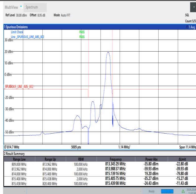
Band26_1.4MHz_QPSK_26697_1RB#5
