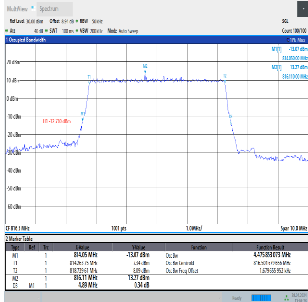
Band26(814-824)-5MHz-16QAM-26715-25RB#0-PASS
