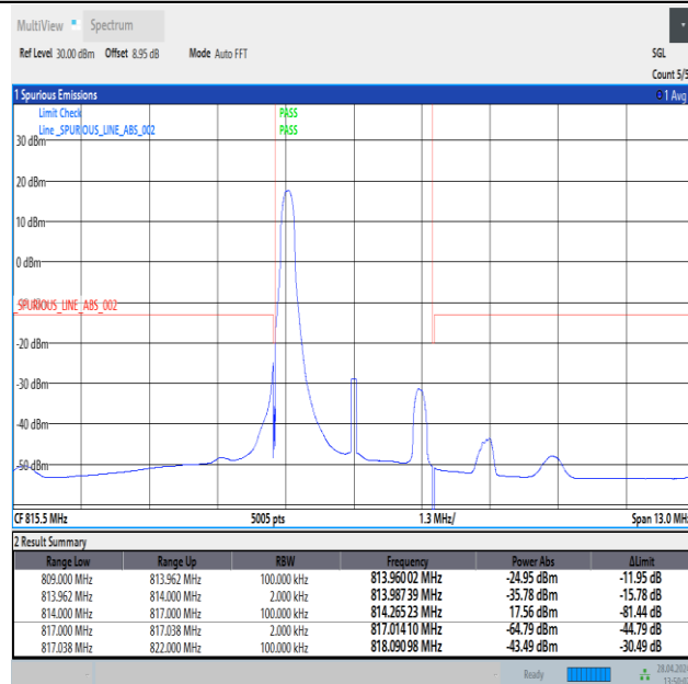
Band26_3MHz_16QAM_26705_1RB#0
