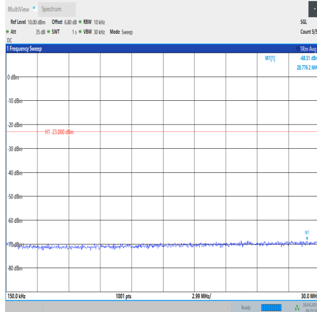
Band12_3MHz_16QAM_23095_1RB#0_0.15~30_0.15~30
