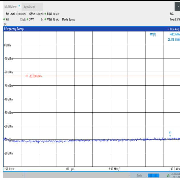
Band12_3MHz_QPSK_23025_1RB#14_0.15~30_0.15~30
