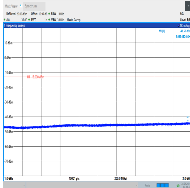
Band12_3MHz_QPSK_23095_15RB#0_1000~3000_1000~3000
