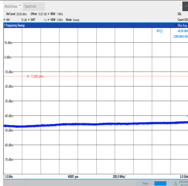
Band12_3MHz_16QAM_23095_1RB#14_1000~3000_1000~3000
