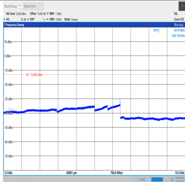
Band12_3MHz_QPSK_23095_15RB#0_3000~10000_3000~10000
