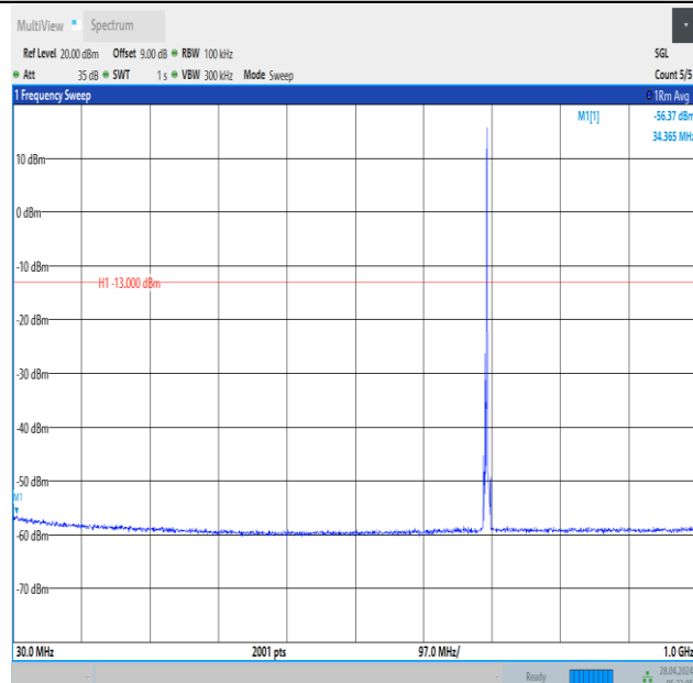
Band12_3MHz_QPSK_23025_1RB#14_30~1000_30~1000
