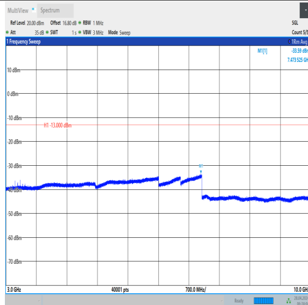
Band12_3MHz_QPSK_23025_15RB#0_3000~10000_3000~10000
