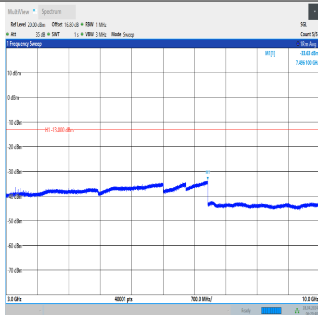
Band12_3MHz_16QAM_23095_15RB#0_3000~10000_3000~10000
