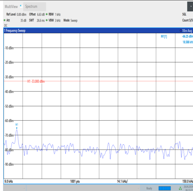
Band12_3MHz_QPSK_23165_1RB#0_0.009~0.15_0.009~0.15
