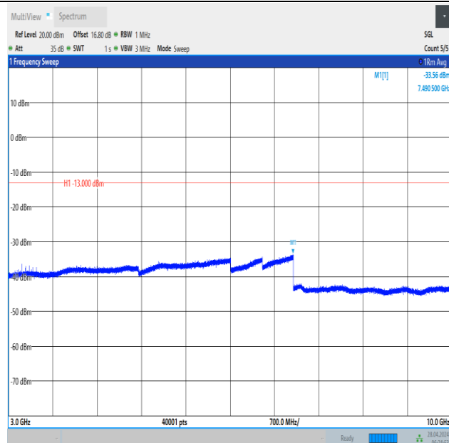
Band12_3MHz_16QAM_23025_15RB#0_3000~10000_3000~10000
