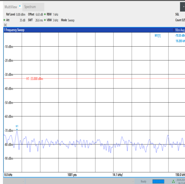
Band12_3MHz_16QAM_23095_1RB#0_0.009~0.15_0.009~0.15
