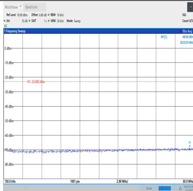
Band12_10MHz_16QAM_23130_1RB#0_0.15~30_0.15~30
