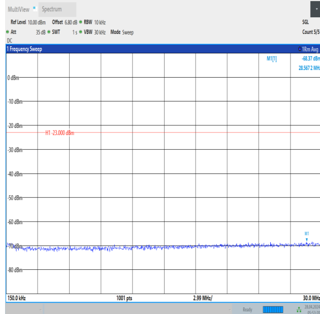
Band12_10MHz_QPSK_23130_1RB#0_0.15~30_0.15~30
