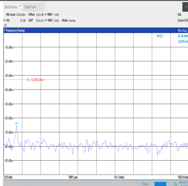
Band12_10MHz_QPSK_23130_1RB#0_0.009~0.15_0.009~0.15
