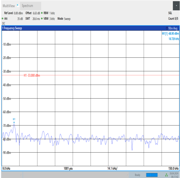
Band12_10MHz_QPSK_23060_50RB#0_0.009~0.15_0.009~0.15
