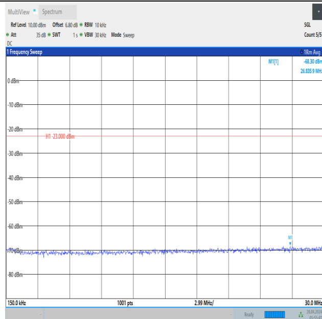
Band12_10MHz_16QAM_23130_1RB#49_0.15~30_0.15~30
