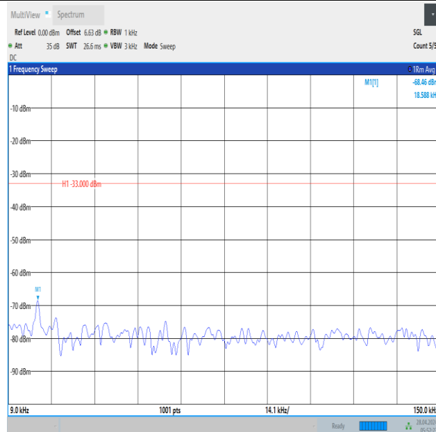
Band12_10MHz_16QAM_23095_1RB#49_0.009~0.15_0.009~0.15
