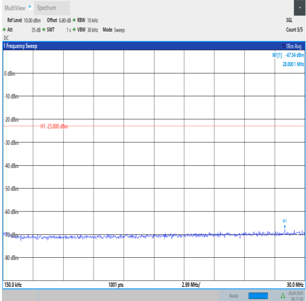
Band12_10MHz_QPSK_23060_50RB#0_0.15~30_0.15~30
