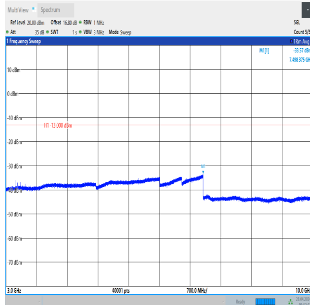
Band12_10MHz_QPSK_23095_1RB#49_3000~10000_3000~10000
