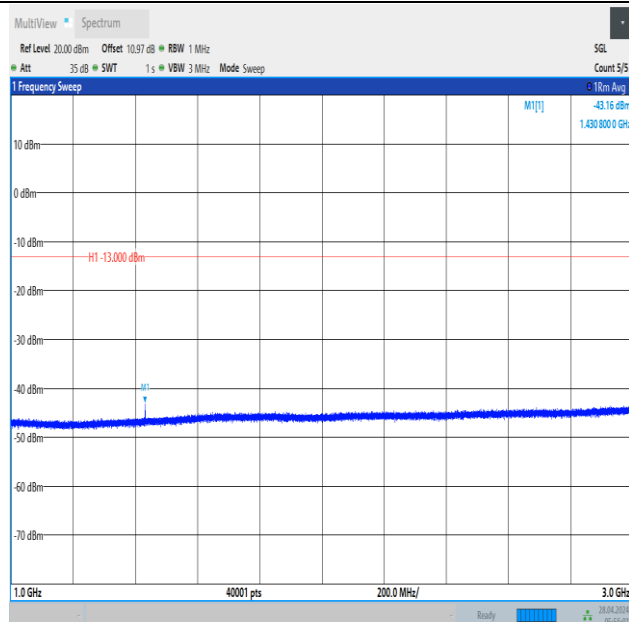
Band12_10MHz_16QAM_23130_1RB#49_1000~3000_1000~3000
