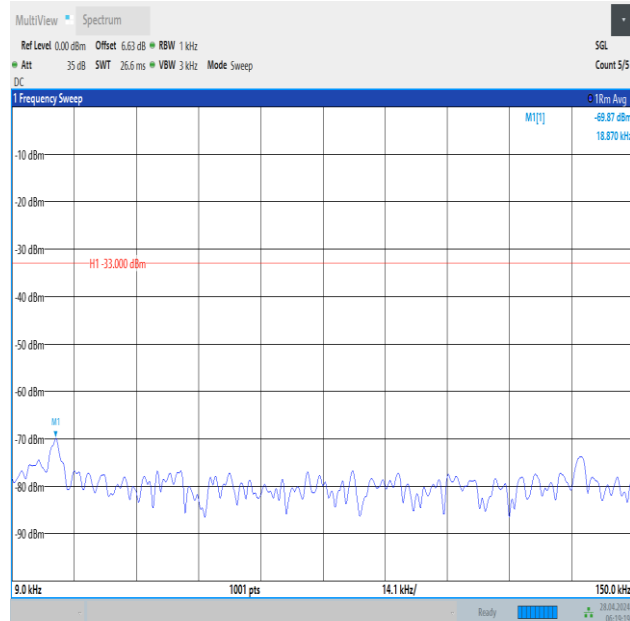
Band12_10MHz_QPSK_23130_50RB#0_0.009~0.15_0.009~0.15
