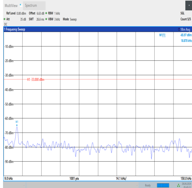
Band12_5MHz_16QAM_23155_25RB#0_0.009~0.15_0.009~0.15
