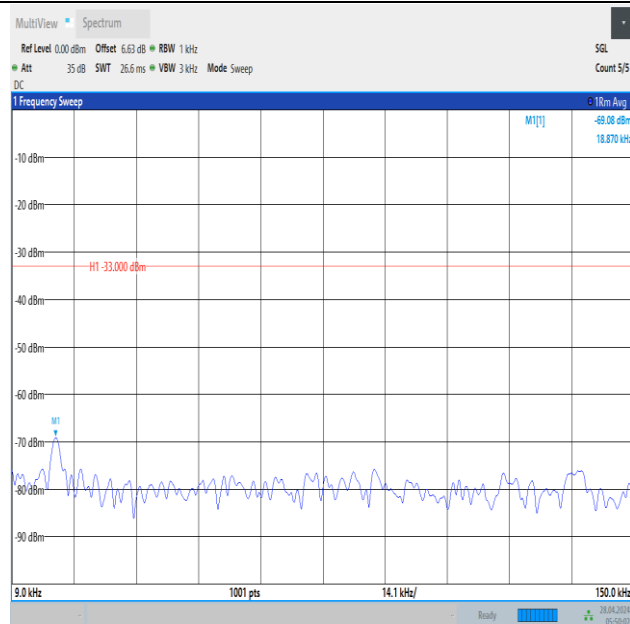
Band12_10MHz_QPSK_23095_1RB#0_0.009~0.15_0.009~0.15
