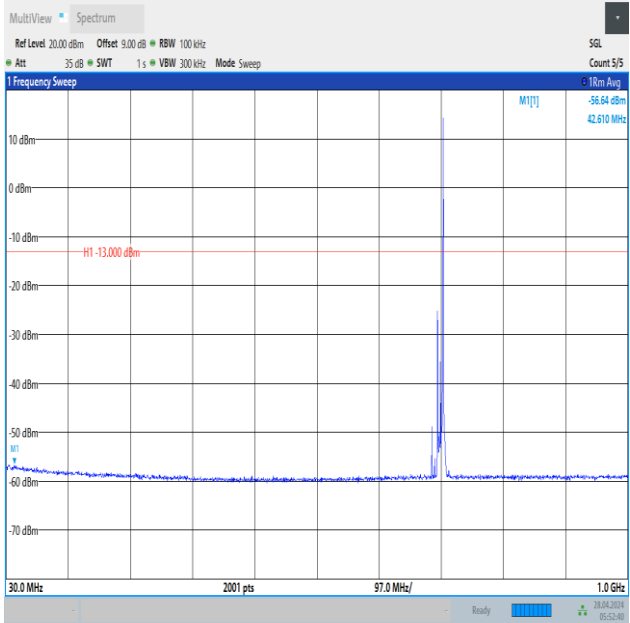
Band12_10MHz_16QAM_23095_1RB#49_30~1000_30~1000
