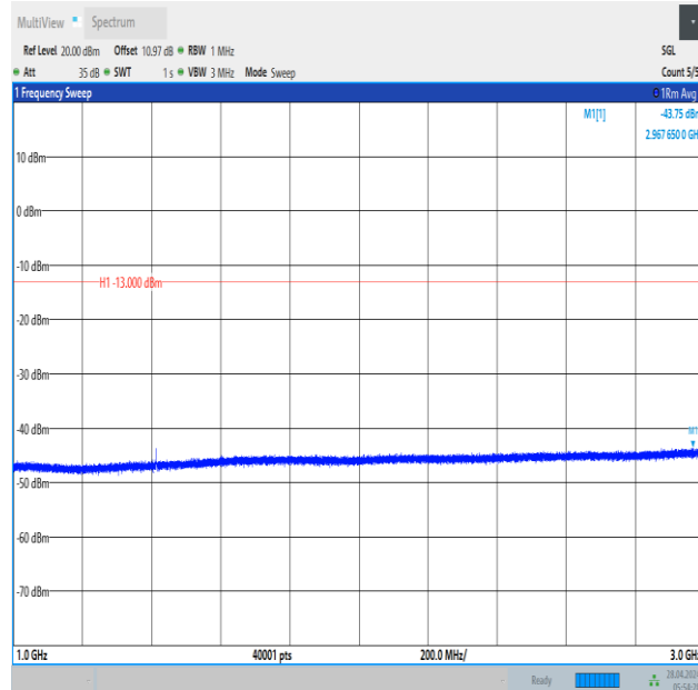
Band12_10MHz_16QAM_23130_1RB#0_1000~3000_1000~3000
