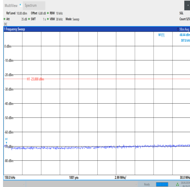
Band12_10MHz_QPSK_23130_50RB#0_0.15~30_0.15~30
