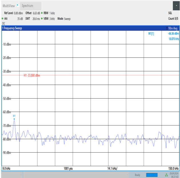
Band12_3MHz_16QAM_23025_1RB#0_0.009~0.15_0.009~0.15
