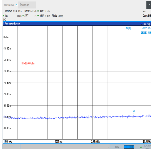
Band12_10MHz_16QAM_23060_1RB#49_0.15~30_0.15~30
