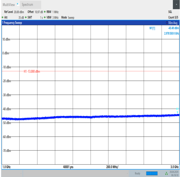
Band12_10MHz_QPSK_23060_50RB#0_1000~3000_1000~3000
