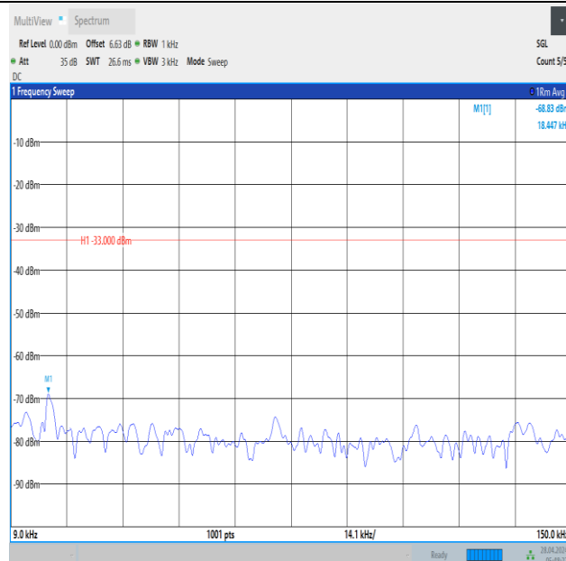
Band12_10MHz_QPSK_23060_1RB#49_0.009~0.15_0.009~0.15
