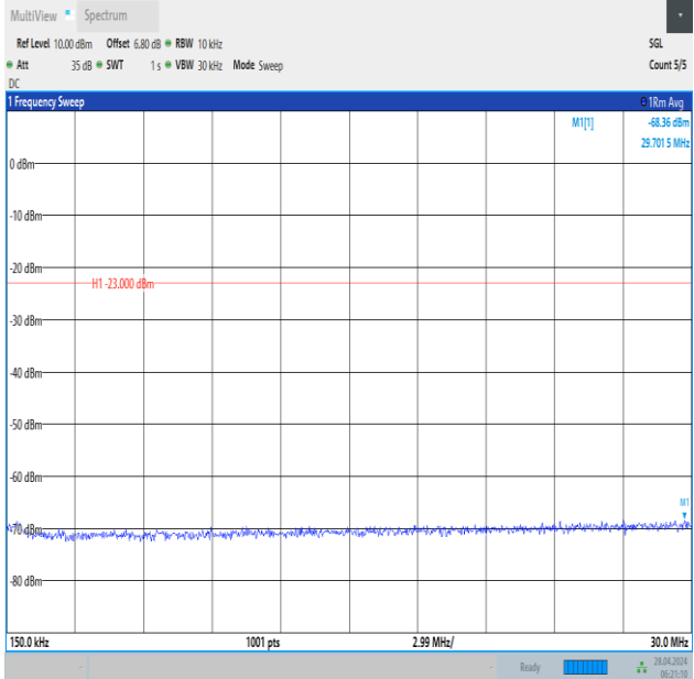
Band12_3MHz_16QAM_23025_1RB#0_0.15~30_0.15~30
