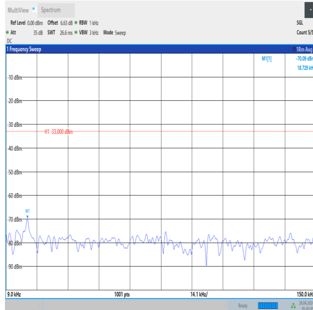
Band12_5MHz_QPSK_23155_25RB#0_0.009~0.15_0.009~0.15
