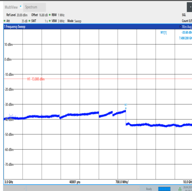
Band12_10MHz_QPSK_23060_50RB#0_3000~10000_3000~10000
