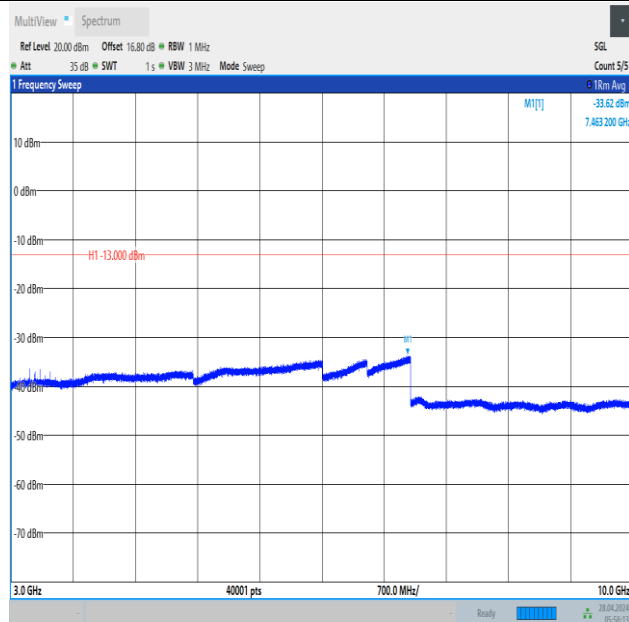
Band12_10MHz_16QAM_23130_1RB#49_3000~10000_3000~10000
