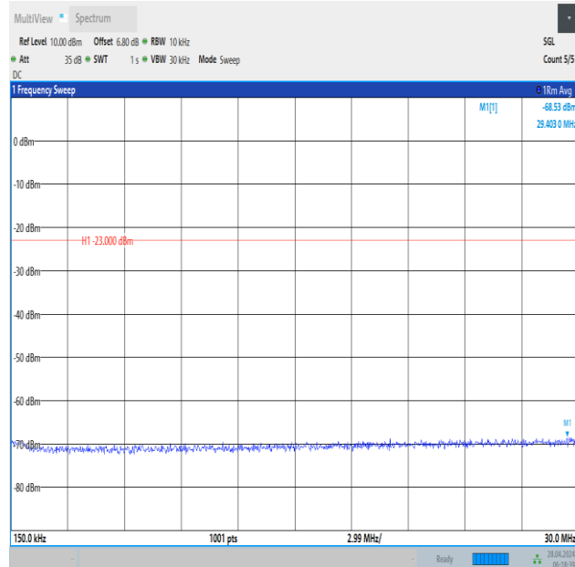
Band12_10MHz_QPSK_23095_50RB#0_0.15~30_0.15~30
