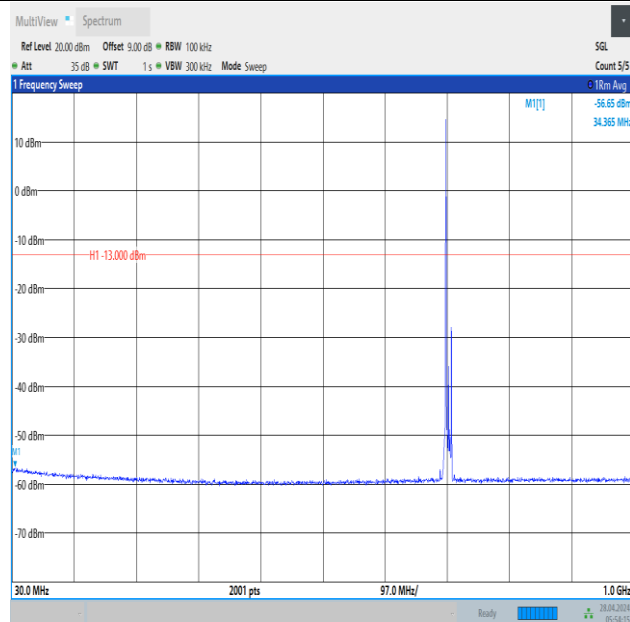
Band12_10MHz_16QAM_23130_1RB#0_30~1000_30~1000
