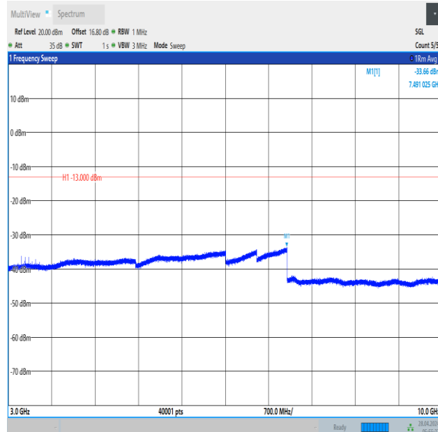
Band12_10MHz_QPSK_23130_1RB#49_3000~10000_3000~10000
