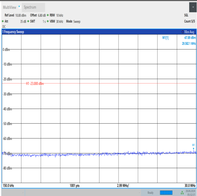
Band12_10MHz_16QAM_23095_1RB#49_0.15~30_0.15~30
