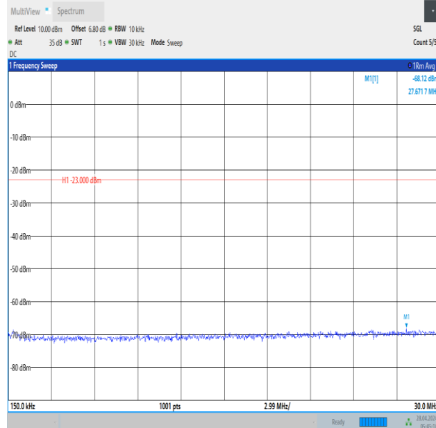
Band12_5MHz_QPSK_23155_25RB#0_0.15~30_0.15~30
