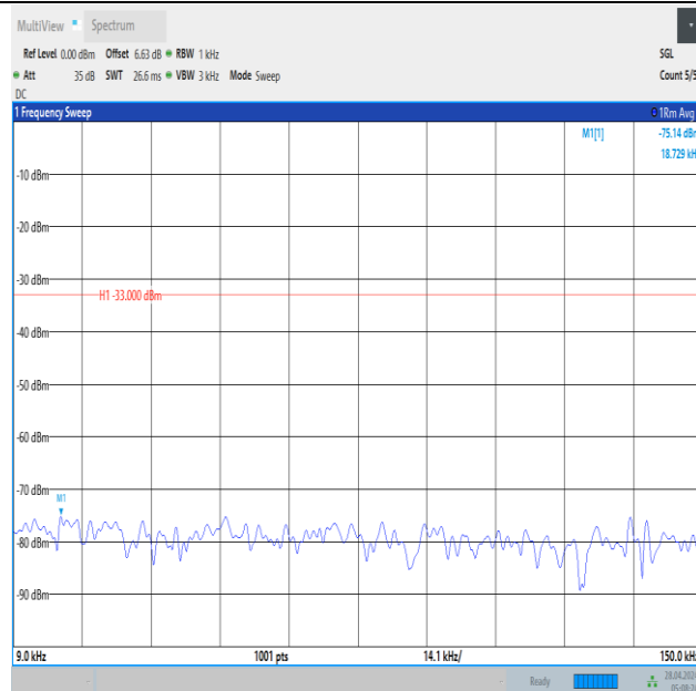
Band12_1.4MHz_QPSK_23017_6RB#0_0.009~0.15_0.009~0.15
