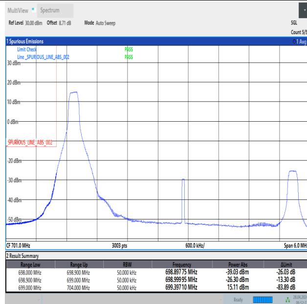
Band12_5MHz_16QAM_23035_1RB#0
