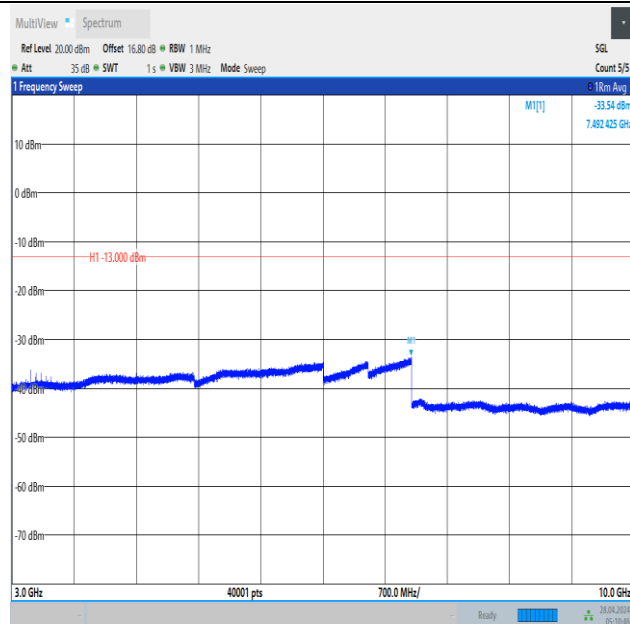
Band12_1.4MHz_QPSK_23095_1RB#0_3000~10000_3000~10000
