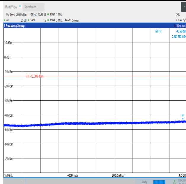
Band12_1.4MHz_16QAM_23017_1RB#0_1000~3000_1000~3000
