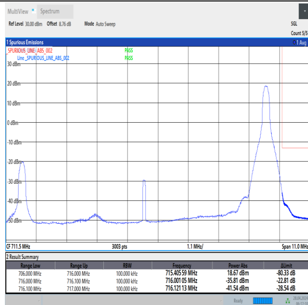
Band12_10MHz_QPSK_23130_1RB#49
