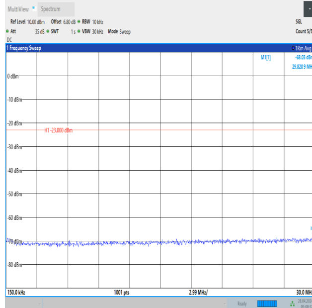
Band12_1.4MHz_QPSK_23017_6RB#0_0.15~30_0.15~30
