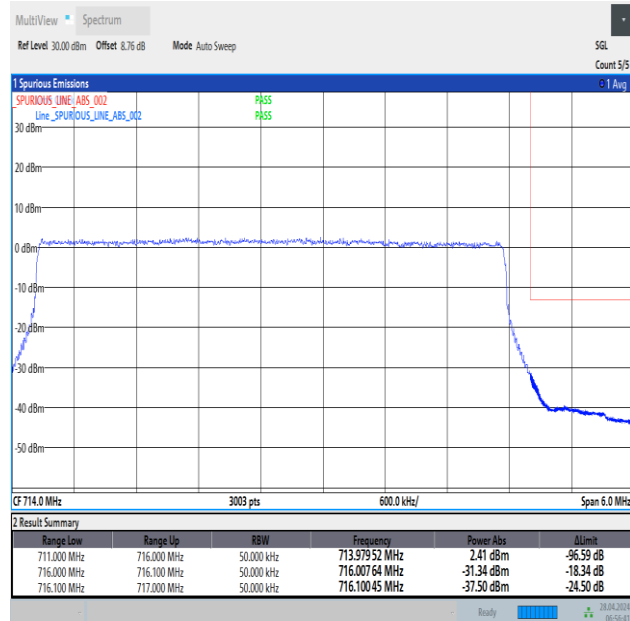
Band12_5MHz_QPSK_23155_25RB#0
