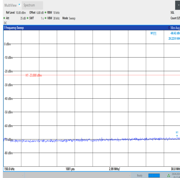
Band12_1.4MHz_QPSK_23095_1RB#5_0.15~30_0.15~30
