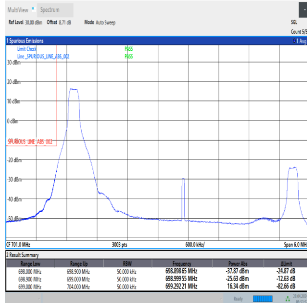
Band12_5MHz_QPSK_23035_1RB#0
