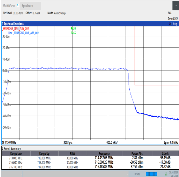
Band12_3MHz_QPSK_23165_15RB#0
