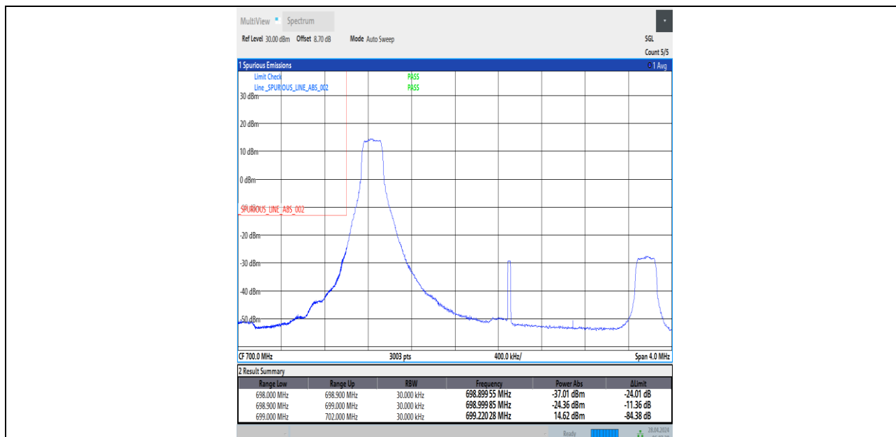
Band12_3MHz_QPSK_23025_1RB#0
