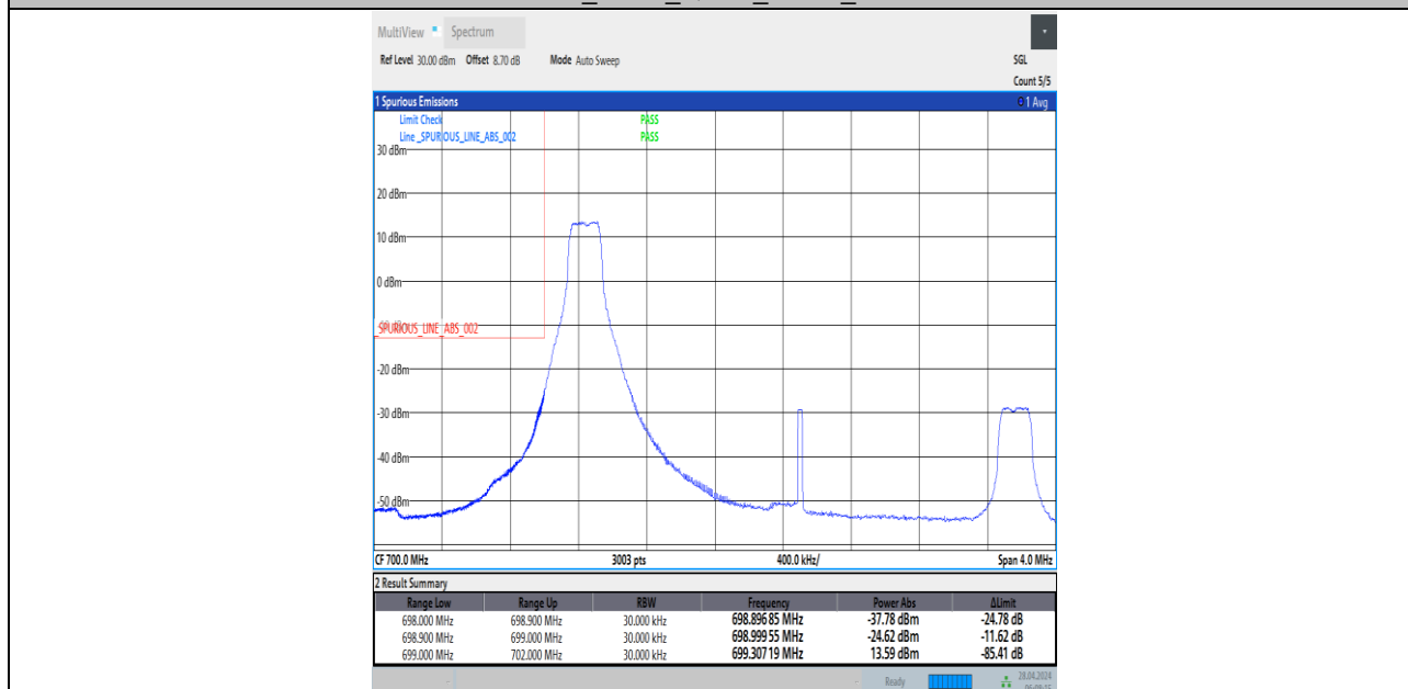
Band12_3MHz_16QAM_23025_1RB#0
