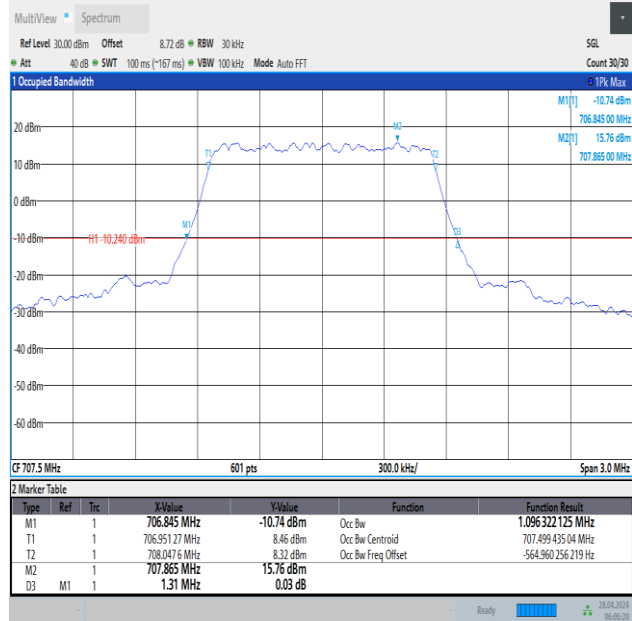
Band12-1.4MHz-QPSK-23095-6RB#0-PASS
