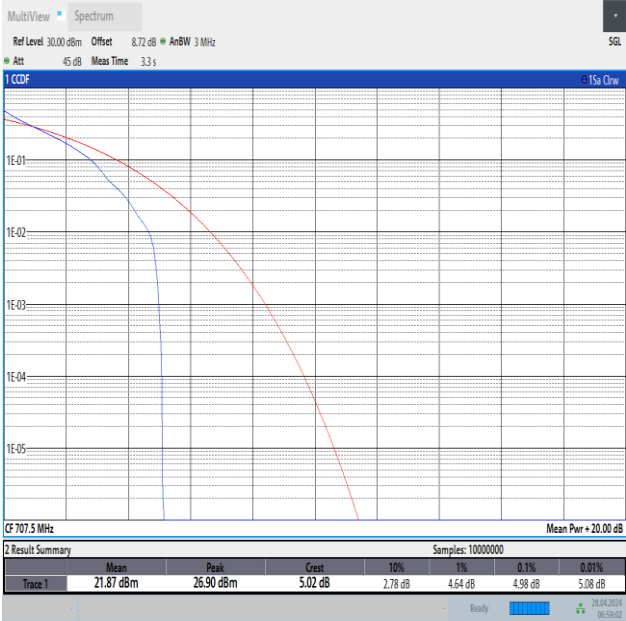
Band12-3MHz-QPSK-23095-1RB#0-PASS
