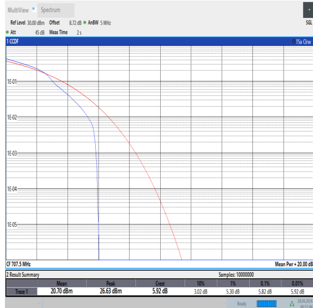
Band12-5MHz-16QAM-23095-1RB#0-PASS
