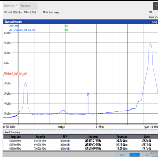
Band12_10MHz_QPSK_23060_1RB#49
