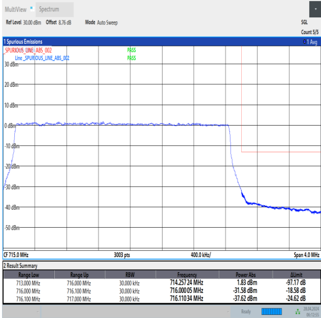
Band12_3MHz_16QAM_23165_15RB#0
