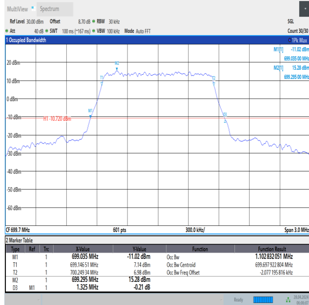
Band12-1.4MHz-16QAM-23017-6RB#0-PASS
