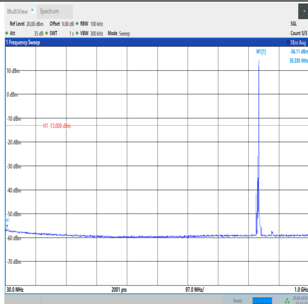
Band5_5MHz_16QAM_20525_1RB#24_30~1000_30~1000
