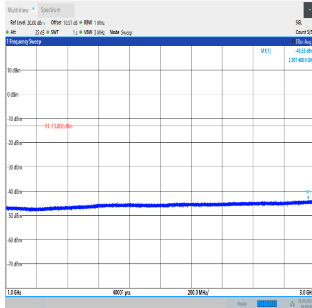
Band5_5MHz_QPSK_20525_1RB#0_1000~3000_1000~3000
