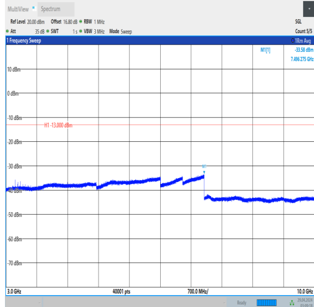
Band5_5MHz_QPSK_20525_1RB#0_3000~10000_3000~10000
