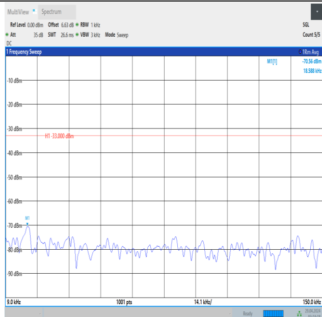
Band5_5MHz_16QAM_20625_1RB#0_0.009~0.15_0.009~0.15
