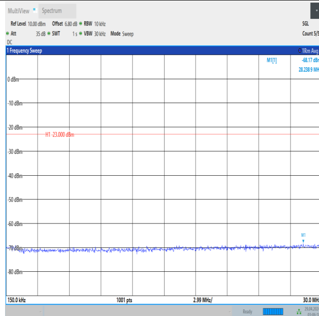
Band5_5MHz_16QAM_20425_1RB#24_0.15~30_0.15~30
