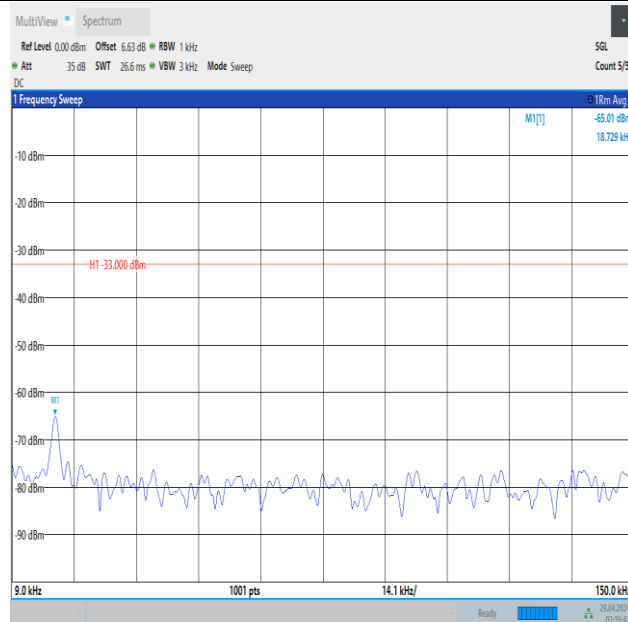
Band5_5MHz_QPSK_20625_25RB#0_0.009~0.15_0.009~0.15
