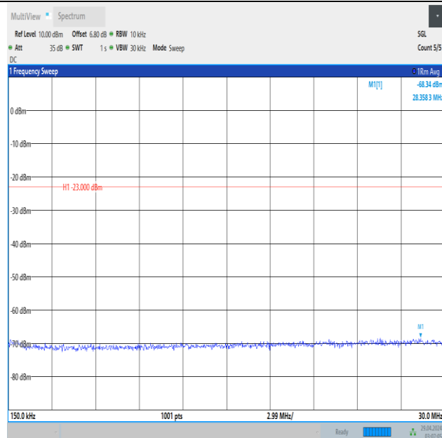
Band5_5MHz_QPSK_20425_25RB#0_0.15~30_0.15~30
