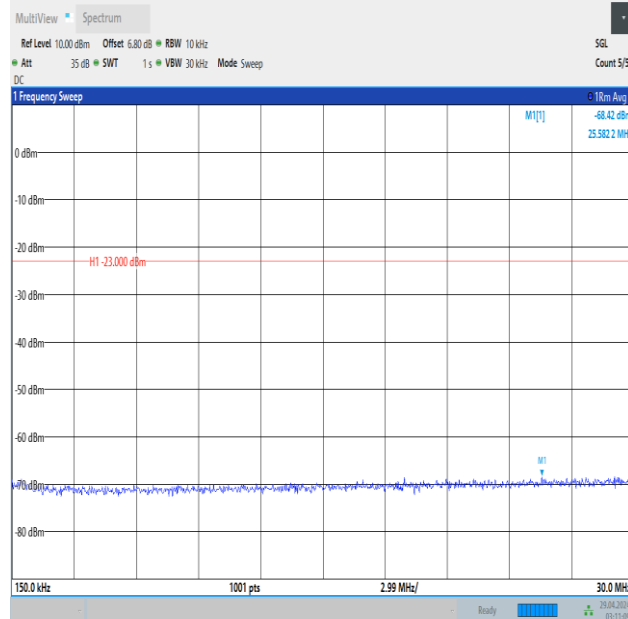
Band5_5MHz_16QAM_20525_1RB#24_0.15~30_0.15~30
