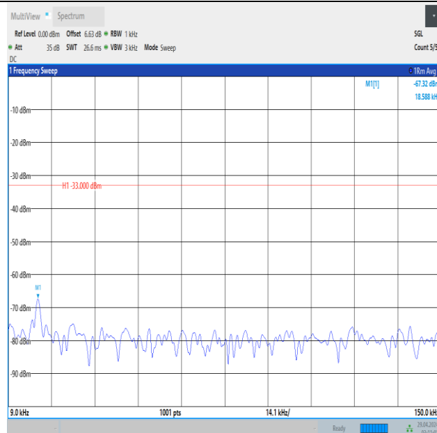
Band5_5MHz_16QAM_20525_1RB#24_0.009~0.15_0.009~0.15
