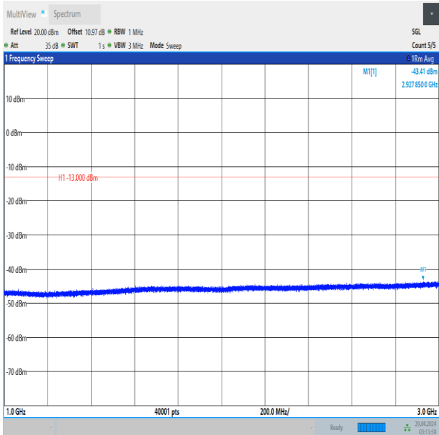
Band5_5MHz_QPSK_20625_1RB#0_1000~3000_1000~3000
