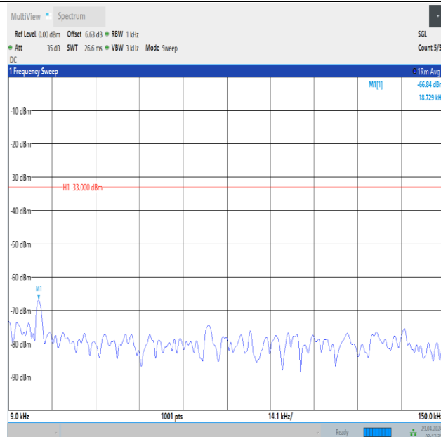
Band5_5MHz_16QAM_20625_25RB#0_0.009~0.15_0.009~0.15
