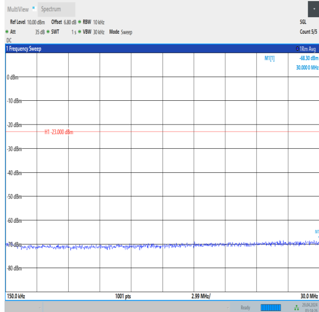
Band5_5MHz_16QAM_20625_1RB#0_0.15~30_0.15~30
