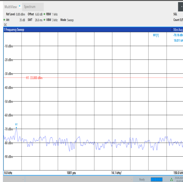
Band5_5MHz_16QAM_20425_25RB#0_0.009~0.15_0.009~0.15
