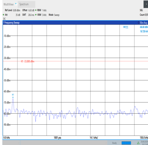
Band5_5MHz_QPSK_20525_25RB#0_0.009~0.15_0.009~0.15
