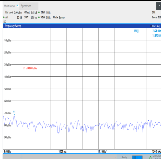
Band5_5MHz_16QAM_20625_1RB#24_0.009~0.15_0.009~0.15
