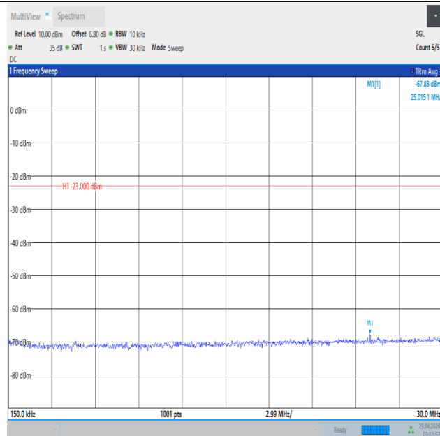
Band5_5MHz_QPSK_20525_25RB#0_0.15~30_0.15~30
