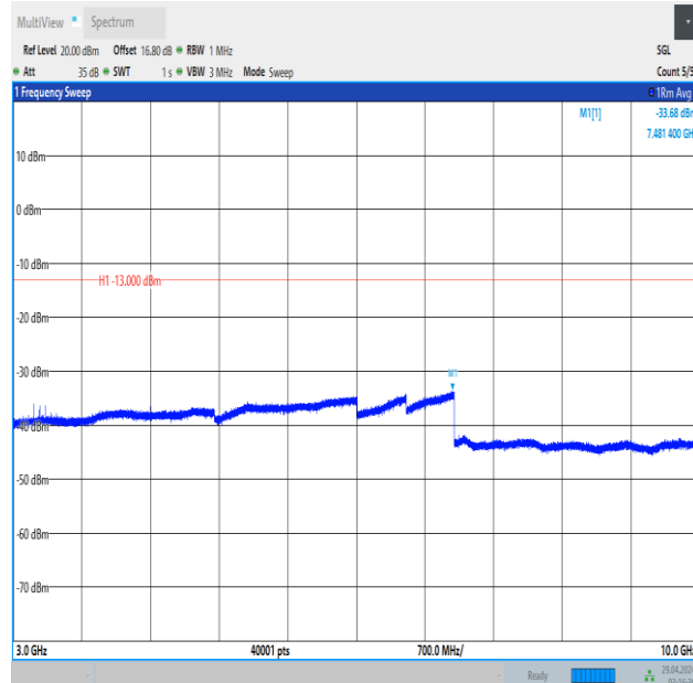
Band5_5MHz_16QAM_20625_1RB#24_3000~10000_3000~10000
