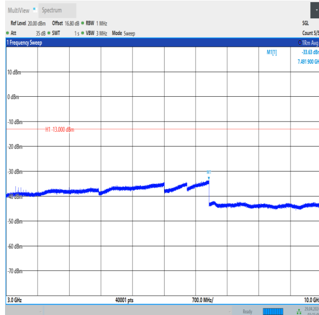
Band5_5MHz_16QAM_20625_1RB#0_3000~10000_3000~10000
