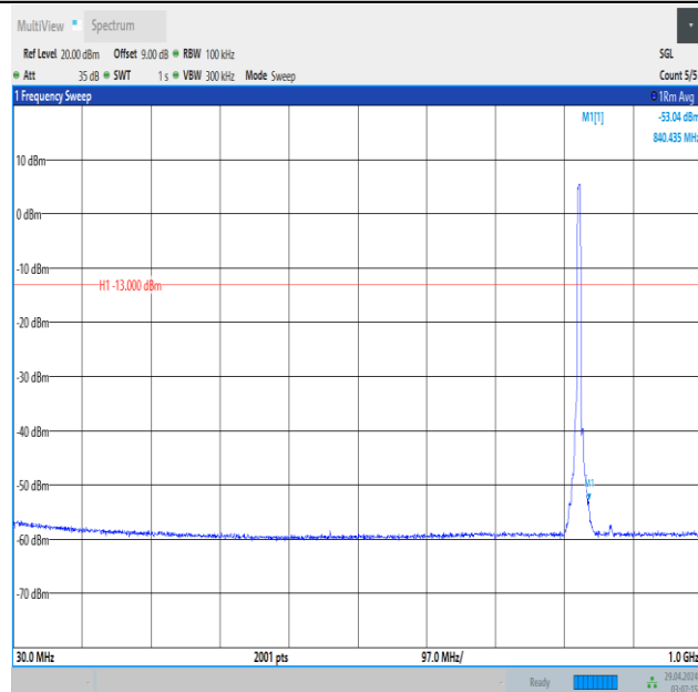
Band5_5MHz_QPSK_20425_25RB#0_30~1000_30~1000
