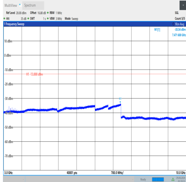
Band5_5MHz_QPSK_20525_1RB#24_3000~10000_3000~10000
