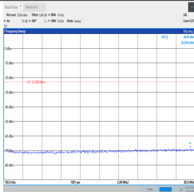
Band5_5MHz_QPSK_20525_1RB#24_0.15~30_0.15~30
