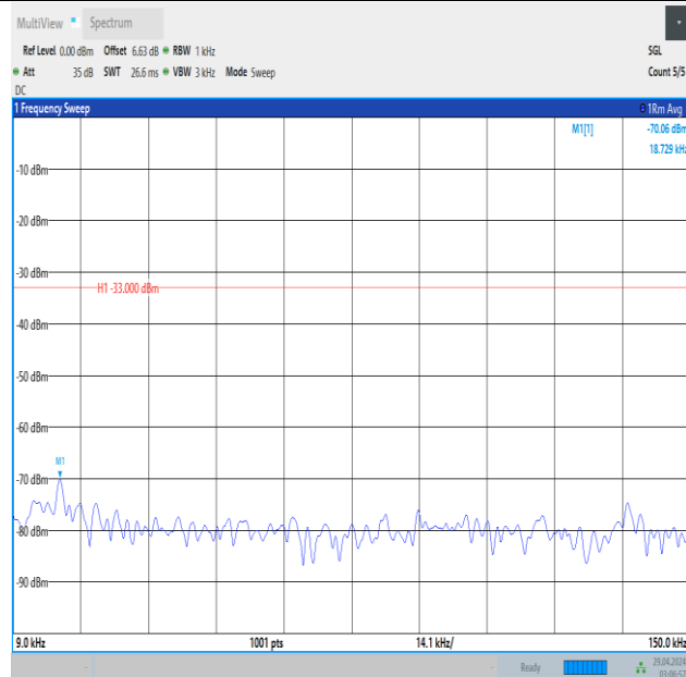
Band5_5MHz_QPSK_20425_25RB#0_0.009~0.15_0.009~0.15
