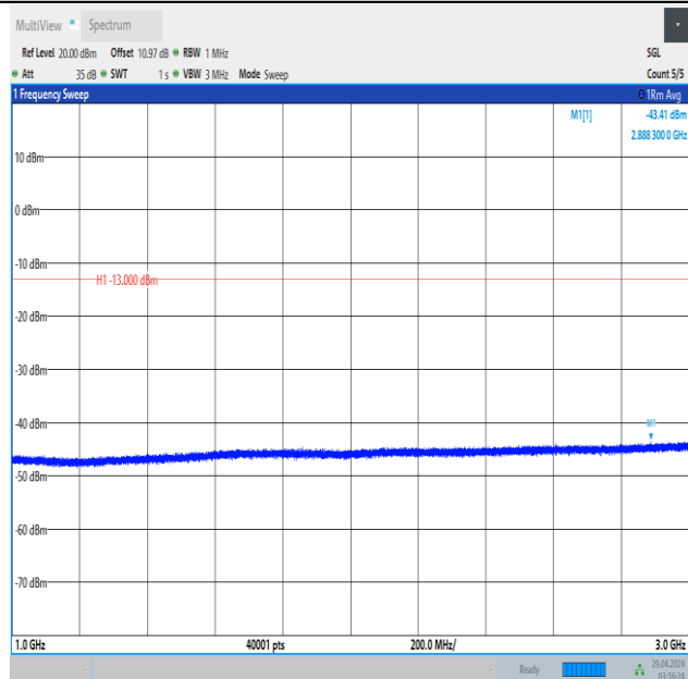
Band5_5MHz_16QAM_20625_1RB#24_1000~3000_1000~3000
