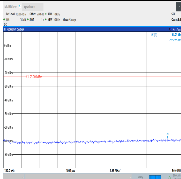
Band5_5MHz_QPSK_20625_1RB#0_0.15~30_0.15~30
