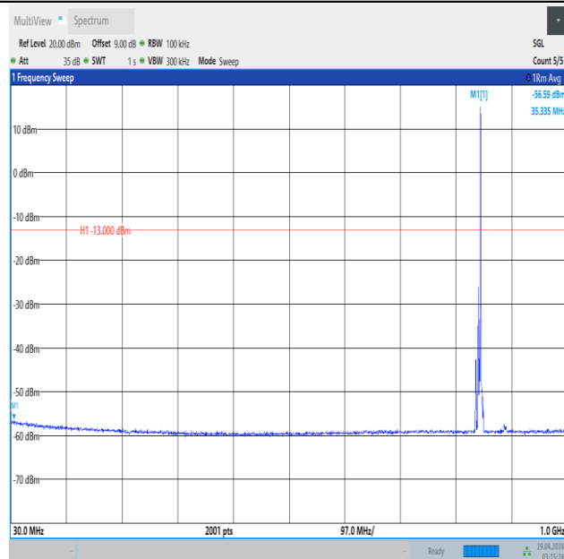
Band5_5MHz_QPSK_20625_1RB#24_30~1000_30~1000
