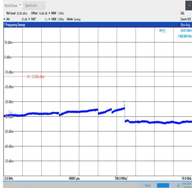
Band5_5MHz_QPSK_20425_1RB#24_3000~10000_3000~10000
