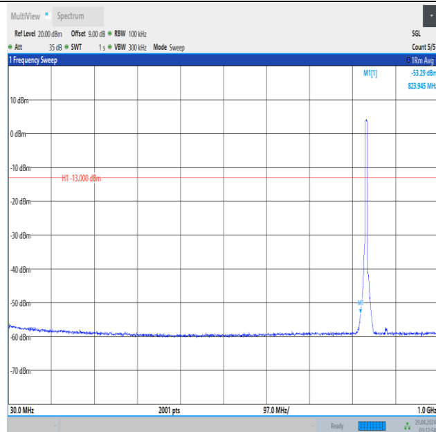
Band5_5MHz_16QAM_20525_25RB#0_30~1000_30~1000
