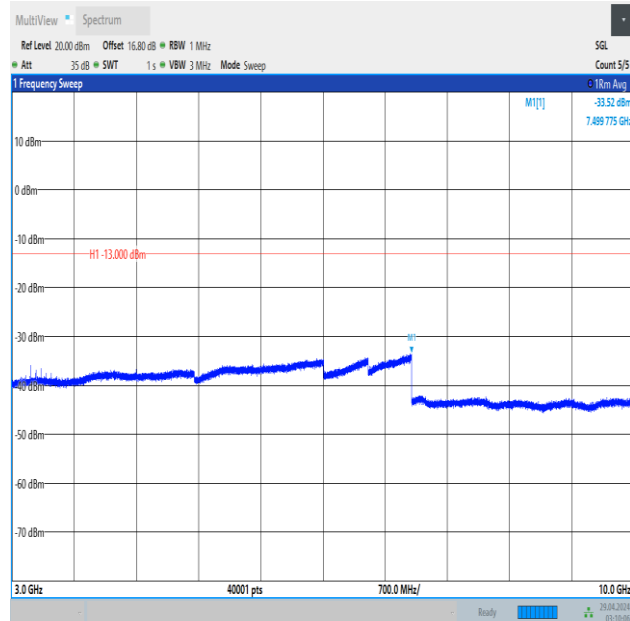
Band5_5MHz_16QAM_20525_1RB#0_3000~10000_3000~10000
