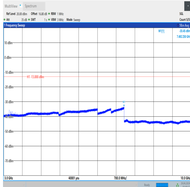
Band5_5MHz_16QAM_20425_1RB#24_3000~10000_3000~10000
