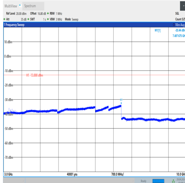
Band5_5MHz_16QAM_20425_25RB#0_3000~10000_3000~10000
