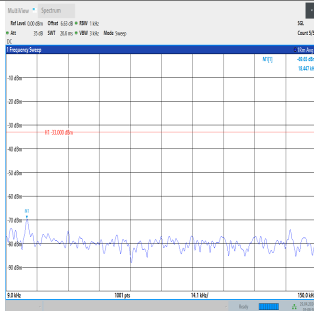
Band5_5MHz_QPSK_20525_1RB#0_0.009~0.15_0.009~0.15
