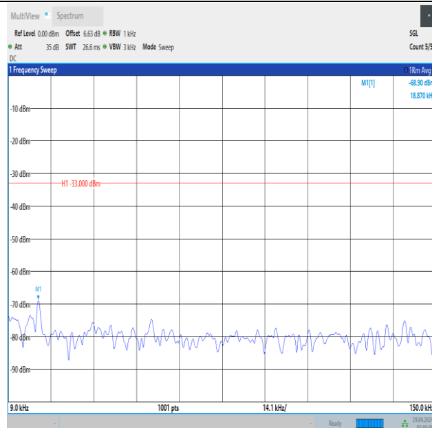
Band5_5MHz_16QAM_20425_1RB#24_0.009~0.15_0.009~0.15
