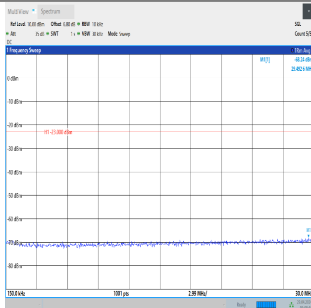
Band5_5MHz_QPSK_20525_1RB#0_0.15~30_0.15~30
