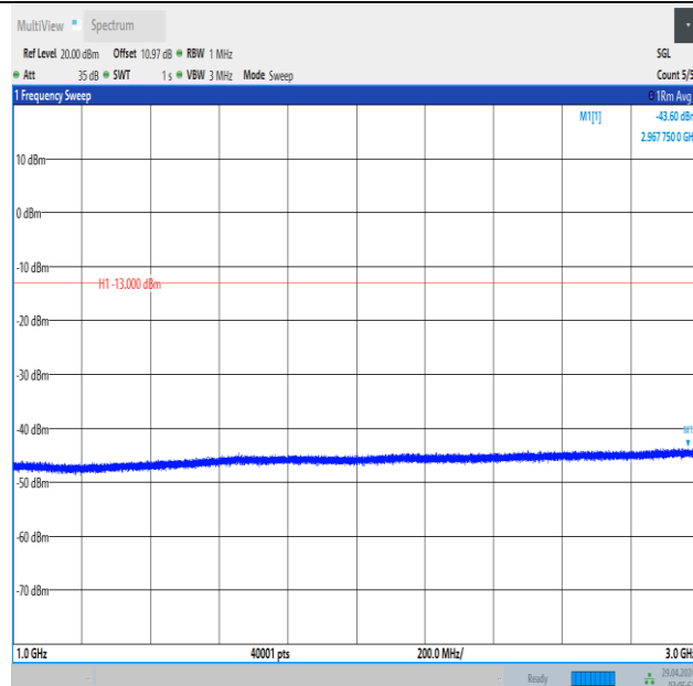
Band5_5MHz_QPSK_20425_1RB#24_1000~3000_1000~3000
