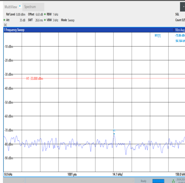
Band5_5MHz_16QAM_20525_1RB#0_0.009~0.15_0.009~0.15
