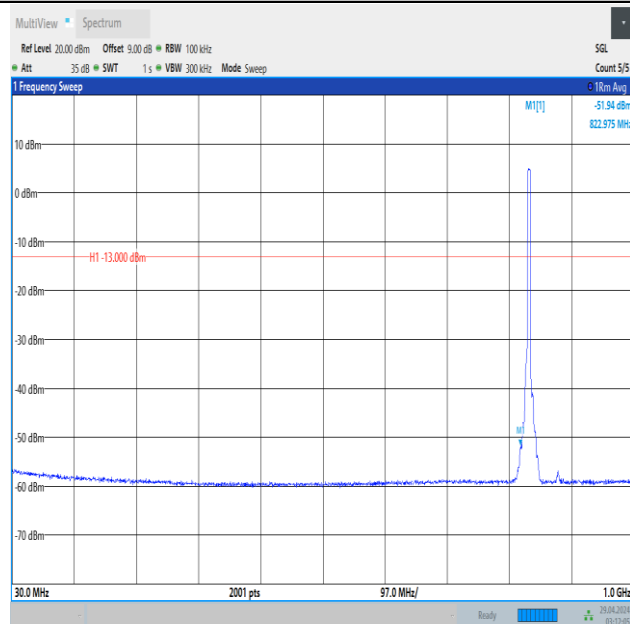
Band5_5MHz_QPSK_20525_25RB#0_30~1000_30~1000
