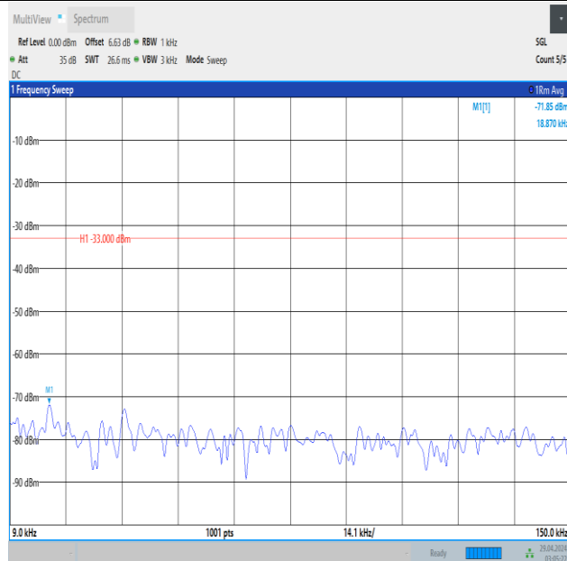
Band5_5MHz_QPSK_20425_1RB#24_0.009~0.15_0.009~0.15
