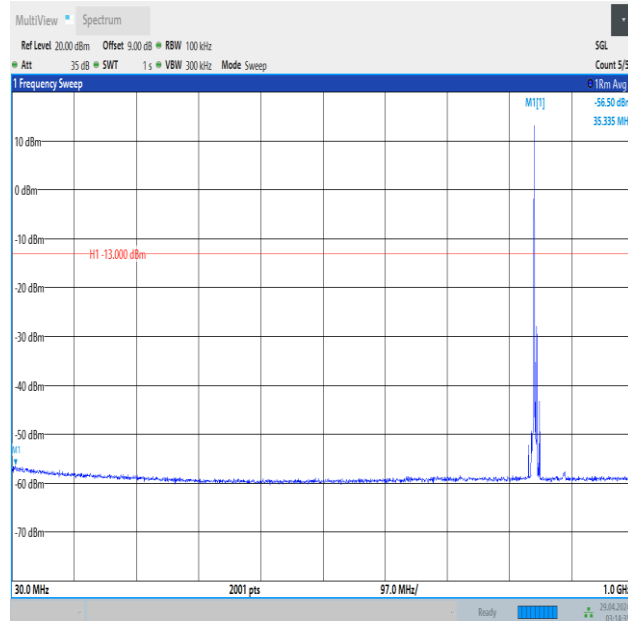
Band5_5MHz_16QAM_20625_1RB#0_30~1000_30~1000
