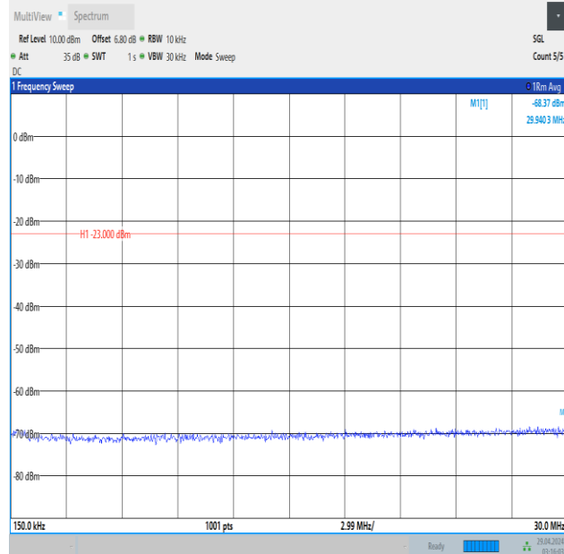
Band5_5MHz_16QAM_20625_1RB#24_0.15~30_0.15~30
