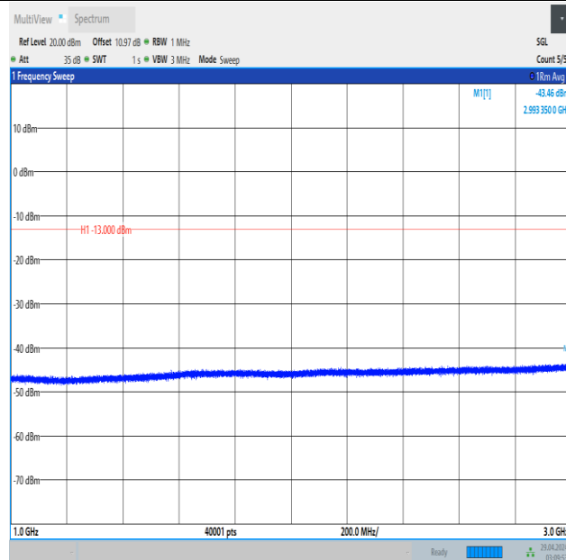
Band5_5MHz_16QAM_20525_1RB#0_1000~3000_1000~3000
