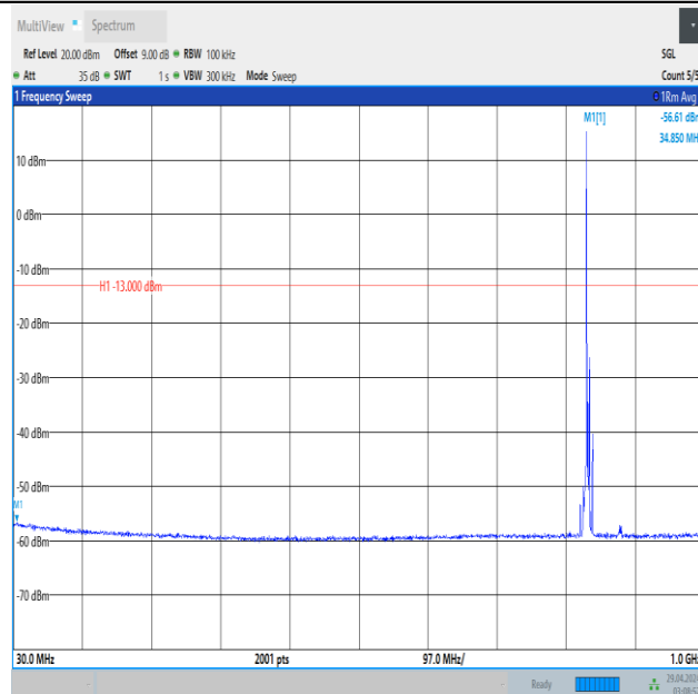
Band5_5MHz_QPSK_20525_1RB#0_30~1000_30~1000
