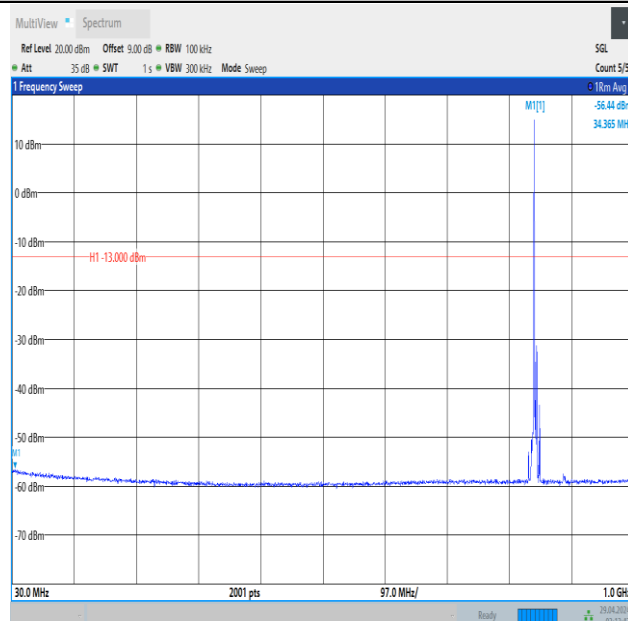
Band5_5MHz_QPSK_20625_1RB#0_30~1000_30~1000
