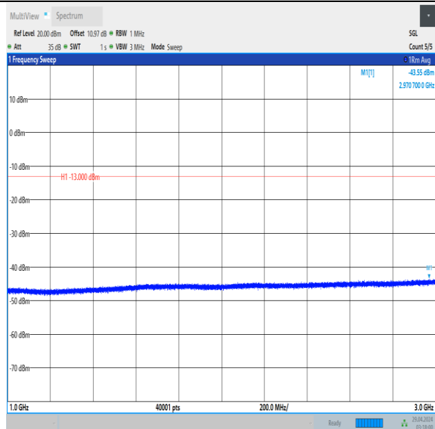
Band5_5MHz_16QAM_20625_25RB#0_1000~3000_1000~3000
