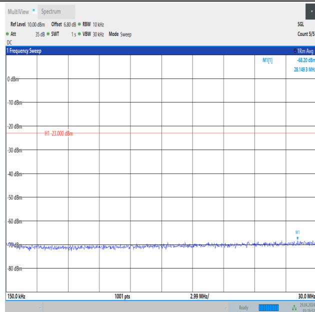
Band5_5MHz_QPSK_20625_25RB#0_0.15~30_0.15~30
