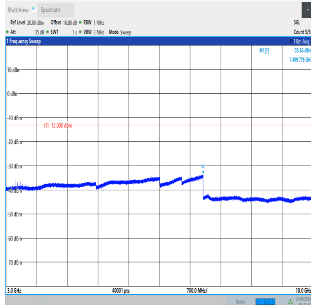
Band5_5MHz_16QAM_20525_1RB#24_3000~10000_3000~10000
