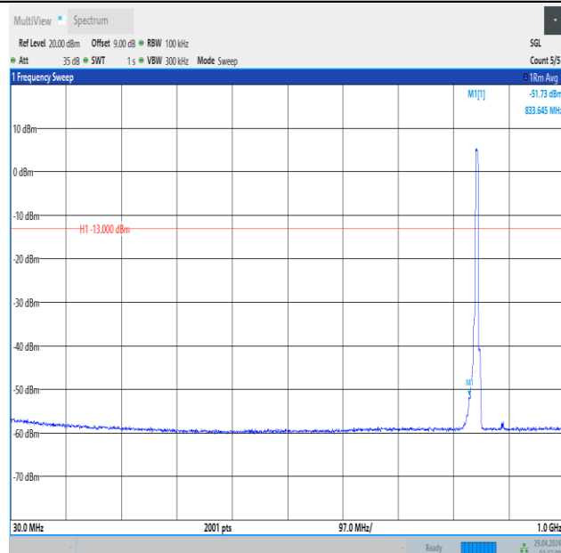
Band5_5MHz_QPSK_20625_25RB#0_30~1000_30~1000
