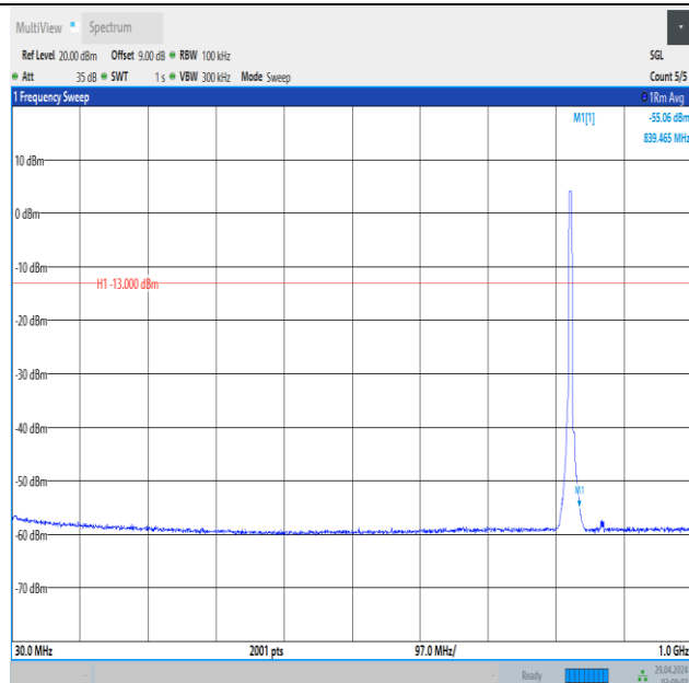
Band5_5MHz_16QAM_20425_25RB#0_30~1000_30~1000
