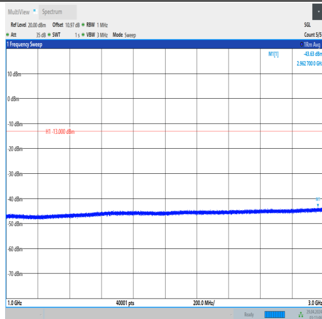
Band5_5MHz_16QAM_20525_25RB#0_1000~3000_1000~3000
