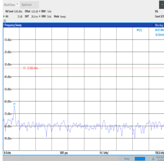
Band5_5MHz_QPSK_20525_1RB#24_0.009~0.15_0.009~0.15
