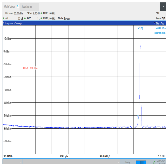
Band5_5MHz_16QAM_20625_25RB#0_30~1000_30~1000
