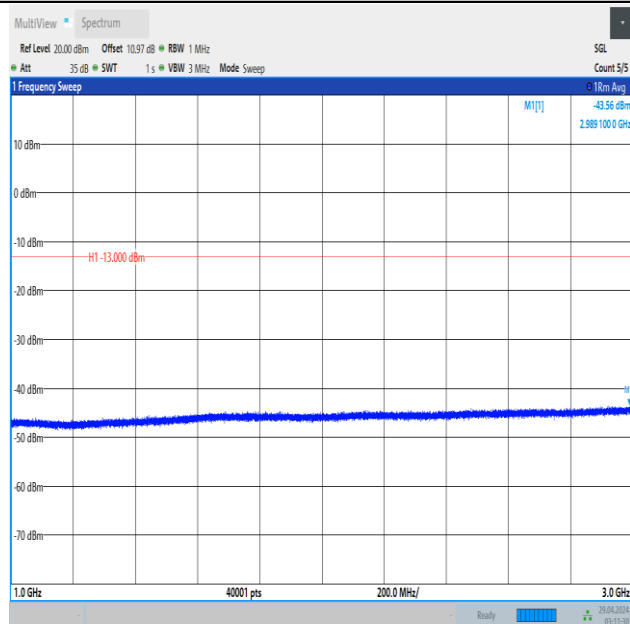
Band5_5MHz_16QAM_20525_1RB#24_1000~3000_1000~3000
