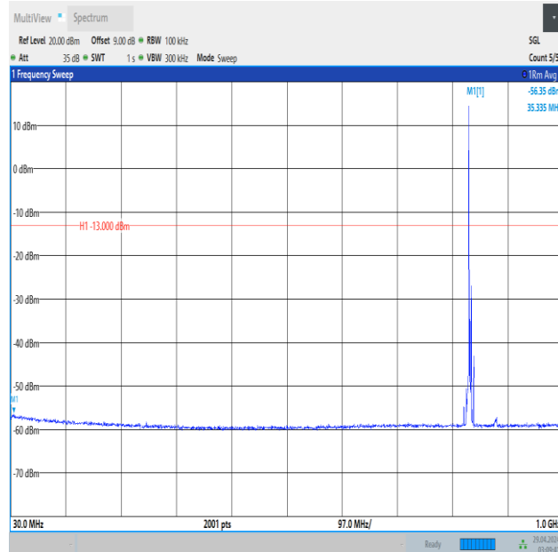
Band5_5MHz_16QAM_20525_1RB#0_30~1000_30~1000
