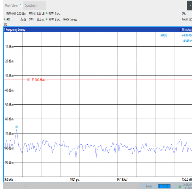
Band5_5MHz_QPSK_20625_1RB#24_0.009~0.15_0.009~0.15
