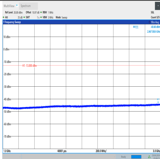
Band5_5MHz_16QAM_20425_25RB#0_1000~3000_1000~3000
