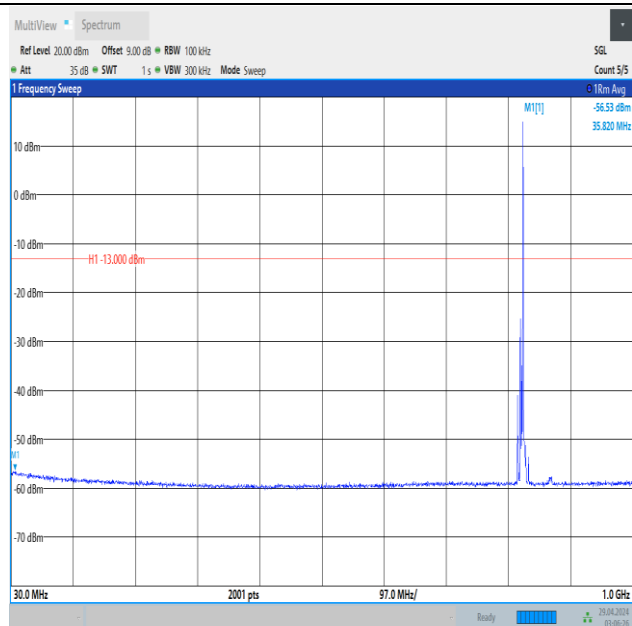
Band5_5MHz_16QAM_20425_1RB#24_30~1000_30~1000
