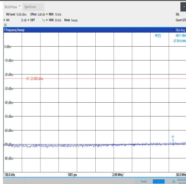
Band5_5MHz_QPSK_20625_1RB#24_0.15~30_0.15~30
