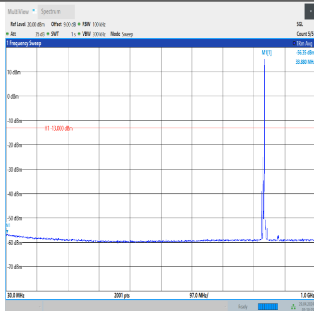
Band5_5MHz_QPSK_20525_1RB#24_30~1000_30~1000
