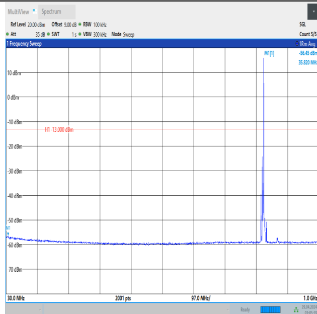
Band5_5MHz_QPSK_20425_1RB#24_30~1000_30~1000
