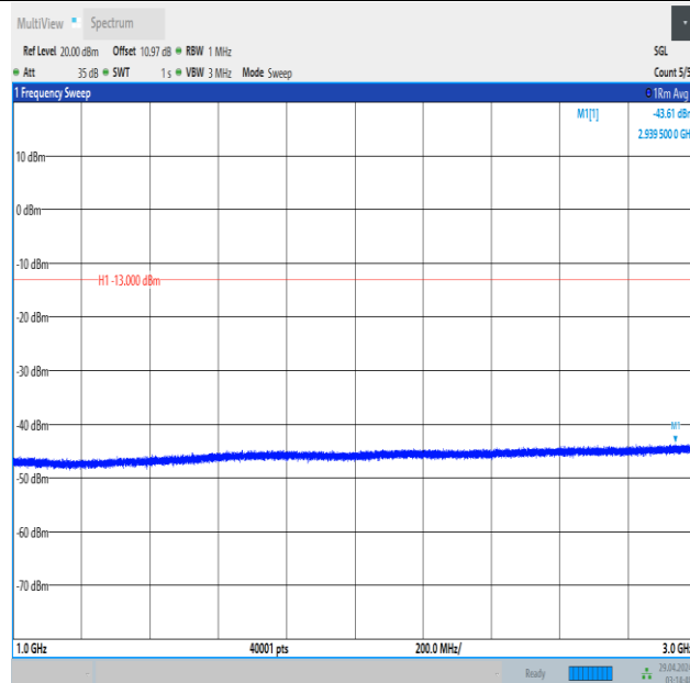
Band5_5MHz_16QAM_20625_1RB#0_1000~3000_1000~3000
