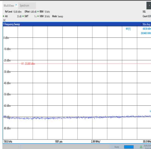
Band5_5MHz_QPSK_20425_1RB#24_0.15~30_0.15~30
