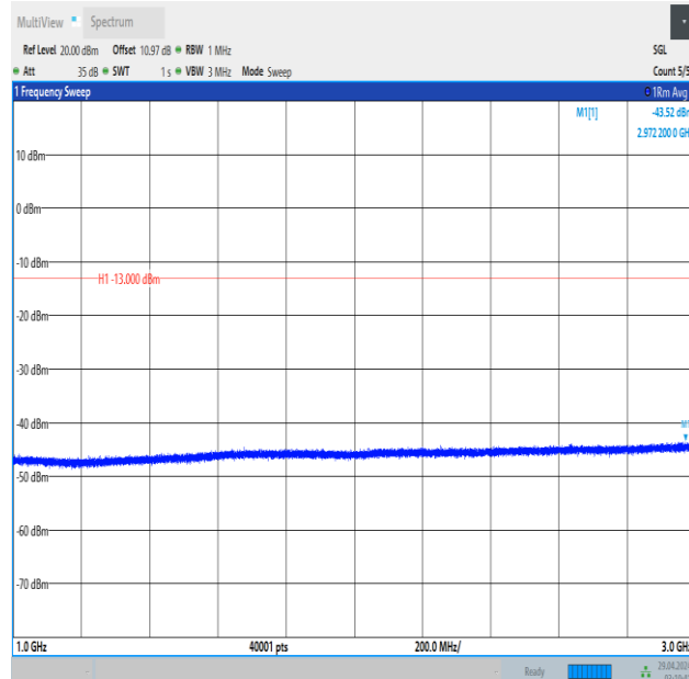
Band5_5MHz_QPSK_20525_1RB#24_1000~3000_1000~3000
