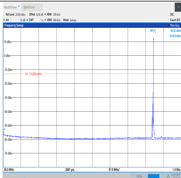
Band5_5MHz_16QAM_20625_1RB#24_30~1000_30~1000
