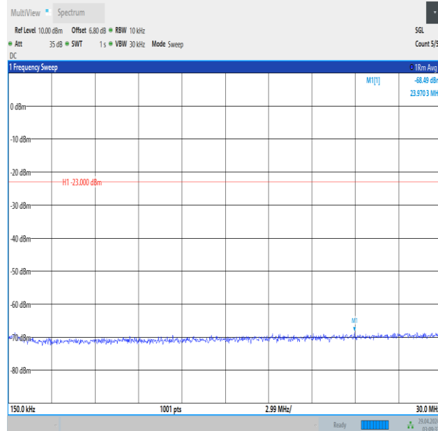
Band5_5MHz_16QAM_20525_1RB#0_0.15~30_0.15~30
