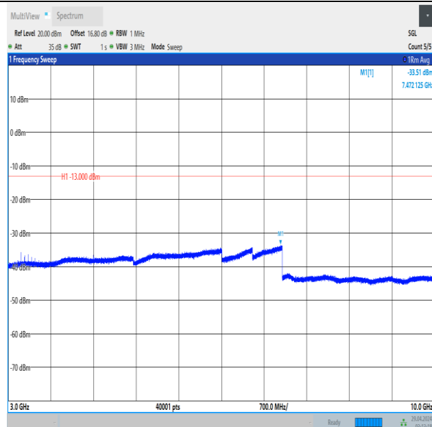
Band5_5MHz_16QAM_20525_25RB#0_3000~10000_3000~10000
