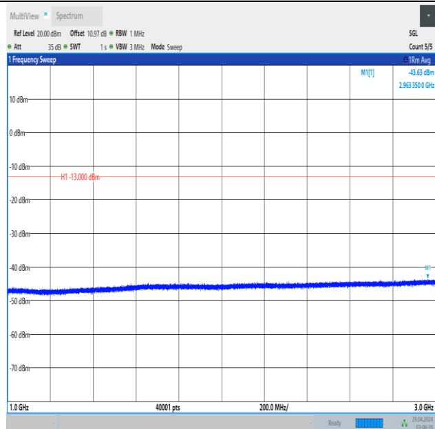
Band5_5MHz_16QAM_20425_1RB#24_1000~3000_1000~3000
