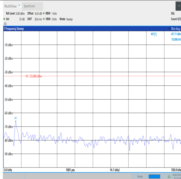
Band5_5MHz_QPSK_20625_1RB#0_0.009~0.15_0.009~0.15
