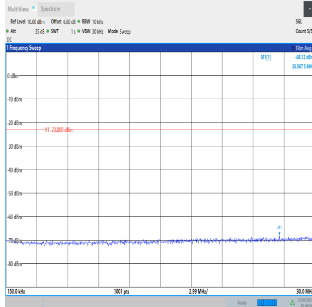
Band5_3MHz_QPSK_20415_15RB#0_0.15~30_0.15~30
