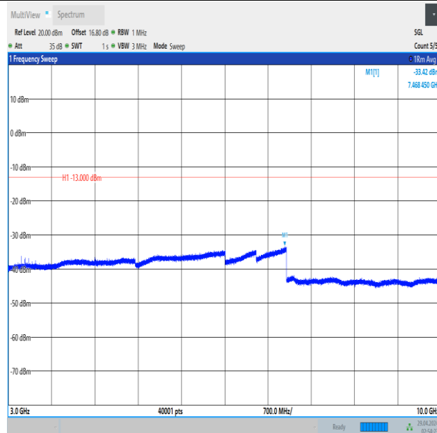
Band5_3MHz_16QAM_20525_15RB#0_3000~10000_3000~10000
