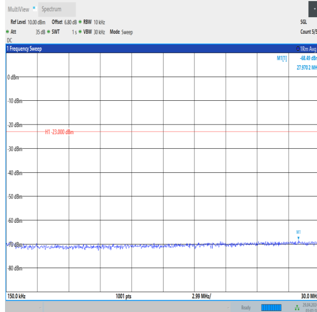
Band5_10MHz_QPSK_20450_50RB#0_0.15~30_0.15~30
