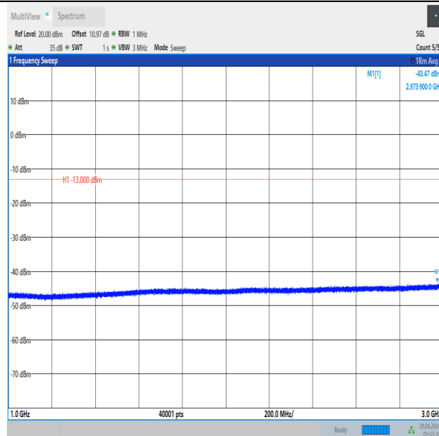
Band5_3MHz_QPSK_20525_15RB#0_1000~3000_1000~3000
