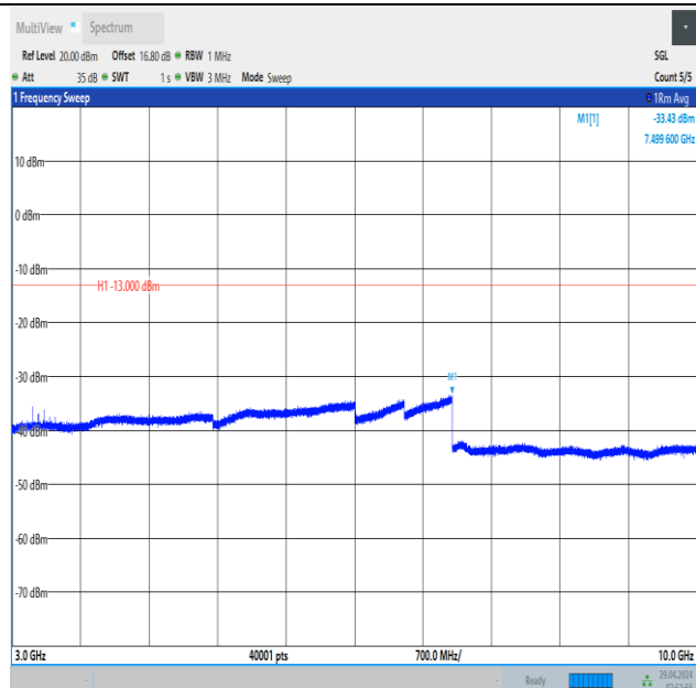
Band5_3MHz_QPSK_20525_1RB#14_3000~10000_3000~10000
