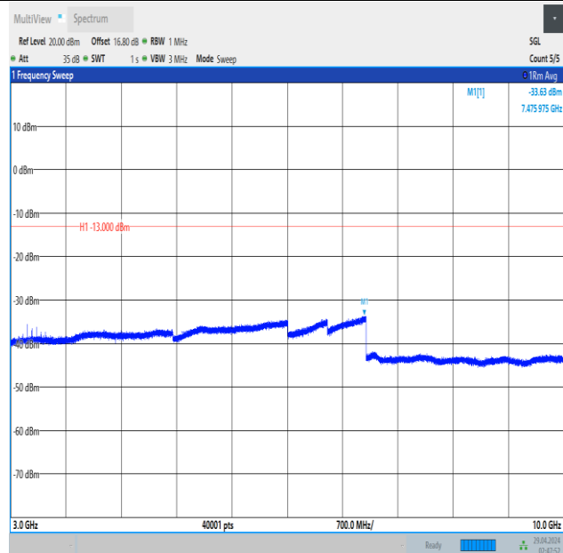
Band5_3MHz_16QAM_20415_1RB#14_3000~10000_3000~10000
