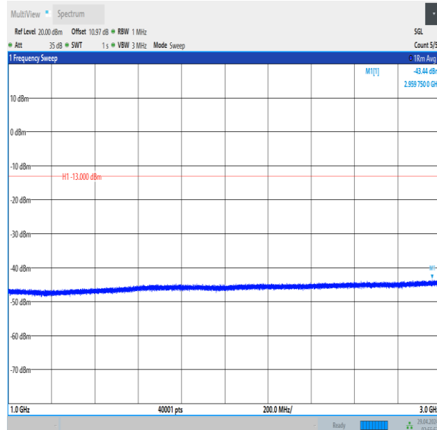
Band5_3MHz_16QAM_20635_1RB#0_1000~3000_1000~3000
