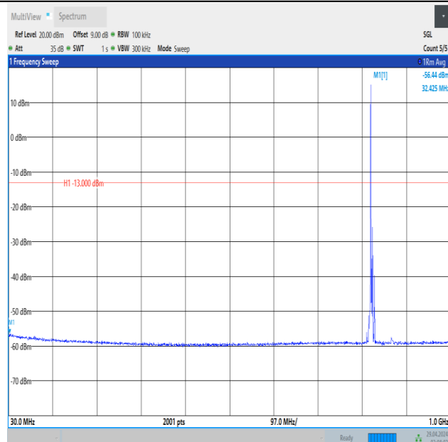
Band5_5MHz_QPSK_20425_1RB#0_30~1000_30~1000
