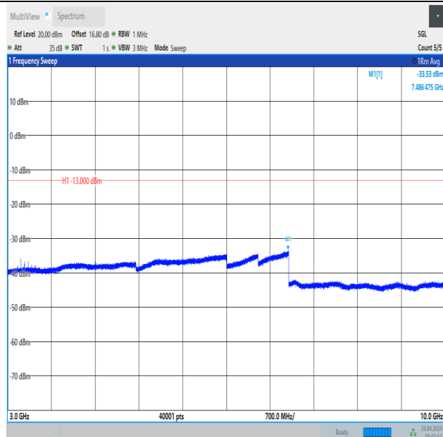
Band5_10MHz_QPSK_20450_50RB#0_3000~10000_3000~10000
