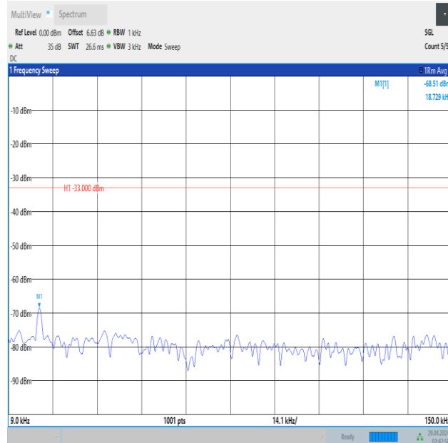
Band5_3MHz_QPSK_20415_15RB#0_0.009~0.15_0.009~0.15
