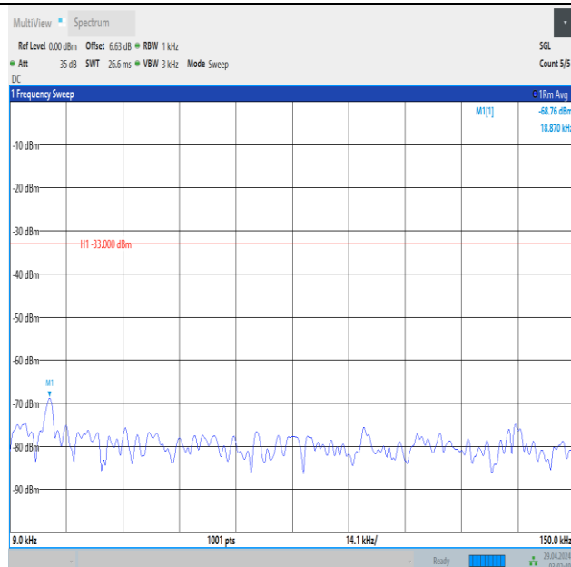
Band5_10MHz_QPSK_20600_50RB#0_0.009~0.15_0.009~0.15
