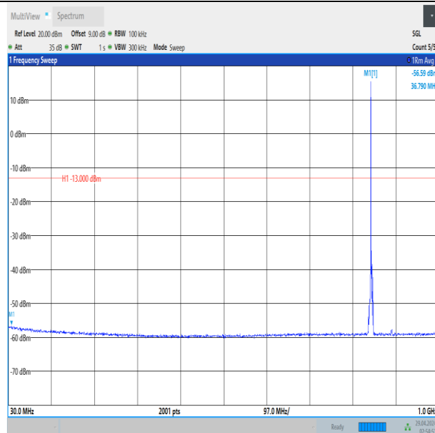
Band5_3MHz_QPSK_20635_1RB#0_30~1000_30~1000
