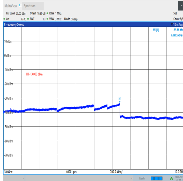
Band5_3MHz_QPSK_20635_1RB#0_3000~10000_3000~10000
