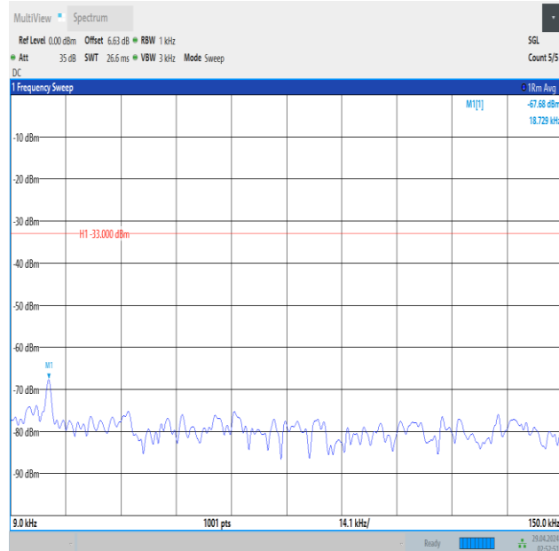
Band5_3MHz_QPSK_20525_15RB#0_0.009~0.15_0.009~0.15
