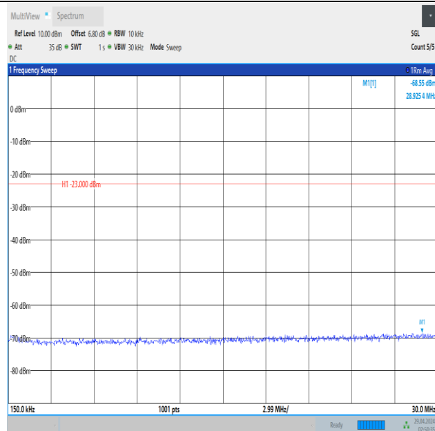
Band5_3MHz_16QAM_20525_1RB#0_0.15~30_0.15~30
