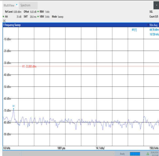
Band5_3MHz_16QAM_20525_1RB#14_0.009~0.15_0.009~0.15
