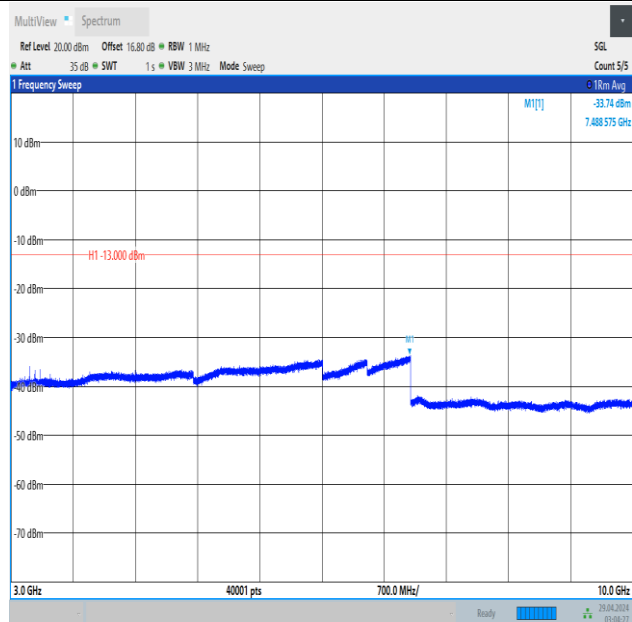
Band5_5MHz_QPSK_20425_1RB#0_3000~10000_3000~10000
