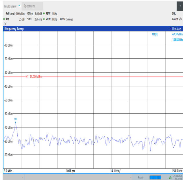
Band5_3MHz_16QAM_20415_1RB#14_0.009~0.15_0.009~0.15
