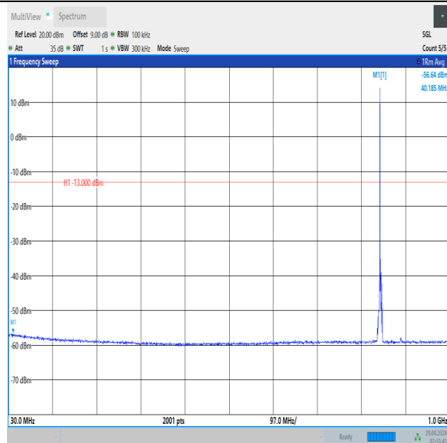
Band5_3MHz_16QAM_20635_1RB#0_30~1000_30~1000
