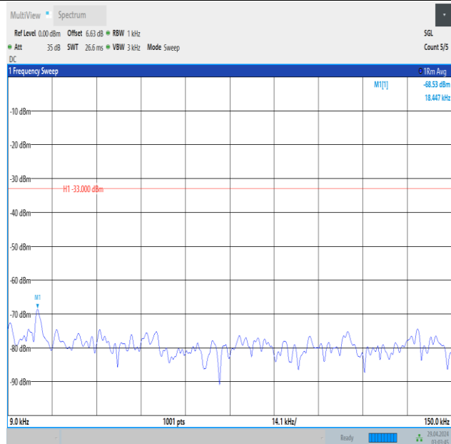
Band5_5MHz_QPSK_20425_1RB#0_0.009~0.15_0.009~0.15
