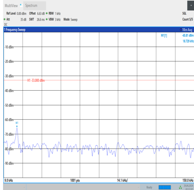
Band5_3MHz_16QAM_20635_1RB#14_0.009~0.15_0.009~0.15
