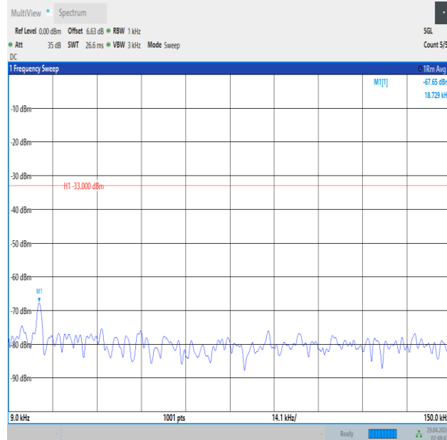
Band5_3MHz_16QAM_20415_15RB#0_0.009~0.15_0.009~0.15
