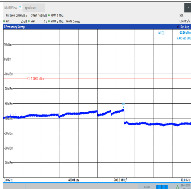
Band5_3MHz_QPSK_20415_1RB#14_3000~10000_3000~10000
