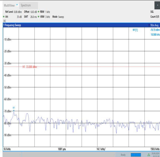
Band5_3MHz_16QAM_20635_1RB#0_0.009~0.15_0.009~0.15
