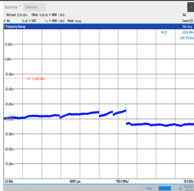
Band5_3MHz_16QAM_20635_1RB#14_3000~10000_3000~10000
