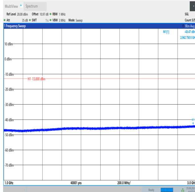
Band5_3MHz_16QAM_20635_1RB#14_1000~3000_1000~3000
