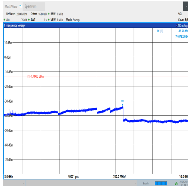
Band5_3MHz_16QAM_20415_15RB#0_3000~10000_3000~10000
