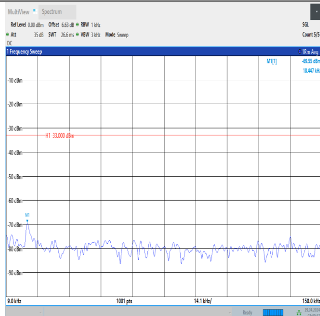
Band5_3MHz_QPSK_20525_1RB#0_0.009~0.15_0.009~0.15
