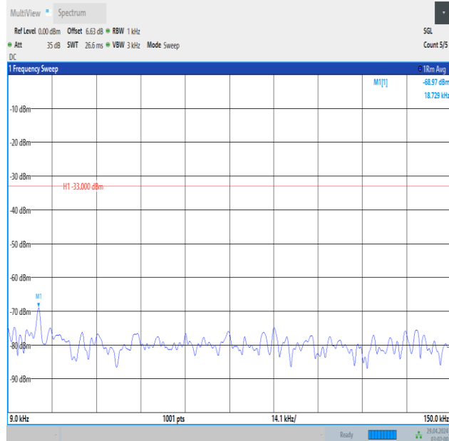
Band5_10MHz_QPSK_20525_50RB#0_0.009~0.15_0.009~0.15
