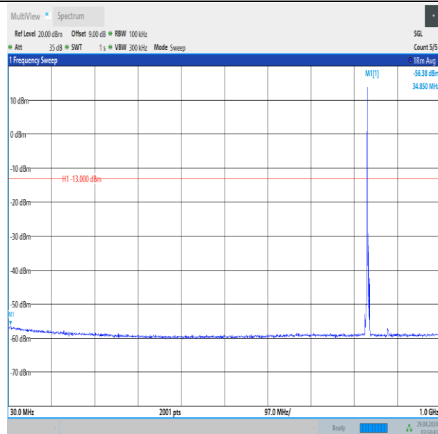
Band5_3MHz_16QAM_20525_1RB#0_30~1000_30~1000
