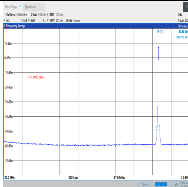
Band5_3MHz_QPSK_20525_15RB#0_30~1000_30~1000
