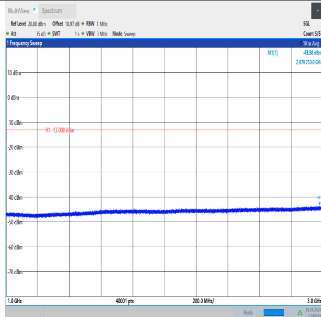
Band5_1.4MHz_QPSK_20643_1RB#5_1000~3000_1000~3000
