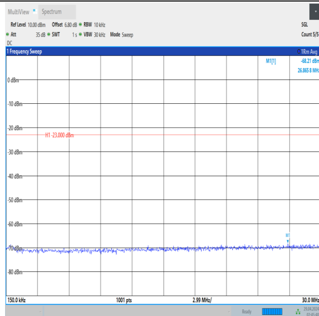
Band5_3MHz_16QAM_20415_1RB#0_0.15~30_0.15~30
