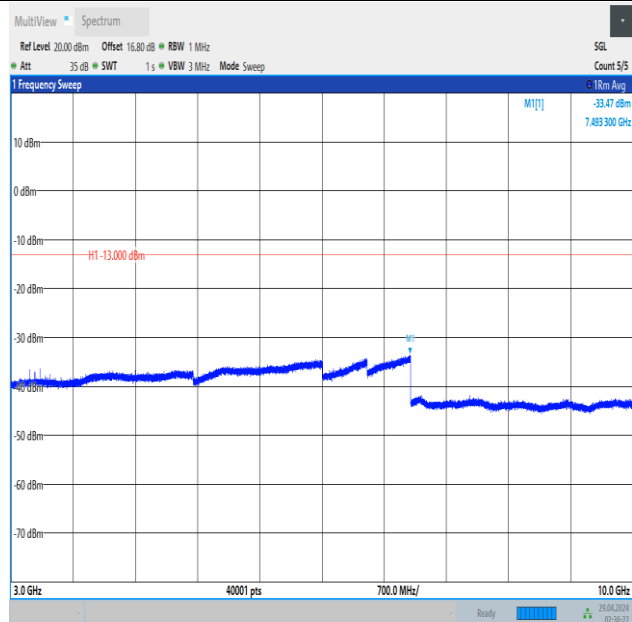
Band5_10MHz_16QAM_20450_1RB#0_3000~10000_3000~10000
