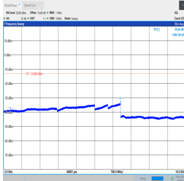
Band5_3MHz_16QAM_20415_1RB#0_3000~10000_3000~10000
