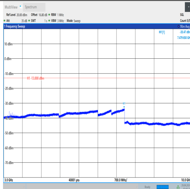
Band5_3MHz_QPSK_20415_1RB#0_3000~10000_3000~10000
