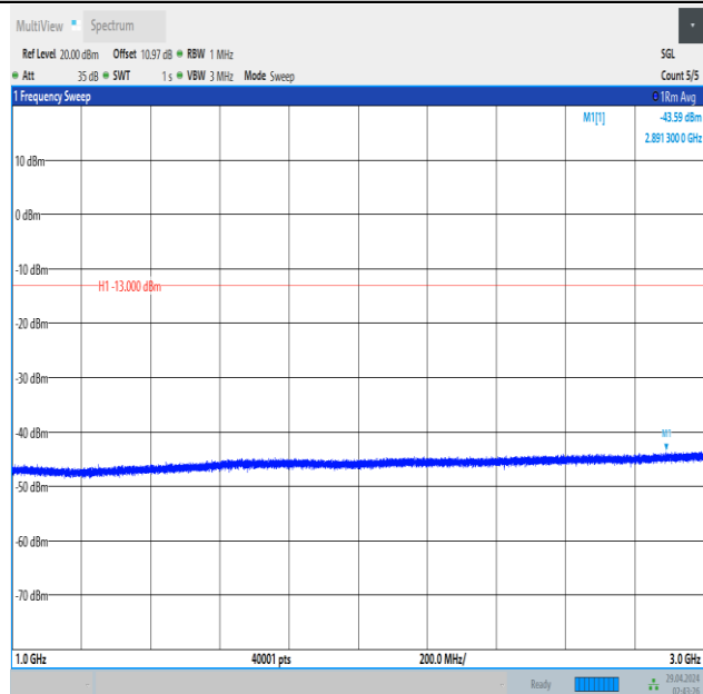
Band5_10MHz_QPSK_20600_1RB#49_1000~3000_1000~3000
