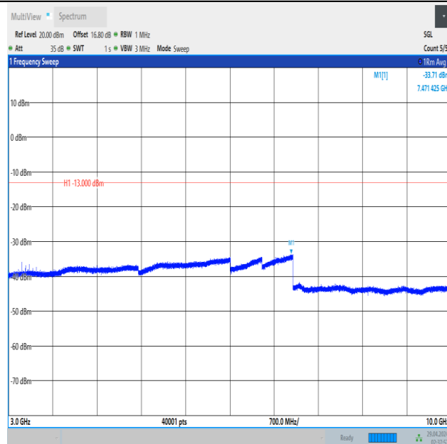
Band5_10MHz_16QAM_20450_1RB#49_3000~10000_3000~10000
