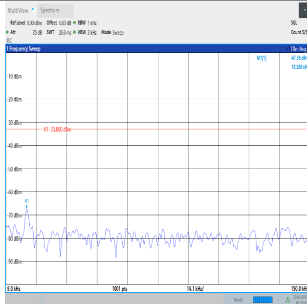
Band5_1.4MHz_16QAM_20643_1RB#5_0.009~0.15_0.009~0.15
