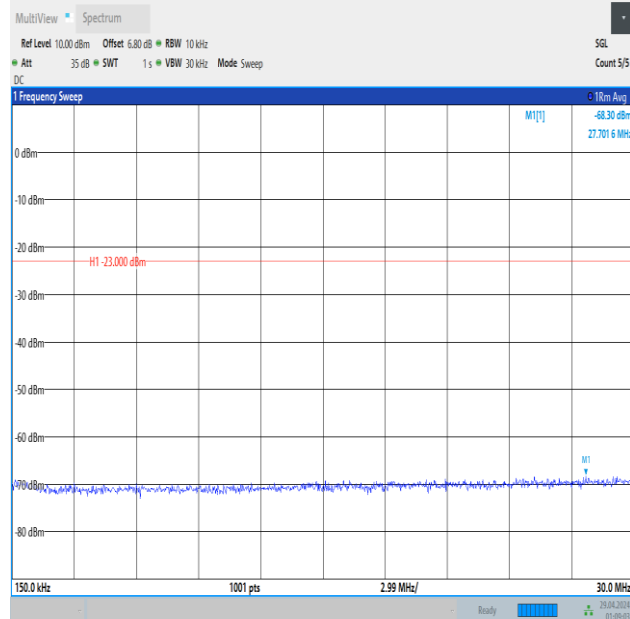
Band5_1.4MHz_QPSK_20643_1RB#5_0.15~30_0.15~30
