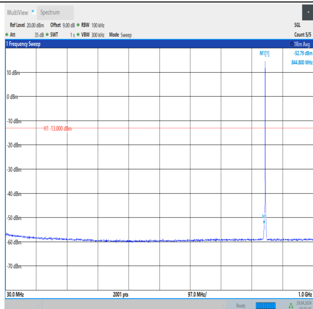
Band5_1.4MHz_QPSK_20643_1RB#0_30~1000_30~1000
