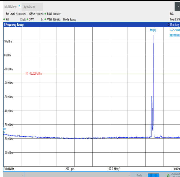
Band5_10MHz_16QAM_20600_1RB#49_30~1000_30~1000
