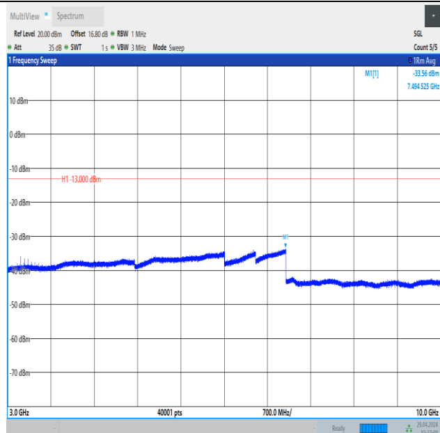
Band5_10MHz_QPSK_20450_1RB#49_3000~10000_3000~10000
