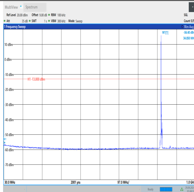
Band5_3MHz_QPSK_20415_1RB#0_30~1000_30~1000
