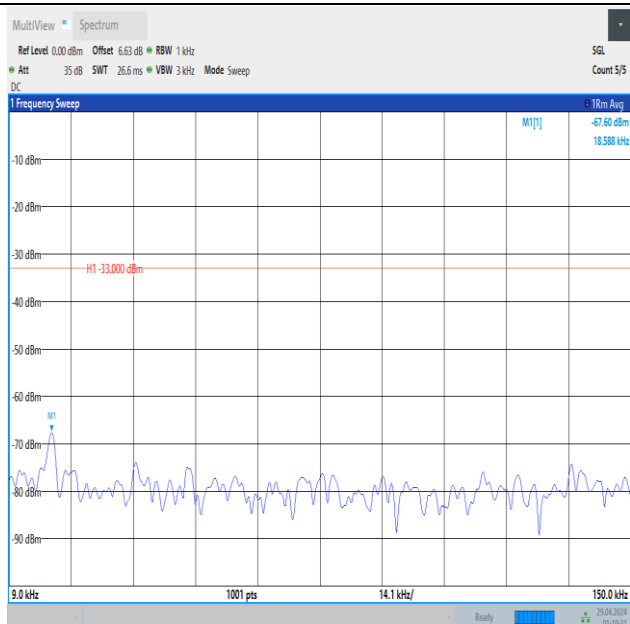
Band5_1.4MHz_QPSK_20643_6RB#0_0.009~0.15_0.009~0.15
