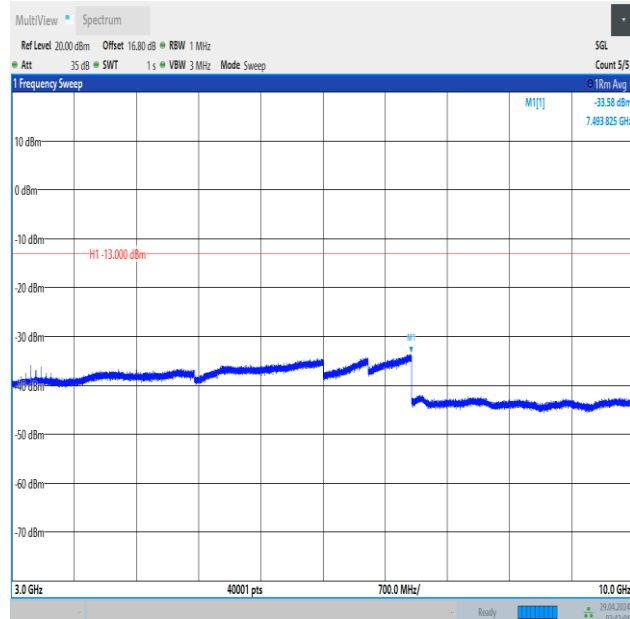
Band5_10MHz_QPSK_20600_1RB#0_3000~10000_3000~10000
