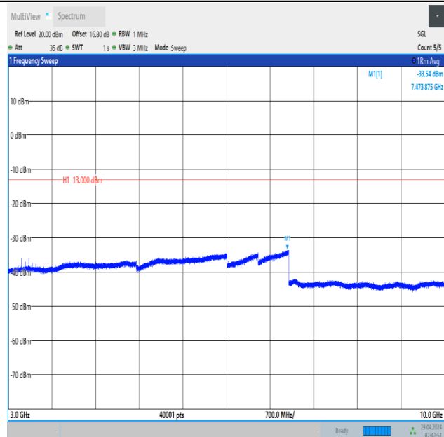
Band5_10MHz_16QAM_20600_1RB#0_3000~10000_3000~10000
