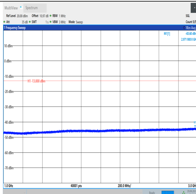
Band5_10MHz_16QAM_20525_1RB#49_1000~3000_1000~3000
