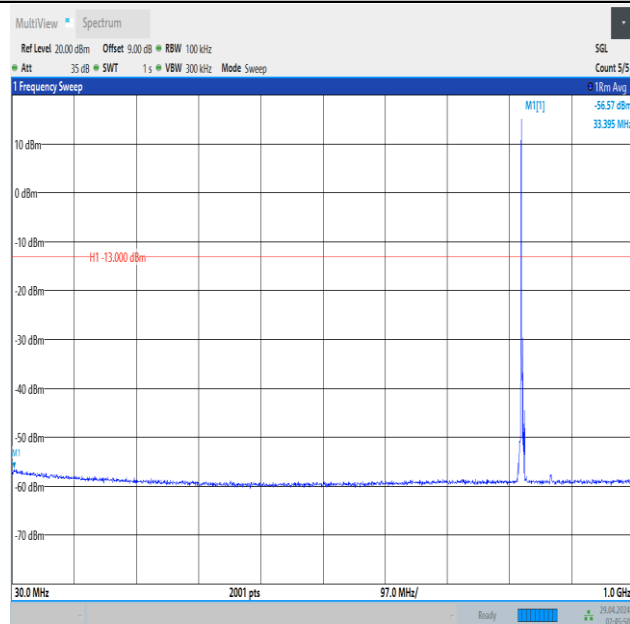
Band5_3MHz_16QAM_20415_1RB#0_30~1000_30~1000
