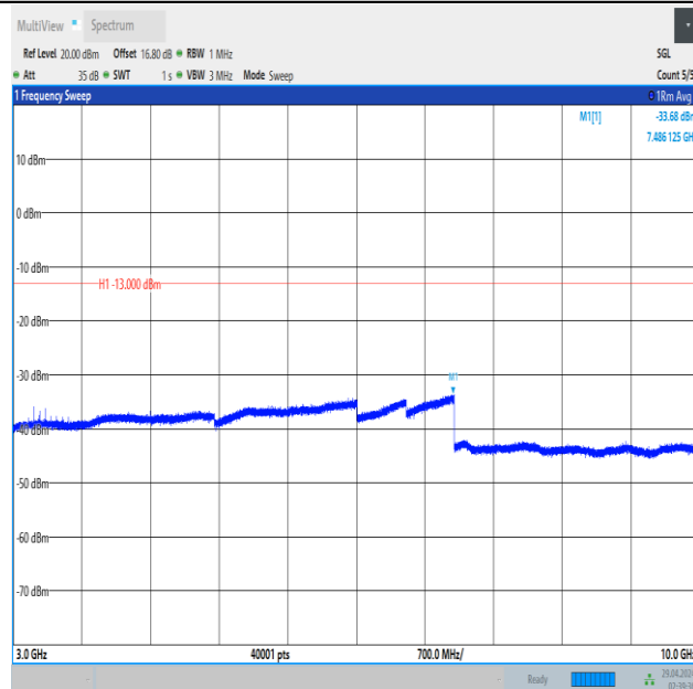
Band5_10MHz_16QAM_20525_1RB#0_3000~10000_3000~10000
