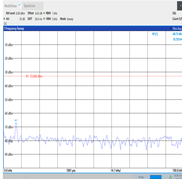
Band5_10MHz_QPSK_20600_1RB#49_0.009~0.15_0.009~0.15
