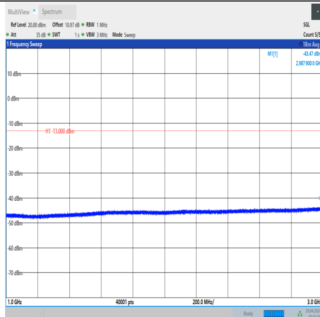
Band5_10MHz_16QAM_20600_1RB#0_1000~3000_1000~3000
