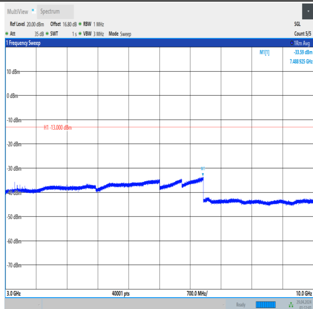
Band5_1.4MHz_16QAM_20643_6RB#0_3000~10000_3000~10000
