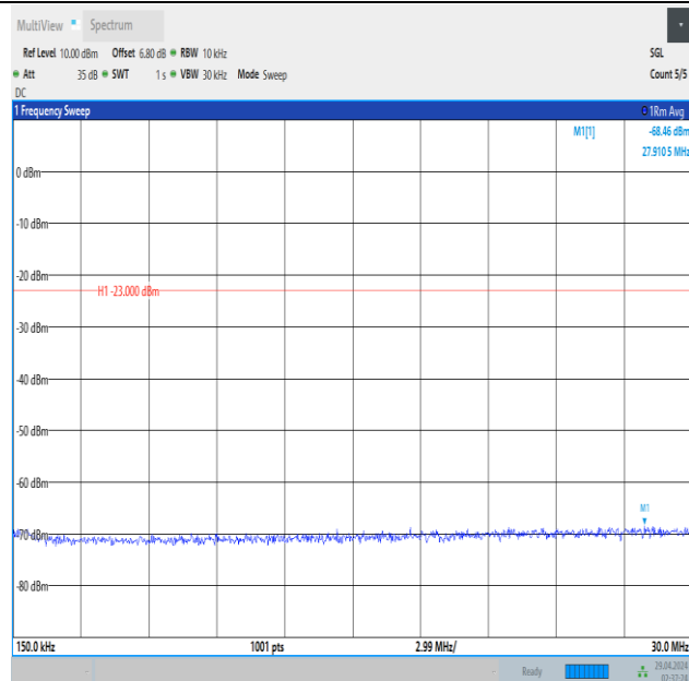
Band5_10MHz_16QAM_20450_1RB#49_0.15~30_0.15~30
