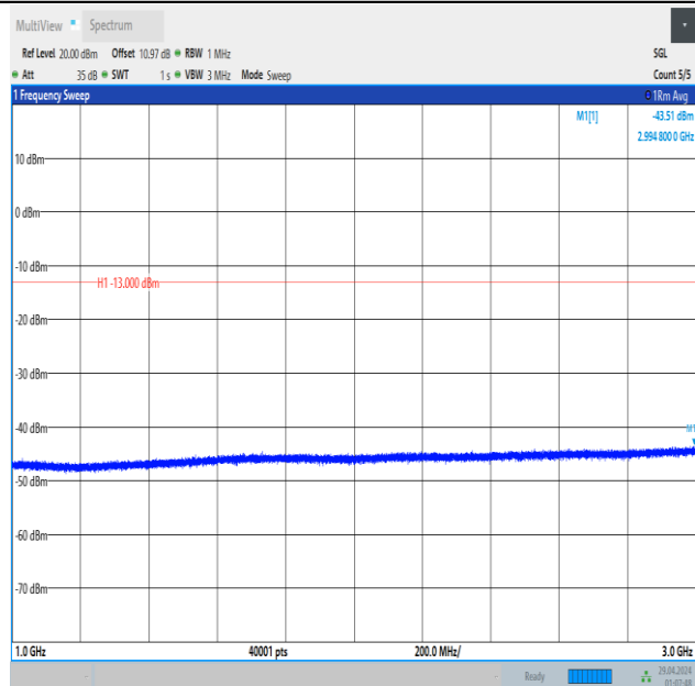
Band5_1.4MHz_QPSK_20643_1RB#0_1000~3000_1000~3000
