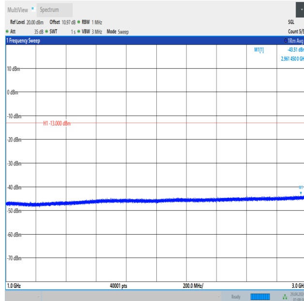
Band5_1.4MHz_16QAM_20643_1RB#0_1000~3000_1000~3000
