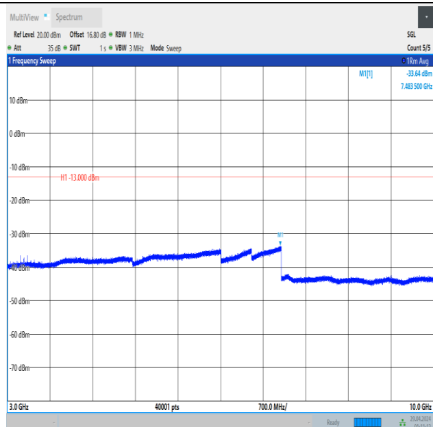
Band5_1.4MHz_QPSK_20643_6RB#0_3000~10000_3000~10000
