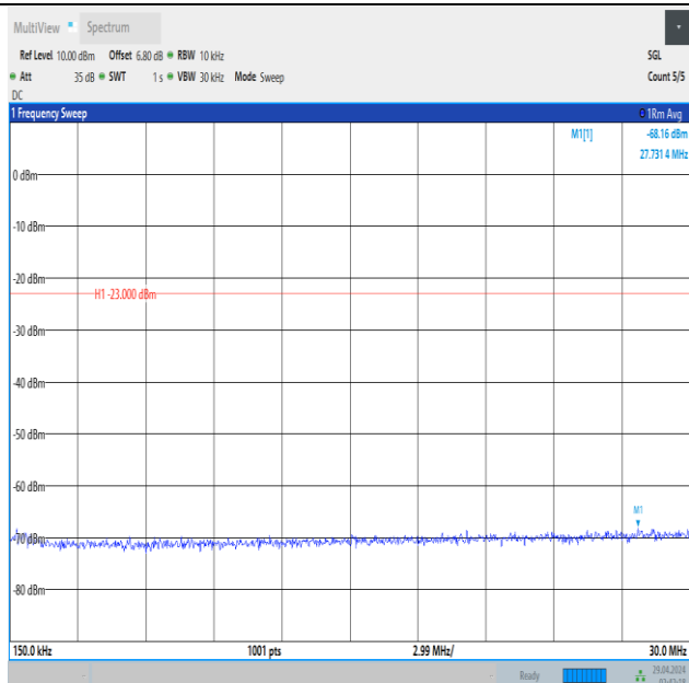
Band5_10MHz_16QAM_20600_1RB#0_0.15~30_0.15~30
