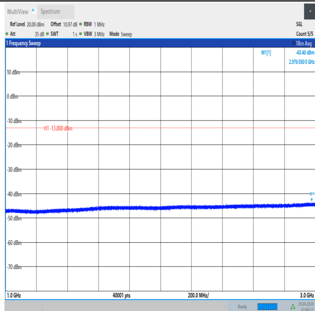
Band5_10MHz_QPSK_20525_1RB#49_1000~3000_1000~3000
