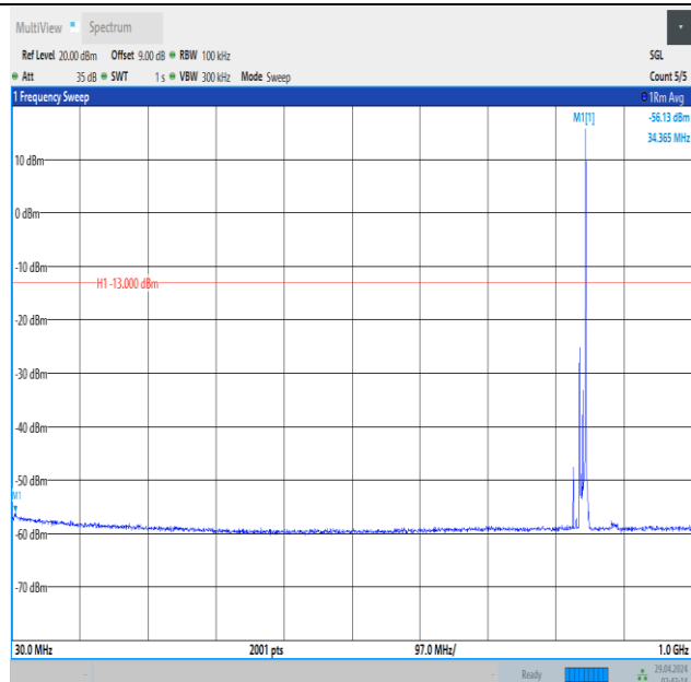
Band5_10MHz_QPSK_20600_1RB#49_30~1000_30~1000
