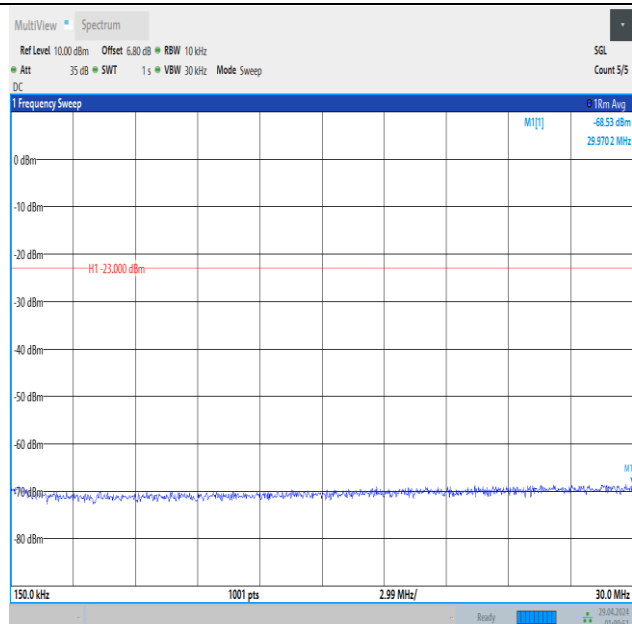
Band5_1.4MHz_16QAM_20643_1RB#5_0.15~30_0.15~30
