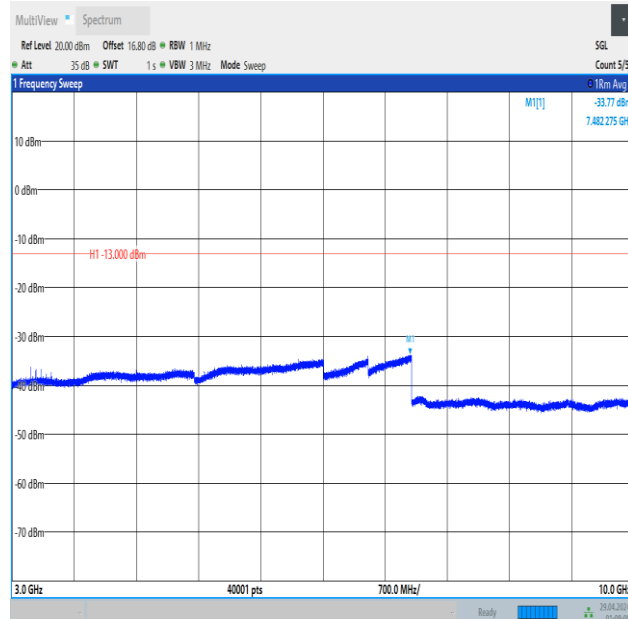
Band5_1.4MHz_QPSK_20643_1RB#0_3000~10000_3000~10000
