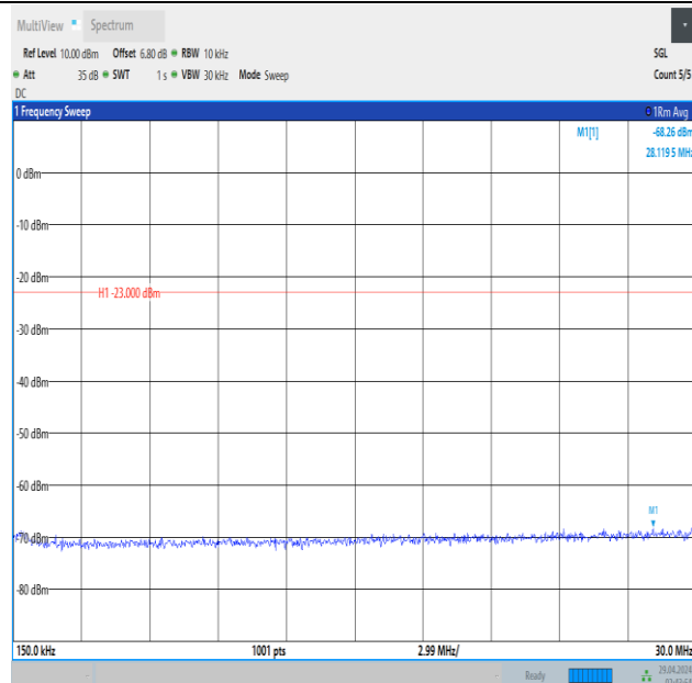
Band5_10MHz_16QAM_20600_1RB#49_0.15~30_0.15~30
