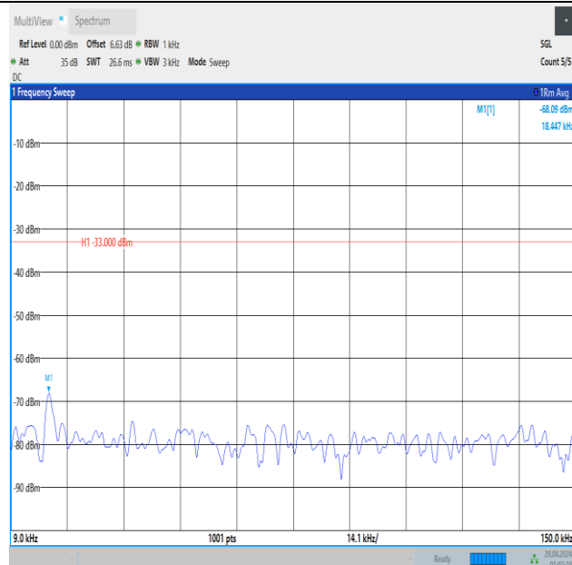
Band5_1.4MHz_QPSK_20643_1RB#0_0.009~0.15_0.009~0.15
