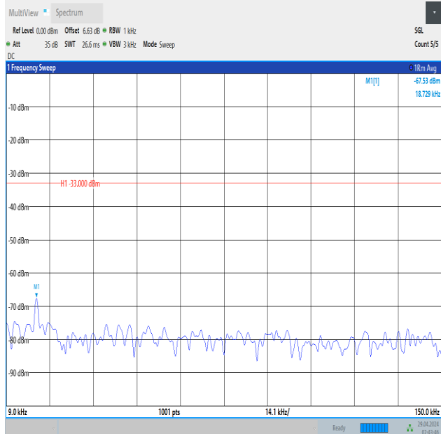
Band5_10MHz_16QAM_20600_1RB#49_0.009~0.15_0.009~0.15
