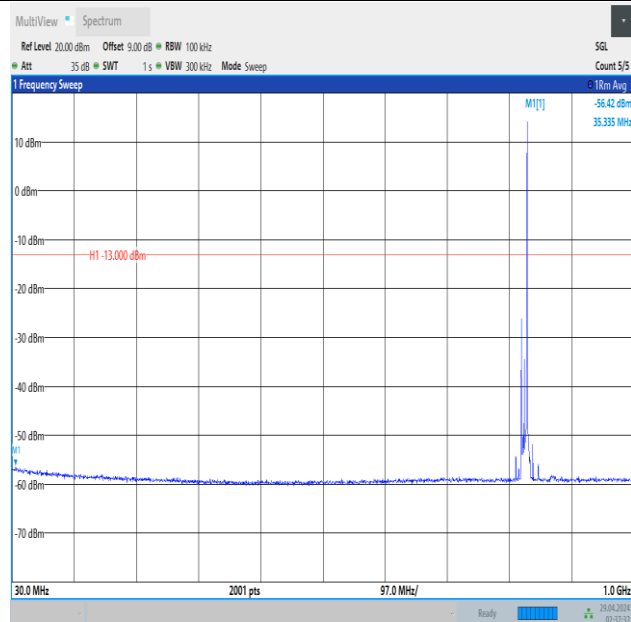
Band5_10MHz_16QAM_20450_1RB#49_30~1000_30~1000
