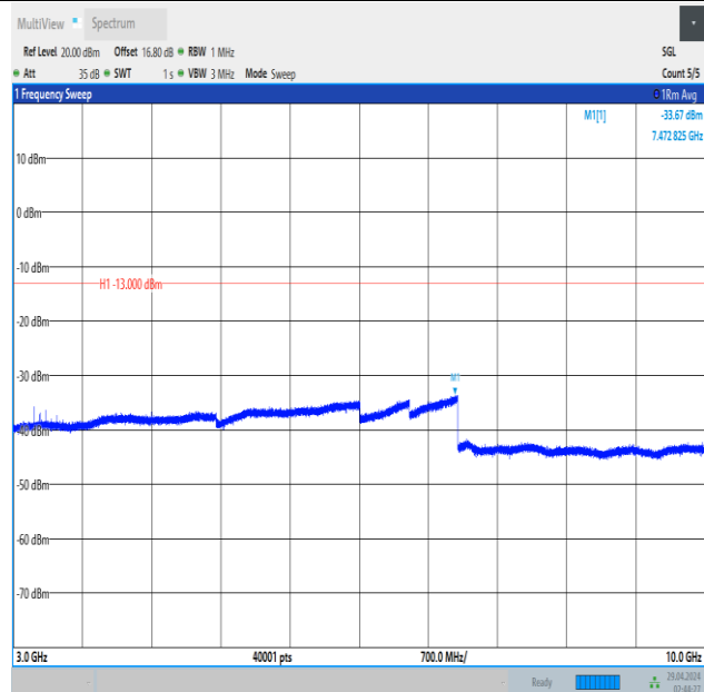
Band5_10MHz_16QAM_20600_1RB#49_3000~10000_3000~10000
