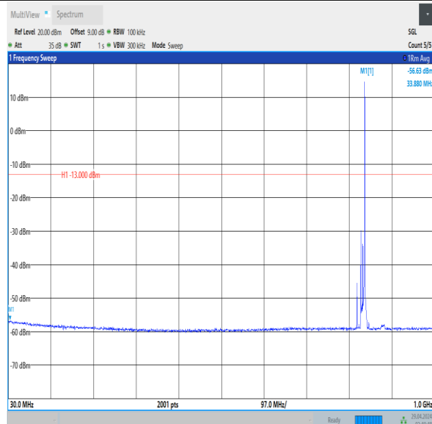
Band5_10MHz_16QAM_20525_1RB#49_30~1000_30~1000
