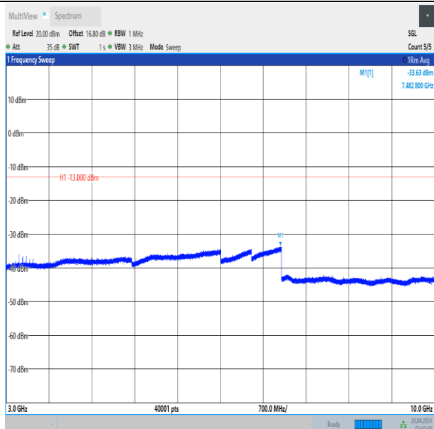
Band5_10MHz_QPSK_20600_1RB#49_3000~10000_3000~10000
