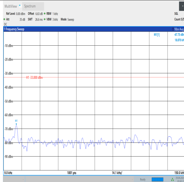
Band5_3MHz_16QAM_20415_1RB#0_0.009~0.15_0.009~0.15
