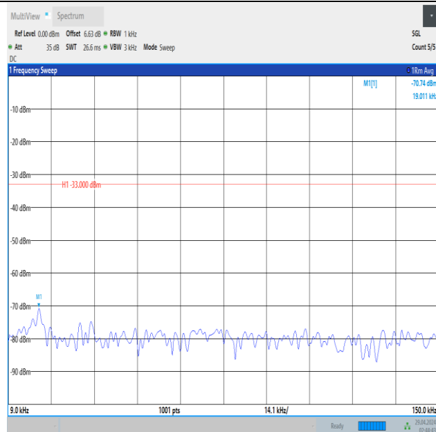
Band5_3MHz_QPSK_20415_1RB#0_0.009~0.15_0.009~0.15
