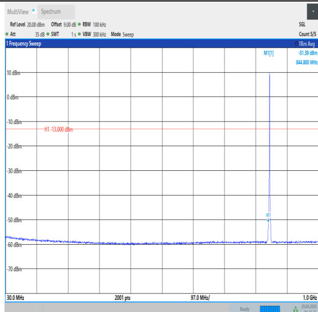
Band5_1.4MHz_16QAM_20643_6RB#0_30~1000_30~1000
