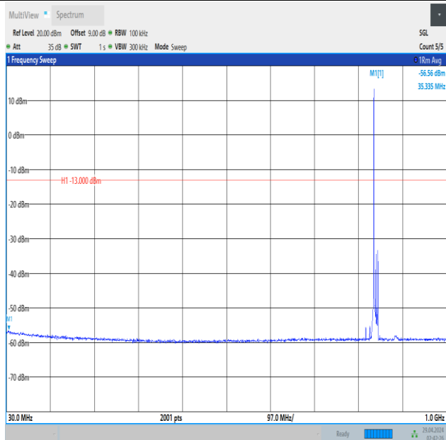
Band5_10MHz_16QAM_20600_1RB#0_30~1000_30~1000
