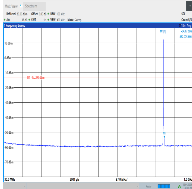
Band5_1.4MHz_QPSK_20643_1RB#5_30~1000_30~1000
