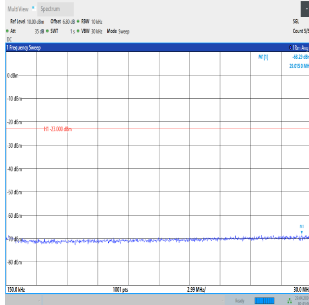
Band5_10MHz_QPSK_20600_1RB#49_0.15~30_0.15~30
