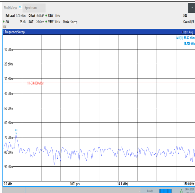
Band5_10MHz_QPSK_20450_1RB#0_0.009~0.15_0.009~0.15
