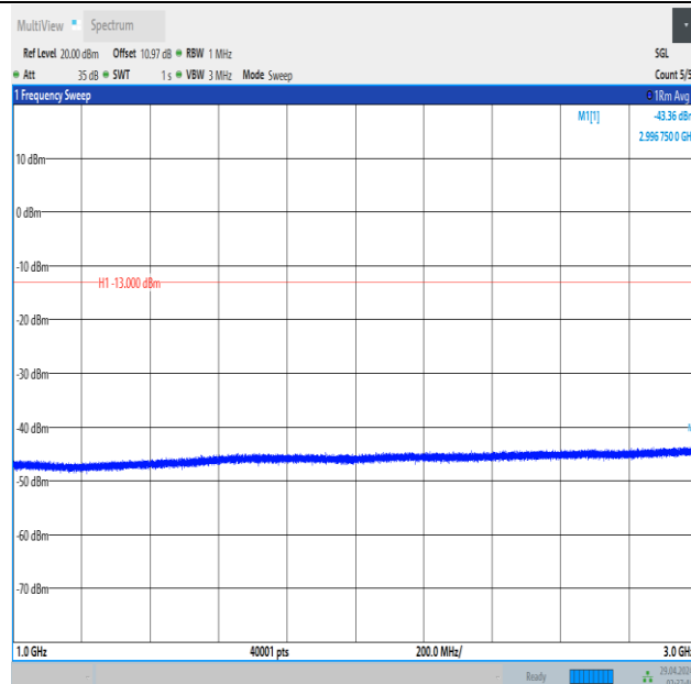
Band5_10MHz_16QAM_20450_1RB#49_1000~3000_1000~3000
