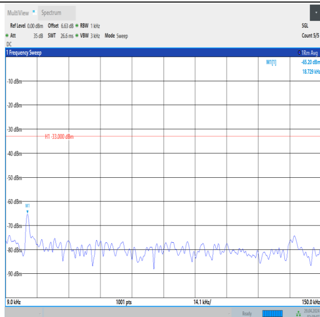
Band5_10MHz_QPSK_20525_1RB#0_0.009~0.15_0.009~0.15
