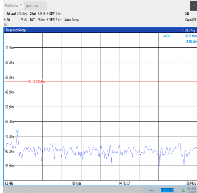
Band5_10MHz_16QAM_20525_1RB#49_0.009~0.15_0.009~0.15
