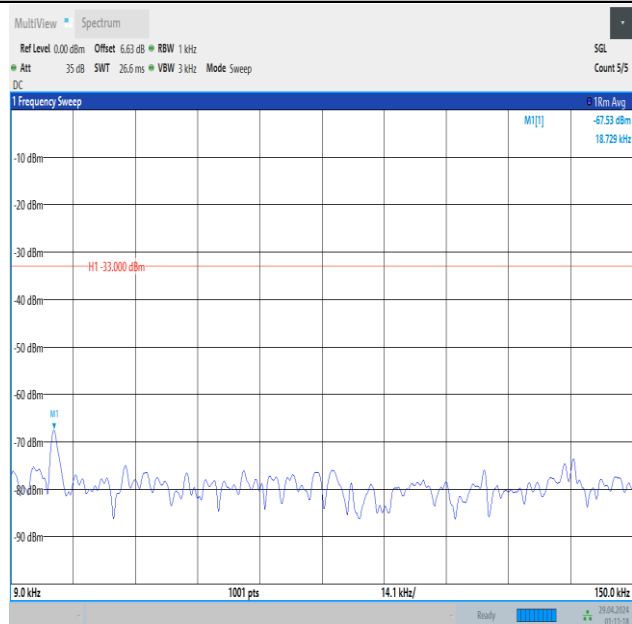
Band5_1.4MHz_16QAM_20643_6RB#0_0.009~0.15_0.009~0.15
