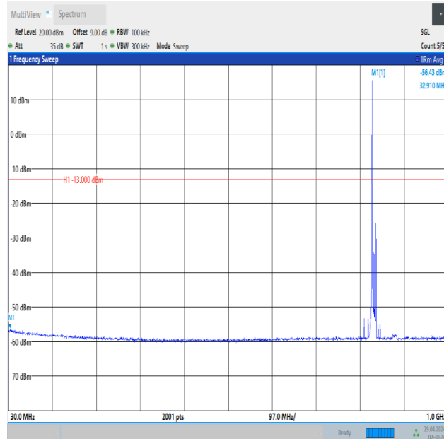
Band5_10MHz_QPSK_20525_1RB#0_30~1000_30~1000
