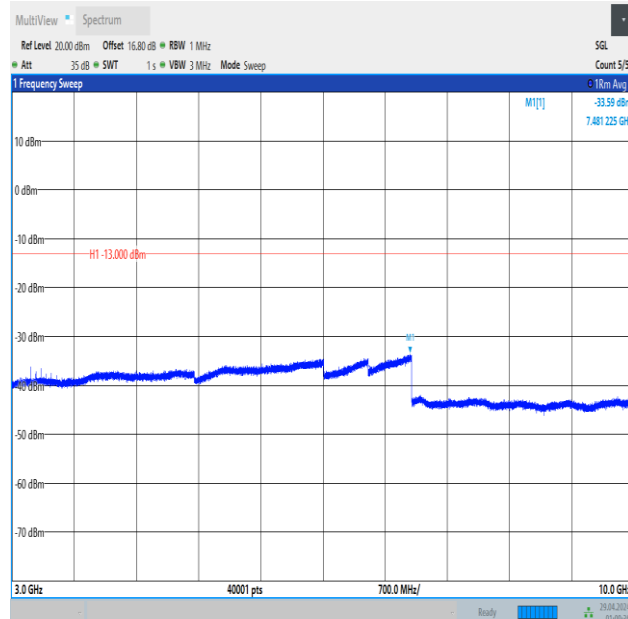
Band5_1.4MHz_QPSK_20643_1RB#5_3000~10000_3000~10000
