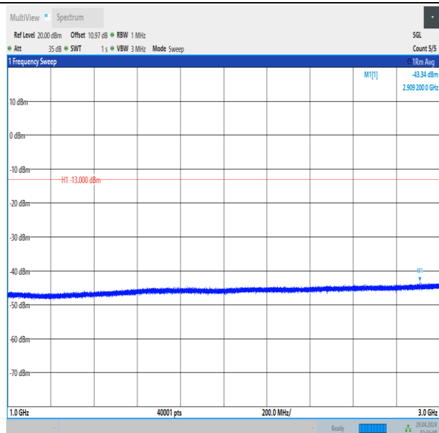
Band5_10MHz_16QAM_20450_1RB#0_1000~3000_1000~3000
