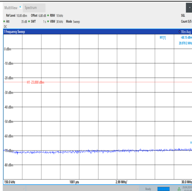
Band5_10MHz_16QAM_20450_1RB#0_0.15~30_0.15~30
