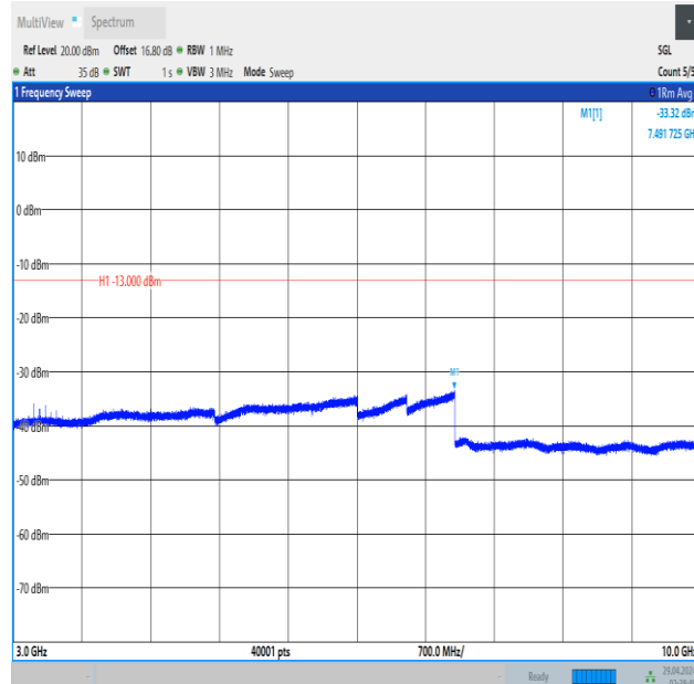
Band5_10MHz_QPSK_20525_1RB#0_3000~10000_3000~10000
