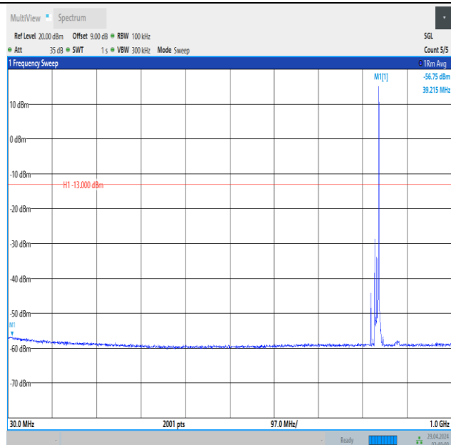
Band5_10MHz_QPSK_20525_1RB#49_30~1000_30~1000
