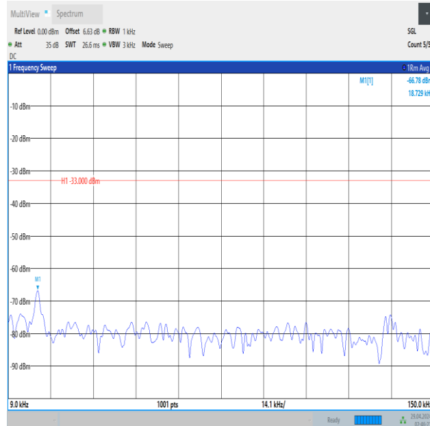
Band5_3MHz_QPSK_20415_1RB#14_0.009~0.15_0.009~0.15
