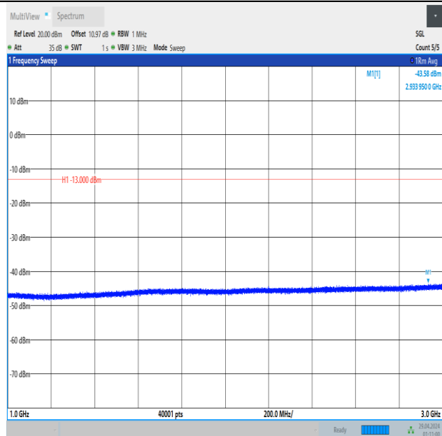
Band5_1.4MHz_QPSK_20643_6RB#0_1000~3000_1000~3000
