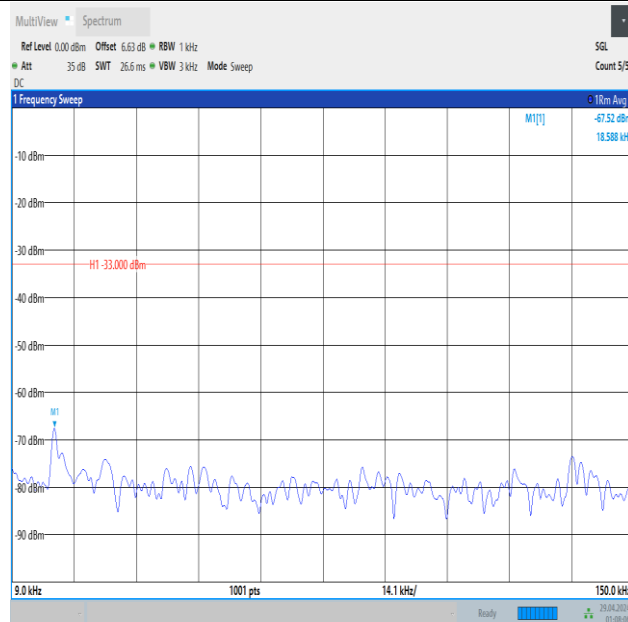
Band5_1.4MHz_16QAM_20643_1RB#0_0.009~0.15_0.009~0.15
