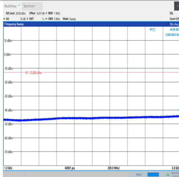
Band5_10MHz_QPSK_20600_1RB#0_1000~3000_1000~3000
