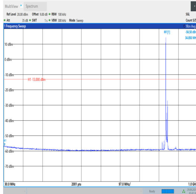
Band5_10MHz_QPSK_20600_1RB#0_30~1000_30~1000
