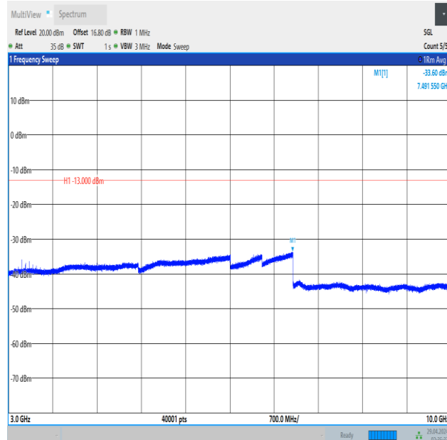
Band5_10MHz_QPSK_20450_1RB#0_3000~10000_3000~10000
