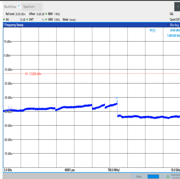
Band5_1.4MHz_16QAM_20643_1RB#5_3000~10000_3000~10000
