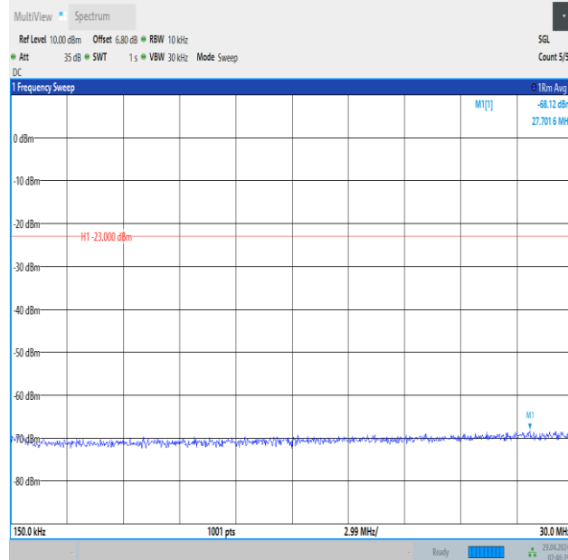
Band5_3MHz_QPSK_20415_1RB#14_0.15~30_0.15~30
