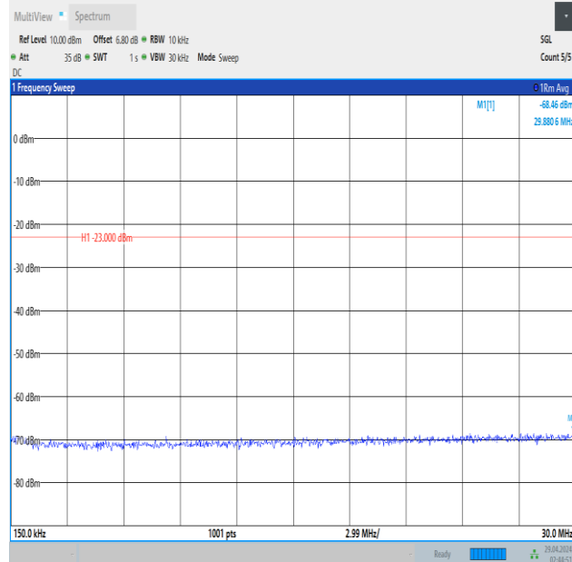
Band5_3MHz_QPSK_20415_1RB#0_0.15~30_0.15~30
