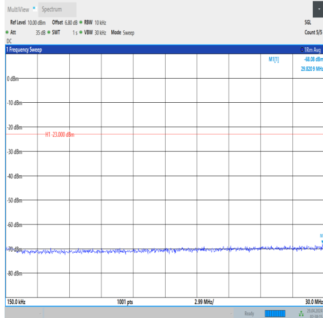
Band5_10MHz_QPSK_20525_1RB#0_0.15~30_0.15~30
