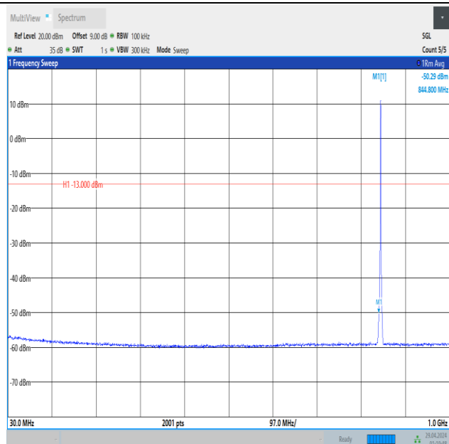
Band5_1.4MHz_QPSK_20643_6RB#0_30~1000_30~1000
