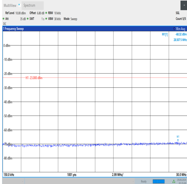
Band5_10MHz_QPSK_20450_1RB#0_0.15~30_0.15~30
