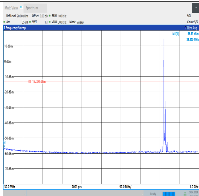
Band5_10MHz_QPSK_20450_1RB#0_30~1000_30~1000
