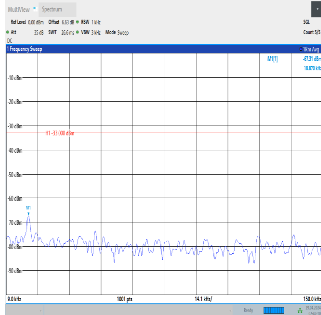
Band5_10MHz_16QAM_20600_1RB#0_0.009~0.15_0.009~0.15
