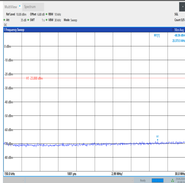
Band5_1.4MHz_16QAM_20643_1RB#0_0.15~30_0.15~30
