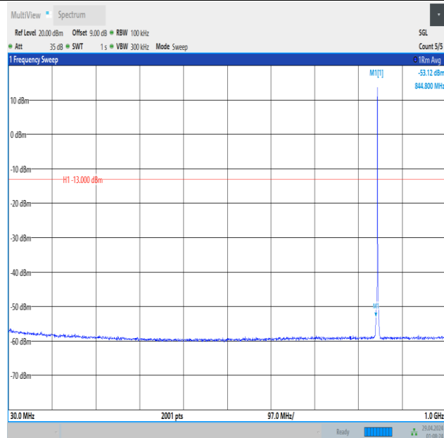
Band5_1.4MHz_16QAM_20643_1RB#0_30~1000_30~1000
