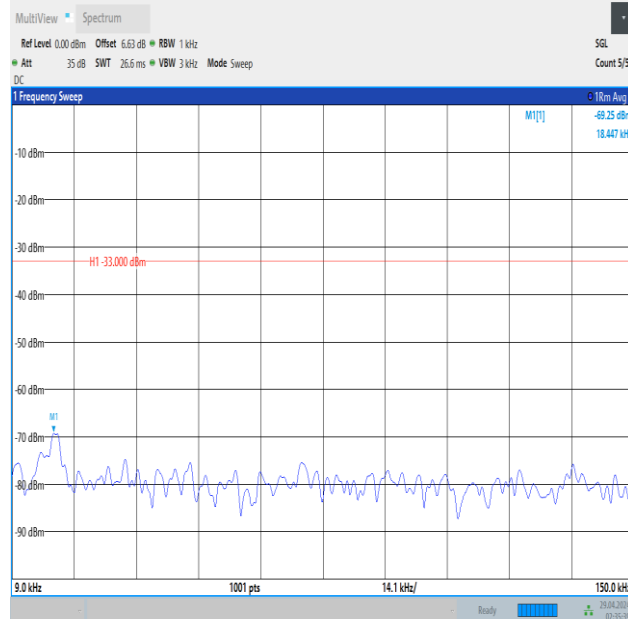
Band5_10MHz_16QAM_20450_1RB#0_0.009~0.15_0.009~0.15
