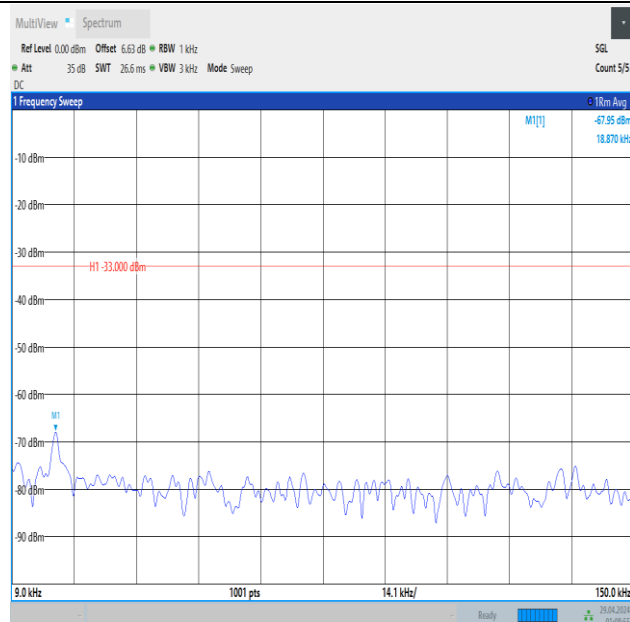
Band5_1.4MHz_QPSK_20643_1RB#5_0.009~0.15_0.009~0.15
