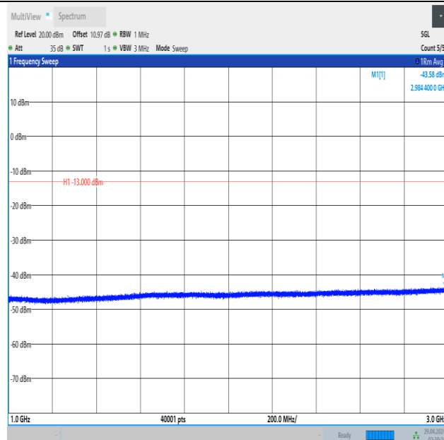
Band5_10MHz_16QAM_20525_1RB#0_1000~3000_1000~3000
