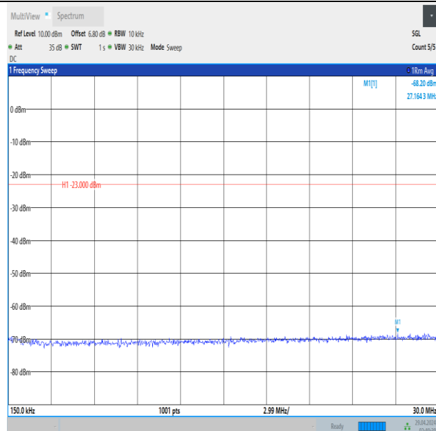
Band5_10MHz_16QAM_20525_1RB#49_0.15~30_0.15~30
