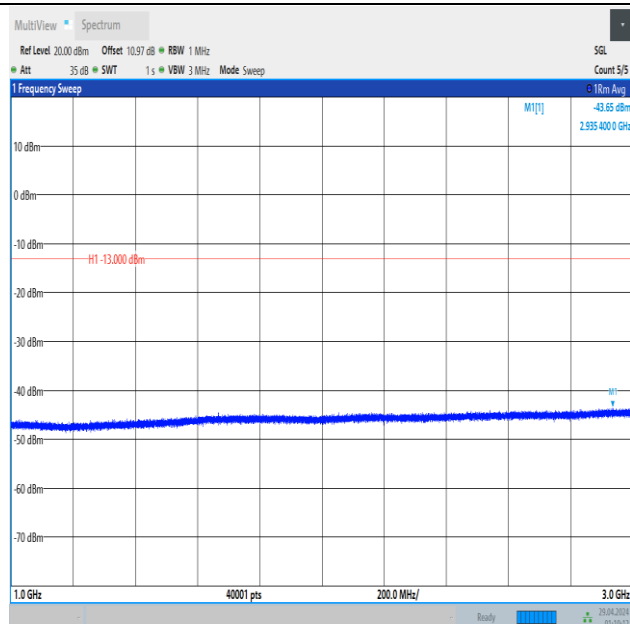
Band5_1.4MHz_16QAM_20643_1RB#5_1000~3000_1000~3000
