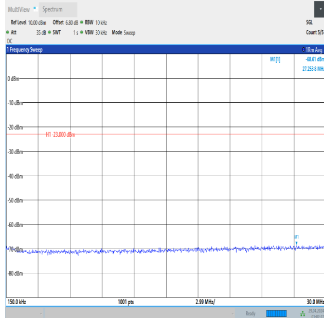
Band5_1.4MHz_QPSK_20643_1RB#0_0.15~30_0.15~30
