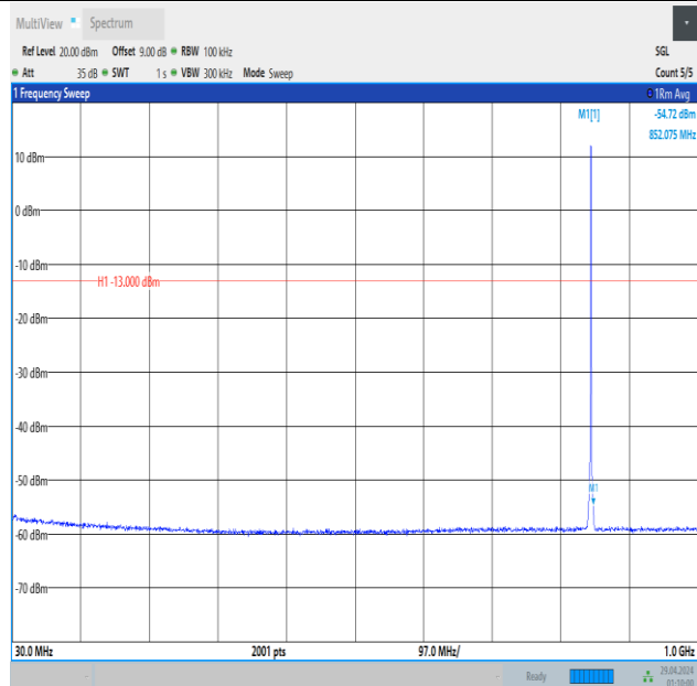
Band5_1.4MHz_16QAM_20643_1RB#5_30~1000_30~1000
