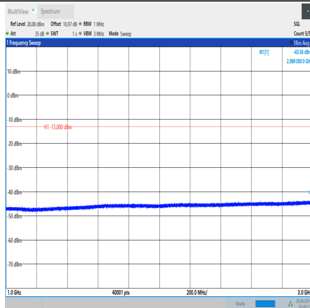
Band5_3MHz_QPSK_20415_1RB#0_1000~3000_1000~3000
