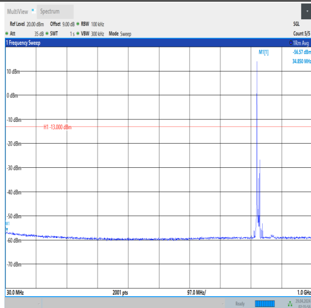
Band5_10MHz_16QAM_20450_1RB#0_30~1000_30~1000
