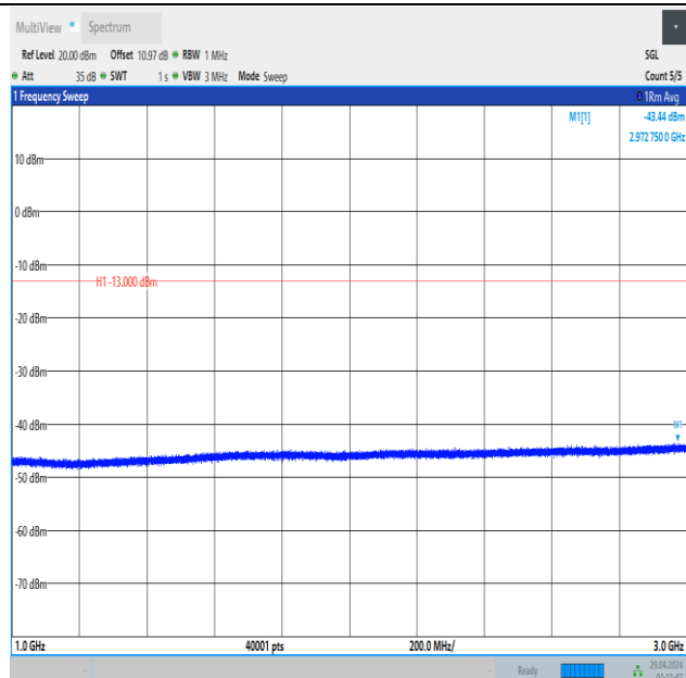
Band5_1.4MHz_16QAM_20643_6RB#0_1000~3000_1000~3000
