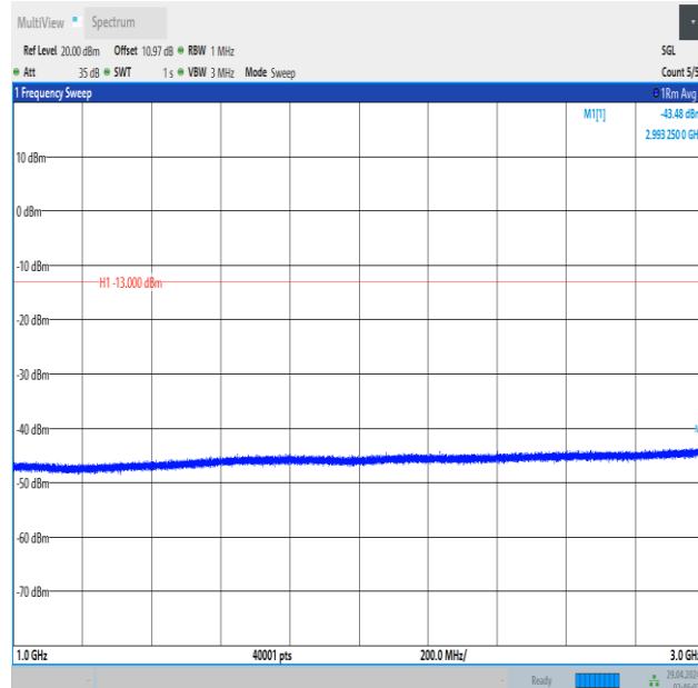
Band5_3MHz_16QAM_20415_1RB#0_1000~3000_1000~3000
