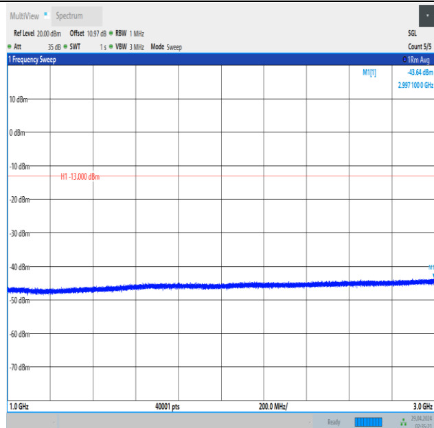
Band5_10MHz_QPSK_20450_1RB#0_1000~3000_1000~3000
