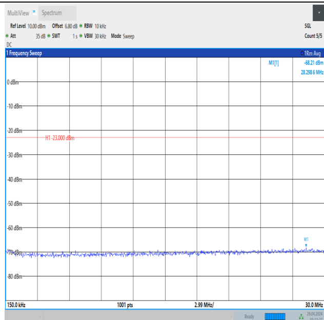
Band5_1.4MHz_16QAM_20643_6RB#0_0.15~30_0.15~30
