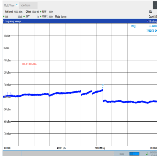
Band5_1.4MHz_16QAM_20643_1RB#0_3000~10000_3000~10000
