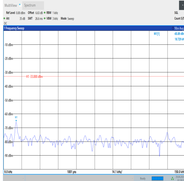
Band5_10MHz_16QAM_20525_1RB#0_0.009~0.15_0.009~0.15
