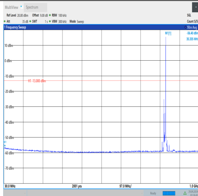
Band5_10MHz_QPSK_20450_1RB#49_30~1000_30~1000
