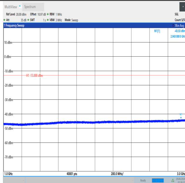
Band5_10MHz_QPSK_20450_1RB#49_1000~3000_1000~3000
