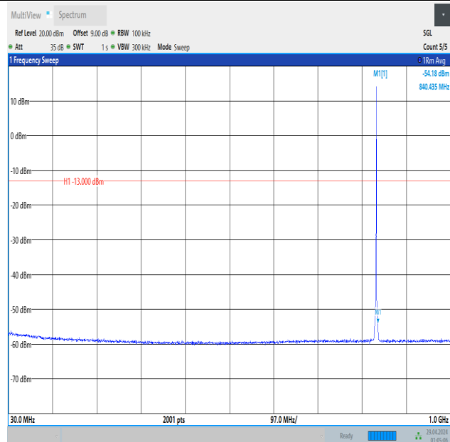
Band5_1.4MHz_16QAM_20525_1RB#5_30~1000_30~1000
