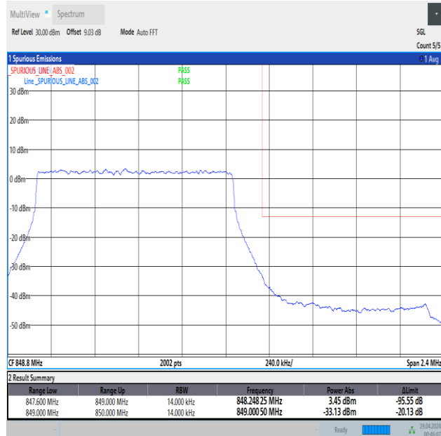
Band5_1.4MHz_QPSK_20643_6RB#0
