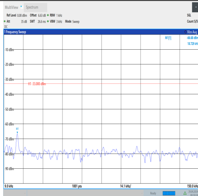
Band5_1.4MHz_16QAM_20407_1RB#5_0.009~0.15_0.009~0.15
