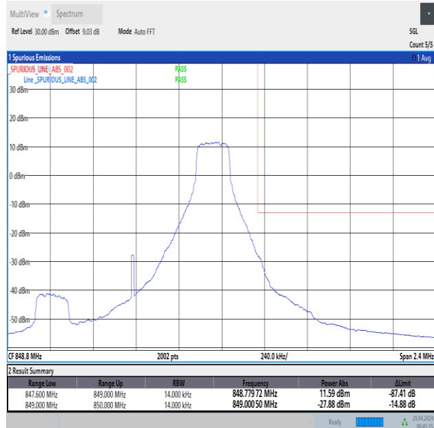
Band5_1.4MHz_QPSK_20643_1RB#5
