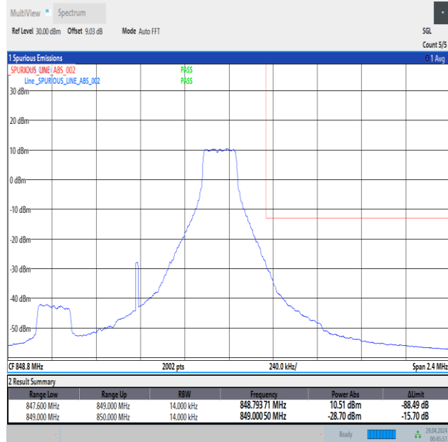
Band5_1.4MHz_16QAM_20643_1RB#5
