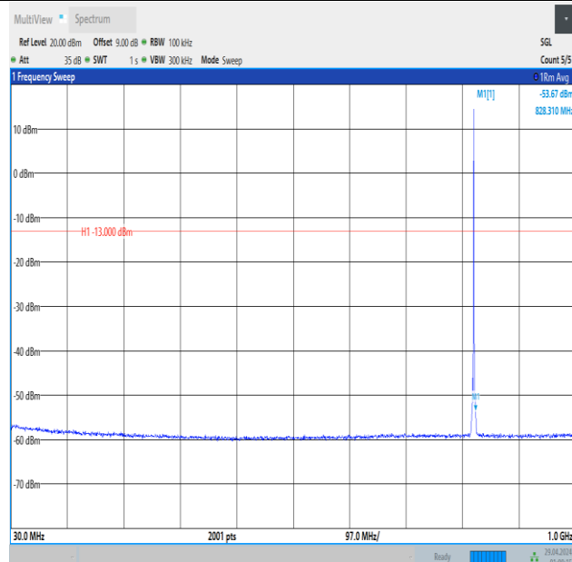
Band5_1.4MHz_16QAM_20407_1RB#5_30~1000_30~1000
