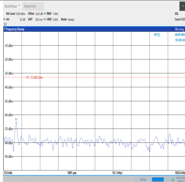
Band5_1.4MHz_16QAM_20407_1RB#0_0.009~0.15_0.009~0.15
