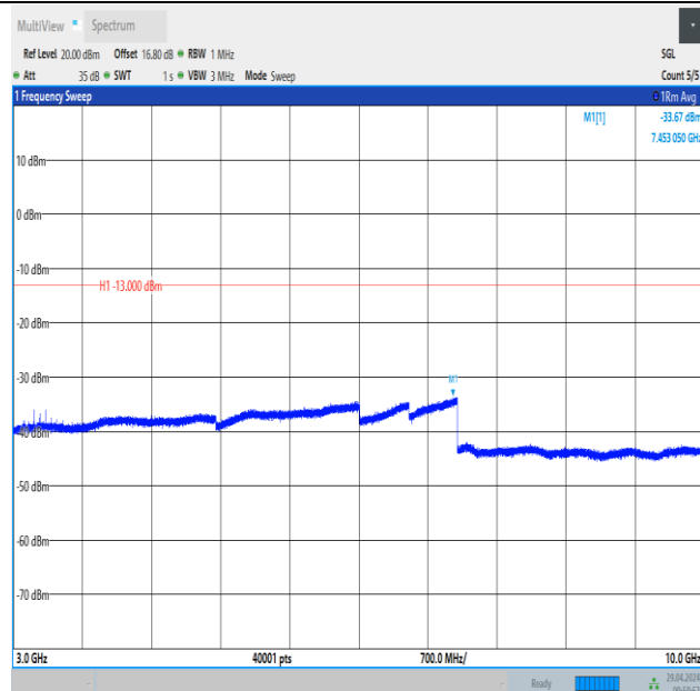
Band5_1.4MHz_QPSK_20407_1RB#5_3000~10000_3000~10000
