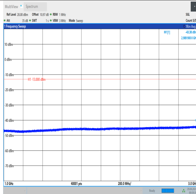
Band5_1.4MHz_QPSK_20407_1RB#5_1000~3000_1000~3000
