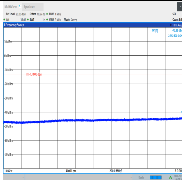
Band5_1.4MHz_16QAM_20407_1RB#0_1000~3000_1000~3000
