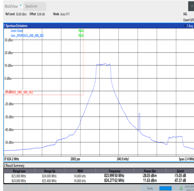
Band5_1.4MHz_QPSK_20407_1RB#0
