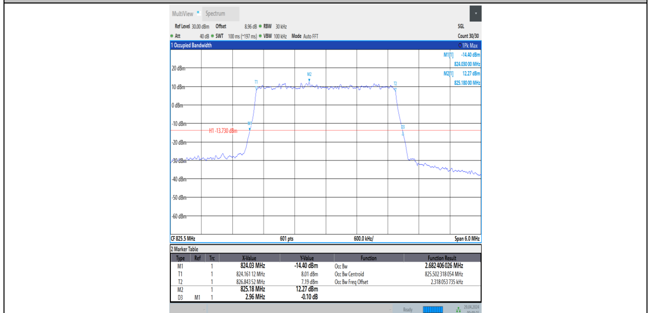
Band5-3MHz-16QAM-20415-15RB#0-PASS
