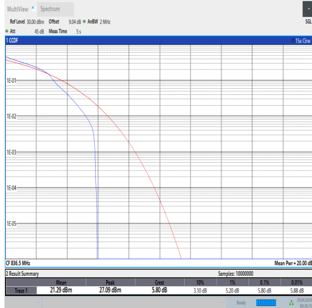
Band5-1.4MHz-16QAM-20525-1RB#0-PASS
