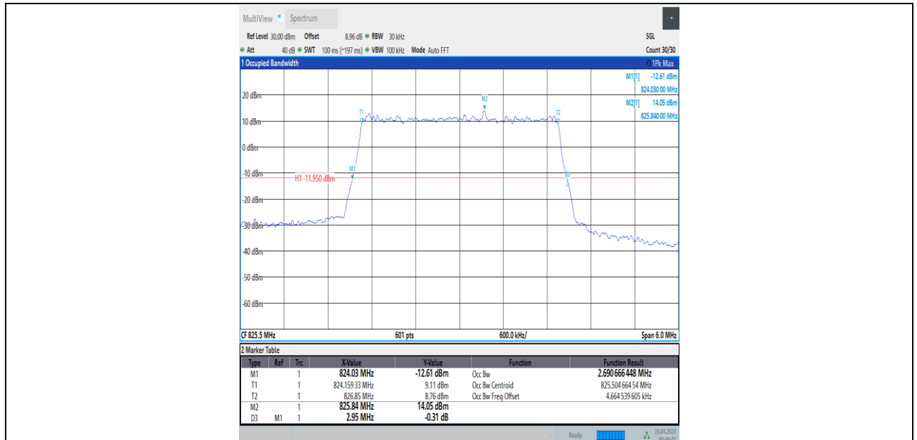
Band5-3MHz-QPSK-20415-15RB#0-PASS
