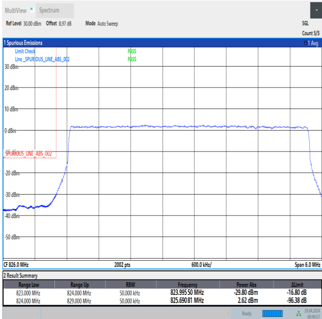
Band5_5MHz_QPSK_20425_25RB#0
