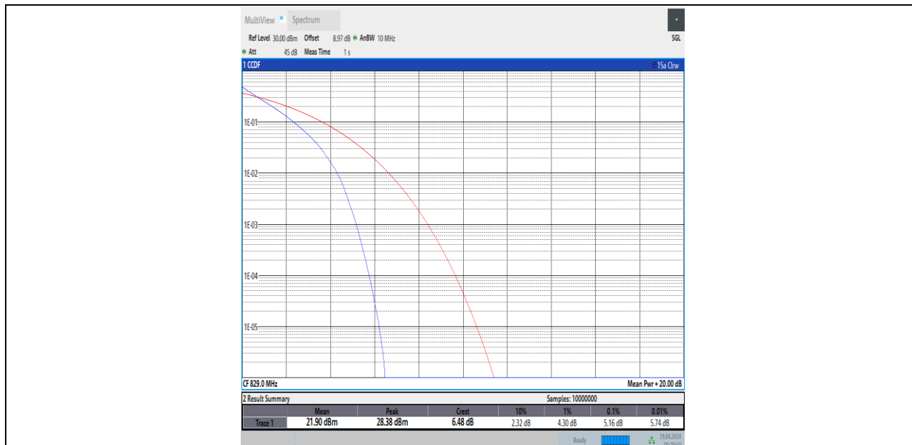
Band5-10MHz-QPSK-20450-50RB#0-PASS
