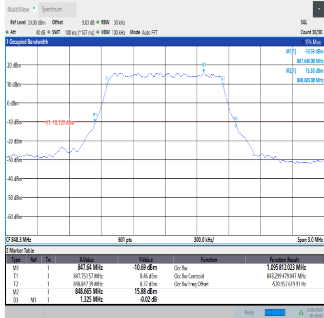
Band5-1.4MHz-QPSK-20643-6RB#0-PASS
