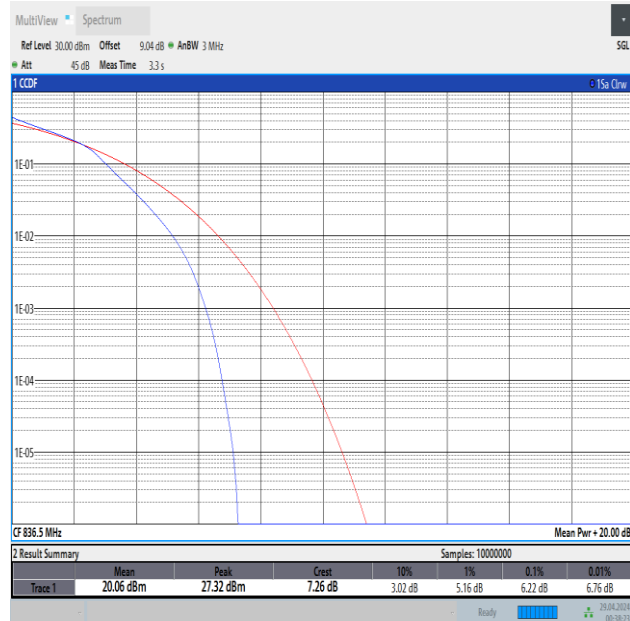
Band5-3MHz-16QAM-20525-15RB#0-PASS
