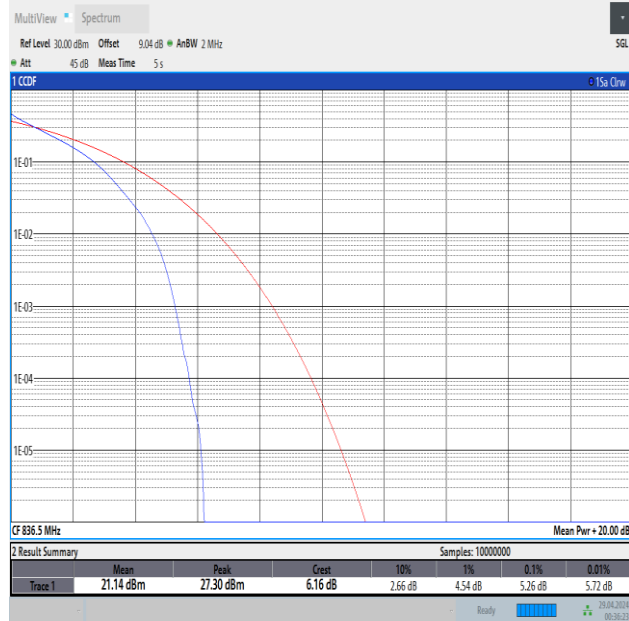
Band5-1.4MHz-QPSK-20525-6RB#0-PASS
