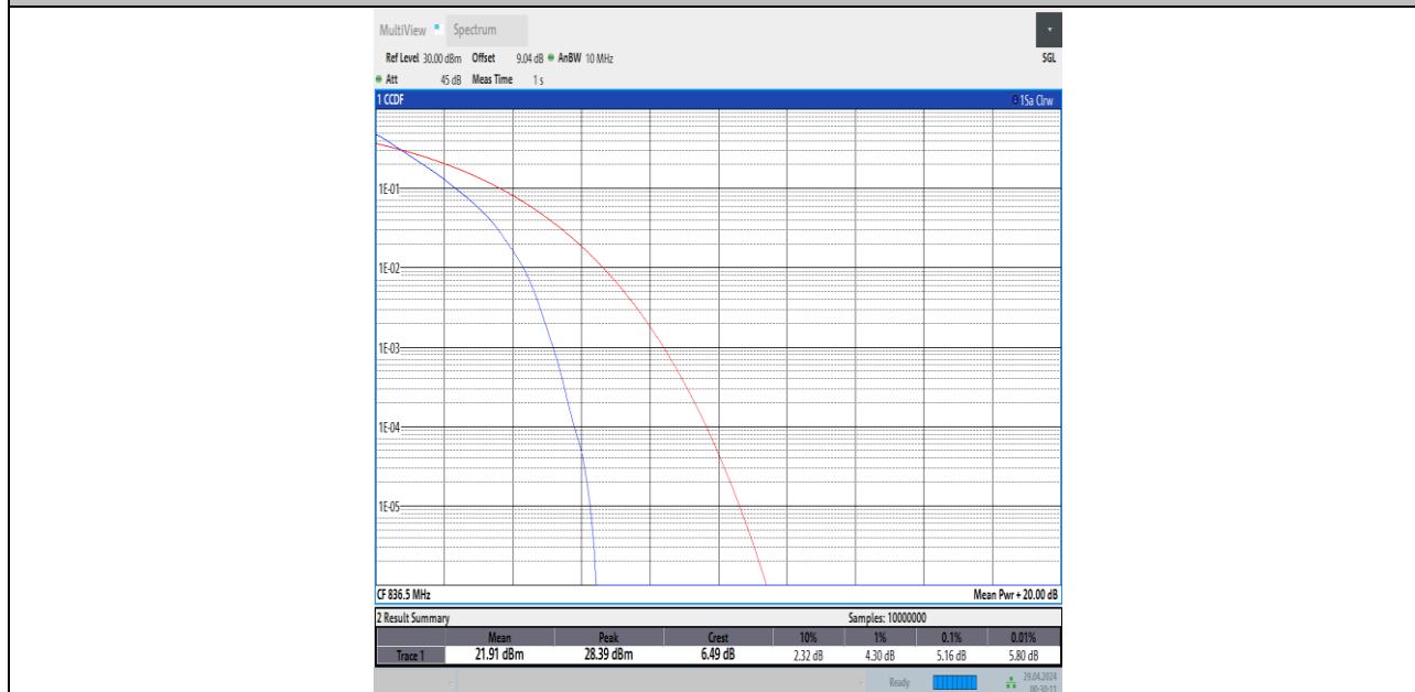
Band5-10MHz-QPSK-20525-50RB#0-PASS
