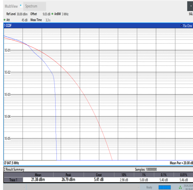
Band5-3MHz-16QAM-20635-1RB#0-PASS
