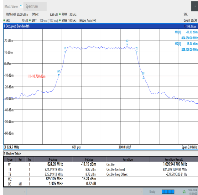
Band5-1.4MHz-16QAM-20407-6RB#0-PASS
