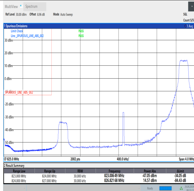
Band5_3MHz_16QAM_20415_1RB#14
