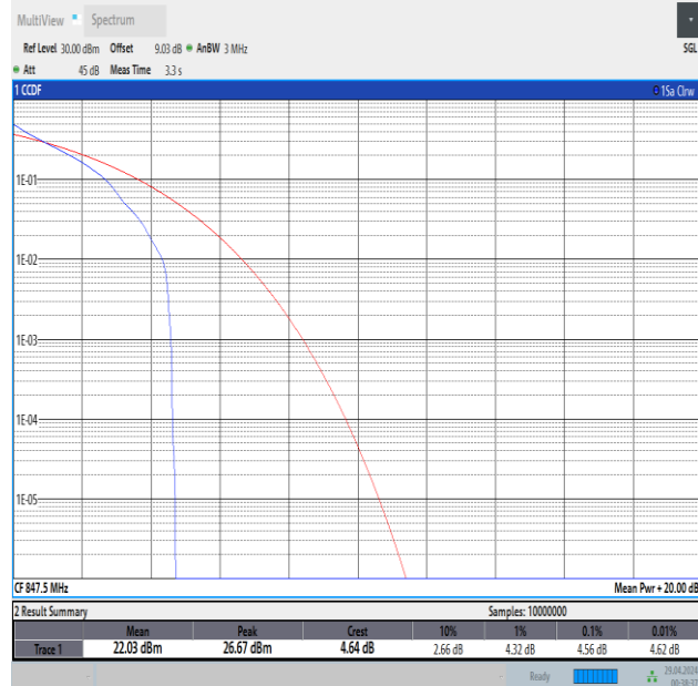
Band5-3MHz-QPSK-20635-1RB#0-PASS
