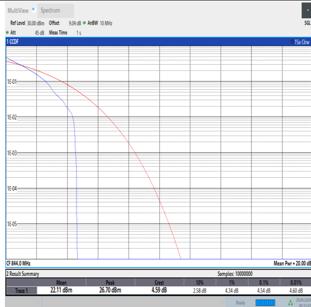
Band5-10MHz-QPSK-20600-1RB#0-PASS
