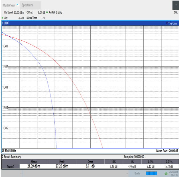
Band5-5MHz-QPSK-20525-25RB#0-PASS
