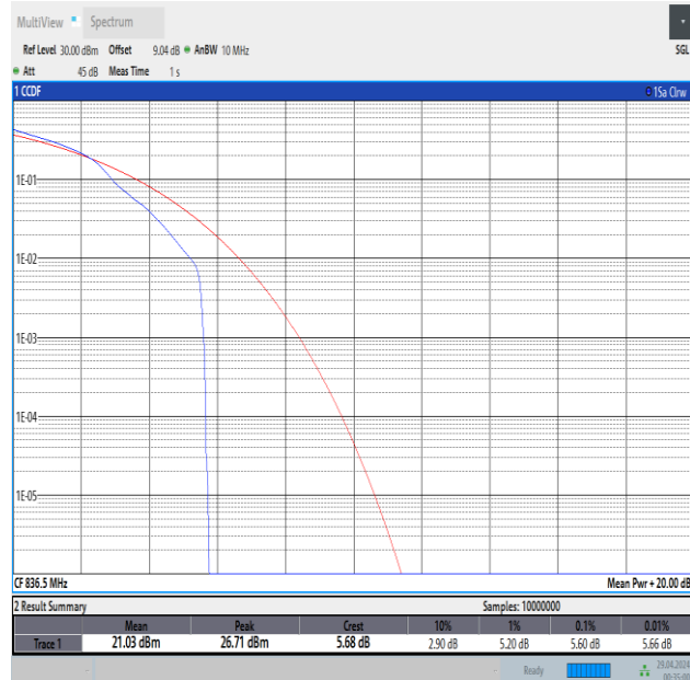
Band5-10MHz-16QAM-20525-1RB#0-PASS
