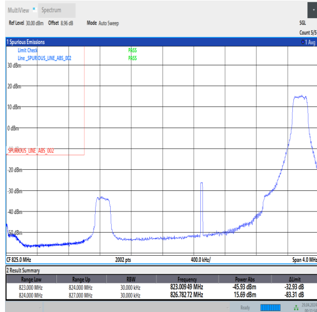
Band5_3MHz_QPSK_20415_1RB#14
