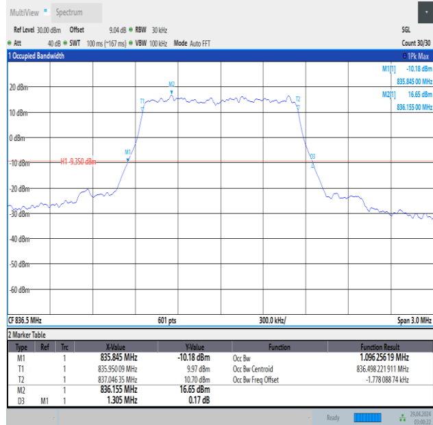
Band5-1.4MHz-QPSK-20525-6RB#0-PASS
