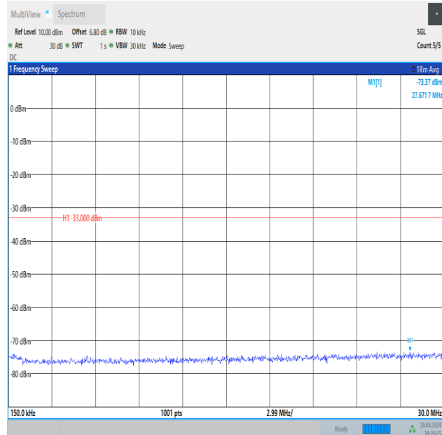
Band4_1.4MHz_QPSK_20175_1RB#0_0.15~30_0.15~30
