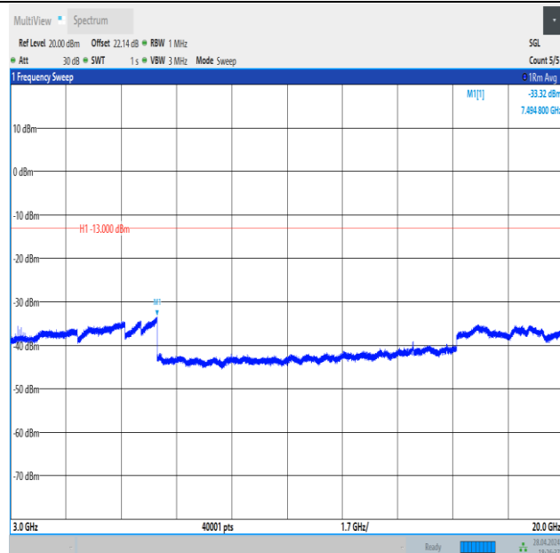
Band4_1.4MHz_16QAM_20393_1RB#0_3000~20000_3000~20000
