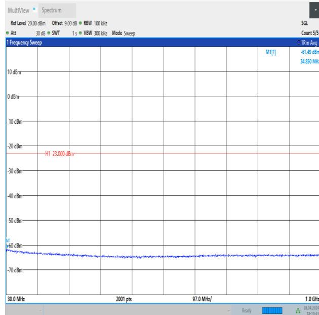
Band4_1.4MHz_16QAM_19957_6RB#0_30~1000_30~1000
