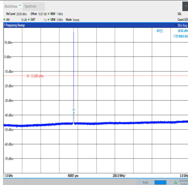
Band4_1.4MHz_16QAM_20393_6RB#0_1000~3000_1000~3000
