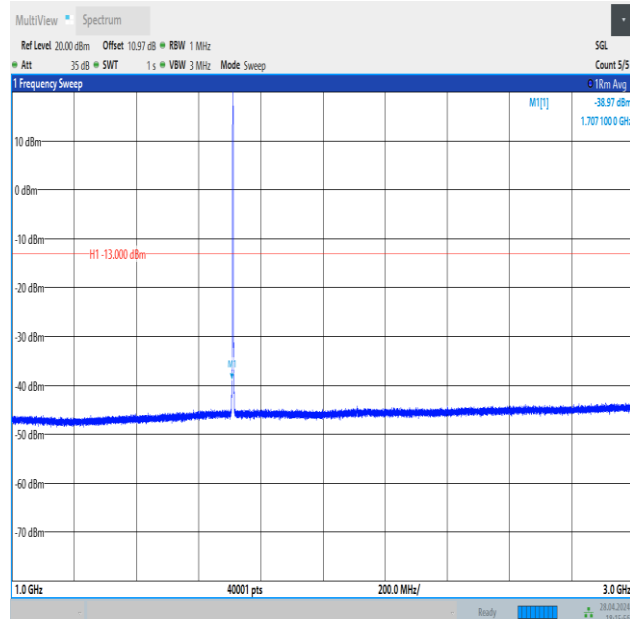
Band4_1.4MHz_QPSK_19957_1RB#0_1000~3000_1000~3000
