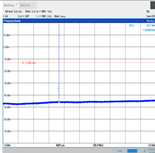
Band4_1.4MHz_16QAM_20175_6RB#0_1000~3000_1000~3000
