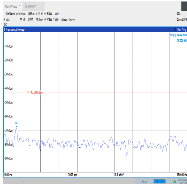
Band4_1.4MHz_QPSK_19957_1RB#0_0.009~0.15_0.009~0.15
