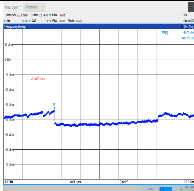
Band4_1.4MHz_16QAM_20175_1RB#0_3000~20000_3000~20000
