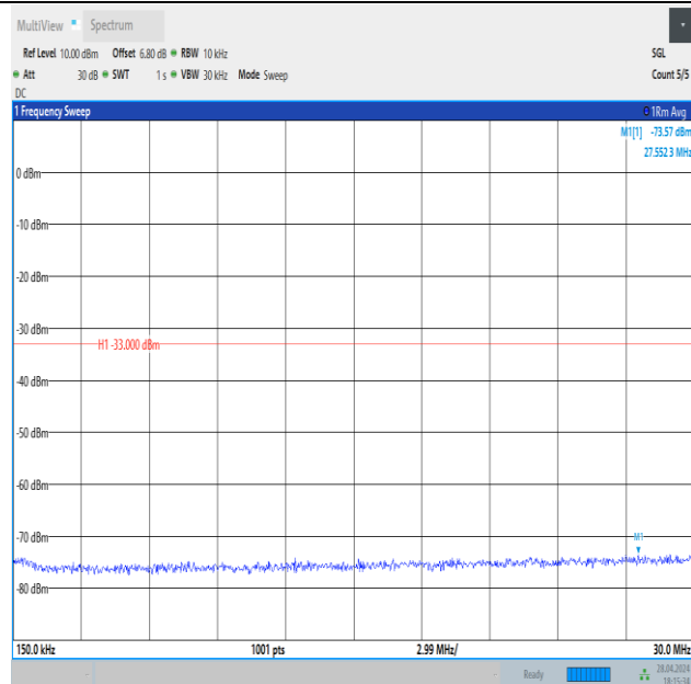
Band4_1.4MHz_QPSK_19957_1RB#0_0.15~30_0.15~30
