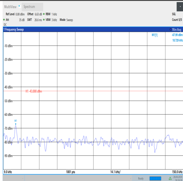
Band4_1.4MHz_QPSK_19957_6RB#0_0.009~0.15_0.009~0.15
