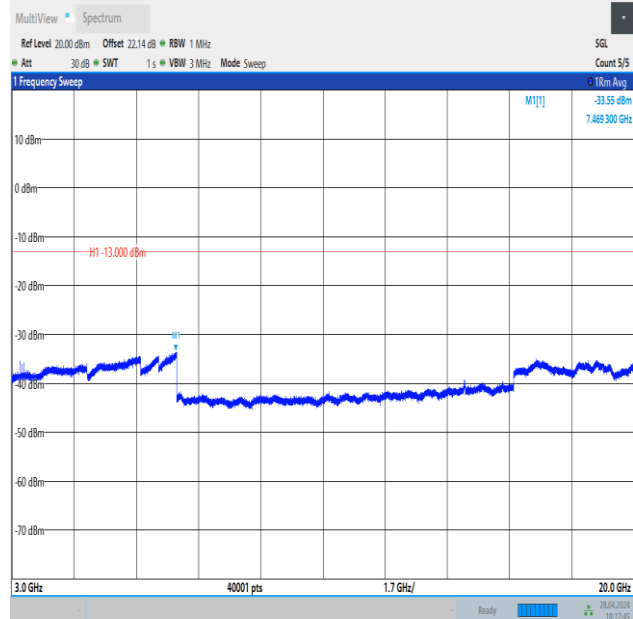
Band4_1.4MHz_QPSK_19957_1RB#5_3000~20000_3000~20000
