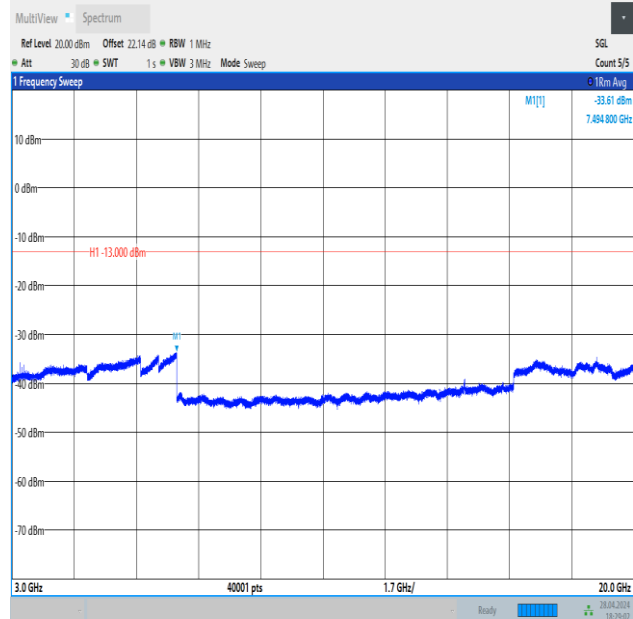
Band4_1.4MHz_QPSK_20393_6RB#0_3000~20000_3000~20000
