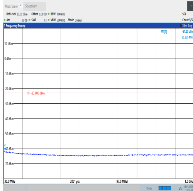
Band4_1.4MHz_16QAM_19957_1RB#0_30~1000_30~1000
