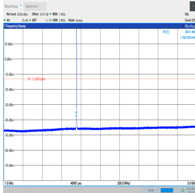
Band4_1.4MHz_QPSK_20393_1RB#0_1000~3000_1000~3000
