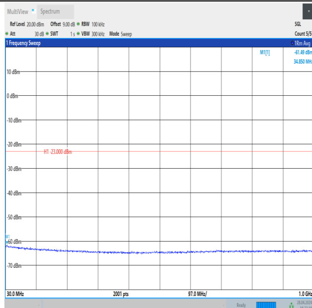
Band4_1.4MHz_QPSK_20175_1RB#5_30~1000_30~1000
