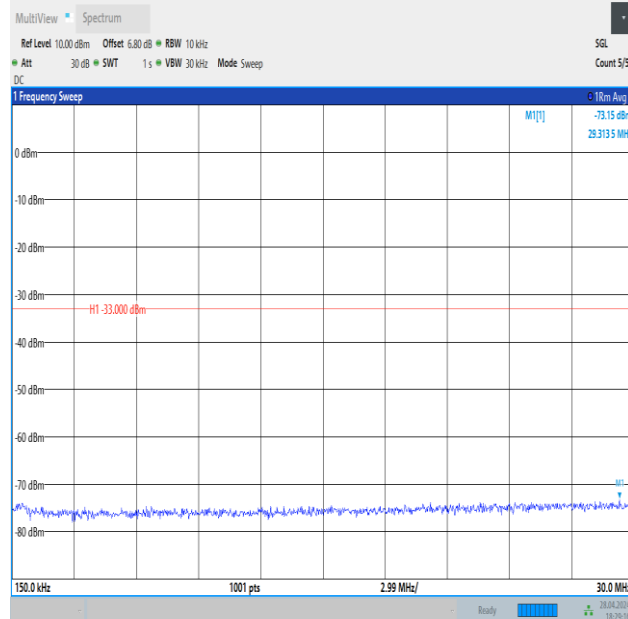
Band4_1.4MHz_16QAM_20393_6RB#0_0.15~30_0.15~30
