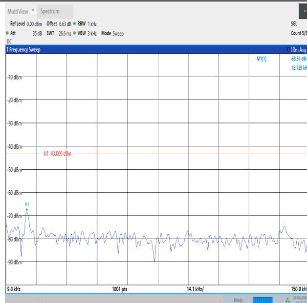
Band4_1.4MHz_QPSK_20393_1RB#0_0.009~0.15_0.009~0.15
