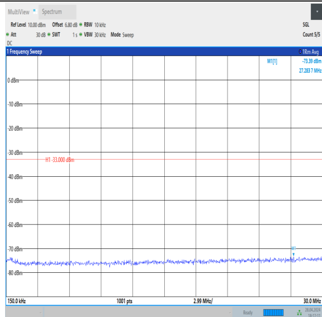
Band4_1.4MHz_QPSK_19957_1RB#5_0.15~30_0.15~30
