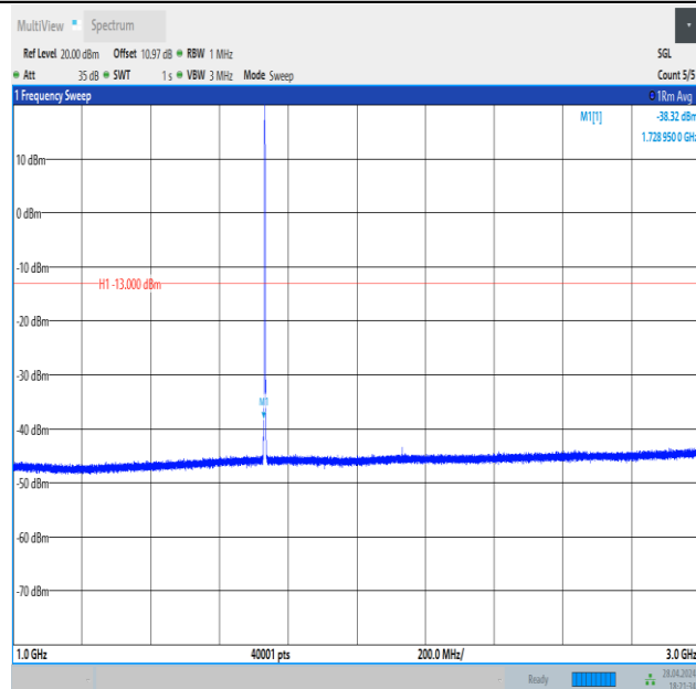
Band4_1.4MHz_16QAM_20175_1RB#0_1000~3000_1000~3000
