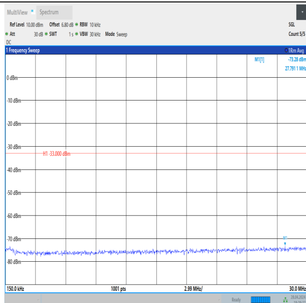
Band4_1.4MHz_QPSK_20393_6RB#0_0.15~30_0.15~30
