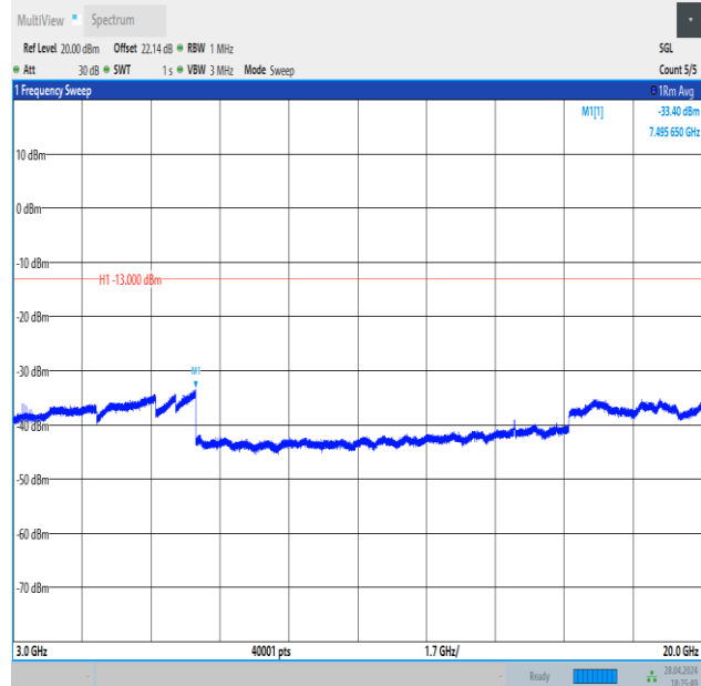
Band4_1.4MHz_QPSK_20393_1RB#0_3000~20000_3000~20000
