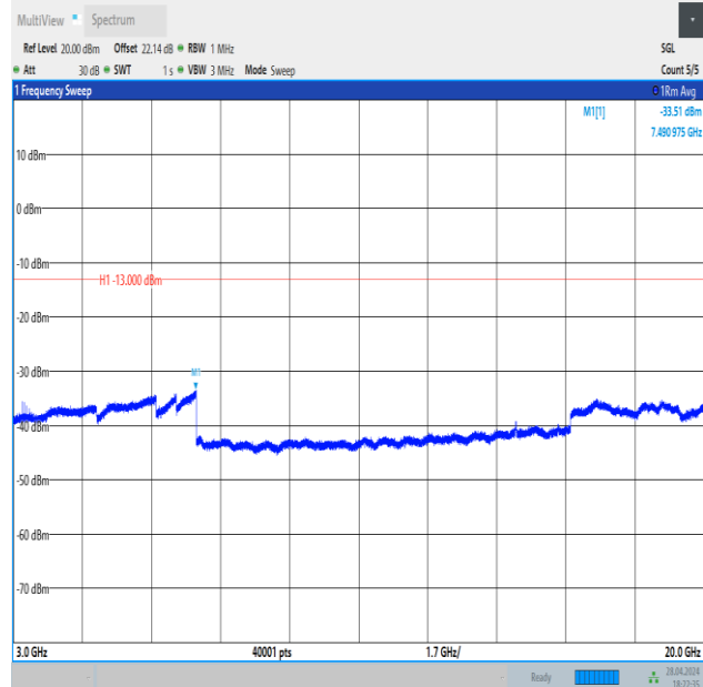
Band4_1.4MHz_QPSK_20175_1RB#5_3000~20000_3000~20000
