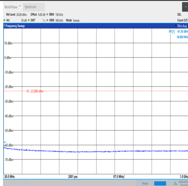
Band4_1.4MHz_QPSK_19957_1RB#0_30~1000_30~1000
