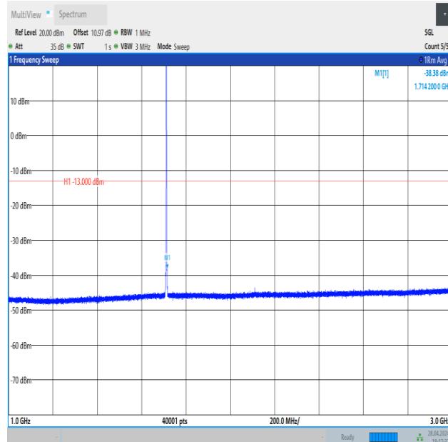
Band4_1.4MHz_QPSK_19957_1RB#5_1000~3000_1000~3000
