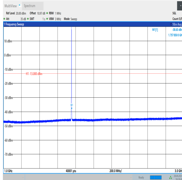
Band4_1.4MHz_QPSK_20393_6RB#0_1000~3000_1000~3000
