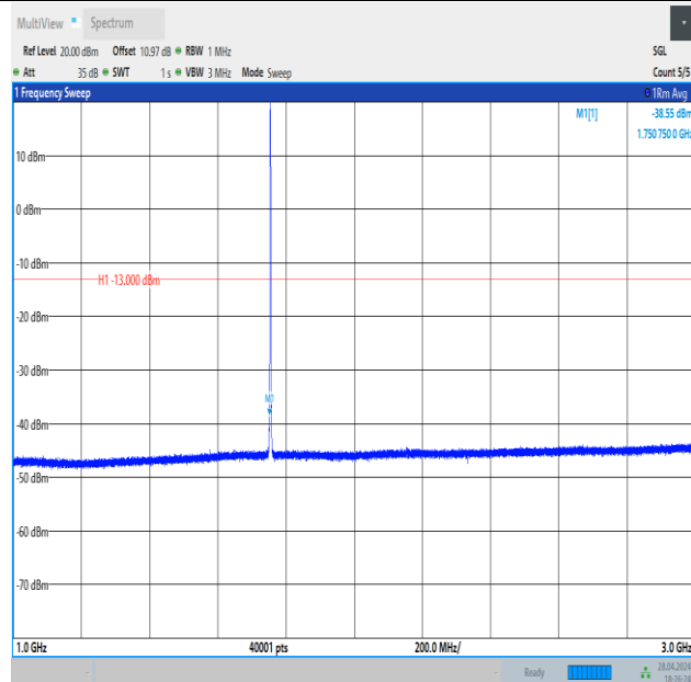
Band4_1.4MHz_16QAM_20393_1RB#0_1000~3000_1000~3000
