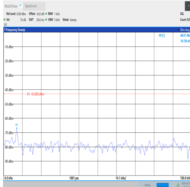
Band4_1.4MHz_16QAM_20175_1RB#5_0.009~0.15_0.009~0.15
