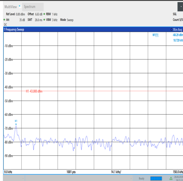
Band4_1.4MHz_QPSK_20175_1RB#5_0.009~0.15_0.009~0.15
