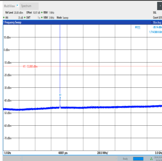
Band4_1.4MHz_16QAM_19957_1RB#5_1000~3000_1000~3000
