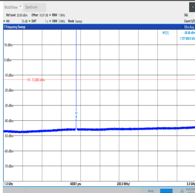
Band4_1.4MHz_QPSK_20393_1RB#5_1000~3000_1000~3000
