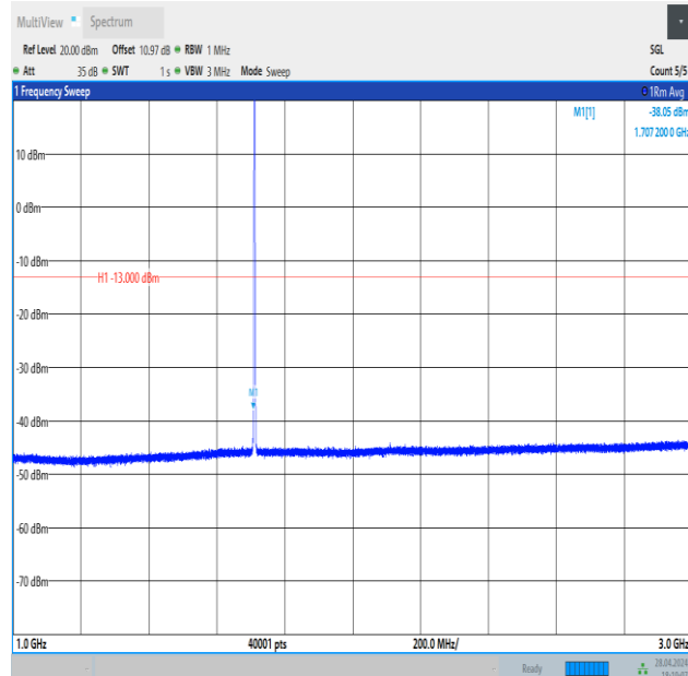
Band4_1.4MHz_QPSK_19957_6RB#0_1000~3000_1000~3000
