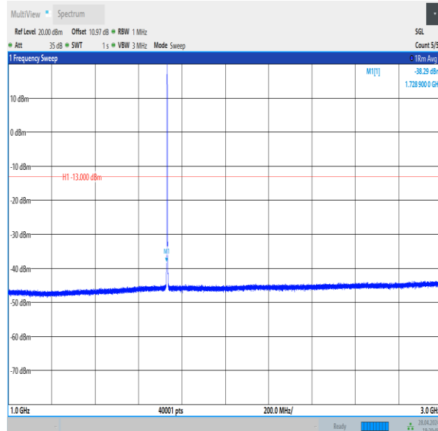
Band4_1.4MHz_QPSK_20175_1RB#0_1000~3000_1000~3000
