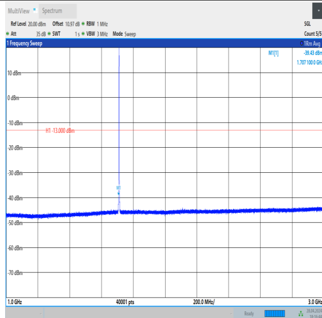
Band4_1.4MHz_16QAM_19957_1RB#0_1000~3000_1000~3000
