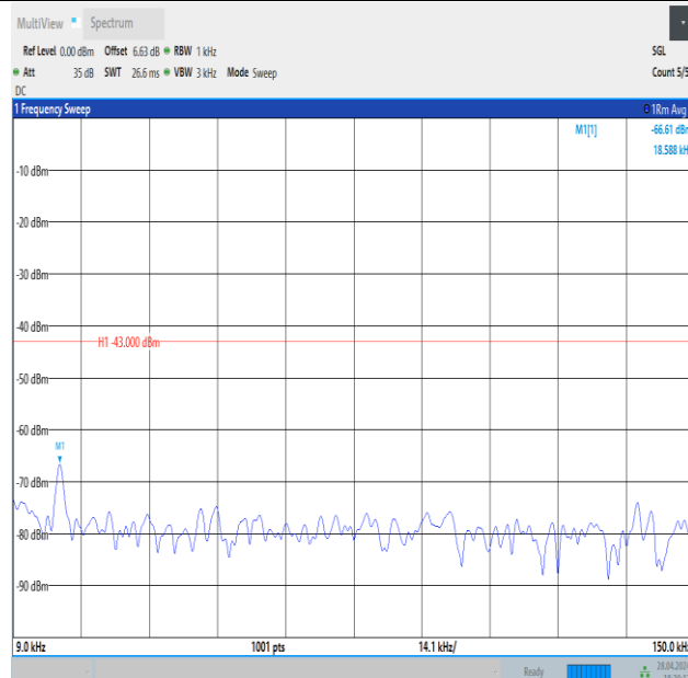
Band4_1.4MHz_QPSK_20175_1RB#0_0.009~0.15_0.009~0.15
