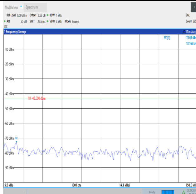
Band4_1.4MHz_QPSK_20393_6RB#0_0.009~0.15_0.009~0.15
