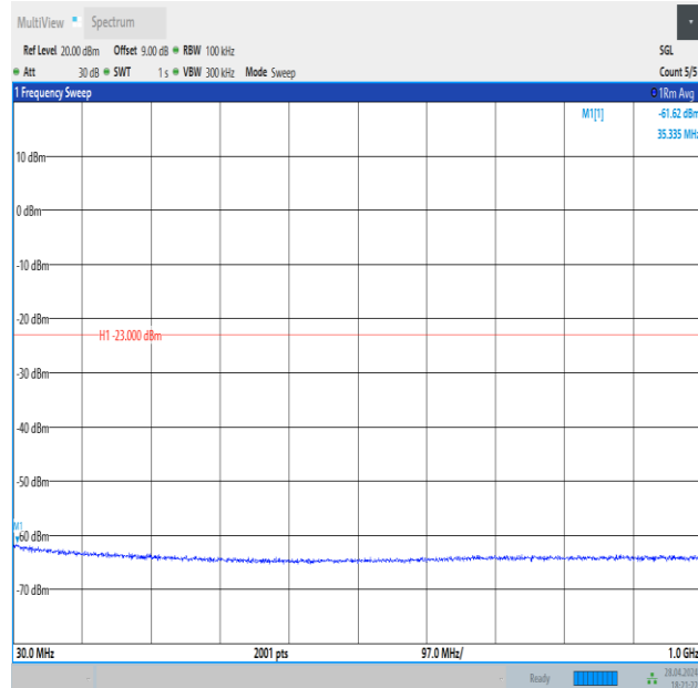
Band4_1.4MHz_16QAM_20175_1RB#0_30~1000_30~1000
