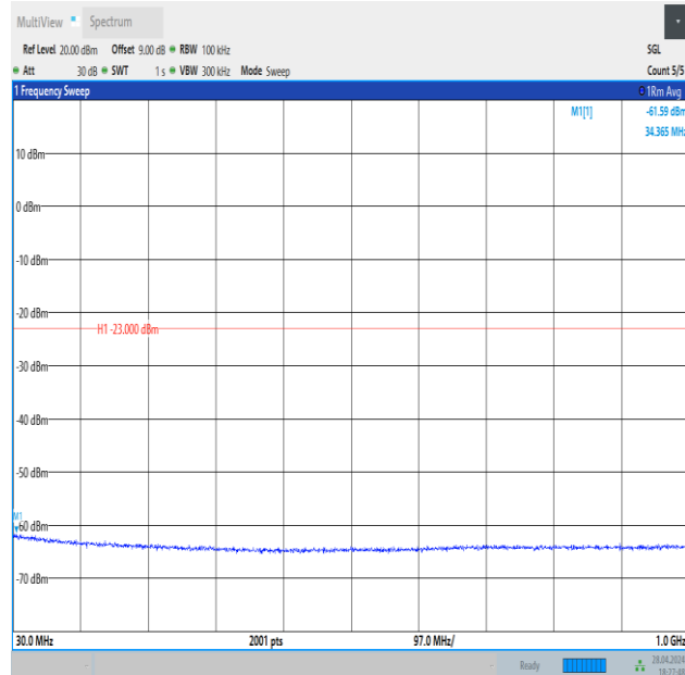
Band4_1.4MHz_16QAM_20393_1RB#5_30~1000_30~1000
