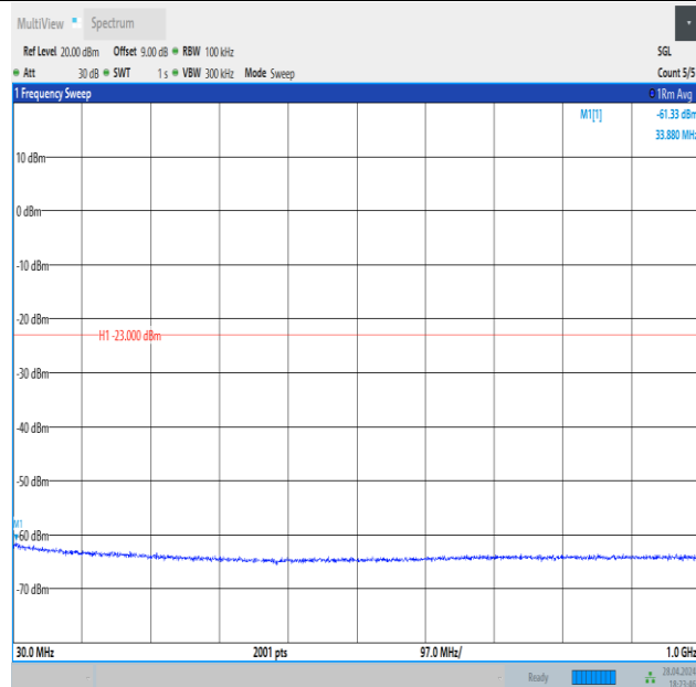
Band4_1.4MHz_QPSK_20175_6RB#0_30~1000_30~1000
