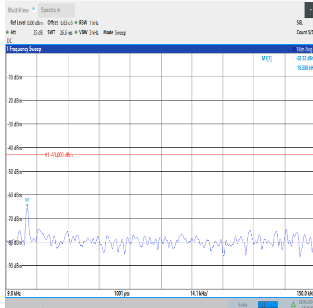
Band4_1.4MHz_16QAM_20393_1RB#0_0.009~0.15_0.009~0.15
