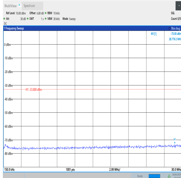
Band4_1.4MHz_QPSK_19957_6RB#0_0.15~30_0.15~30
