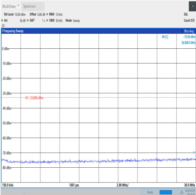
Band4_1.4MHz_QPSK_20393_1RB#0_0.15~30_0.15~30
