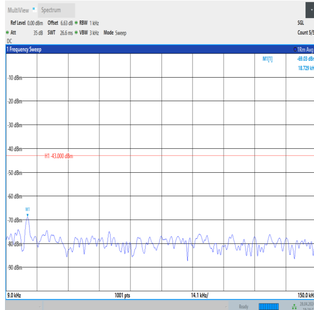
Band4_1.4MHz_16QAM_20175_6RB#0_0.009~0.15_0.009~0.15
