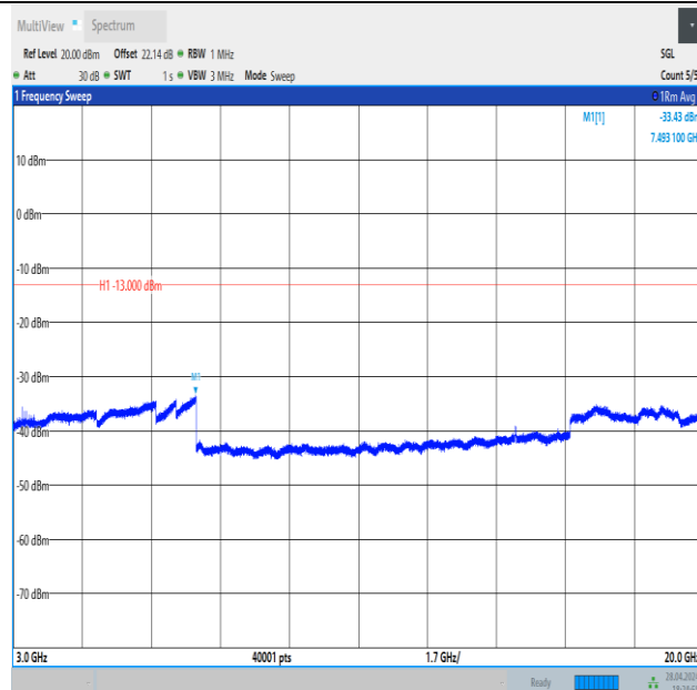
Band4_1.4MHz_16QAM_20175_6RB#0_3000~20000_3000~20000
