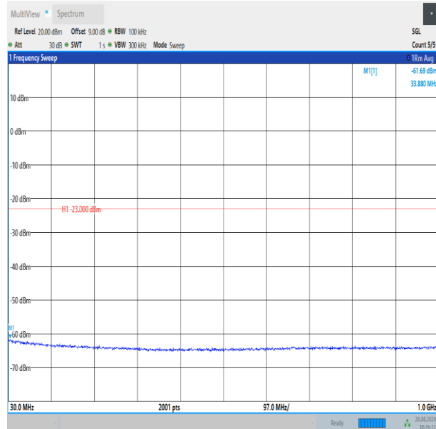
Band4_1.4MHz_16QAM_20393_1RB#0_30~1000_30~1000
