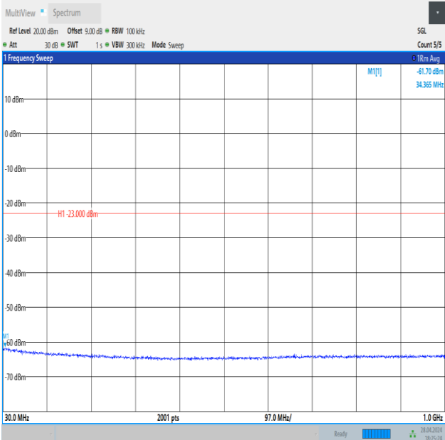
Band4_1.4MHz_QPSK_20393_1RB#0_30~1000_30~1000
