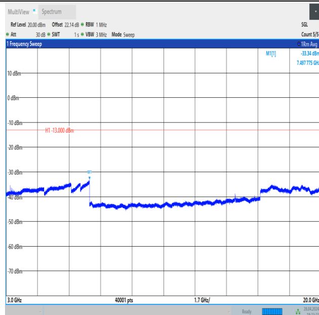
Band4_1.4MHz_16QAM_20175_1RB#5_3000~20000_3000~20000
