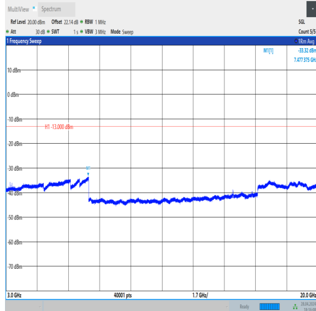
Band4_1.4MHz_QPSK_19957_1RB#0_3000~20000_3000~20000
