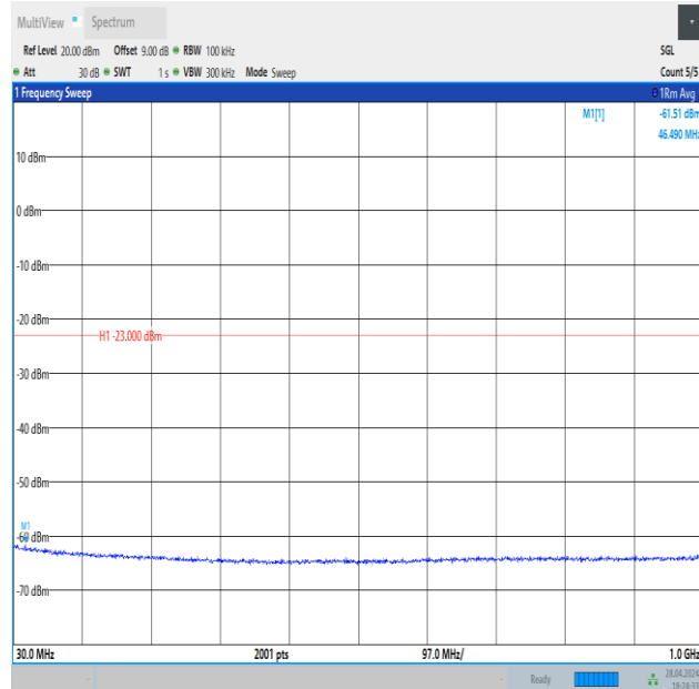
Band4_1.4MHz_16QAM_20175_6RB#0_30~1000_30~1000
