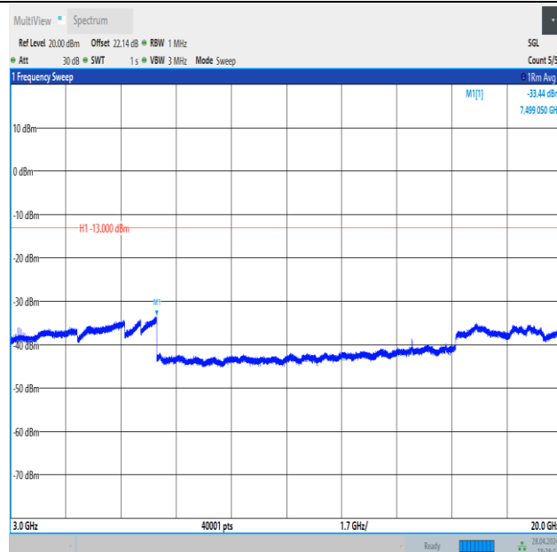
Band4_1.4MHz_16QAM_20393_1RB#5_3000~20000_3000~20000
