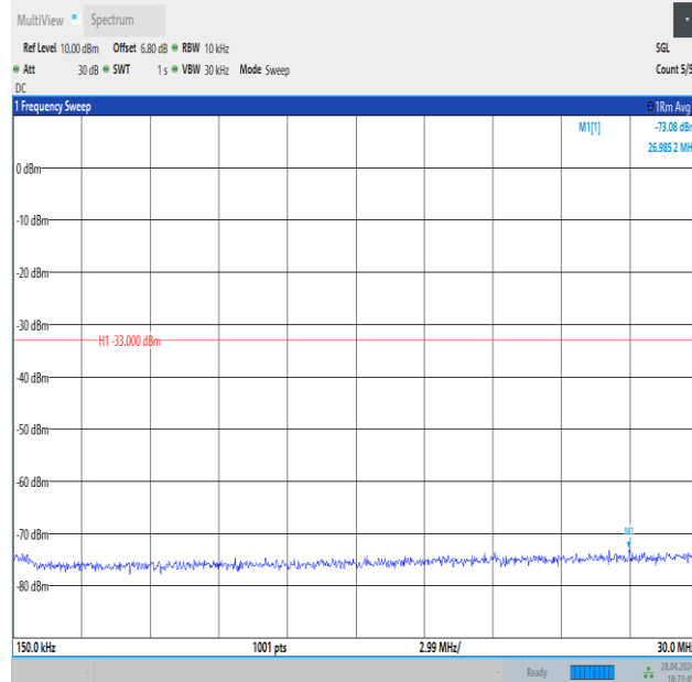
Band4_1.4MHz_16QAM_20175_1RB#5_0.15~30_0.15~30
