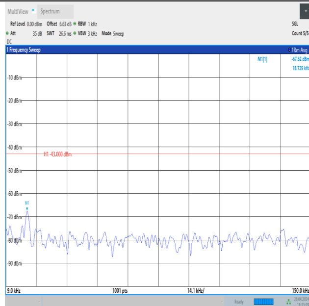
Band4_1.4MHz_QPSK_20175_6RB#0_0.009~0.15_0.009~0.15
