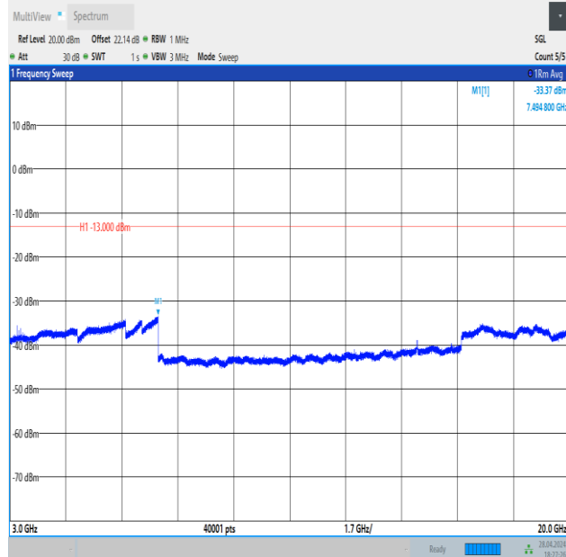
Band4_1.4MHz_QPSK_20393_1RB#5_3000~20000_3000~20000
