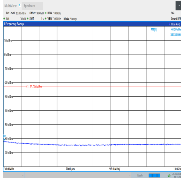
Band4_1.4MHz_16QAM_20393_6RB#0_30~1000_30~1000
