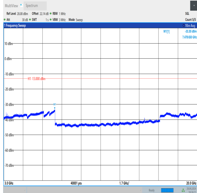
Band4_1.4MHz_QPSK_20175_6RB#0_3000~20000_3000~20000
