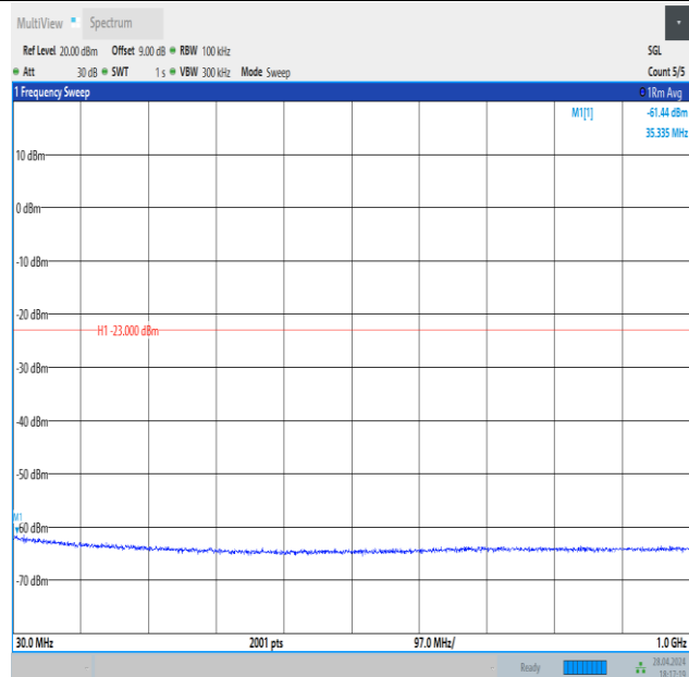
Band4_1.4MHz_QPSK_19957_1RB#5_30~1000_30~1000
