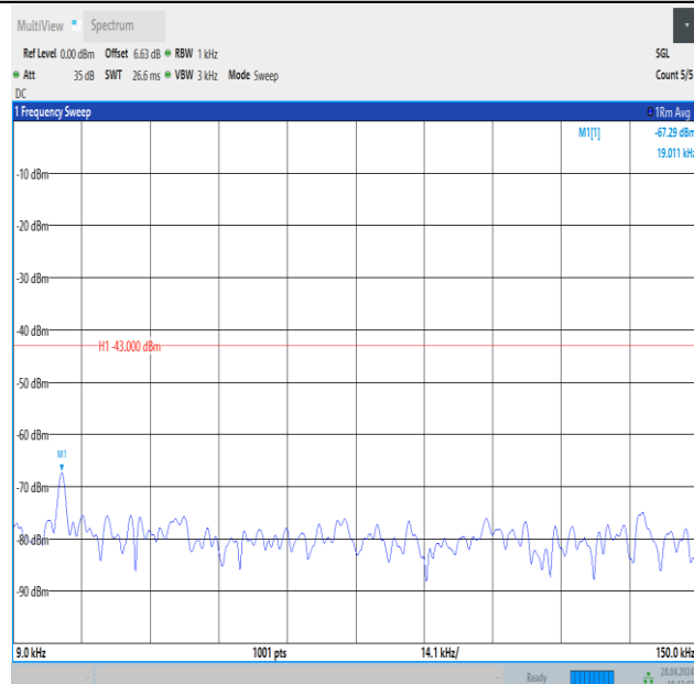
Band4_1.4MHz_QPSK_19957_1RB#5_0.009~0.15_0.009~0.15
