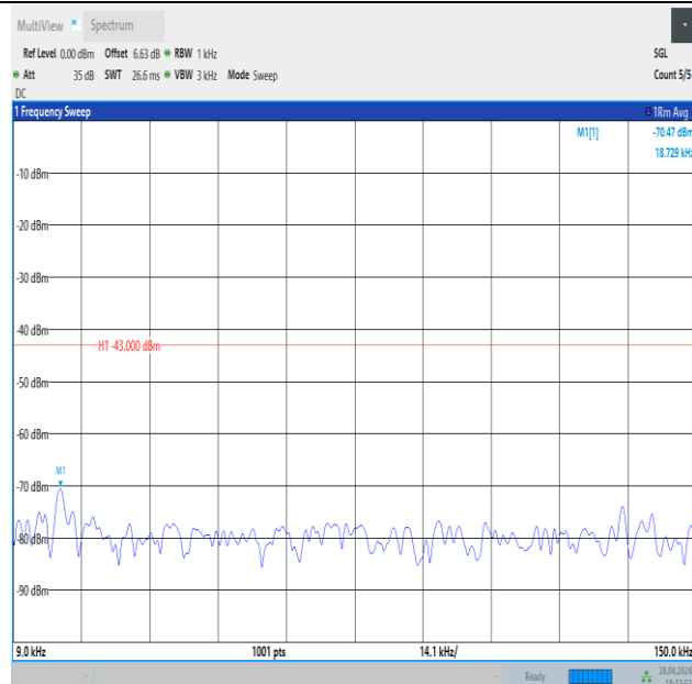
Band4_1.4MHz_16QAM_19957_1RB#5_0.009~0.15_0.009~0.15
