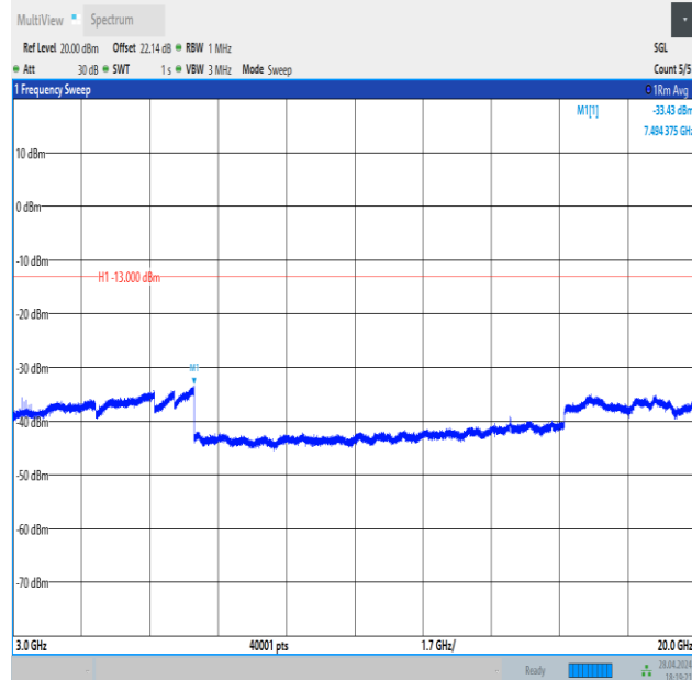
Band4_1.4MHz_QPSK_19957_6RB#0_3000~20000_3000~20000
