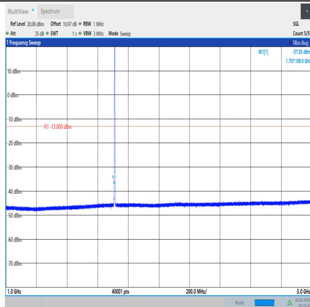
Band4_1.4MHz_16QAM_19957_6RB#0_1000~3000_1000~3000
