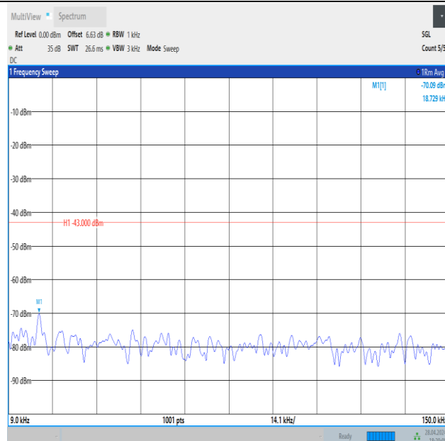
Band4_1.4MHz_16QAM_20393_6RB#0_0.009~0.15_0.009~0.15
