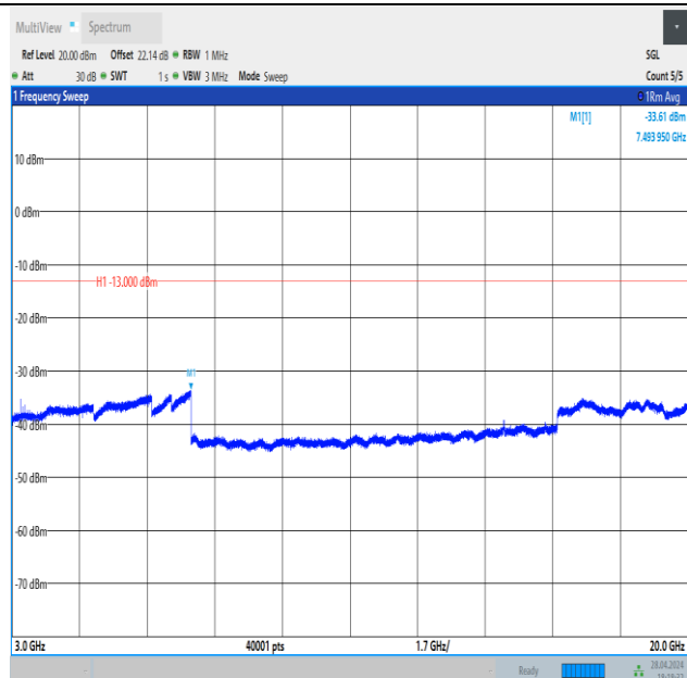
Band4_1.4MHz_16QAM_19957_1RB#5_3000~20000_3000~20000
