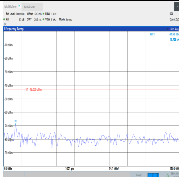
Band4_1.4MHz_16QAM_20175_1RB#0_0.009~0.15_0.009~0.15
