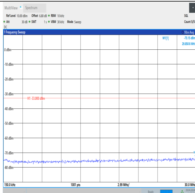
Band4_1.4MHz_QPSK_20175_1RB#5_0.15~30_0.15~30
