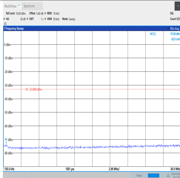
Band4_1.4MHz_16QAM_19957_1RB#5_0.15~30_0.15~30
