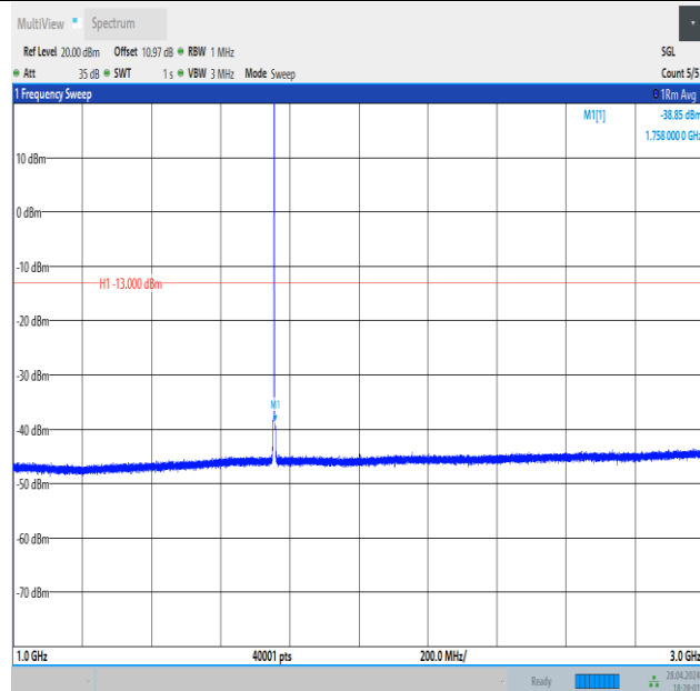
Band4_1.4MHz_16QAM_20393_1RB#5_1000~3000_1000~3000
