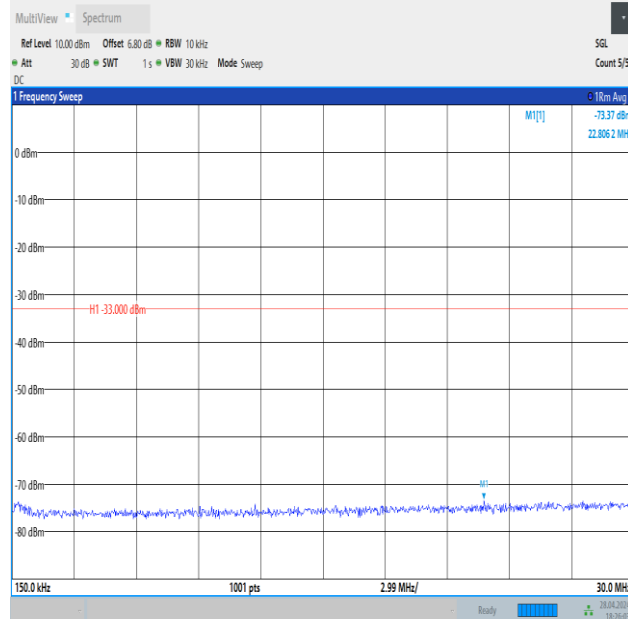
Band4_1.4MHz_16QAM_20393_1RB#0_0.15~30_0.15~30
