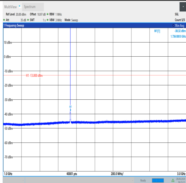
Band4_1.4MHz_16QAM_20175_1RB#5_1000~3000_1000~3000
