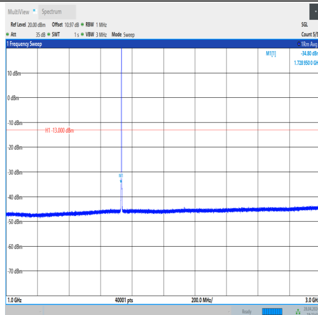
Band4_1.4MHz_QPSK_20175_6RB#0_1000~3000_1000~3000
