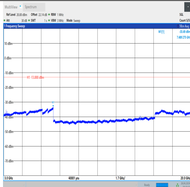
Band4_1.4MHz_16QAM_19957_1RB#0_3000~20000_3000~20000
