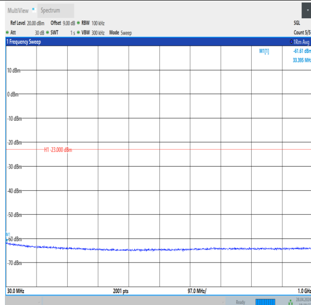
Band4_1.4MHz_QPSK_19957_6RB#0_30~1000_30~1000
