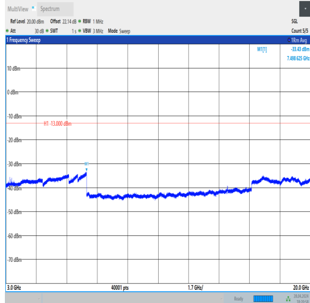
Band4_1.4MHz_QPSK_20175_1RB#0_3000~20000_3000~20000
