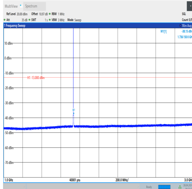
Band4_1.4MHz_QPSK_20175_1RB#5_1000~3000_1000~3000
