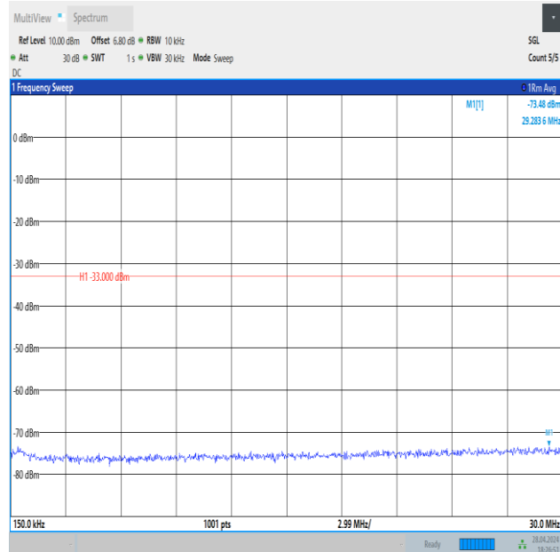
Band4_1.4MHz_QPSK_20393_1RB#5_0.15~30_0.15~30
