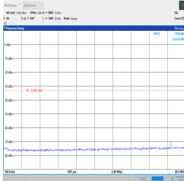
Band4_1.4MHz_16QAM_19957_6RB#0_0.15~30_0.15~30
