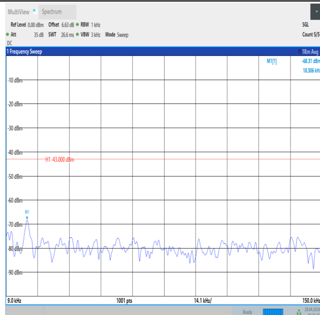
Band4_1.4MHz_QPSK_20393_1RB#5_0.009~0.15_0.009~0.15
