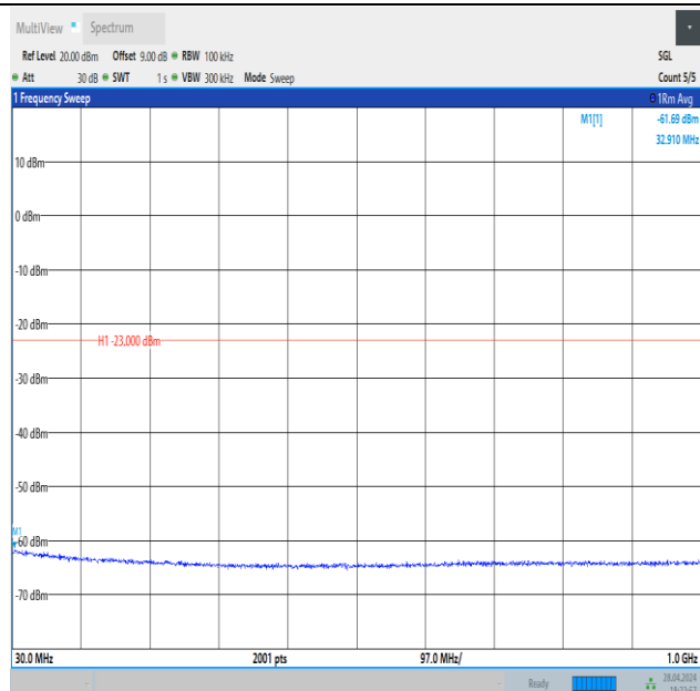
Band4_1.4MHz_16QAM_20175_1RB#5_30~1000_30~1000
