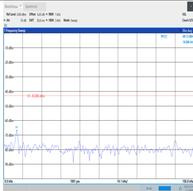
Band4_10MHz_QPSK_20175_1RB#49_0.009~0.15_0.009~0.15
