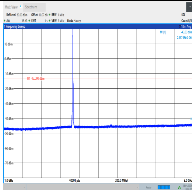
Band4_15MHz_16QAM_20175_1RB#0_1000~3000_1000~3000
