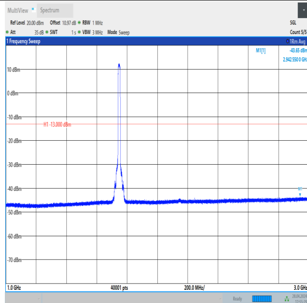
Band4_15MHz_QPSK_20325_75RB#0_1000~3000_1000~3000
