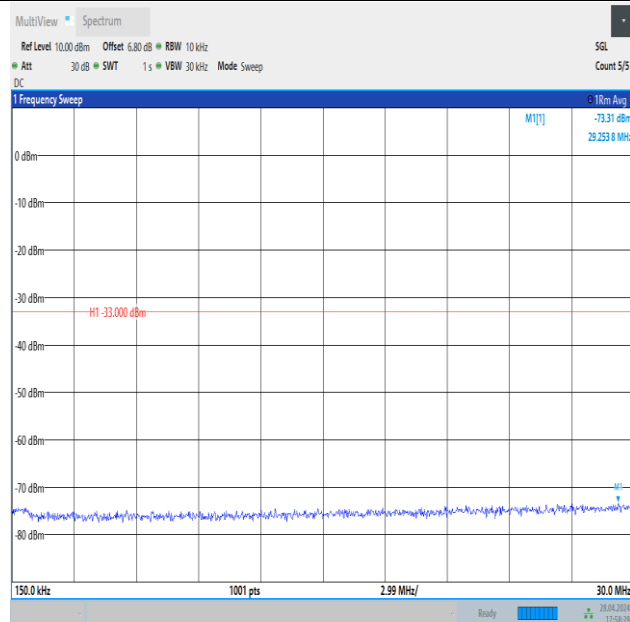
Band4_15MHz_16QAM_20025_1RB#74_0.15~30_0.15~30
