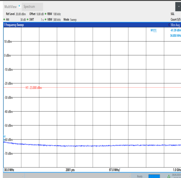
Band4_10MHz_QPSK_20350_1RB#49_30~1000_30~1000
