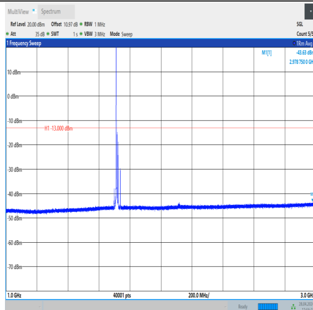
Band4_15MHz_QPSK_20025_1RB#0_1000~3000_1000~3000
