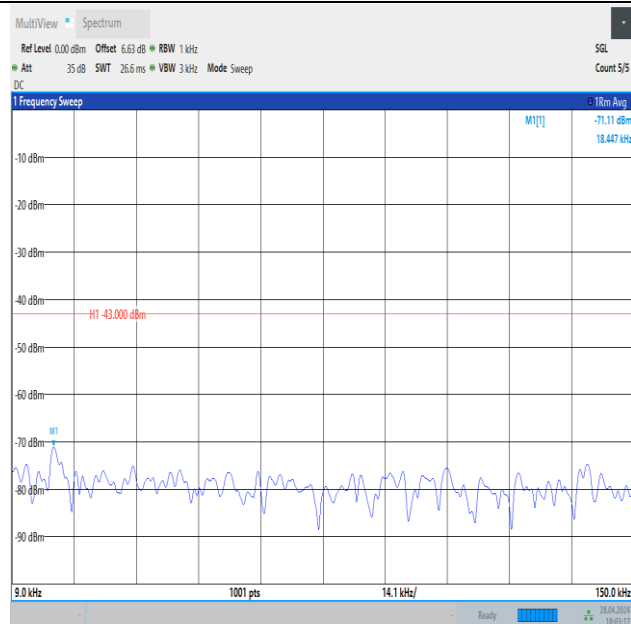
Band4_15MHz_16QAM_20325_1RB#0_0.009~0.15_0.009~0.15
