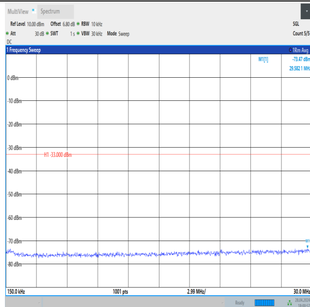
Band4_15MHz_QPSK_20175_1RB#74_0.15~30_0.15~30
