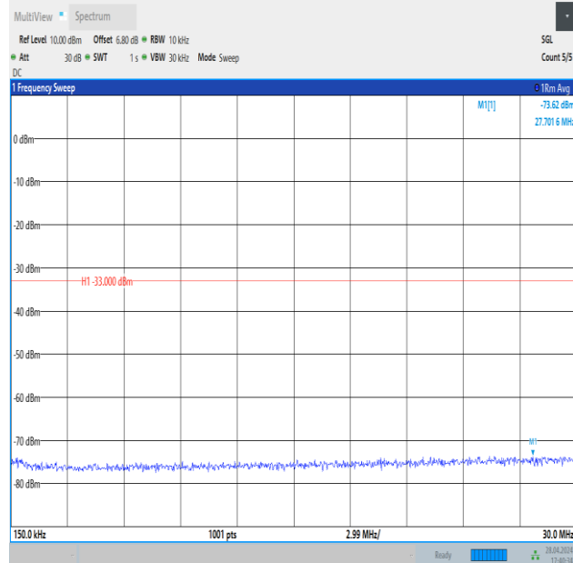
Band4_10MHz_16QAM_20350_1RB#0_0.15~30_0.15~30
