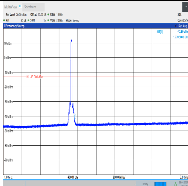
Band4_15MHz_QPSK_20175_75RB#0_1000~3000_1000~3000
