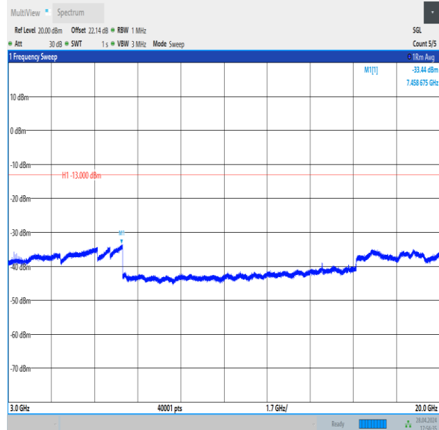
Band4_15MHz_QPSK_20025_1RB#0_3000~20000_3000~20000
