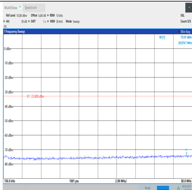
Band4_15MHz_QPSK_20175_1RB#0_0.15~30_0.15~30
