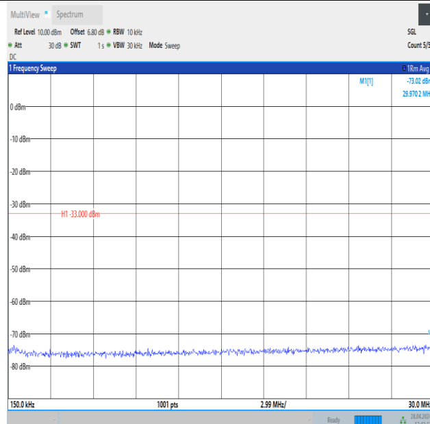
Band4_10MHz_16QAM_20350_1RB#49_0.15~30_0.15~30
