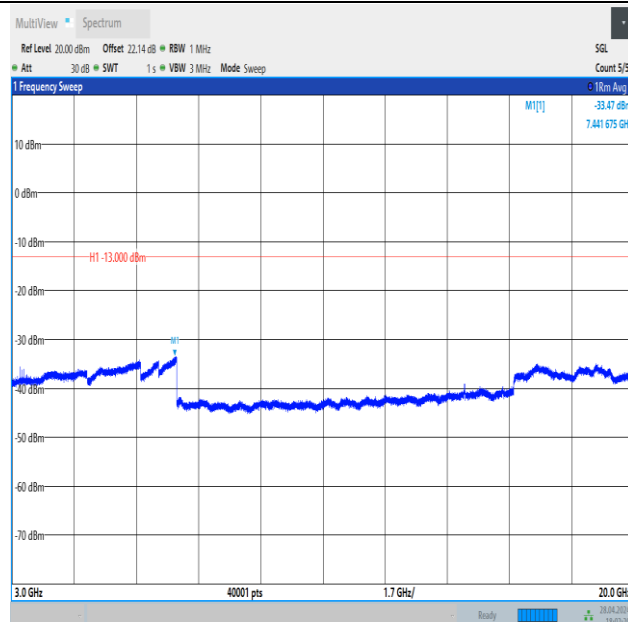
Band4_15MHz_16QAM_20175_1RB#74_3000~20000_3000~20000
