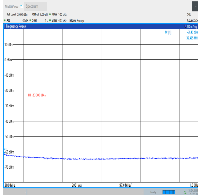
Band4_15MHz_QPSK_20325_75RB#0_30~1000_30~1000
