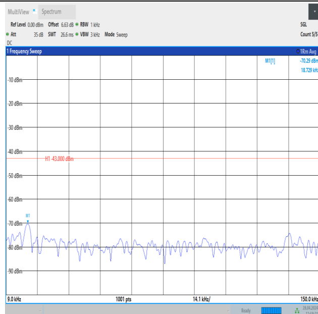
Band4_15MHz_16QAM_20025_1RB#74_0.009~0.15_0.009~0.15
