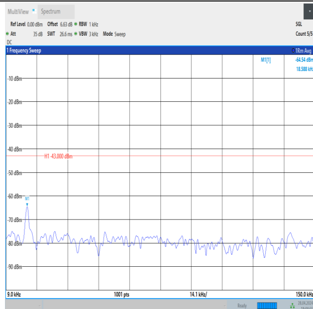
Band4_15MHz_16QAM_20325_1RB#74_0.009~0.15_0.009~0.15
