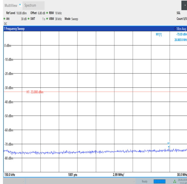
Band4_10MHz_QPSK_20175_50RB#0_0.15~30_0.15~30
