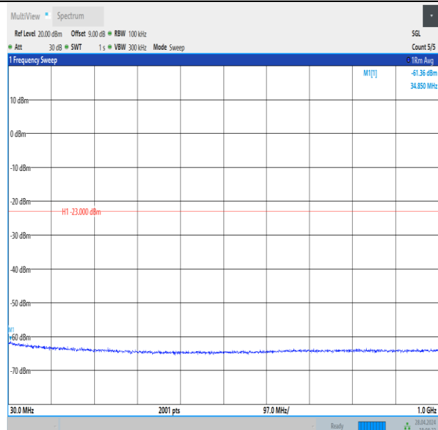
Band4_15MHz_QPSK_20325_1RB#74_30~1000_30~1000
