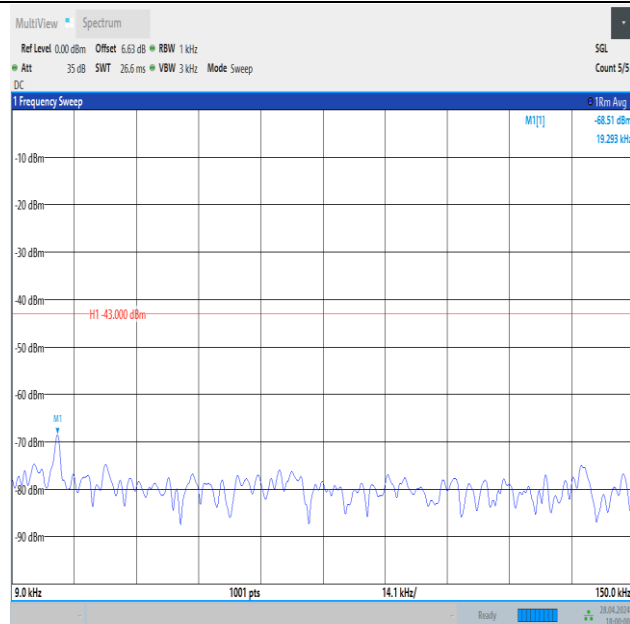
Band4_15MHz_16QAM_20175_1RB#0_0.009~0.15_0.009~0.15
