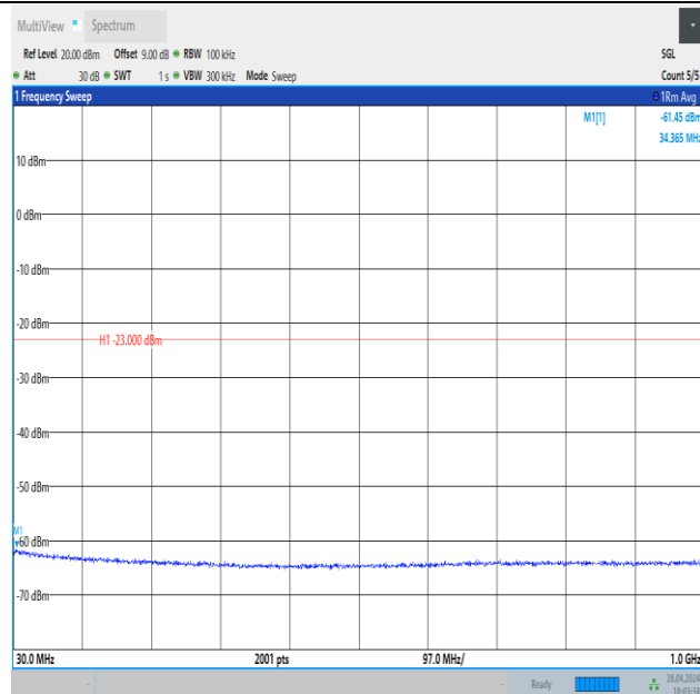
Band4_15MHz_16QAM_20325_1RB#0_30~1000_30~1000
