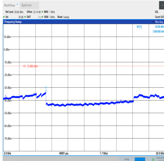
Band4_10MHz_QPSK_20175_50RB#0_3000~20000_3000~20000
