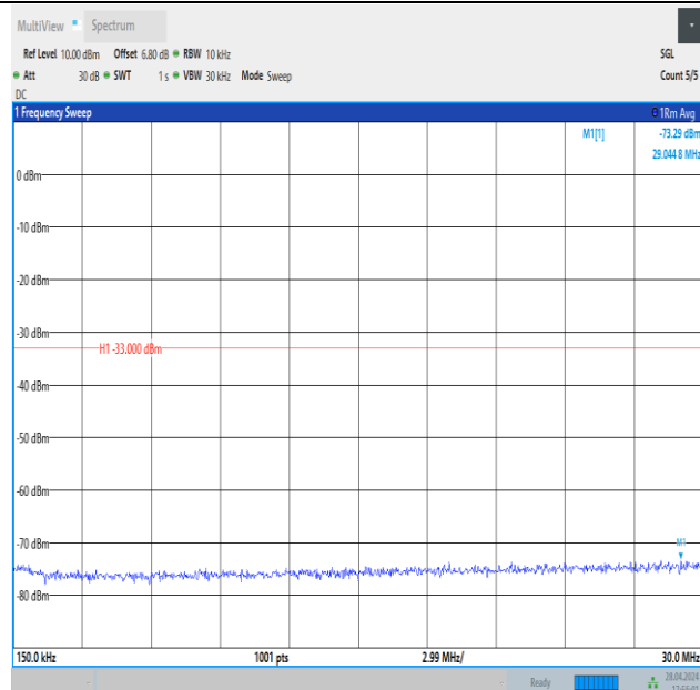
Band4_15MHz_QPSK_20025_1RB#0_0.15~30_0.15~30
