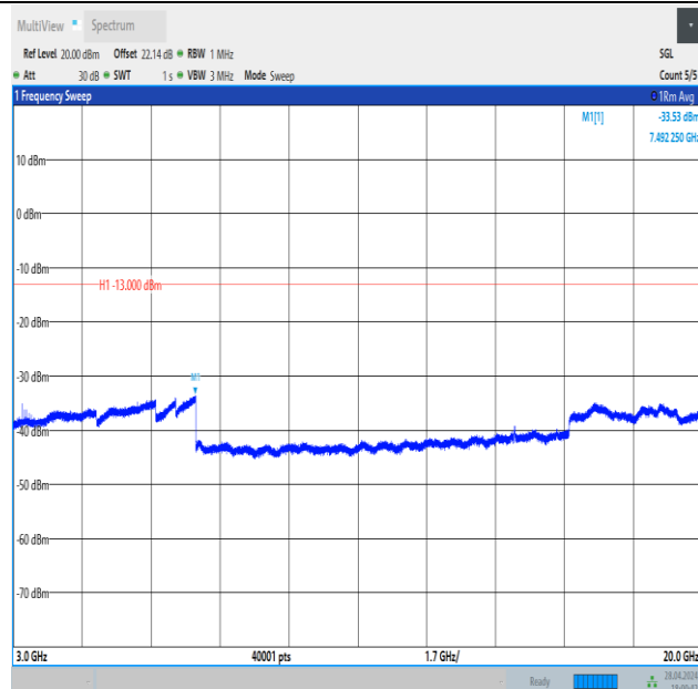
Band4_15MHz_16QAM_20175_1RB#0_3000~20000_3000~20000
