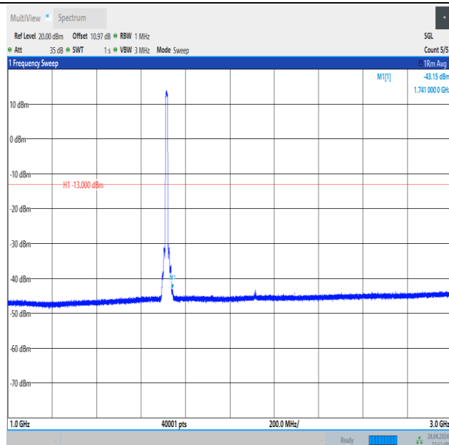
Band4_10MHz_QPSK_20000_50RB#0_1000~3000_1000~3000
