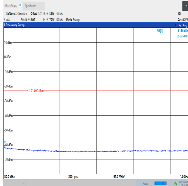
Band4_10MHz_16QAM_20350_1RB#0_30~1000_30~1000
