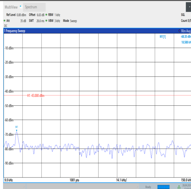
Band4_15MHz_16QAM_20025_1RB#0_0.009~0.15_0.009~0.15
