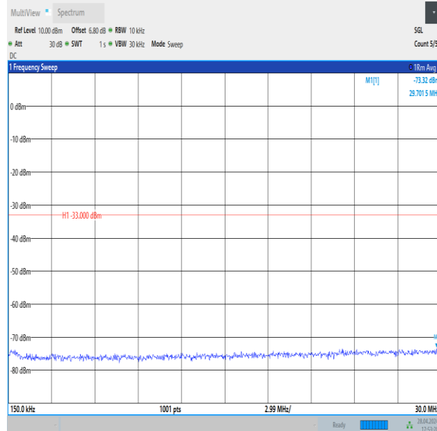
Band4_15MHz_QPSK_20025_75RB#0_0.15~30_0.15~30
