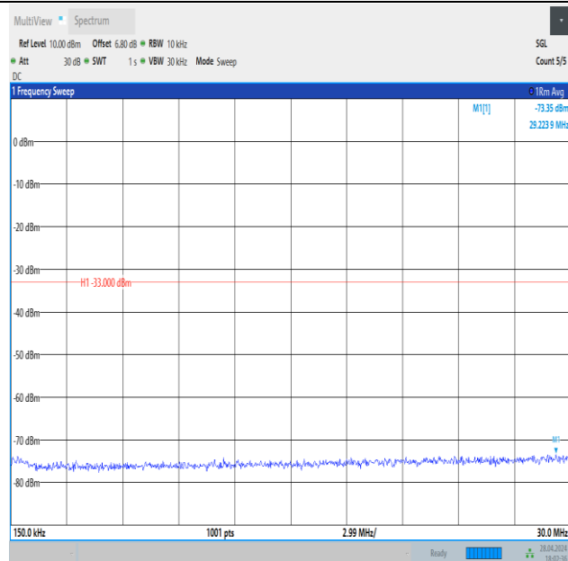
Band4_15MHz_QPSK_20325_1RB#0_0.15~30_0.15~30
