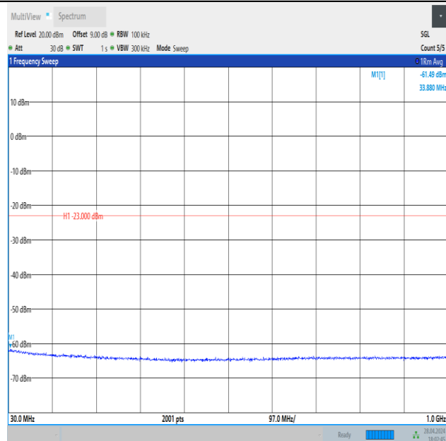
Band4_15MHz_QPSK_20325_1RB#0_30~1000_30~1000
