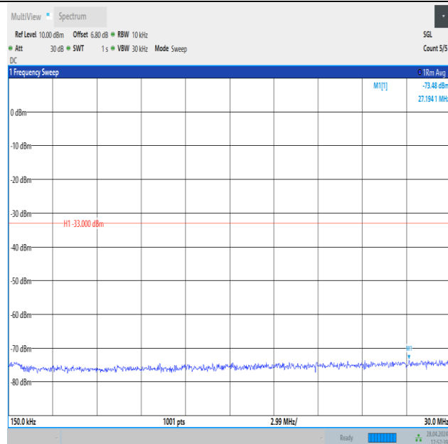
Band4_15MHz_QPSK_20025_1RB#74_0.15~30_0.15~30
