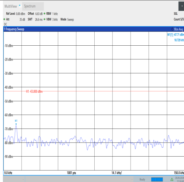
Band4_10MHz_QPSK_20000_50RB#0_0.009~0.15_0.009~0.15
