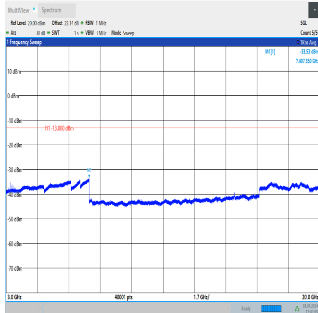
Band4_10MHz_16QAM_20350_1RB#0_3000~20000_3000~20000
