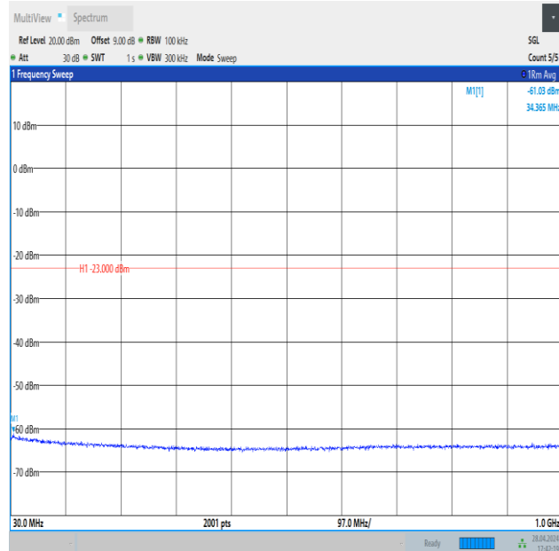
Band4_10MHz_16QAM_20350_1RB#49_30~1000_30~1000
