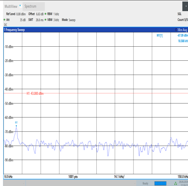
Band4_15MHz_QPSK_20175_1RB#0_0.009~0.15_0.009~0.15
