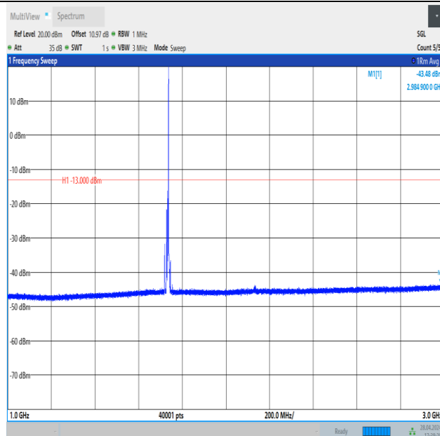
Band4_10MHz_QPSK_20175_1RB#49_1000~3000_1000~3000
