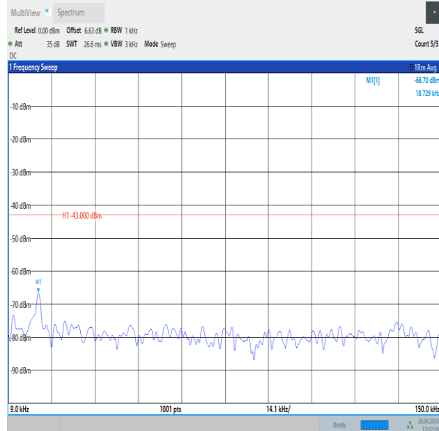
Band4_10MHz_QPSK_20350_50RB#0_0.009~0.15_0.009~0.15
