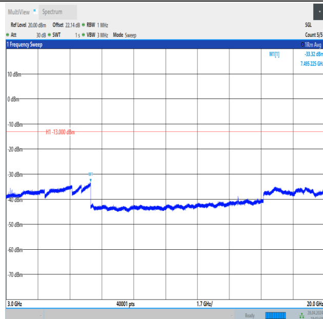
Band4_15MHz_16QAM_20325_1RB#0_3000~20000_3000~20000
