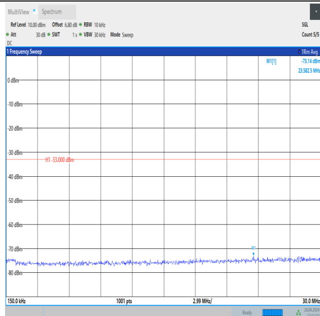
Band4_10MHz_QPSK_20350_50RB#0_0.15~30_0.15~30
