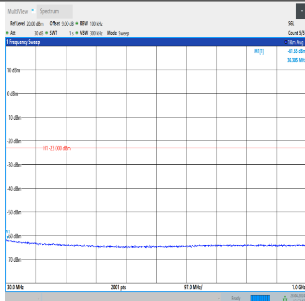
Band4_15MHz_QPSK_20025_1RB#74_30~1000_30~1000
