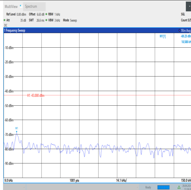
Band4_10MHz_QPSK_20350_1RB#0_0.009~0.15_0.009~0.15
