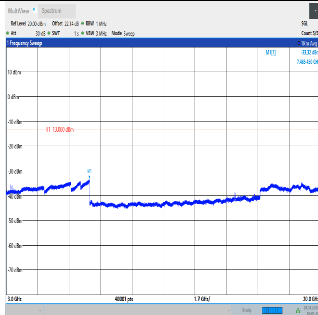
Band4_15MHz_QPSK_20175_1RB#74_3000~20000_3000~20000
