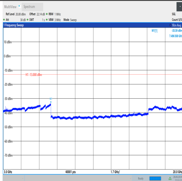
Band4_10MHz_QPSK_20000_50RB#0_3000~20000_3000~20000
