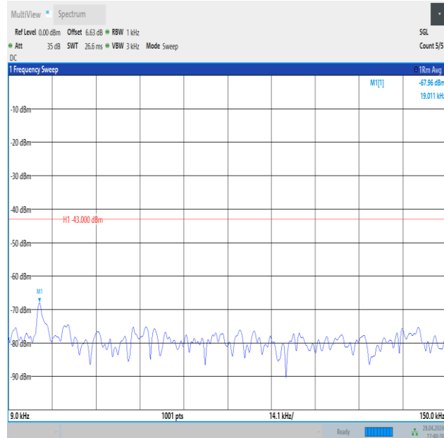
Band4_10MHz_16QAM_20350_1RB#0_0.009~0.15_0.009~0.15
