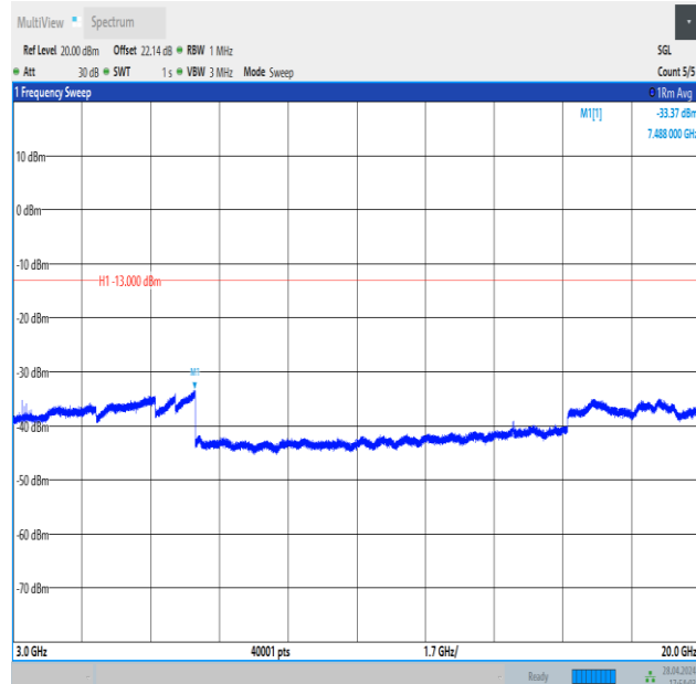
Band4_15MHz_QPSK_20025_75RB#0_3000~20000_3000~20000
