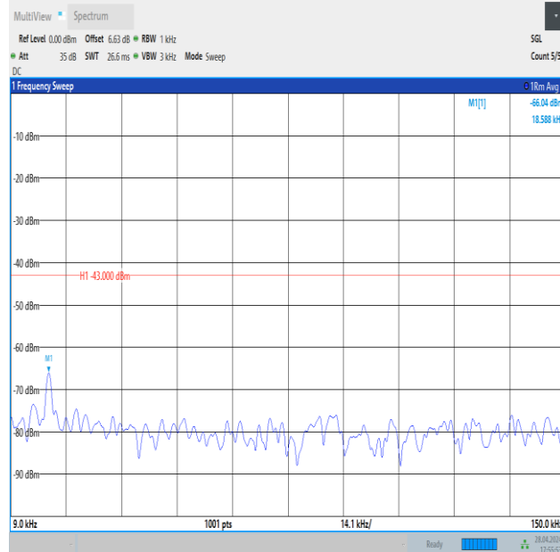
Band4_15MHz_QPSK_20025_1RB#0_0.009~0.15_0.009~0.15
