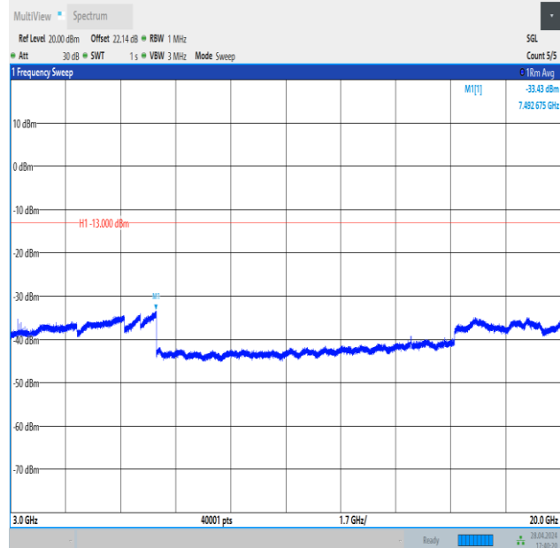
Band4_10MHz_QPSK_20350_1RB#0_3000~20000_3000~20000
