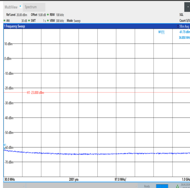
Band4_15MHz_QPSK_20175_1RB#74_30~1000_30~1000
