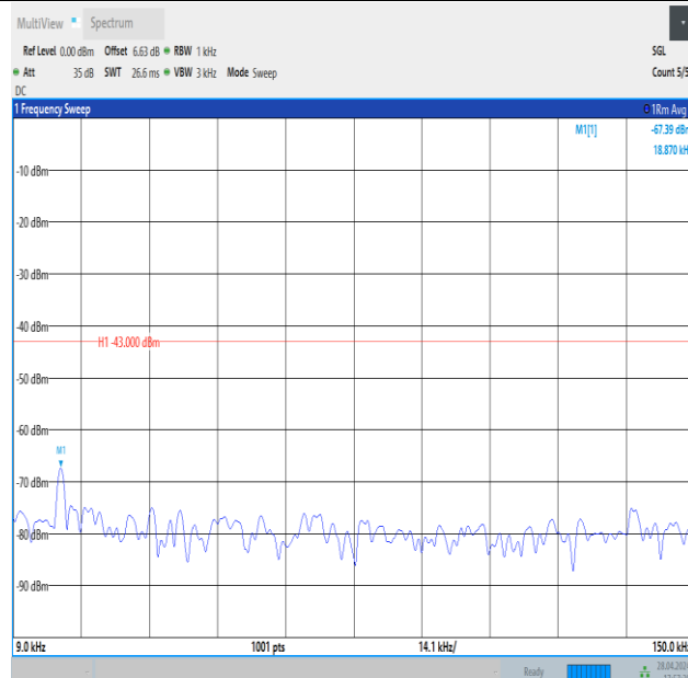
Band4_15MHz_QPSK_20025_1RB#74_0.009~0.15_0.009~0.15
