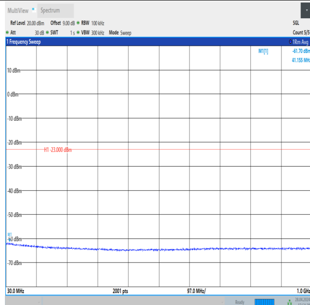
Band4_15MHz_QPSK_20175_75RB#0_30~1000_30~1000
