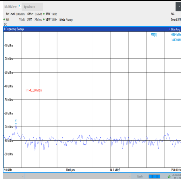
Band4_10MHz_QPSK_20175_50RB#0_0.009~0.15_0.009~0.15
