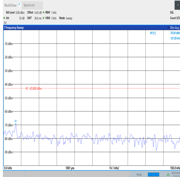
Band4_10MHz_QPSK_20350_1RB#49_0.009~0.15_0.009~0.15
