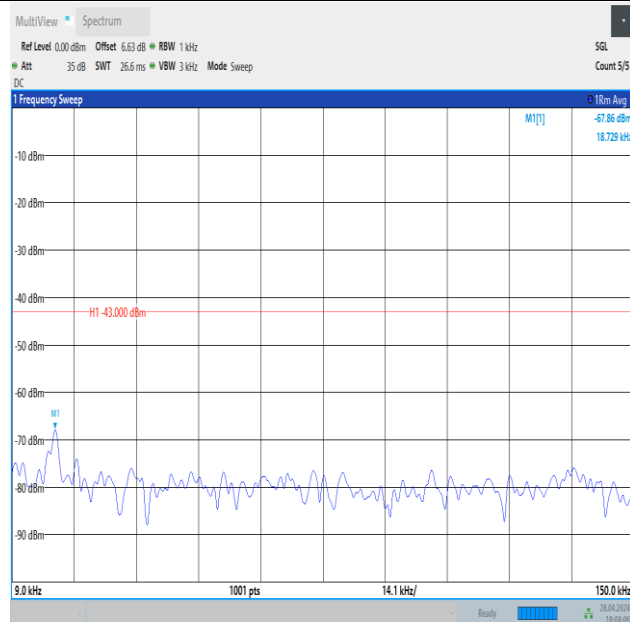
Band4_15MHz_QPSK_20325_1RB#74_0.009~0.15_0.009~0.15
