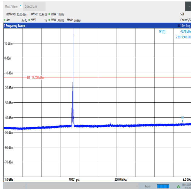
Band4_10MHz_16QAM_20175_1RB#49_1000~3000_1000~3000
