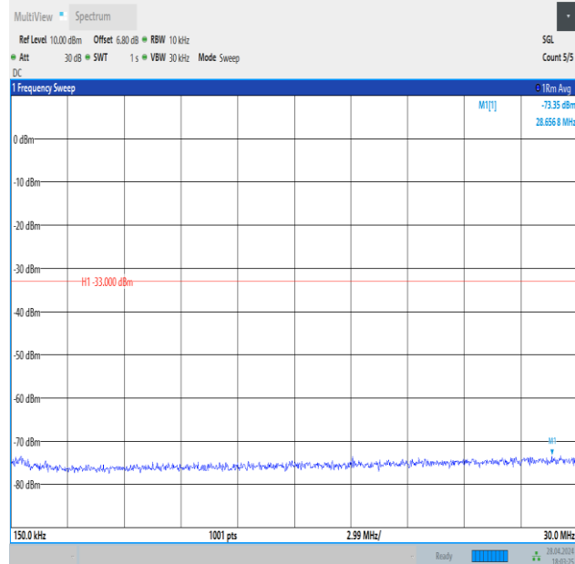
Band4_15MHz_16QAM_20325_1RB#0_0.15~30_0.15~30
