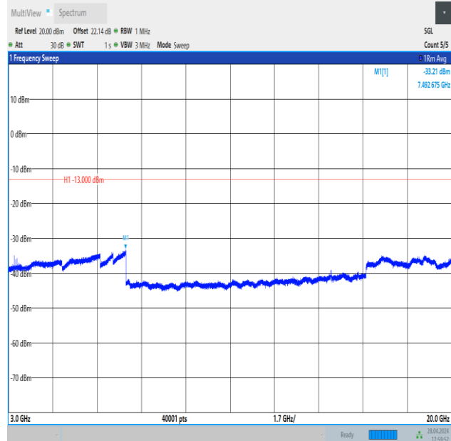
Band4_15MHz_QPSK_20175_1RB#0_3000~20000_3000~20000
