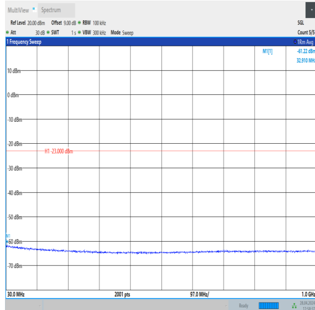
Band4_15MHz_16QAM_20025_1RB#74_30~1000_30~1000
