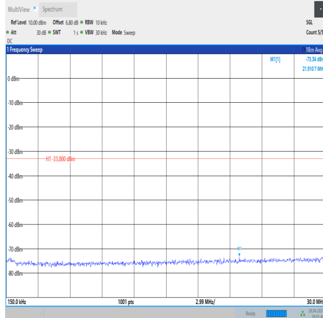
Band4_15MHz_16QAM_20175_1RB#74_0.15~30_0.15~30
