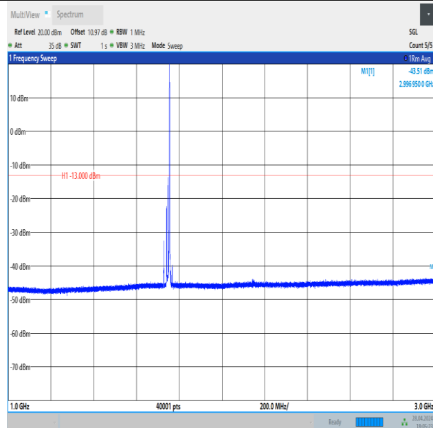
Band4_15MHz_16QAM_20325_1RB#74_1000~3000_1000~3000
