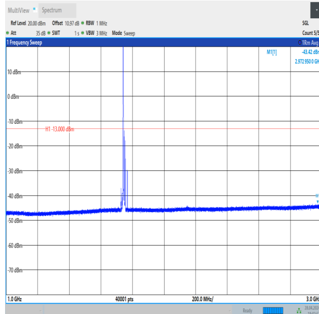
Band4_15MHz_QPSK_20325_1RB#0_1000~3000_1000~3000
