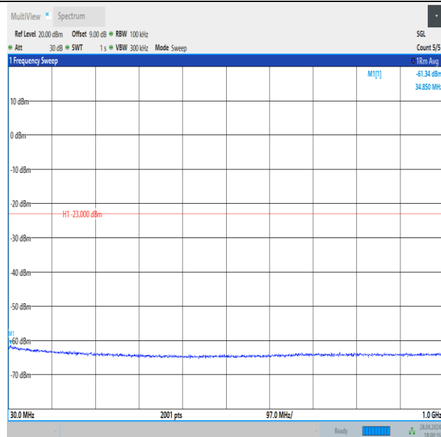
Band4_15MHz_16QAM_20175_1RB#0_30~1000_30~1000
