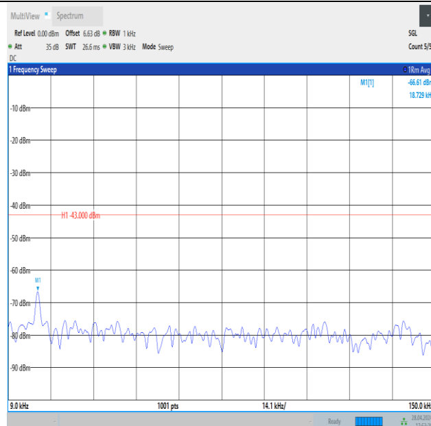
Band4_15MHz_QPSK_20025_75RB#0_0.009~0.15_0.009~0.15
