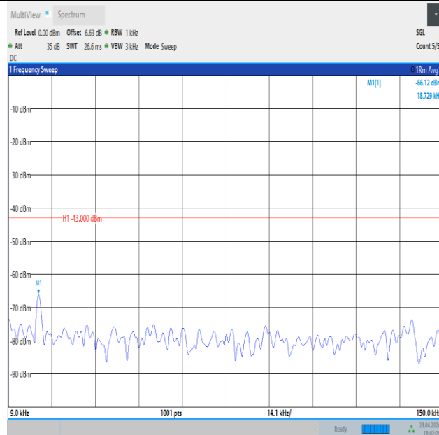
Band4_15MHz_QPSK_20325_1RB#0_0.009~0.15_0.009~0.15
