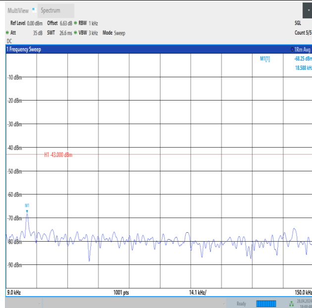
Band4_15MHz_QPSK_20175_1RB#74_0.009~0.15_0.009~0.15
