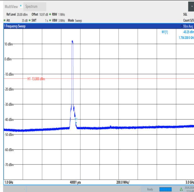
Band4_15MHz_QPSK_20025_75RB#0_1000~3000_1000~3000
