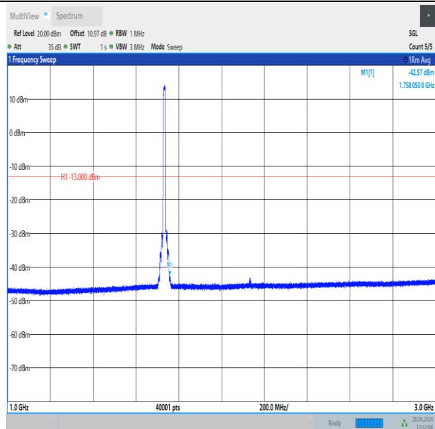
Band4_10MHz_QPSK_20175_50RB#0_1000~3000_1000~3000
