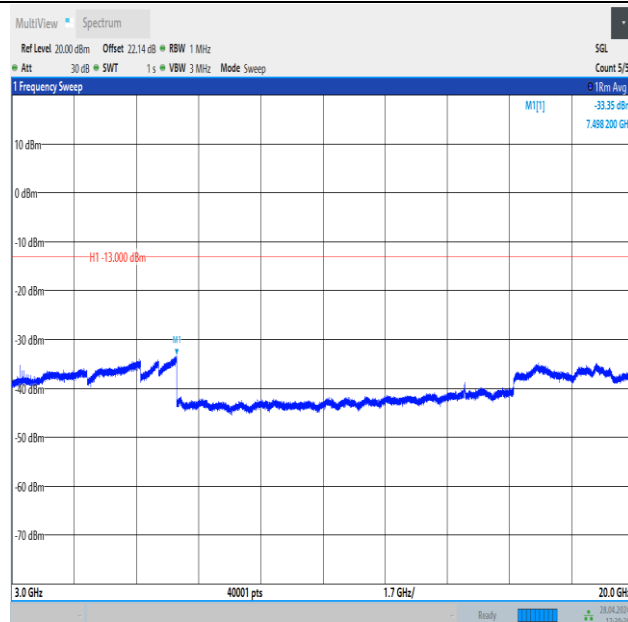
Band4_10MHz_16QAM_20175_1RB#49_3000~20000_3000~20000
