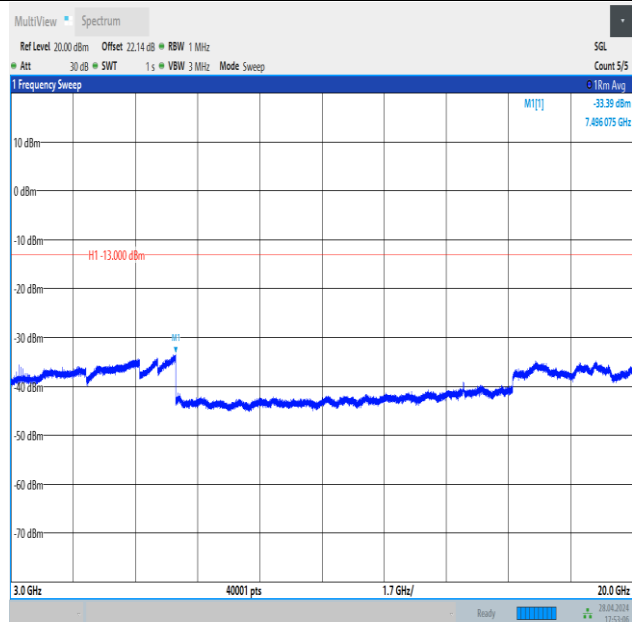
Band4_10MHz_QPSK_20350_50RB#0_3000~20000_3000~20000
