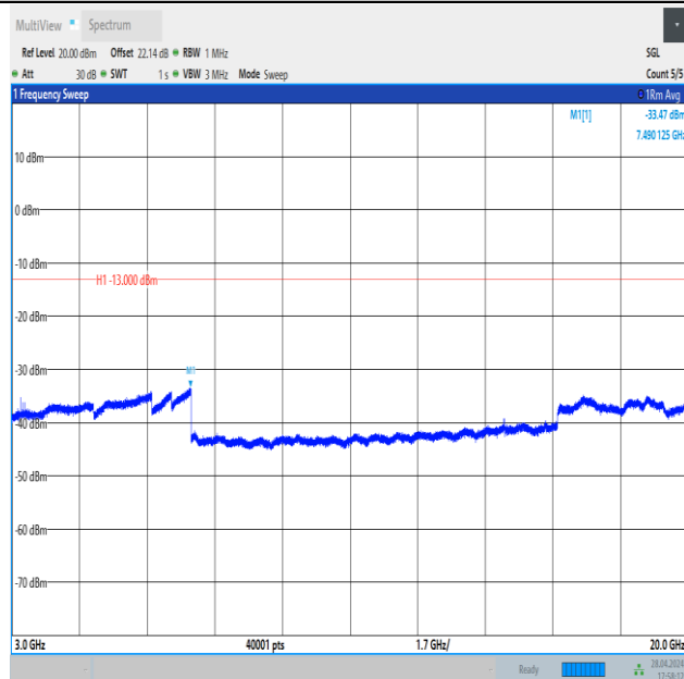
Band4_15MHz_QPSK_20025_1RB#74_3000~20000_3000~20000
