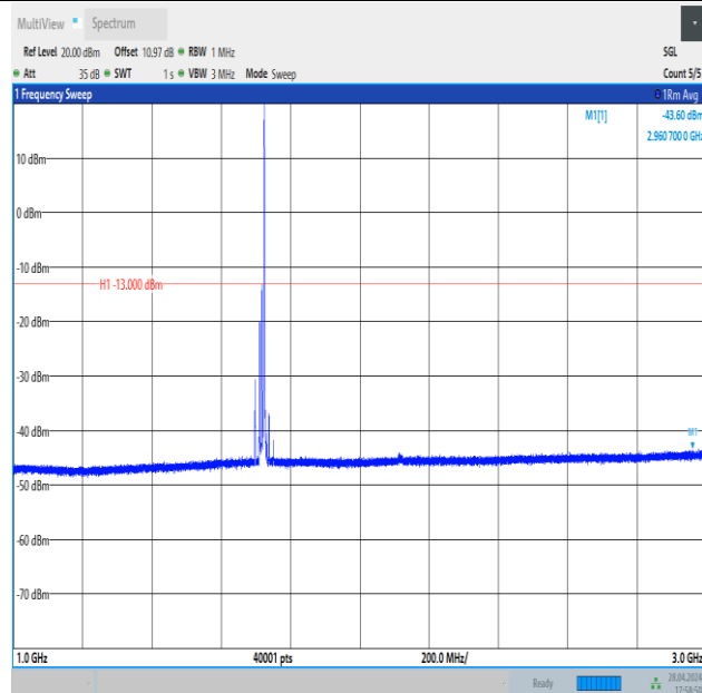
Band4_15MHz_16QAM_20025_1RB#74_1000~3000_1000~3000
