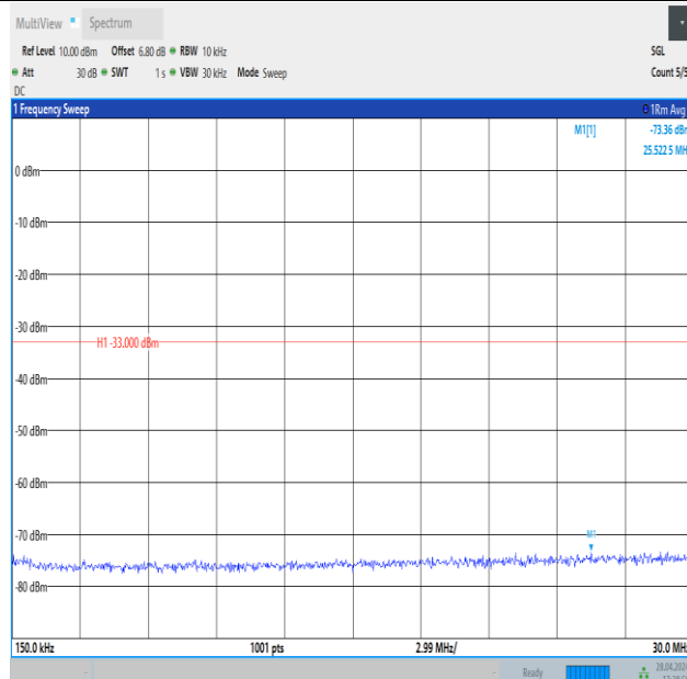
Band4_10MHz_16QAM_20175_1RB#49_0.15~30_0.15~30
