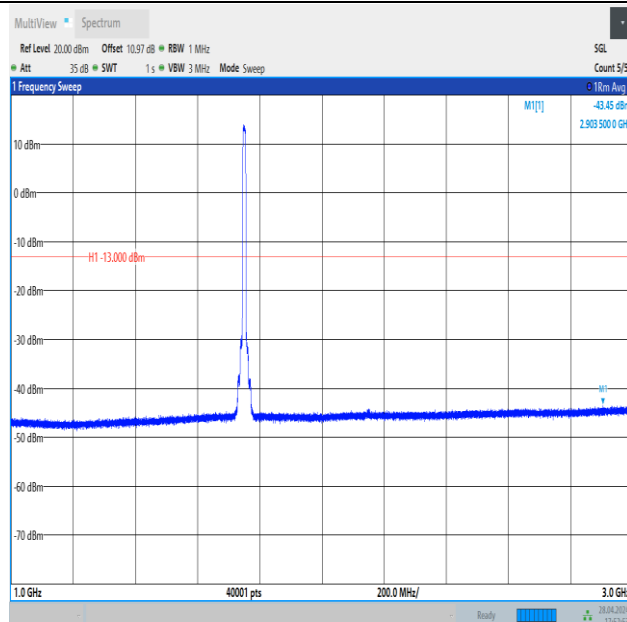
Band4_10MHz_QPSK_20350_50RB#0_1000~3000_1000~3000
