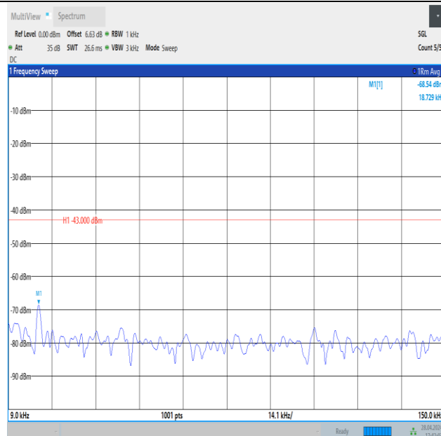
Band4_10MHz_16QAM_20350_1RB#49_0.009~0.15_0.009~0.15
