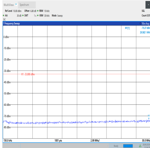
Band4_15MHz_QPSK_20175_75RB#0_0.15~30_0.15~30
