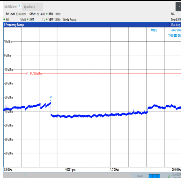
Band4_15MHz_16QAM_20025_1RB#74_3000~20000_3000~20000
