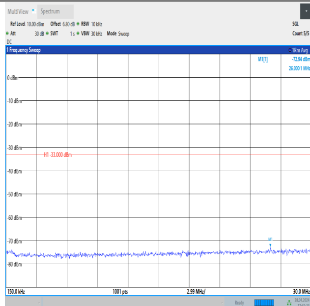
Band4_10MHz_QPSK_20350_1RB#49_0.15~30_0.15~30
