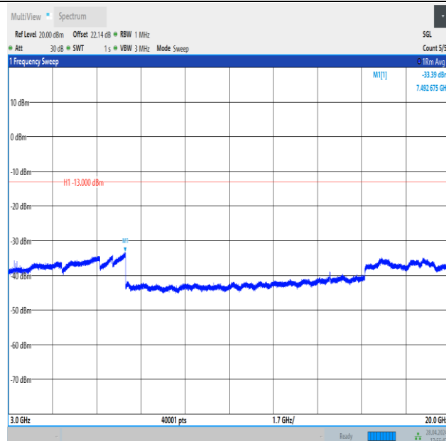
Band4_15MHz_QPSK_20325_75RB#0_3000~20000_3000~20000
