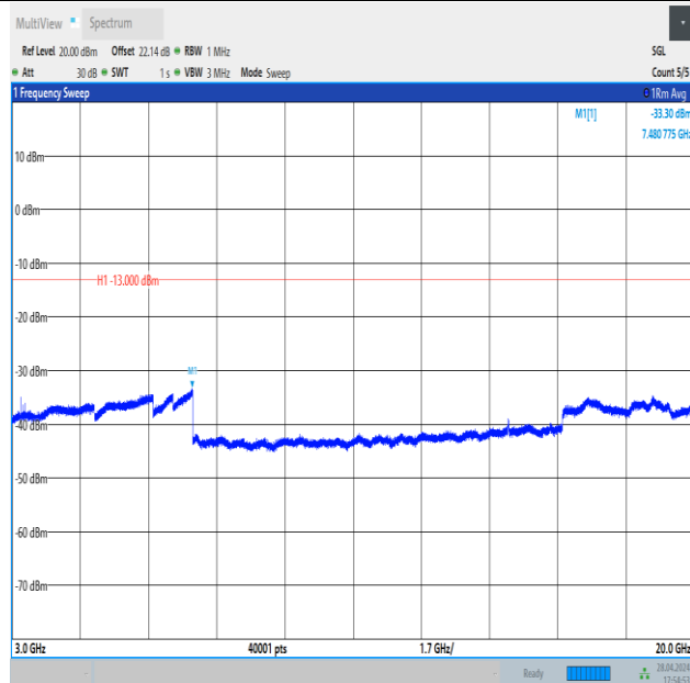
Band4_15MHz_QPSK_20175_75RB#0_3000~20000_3000~20000
