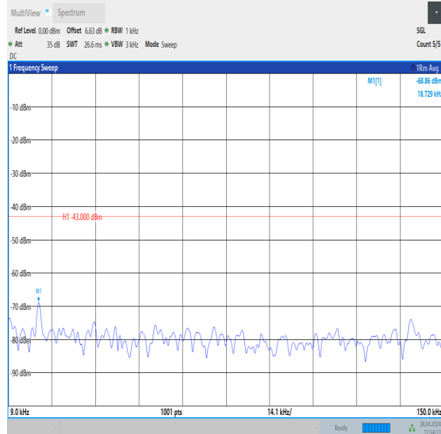
Band4_15MHz_QPSK_20175_75RB#0_0.009~0.15_0.009~0.15
