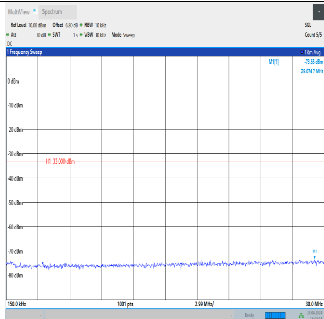
Band4_15MHz_QPSK_20325_1RB#74_0.15~30_0.15~30
