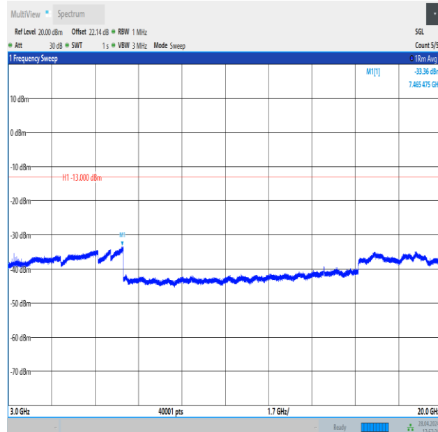
Band4_15MHz_16QAM_20025_1RB#0_3000~20000_3000~20000
