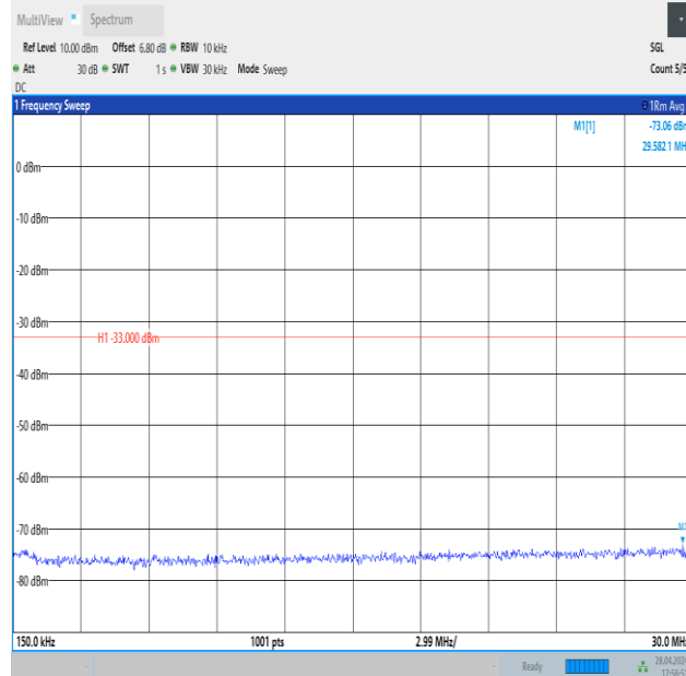
Band4_15MHz_16QAM_20025_1RB#0_0.15~30_0.15~30
