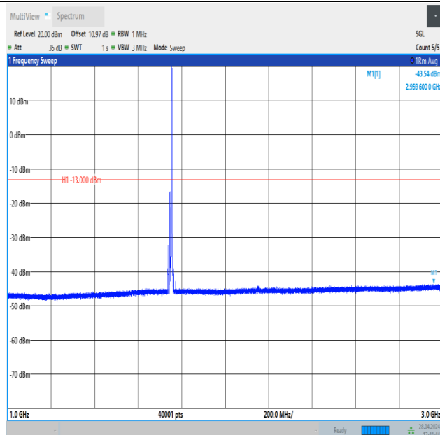
Band4_10MHz_QPSK_20350_1RB#49_1000~3000_1000~3000
