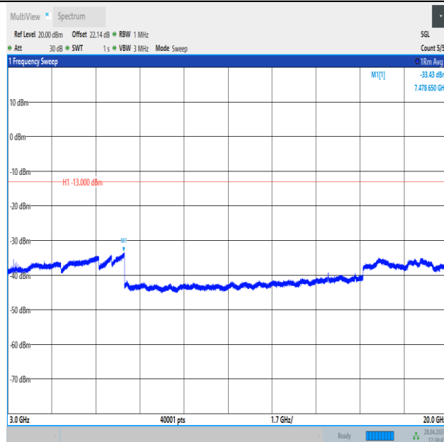
Band4_10MHz_QPSK_20175_1RB#49_3000~20000_3000~20000
