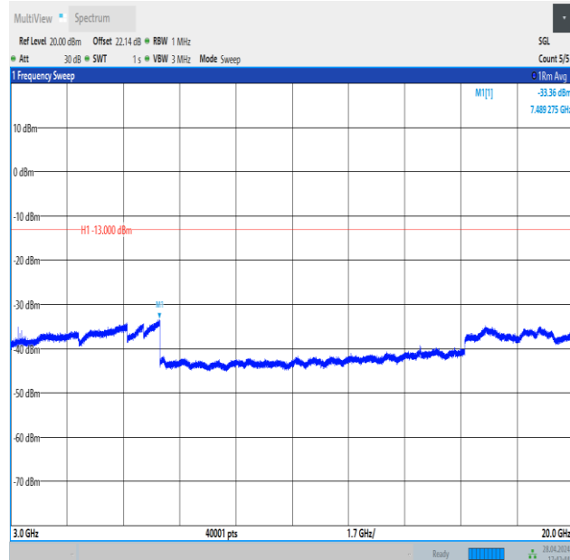
Band4_10MHz_16QAM_20350_1RB#49_3000~20000_3000~20000
