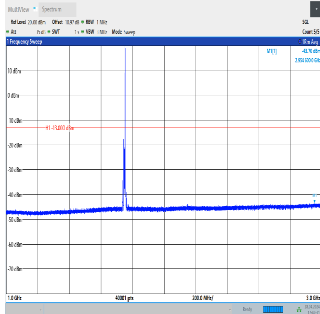
Band4_10MHz_16QAM_20350_1RB#49_1000~3000_1000~3000
