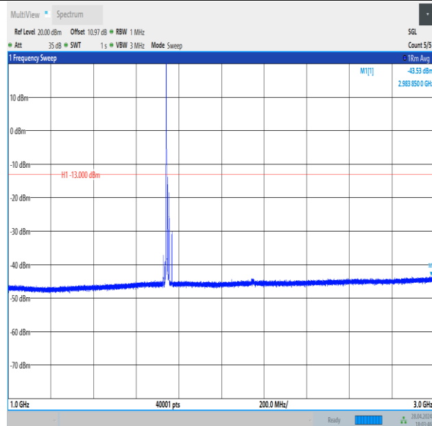
Band4_15MHz_16QAM_20325_1RB#0_1000~3000_1000~3000
