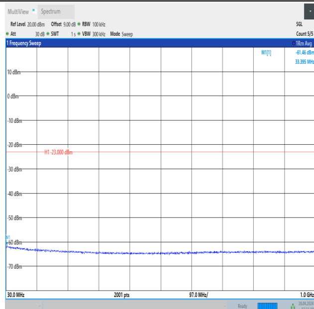
Band4_15MHz_QPSK_20025_1RB#0_30~1000_30~1000
