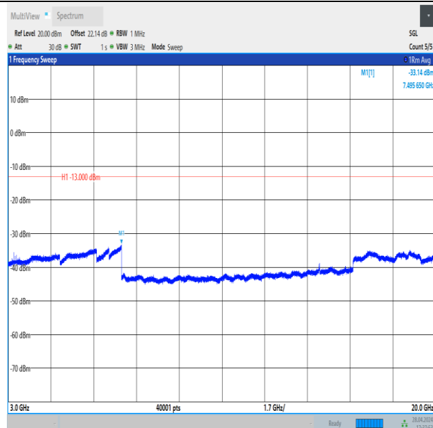
Band4_10MHz_16QAM_20175_1RB#0_3000~20000_3000~20000
