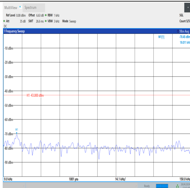
Band4_15MHz_QPSK_20325_75RB#0_0.009~0.15_0.009~0.15
