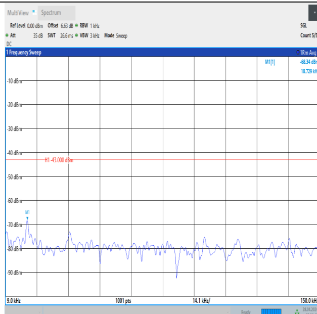
Band4_10MHz_16QAM_20175_1RB#49_0.009~0.15_0.009~0.15
