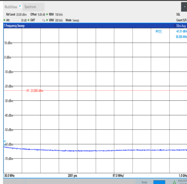
Band4_10MHz_QPSK_20350_50RB#0_30~1000_30~1000
