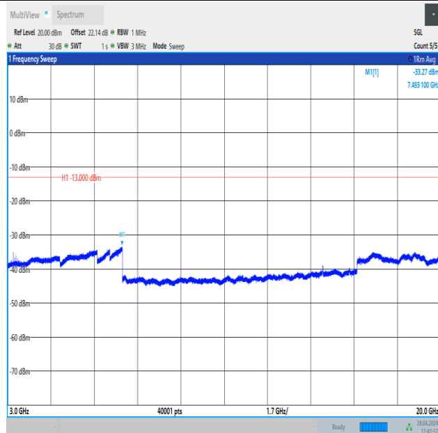
Band4_10MHz_QPSK_20350_1RB#49_3000~20000_3000~20000
