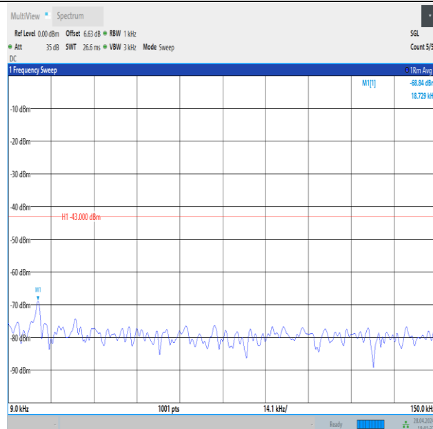
Band4_15MHz_16QAM_20175_1RB#74_0.009~0.15_0.009~0.15
