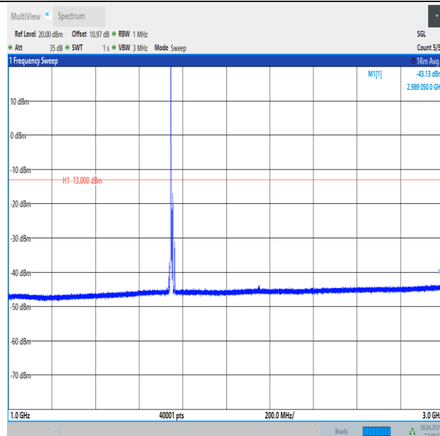
Band4_10MHz_QPSK_20350_1RB#0_1000~3000_1000~3000
