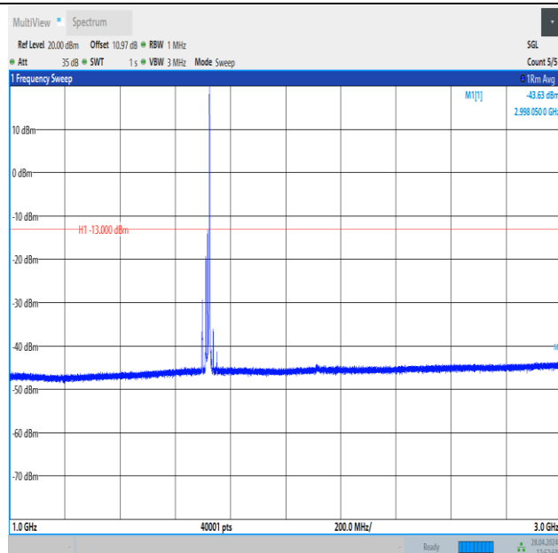
Band4_15MHz_QPSK_20025_1RB#74_1000~3000_1000~3000
