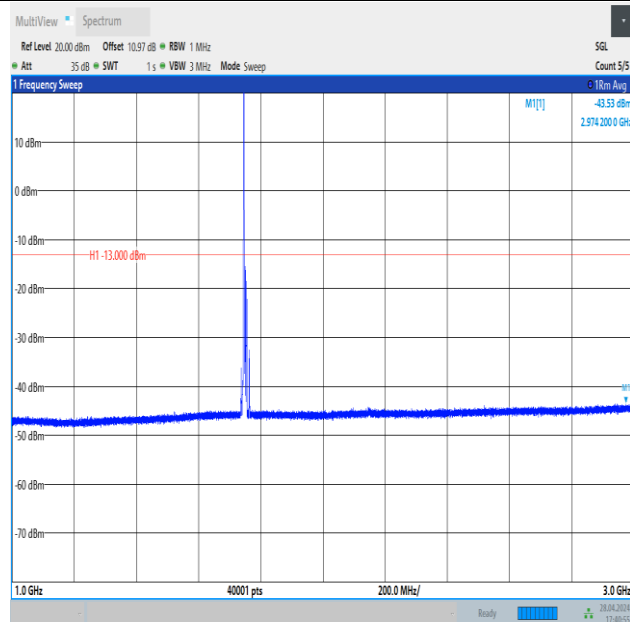
Band4_10MHz_16QAM_20350_1RB#0_1000~3000_1000~3000
