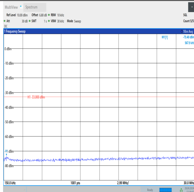
Band4_10MHz_QPSK_20350_1RB#0_0.15~30_0.15~30
