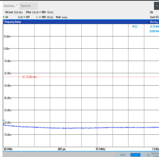
Band4_5MHz_QPSK_20375_25RB#0_30~1000_30~1000
