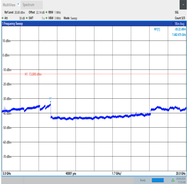
Band4_10MHz_QPSK_20000_1RB#0_3000~20000_3000~20000
