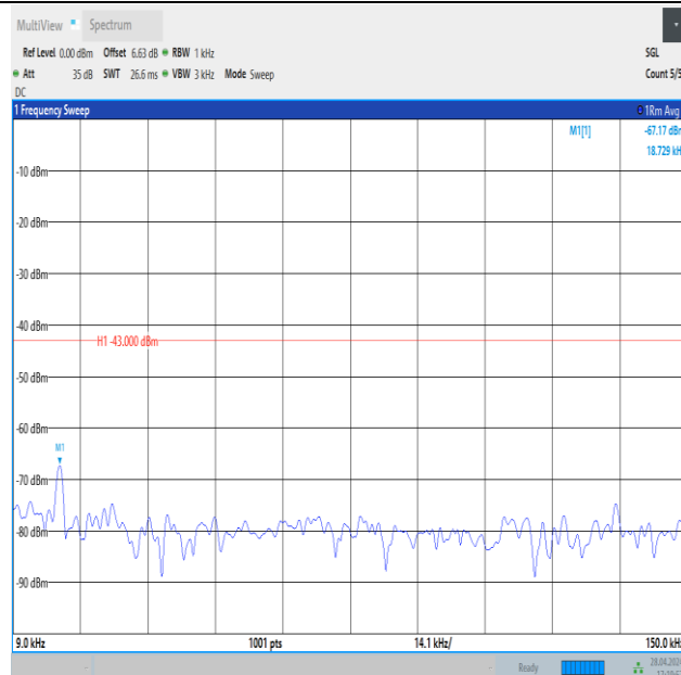
Band4_20MHz_16QAM_20175_1RB#99_0.009~0.15_0.009~0.15
