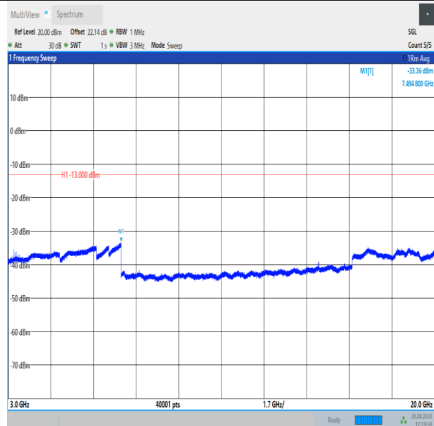
Band4_20MHz_QPSK_20175_1RB#99_3000~20000_3000~20000
