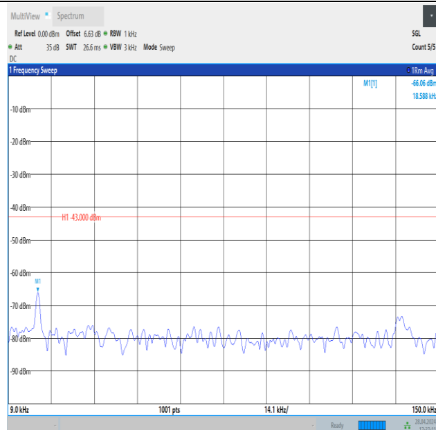
Band4_10MHz_16QAM_20175_1RB#0_0.009~0.15_0.009~0.15
