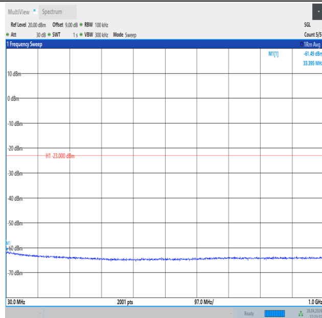
Band4_20MHz_16QAM_20300_1RB#99_30~1000_30~1000
