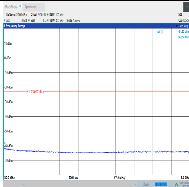
Band4_10MHz_16QAM_20175_1RB#0_30~1000_30~1000
