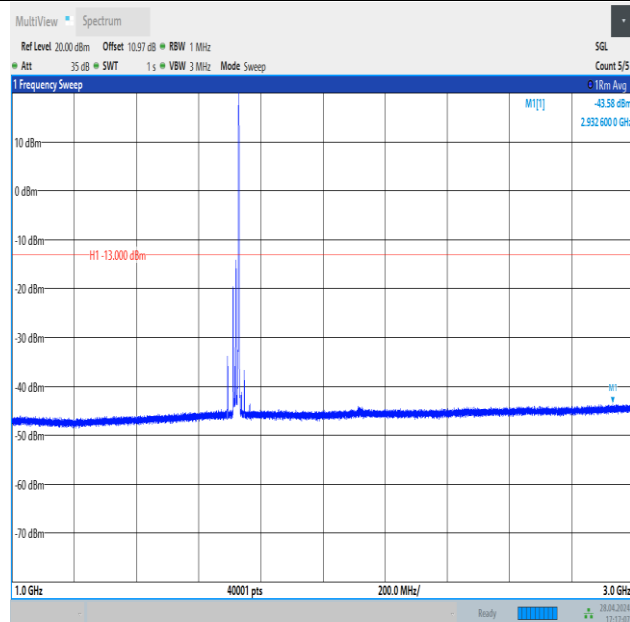
Band4_20MHz_16QAM_20050_1RB#99_1000~3000_1000~3000
