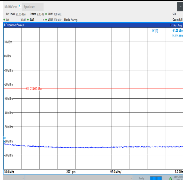
Band4_20MHz_QPSK_20050_1RB#99_30~1000_30~1000
