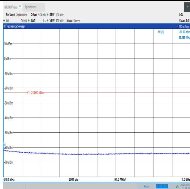
Band4_5MHz_QPSK_20375_1RB#24_30~1000_30~1000
