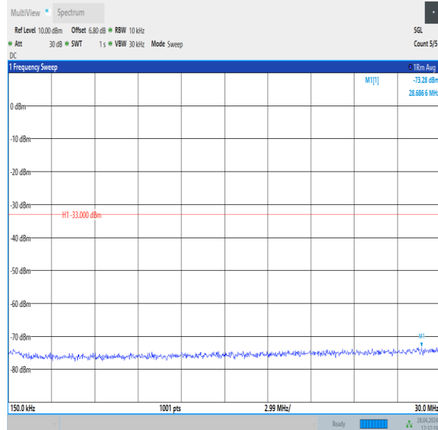
Band4_10MHz_16QAM_20175_1RB#0_0.15~30_0.15~30
