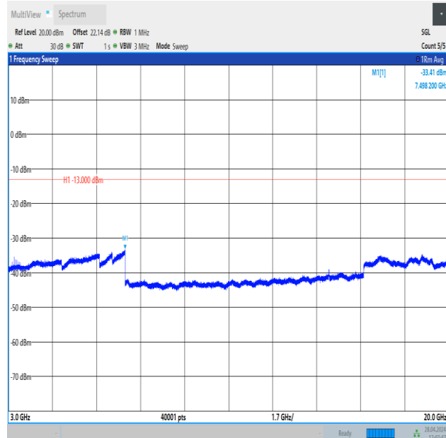
Band4_5MHz_16QAM_20375_1RB#0_3000~20000_3000~20000
