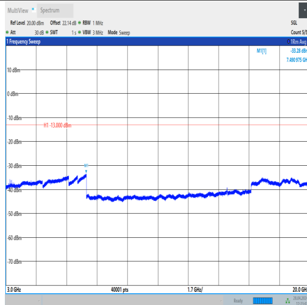
Band4_20MHz_QPSK_20300_1RB#99_3000~20000_3000~20000
