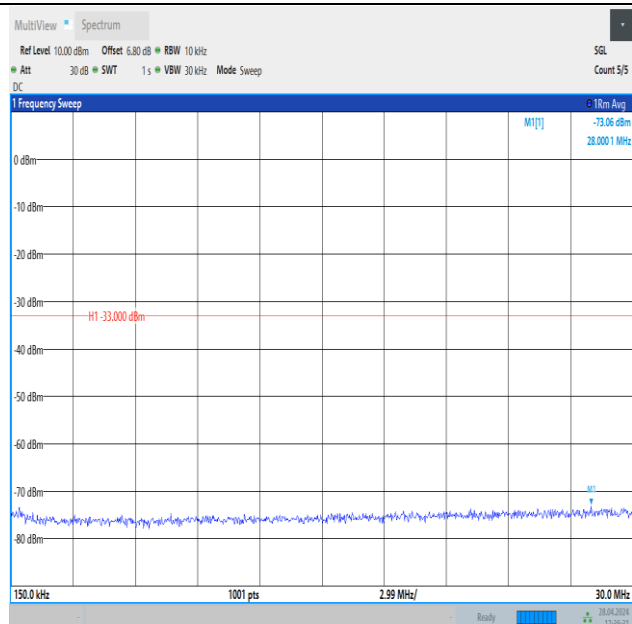
Band4_10MHz_QPSK_20175_1RB#0_0.15~30_0.15~30
