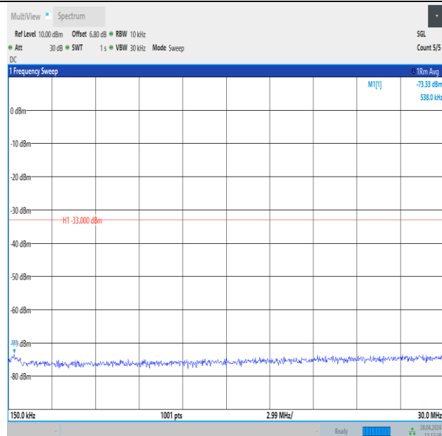
Band4_20MHz_QPSK_20175_1RB#0_0.15~30_0.15~30
