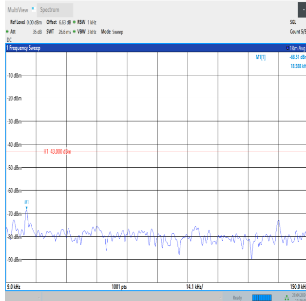
Band4_20MHz_16QAM_20050_1RB#99_0.009~0.15_0.009~0.15
