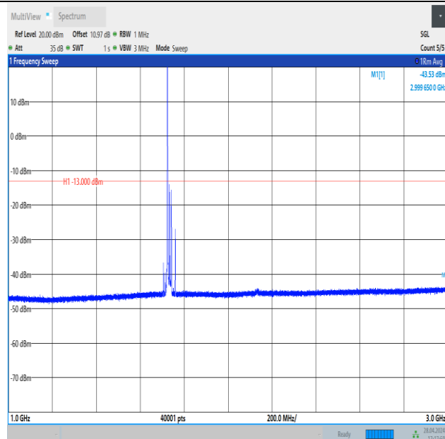
Band4_20MHz_QPSK_20175_1RB#0_1000~3000_1000~3000
