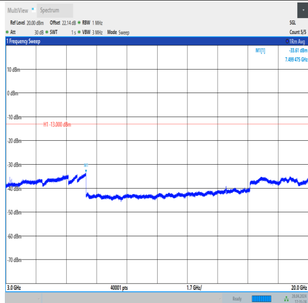
Band4_10MHz_QPSK_20000_1RB#49_3000~20000_3000~20000
