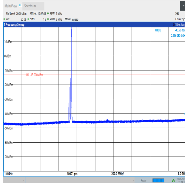
Band4_20MHz_QPSK_20175_1RB#99_1000~3000_1000~3000
