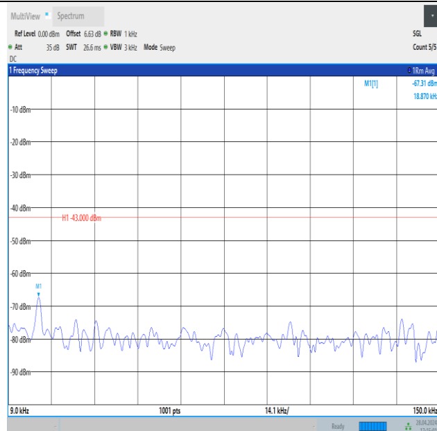
Band4_20MHz_16QAM_20050_1RB#0_0.009~0.15_0.009~0.15
