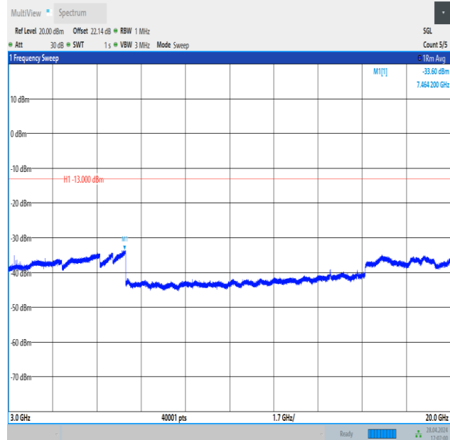
Band4_5MHz_QPSK_20375_1RB#0_3000~20000_3000~20000
