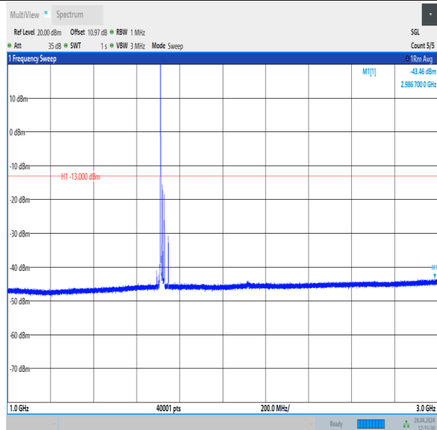
Band4_20MHz_16QAM_20050_1RB#0_1000~3000_1000~3000
