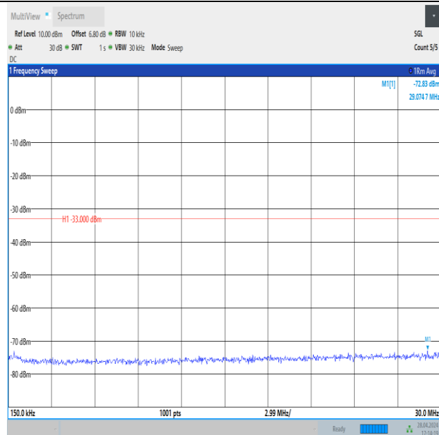
Band4_20MHz_QPSK_20050_1RB#0_0.15~30_0.15~30
