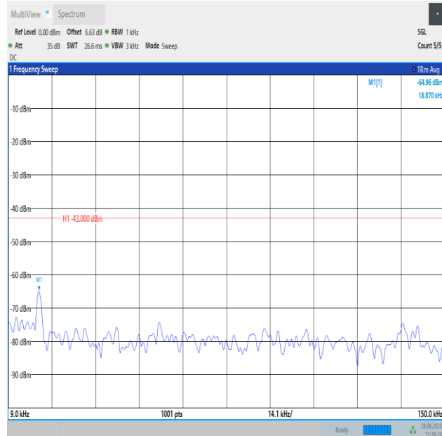
Band4_20MHz_16QAM_20175_1RB#0_0.009~0.15_0.009~0.15
