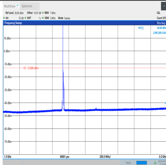
Band4_10MHz_16QAM_20175_1RB#0_1000~3000_1000~3000
