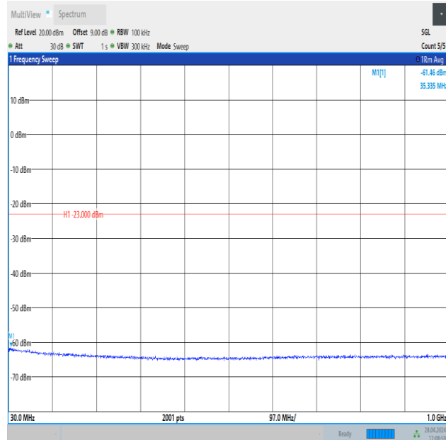
Band4_5MHz_16QAM_20375_1RB#24_30~1000_30~1000
