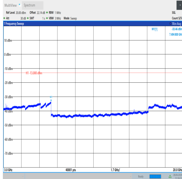
Band4_20MHz_QPSK_20175_1RB#0_3000~20000_3000~20000
