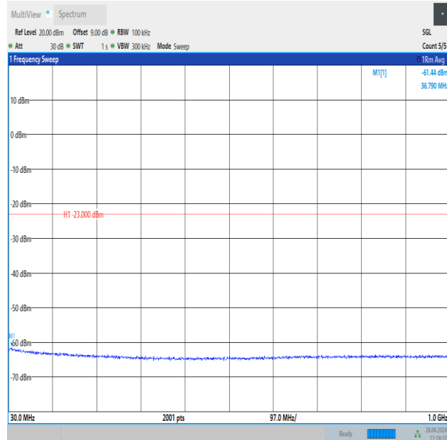
Band4_20MHz_16QAM_20175_1RB#0_30~1000_30~1000
