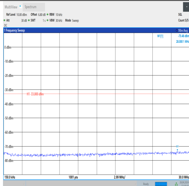
Band4_20MHz_QPSK_20175_1RB#99_0.15~30_0.15~30
