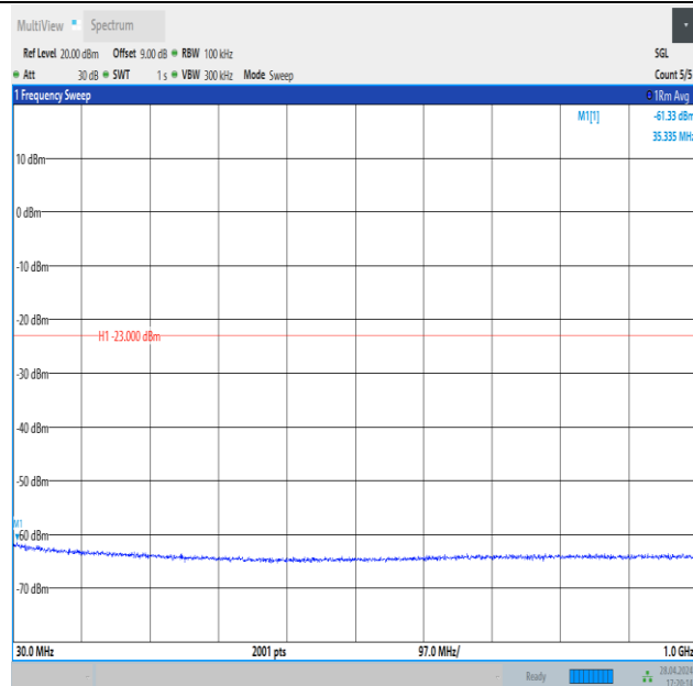
Band4_20MHz_16QAM_20175_1RB#99_30~1000_30~1000
