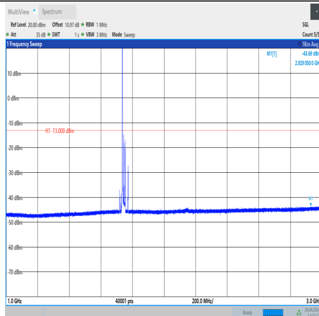
Band4_20MHz_QPSK_20300_1RB#0_1000~3000_1000~3000
