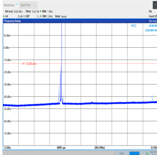
Band4_20MHz_QPSK_20300_1RB#99_1000~3000_1000~3000
