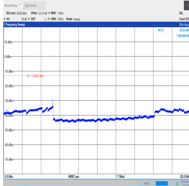
Band4_20MHz_QPSK_20300_1RB#0_3000~20000_3000~20000
