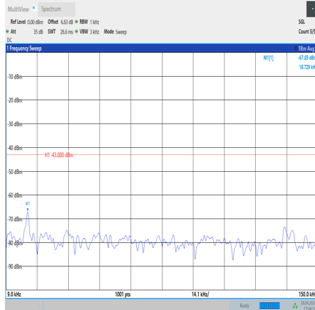
Band4_5MHz_QPSK_20375_1RB#0_0.009~0.15_0.009~0.15
