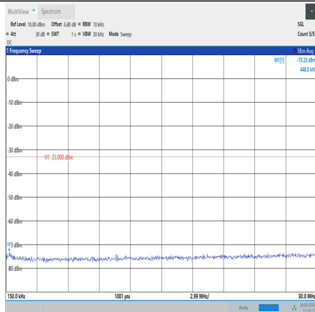
Band4_10MHz_QPSK_20000_1RB#0_0.15~30_0.15~30
