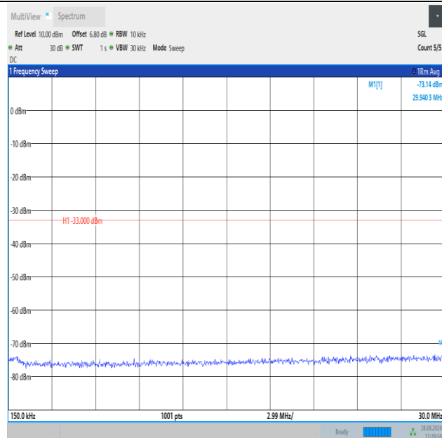
Band4_20MHz_QPSK_20300_1RB#0_0.15~30_0.15~30
