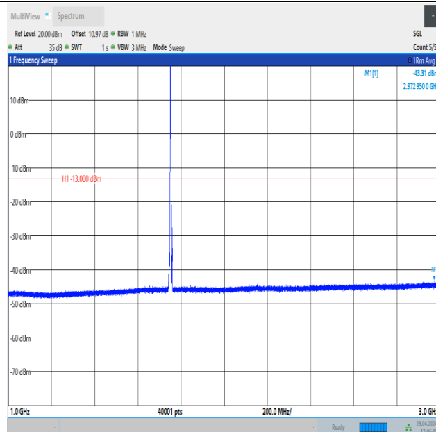
Band4_5MHz_QPSK_20375_1RB#0_1000~3000_1000~3000
