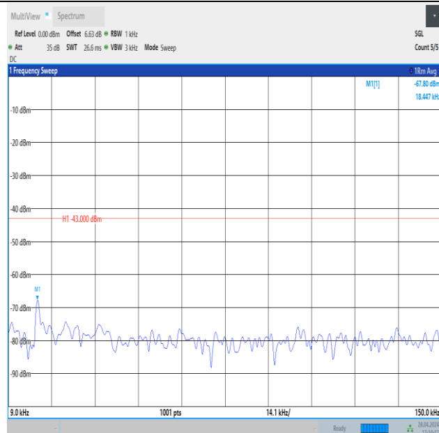
Band4_5MHz_16QAM_20375_25RB#0_0.009~0.15_0.009~0.15
