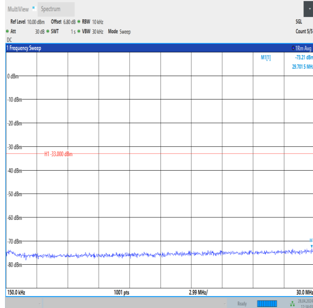
Band4_10MHz_16QAM_20000_1RB#0_0.15~30_0.15~30
