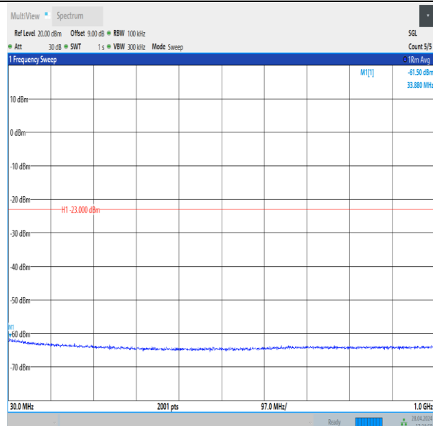
Band4_10MHz_QPSK_20000_1RB#49_30~1000_30~1000
