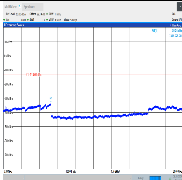
Band4_20MHz_16QAM_20050_1RB#99_3000~20000_3000~20000
