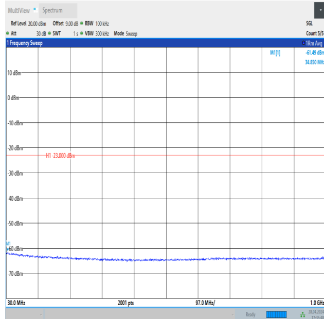
Band4_10MHz_16QAM_20000_1RB#49_30~1000_30~1000
