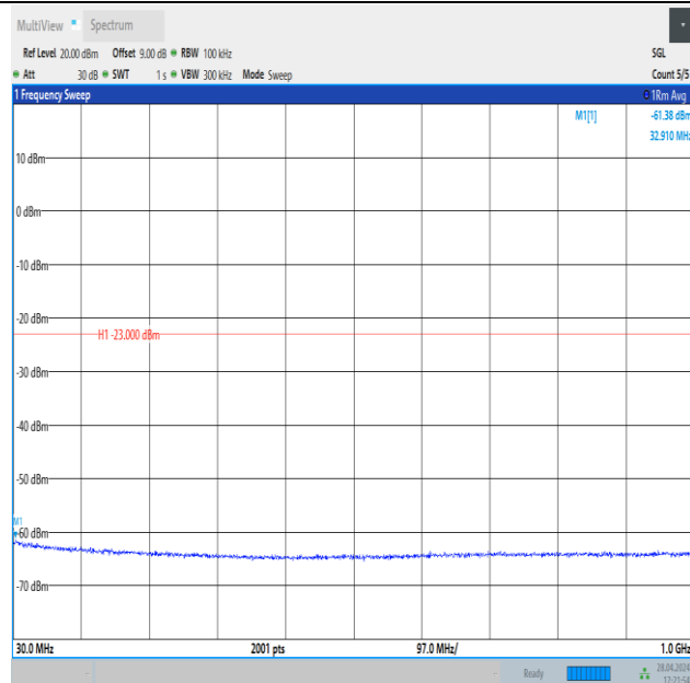
Band4_20MHz_16QAM_20300_1RB#0_30~1000_30~1000
