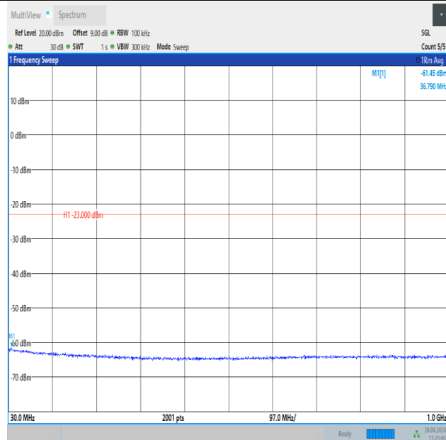
Band4_20MHz_QPSK_20300_1RB#0_30~1000_30~1000
