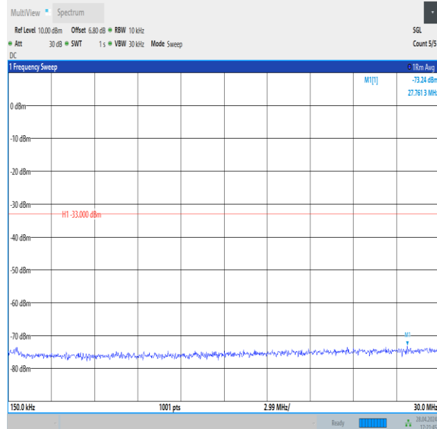
Band4_20MHz_16QAM_20300_1RB#0_0.15~30_0.15~30
