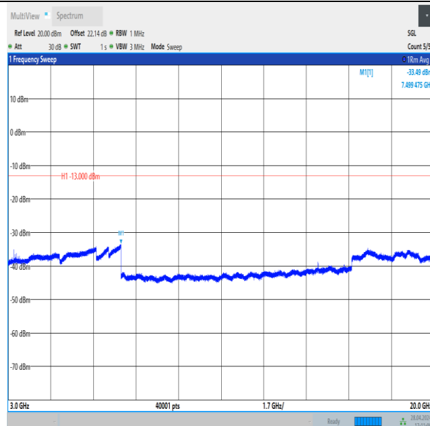
Band4_5MHz_16QAM_20375_25RB#0_3000~20000_3000~20000
