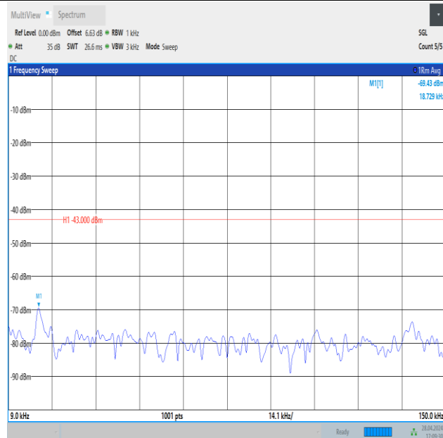
Band4_5MHz_QPSK_20375_25RB#0_0.009~0.15_0.009~0.15
