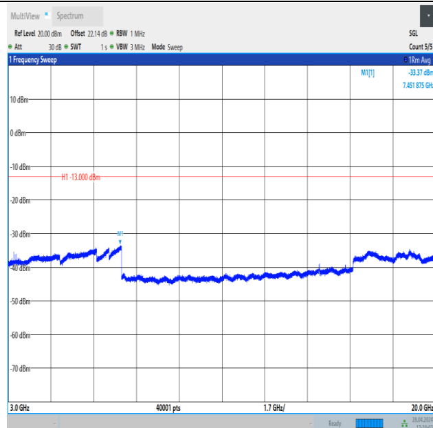
Band4_20MHz_16QAM_20175_1RB#0_3000~20000_3000~20000
