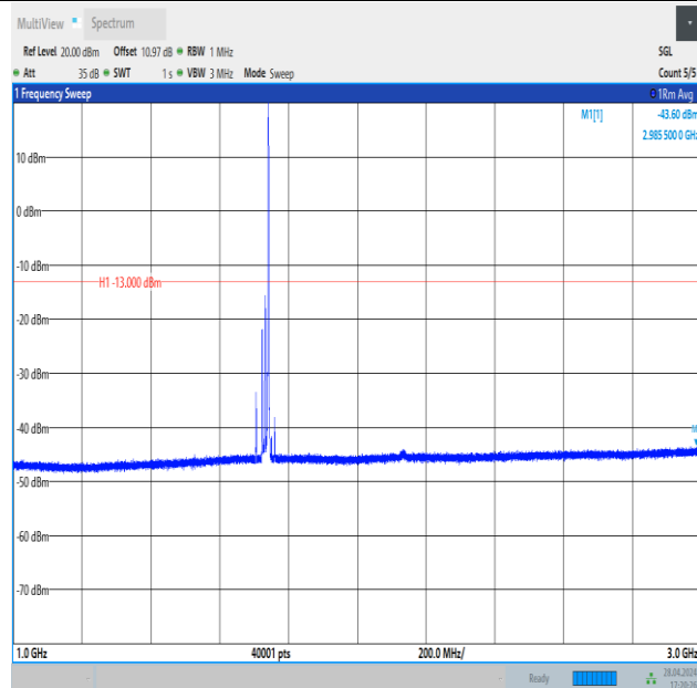
Band4_20MHz_16QAM_20175_1RB#99_1000~3000_1000~3000
