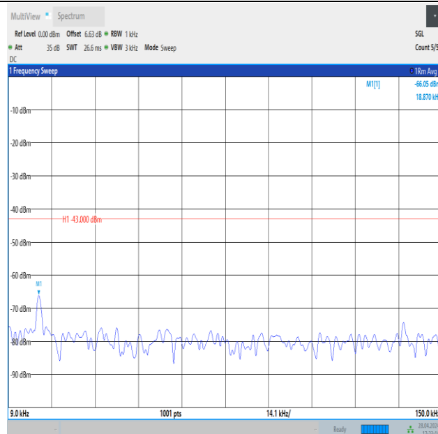
Band4_20MHz_16QAM_20300_1RB#99_0.009~0.15_0.009~0.15
