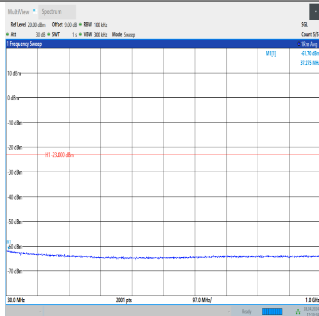
Band4_5MHz_16QAM_20375_25RB#0_30~1000_30~1000
