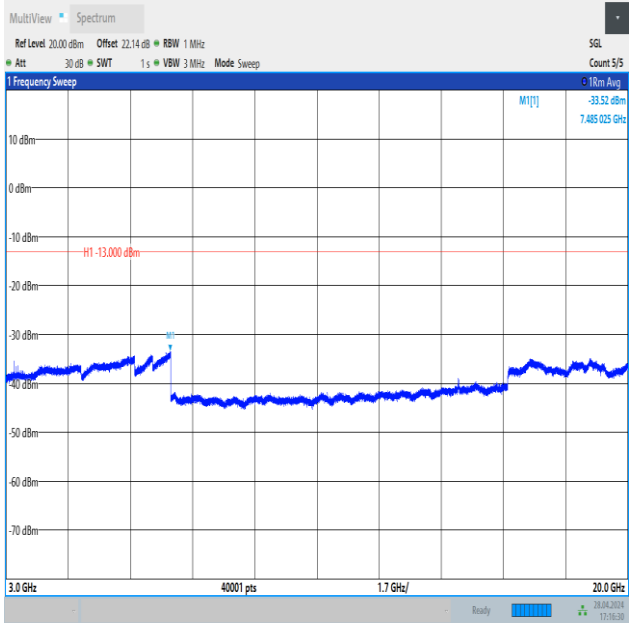
Band4_20MHz_QPSK_20050_1RB#99_3000~20000_3000~20000
