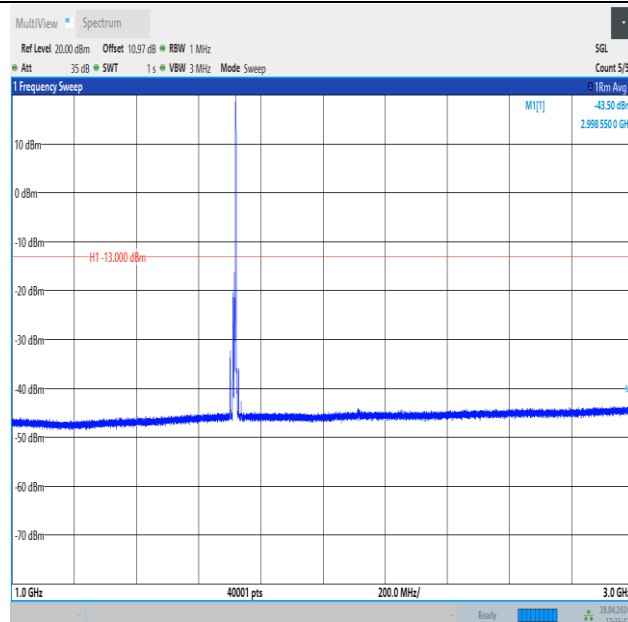
Band4_10MHz_QPSK_20000_1RB#49_1000~3000_1000~3000
