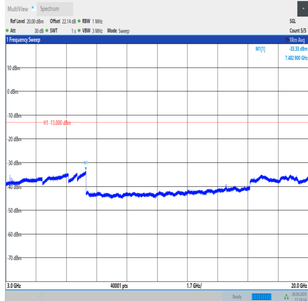
Band4_20MHz_QPSK_20050_1RB#0_3000~20000_3000~20000
