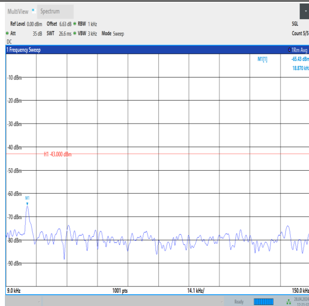
Band4_20MHz_16QAM_20300_1RB#0_0.009~0.15_0.009~0.15
