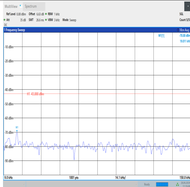
Band4_20MHz_QPSK_20175_1RB#99_0.009~0.15_0.009~0.15
