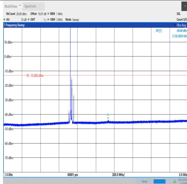
Band4_20MHz_16QAM_20175_1RB#0_1000~3000_1000~3000
