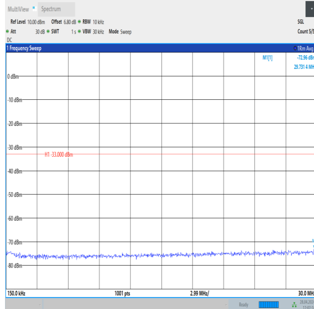
Band4_5MHz_16QAM_20375_1RB#0_0.15~30_0.15~30
