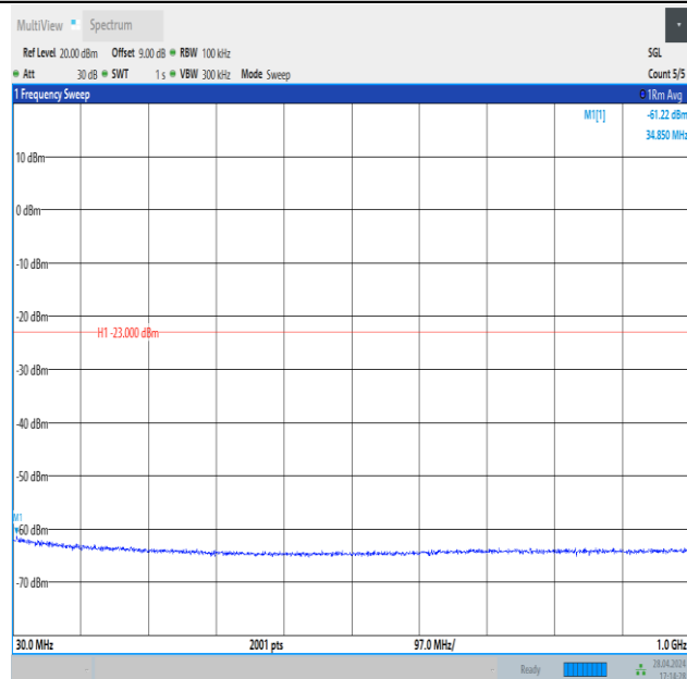
Band4_20MHz_QPSK_20050_1RB#0_30~1000_30~1000
