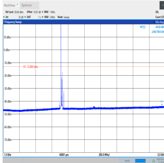
Band4_20MHz_QPSK_20050_1RB#0_1000~3000_1000~3000
