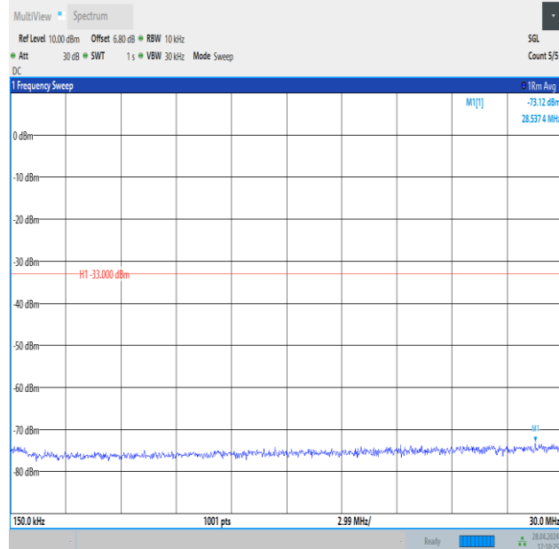
Band4_5MHz_16QAM_20375_25RB#0_0.15~30_0.15~30
