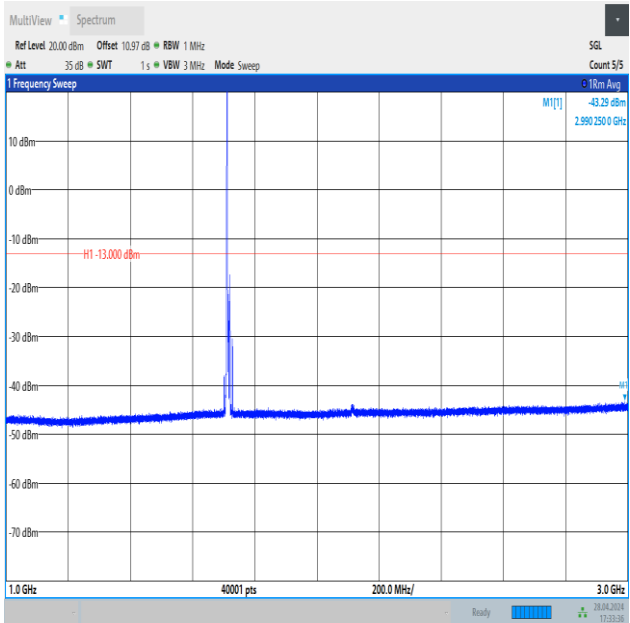
Band4_10MHz_QPSK_20000_1RB#0_1000~3000_1000~3000
