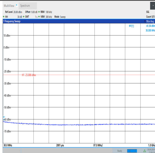
Band4_5MHz_QPSK_20375_1RB#0_30~1000_30~1000
