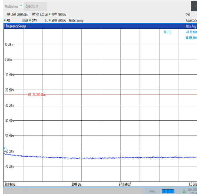
Band4_20MHz_16QAM_20050_1RB#99_30~1000_30~1000
