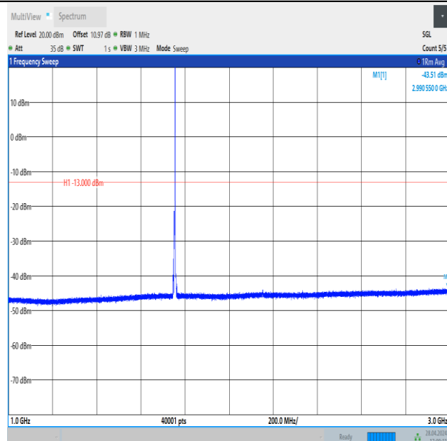
Band4_5MHz_16QAM_20375_1RB#24_1000~3000_1000~3000
