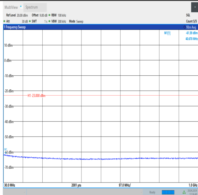
Band4_10MHz_QPSK_20175_1RB#0_30~1000_30~1000
