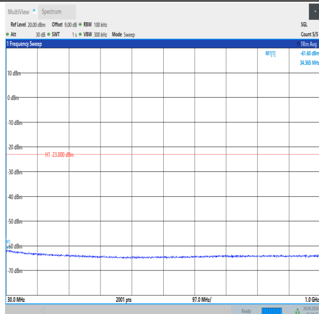
Band4_20MHz_QPSK_20175_1RB#99_30~1000_30~1000
