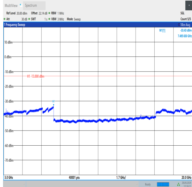
Band4_5MHz_QPSK_20375_25RB#0_3000~20000_3000~20000
