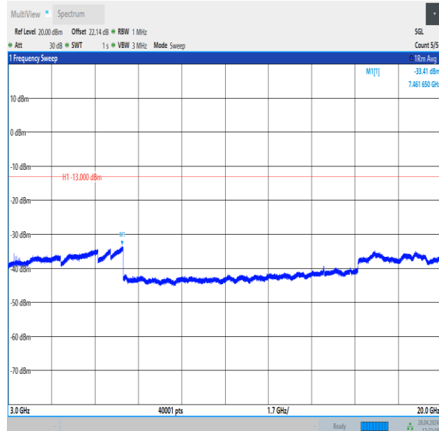
Band4_20MHz_16QAM_20300_1RB#0_3000~20000_3000~20000
