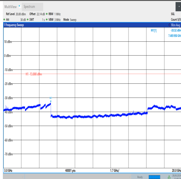
Band4_5MHz_16QAM_20375_1RB#24_3000~20000_3000~20000
