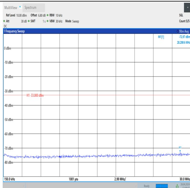
Band4_5MHz_QPSK_20375_1RB#24_0.15~30_0.15~30
