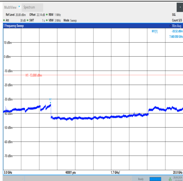
Band4_20MHz_16QAM_20300_1RB#99_3000~20000_3000~20000
