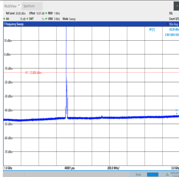
Band4_10MHz_16QAM_20000_1RB#0_1000~3000_1000~3000
