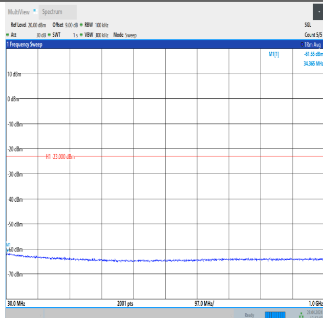
Band4_20MHz_QPSK_20175_1RB#0_30~1000_30~1000
