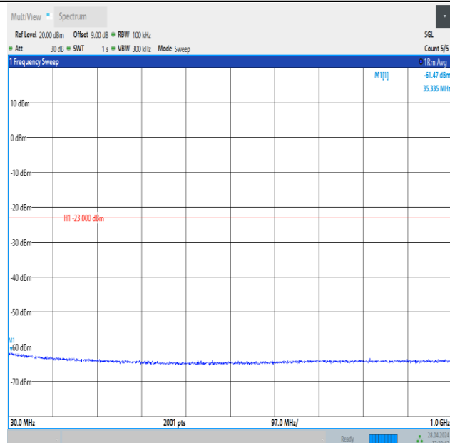
Band4_20MHz_QPSK_20300_1RB#99_30~1000_30~1000
