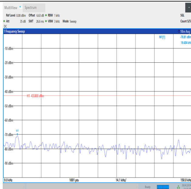
Band4_10MHz_16QAM_20000_1RB#49_0.009~0.15_0.009~0.15
