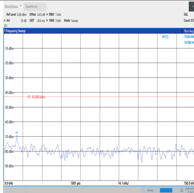
Band4_10MHz_QPSK_20175_1RB#0_0.009~0.15_0.009~0.15
