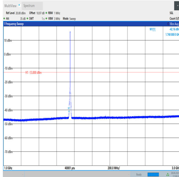
Band4_5MHz_QPSK_20375_25RB#0_1000~3000_1000~3000
