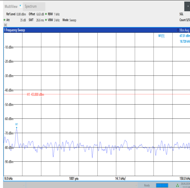
Band4_20MHz_QPSK_20175_1RB#0_0.009~0.15_0.009~0.15
