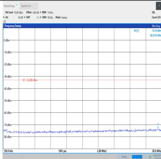
Band4_5MHz_QPSK_20375_25RB#0_0.15~30_0.15~30
