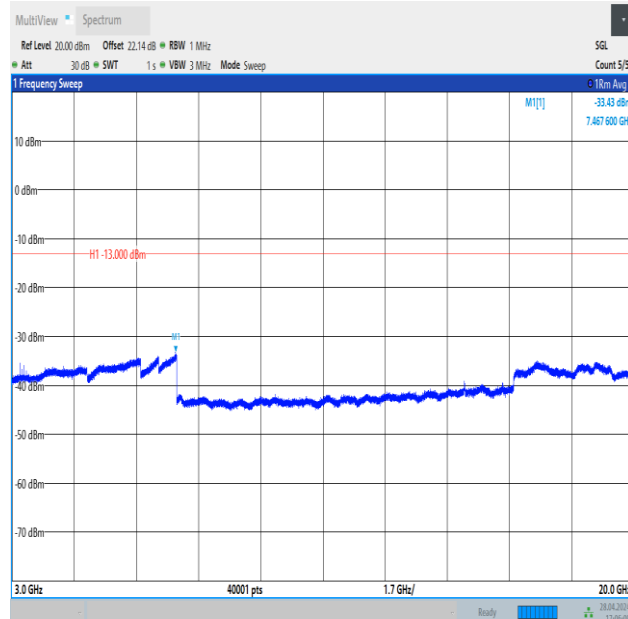
Band4_5MHz_16QAM_20175_25RB#0_3000~20000_3000~20000
