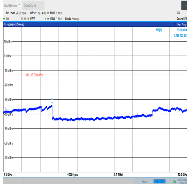
Band4_5MHz_QPSK_20375_1RB#24_3000~20000_3000~20000
