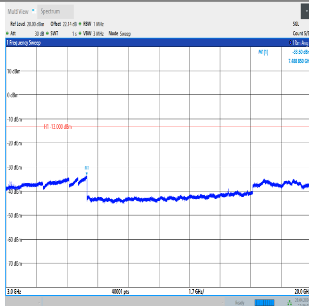
Band4_10MHz_16QAM_20000_1RB#49_3000~20000_3000~20000
