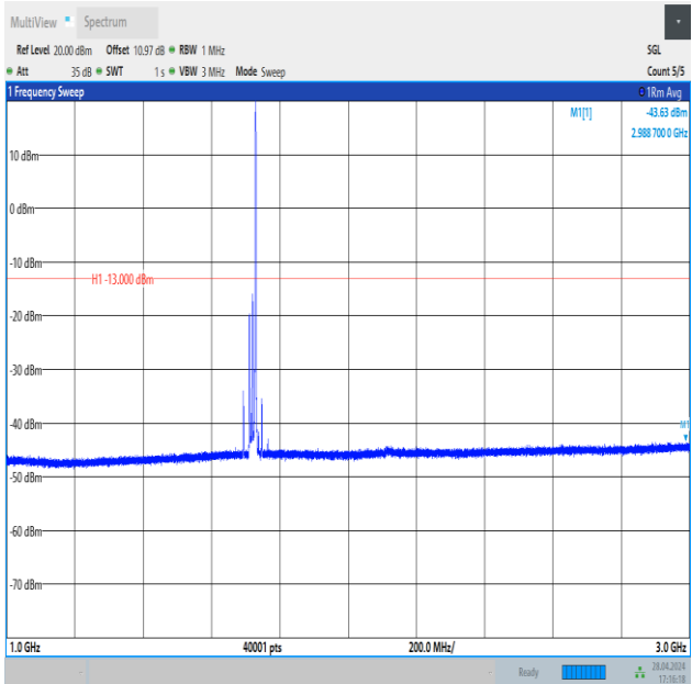
Band4_20MHz_QPSK_20050_1RB#99_1000~3000_1000~3000
