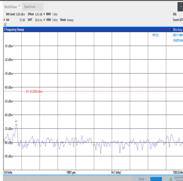
Band4_10MHz_16QAM_20000_1RB#0_0.009~0.15_0.009~0.15
