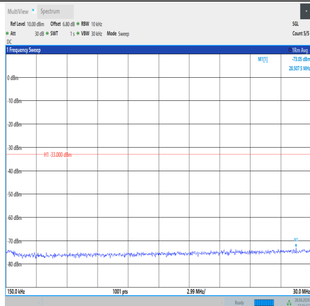
Band4_20MHz_QPSK_20050_1RB#99_0.15~30_0.15~30
