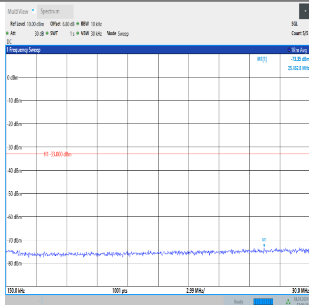
Band4_5MHz_QPSK_20375_1RB#0_0.15~30_0.15~30
