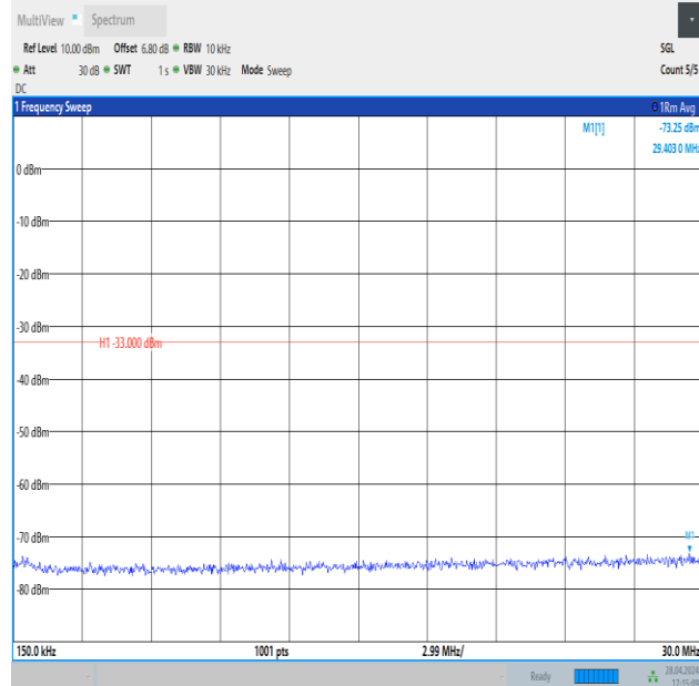
Band4_20MHz_16QAM_20050_1RB#0_0.15~30_0.15~30
