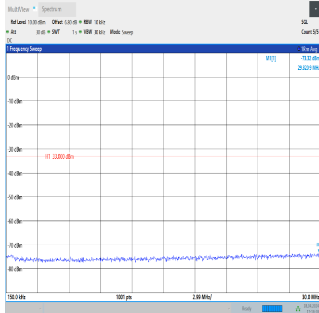
Band4_20MHz_16QAM_20175_1RB#0_0.15~30_0.15~30
