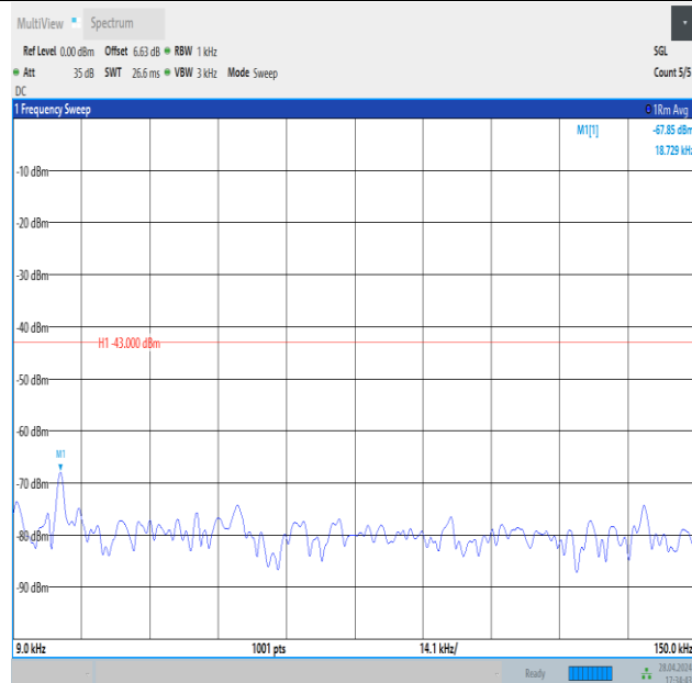
Band4_10MHz_QPSK_20000_1RB#49_0.009~0.15_0.009~0.15
