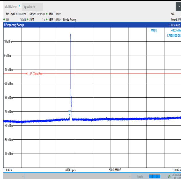
Band4_5MHz_16QAM_20375_25RB#0_1000~3000_1000~3000
