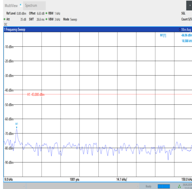
Band4_20MHz_QPSK_20300_1RB#99_0.009~0.15_0.009~0.15
