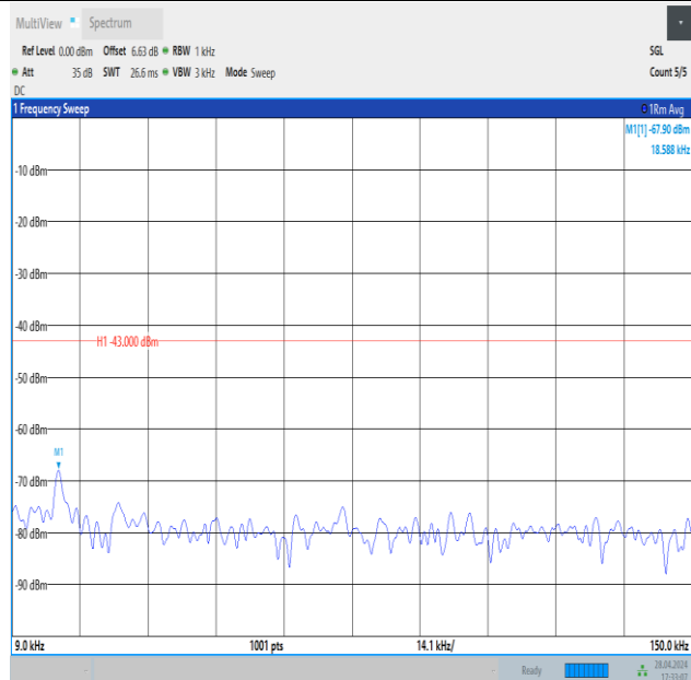
Band4_10MHz_QPSK_20000_1RB#0_0.009~0.15_0.009~0.15
