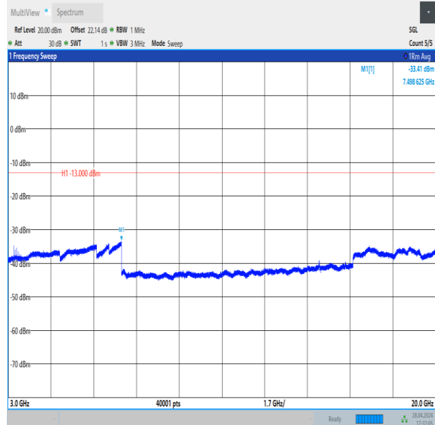
Band4_10MHz_QPSK_20175_1RB#0_3000~20000_3000~20000
