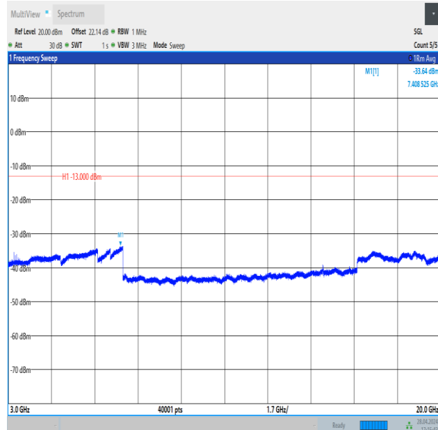
Band4_20MHz_16QAM_20050_1RB#0_3000~20000_3000~20000
