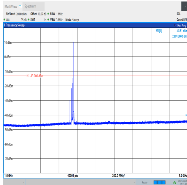
Band4_20MHz_16QAM_20300_1RB#99_1000~3000_1000~3000
