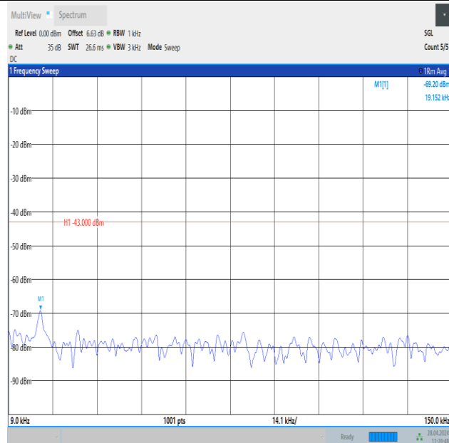
Band4_20MHz_QPSK_20300_1RB#0_0.009~0.15_0.009~0.15
