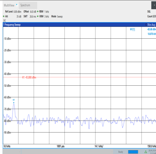
Band4_20MHz_QPSK_20050_1RB#99_0.009~0.15_0.009~0.15
