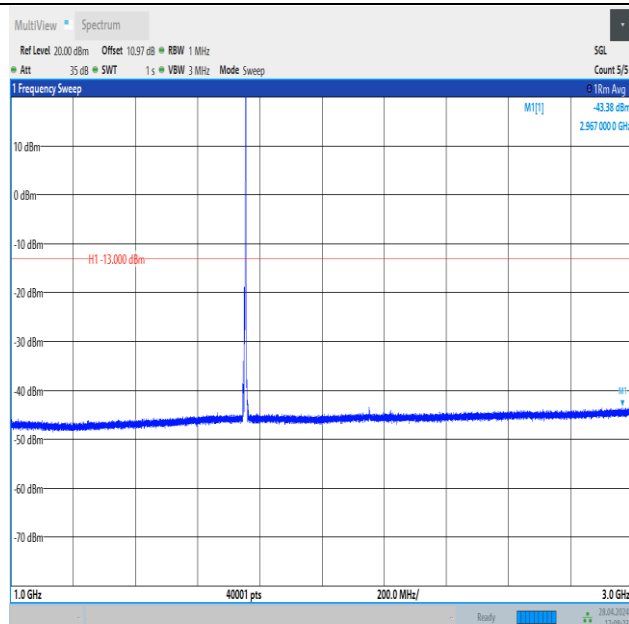
Band4_5MHz_QPSK_20375_1RB#24_1000~3000_1000~3000
