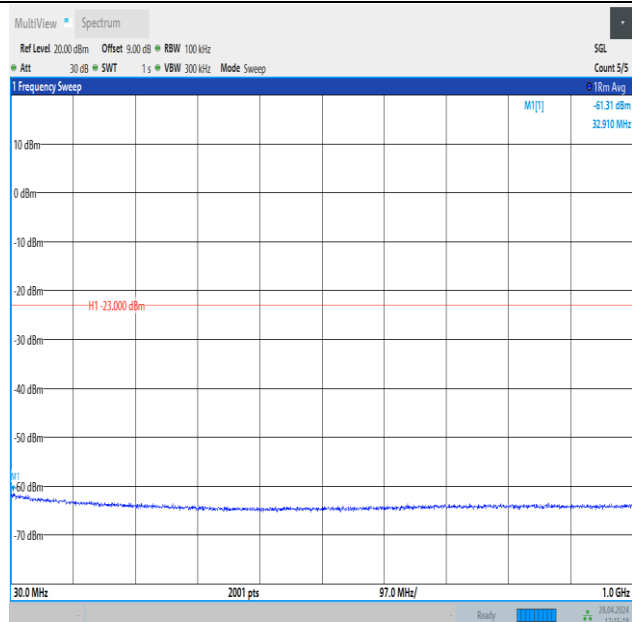
Band4_20MHz_16QAM_20050_1RB#0_30~1000_30~1000
