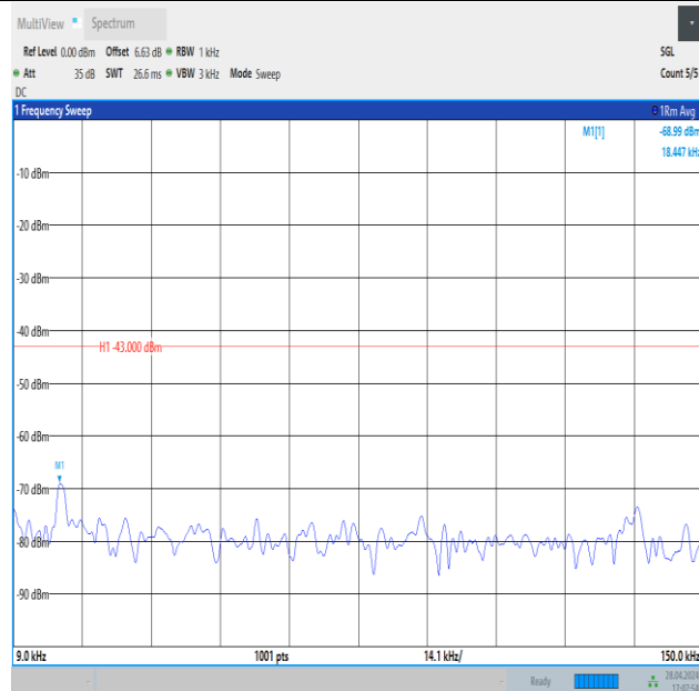
Band4_5MHz_QPSK_20375_1RB#24_0.009~0.15_0.009~0.15
