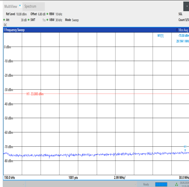
Band4_10MHz_16QAM_20000_1RB#49_0.15~30_0.15~30
