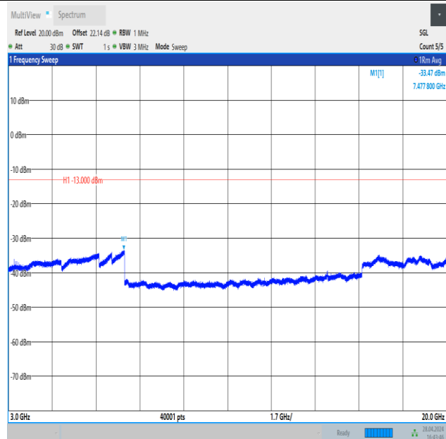
Band4_3MHz_16QAM_20385_15RB#0_3000~20000_3000~20000
