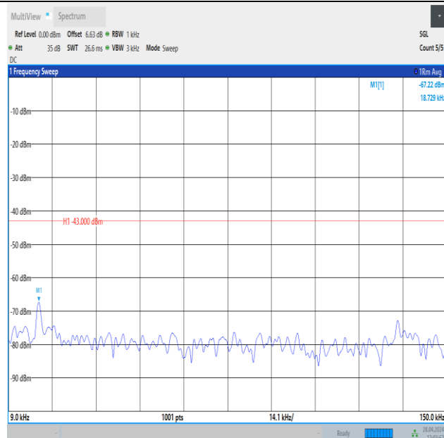
Band4_5MHz_16QAM_20175_1RB#24_0.009~0.15_0.009~0.15
