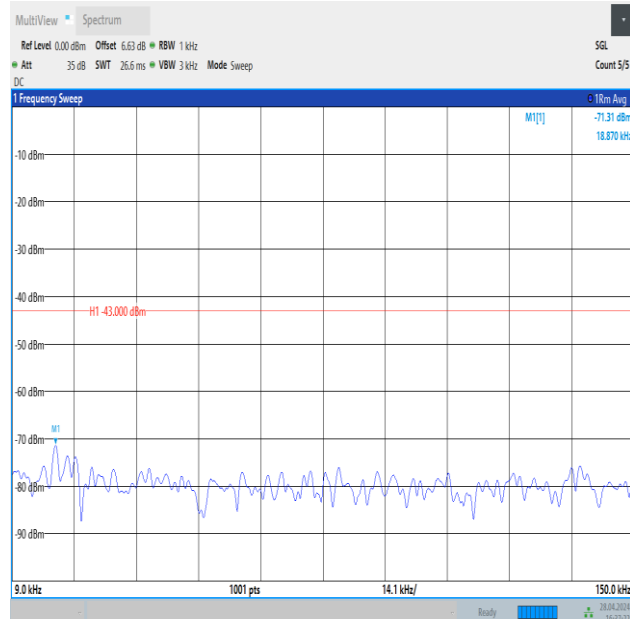
Band4_3MHz_QPSK_20175_15RB#0_0.009~0.15_0.009~0.15
