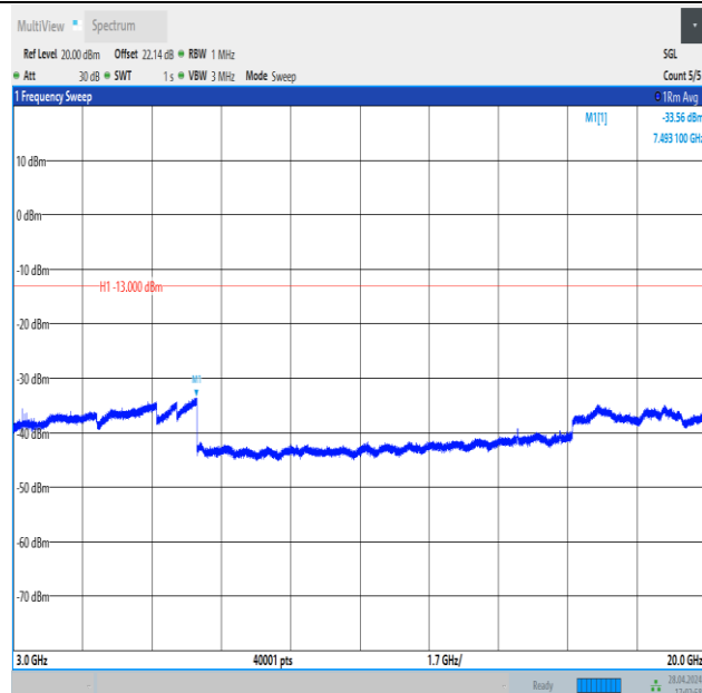
Band4_5MHz_16QAM_20175_1RB#0_3000~20000_3000~20000
