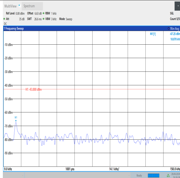
Band4_3MHz_16QAM_20175_1RB#14_0.009~0.15_0.009~0.15
