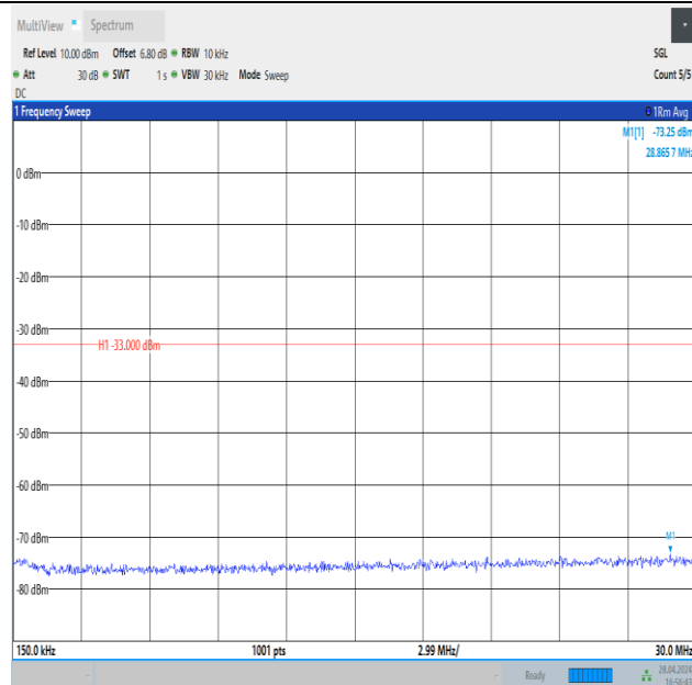
Band4_5MHz_QPSK_19975_1RB#0_0.15~30_0.15~30
