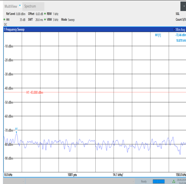
Band4_3MHz_16QAM_20385_15RB#0_0.009~0.15_0.009~0.15
