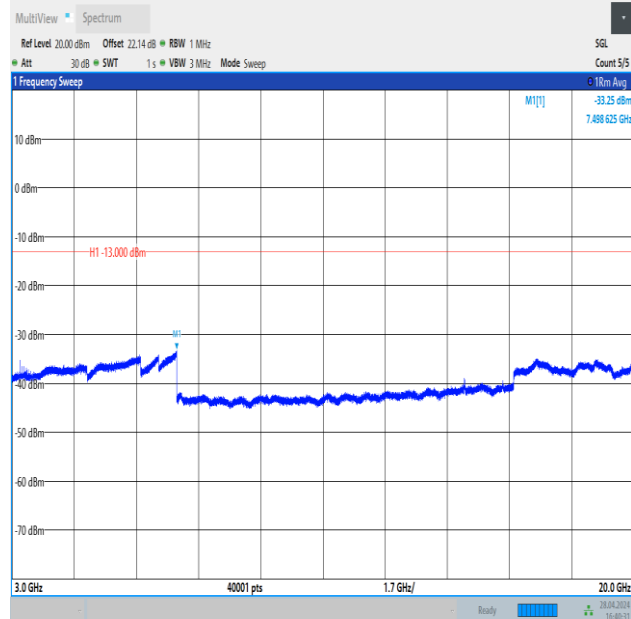
Band4_3MHz_16QAM_20385_1RB#0_3000~20000_3000~20000
