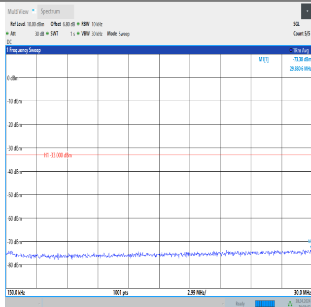
Band4_3MHz_16QAM_20175_1RB#14_0.15~30_0.15~30
