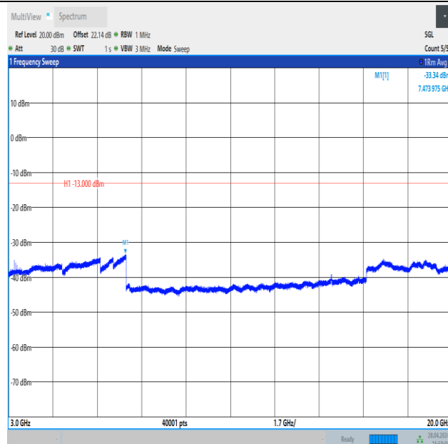
Band4_5MHz_16QAM_19975_1RB#0_3000~20000_3000~20000
