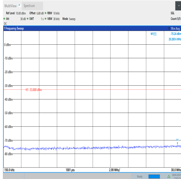
Band4_5MHz_QPSK_20175_1RB#24_0.15~30_0.15~30
