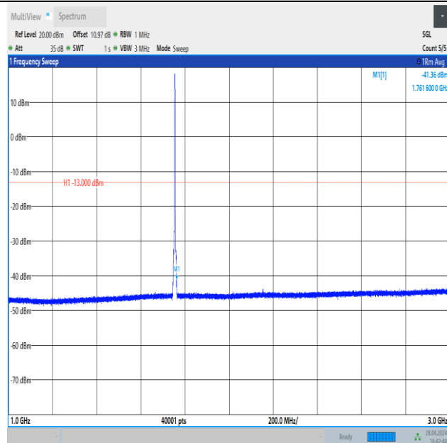
Band4_3MHz_QPSK_20385_15RB#0_1000~3000_1000~3000
