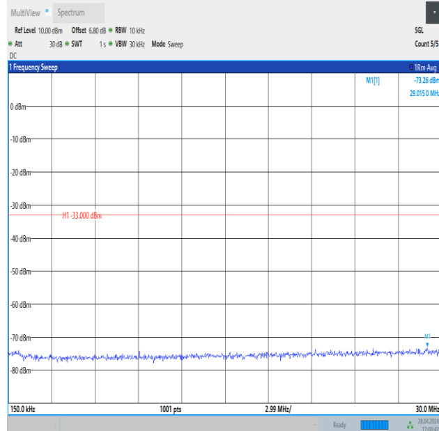
Band4_5MHz_16QAM_19975_25RB#0_0.15~30_0.15~30
