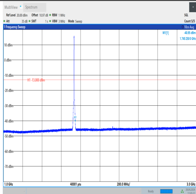
Band4_5MHz_16QAM_20175_25RB#0_1000~3000_1000~3000
