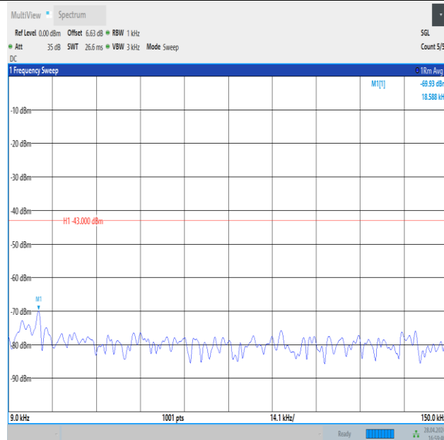
Band4_5MHz_QPSK_19975_25RB#0_0.009~0.15_0.009~0.15
