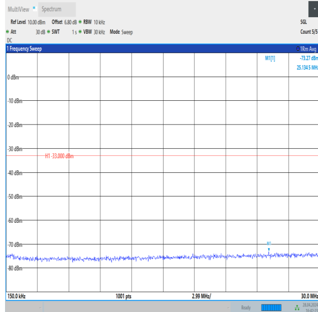
Band4_3MHz_QPSK_20385_15RB#0_0.15~30_0.15~30
