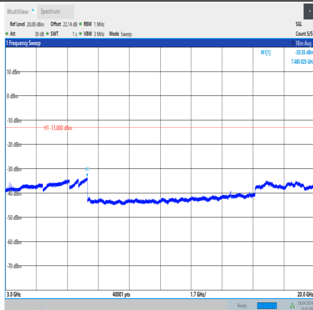
Band4_3MHz_16QAM_20385_1RB#14_3000~20000_3000~20000
