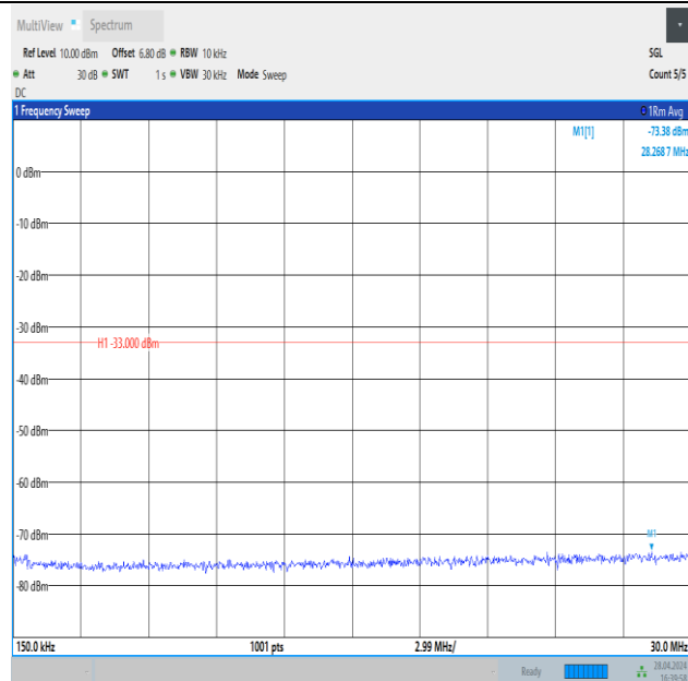
Band4_3MHz_16QAM_20385_1RB#0_0.15~30_0.15~30
