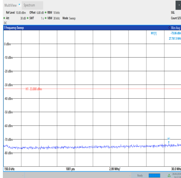
Band4_5MHz_16QAM_19975_1RB#0_0.15~30_0.15~30
