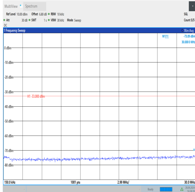
Band4_5MHz_QPSK_19975_1RB#24_0.15~30_0.15~30
