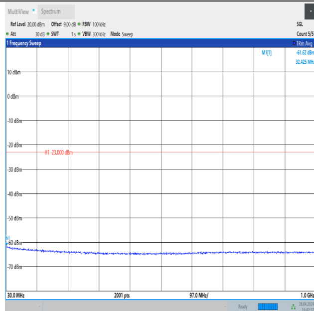
Band4_3MHz_QPSK_20385_15RB#0_30~1000_30~1000
