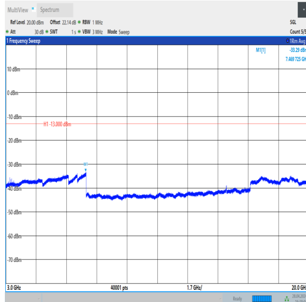
Band4_3MHz_QPSK_20175_15RB#0_3000~20000_3000~20000
