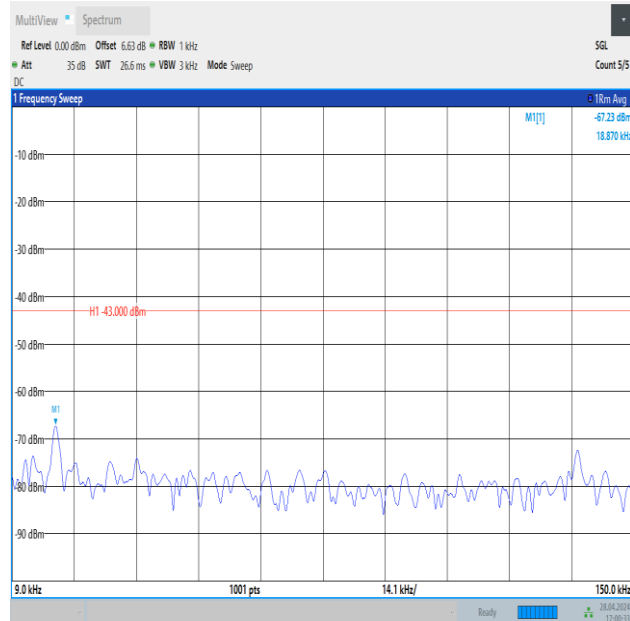
Band4_5MHz_16QAM_19975_25RB#0_0.009~0.15_0.009~0.15
