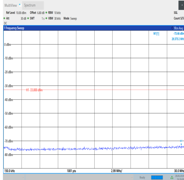
Band4_3MHz_QPSK_20385_1RB#0_0.15~30_0.15~30
