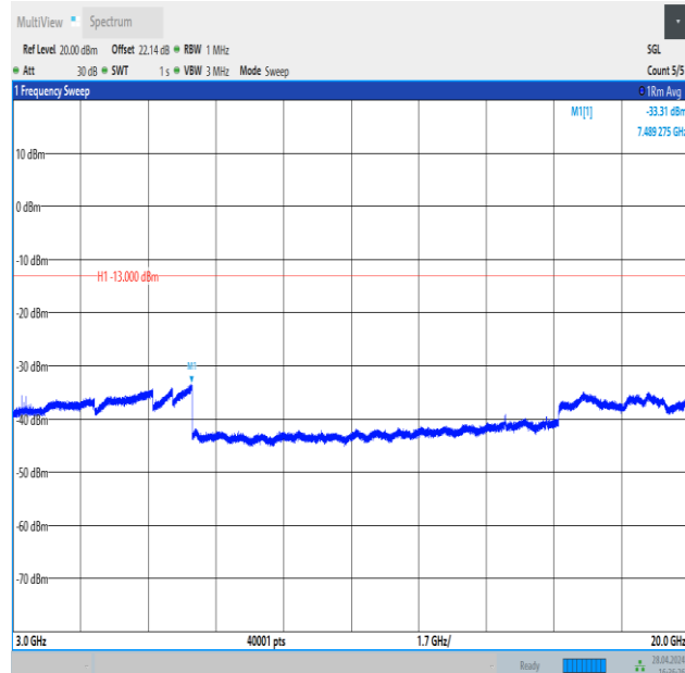
Band4_3MHz_QPSK_20175_1RB#14_3000~20000_3000~20000
