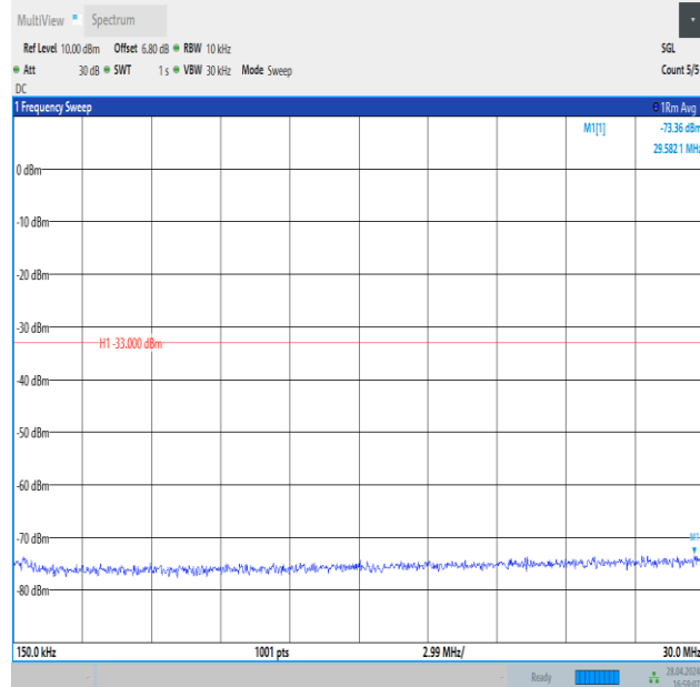
Band4_5MHz_16QAM_19975_1RB#24_0.15~30_0.15~30
