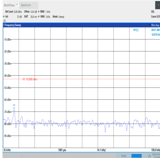
Band4_3MHz_QPSK_20385_1RB#0_0.009~0.15_0.009~0.15
