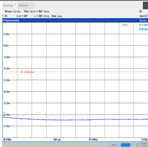
Band4_5MHz_16QAM_20175_25RB#0_30~1000_30~1000
