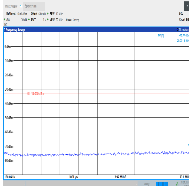
Band4_5MHz_QPSK_20175_25RB#0_0.15~30_0.15~30
