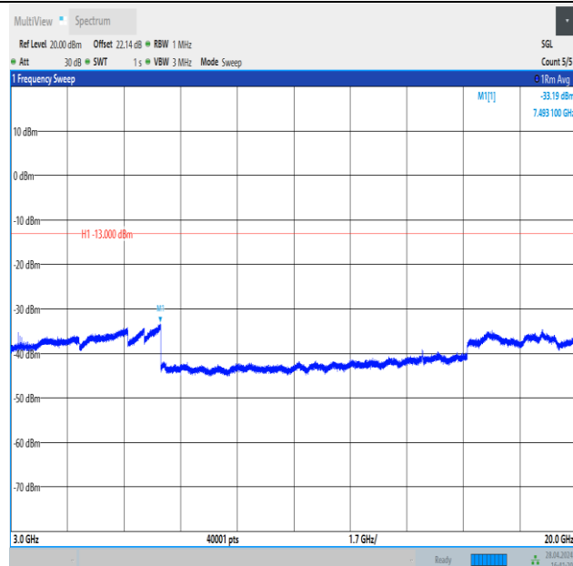
Band4_3MHz_QPSK_20385_1RB#14_3000~20000_3000~20000
