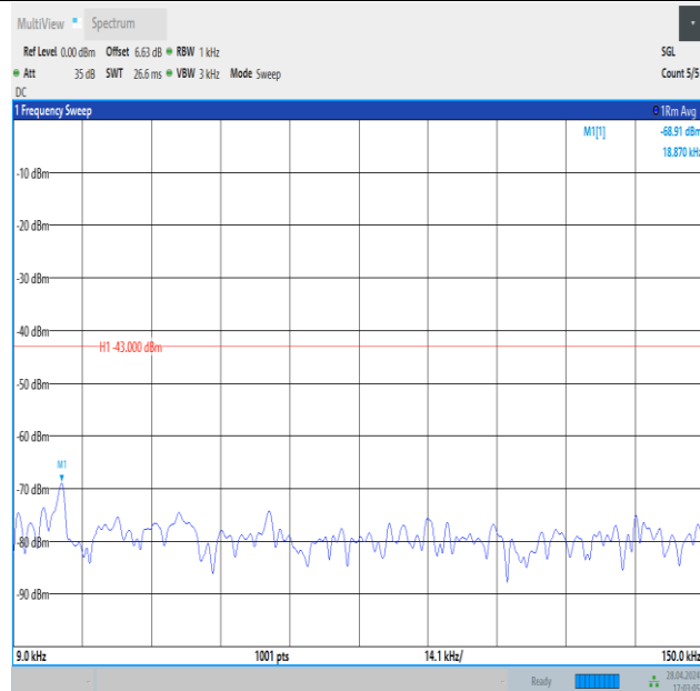
Band4_5MHz_QPSK_20175_1RB#24_0.009~0.15_0.009~0.15
