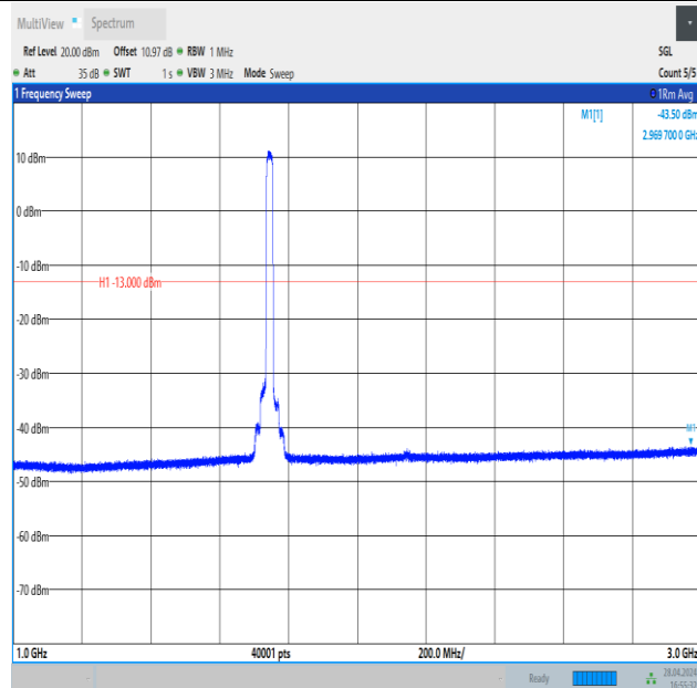
Band4_20MHz_QPSK_20300_100RB#0_1000~3000_1000~3000
