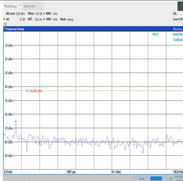
Band4_20MHz_QPSK_20175_100RB#0_0.009~0.15_0.009~0.15
