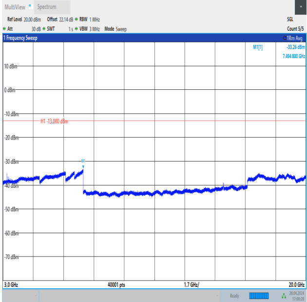
Band4_5MHz_QPSK_19975_25RB#0_3000~20000_3000~20000
