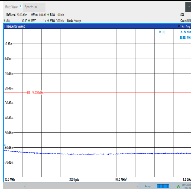
Band4_5MHz_16QAM_20175_1RB#24_30~1000_30~1000
