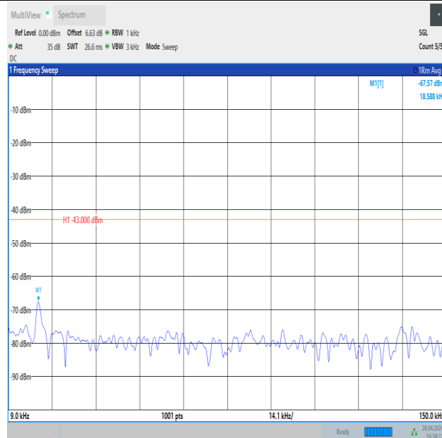
Band4_3MHz_16QAM_20175_15RB#0_0.009~0.15_0.009~0.15
