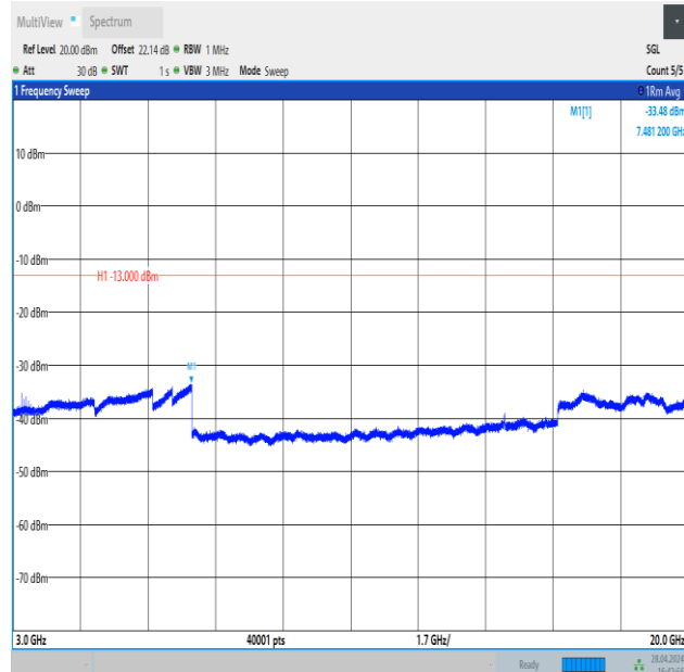
Band4_3MHz_QPSK_20385_15RB#0_3000~20000_3000~20000
