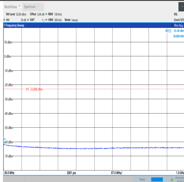
Band4_5MHz_QPSK_19975_1RB#0_30~1000_30~1000
