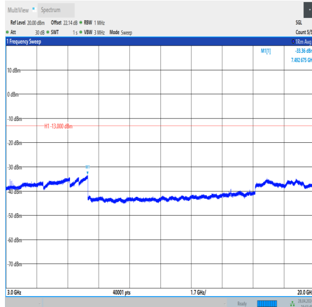
Band4_20MHz_QPSK_20300_100RB#0_3000~20000_3000~20000
