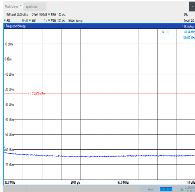
Band4_5MHz_QPSK_20175_1RB#24_30~1000_30~1000
