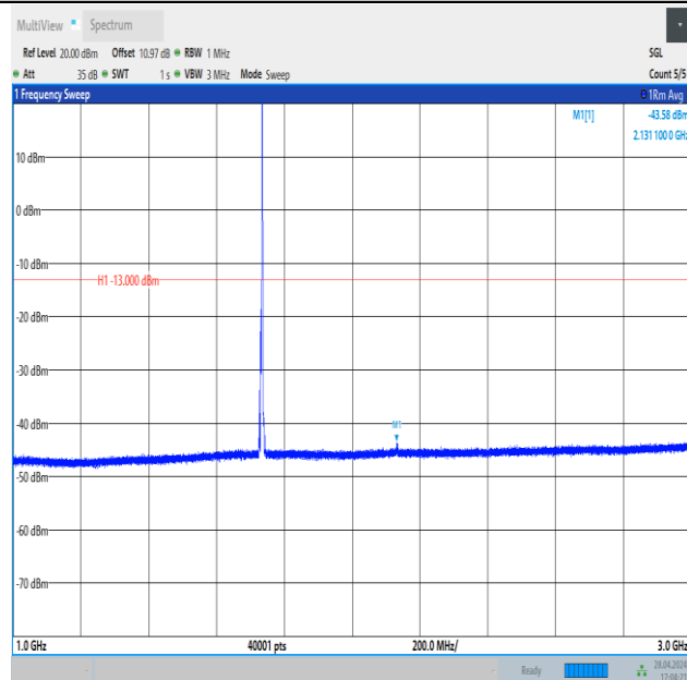
Band4_5MHz_16QAM_20175_1RB#24_1000~3000_1000~3000
