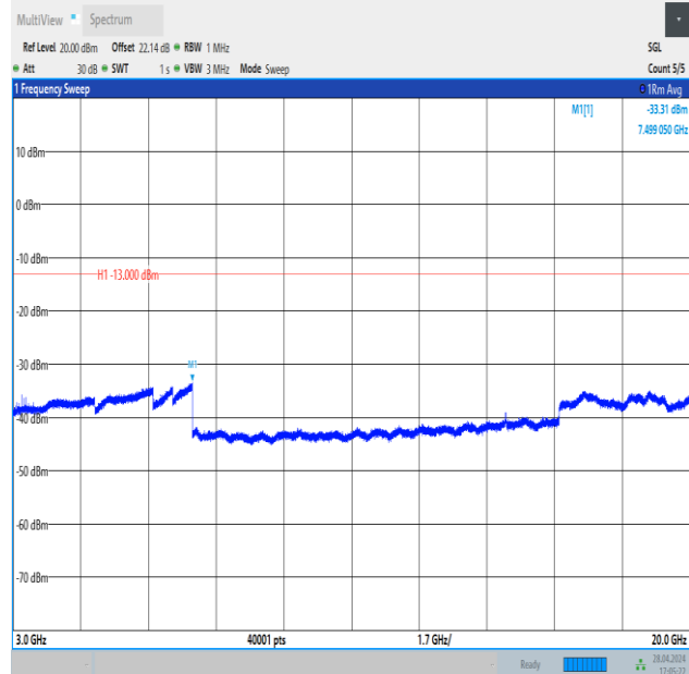
Band4_5MHz_QPSK_20175_25RB#0_3000~20000_3000~20000
