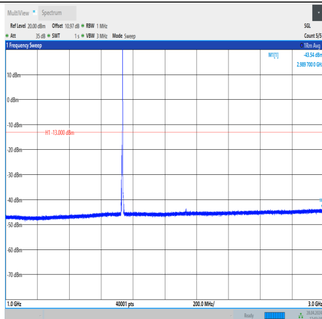
Band4_5MHz_QPSK_20175_1RB#24_1000~3000_1000~3000
