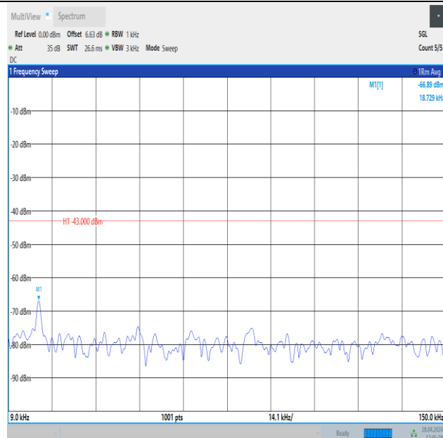
Band4_5MHz_16QAM_20175_25RB#0_0.009~0.15_0.009~0.15
