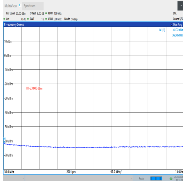
Band4_20MHz_QPSK_20050_100RB#0_30~1000_30~1000
