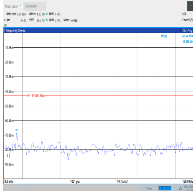
Band4_5MHz_16QAM_19975_1RB#0_0.009~0.15_0.009~0.15
