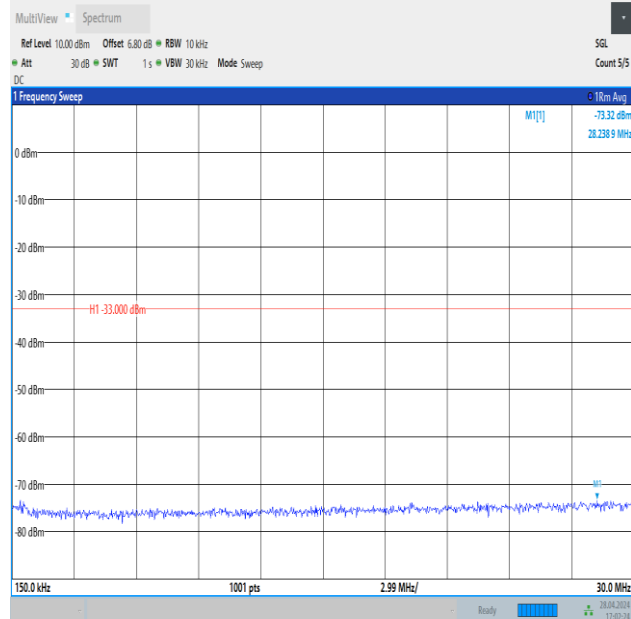
Band4_5MHz_16QAM_20175_1RB#0_0.15~30_0.15~30
