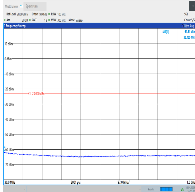
Band4_20MHz_QPSK_20300_100RB#0_30~1000_30~1000
