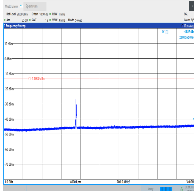
Band4_3MHz_16QAM_20385_1RB#0_1000~3000_1000~3000
