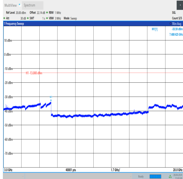
Band4_5MHz_QPSK_20175_1RB#0_3000~20000_3000~20000
