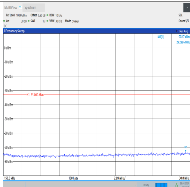
Band4_5MHz_QPSK_19975_25RB#0_0.15~30_0.15~30
