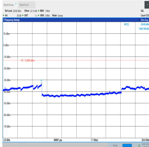
Band4_5MHz_16QAM_19975_25RB#0_3000~20000_3000~20000
