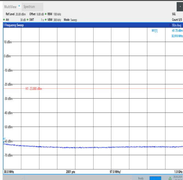
Band4_3MHz_16QAM_20175_15RB#0_30~1000_30~1000
