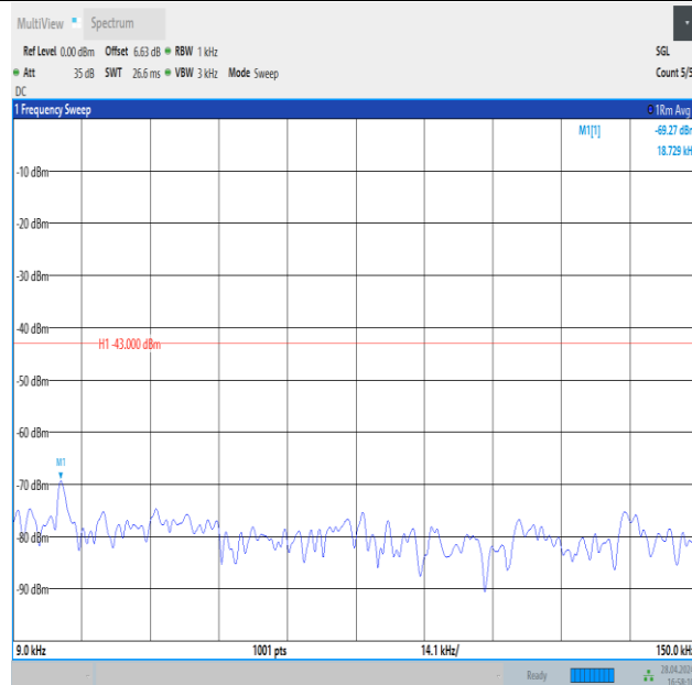
Band4_5MHz_QPSK_19975_1RB#24_0.009~0.15_0.009~0.15
