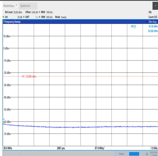
Band4_5MHz_QPSK_19975_25RB#0_30~1000_30~1000
