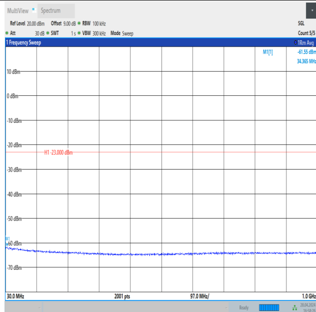
Band4_5MHz_QPSK_19975_1RB#24_30~1000_30~1000
