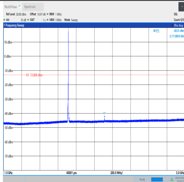
Band4_5MHz_16QAM_19975_1RB#24_1000~3000_1000~3000
