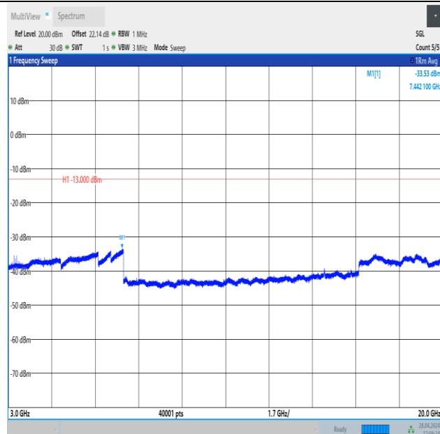
Band4_5MHz_16QAM_20175_1RB#24_3000~20000_3000~20000
