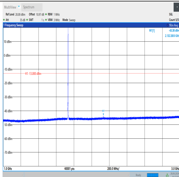
Band4_3MHz_16QAM_20175_1RB#14_1000~3000_1000~3000
