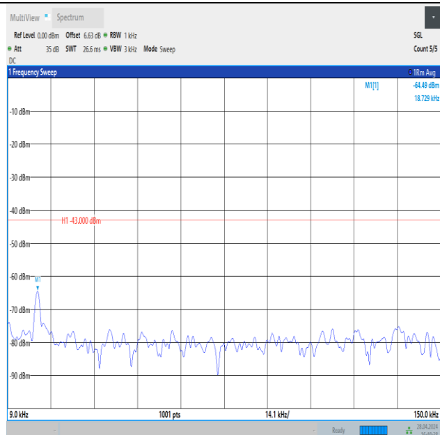
Band4_3MHz_QPSK_20385_1RB#14_0.009~0.15_0.009~0.15
