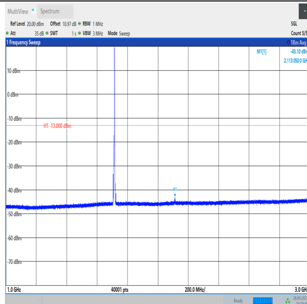
Band4_5MHz_QPSK_19975_1RB#24_1000~3000_1000~3000
