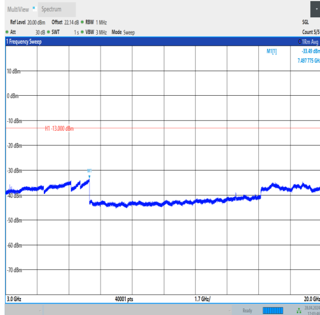
Band4_5MHz_QPSK_20175_1RB#24_3000~20000_3000~20000
