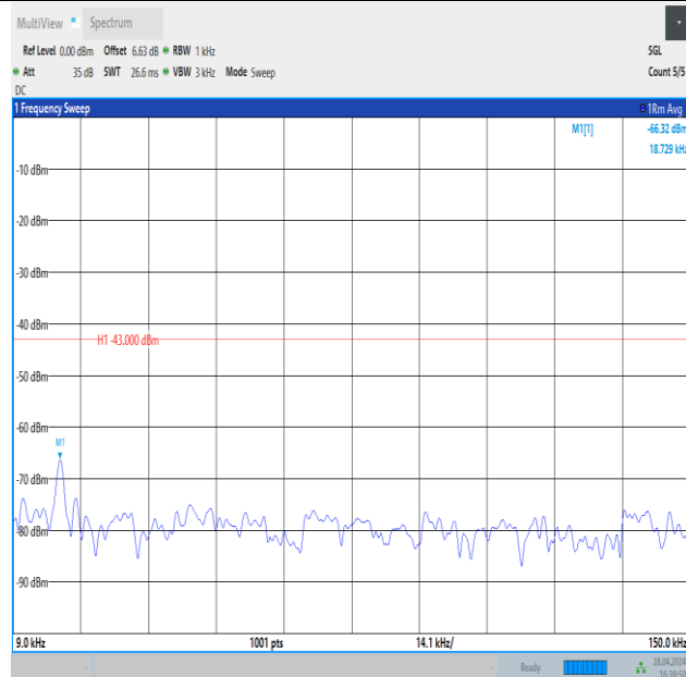
Band4_3MHz_16QAM_20385_1RB#0_0.009~0.15_0.009~0.15
