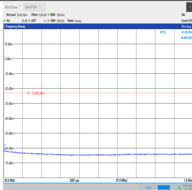
Band4_5MHz_16QAM_19975_1RB#0_30~1000_30~1000
