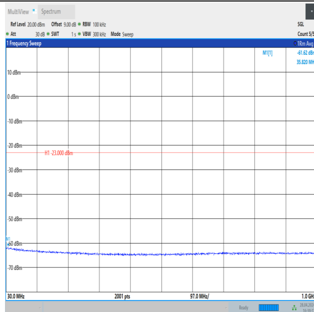
Band4_3MHz_QPSK_20385_1RB#0_30~1000_30~1000
