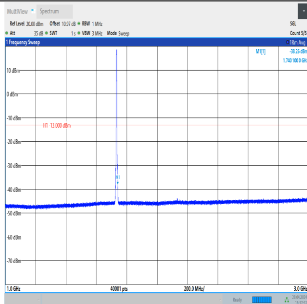
Band4_3MHz_QPSK_20175_15RB#0_1000~3000_1000~3000
