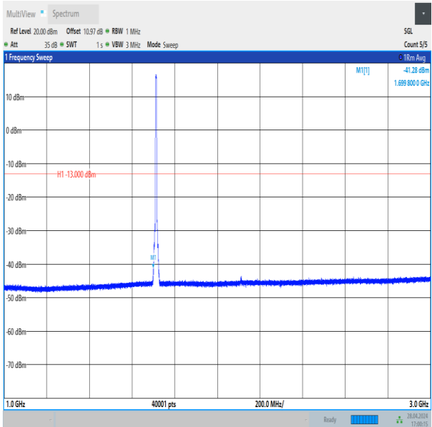
Band4_5MHz_QPSK_19975_25RB#0_1000~3000_1000~3000
