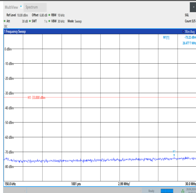
Band4_3MHz_16QAM_20385_15RB#0_0.15~30_0.15~30
