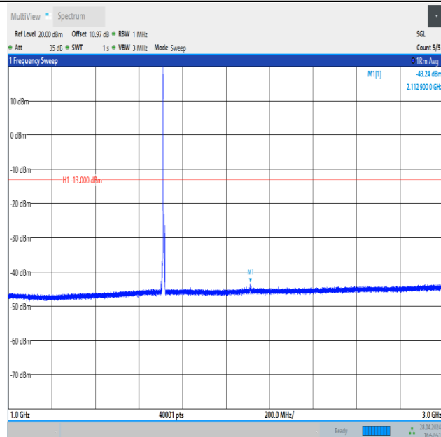
Band4_5MHz_16QAM_19975_1RB#0_1000~3000_1000~3000
