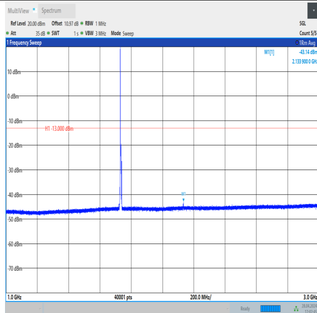
Band4_5MHz_16QAM_20175_1RB#0_1000~3000_1000~3000
