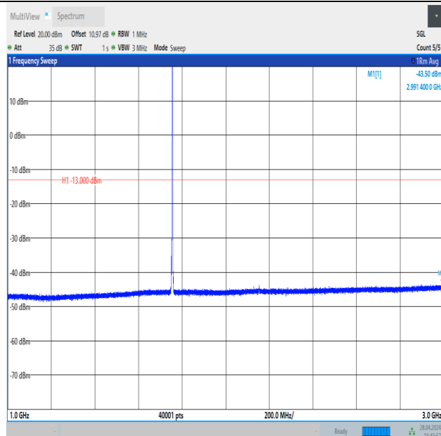
Band4_3MHz_16QAM_20385_1RB#14_1000~3000_1000~3000
