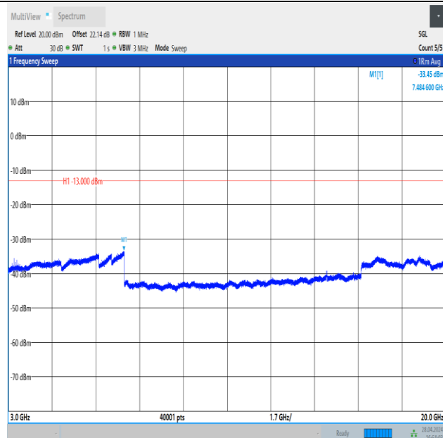
Band4_20MHz_QPSK_20050_100RB#0_3000~20000_3000~20000
