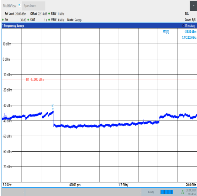
Band4_20MHz_QPSK_20175_100RB#0_3000~20000_3000~20000
