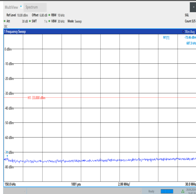
Band4_3MHz_16QAM_20385_1RB#14_0.15~30_0.15~30
