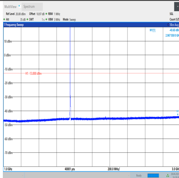
Band4_3MHz_QPSK_20385_1RB#0_1000~3000_1000~3000
