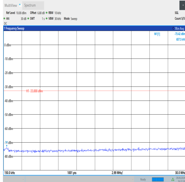
Band4_3MHz_QPSK_20175_15RB#0_0.15~30_0.15~30
