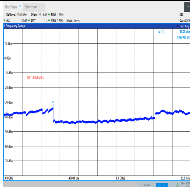
Band4_3MHz_QPSK_20385_1RB#0_3000~20000_3000~20000
