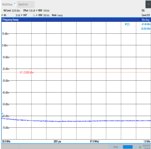
Band4_20MHz_QPSK_20175_100RB#0_30~1000_30~1000
