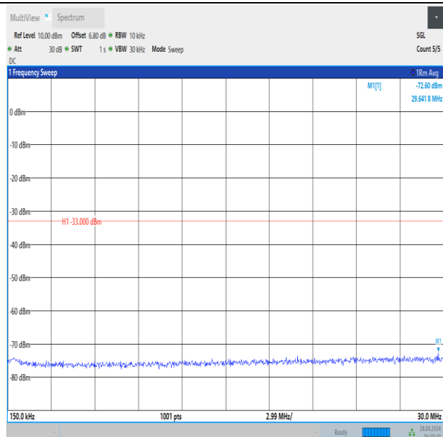
Band4_3MHz_16QAM_20175_15RB#0_0.15~30_0.15~30
