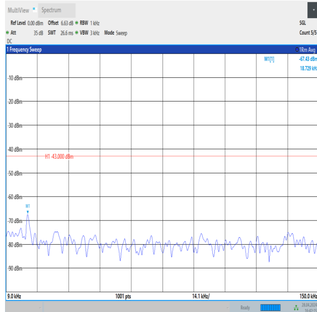
Band4_3MHz_QPSK_20385_15RB#0_0.009~0.15_0.009~0.15
