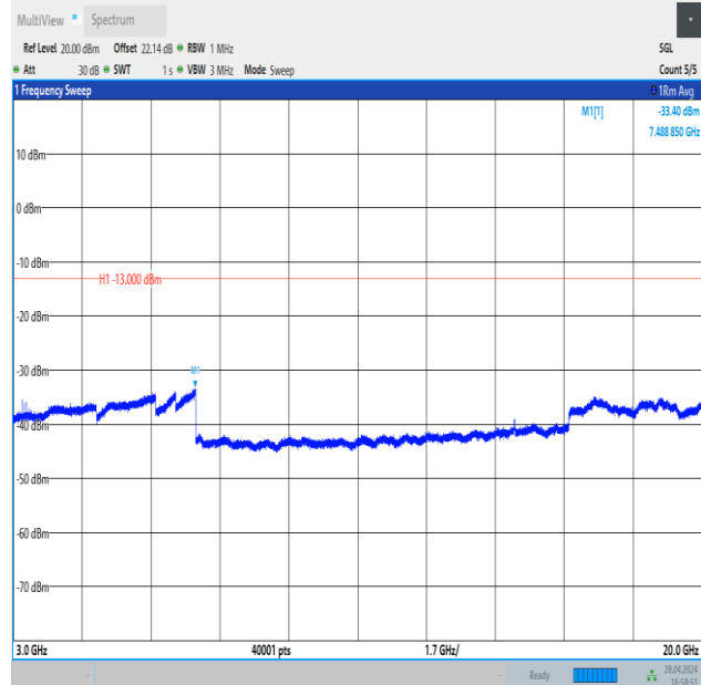
Band4_5MHz_QPSK_19975_1RB#24_3000~20000_3000~20000
