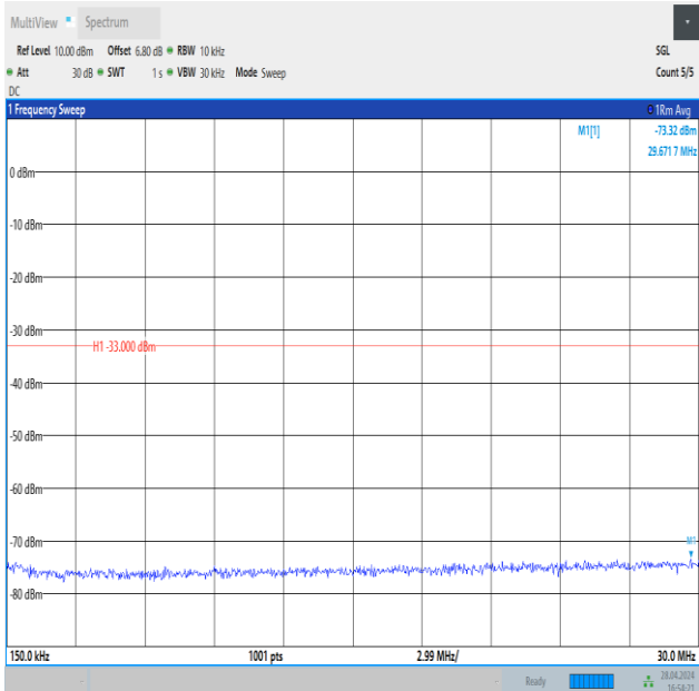
Band4_20MHz_QPSK_20175_100RB#0_0.15~30_0.15~30
