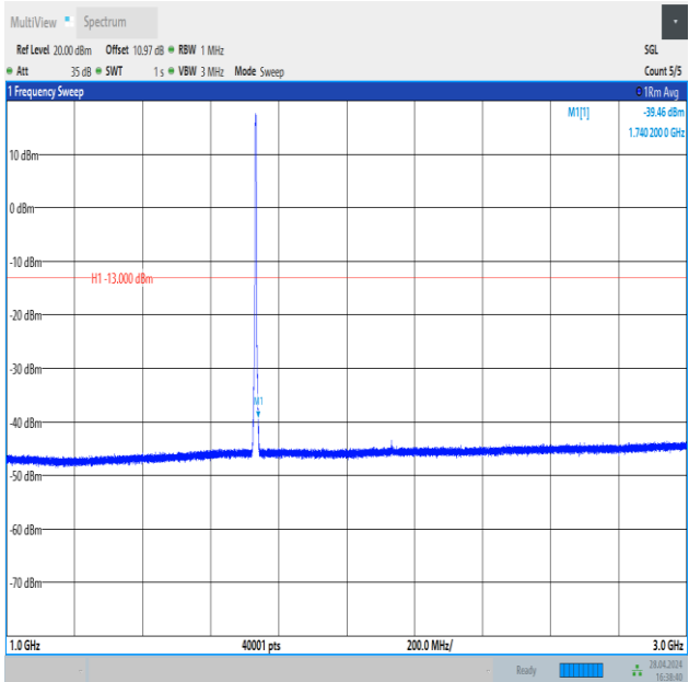
Band4_3MHz_16QAM_20175_15RB#0_1000~3000_1000~3000
