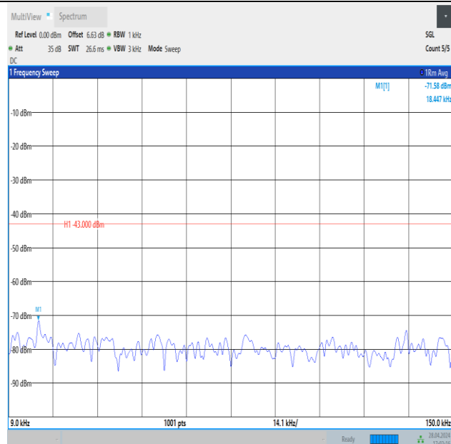
Band4_5MHz_16QAM_20175_1RB#0_0.009~0.15_0.009~0.15
