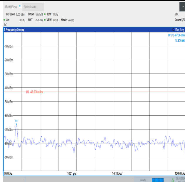
Band4_20MHz_QPSK_20050_100RB#0_0.009~0.15_0.009~0.15
