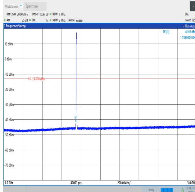
Band4_3MHz_16QAM_20385_15RB#0_1000~3000_1000~3000
