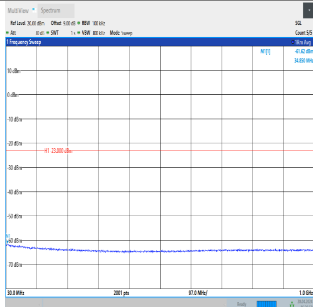
Band4_3MHz_16QAM_20175_1RB#14_30~1000_30~1000
