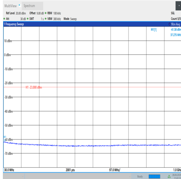
Band4_5MHz_16QAM_20175_1RB#0_30~1000_30~1000
