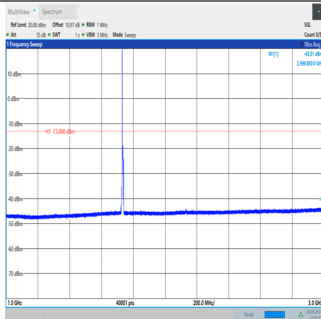
Band4_5MHz_QPSK_20175_1RB#0_1000~3000_1000~3000
