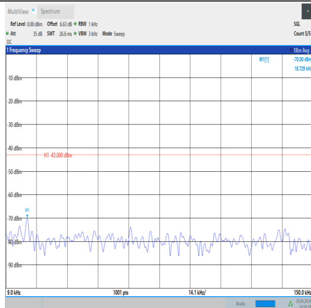
Band4_5MHz_16QAM_19975_1RB#24_0.009~0.15_0.009~0.15
