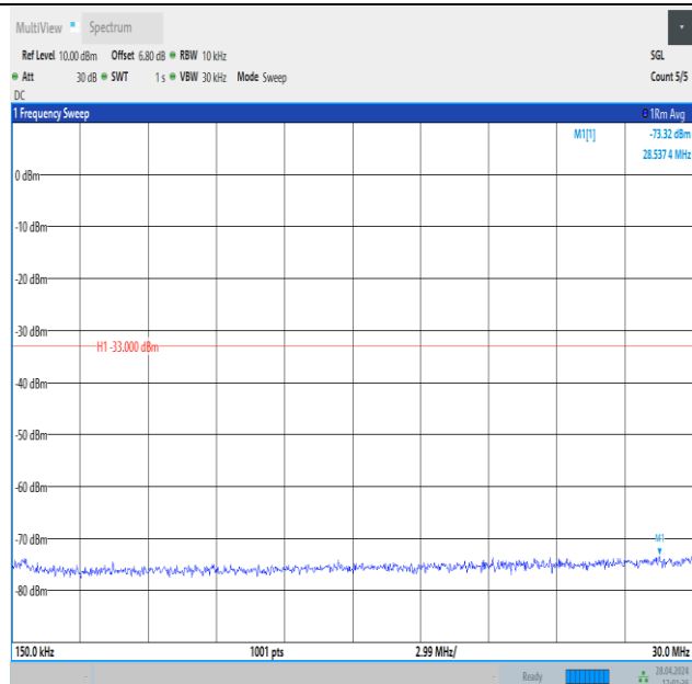
Band4_5MHz_QPSK_20175_1RB#0_0.15~30_0.15~30
