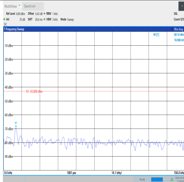
Band4_5MHz_QPSK_20175_25RB#0_0.009~0.15_0.009~0.15
