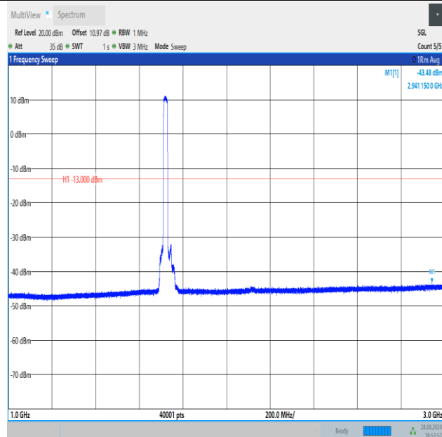
Band4_20MHz_QPSK_20050_100RB#0_1000~3000_1000~3000
