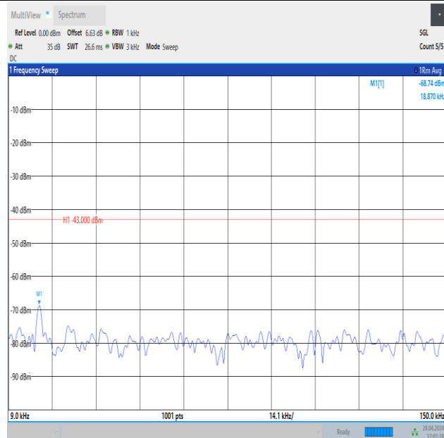
Band4_5MHz_QPSK_20175_1RB#0_0.009~0.15_0.009~0.15
