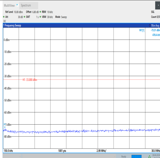
Band4_20MHz_QPSK_20050_100RB#0_0.15~30_0.15~30
