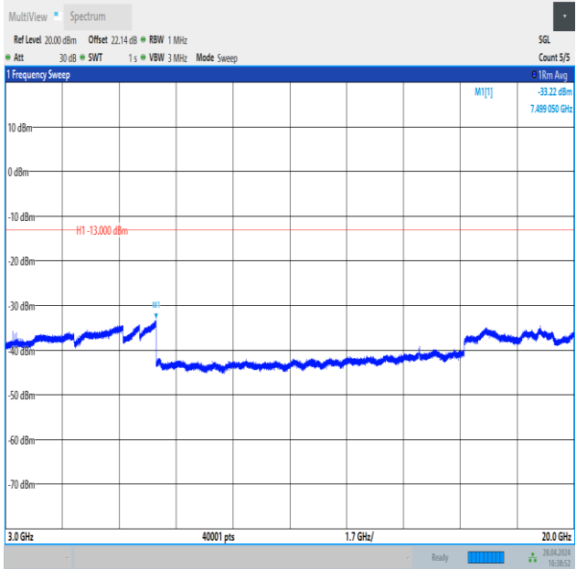
Band4_3MHz_16QAM_20175_15RB#0_3000~20000_3000~20000
