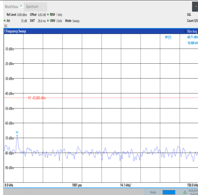
Band4_3MHz_16QAM_20385_1RB#14_0.009~0.15_0.009~0.15
