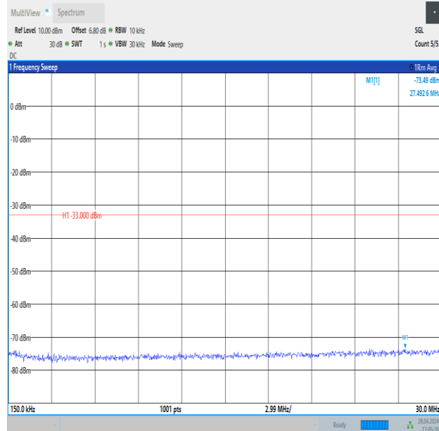
Band4_5MHz_16QAM_20175_25RB#0_0.15~30_0.15~30
