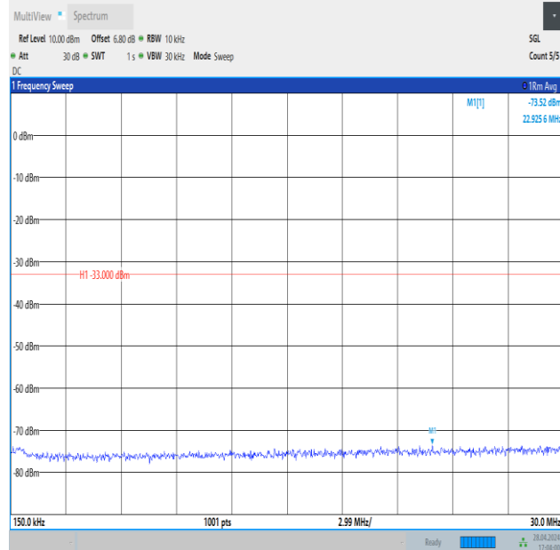
Band4_5MHz_16QAM_20175_1RB#24_0.15~30_0.15~30
