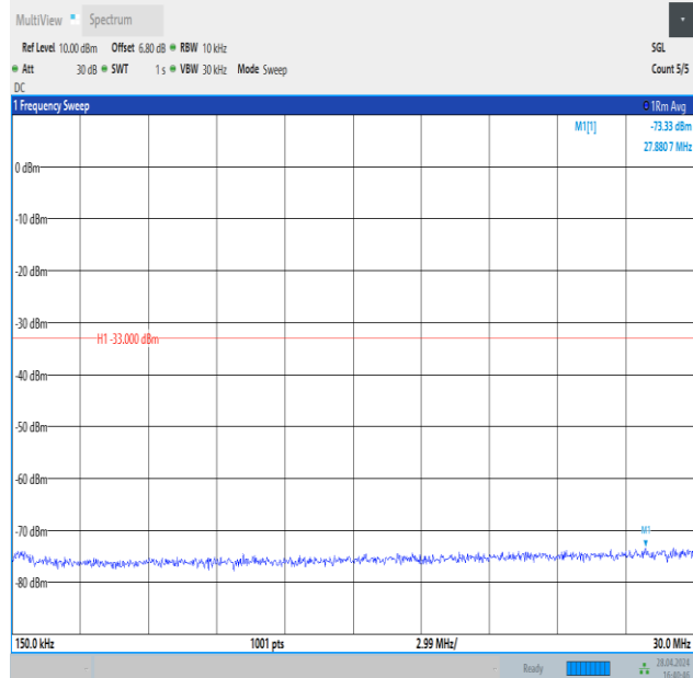
Band4_3MHz_QPSK_20385_1RB#14_0.15~30_0.15~30
