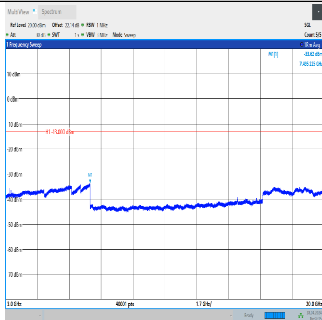
Band4_3MHz_16QAM_20175_1RB#14_3000~20000_3000~20000
