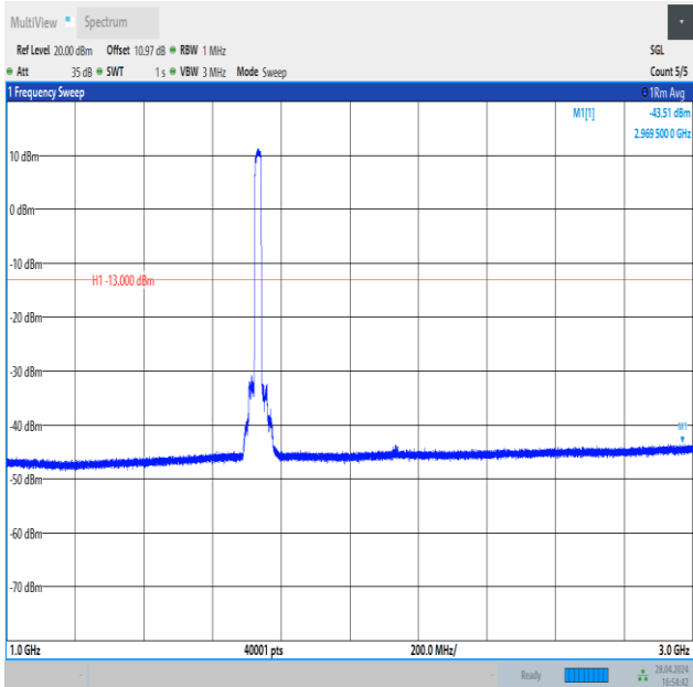
Band4_20MHz_QPSK_20175_100RB#0_1000~3000_1000~3000
