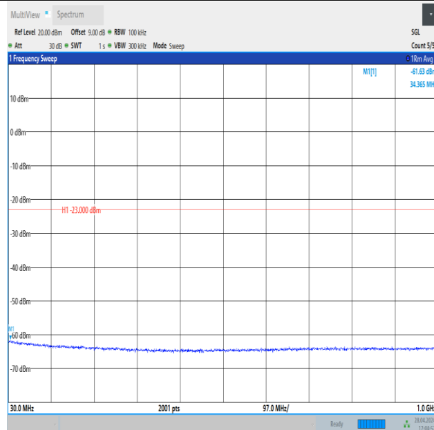
Band4_5MHz_QPSK_20175_25RB#0_30~1000_30~1000
