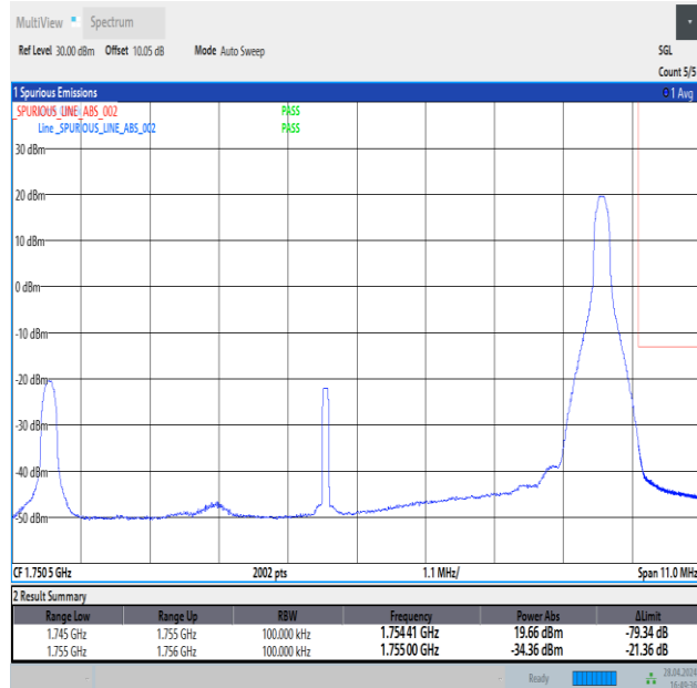
Band4_10MHz_QPSK_20350_1RB#49
