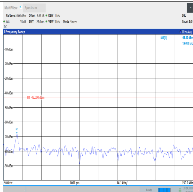
Band4_3MHz_QPSK_19965_1RB#14_0.009~0.15_0.009~0.15
