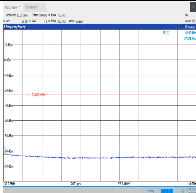
Band4_3MHz_QPSK_19965_15RB#0_30~1000_30~1000
