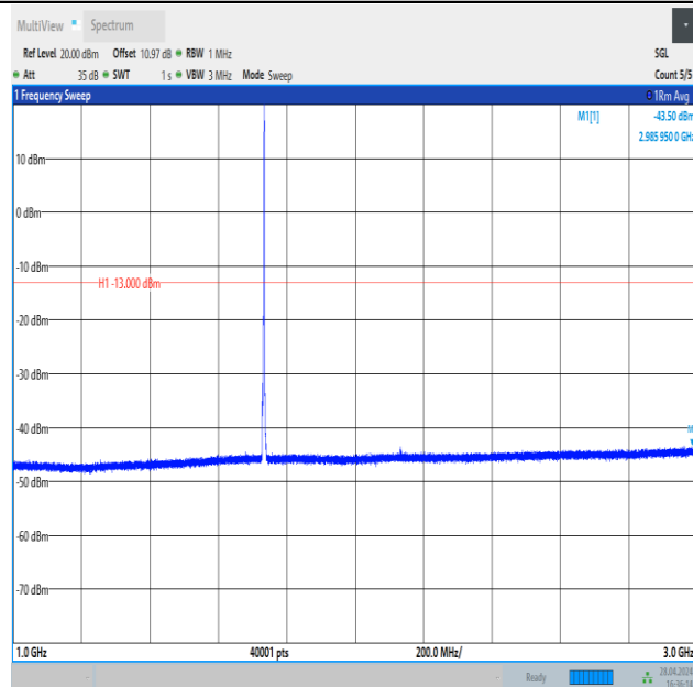
Band4_3MHz_QPSK_20175_1RB#14_1000~3000_1000~3000
