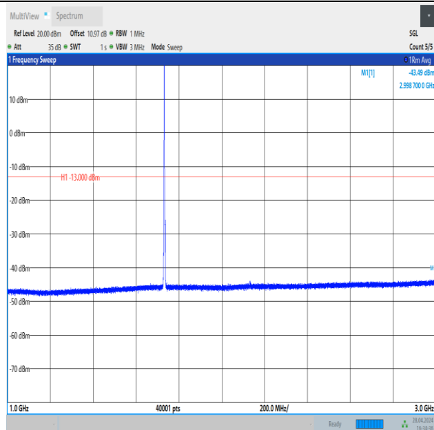
Band4_3MHz_QPSK_20175_1RB#0_1000~3000_1000~3000
