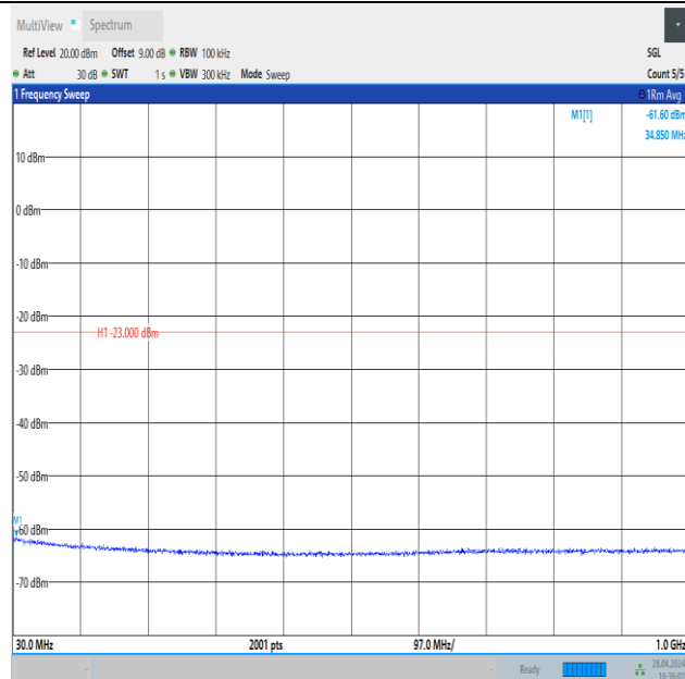
Band4_3MHz_QPSK_20175_1RB#14_30~1000_30~1000
