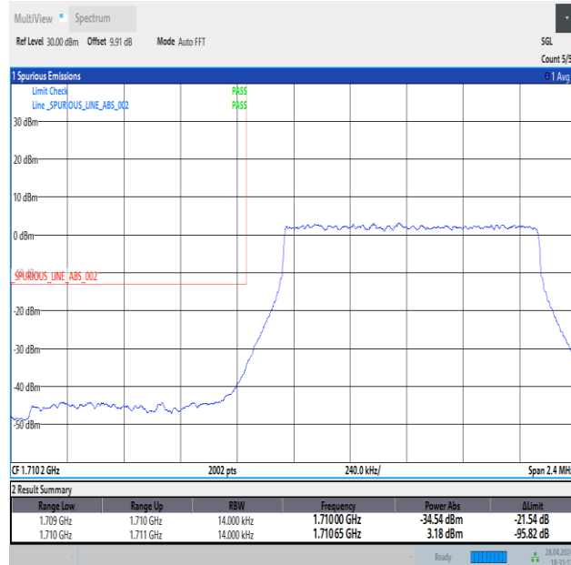
Band4_1.4MHz_QPSK_19957_6RB#0
