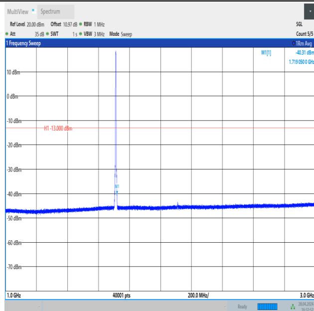
Band4_3MHz_QPSK_19965_15RB#0_1000~3000_1000~3000
