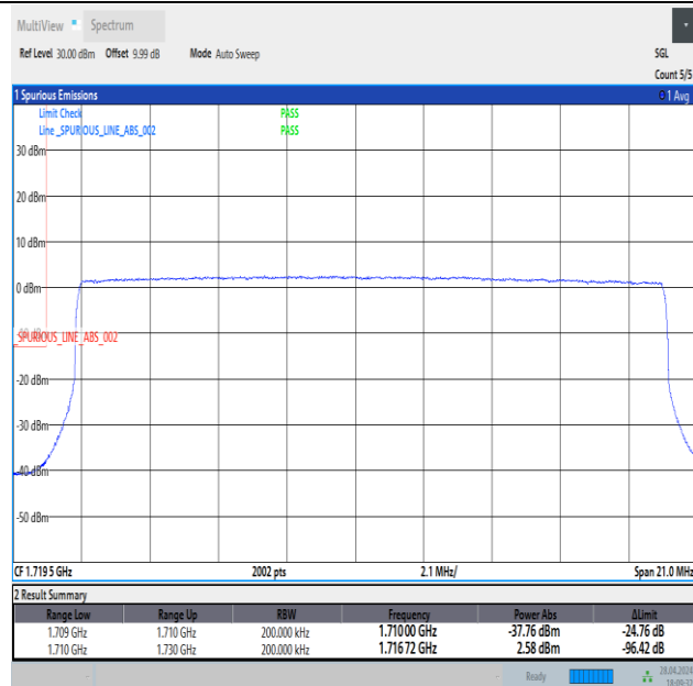
Band4_20MHz_QPSK_20050_100RB#0
