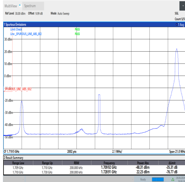
Band4_20MHz_QPSK_20050_1RB#99
