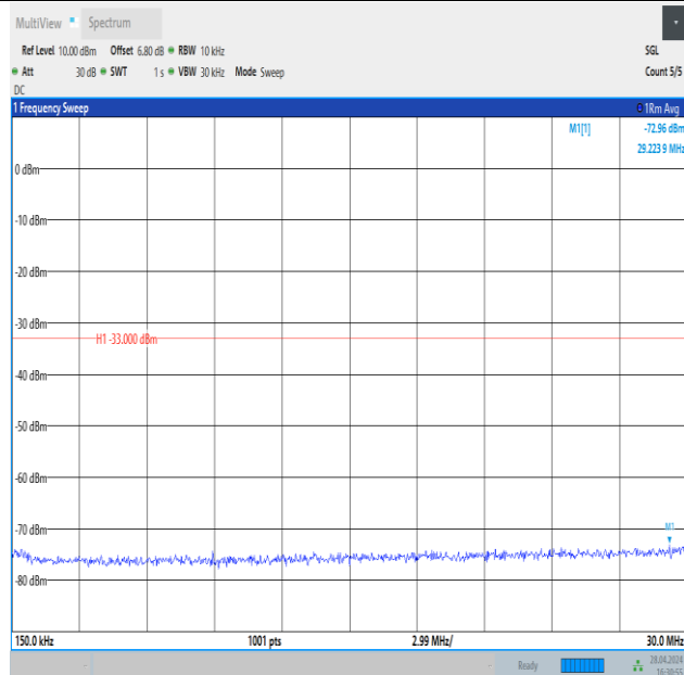
Band4_3MHz_QPSK_19965_1RB#14_0.15~30_0.15~30
