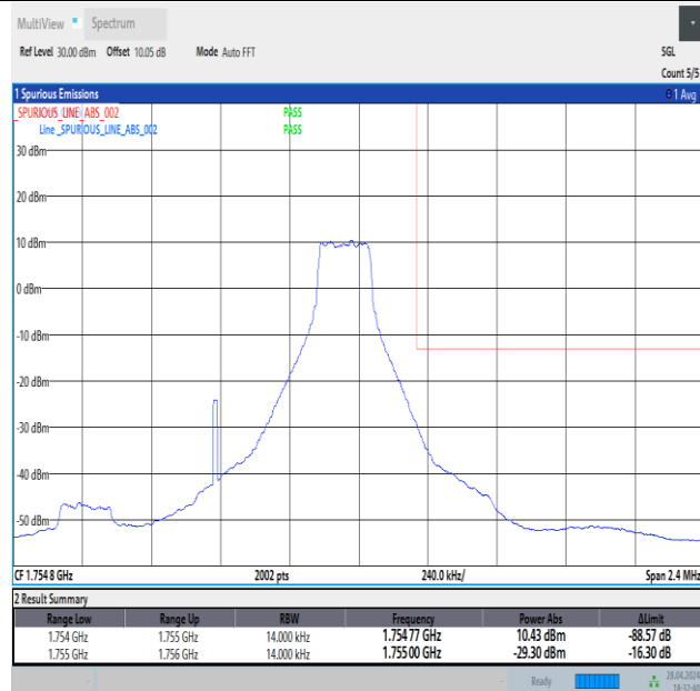
Band4_1.4MHz_16QAM_20393_1RB#5
