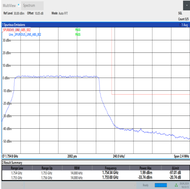
Band4_1.4MHz_16QAM_20393_6RB#0
