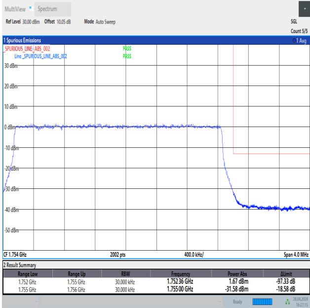
Band4_3MHz_16QAM_20385_15RB#0
