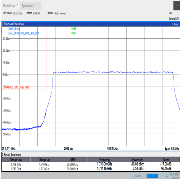
Band4_3MHz_QPSK_19965_15RB#0
