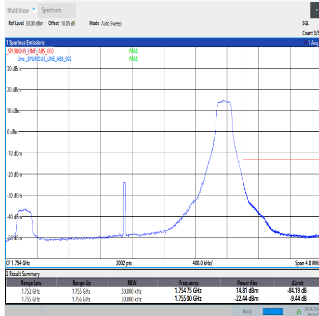
Band4_3MHz_QPSK_20385_1RB#14
