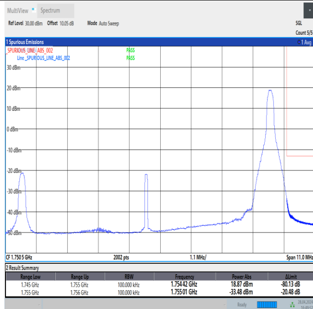
Band4_10MHz_16QAM_20350_1RB#49
