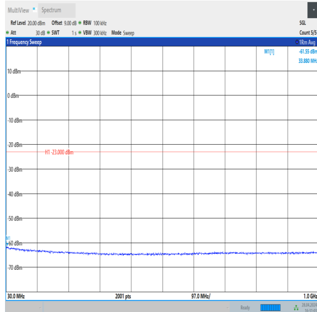
Band4_3MHz_QPSK_19965_1RB#14_30~1000_30~1000
