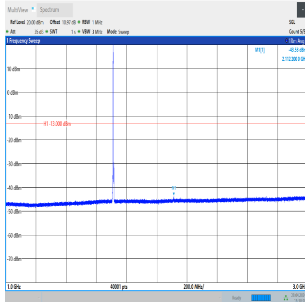
Band4_3MHz_16QAM_19965_1RB#0_1000~3000_1000~3000
