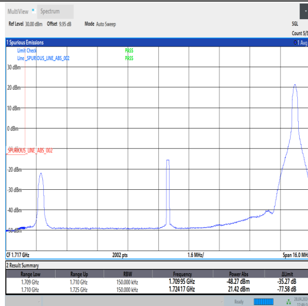
Band4_15MHz_QPSK_20025_1RB#74
