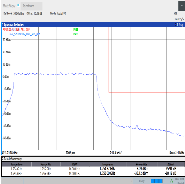
Band4_1.4MHz_QPSK_20393_6RB#0
