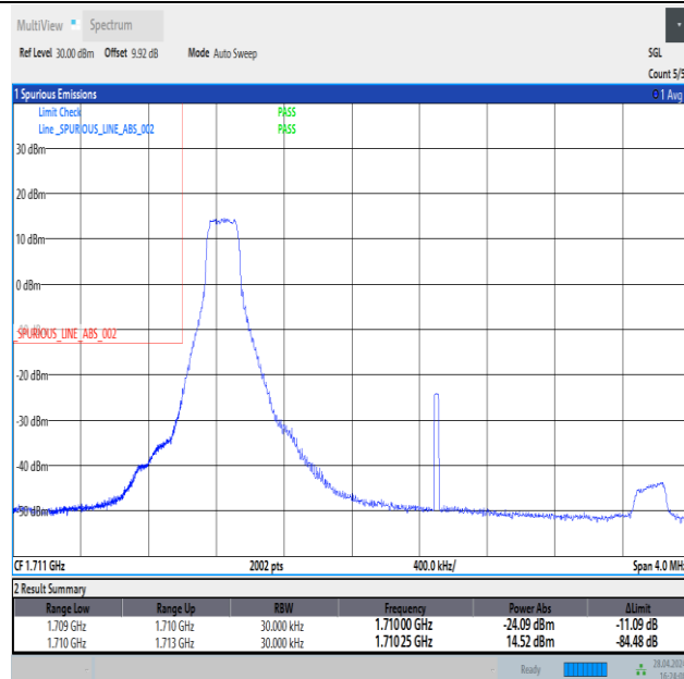
Band4_3MHz_QPSK_19965_1RB#0
