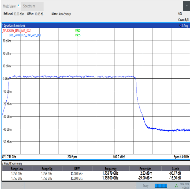
Band4_3MHz_QPSK_20385_15RB#0
