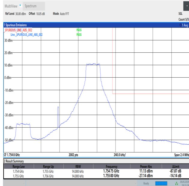
Band4_1.4MHz_QPSK_20393_1RB#5
