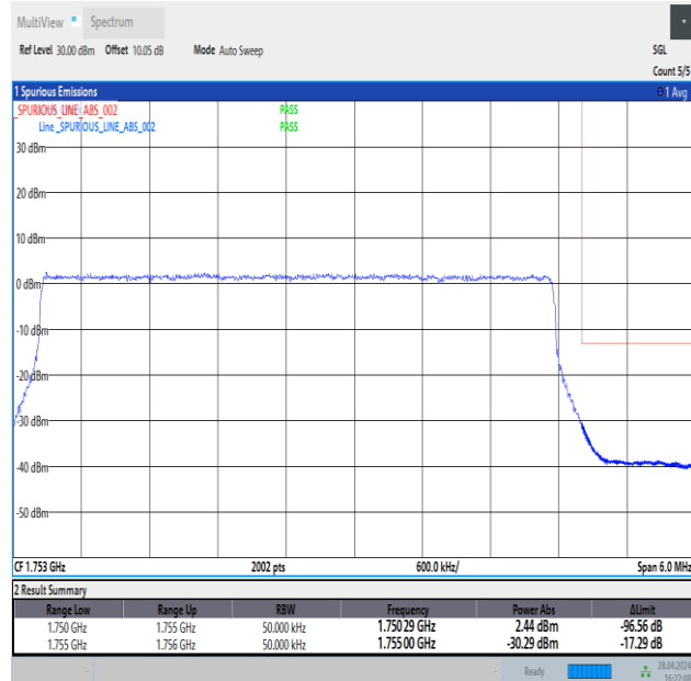
Band4_5MHz_QPSK_20375_25RB#0
