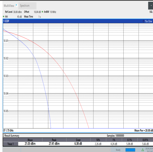
Band4-10MHz-QPSK-20350-50RB#0-PASS
