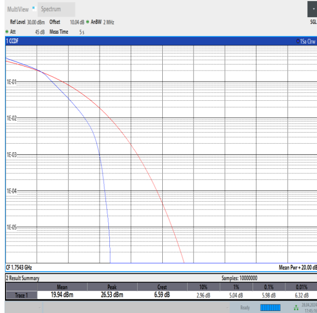
Band4-1.4MHz-16QAM-20393-6RB#0-PASS
