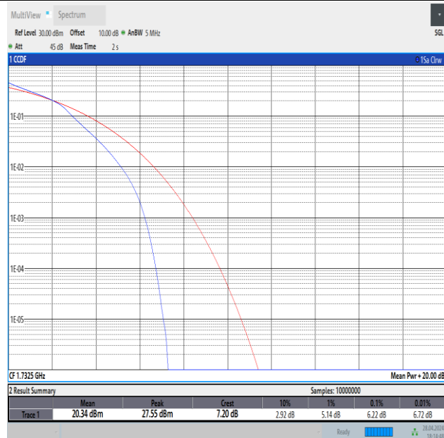
Band4-5MHz-16QAM-20175-25RB#0-PASS
