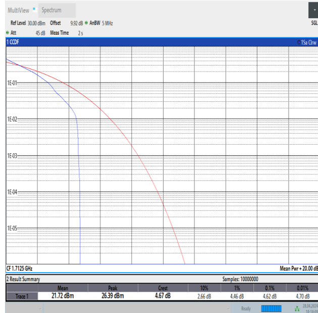
Band4-5MHz-QPSK-19975-1RB#0-PASS
