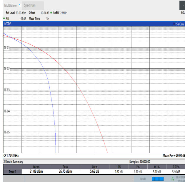
Band4-1.4MHz-QPSK-20393-6RB#0-PASS
