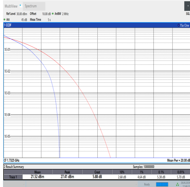
Band4-1.4MHz-QPSK-20175-6RB#0-PASS
