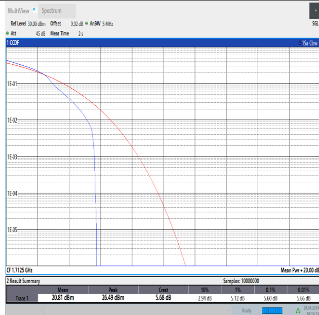
Band4-5MHz-16QAM-19975-1RB#0-PASS
