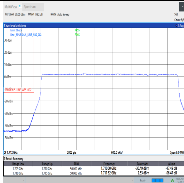
Band4_5MHz_QPSK_19975_25RB#0
