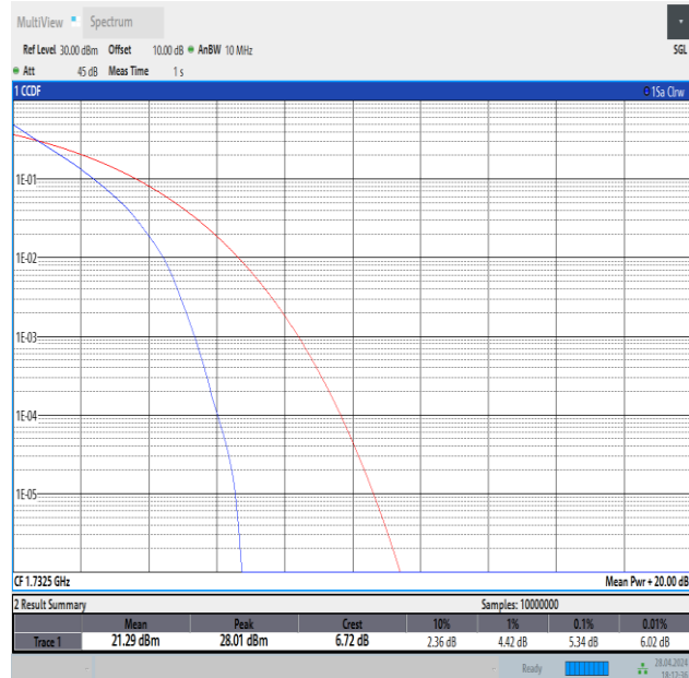
Band4-10MHz-QPSK-20175-50RB#0-PASS
