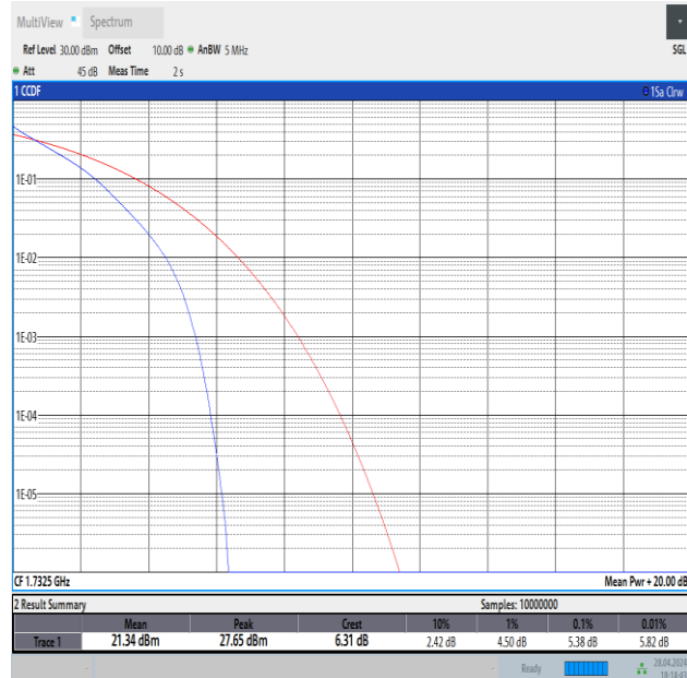
Band4-5MHz-QPSK-20175-25RB#0-PASS
