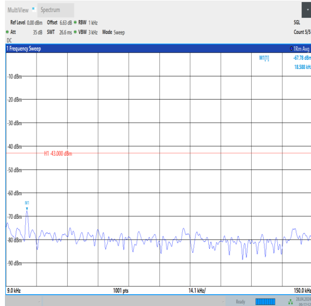
Band2_3MHz_16QAM_18615_1RB#14_0.009~0.15_0.009~0.15
