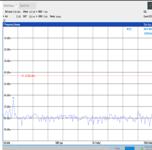
Band2_5MHz_16QAM_19175_25RB#0_0.009~0.15_0.009~0.15
