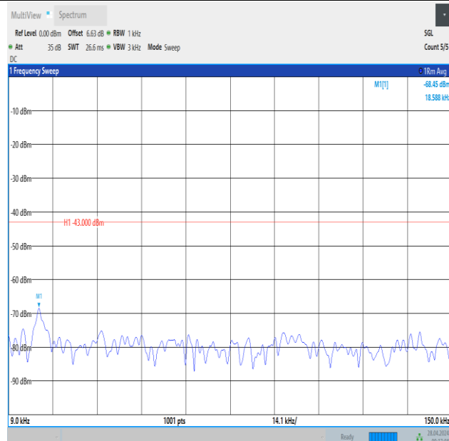
Band2_3MHz_QPSK_18615_1RB#14_0.009~0.15_0.009~0.15
