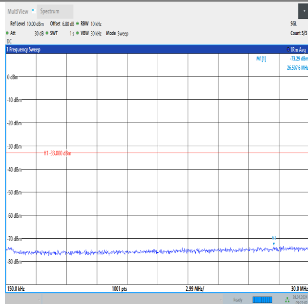
Band2_3MHz_QPSK_18900_1RB#14_0.15~30_0.15~30
