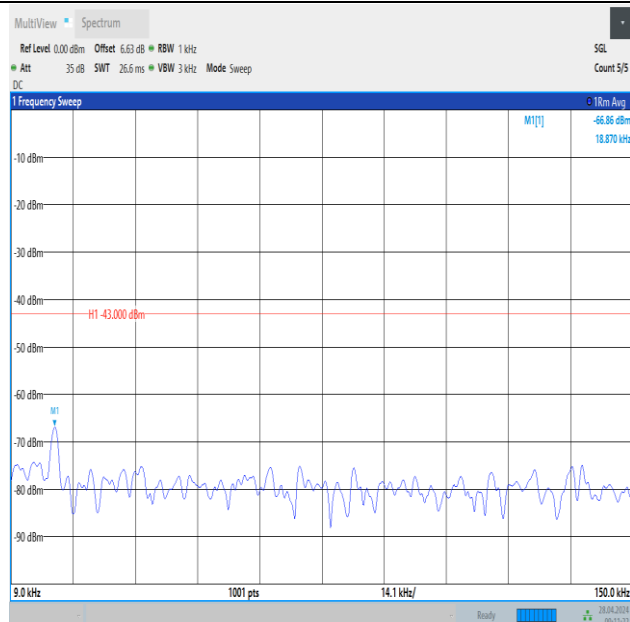
Band2_5MHz_16QAM_19175_1RB#0_0.009~0.15_0.009~0.15
