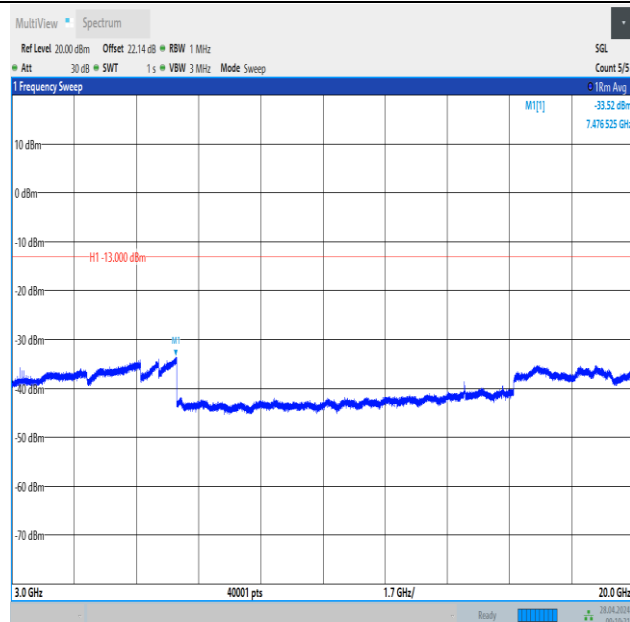
Band2_5MHz_16QAM_18900_25RB#0_3000~20000_3000~20000
