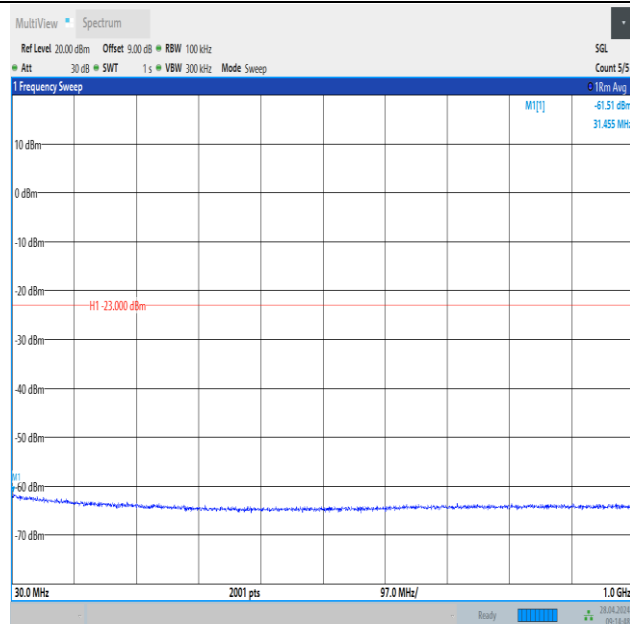
Band2_5MHz_16QAM_19175_25RB#0_30~1000_30~1000
