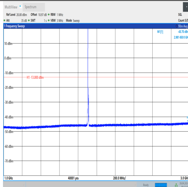
Band2_5MHz_QPSK_19175_1RB#0_1000~3000_1000~3000
