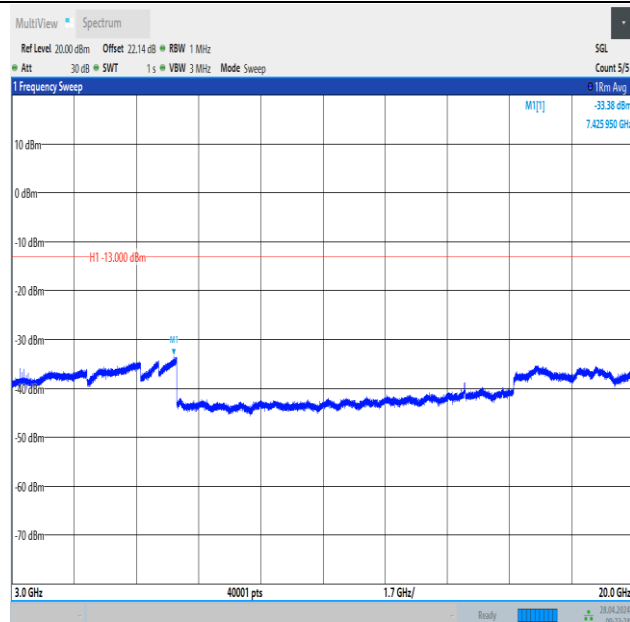
Band2_3MHz_16QAM_18900_1RB#14_3000~20000_3000~20000
