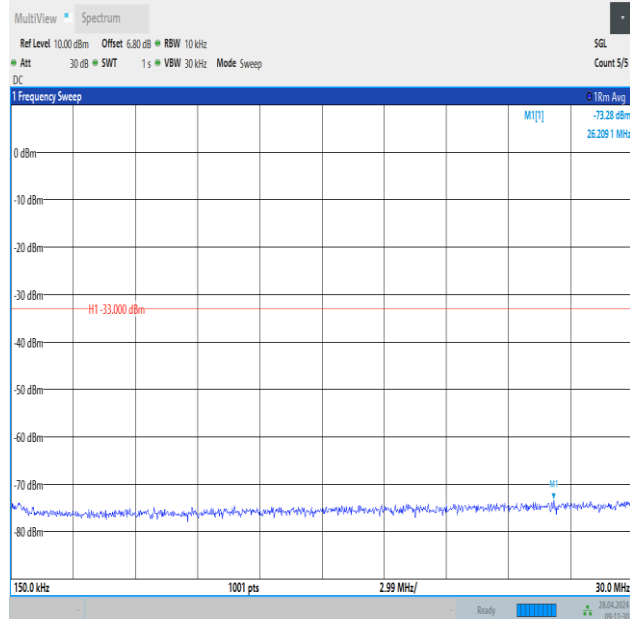
Band2_5MHz_16QAM_19175_1RB#0_0.15~30_0.15~30
