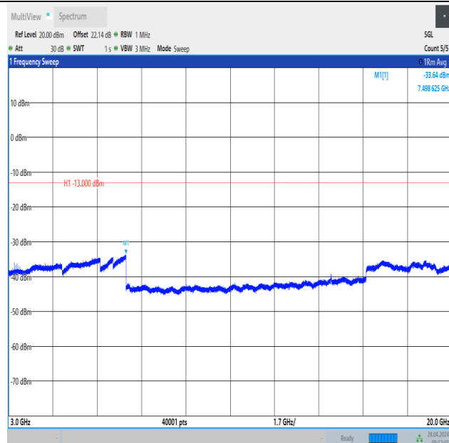
Band2_5MHz_16QAM_19175_1RB#0_3000~20000_3000~20000
