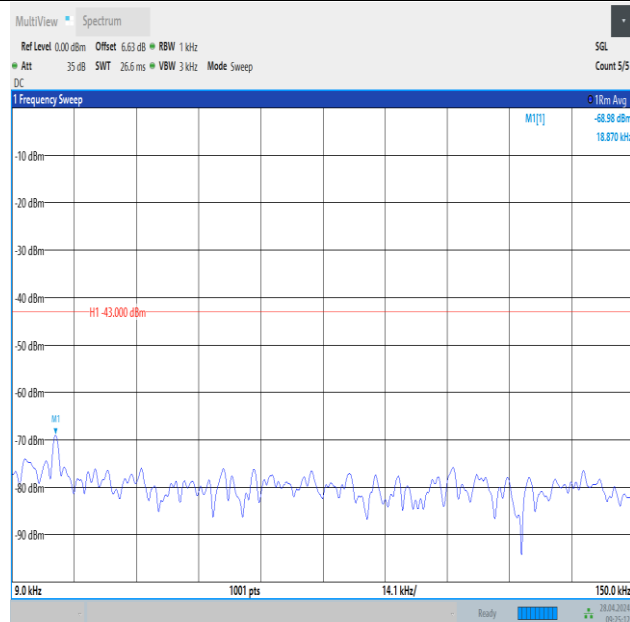
Band2_3MHz_QPSK_19185_1RB#0_0.009~0.15_0.009~0.15
