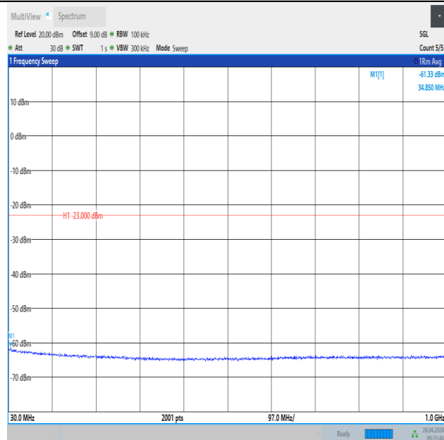
Band2_3MHz_QPSK_18900_15RB#0_30~1000_30~1000
