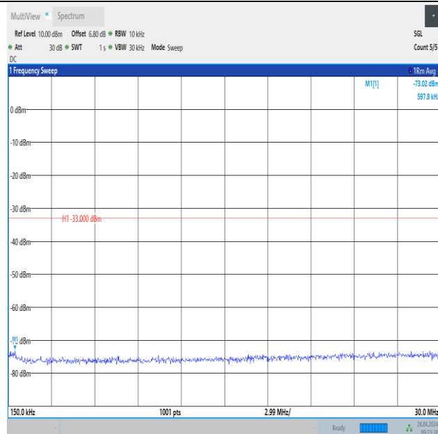
Band2_3MHz_QPSK_18900_15RB#0_0.15~30_0.15~30
