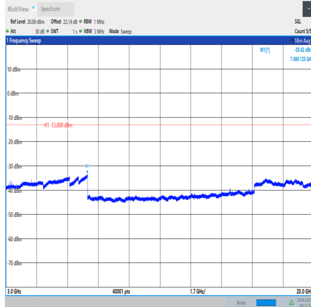
Band2_5MHz_QPSK_19175_1RB#0_3000~20000_3000~20000
