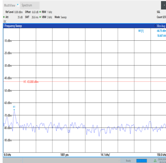
Band2_3MHz_16QAM_18615_1RB#0_0.009~0.15_0.009~0.15
