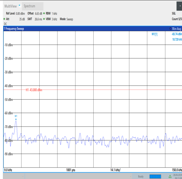
Band2_5MHz_QPSK_19175_1RB#24_0.009~0.15_0.009~0.15
