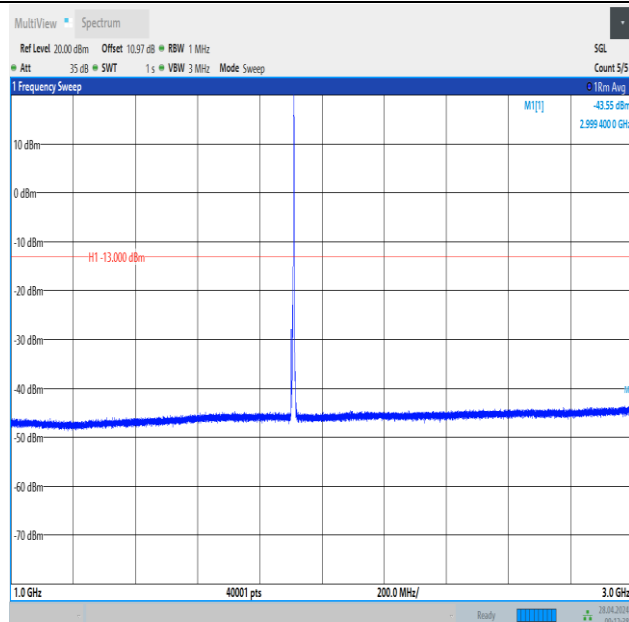
Band2_5MHz_QPSK_19175_1RB#24_1000~3000_1000~3000
