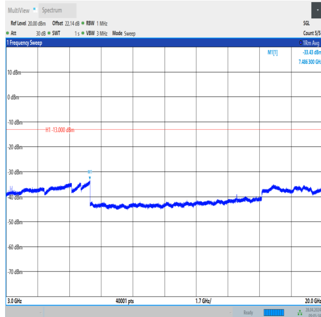
Band2_5MHz_16QAM_18625_25RB#0_3000~20000_3000~20000
