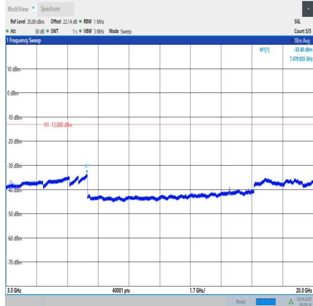
Band2_5MHz_QPSK_18900_25RB#0_3000~20000_3000~20000
