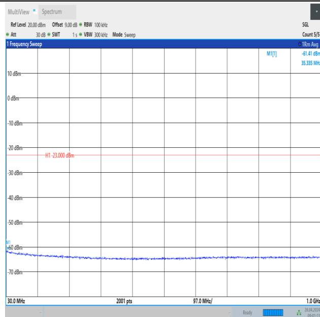
Band2_5MHz_QPSK_18625_1RB#0_30~1000_30~1000
