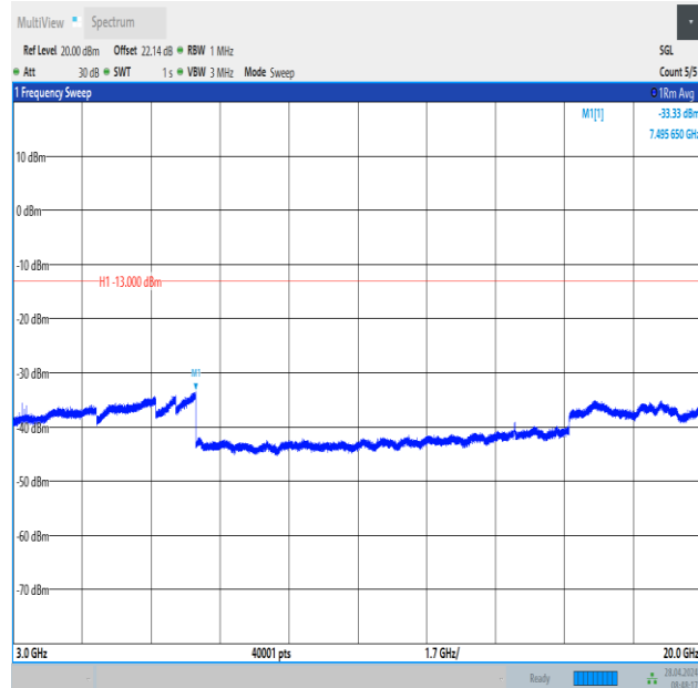
Band2_15MHz_QPSK_19125_75RB#0_3000~20000_3000~20000
