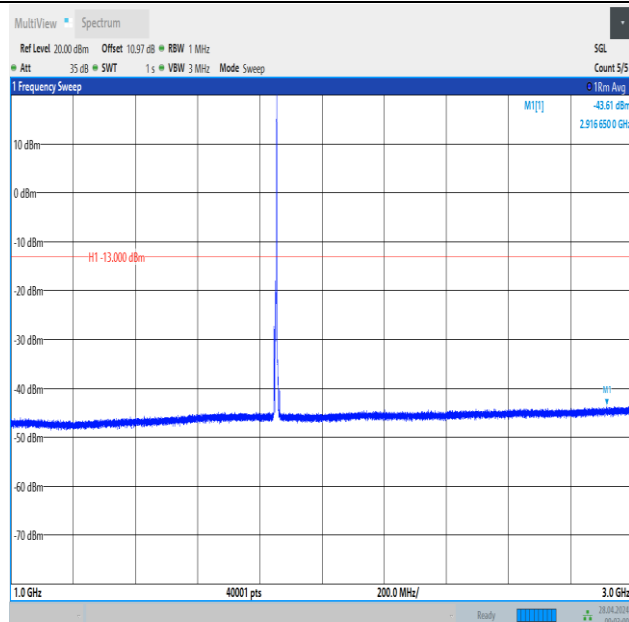
Band2_5MHz_QPSK_18625_1RB#24_1000~3000_1000~3000
