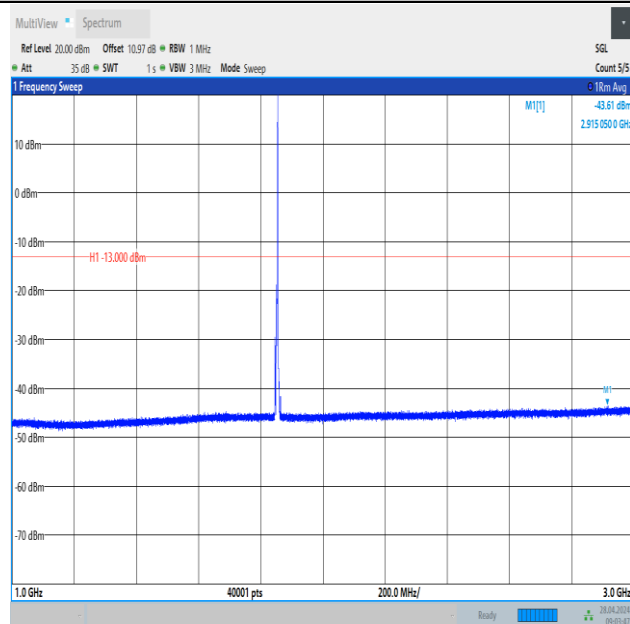
Band2_5MHz_16QAM_18625_1RB#24_1000~3000_1000~3000
