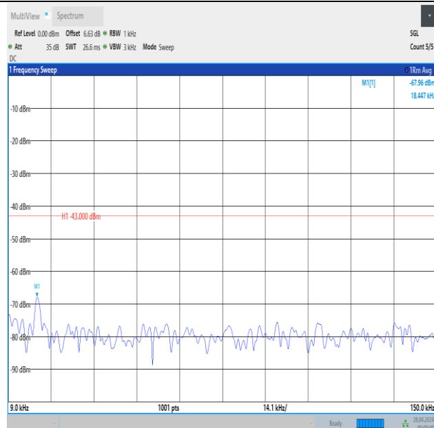
Band2_15MHz_16QAM_19125_1RB#74_0.009~0.15_0.009~0.15
