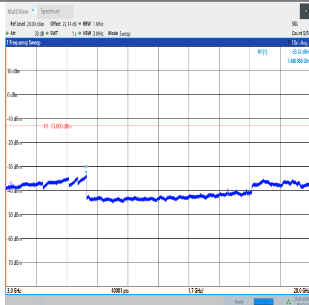
Band2_5MHz_16QAM_18625_1RB#0_3000~20000_3000~20000
