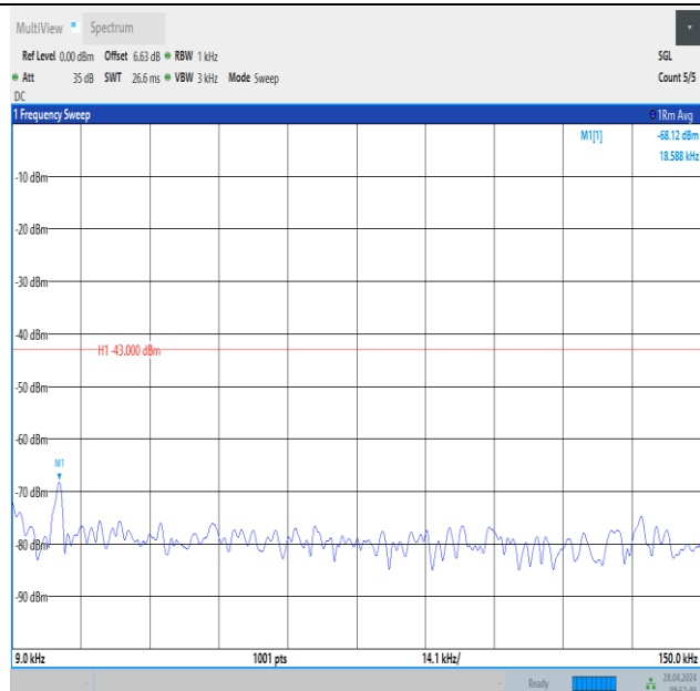
Band2_15MHz_16QAM_18675_1RB#0_0.009~0.15_0.009~0.15
