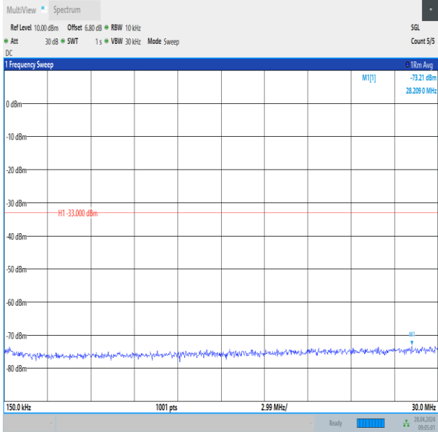
Band2_5MHz_16QAM_18625_25RB#0_0.15~30_0.15~30
