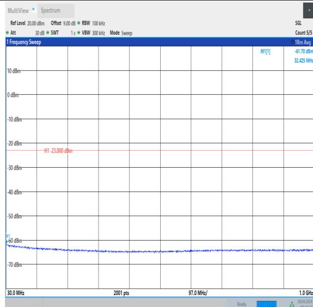
Band2_15MHz_QPSK_19125_1RB#74_30~1000_30~1000
