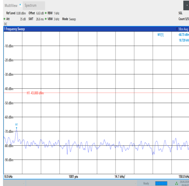
Band2_5MHz_QPSK_18625_25RB#0_0.009~0.15_0.009~0.15
