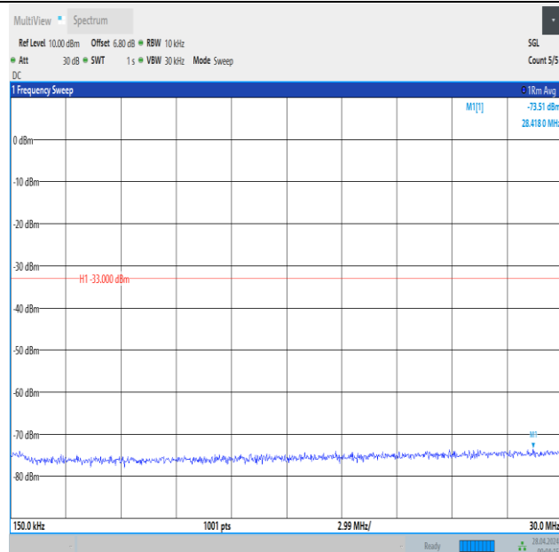
Band2_5MHz_QPSK_18625_25RB#0_0.15~30_0.15~30
