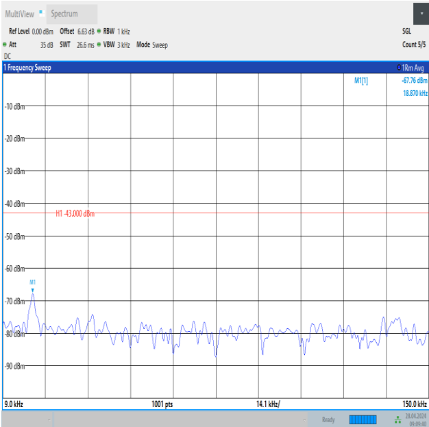
Band2_5MHz_16QAM_18900_25RB#0_0.009~0.15_0.009~0.15
