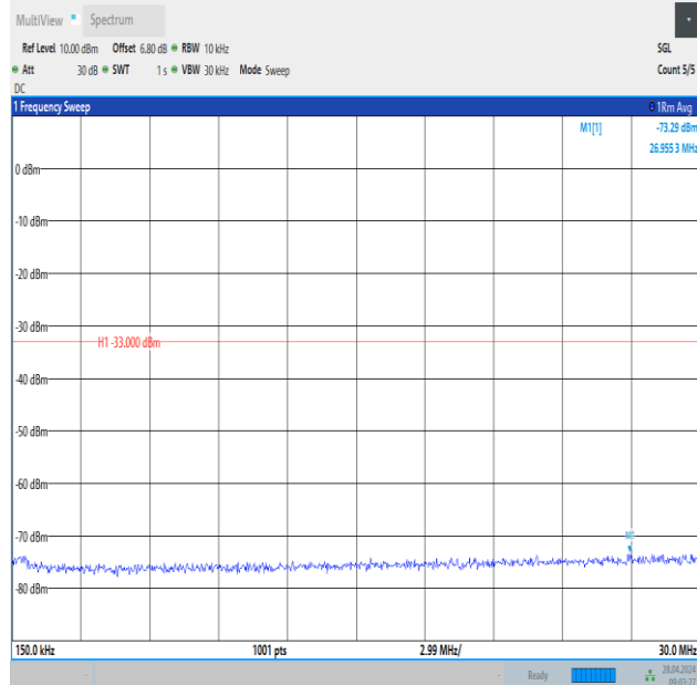
Band2_5MHz_16QAM_18625_1RB#24_0.15~30_0.15~30
