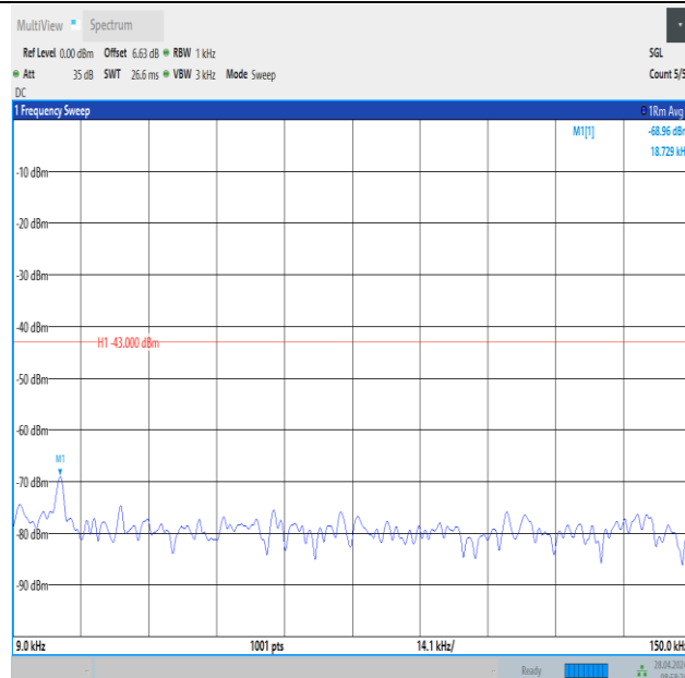
Band2_15MHz_16QAM_19125_1RB#0_0.009~0.15_0.009~0.15
