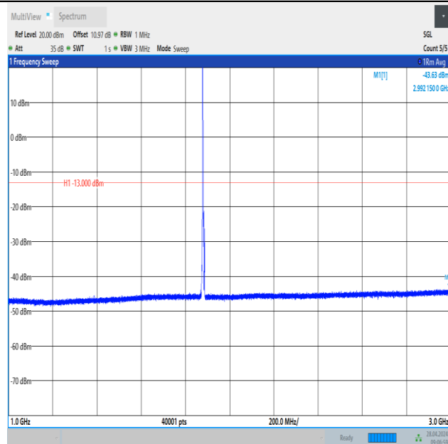
Band2_5MHz_16QAM_18900_1RB#0_1000~3000_1000~3000
