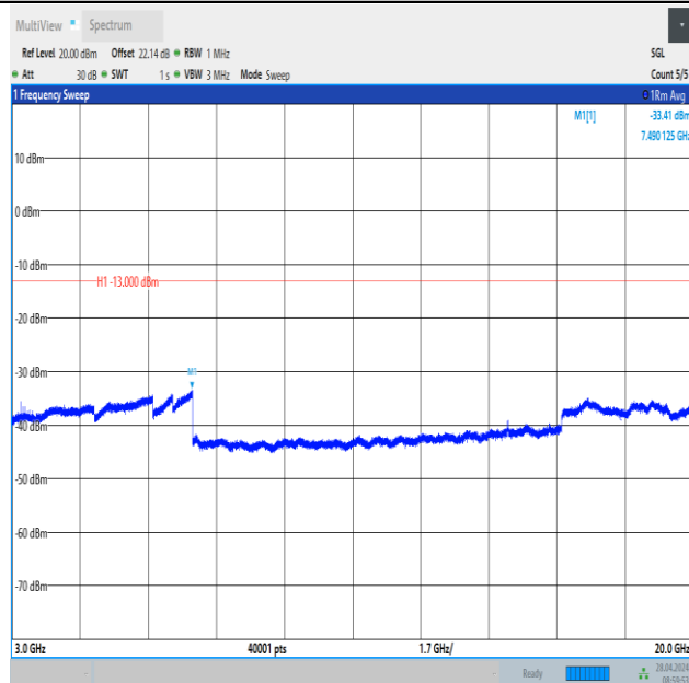
Band2_15MHz_QPSK_19125_1RB#74_3000~20000_3000~20000
