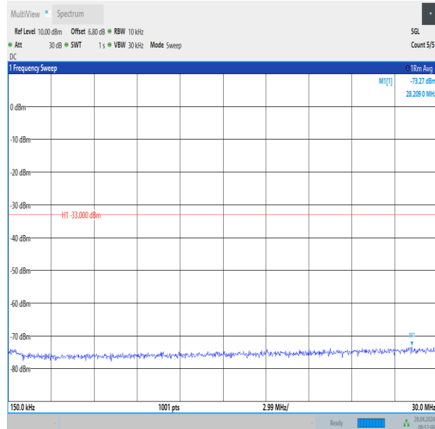
Band2_15MHz_QPSK_18675_1RB#0_0.15~30_0.15~30
