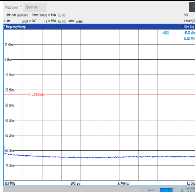
Band2_5MHz_QPSK_18625_25RB#0_30~1000_30~1000
