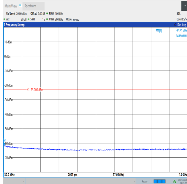
Band2_5MHz_16QAM_18625_25RB#0_30~1000_30~1000
