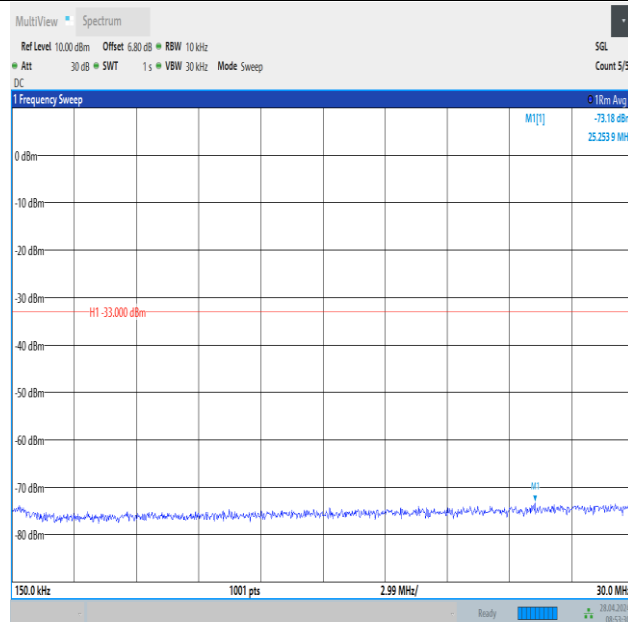
Band2_15MHz_16QAM_18675_1RB#74_0.15~30_0.15~30
