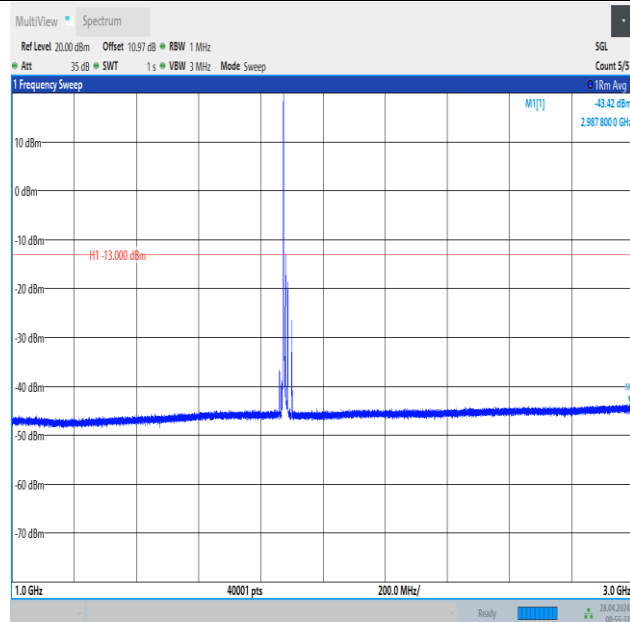
Band2_15MHz_16QAM_18900_1RB#0_1000~3000_1000~3000
