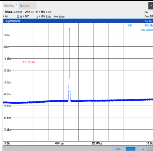
Band2_5MHz_16QAM_18900_25RB#0_1000~3000_1000~3000
