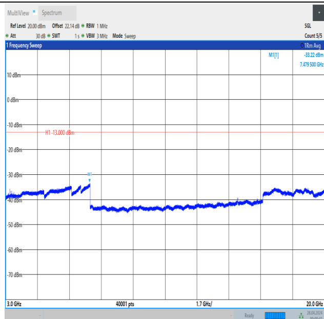
Band2_15MHz_16QAM_19125_1RB#74_3000~20000_3000~20000
