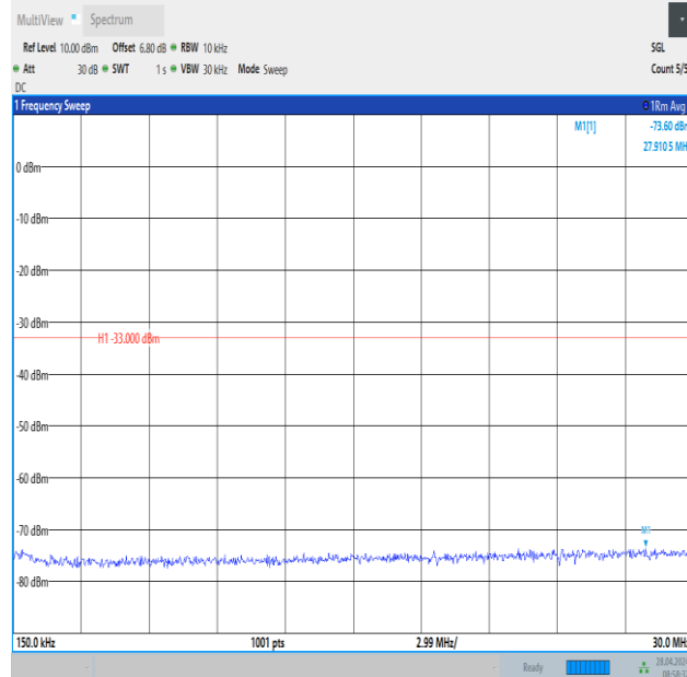
Band2_15MHz_16QAM_19125_1RB#0_0.15~30_0.15~30
