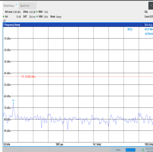
Band2_15MHz_16QAM_18900_1RB#0_0.009~0.15_0.009~0.15
