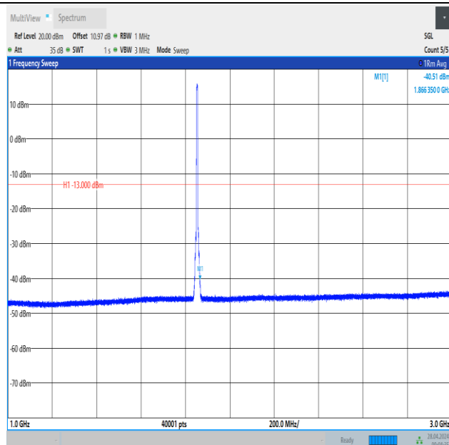
Band2_5MHz_QPSK_18625_25RB#0_1000~3000_1000~3000
