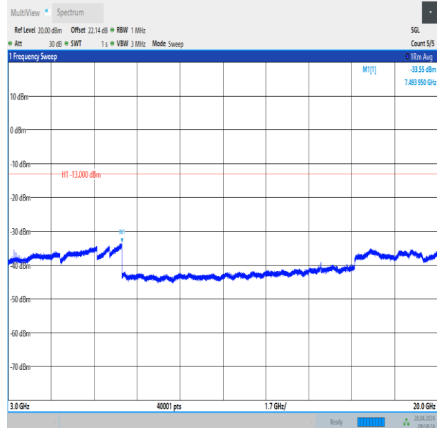
Band2_15MHz_QPSK_19125_1RB#0_3000~20000_3000~20000
