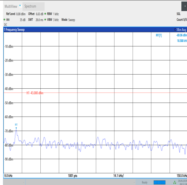
Band2_15MHz_QPSK_18675_1RB#74_0.009~0.15_0.009~0.15
