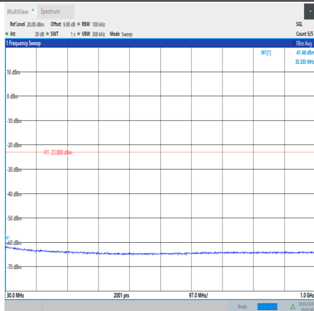
Band2_5MHz_QPSK_18625_1RB#24_30~1000_30~1000
