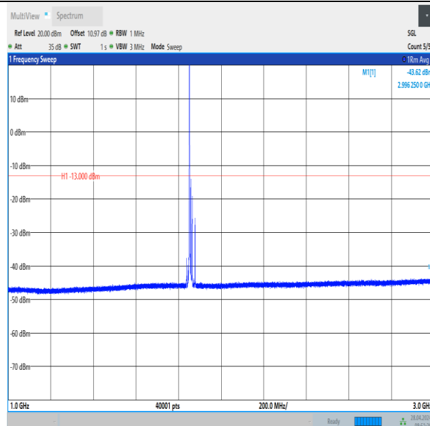
Band2_15MHz_QPSK_18675_1RB#0_1000~3000_1000~3000
