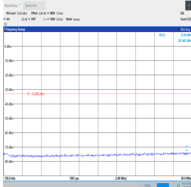
Band2_15MHz_16QAM_19125_1RB#74_0.15~30_0.15~30
