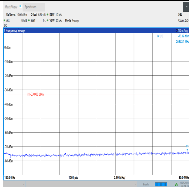
Band2_15MHz_QPSK_19125_1RB#74_0.15~30_0.15~30
