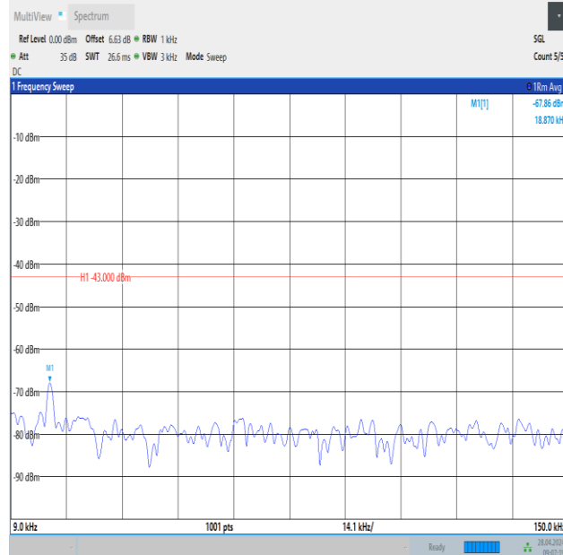
Band2_5MHz_QPSK_18900_1RB#24_0.009~0.15_0.009~0.15
