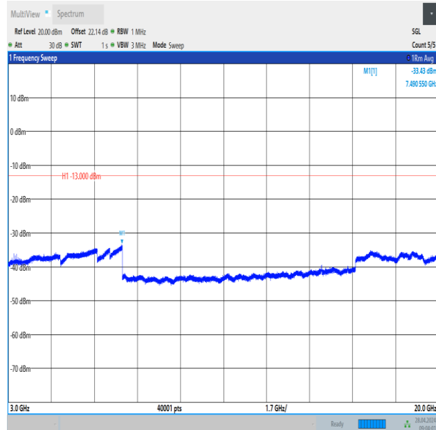
Band2_5MHz_16QAM_18625_1RB#24_3000~20000_3000~20000
