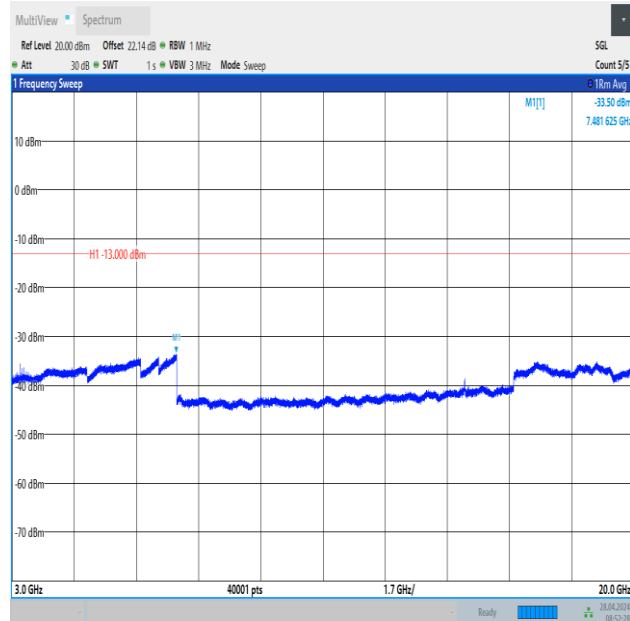
Band2_15MHz_16QAM_18675_1RB#0_3000~20000_3000~20000
