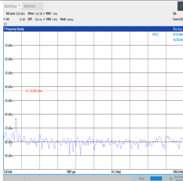
Band2_5MHz_QPSK_18625_1RB#24_0.009~0.15_0.009~0.15
