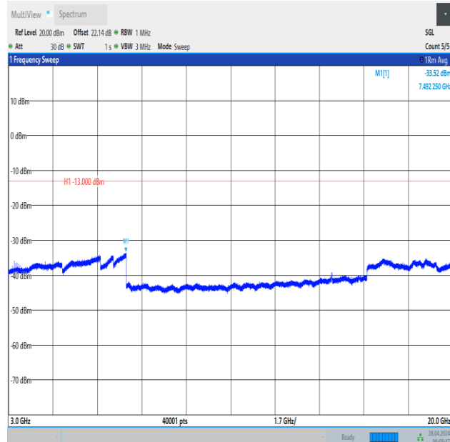
Band2_5MHz_16QAM_18900_1RB#24_3000~20000_3000~20000
