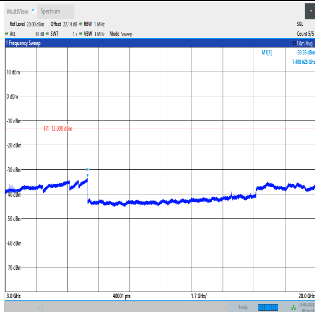
Band2_15MHz_QPSK_18900_1RB#74_3000~20000_3000~20000
