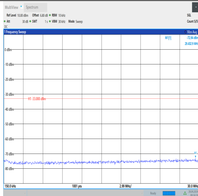
Band2_15MHz_QPSK_18900_1RB#0_0.15~30_0.15~30
