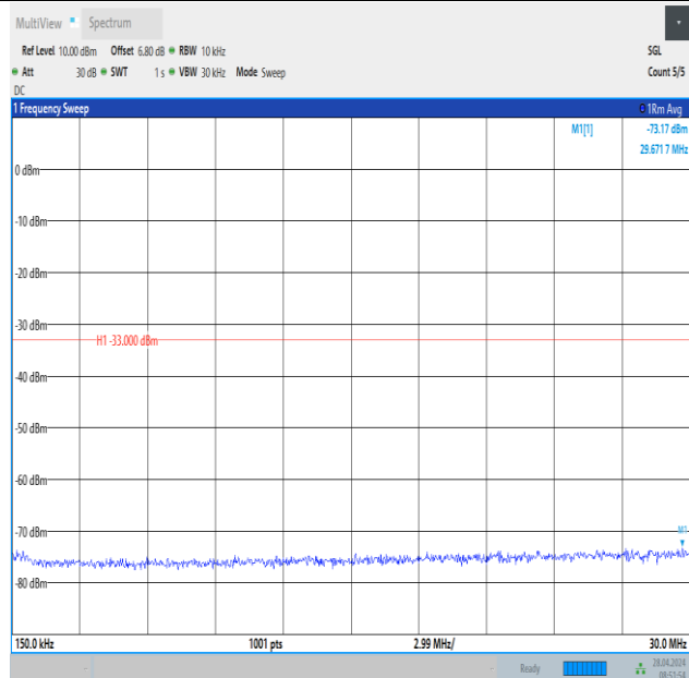
Band2_15MHz_16QAM_18675_1RB#0_0.15~30_0.15~30
