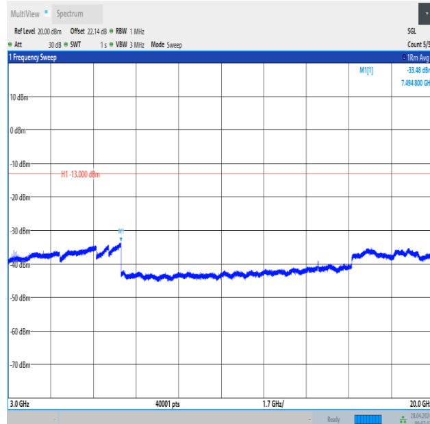
Band2_5MHz_16QAM_18900_1RB#0_3000~20000_3000~20000
