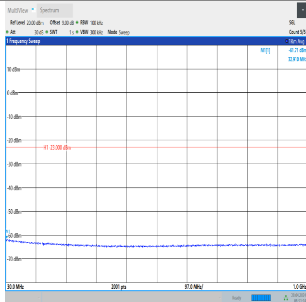
Band2_15MHz_QPSK_18675_1RB#0_30~1000_30~1000
