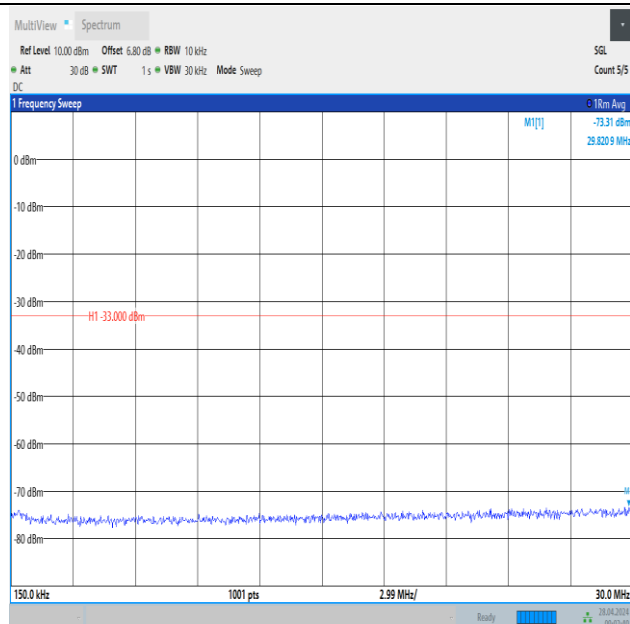
Band2_5MHz_QPSK_18625_1RB#24_0.15~30_0.15~30
