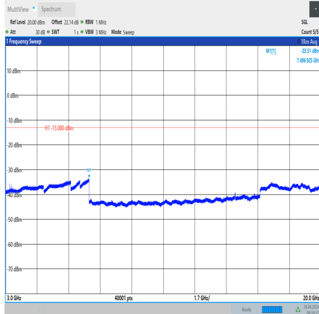
Band2_15MHz_QPSK_18900_1RB#0_3000~20000_3000~20000
