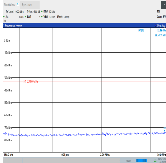
Band2_15MHz_16QAM_18900_1RB#0_0.15~30_0.15~30
