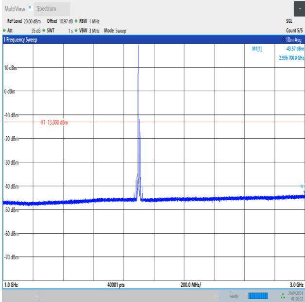
Band2_15MHz_16QAM_19125_1RB#0_1000~3000_1000~3000
