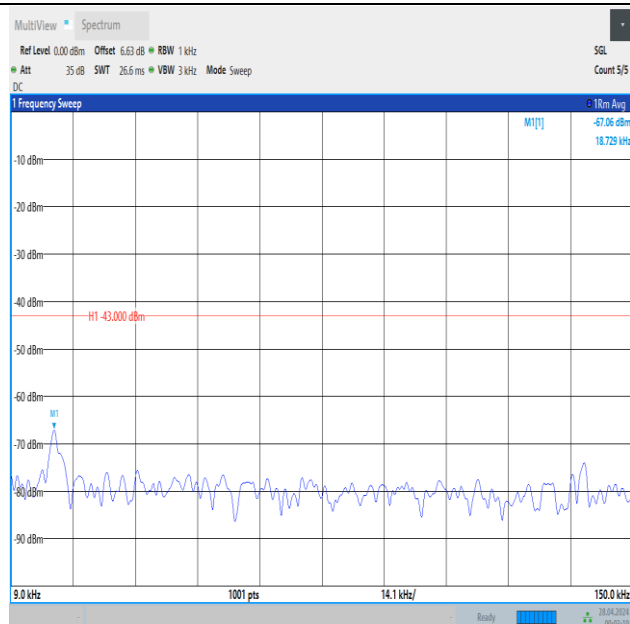
Band2_5MHz_16QAM_18625_1RB#24_0.009~0.15_0.009~0.15
