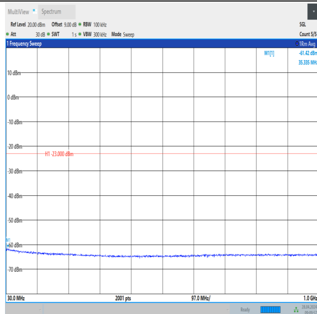
Band2_5MHz_16QAM_18900_25RB#0_30~1000_30~1000
