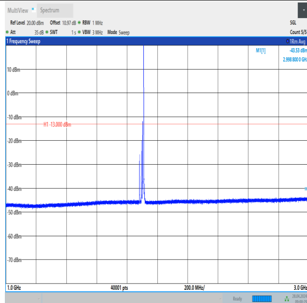
Band2_15MHz_16QAM_19125_1RB#74_1000~3000_1000~3000
