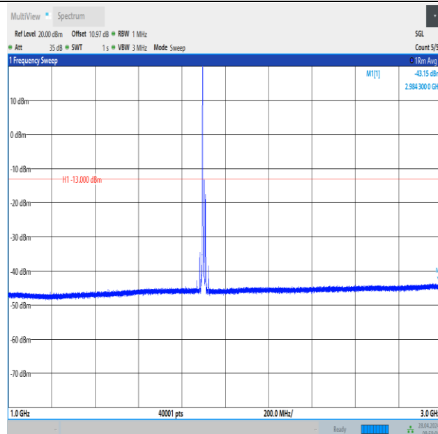
Band2_15MHz_QPSK_19125_1RB#0_1000~3000_1000~3000
