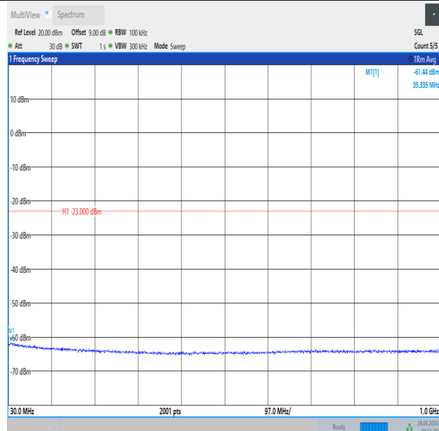
Band2_15MHz_QPSK_18900_1RB#74_30~1000_30~1000
