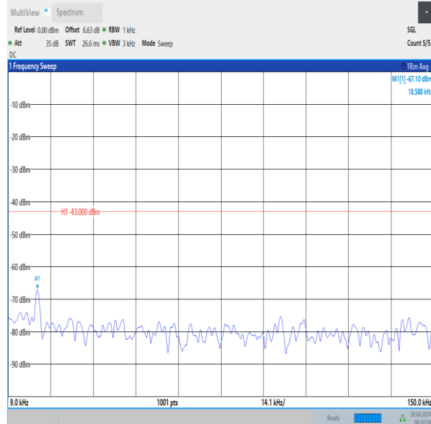
Band2_15MHz_QPSK_18675_1RB#0_0.009~0.15_0.009~0.15
