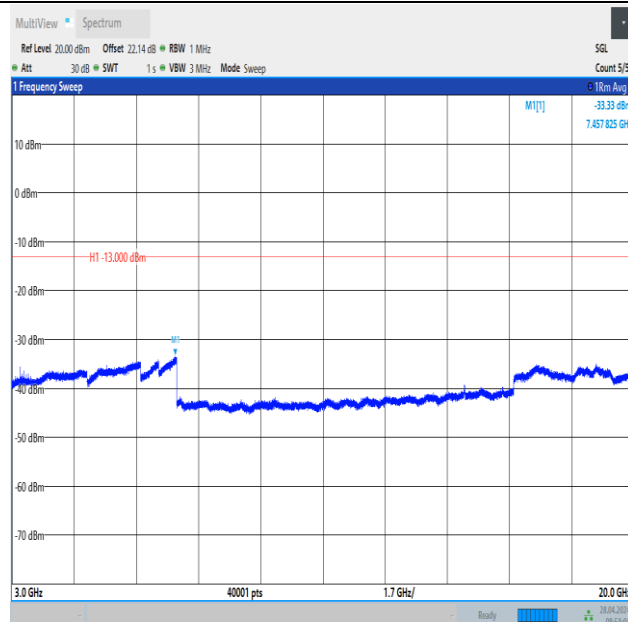
Band2_15MHz_16QAM_18675_1RB#74_3000~20000_3000~20000
