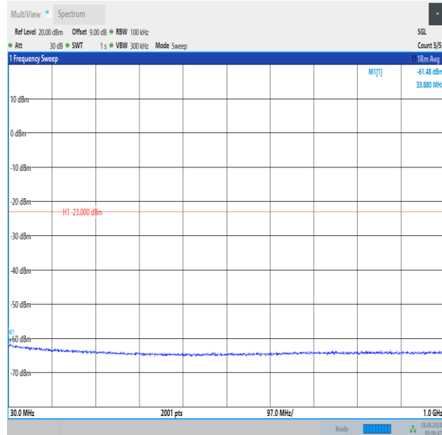
Band2_5MHz_16QAM_18900_1RB#0_30~1000_30~1000
