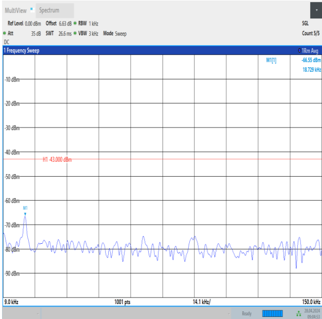
Band2_5MHz_16QAM_18625_25RB#0_0.009~0.15_0.009~0.15
