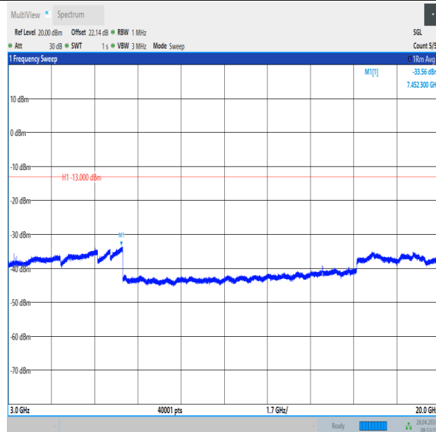
Band2_15MHz_QPSK_18675_1RB#74_3000~20000_3000~20000
