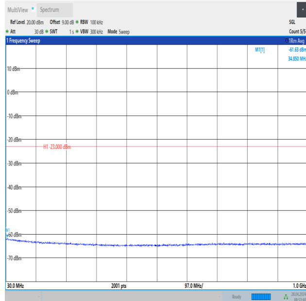
Band2_15MHz_16QAM_18675_1RB#74_30~1000_30~1000
