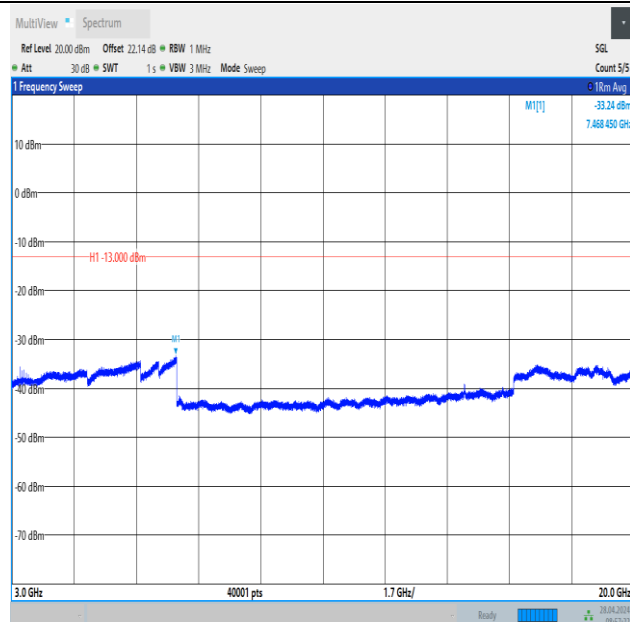
Band2_15MHz_16QAM_18900_1RB#74_3000~20000_3000~20000
