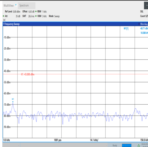
Band2_5MHz_16QAM_18900_1RB#24_0.009~0.15_0.009~0.15
