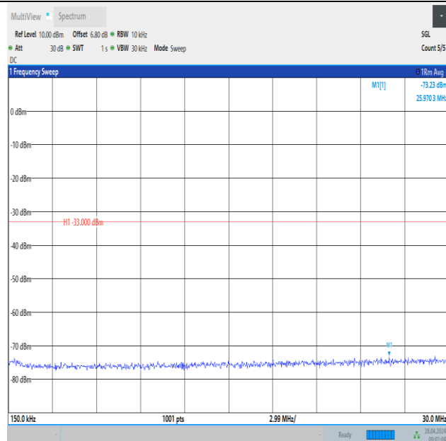
Band2_5MHz_QPSK_18625_1RB#0_0.15~30_0.15~30
