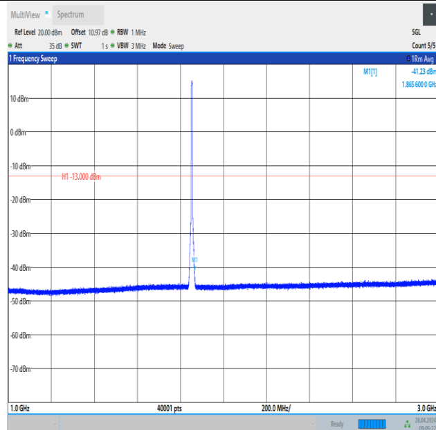
Band2_5MHz_16QAM_18625_25RB#0_1000~3000_1000~3000
