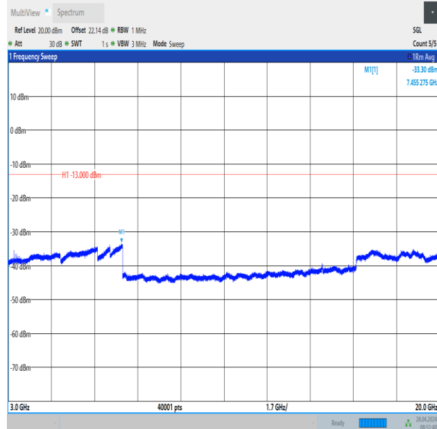
Band2_15MHz_QPSK_18675_1RB#0_3000~20000_3000~20000
