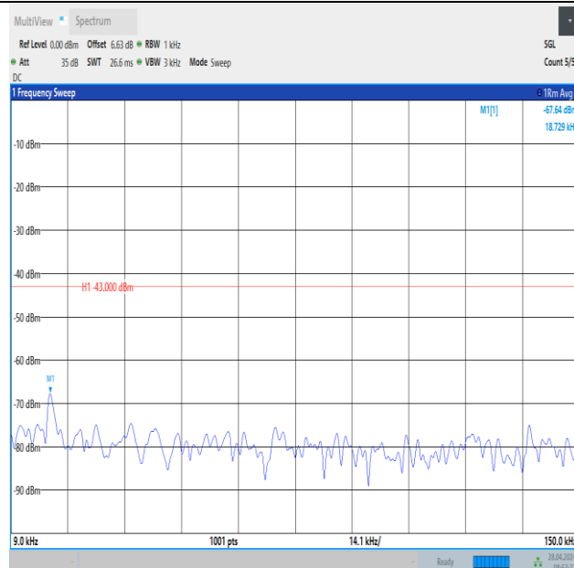
Band2_15MHz_16QAM_18675_1RB#74_0.009~0.15_0.009~0.15
