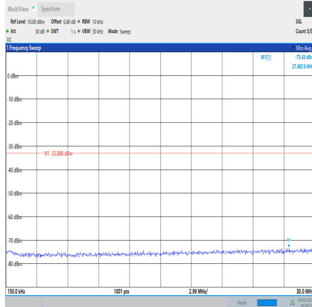
Band2_5MHz_16QAM_18900_1RB#24_0.15~30_0.15~30
