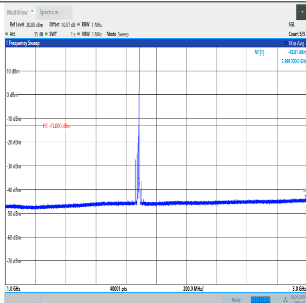
Band2_15MHz_QPSK_18900_1RB#74_1000~3000_1000~3000
