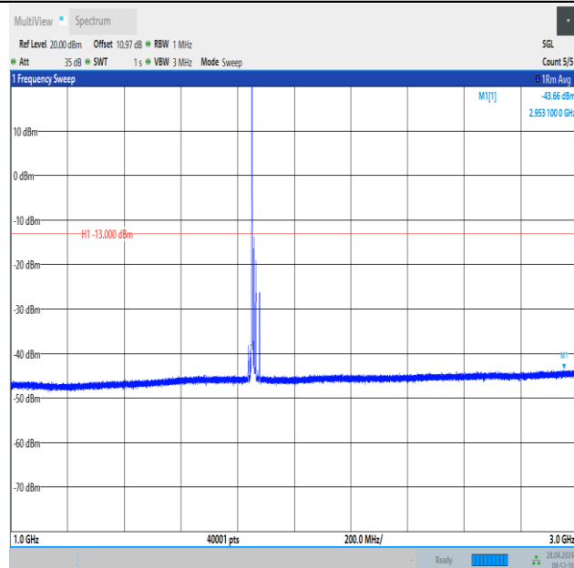
Band2_15MHz_16QAM_18675_1RB#0_1000~3000_1000~3000
