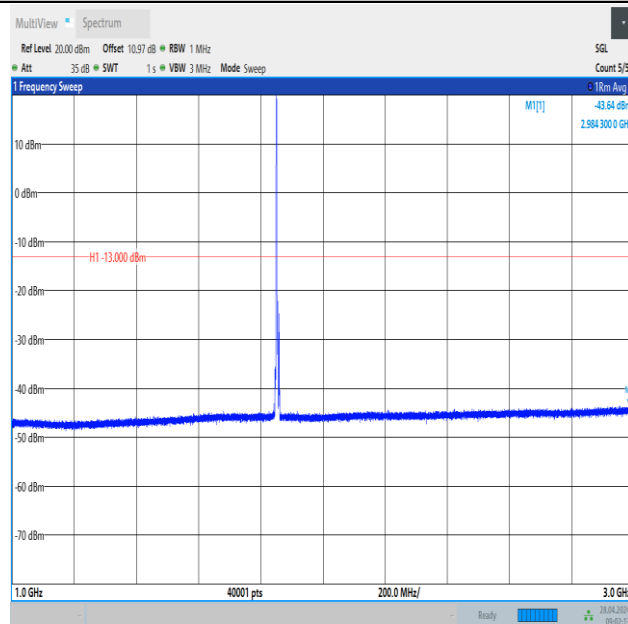
Band2_5MHz_16QAM_18625_1RB#0_1000~3000_1000~3000
