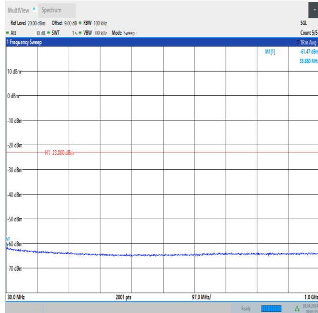
Band2_5MHz_16QAM_18625_1RB#24_30~1000_30~1000
