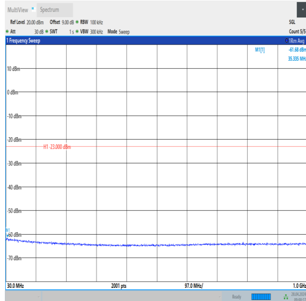
Band2_15MHz_16QAM_19125_1RB#74_30~1000_30~1000
