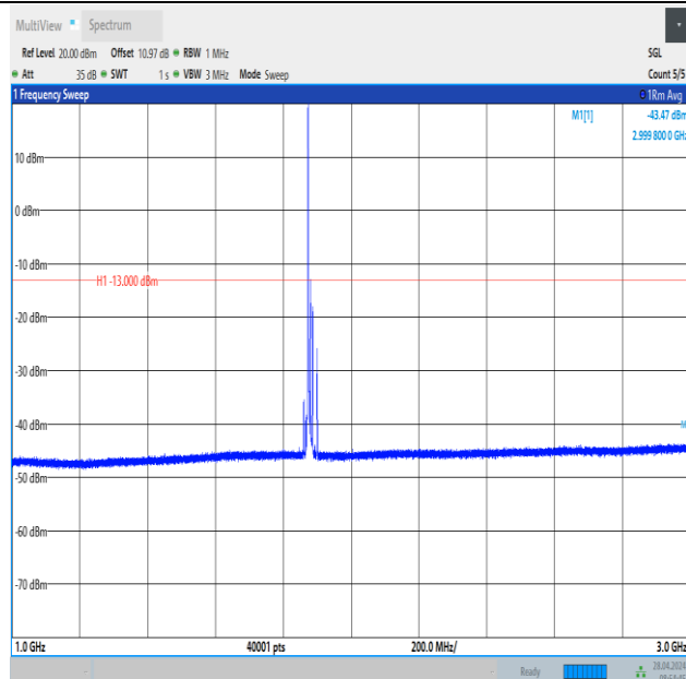
Band2_15MHz_QPSK_18900_1RB#0_1000~3000_1000~3000
