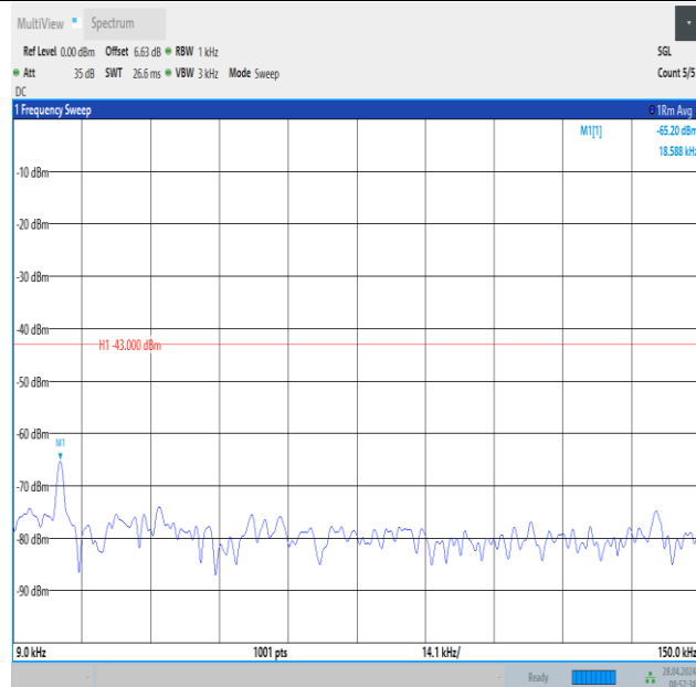
Band2_15MHz_QPSK_19125_1RB#0_0.009~0.15_0.009~0.15
