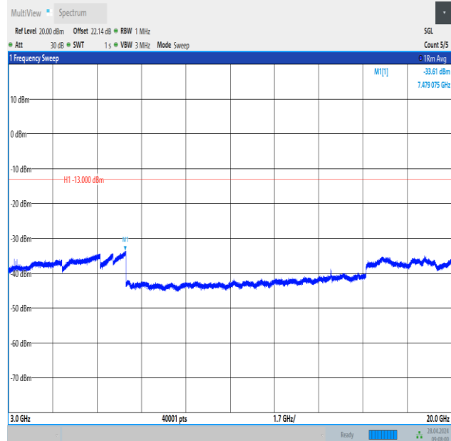
Band2_5MHz_QPSK_18900_1RB#24_3000~20000_3000~20000
