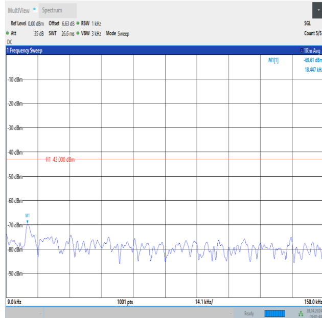
Band2_5MHz_16QAM_18625_1RB#0_0.009~0.15_0.009~0.15
