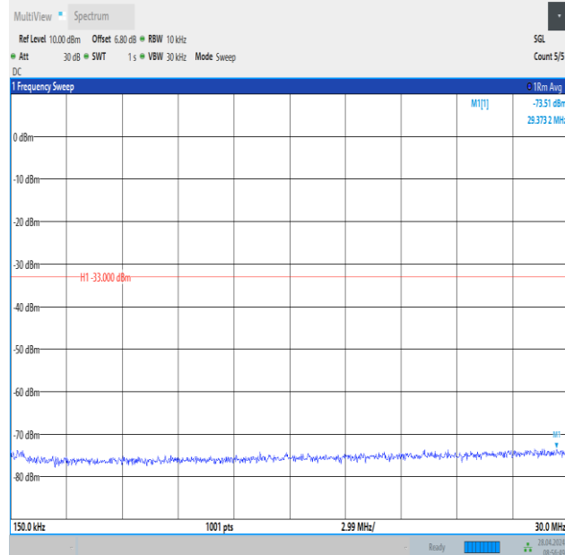
Band2_15MHz_16QAM_18900_1RB#74_0.15~30_0.15~30
