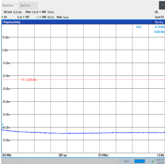
Band2_15MHz_16QAM_19125_1RB#0_30~1000_30~1000
