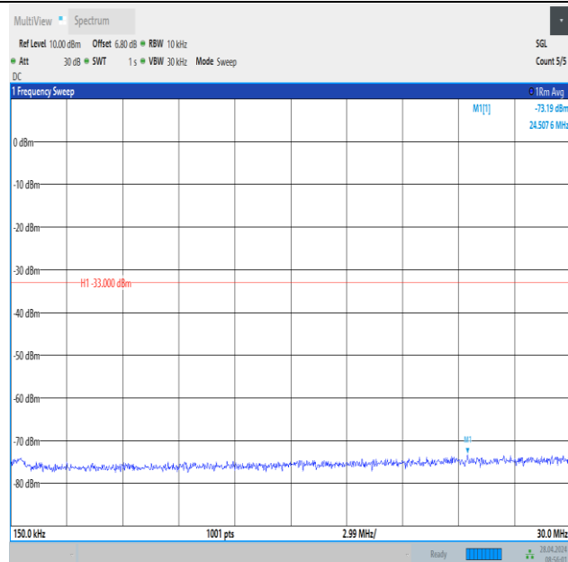
Band2_15MHz_QPSK_18900_1RB#74_0.15~30_0.15~30
