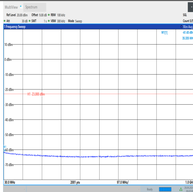
Band2_5MHz_16QAM_18625_1RB#0_30~1000_30~1000
