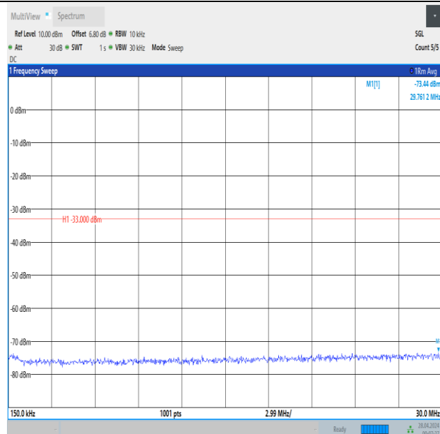
Band2_5MHz_QPSK_18900_1RB#24_0.15~30_0.15~30
