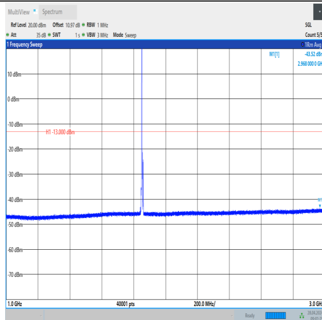
Band2_5MHz_QPSK_18625_1RB#0_1000~3000_1000~3000
