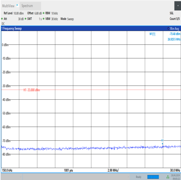
Band2_5MHz_QPSK_18900_1RB#0_0.15~30_0.15~30
