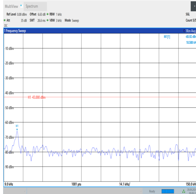
Band2_5MHz_16QAM_18900_1RB#0_0.009~0.15_0.009~0.15
