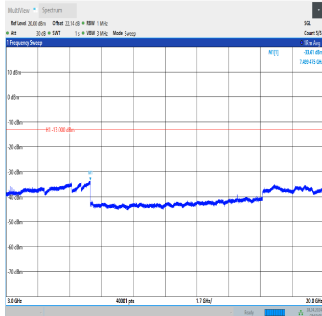
Band2_15MHz_16QAM_19125_1RB#0_3000~20000_3000~20000
