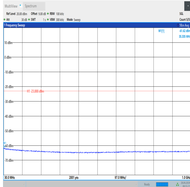
Band2_15MHz_16QAM_18900_1RB#0_30~1000_30~1000
