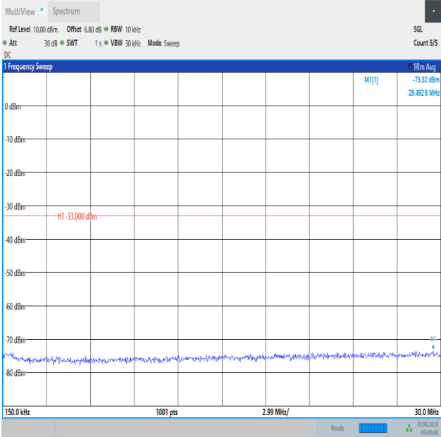
Band2_5MHz_16QAM_18900_25RB#0_0.15~30_0.15~30
