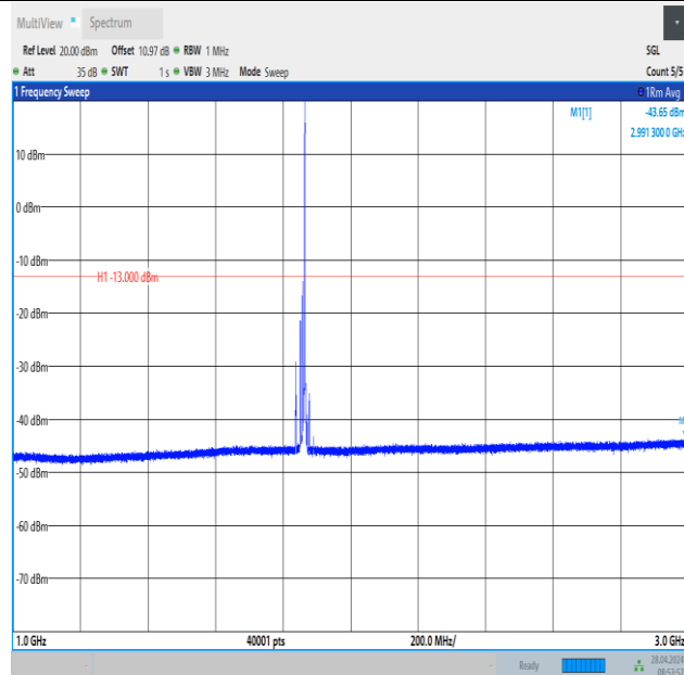
Band2_15MHz_16QAM_18675_1RB#74_1000~3000_1000~3000
