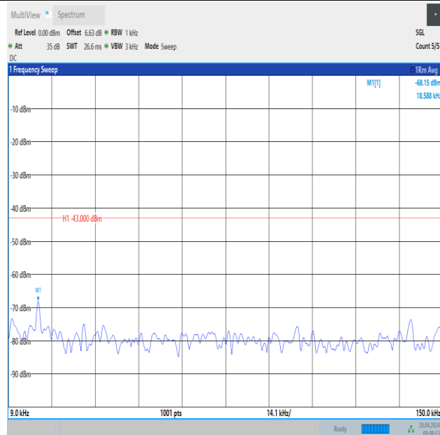
Band2_5MHz_QPSK_18900_25RB#0_0.009~0.15_0.009~0.15
