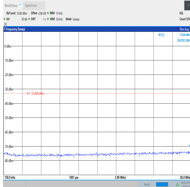
Band2_5MHz_16QAM_18625_1RB#0_0.15~30_0.15~30
