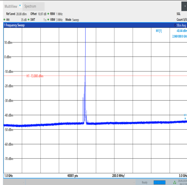
Band2_15MHz_16QAM_18900_1RB#74_1000~3000_1000~3000
