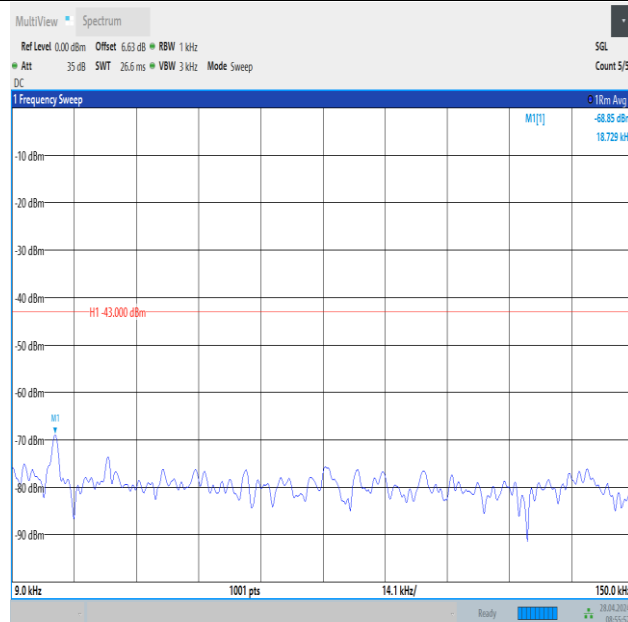
Band2_15MHz_QPSK_18900_1RB#74_0.009~0.15_0.009~0.15
