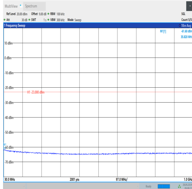
Band2_5MHz_16QAM_18900_1RB#24_30~1000_30~1000
