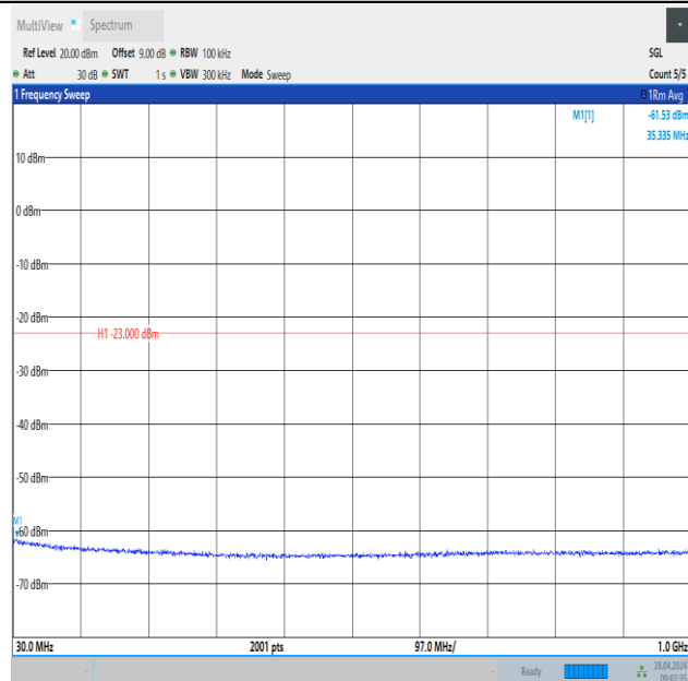
Band2_5MHz_QPSK_18900_1RB#24_30~1000_30~1000
