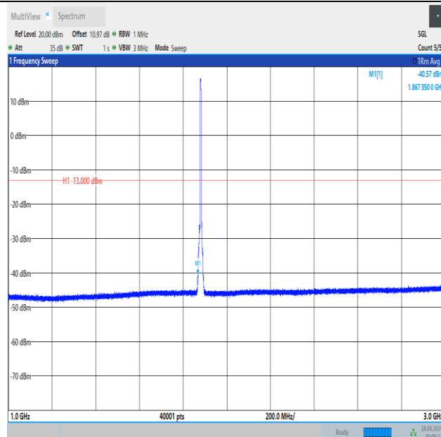
Band2_5MHz_QPSK_18900_25RB#0_1000~3000_1000~3000
