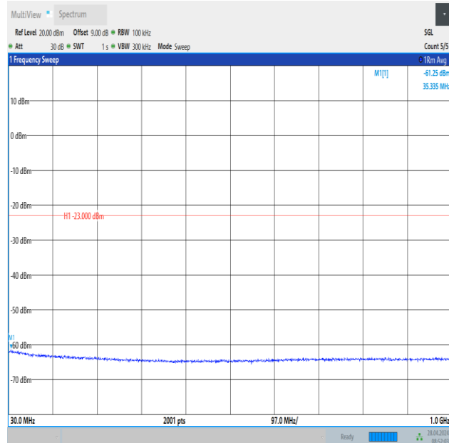
Band2_15MHz_16QAM_18675_1RB#0_30~1000_30~1000
