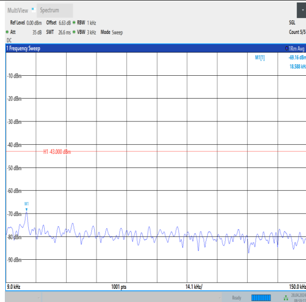
Band2_15MHz_QPSK_19125_1RB#74_0.009~0.15_0.009~0.15
