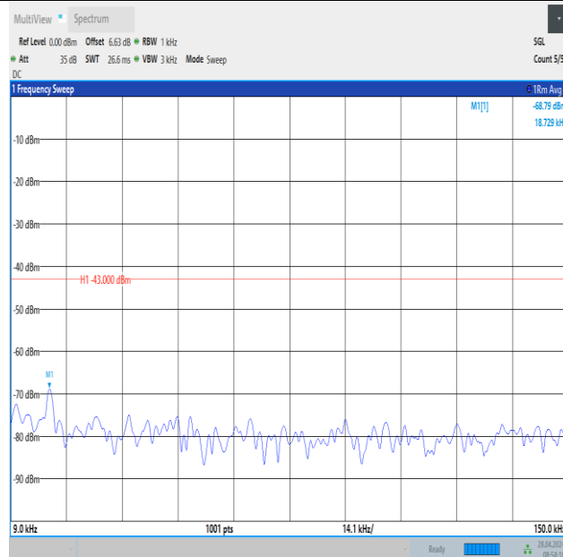
Band2_15MHz_QPSK_18900_1RB#0_0.009~0.15_0.009~0.15
