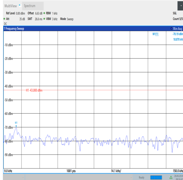
Band2_15MHz_16QAM_18900_1RB#74_0.009~0.15_0.009~0.15
