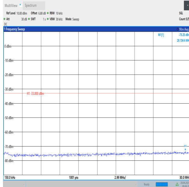
Band2_5MHz_16QAM_18900_1RB#0_0.15~30_0.15~30
