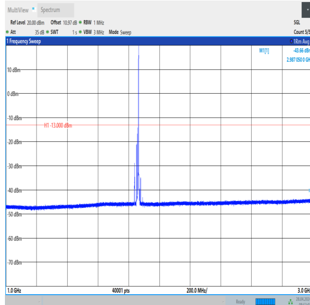
Band2_15MHz_QPSK_18675_1RB#74_1000~3000_1000~3000
