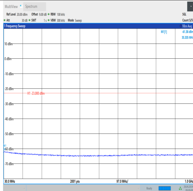
Band2_5MHz_QPSK_18900_25RB#0_30~1000_30~1000
