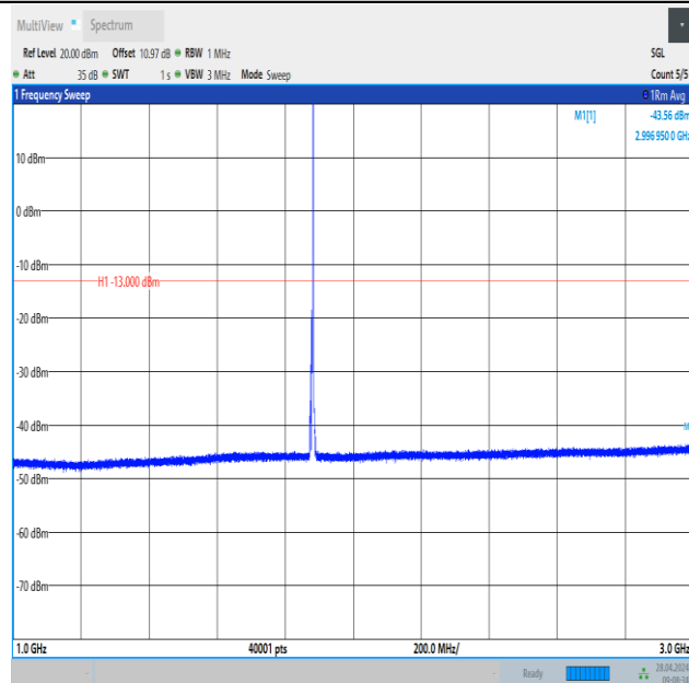
Band2_5MHz_16QAM_18900_1RB#24_1000~3000_1000~3000
