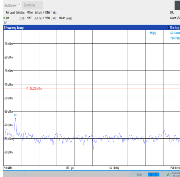
Band2_10MHz_QPSK_19150_1RB#49_0.009~0.15_0.009~0.15
