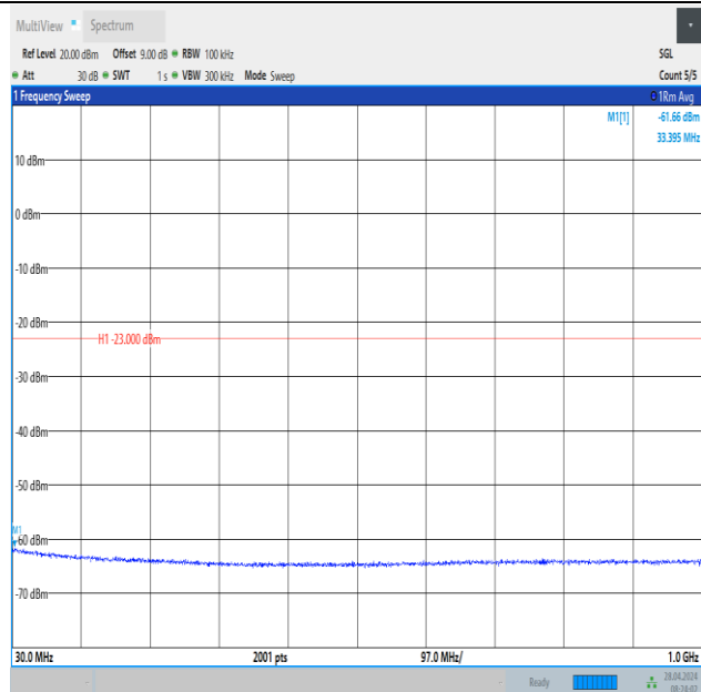
Band2_10MHz_QPSK_18650_50RB#0_30~1000_30~1000
