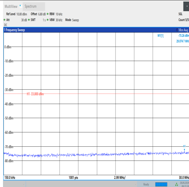
Band2_10MHz_16QAM_18900_1RB#49_0.15~30_0.15~30
