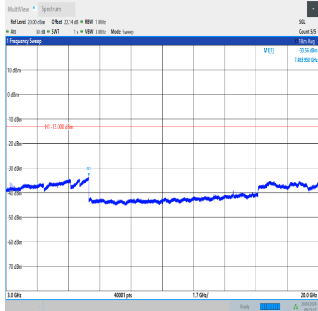
Band2_10MHz_QPSK_19150_1RB#0_3000~20000_3000~20000
