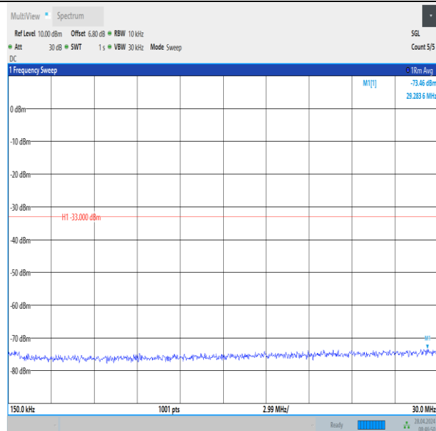
Band2_15MHz_QPSK_18900_75RB#0_0.15~30_0.15~30
