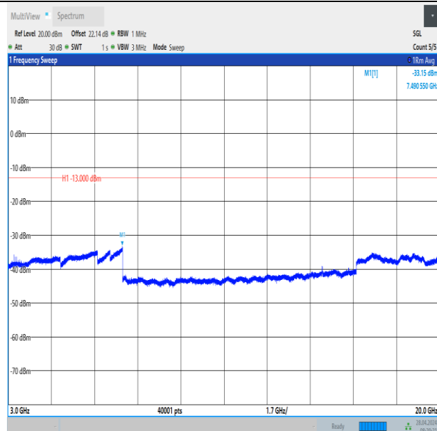
Band2_10MHz_16QAM_18650_1RB#49_3000~20000_3000~20000
