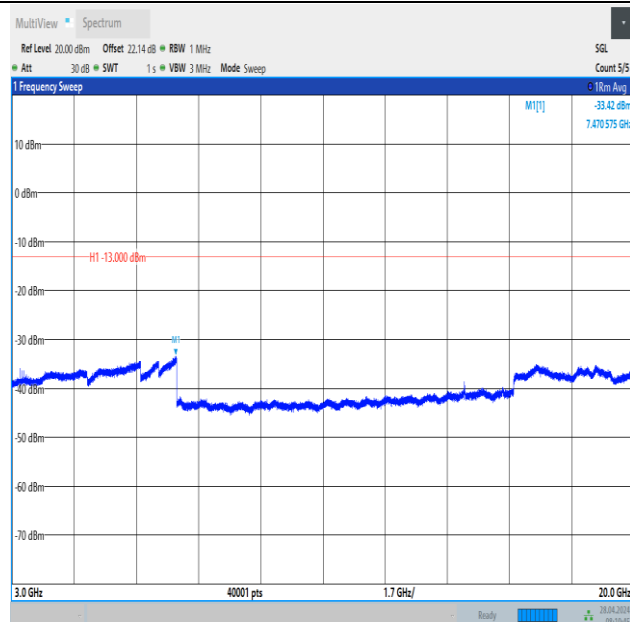
Band2_20MHz_QPSK_19100_1RB#99_3000~20000_3000~20000
