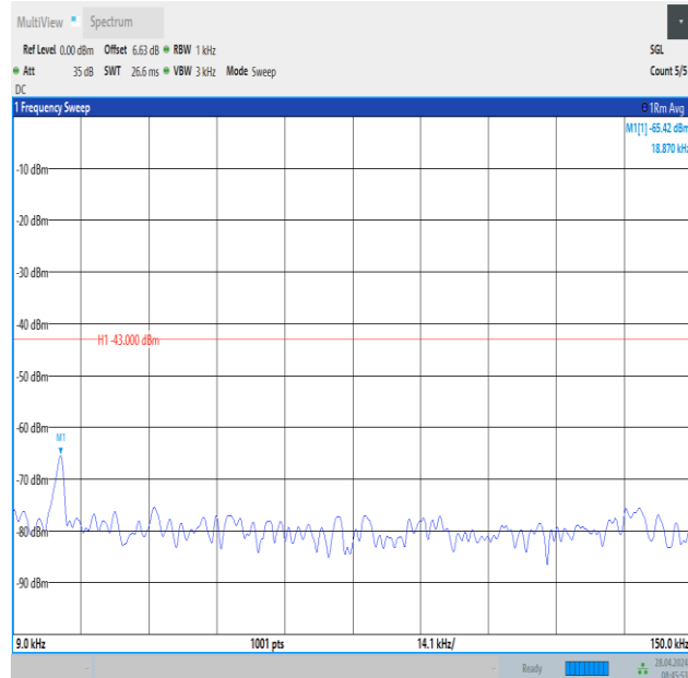
Band2_15MHz_QPSK_18675_75RB#0_0.009~0.15_0.009~0.15
