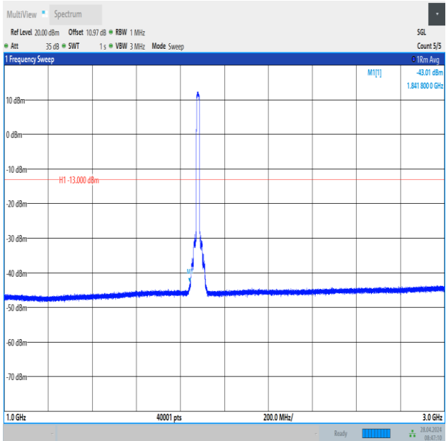
Band2_15MHz_QPSK_18900_75RB#0_1000~3000_1000~3000
