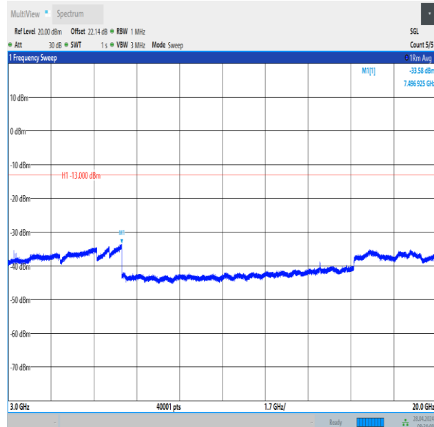
Band2_10MHz_16QAM_19150_1RB#0_3000~20000_3000~20000
