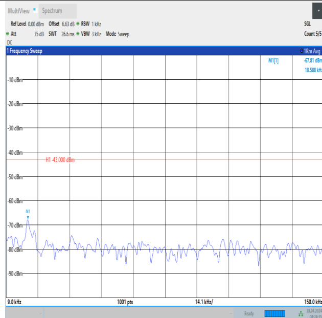
Band2_10MHz_QPSK_18900_50RB#0_0.009~0.15_0.009~0.15
