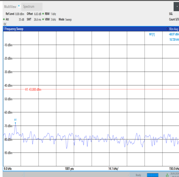
Band2_10MHz_16QAM_19150_1RB#49_0.009~0.15_0.009~0.15
