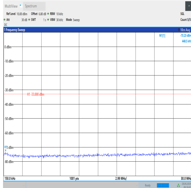
Band2_10MHz_QPSK_18900_50RB#0_0.15~30_0.15~30
