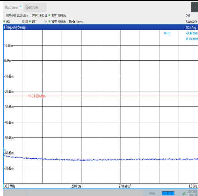
Band2_15MHz_QPSK_19125_75RB#0_30~1000_30~1000
