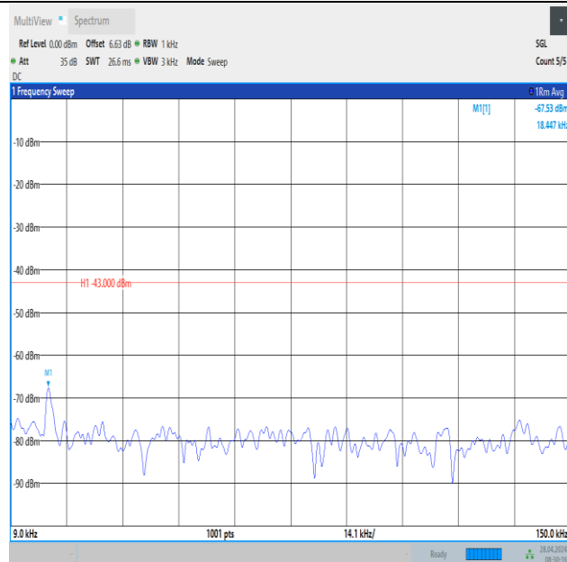
Band2_10MHz_16QAM_18900_1RB#0_0.009~0.15_0.009~0.15
