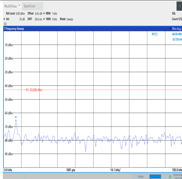
Band2_10MHz_QPSK_18900_1RB#49_0.009~0.15_0.009~0.15
