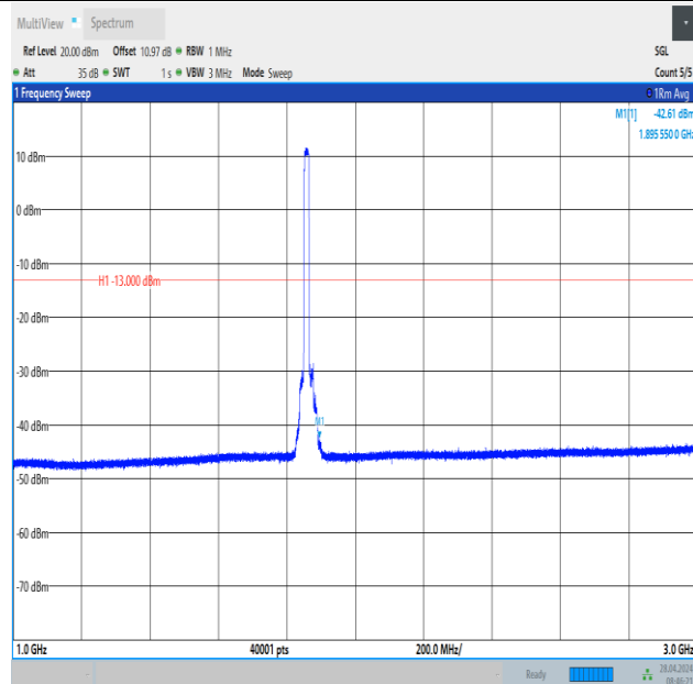
Band2_15MHz_QPSK_18675_75RB#0_1000~3000_1000~3000
