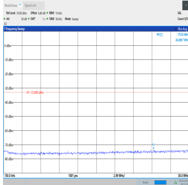
Band2_10MHz_16QAM_19150_1RB#0_0.15~30_0.15~30
