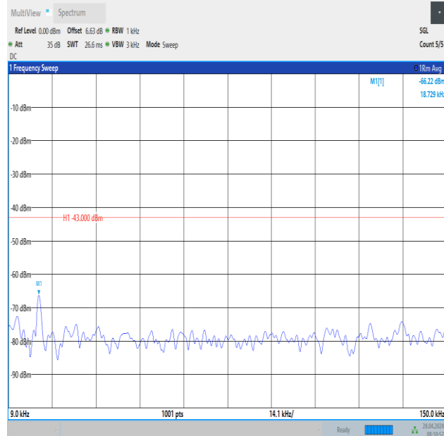
Band2_20MHz_16QAM_19100_1RB#99_0.009~0.15_0.009~0.15
