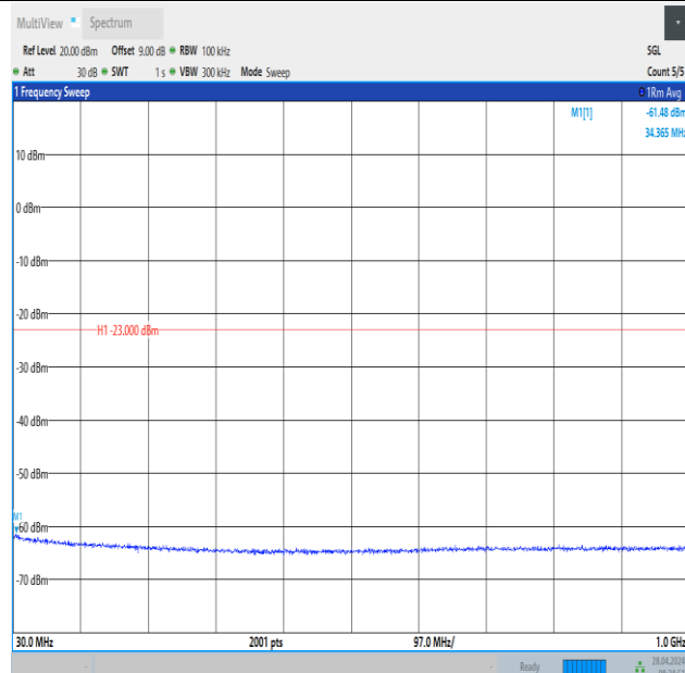
Band2_10MHz_QPSK_18900_50RB#0_30~1000_30~1000
