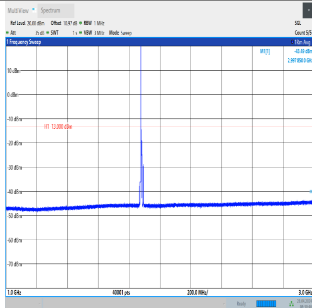
Band2_10MHz_16QAM_18900_1RB#0_1000~3000_1000~3000
