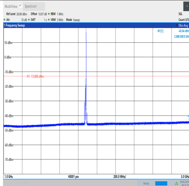
Band2_10MHz_16QAM_18900_1RB#49_1000~3000_1000~3000
