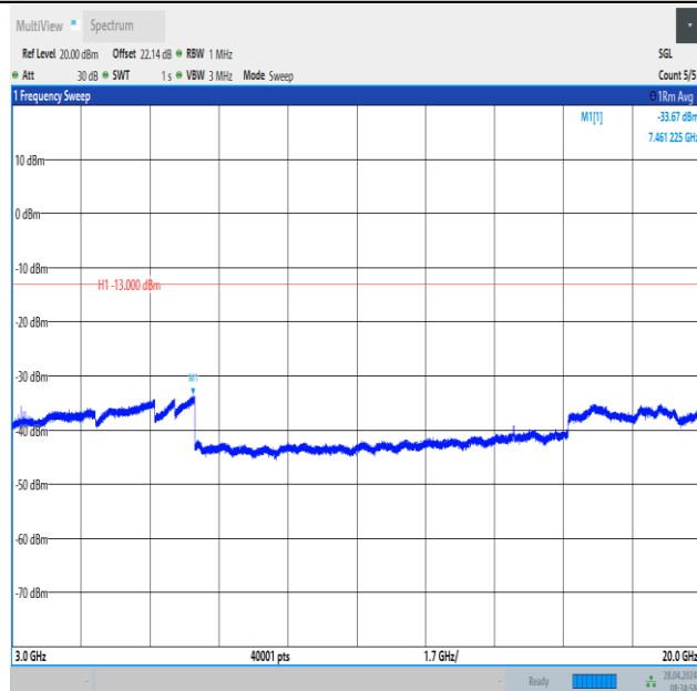
Band2_10MHz_QPSK_19150_1RB#49_3000~20000_3000~20000
