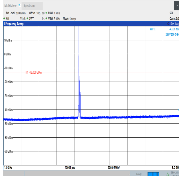
Band2_10MHz_QPSK_18650_1RB#0_1000~3000_1000~3000
