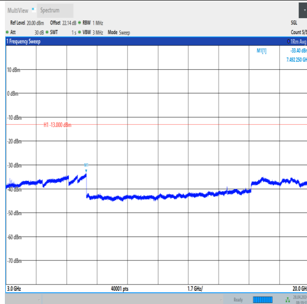
Band2_20MHz_QPSK_18700_100RB#0_3000~20000_3000~20000
