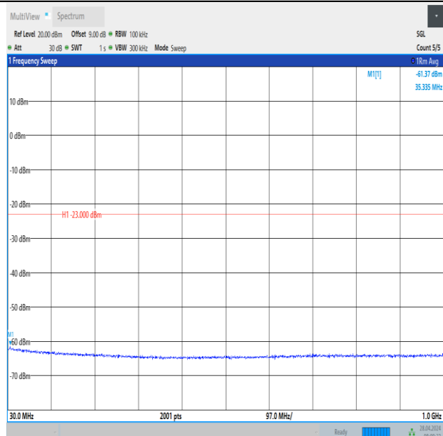
Band2_20MHz_16QAM_19100_1RB#0_30~1000_30~1000
