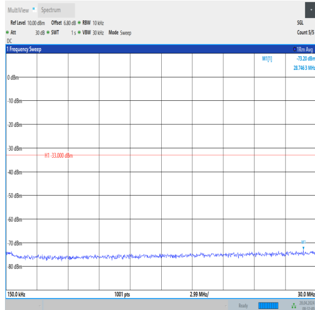
Band2_10MHz_QPSK_19150_1RB#0_0.15~30_0.15~30
