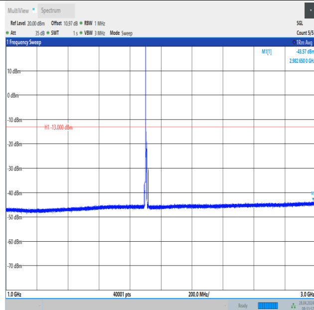
Band2_10MHz_16QAM_19150_1RB#0_1000~3000_1000~3000
