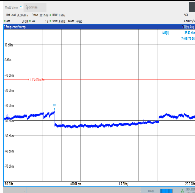
Band2_10MHz_16QAM_18900_1RB#49_3000~20000_3000~20000
