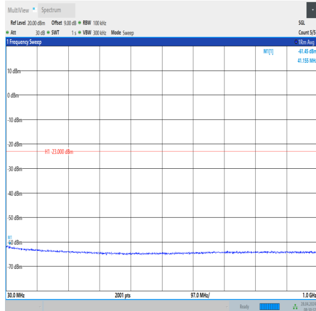
Band2_10MHz_16QAM_18900_1RB#0_30~1000_30~1000
