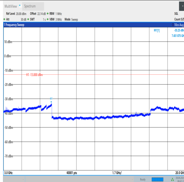
Band2_20MHz_QPSK_19100_100RB#0_3000~20000_3000~20000
