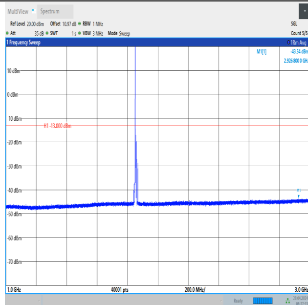
Band2_10MHz_16QAM_18650_1RB#0_1000~3000_1000~3000
