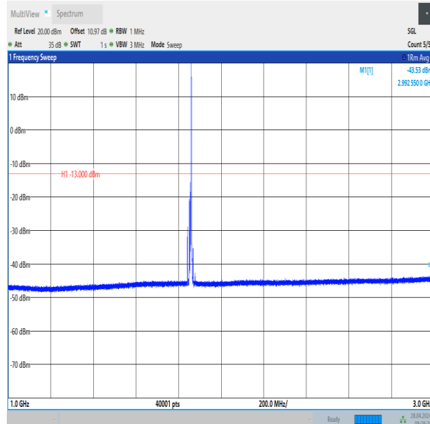
Band2_10MHz_QPSK_18650_1RB#49_1000~3000_1000~3000
