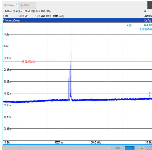
Band2_20MHz_QPSK_19100_1RB#99_1000~3000_1000~3000
