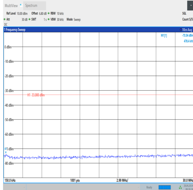
Band2_10MHz_16QAM_18900_1RB#0_0.15~30_0.15~30
