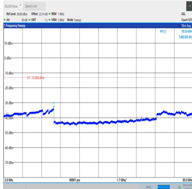
Band2_15MHz_QPSK_18675_75RB#0_3000~20000_3000~20000
