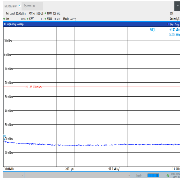
Band2_10MHz_QPSK_19150_1RB#0_30~1000_30~1000
