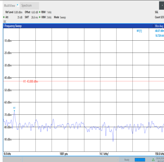
Band2_10MHz_QPSK_19150_1RB#0_0.009~0.15_0.009~0.15
