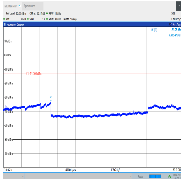
Band2_10MHz_QPSK_18900_1RB#49_3000~20000_3000~20000
