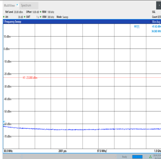
Band2_10MHz_QPSK_18900_1RB#0_30~1000_30~1000
