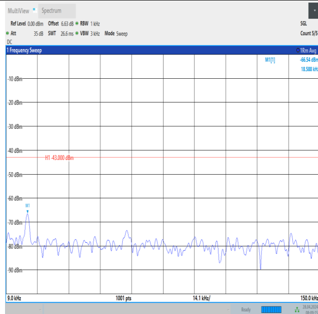
Band2_20MHz_16QAM_19100_1RB#0_0.009~0.15_0.009~0.15
