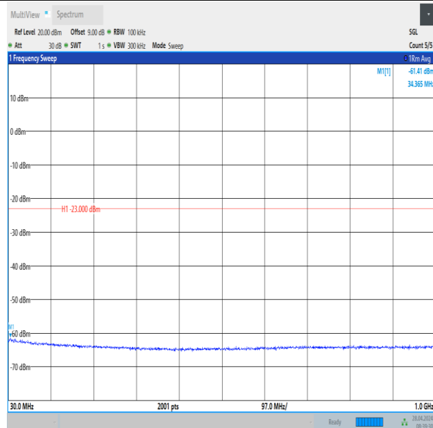
Band2_20MHz_QPSK_18700_100RB#0_30~1000_30~1000
