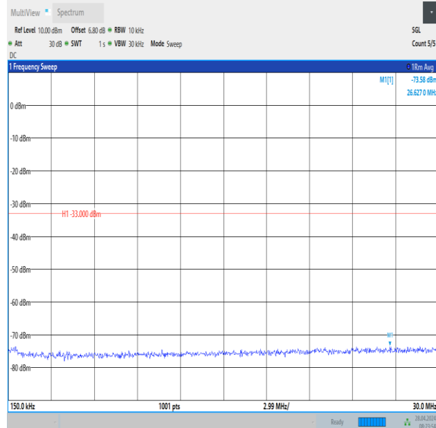
Band2_10MHz_QPSK_18650_50RB#0_0.15~30_0.15~30
