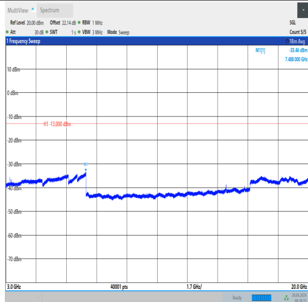
Band2_10MHz_QPSK_18650_1RB#49_3000~20000_3000~20000
