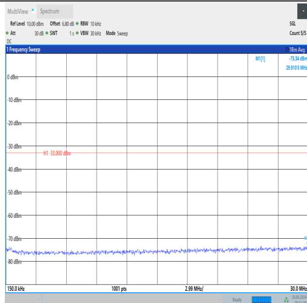
Band2_20MHz_16QAM_19100_1RB#99_0.15~30_0.15~30
