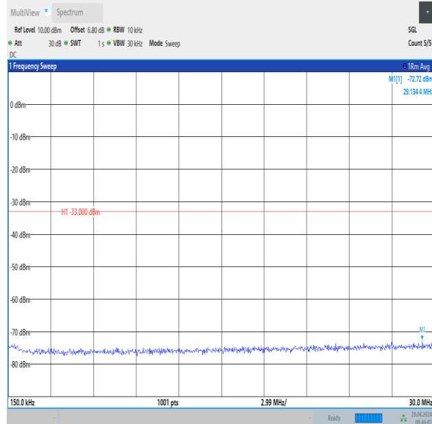
Band2_15MHz_QPSK_18675_75RB#0_0.15~30_0.15~30
