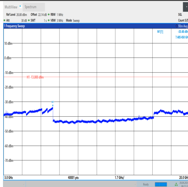
Band2_20MHz_16QAM_19100_1RB#99_3000~20000_3000~20000
