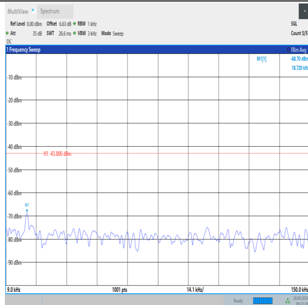
Band2_10MHz_16QAM_19150_1RB#0_0.009~0.15_0.009~0.15
