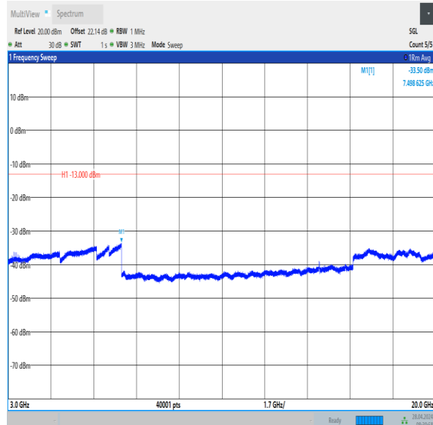
Band2_10MHz_16QAM_18900_1RB#0_3000~20000_3000~20000
