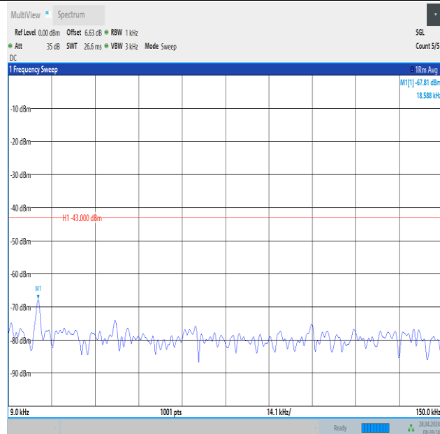
Band2_20MHz_QPSK_18700_100RB#0_0.009~0.15_0.009~0.15
