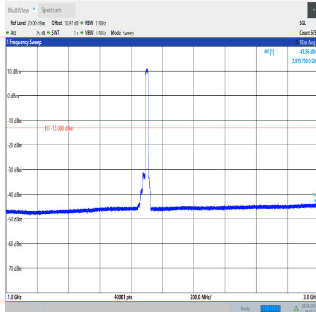
Band2_20MHz_QPSK_19100_100RB#0_1000~3000_1000~3000
