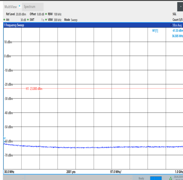
Band2_15MHz_QPSK_18900_75RB#0_30~1000_30~1000
