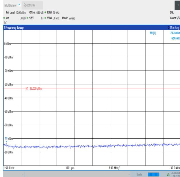
Band2_10MHz_16QAM_18650_1RB#0_0.15~30_0.15~30
