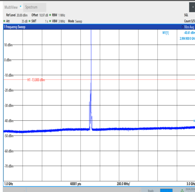
Band2_10MHz_QPSK_19150_1RB#49_1000~3000_1000~3000
