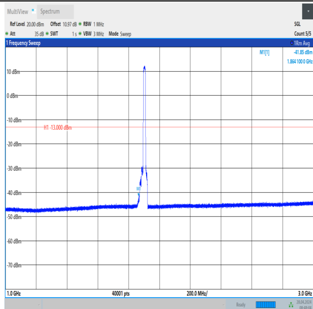
Band2_15MHz_QPSK_19125_75RB#0_1000~3000_1000~3000
