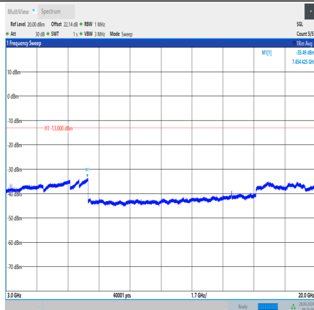
Band2_10MHz_QPSK_19150_50RB#0_3000~20000_3000~20000
