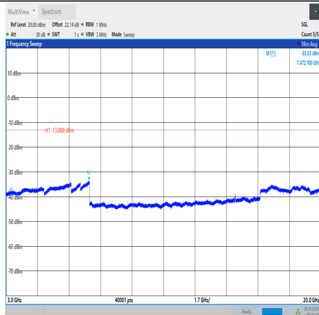
Band2_10MHz_16QAM_19150_1RB#49_3000~20000_3000~20000
