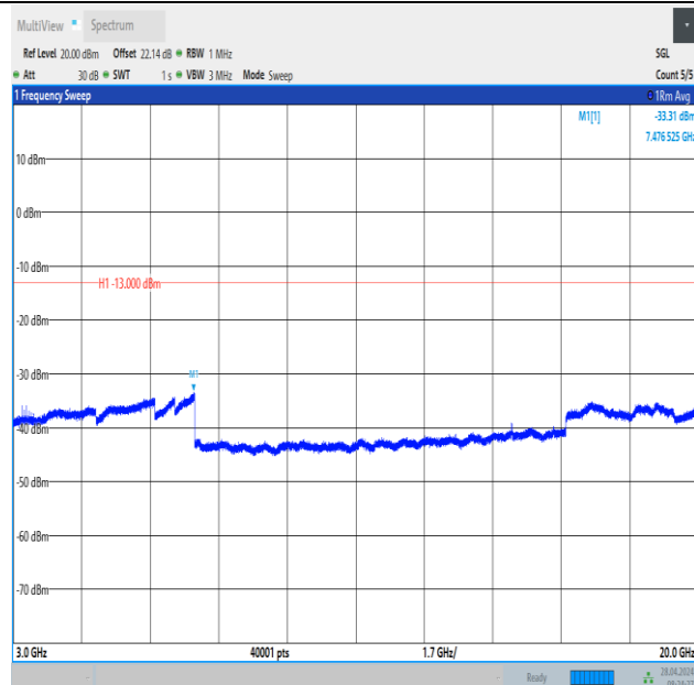
Band2_10MHz_QPSK_18650_50RB#0_3000~20000_3000~20000
