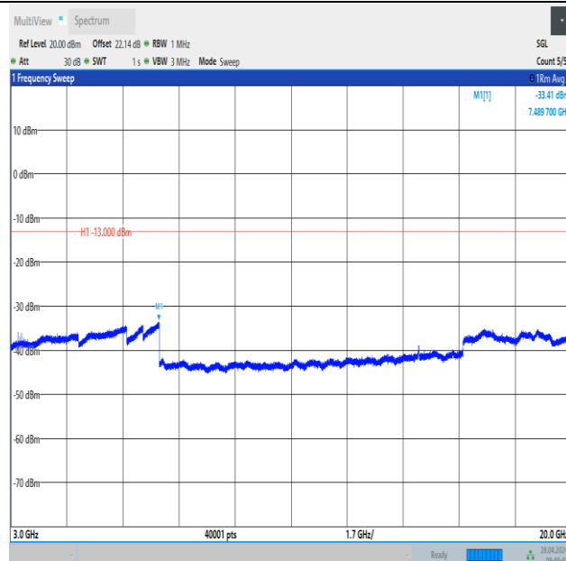
Band2_20MHz_QPSK_18900_100RB#0_3000~20000_3000~20000
