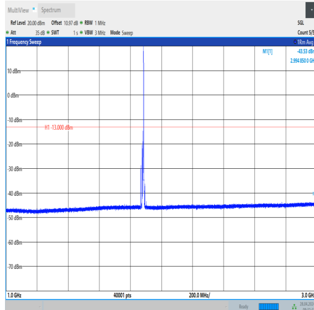
Band2_10MHz_QPSK_18900_1RB#49_1000~3000_1000~3000
