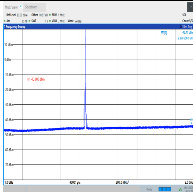
Band2_10MHz_16QAM_18650_1RB#49_1000~3000_1000~3000
