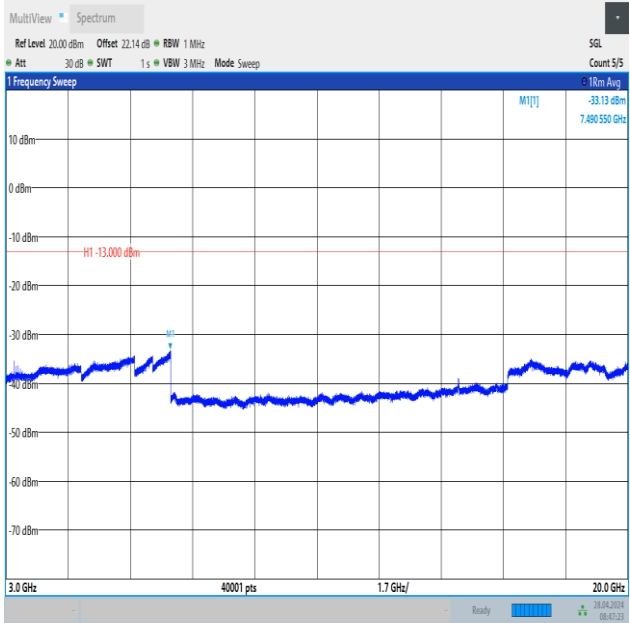
Band2_15MHz_QPSK_18900_75RB#0_3000~20000_3000~20000
