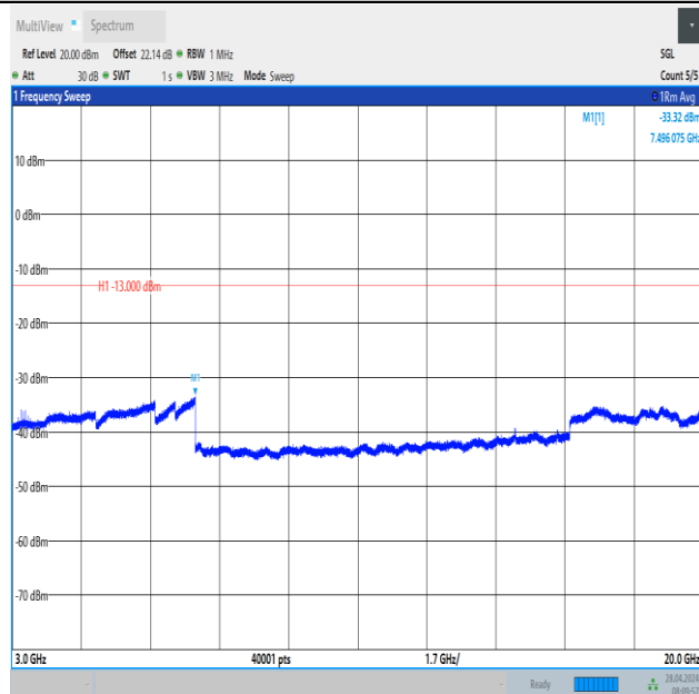
Band2_20MHz_16QAM_19100_1RB#0_3000~20000_3000~20000
