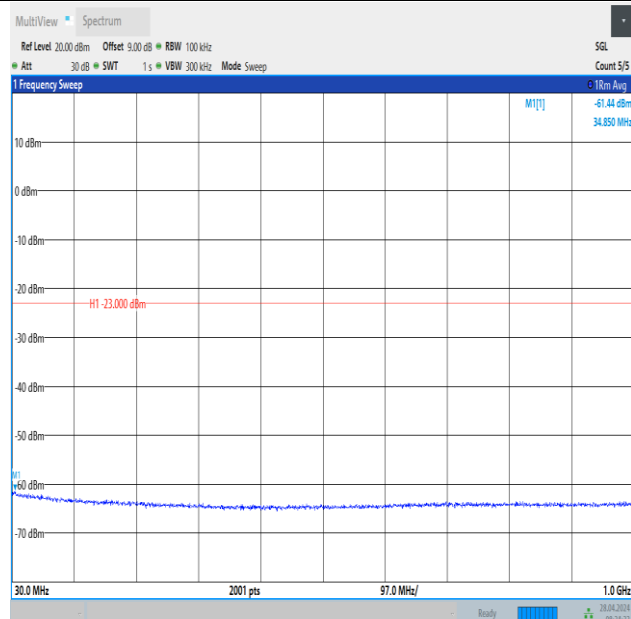
Band2_10MHz_QPSK_19150_1RB#49_30~1000_30~1000
