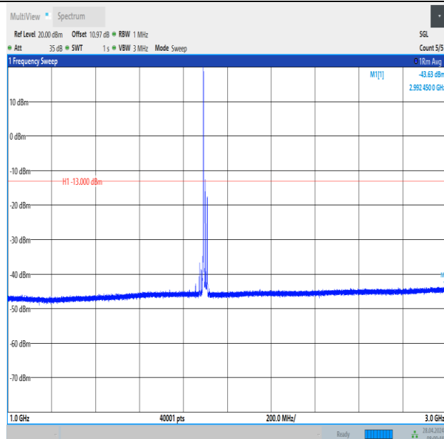
Band2_20MHz_16QAM_19100_1RB#0_1000~3000_1000~3000
