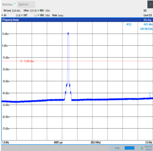
Band2_20MHz_QPSK_18900_100RB#0_1000~3000_1000~3000
