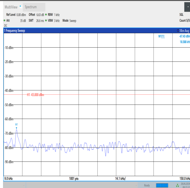
Band2_10MHz_16QAM_18900_1RB#49_0.009~0.15_0.009~0.15
