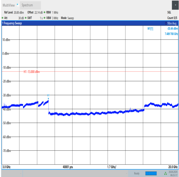
Band2_10MHz_QPSK_18900_50RB#0_3000~20000_3000~20000
