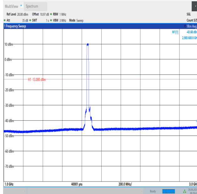
Band2_20MHz_QPSK_18700_100RB#0_1000~3000_1000~3000
