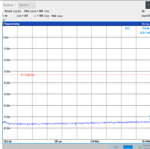
Band2_10MHz_16QAM_19150_1RB#49_0.15~30_0.15~30
