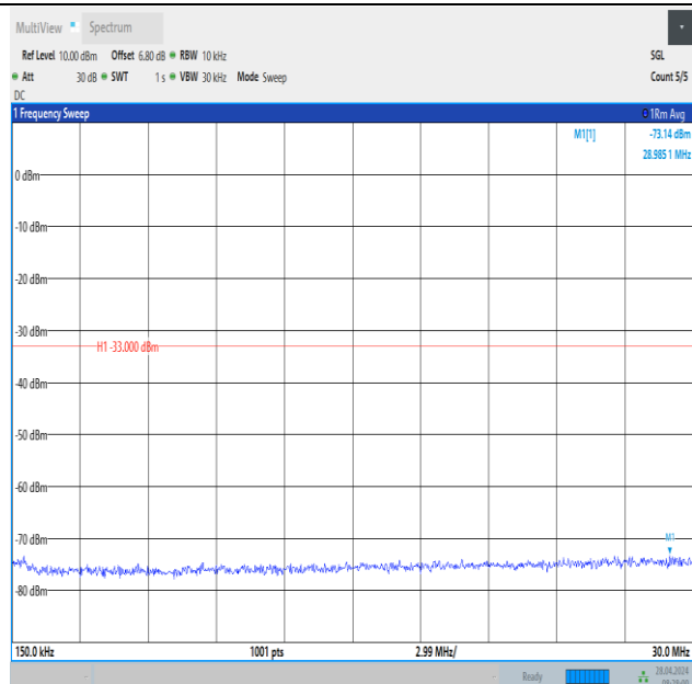
Band2_10MHz_QPSK_18650_1RB#49_0.15~30_0.15~30
