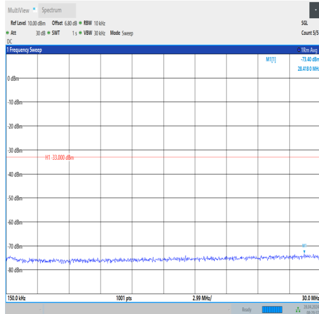
Band2_10MHz_QPSK_18900_1RB#0_0.15~30_0.15~30
