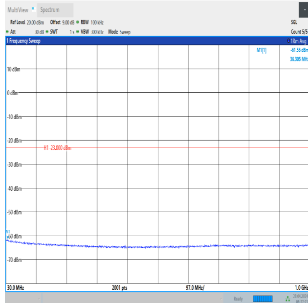
Band2_10MHz_16QAM_18650_1RB#0_30~1000_30~1000
