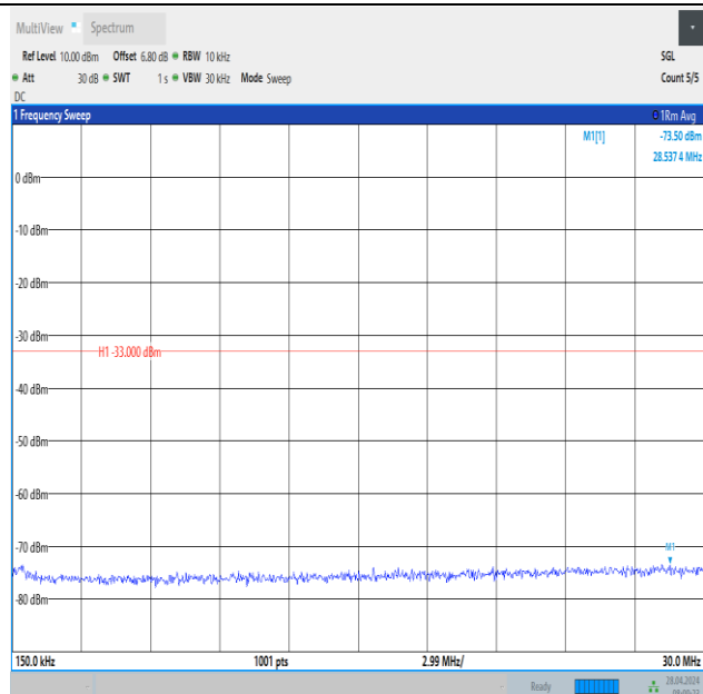
Band2_20MHz_16QAM_19100_1RB#0_0.15~30_0.15~30
