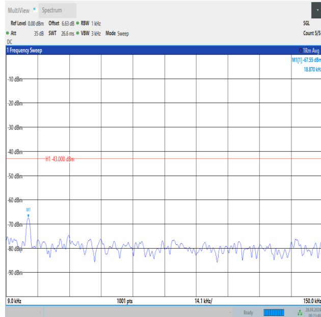
Band2_10MHz_QPSK_18650_50RB#0_0.009~0.15_0.009~0.15
