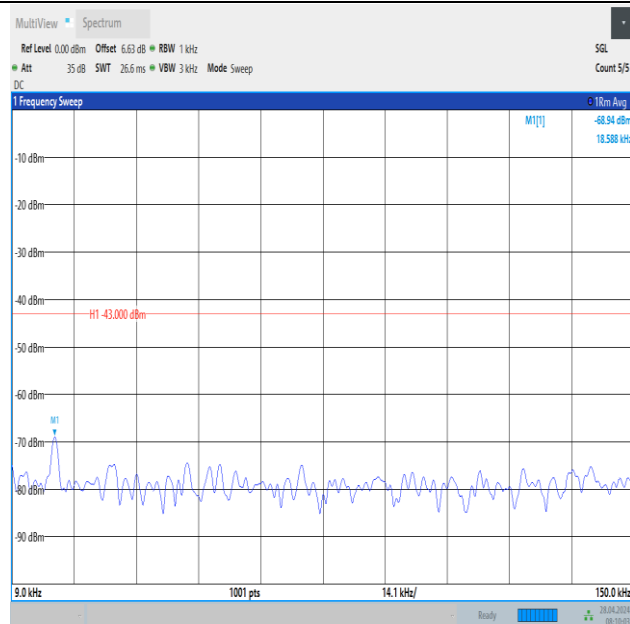
Band2_20MHz_QPSK_19100_1RB#99_0.009~0.15_0.009~0.15
