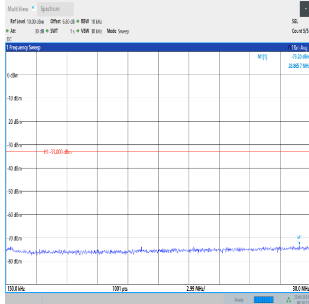
Band2_20MHz_QPSK_19100_1RB#99_0.15~30_0.15~30
