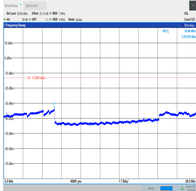
Band2_10MHz_QPSK_18650_1RB#0_3000~20000_3000~20000
