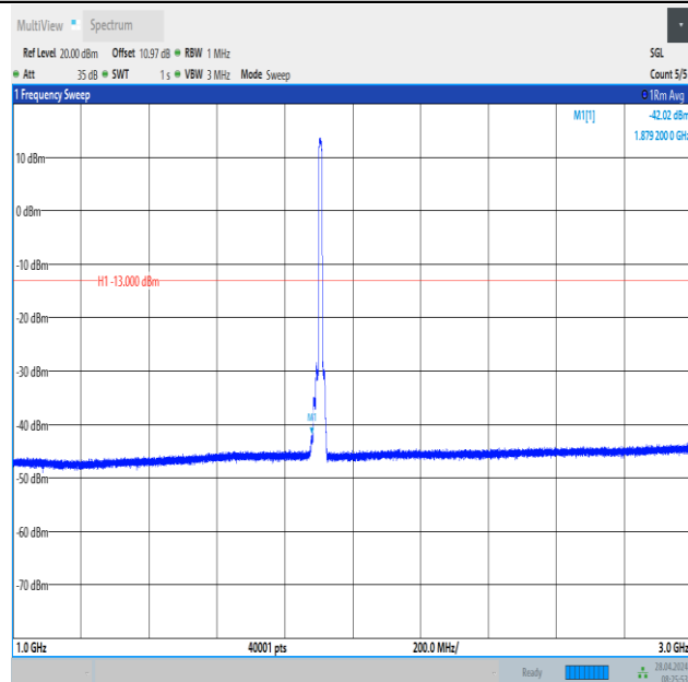
Band2_10MHz_QPSK_19150_50RB#0_1000~3000_1000~3000
