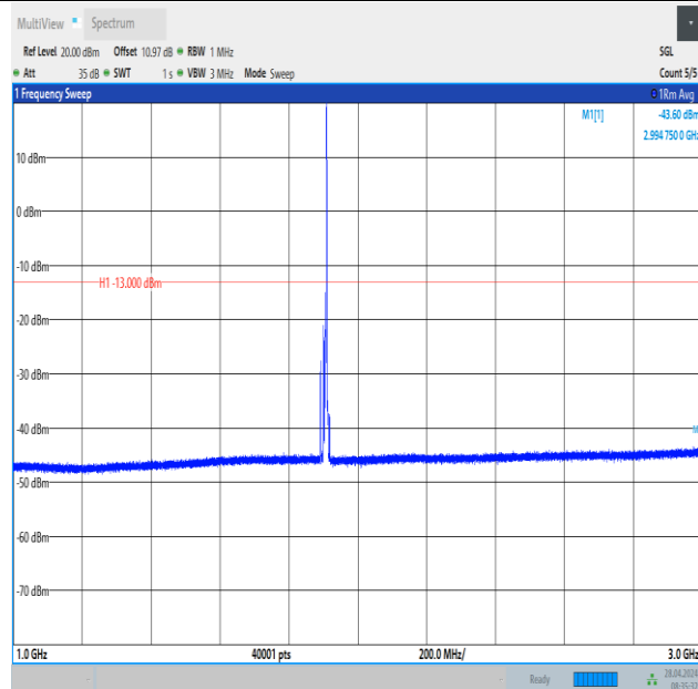
Band2_10MHz_16QAM_19150_1RB#49_1000~3000_1000~3000
