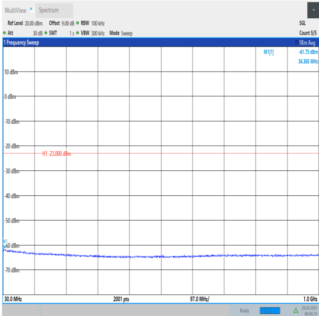
Band2_20MHz_QPSK_18900_100RB#0_30~1000_30~1000
