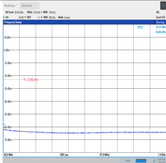
Band2_20MHz_QPSK_19100_100RB#0_30~1000_30~1000
