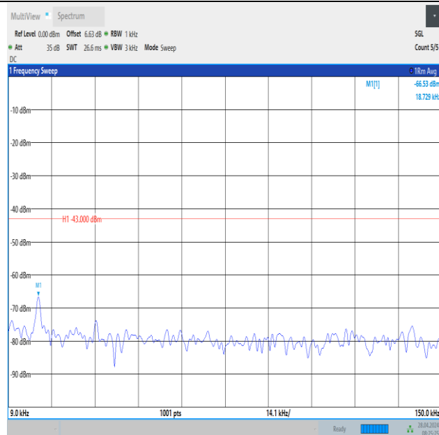
Band2_10MHz_QPSK_19150_50RB#0_0.009~0.15_0.009~0.15
