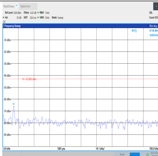
Band2_20MHz_QPSK_18900_100RB#0_0.009~0.15_0.009~0.15
