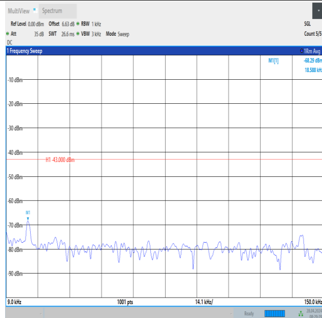
Band2_10MHz_QPSK_18900_1RB#0_0.009~0.15_0.009~0.15
