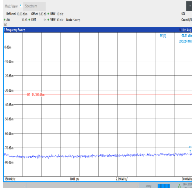
Band2_10MHz_QPSK_18900_1RB#49_0.15~30_0.15~30
