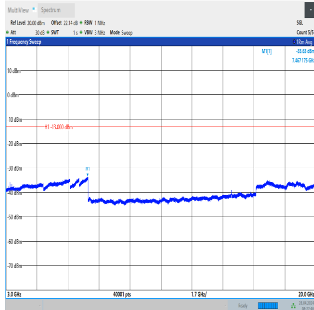
Band2_10MHz_16QAM_18650_1RB#0_3000~20000_3000~20000
