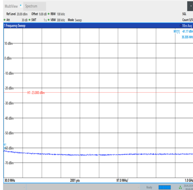
Band2_15MHz_QPSK_18675_75RB#0_30~1000_30~1000
