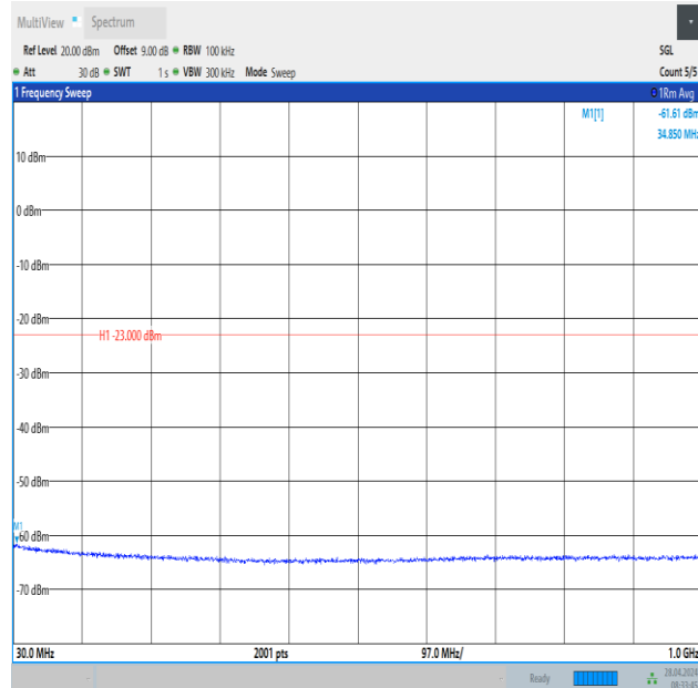
Band2_10MHz_16QAM_19150_1RB#0_30~1000_30~1000
