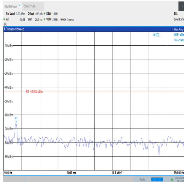
Band2_15MHz_QPSK_18900_75RB#0_0.009~0.15_0.009~0.15
