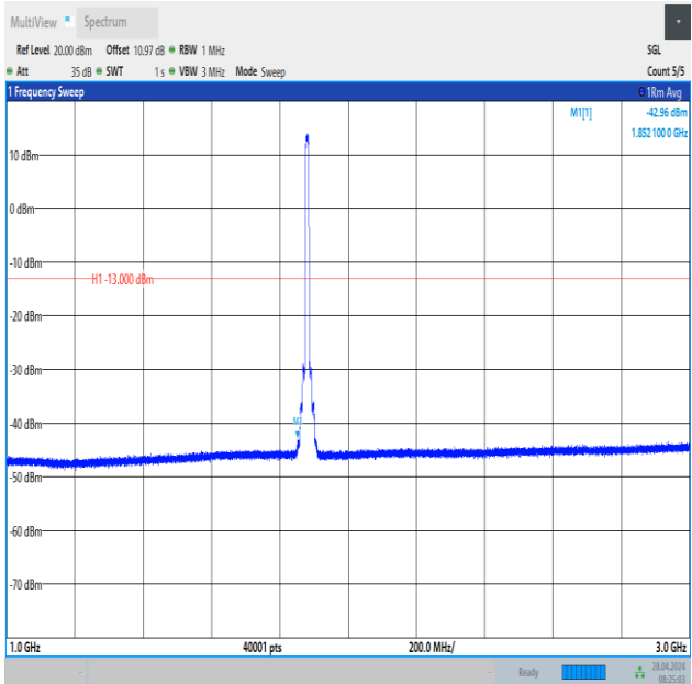
Band2_10MHz_QPSK_18900_50RB#0_1000~3000_1000~3000
