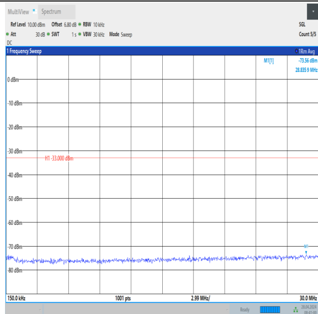
Band2_20MHz_QPSK_19100_100RB#0_0.15~30_0.15~30
