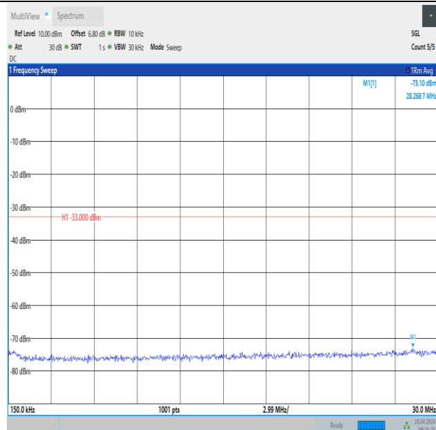
Band2_10MHz_QPSK_18650_1RB#0_0.15~30_0.15~30
