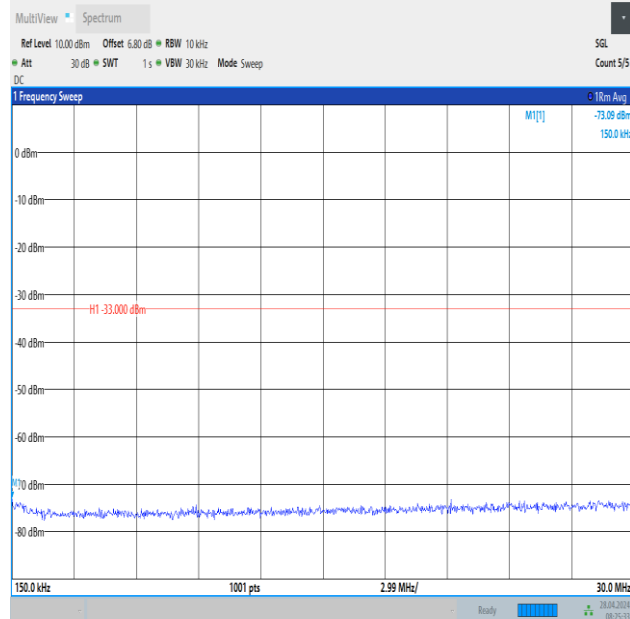
Band2_10MHz_QPSK_19150_50RB#0_0.15~30_0.15~30
