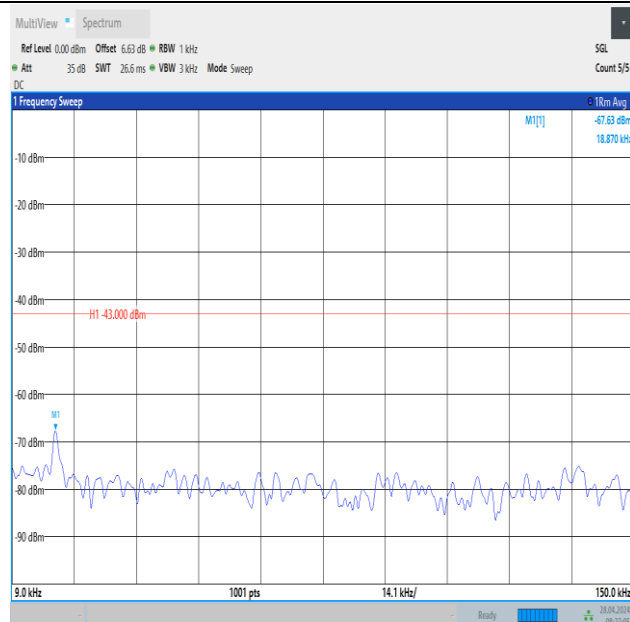
Band2_10MHz_16QAM_18650_1RB#0_0.009~0.15_0.009~0.15
