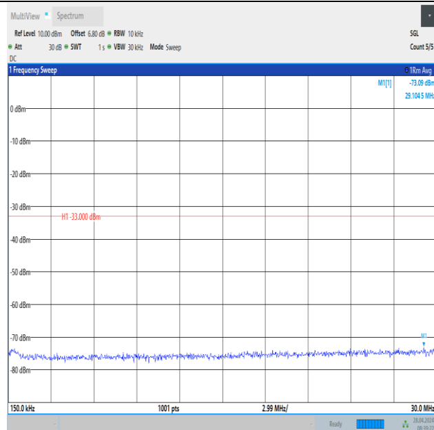
Band2_20MHz_QPSK_18700_100RB#0_0.15~30_0.15~30
