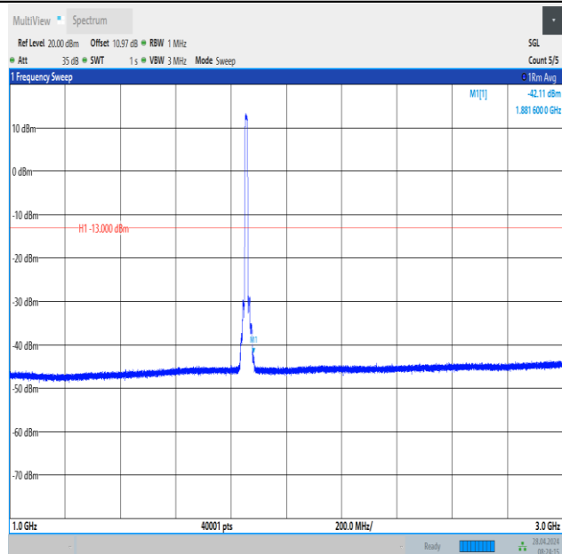
Band2_10MHz_QPSK_18650_50RB#0_1000~3000_1000~3000
