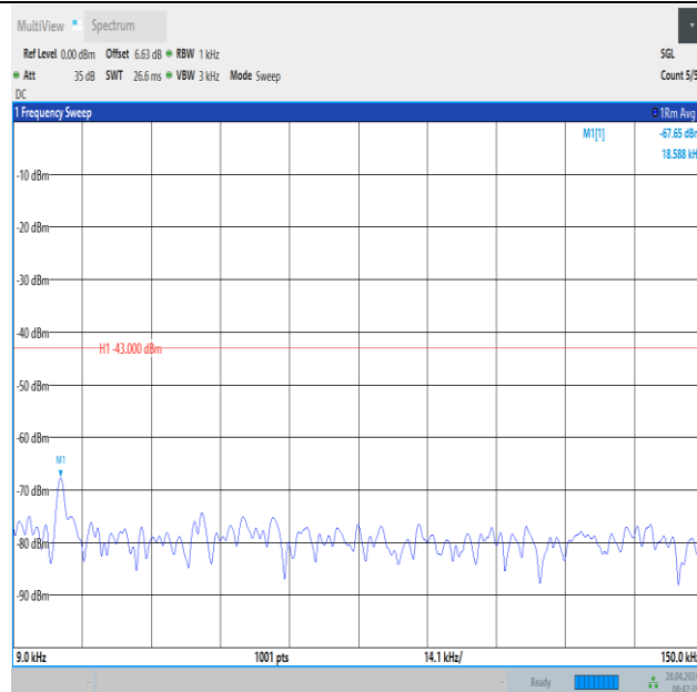
Band2_15MHz_QPSK_19125_75RB#0_0.009~0.15_0.009~0.15
