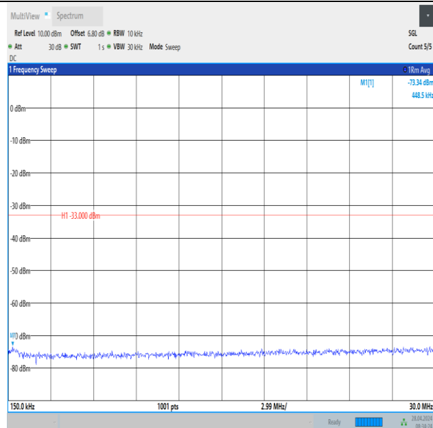
Band2_10MHz_QPSK_19150_1RB#49_0.15~30_0.15~30
