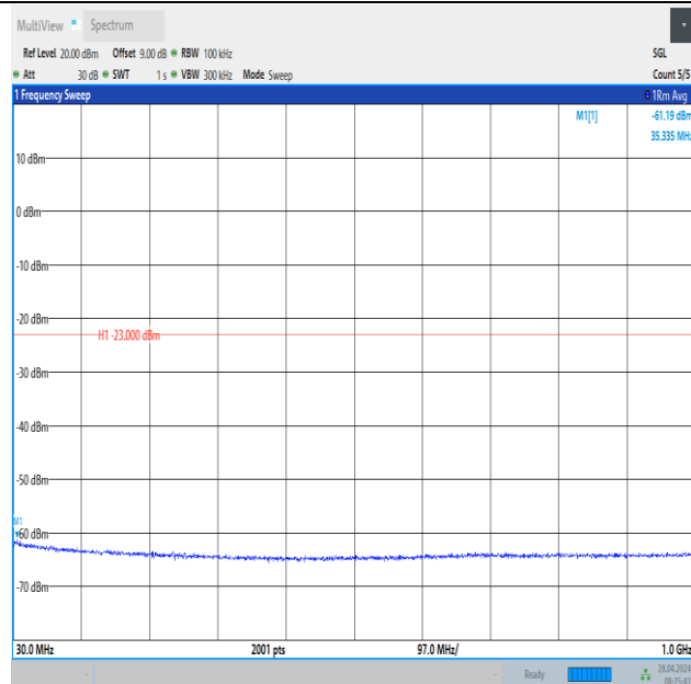
Band2_10MHz_QPSK_19150_50RB#0_30~1000_30~1000
