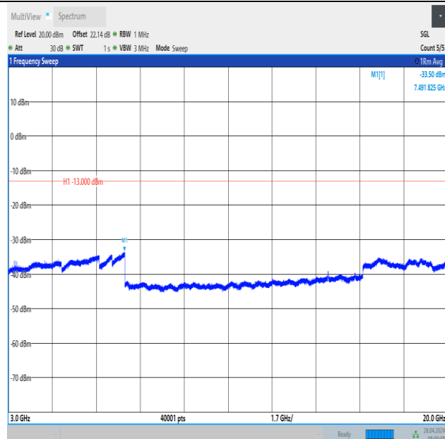
Band2_20MHz_QPSK_19100_1RB#0_3000~20000_3000~20000
